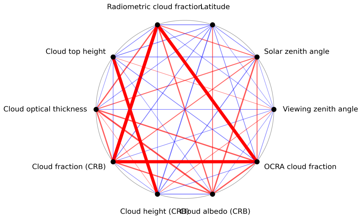
Figure 1: Map of correlation graph for 2024-04-01 to 2024-04-03.
