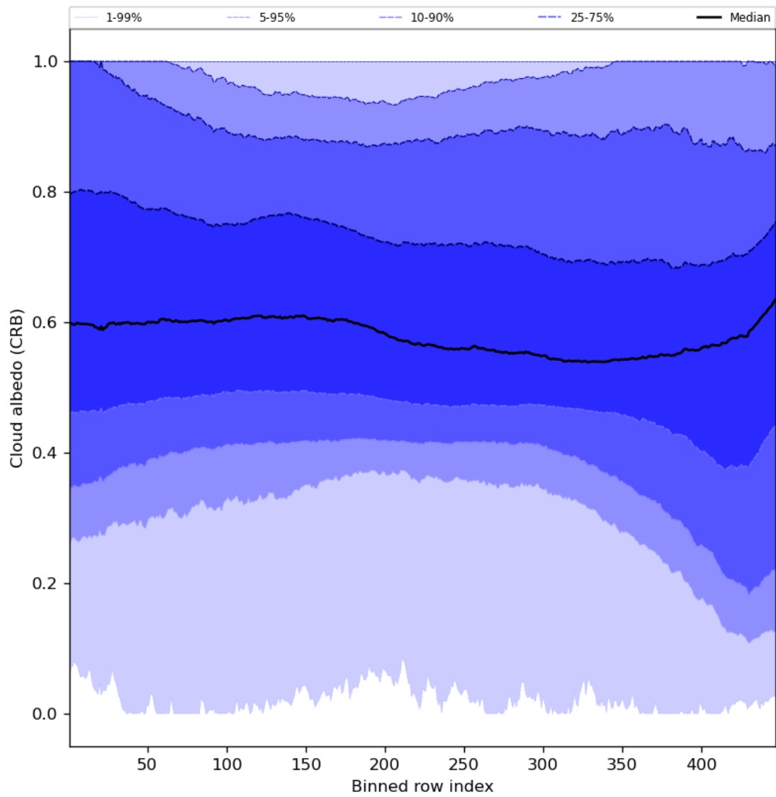
Figure 60: Along track statistics of “Cloud albedo (CRB)” for 2024-04-01 to 2024-04-03
