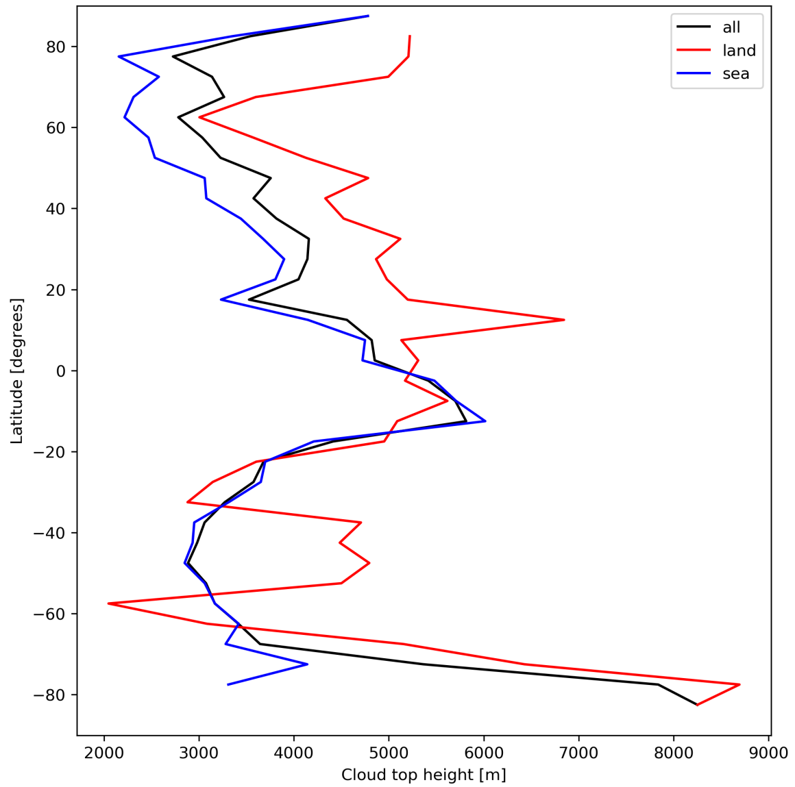
Figure 24: Zonal average of “Cloud top height” for 2024-04-01 to 2024-04-03.
