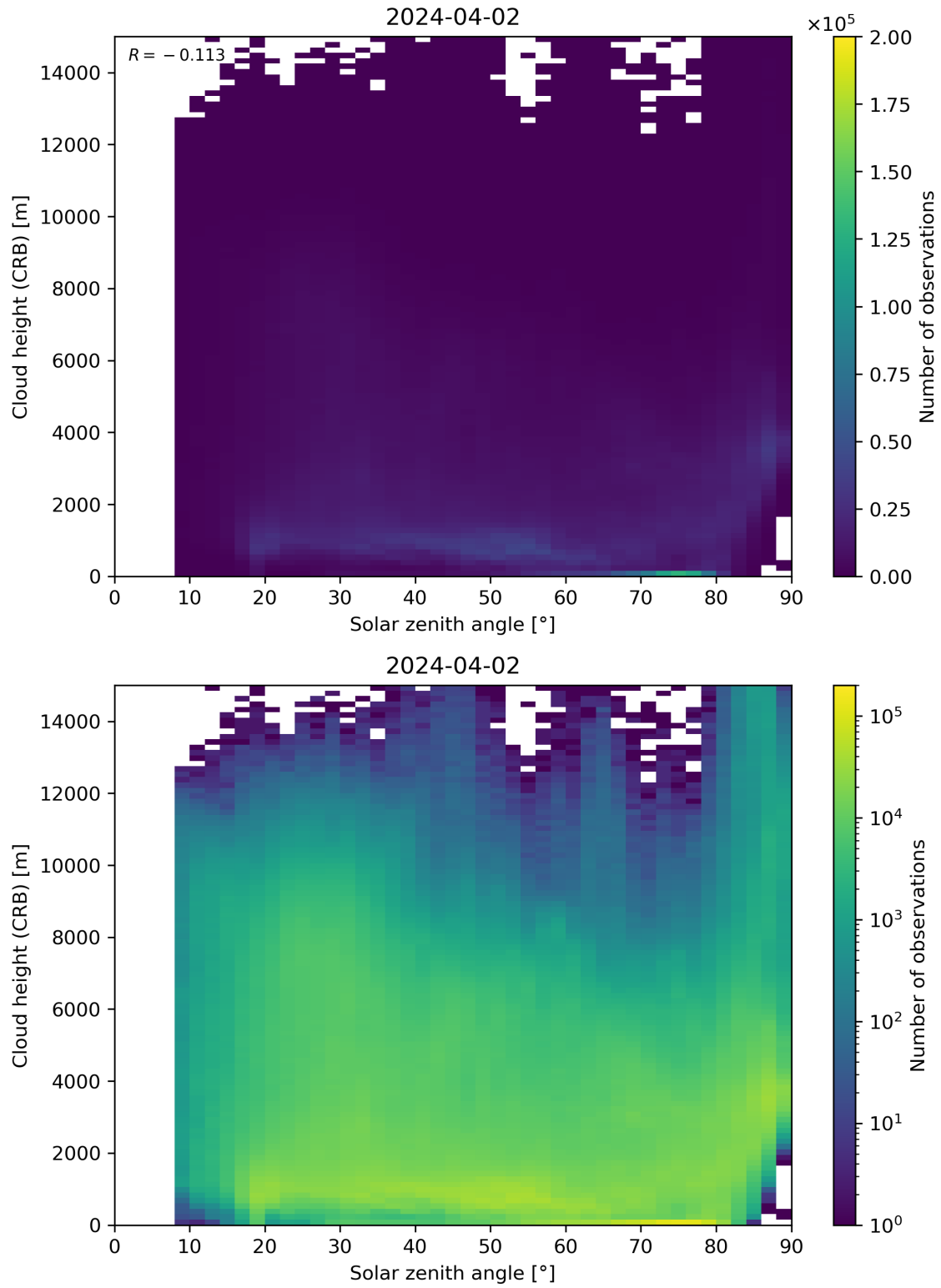
Figure 102: Scatter density plot of “Solar zenith angle” against “Cloud height (CRB)” for 2024-04-01 to 2024-04-03.
