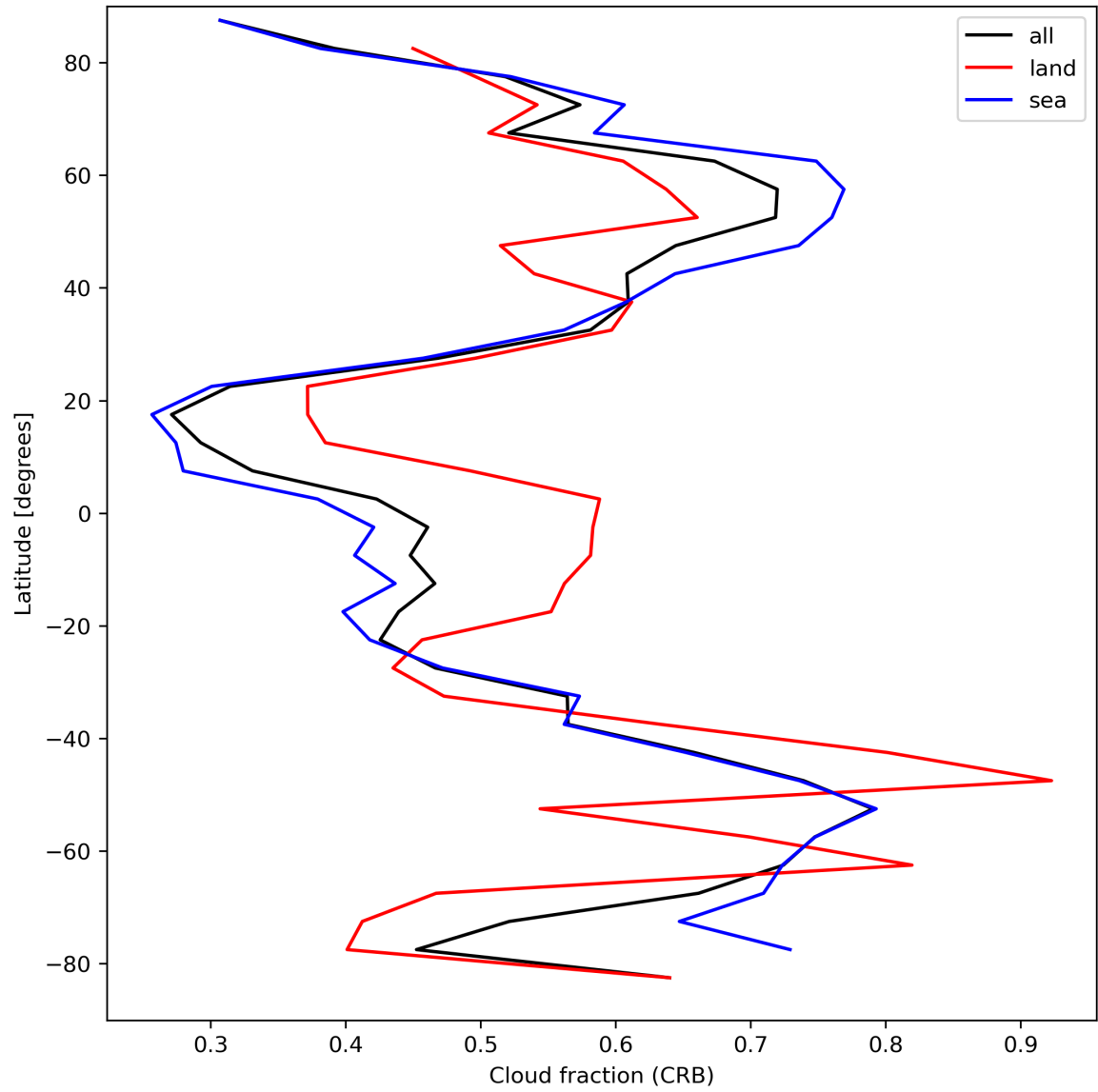
Figure 26: Zonal average of “Cloud fraction (CRB)” for 2024-04-01 to 2024-04-03.
