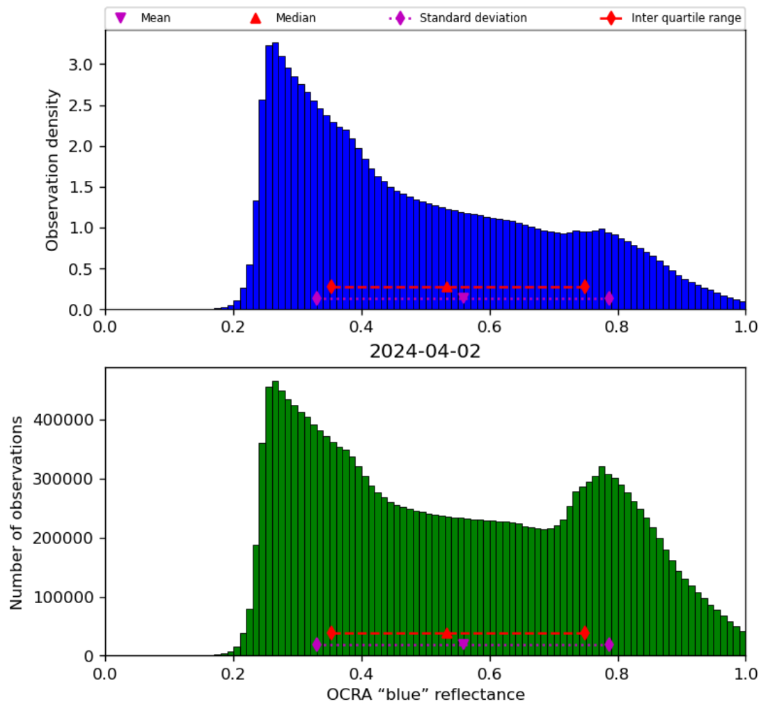
Figure 51: Histogram of “OCRA “blue” reflectance” for 2024-04-01 to 2024-04-03
