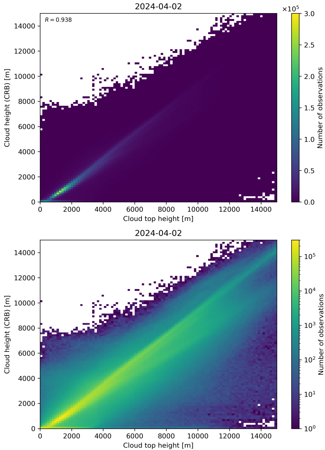
Figure 89: Scatter density plot of “Cloud top height” against “Cloud height (CRB)” for 2024-04-01 to 2024-04-03.
