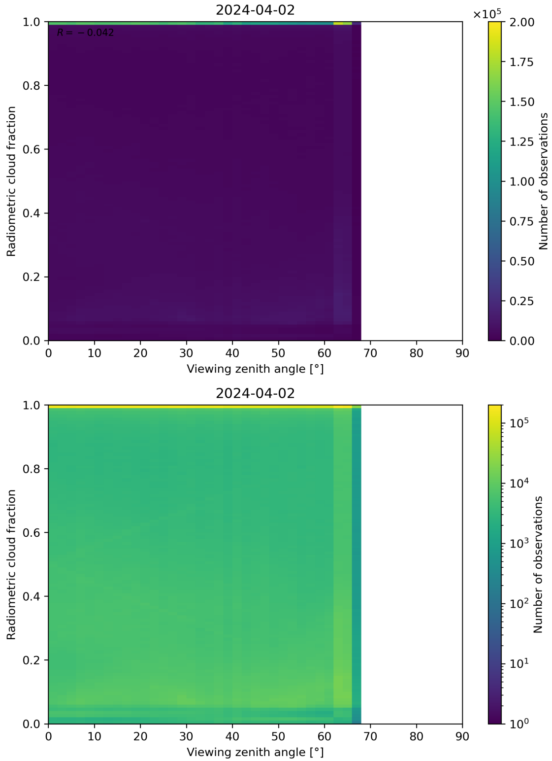
Figure 107: Scatter density plot of “Viewing zenith angle” against “Radiometric cloud fraction” for 2024-04-01 to 2024-04-03.
