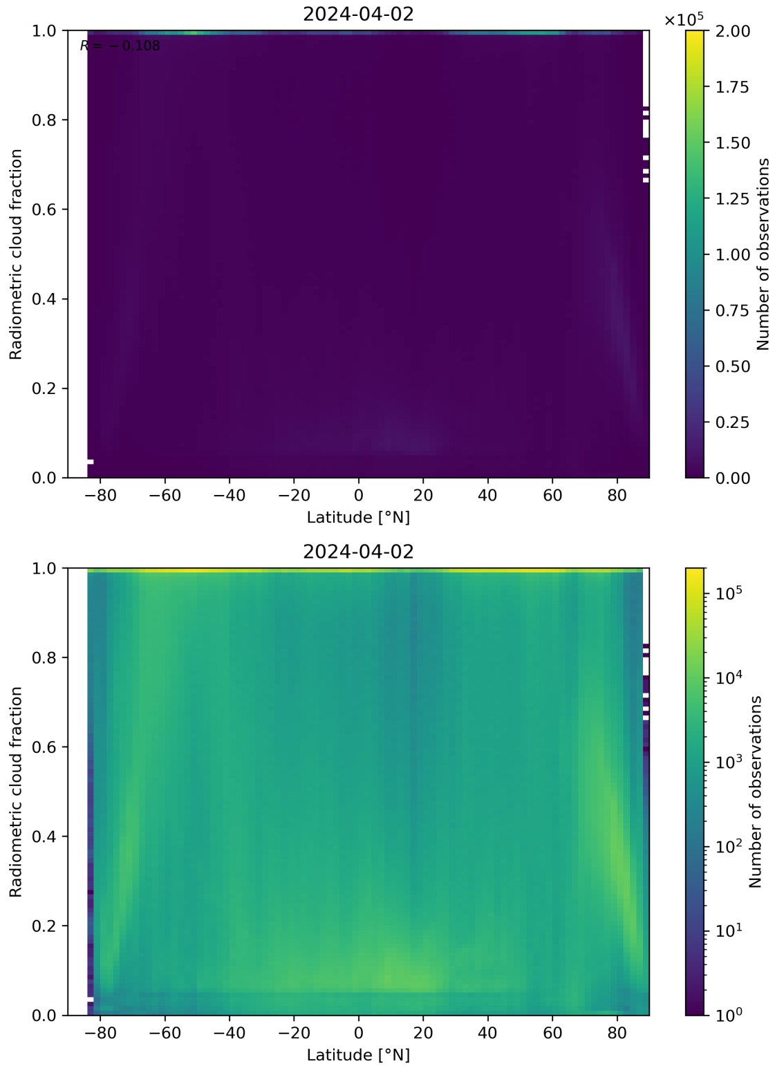
Figure 92: Scatter density plot of “Latitude” against “Radiometric cloud fraction” for 2024-04-01 to 2024-04-03.
