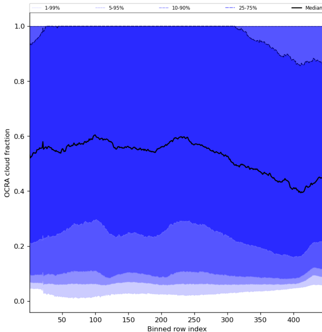
Figure 66: Along track statistics of “OCRA cloud fraction” for 2024-04-01 to 2024-04-03
