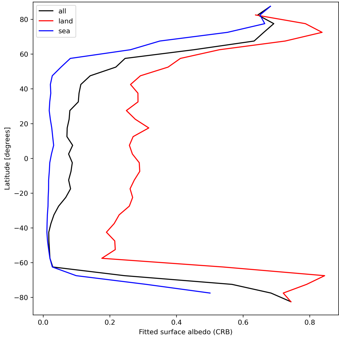
Figure 30: Zonal average of “Fitted surface albedo (CRB)” for 2024-04-01 to 2024-04-03.
