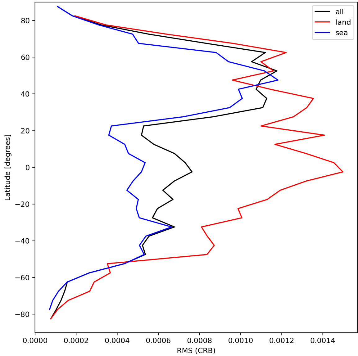
Figure 32: Zonal average of “RMS (CRB)” for 2024-04-01 to 2024-04-03.
