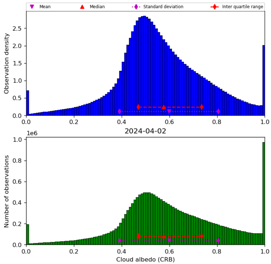
Figure 44: Histogram of “Cloud albedo (CRB)” for 2024-04-01 to 2024-04-03
