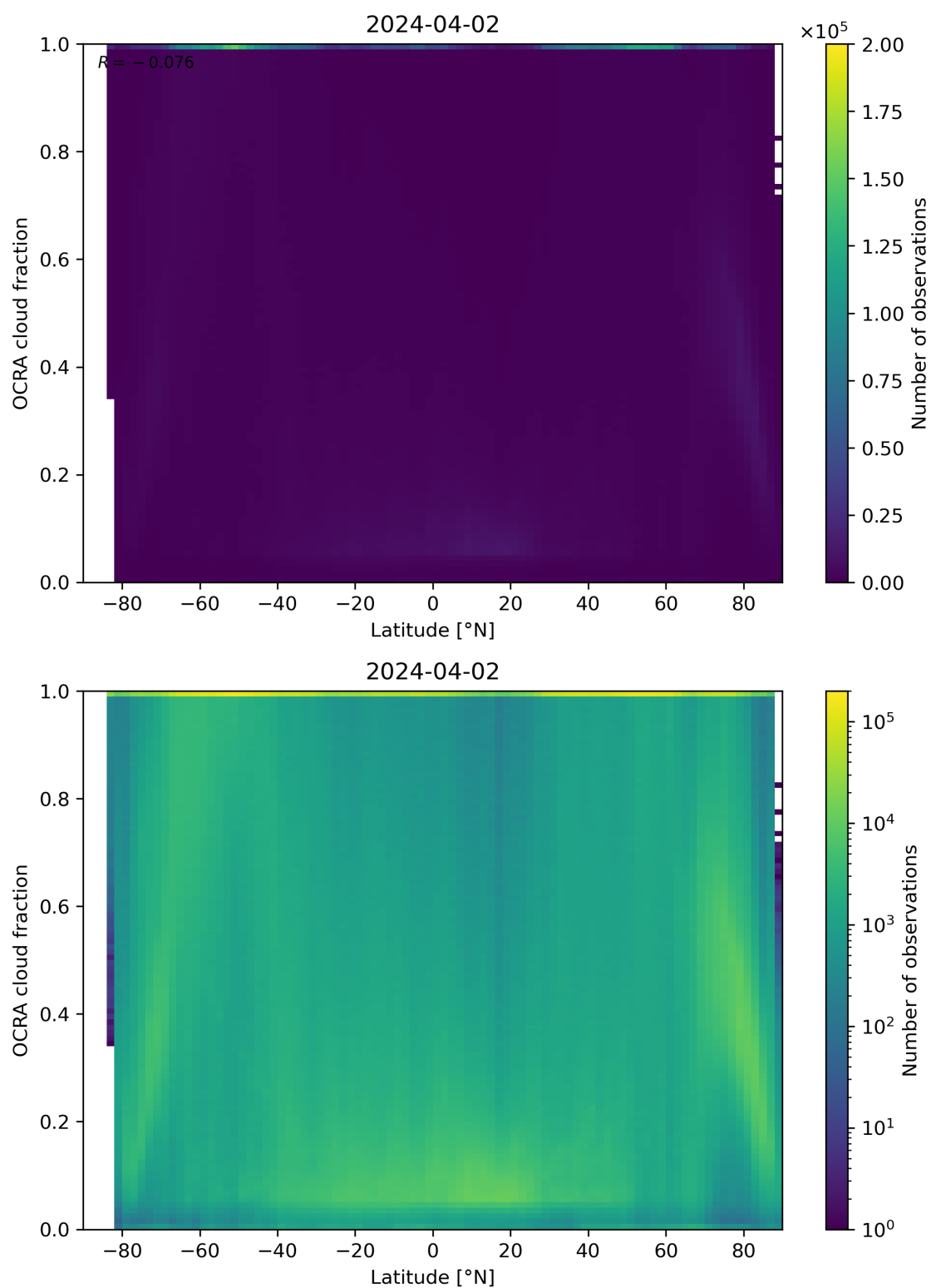
Figure 93: Scatter density plot of “Latitude” against “OCRA cloud fraction” for 2024-04-01 to 2024-04-03.
