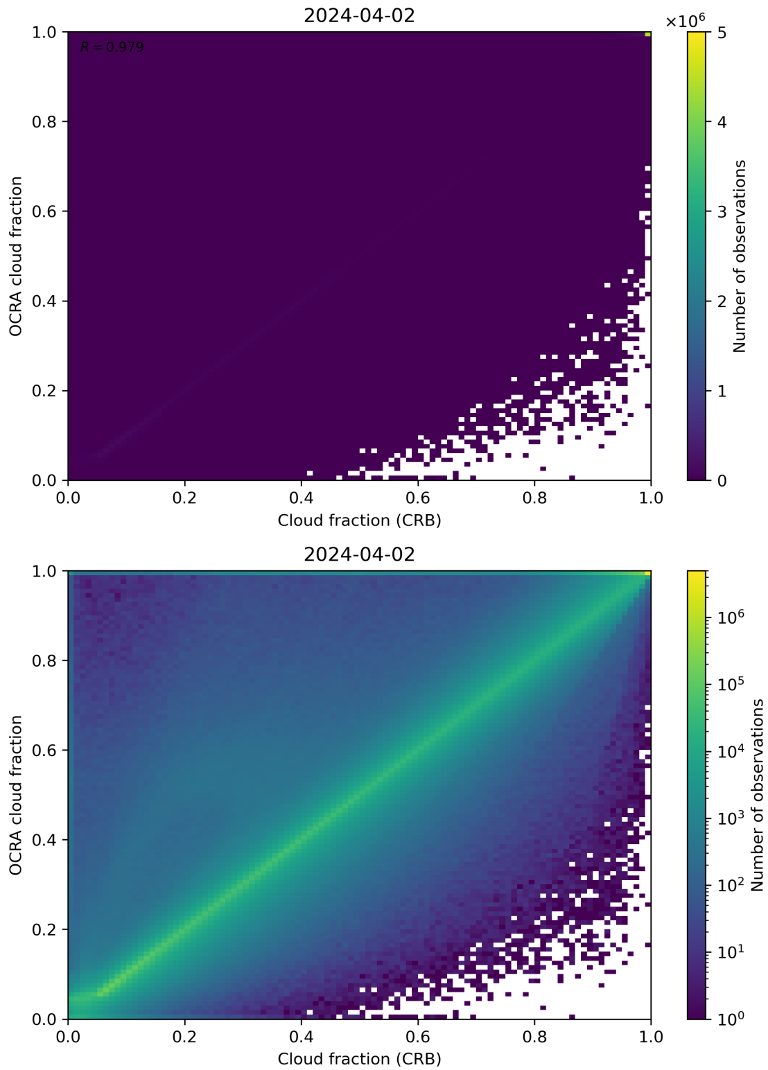
Figure 78: Scatter density plot of “Cloud fraction (CRB)” against “OCRA cloud fraction” for 2024-04-01 to 2024-04-03.
