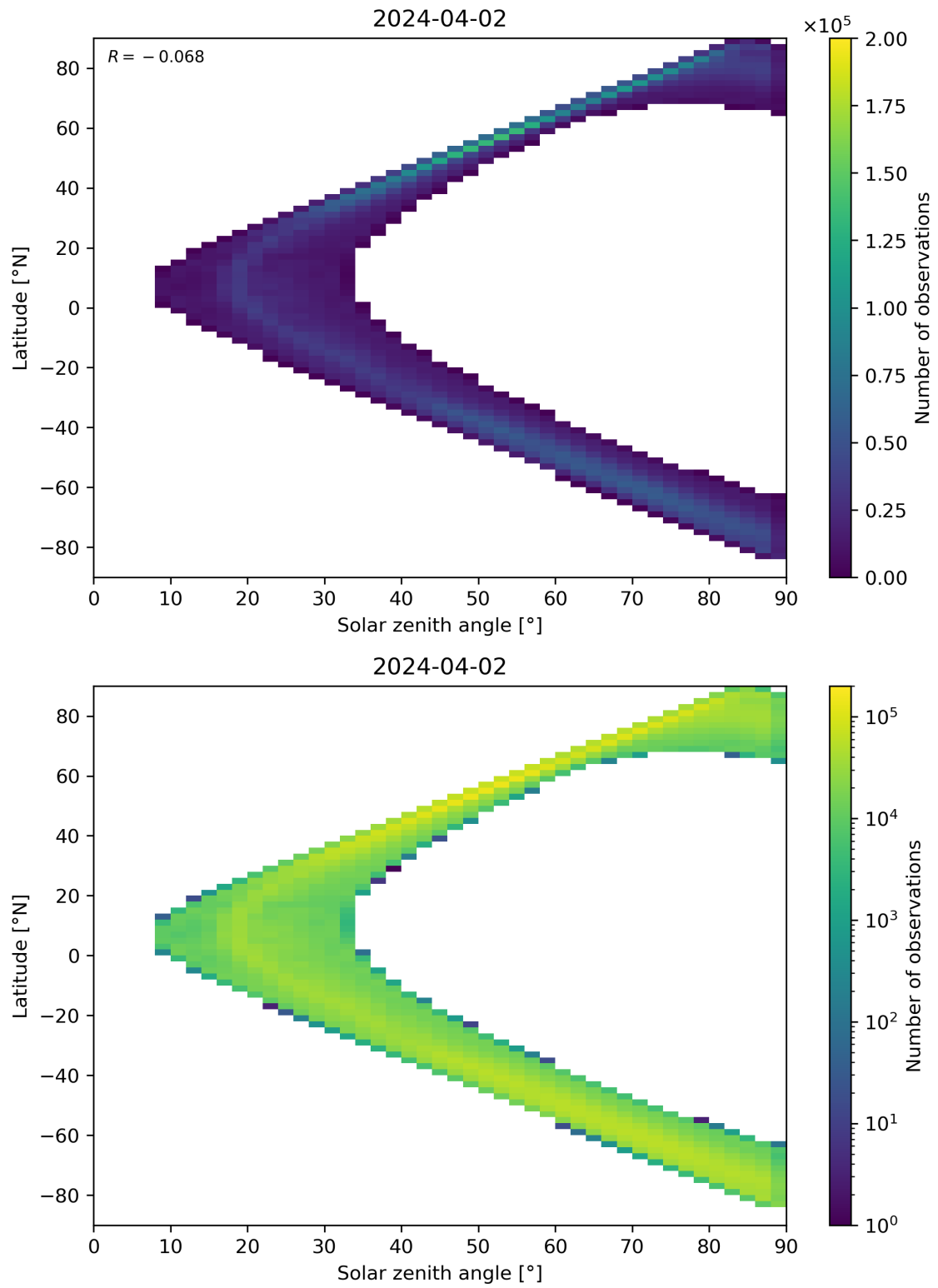
Figure 105: Scatter density plot of “Solar zenith angle” against “Latitude” for 2024-04-01 to 2024-04-03.
