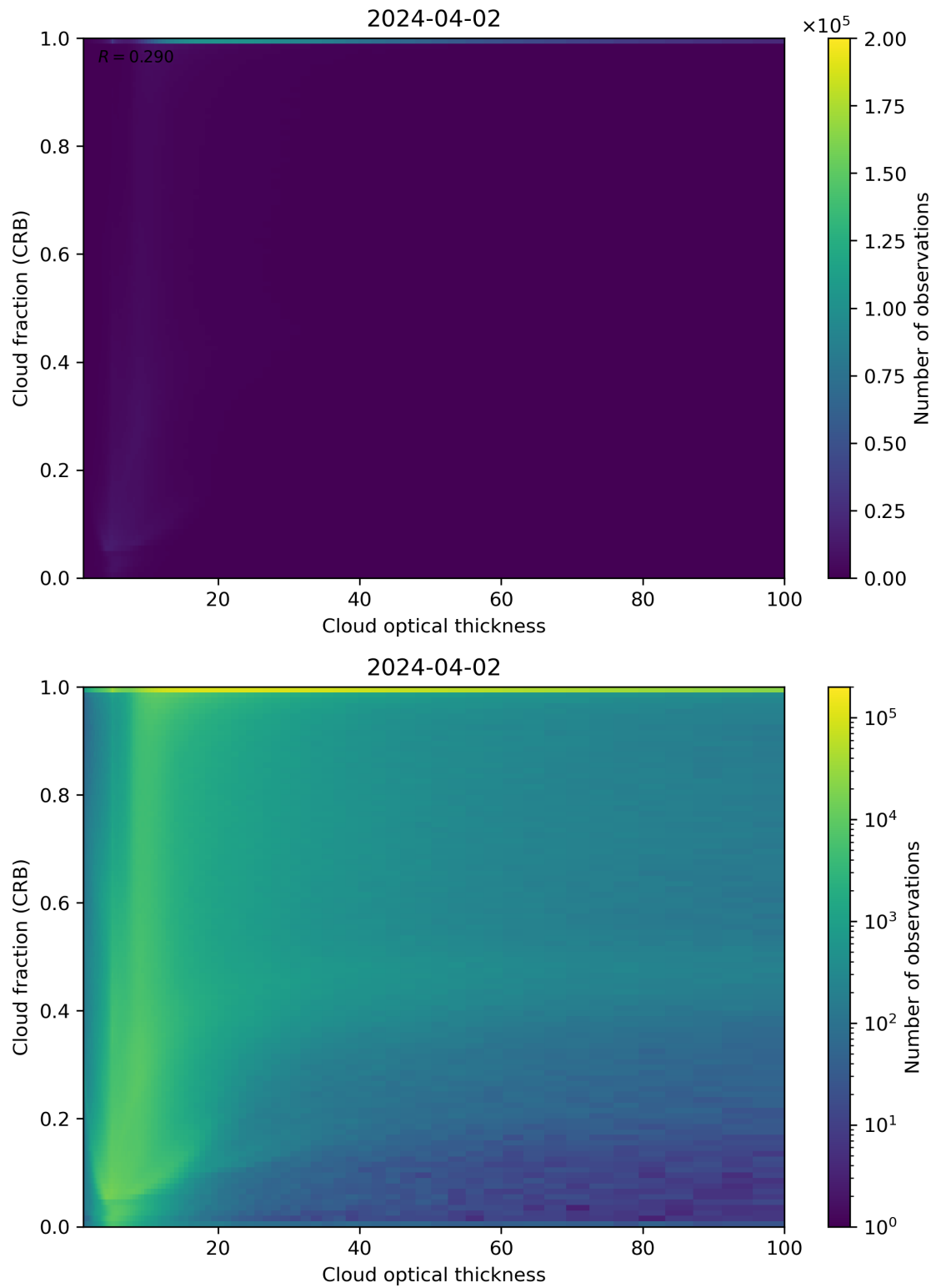
Figure 84: Scatter density plot of “Cloud optical thickness” against “Cloud fraction (CRB)” for 2024-04-01 to 2024-04-03.
