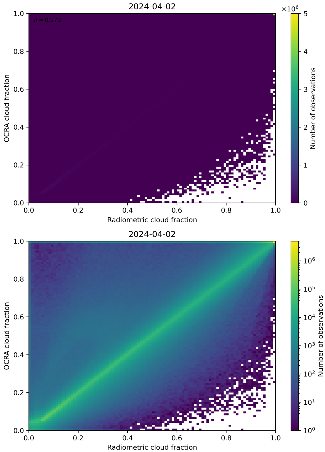
Figure 72: Scatter density plot of “Radiometric cloud fraction” against “OCRA cloud fraction” for 2024-04-01 to 2024-04-03.
