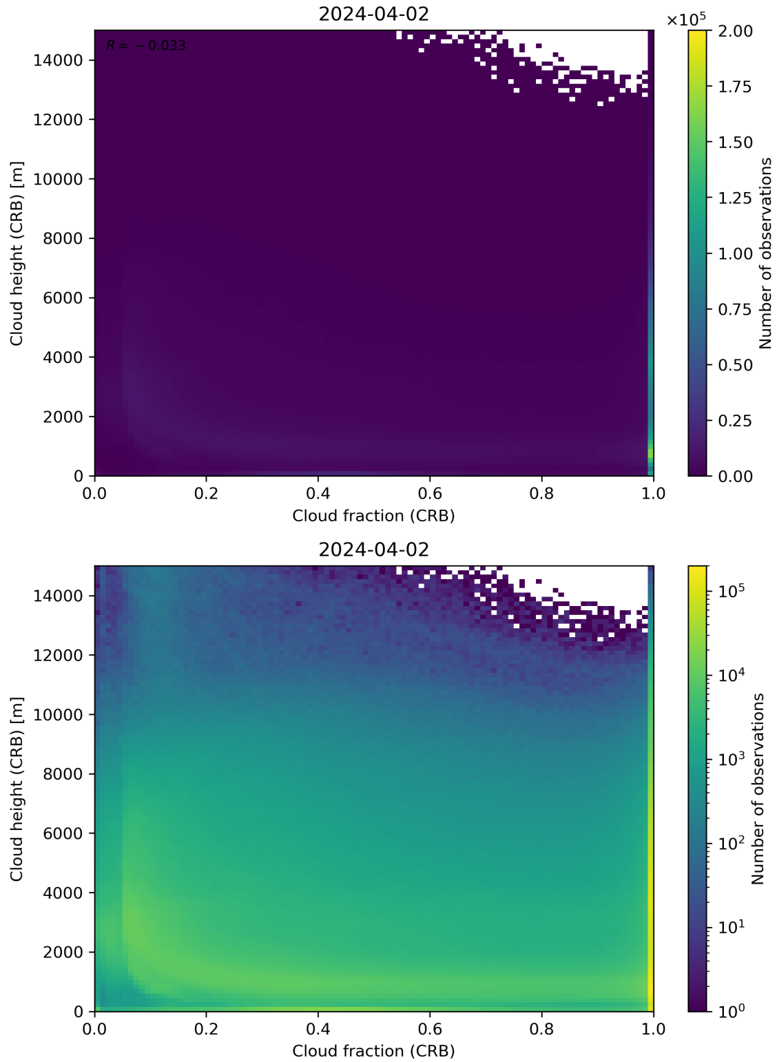
Figure 79: Scatter density plot of “Cloud fraction (CRB)” against “Cloud height (CRB)” for 2024-04-01 to 2024-04-03.
