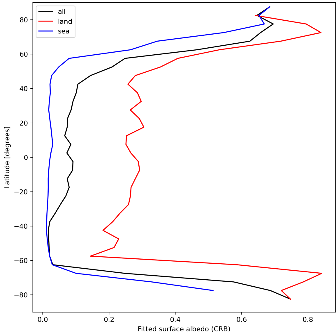
Figure 30: Zonal average of “Fitted surface albedo (CRB)” for 2024-04-02 to 2024-04-04.
