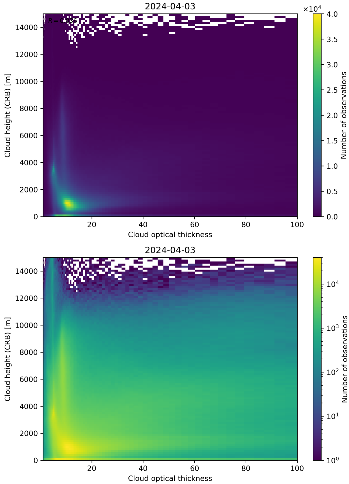
Figure 85: Scatter density plot of “Cloud optical thickness” against “Cloud height (CRB)” for 2024-04-02 to 2024-04-04.
