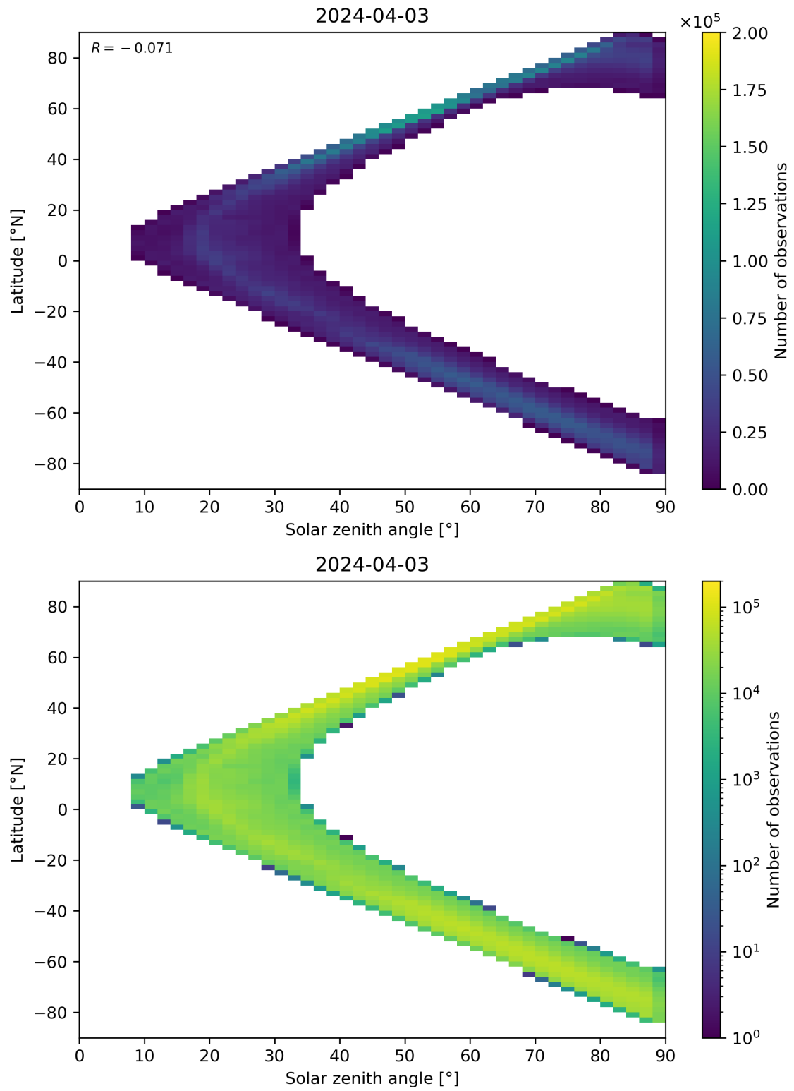
Figure 105: Scatter density plot of “Solar zenith angle” against “Latitude” for 2024-04-02 to 2024-04-04.
