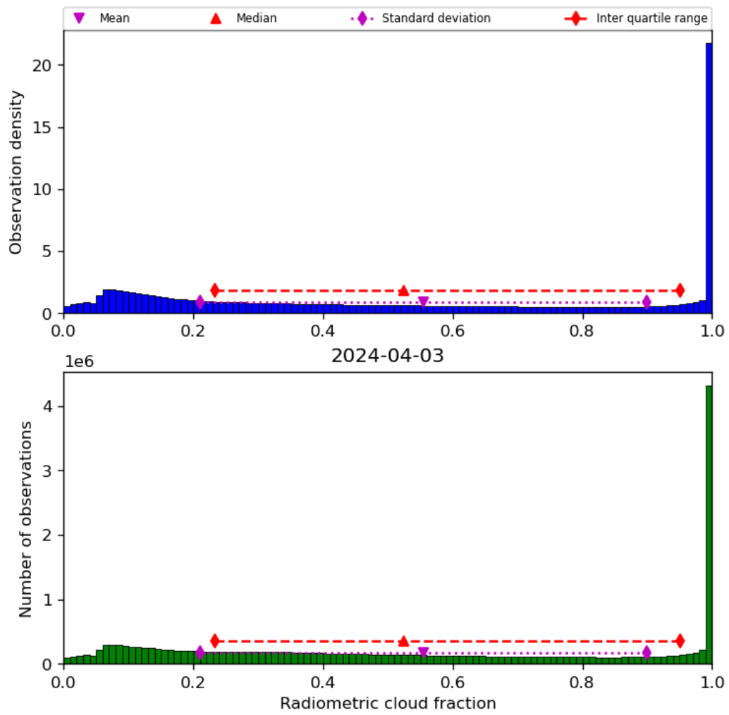
Figure 39: Histogram of “Radiometric cloud fraction” for 2024-04-02 to 2024-04-04
