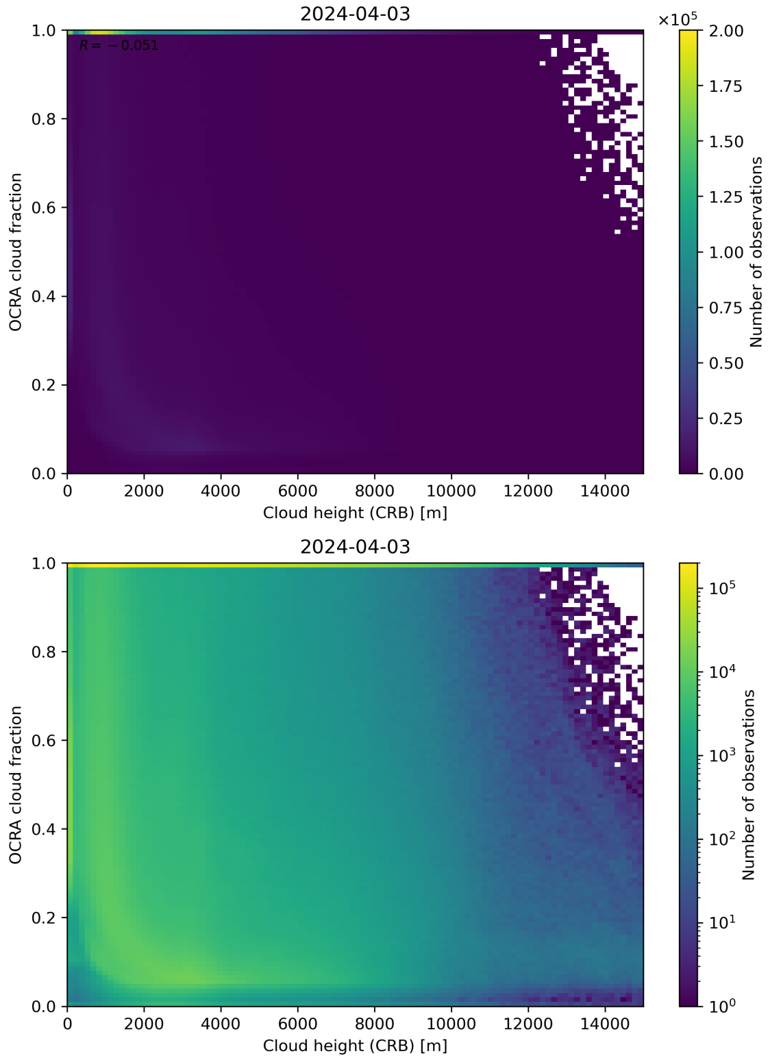
Figure 81: Scatter density plot of “Cloud height (CRB)” against “OCRA cloud fraction” for 2024-04-02 to 2024-04-04.
