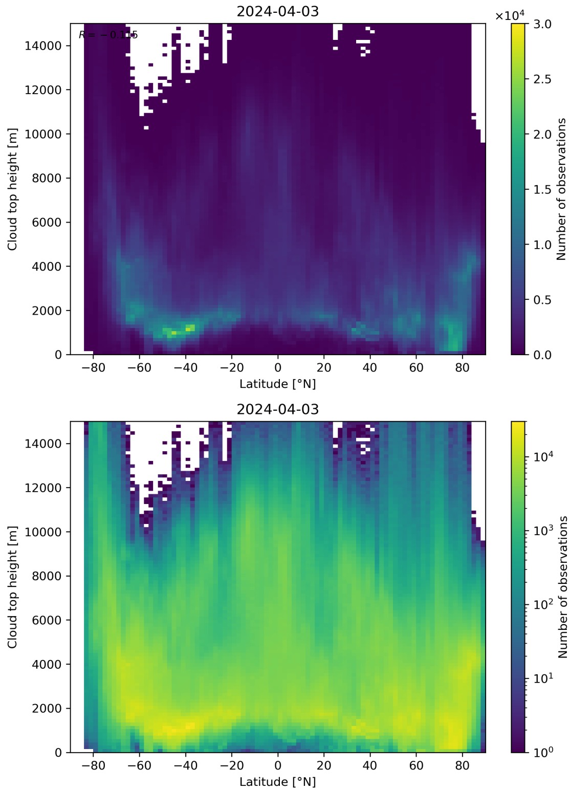
Figure 97: Scatter density plot of “Latitude” against “Cloud top height” for 2024-04-02 to 2024-04-04.
