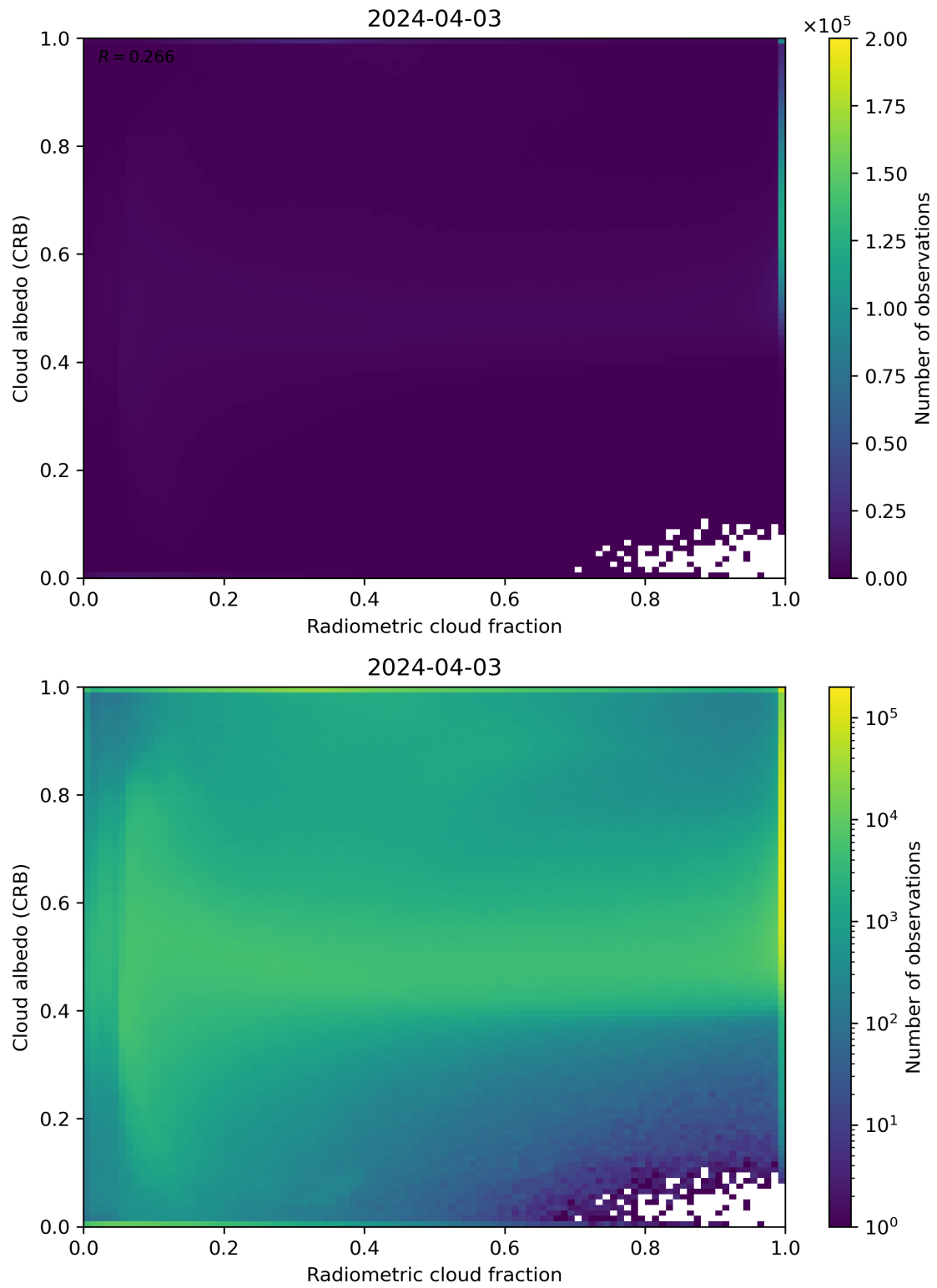
Figure 71: Scatter density plot of “Radiometric cloud fraction” against “Cloud albedo (CRB)” for 2024-04-02 to 2024-04-04.
