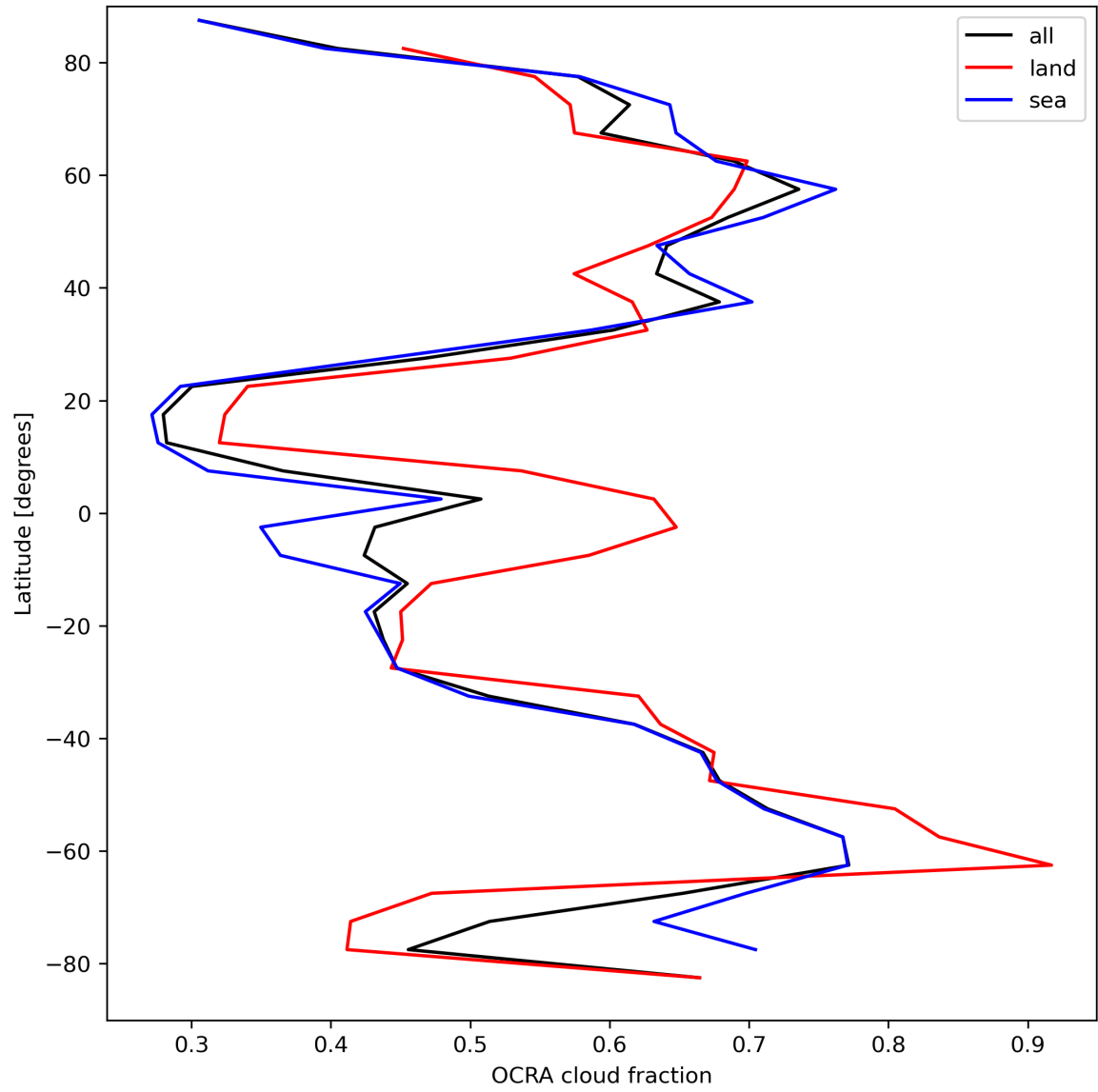
Figure 34: Zonal average of “OCRA cloud fraction” for 2024-04-02 to 2024-04-04.
