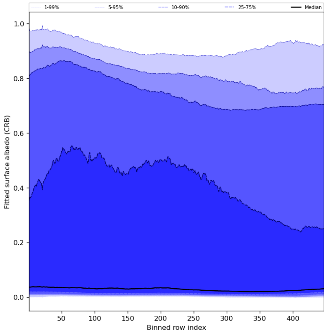
Figure 62: Along track statistics of “Fitted surface albedo (CRB)” for 2024-04-02 to 2024-04-04
