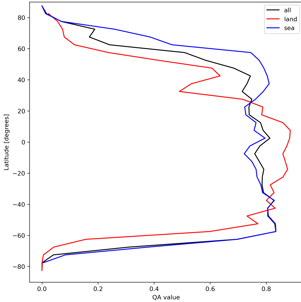
Figure 22: Zonal average of “QA value” for 2024-04-02 to 2024-04-04.
