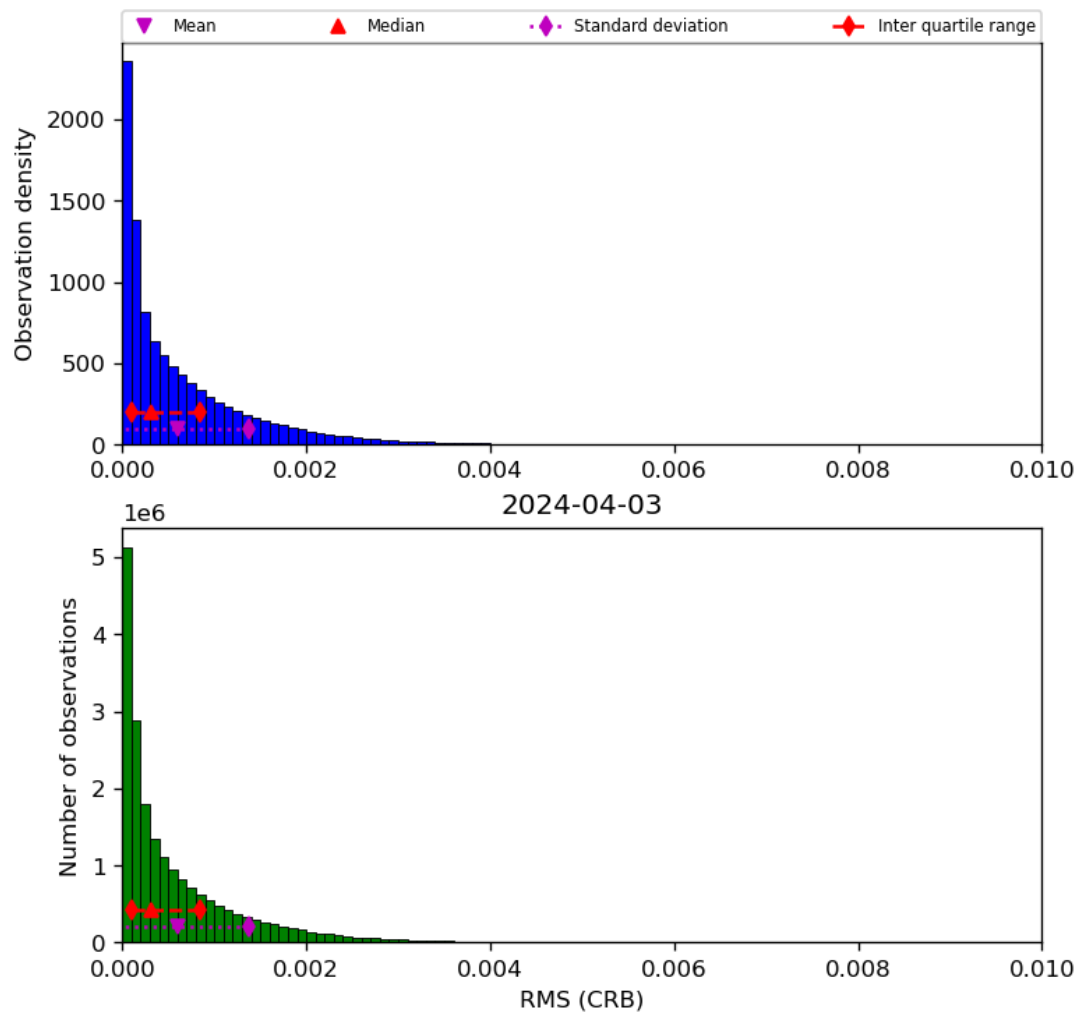
Figure 48: Histogram of “RMS (CRB)” for 2024-04-02 to 2024-04-04
