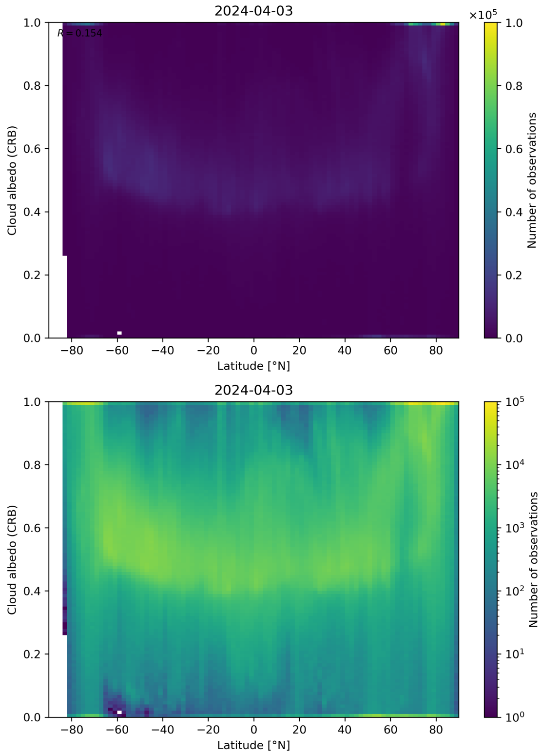
Figure 91: Scatter density plot of “Latitude” against “Cloud albedo (CRB)” for 2024-04-02 to 2024-04-04.
