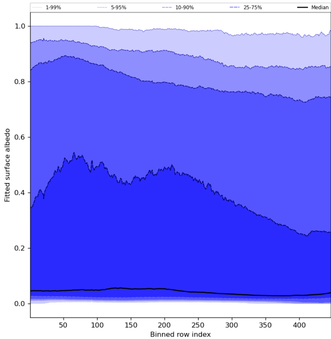
Figure 61: Along track statistics of “Fitted surface albedo” for 2024-04-02 to 2024-04-04
