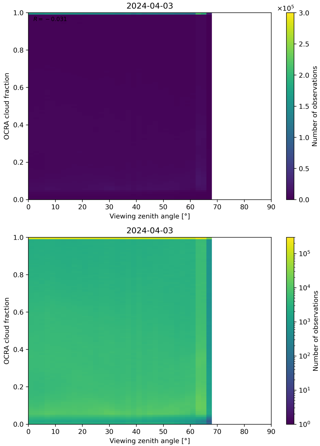
Figure 108: Scatter density plot of “Viewing zenith angle” against “OCRA cloud fraction” for 2024-04-02 to 2024-04-04.
