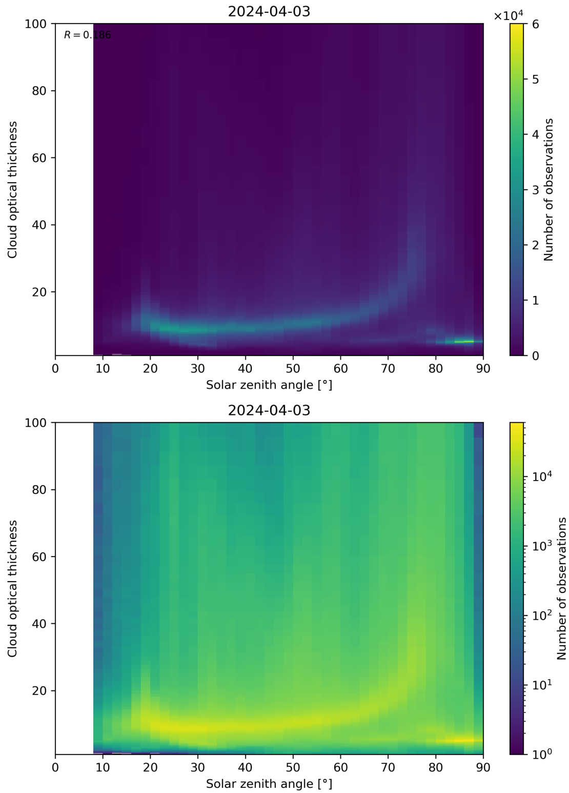
Figure 103: Scatter density plot of “Solar zenith angle” against “Cloud optical thickness” for 2024-04-02 to 2024-04-04.
