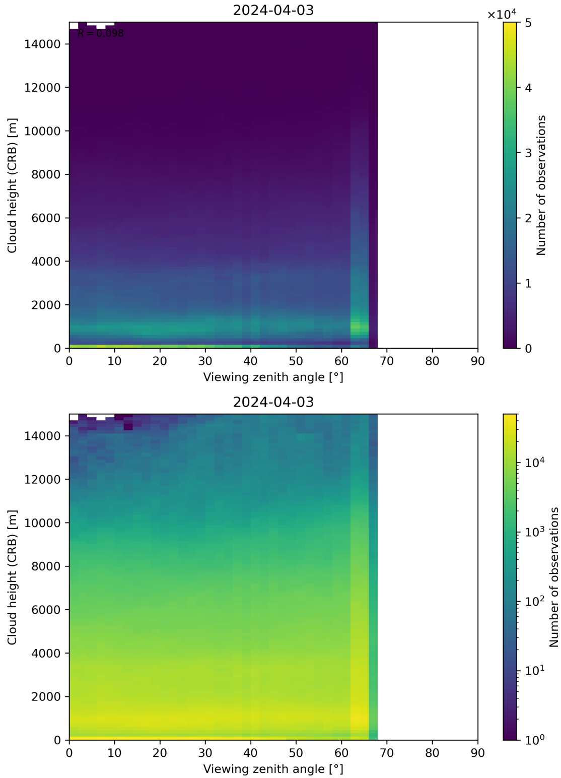
Figure 110: Scatter density plot of “Viewing zenith angle” against “Cloud height (CRB)” for 2024-04-02 to 2024-04-04.
