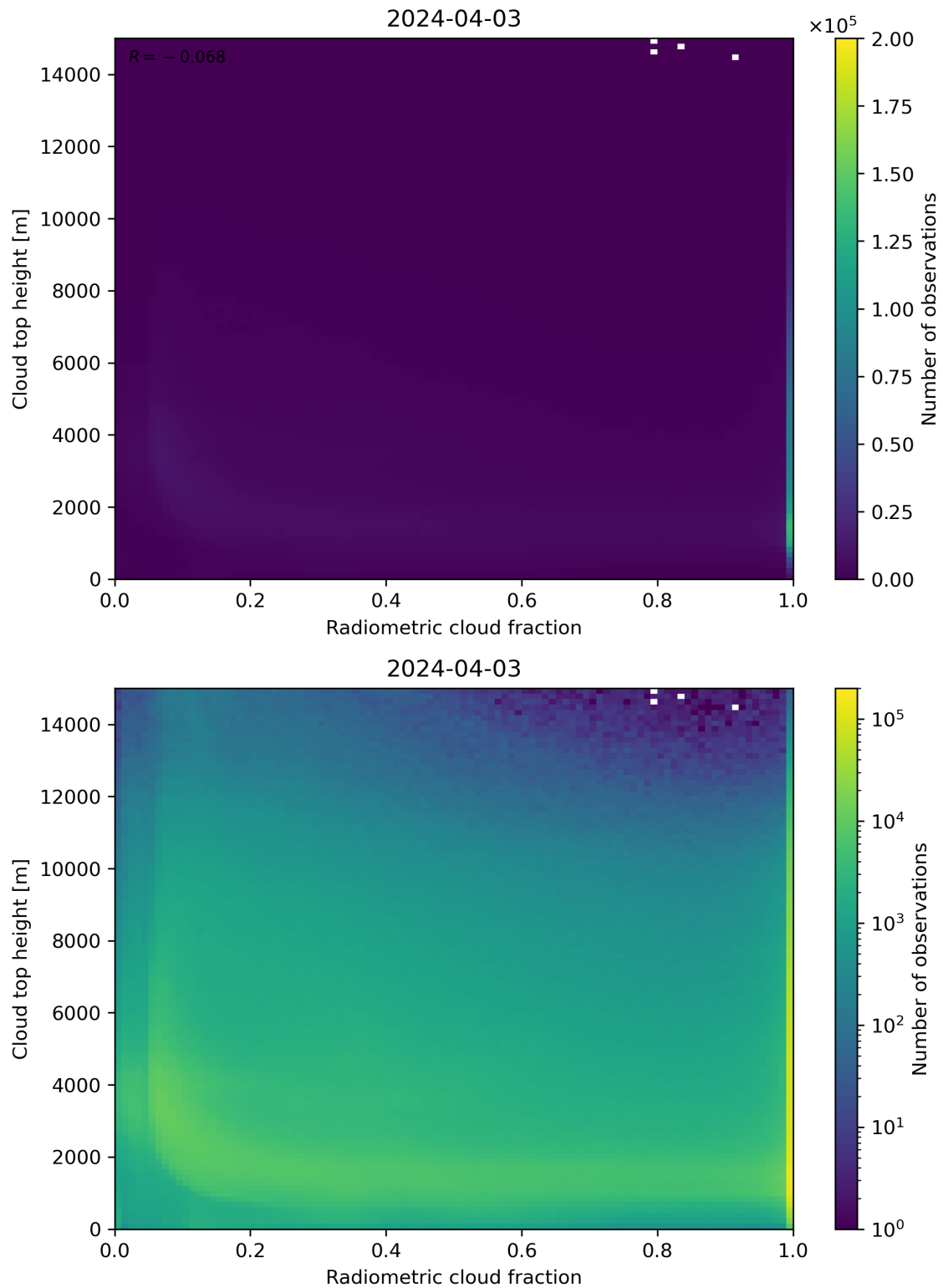
Figure 76: Scatter density plot of “Radiometric cloud fraction” against “Cloud top height” for 2024-04-02 to 2024-04-04.
