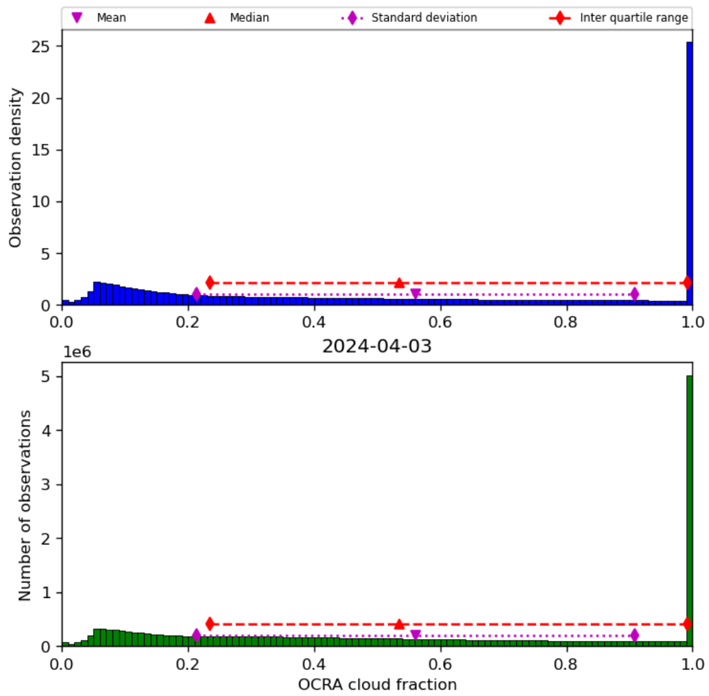
Figure 50: Histogram of “OCRA cloud fraction” for 2024-04-02 to 2024-04-04
