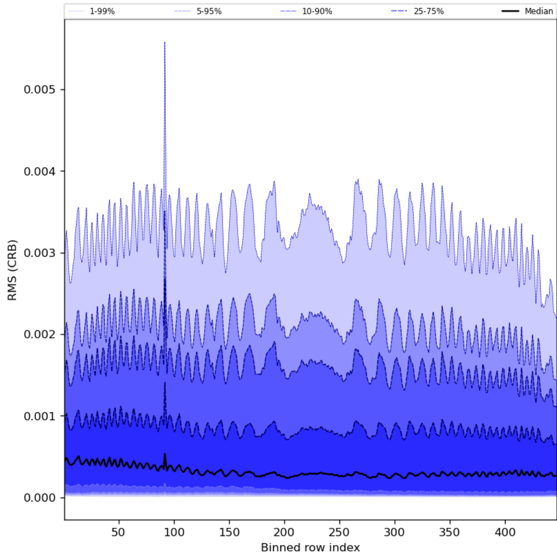
Figure 64: Along track statistics of “RMS (CRB)” for 2024-04-02 to 2024-04-04
