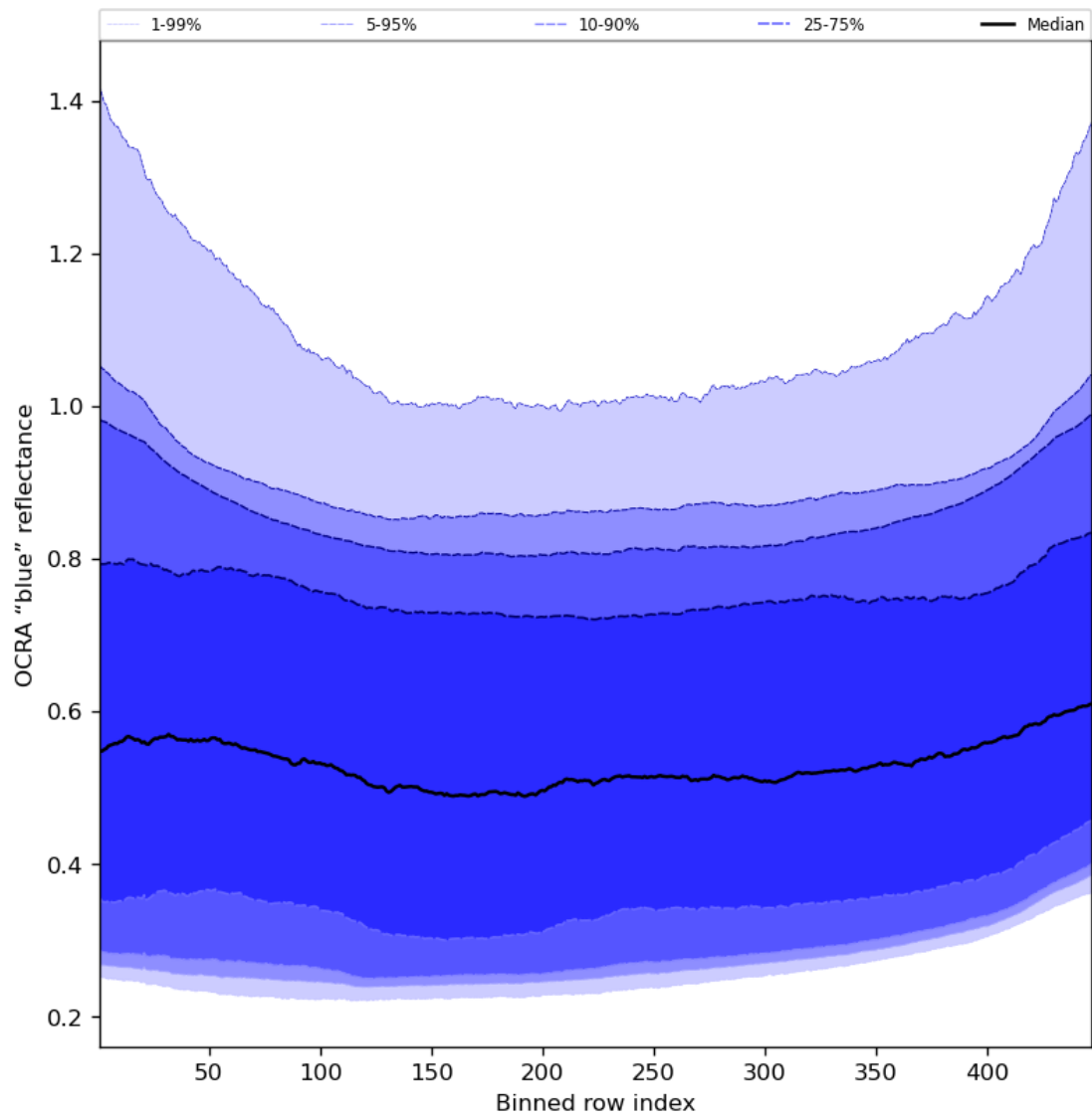
Figure 67: Along track statistics of "OCRA "blue" reflectance" for 2024-04-02 to 2024-04-04
