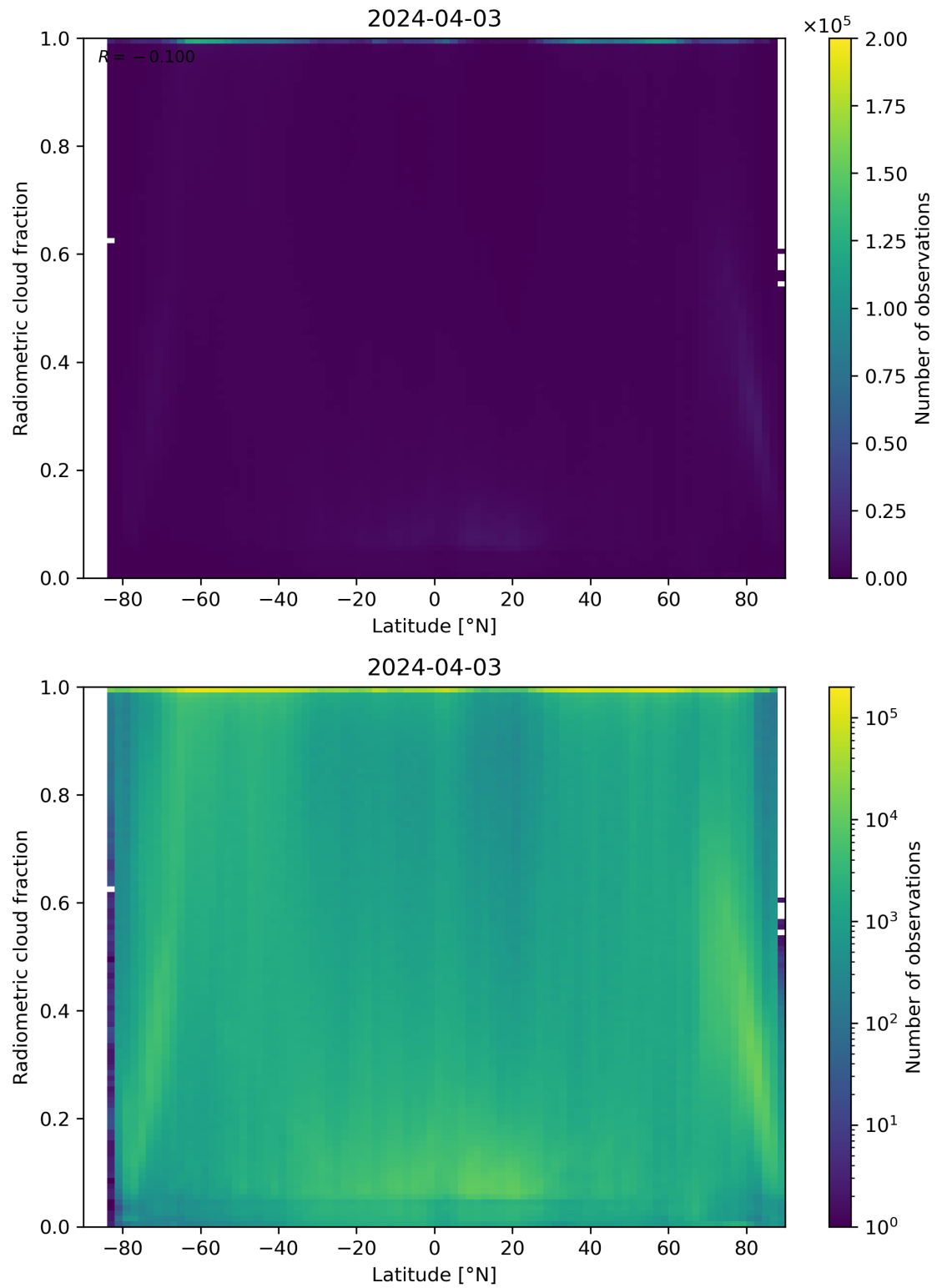
Figure 92: Scatter density plot of “Latitude” against “Radiometric cloud fraction” for 2024-04-02 to 2024-04-04.
