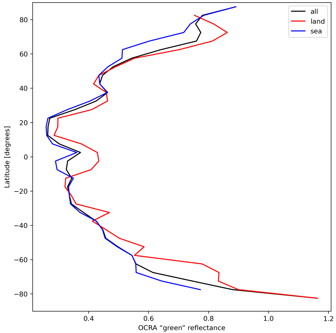
Figure 36: Zonal average of “OCRA “green” reflectance” for 2024-04-02 to 2024-04-04.
