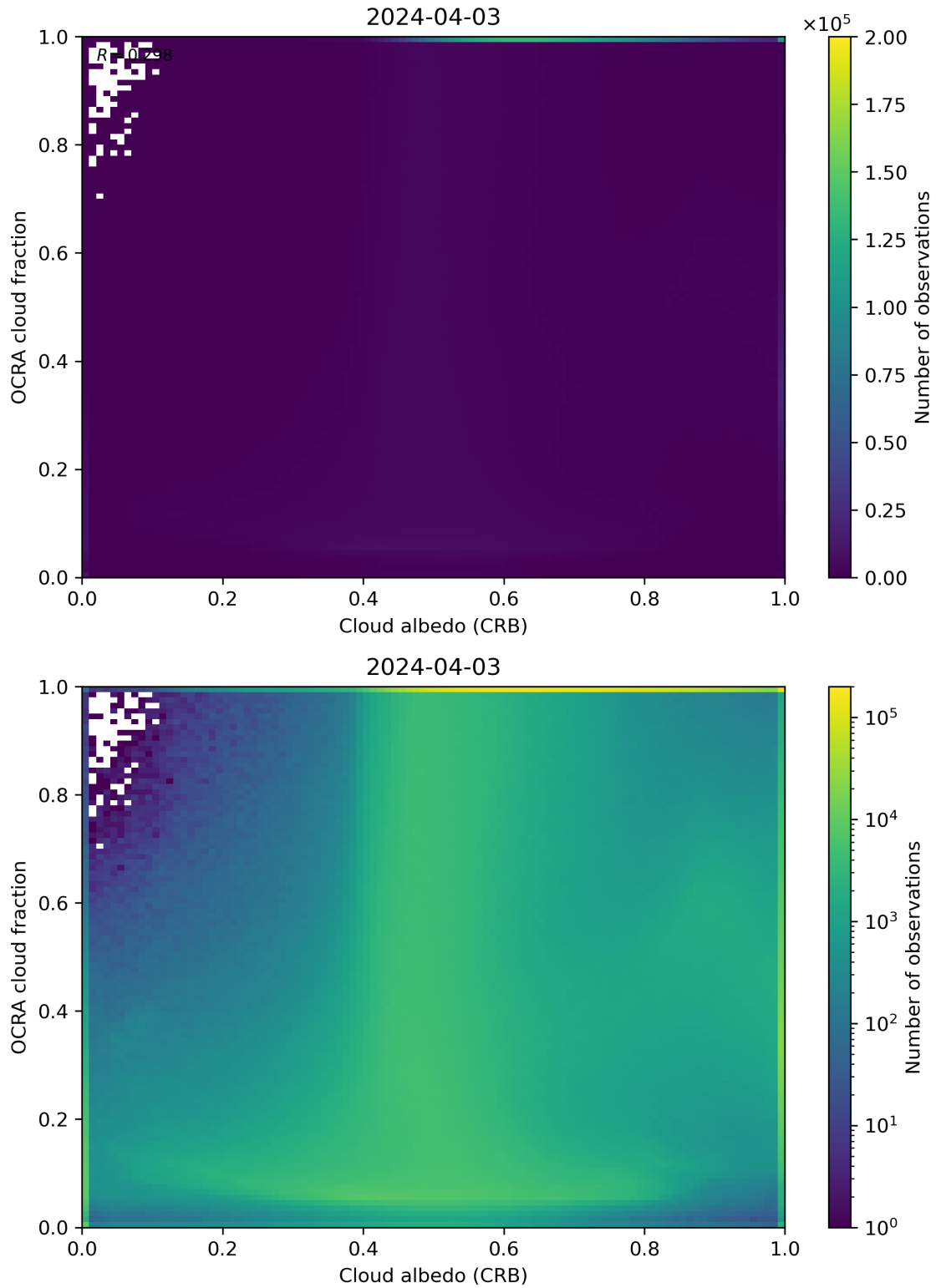
Figure 70: Scatter density plot of “Cloud albedo (CRB)” against “OCRA cloud fraction” for 2024-04-02 to 2024-04-04.
