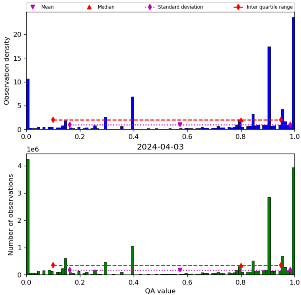
Figure 38: Histogram of “QA value” for 2024-04-02 to 2024-04-04
