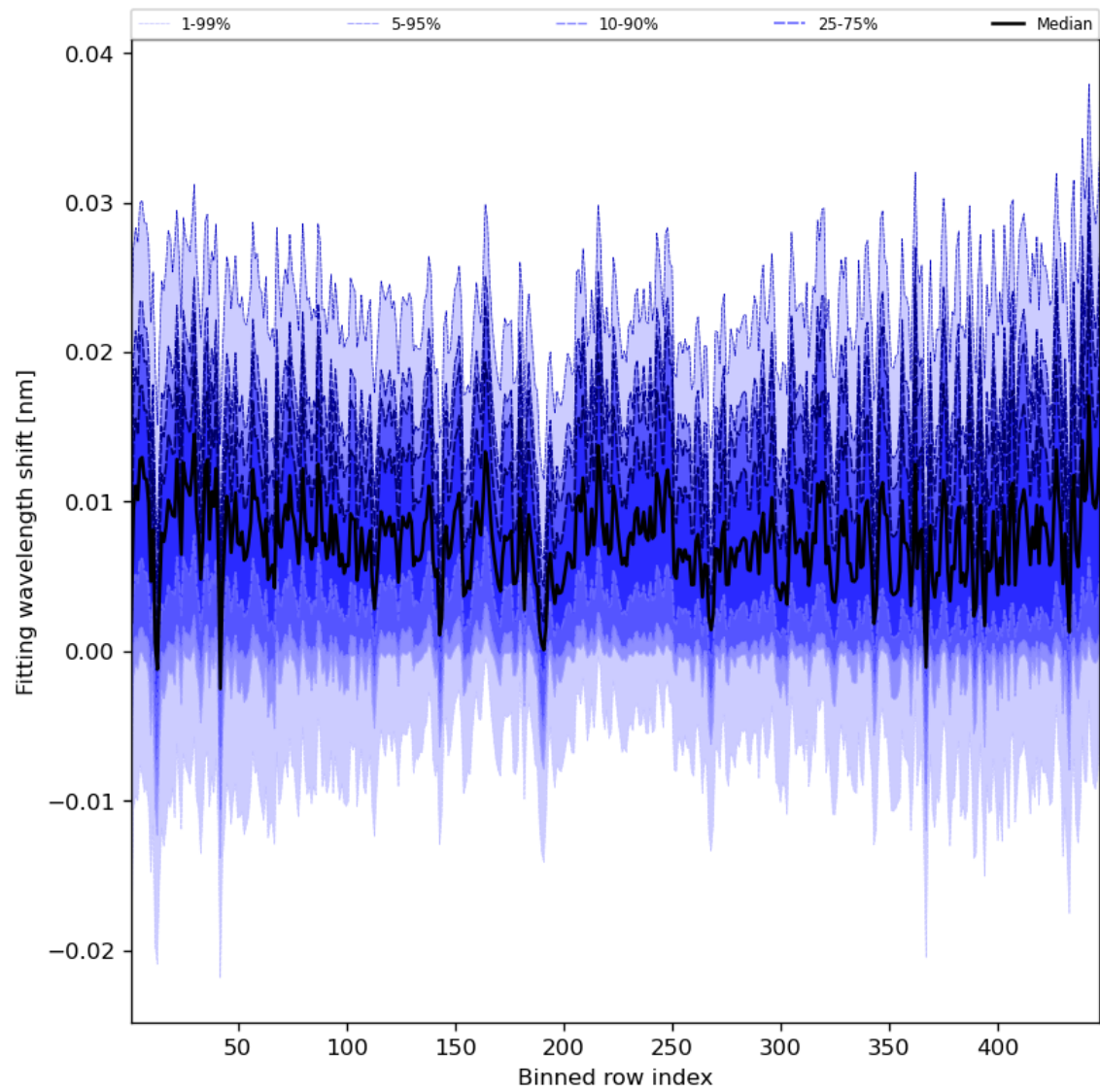
Figure 65: Along track statistics of “Fitting wavelength shift” for 2024-04-02 to 2024-04-04
