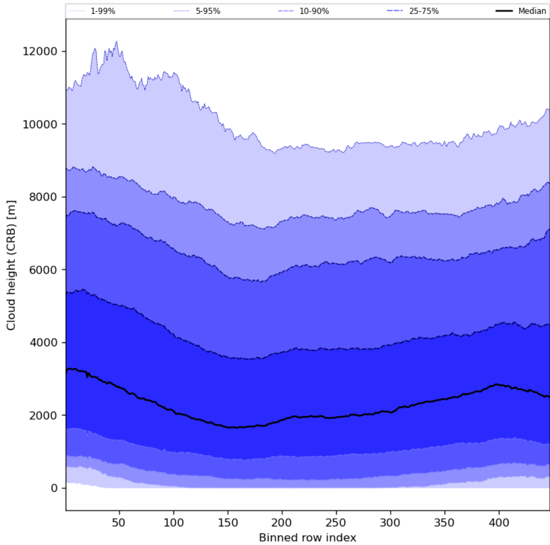
Figure 59: Along track statistics of “Cloud height (CRB)” for 2024-04-05 to 2024-04-06
