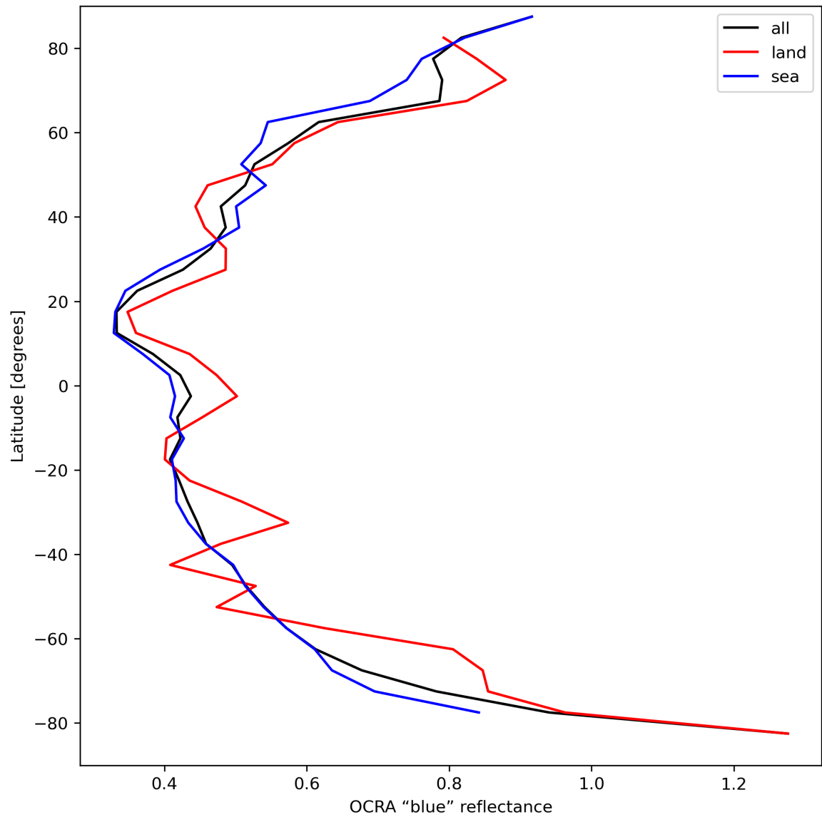
Figure 35: Zonal average of “OCRA “blue” reflectance” for 2024-04-05 to 2024-04-06.
