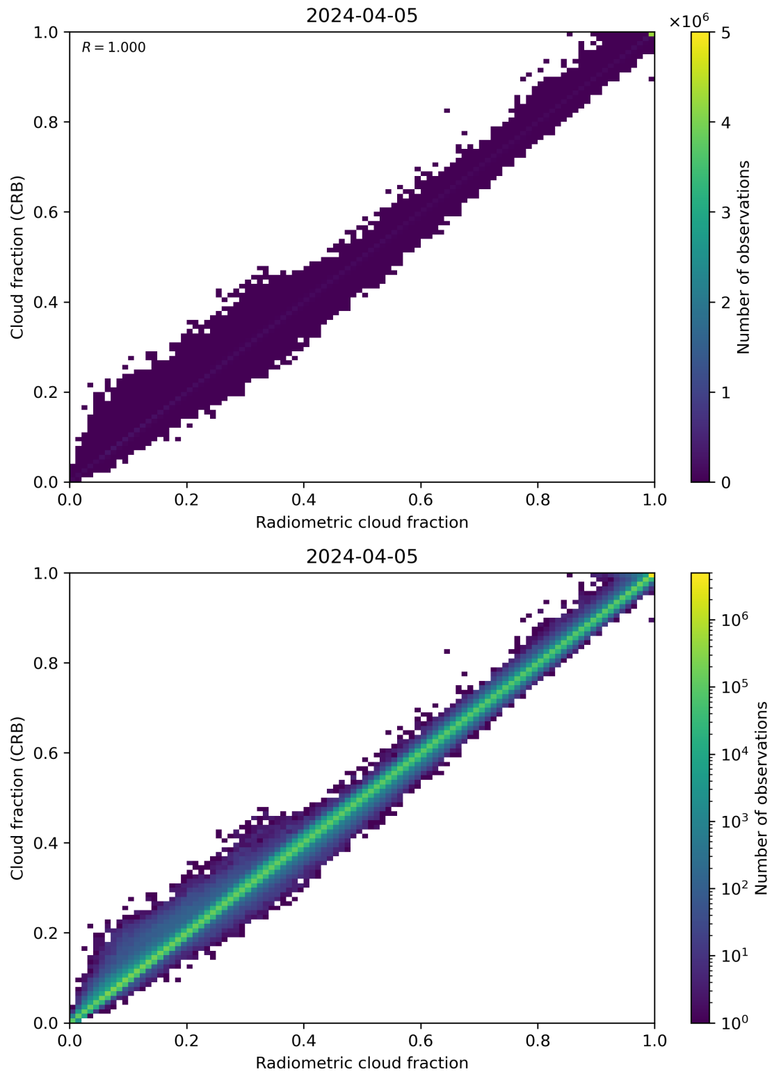
Figure 73: Scatter density plot of “Radiometric cloud fraction” against “Cloud fraction (CRB)” for 2024-04-05 to 2024-04-06.
