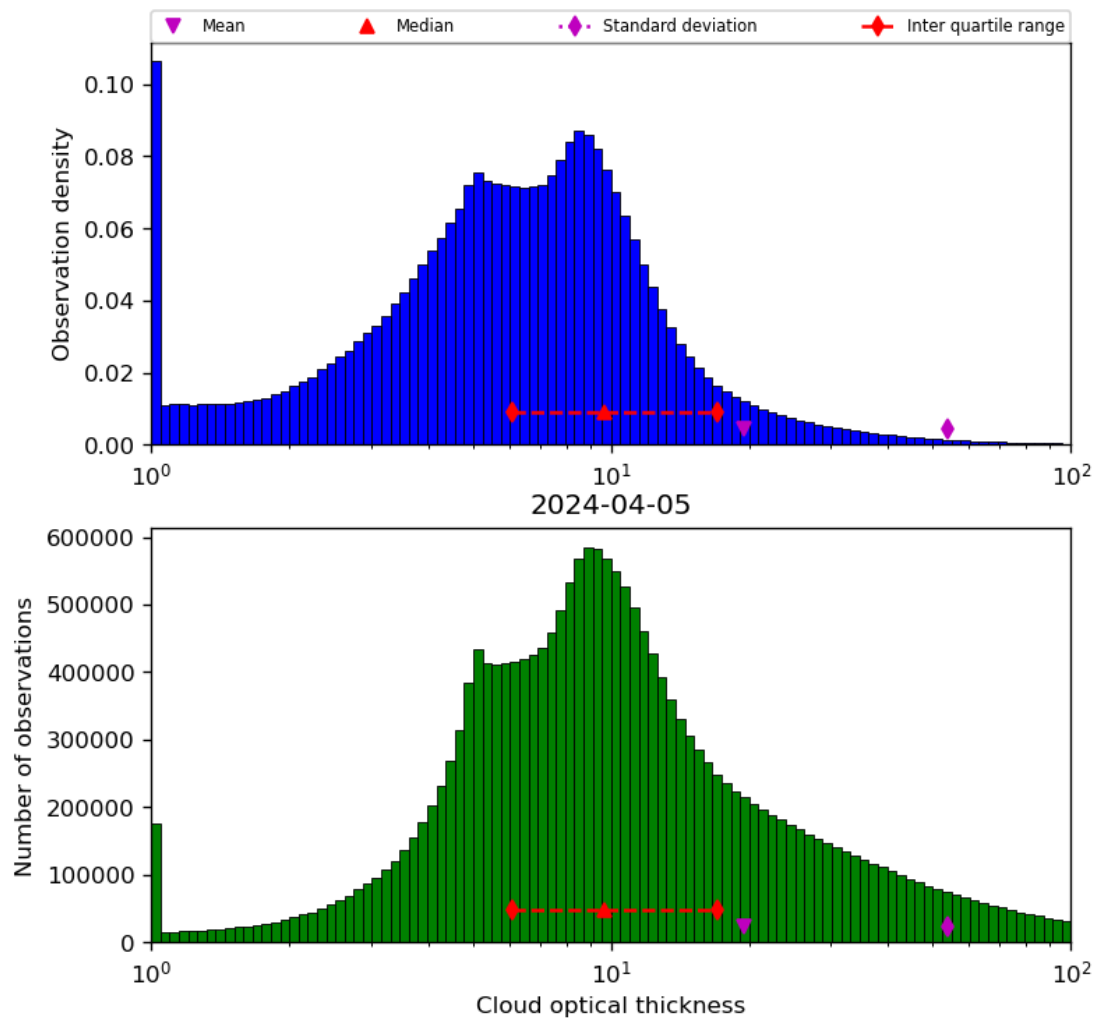
Figure 41: Histogram of “Cloud optical thickness” for 2024-04-05 to 2024-04-06
