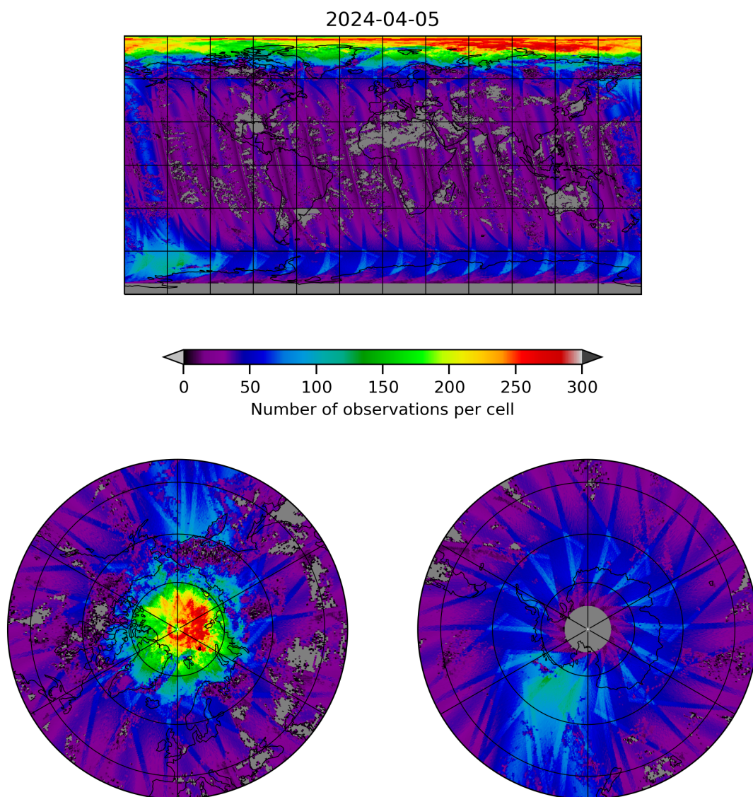
Figure 21: Map of the number of observations for 2024-04-05 to 2024-04-06
