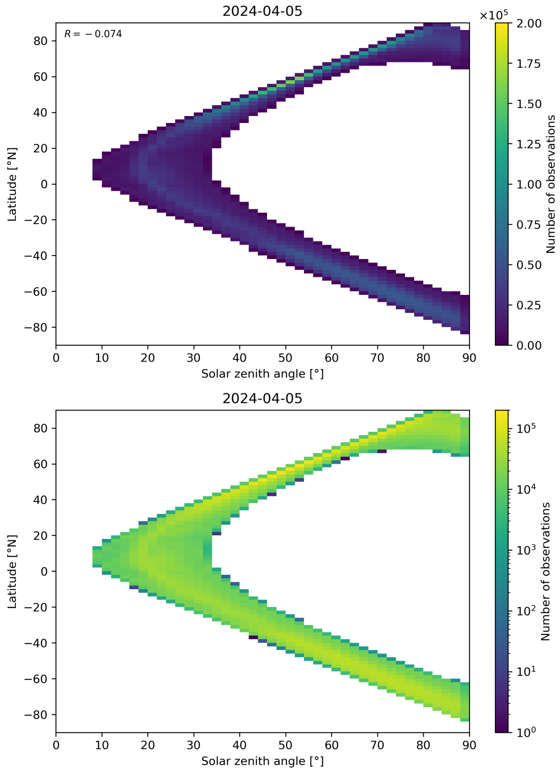
Figure 105: Scatter density plot of “Solar zenith angle” against “Latitude” for 2024-04-05 to 2024-04-06.
