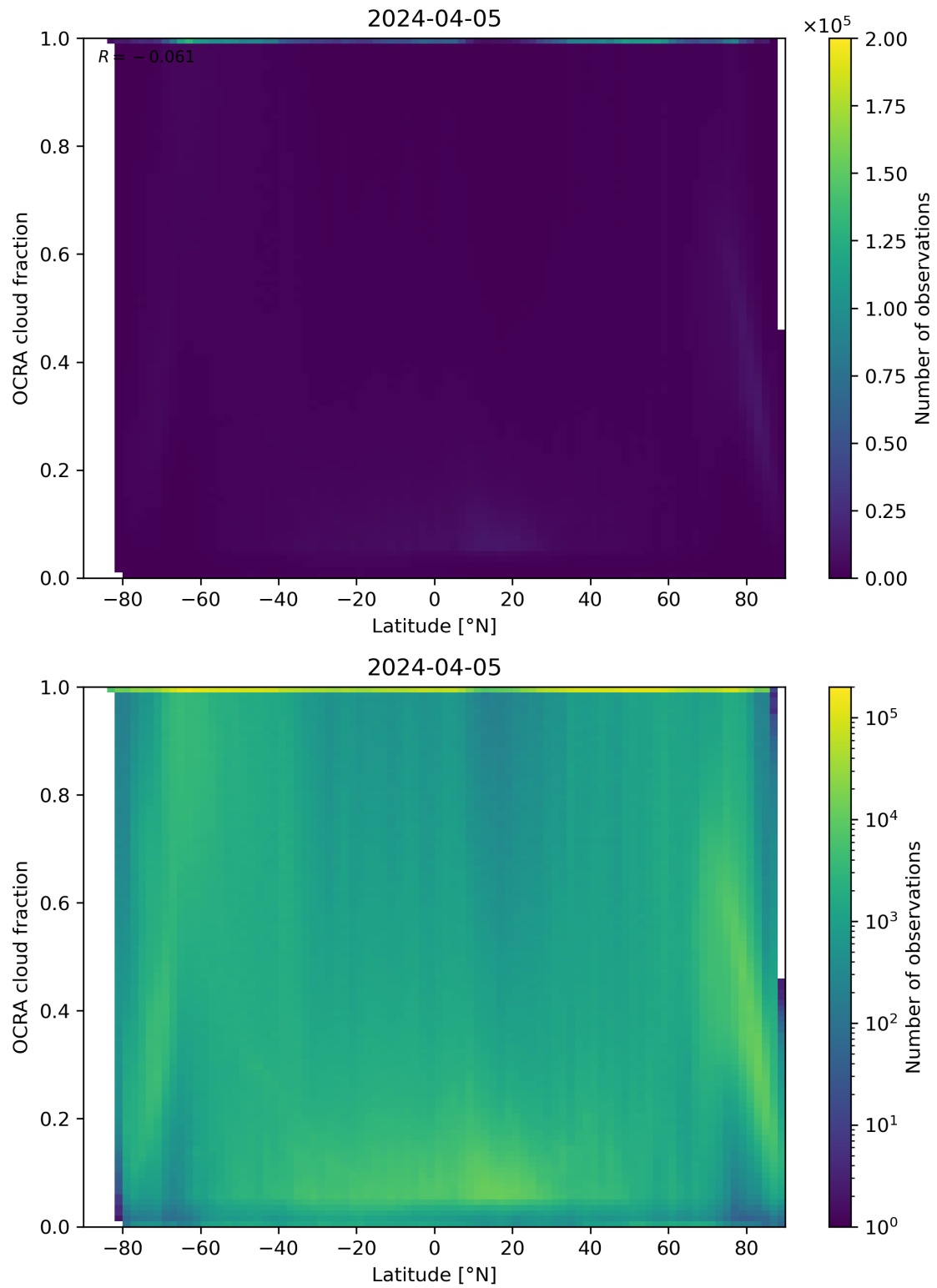
Figure 93: Scatter density plot of “Latitude” against “OCRA cloud fraction” for 2024-04-05 to 2024-04-06.
