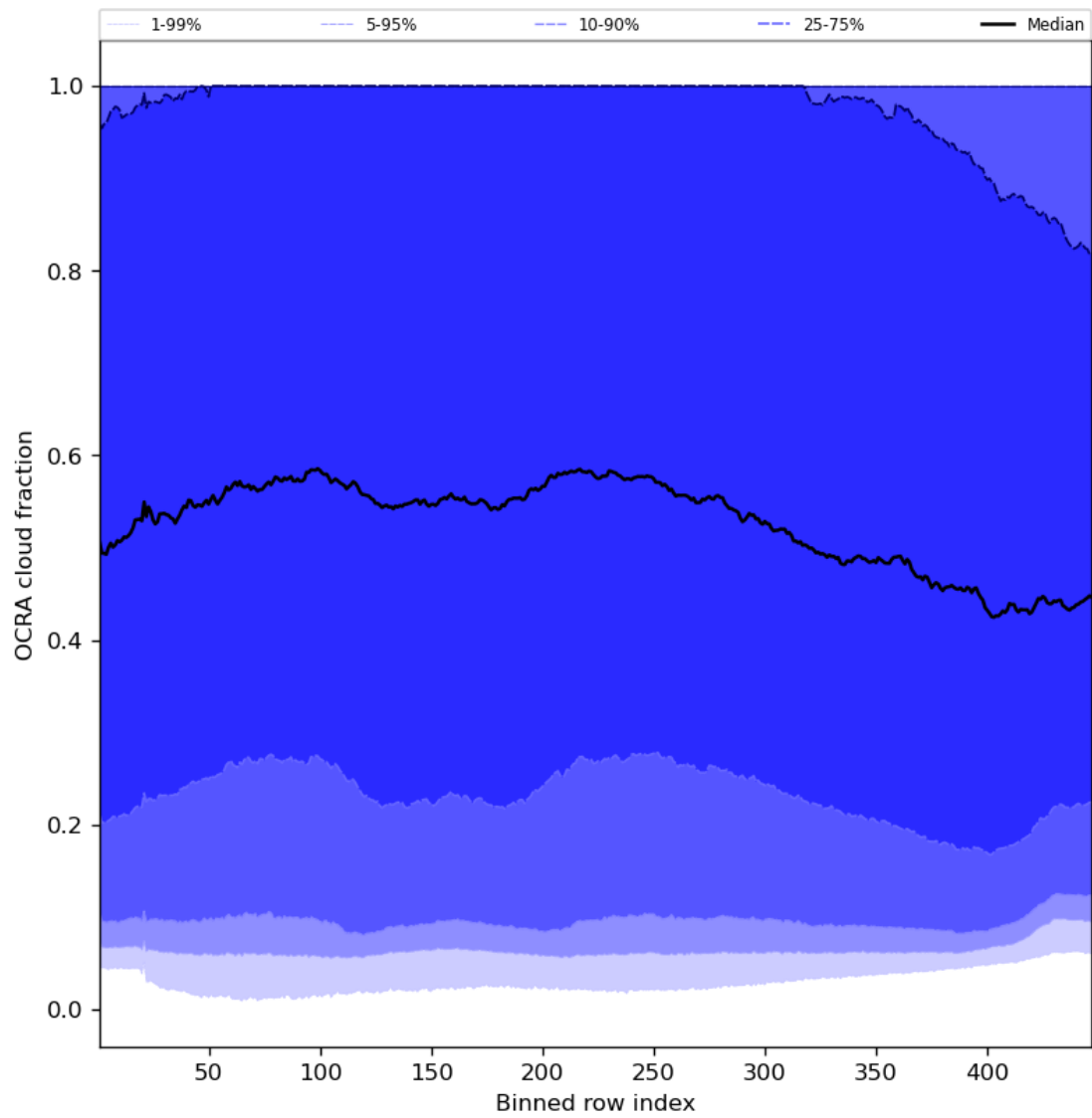
Figure 66: Along track statistics of “OCRA cloud fraction” for 2024-04-05 to 2024-04-06
