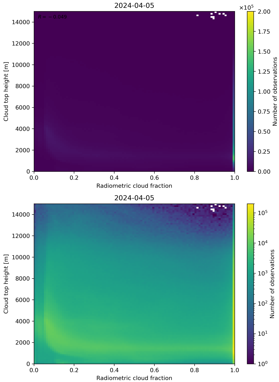
Figure 76: Scatter density plot of “Radiometric cloud fraction” against “Cloud top height” for 2024-04-05 to 2024-04-06.
