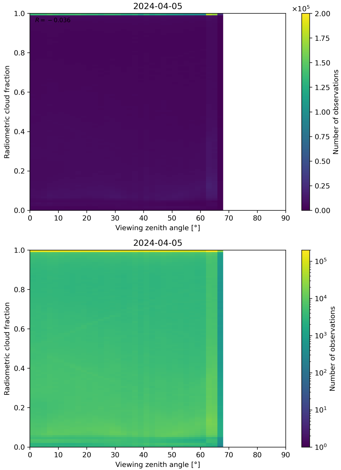
Figure 107: Scatter density plot of “Viewing zenith angle” against “Radiometric cloud fraction” for 2024-04-05 to 2024-04-06.
