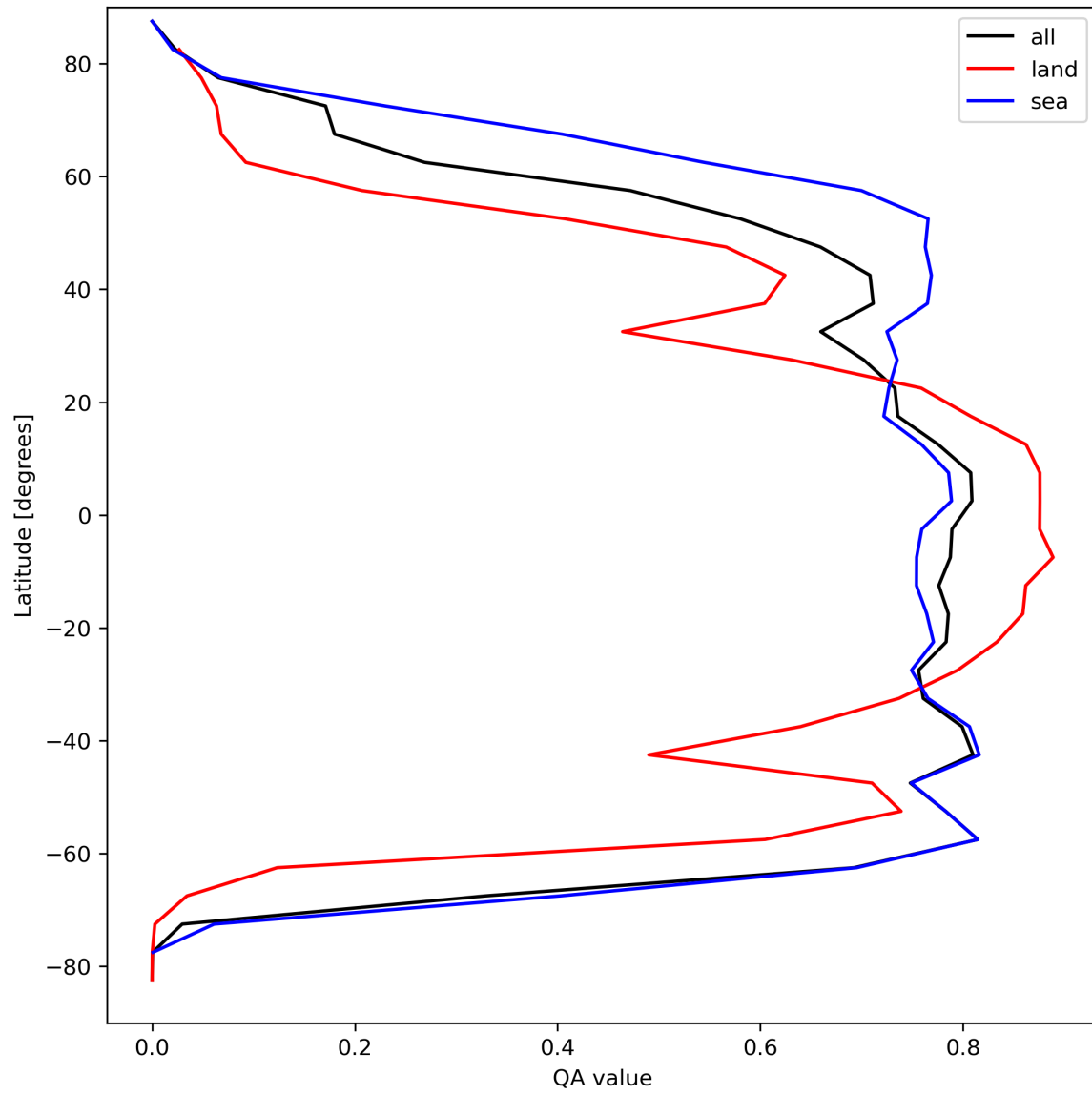
Figure 22: Zonal average of “QA value” for 2024-04-05 to 2024-04-06.
