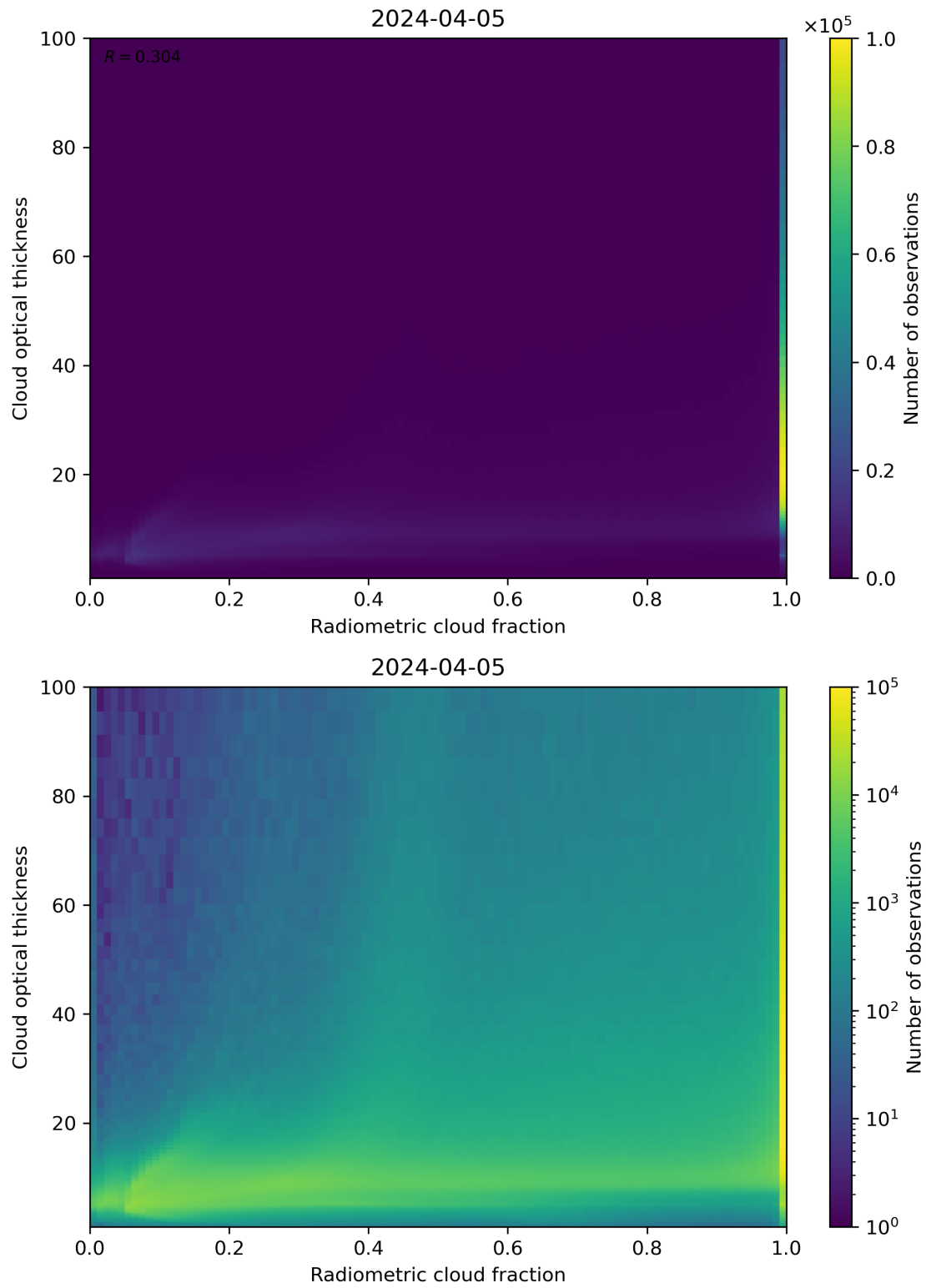
Figure 75: Scatter density plot of “Radiometric cloud fraction” against “Cloud optical thickness” for 2024-04-05 to 2024-04-06.
