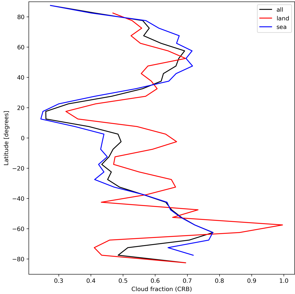
Figure 26: Zonal average of “Cloud fraction (CRB)” for 2024-04-05 to 2024-04-06.
