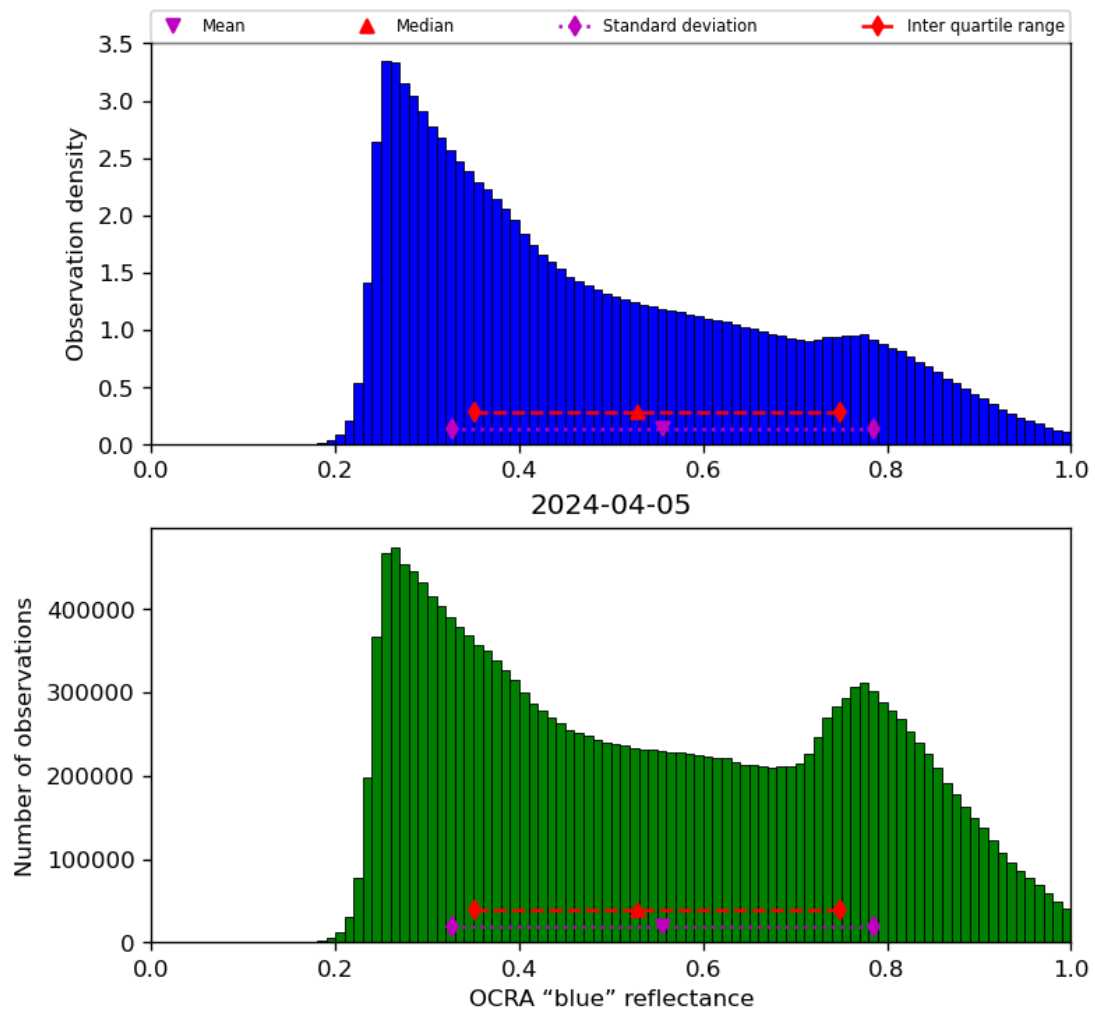
Figure 51: Histogram of “OCRA “blue” reflectance” for 2024-04-05 to 2024-04-06
