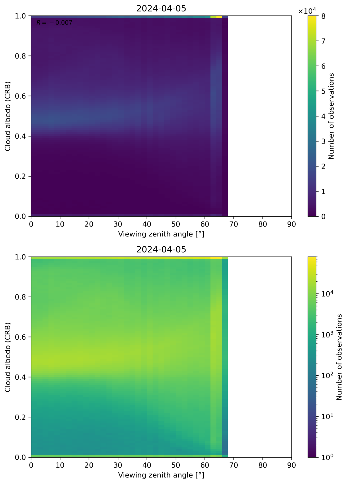
Figure 106: Scatter density plot of “Viewing zenith angle” against “Cloud albedo (CRB)” for 2024-04-05 to 2024-04-06.
