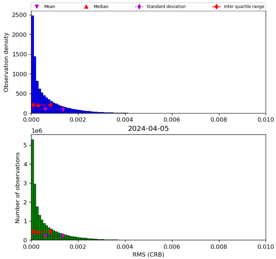
Figure 48: Histogram of "RMS (CRB)" for 2024-04-05 to 2024-04-06
