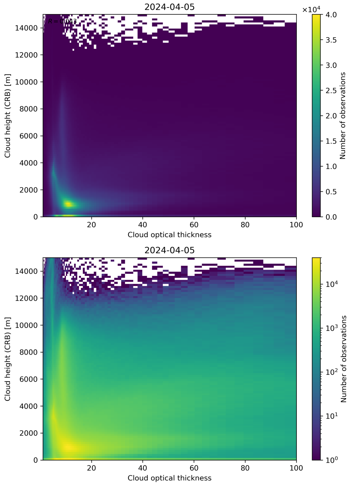
Figure 85: Scatter density plot of “Cloud optical thickness” against “Cloud height (CRB)” for 2024-04-05 to 2024-04-06.
