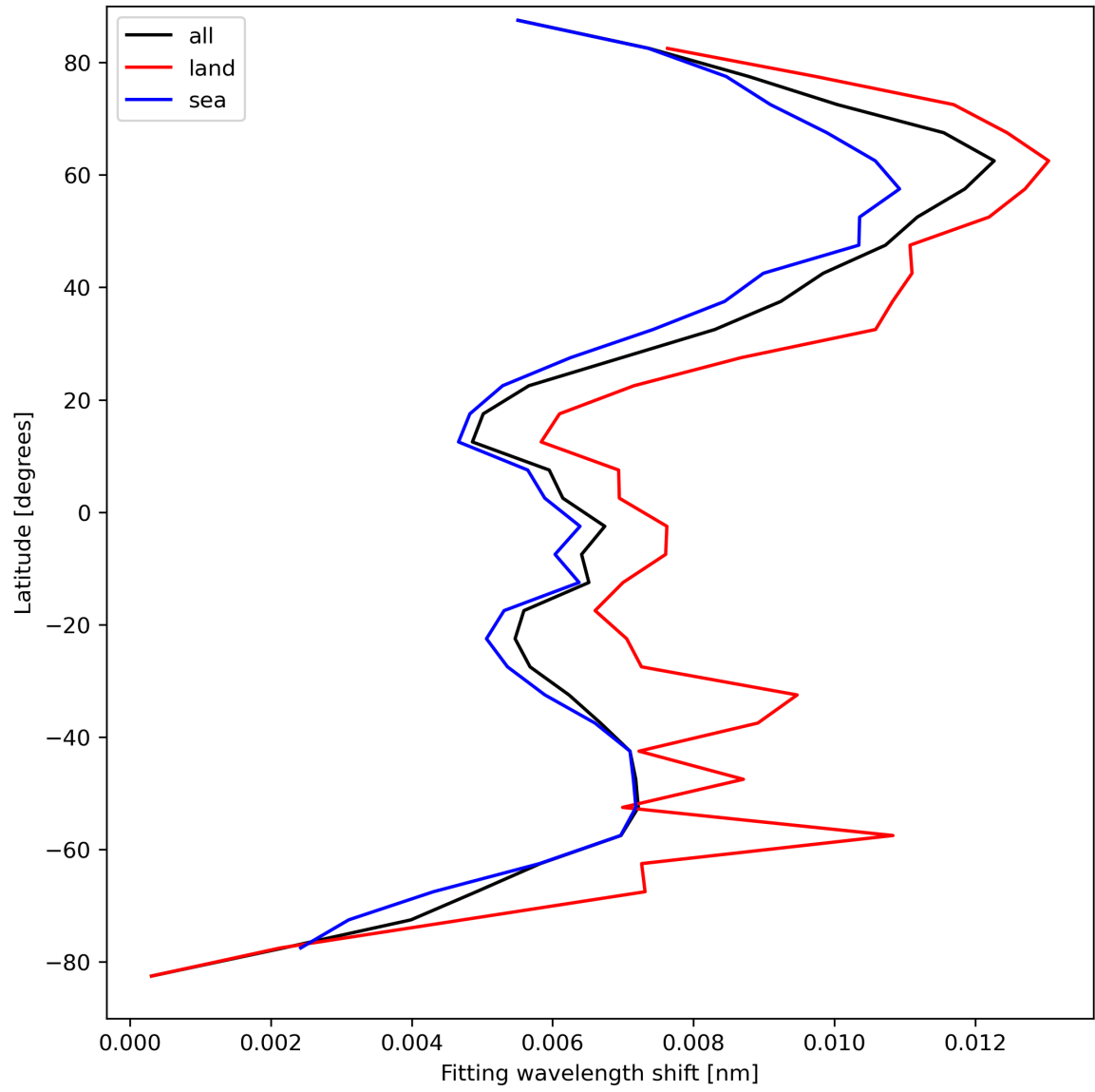
Figure 33: Zonal average of “Fitting wavelength shift” for 2024-04-05 to 2024-04-06.
