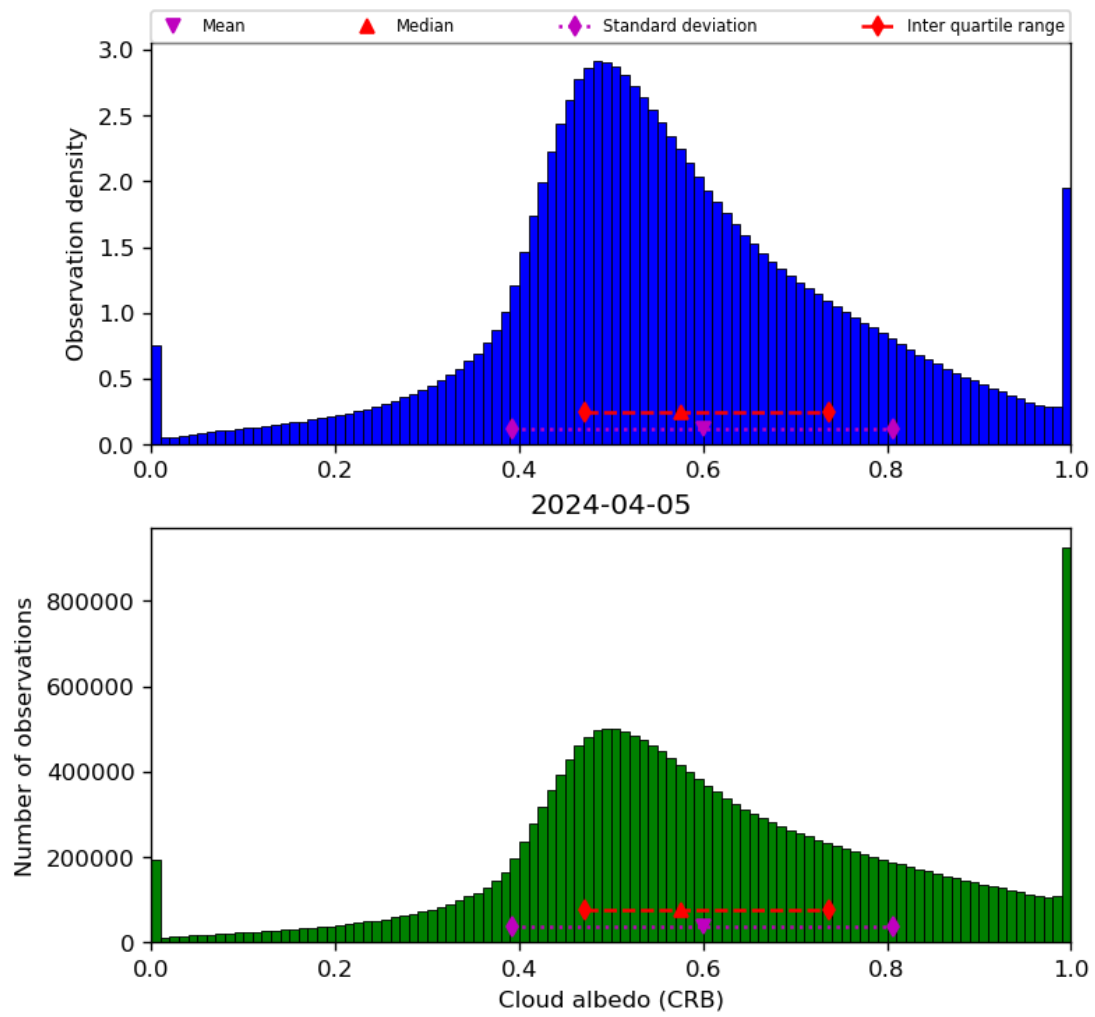
Figure 44: Histogram of “Cloud albedo (CRB)” for 2024-04-05 to 2024-04-06
