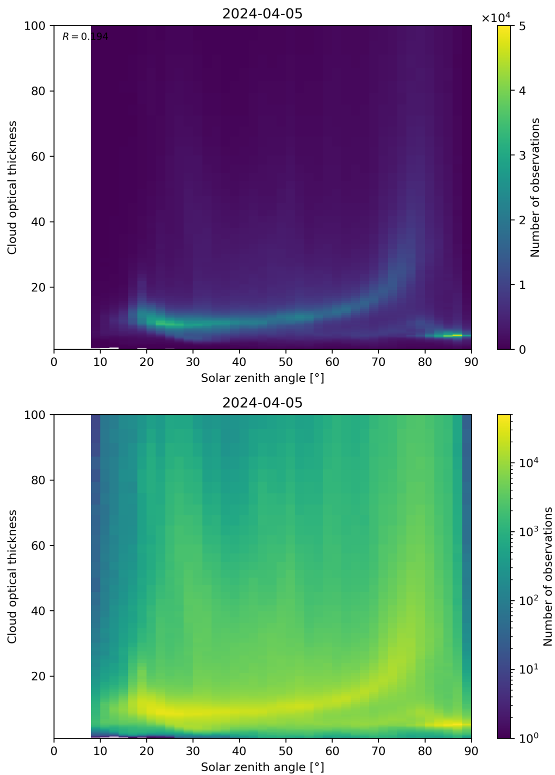
Figure 103: Scatter density plot of “Solar zenith angle” against “Cloud optical thickness” for 2024-04-05 to 2024-04-06.
