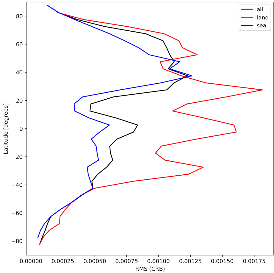
Figure 32: Zonal average of “RMS (CRB)” for 2024-04-05 to 2024-04-06.
