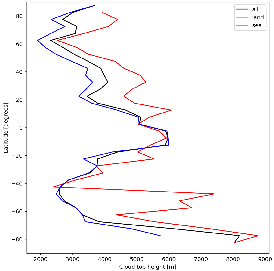
Figure 24: Zonal average of “Cloud top height” for 2024-04-05 to 2024-04-06.
