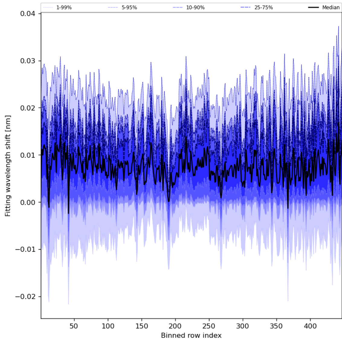
Figure 65: Along track statistics of “Fitting wavelength shift” for 2024-04-05 to 2024-04-06
