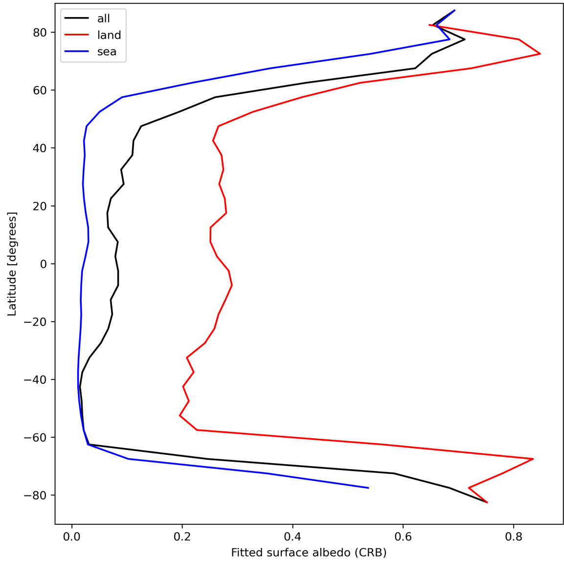
Figure 30: Zonal average of “Fitted surface albedo (CRB)” for 2024-04-05 to 2024-04-06.
