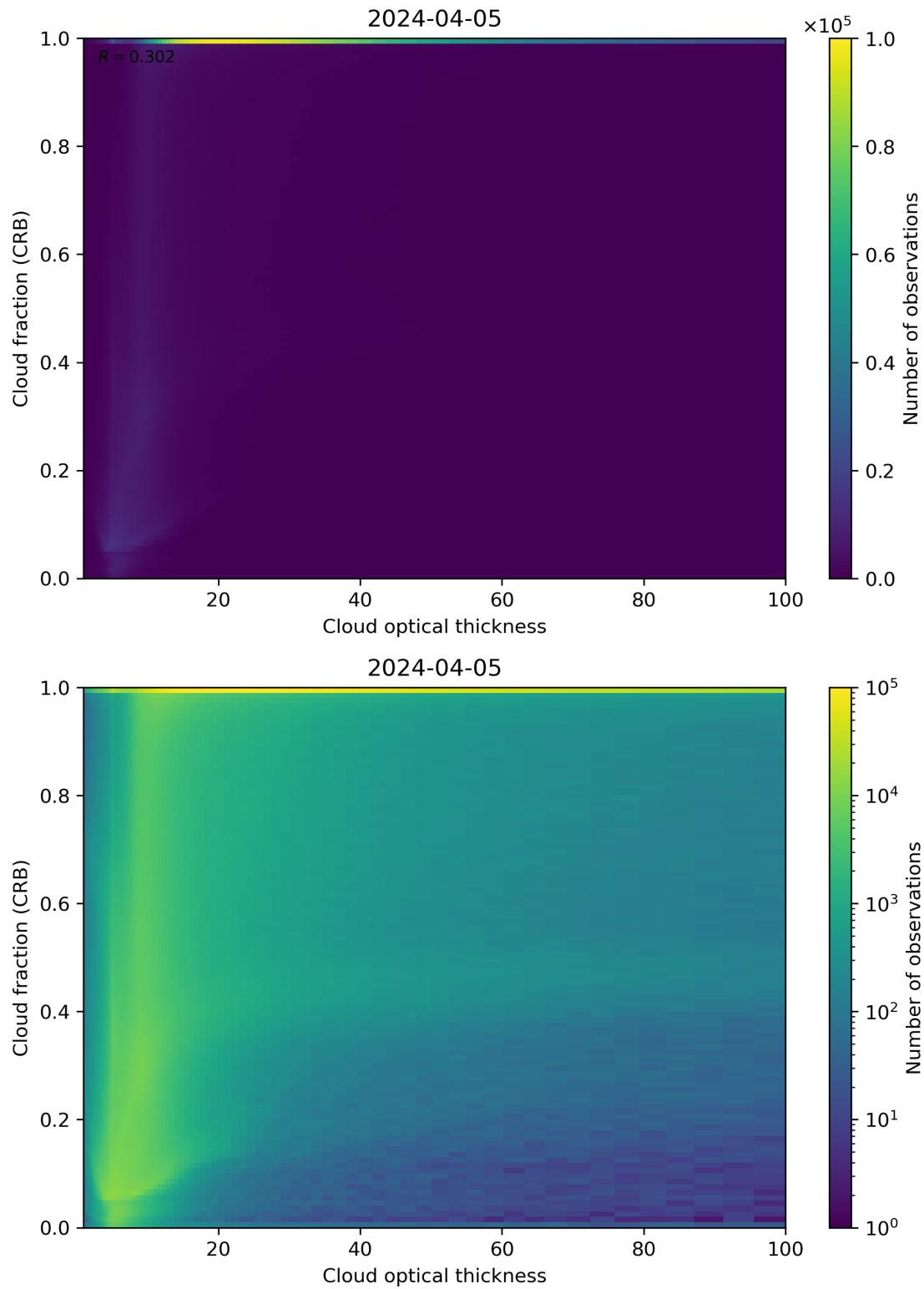
Figure 84: Scatter density plot of “Cloud optical thickness” against “Cloud fraction (CRB)” for 2024-04-05 to 2024-04-06.
