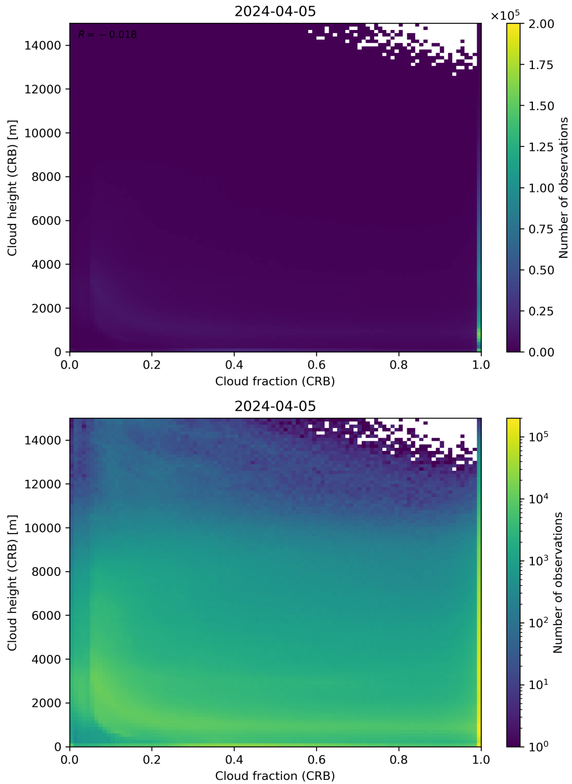
Figure 79: Scatter density plot of “Cloud fraction (CRB)” against “Cloud height (CRB)” for 2024-04-05 to 2024-04-06.
