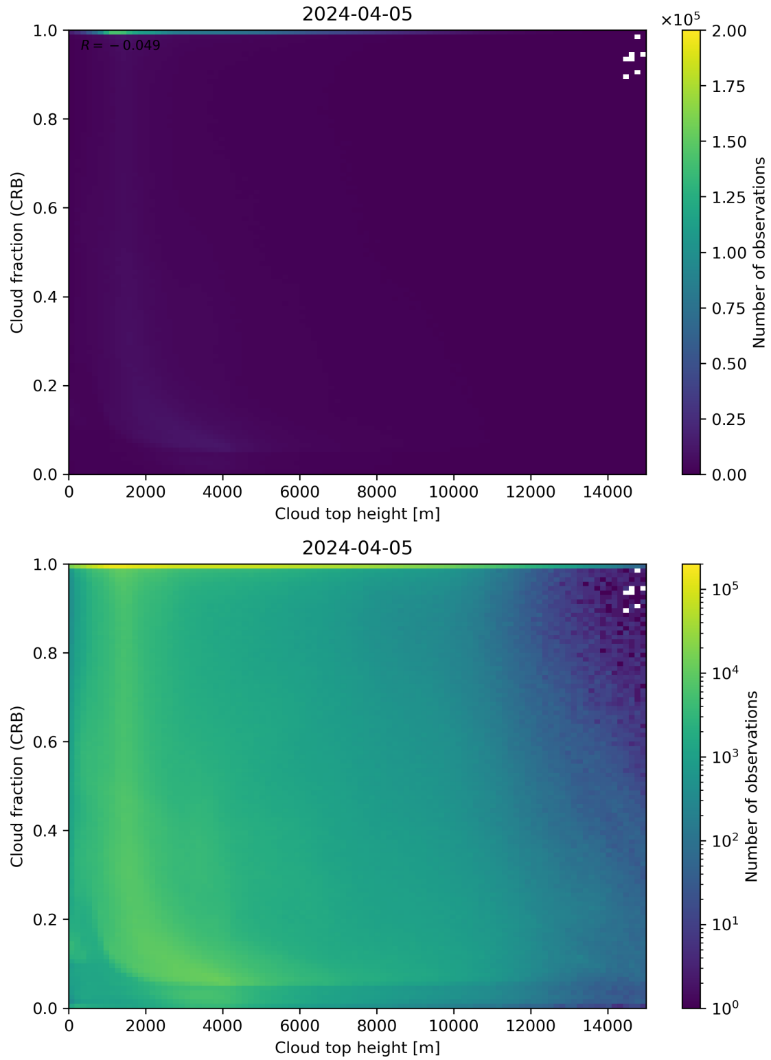
Figure 88: Scatter density plot of “Cloud top height” against “Cloud fraction (CRB)” for 2024-04-05 to 2024-04-06.
