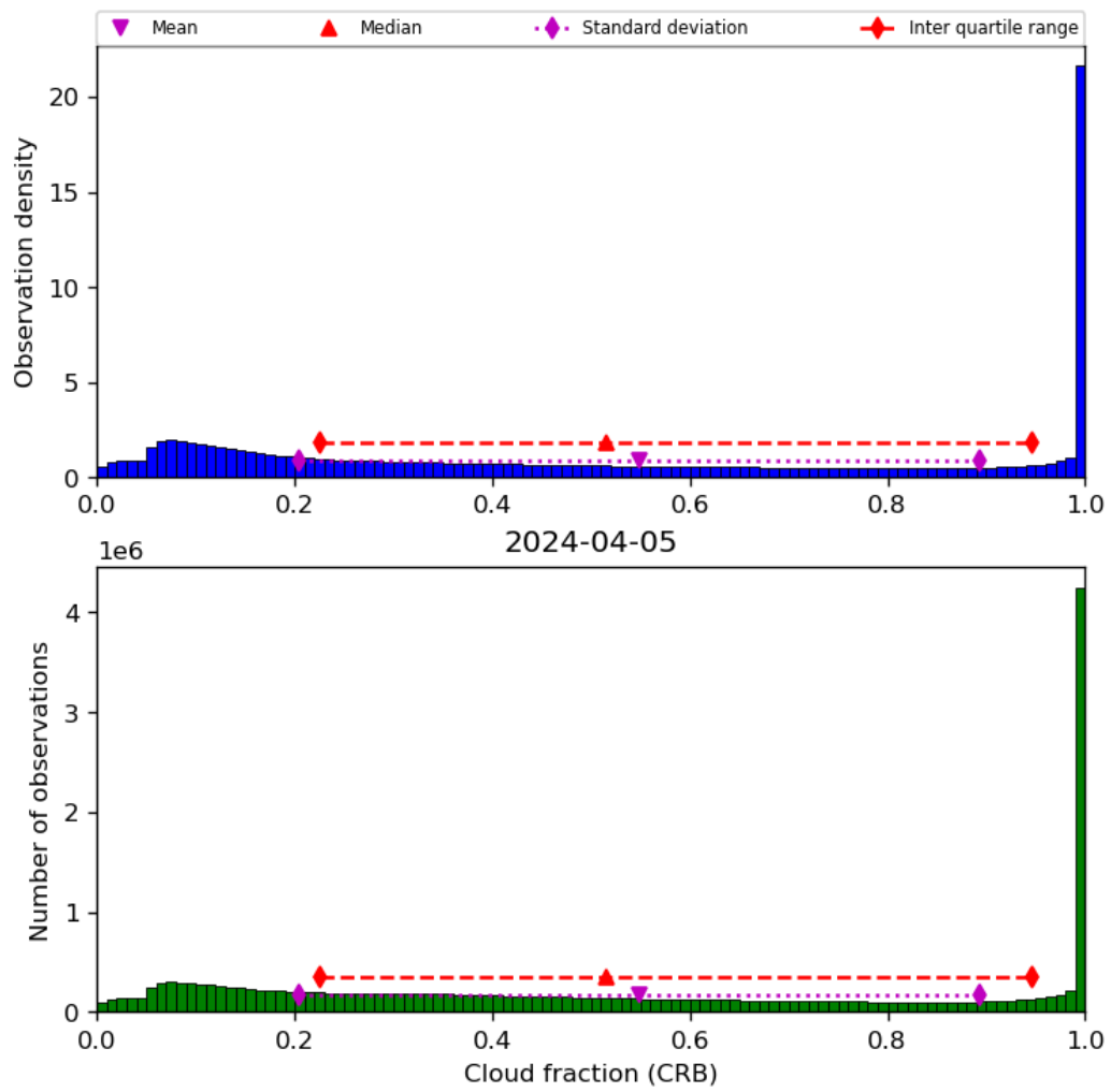
Figure 42: Histogram of “Cloud fraction (CRB)” for 2024-04-05 to 2024-04-06
