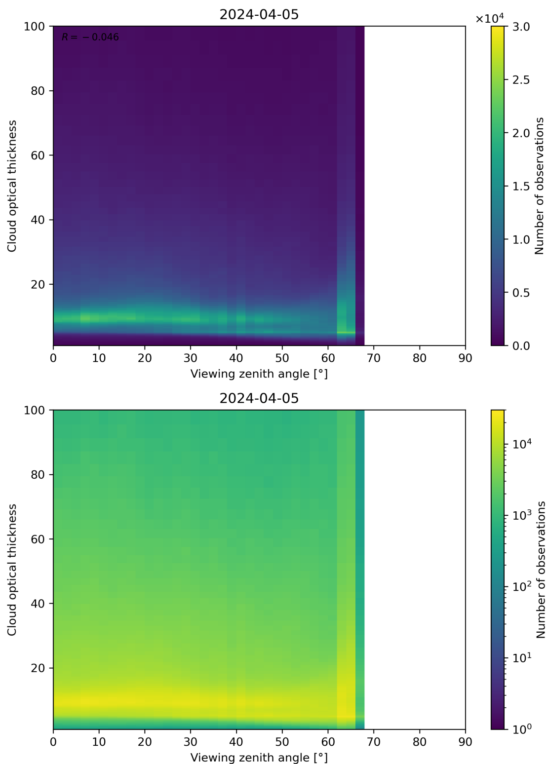
Figure 111: Scatter density plot of “Viewing zenith angle” against “Cloud optical thickness” for 2024-04-05 to 2024-04-06.
