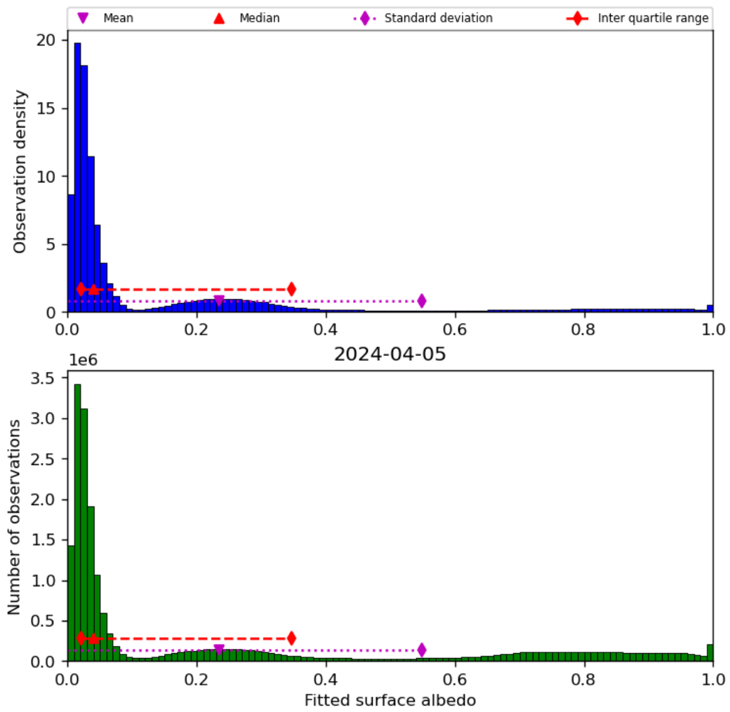
Figure 45: Histogram of “Fitted surface albedo” for 2024-04-05 to 2024-04-06
