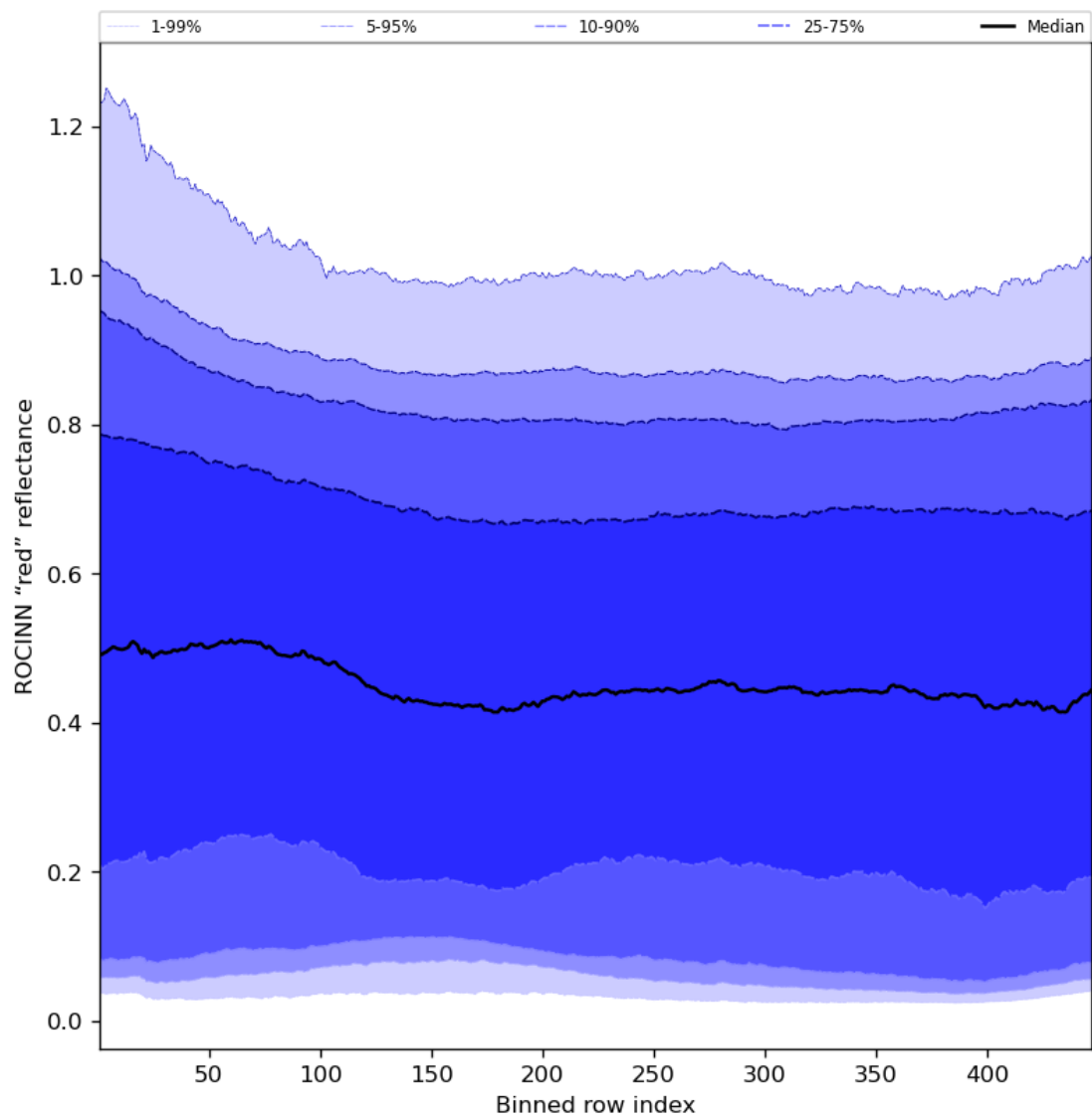
Figure 69: Along track statistics of “ROCINN “red” reflectance” for 2024-04-05 to 2024-04-06
