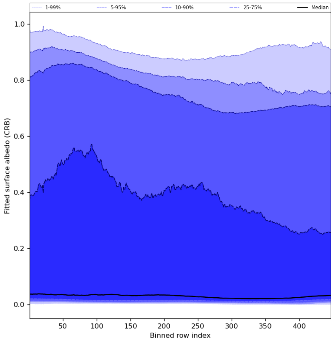
Figure 62: Along track statistics of “Fitted surface albedo (CRB)” for 2024-04-05 to 2024-04-06
