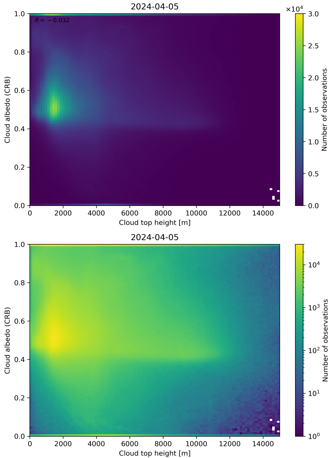
Figure 86: Scatter density plot of “Cloud top height” against “Cloud albedo (CRB)” for 2024-04-05 to 2024-04-06.
