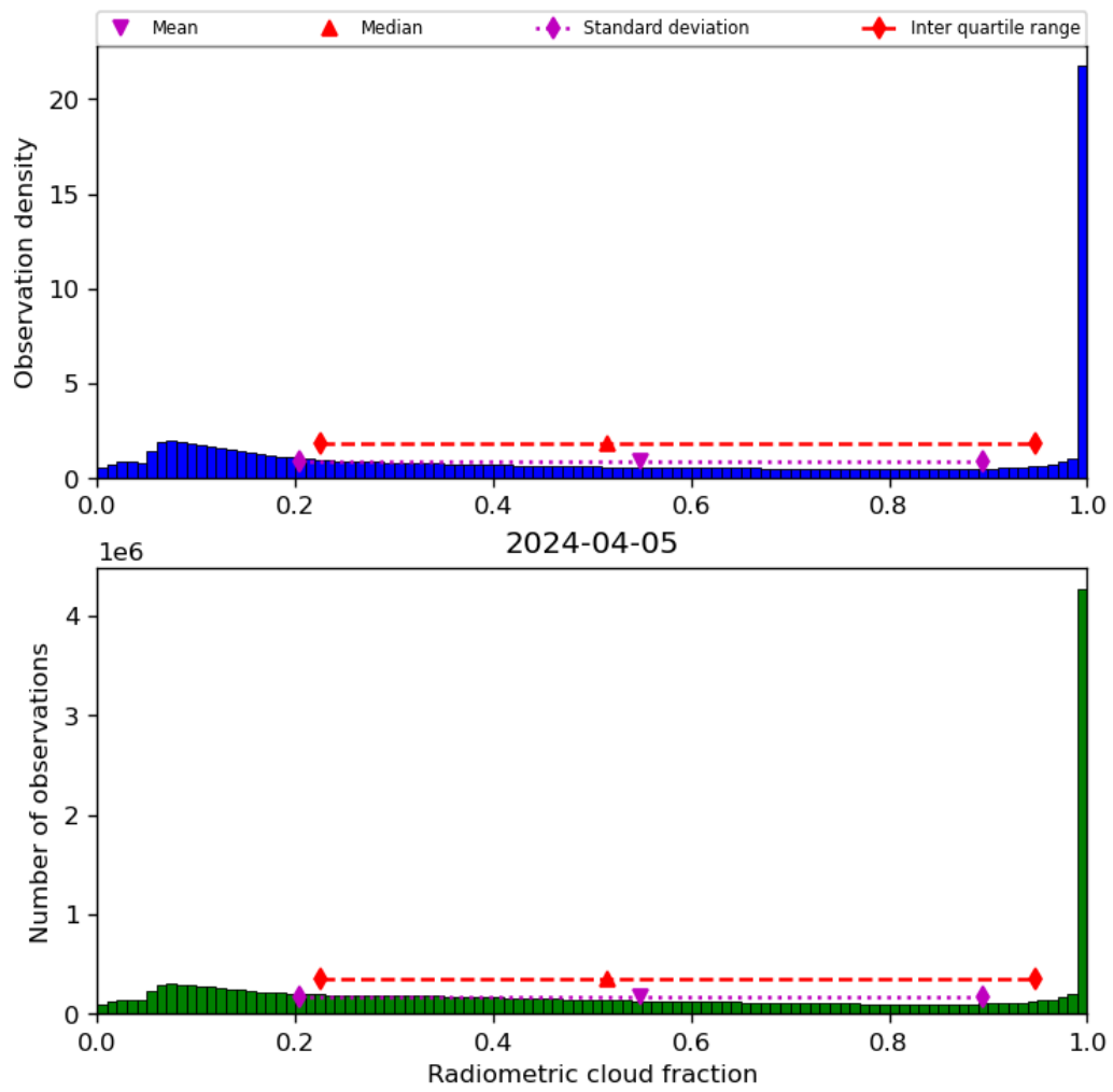
Figure 39: Histogram of “Radiometric cloud fraction” for 2024-04-05 to 2024-04-06
