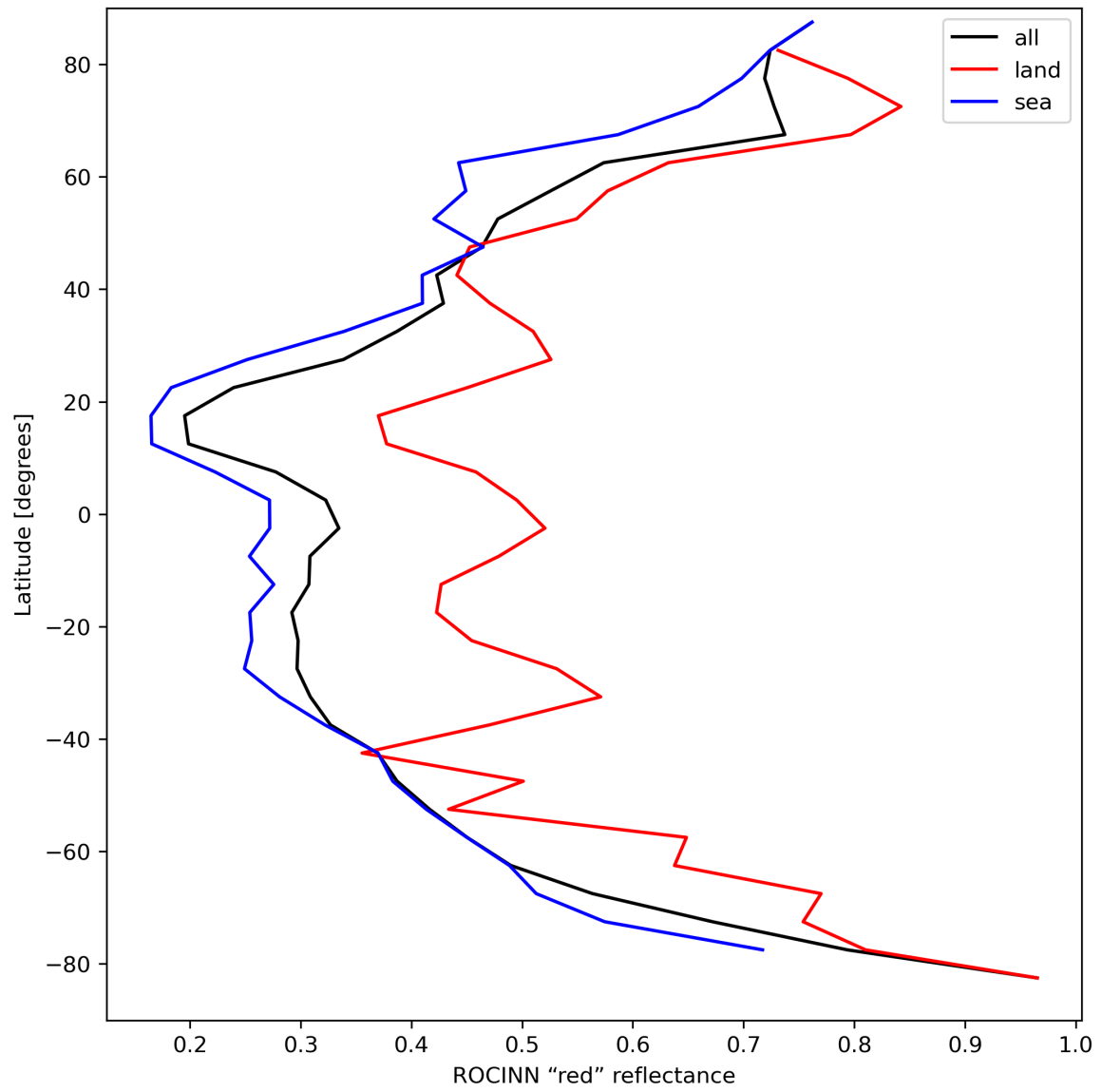
Figure 37: Zonal average of “ROCINN “red” reflectance” for 2024-04-05 to 2024-04-06.
