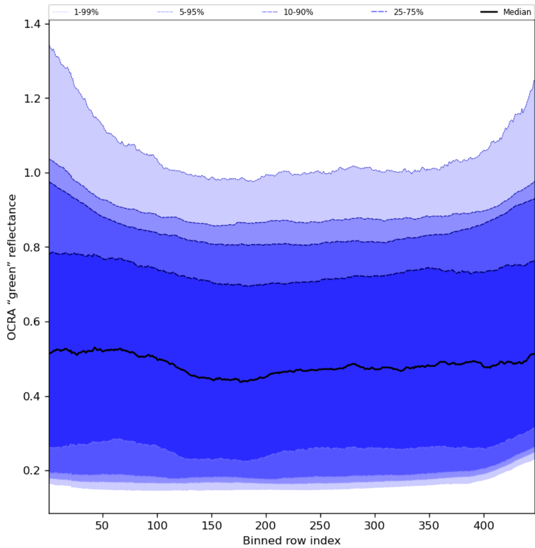
Figure 68: Along track statistics of "OCRA "green" reflectance" for 2024-04-05 to 2024-04-06
