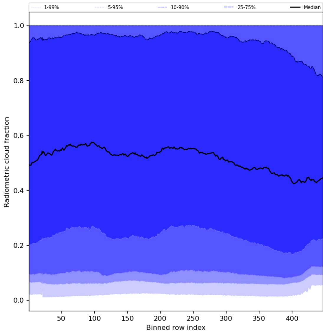
Figure 55: Along track statistics of “Radiometric cloud fraction” for 2024-04-05 to 2024-04-06
