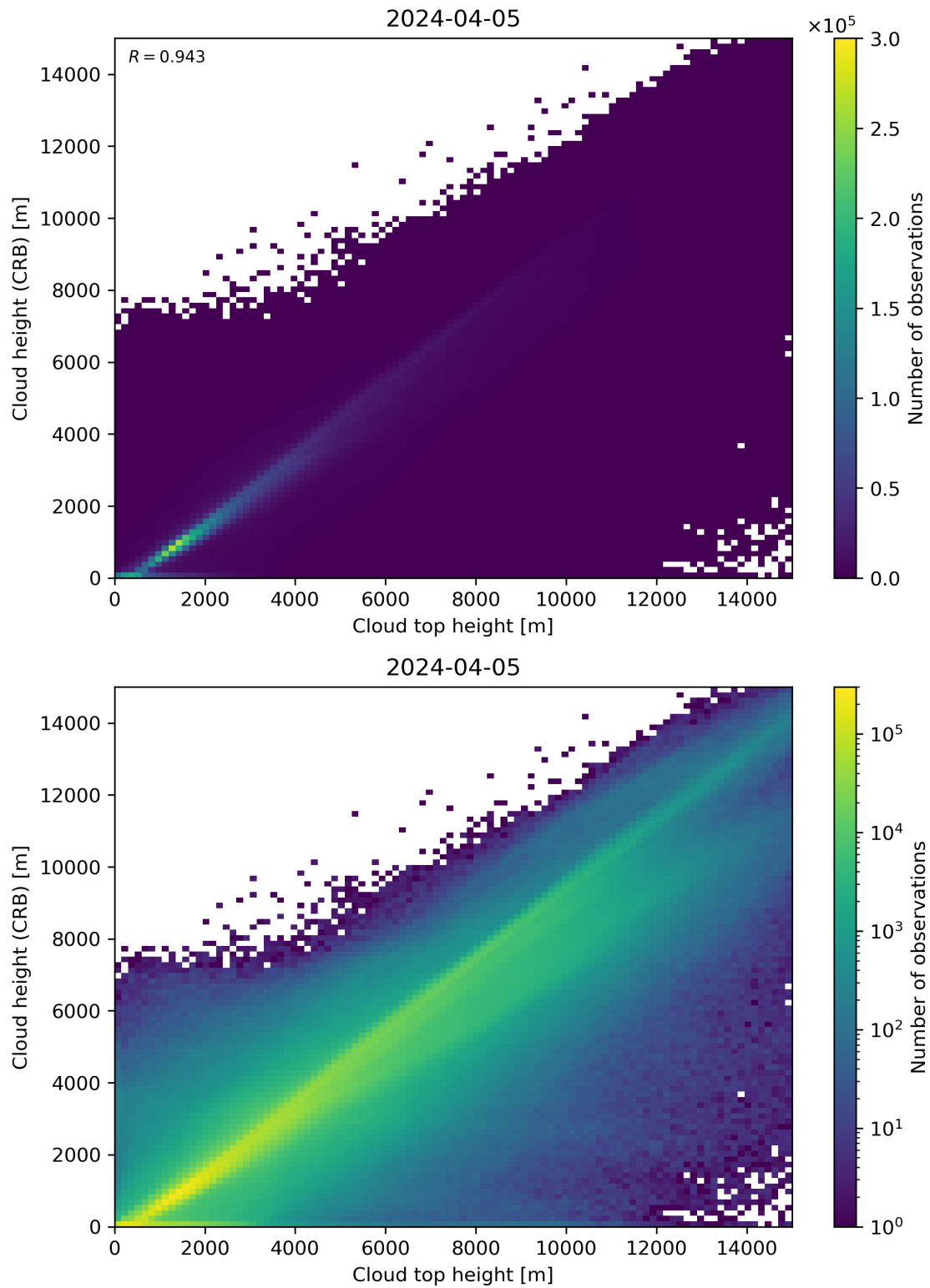
Figure 89: Scatter density plot of “Cloud top height” against “Cloud height (CRB)” for 2024-04-05 to 2024-04-06.
