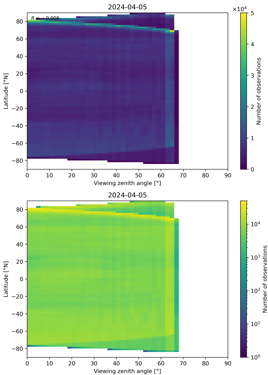
Figure 113: Scatter density plot of “Viewing zenith angle” against “Latitude” for 2024-04-05 to 2024-04-06.
