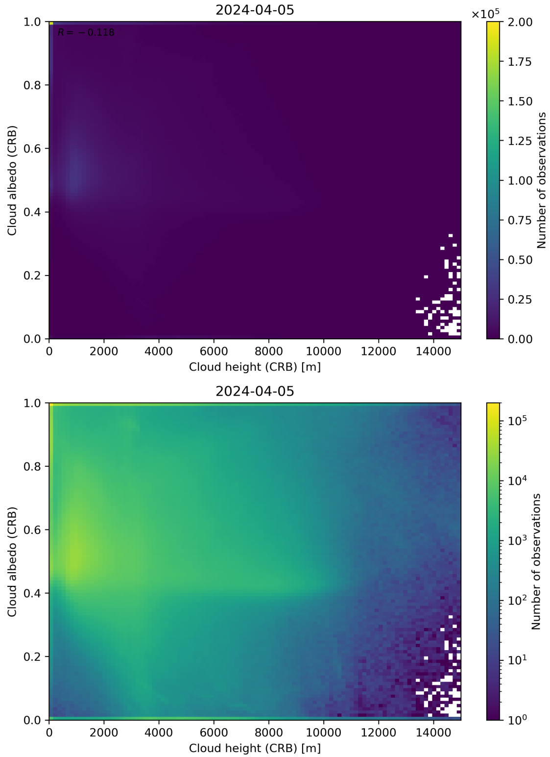
Figure 80: Scatter density plot of “Cloud height (CRB)” against “Cloud albedo (CRB)” for 2024-04-05 to 2024-04-06.
