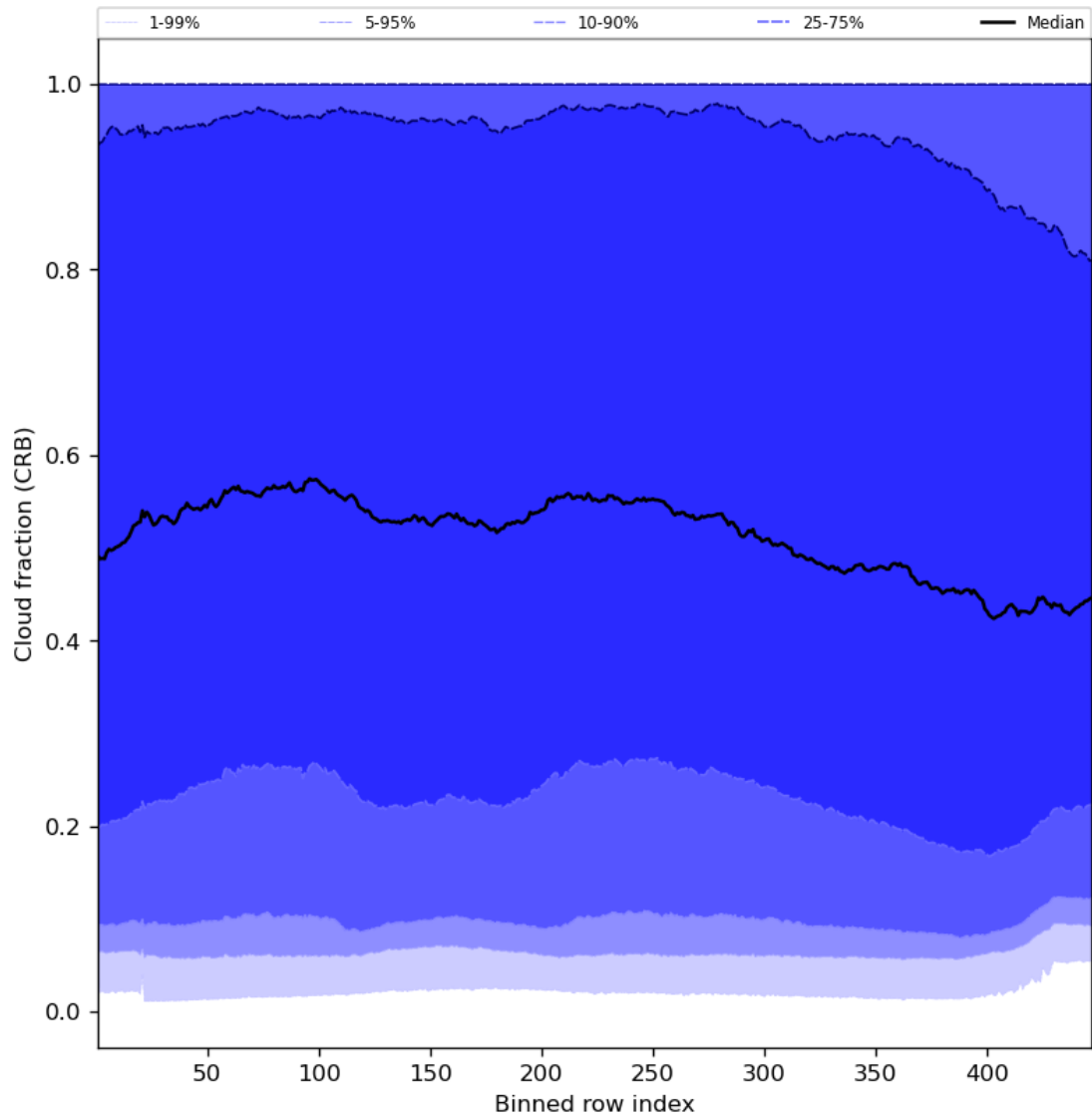
Figure 58: Along track statistics of “Cloud fraction (CRB)” for 2024-04-05 to 2024-04-06
