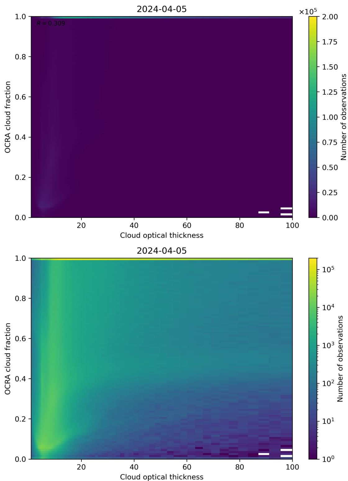
Figure 83: Scatter density plot of “Cloud optical thickness” against “OCRA cloud fraction” for 2024-04-05 to 2024-04-06.
