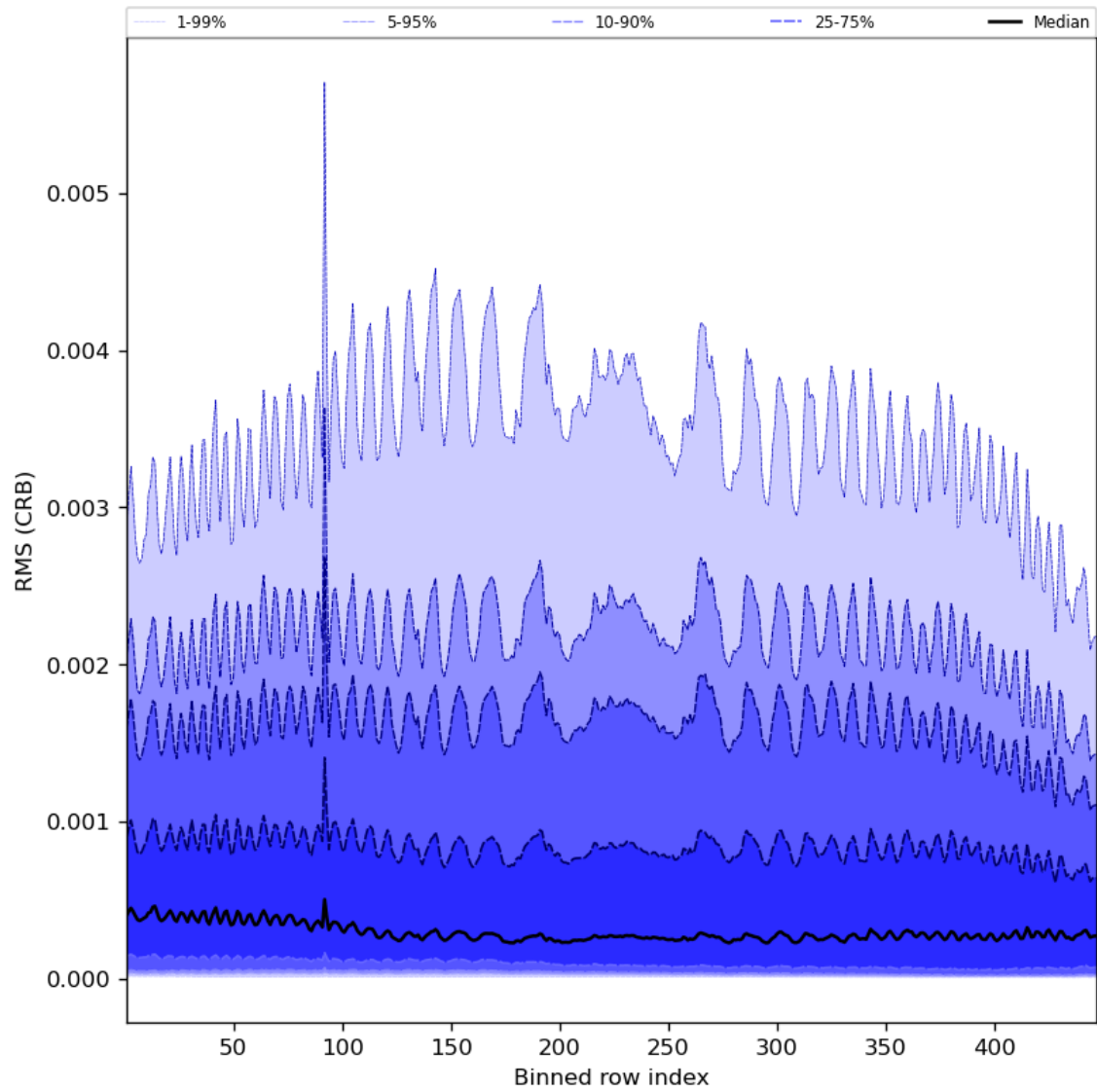
Figure 64: Along track statistics of “RMS (CRB)” for 2024-04-05 to 2024-04-06
