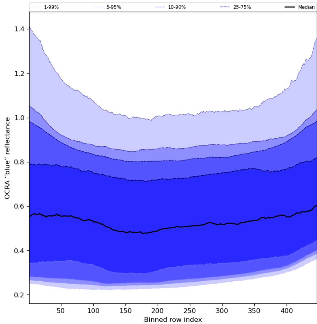
Figure 67: Along track statistics of “OCRA “blue” reflectance” for 2024-04-05 to 2024-04-06
