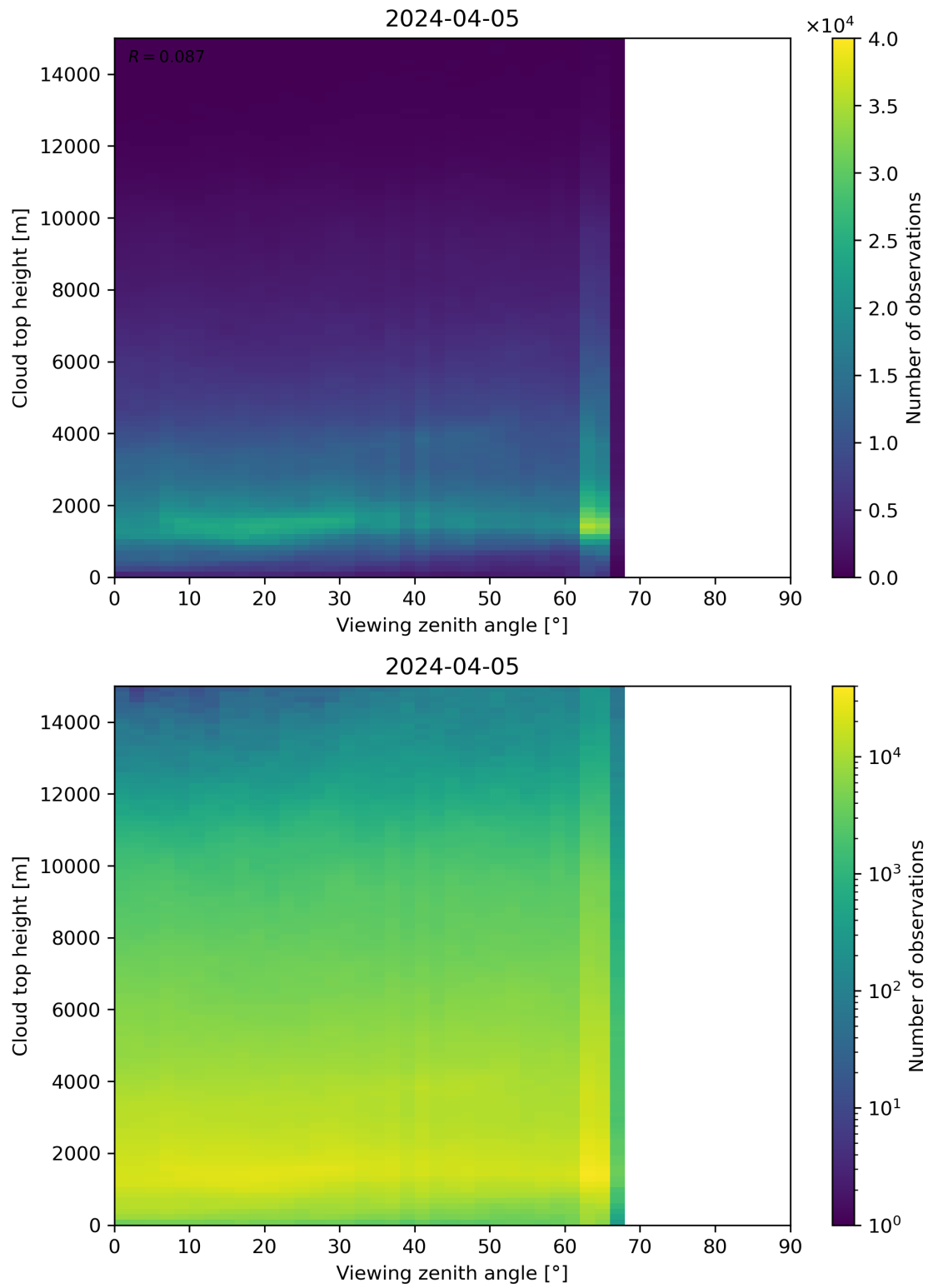
Figure 112: Scatter density plot of “Viewing zenith angle” against “Cloud top height” for 2024-04-05 to 2024-04-06.
