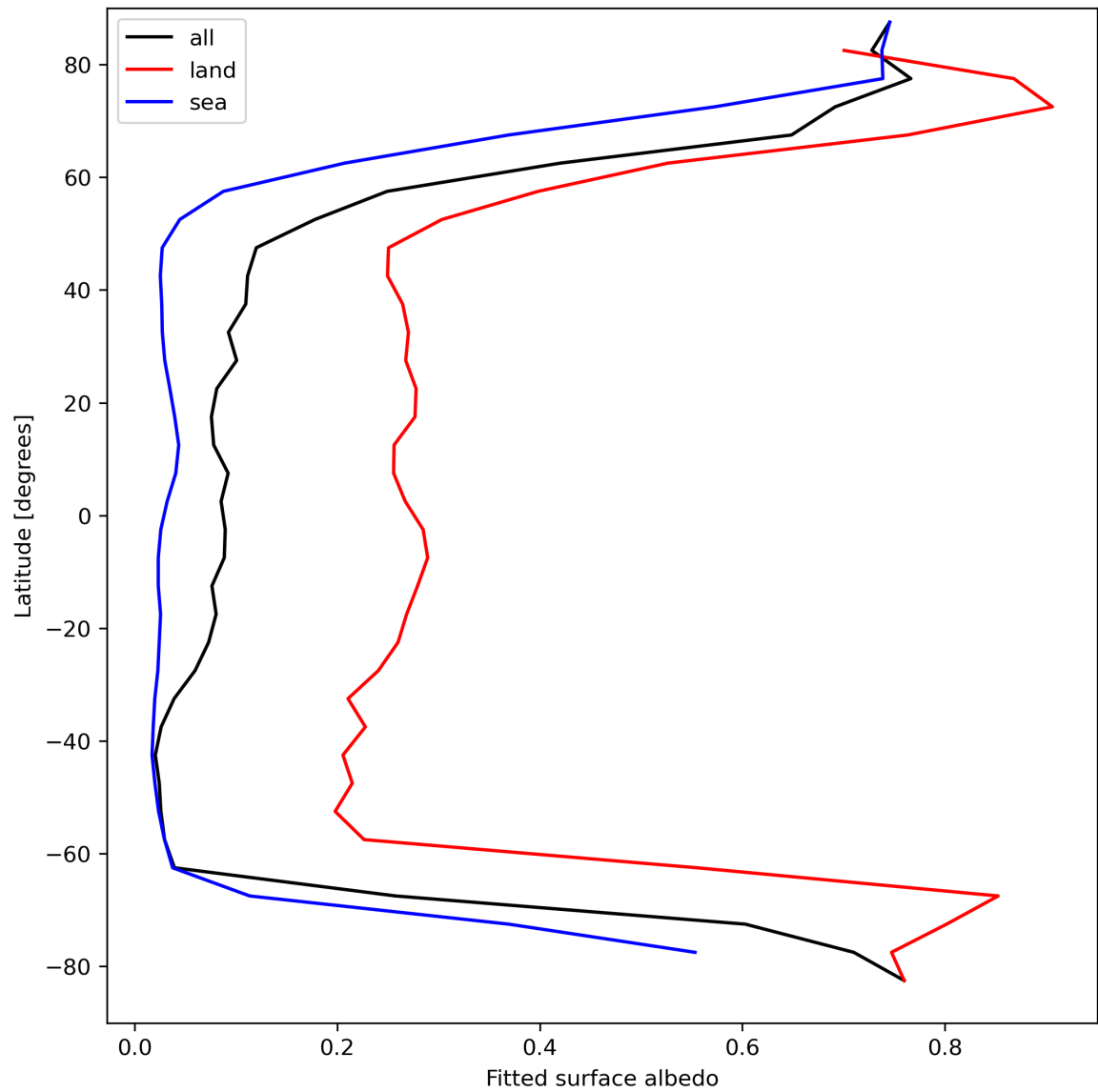
Figure 29: Zonal average of “Fitted surface albedo” for 2024-04-05 to 2024-04-06.
