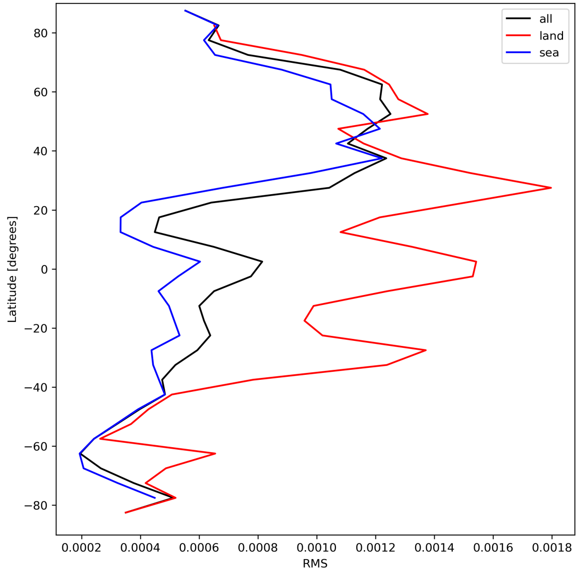
Figure 31: Zonal average of “RMS” for 2024-04-05 to 2024-04-06.
