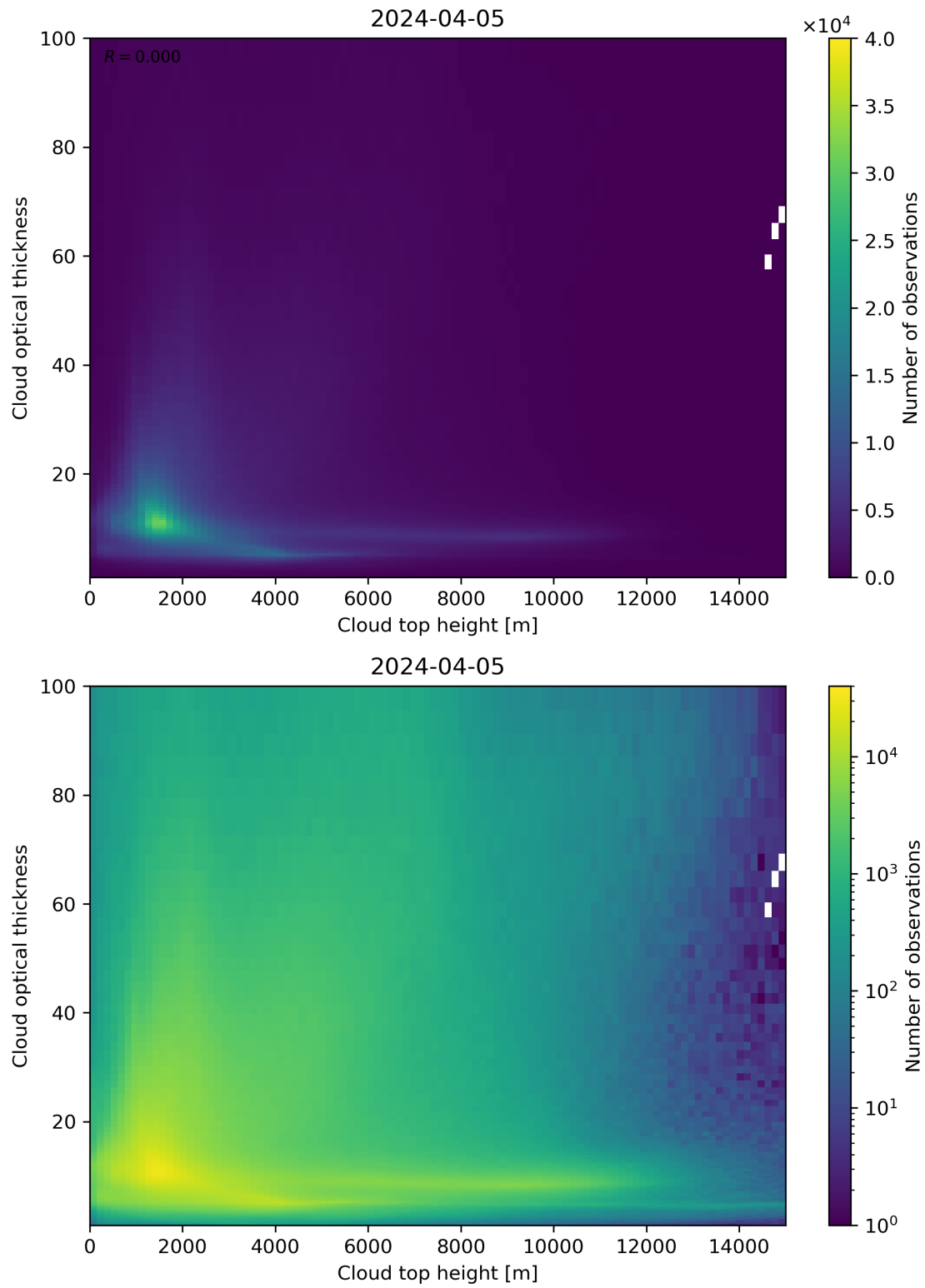
Figure 90: Scatter density plot of “Cloud top height” against “Cloud optical thickness” for 2024-04-05 to 2024-04-06.
