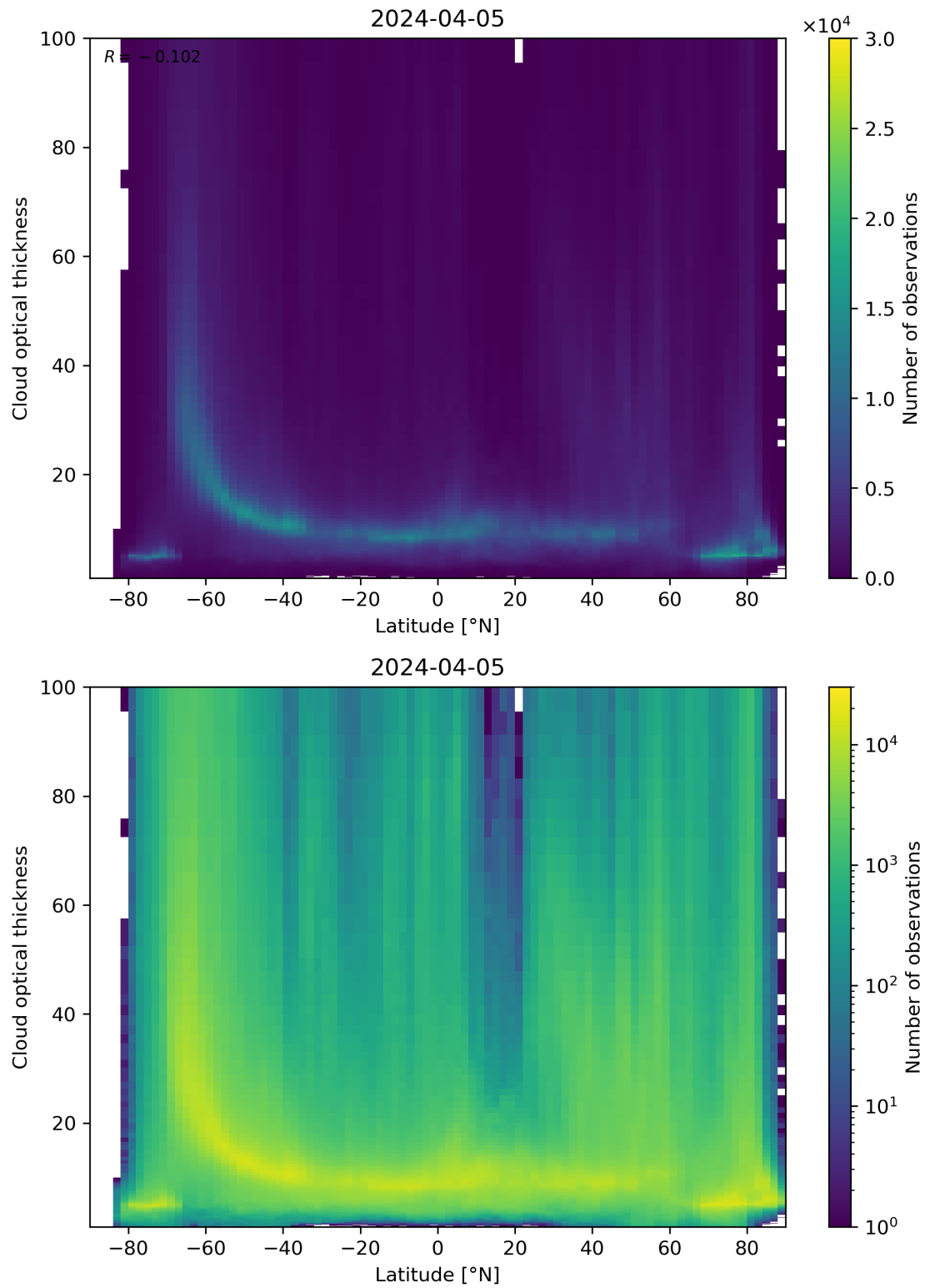
Figure 96: Scatter density plot of “Latitude” against “Cloud optical thickness” for 2024-04-05 to 2024-04-06.
