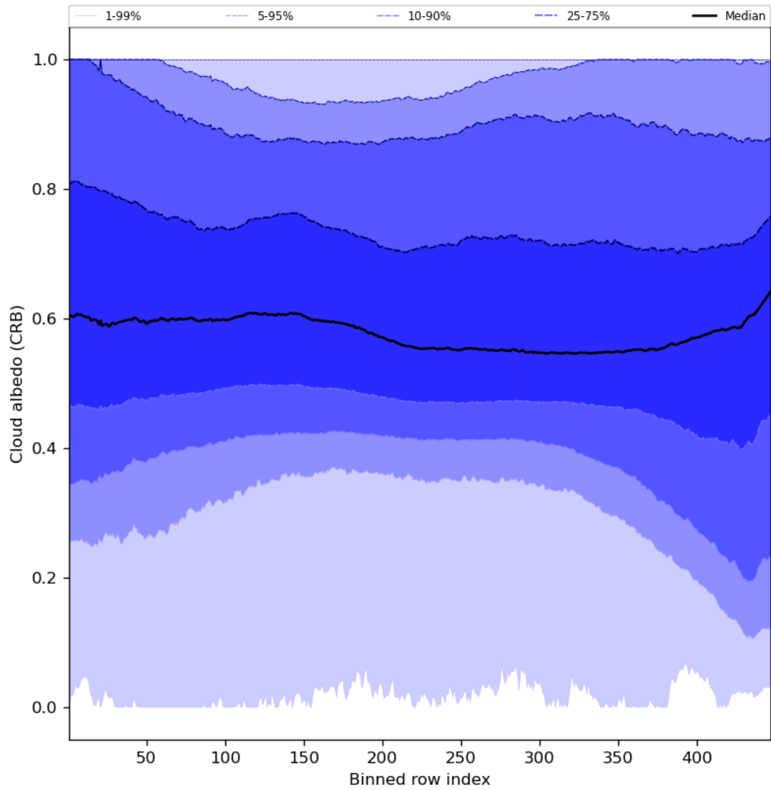
Figure 60: Along track statistics of “Cloud albedo (CRB)” for 2024-04-05 to 2024-04-06
