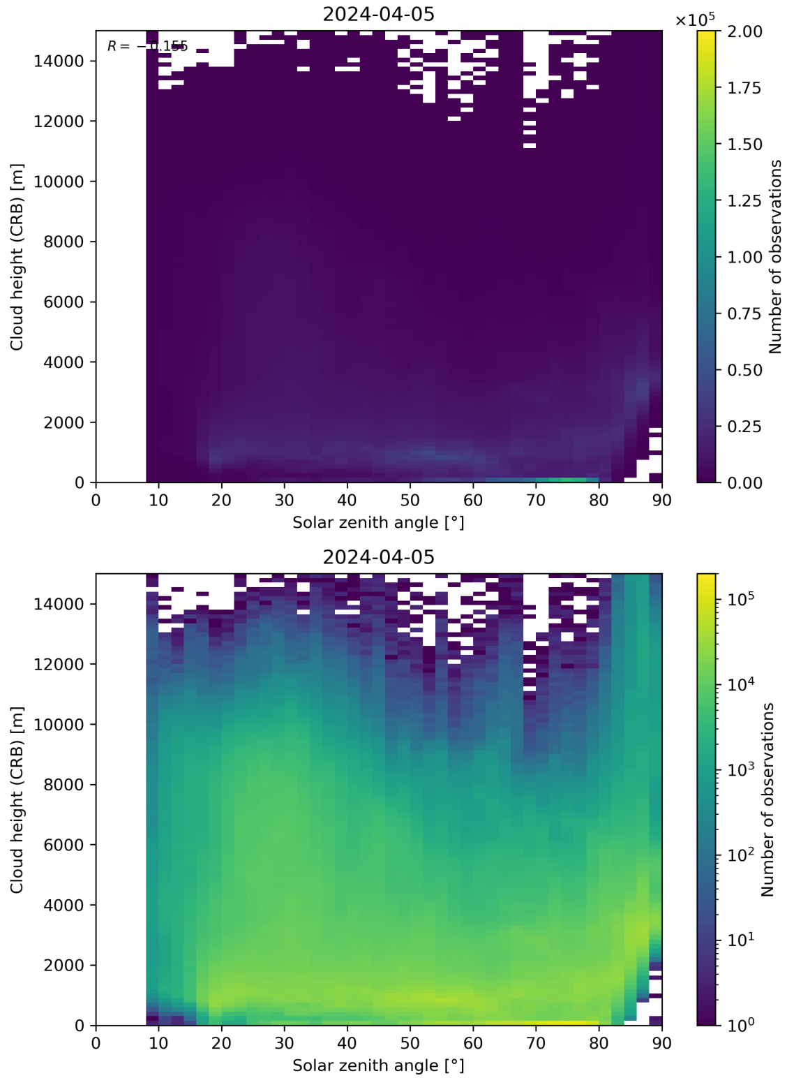
Figure 102: Scatter density plot of “Solar zenith angle” against “Cloud height (CRB)” for 2024-04-05 to 2024-04-06.
