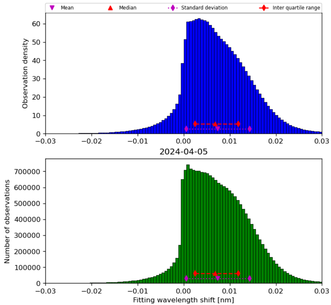
Figure 49: Histogram of “Fitting wavelength shift” for 2024-04-05 to 2024-04-06
