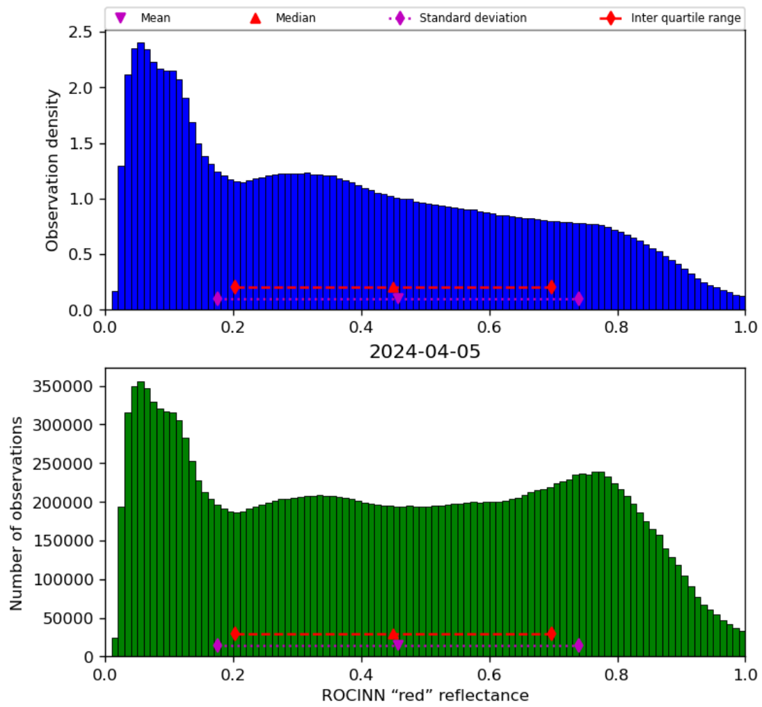
Figure 53: Histogram of “ROCINN “red” reflectance” for 2024-04-05 to 2024-04-06
