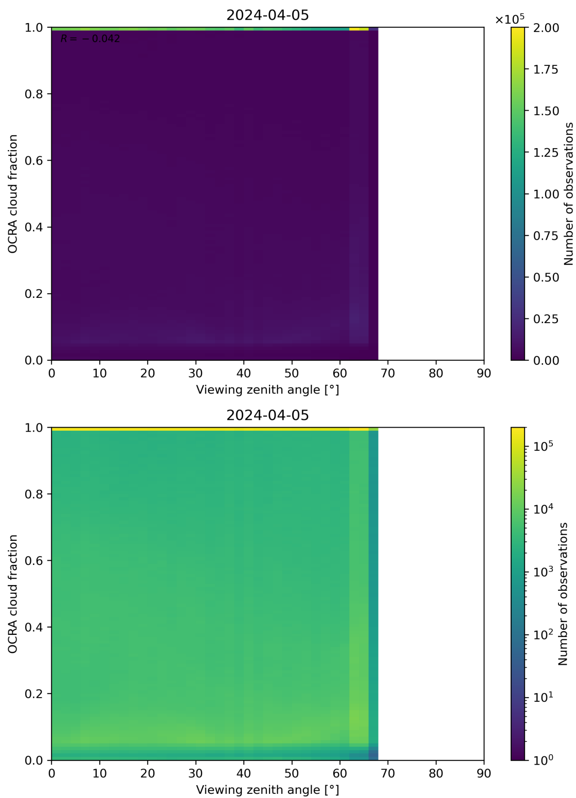
Figure 108: Scatter density plot of “Viewing zenith angle” against “OCRA cloud fraction” for 2024-04-05 to 2024-04-06.
