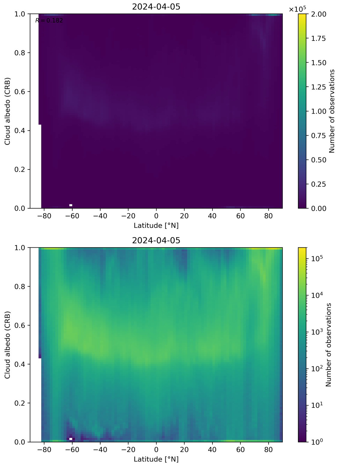
Figure 91: Scatter density plot of “Latitude” against “Cloud albedo (CRB)” for 2024-04-05 to 2024-04-06.
