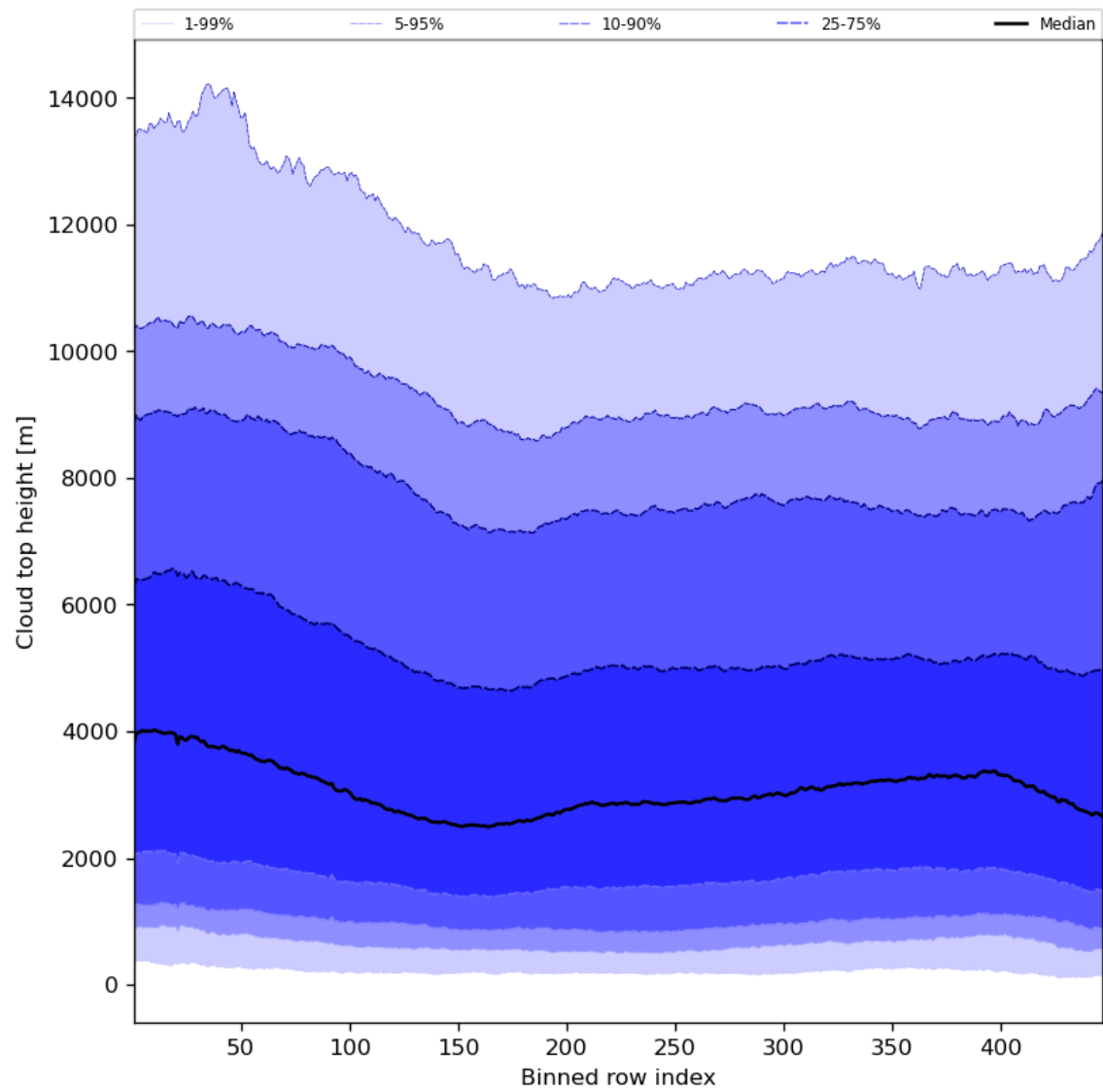
Figure 56: Along track statistics of “Cloud top height” for 2024-04-05 to 2024-04-06
