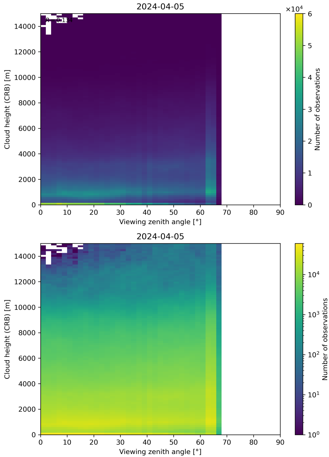
Figure 110: Scatter density plot of “Viewing zenith angle” against “Cloud height (CRB)” for 2024-04-05 to 2024-04-06.
