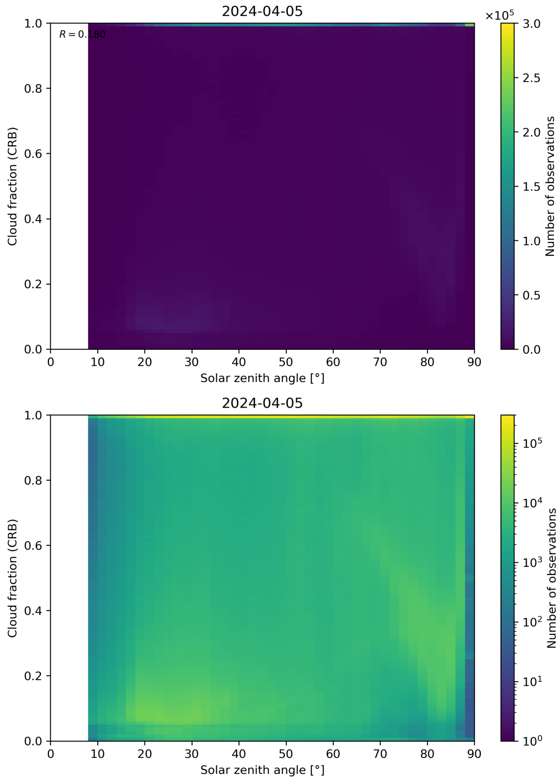
Figure 101: Scatter density plot of “Solar zenith angle” against “Cloud fraction (CRB)” for 2024-04-05 to 2024-04-06.
