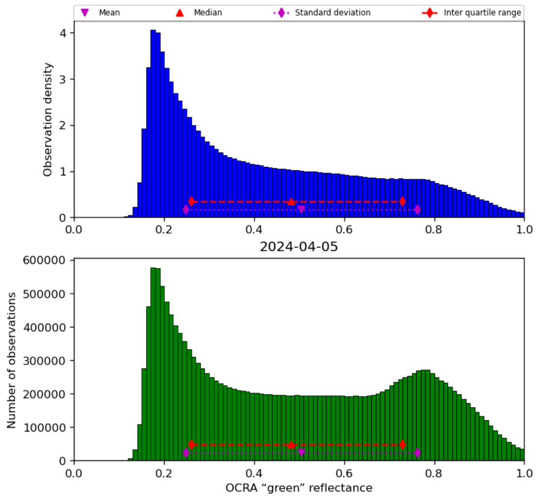
Figure 52: Histogram of “OCRA “green” reflectance” for 2024-04-05 to 2024-04-06
