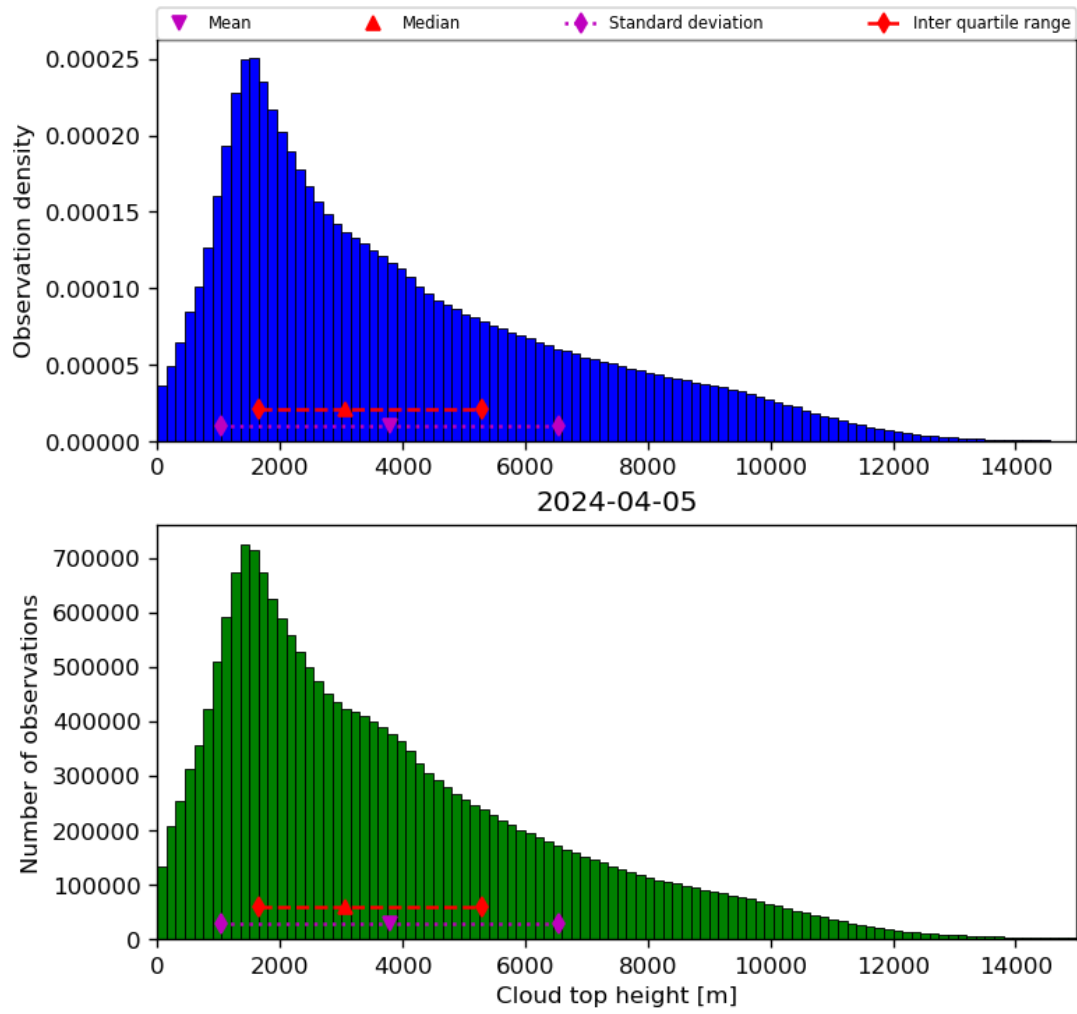
Figure 40: Histogram of “Cloud top height” for 2024-04-05 to 2024-04-06
