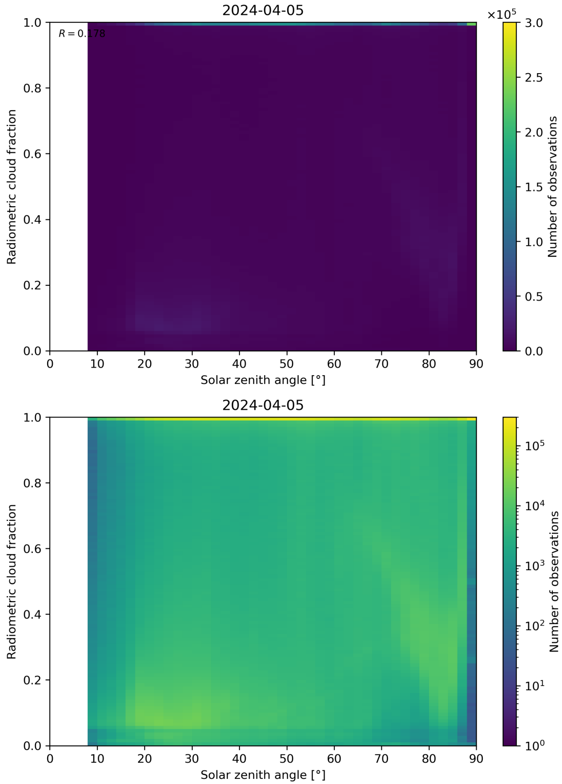
Figure 99: Scatter density plot of “Solar zenith angle” against “Radiometric cloud fraction” for 2024-04-05 to 2024-04-06.
