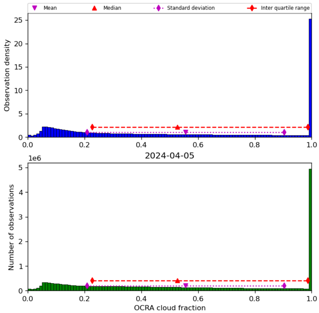
Figure 50: Histogram of “OCRA cloud fraction” for 2024-04-05 to 2024-04-06
