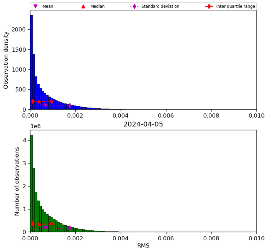
Figure 47: Histogram of “RMS” for 2024-04-05 to 2024-04-06
