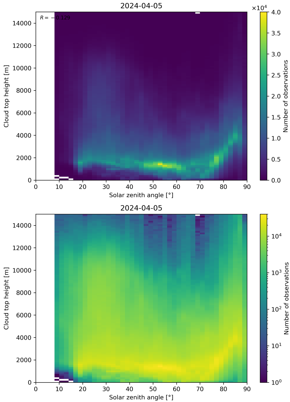
Figure 104: Scatter density plot of “Solar zenith angle” against “Cloud top height” for 2024-04-05 to 2024-04-06.
