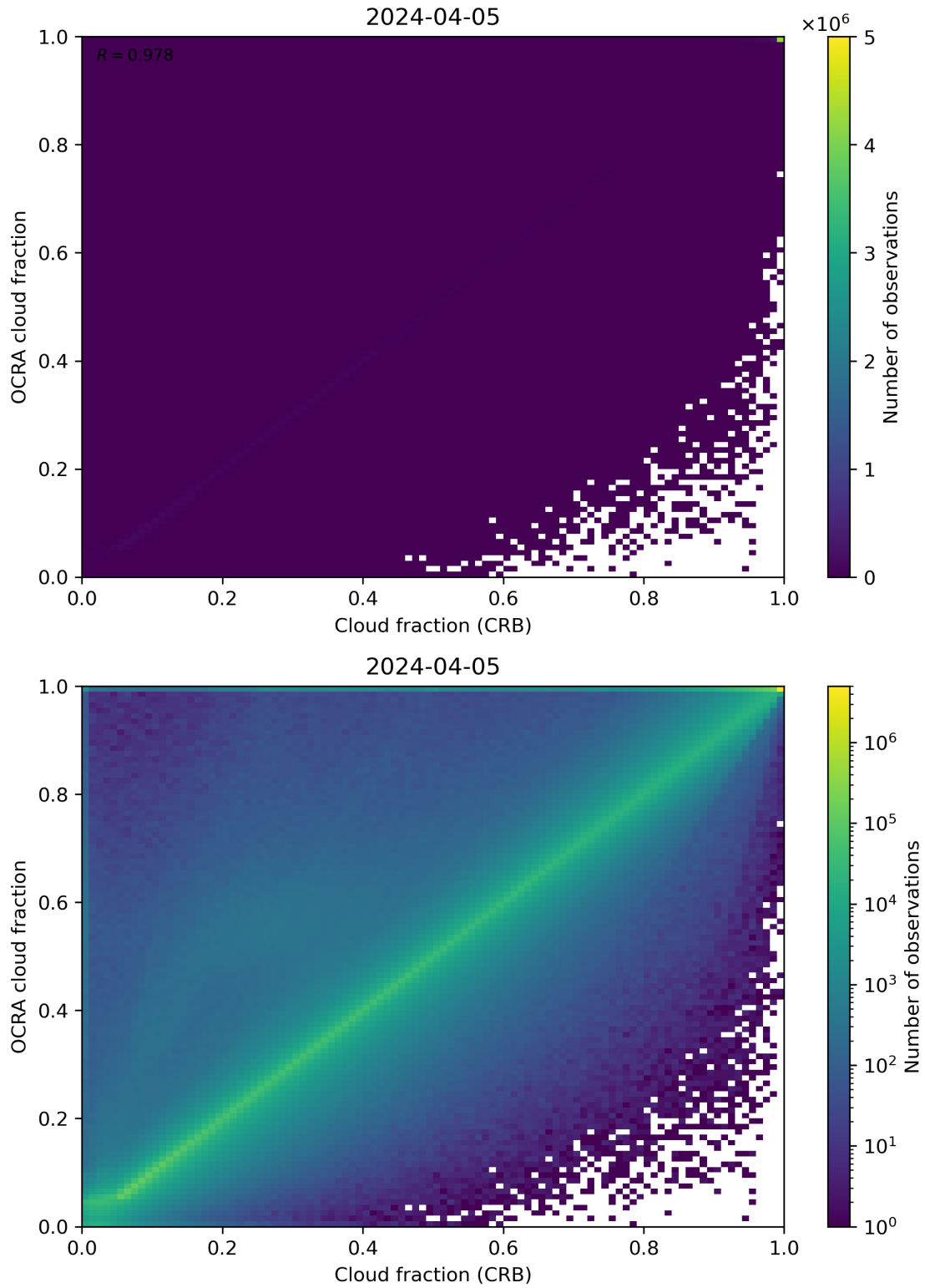
Figure 78: Scatter density plot of “Cloud fraction (CRB)” against “OCRA cloud fraction” for 2024-04-05 to 2024-04-06.
