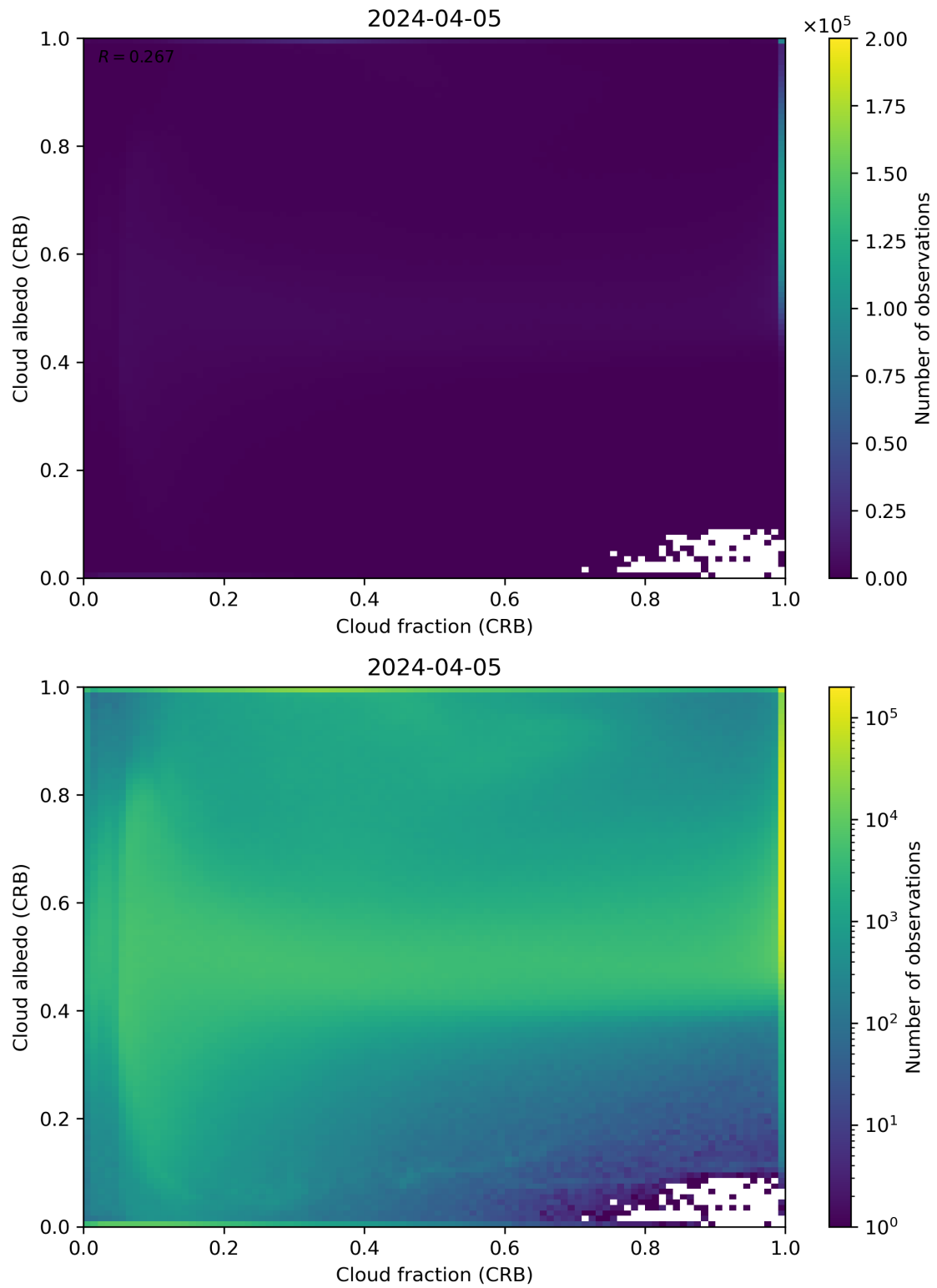
Figure 77: Scatter density plot of “Cloud fraction (CRB)” against “Cloud albedo (CRB)” for 2024-04-05 to 2024-04-06.
