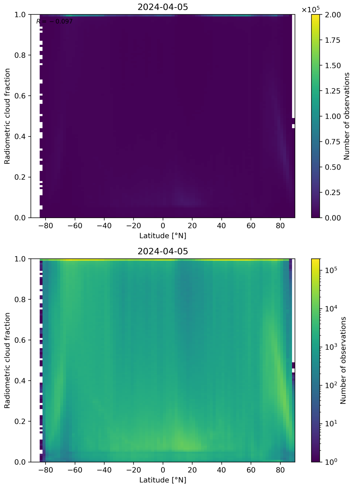
Figure 92: Scatter density plot of “Latitude” against “Radiometric cloud fraction” for 2024-04-05 to 2024-04-06.
