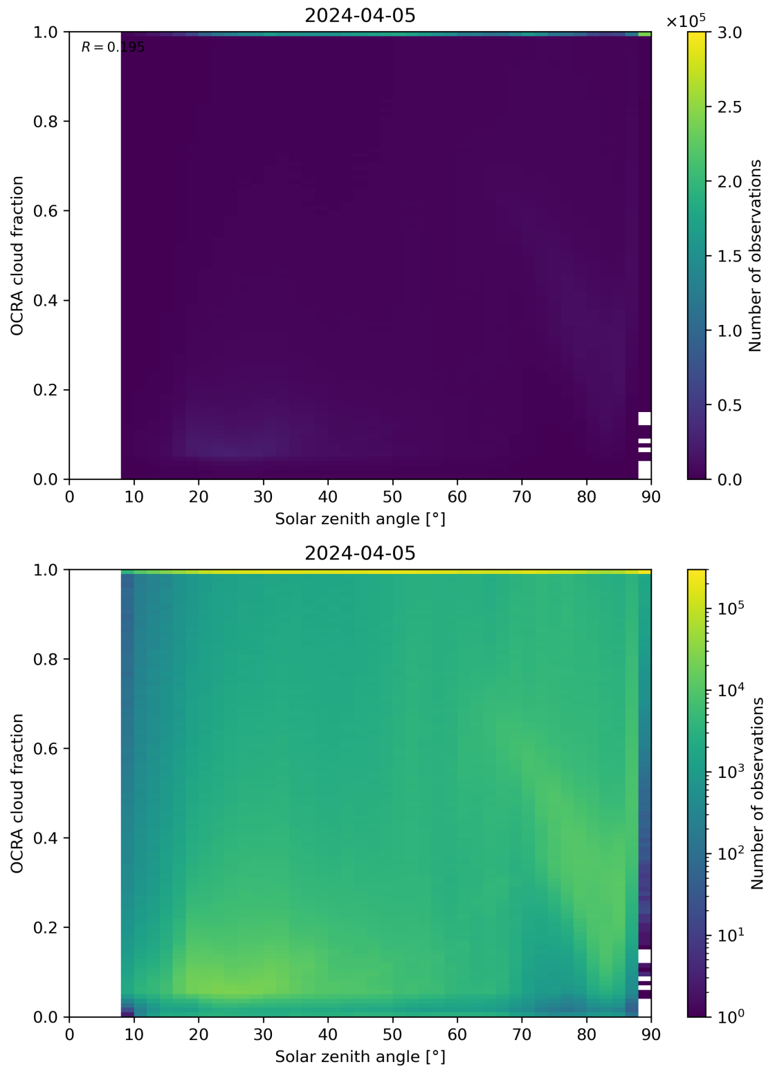
Figure 100: Scatter density plot of “Solar zenith angle” against “OCRA cloud fraction” for 2024-04-05 to 2024-04-06.
