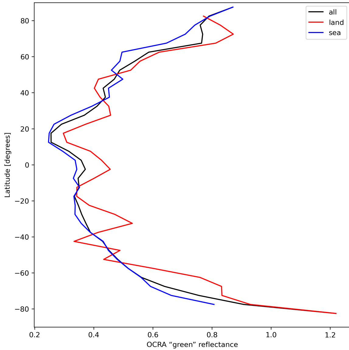
Figure 36: Zonal average of “OCRA “green” reflectance” for 2024-04-05 to 2024-04-06.
