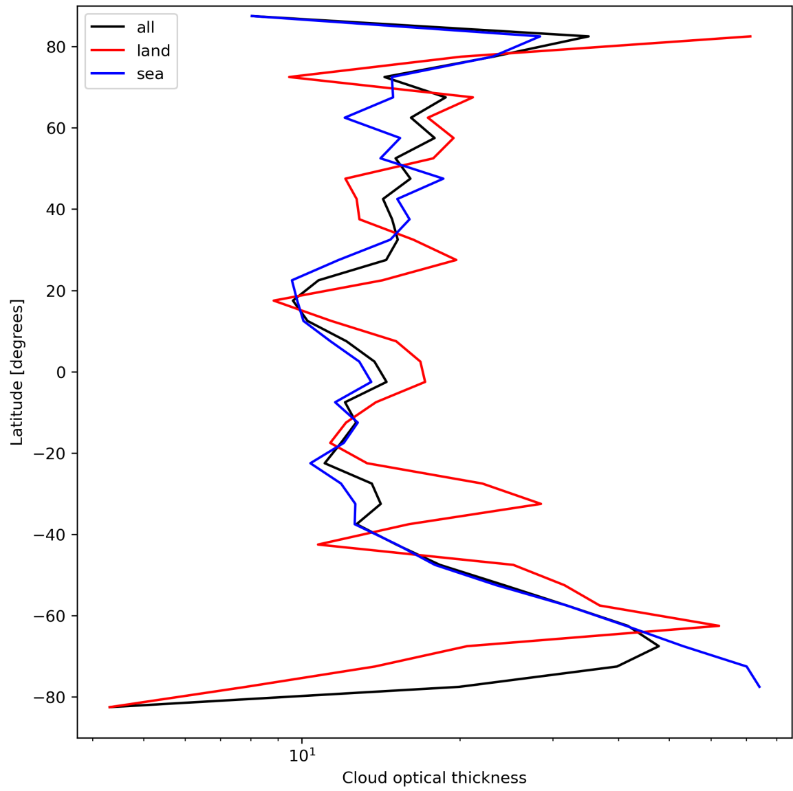
Figure 25: Zonal average of “Cloud optical thickness” for 2024-04-05 to 2024-04-06.
