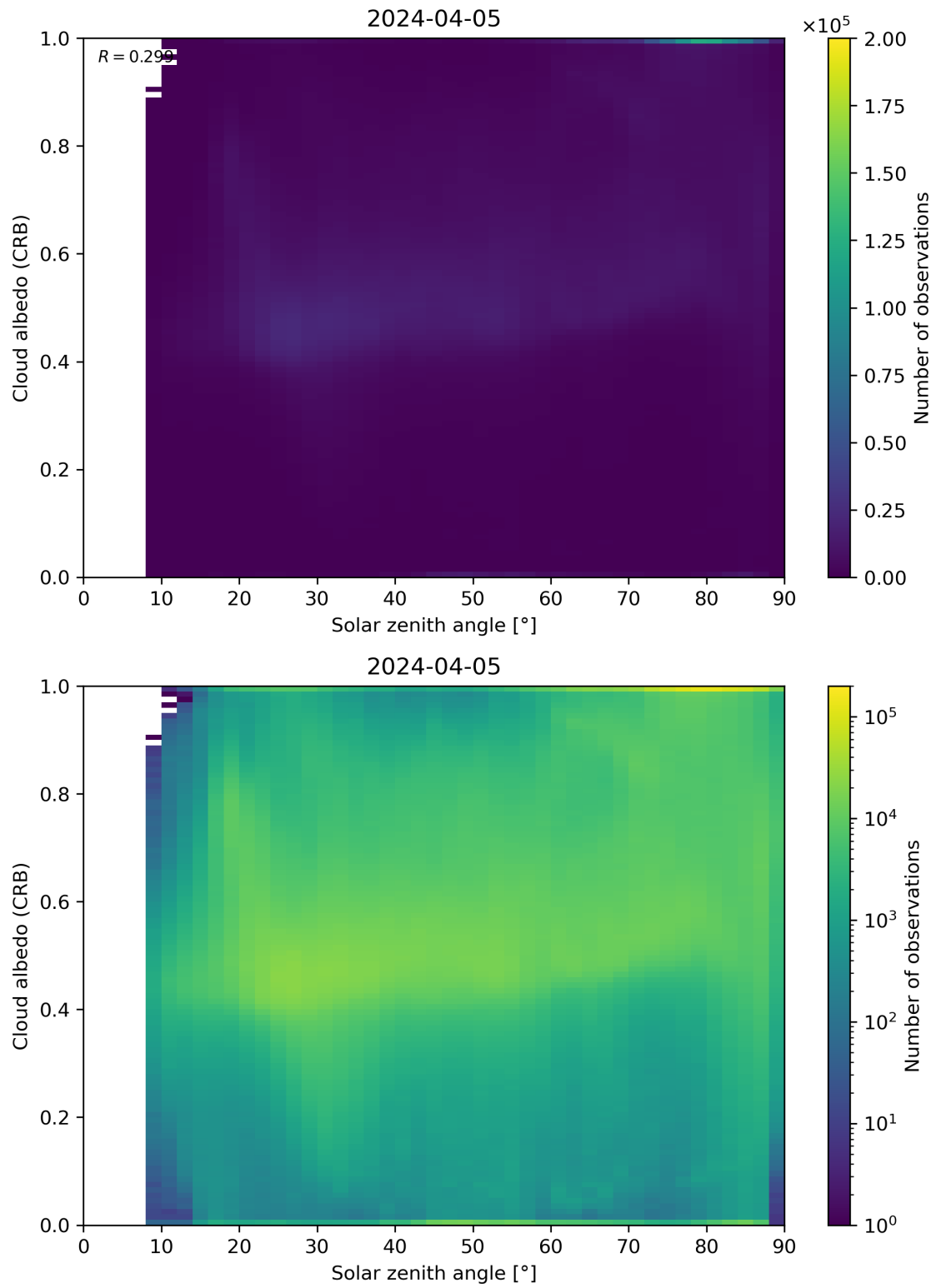
Figure 98: Scatter density plot of “Solar zenith angle” against “Cloud albedo (CRB)” for 2024-04-05 to 2024-04-06.
