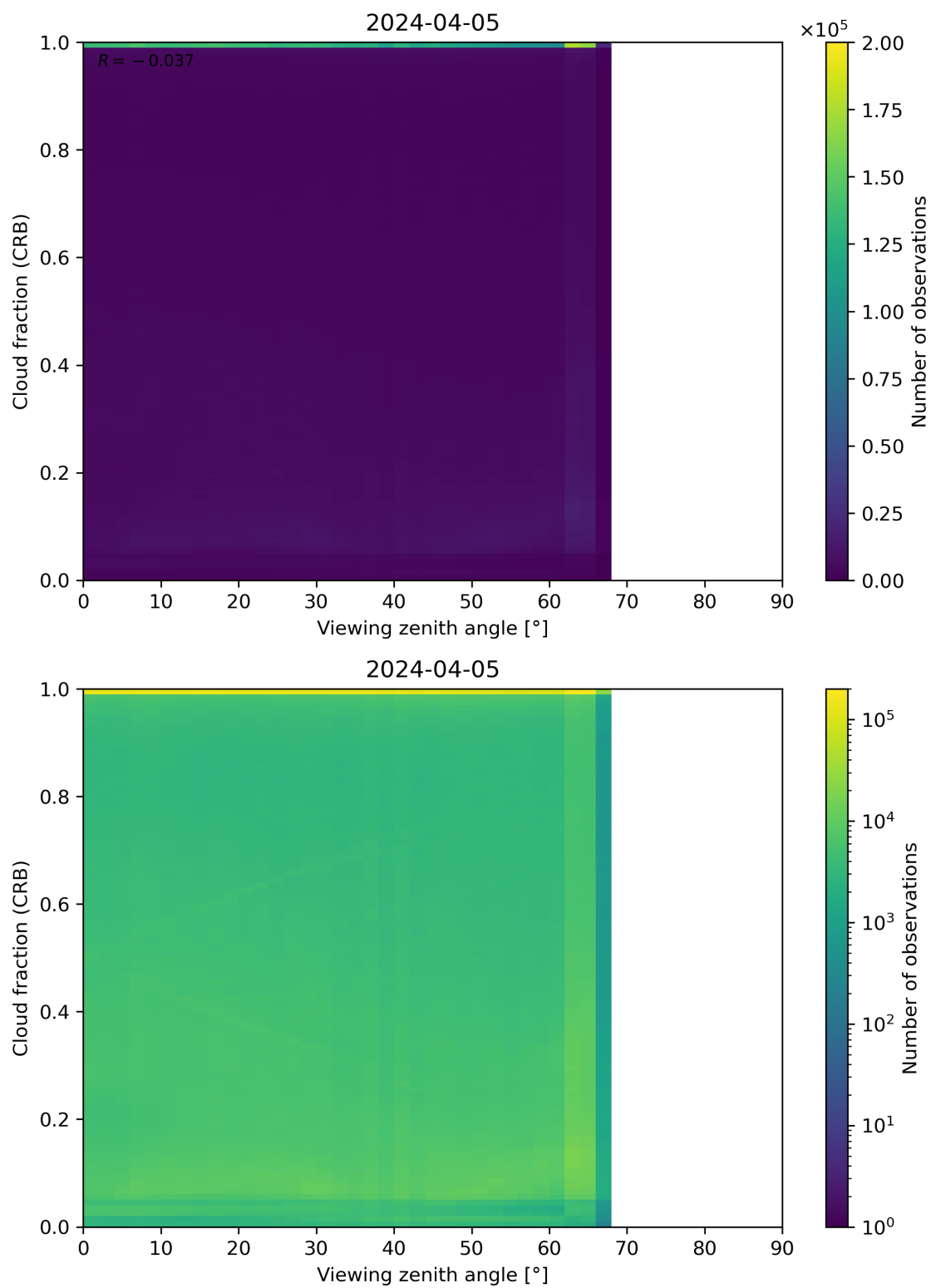
Figure 109: Scatter density plot of “Viewing zenith angle” against “Cloud fraction (CRB)” for 2024-04-05 to 2024-04-06.
