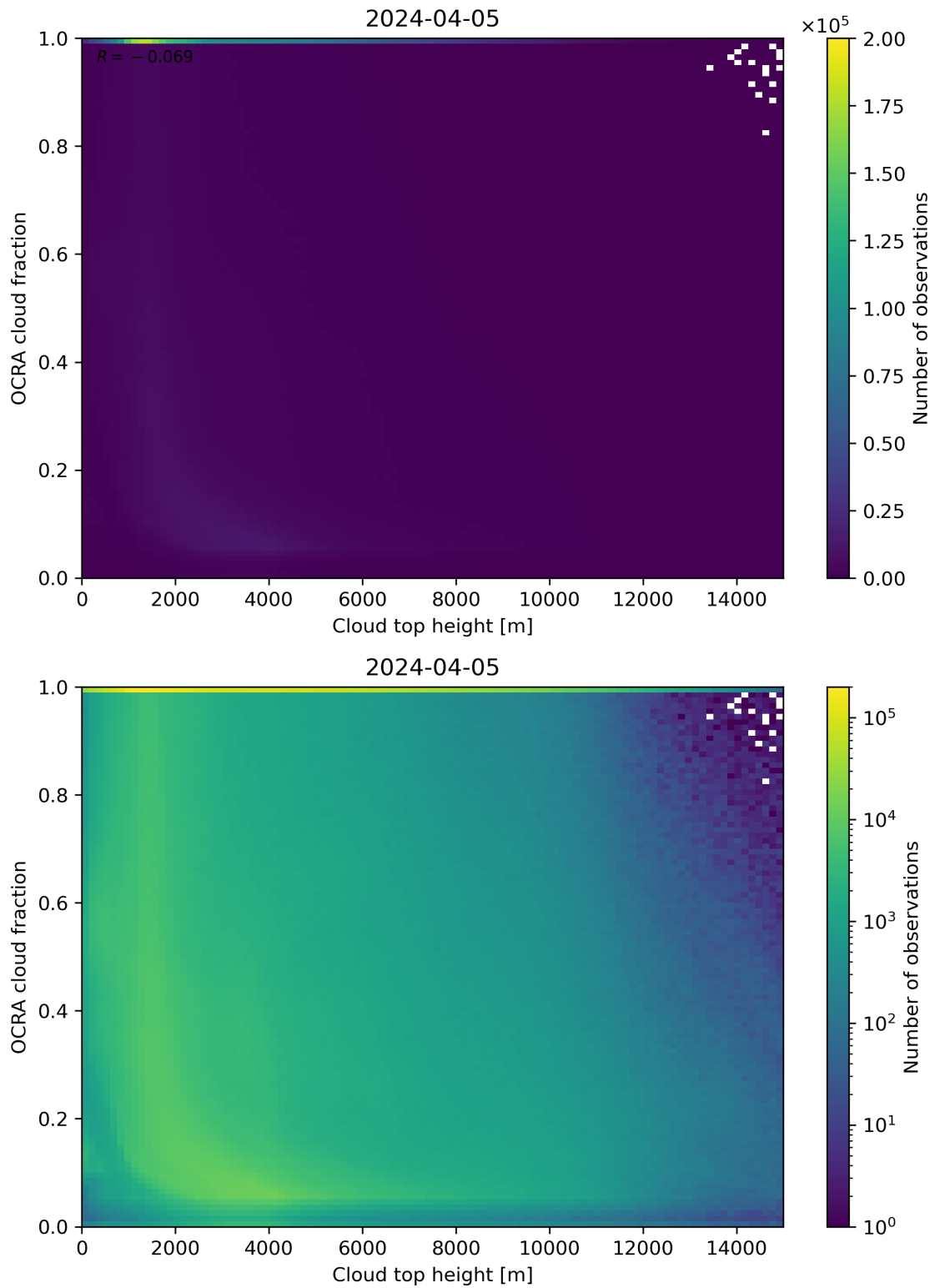
Figure 87: Scatter density plot of “Cloud top height” against “OCRA cloud fraction” for 2024-04-05 to 2024-04-06.
