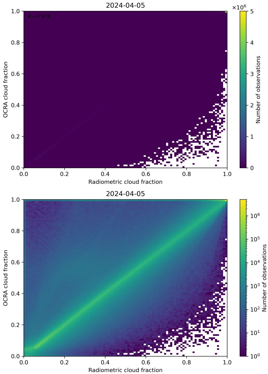
Figure 72: Scatter density plot of “Radiometric cloud fraction” against “OCRA cloud fraction” for 2024-04-05 to 2024-04-06.
