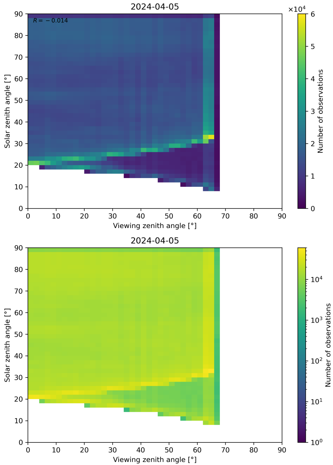
Figure 114: Scatter density plot of “Viewing zenith angle” against “Solar zenith angle” for 2024-04-05 to 2024-04-06.
