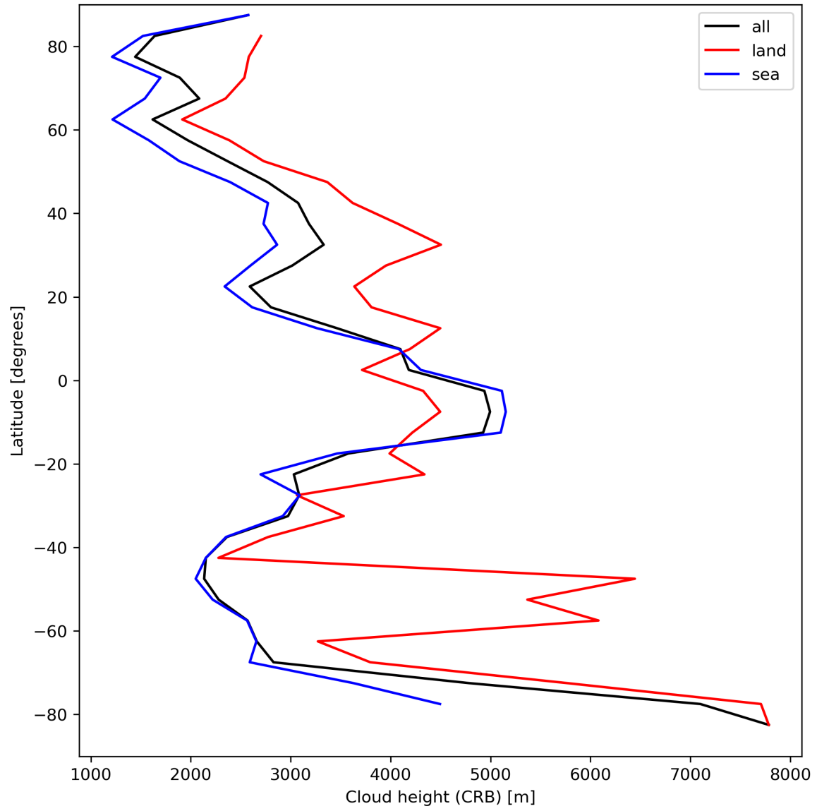
Figure 27: Zonal average of “Cloud height (CRB)” for 2024-04-05 to 2024-04-06.
