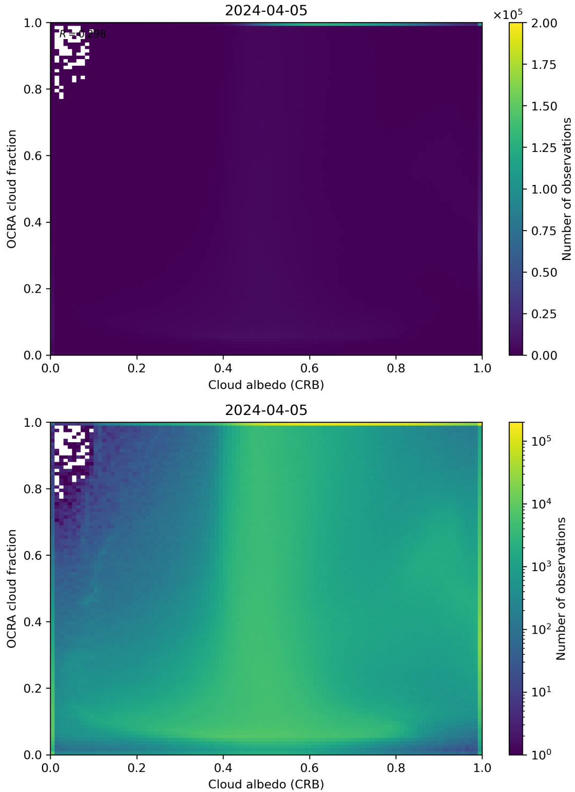
Figure 70: Scatter density plot of “Cloud albedo (CRB)” against “OCRA cloud fraction” for 2024-04-05 to 2024-04-06.
