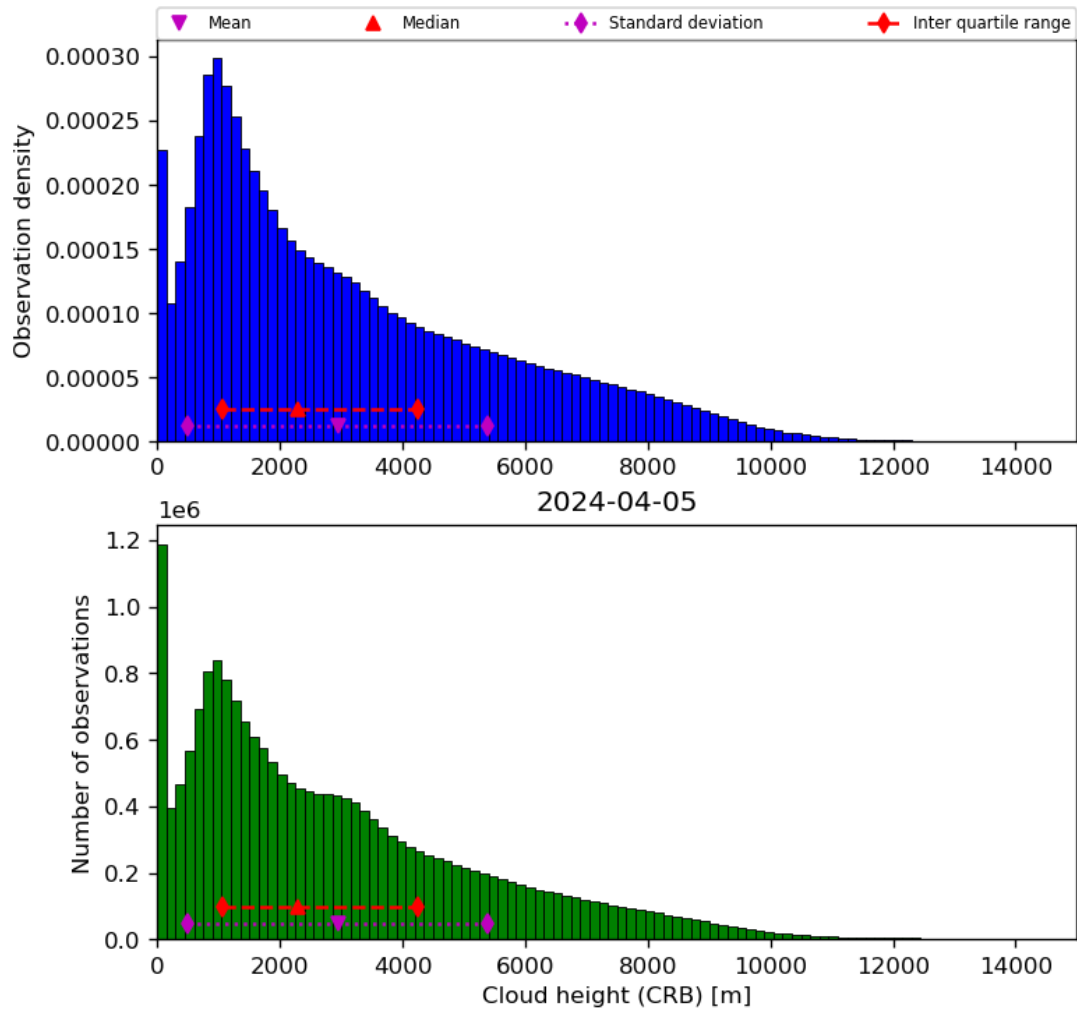
Figure 43: Histogram of “Cloud height (CRB)” for 2024-04-05 to 2024-04-06
