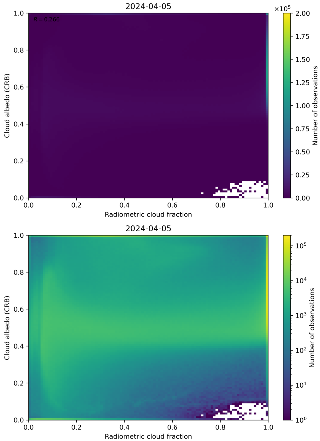
Figure 71: Scatter density plot of “Radiometric cloud fraction” against “Cloud albedo (CRB)” for 2024-04-05 to 2024-04-06.
