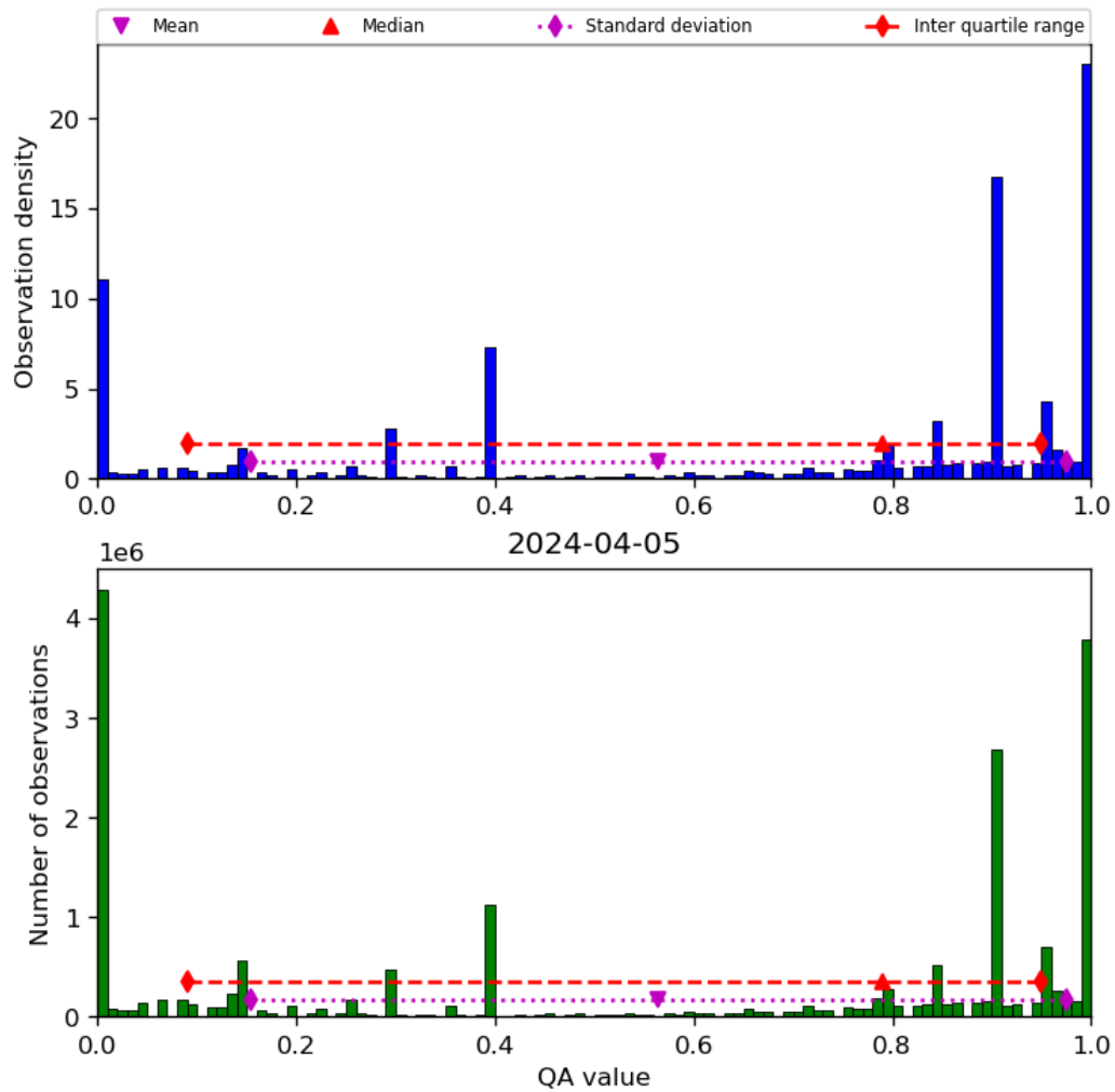
Figure 38: Histogram of “QA value” for 2024-04-05 to 2024-04-06
