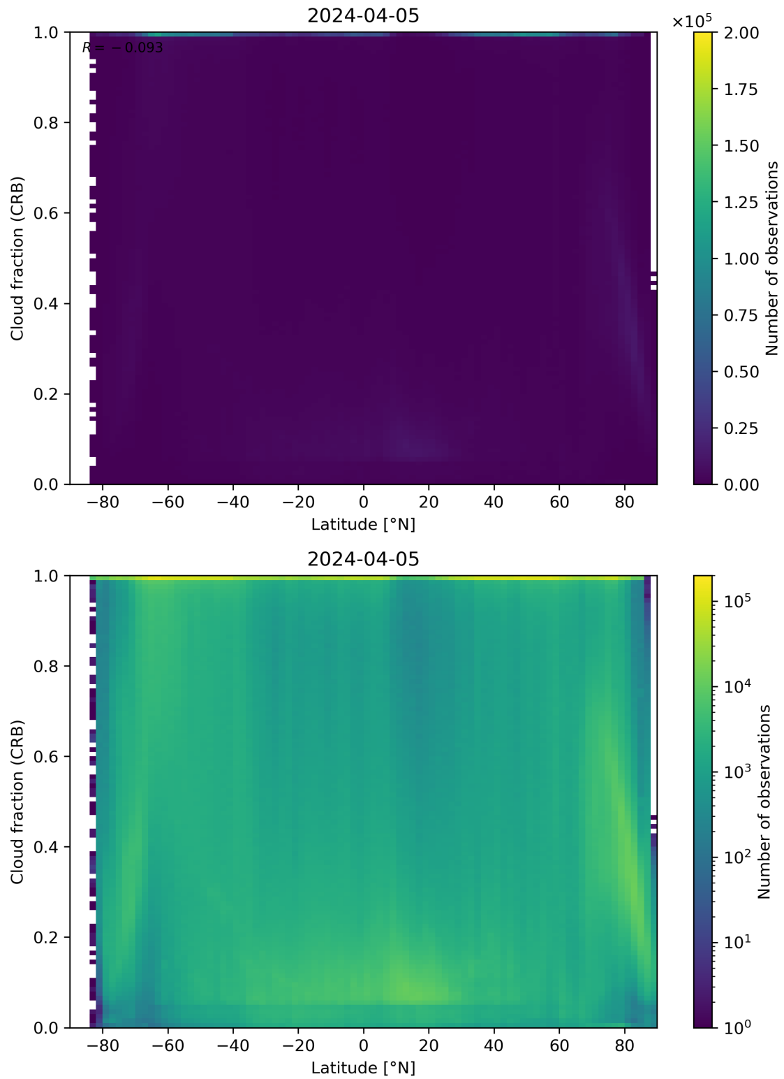
Figure 94: Scatter density plot of “Latitude” against “Cloud fraction (CRB)” for 2024-04-05 to 2024-04-06.
