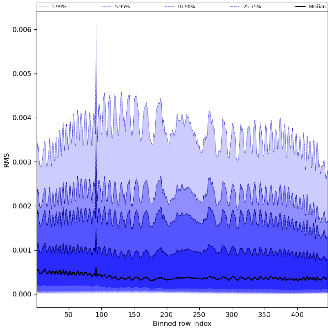
Figure 63: Along track statistics of “RMS” for 2024-04-05 to 2024-04-06
