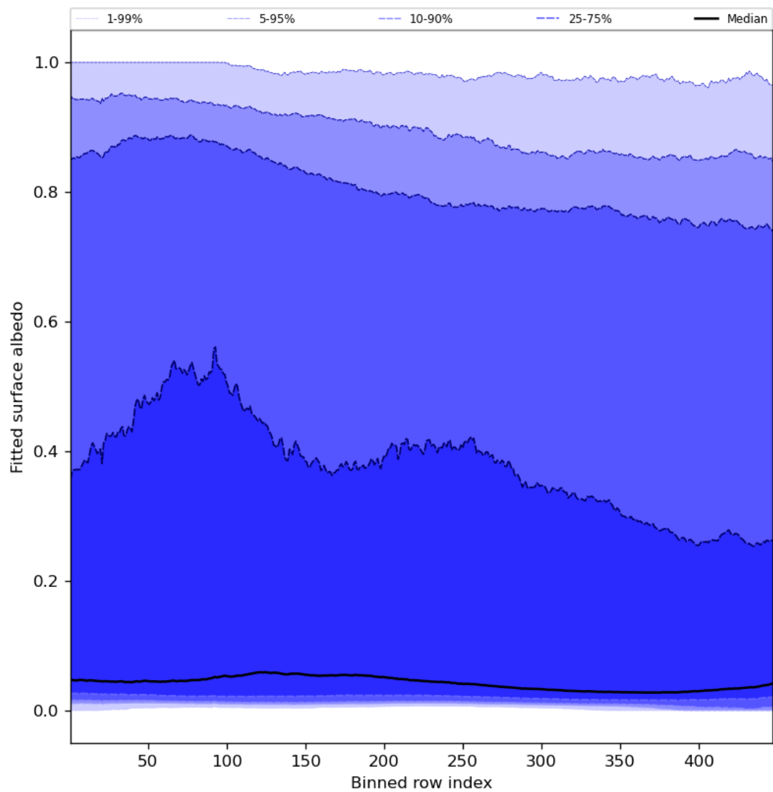
Figure 61: Along track statistics of “Fitted surface albedo” for 2024-04-05 to 2024-04-06
