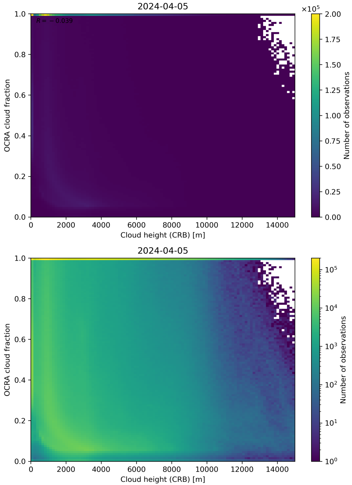
Figure 81: Scatter density plot of “Cloud height (CRB)” against “OCRA cloud fraction” for 2024-04-05 to 2024-04-06.
