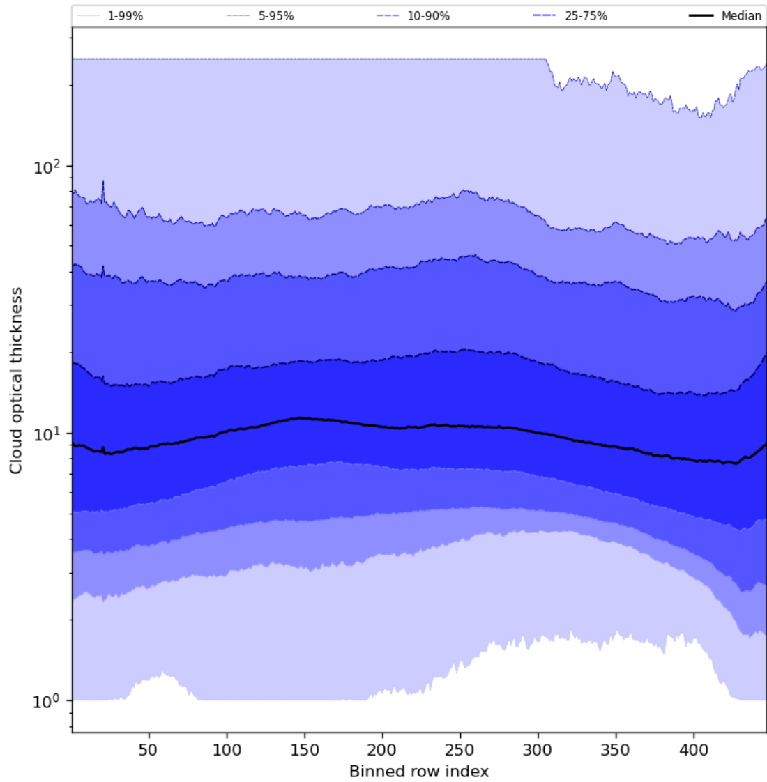
Figure 57: Along track statistics of “Cloud optical thickness” for 2024-04-05 to 2024-04-06
