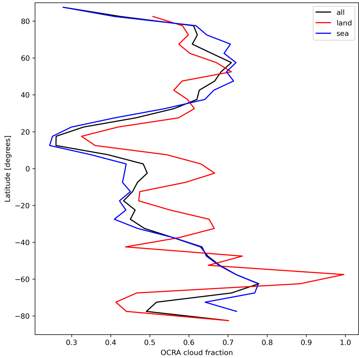
Figure 34: Zonal average of “OCRA cloud fraction” for 2024-04-05 to 2024-04-06.
