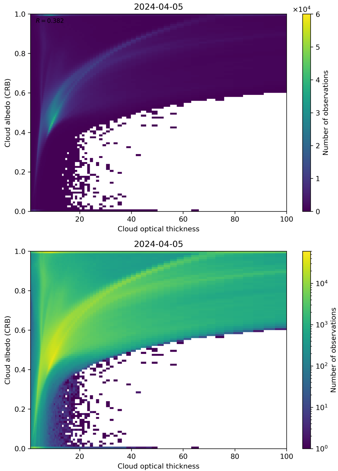
Figure 82: Scatter density plot of “Cloud optical thickness” against “Cloud albedo (CRB)” for 2024-04-05 to 2024-04-06.
