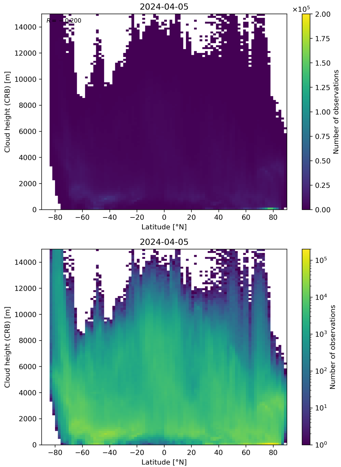
Figure 95: Scatter density plot of “Latitude” against “Cloud height (CRB)” for 2024-04-05 to 2024-04-06.
