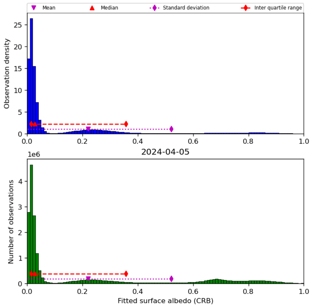
Figure 46: Histogram of “Fitted surface albedo (CRB)” for 2024-04-05 to 2024-04-06
