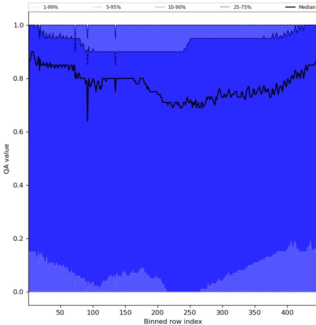
Figure 54: Along track statistics of “QA value” for 2024-04-05 to 2024-04-06
