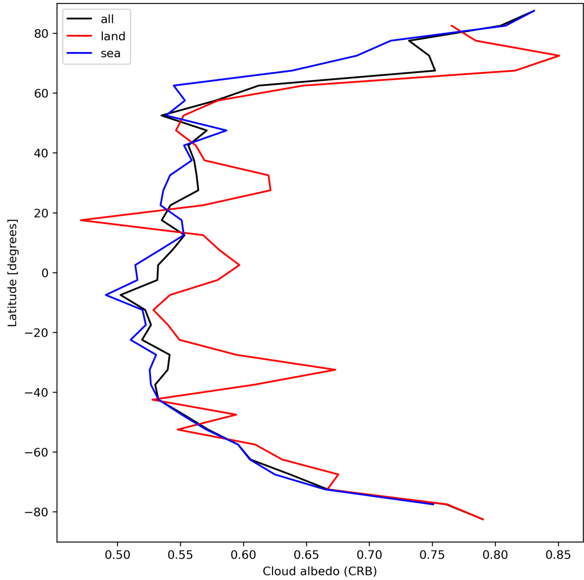
Figure 28: Zonal average of “Cloud albedo (CRB)” for 2024-04-05 to 2024-04-06.
