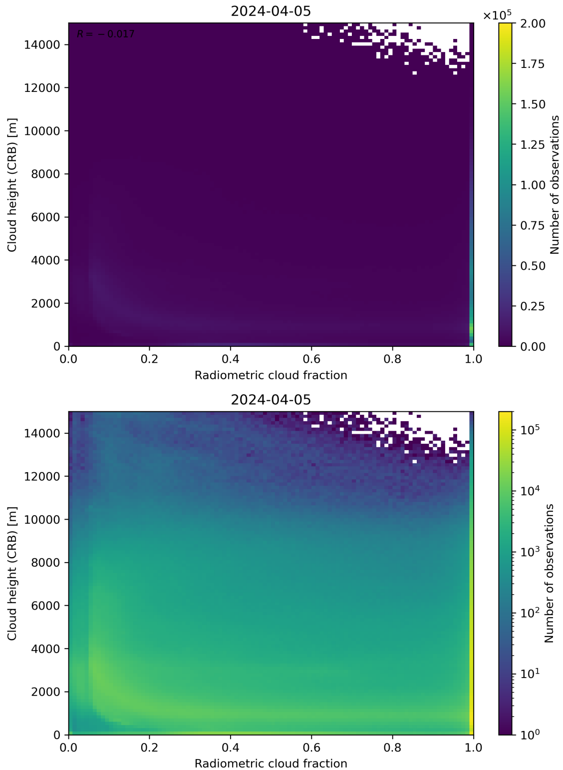
Figure 74: Scatter density plot of “Radiometric cloud fraction” against “Cloud height (CRB)” for 2024-04-05 to 2024-04-06.
