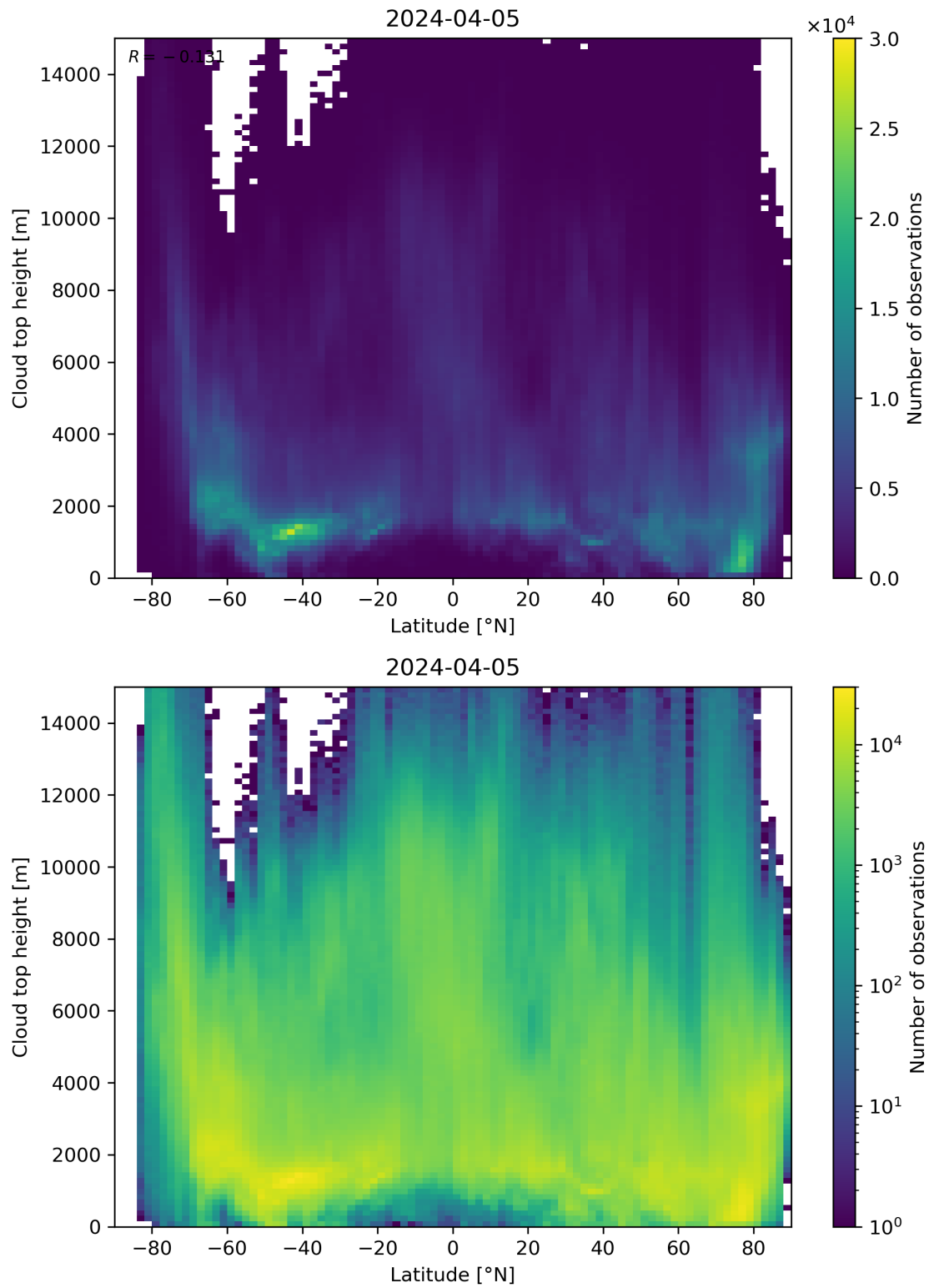
Figure 97: Scatter density plot of “Latitude” against “Cloud top height” for 2024-04-05 to 2024-04-06.
