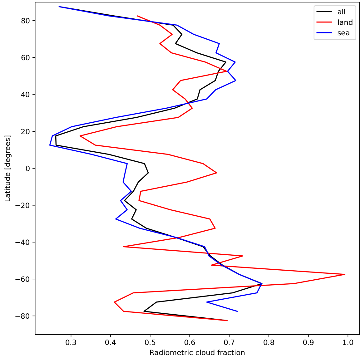
Figure 23: Zonal average of “Radiometric cloud fraction” for 2024-04-05 to 2024-04-06.
