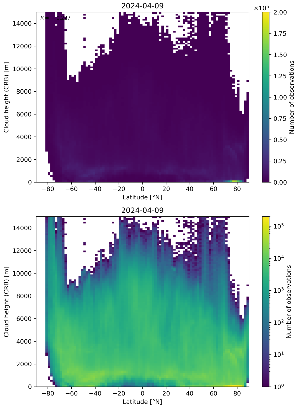
Figure 95: Scatter density plot of “Latitude” against “Cloud height (CRB)” for 2024-04-08 to 2024-04-10.
