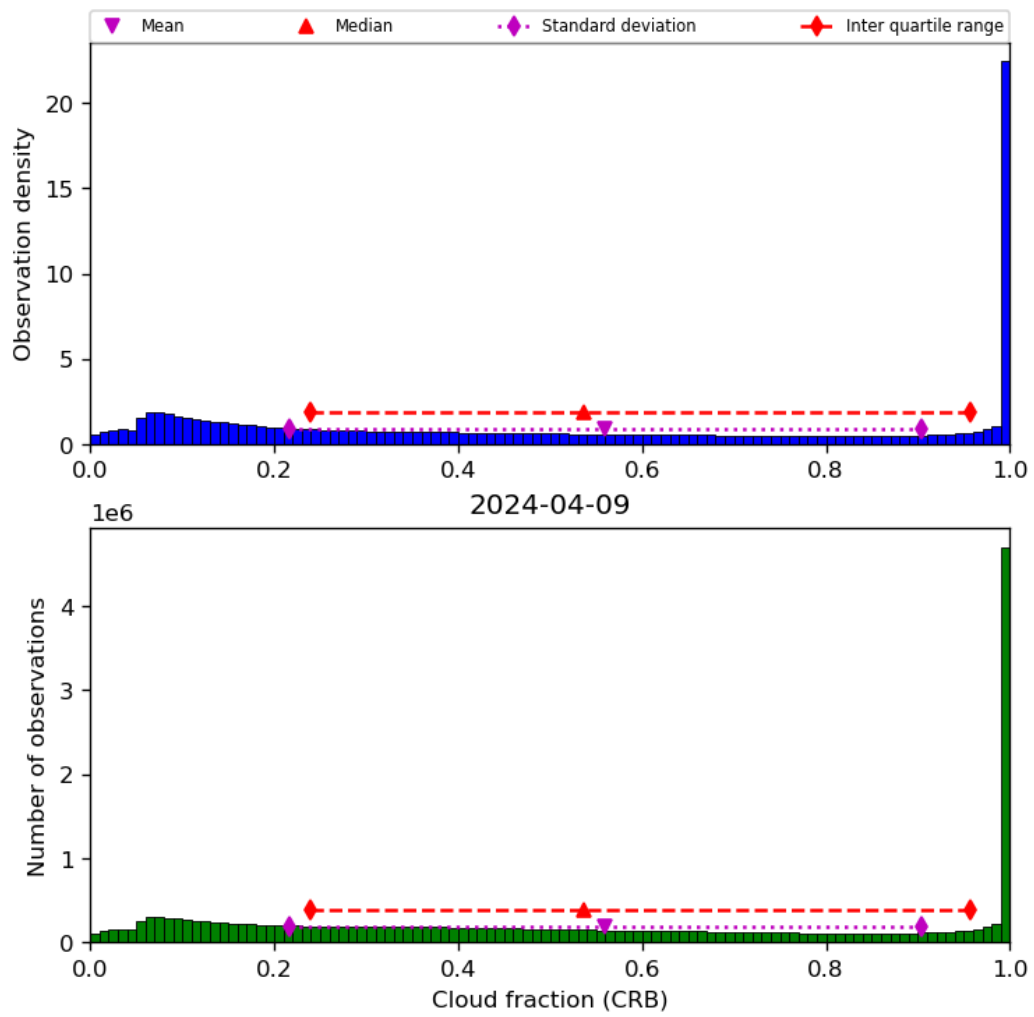
Figure 42: Histogram of “Cloud fraction (CRB)” for 2024-04-08 to 2024-04-10
