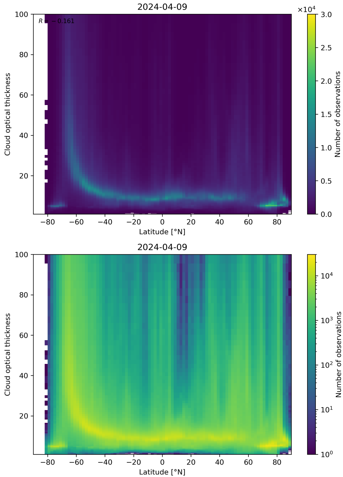
Figure 96: Scatter density plot of “Latitude” against “Cloud optical thickness” for 2024-04-08 to 2024-04-10.
