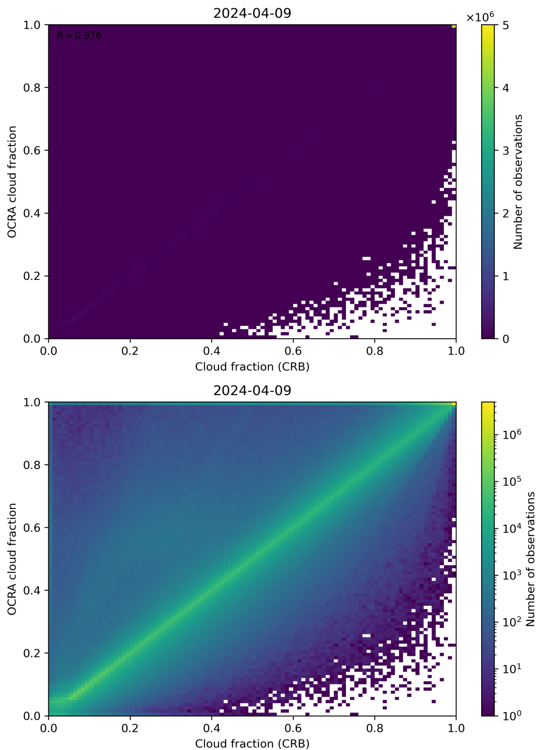
Figure 78: Scatter density plot of “Cloud fraction (CRB)” against “OCRA cloud fraction” for 2024-04-08 to 2024-04-10.
