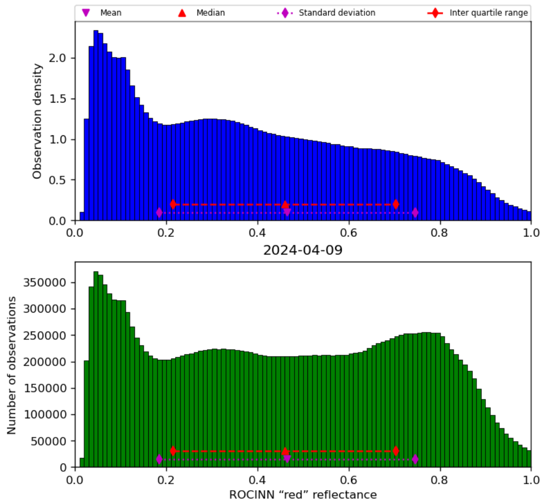
Figure 53: Histogram of “ROCINN “red” reflectance” for 2024-04-08 to 2024-04-10
