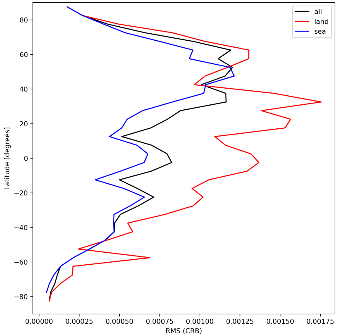
Figure 32: Zonal average of “RMS (CRB)” for 2024-04-08 to 2024-04-10.
