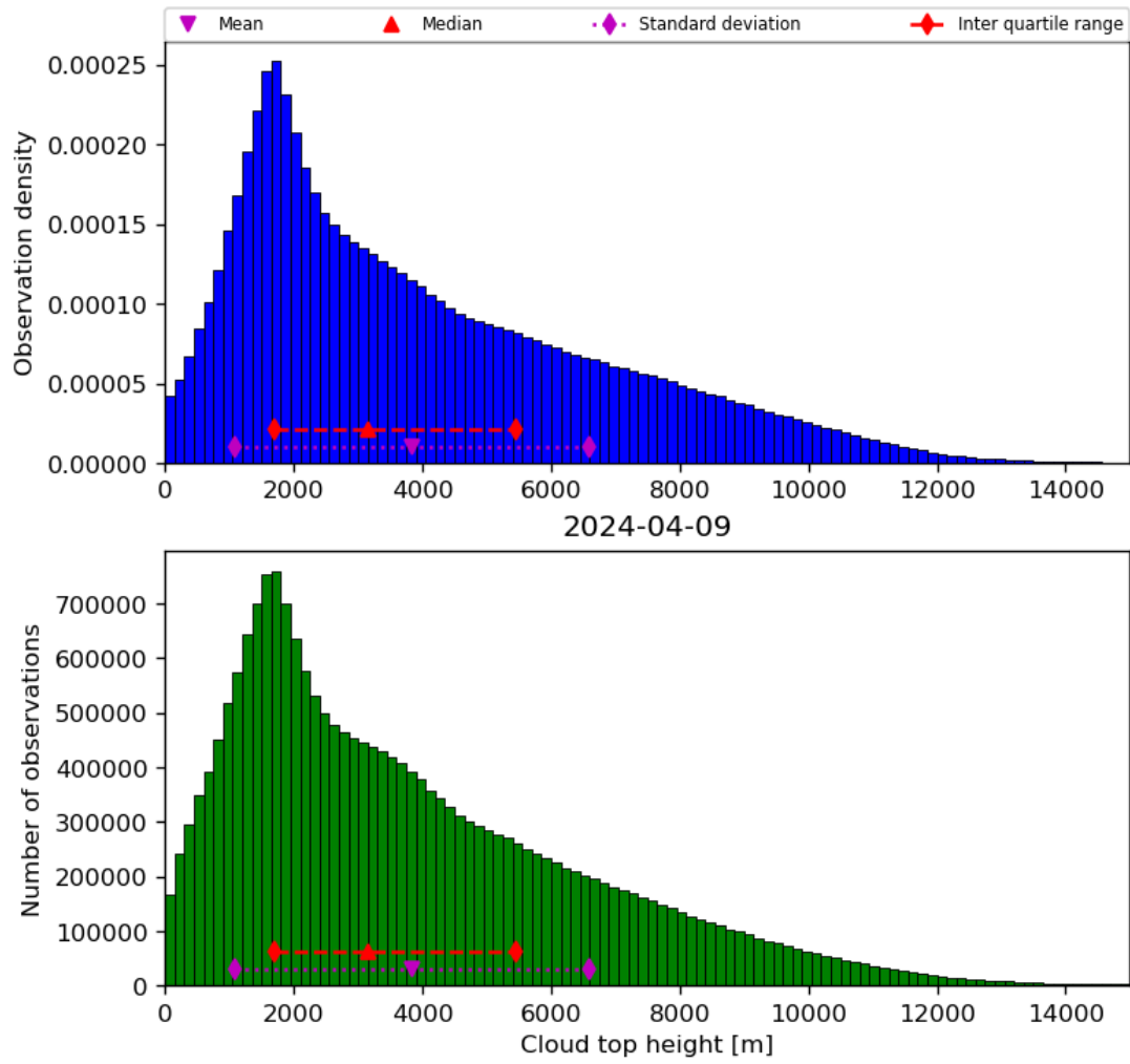
Figure 40: Histogram of “Cloud top height” for 2024-04-08 to 2024-04-10
