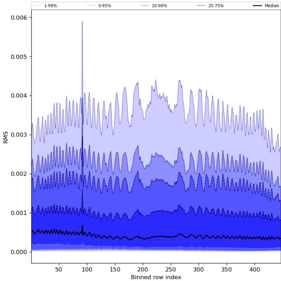
Figure 63: Along track statistics of “RMS” for 2024-04-08 to 2024-04-10
