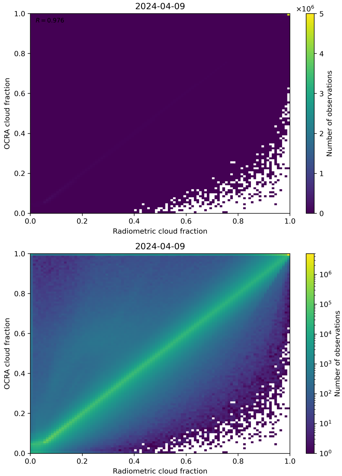
Figure 72: Scatter density plot of “Radiometric cloud fraction” against “OCRA cloud fraction” for 2024-04-08 to 2024-04-10.
