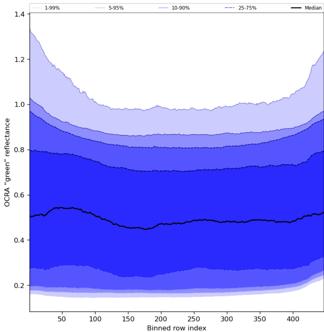
Figure 68: Along track statistics of “OCRA “green” reflectance” for 2024-04-08 to 2024-04-10
