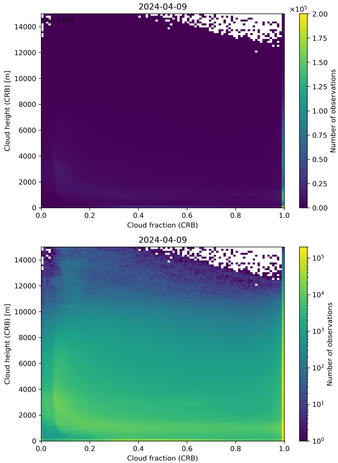
Figure 79: Scatter density plot of “Cloud fraction (CRB)” against “Cloud height (CRB)” for 2024-04-08 to 2024-04-10.
