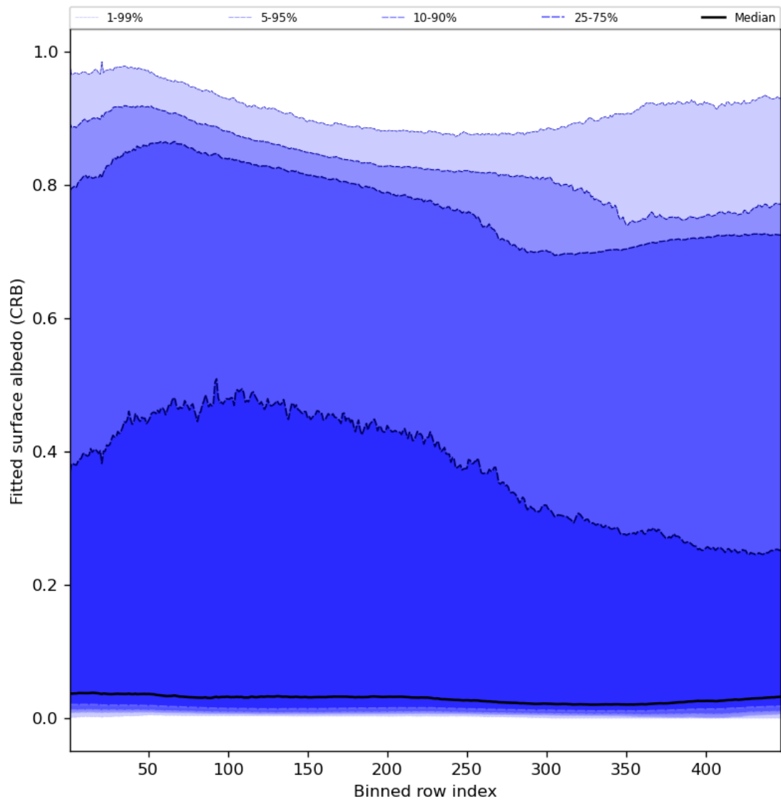
Figure 62: Along track statistics of “Fitted surface albedo (CRB)” for 2024-04-08 to 2024-04-10
