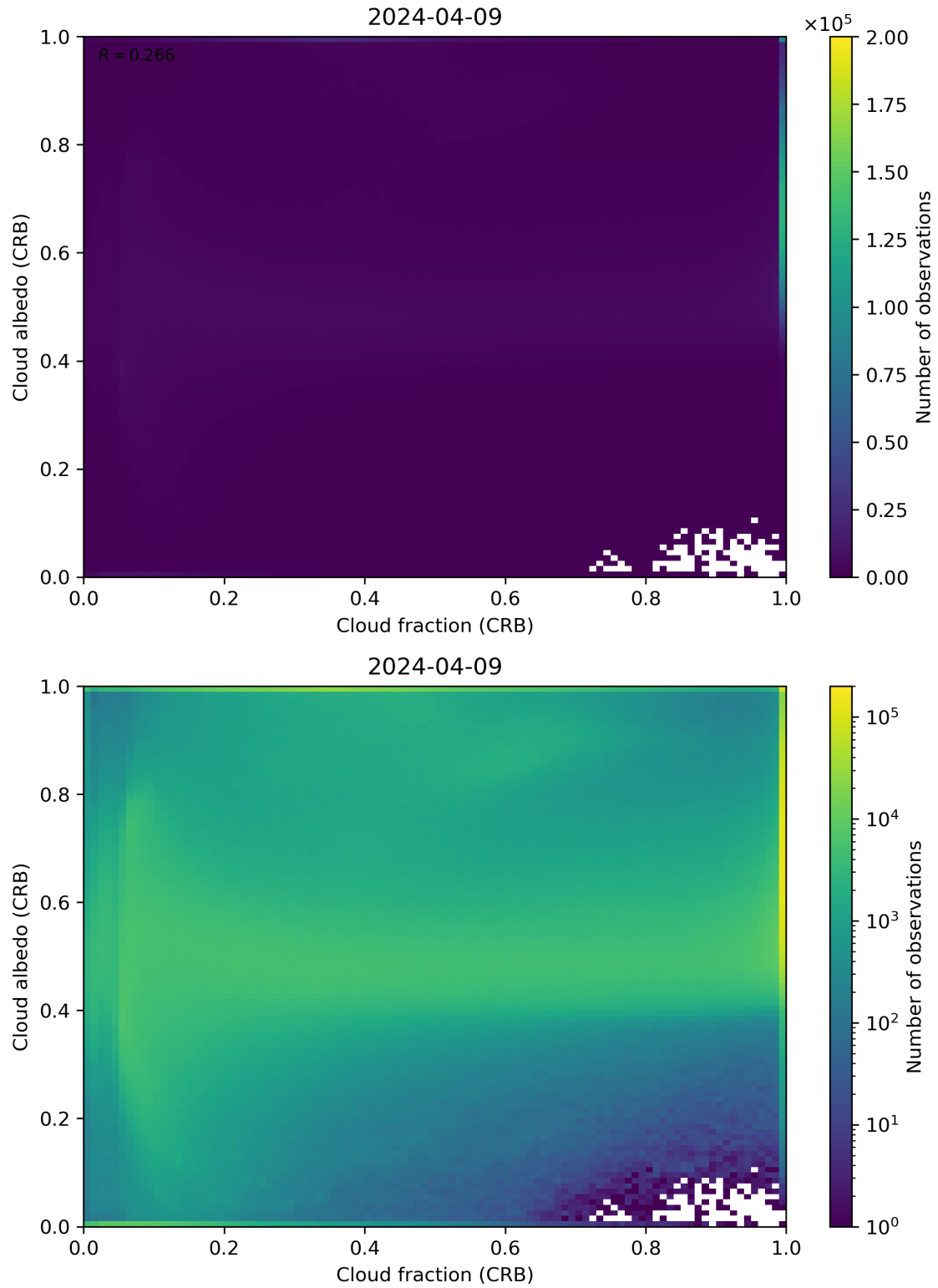
Figure 77: Scatter density plot of “Cloud fraction (CRB)” against “Cloud albedo (CRB)” for 2024-04-08 to 2024-04-10.
