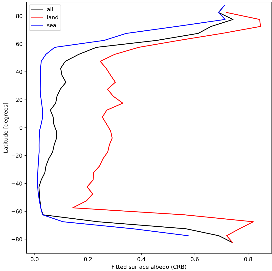
Figure 30: Zonal average of “Fitted surface albedo (CRB)” for 2024-04-08 to 2024-04-10.
