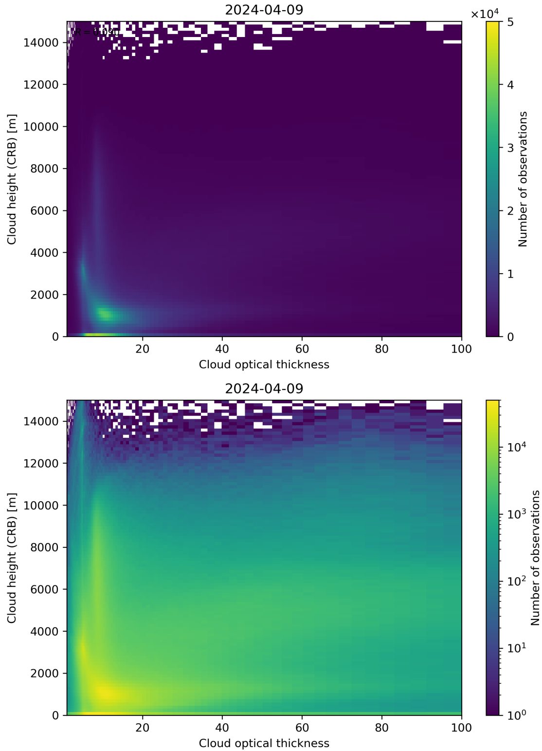
Figure 85: Scatter density plot of “Cloud optical thickness” against “Cloud height (CRB)” for 2024-04-08 to 2024-04-10.
