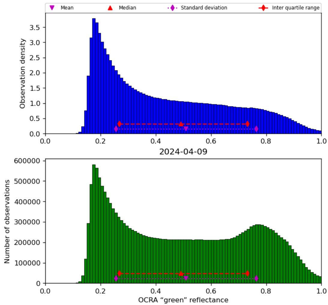
Figure 52: Histogram of “OCRA “green” reflectance” for 2024-04-08 to 2024-04-10
