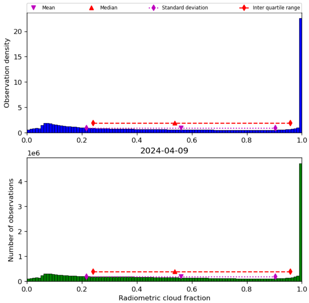
Figure 39: Histogram of “Radiometric cloud fraction” for 2024-04-08 to 2024-04-10
