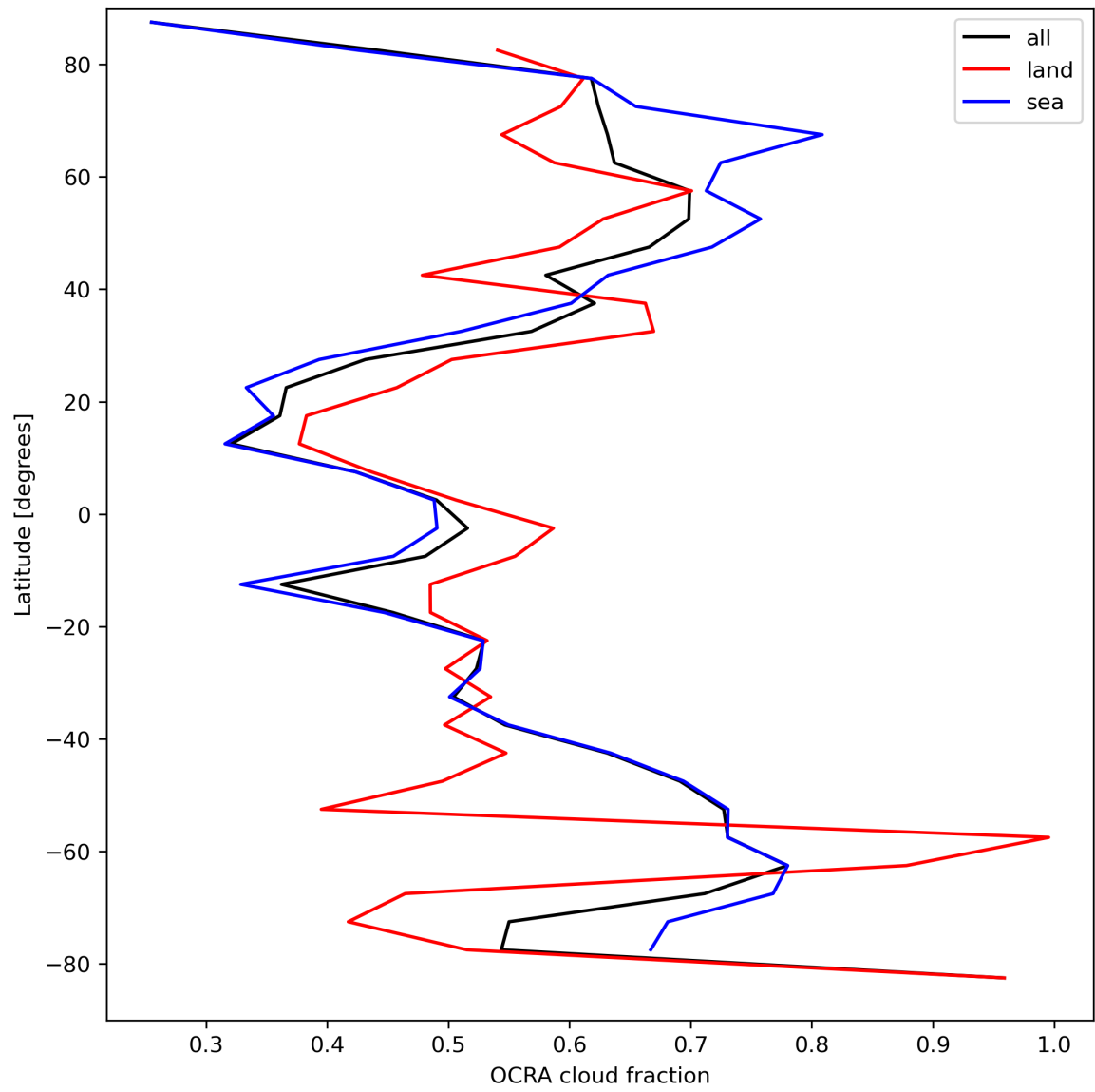
Figure 34: Zonal average of “OCRA cloud fraction” for 2024-04-08 to 2024-04-10.
