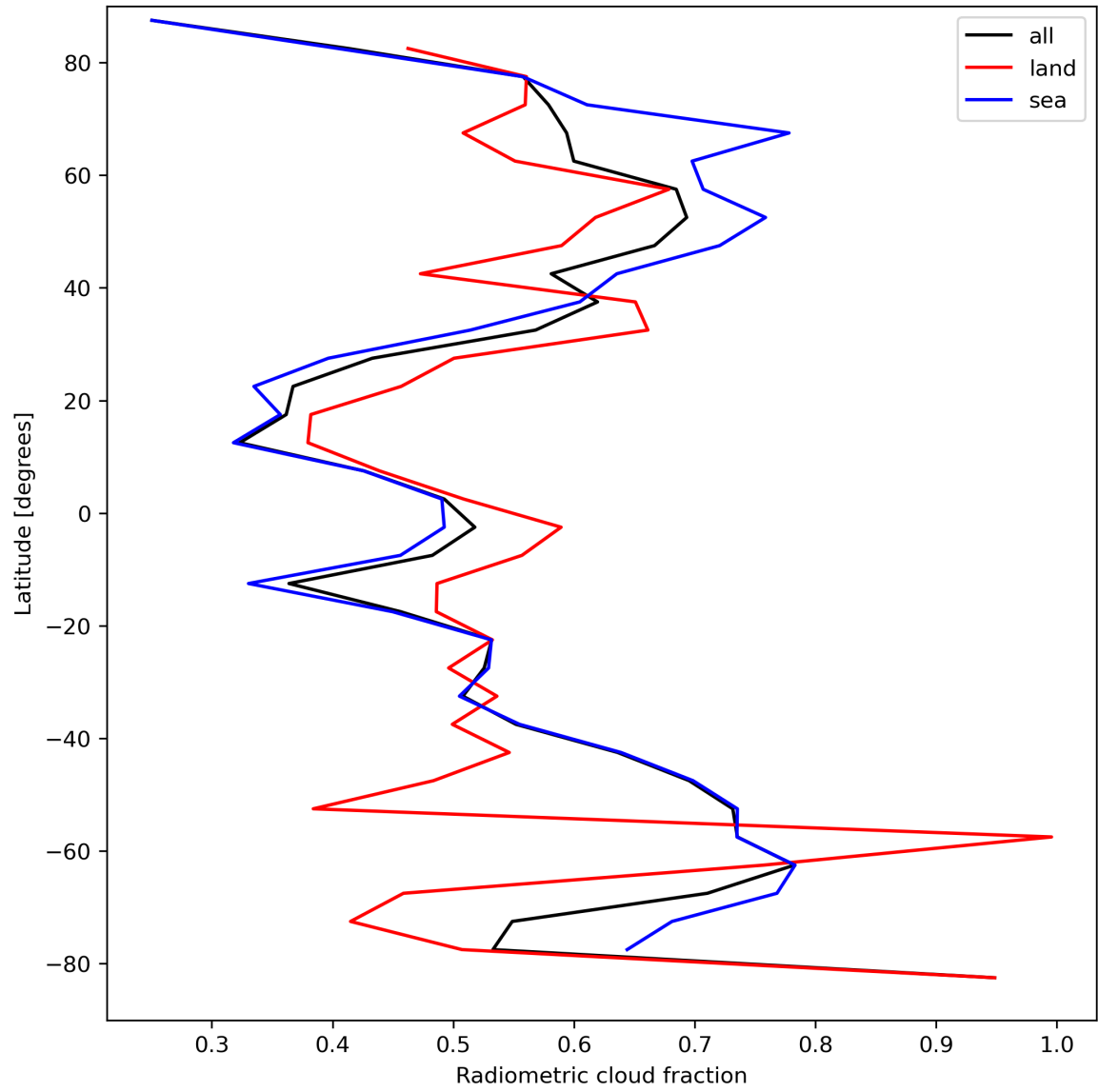
Figure 23: Zonal average of “Radiometric cloud fraction” for 2024-04-08 to 2024-04-10.
