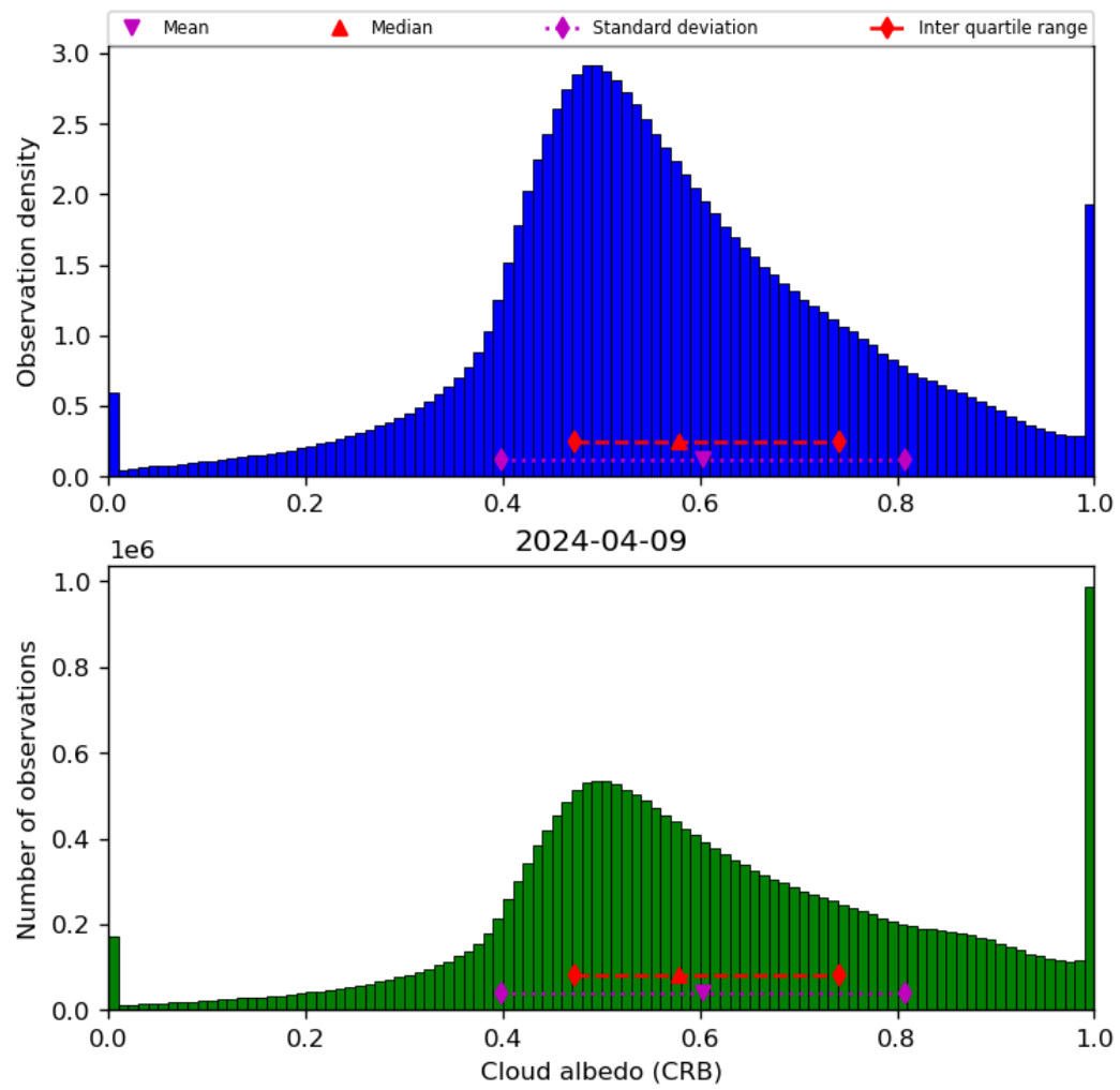
Figure 44: Histogram of “Cloud albedo (CRB)” for 2024-04-08 to 2024-04-10
