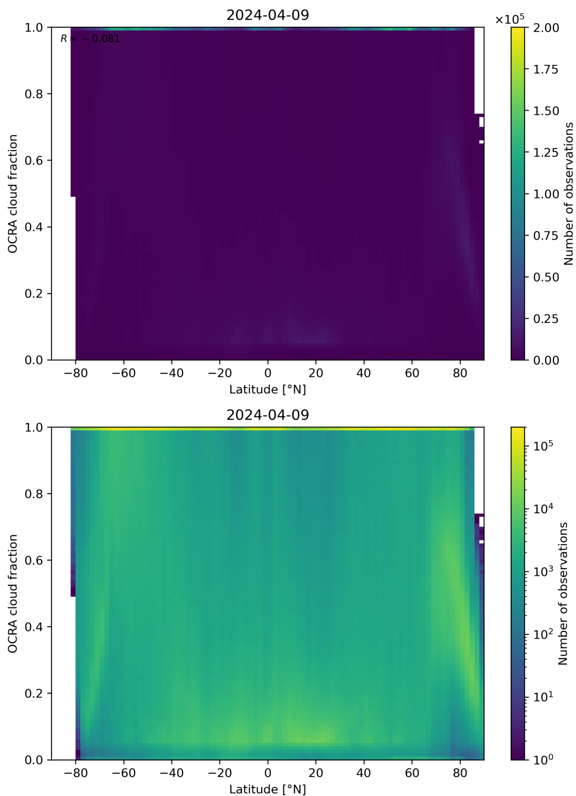
Figure 93: Scatter density plot of “Latitude” against “OCRA cloud fraction” for 2024-04-08 to 2024-04-10.
