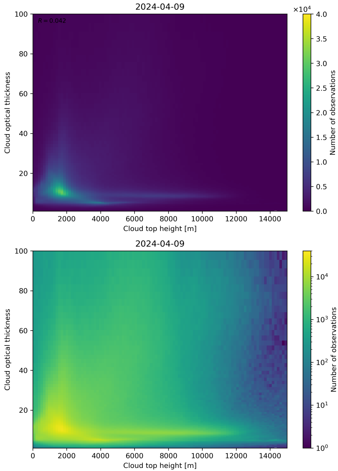
Figure 90: Scatter density plot of “Cloud top height” against “Cloud optical thickness” for 2024-04-08 to 2024-04-10.
