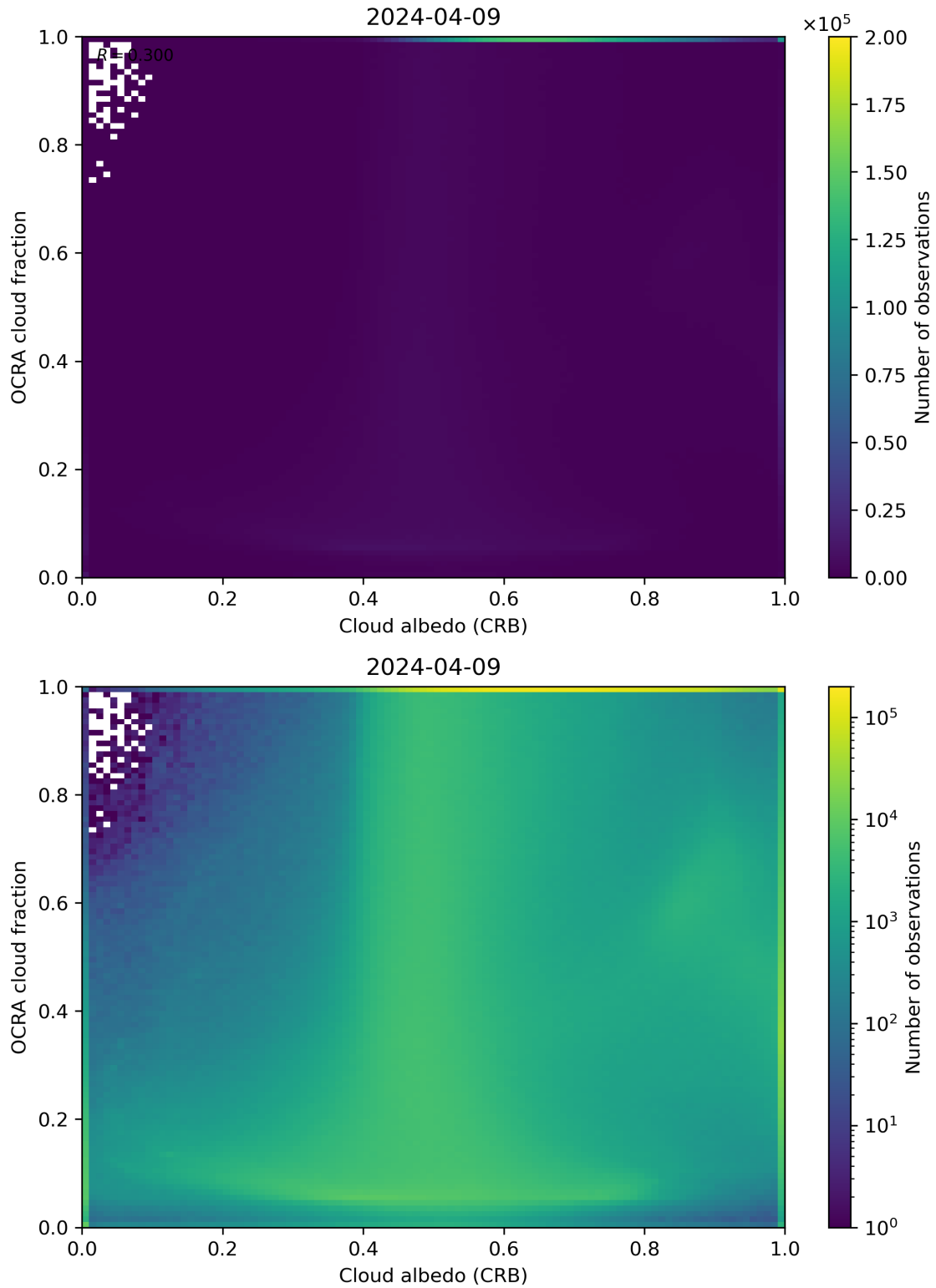
Figure 70: Scatter density plot of “Cloud albedo (CRB)” against “OCRA cloud fraction” for 2024-04-08 to 2024-04-10.
