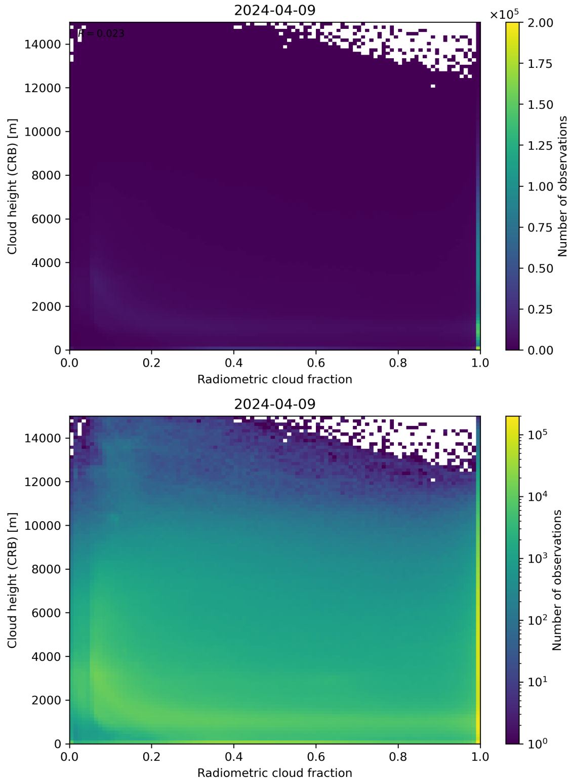
Figure 74: Scatter density plot of “Radiometric cloud fraction” against “Cloud height (CRB)” for 2024-04-08 to 2024-04-10.
