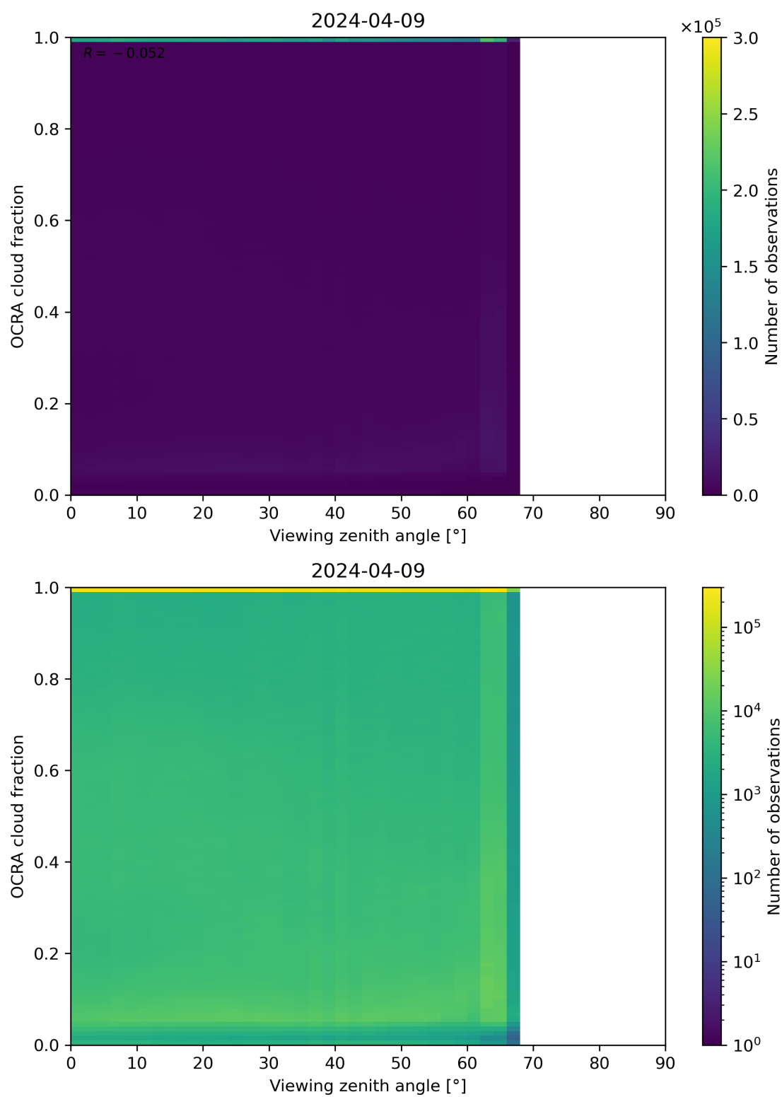
Figure 108: Scatter density plot of “Viewing zenith angle” against “OCRA cloud fraction” for 2024-04-08 to 2024-04-10.
