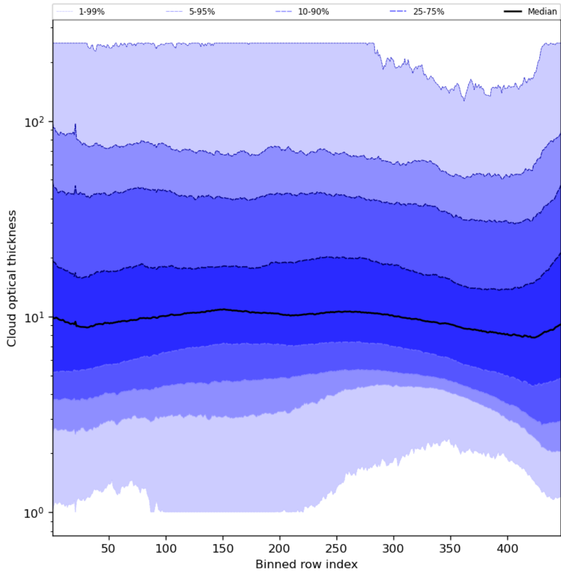
Figure 57: Along track statistics of “Cloud optical thickness” for 2024-04-08 to 2024-04-10
