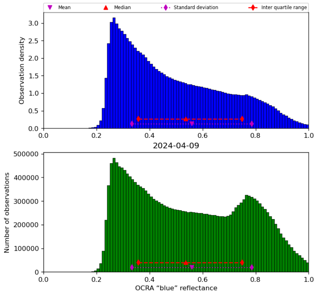
Figure 51: Histogram of “OCRA “blue” reflectance” for 2024-04-08 to 2024-04-10
