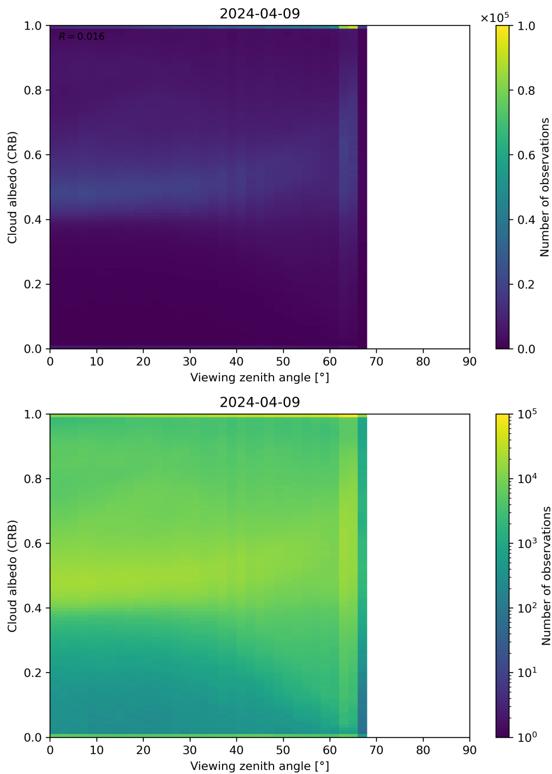
Figure 106: Scatter density plot of “Viewing zenith angle” against “Cloud albedo (CRB)” for 2024-04-08 to 2024-04-10.
