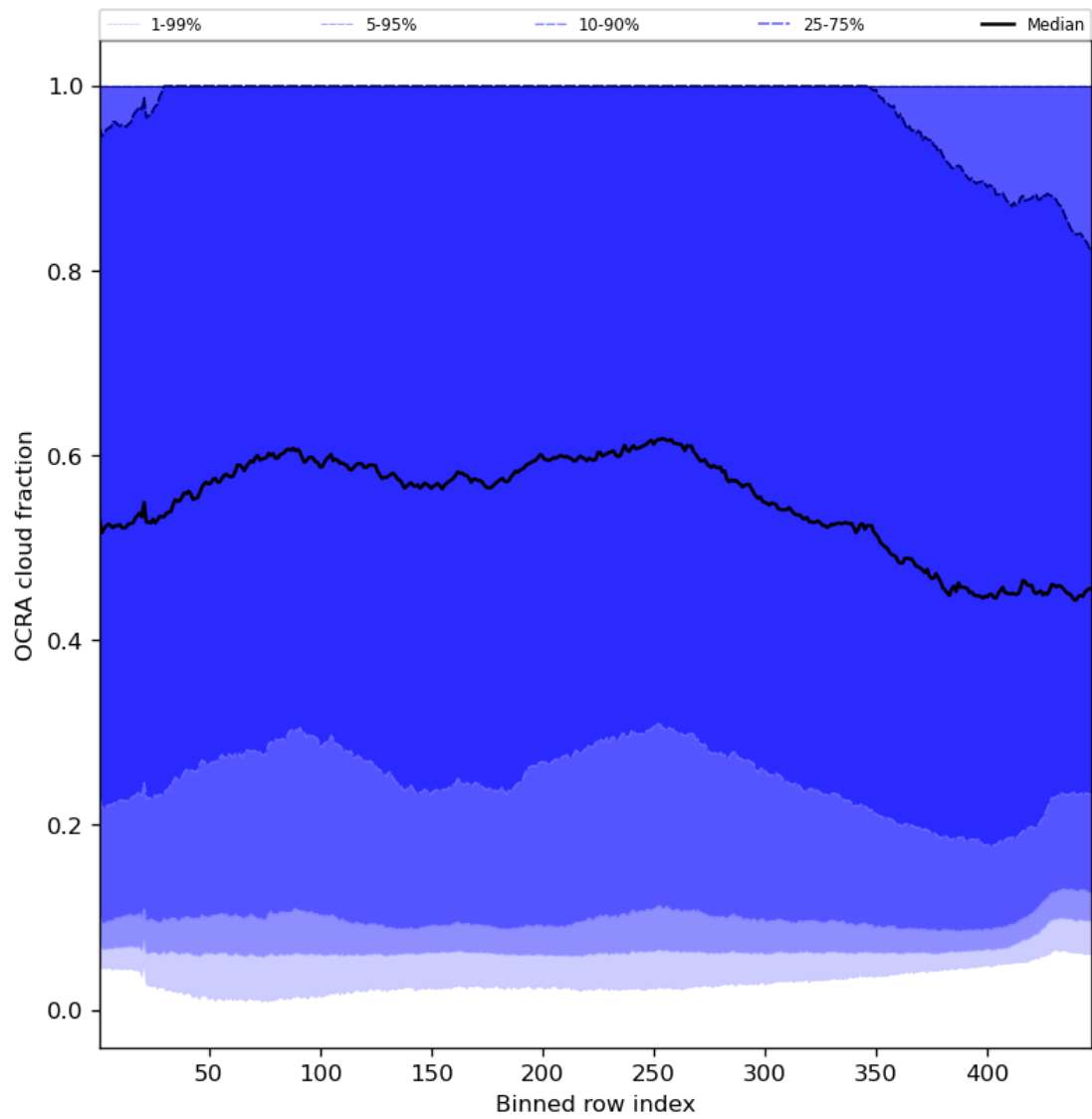
Figure 66: Along track statistics of “OCRA cloud fraction” for 2024-04-08 to 2024-04-10
