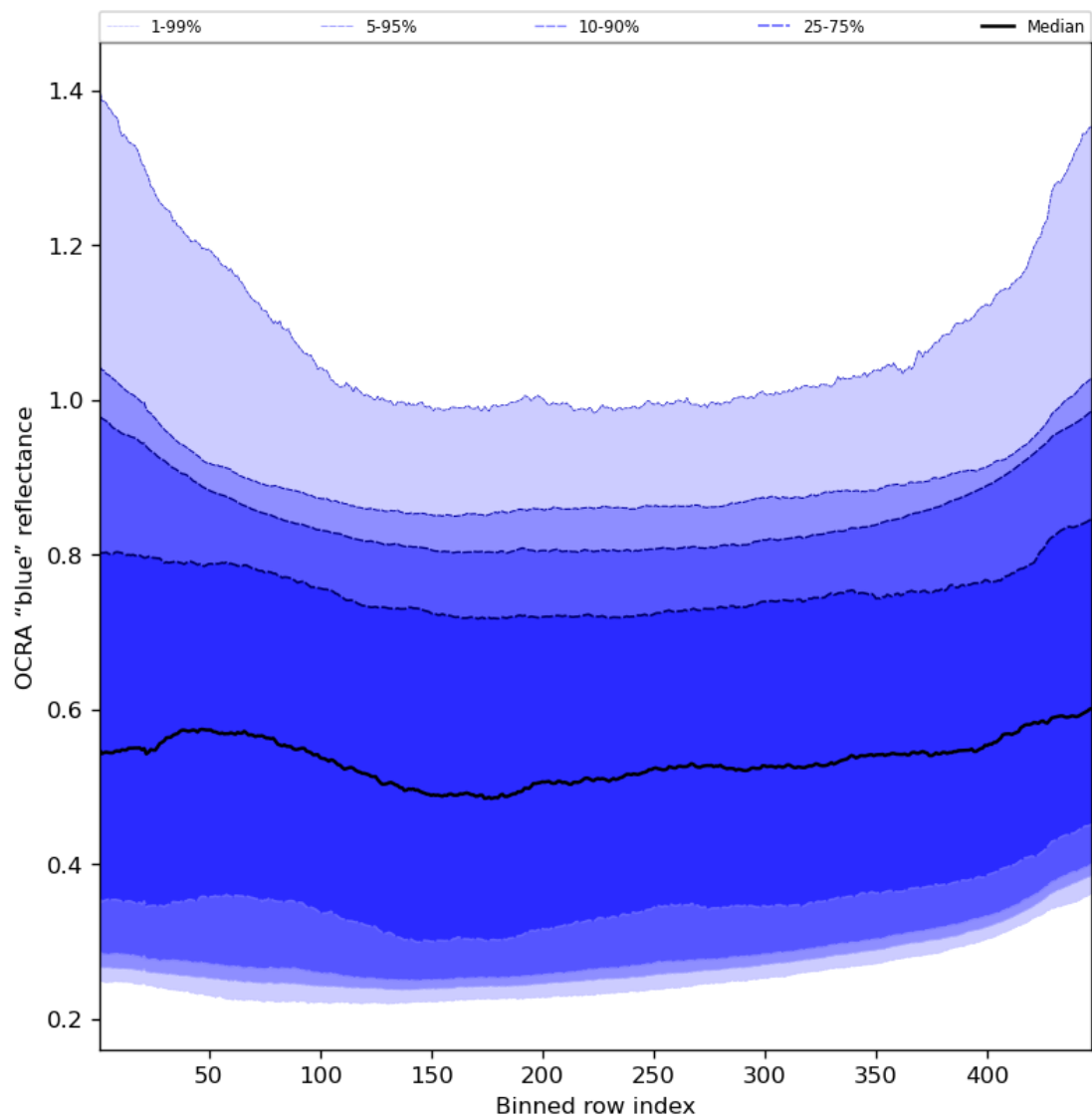
Figure 67: Along track statistics of “OCRA “blue” reflectance” for 2024-04-08 to 2024-04-10
