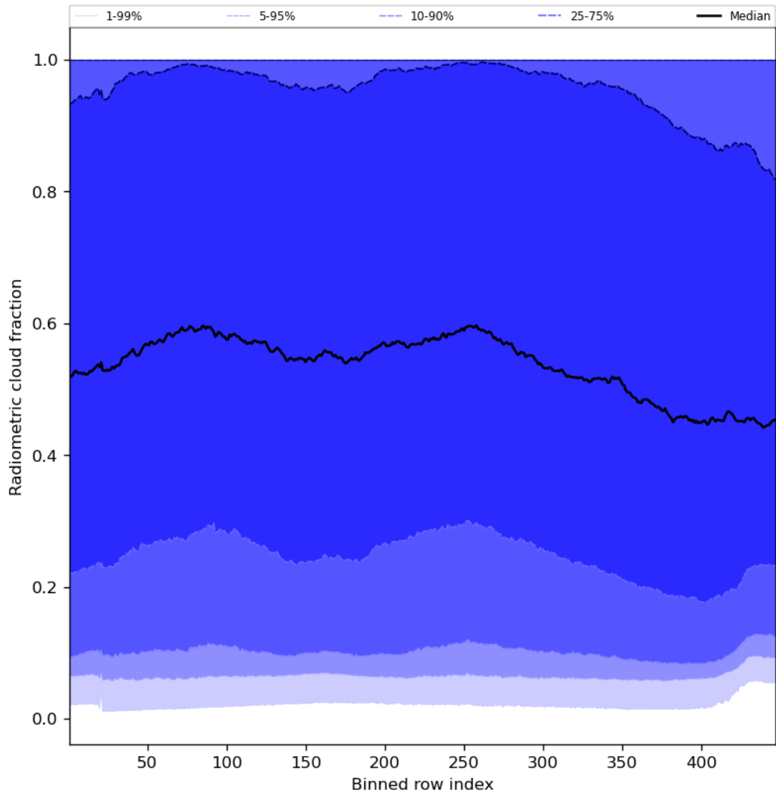
Figure 55: Along track statistics of “Radiometric cloud fraction” for 2024-04-08 to 2024-04-10
