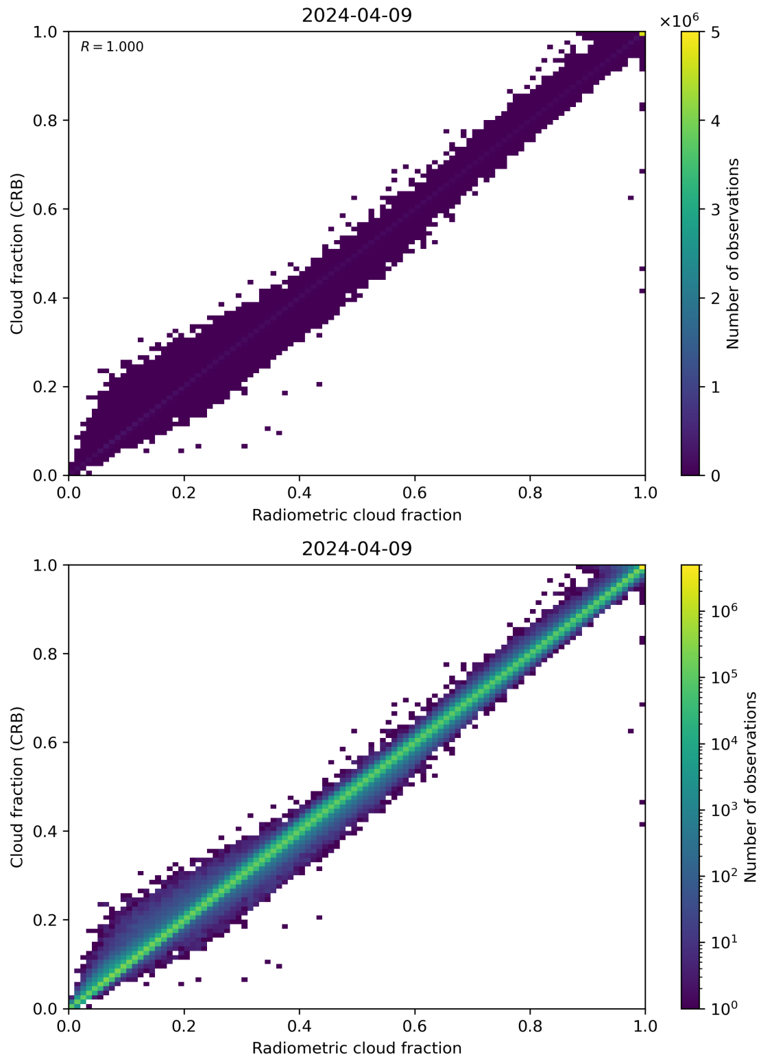
Figure 73: Scatter density plot of “Radiometric cloud fraction” against “Cloud fraction (CRB)” for 2024-04-08 to 2024-04-10.
