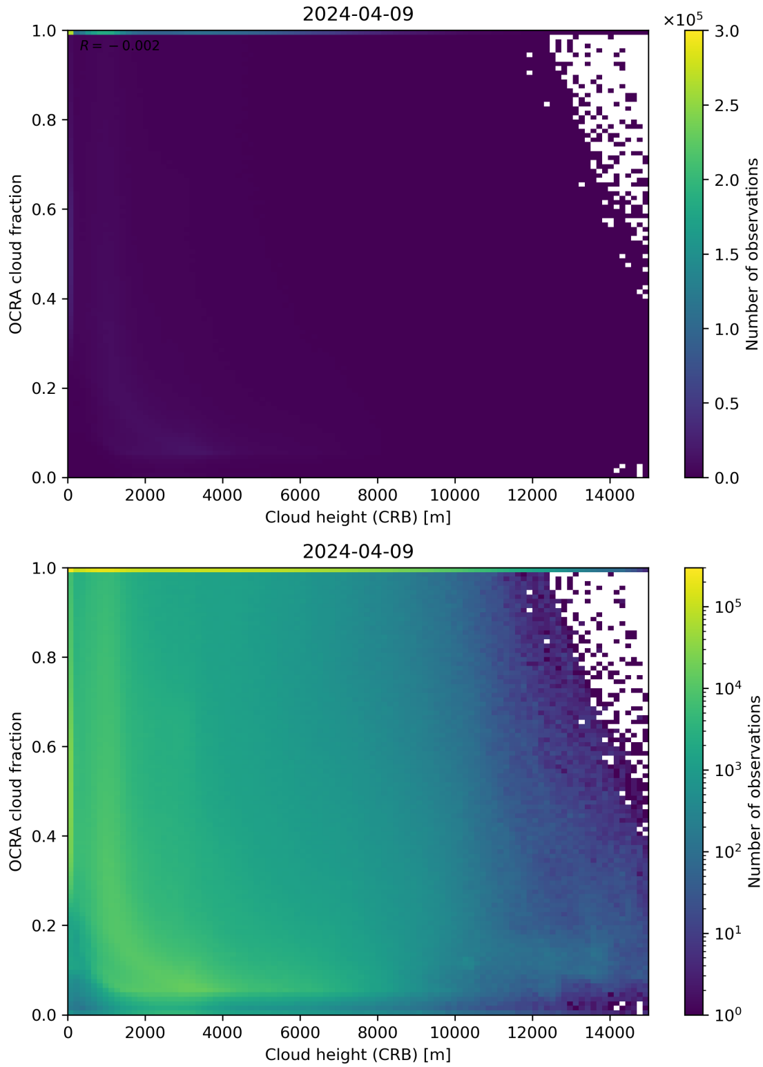
Figure 81: Scatter density plot of “Cloud height (CRB)” against “OCRA cloud fraction” for 2024-04-08 to 2024-04-10.
