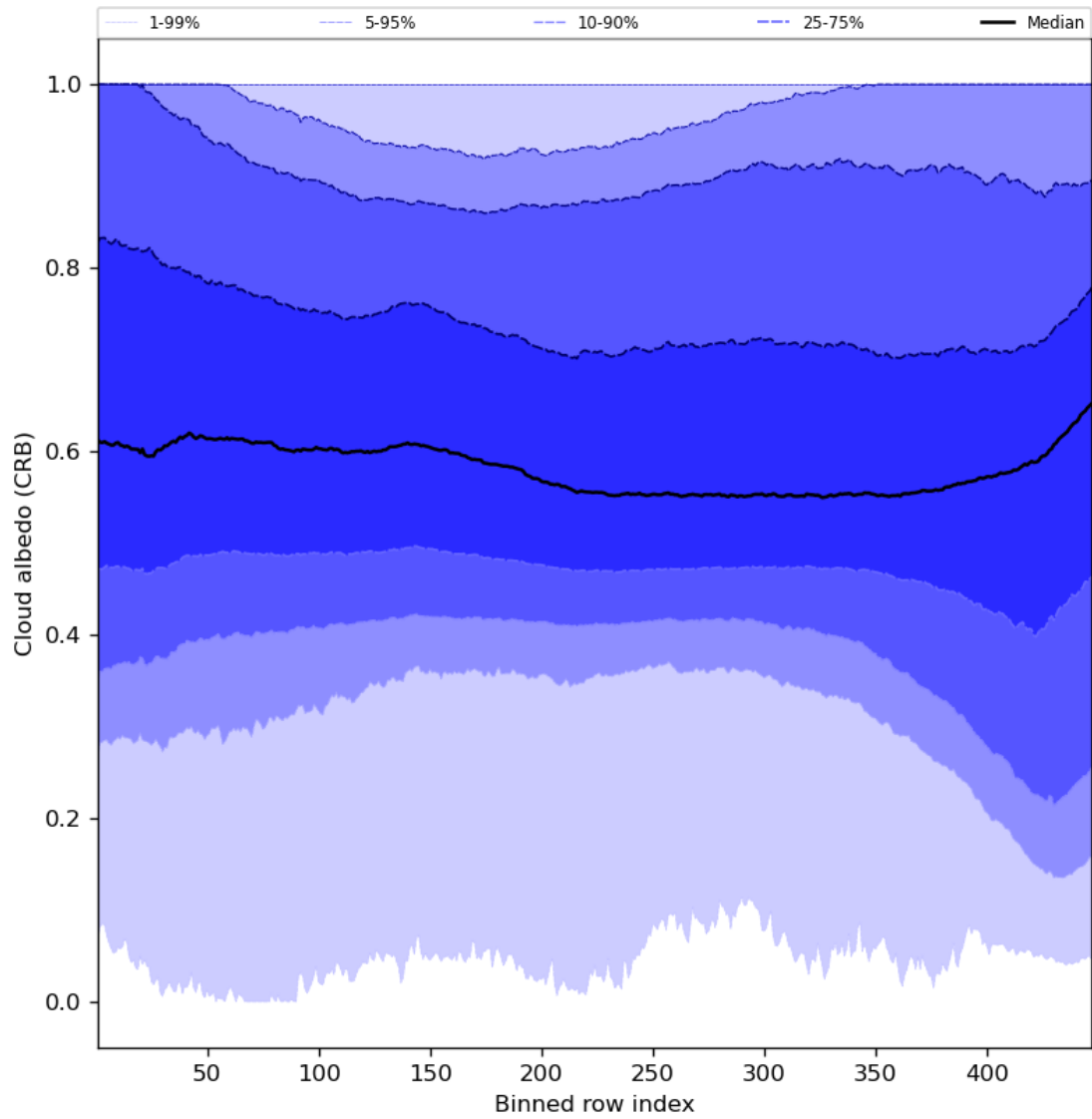
Figure 60: Along track statistics of “Cloud albedo (CRB)” for 2024-04-08 to 2024-04-10
