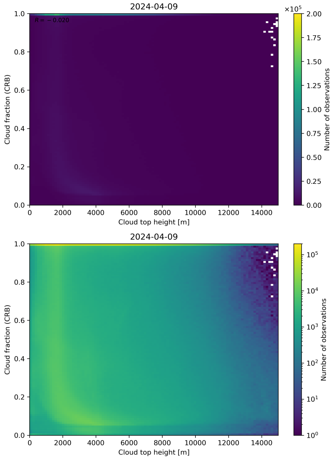
Figure 88: Scatter density plot of “Cloud top height” against “Cloud fraction (CRB)” for 2024-04-08 to 2024-04-10.
