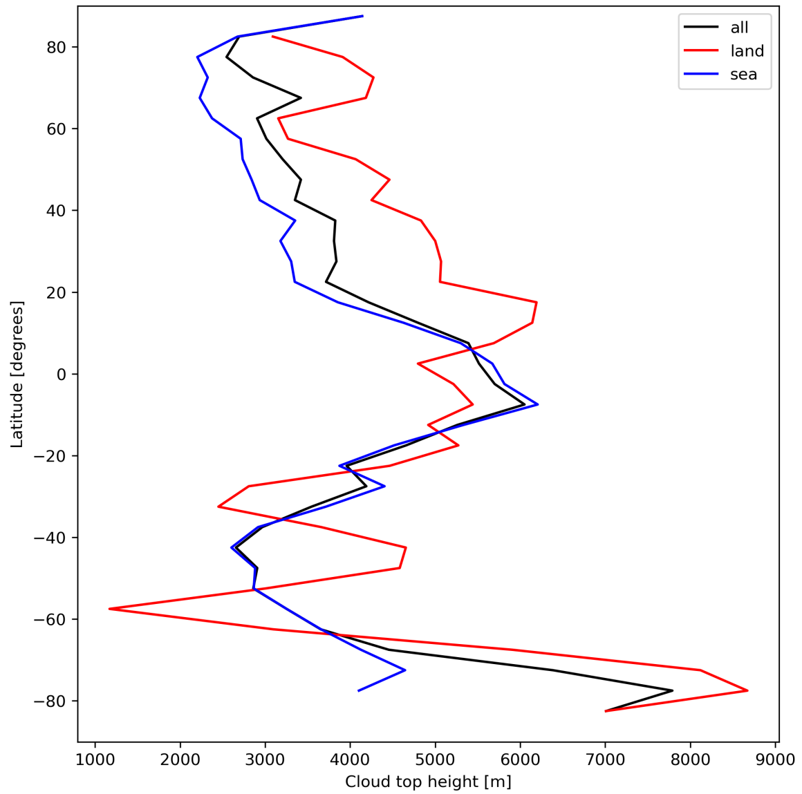
Figure 24: Zonal average of “Cloud top height” for 2024-04-08 to 2024-04-10.
