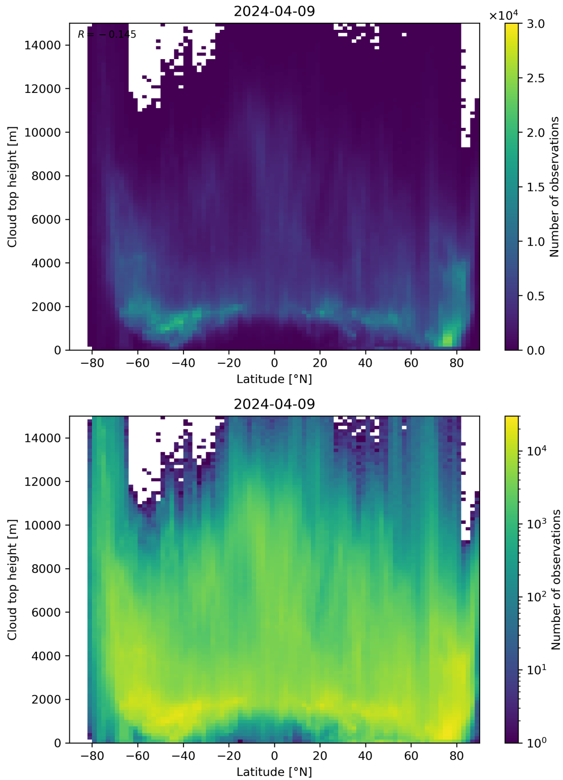
Figure 97: Scatter density plot of “Latitude” against “Cloud top height” for 2024-04-08 to 2024-04-10.
