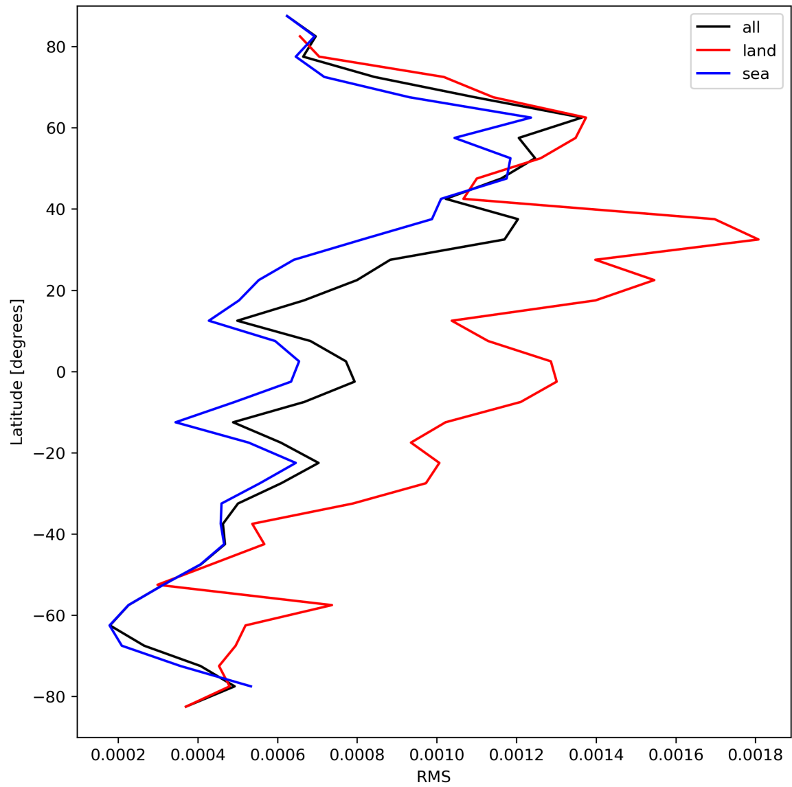
Figure 31: Zonal average of “RMS” for 2024-04-08 to 2024-04-10.
