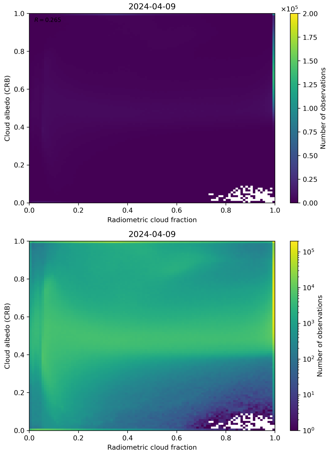
Figure 71: Scatter density plot of “Radiometric cloud fraction” against “Cloud albedo (CRB)” for 2024-04-08 to 2024-04-10.
