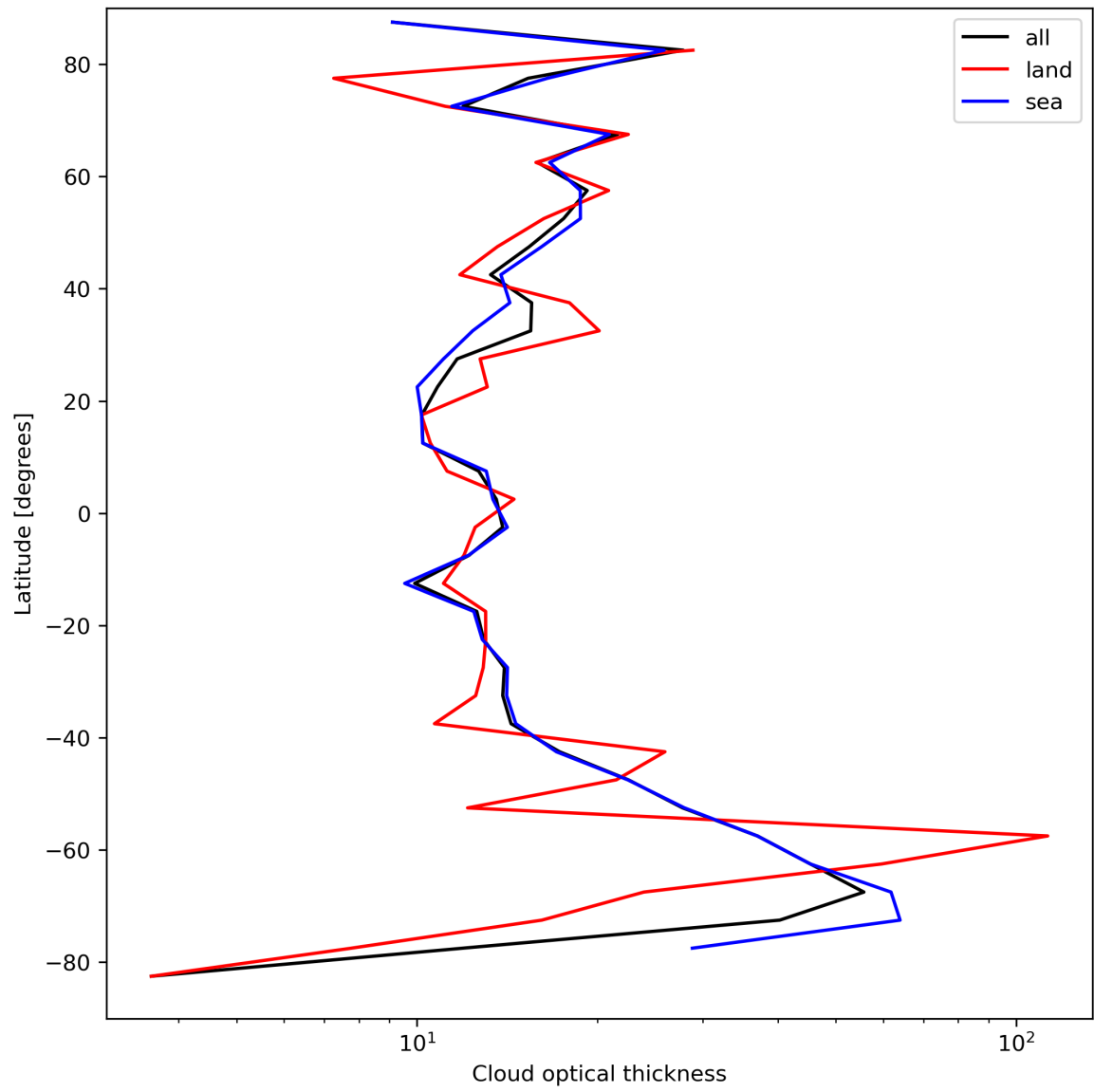
Figure 25: Zonal average of “Cloud optical thickness” for 2024-04-08 to 2024-04-10.
