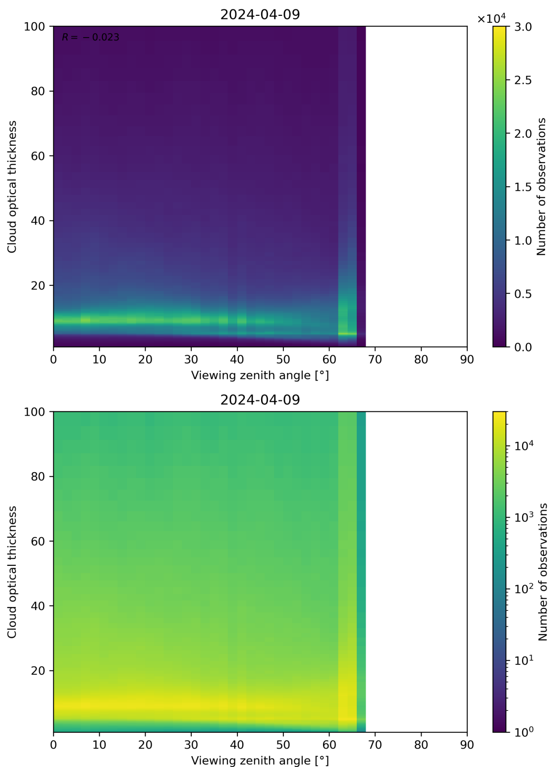
Figure 111: Scatter density plot of “Viewing zenith angle” against “Cloud optical thickness” for 2024-04-08 to 2024-04-10.
