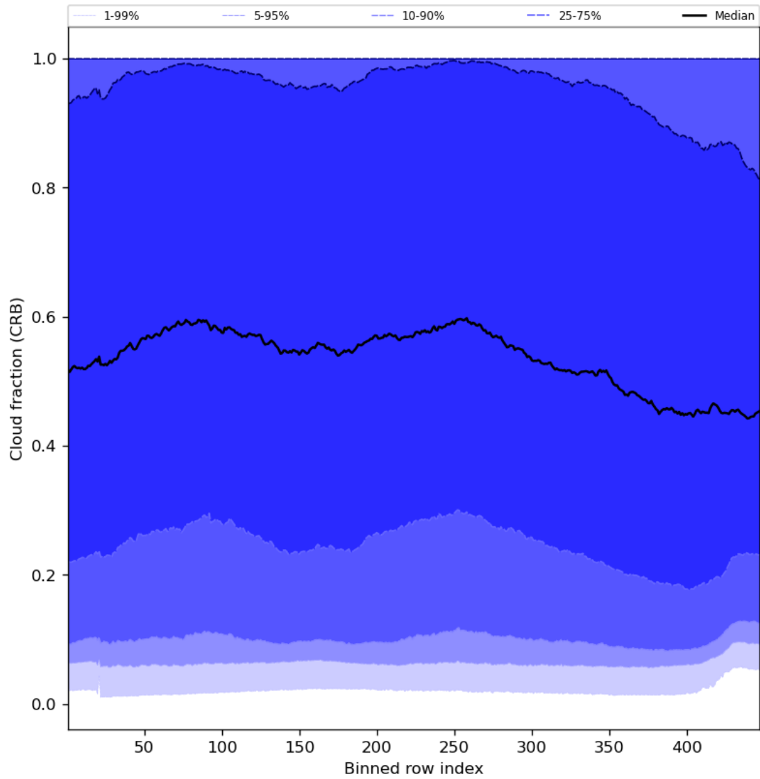
Figure 58: Along track statistics of “Cloud fraction (CRB)” for 2024-04-08 to 2024-04-10
