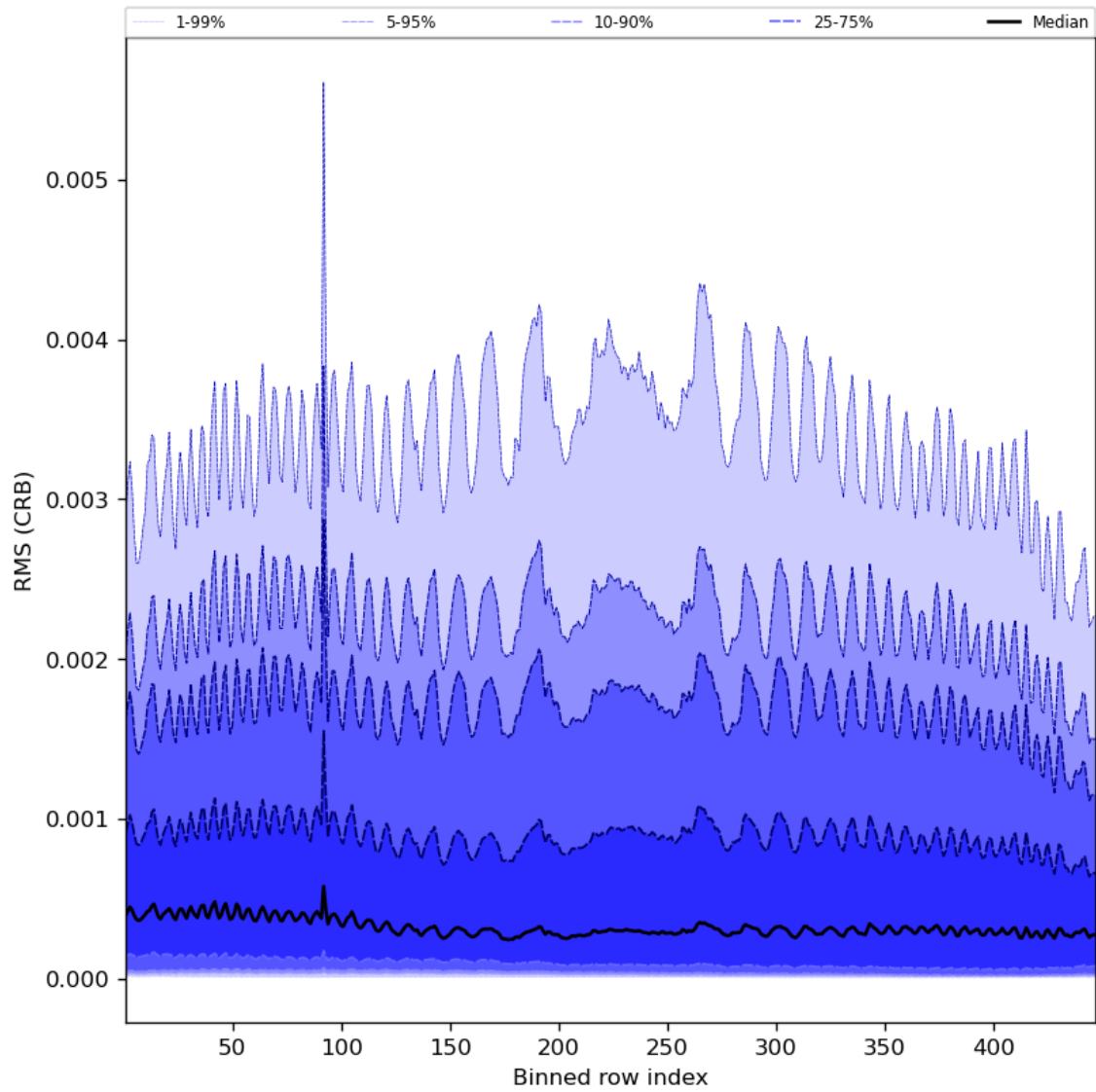
Figure 64: Along track statistics of “RMS (CRB)” for 2024-04-08 to 2024-04-10
