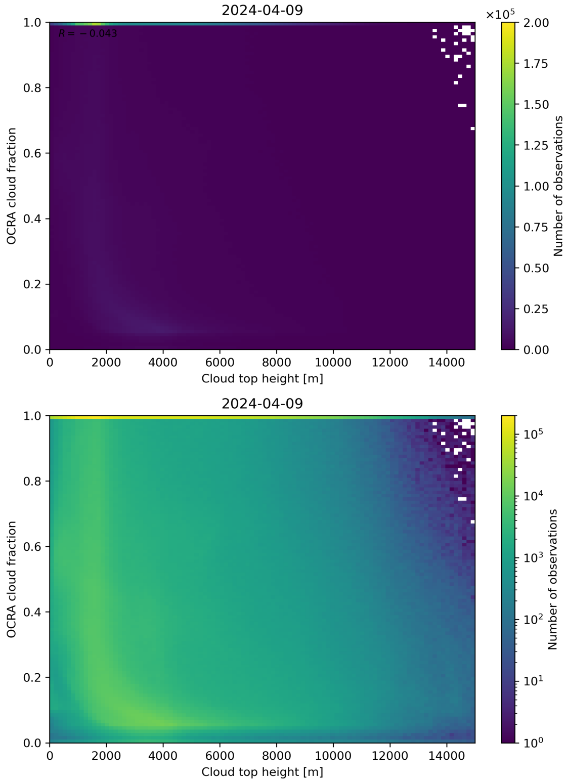
Figure 87: Scatter density plot of “Cloud top height” against “OCRA cloud fraction” for 2024-04-08 to 2024-04-10.
