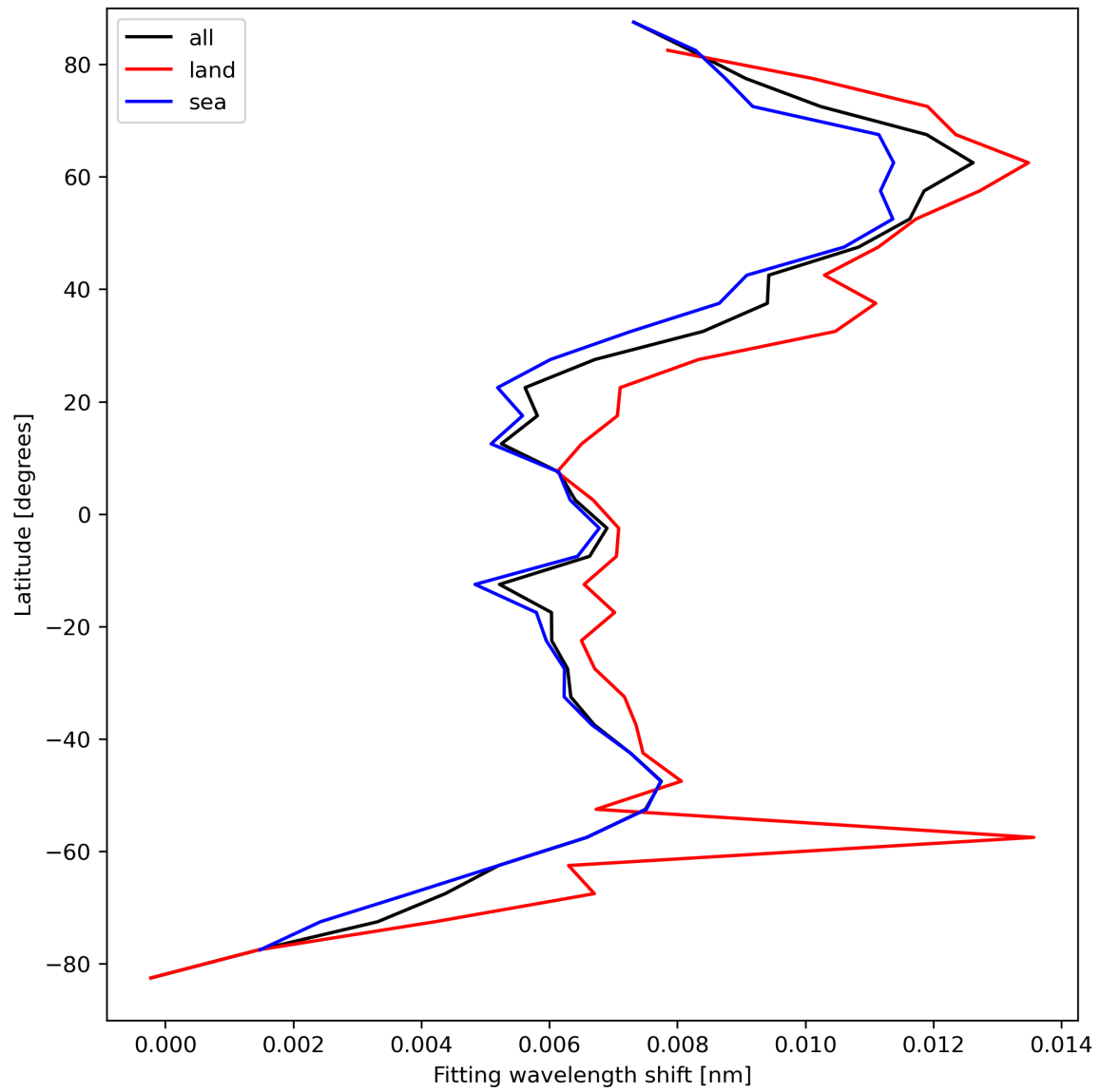
Figure 33: Zonal average of “Fitting wavelength shift” for 2024-04-08 to 2024-04-10.
