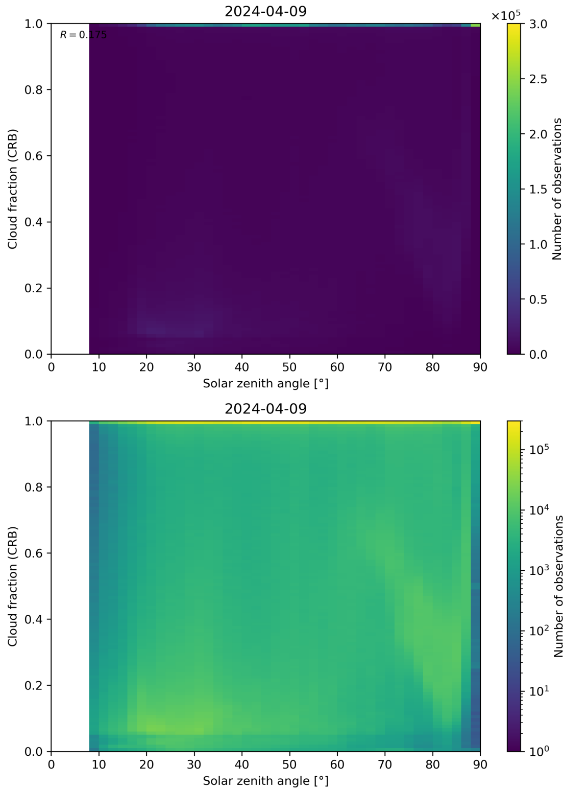
Figure 101: Scatter density plot of “Solar zenith angle” against “Cloud fraction (CRB)” for 2024-04-08 to 2024-04-10.
