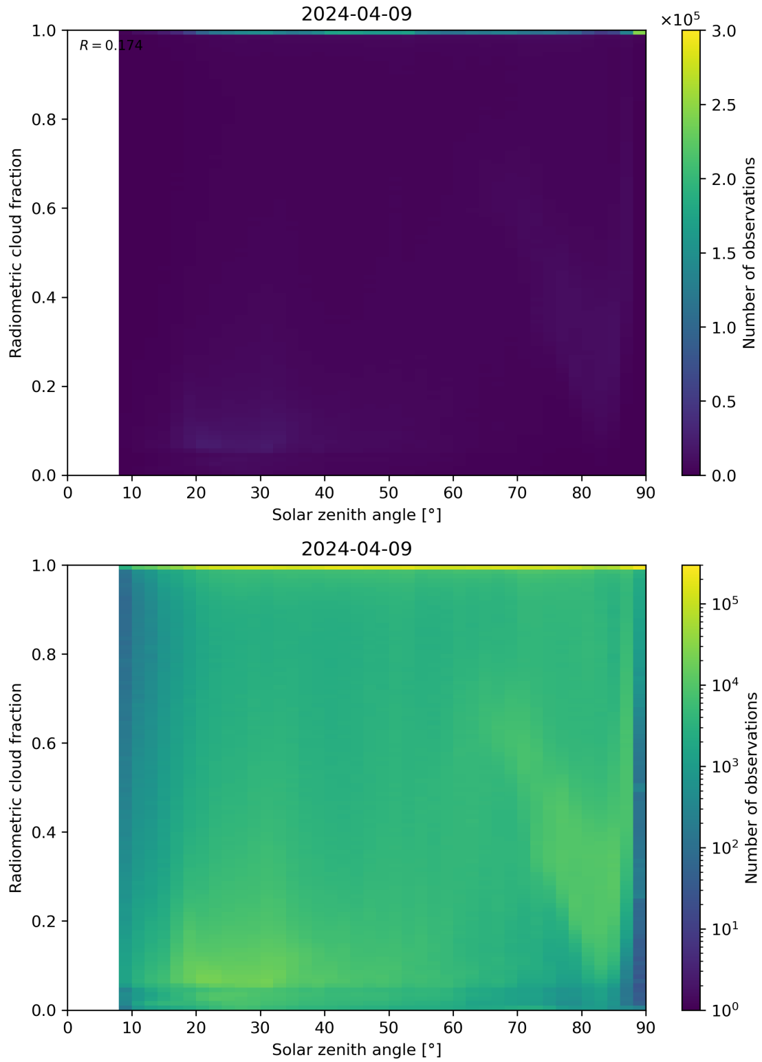
Figure 99: Scatter density plot of “Solar zenith angle” against “Radiometric cloud fraction” for 2024-04-08 to 2024-04-10.
