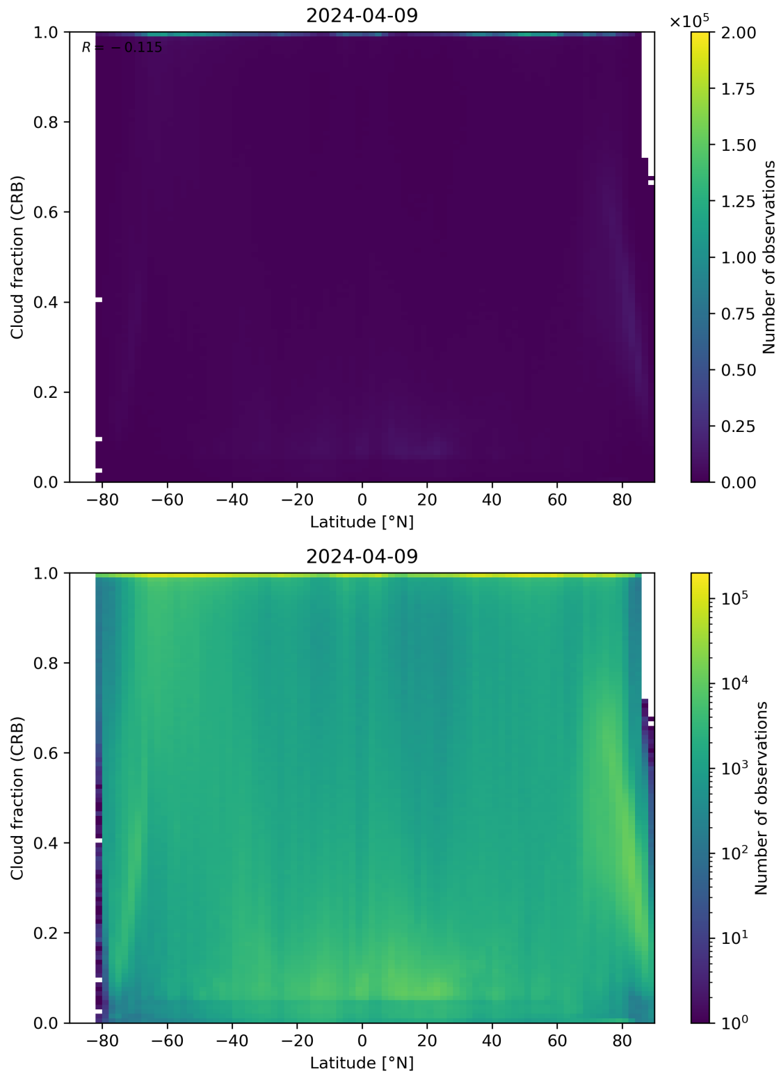
Figure 94: Scatter density plot of “Latitude” against “Cloud fraction (CRB)” for 2024-04-08 to 2024-04-10.
