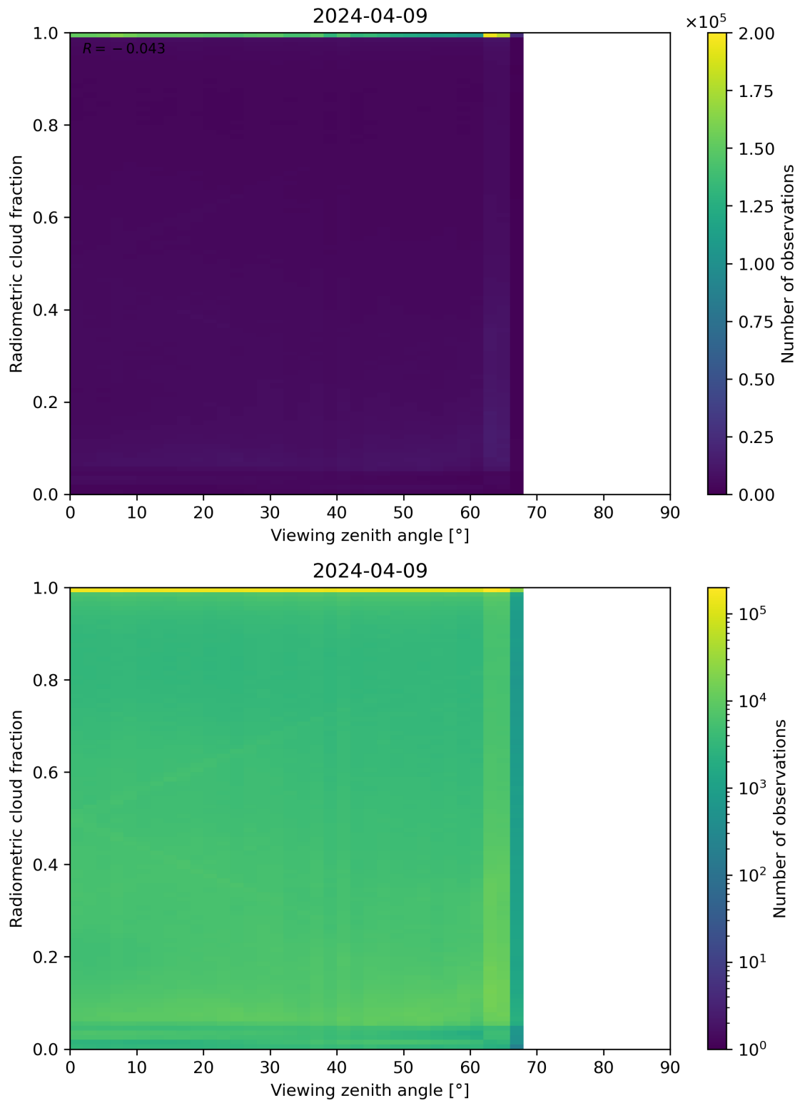
Figure 107: Scatter density plot of “Viewing zenith angle” against “Radiometric cloud fraction” for 2024-04-08 to 2024-04-10.
