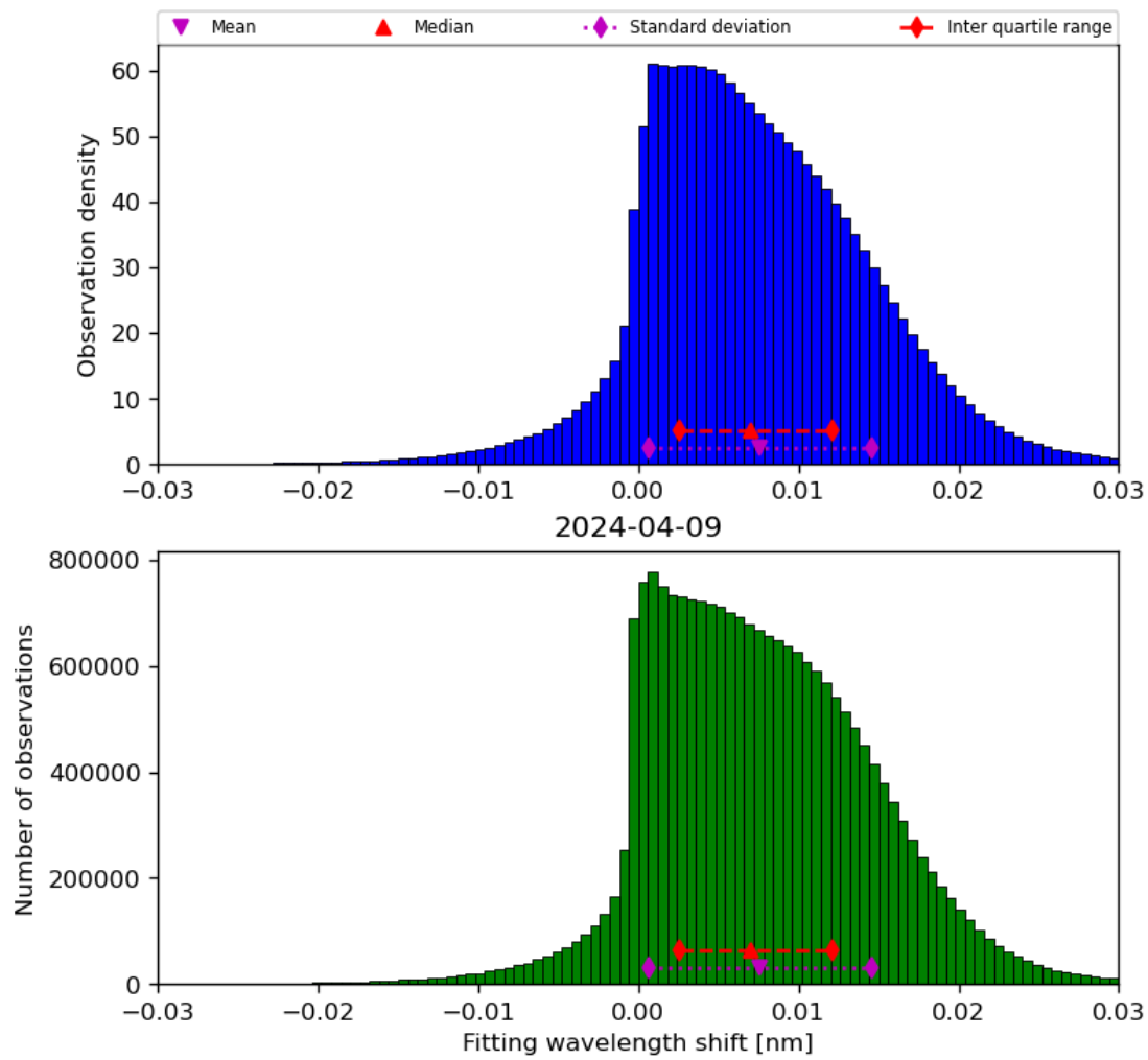
Figure 49: Histogram of “Fitting wavelength shift” for 2024-04-08 to 2024-04-10
