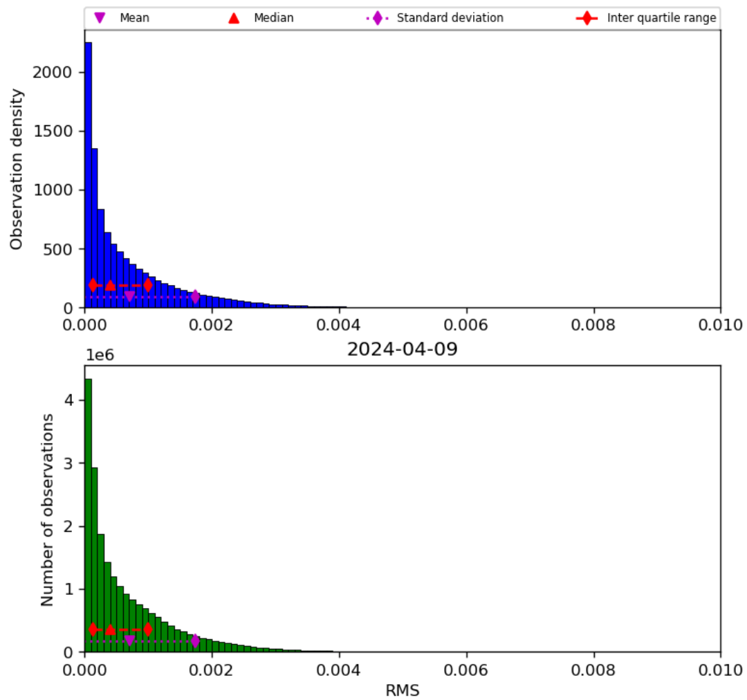
Figure 47: Histogram of “RMS” for 2024-04-08 to 2024-04-10
