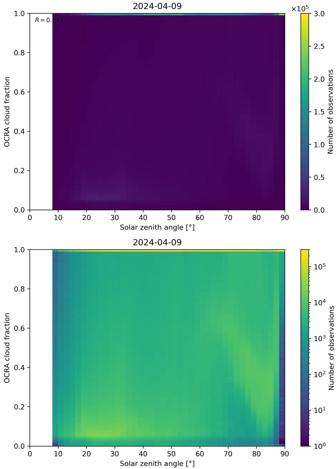
Figure 100: Scatter density plot of “Solar zenith angle” against “OCRA cloud fraction” for 2024-04-08 to 2024-04-10.
