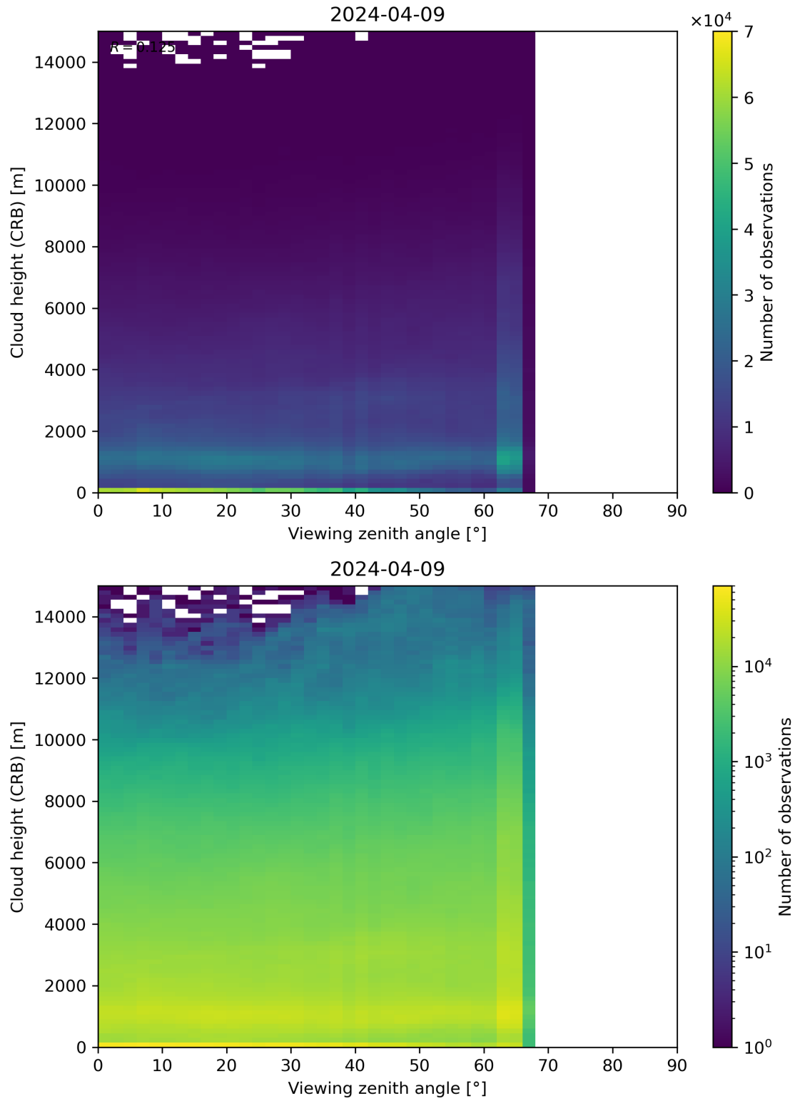
Figure 110: Scatter density plot of “Viewing zenith angle” against “Cloud height (CRB)” for 2024-04-08 to 2024-04-10.
