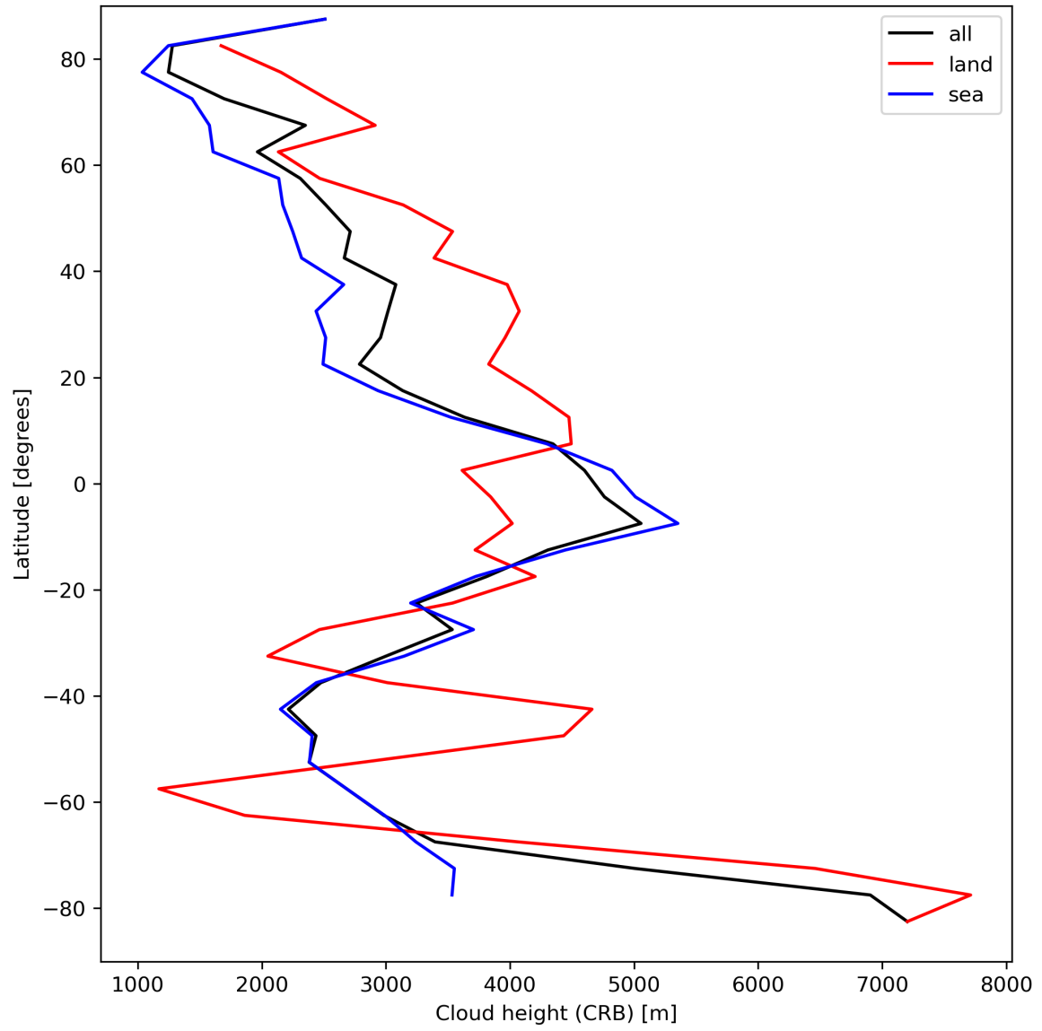
Figure 27: Zonal average of “Cloud height (CRB)” for 2024-04-08 to 2024-04-10.
