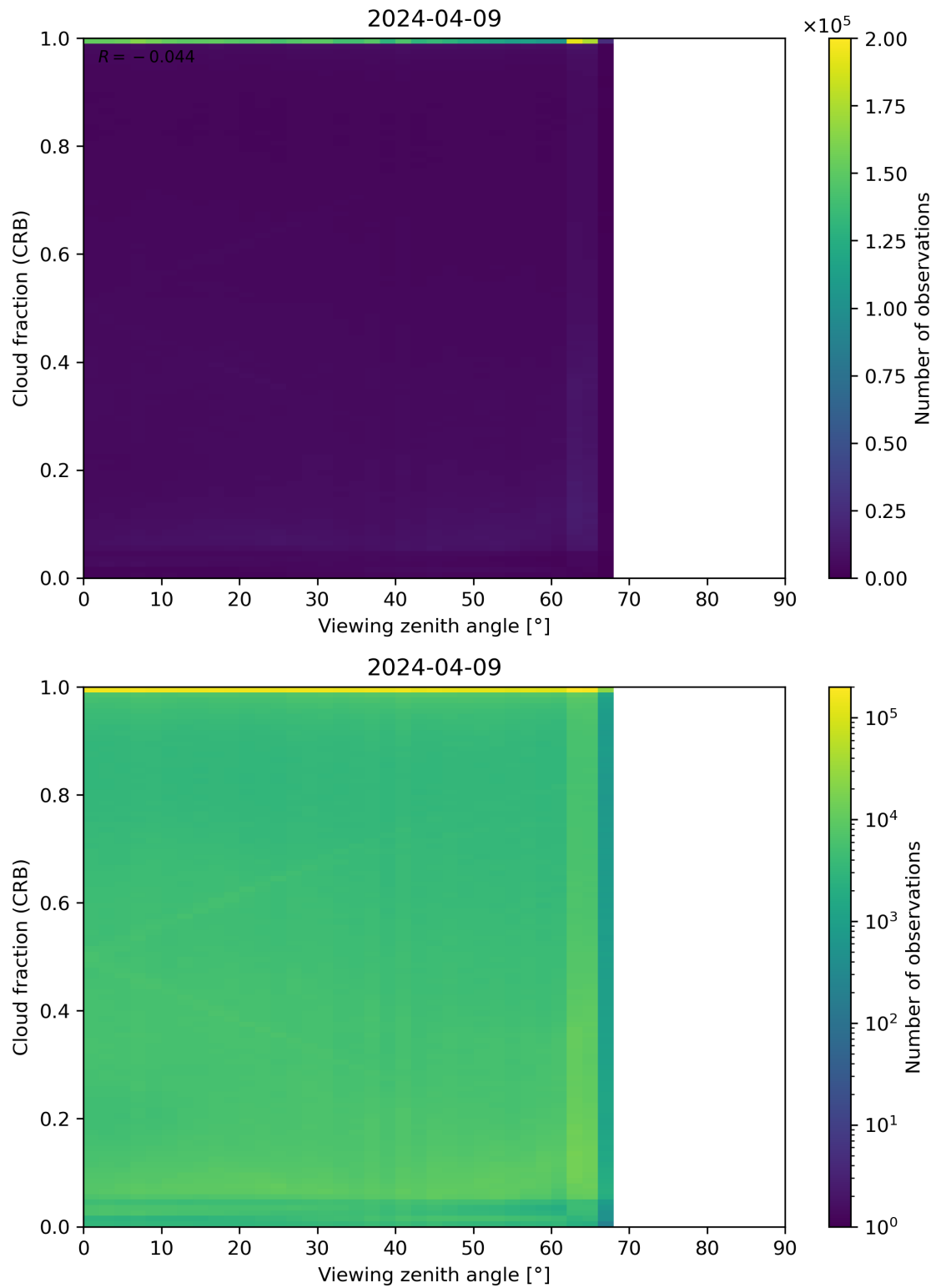
Figure 109: Scatter density plot of “Viewing zenith angle” against “Cloud fraction (CRB)” for 2024-04-08 to 2024-04-10.
