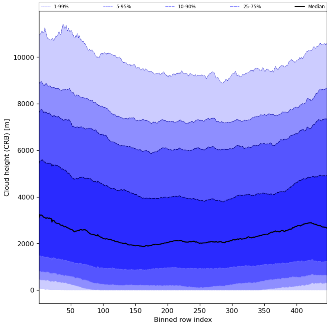
Figure 59: Along track statistics of “Cloud height (CRB)” for 2024-04-08 to 2024-04-10
