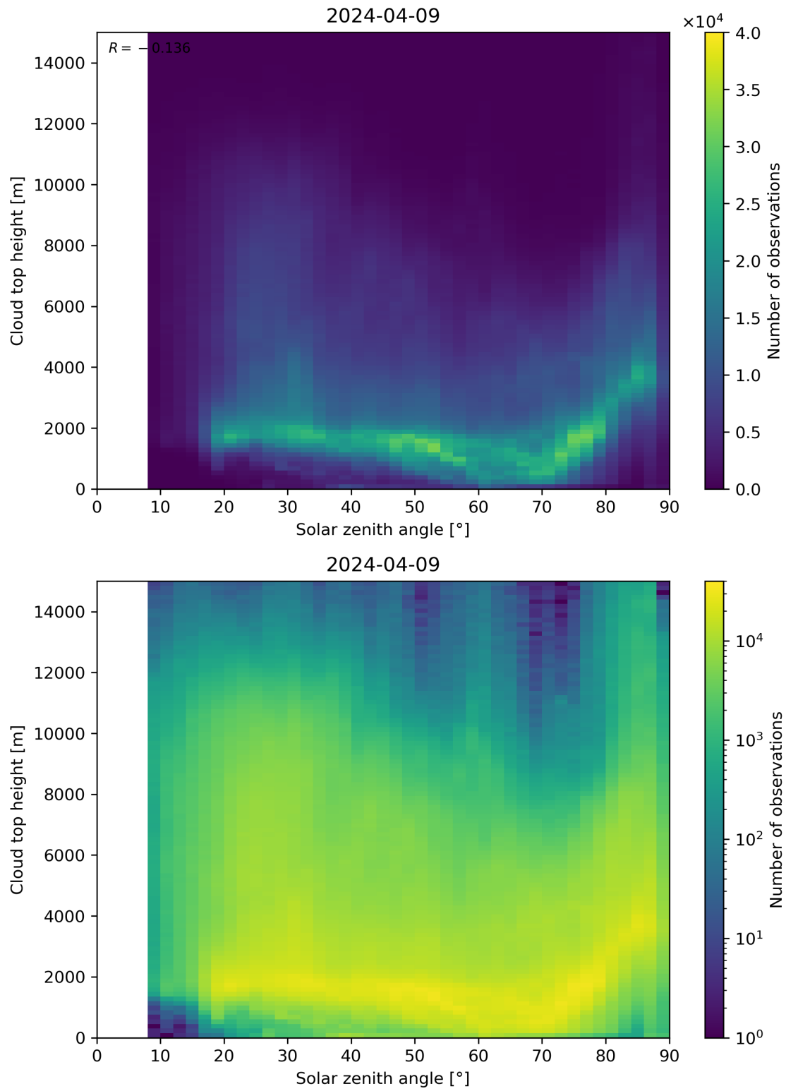
Figure 104: Scatter density plot of “Solar zenith angle” against “Cloud top height” for 2024-04-08 to 2024-04-10.
