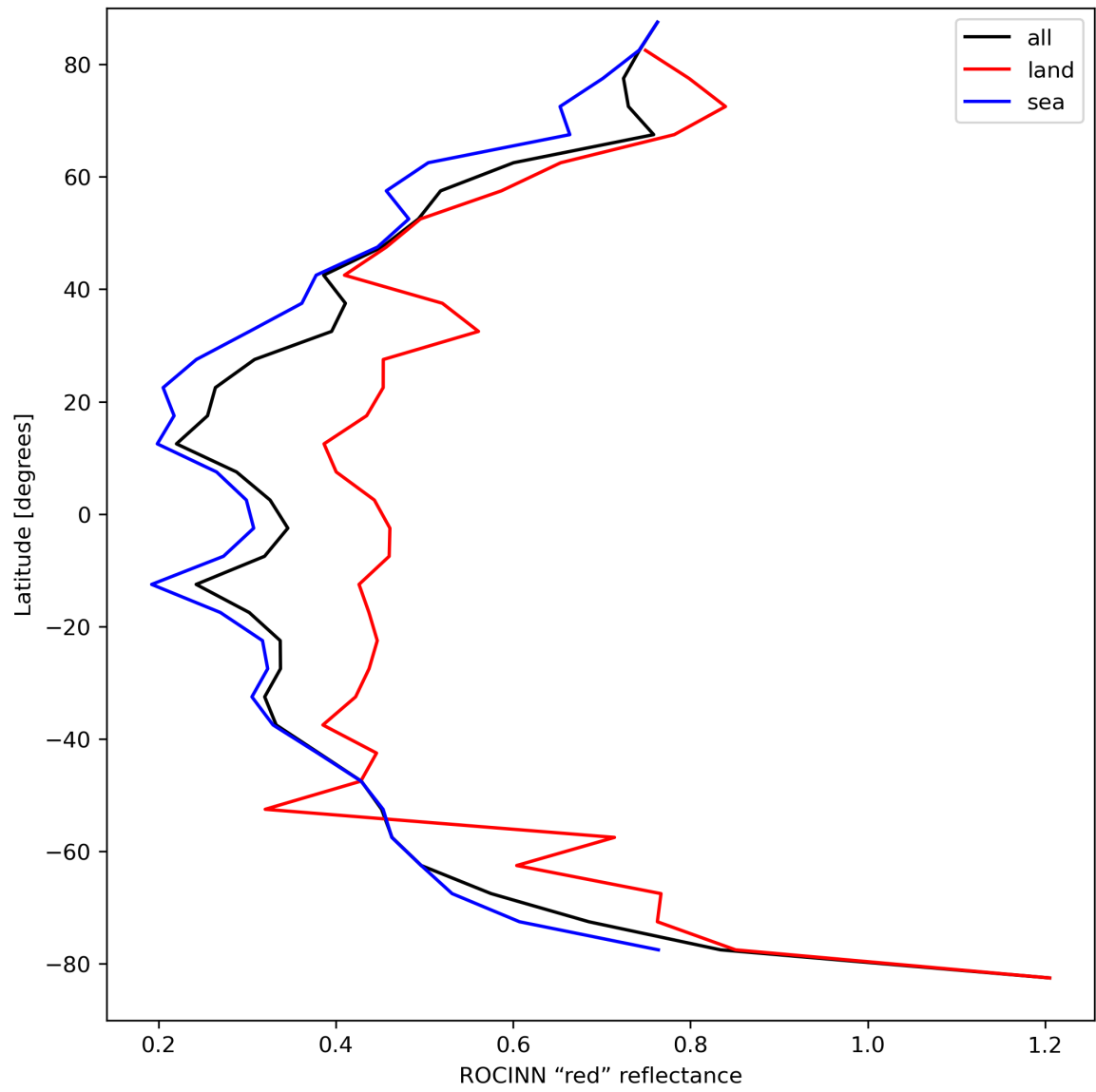
Figure 37: Zonal average of “ROCINN “red” reflectance” for 2024-04-08 to 2024-04-10.
