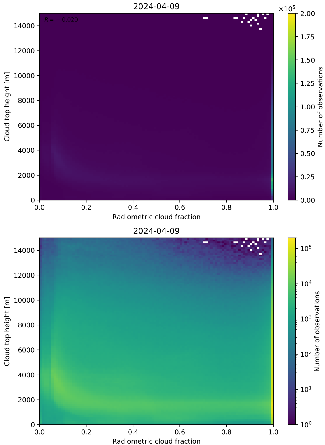
Figure 76: Scatter density plot of “Radiometric cloud fraction” against “Cloud top height” for 2024-04-08 to 2024-04-10.
