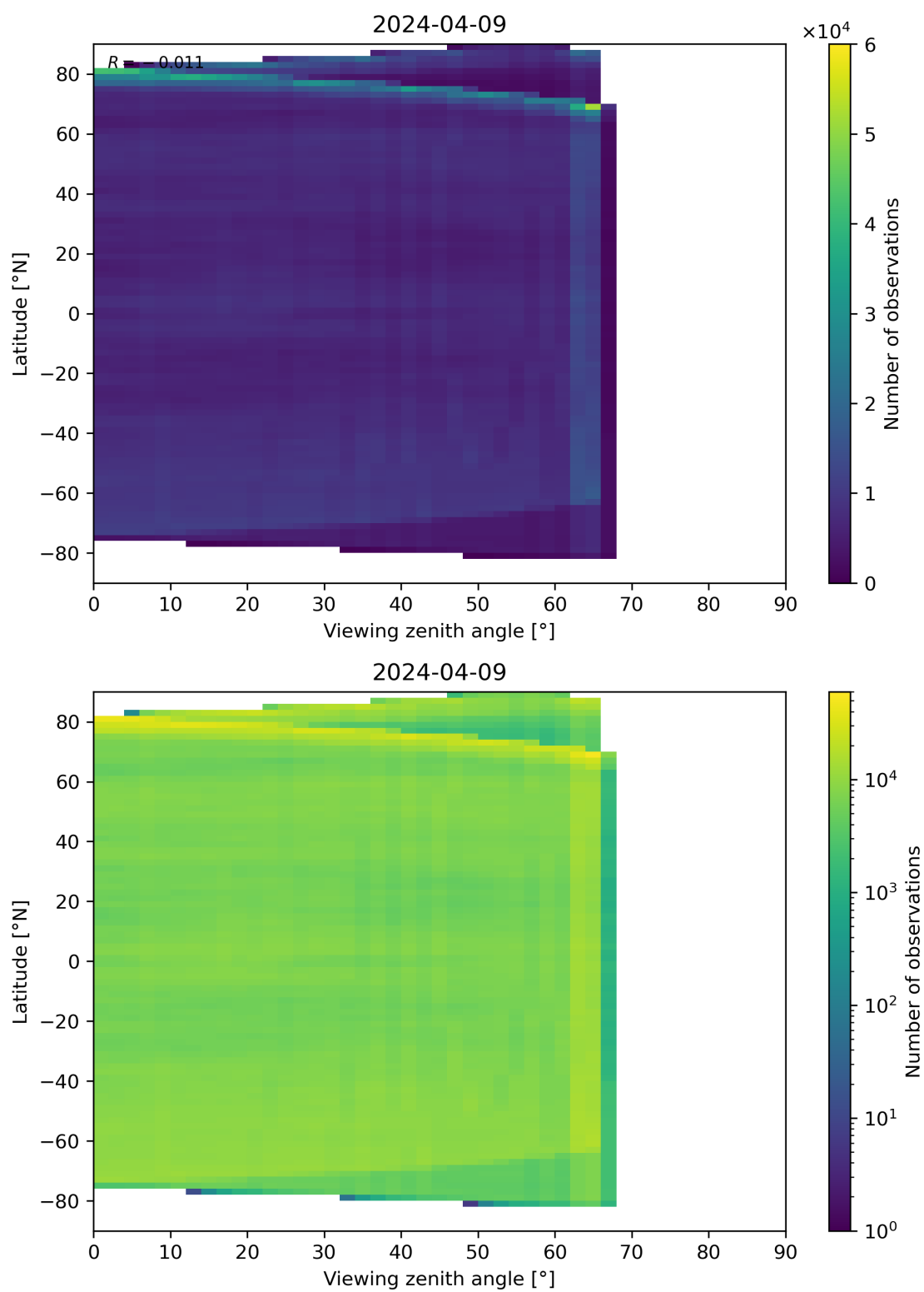
Figure 113: Scatter density plot of “Viewing zenith angle” against “Latitude” for 2024-04-08 to 2024-04-10.
