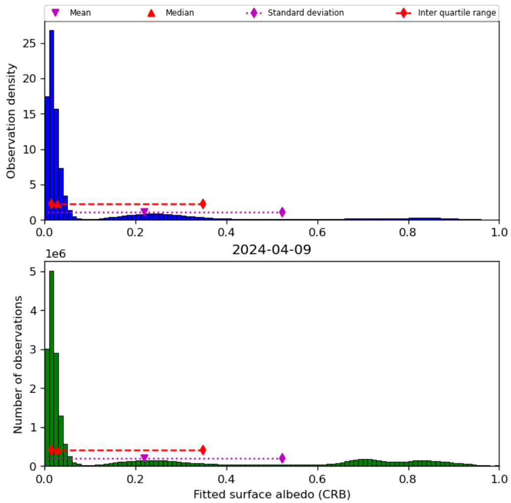
Figure 46: Histogram of “Fitted surface albedo (CRB)” for 2024-04-08 to 2024-04-10
