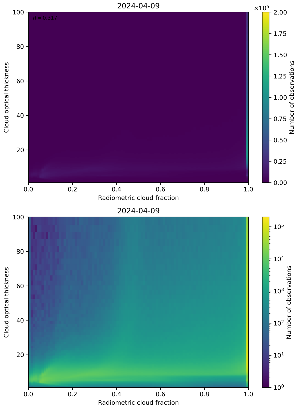
Figure 75: Scatter density plot of “Radiometric cloud fraction” against “Cloud optical thickness” for 2024-04-08 to 2024-04-10.
