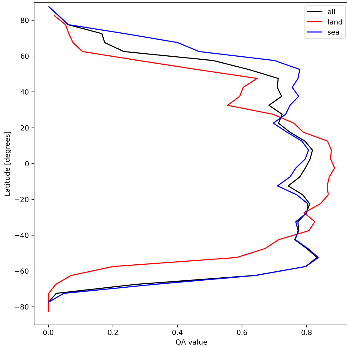
Figure 22: Zonal average of “QA value” for 2024-04-08 to 2024-04-10.
