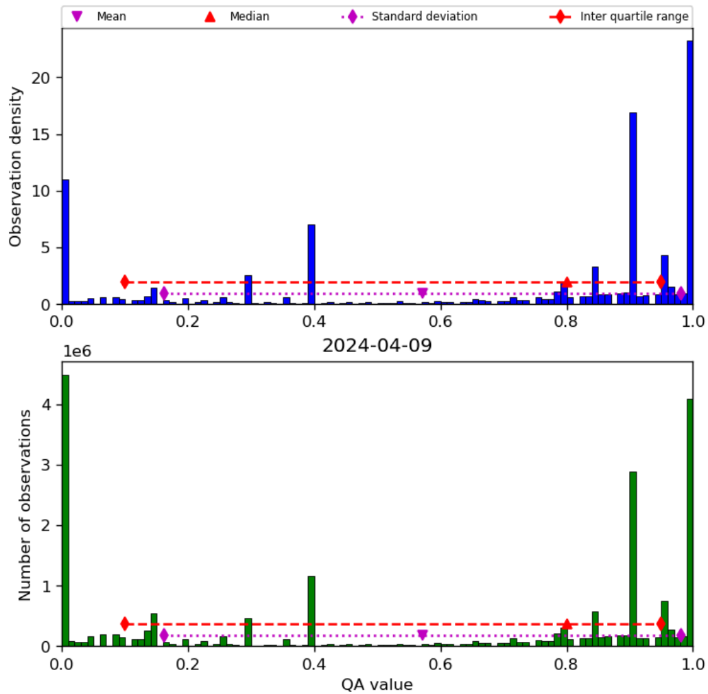
Figure 38: Histogram of “QA value” for 2024-04-08 to 2024-04-10
