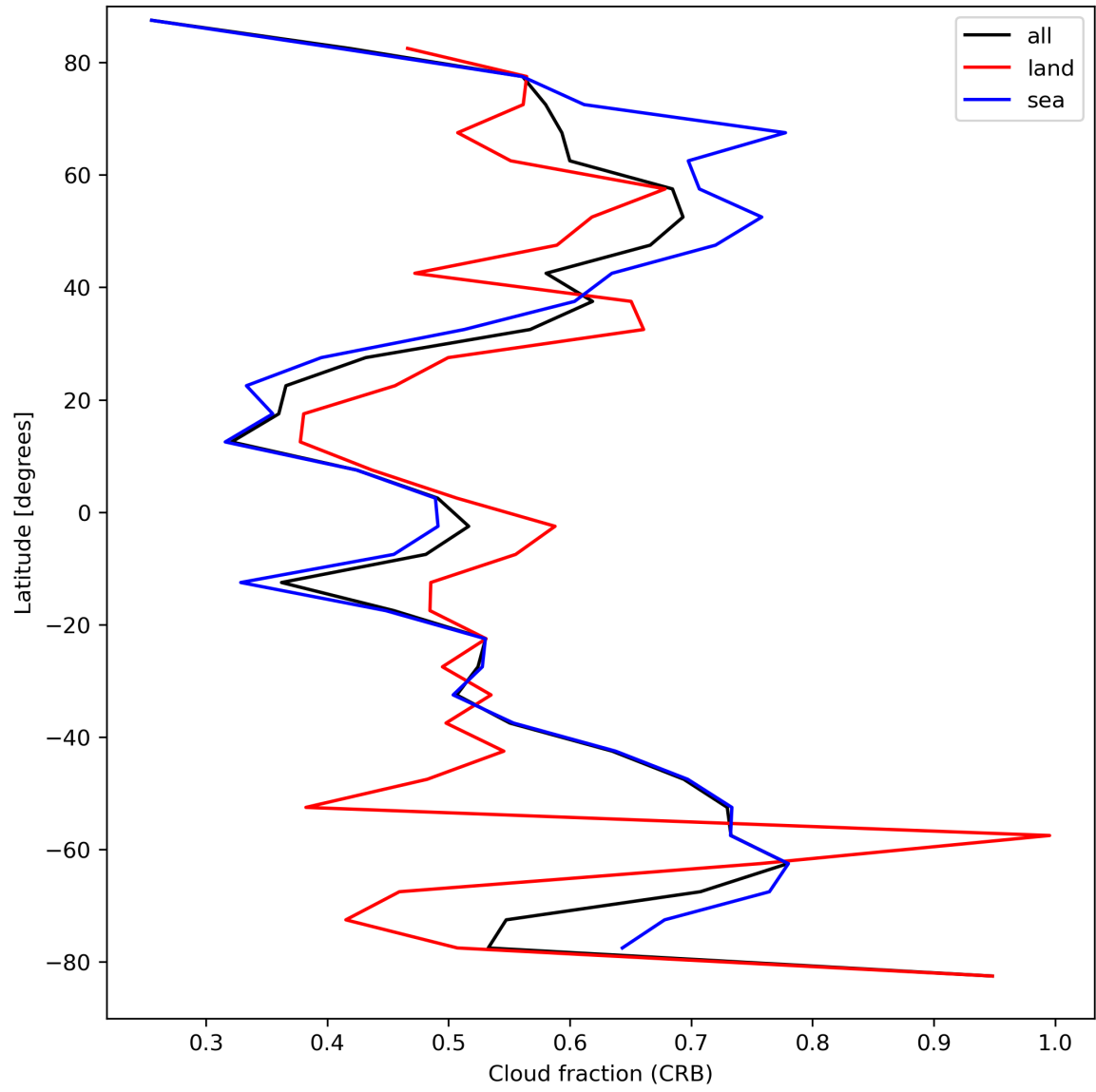
Figure 26: Zonal average of “Cloud fraction (CRB)” for 2024-04-08 to 2024-04-10.
