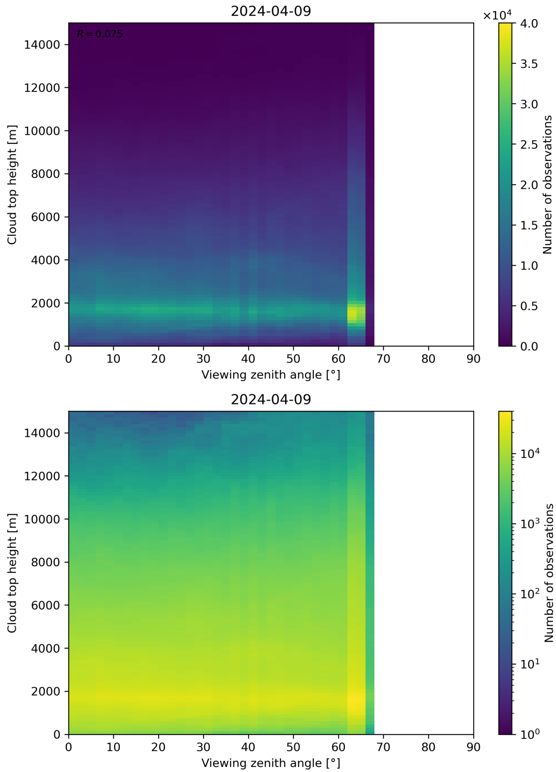
Figure 112: Scatter density plot of “Viewing zenith angle” against “Cloud top height” for 2024-04-08 to 2024-04-10.
