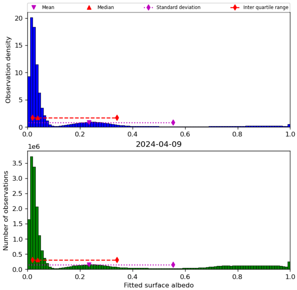
Figure 45: Histogram of “Fitted surface albedo” for 2024-04-08 to 2024-04-10
