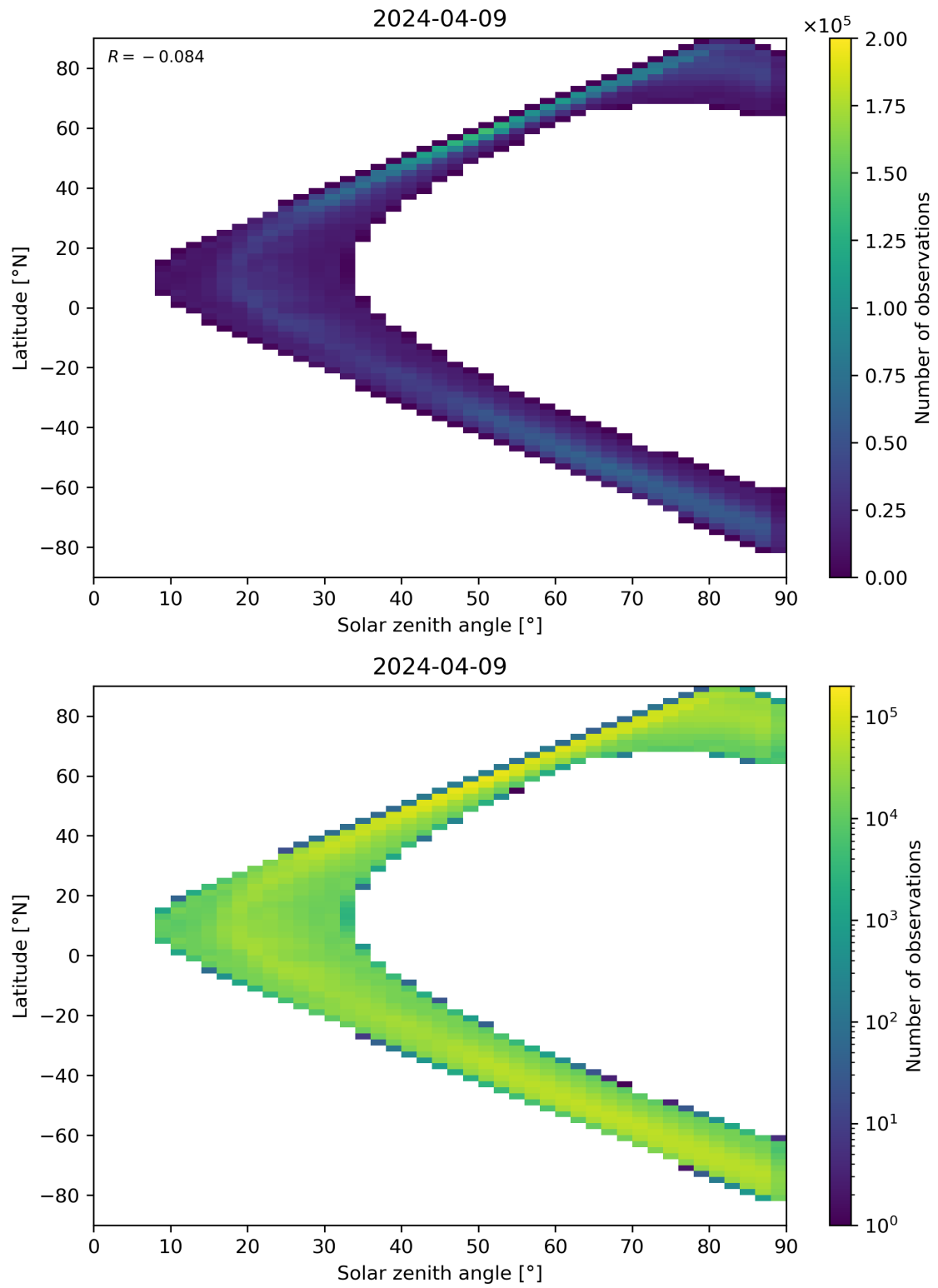
Figure 105: Scatter density plot of “Solar zenith angle” against “Latitude” for 2024-04-08 to 2024-04-10.
