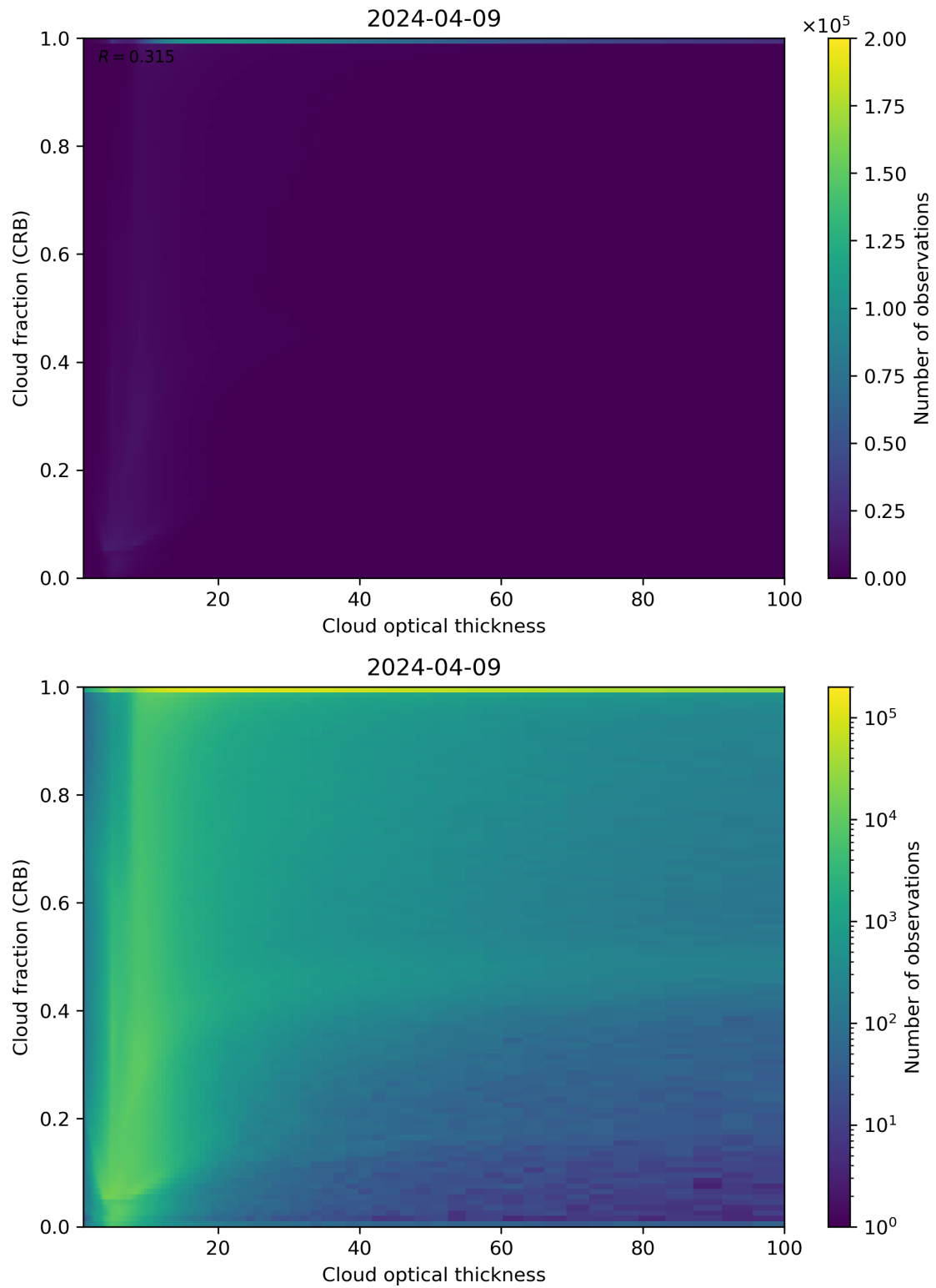
Figure 84: Scatter density plot of “Cloud optical thickness” against “Cloud fraction (CRB)” for 2024-04-08 to 2024-04-10.
