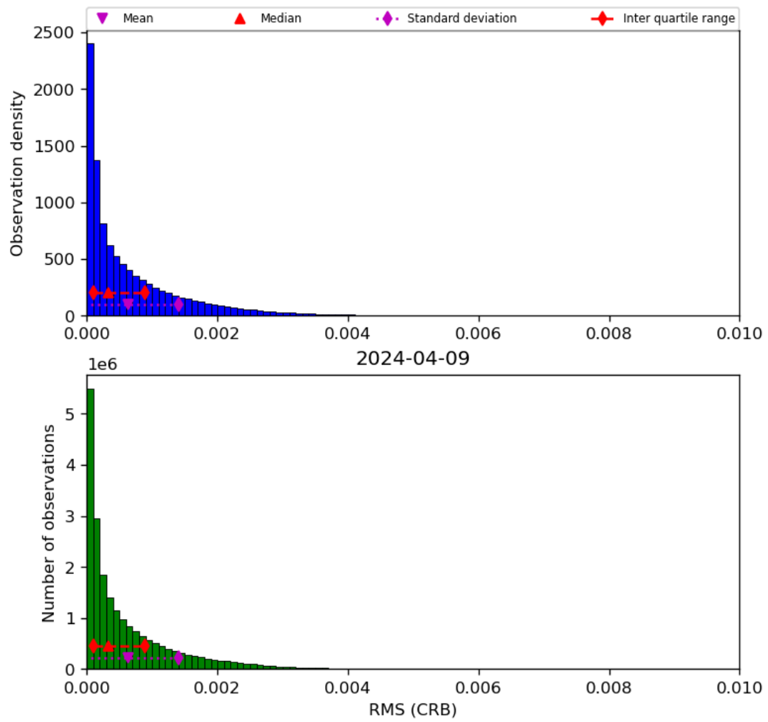
Figure 48: Histogram of “RMS (CRB)” for 2024-04-08 to 2024-04-10
