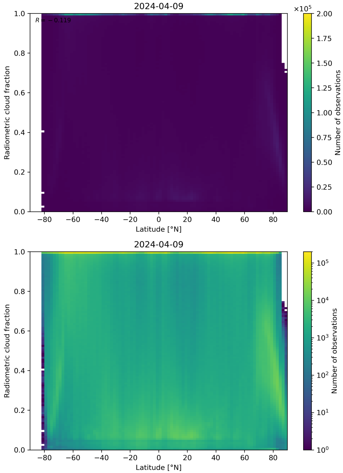
Figure 92: Scatter density plot of “Latitude” against “Radiometric cloud fraction” for 2024-04-08 to 2024-04-10.
