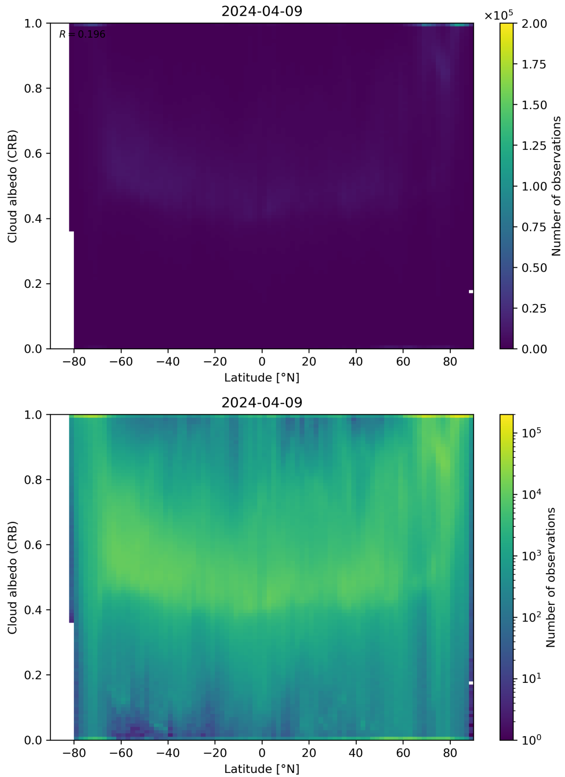
Figure 91: Scatter density plot of “Latitude” against “Cloud albedo (CRB)” for 2024-04-08 to 2024-04-10.
