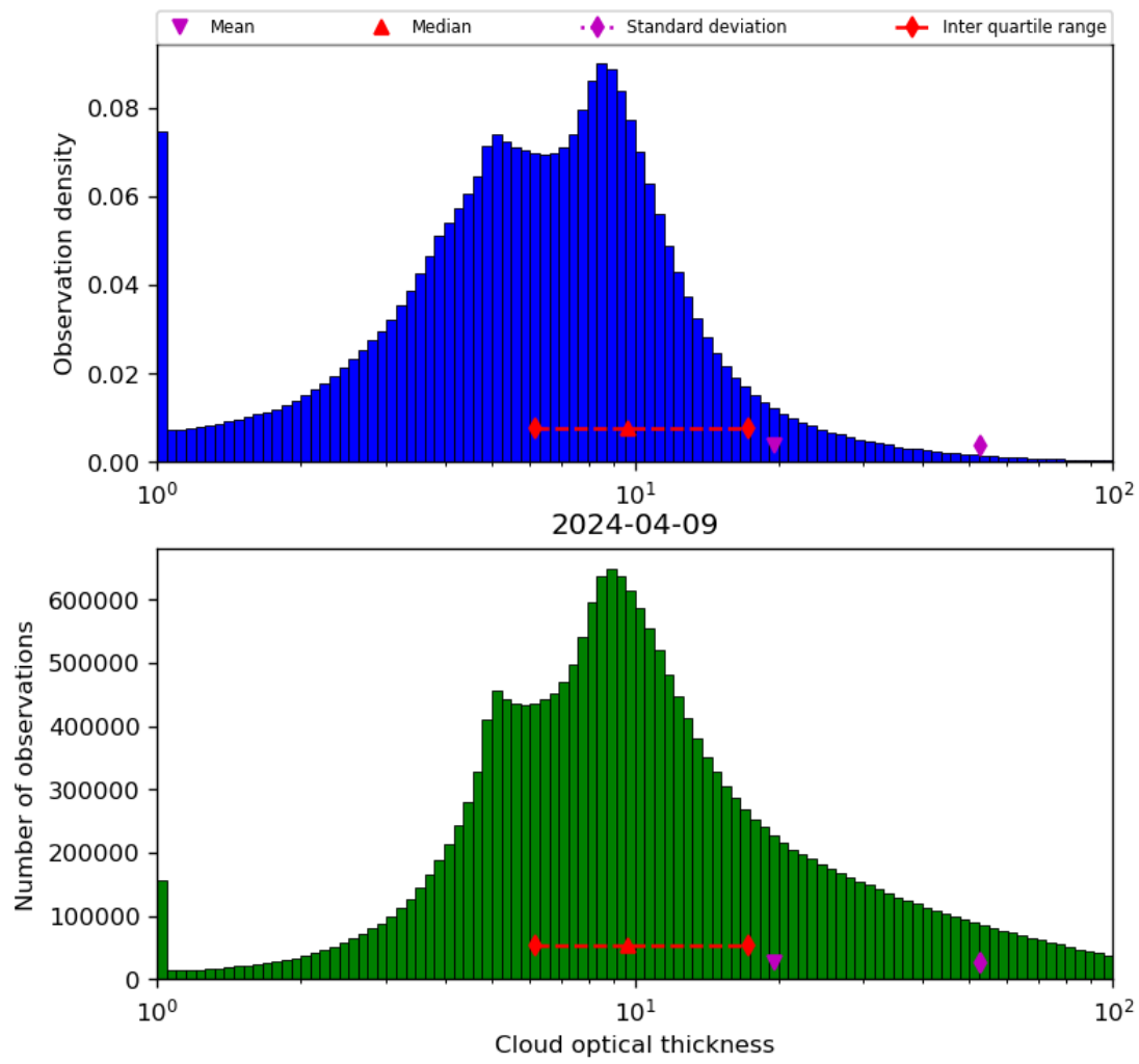
Figure 41: Histogram of “Cloud optical thickness” for 2024-04-08 to 2024-04-10
