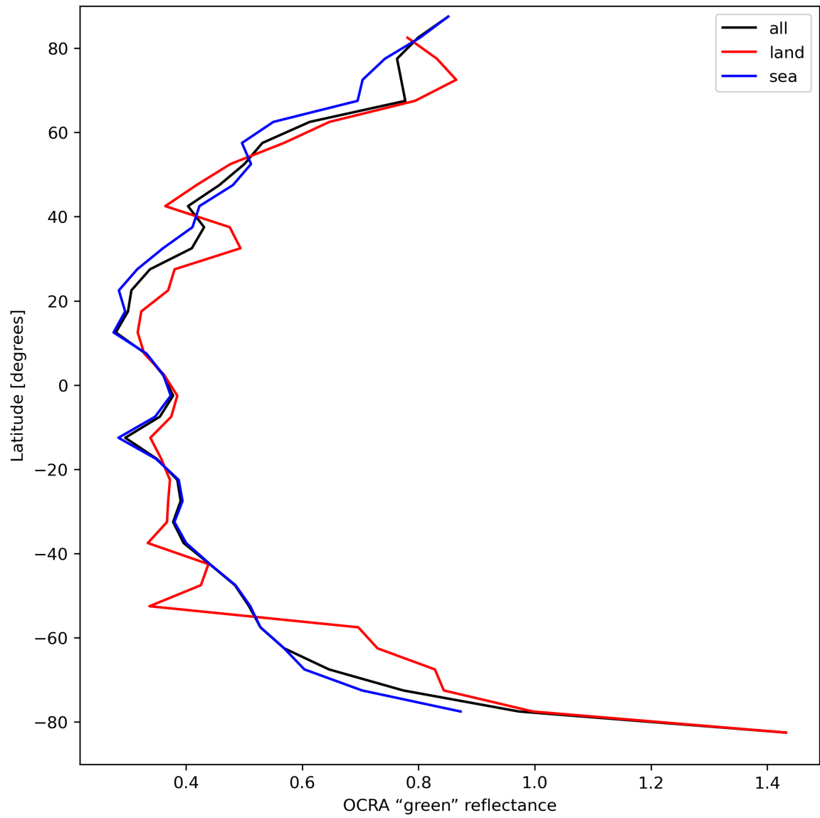
Figure 36: Zonal average of “OCRA “green” reflectance” for 2024-04-08 to 2024-04-10.
