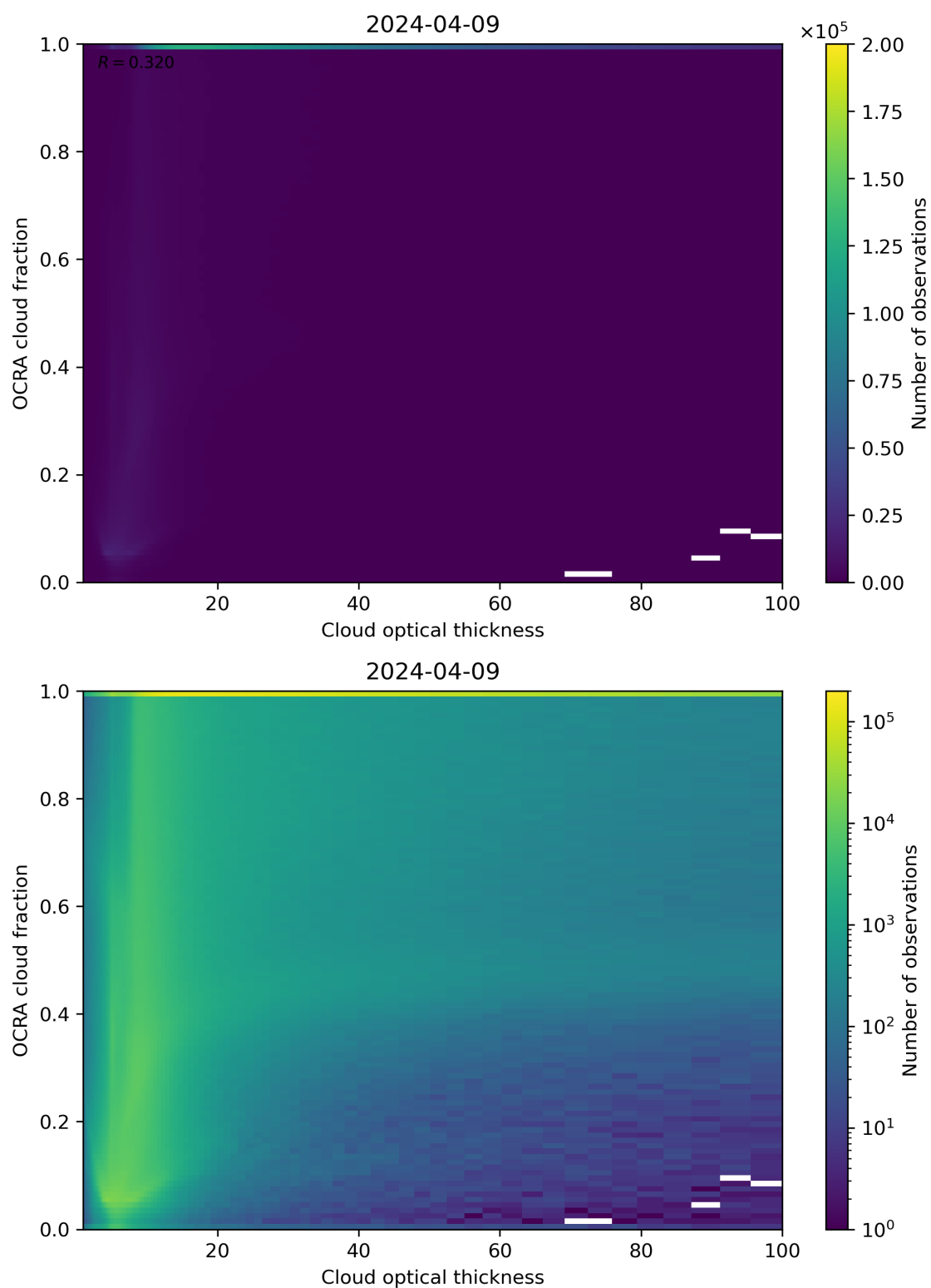
Figure 83: Scatter density plot of “Cloud optical thickness” against “OCRA cloud fraction” for 2024-04-08 to 2024-04-10.
