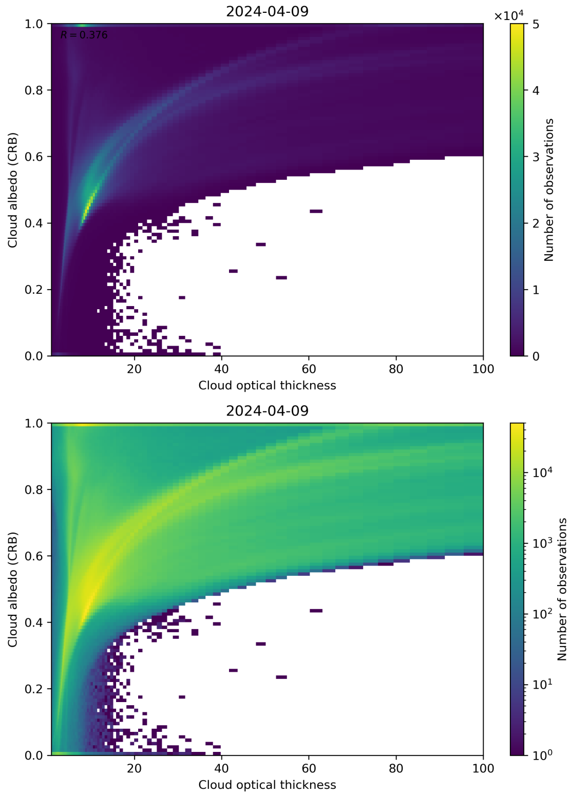
Figure 82: Scatter density plot of “Cloud optical thickness” against “Cloud albedo (CRB)” for 2024-04-08 to 2024-04-10.
