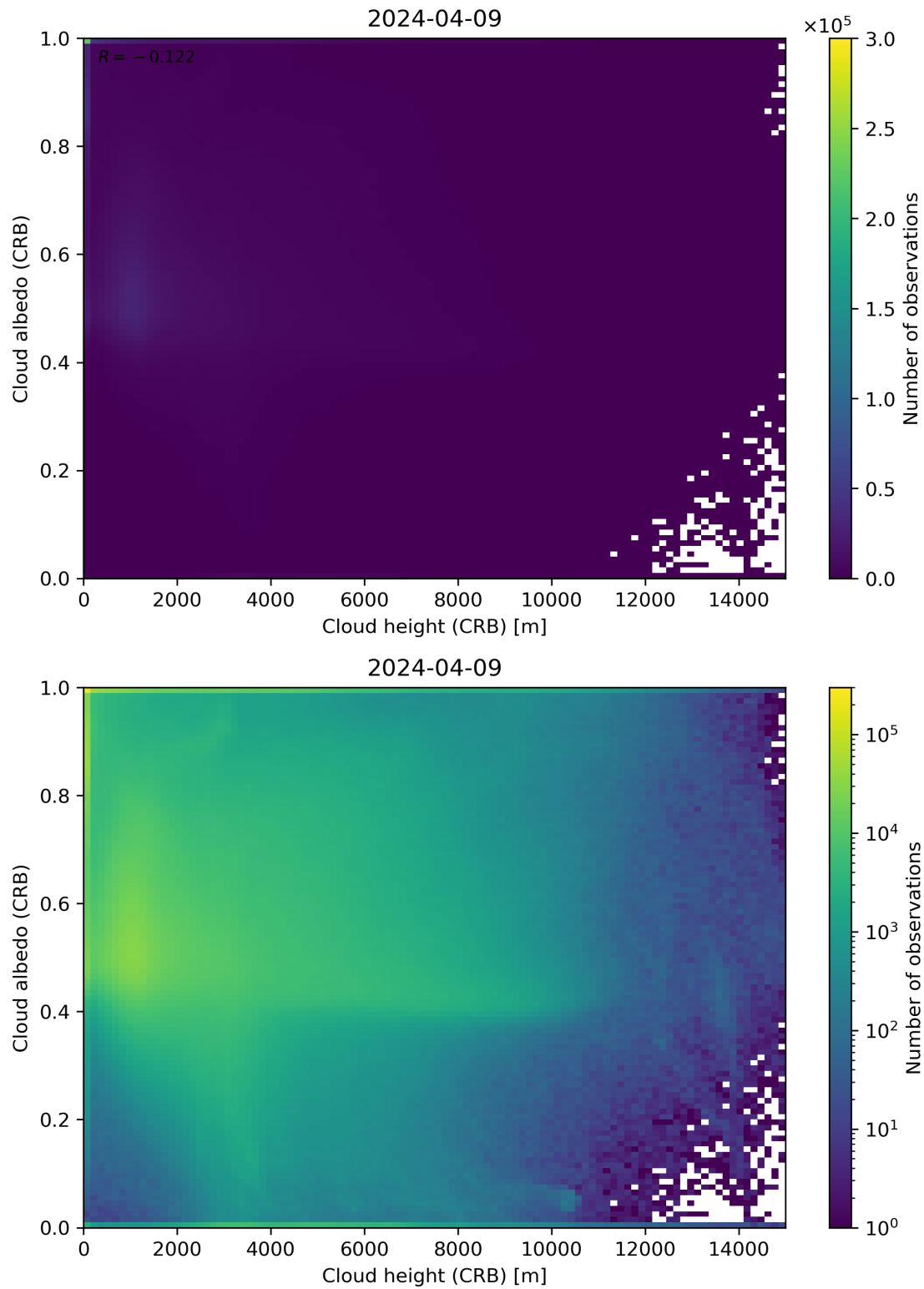
Figure 80: Scatter density plot of “Cloud height (CRB)” against “Cloud albedo (CRB)” for 2024-04-08 to 2024-04-10.
