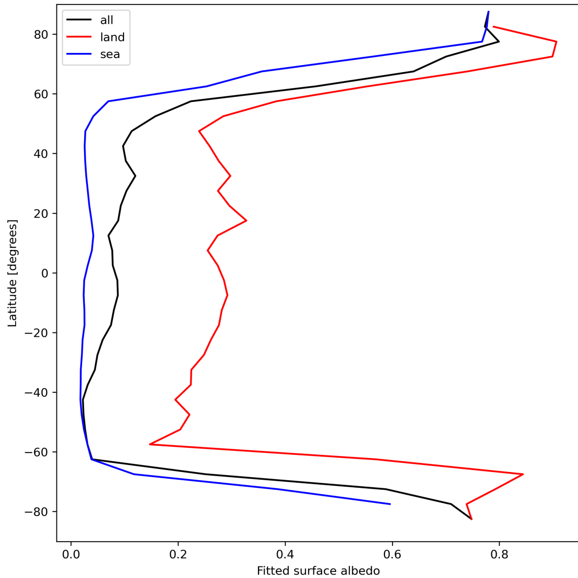
Figure 29: Zonal average of “Fitted surface albedo” for 2024-04-08 to 2024-04-10.
