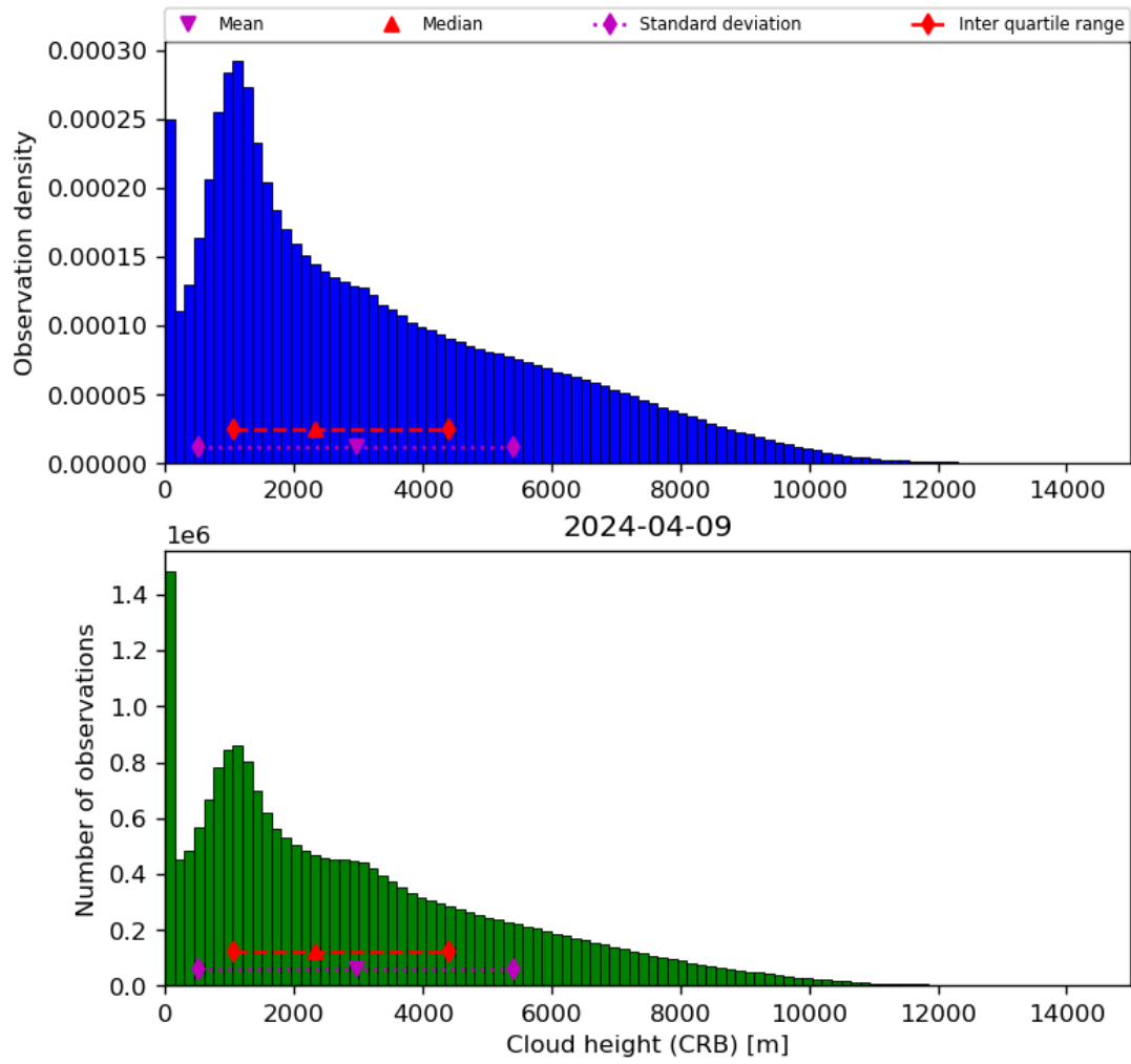
Figure 43: Histogram of “Cloud height (CRB)” for 2024-04-08 to 2024-04-10
