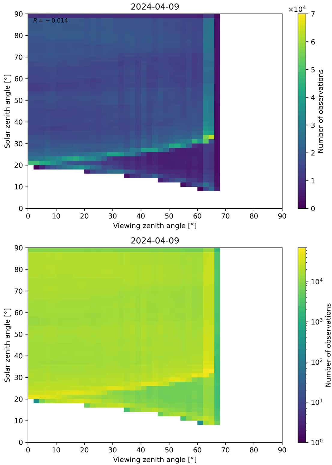
Figure 114: Scatter density plot of “Viewing zenith angle” against “Solar zenith angle” for 2024-04-08 to 2024-04-10.
