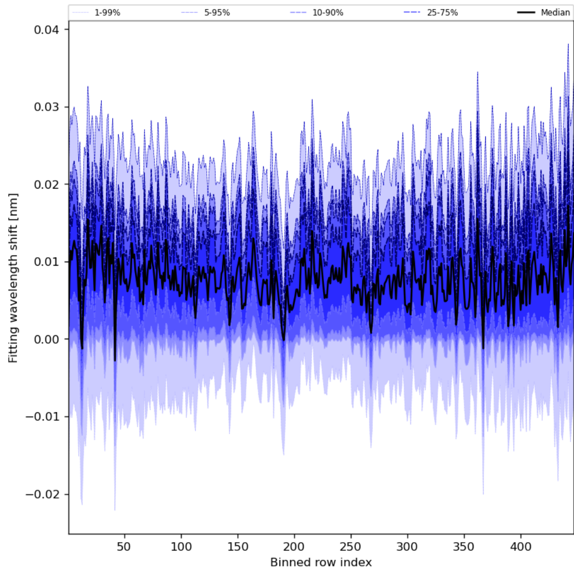
Figure 65: Along track statistics of “Fitting wavelength shift” for 2024-04-08 to 2024-04-10
