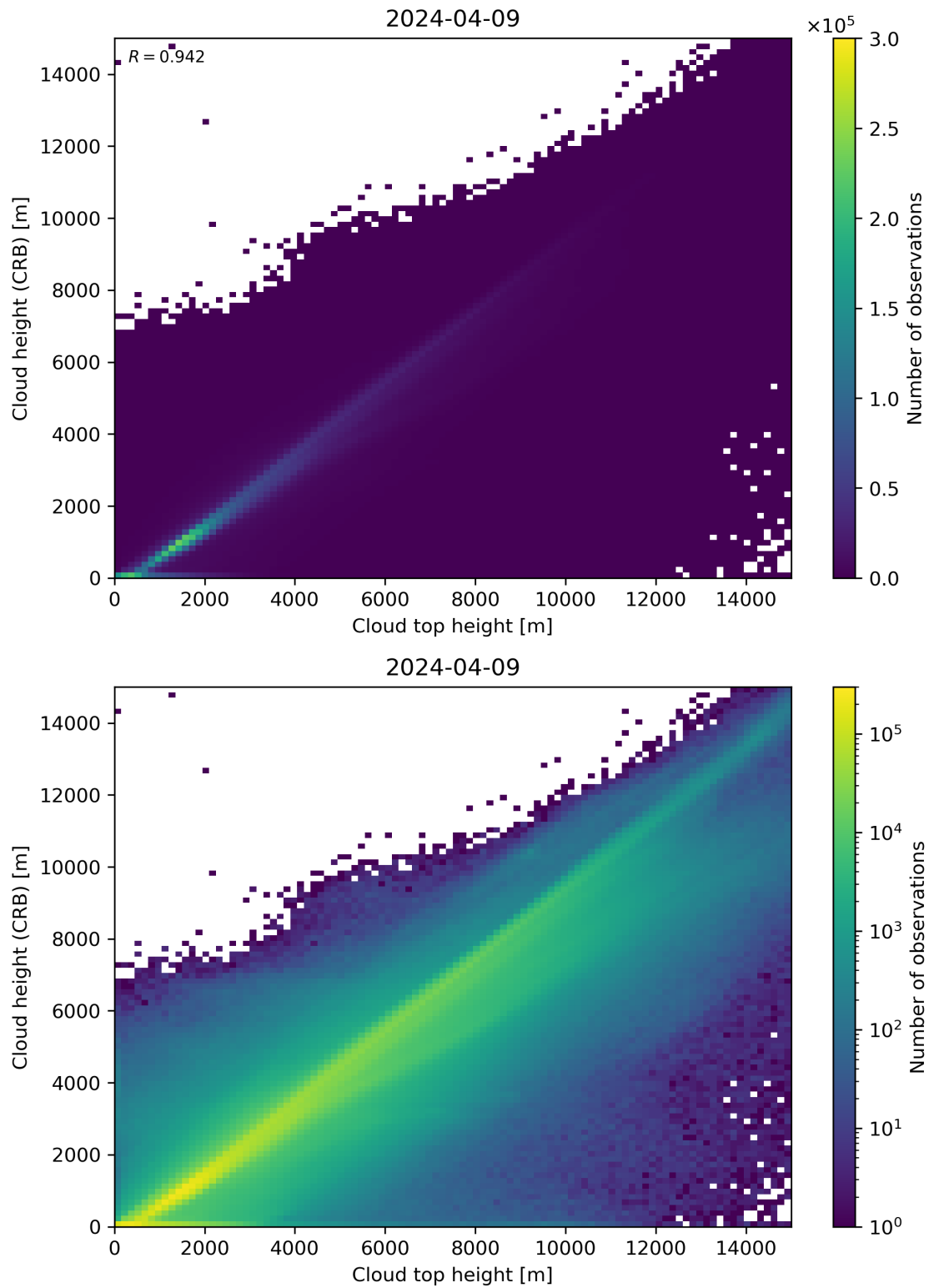
Figure 89: Scatter density plot of “Cloud top height” against “Cloud height (CRB)” for 2024-04-08 to 2024-04-10.
