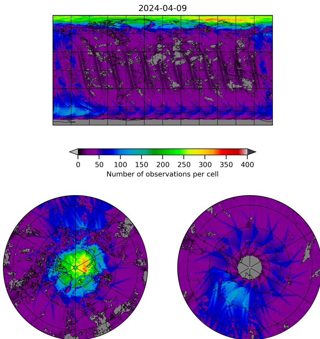
Figure 21: Map of the number of observations for 2024-04-08 to 2024-04-10
