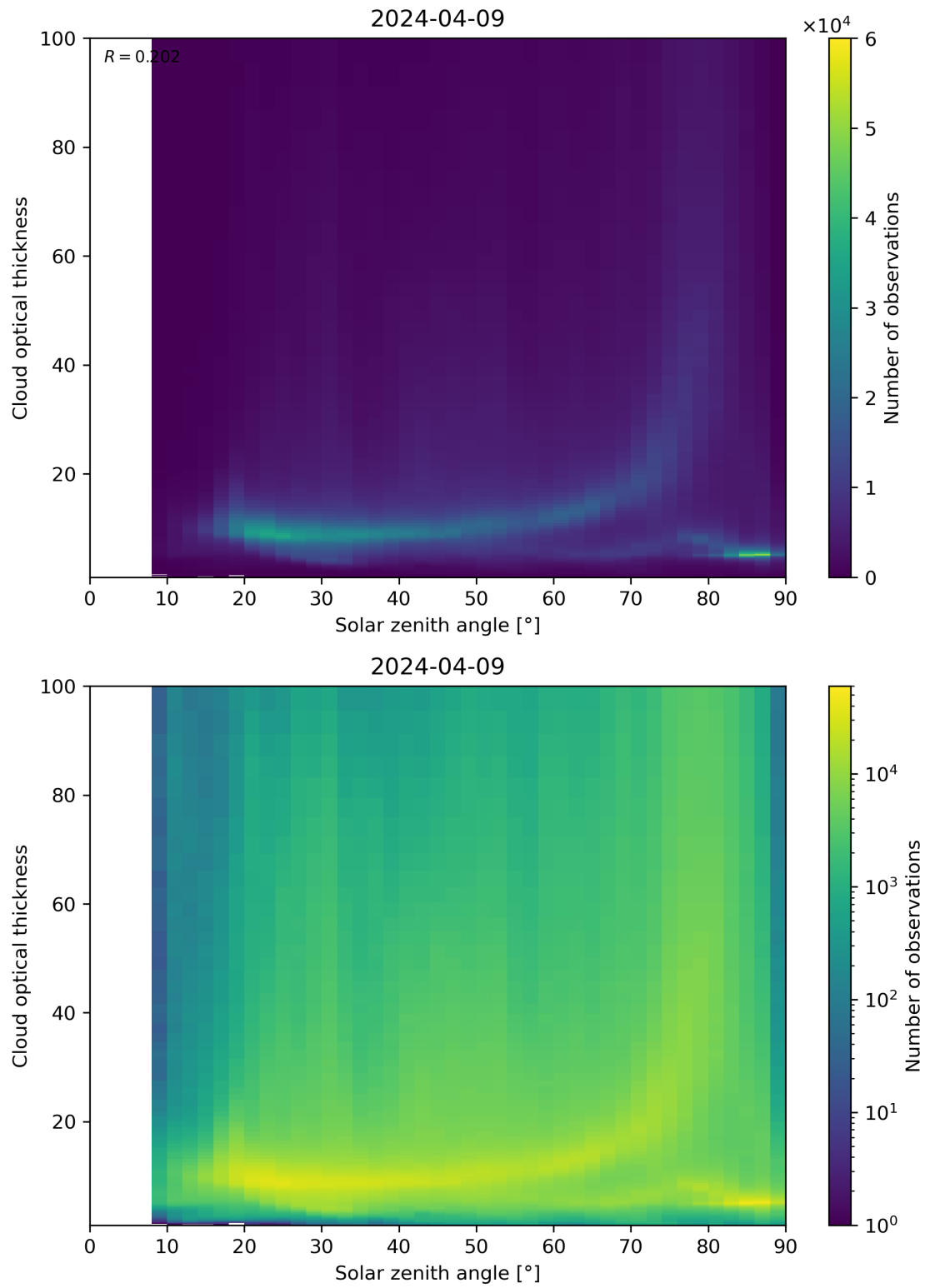
Figure 103: Scatter density plot of “Solar zenith angle” against “Cloud optical thickness” for 2024-04-08 to 2024-04-10.
