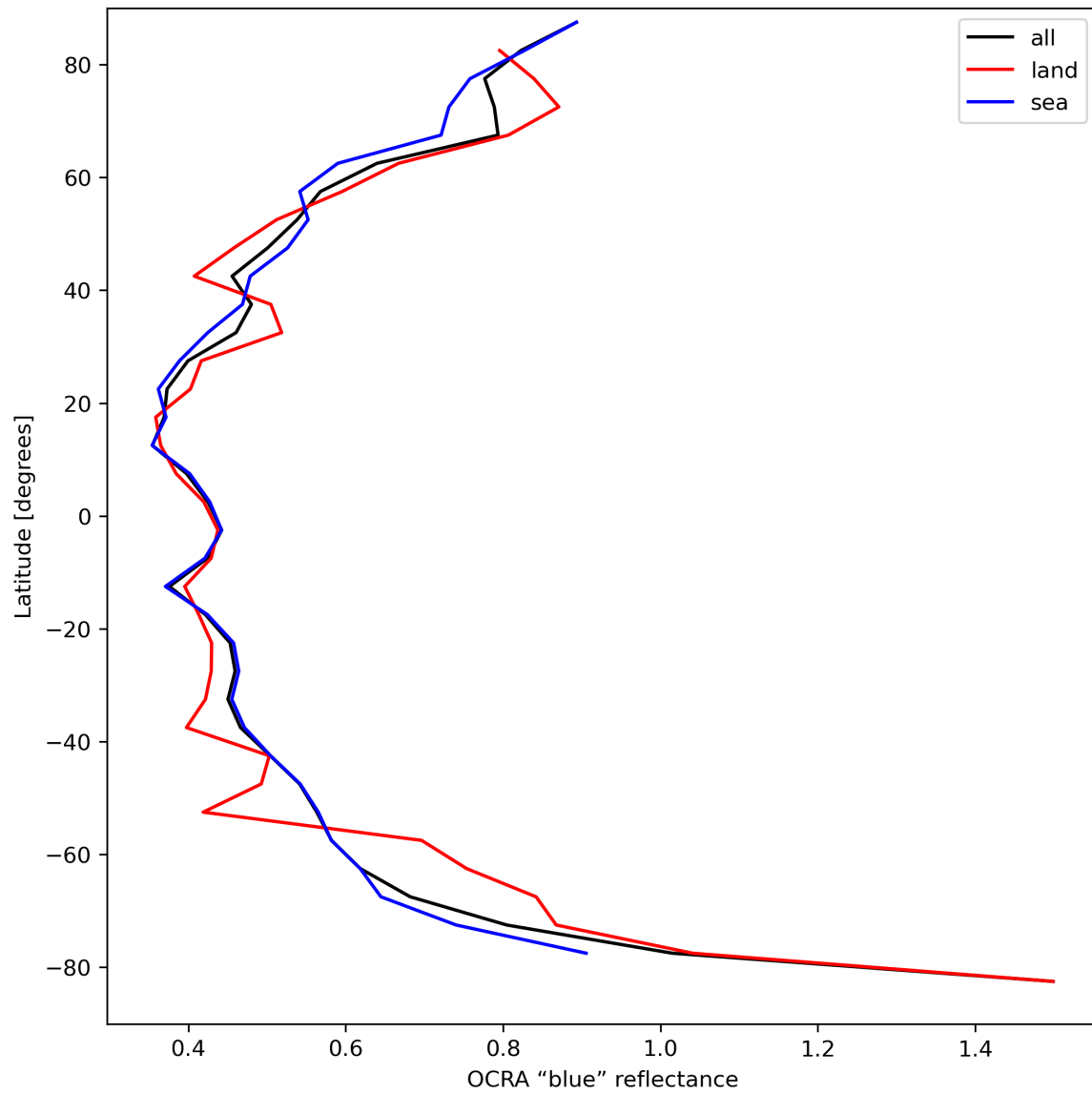
Figure 35: Zonal average of “OCRA “blue” reflectance” for 2024-04-08 to 2024-04-10.
