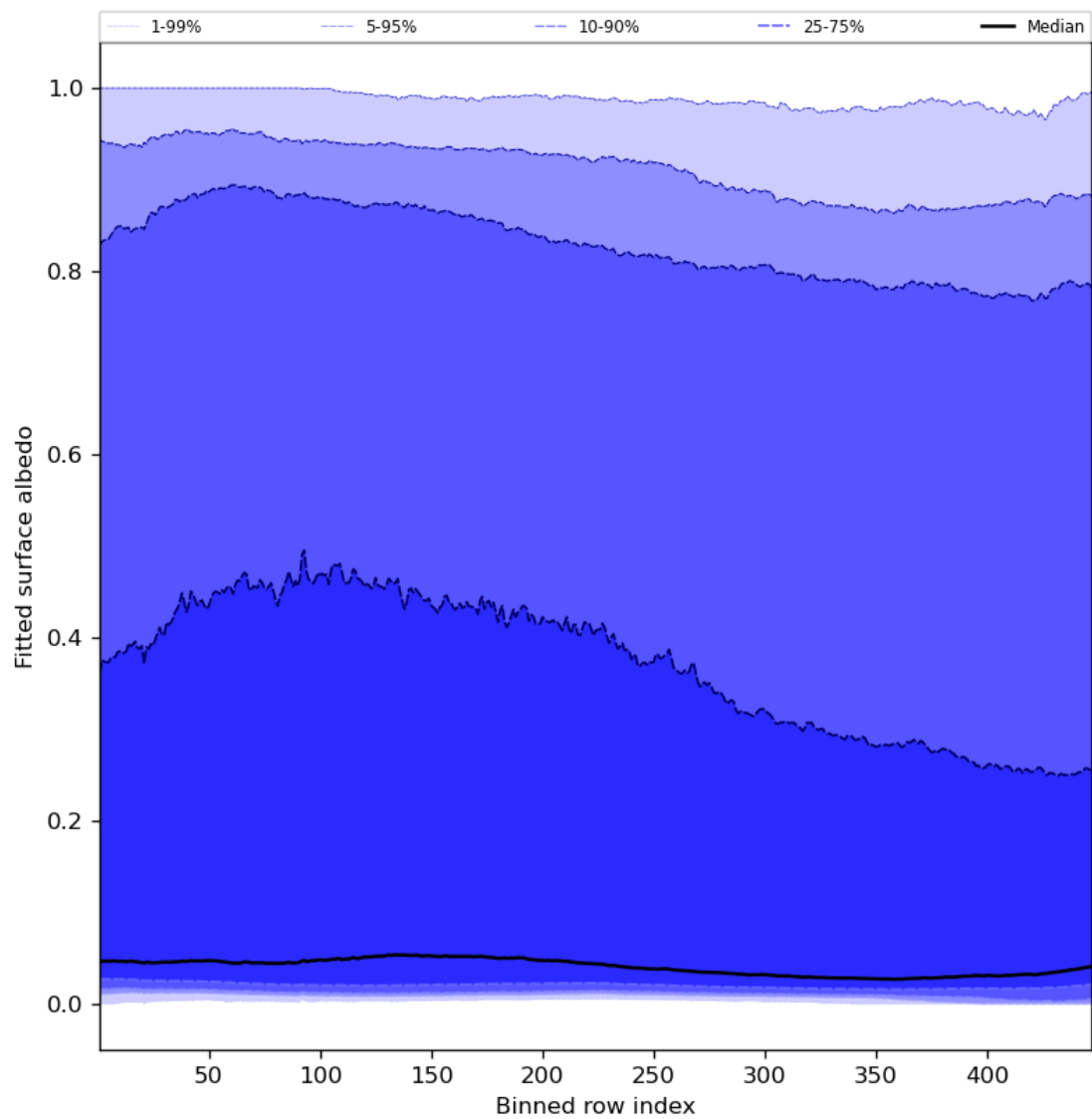
Figure 61: Along track statistics of “Fitted surface albedo” for 2024-04-08 to 2024-04-10
