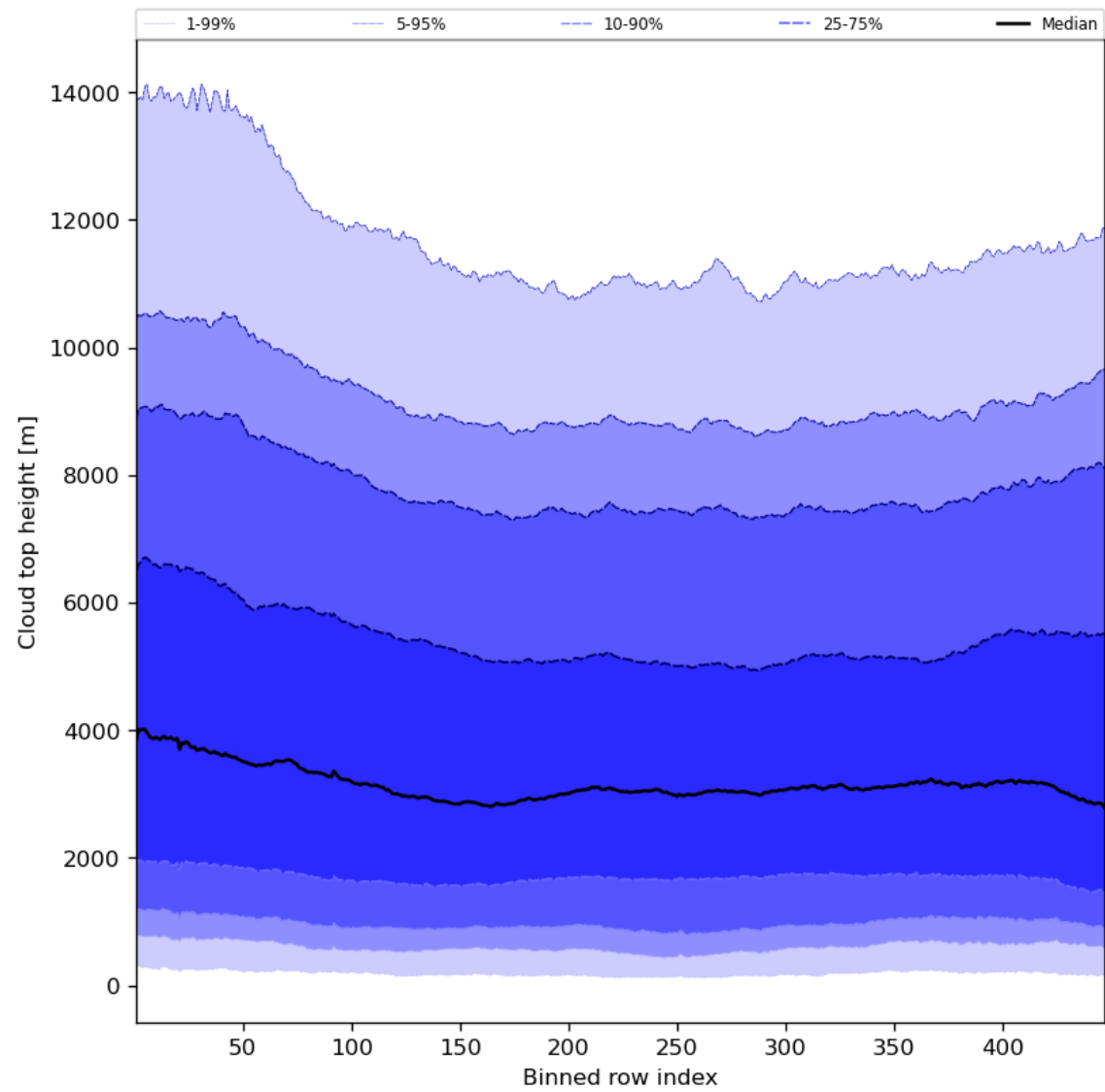
Figure 56: Along track statistics of “Cloud top height” for 2024-04-08 to 2024-04-10
