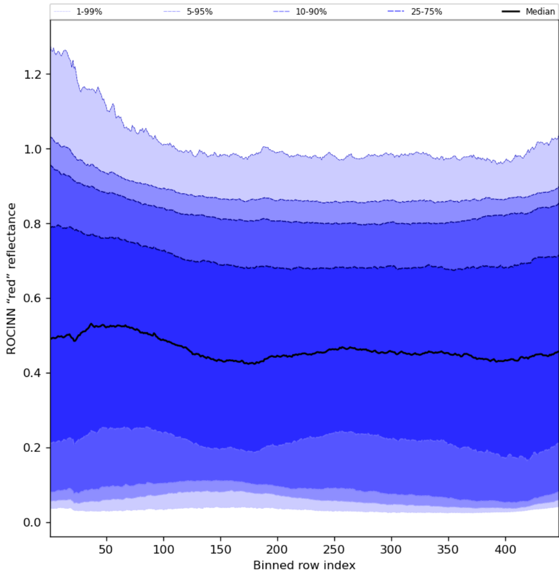
Figure 69: Along track statistics of “ROCINN “red” reflectance” for 2024-04-08 to 2024-04-10
