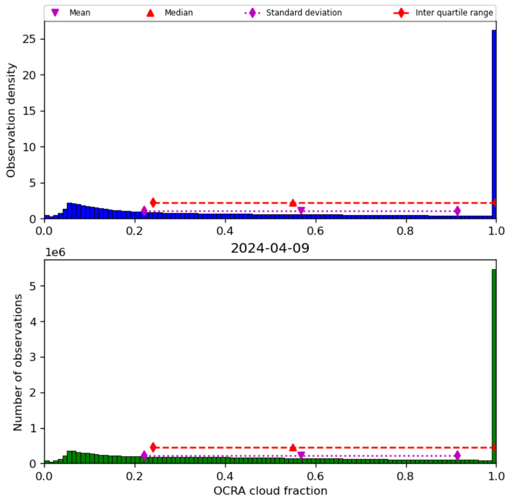
Figure 50: Histogram of “OCRA cloud fraction” for 2024-04-08 to 2024-04-10
