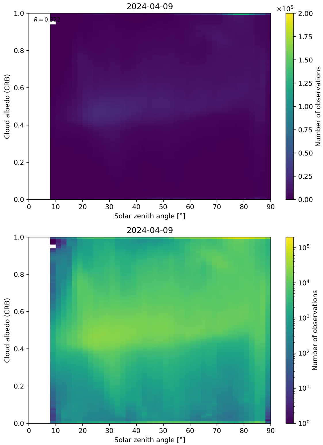
Figure 98: Scatter density plot of “Solar zenith angle” against “Cloud albedo (CRB)” for 2024-04-08 to 2024-04-10.
