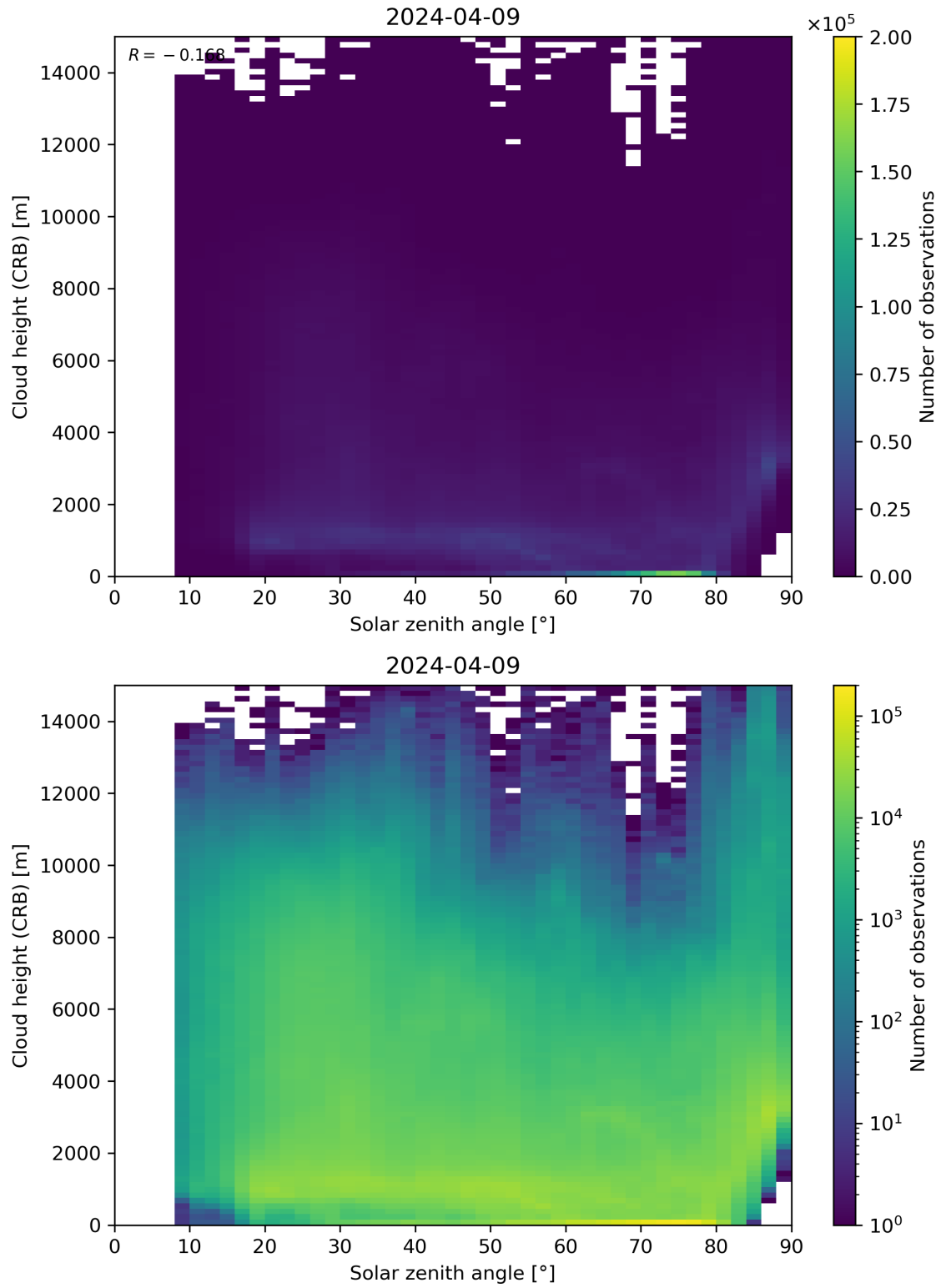
Figure 102: Scatter density plot of “Solar zenith angle” against “Cloud height (CRB)” for 2024-04-08 to 2024-04-10.
