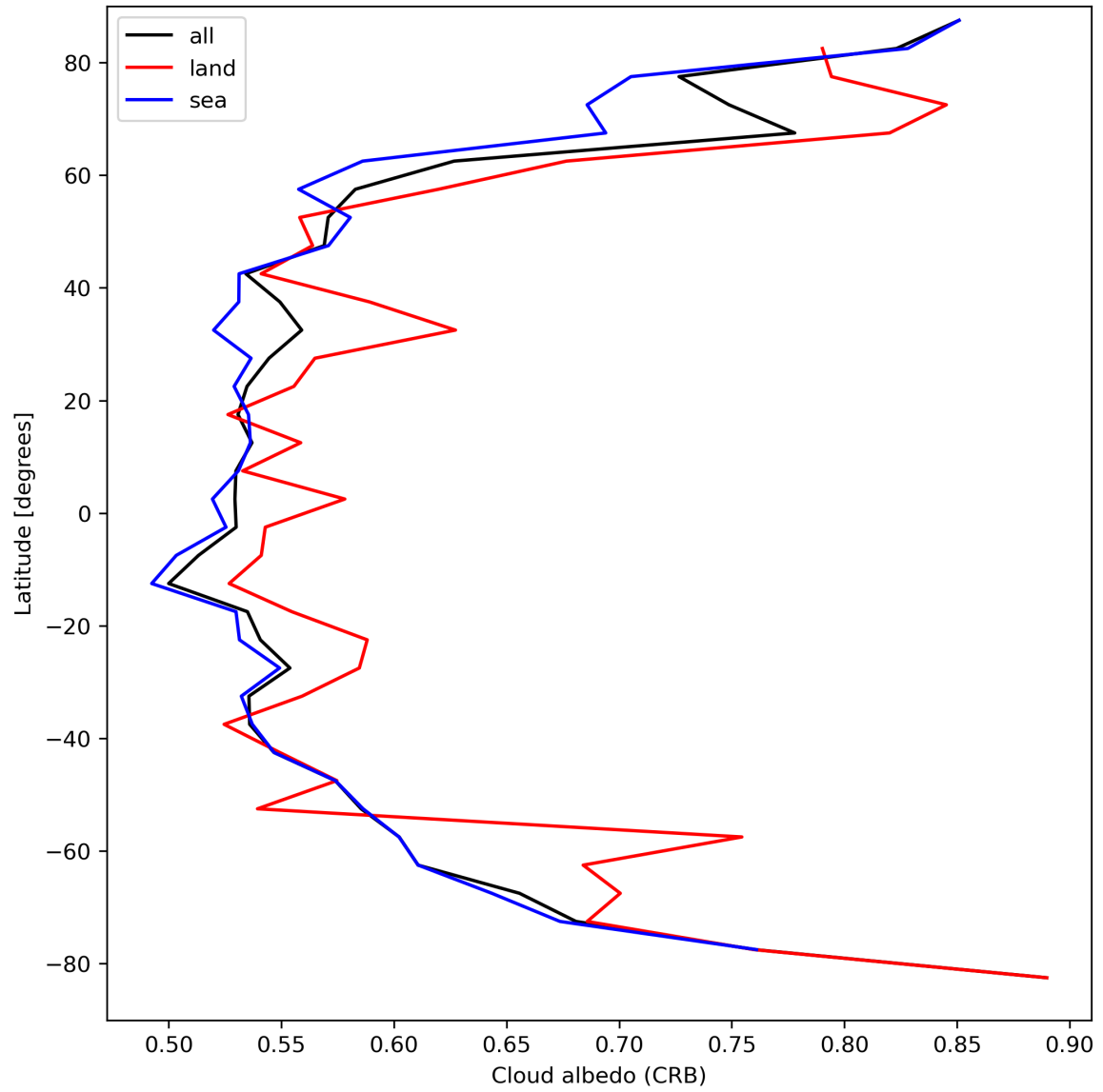
Figure 28: Zonal average of “Cloud albedo (CRB)” for 2024-04-08 to 2024-04-10.
