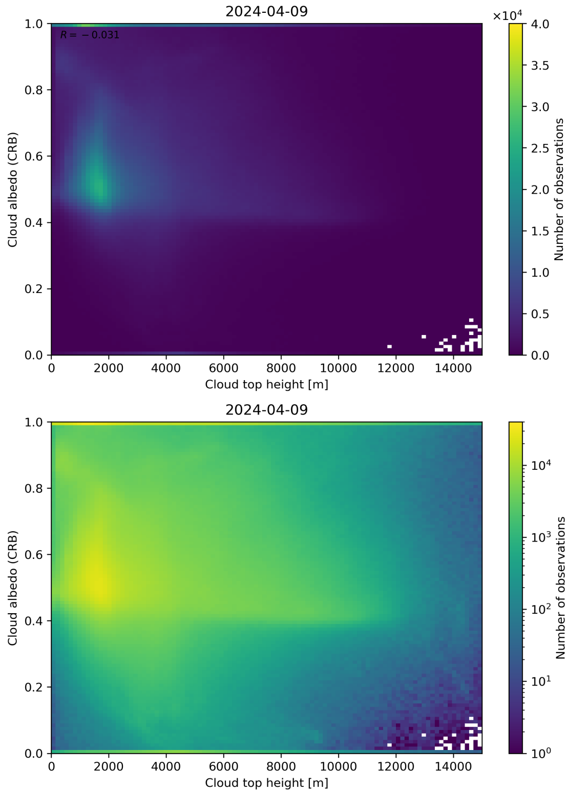
Figure 86: Scatter density plot of “Cloud top height” against “Cloud albedo (CRB)” for 2024-04-08 to 2024-04-10.
