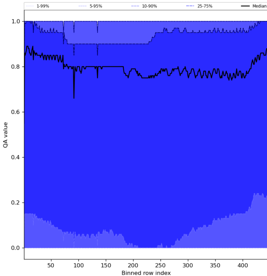
Figure 54: Along track statistics of “QA value” for 2024-04-08 to 2024-04-10
