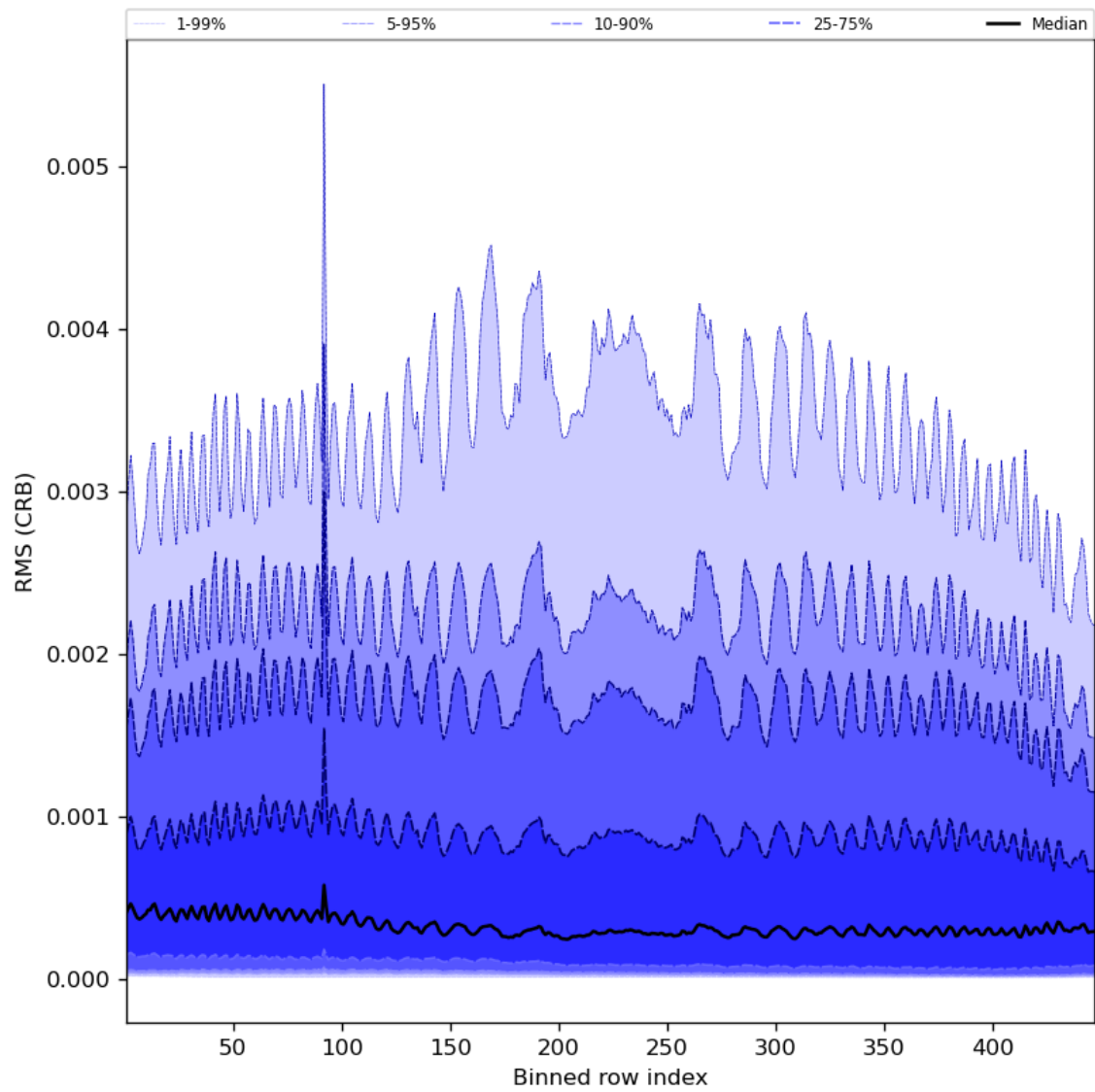
Figure 64: Along track statistics of “RMS (CRB)” for 2024-04-10 to 2024-04-11
