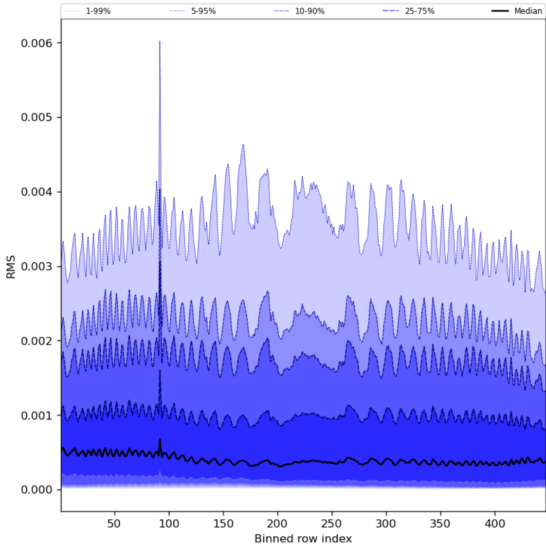
Figure 63: Along track statistics of “RMS” for 2024-04-10 to 2024-04-11
