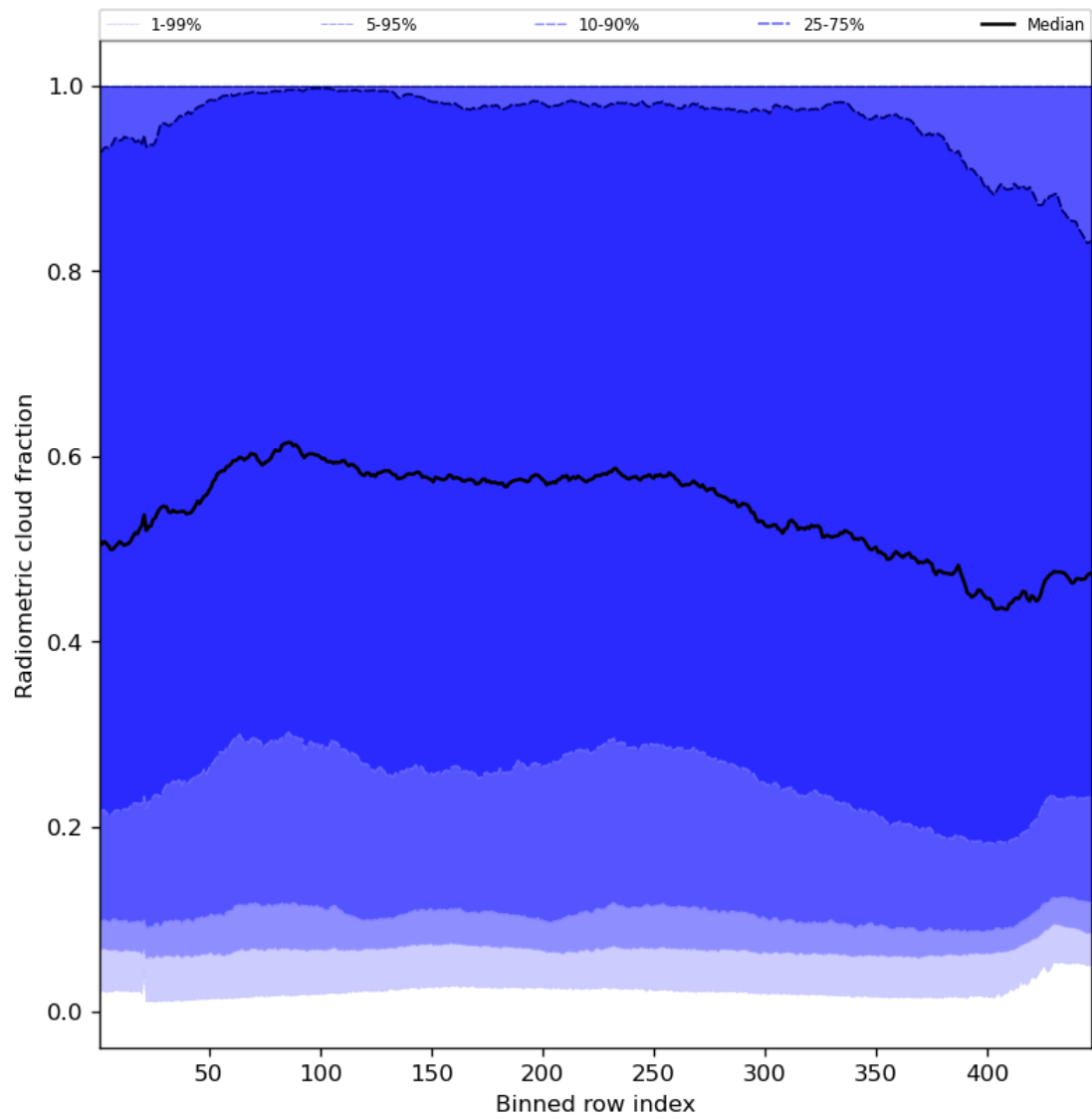
Figure 55: Along track statistics of “Radiometric cloud fraction” for 2024-04-10 to 2024-04-11
