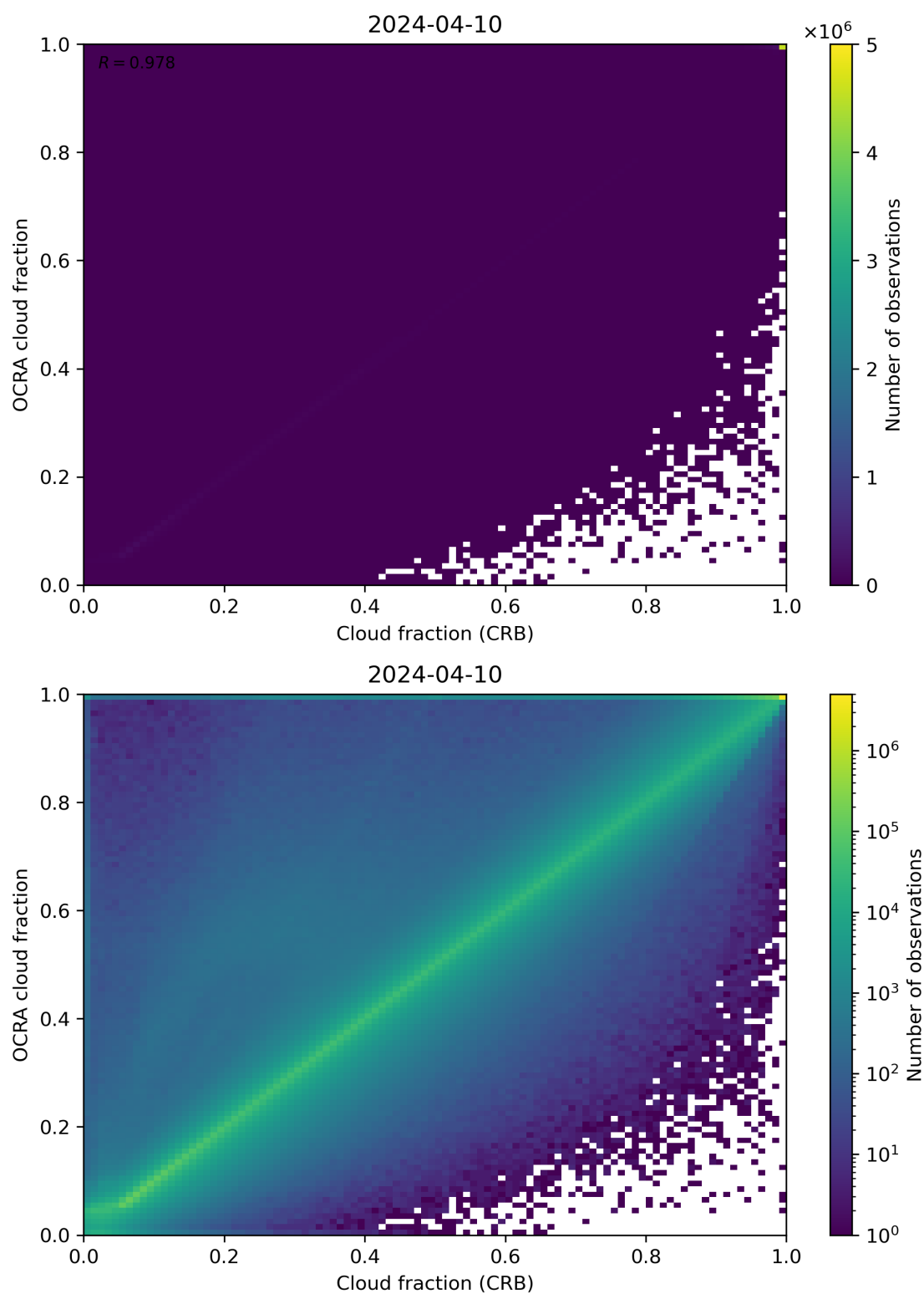
Figure 78: Scatter density plot of “Cloud fraction (CRB)” against “OCRA cloud fraction” for 2024-04-10 to 2024-04-11.
