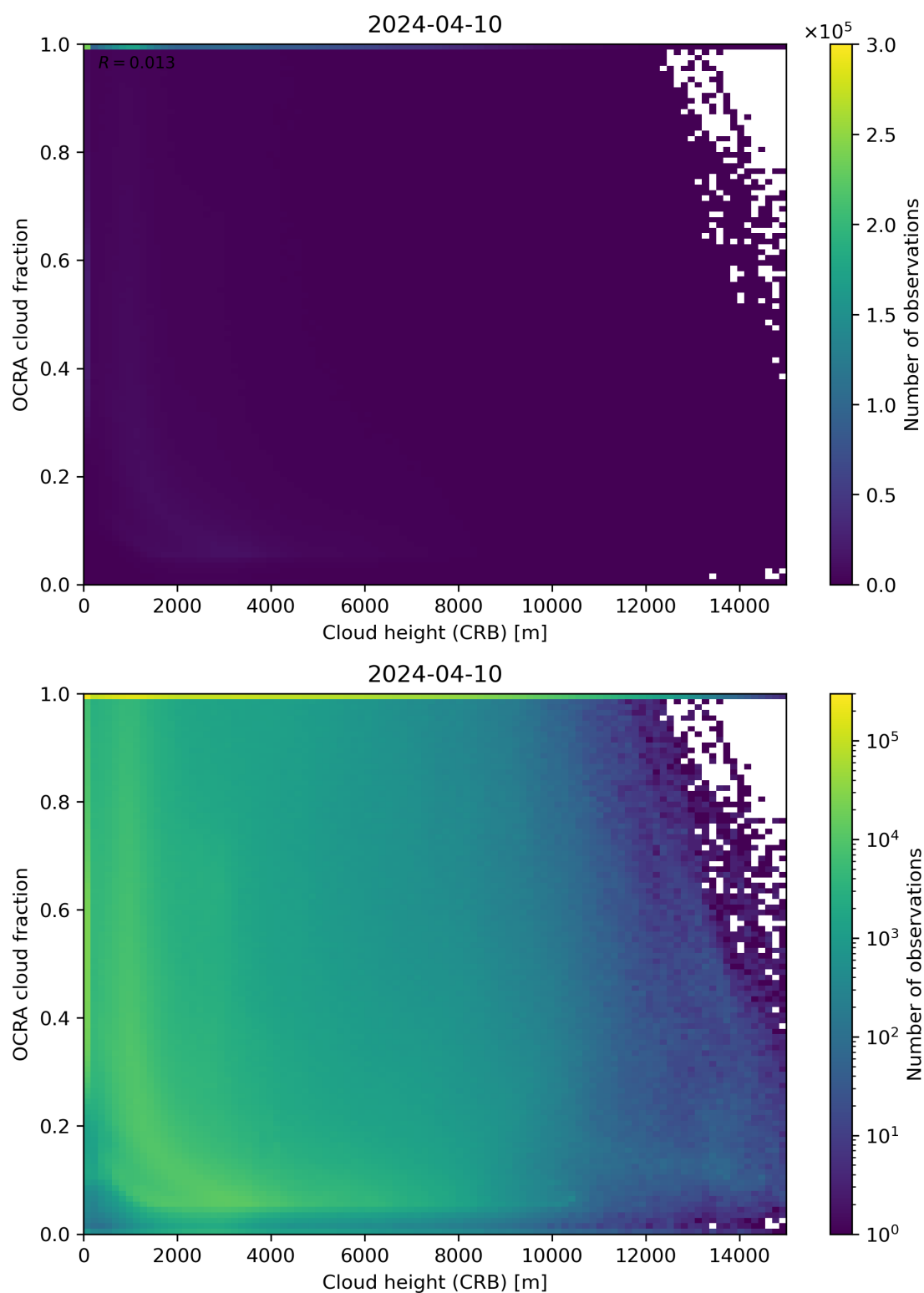
Figure 81: Scatter density plot of “Cloud height (CRB)” against “OCRA cloud fraction” for 2024-04-10 to 2024-04-11.
