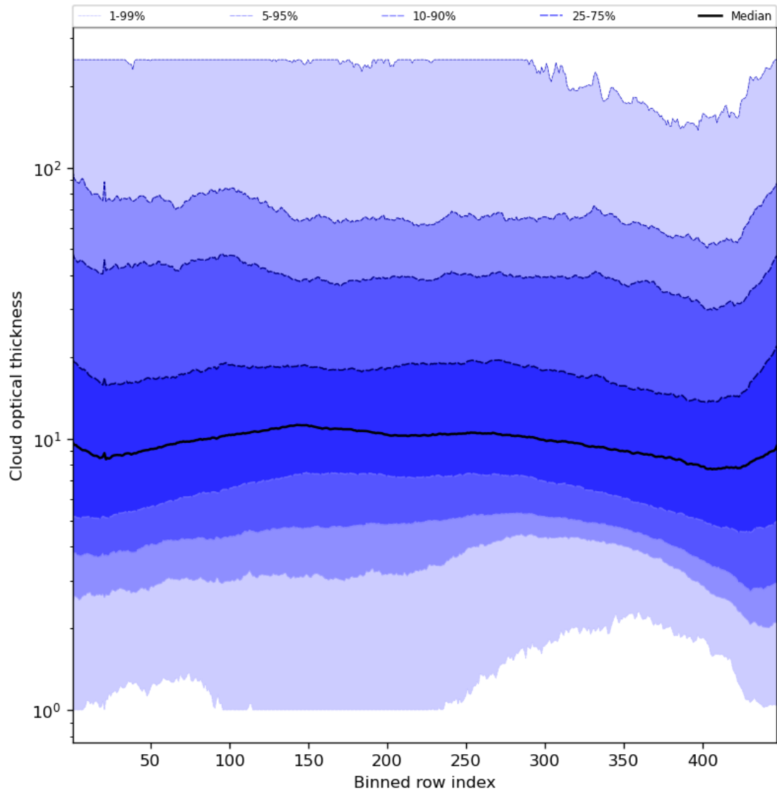
Figure 57: Along track statistics of “Cloud optical thickness” for 2024-04-10 to 2024-04-11
