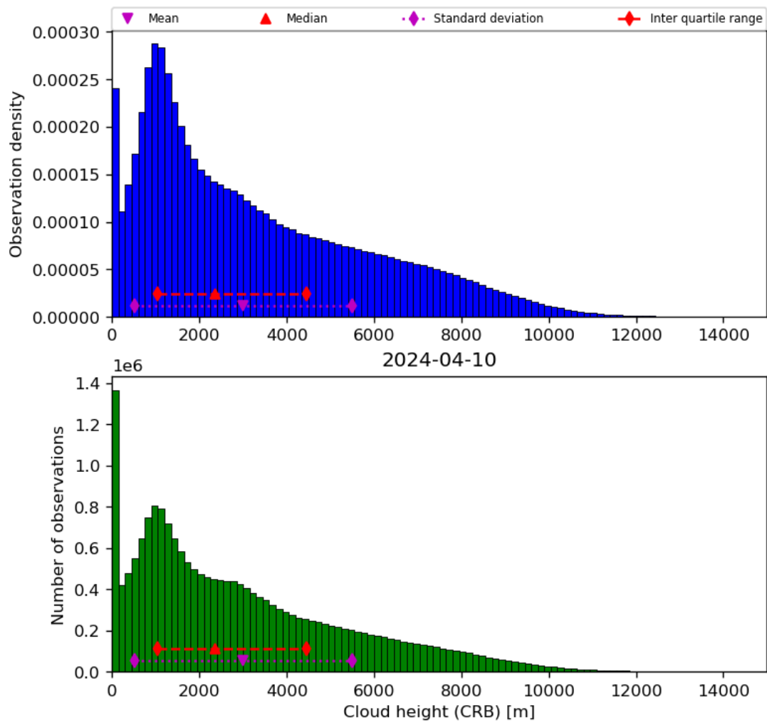
Figure 43: Histogram of “Cloud height (CRB)” for 2024-04-10 to 2024-04-11
