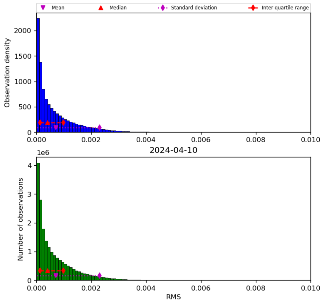
Figure 47: Histogram of “RMS” for 2024-04-10 to 2024-04-11
