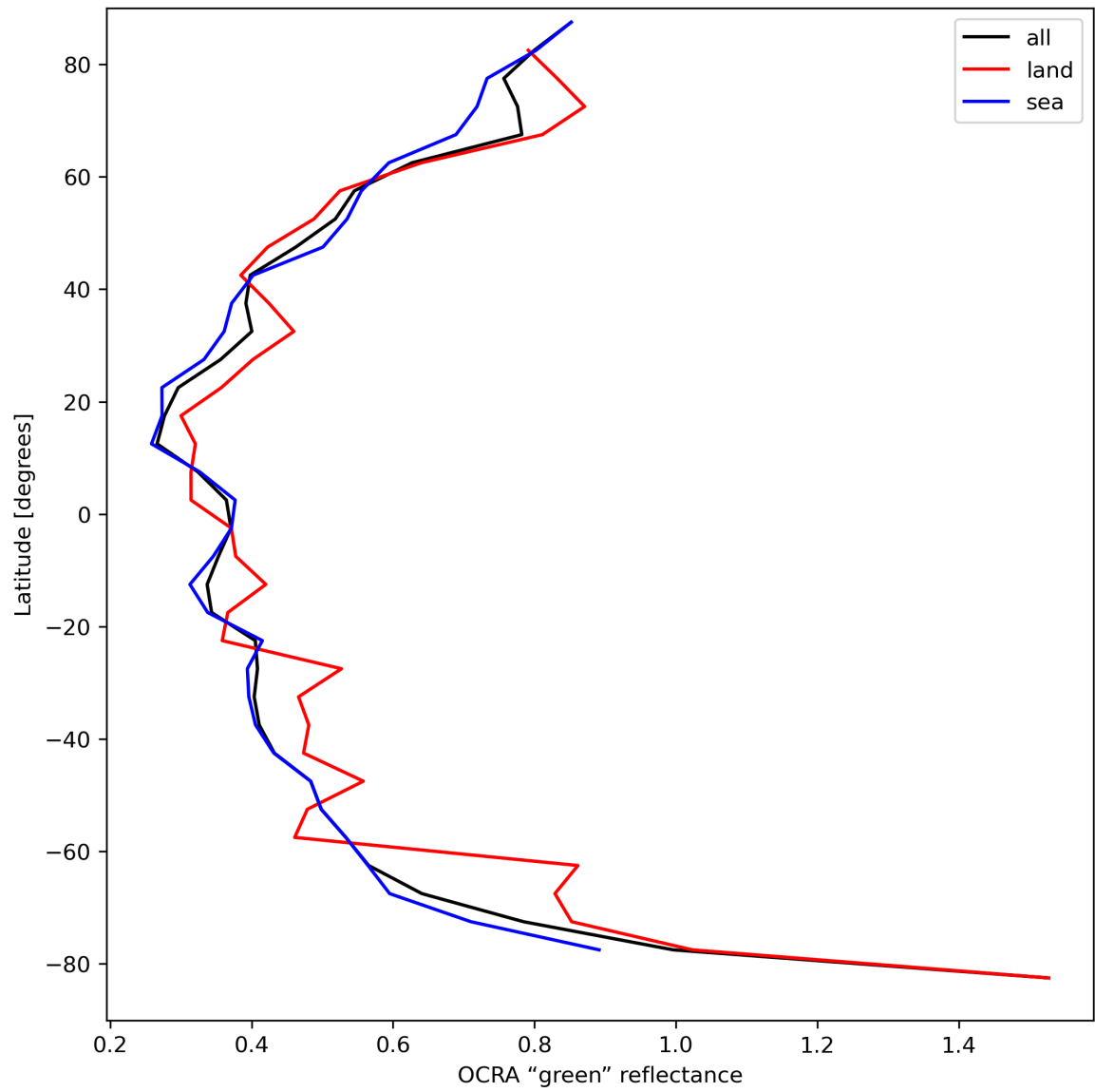
Figure 36: Zonal average of “OCRA “green” reflectance” for 2024-04-10 to 2024-04-11.
