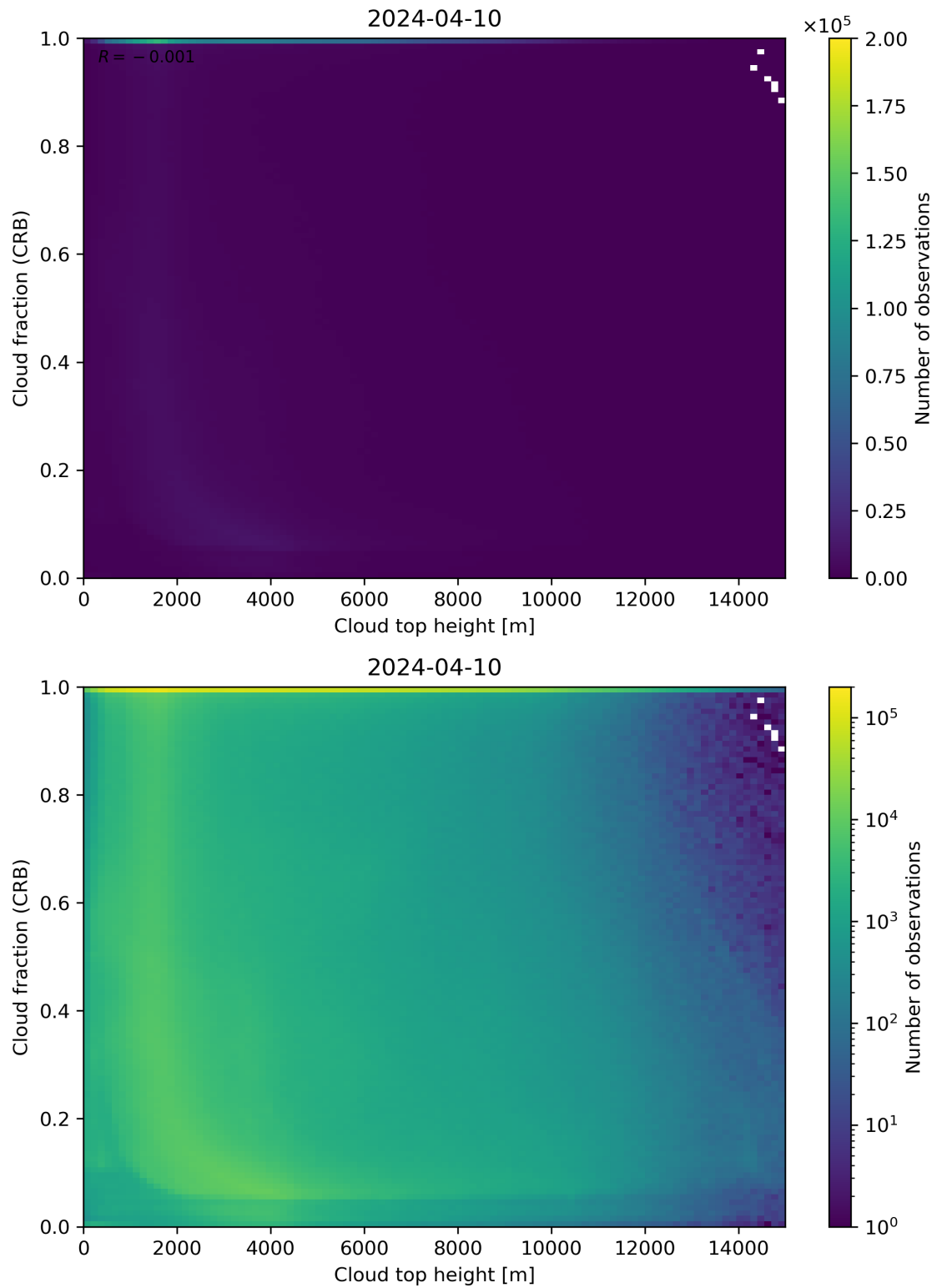
Figure 88: Scatter density plot of “Cloud top height” against “Cloud fraction (CRB)” for 2024-04-10 to 2024-04-11.
