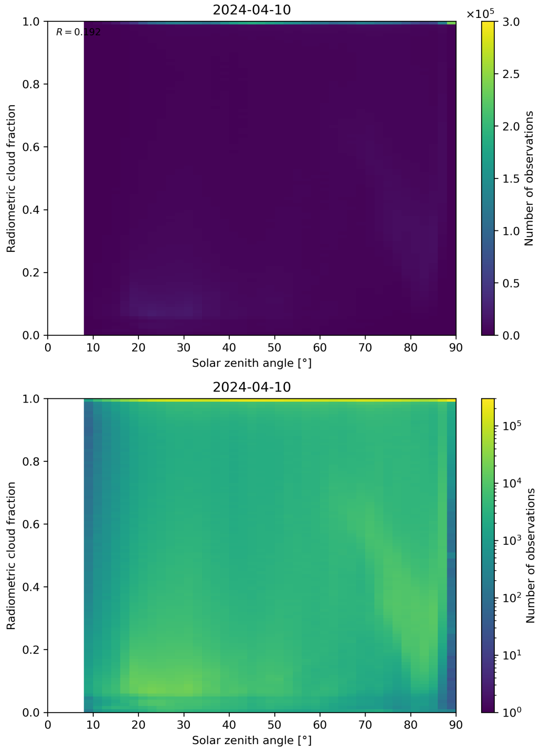
Figure 99: Scatter density plot of “Solar zenith angle” against “Radiometric cloud fraction” for 2024-04-10 to 2024-04-11.
