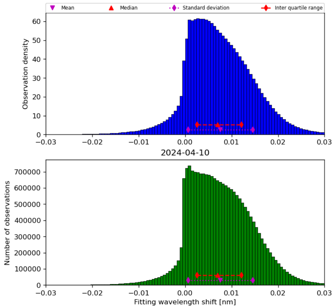
Figure 49: Histogram of “Fitting wavelength shift” for 2024-04-10 to 2024-04-11
