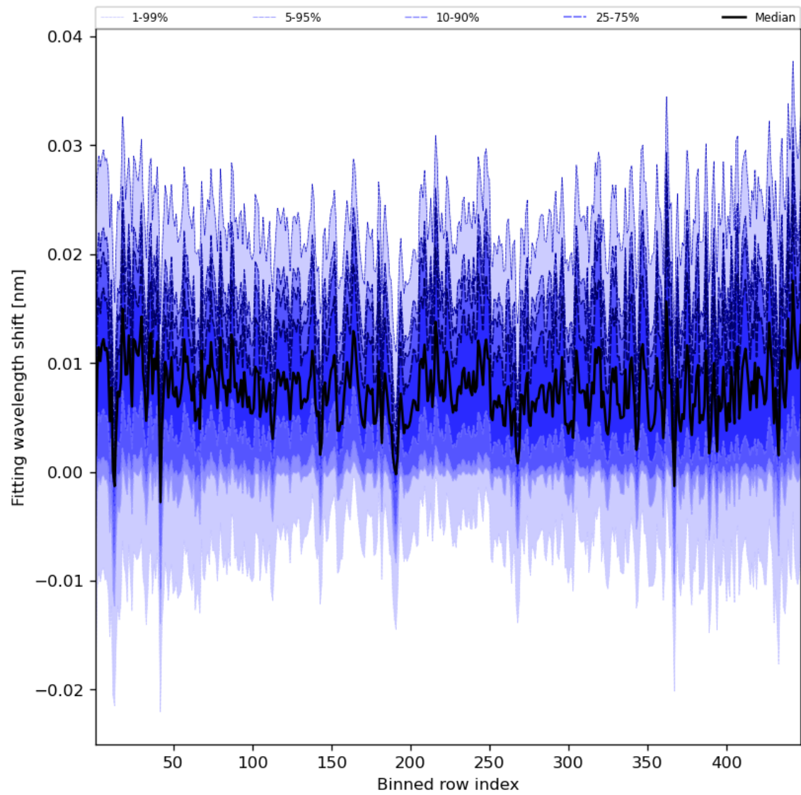
Figure 65: Along track statistics of “Fitting wavelength shift” for 2024-04-10 to 2024-04-11
