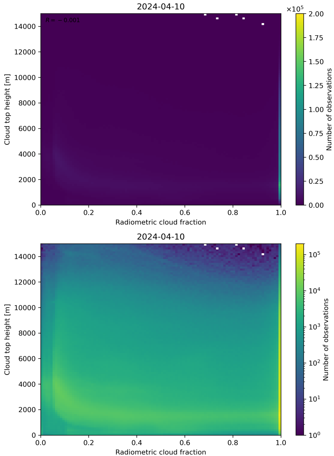
Figure 76: Scatter density plot of “Radiometric cloud fraction” against “Cloud top height” for 2024-04-10 to 2024-04-11.
