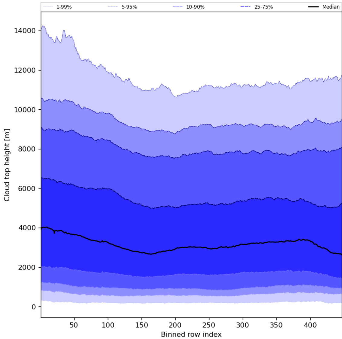
Figure 56: Along track statistics of “Cloud top height” for 2024-04-10 to 2024-04-11
