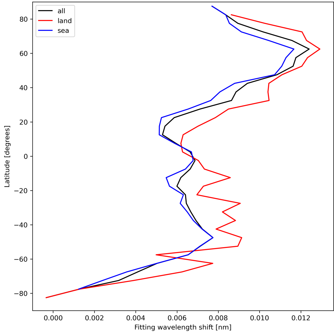
Figure 33: Zonal average of “Fitting wavelength shift” for 2024-04-10 to 2024-04-11.
