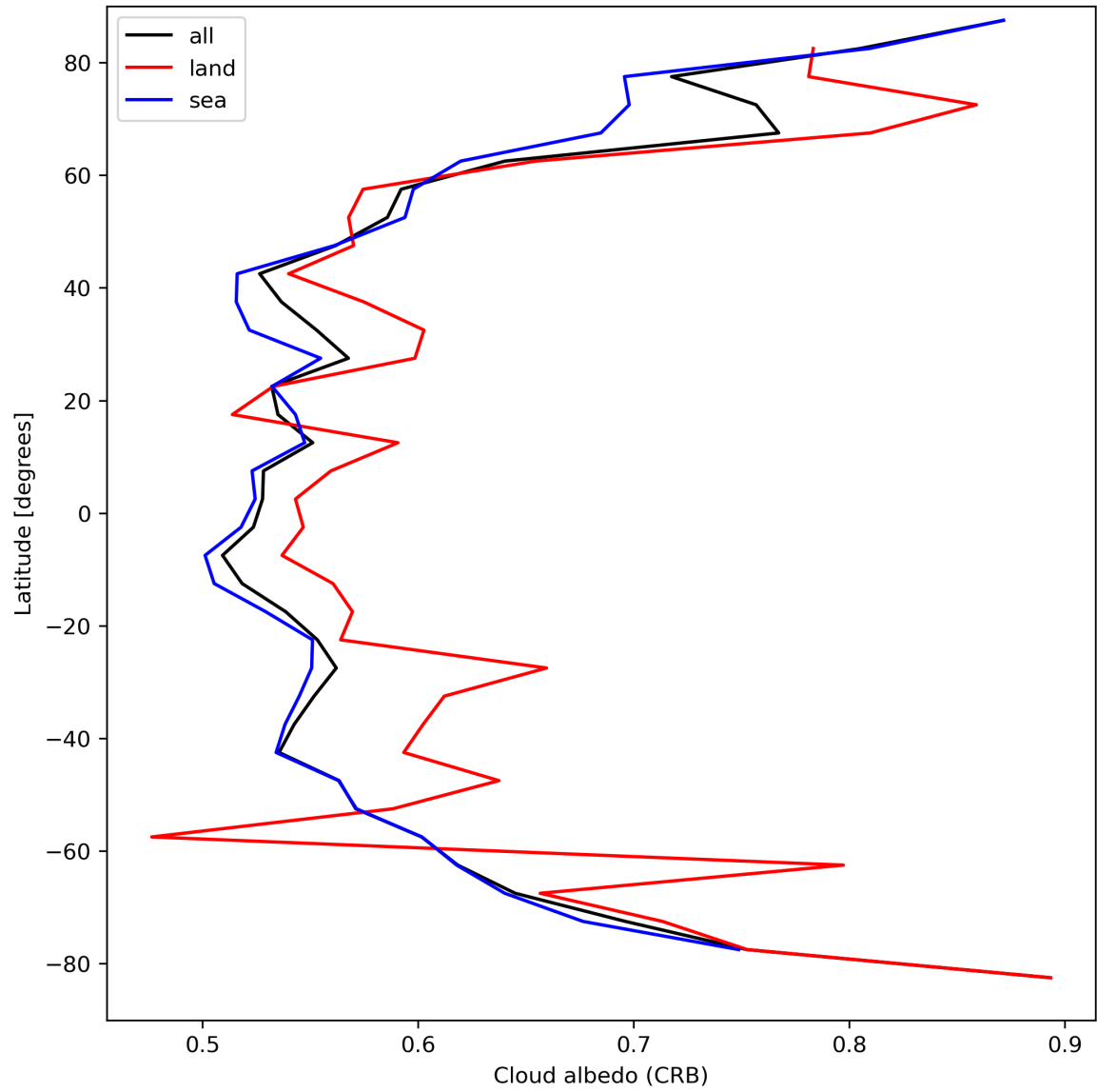
Figure 28: Zonal average of “Cloud albedo (CRB)” for 2024-04-10 to 2024-04-11.
