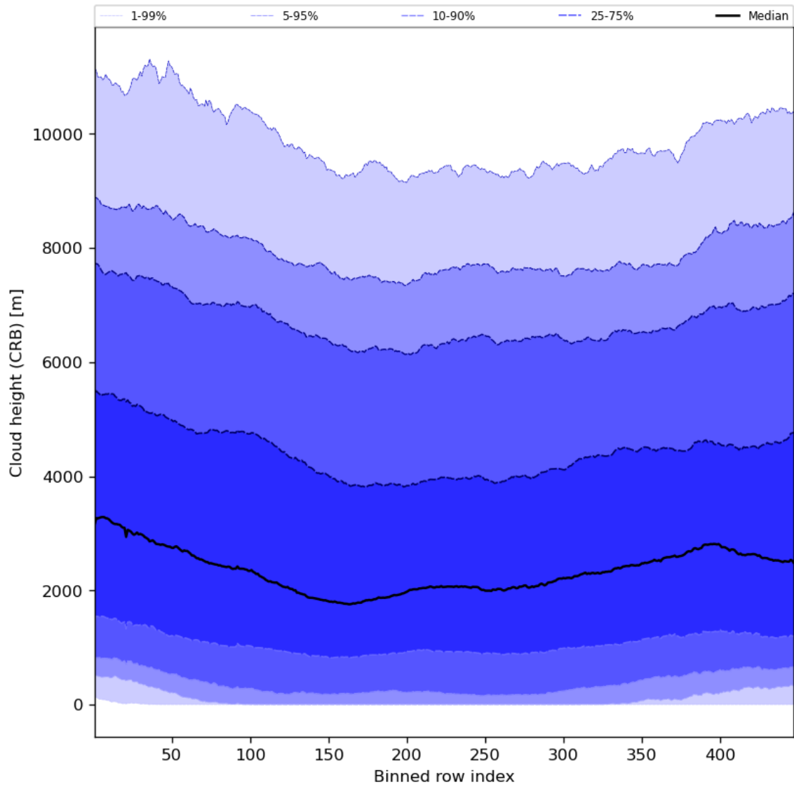
Figure 59: Along track statistics of “Cloud height (CRB)” for 2024-04-10 to 2024-04-11
