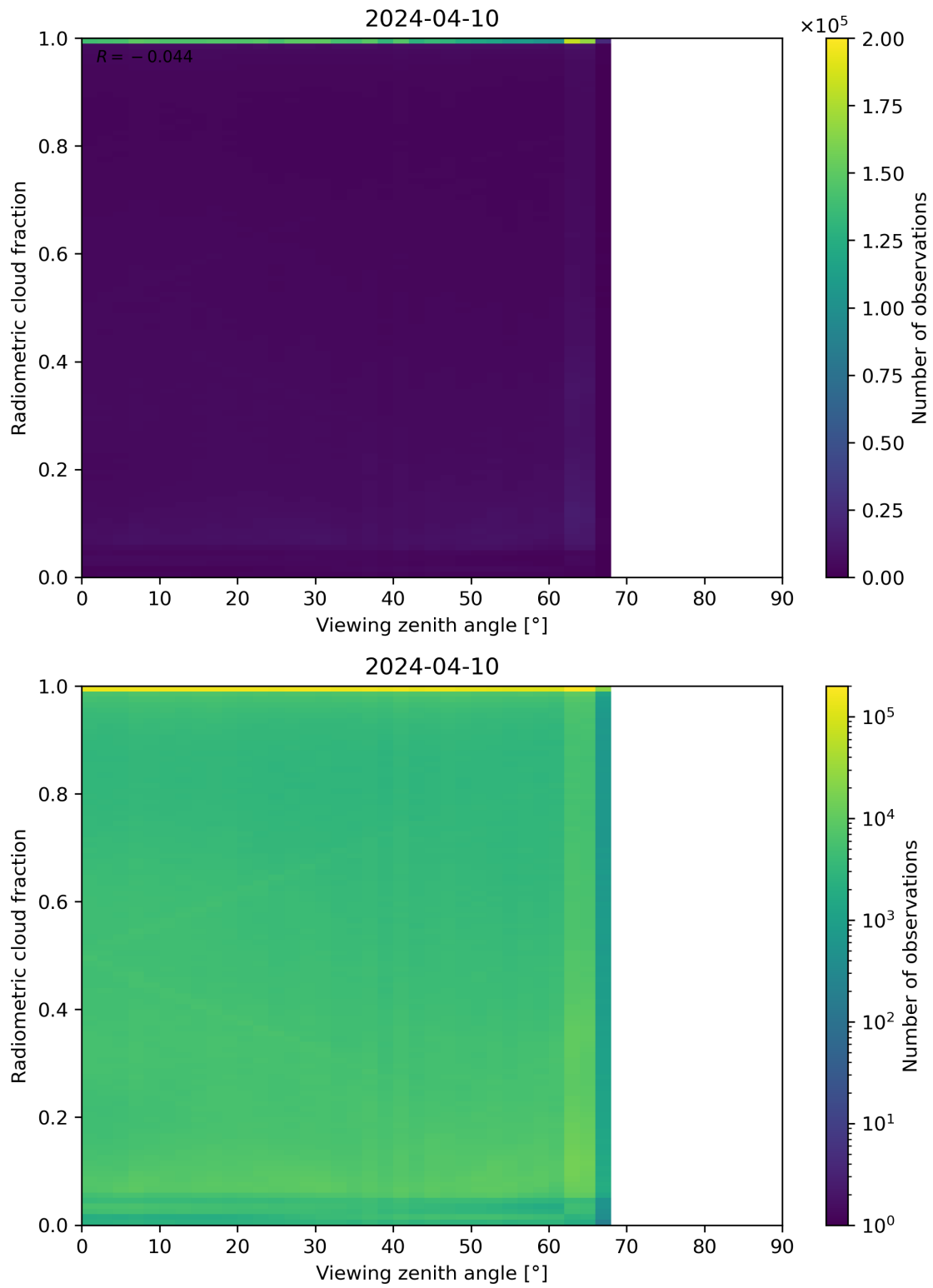
Figure 107: Scatter density plot of “Viewing zenith angle” against “Radiometric cloud fraction” for 2024-04-10 to 2024-04-11.
