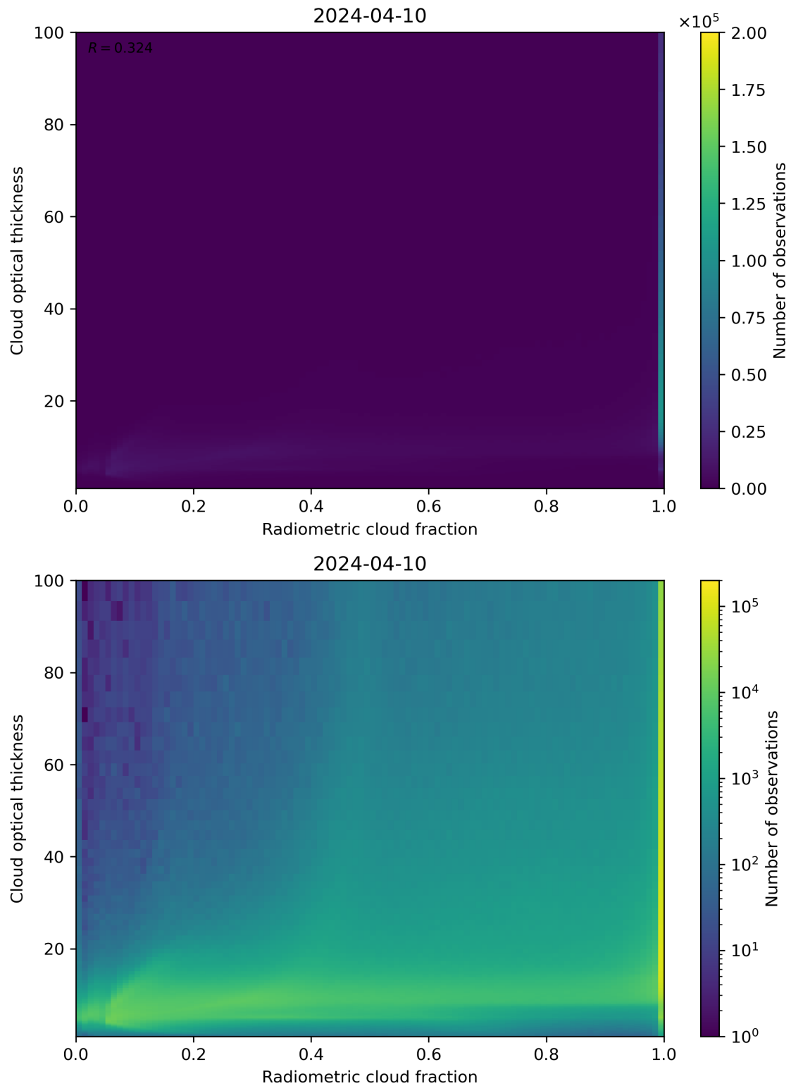
Figure 75: Scatter density plot of “Radiometric cloud fraction” against “Cloud optical thickness” for 2024-04-10 to 2024-04-11.
