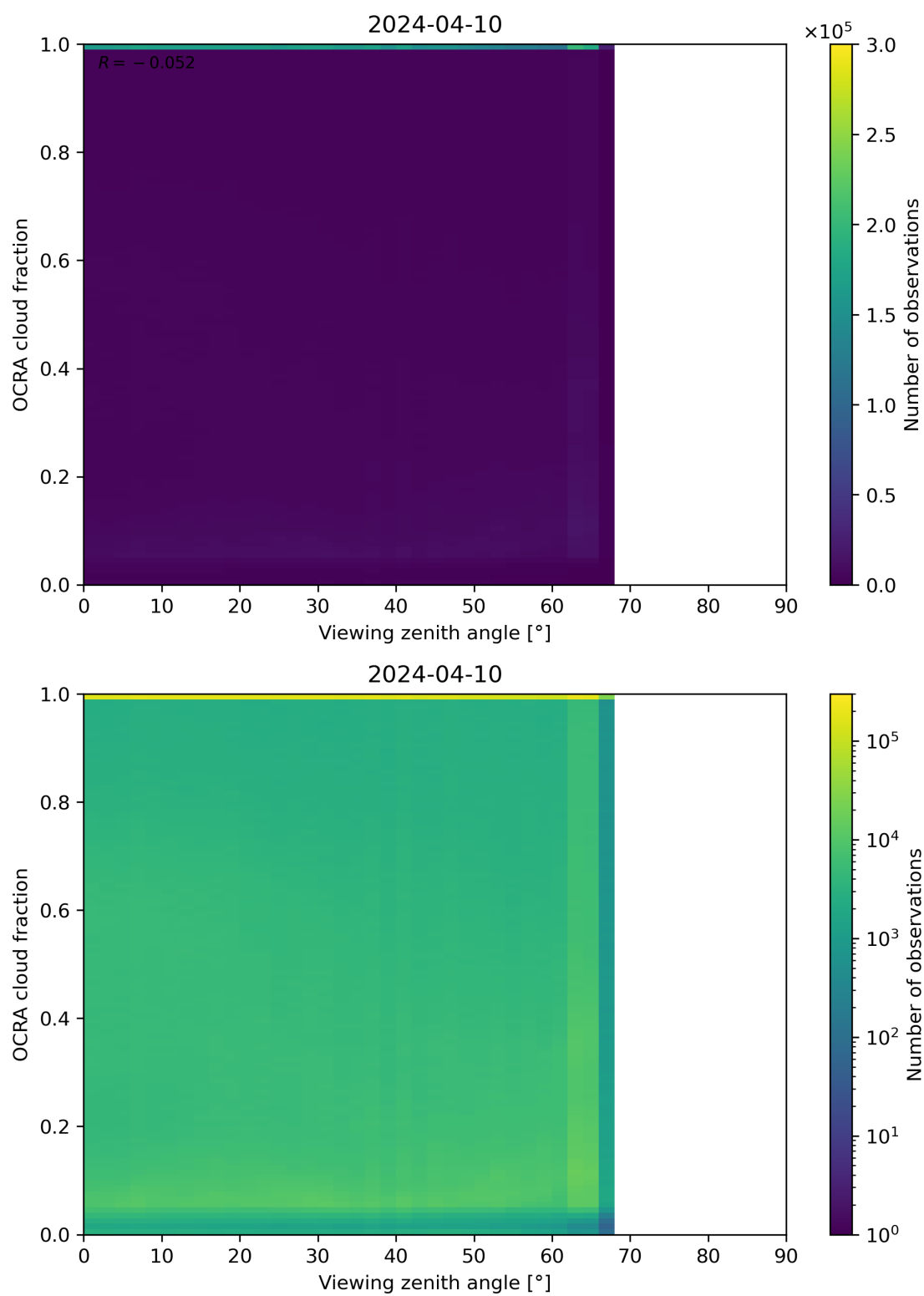
Figure 108: Scatter density plot of “Viewing zenith angle” against “OCRA cloud fraction” for 2024-04-10 to 2024-04-11.
