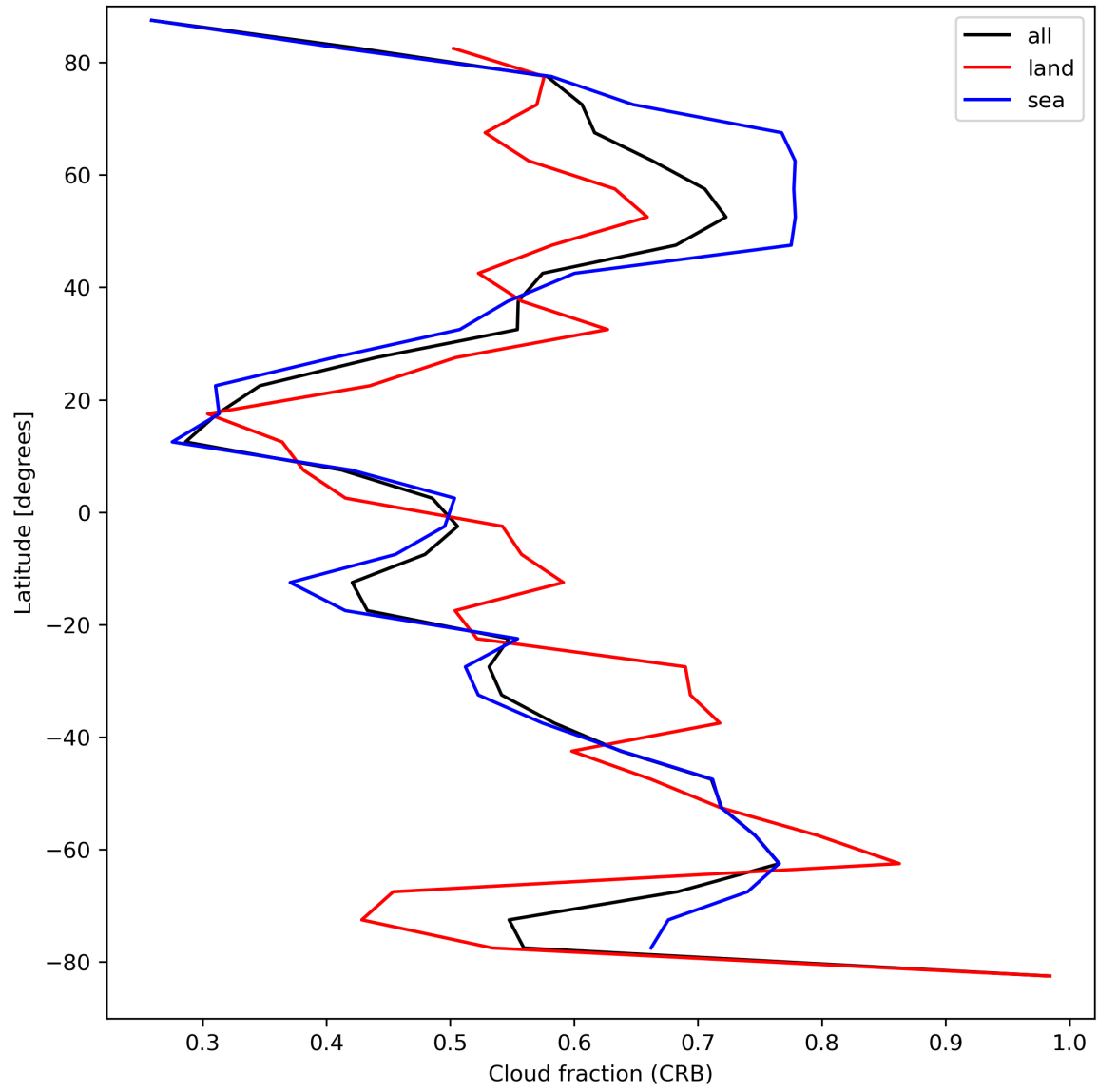
Figure 26: Zonal average of “Cloud fraction (CRB)” for 2024-04-10 to 2024-04-11.
