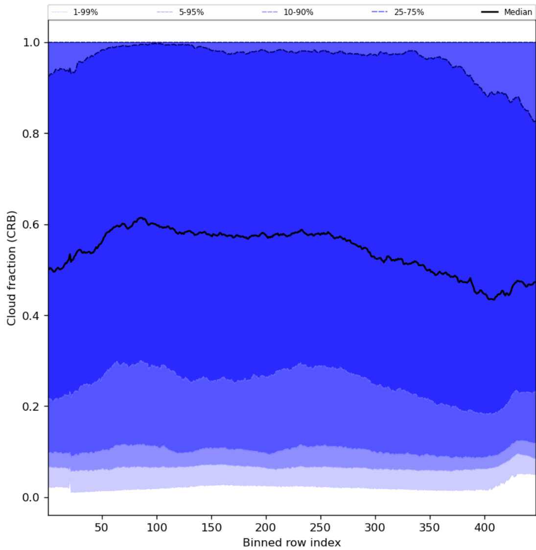
Figure 58: Along track statistics of “Cloud fraction (CRB)” for 2024-04-10 to 2024-04-11
