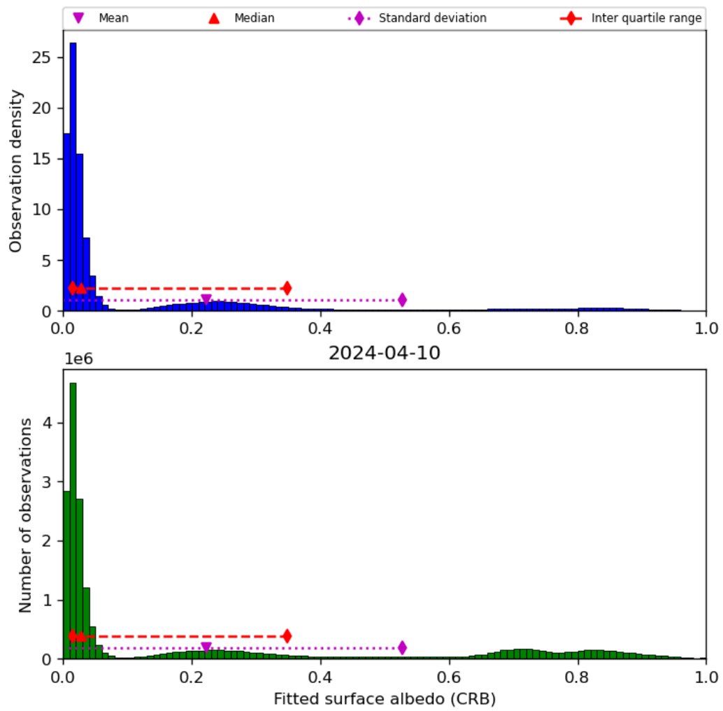
Figure 46: Histogram of “Fitted surface albedo (CRB)” for 2024-04-10 to 2024-04-11
