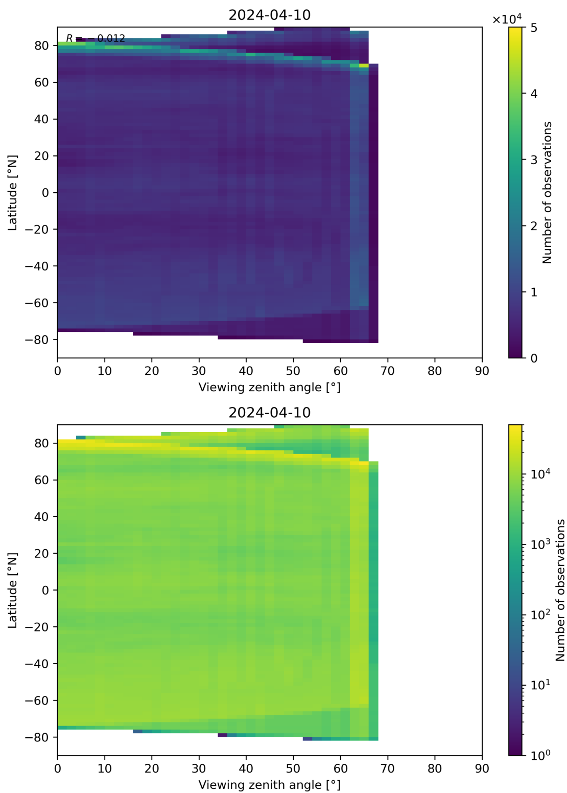
Figure 113: Scatter density plot of “Viewing zenith angle” against “Latitude” for 2024-04-10 to 2024-04-11.
