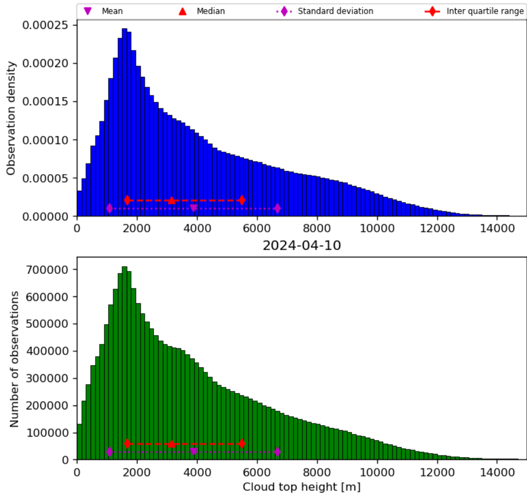
Figure 40: Histogram of “Cloud top height” for 2024-04-10 to 2024-04-11
