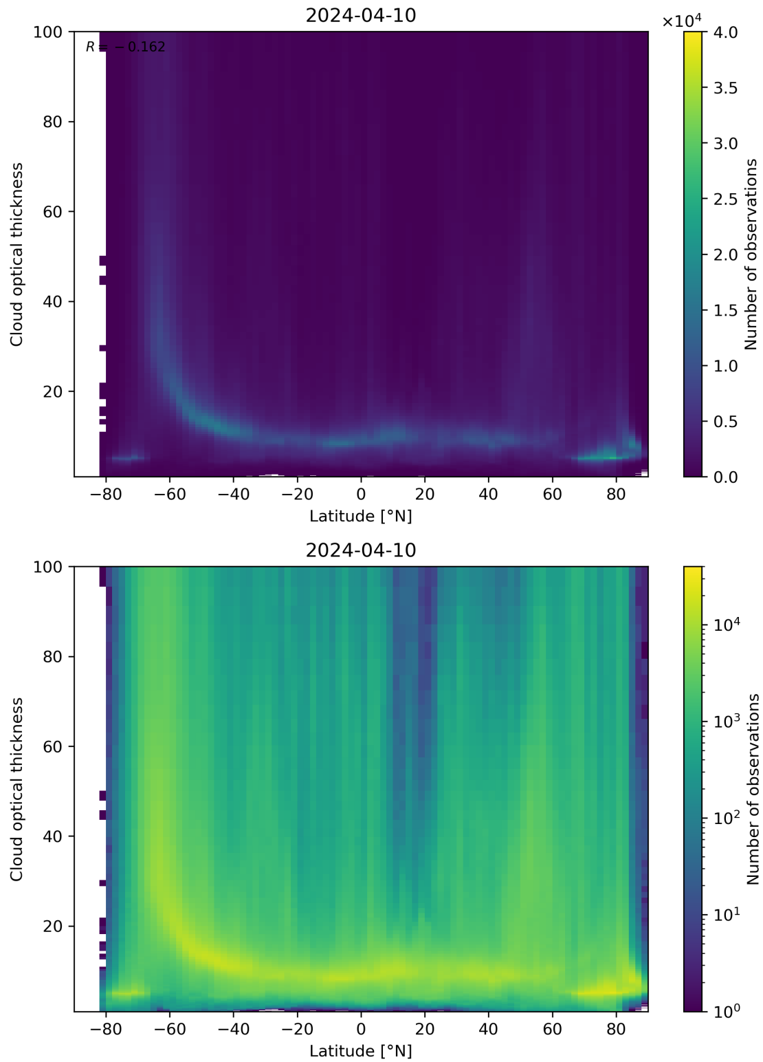
Figure 96: Scatter density plot of “Latitude” against “Cloud optical thickness” for 2024-04-10 to 2024-04-11.
