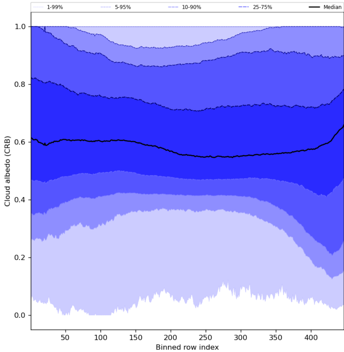
Figure 60: Along track statistics of “Cloud albedo (CRB)” for 2024-04-10 to 2024-04-11
