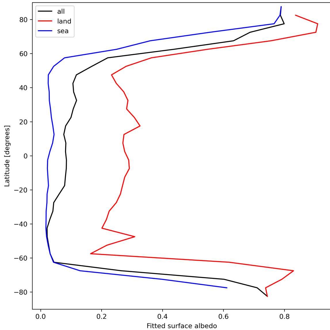
Figure 29: Zonal average of “Fitted surface albedo” for 2024-04-10 to 2024-04-11.
