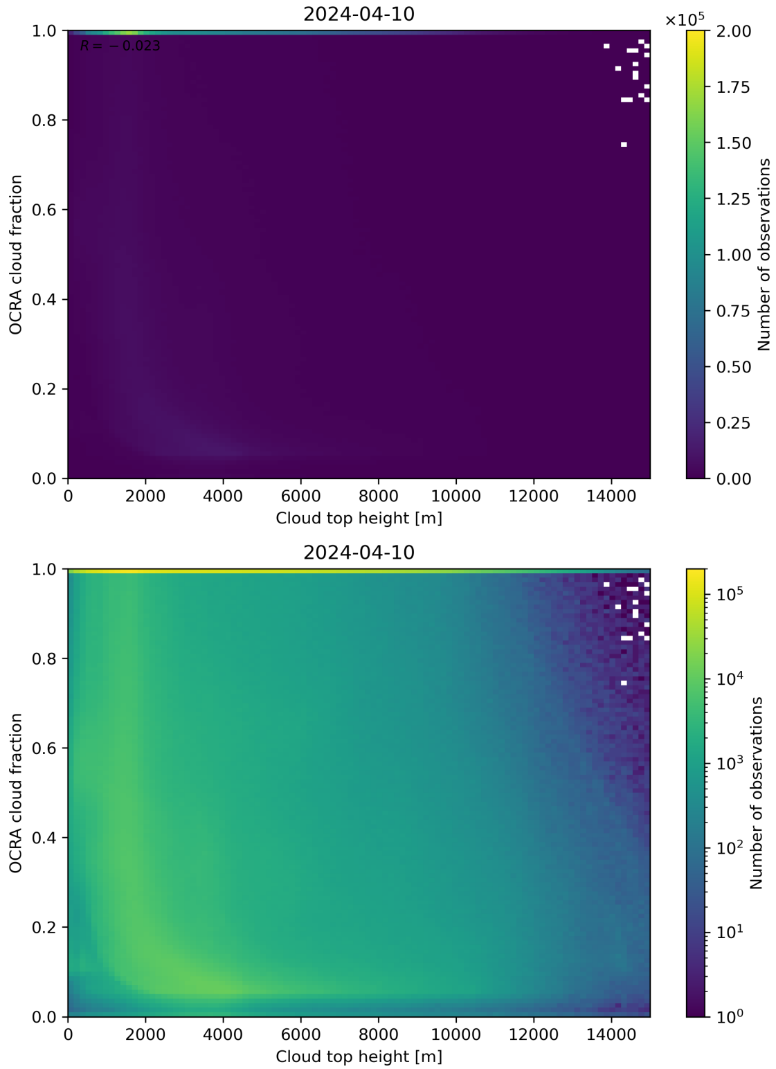
Figure 87: Scatter density plot of “Cloud top height” against “OCRA cloud fraction” for 2024-04-10 to 2024-04-11.
