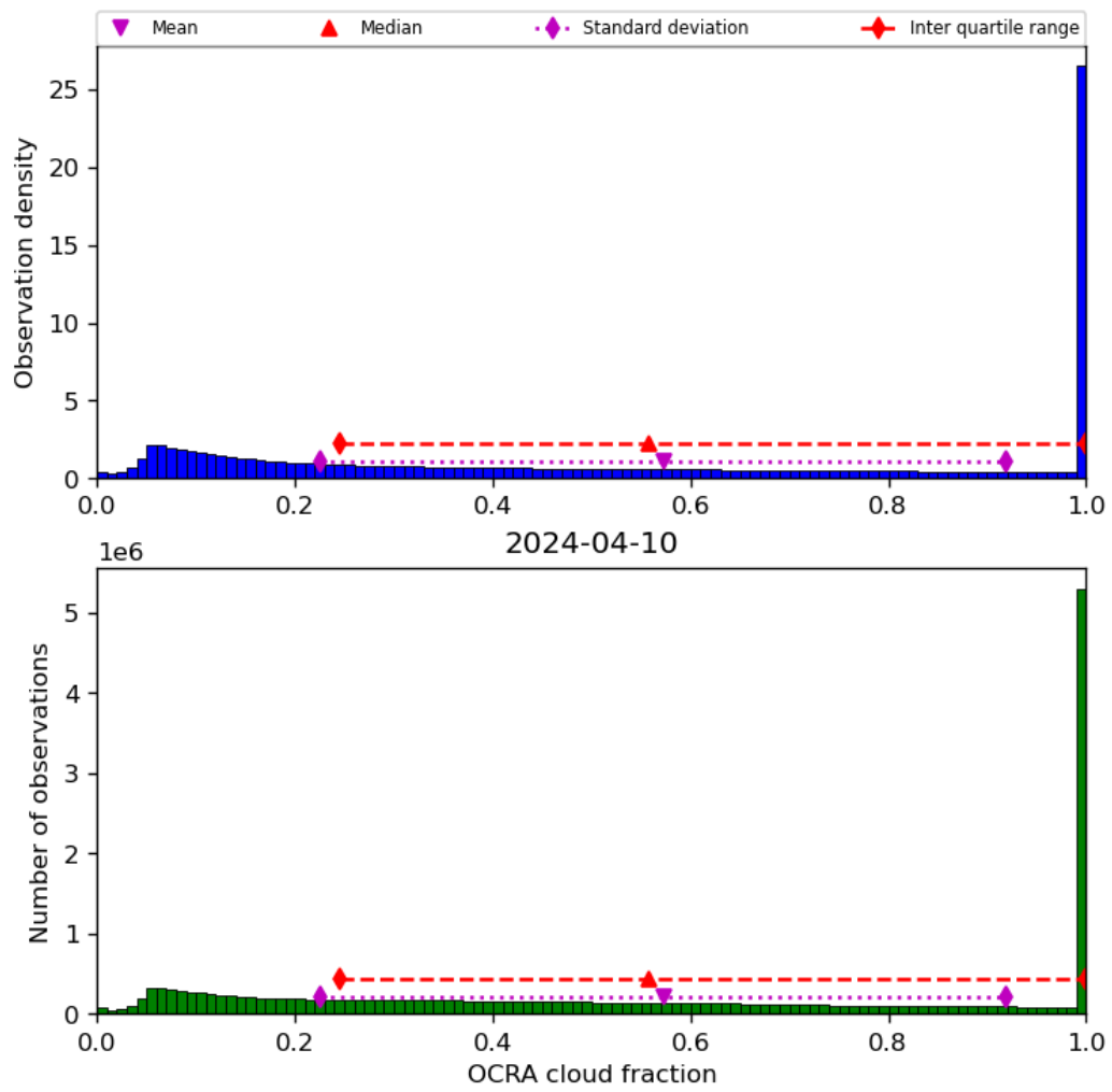
Figure 50: Histogram of “OCRA cloud fraction” for 2024-04-10 to 2024-04-11
