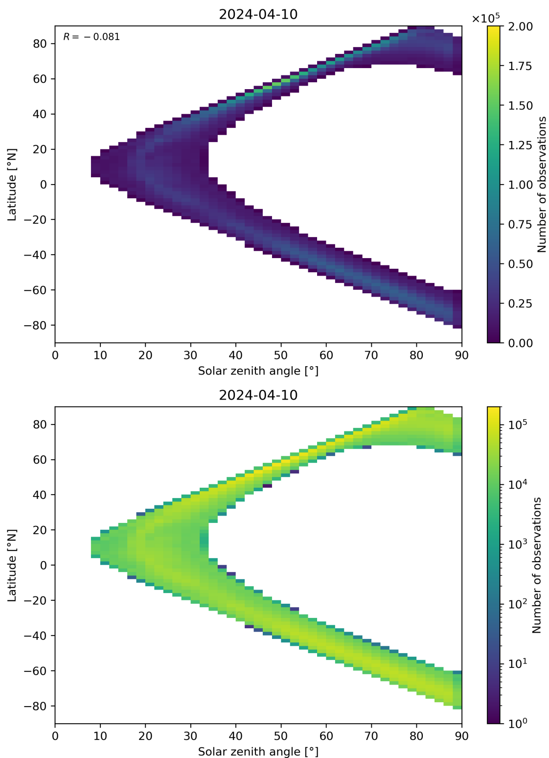
Figure 105: Scatter density plot of “Solar zenith angle” against “Latitude” for 2024-04-10 to 2024-04-11.
