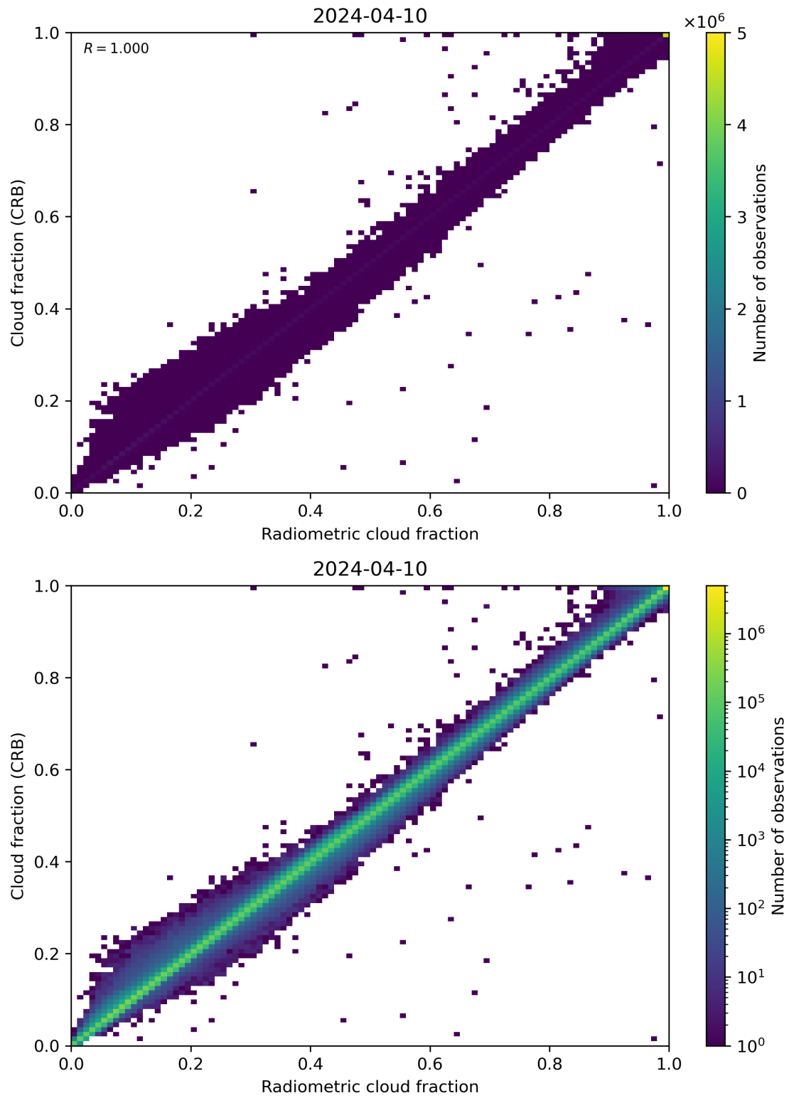
Figure 73: Scatter density plot of “Radiometric cloud fraction” against “Cloud fraction (CRB)” for 2024-04-10 to 2024-04-11.
