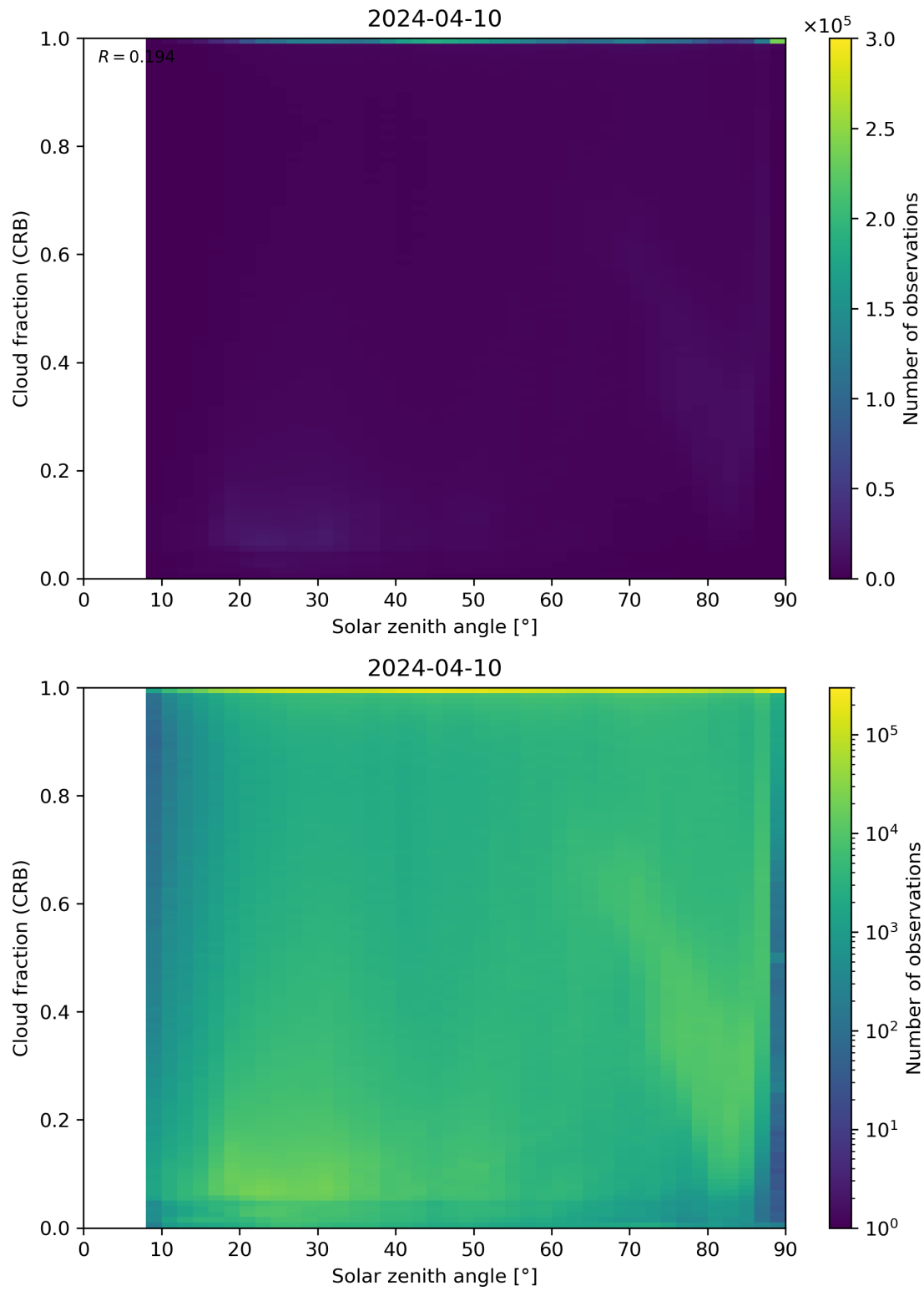
Figure 101: Scatter density plot of “Solar zenith angle” against “Cloud fraction (CRB)” for 2024-04-10 to 2024-04-11.
