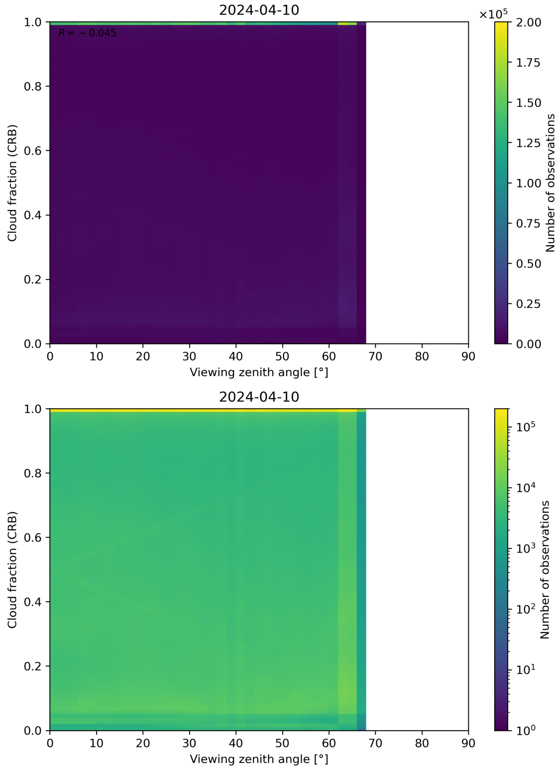
Figure 109: Scatter density plot of “Viewing zenith angle” against “Cloud fraction (CRB)” for 2024-04-10 to 2024-04-11.
