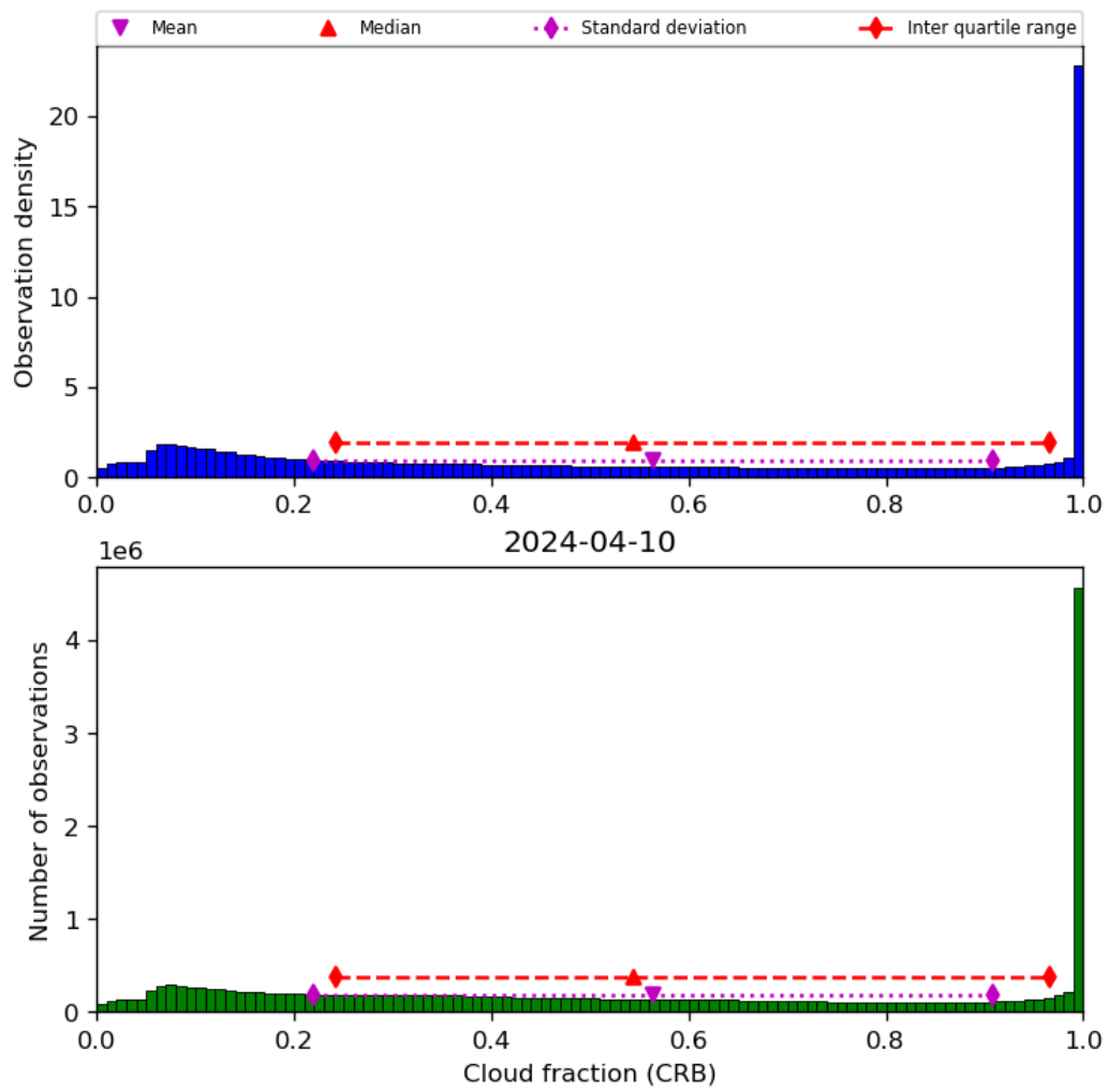
Figure 42: Histogram of “Cloud fraction (CRB)” for 2024-04-10 to 2024-04-11
