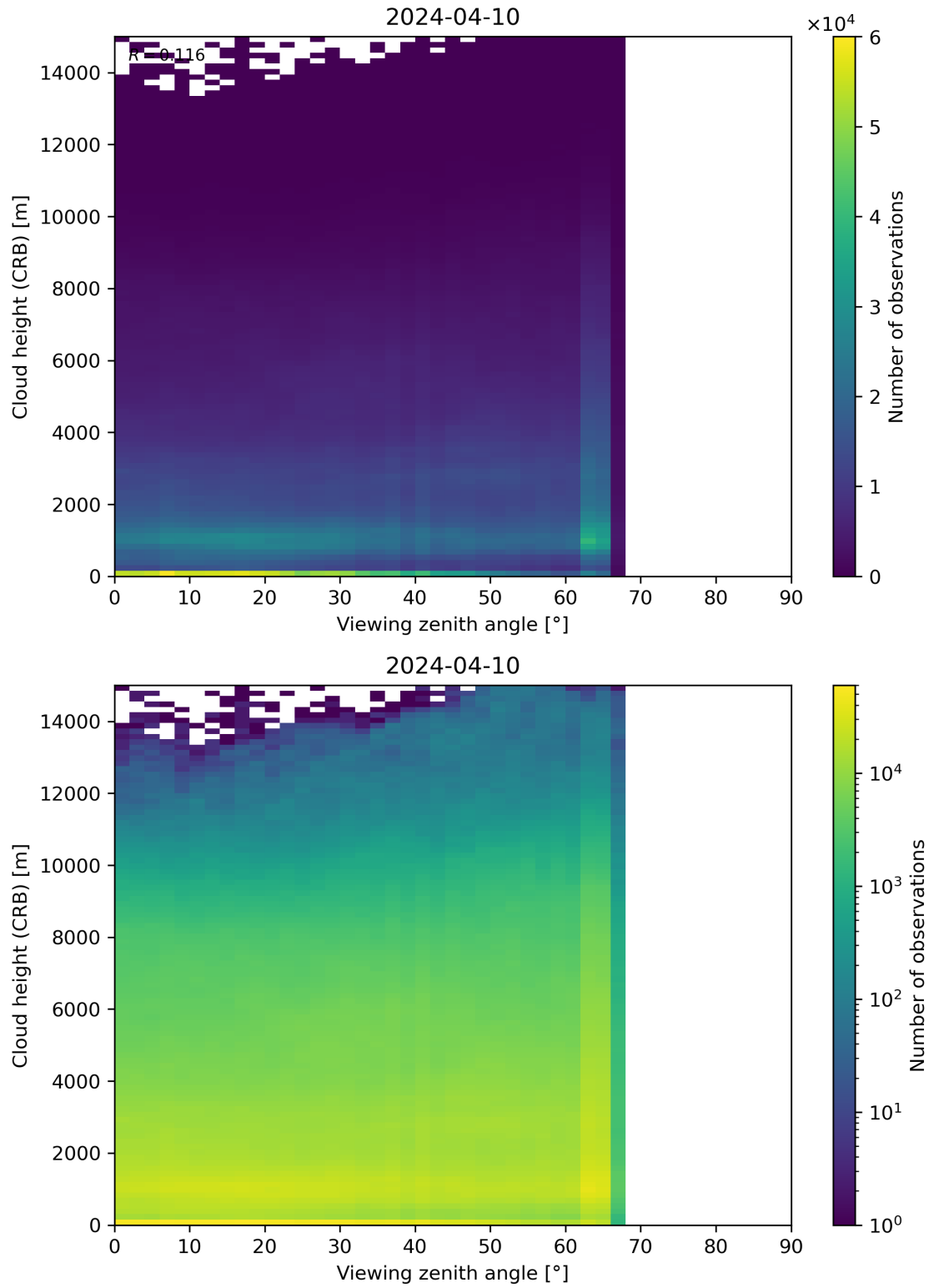
Figure 110: Scatter density plot of “Viewing zenith angle” against “Cloud height (CRB)” for 2024-04-10 to 2024-04-11.
