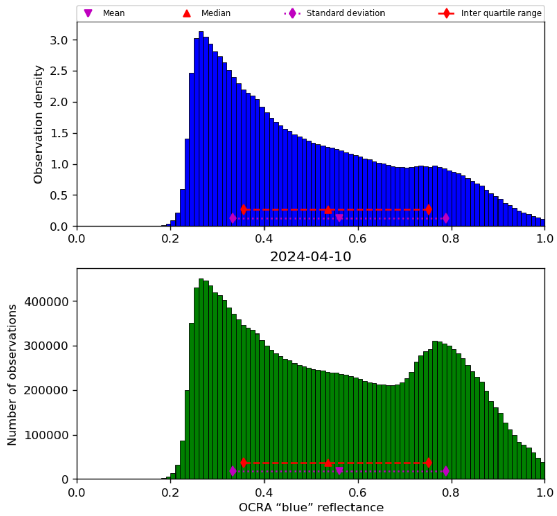
Figure 51: Histogram of “OCRA “blue” reflectance” for 2024-04-10 to 2024-04-11
