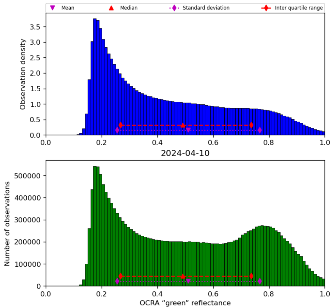
Figure 52: Histogram of “OCRA “green” reflectance” for 2024-04-10 to 2024-04-11
