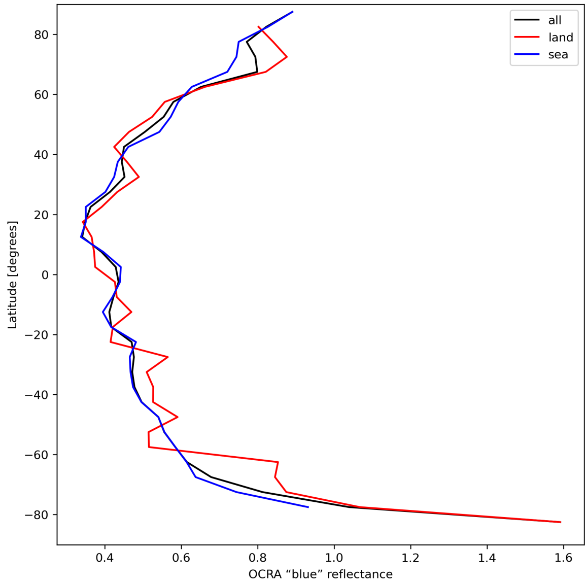
Figure 35: Zonal average of “OCRA “blue” reflectance” for 2024-04-10 to 2024-04-11.
