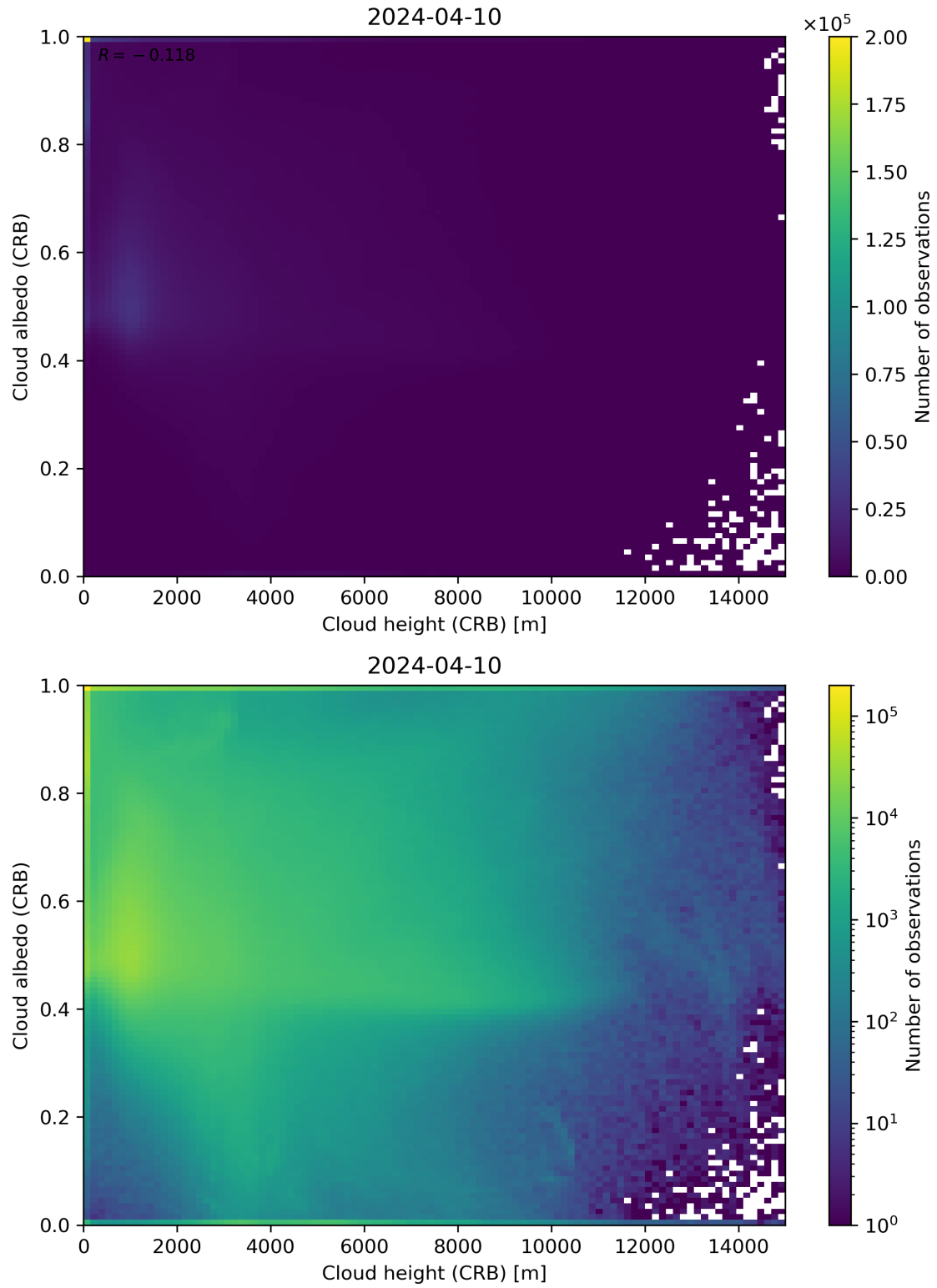
Figure 80: Scatter density plot of “Cloud height (CRB)” against “Cloud albedo (CRB)” for 2024-04-10 to 2024-04-11.
