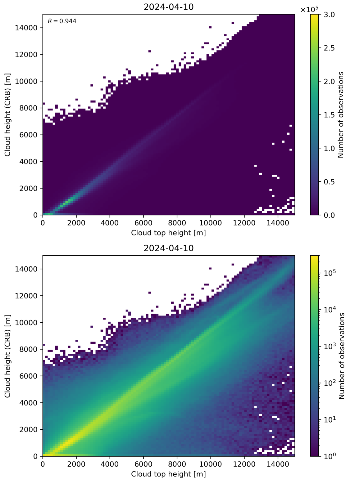
Figure 89: Scatter density plot of “Cloud top height” against “Cloud height (CRB)” for 2024-04-10 to 2024-04-11.
