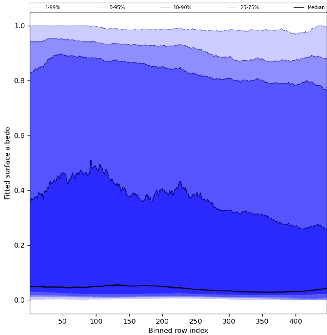
Figure 61: Along track statistics of “Fitted surface albedo” for 2024-04-10 to 2024-04-11
