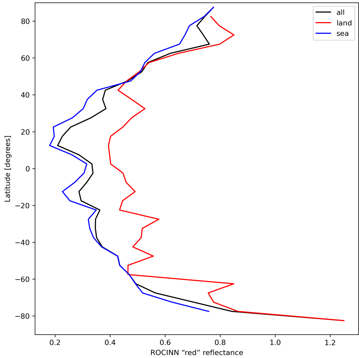
Figure 37: Zonal average of “ROCINN “red” reflectance” for 2024-04-10 to 2024-04-11.
