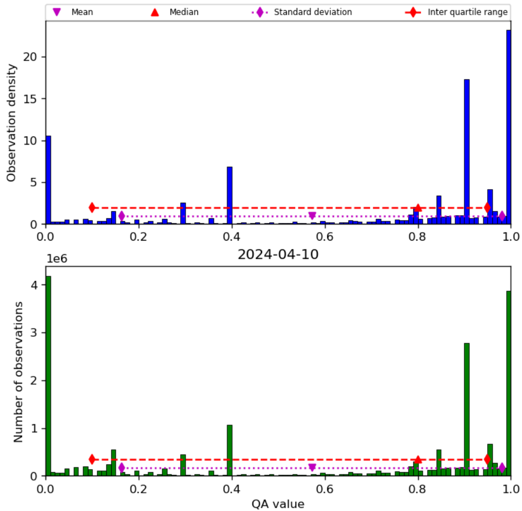
Figure 38: Histogram of “QA value” for 2024-04-10 to 2024-04-11
