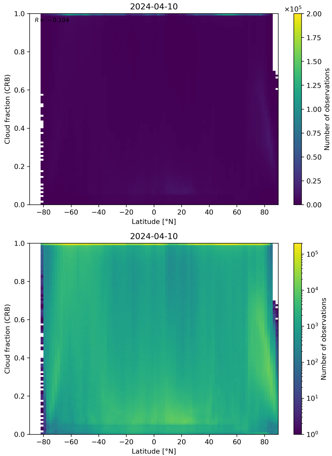
Figure 94: Scatter density plot of “Latitude” against “Cloud fraction (CRB)” for 2024-04-10 to 2024-04-11.
