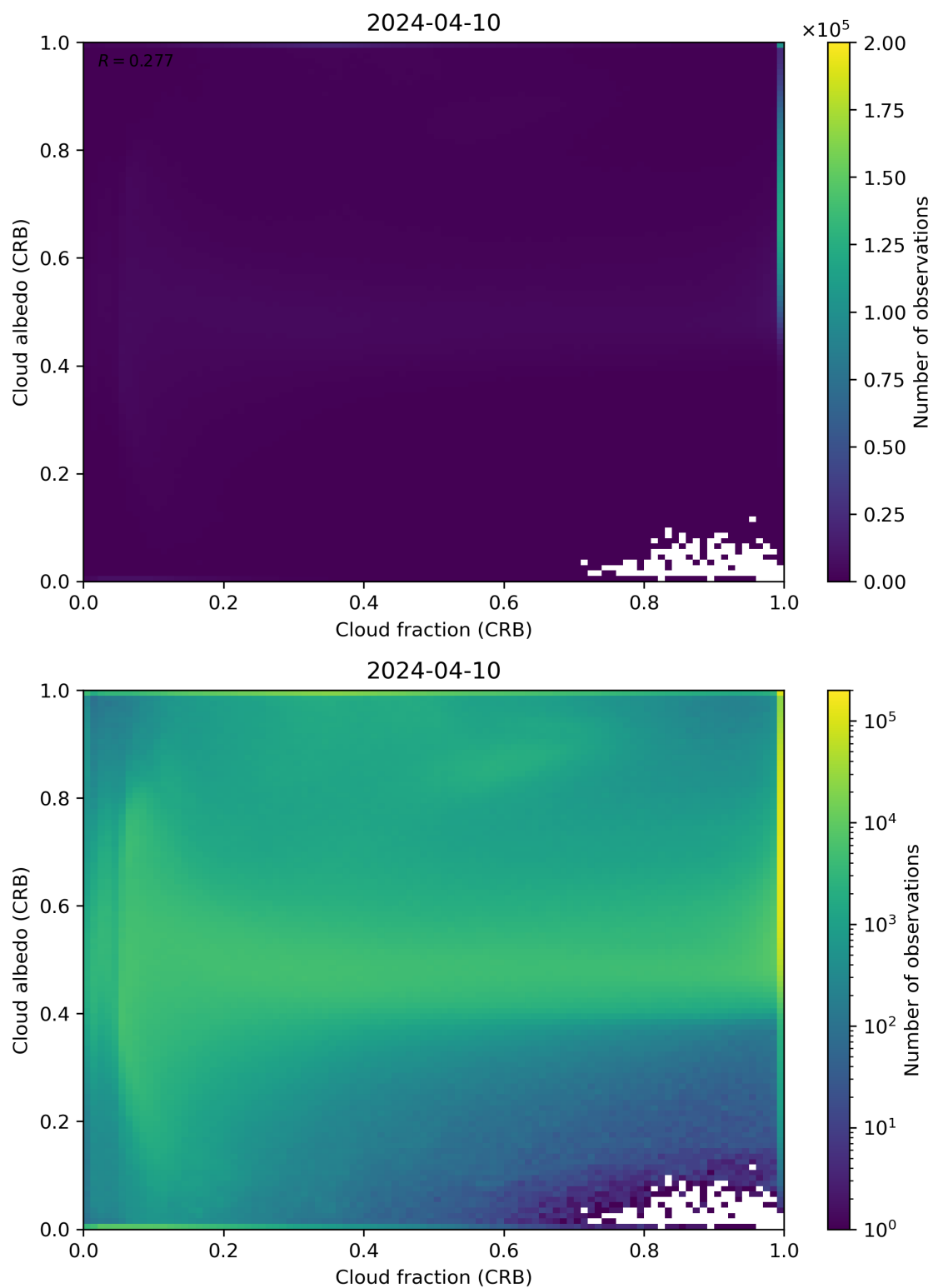
Figure 77: Scatter density plot of “Cloud fraction (CRB)” against “Cloud albedo (CRB)” for 2024-04-10 to 2024-04-11.
