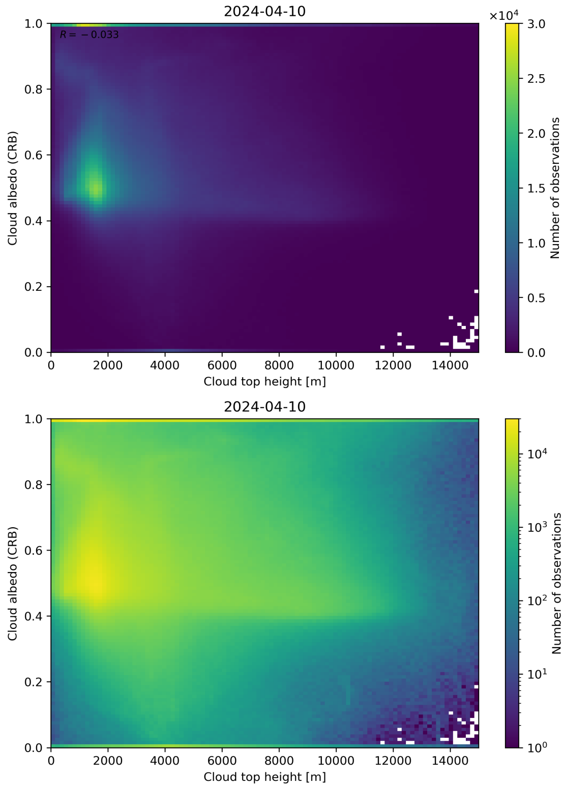
Figure 86: Scatter density plot of “Cloud top height” against “Cloud albedo (CRB)” for 2024-04-10 to 2024-04-11.
