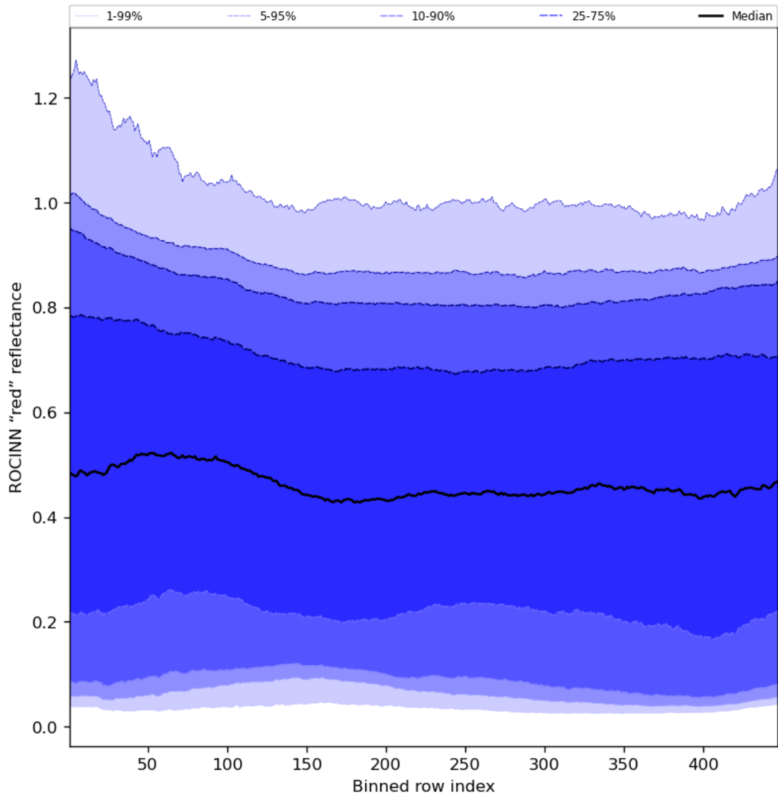
Figure 69: Along track statistics of “ROCINN “red” reflectance” for 2024-04-10 to 2024-04-11
