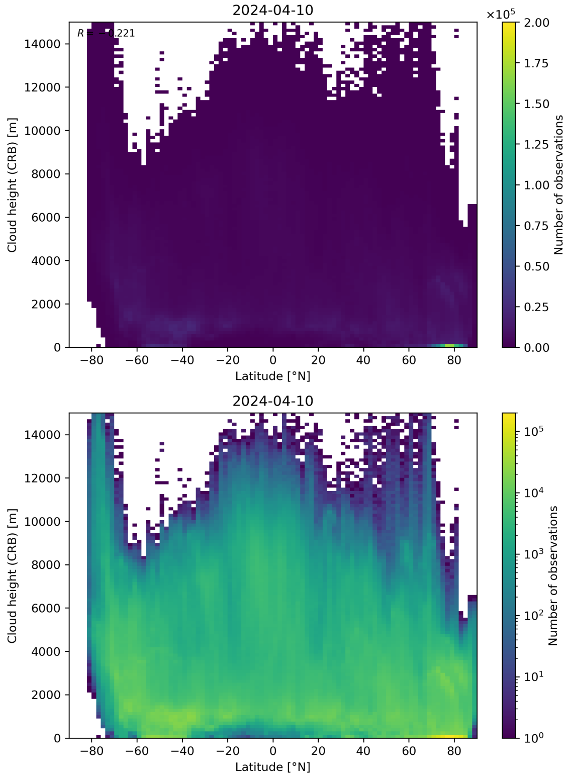
Figure 95: Scatter density plot of “Latitude” against “Cloud height (CRB)” for 2024-04-10 to 2024-04-11.
