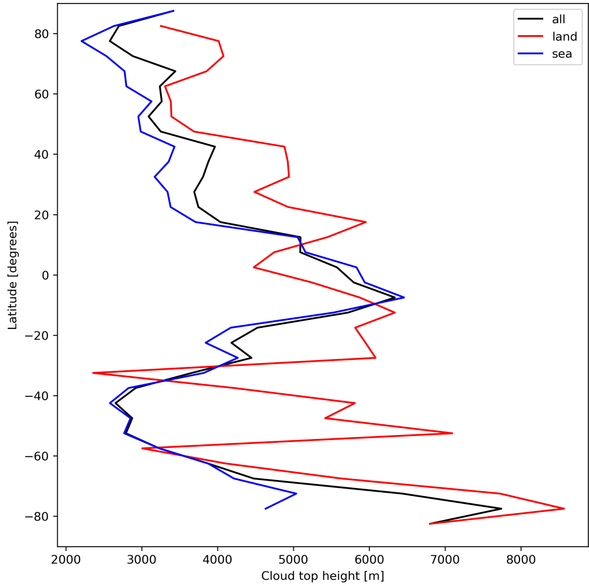
Figure 24: Zonal average of “Cloud top height” for 2024-04-10 to 2024-04-11.
