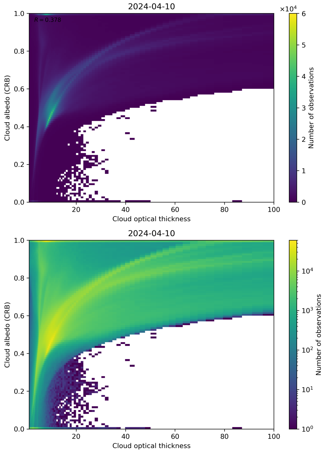
Figure 82: Scatter density plot of “Cloud optical thickness” against “Cloud albedo (CRB)” for 2024-04-10 to 2024-04-11.
