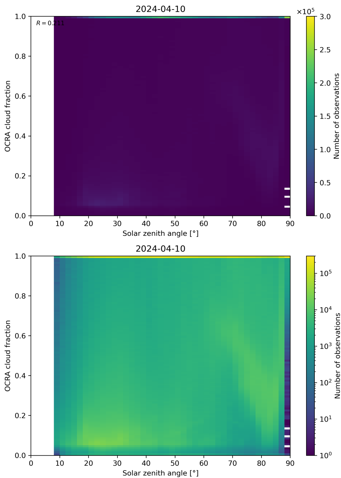
Figure 100: Scatter density plot of “Solar zenith angle” against “OCRA cloud fraction” for 2024-04-10 to 2024-04-11.
