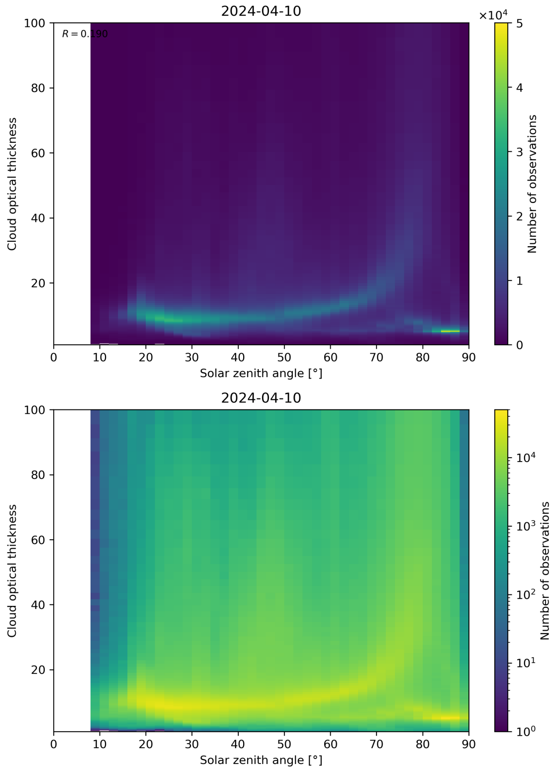
Figure 103: Scatter density plot of “Solar zenith angle” against “Cloud optical thickness” for 2024-04-10 to 2024-04-11.
