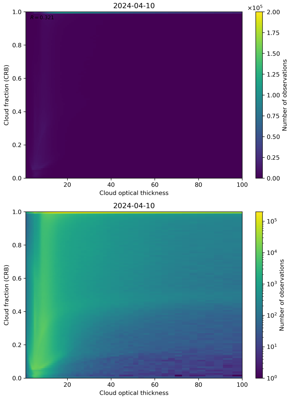
Figure 84: Scatter density plot of “Cloud optical thickness” against “Cloud fraction (CRB)” for 2024-04-10 to 2024-04-11.
