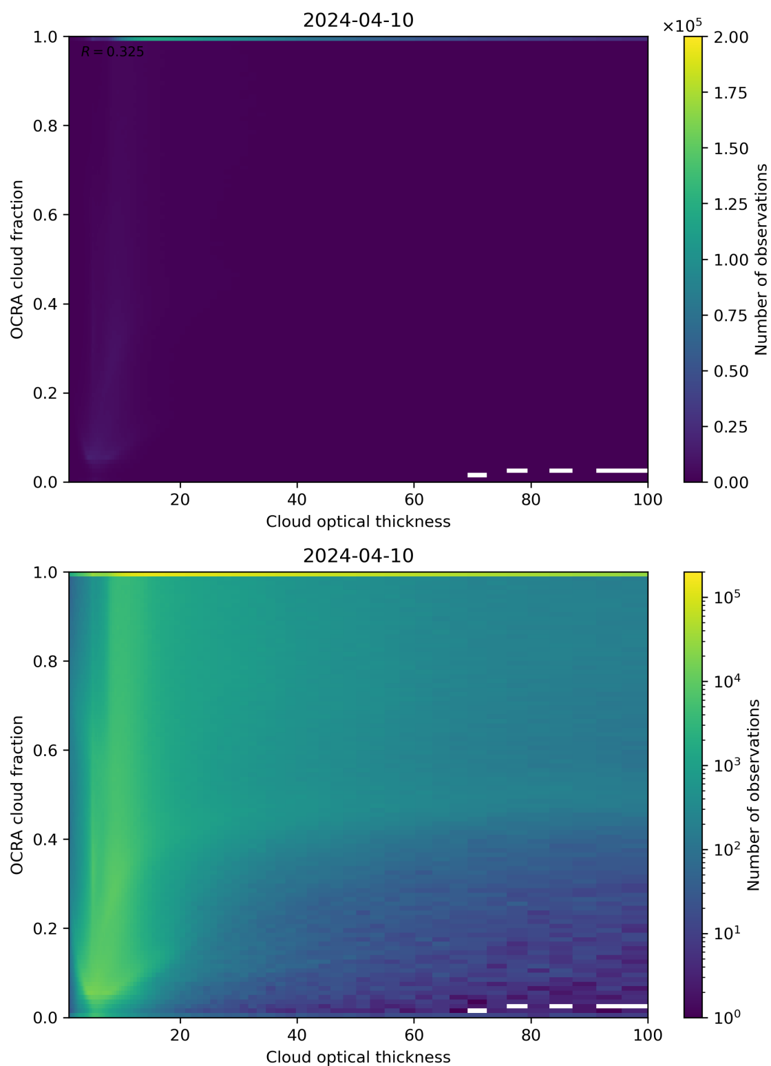
Figure 83: Scatter density plot of “Cloud optical thickness” against “OCRA cloud fraction” for 2024-04-10 to 2024-04-11.
