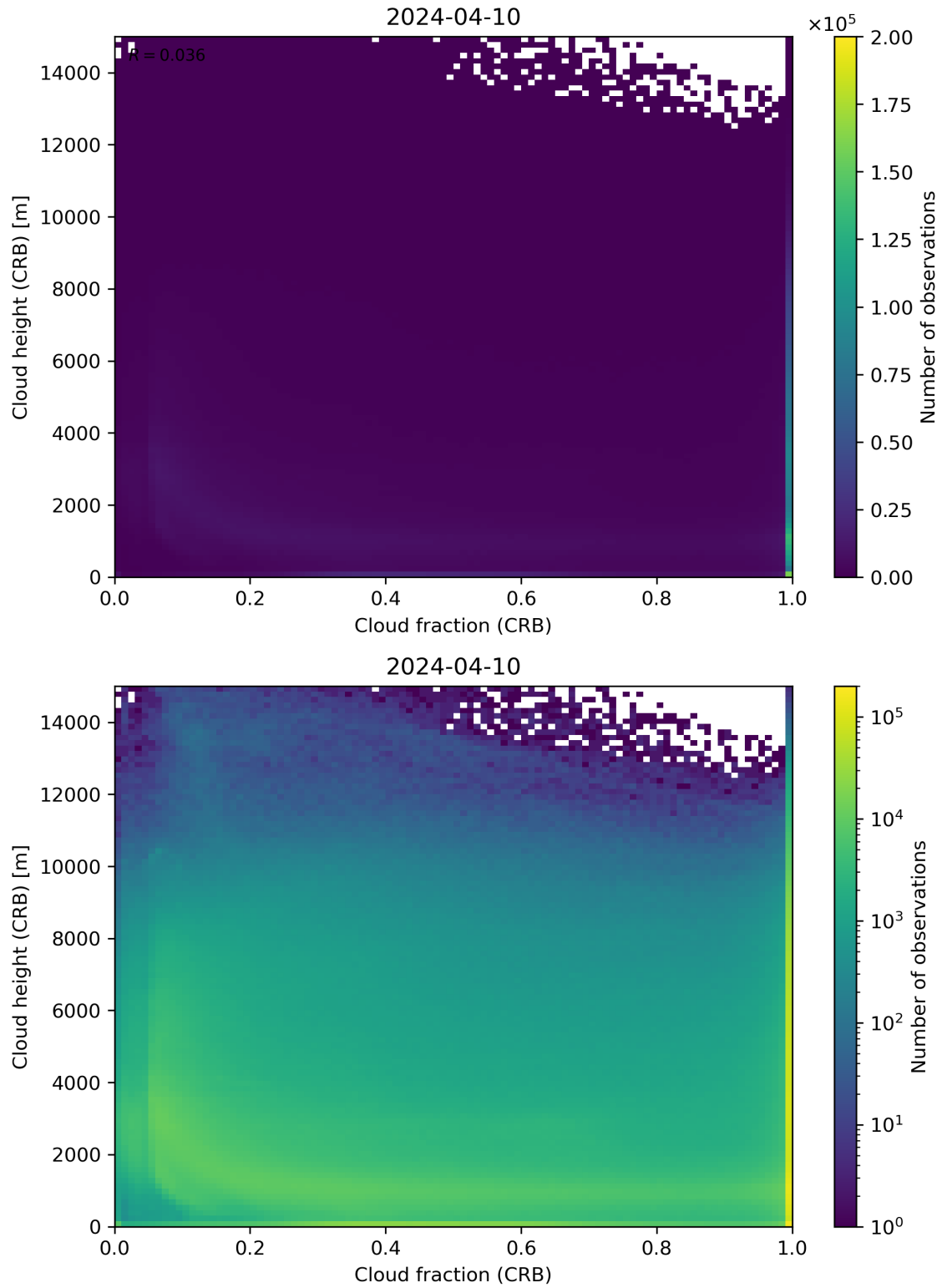
Figure 79: Scatter density plot of “Cloud fraction (CRB)” against “Cloud height (CRB)” for 2024-04-10 to 2024-04-11.
