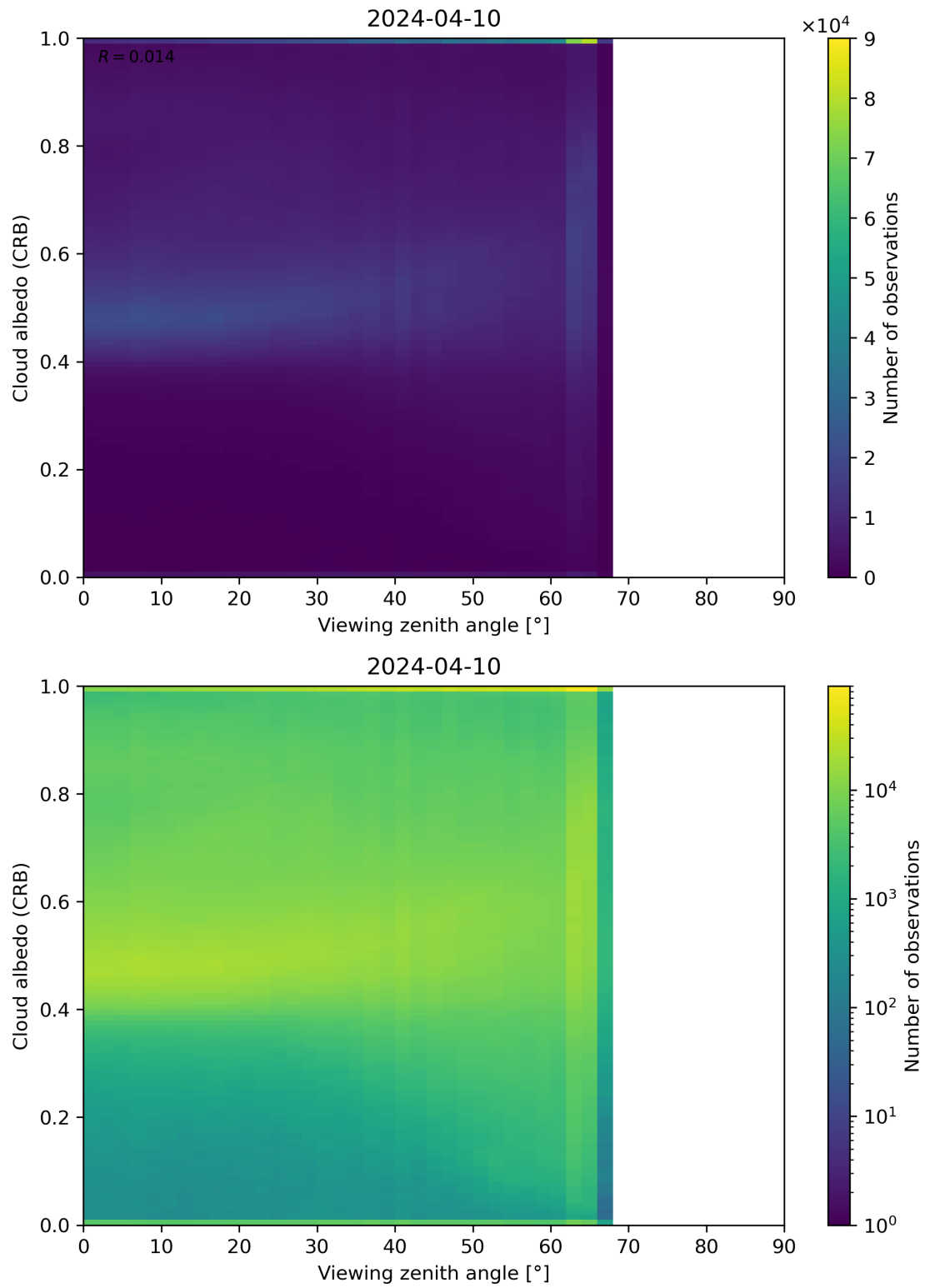
Figure 106: Scatter density plot of “Viewing zenith angle” against “Cloud albedo (CRB)” for 2024-04-10 to 2024-04-11.
