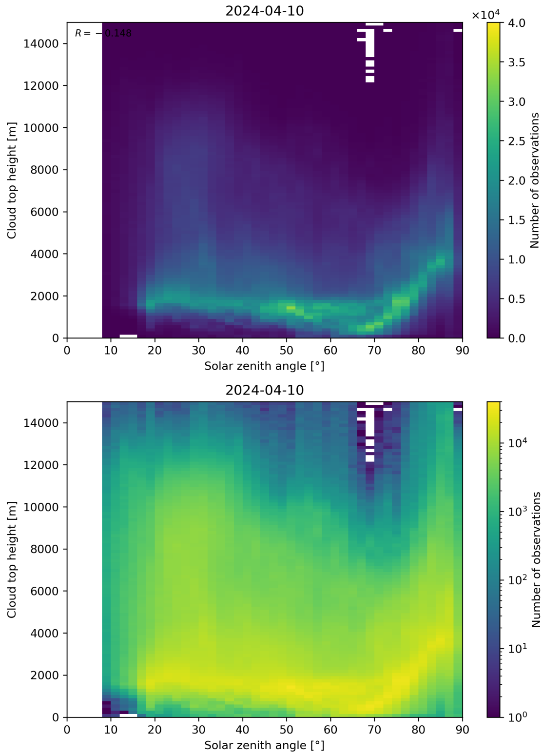
Figure 104: Scatter density plot of “Solar zenith angle” against “Cloud top height” for 2024-04-10 to 2024-04-11.
