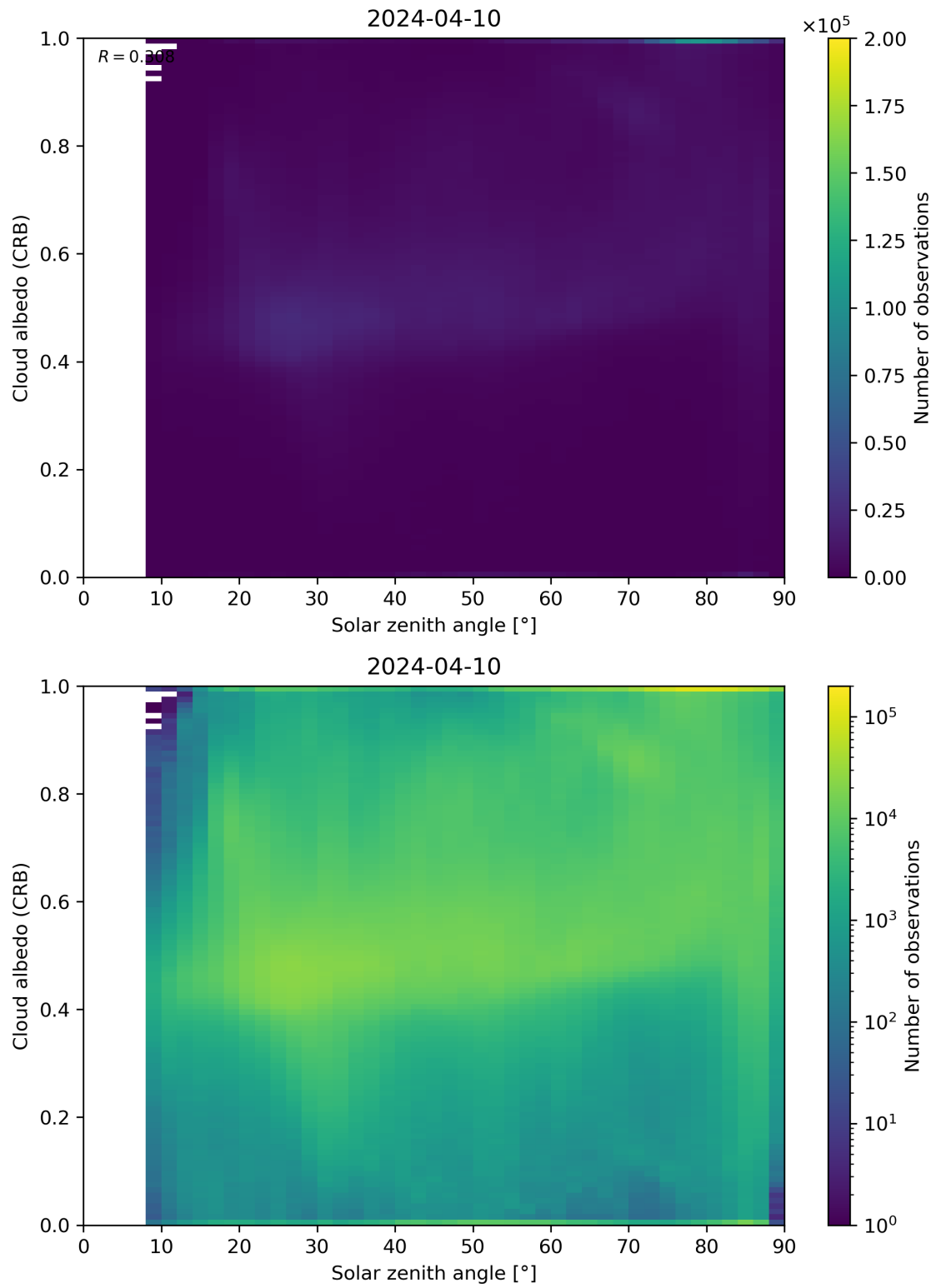
Figure 98: Scatter density plot of “Solar zenith angle” against “Cloud albedo (CRB)” for 2024-04-10 to 2024-04-11.
