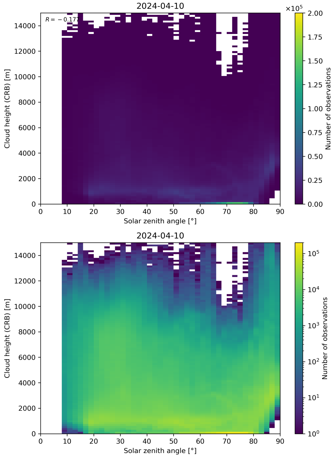
Figure 102: Scatter density plot of “Solar zenith angle” against “Cloud height (CRB)” for 2024-04-10 to 2024-04-11.
