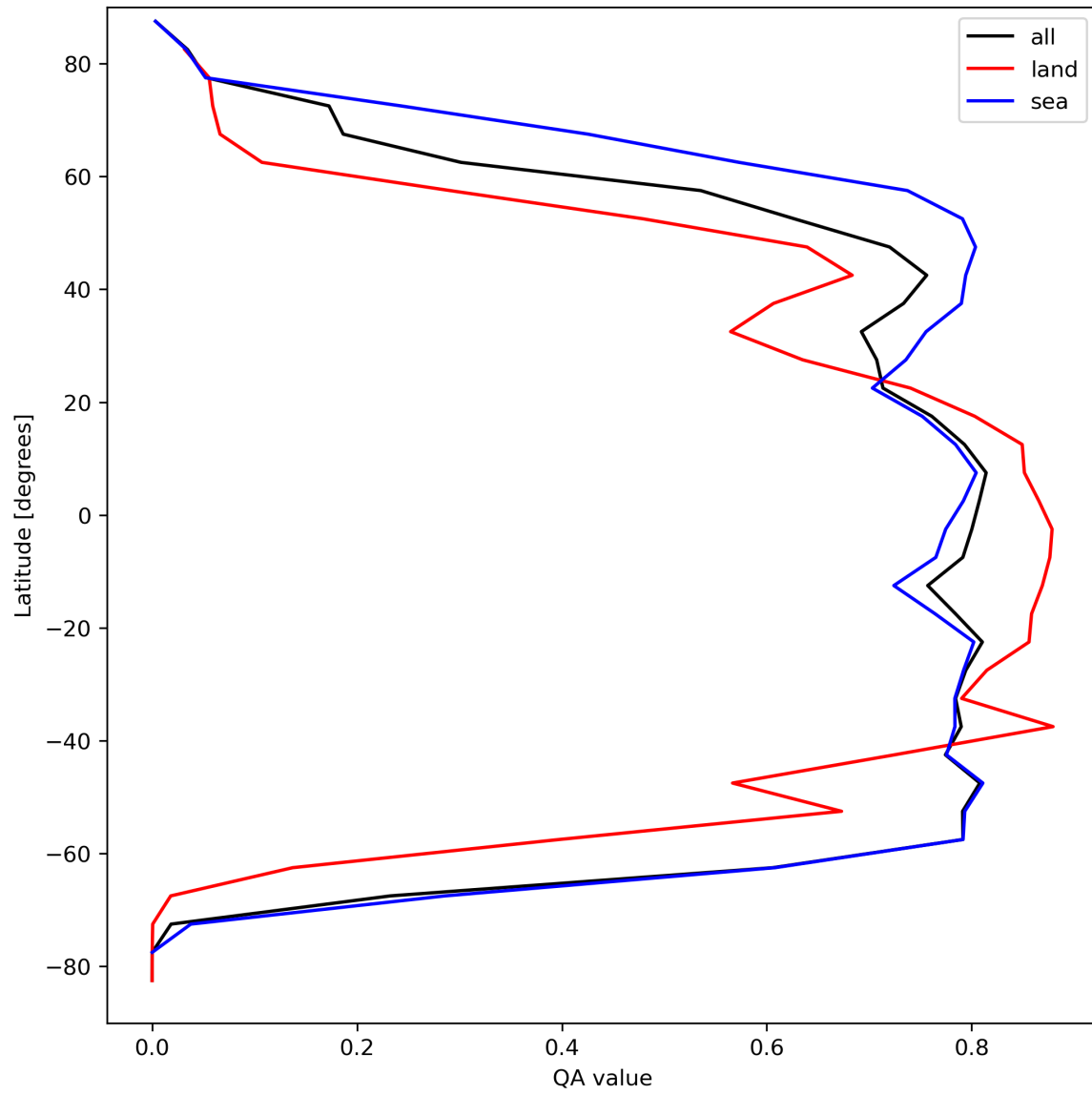
Figure 22: Zonal average of “QA value” for 2024-04-10 to 2024-04-11.
