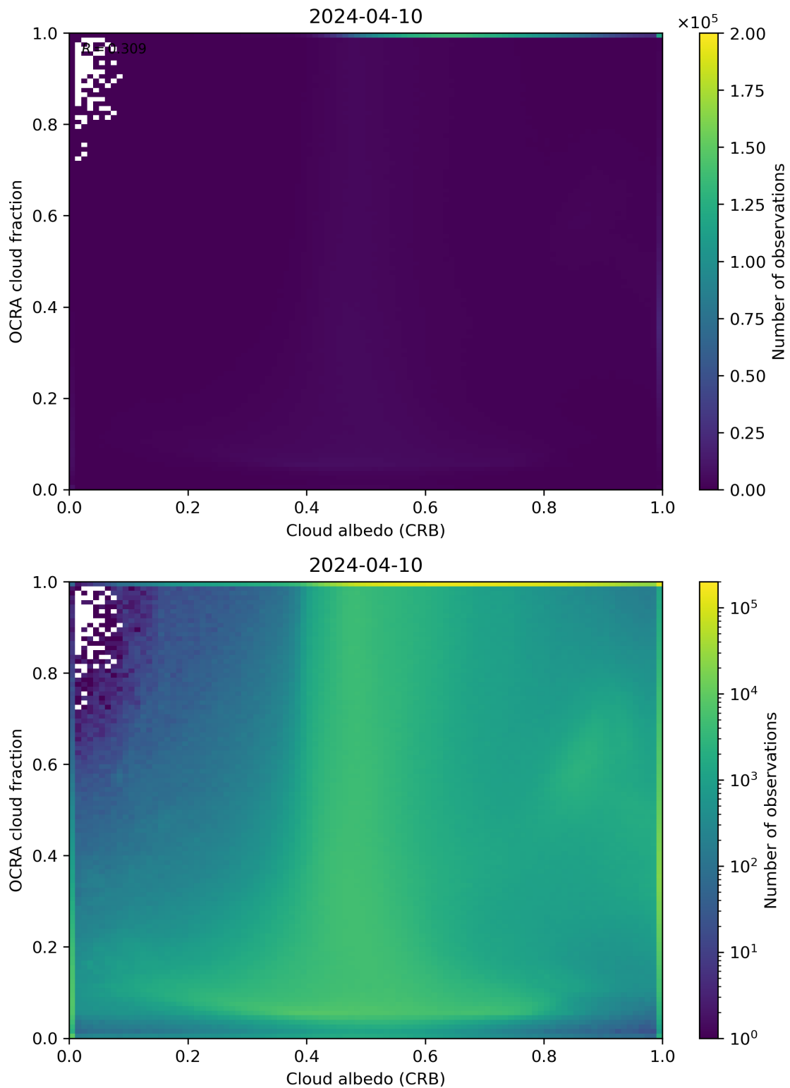
Figure 70: Scatter density plot of “Cloud albedo (CRB)” against “OCRA cloud fraction” for 2024-04-10 to 2024-04-11.
