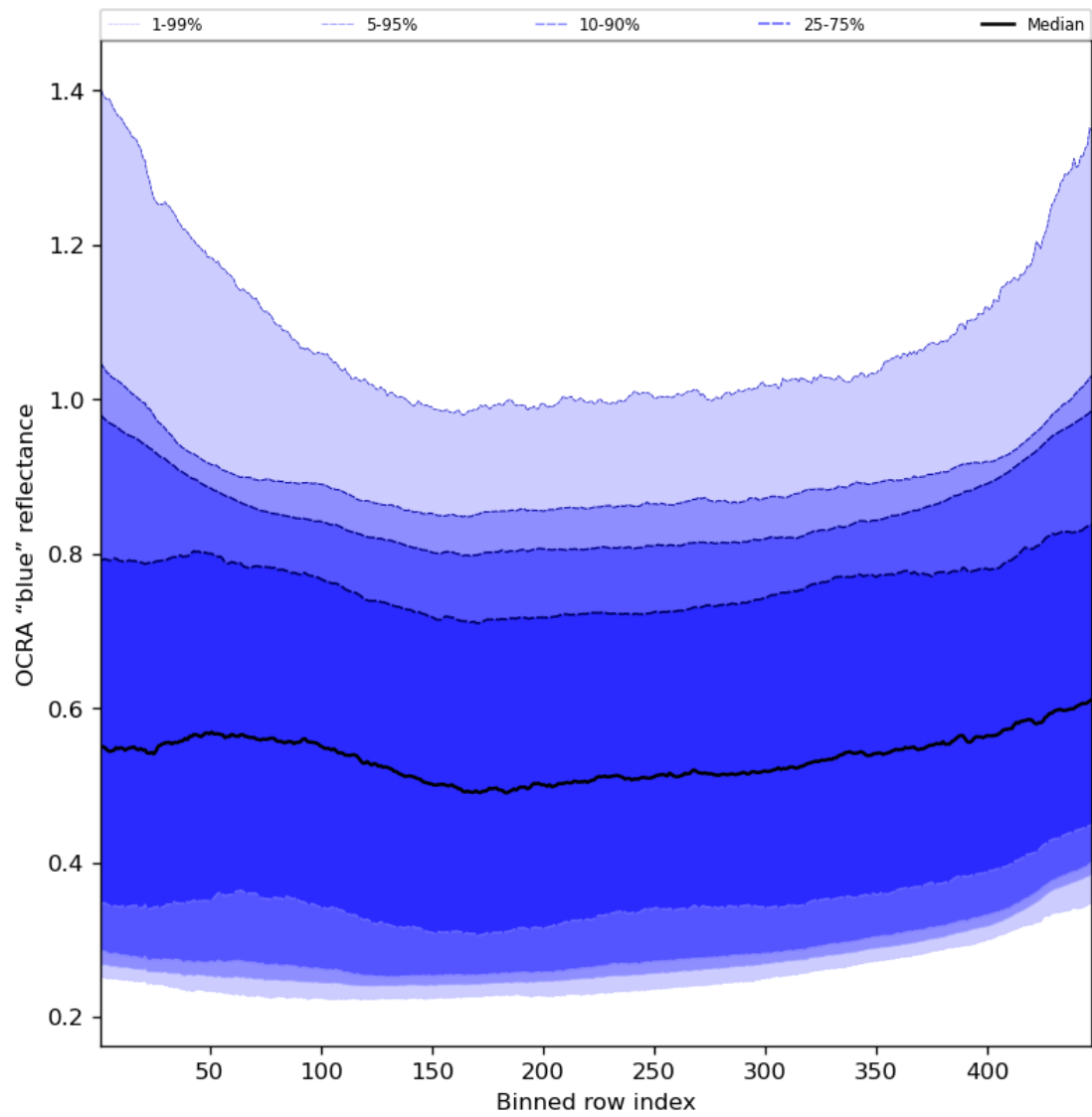
Figure 67: Along track statistics of “OCRA “blue” reflectance” for 2024-04-10 to 2024-04-11
