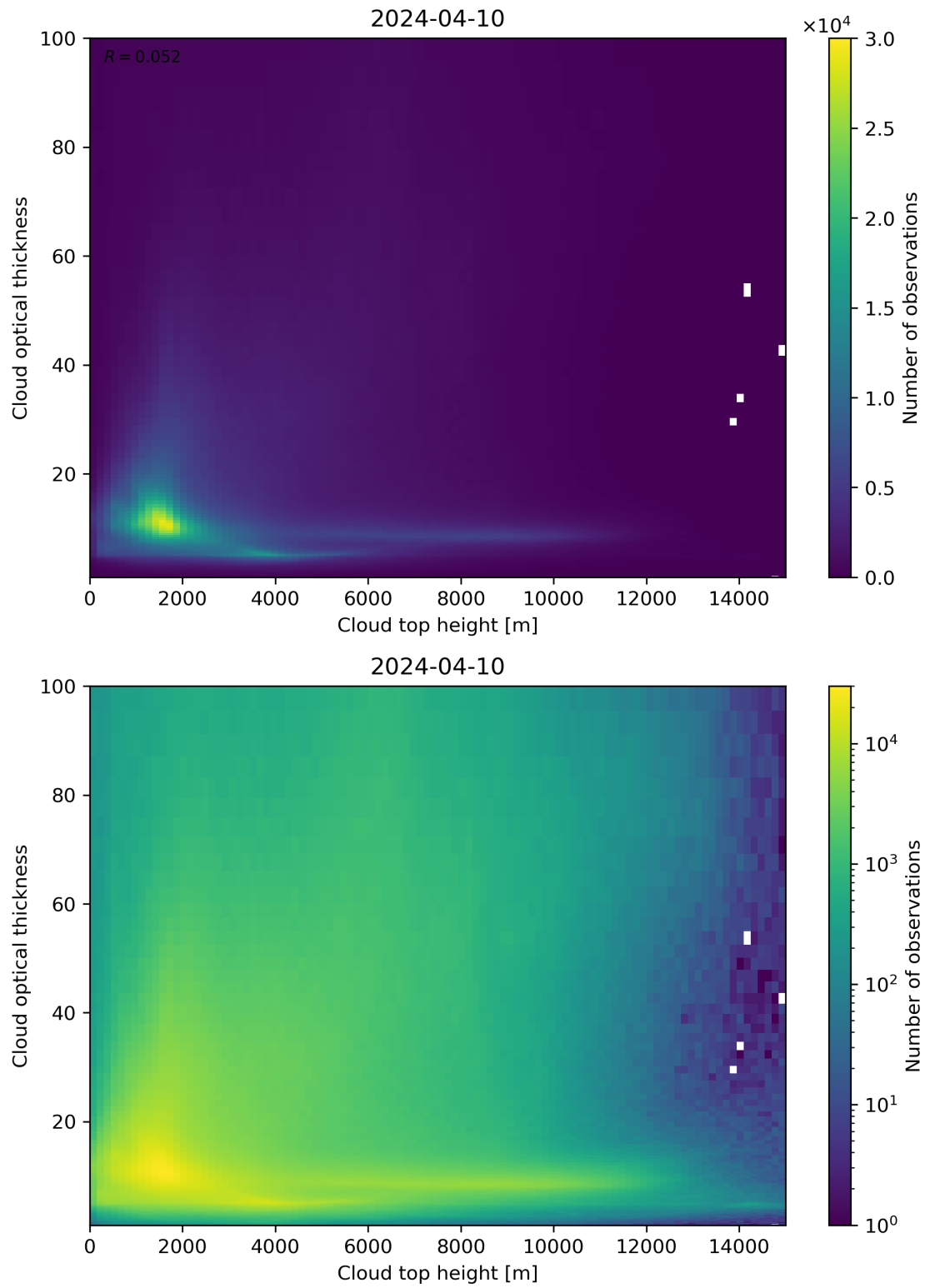
Figure 90: Scatter density plot of “Cloud top height” against “Cloud optical thickness” for 2024-04-10 to 2024-04-11.
