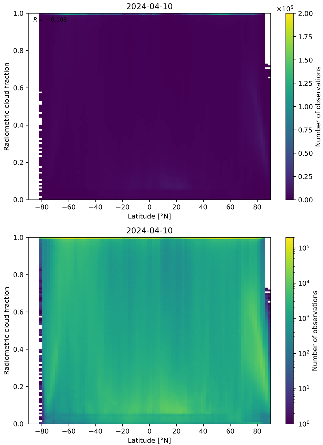
Figure 92: Scatter density plot of “Latitude” against “Radiometric cloud fraction” for 2024-04-10 to 2024-04-11.
