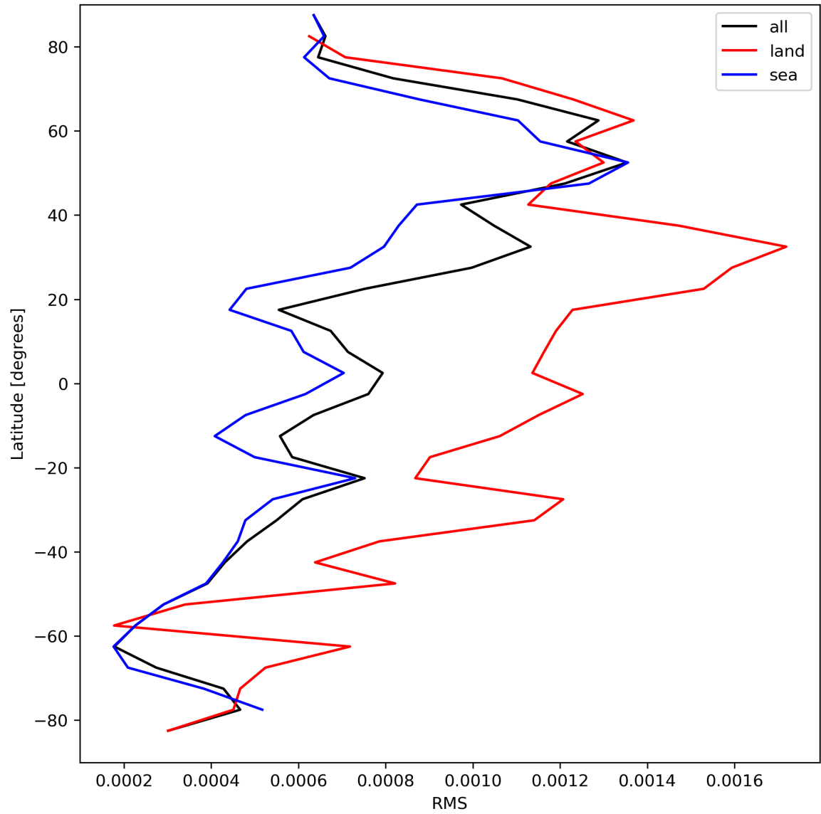
Figure 31: Zonal average of “RMS” for 2024-04-10 to 2024-04-11.
