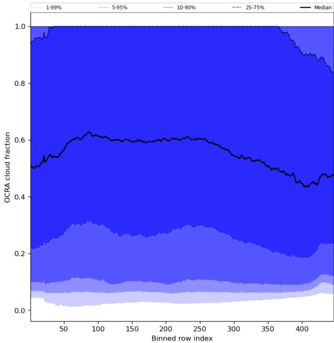
Figure 66: Along track statistics of “OCRA cloud fraction” for 2024-04-10 to 2024-04-11
