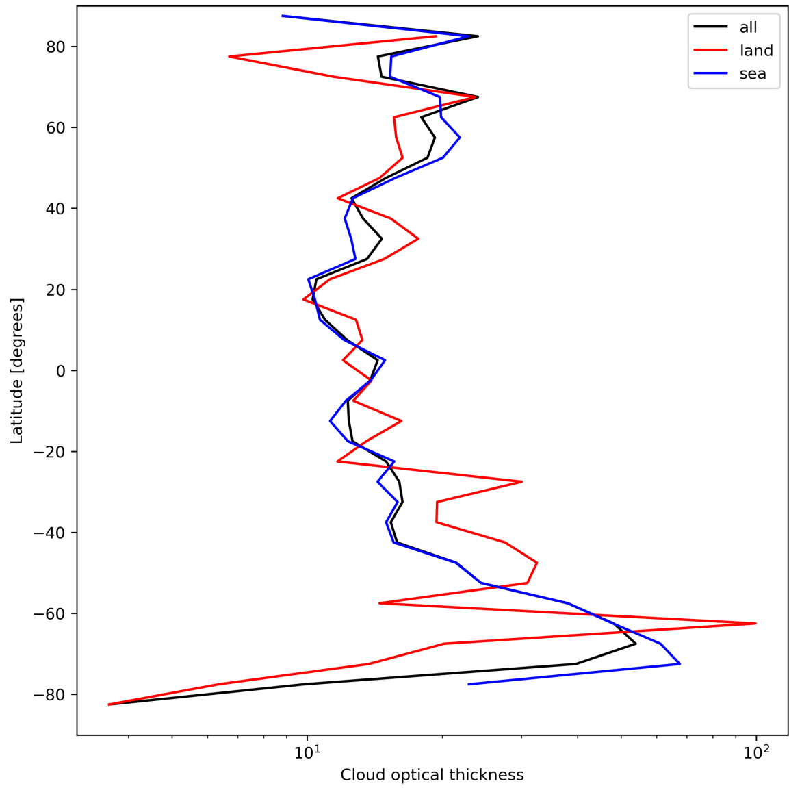
Figure 25: Zonal average of “Cloud optical thickness” for 2024-04-10 to 2024-04-11.
