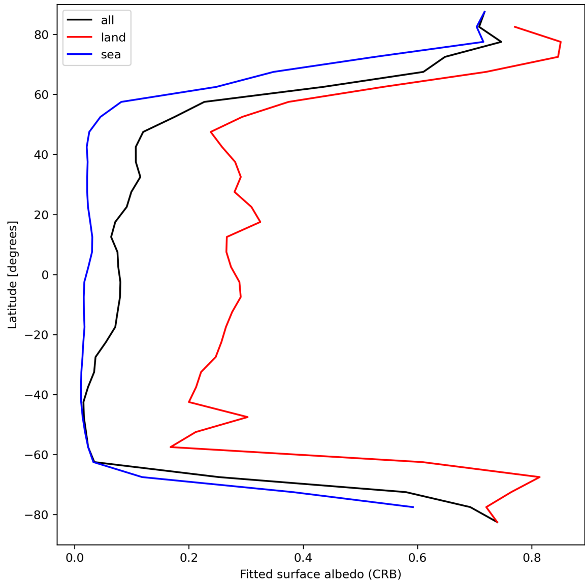
Figure 30: Zonal average of “Fitted surface albedo (CRB)” for 2024-04-10 to 2024-04-11.
