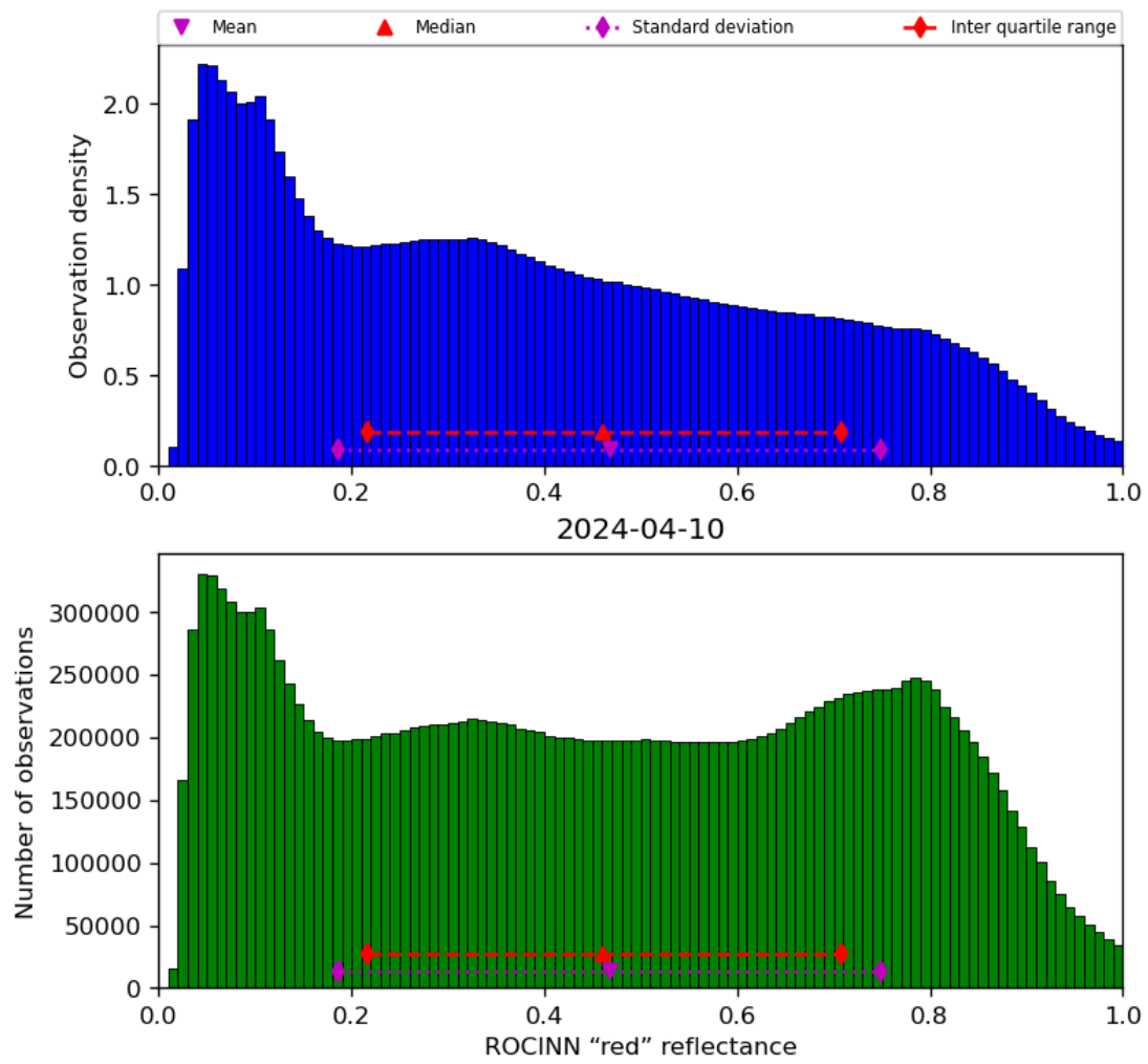
Figure 53: Histogram of “ROCINN “red” reflectance” for 2024-04-10 to 2024-04-11
