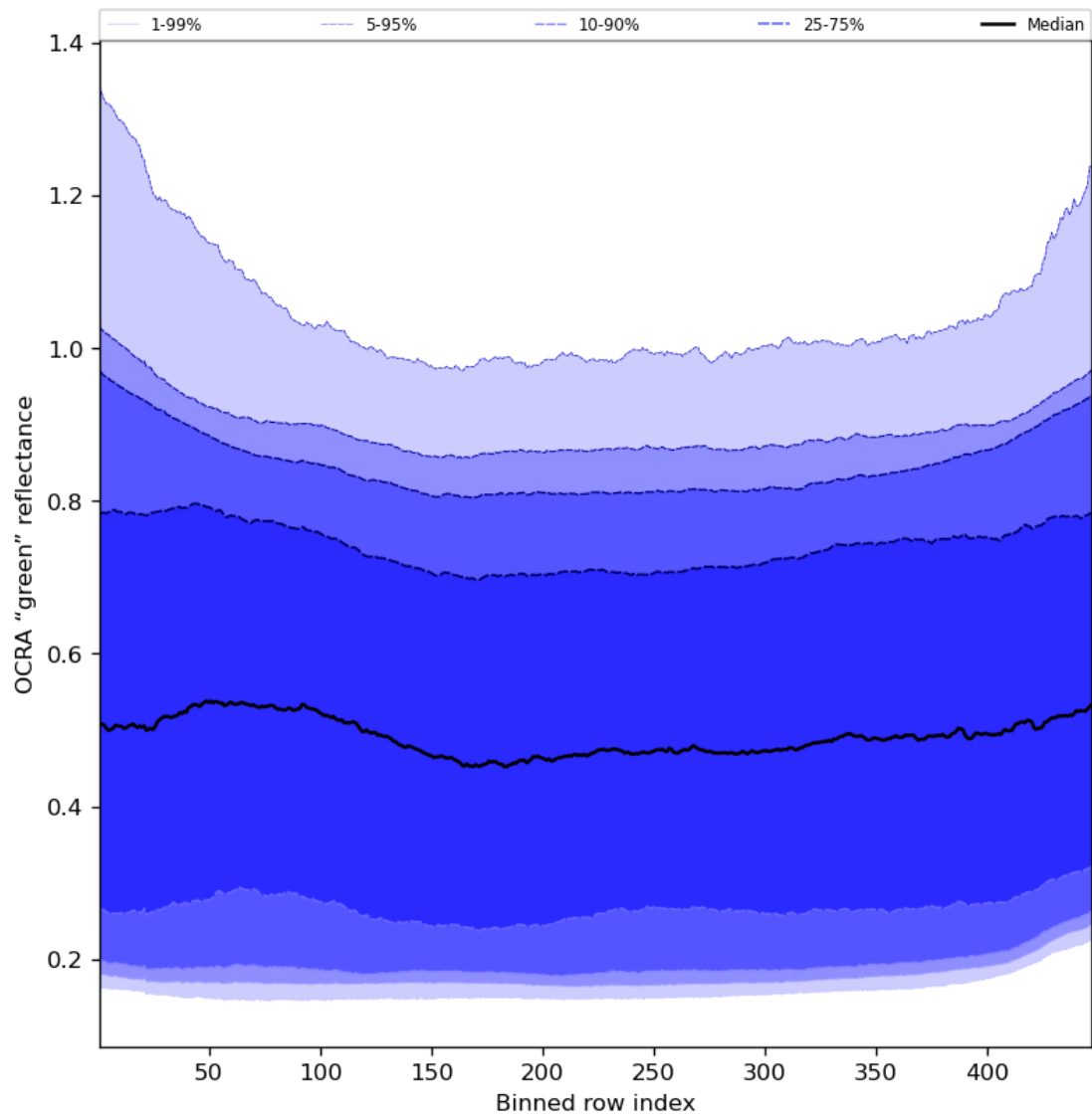
Figure 68: Along track statistics of "OCRA "green" reflectance" for 2024-04-10 to 2024-04-11
