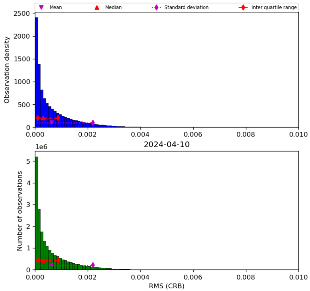
Figure 48: Histogram of “RMS (CRB)” for 2024-04-10 to 2024-04-11
