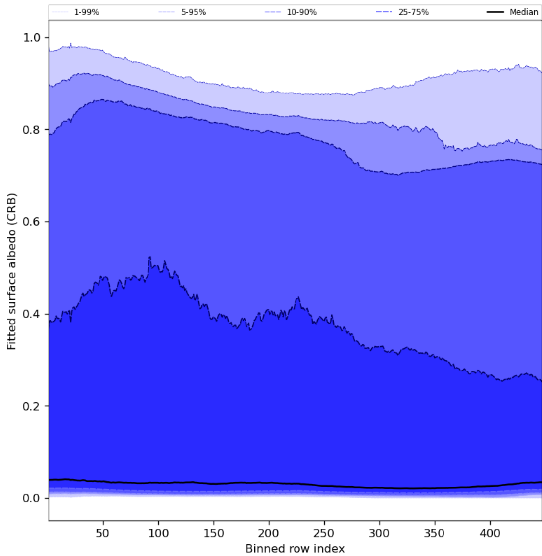
Figure 62: Along track statistics of “Fitted surface albedo (CRB)” for 2024-04-10 to 2024-04-11
