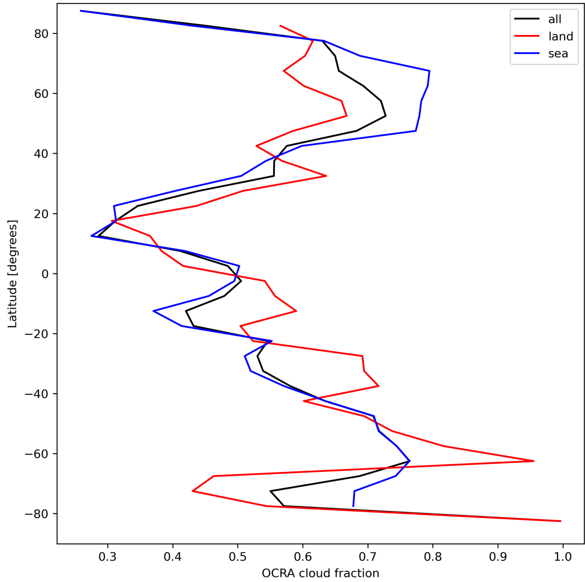
Figure 34: Zonal average of “OCRA cloud fraction” for 2024-04-10 to 2024-04-11.
