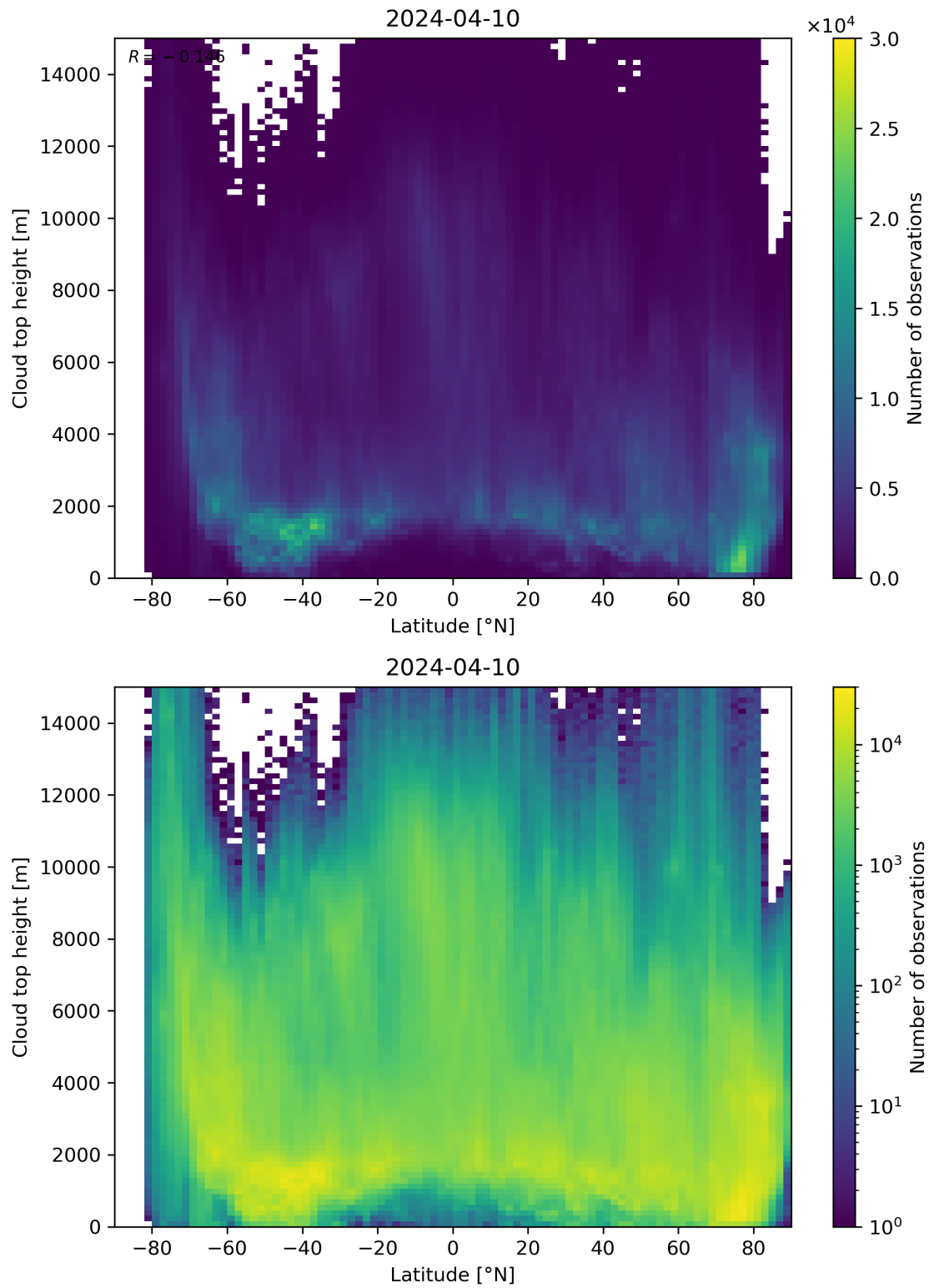
Figure 97: Scatter density plot of “Latitude” against “Cloud top height” for 2024-04-10 to 2024-04-11.
