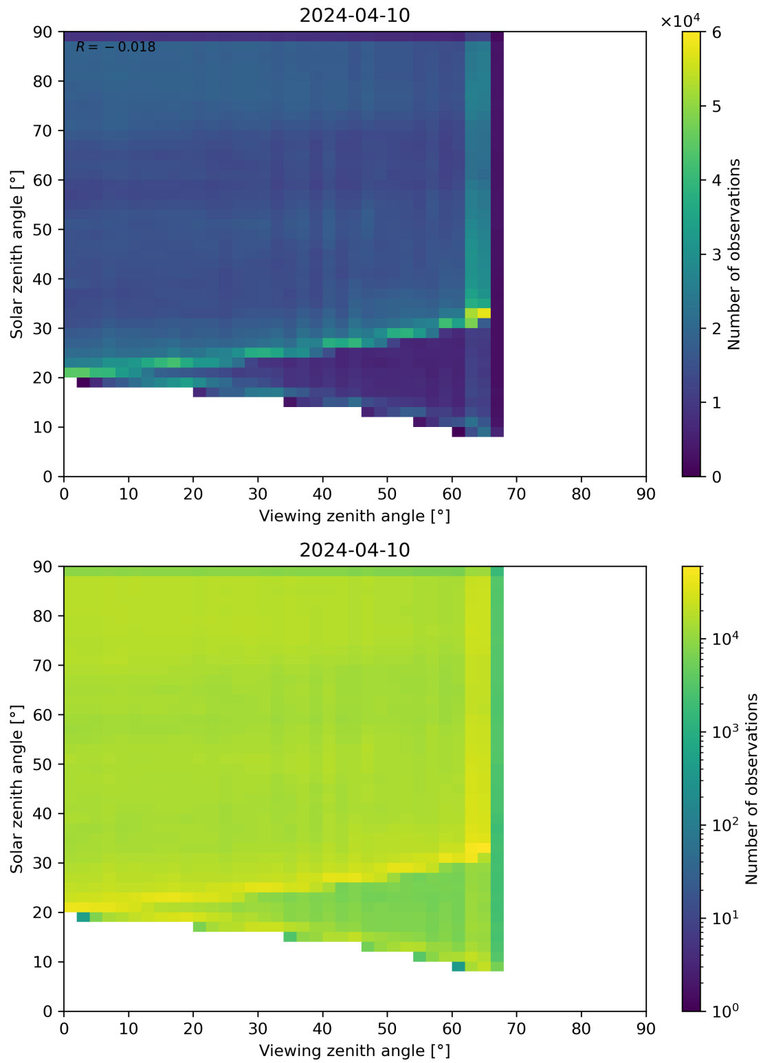
Figure 114: Scatter density plot of “Viewing zenith angle” against “Solar zenith angle” for 2024-04-10 to 2024-04-11.
