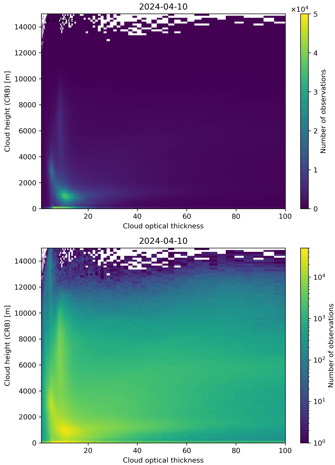
Figure 85: Scatter density plot of “Cloud optical thickness” against “Cloud height (CRB)” for 2024-04-10 to 2024-04-11.
