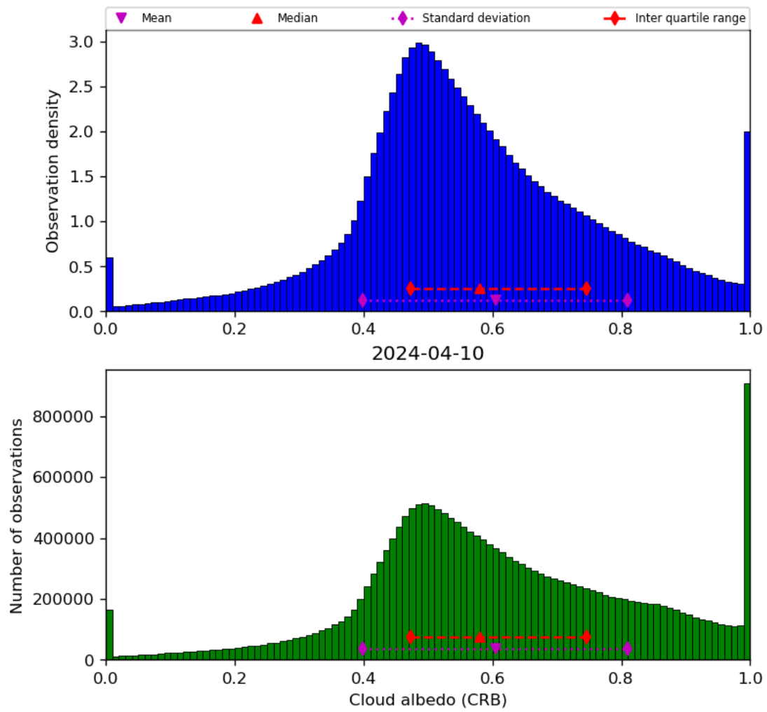
Figure 44: Histogram of “Cloud albedo (CRB)” for 2024-04-10 to 2024-04-11
