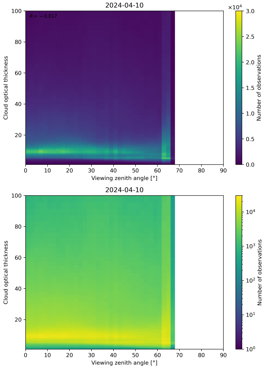
Figure 111: Scatter density plot of “Viewing zenith angle” against “Cloud optical thickness” for 2024-04-10 to 2024-04-11.
