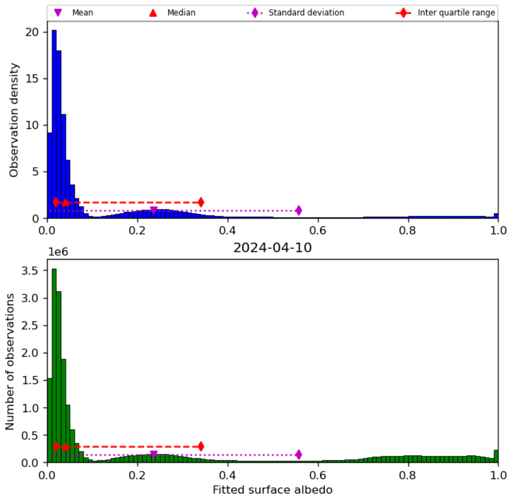
Figure 45: Histogram of “Fitted surface albedo” for 2024-04-10 to 2024-04-11
