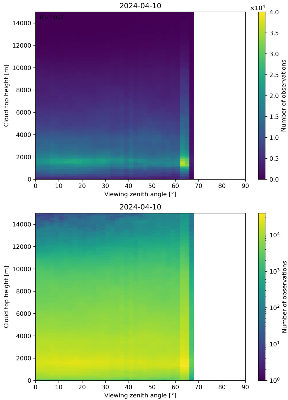
Figure 112: Scatter density plot of “Viewing zenith angle” against “Cloud top height” for 2024-04-10 to 2024-04-11.
