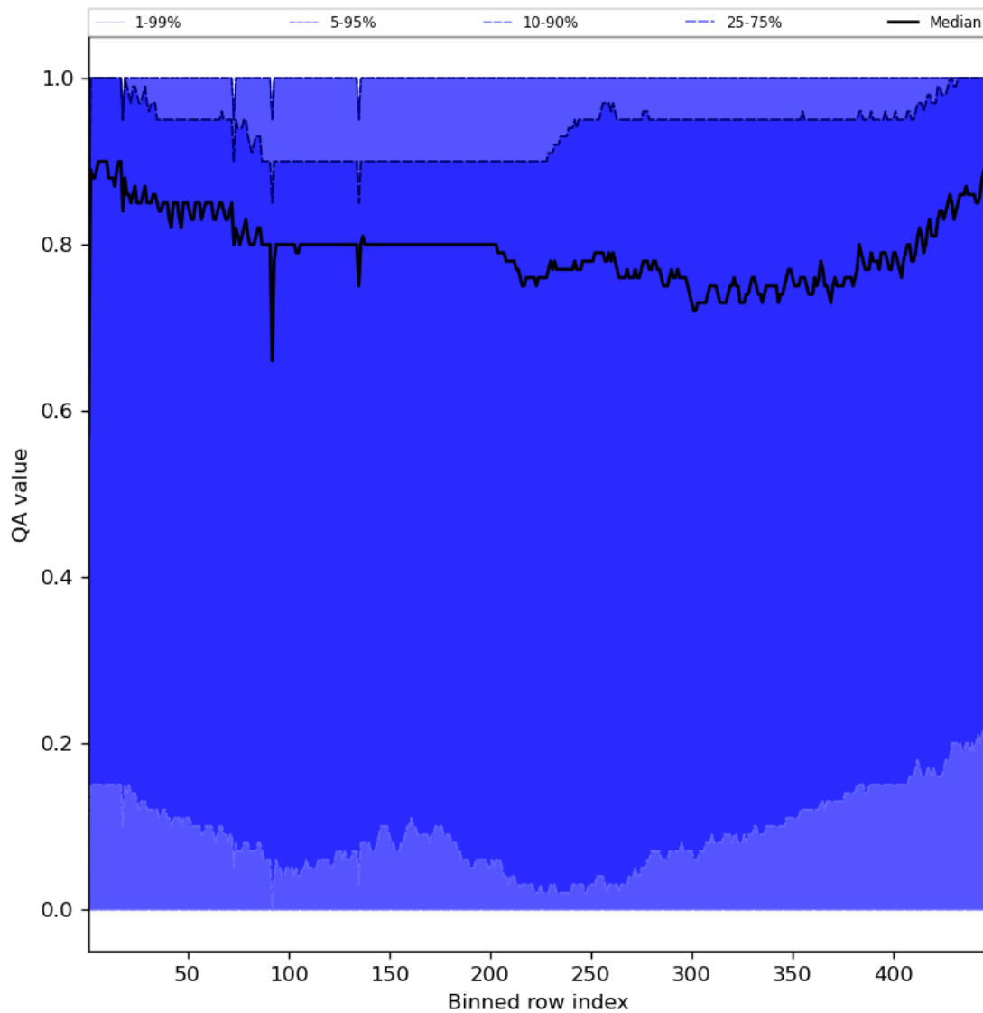
Figure 54: Along track statistics of “QA value” for 2024-04-10 to 2024-04-11
