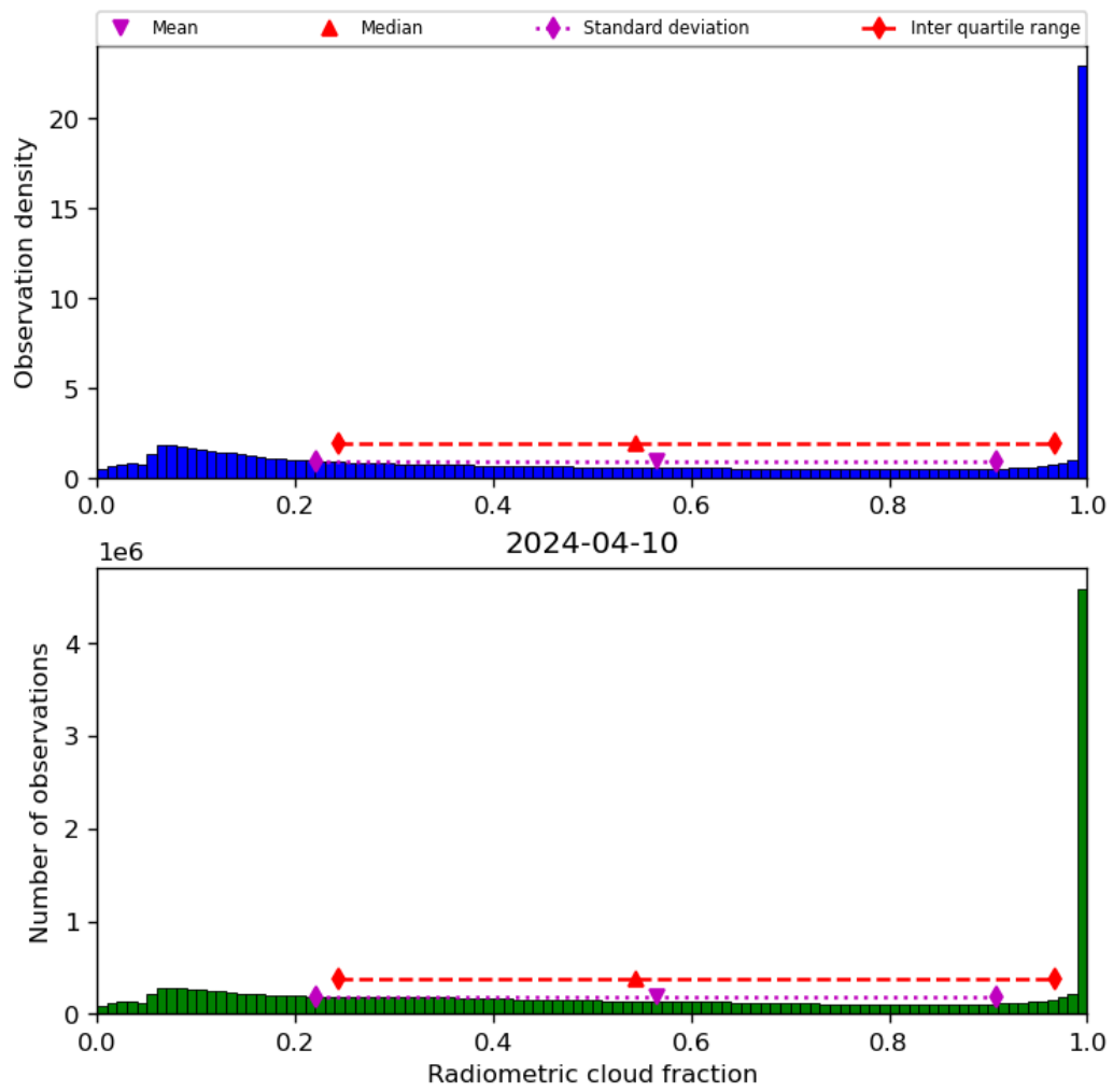
Figure 39: Histogram of “Radiometric cloud fraction” for 2024-04-10 to 2024-04-11
