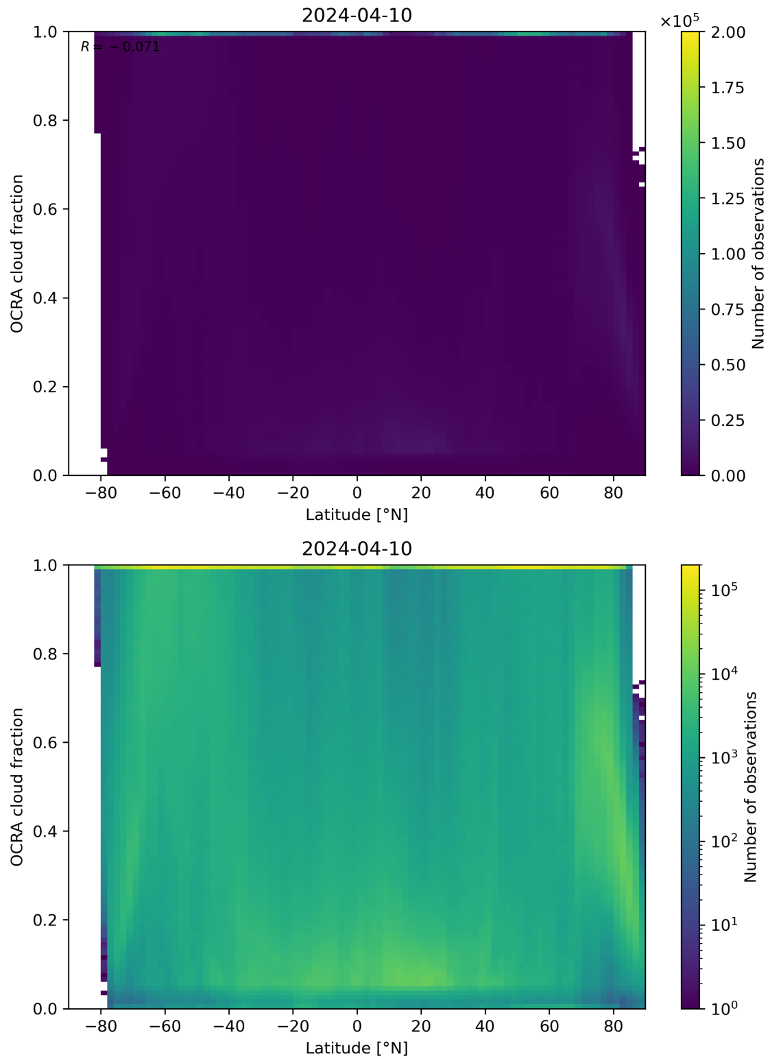
Figure 93: Scatter density plot of “Latitude” against “OCRA cloud fraction” for 2024-04-10 to 2024-04-11.
