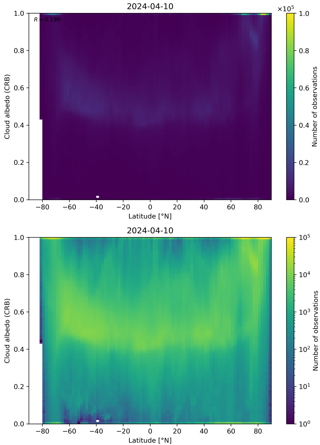
Figure 91: Scatter density plot of “Latitude” against “Cloud albedo (CRB)” for 2024-04-10 to 2024-04-11.
