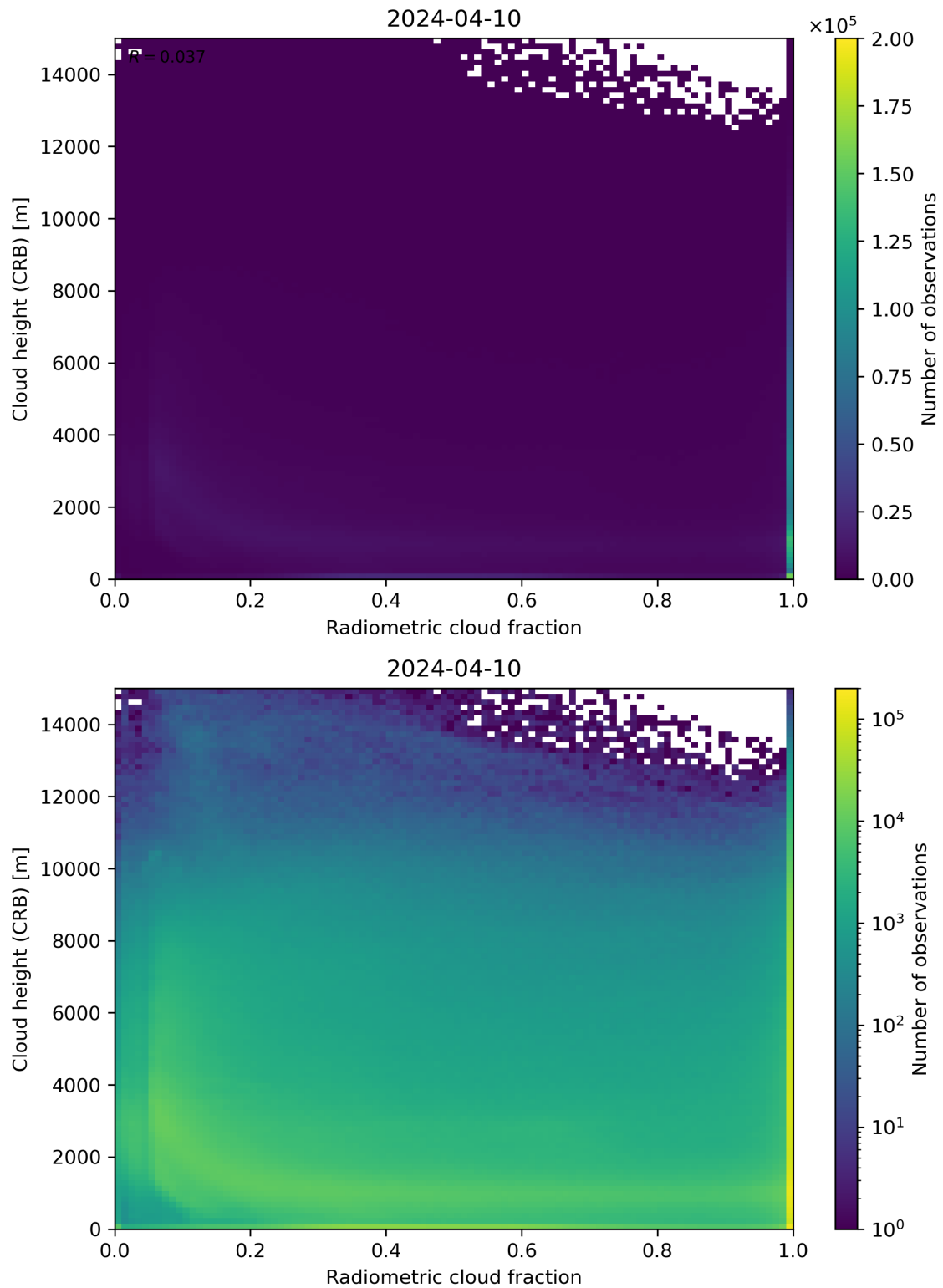
Figure 74: Scatter density plot of “Radiometric cloud fraction” against “Cloud height (CRB)” for 2024-04-10 to 2024-04-11.
