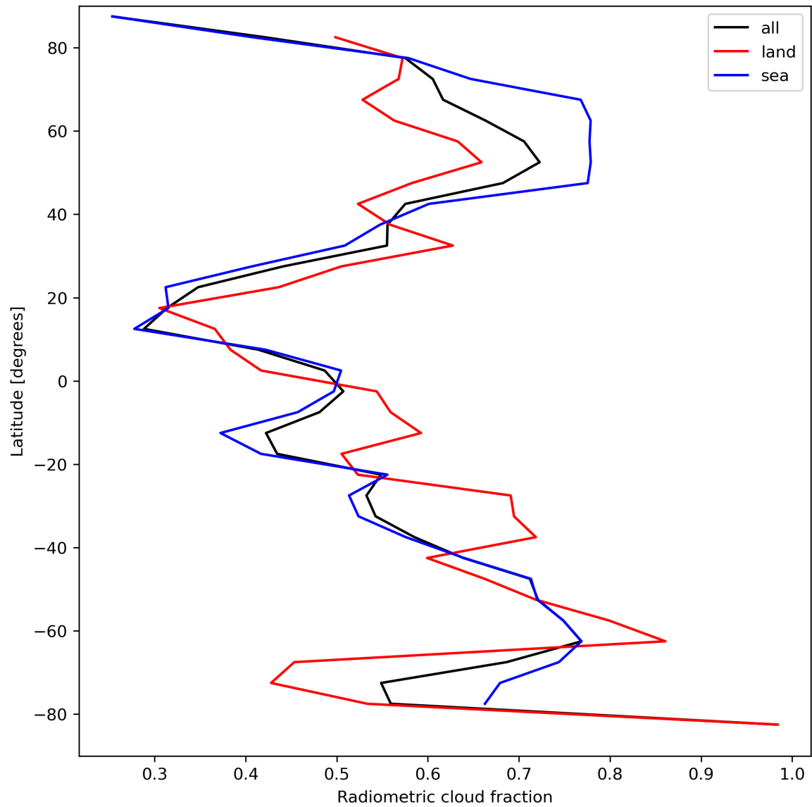
Figure 23: Zonal average of “Radiometric cloud fraction” for 2024-04-10 to 2024-04-11.
