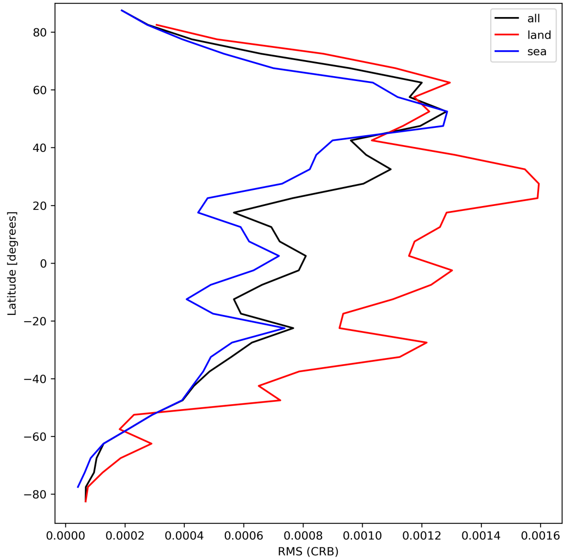
Figure 32: Zonal average of “RMS (CRB)” for 2024-04-10 to 2024-04-11.
