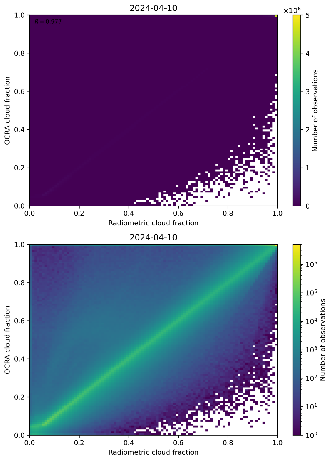
Figure 72: Scatter density plot of “Radiometric cloud fraction” against “OCRA cloud fraction” for 2024-04-10 to 2024-04-11.
