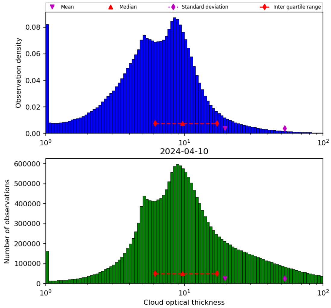
Figure 41: Histogram of “Cloud optical thickness” for 2024-04-10 to 2024-04-11
