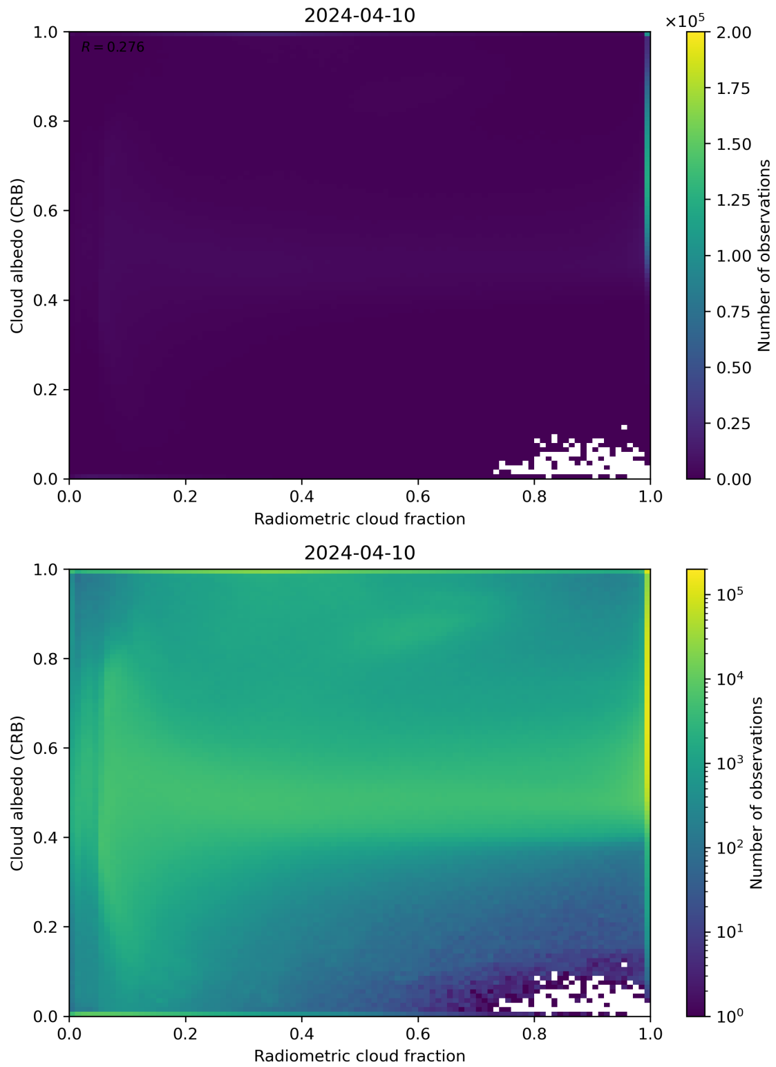
Figure 71: Scatter density plot of “Radiometric cloud fraction” against “Cloud albedo (CRB)” for 2024-04-10 to 2024-04-11.
