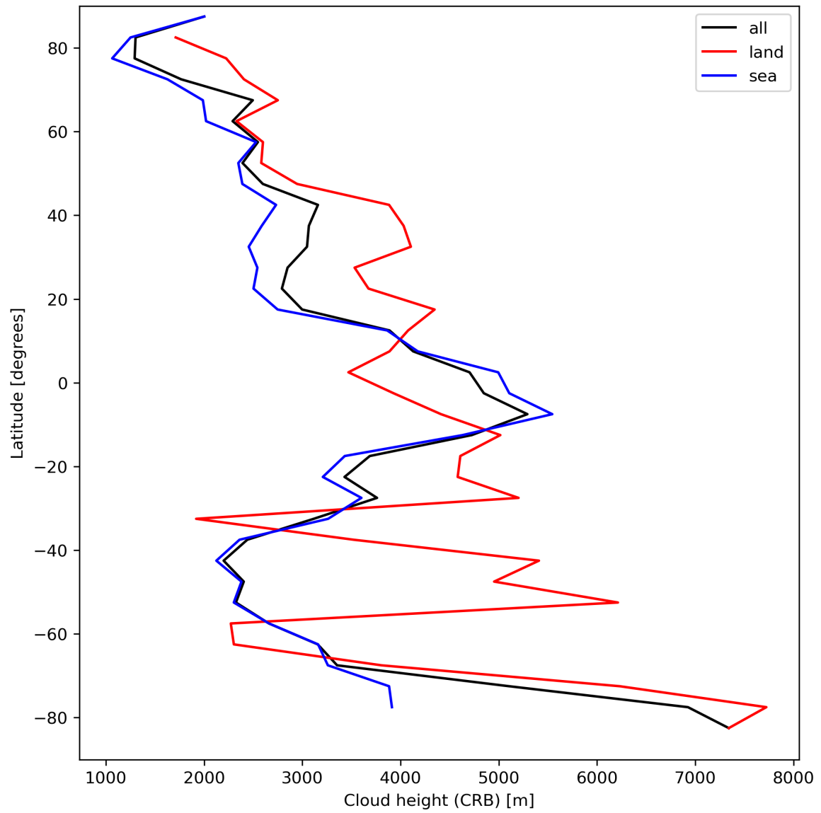
Figure 27: Zonal average of “Cloud height (CRB)” for 2024-04-10 to 2024-04-11.
