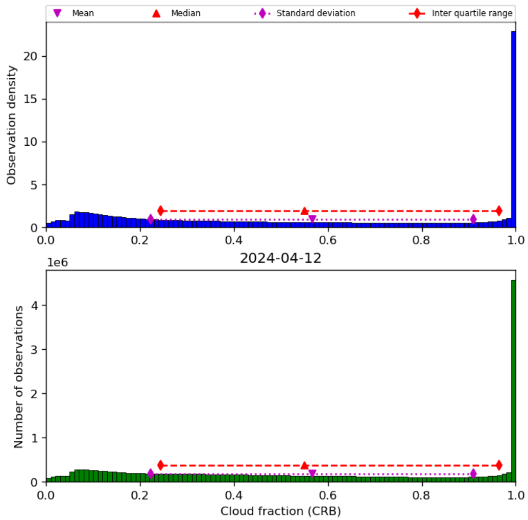
Figure 42: Histogram of “Cloud fraction (CRB)” for 2024-04-11 to 2024-04-13
