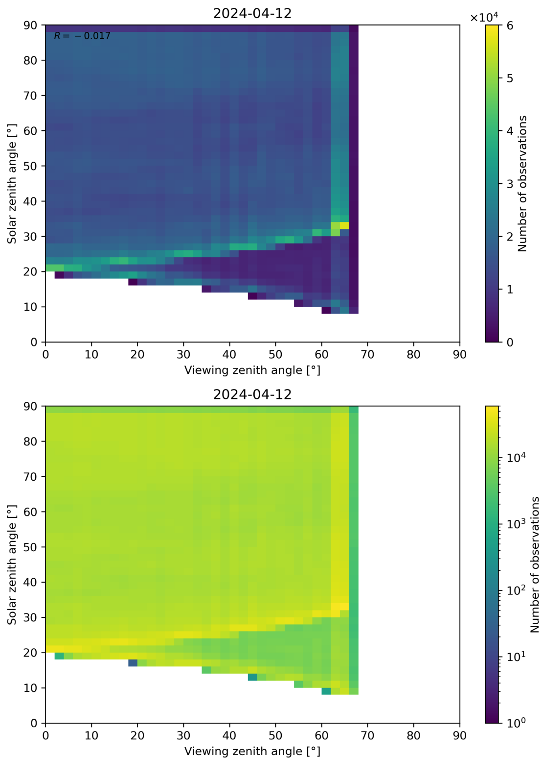
Figure 114: Scatter density plot of “Viewing zenith angle” against “Solar zenith angle” for 2024-04-11 to 2024-04-13.
