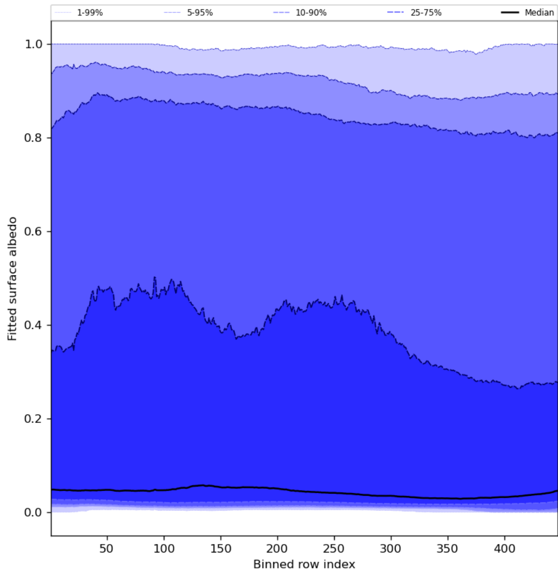
Figure 61: Along track statistics of “Fitted surface albedo” for 2024-04-11 to 2024-04-13
