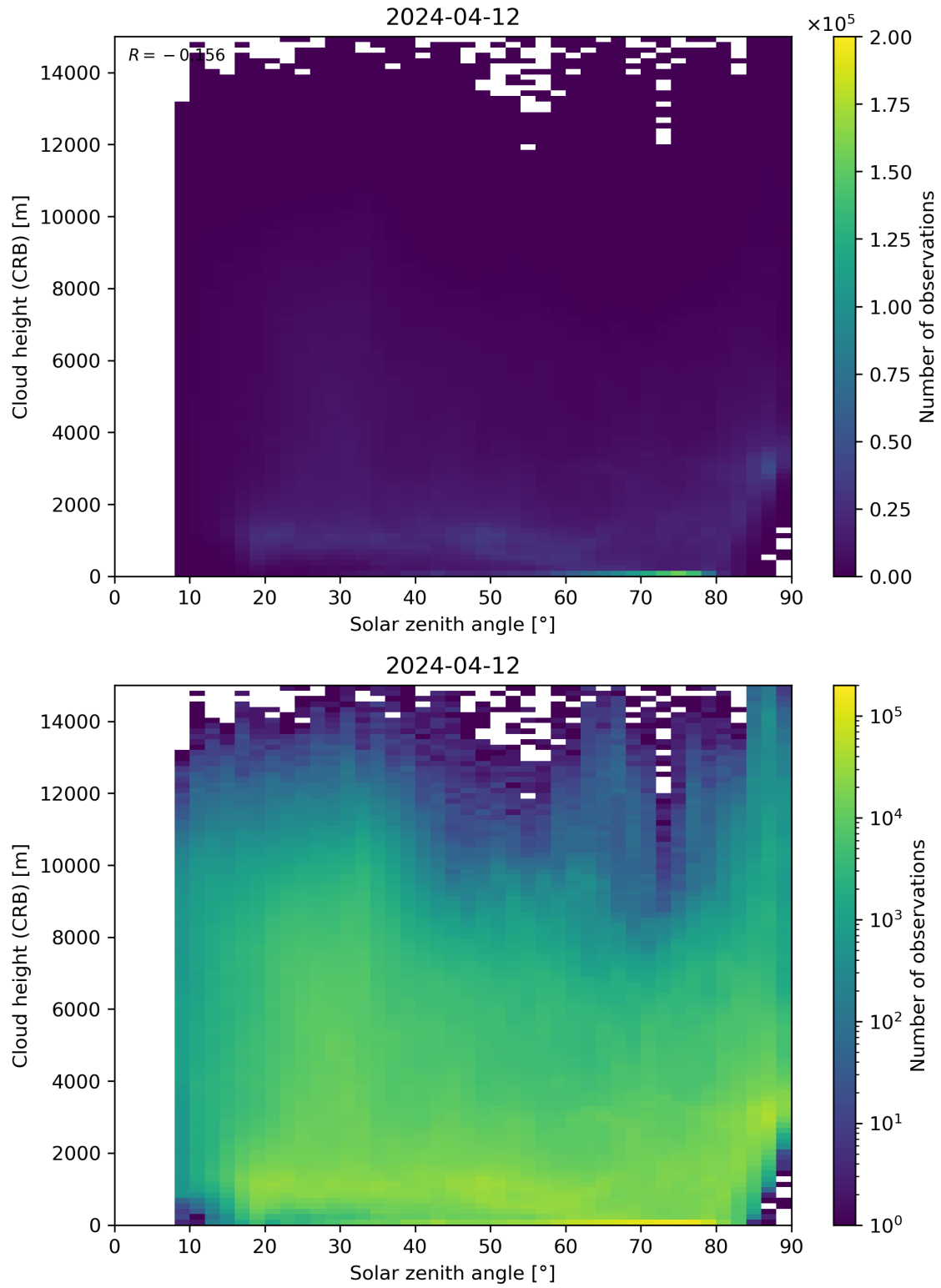
Figure 102: Scatter density plot of “Solar zenith angle” against “Cloud height (CRB)” for 2024-04-11 to 2024-04-13.
