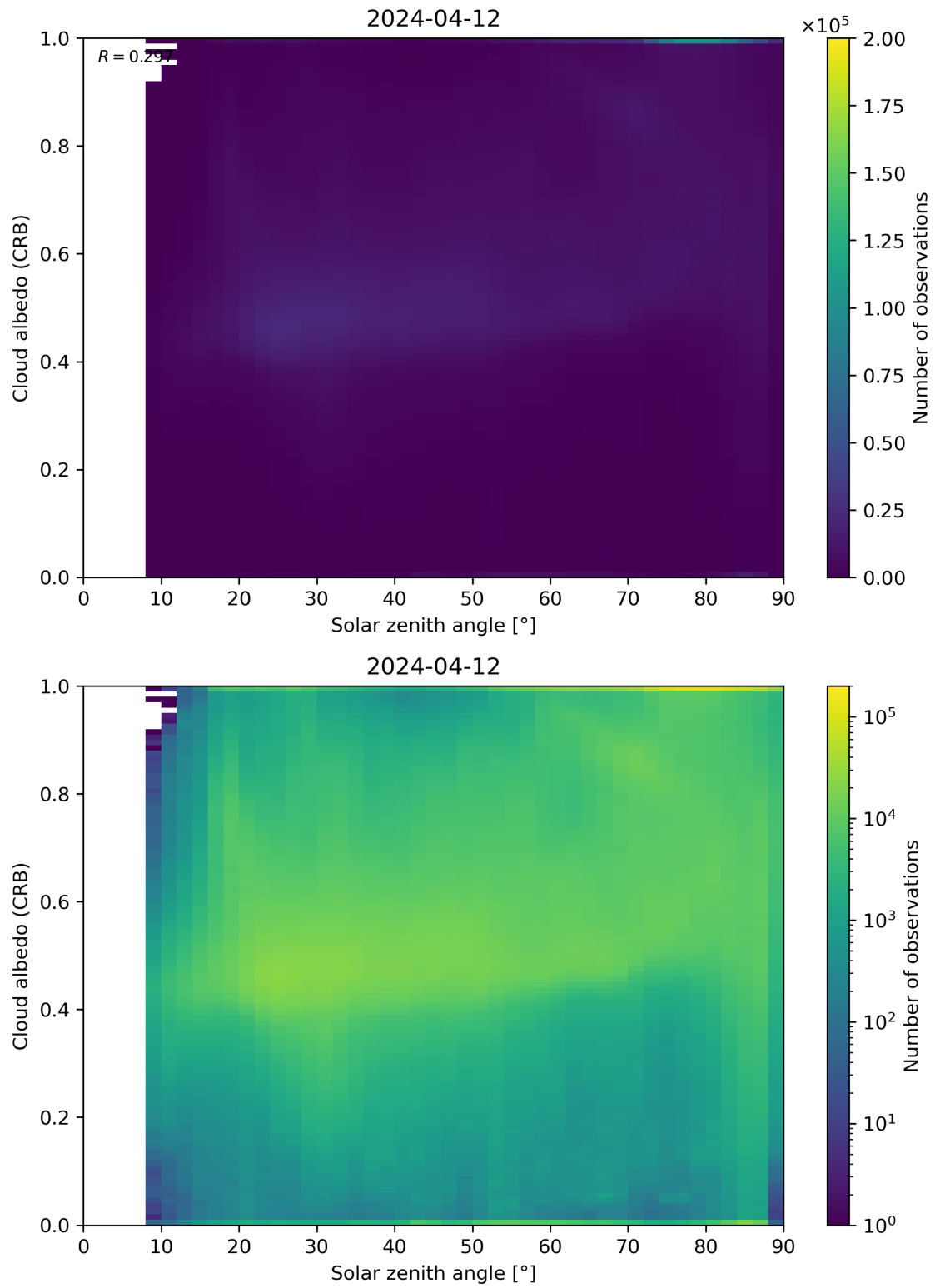
Figure 98: Scatter density plot of “Solar zenith angle” against “Cloud albedo (CRB)” for 2024-04-11 to 2024-04-13.
