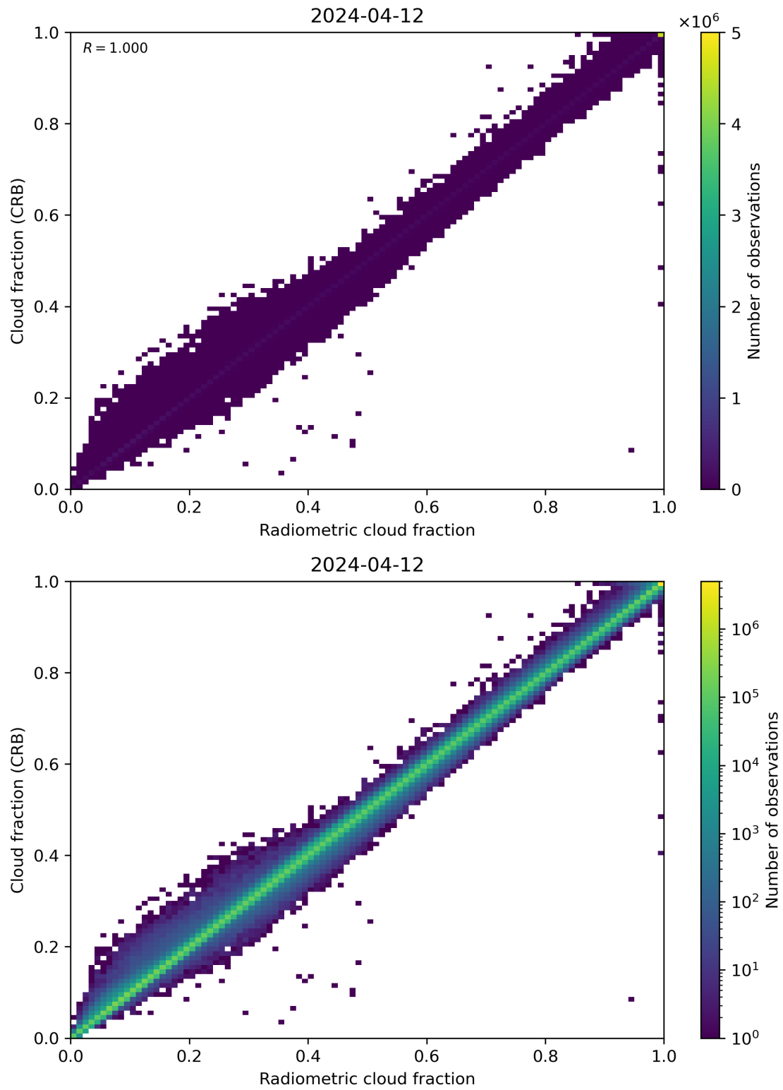
Figure 73: Scatter density plot of “Radiometric cloud fraction” against “Cloud fraction (CRB)” for 2024-04-11 to 2024-04-13.
