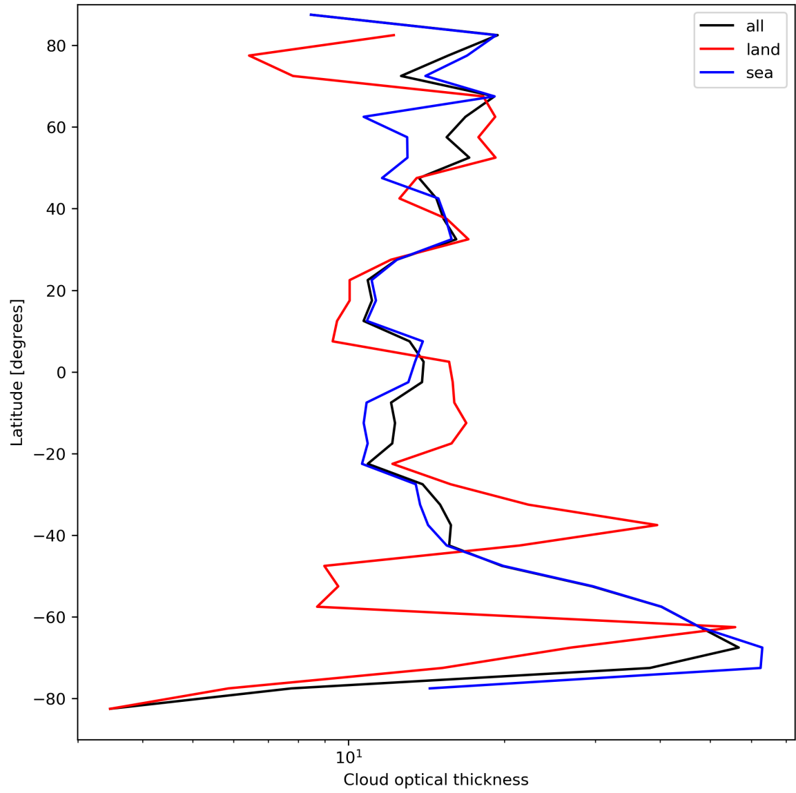
Figure 25: Zonal average of “Cloud optical thickness” for 2024-04-11 to 2024-04-13.
