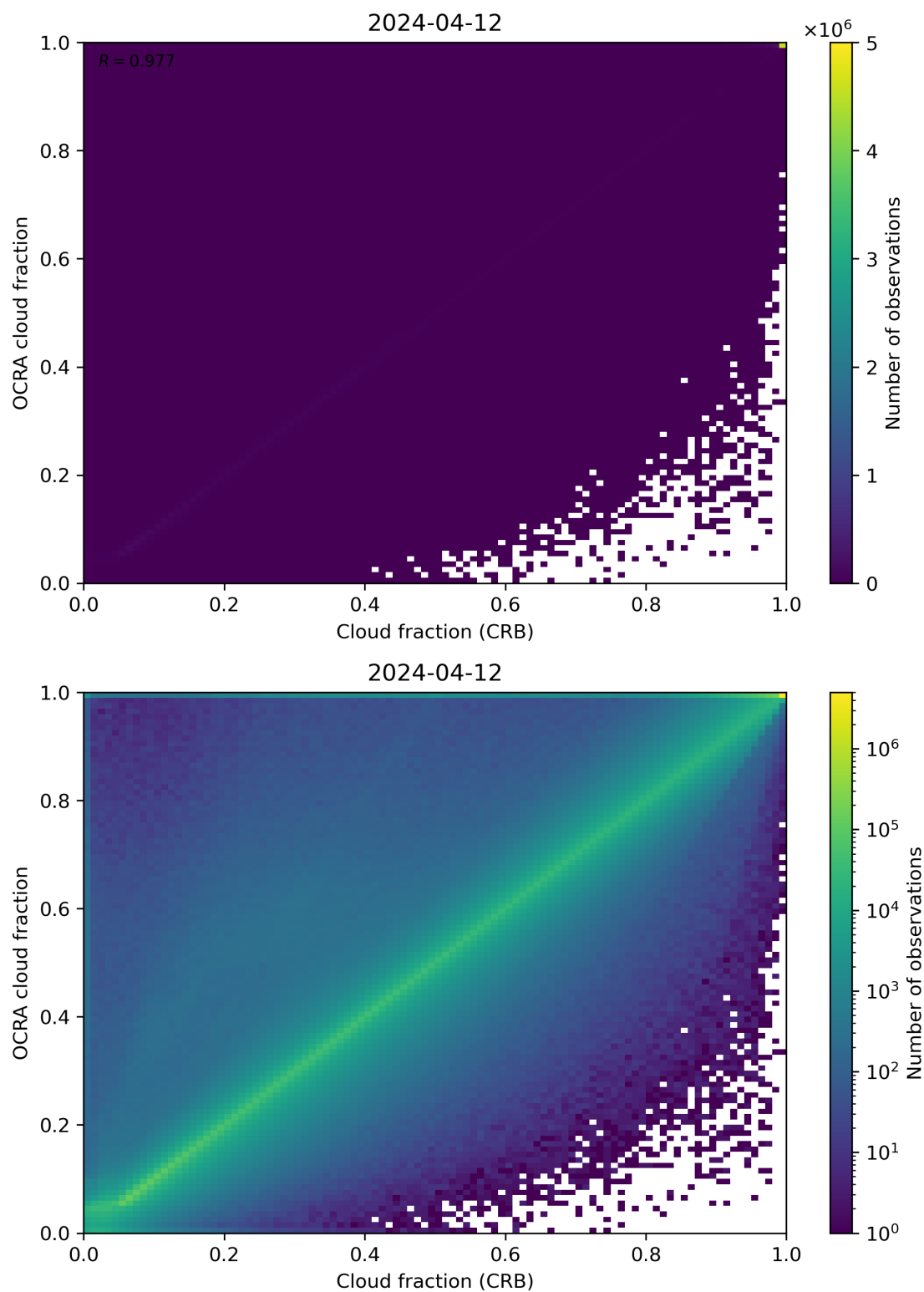
Figure 78: Scatter density plot of “Cloud fraction (CRB)” against “OCRA cloud fraction” for 2024-04-11 to 2024-04-13.
