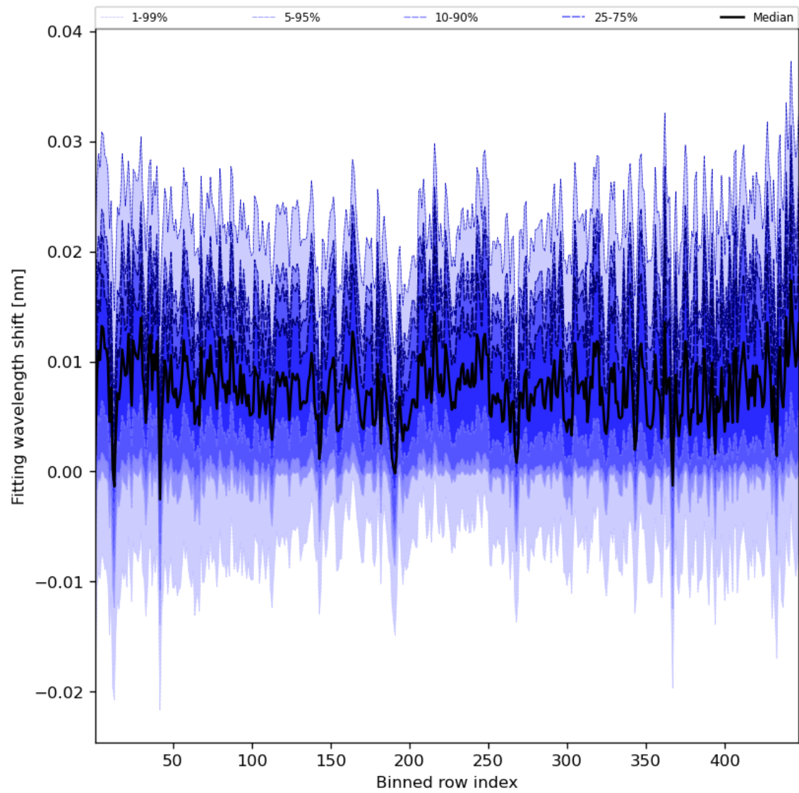
Figure 65: Along track statistics of “Fitting wavelength shift” for 2024-04-11 to 2024-04-13
