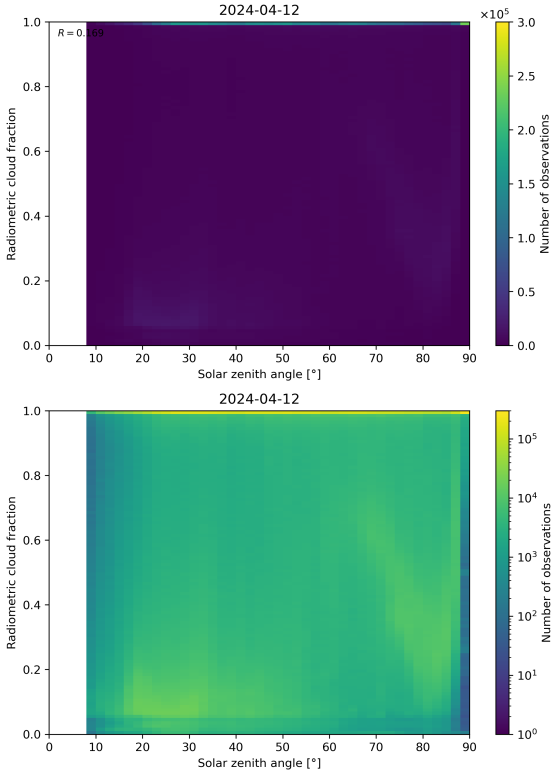
Figure 99: Scatter density plot of “Solar zenith angle” against “Radiometric cloud fraction” for 2024-04-11 to 2024-04-13.
