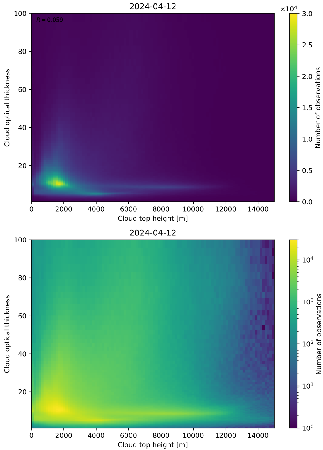
Figure 90: Scatter density plot of “Cloud top height” against “Cloud optical thickness” for 2024-04-11 to 2024-04-13.
