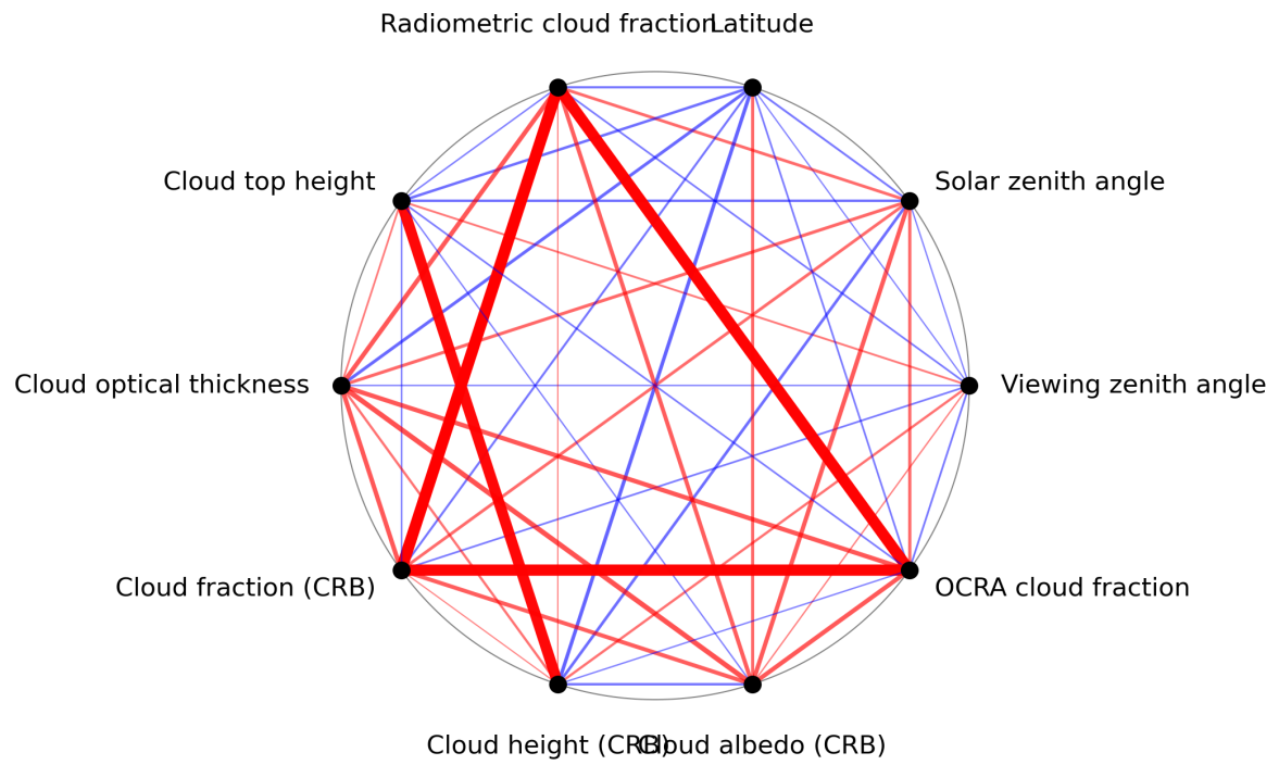
Figure 1: Map of correlation graph for 2024-04-11 to 2024-04-13.
