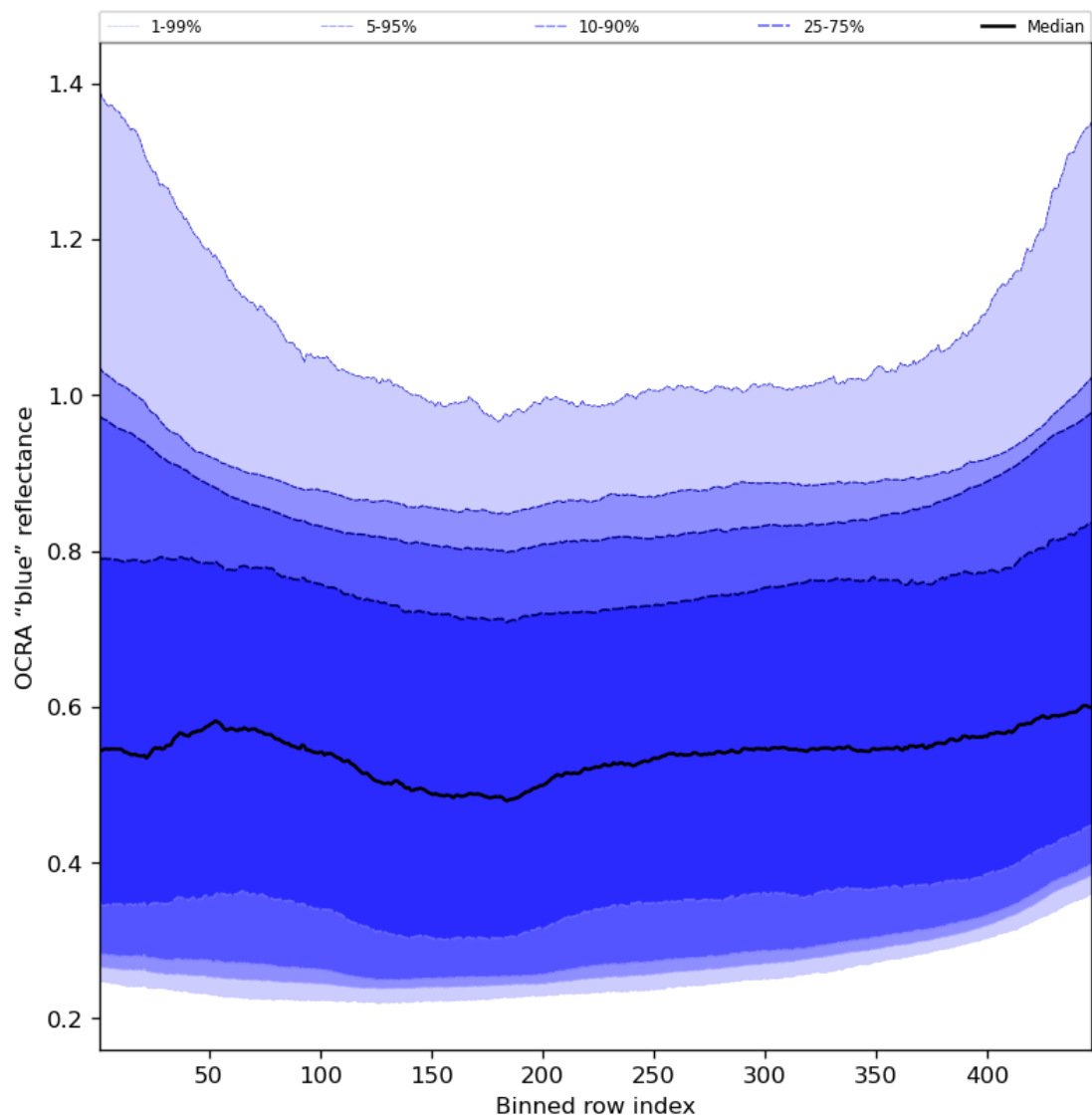
Figure 67: Along track statistics of “OCRA “blue” reflectance” for 2024-04-11 to 2024-04-13
