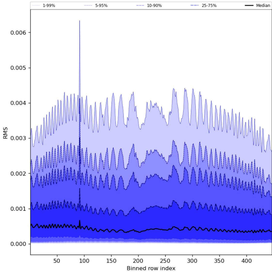
Figure 63: Along track statistics of “RMS” for 2024-04-11 to 2024-04-13
