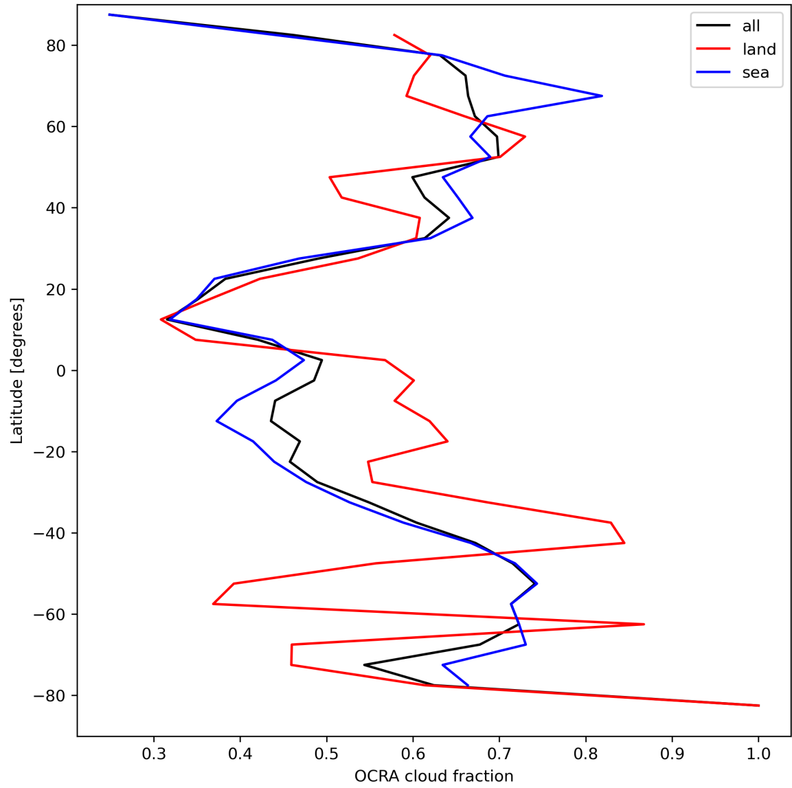
Figure 34: Zonal average of “OCRA cloud fraction” for 2024-04-11 to 2024-04-13.
