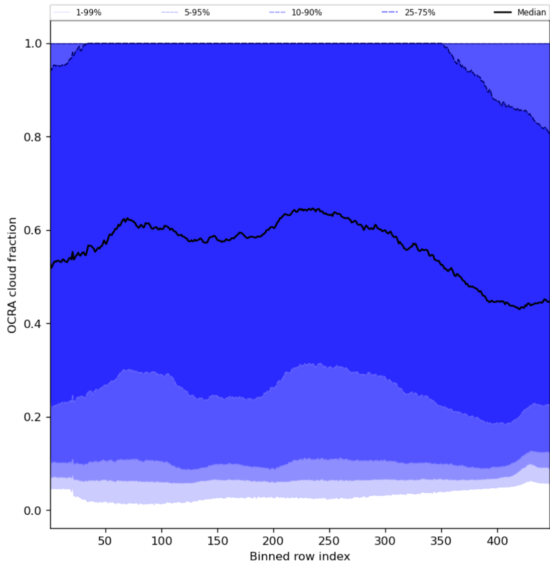
Figure 66: Along track statistics of “OCRA cloud fraction” for 2024-04-11 to 2024-04-13
