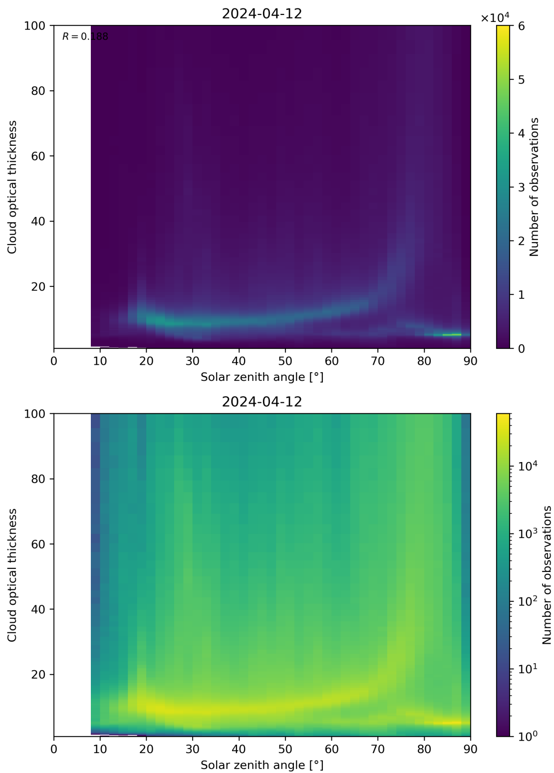
Figure 103: Scatter density plot of “Solar zenith angle” against “Cloud optical thickness” for 2024-04-11 to 2024-04-13.
