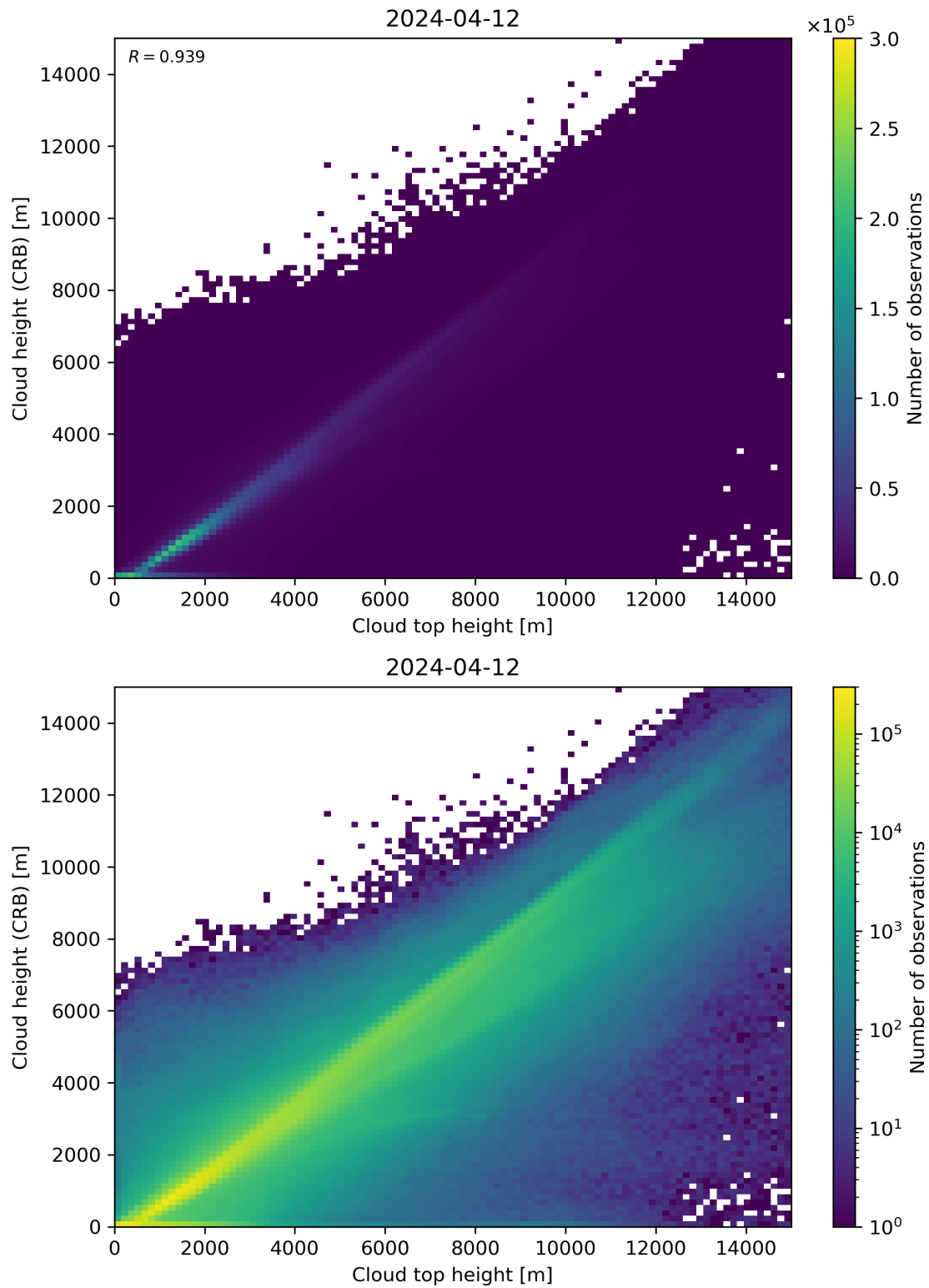
Figure 89: Scatter density plot of “Cloud top height” against “Cloud height (CRB)” for 2024-04-11 to 2024-04-13.
