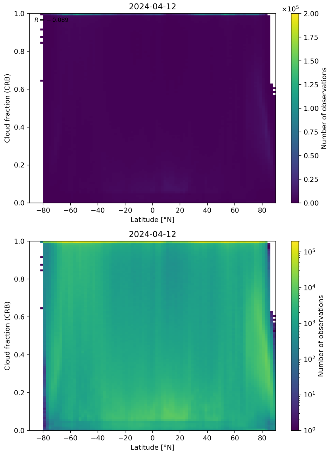
Figure 94: Scatter density plot of “Latitude” against “Cloud fraction (CRB)” for 2024-04-11 to 2024-04-13.
