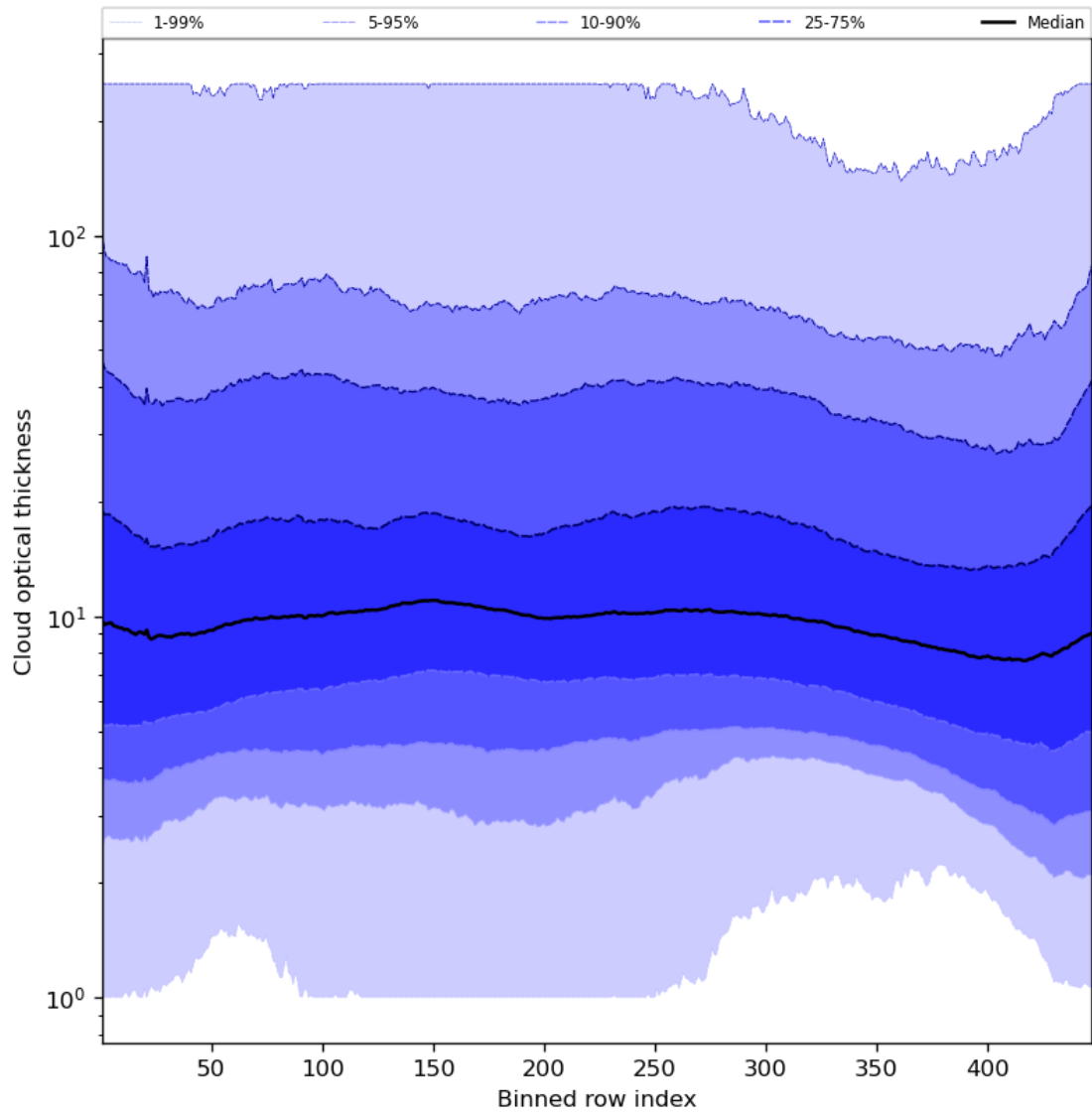
Figure 57: Along track statistics of “Cloud optical thickness” for 2024-04-11 to 2024-04-13
