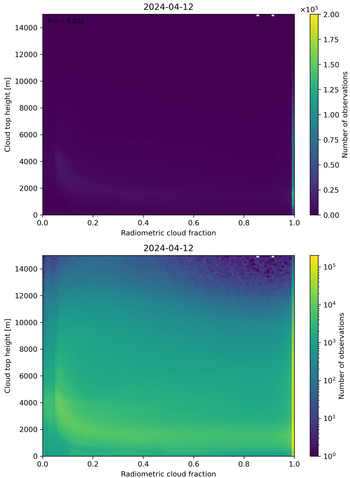
Figure 76: Scatter density plot of “Radiometric cloud fraction” against “Cloud top height” for 2024-04-11 to 2024-04-13.
