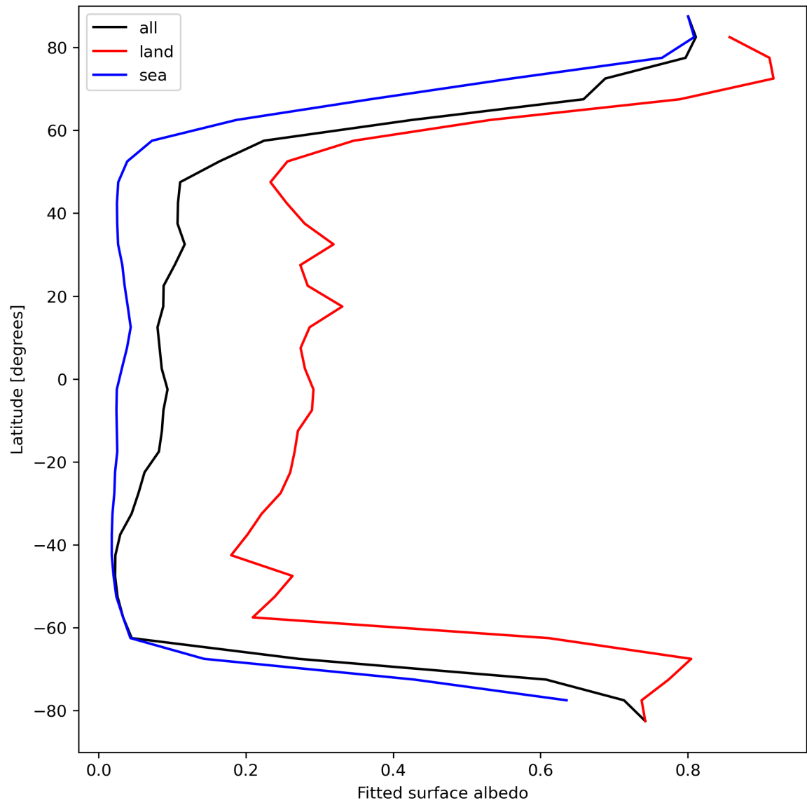
Figure 29: Zonal average of “Fitted surface albedo” for 2024-04-11 to 2024-04-13.
