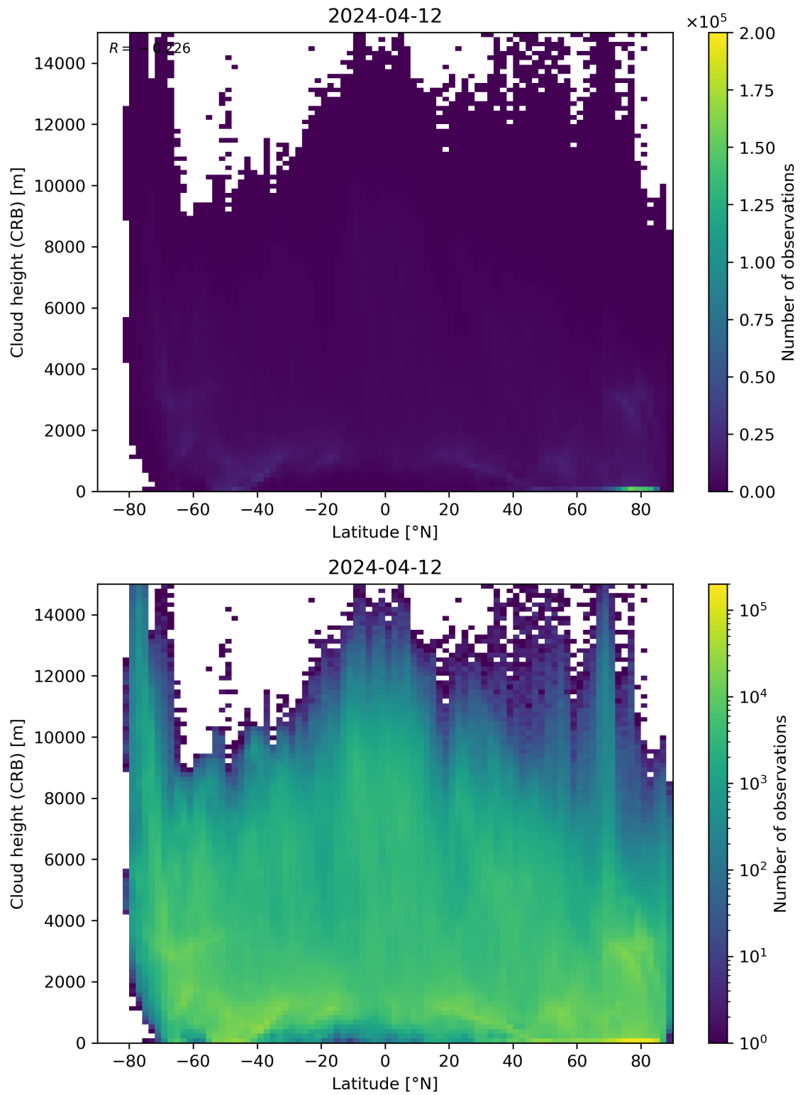
Figure 95: Scatter density plot of “Latitude” against “Cloud height (CRB)” for 2024-04-11 to 2024-04-13.
