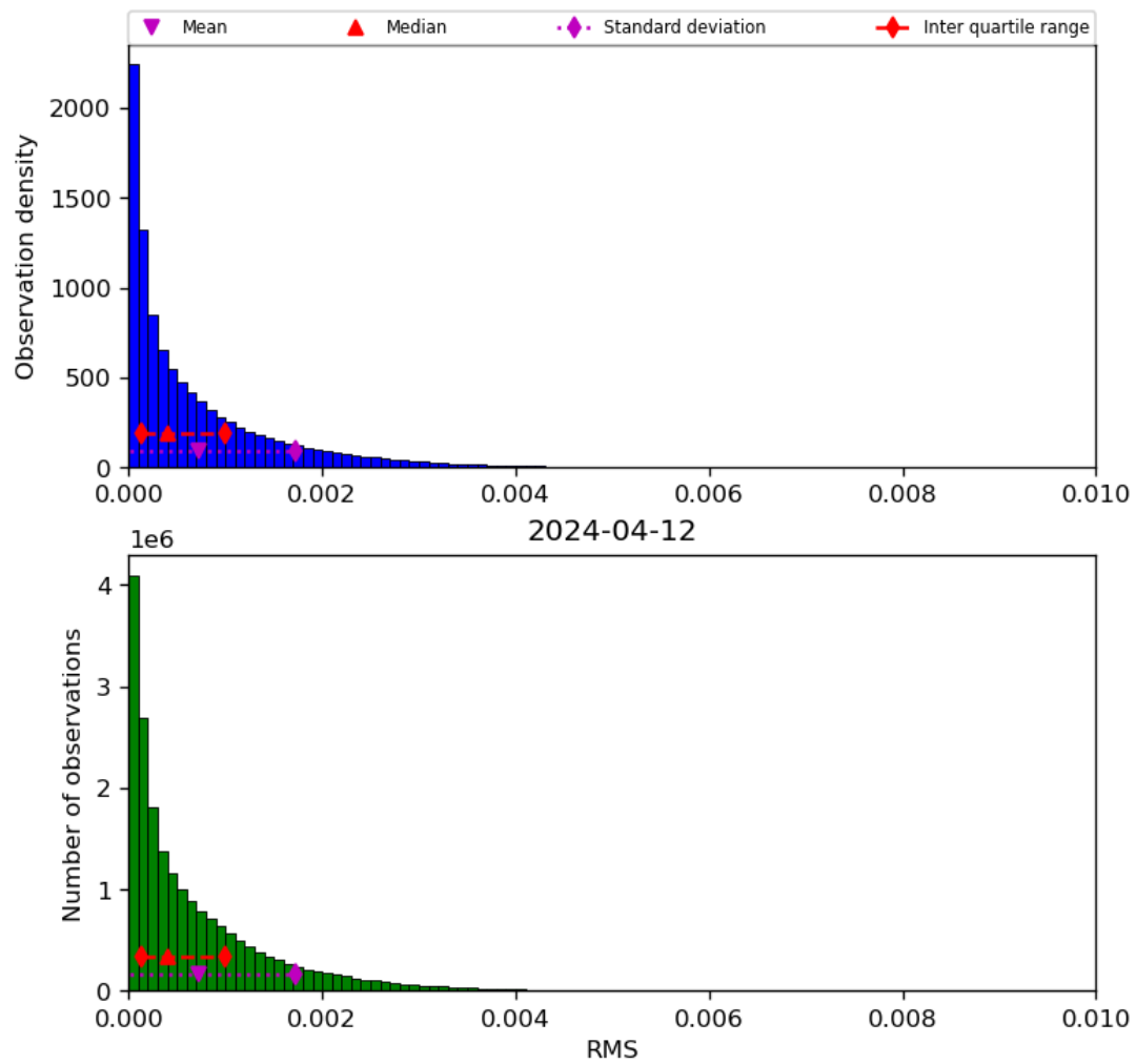
Figure 47: Histogram of “RMS” for 2024-04-11 to 2024-04-13
