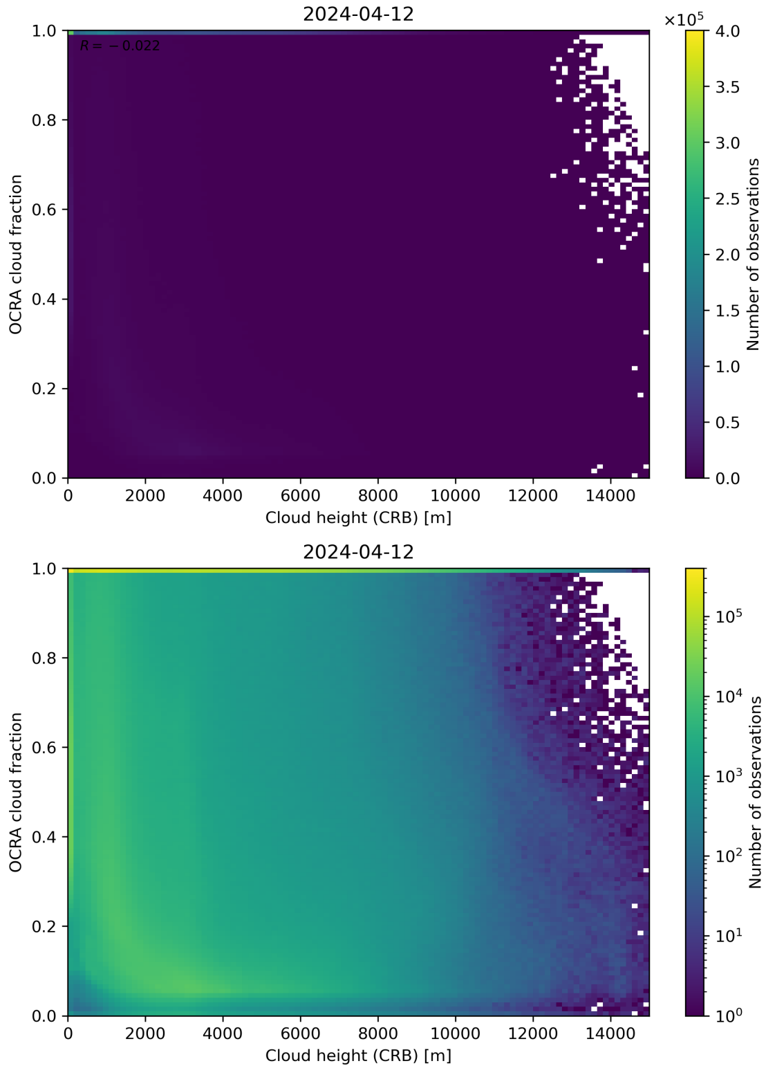
Figure 81: Scatter density plot of “Cloud height (CRB)” against “OCRA cloud fraction” for 2024-04-11 to 2024-04-13.
