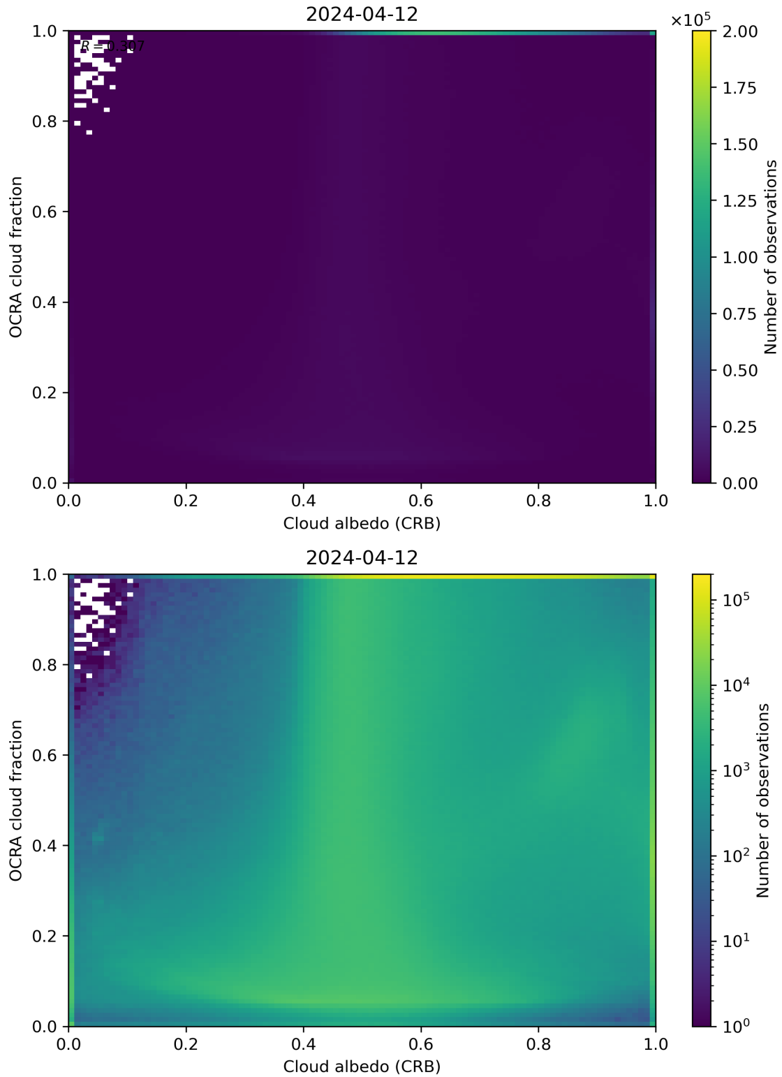
Figure 70: Scatter density plot of “Cloud albedo (CRB)” against “OCRA cloud fraction” for 2024-04-11 to 2024-04-13.
