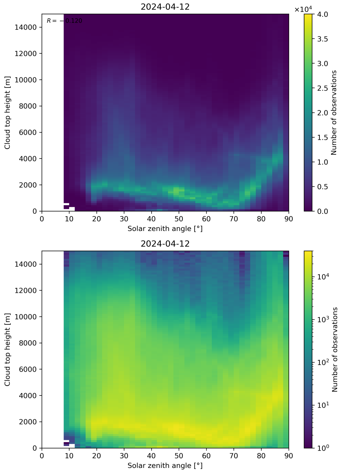
Figure 104: Scatter density plot of “Solar zenith angle” against “Cloud top height” for 2024-04-11 to 2024-04-13.
