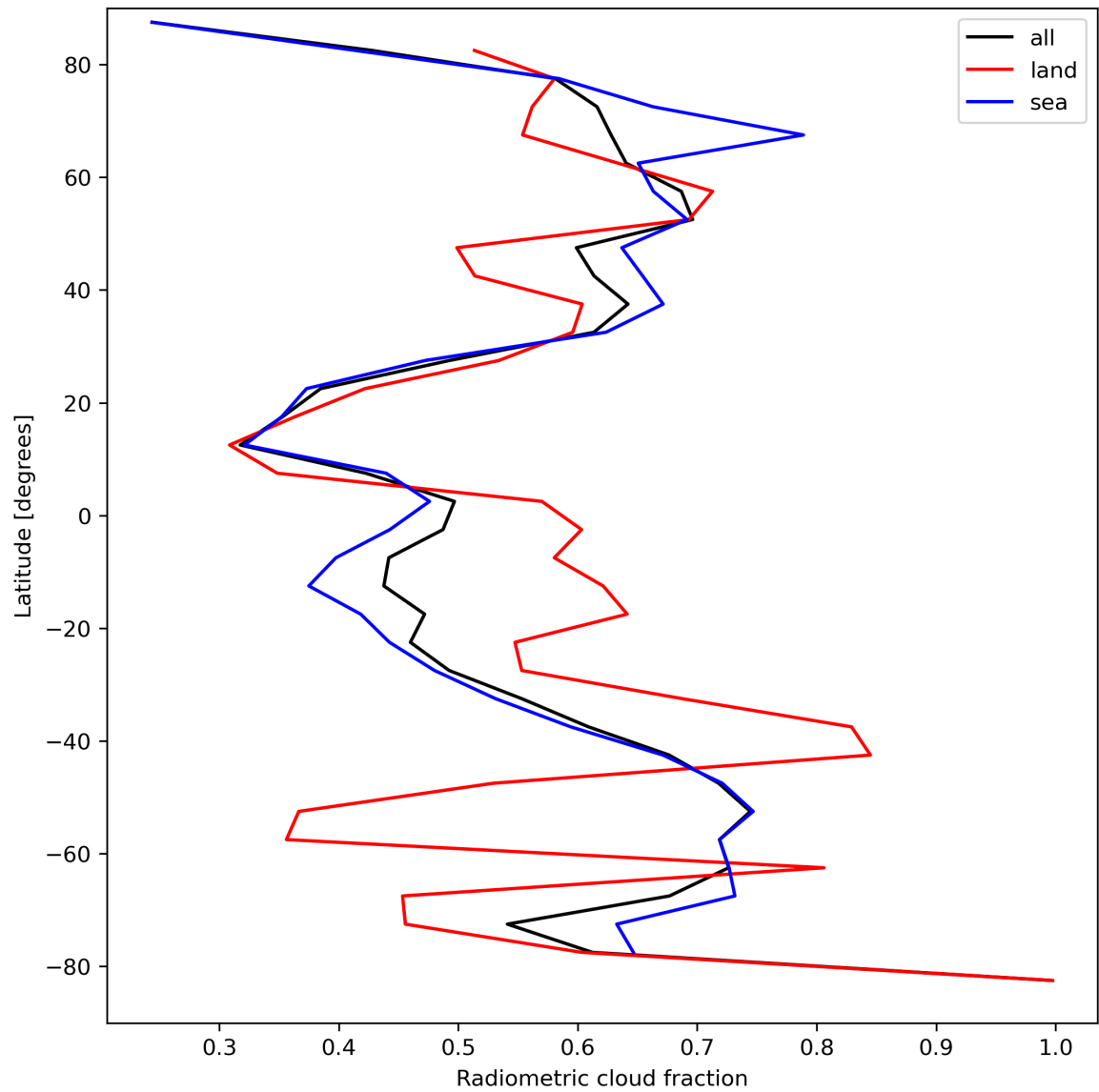
Figure 23: Zonal average of “Radiometric cloud fraction” for 2024-04-11 to 2024-04-13.
