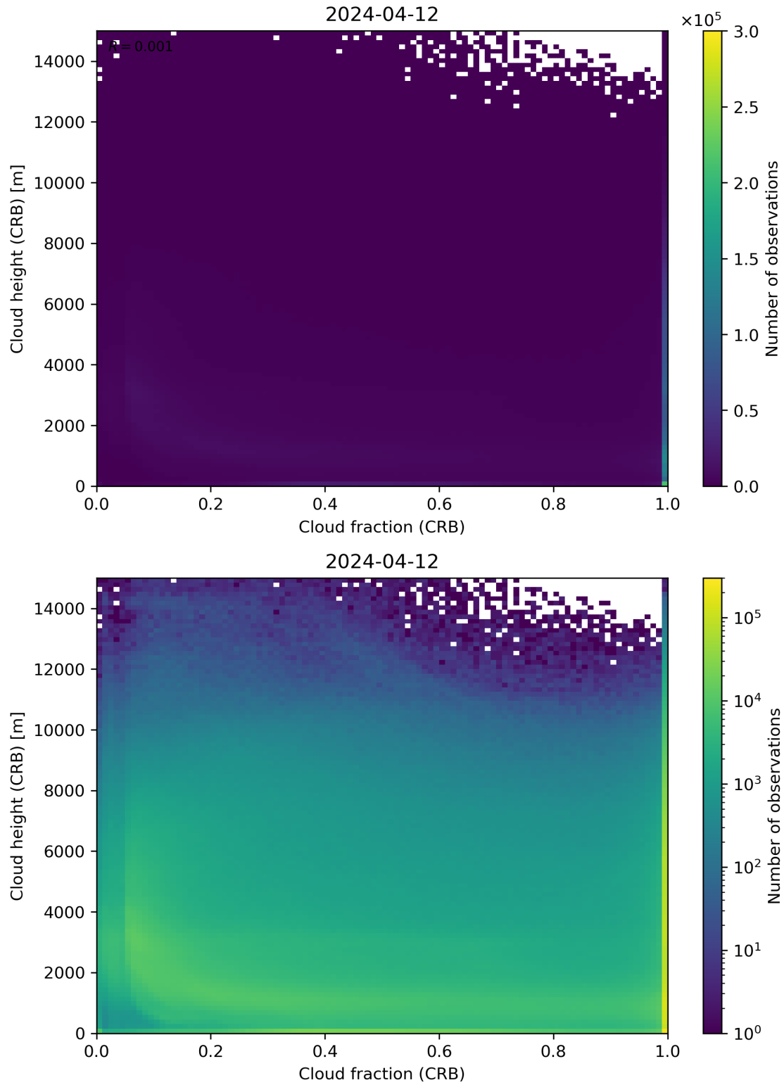
Figure 79: Scatter density plot of “Cloud fraction (CRB)” against “Cloud height (CRB)” for 2024-04-11 to 2024-04-13.
