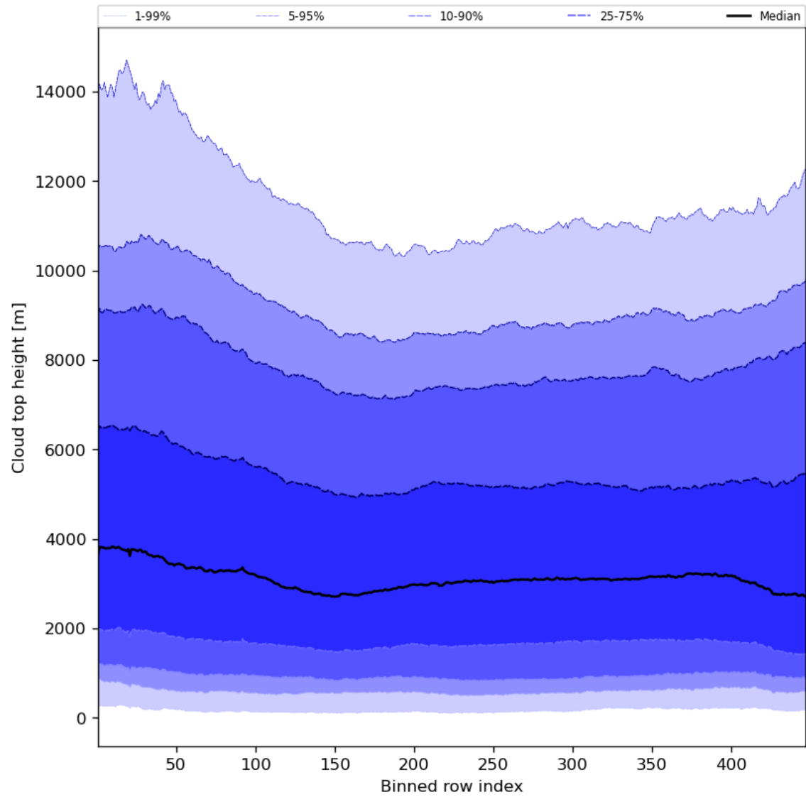
Figure 56: Along track statistics of “Cloud top height” for 2024-04-11 to 2024-04-13
