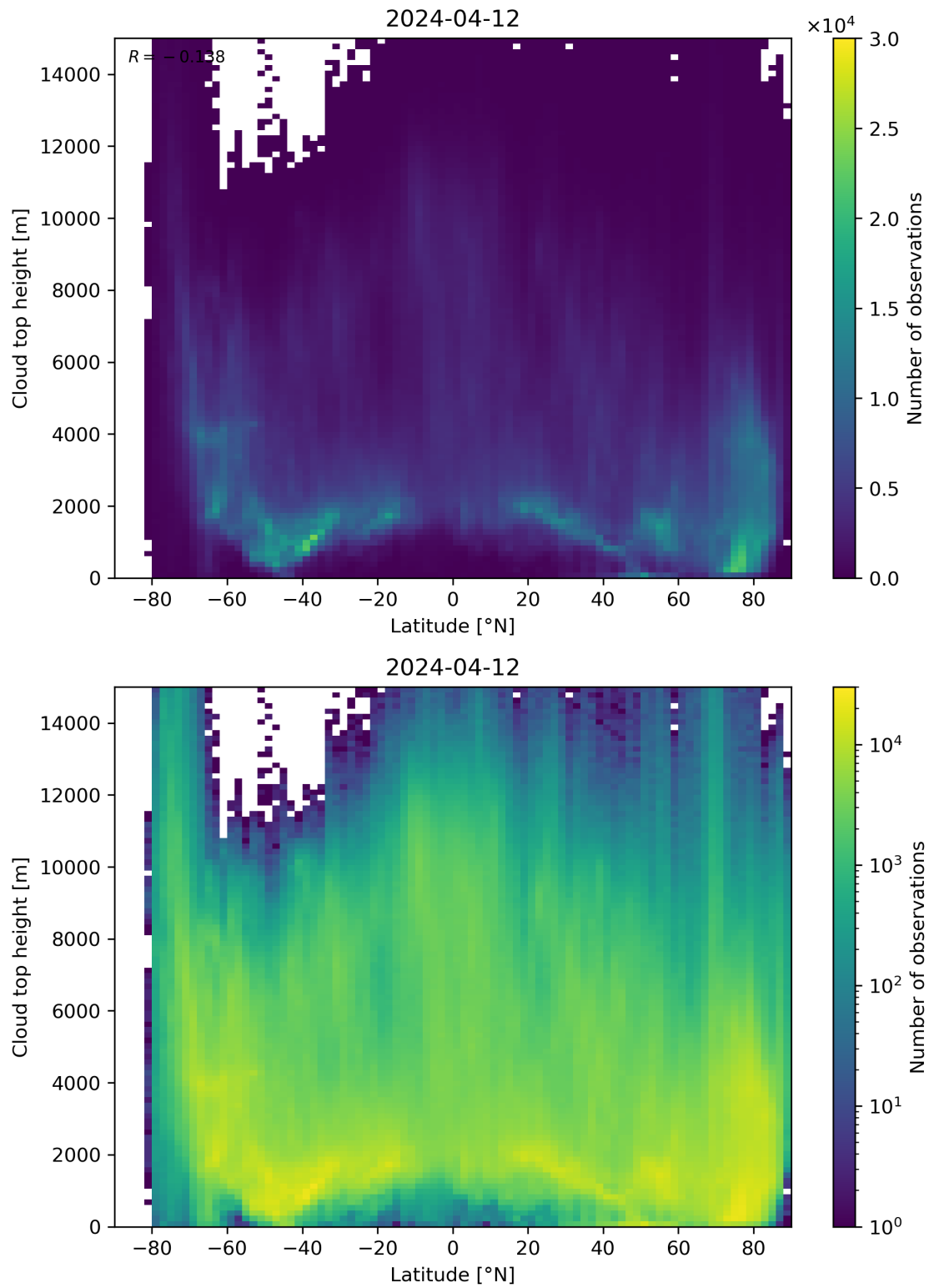
Figure 97: Scatter density plot of “Latitude” against “Cloud top height” for 2024-04-11 to 2024-04-13.
