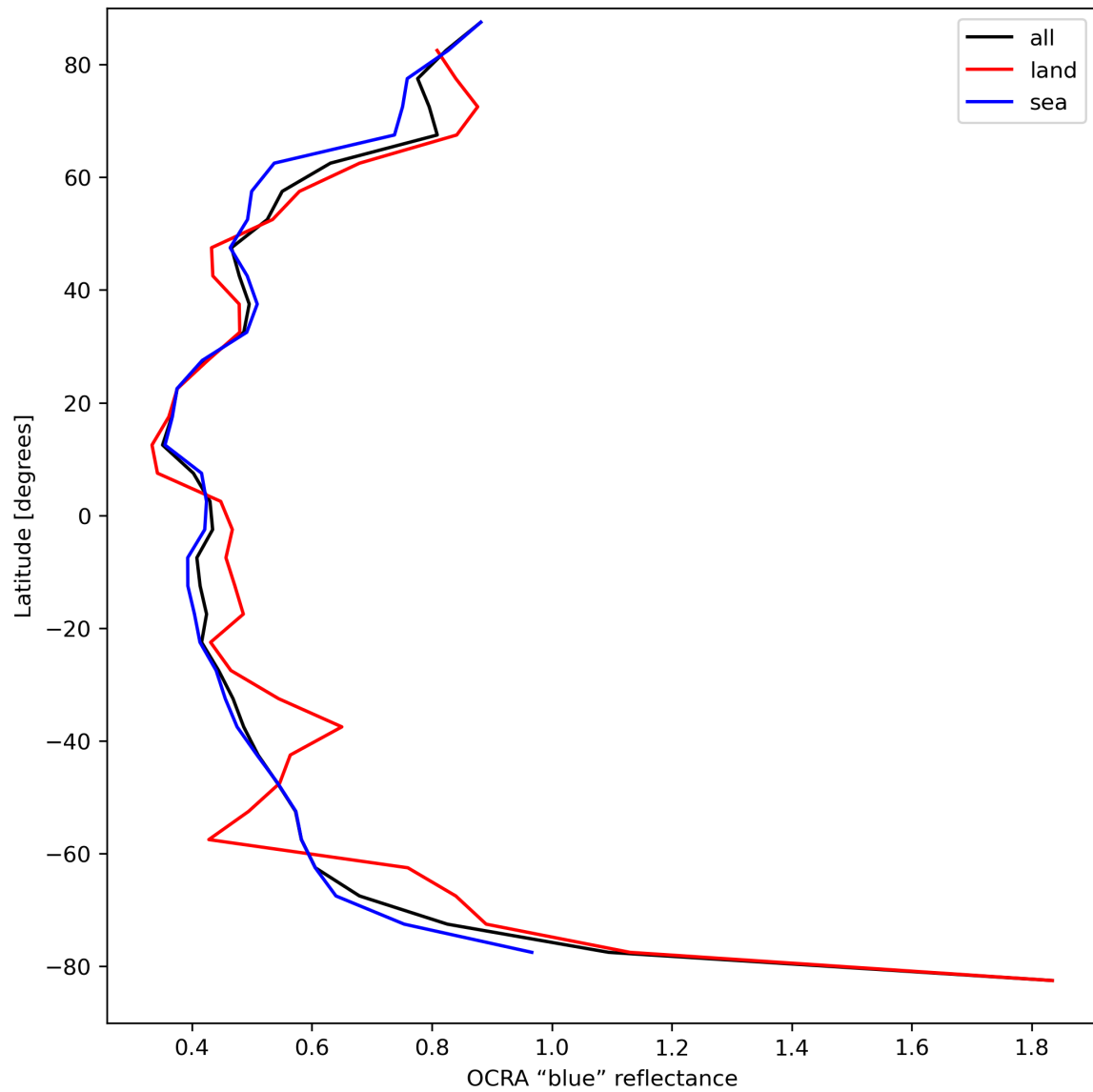
Figure 35: Zonal average of “OCRA “blue” reflectance” for 2024-04-11 to 2024-04-13.
