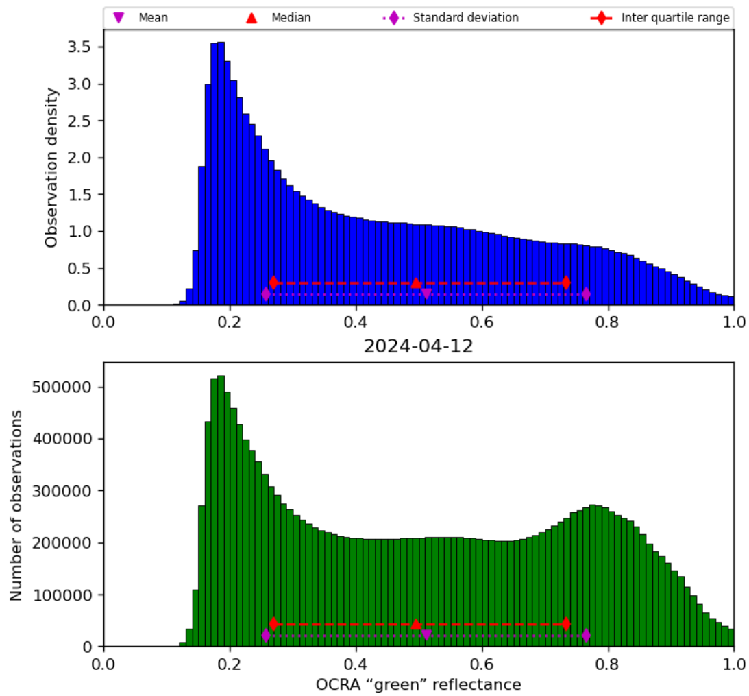
Figure 52: Histogram of “OCRA “green” reflectance” for 2024-04-11 to 2024-04-13
