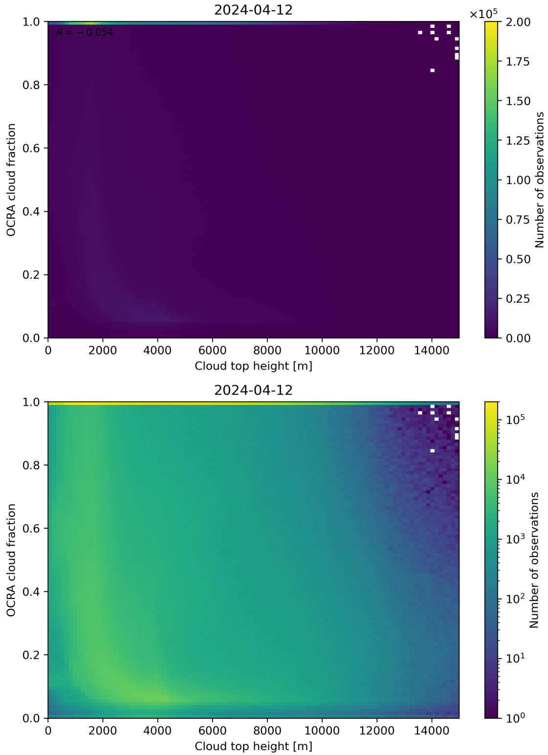
Figure 87: Scatter density plot of “Cloud top height” against “OCRA cloud fraction” for 2024-04-11 to 2024-04-13.
