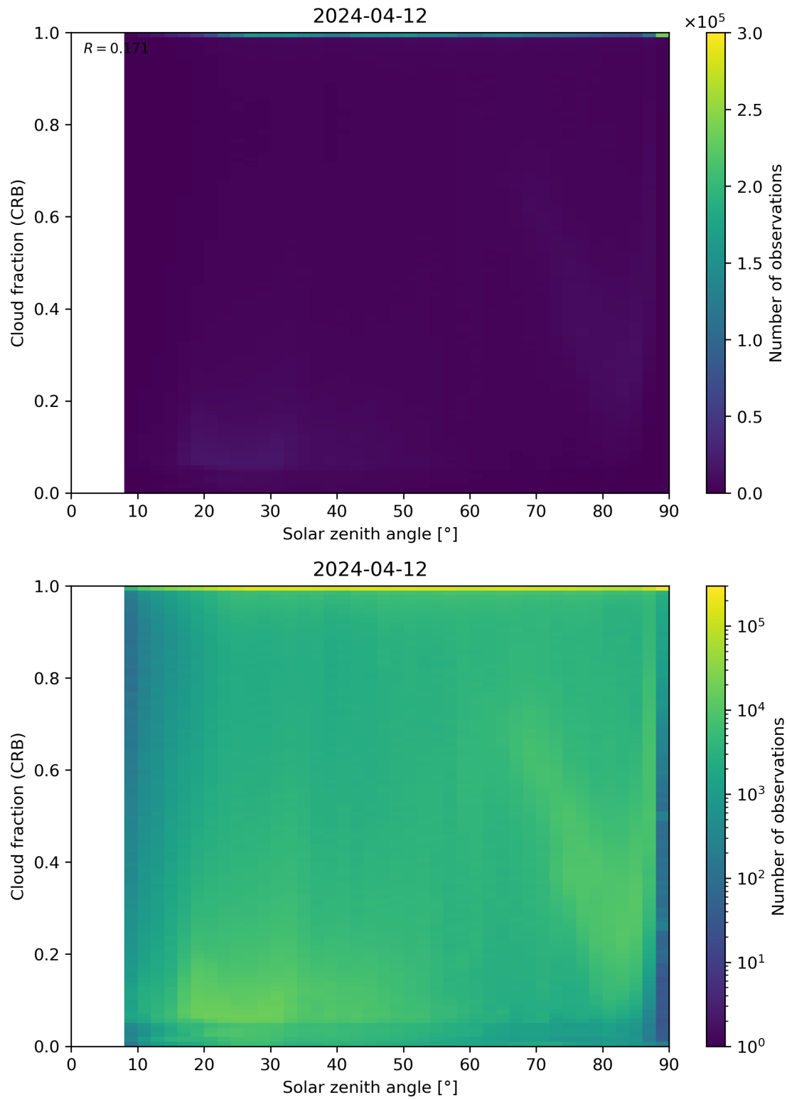
Figure 101: Scatter density plot of “Solar zenith angle” against “Cloud fraction (CRB)” for 2024-04-11 to 2024-04-13.
