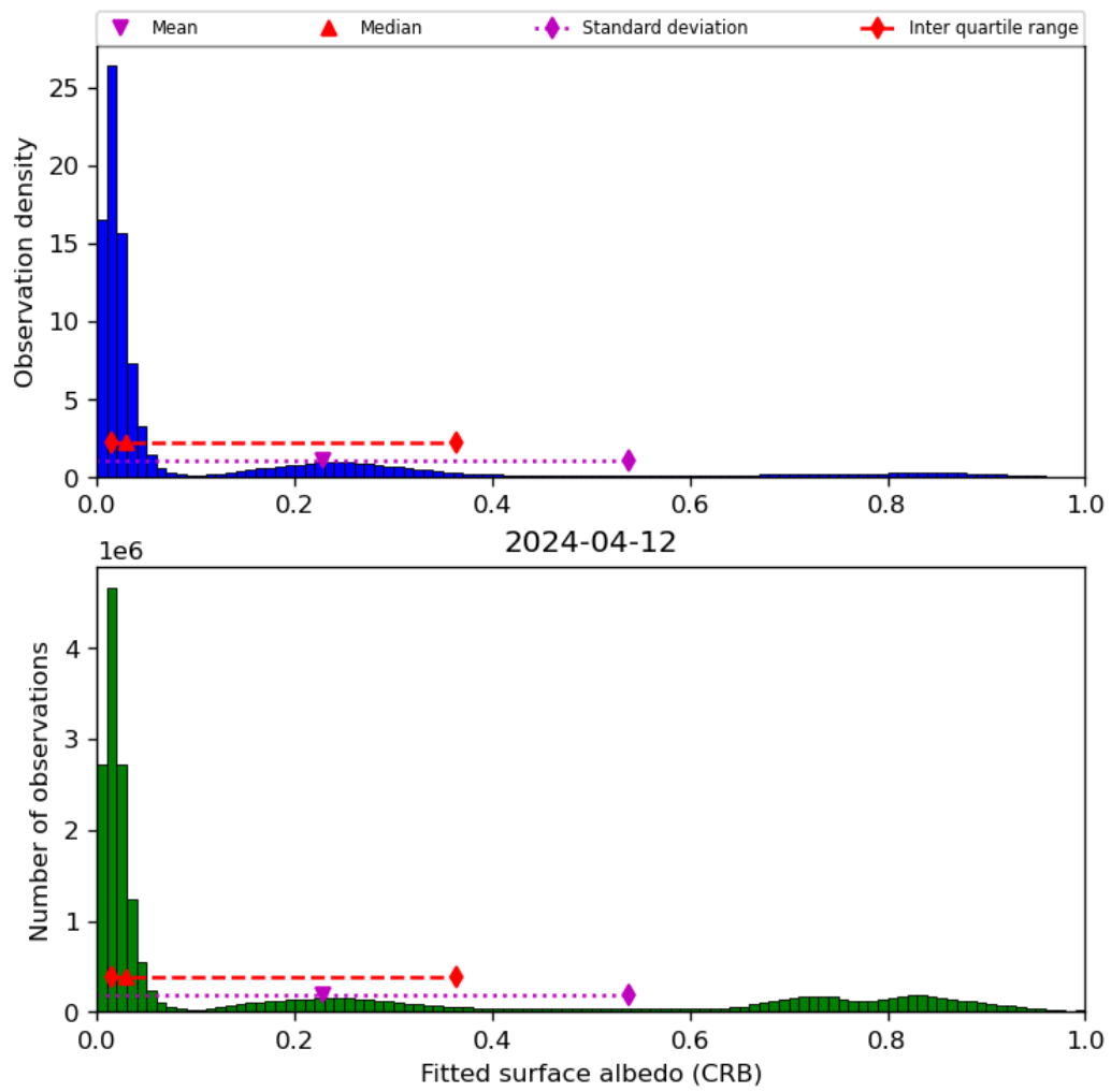
Figure 46: Histogram of “Fitted surface albedo (CRB)” for 2024-04-11 to 2024-04-13
