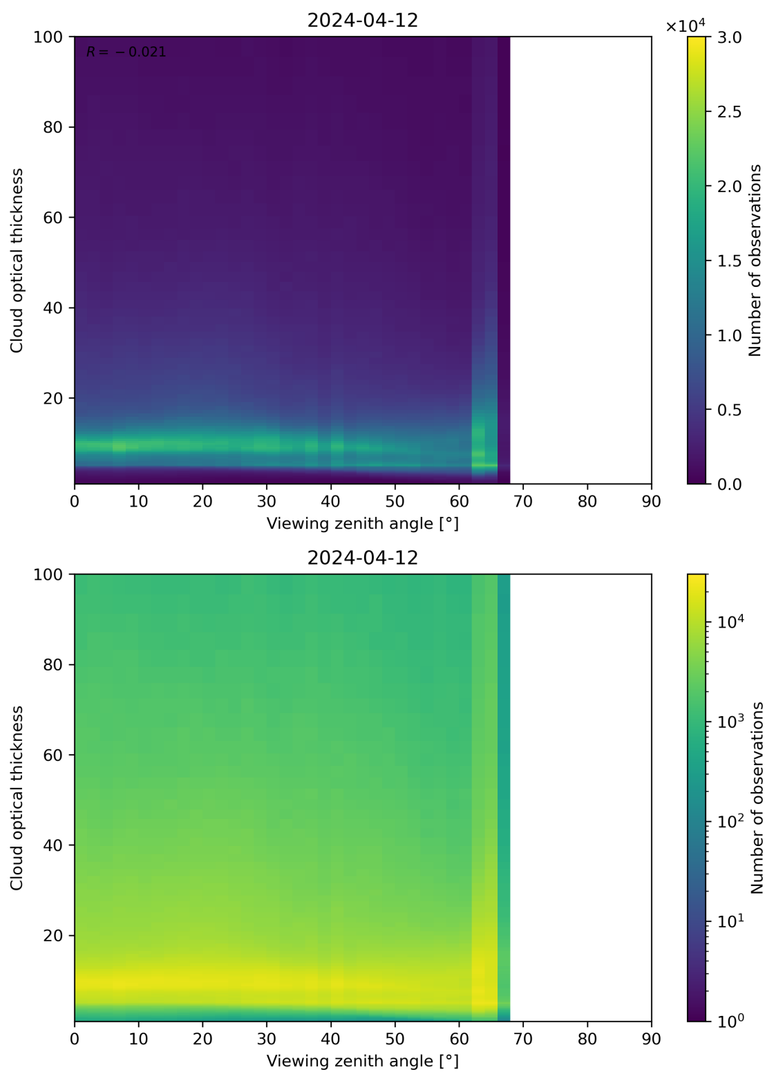
Figure 111: Scatter density plot of “Viewing zenith angle” against “Cloud optical thickness” for 2024-04-11 to 2024-04-13.
