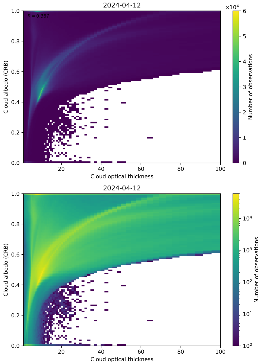
Figure 82: Scatter density plot of “Cloud optical thickness” against “Cloud albedo (CRB)” for 2024-04-11 to 2024-04-13.
