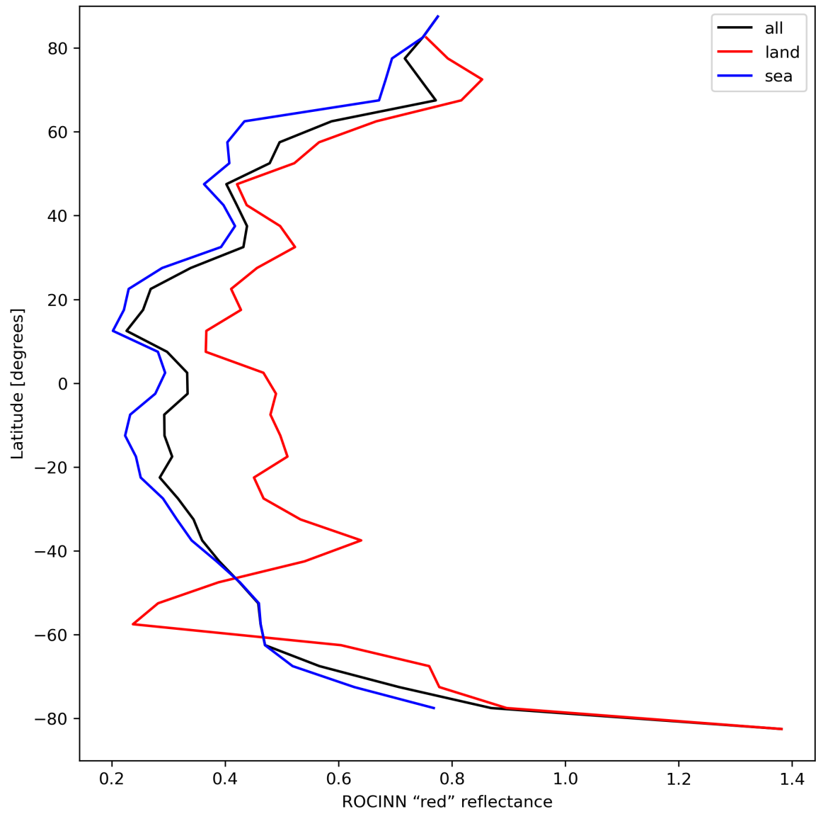
Figure 37: Zonal average of “ROCINN “red” reflectance” for 2024-04-11 to 2024-04-13.
