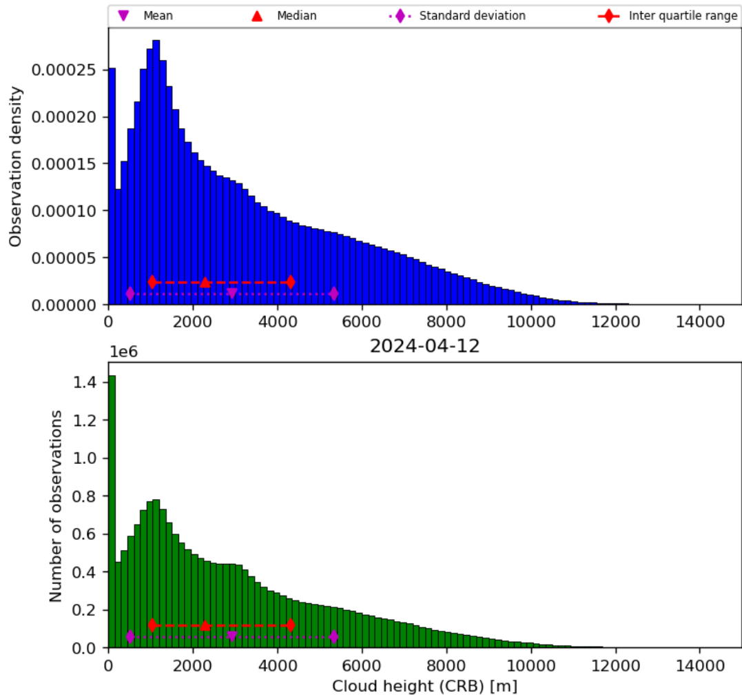
Figure 43: Histogram of “Cloud height (CRB)” for 2024-04-11 to 2024-04-13
