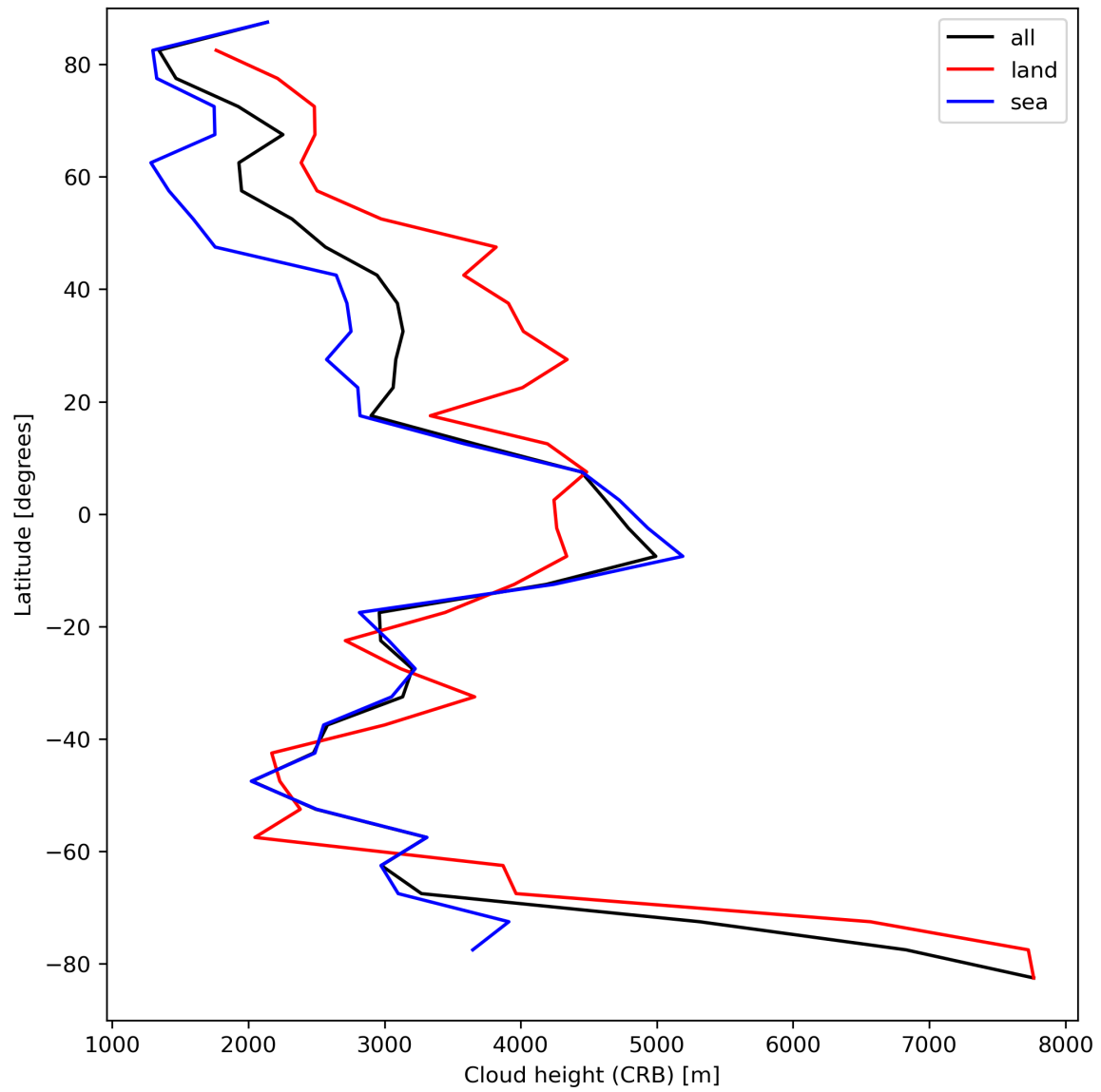
Figure 27: Zonal average of “Cloud height (CRB)” for 2024-04-11 to 2024-04-13.
