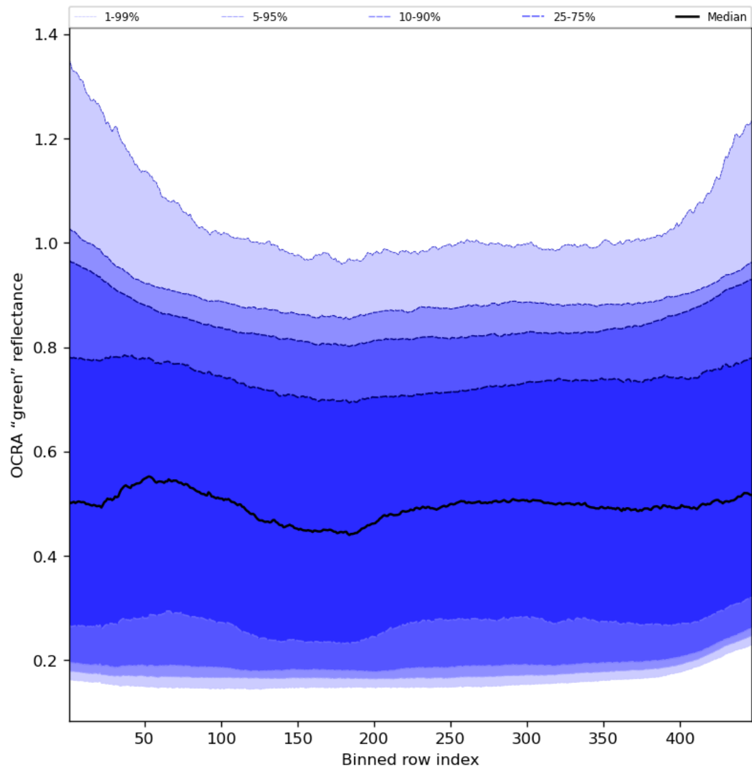
Figure 68: Along track statistics of "OCRA "green" reflectance" for 2024-04-11 to 2024-04-13
