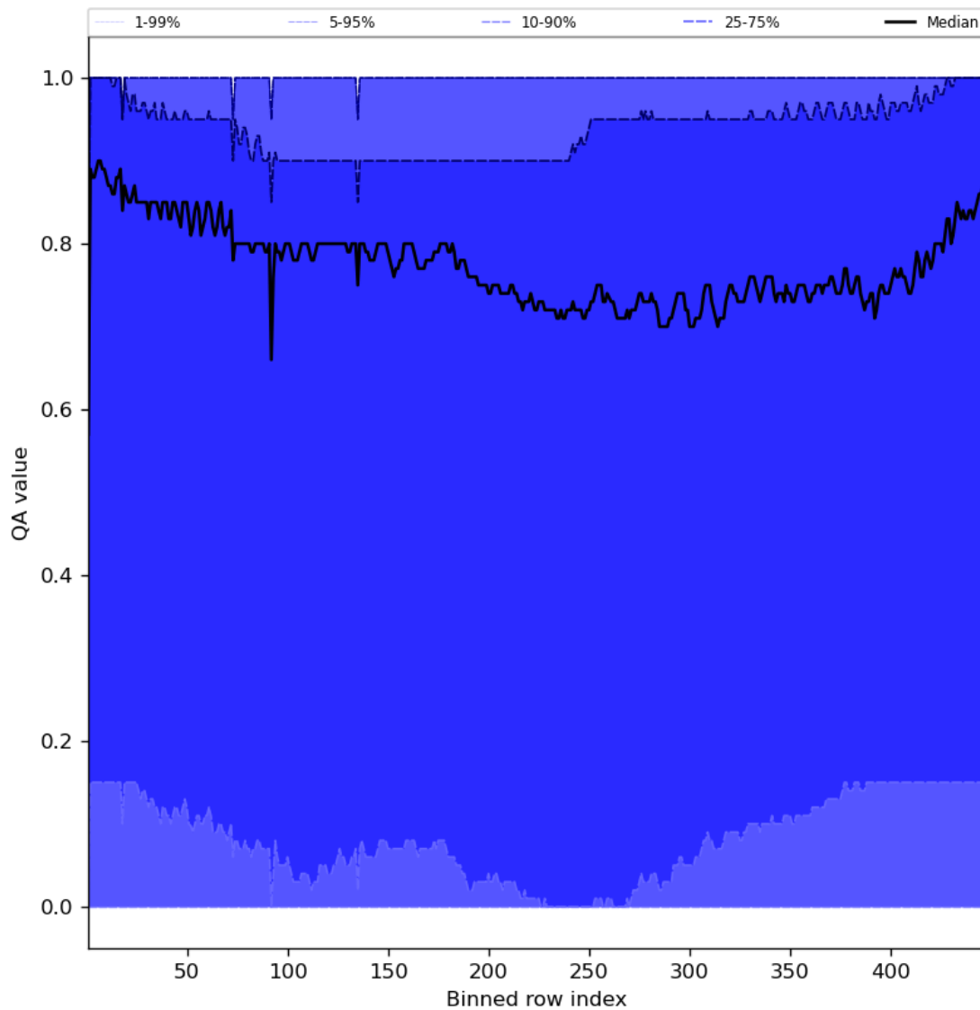
Figure 54: Along track statistics of “QA value” for 2024-04-11 to 2024-04-13
