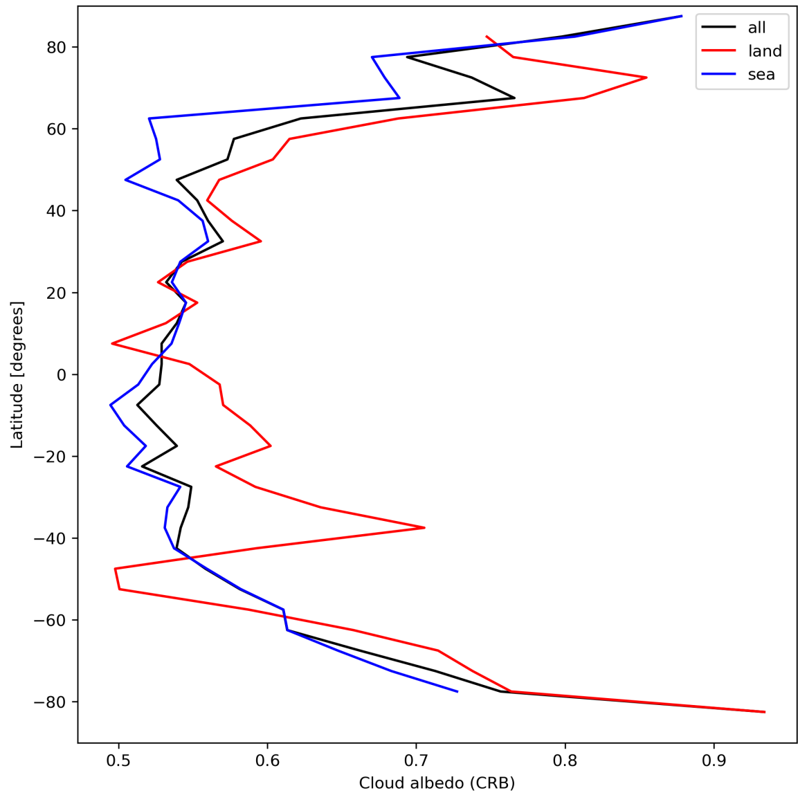
Figure 28: Zonal average of “Cloud albedo (CRB)” for 2024-04-11 to 2024-04-13.
