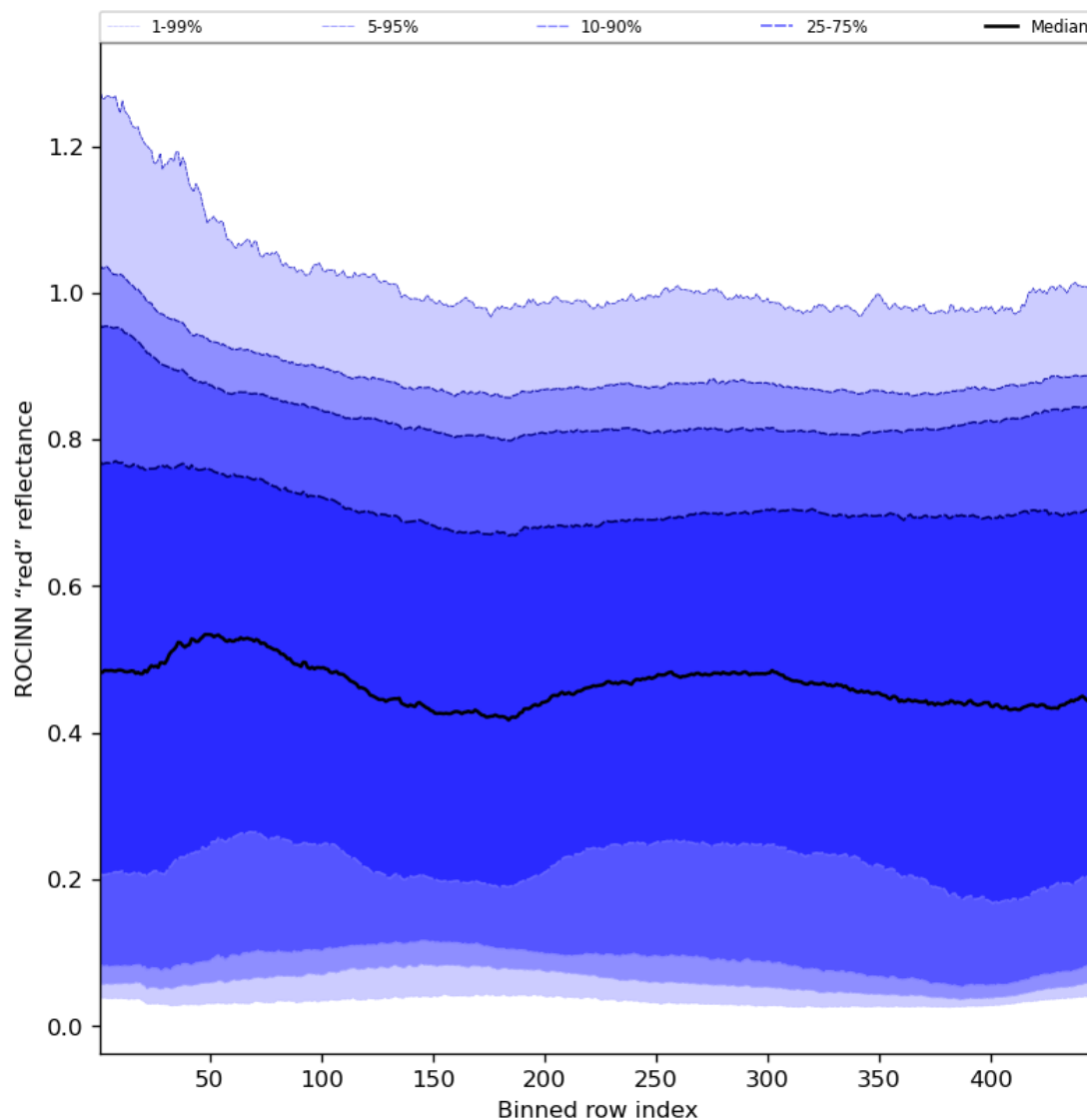
Figure 69: Along track statistics of “ROCINN “red” reflectance” for 2024-04-11 to 2024-04-13
