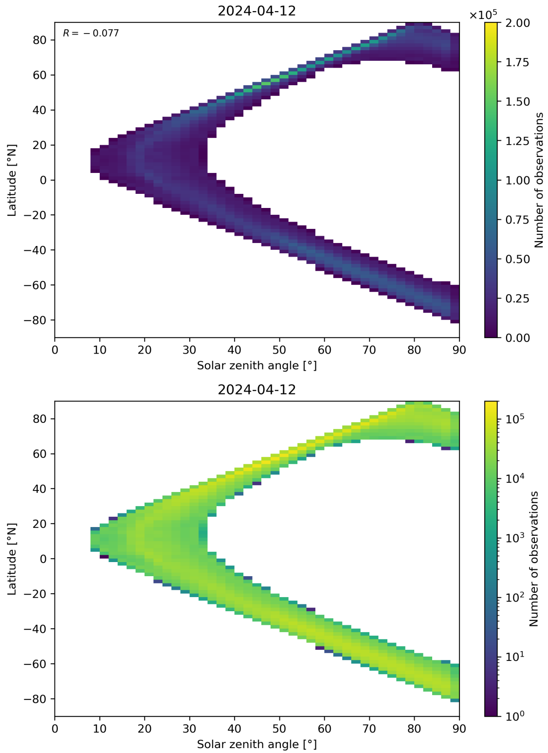
Figure 105: Scatter density plot of “Solar zenith angle” against “Latitude” for 2024-04-11 to 2024-04-13.
