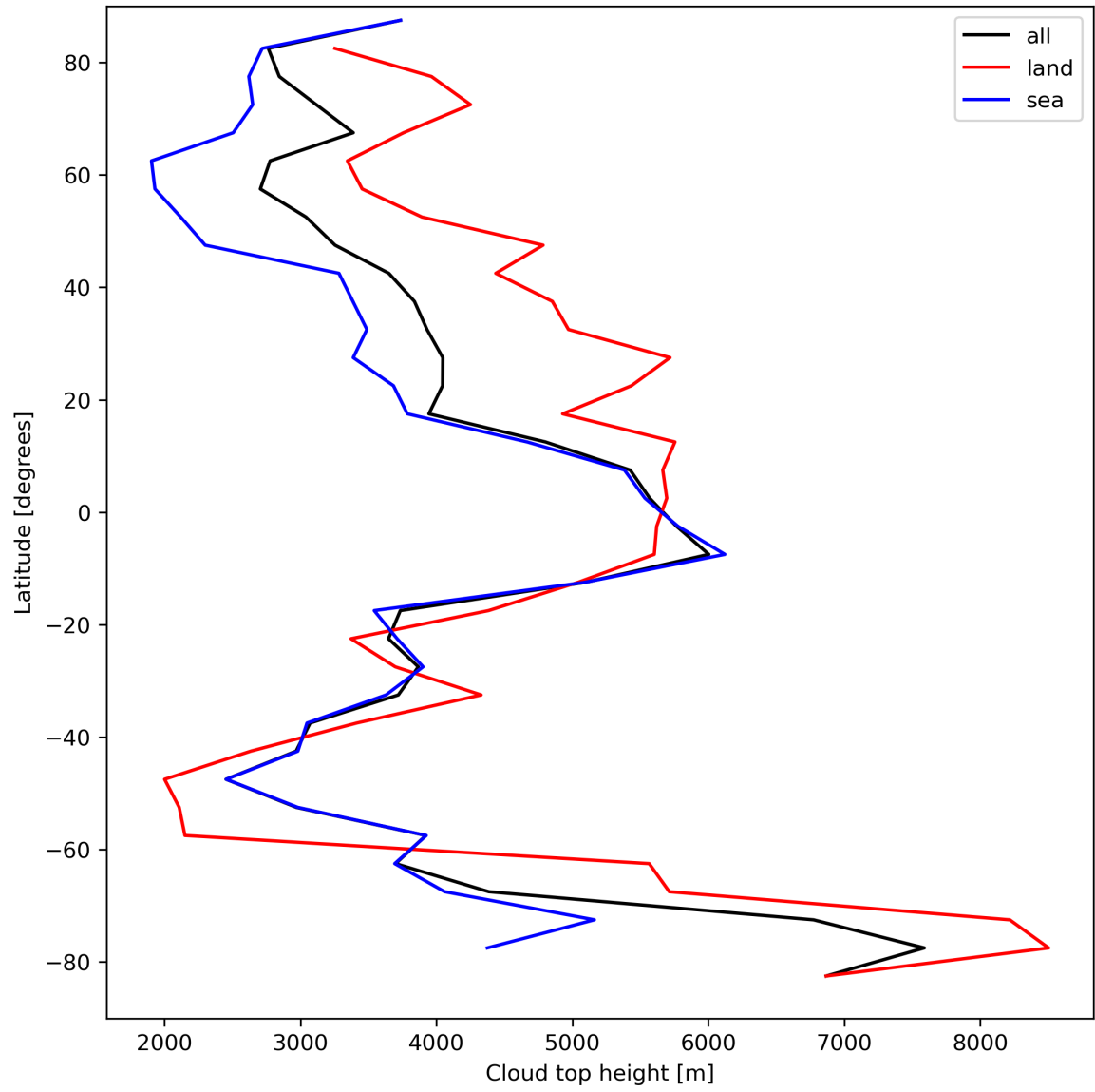
Figure 24: Zonal average of “Cloud top height” for 2024-04-11 to 2024-04-13.
