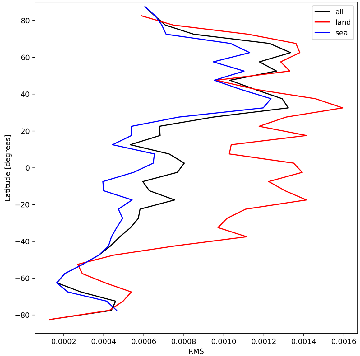
Figure 31: Zonal average of “RMS” for 2024-04-11 to 2024-04-13.
