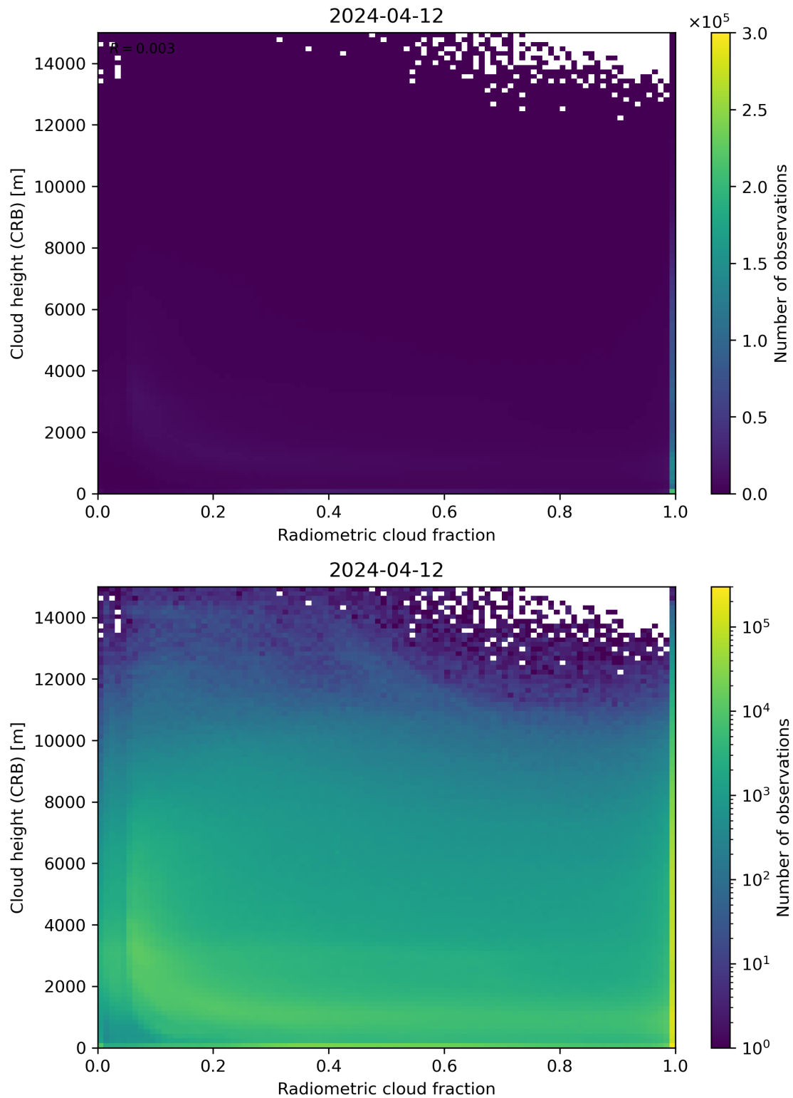
Figure 74: Scatter density plot of “Radiometric cloud fraction” against “Cloud height (CRB)” for 2024-04-11 to 2024-04-13.
