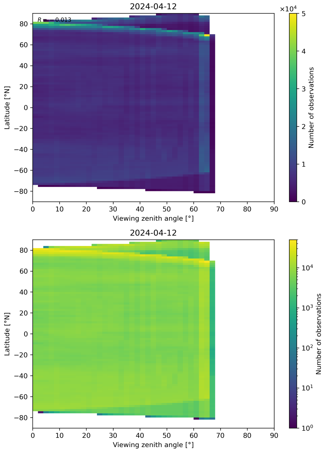
Figure 113: Scatter density plot of “Viewing zenith angle” against “Latitude” for 2024-04-11 to 2024-04-13.
