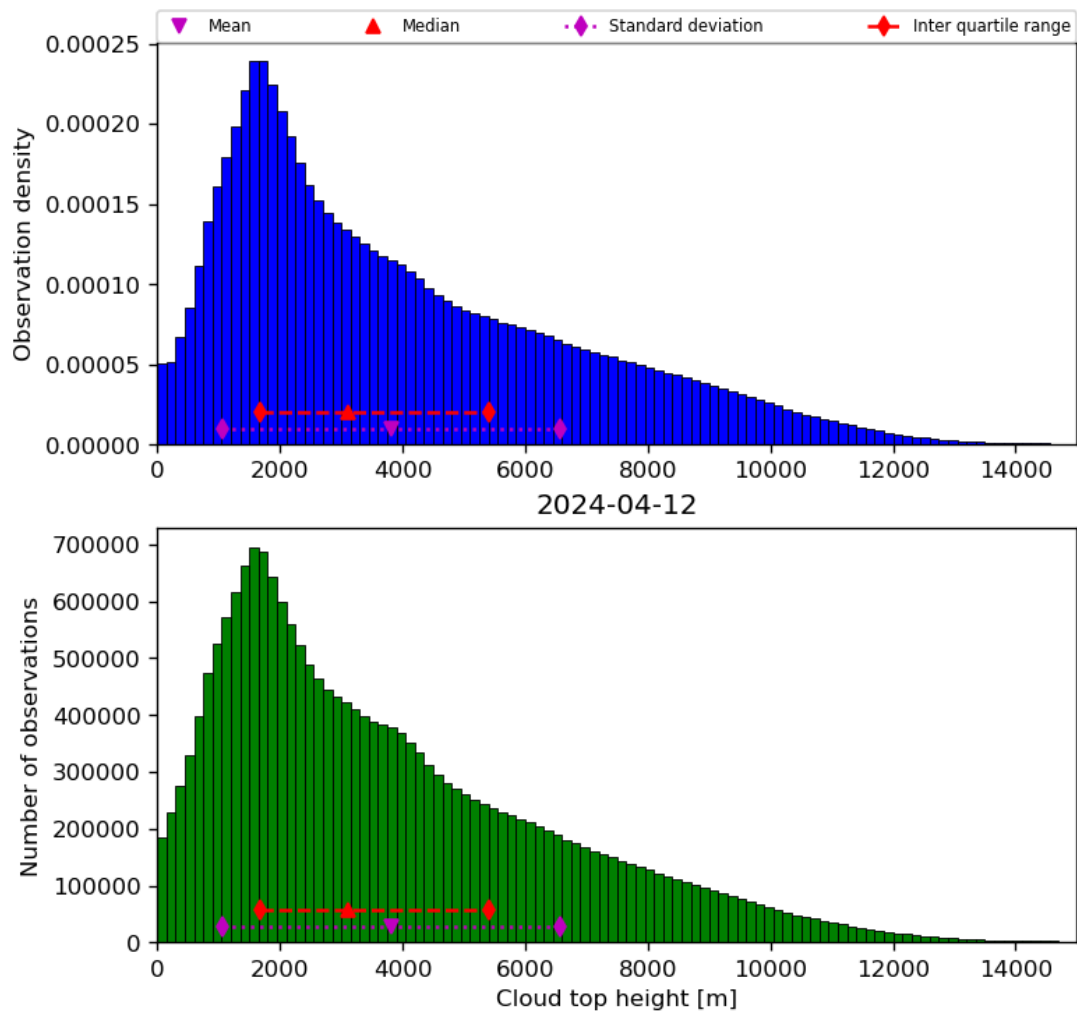
Figure 40: Histogram of “Cloud top height” for 2024-04-11 to 2024-04-13
