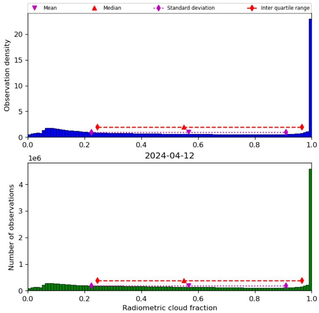
Figure 39: Histogram of “Radiometric cloud fraction” for 2024-04-11 to 2024-04-13
