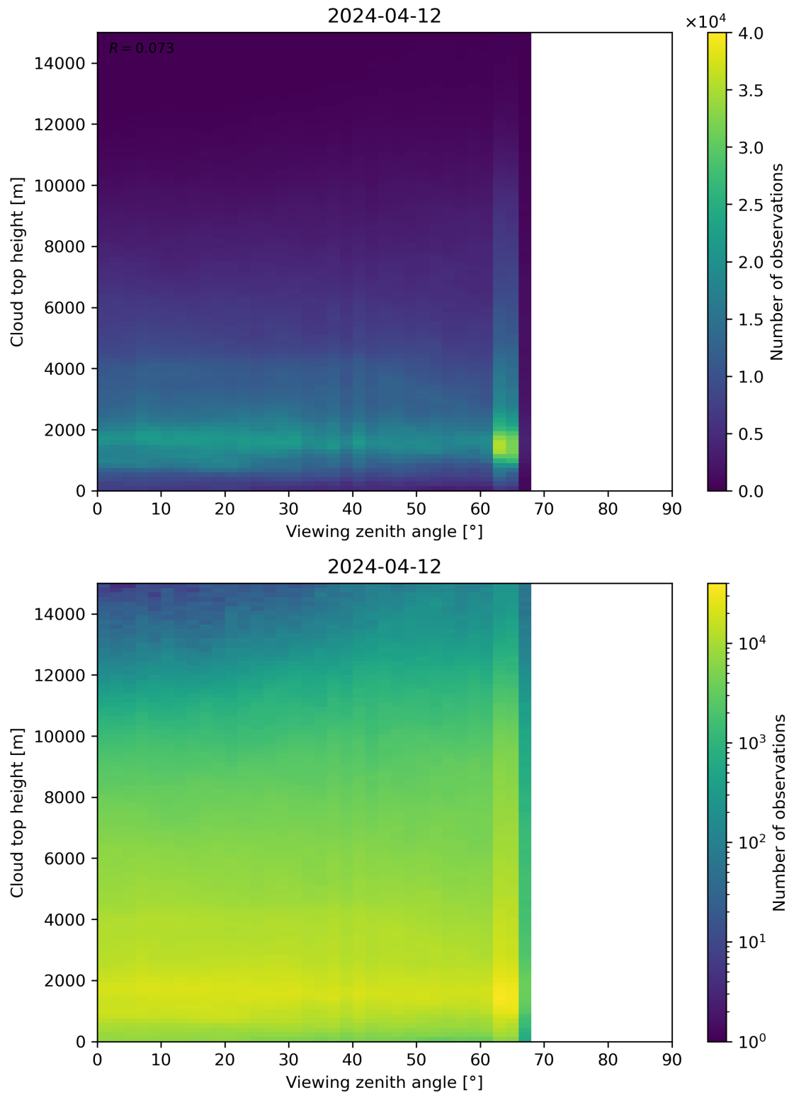
Figure 112: Scatter density plot of “Viewing zenith angle” against “Cloud top height” for 2024-04-11 to 2024-04-13.
