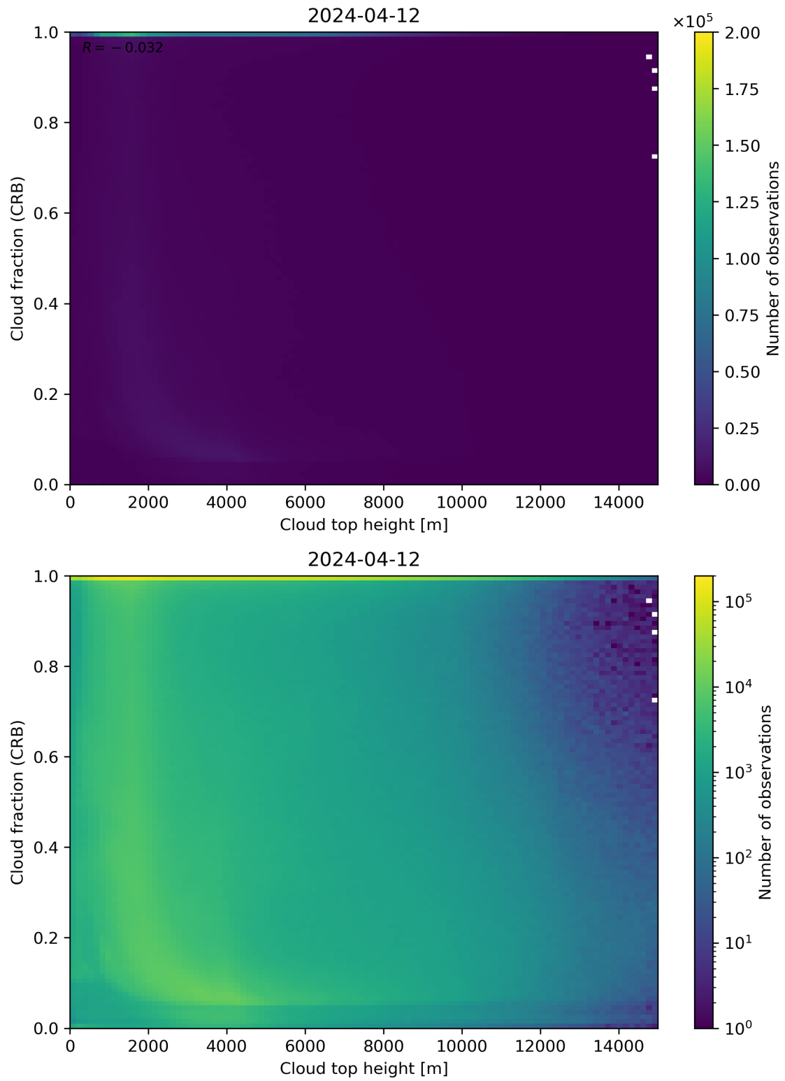
Figure 88: Scatter density plot of “Cloud top height” against “Cloud fraction (CRB)” for 2024-04-11 to 2024-04-13.
