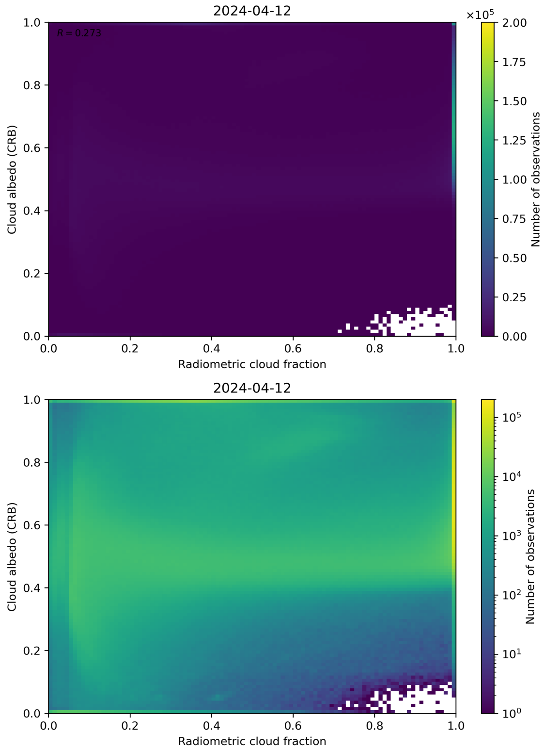
Figure 71: Scatter density plot of “Radiometric cloud fraction” against “Cloud albedo (CRB)” for 2024-04-11 to 2024-04-13.
