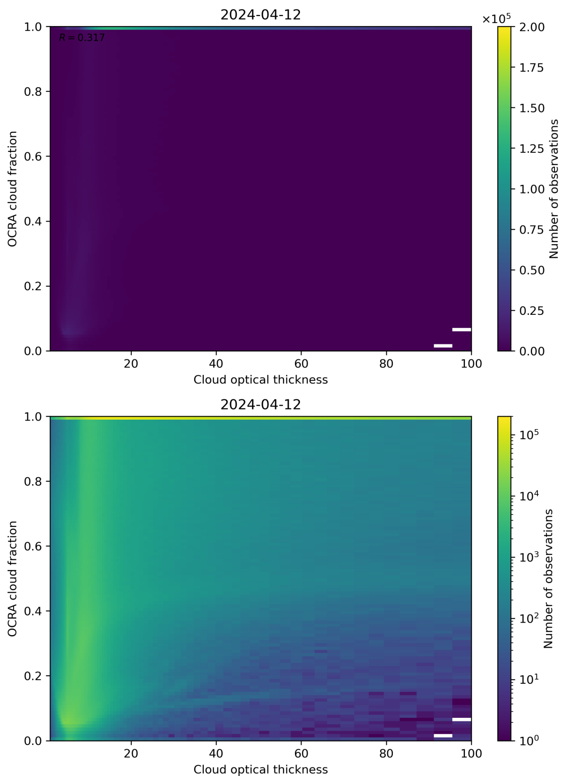
Figure 83: Scatter density plot of “Cloud optical thickness” against “OCRA cloud fraction” for 2024-04-11 to 2024-04-13.
