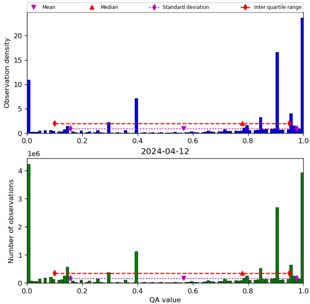
Figure 38: Histogram of “QA value” for 2024-04-11 to 2024-04-13
