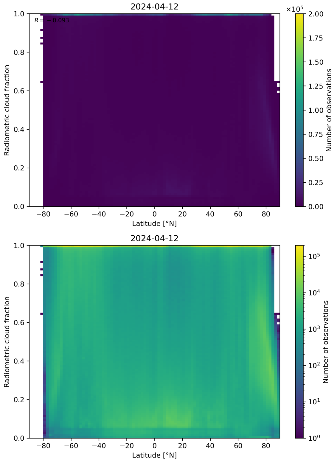
Figure 92: Scatter density plot of “Latitude” against “Radiometric cloud fraction” for 2024-04-11 to 2024-04-13.
