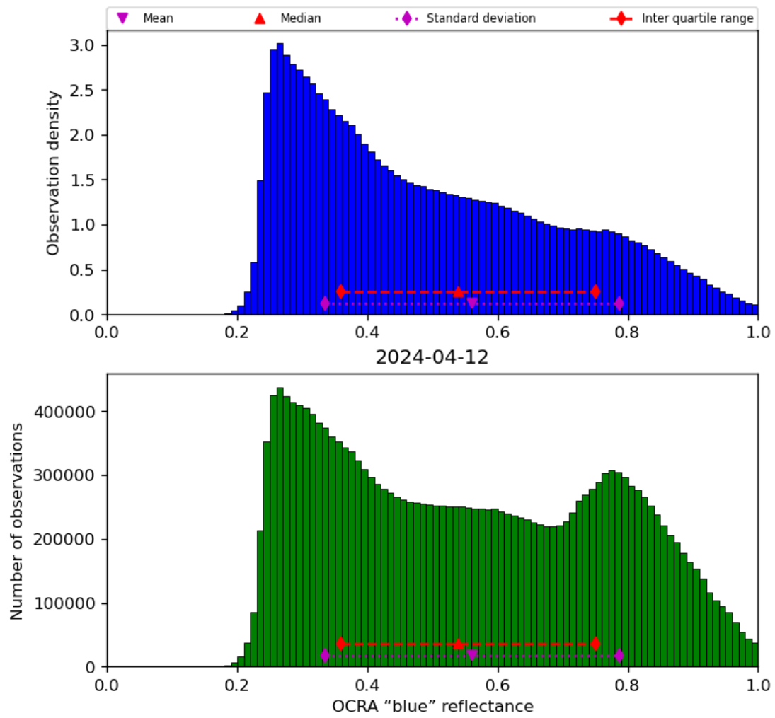
Figure 51: Histogram of “OCRA “blue” reflectance” for 2024-04-11 to 2024-04-13
