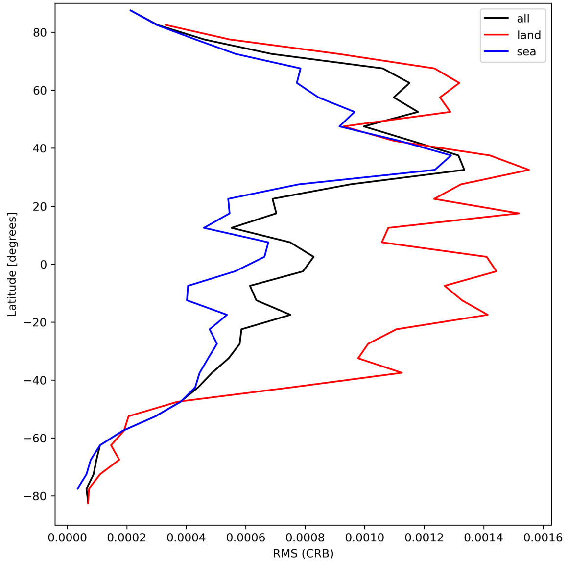
Figure 32: Zonal average of “RMS (CRB)” for 2024-04-11 to 2024-04-13.
