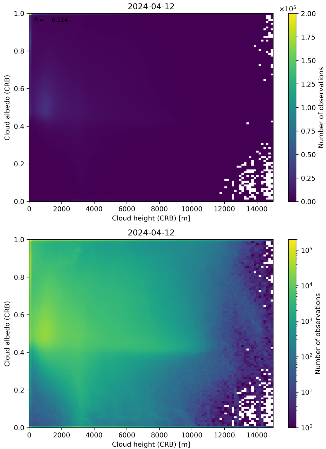
Figure 80: Scatter density plot of “Cloud height (CRB)” against “Cloud albedo (CRB)” for 2024-04-11 to 2024-04-13.
