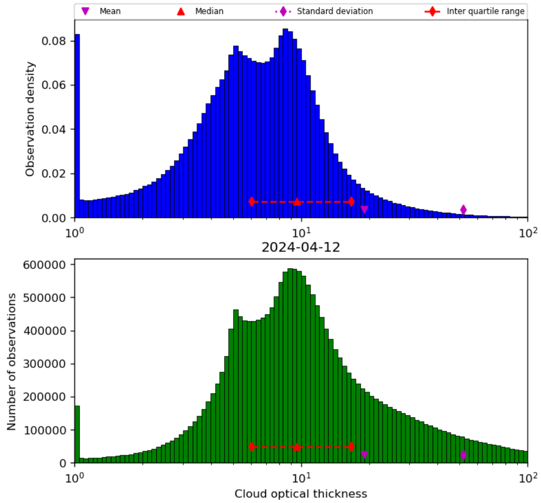
Figure 41: Histogram of “Cloud optical thickness” for 2024-04-11 to 2024-04-13
