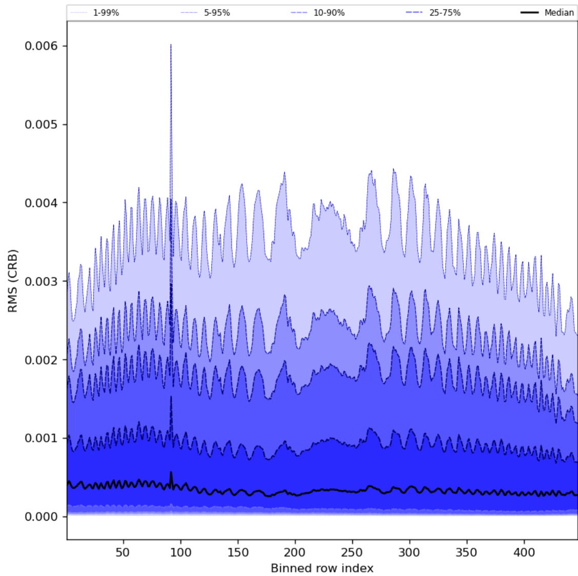
Figure 64: Along track statistics of “RMS (CRB)” for 2024-04-11 to 2024-04-13
