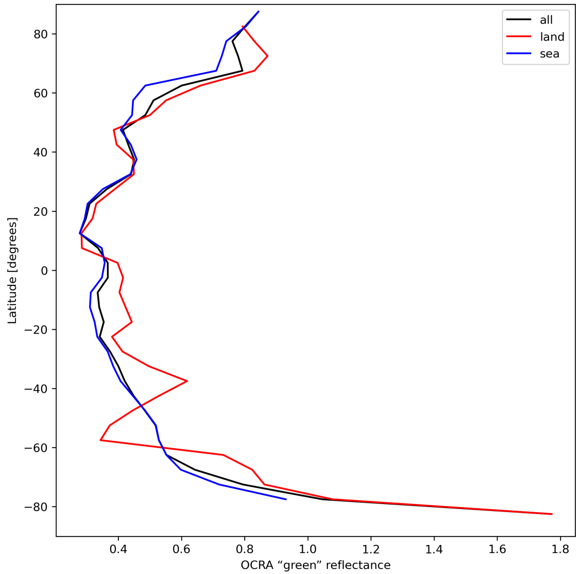
Figure 36: Zonal average of “OCRA “green” reflectance” for 2024-04-11 to 2024-04-13.
