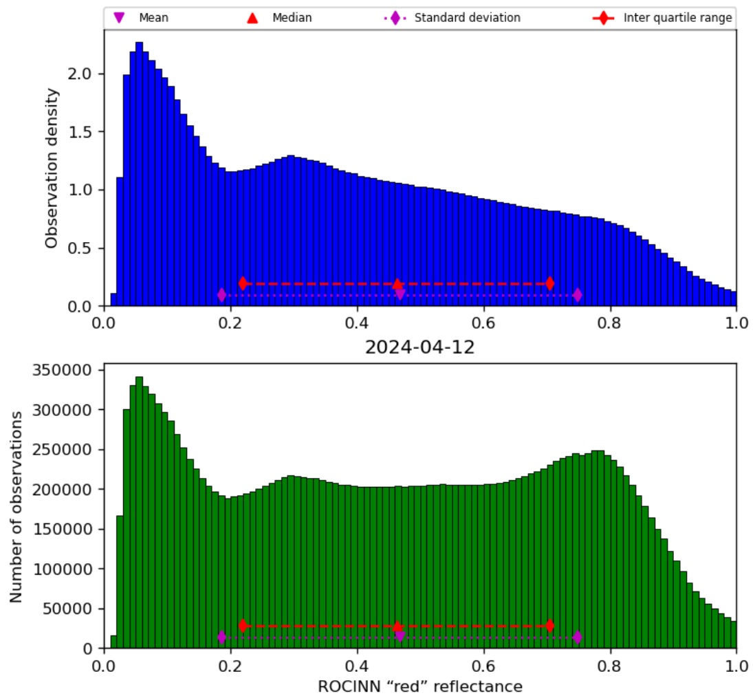
Figure 53: Histogram of “ROCINN “red” reflectance” for 2024-04-11 to 2024-04-13
