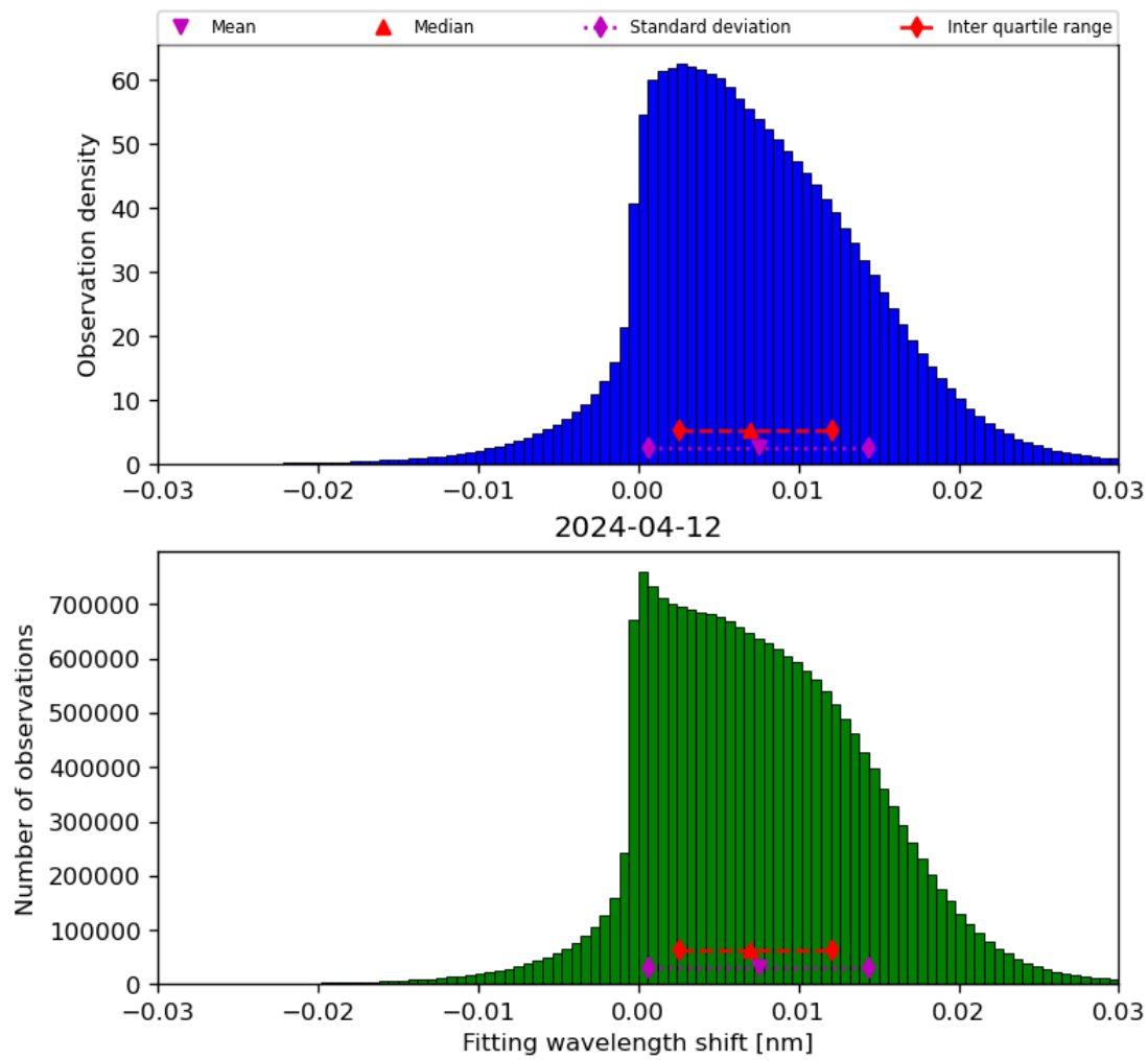
Figure 49: Histogram of “Fitting wavelength shift” for 2024-04-11 to 2024-04-13
