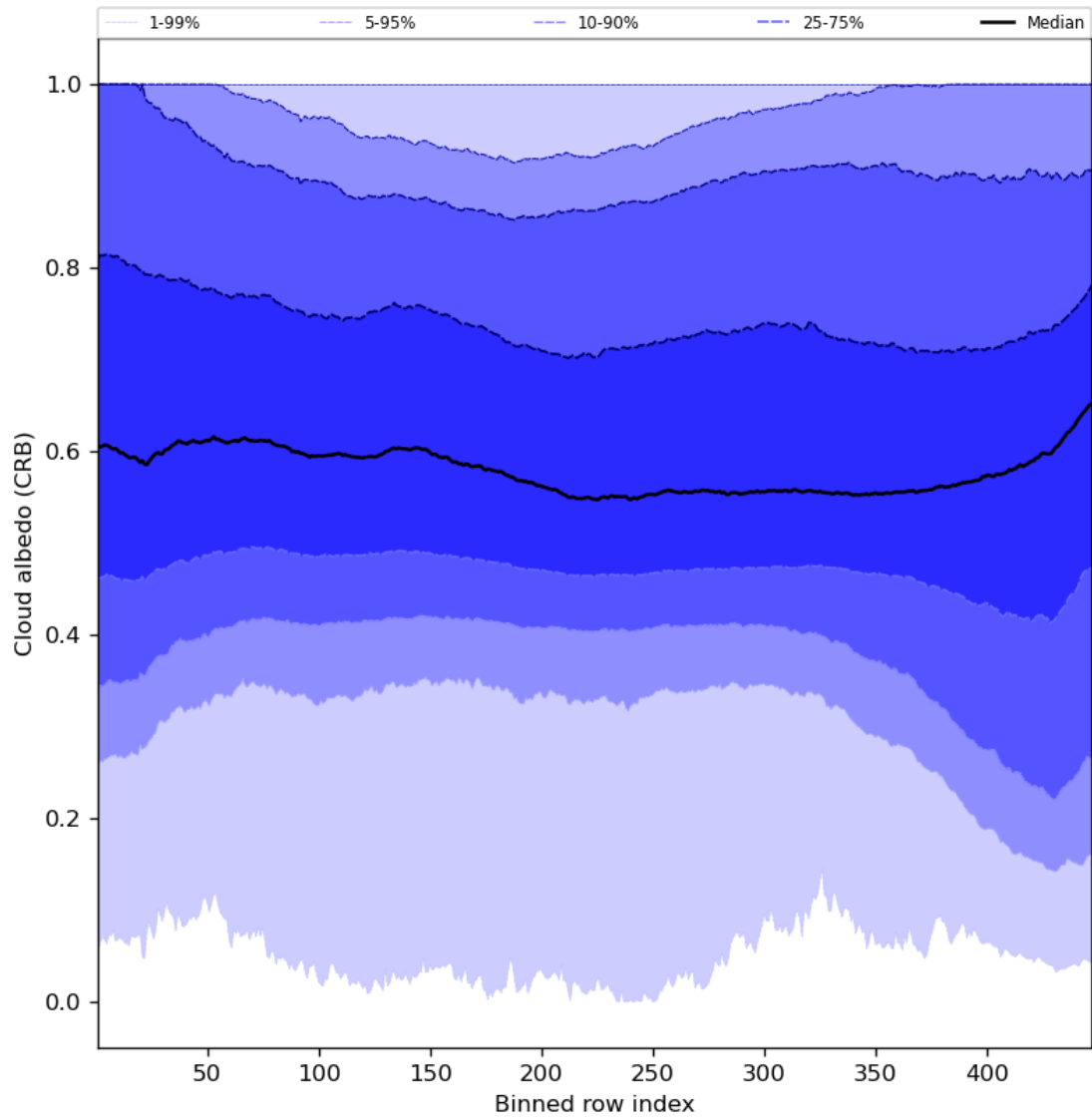
Figure 60: Along track statistics of “Cloud albedo (CRB)” for 2024-04-11 to 2024-04-13
