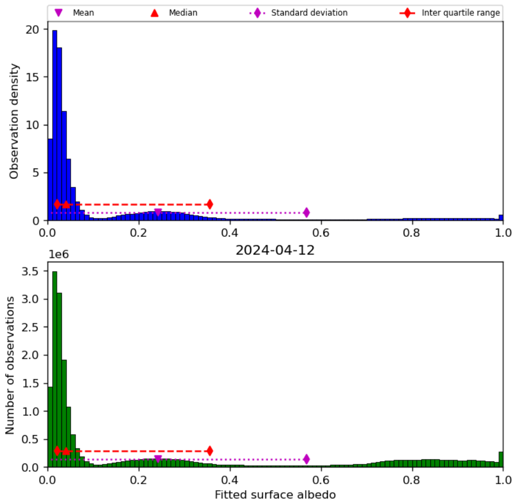
Figure 45: Histogram of “Fitted surface albedo” for 2024-04-11 to 2024-04-13
