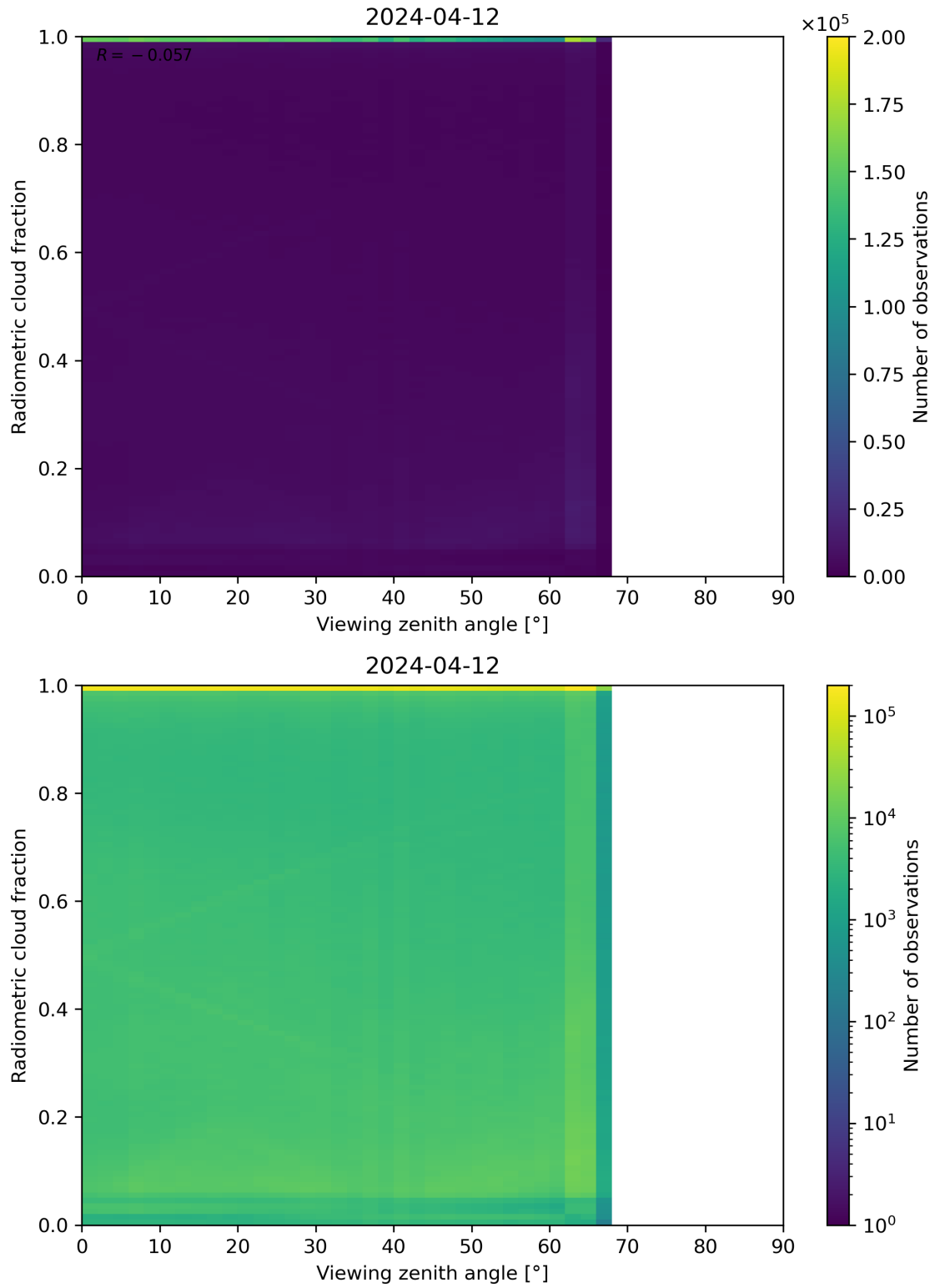
Figure 107: Scatter density plot of “Viewing zenith angle” against “Radiometric cloud fraction” for 2024-04-11 to 2024-04-13.
