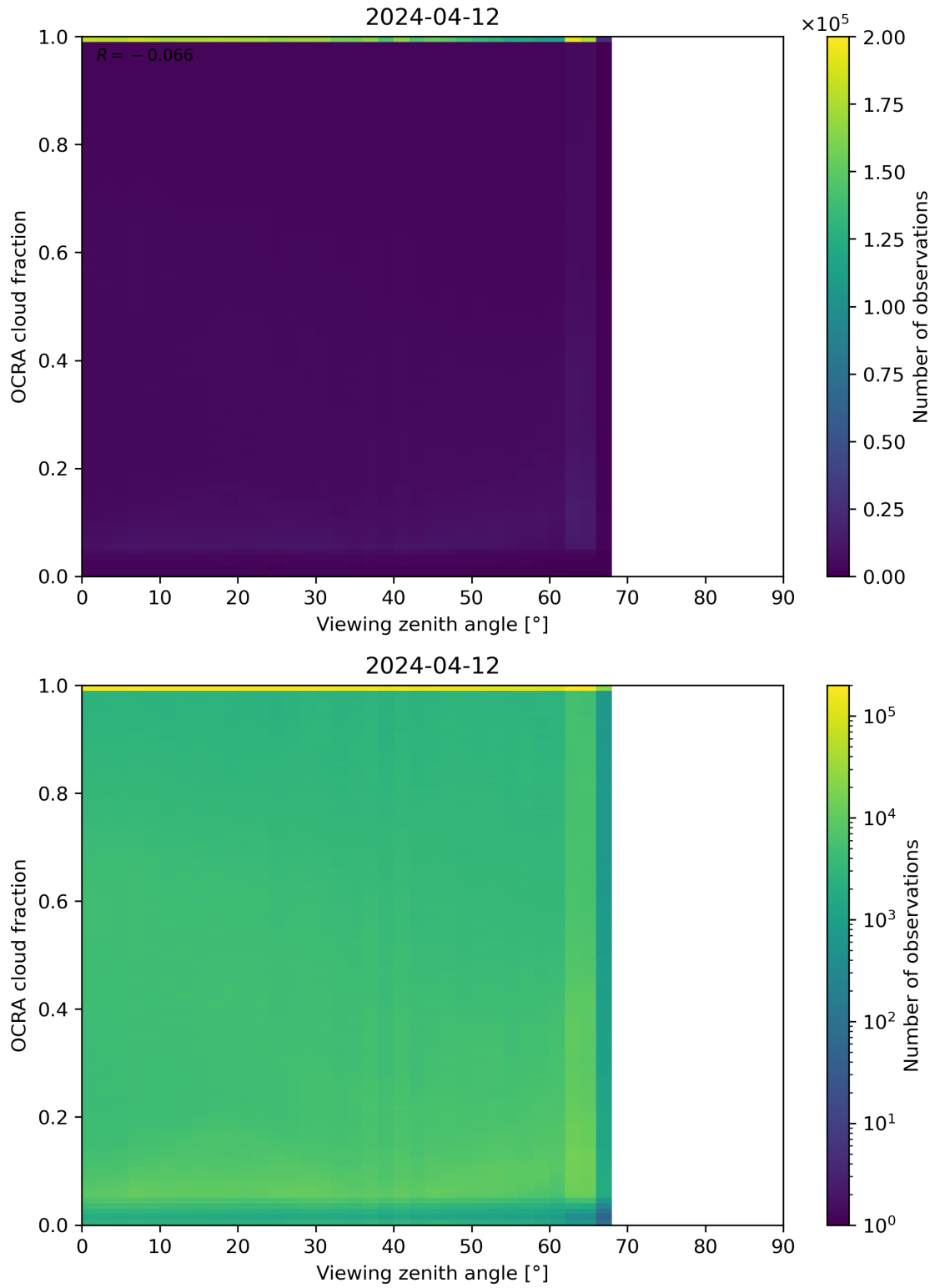
Figure 108: Scatter density plot of “Viewing zenith angle” against “OCRA cloud fraction” for 2024-04-11 to 2024-04-13.
