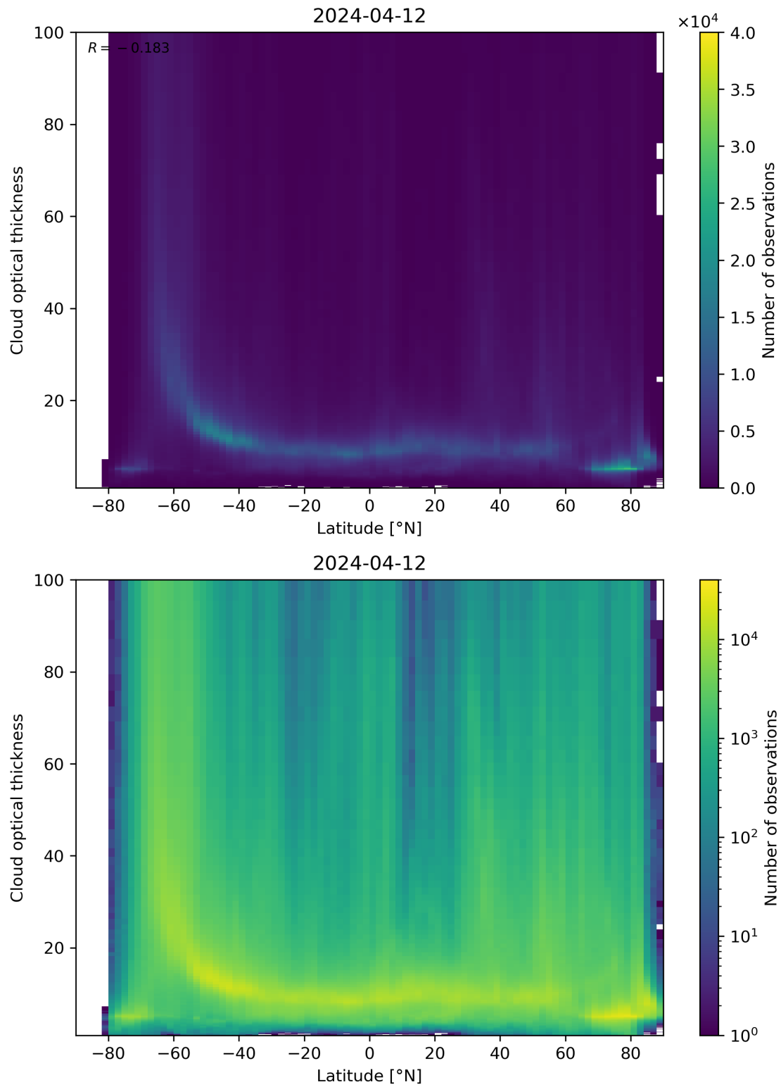
Figure 96: Scatter density plot of “Latitude” against “Cloud optical thickness” for 2024-04-11 to 2024-04-13.
