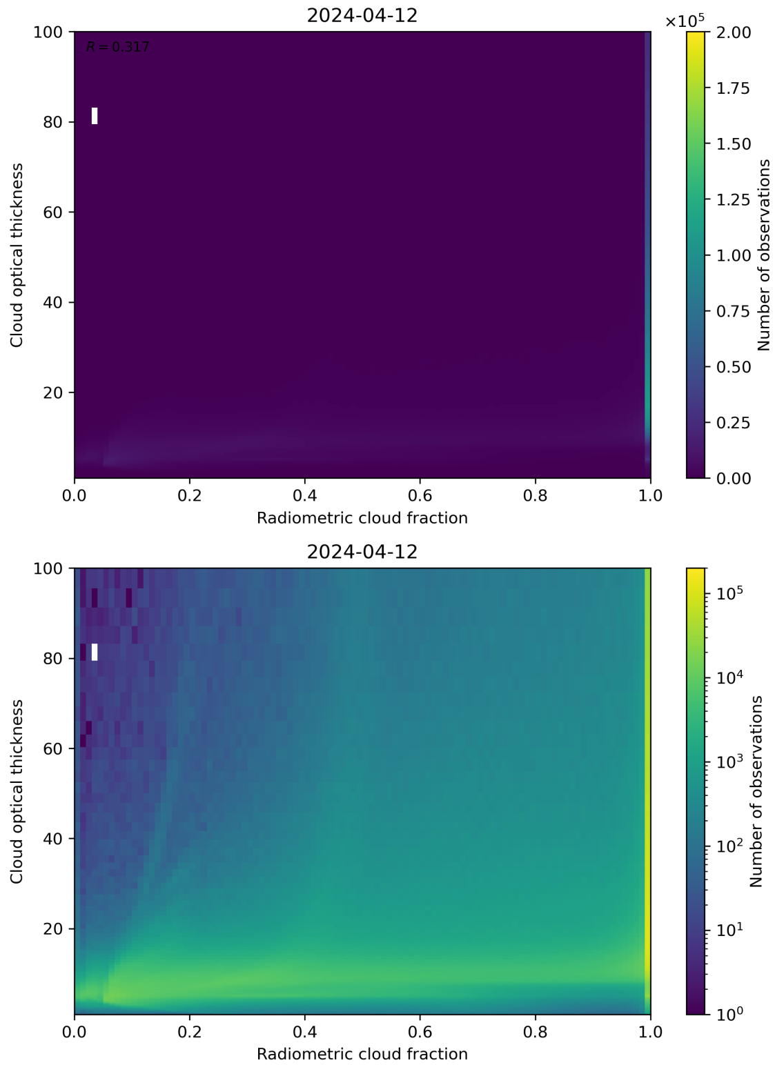
Figure 75: Scatter density plot of “Radiometric cloud fraction” against “Cloud optical thickness” for 2024-04-11 to 2024-04-13.
