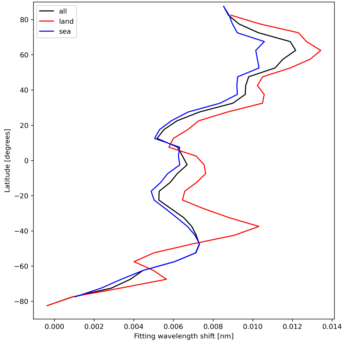
Figure 33: Zonal average of “Fitting wavelength shift” for 2024-04-11 to 2024-04-13.
