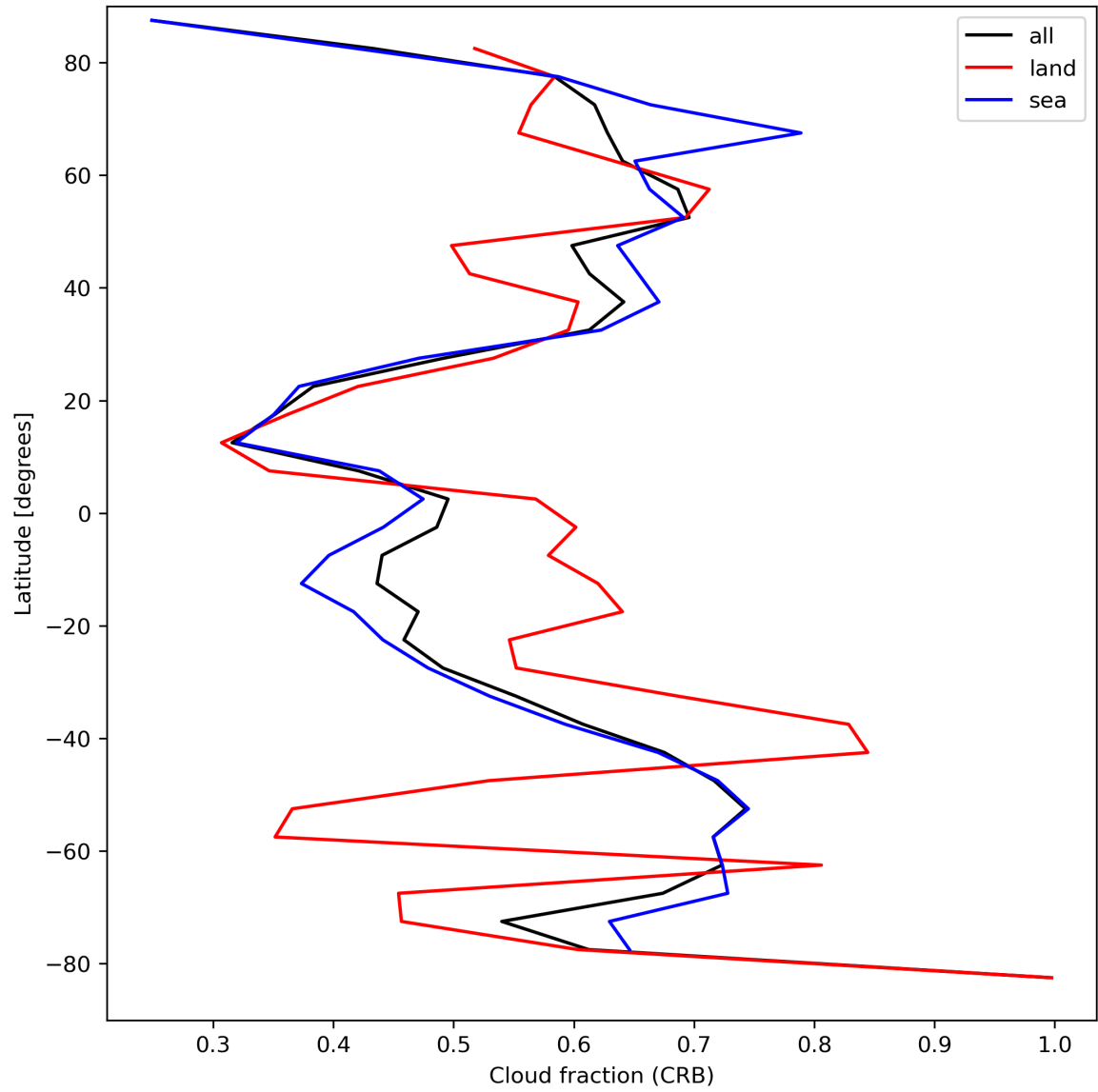
Figure 26: Zonal average of “Cloud fraction (CRB)” for 2024-04-11 to 2024-04-13.
