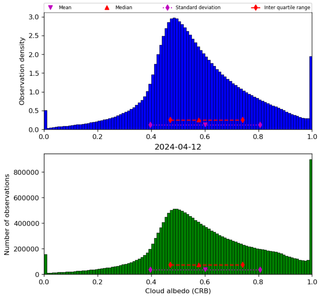
Figure 44: Histogram of “Cloud albedo (CRB)” for 2024-04-11 to 2024-04-13
