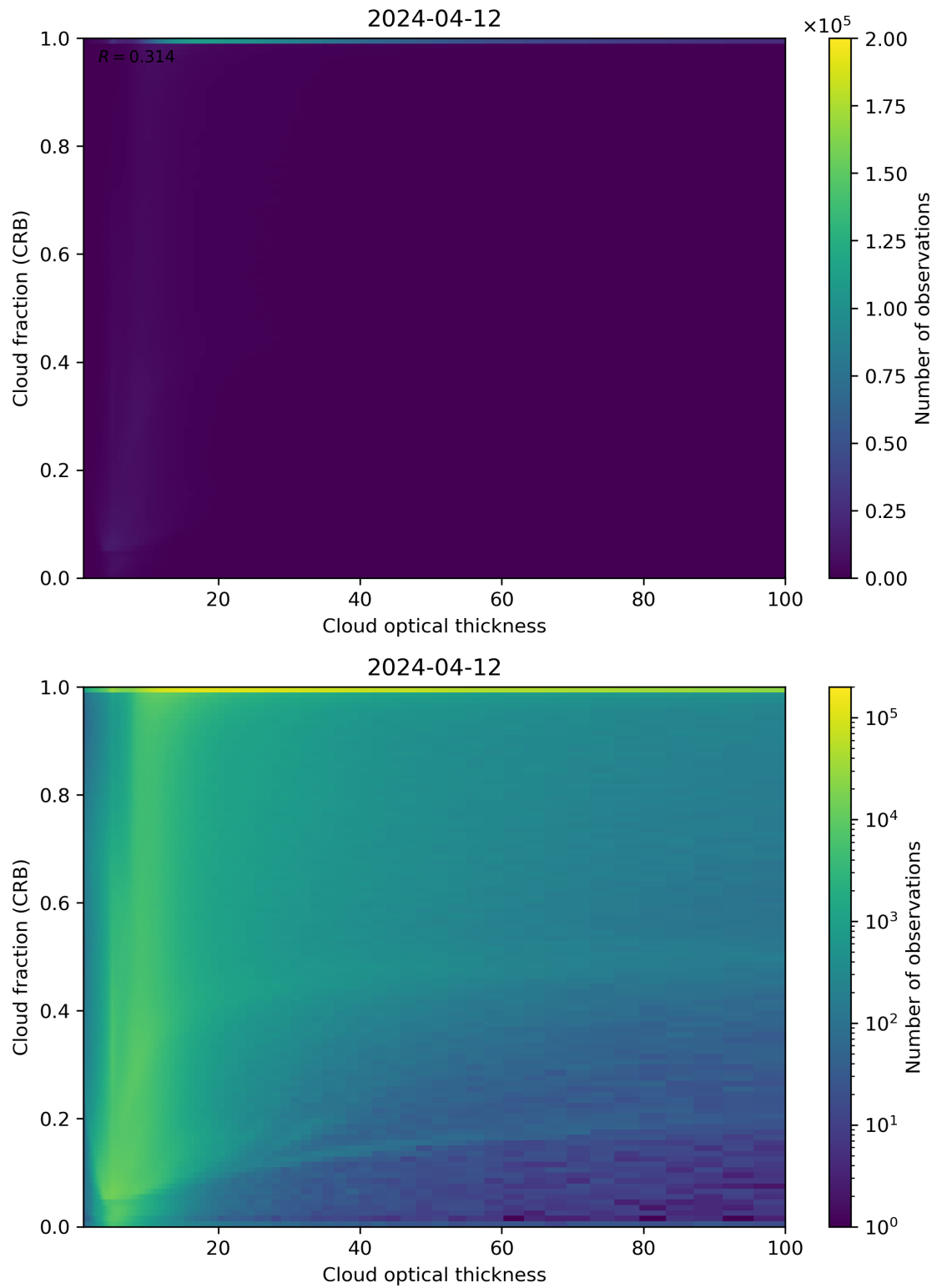
Figure 84: Scatter density plot of “Cloud optical thickness” against “Cloud fraction (CRB)” for 2024-04-11 to 2024-04-13.
