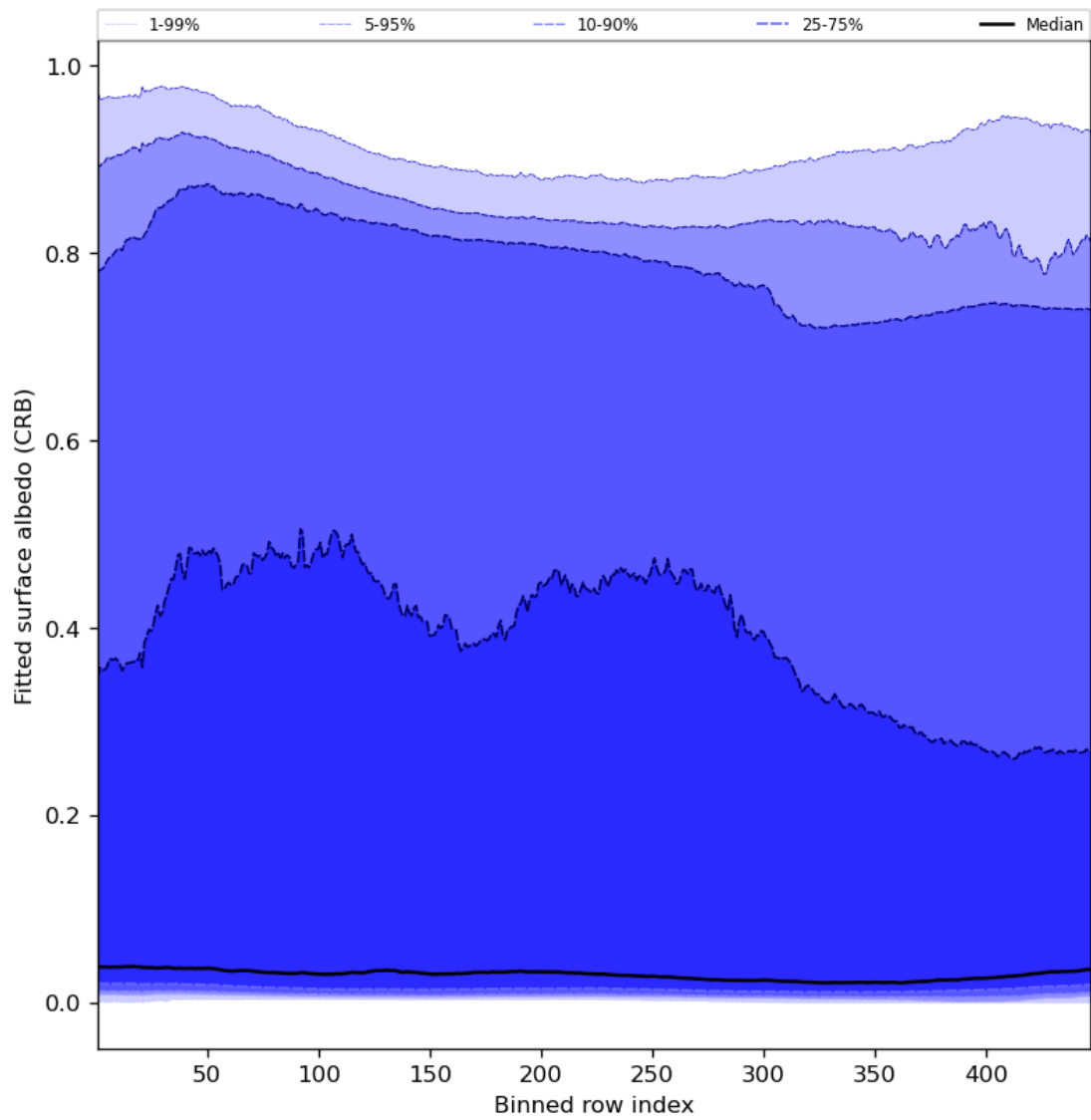
Figure 62: Along track statistics of “Fitted surface albedo (CRB)” for 2024-04-11 to 2024-04-13
