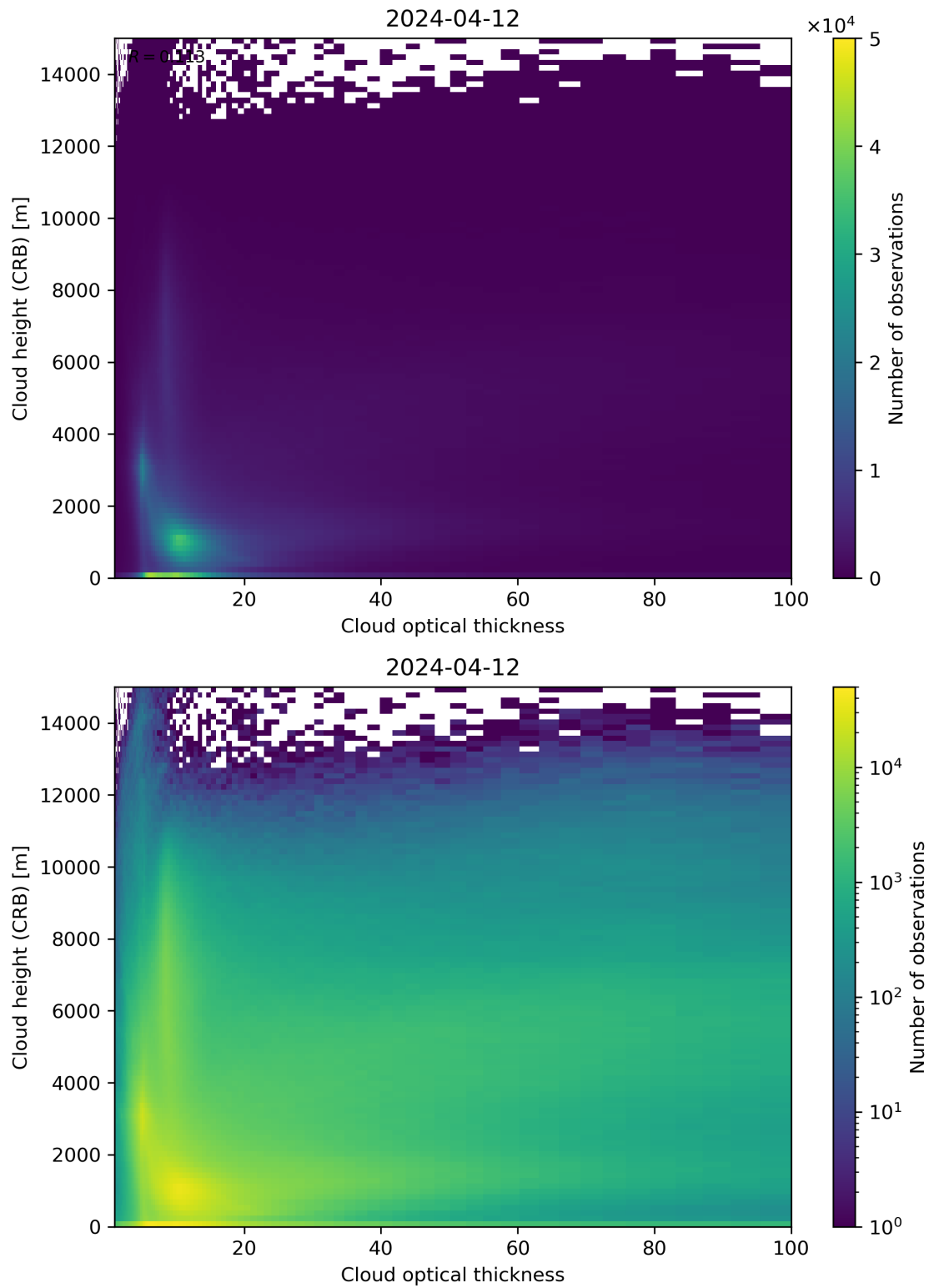
Figure 85: Scatter density plot of “Cloud optical thickness” against “Cloud height (CRB)” for 2024-04-11 to 2024-04-13.
