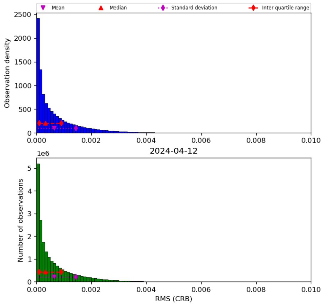
Figure 48: Histogram of “RMS (CRB)” for 2024-04-11 to 2024-04-13
