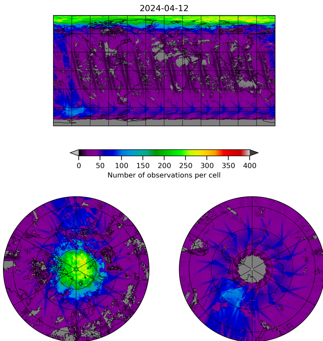
Figure 21: Map of the number of observations for 2024-04-11 to 2024-04-13
