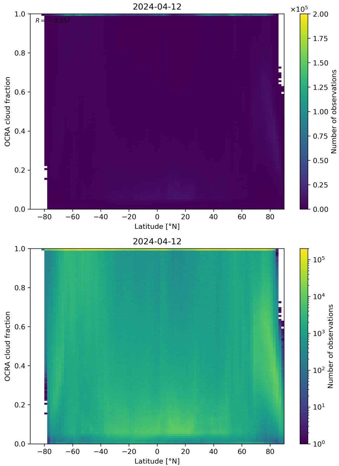
Figure 93: Scatter density plot of “Latitude” against “OCRA cloud fraction” for 2024-04-11 to 2024-04-13.
