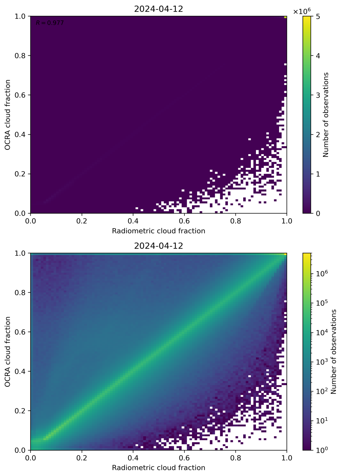
Figure 72: Scatter density plot of “Radiometric cloud fraction” against “OCRA cloud fraction” for 2024-04-11 to 2024-04-13.
