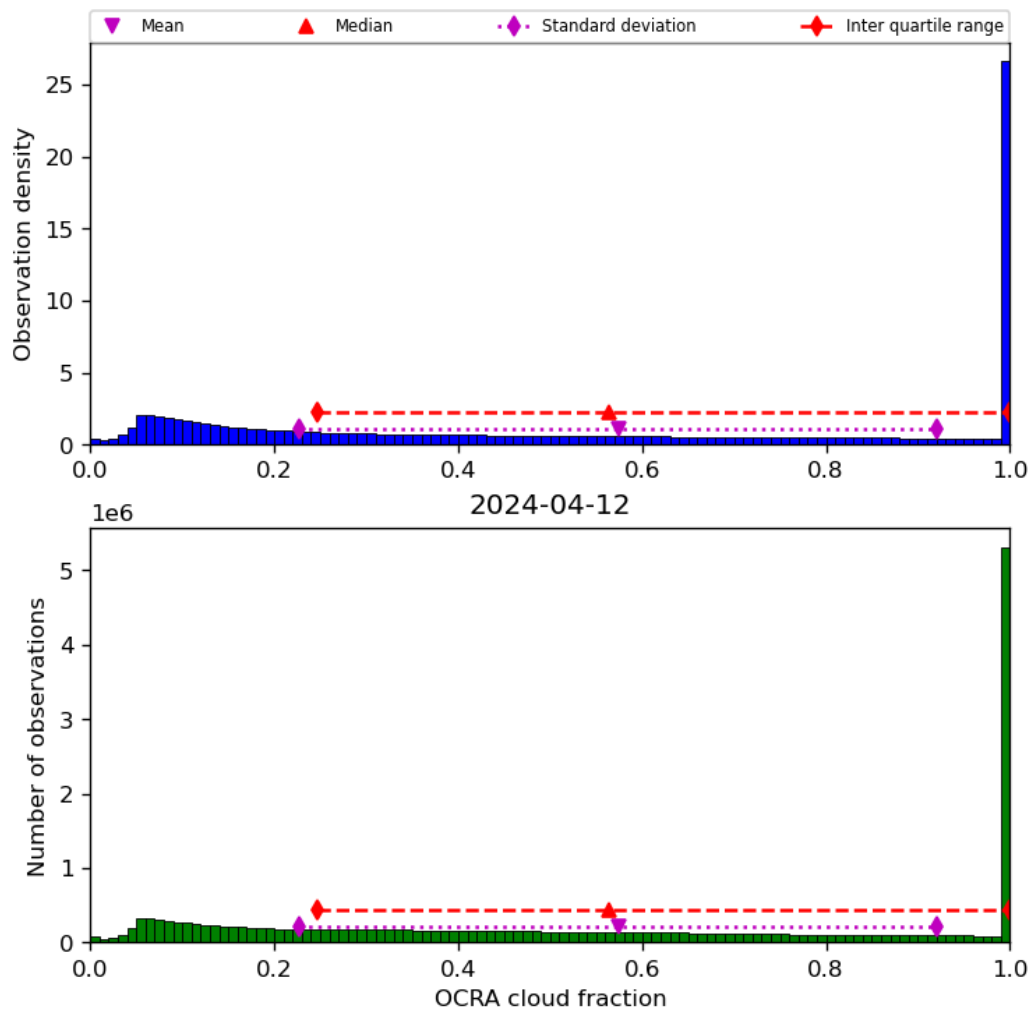
Figure 50: Histogram of “OCRA cloud fraction” for 2024-04-11 to 2024-04-13
