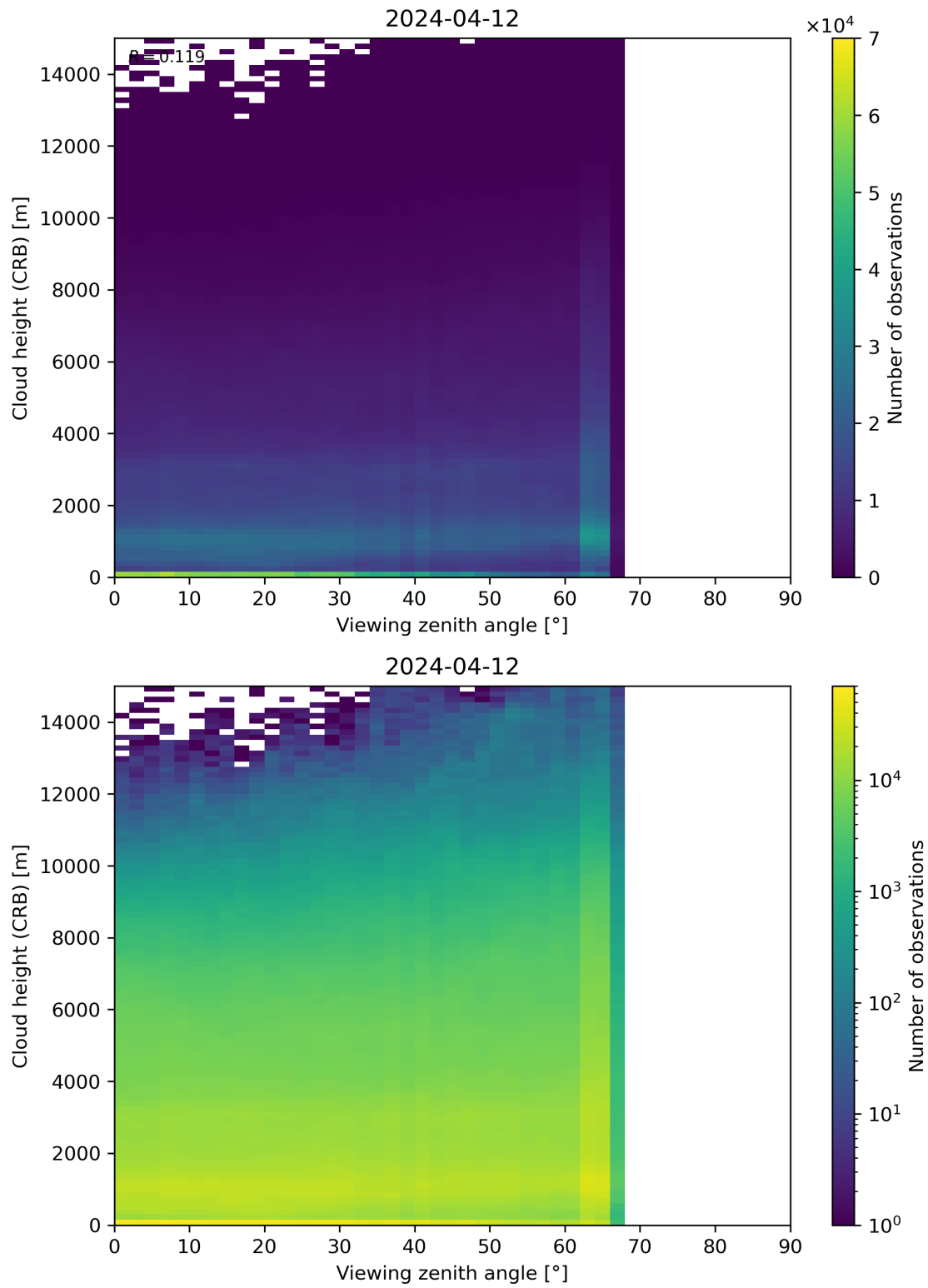
Figure 110: Scatter density plot of “Viewing zenith angle” against “Cloud height (CRB)” for 2024-04-11 to 2024-04-13.
