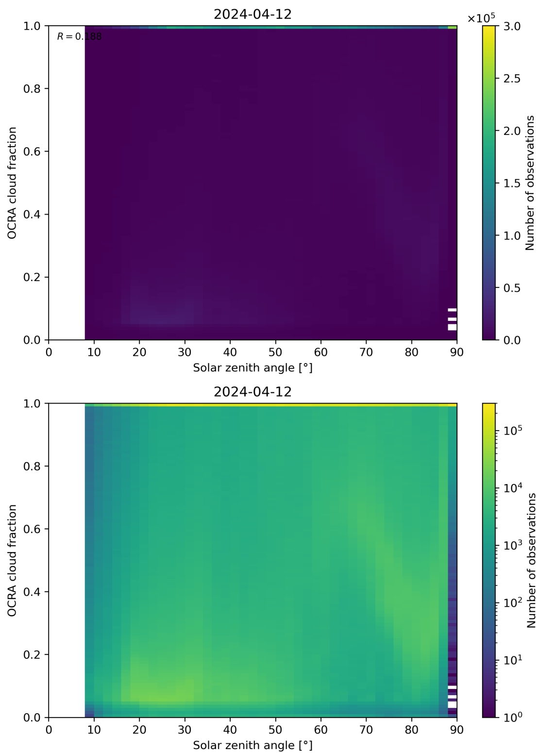
Figure 100: Scatter density plot of “Solar zenith angle” against “OCRA cloud fraction” for 2024-04-11 to 2024-04-13.
