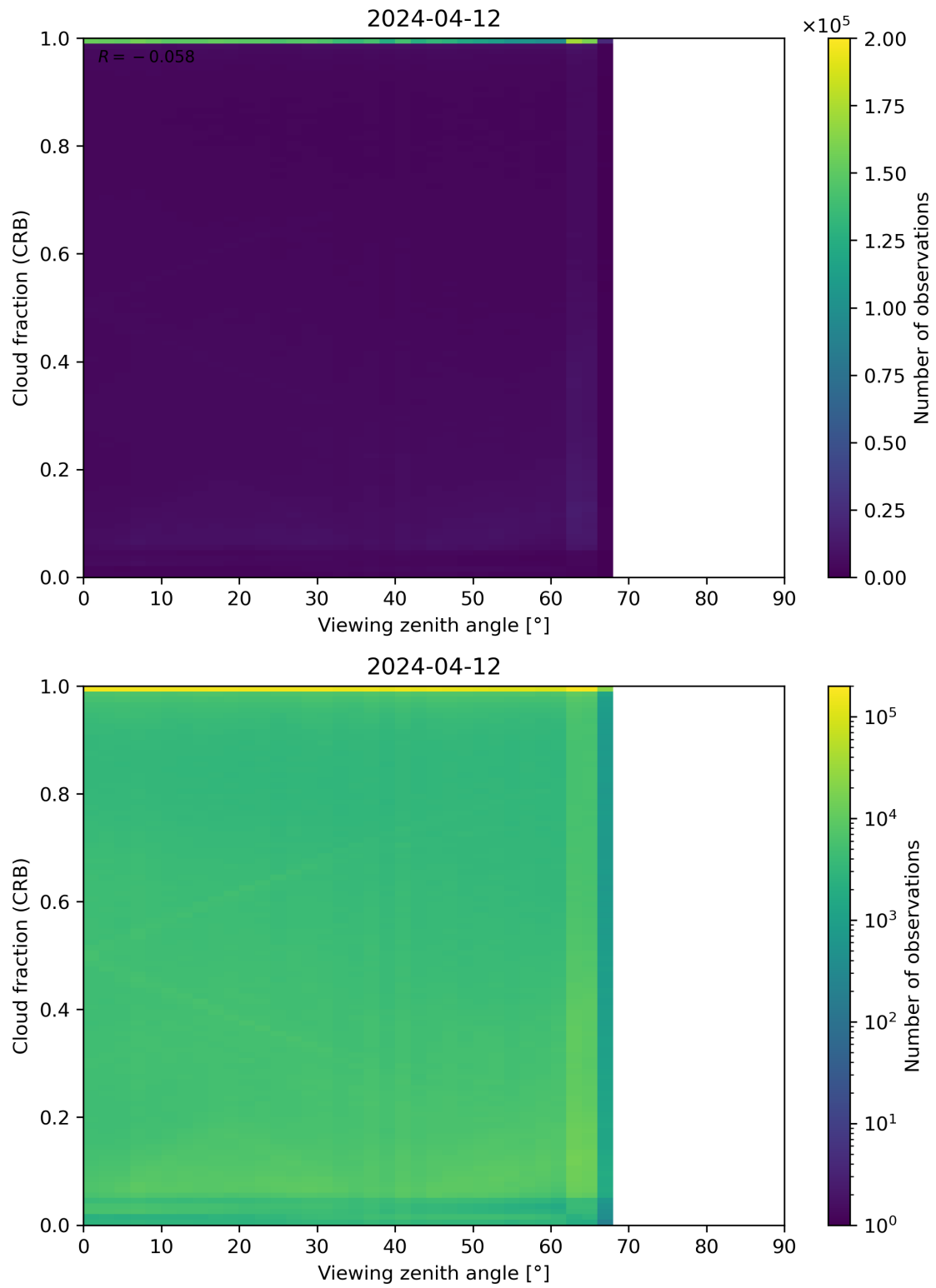
Figure 109: Scatter density plot of “Viewing zenith angle” against “Cloud fraction (CRB)” for 2024-04-11 to 2024-04-13.
