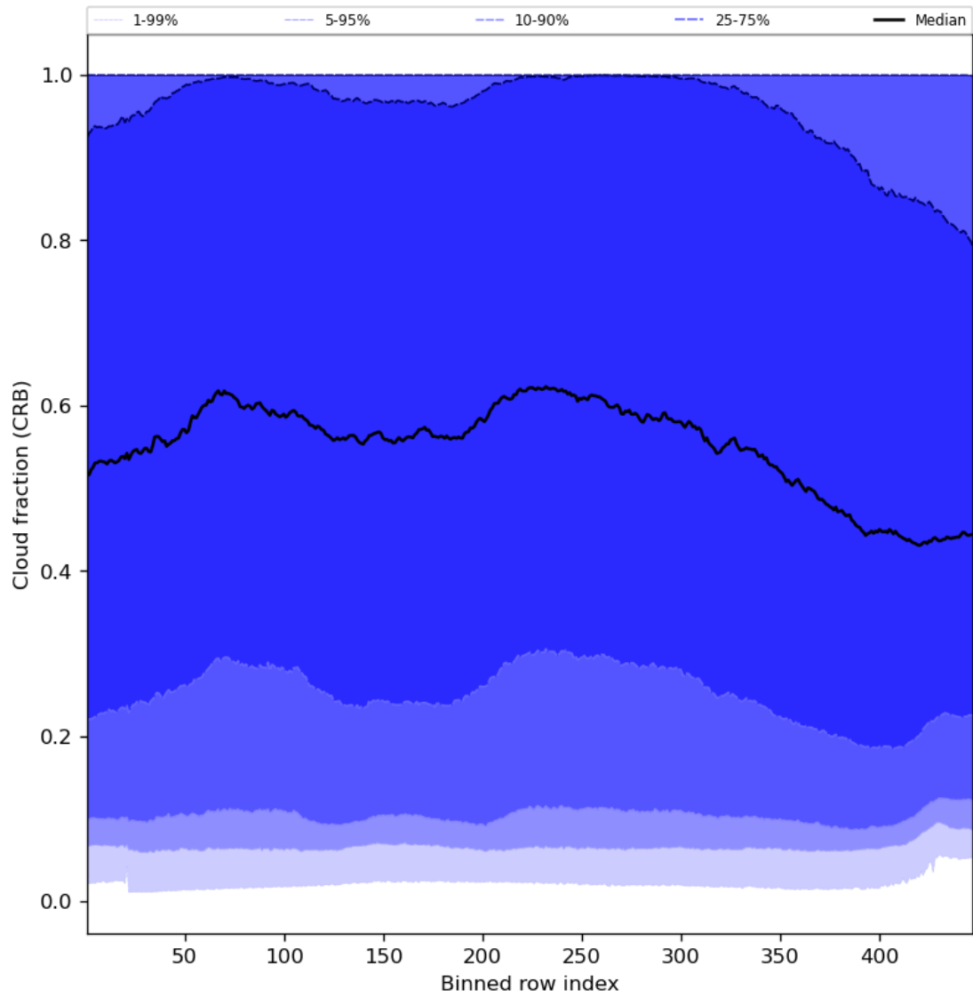
Figure 58: Along track statistics of “Cloud fraction (CRB)” for 2024-04-11 to 2024-04-13
