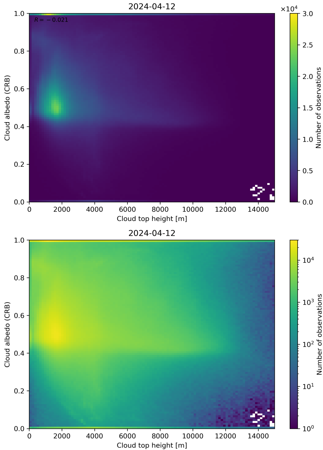
Figure 86: Scatter density plot of “Cloud top height” against “Cloud albedo (CRB)” for 2024-04-11 to 2024-04-13.
