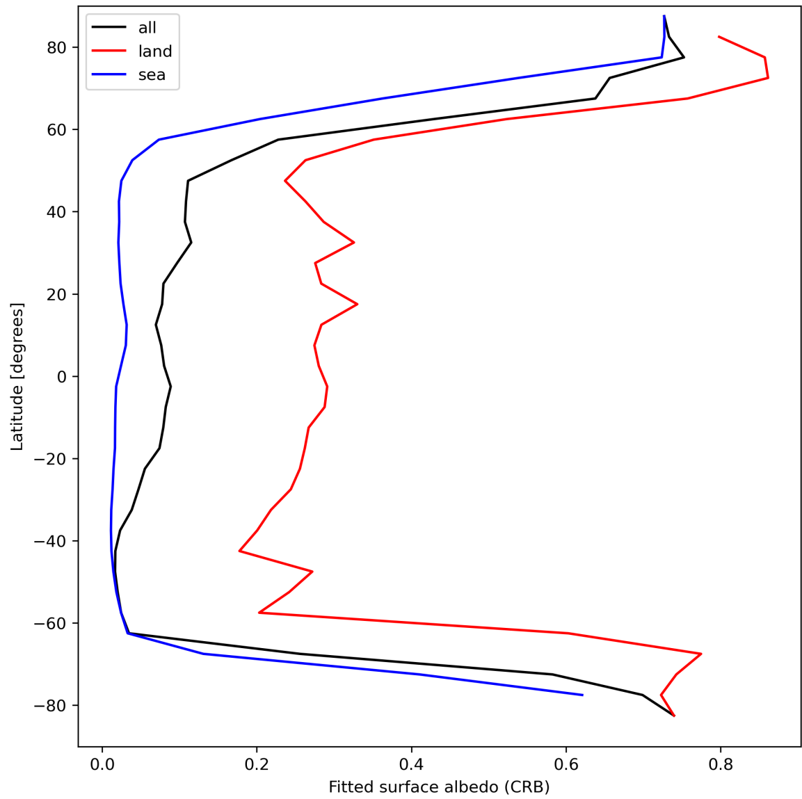
Figure 30: Zonal average of “Fitted surface albedo (CRB)” for 2024-04-11 to 2024-04-13.
