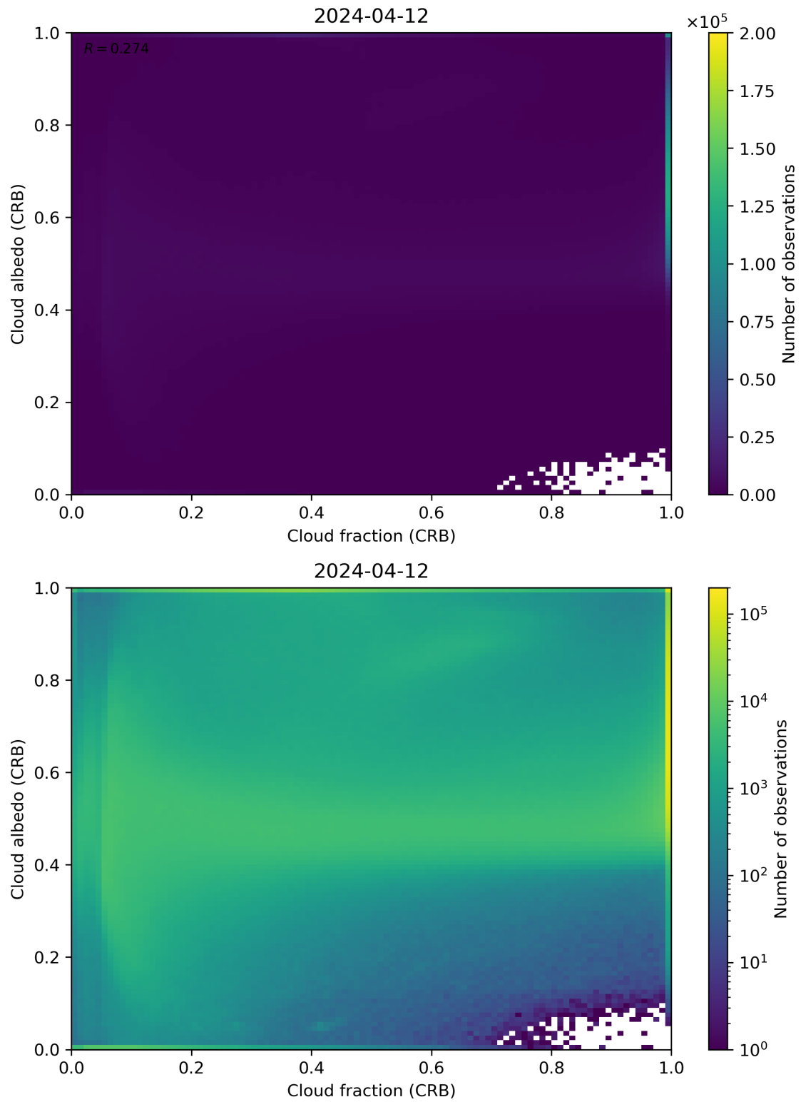
Figure 77: Scatter density plot of “Cloud fraction (CRB)” against “Cloud albedo (CRB)” for 2024-04-11 to 2024-04-13.
