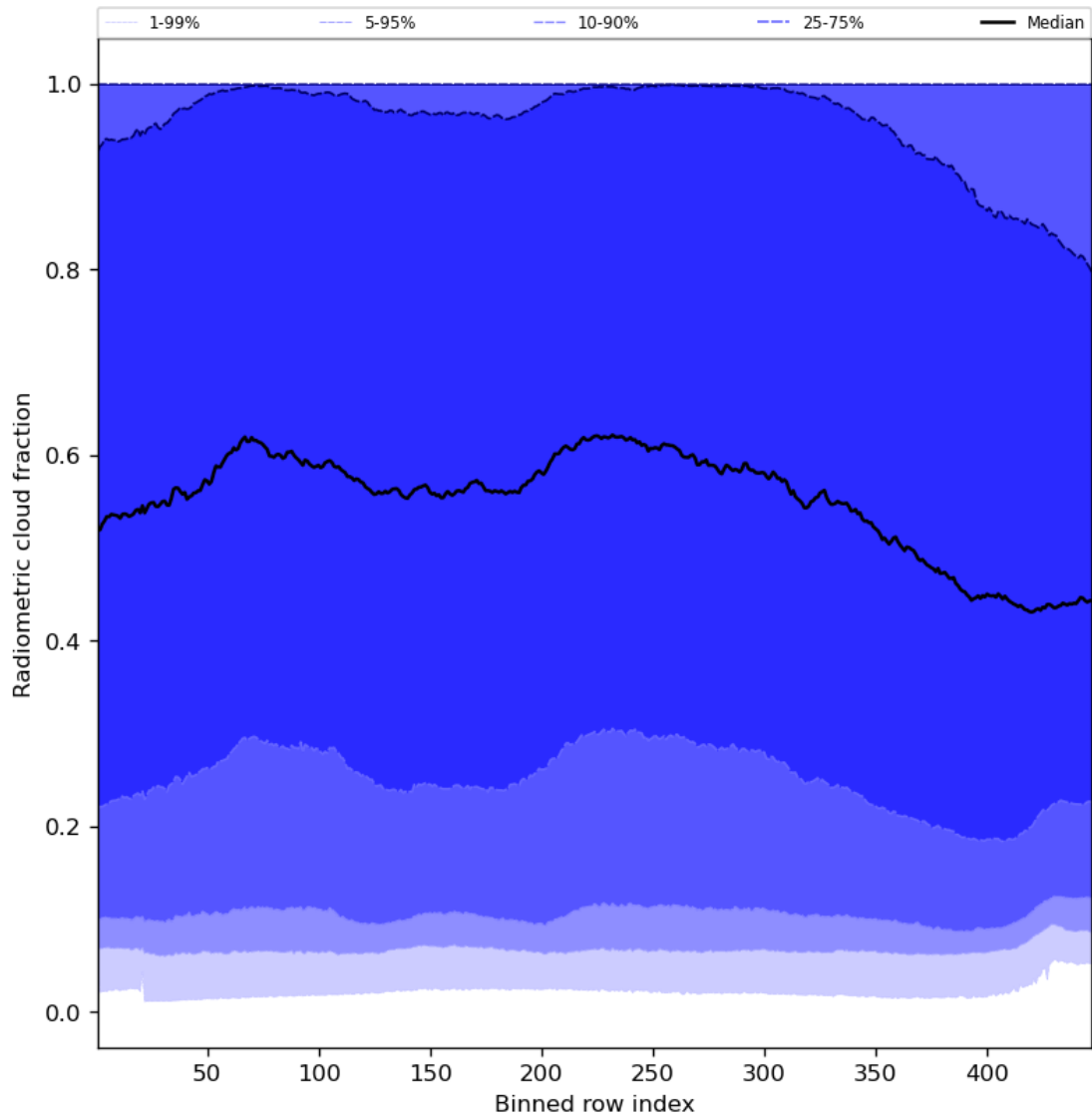
Figure 55: Along track statistics of “Radiometric cloud fraction” for 2024-04-11 to 2024-04-13
