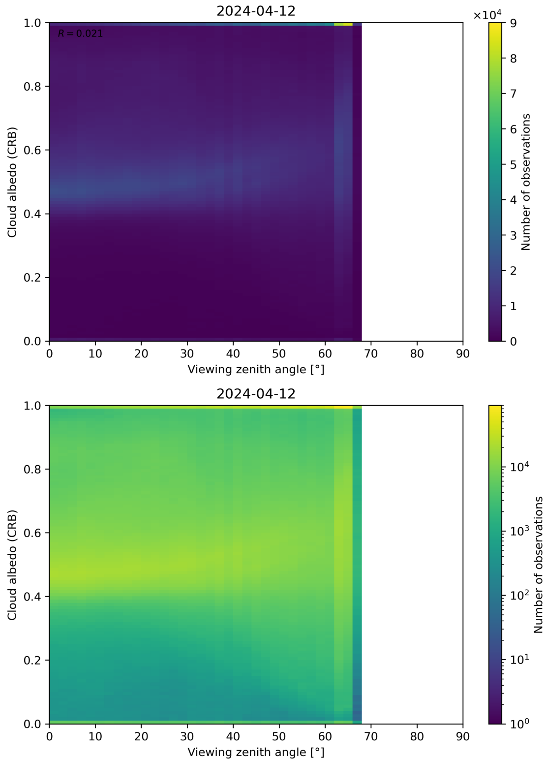
Figure 106: Scatter density plot of “Viewing zenith angle” against “Cloud albedo (CRB)” for 2024-04-11 to 2024-04-13.
