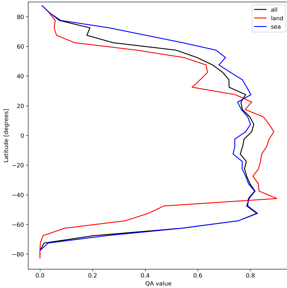
Figure 22: Zonal average of “QA value” for 2024-04-11 to 2024-04-13.
