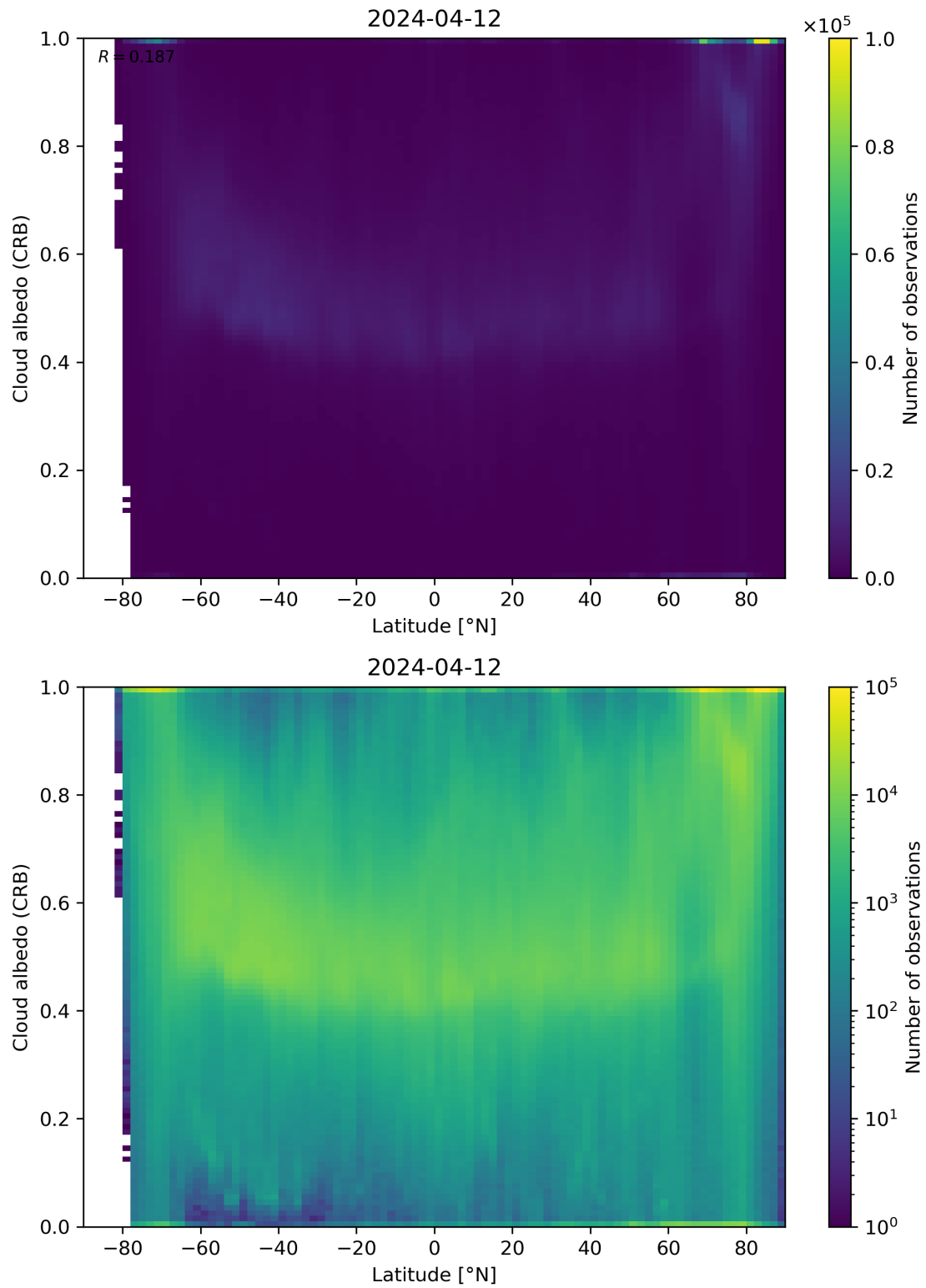
Figure 91: Scatter density plot of “Latitude” against “Cloud albedo (CRB)” for 2024-04-11 to 2024-04-13.
