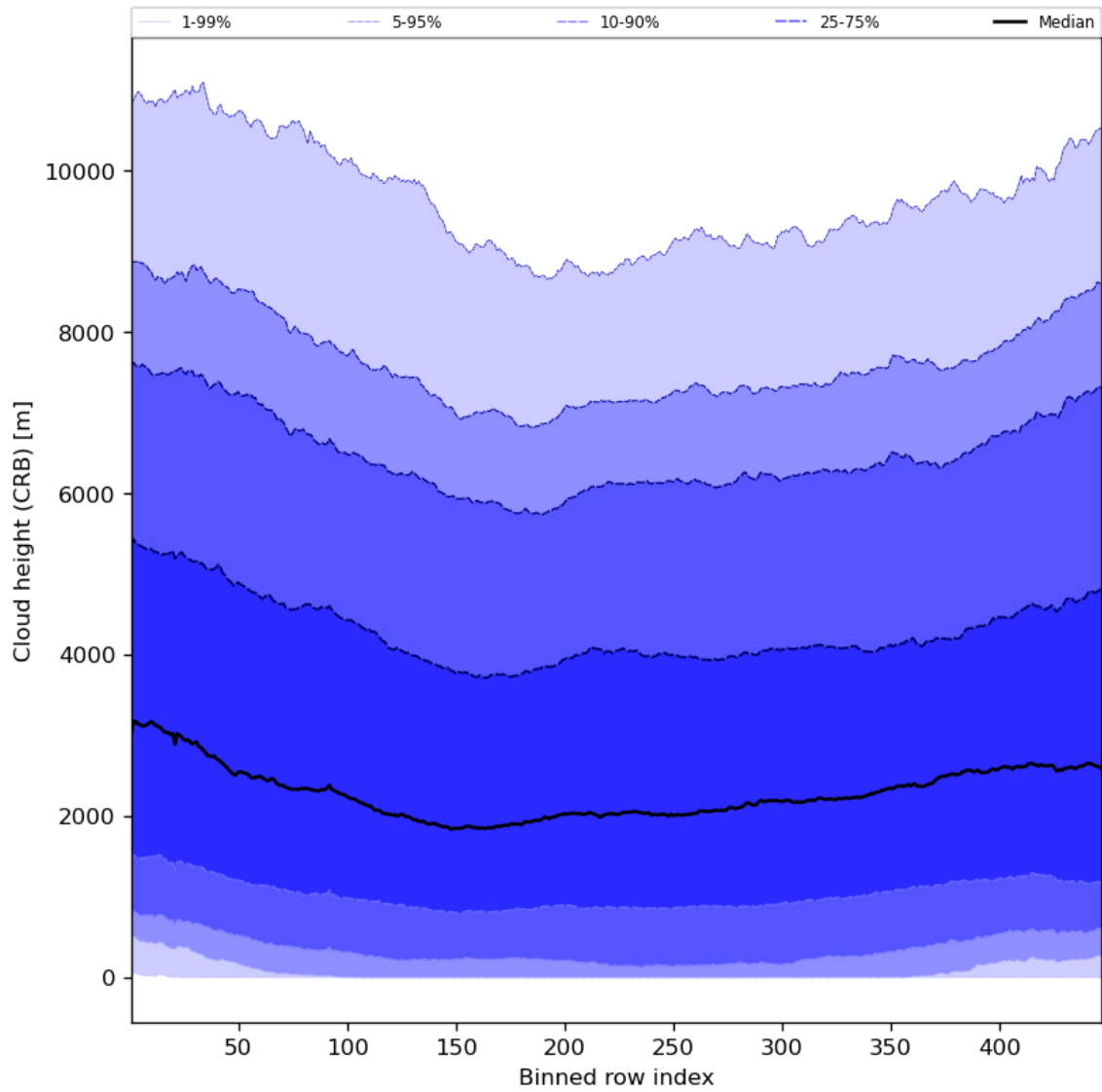
Figure 59: Along track statistics of “Cloud height (CRB)” for 2024-04-11 to 2024-04-13
