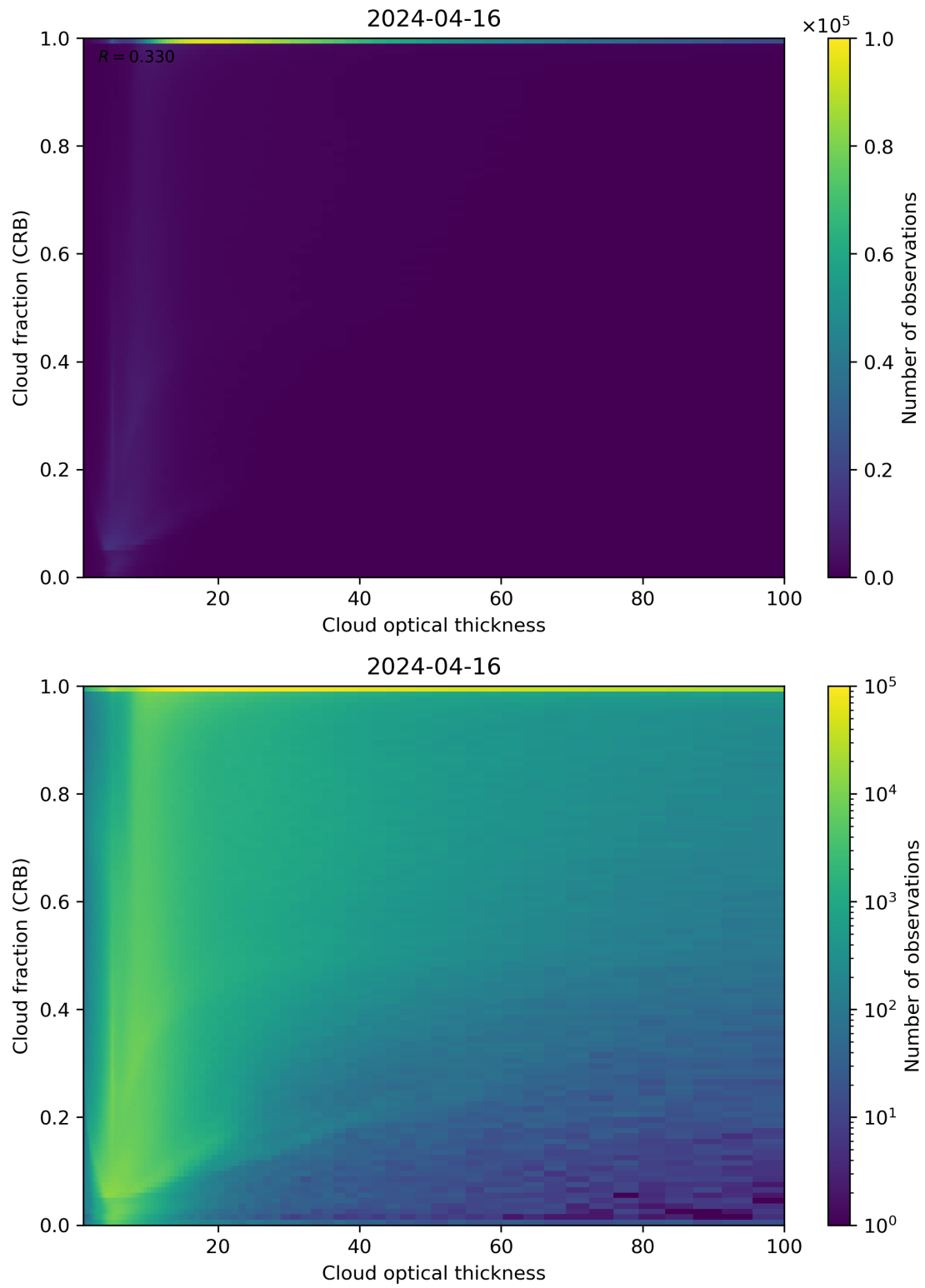
Figure 84: Scatter density plot of “Cloud optical thickness” against “Cloud fraction (CRB)” for 2024-04-16 to 2024-04-17.
