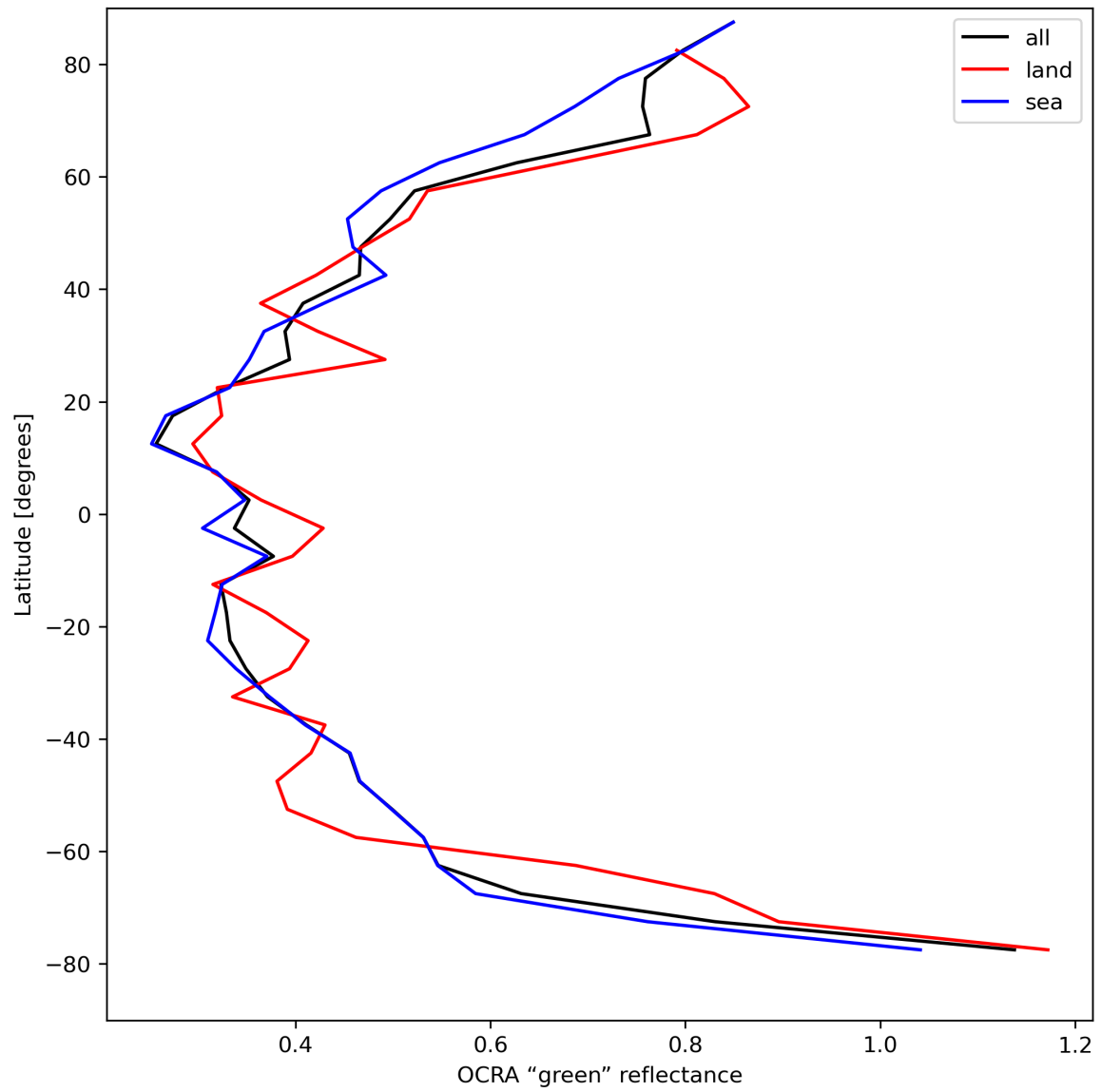
Figure 36: Zonal average of “OCRA “green” reflectance” for 2024-04-16 to 2024-04-17.
