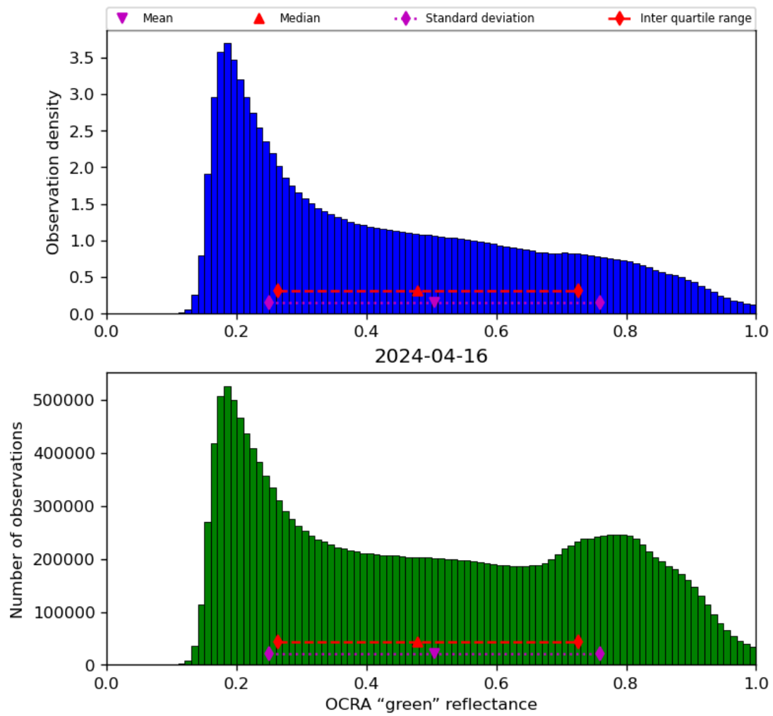
Figure 52: Histogram of “OCRA “green” reflectance” for 2024-04-16 to 2024-04-17
