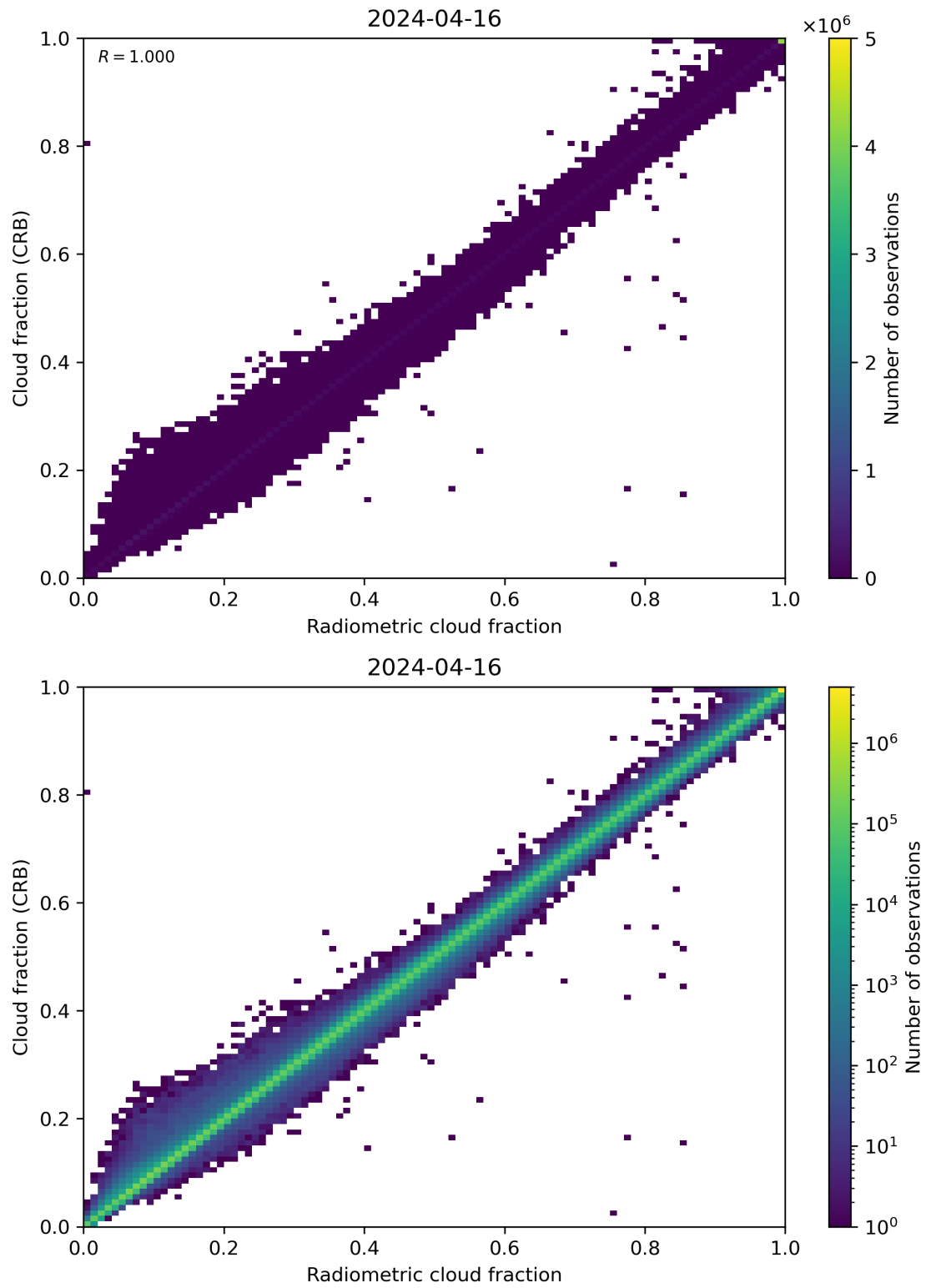
Figure 73: Scatter density plot of “Radiometric cloud fraction” against “Cloud fraction (CRB)” for 2024-04-16 to 2024-04-17.
