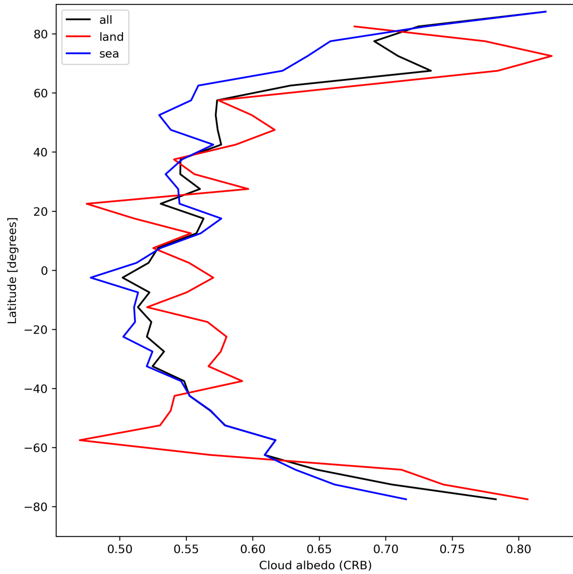
Figure 28: Zonal average of “Cloud albedo (CRB)” for 2024-04-16 to 2024-04-17.
