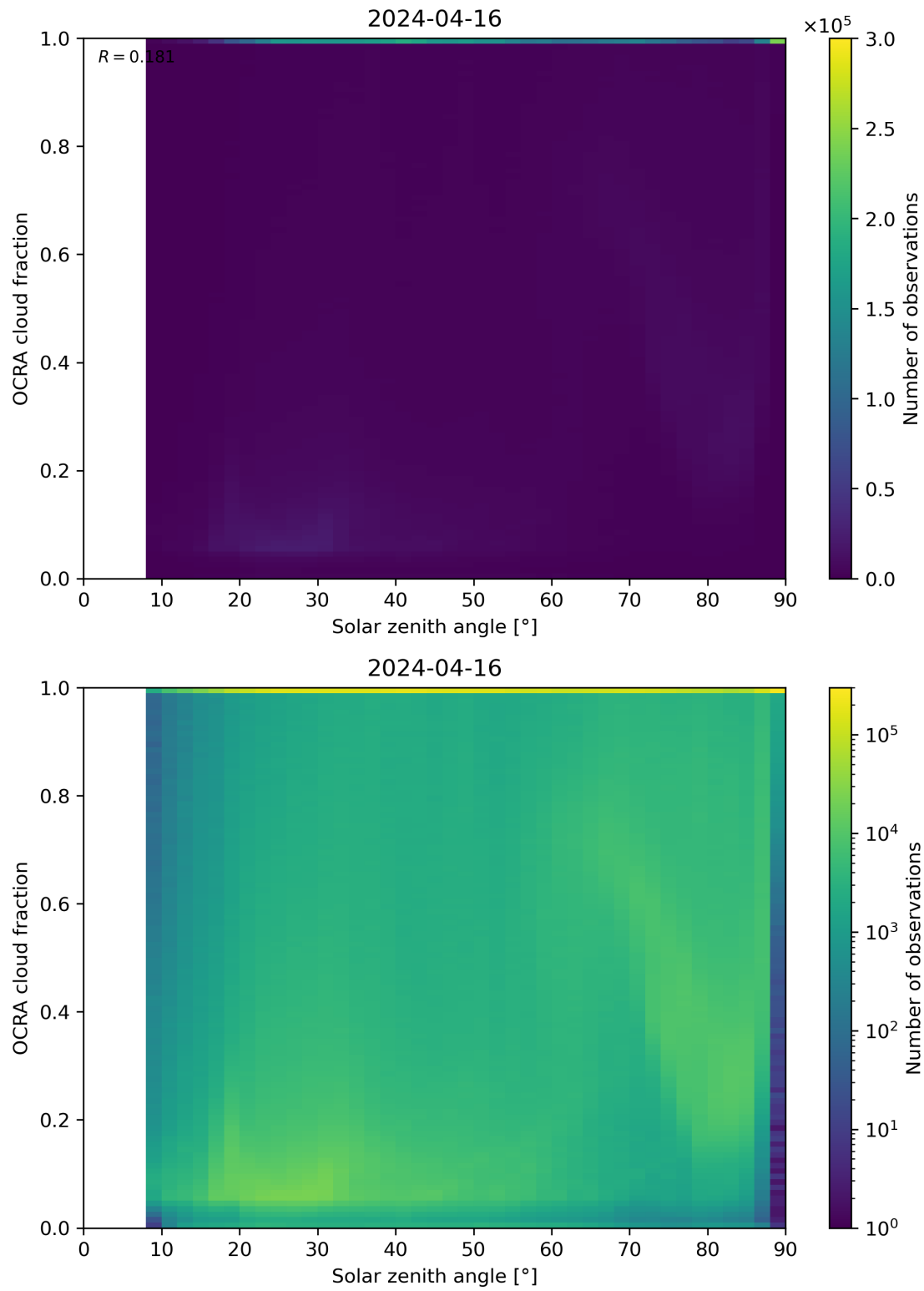
Figure 100: Scatter density plot of “Solar zenith angle” against “OCRA cloud fraction” for 2024-04-16 to 2024-04-17.
