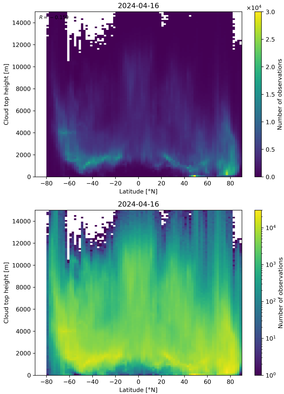
Figure 97: Scatter density plot of “Latitude” against “Cloud top height” for 2024-04-16 to 2024-04-17.
