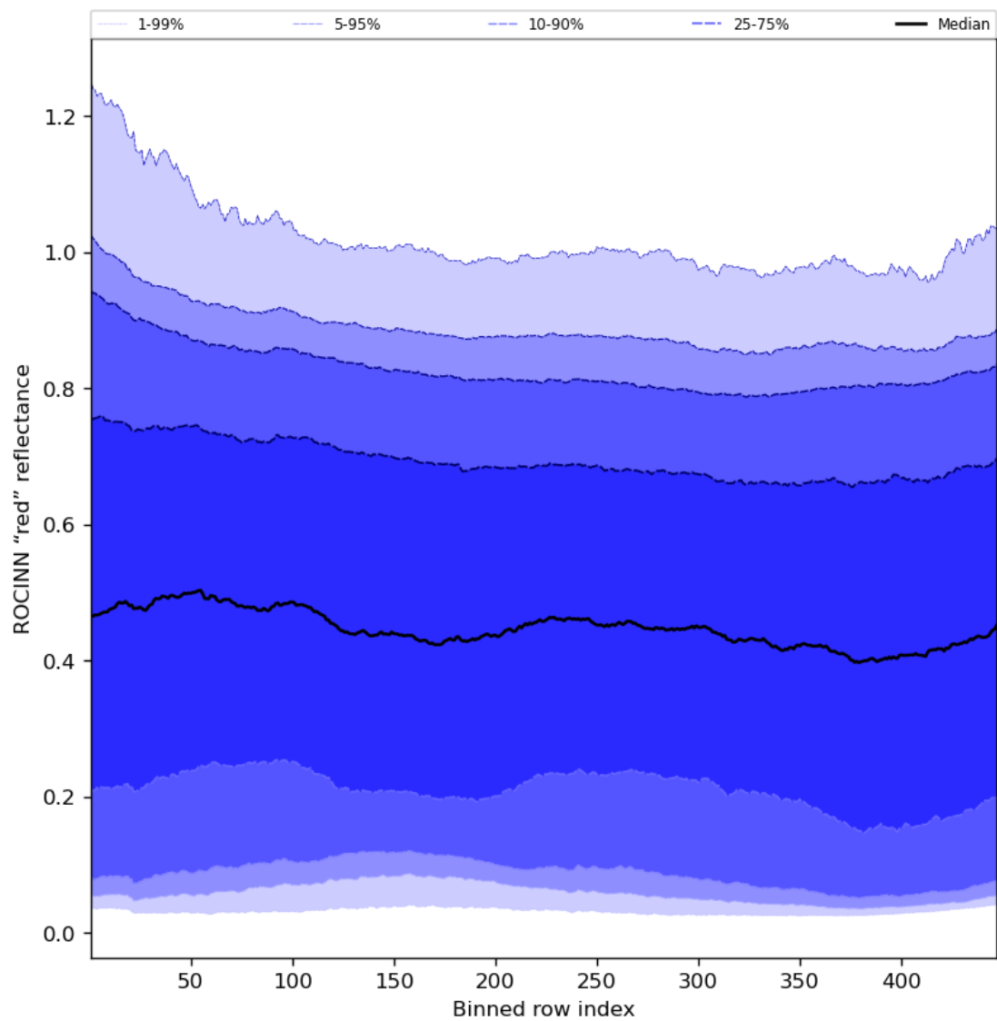
Figure 69: Along track statistics of “ROCINN “red” reflectance” for 2024-04-16 to 2024-04-17
