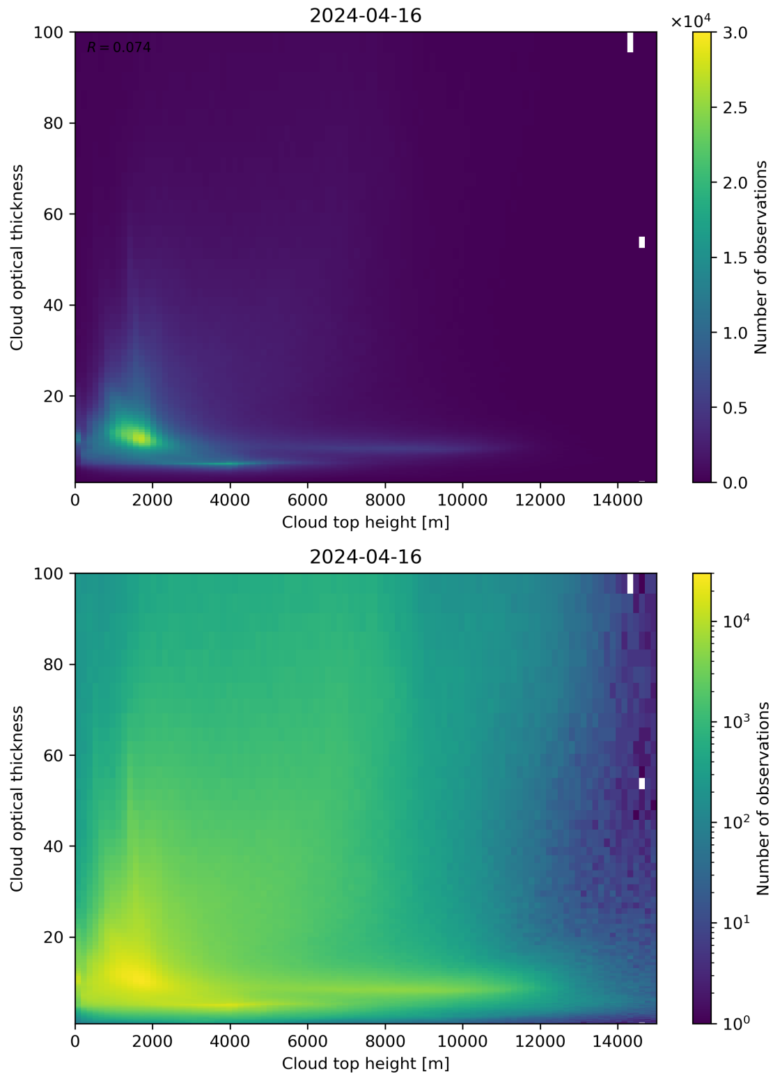
Figure 90: Scatter density plot of “Cloud top height” against “Cloud optical thickness” for 2024-04-16 to 2024-04-17.
