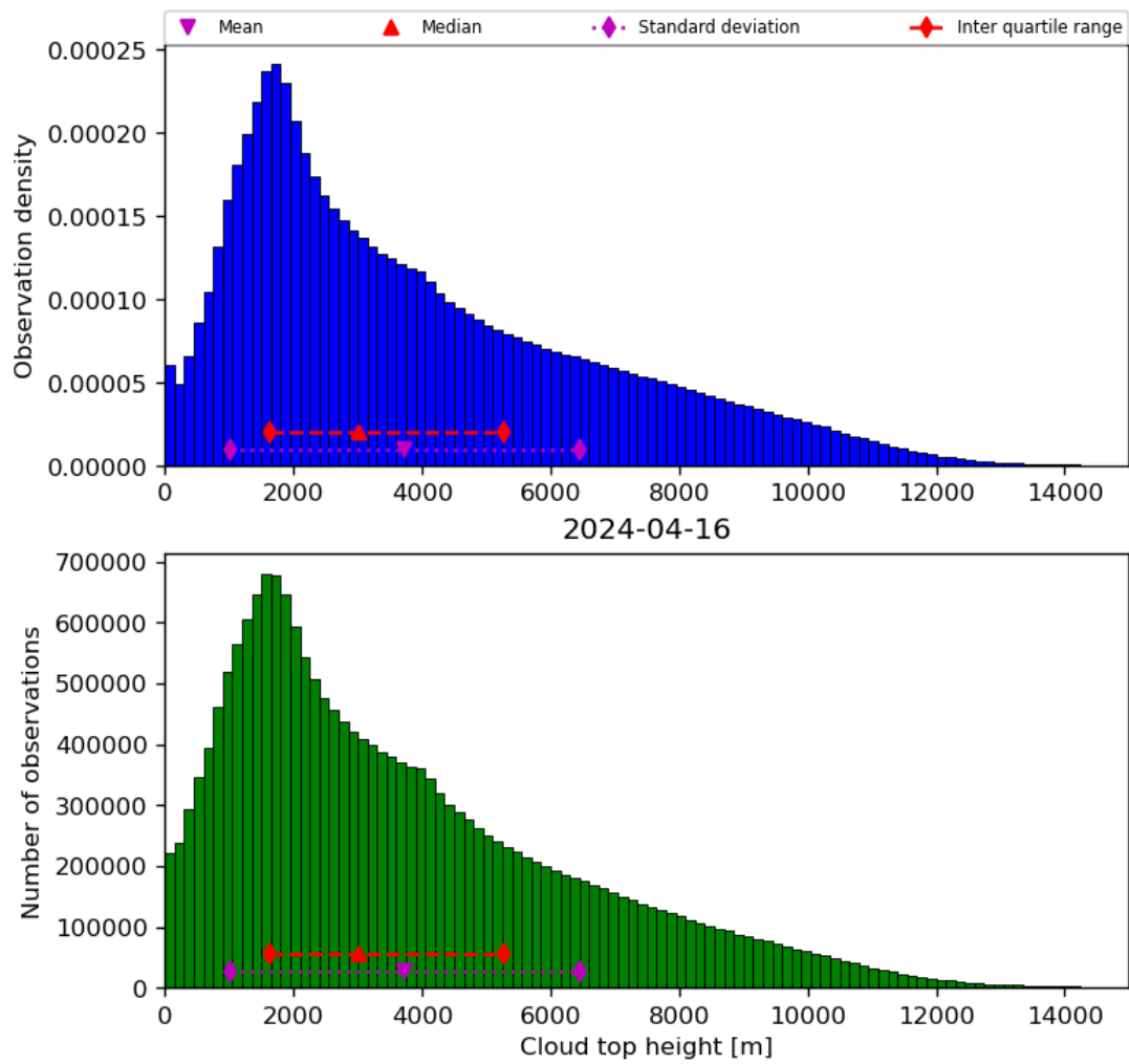
Figure 40: Histogram of “Cloud top height” for 2024-04-16 to 2024-04-17
