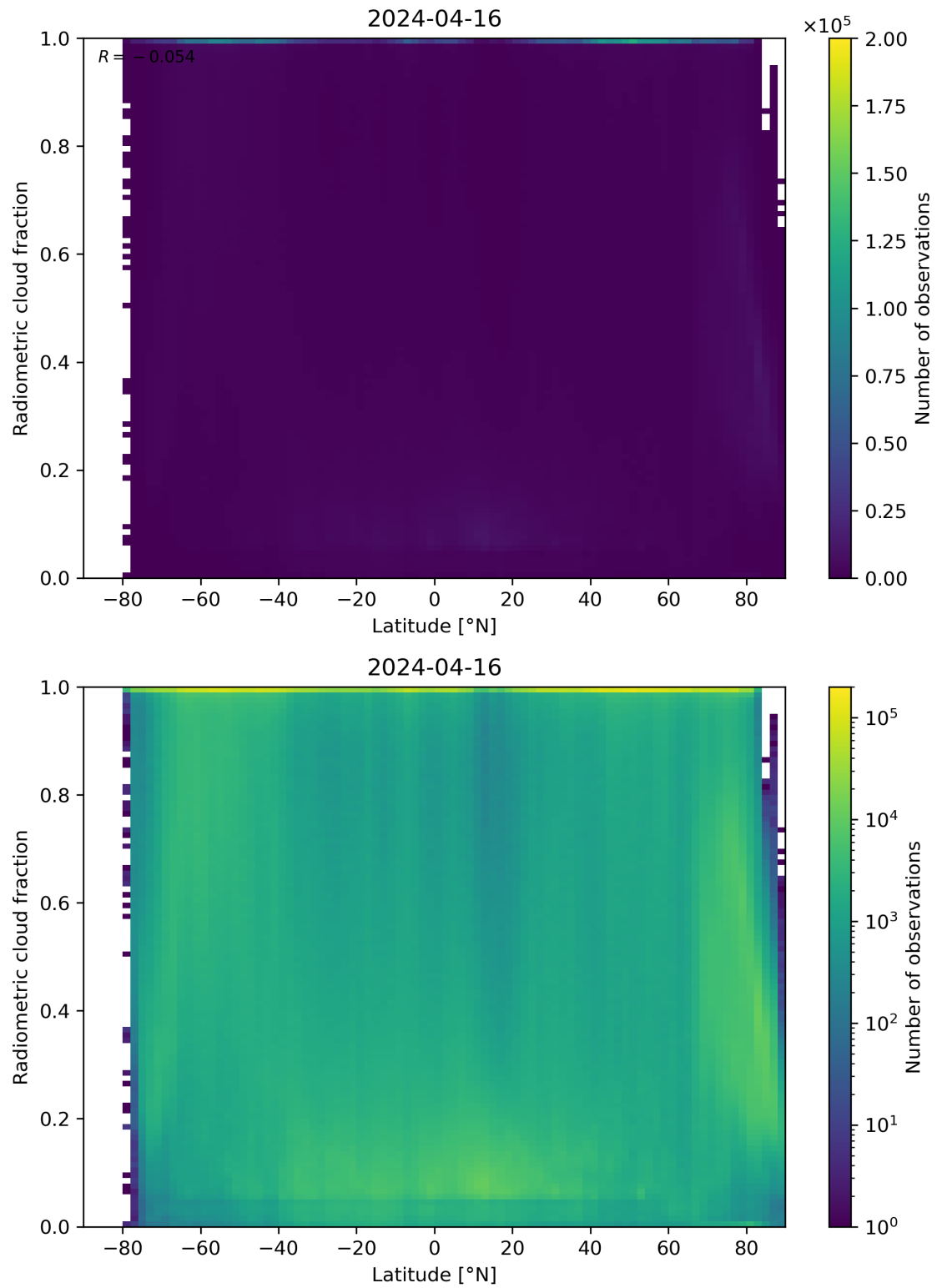
Figure 92: Scatter density plot of “Latitude” against “Radiometric cloud fraction” for 2024-04-16 to 2024-04-17.
