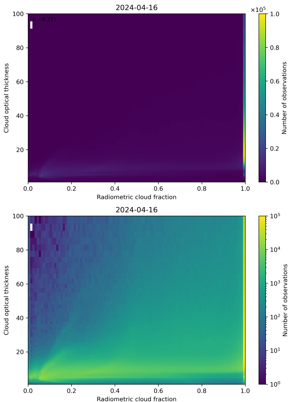
Figure 75: Scatter density plot of “Radiometric cloud fraction” against “Cloud optical thickness” for 2024-04-16 to 2024-04-17.
