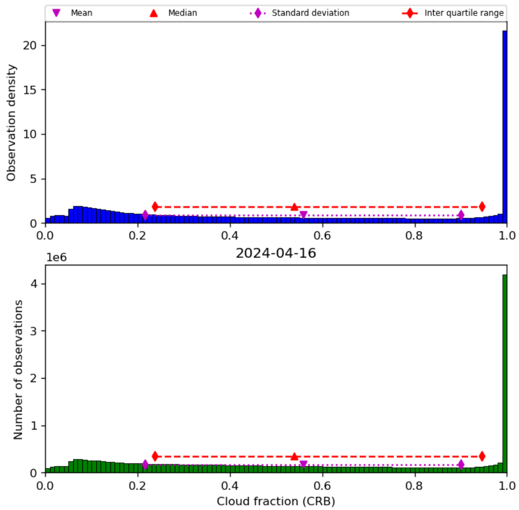
Figure 42: Histogram of “Cloud fraction (CRB)” for 2024-04-16 to 2024-04-17
