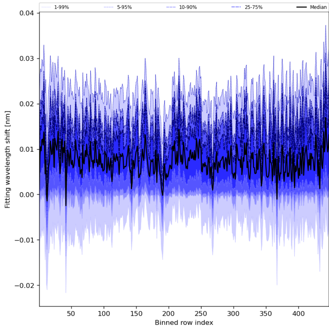
Figure 65: Along track statistics of “Fitting wavelength shift” for 2024-04-16 to 2024-04-17
