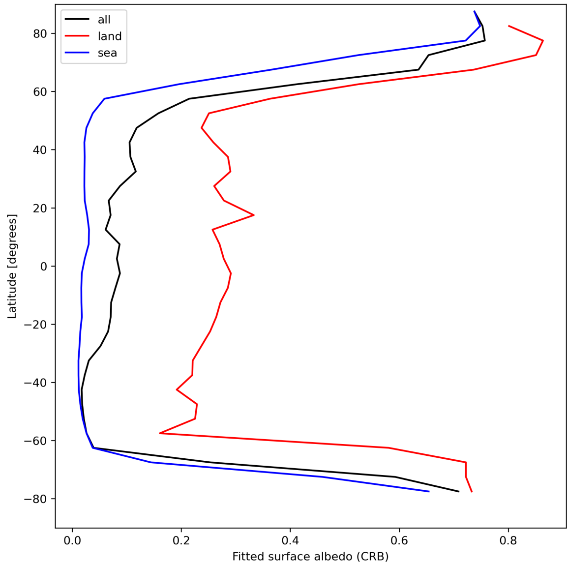
Figure 30: Zonal average of “Fitted surface albedo (CRB)” for 2024-04-16 to 2024-04-17.
