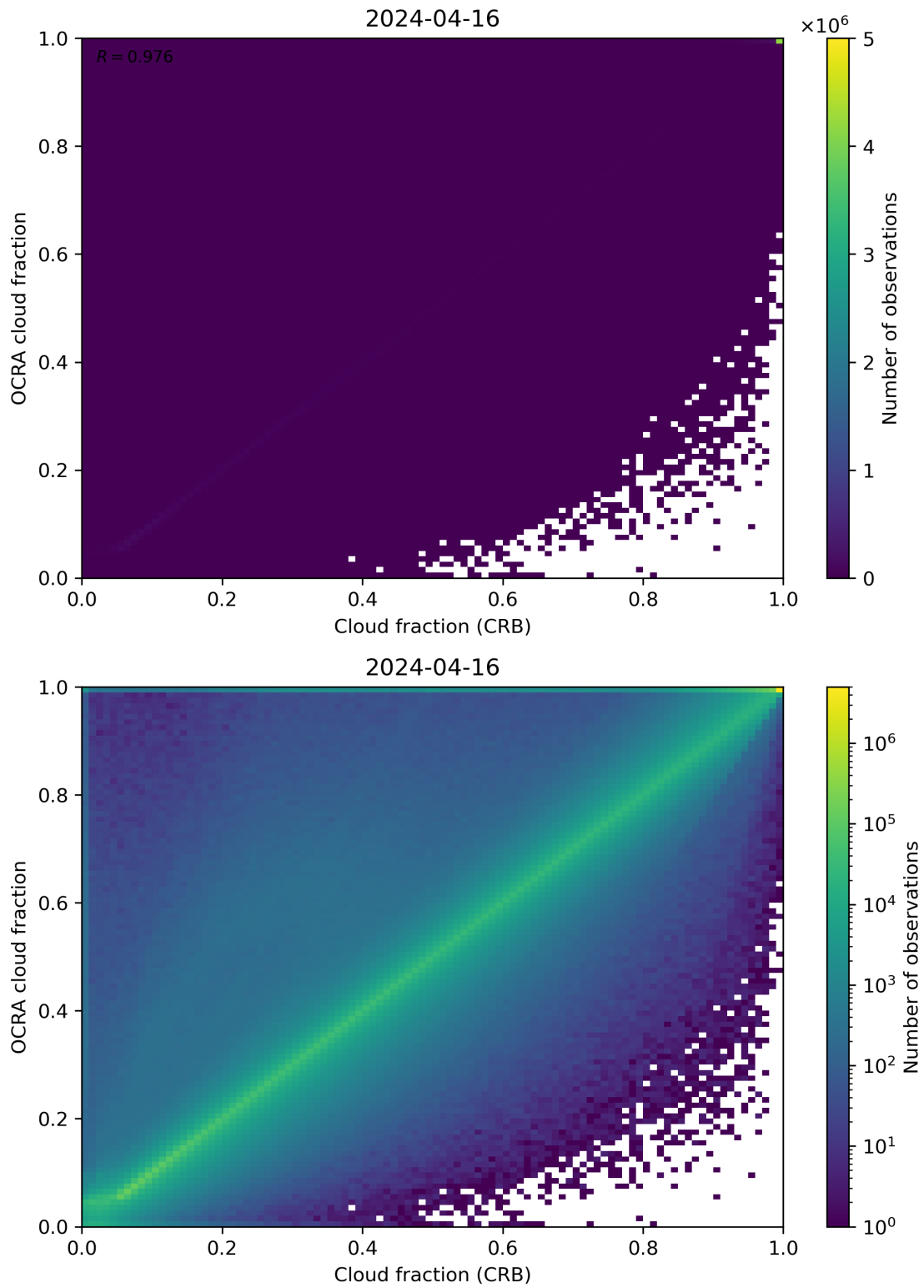
Figure 78: Scatter density plot of “Cloud fraction (CRB)” against “OCRA cloud fraction” for 2024-04-16 to 2024-04-17.
