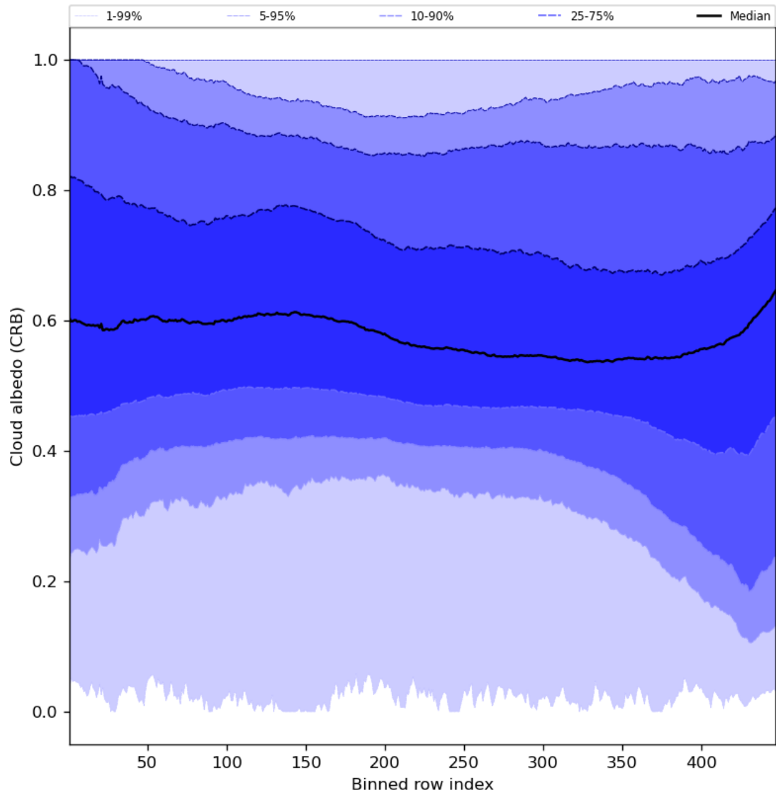
Figure 60: Along track statistics of “Cloud albedo (CRB)” for 2024-04-16 to 2024-04-17
