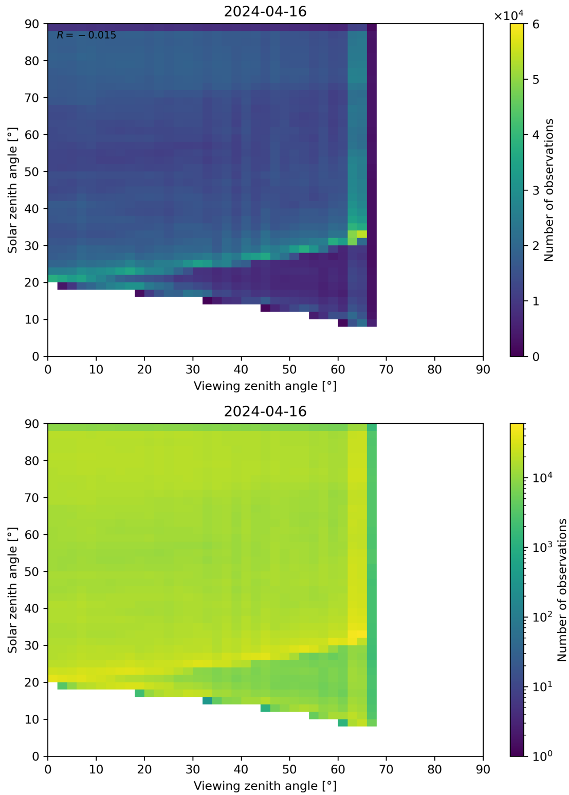
Figure 114: Scatter density plot of “Viewing zenith angle” against “Solar zenith angle” for 2024-04-16 to 2024-04-17.
