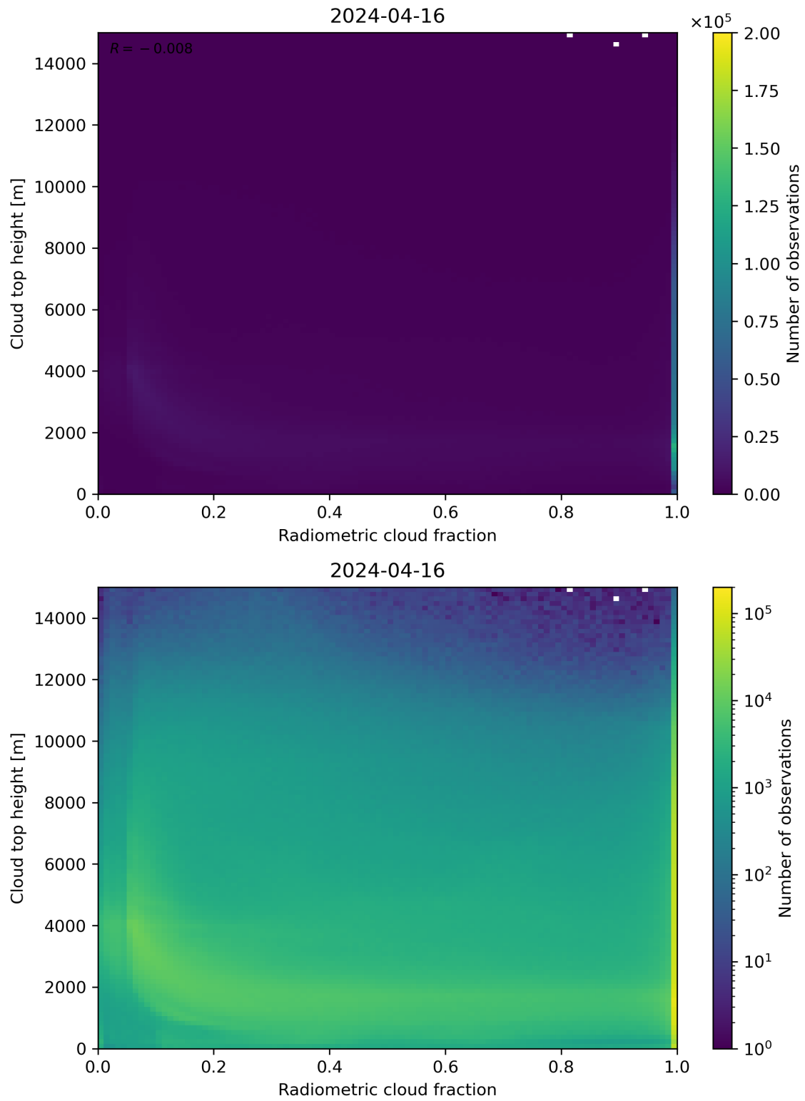
Figure 76: Scatter density plot of “Radiometric cloud fraction” against “Cloud top height” for 2024-04-16 to 2024-04-17.
