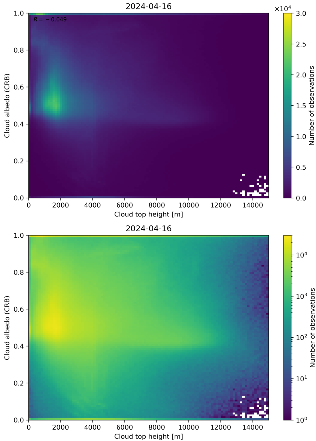
Figure 86: Scatter density plot of “Cloud top height” against “Cloud albedo (CRB)” for 2024-04-16 to 2024-04-17.
