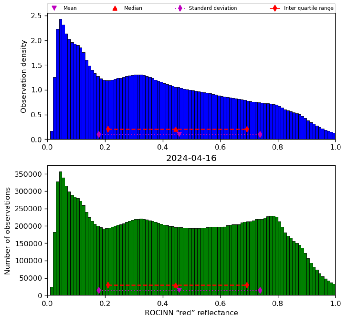
Figure 53: Histogram of “ROCINN “red” reflectance” for 2024-04-16 to 2024-04-17
