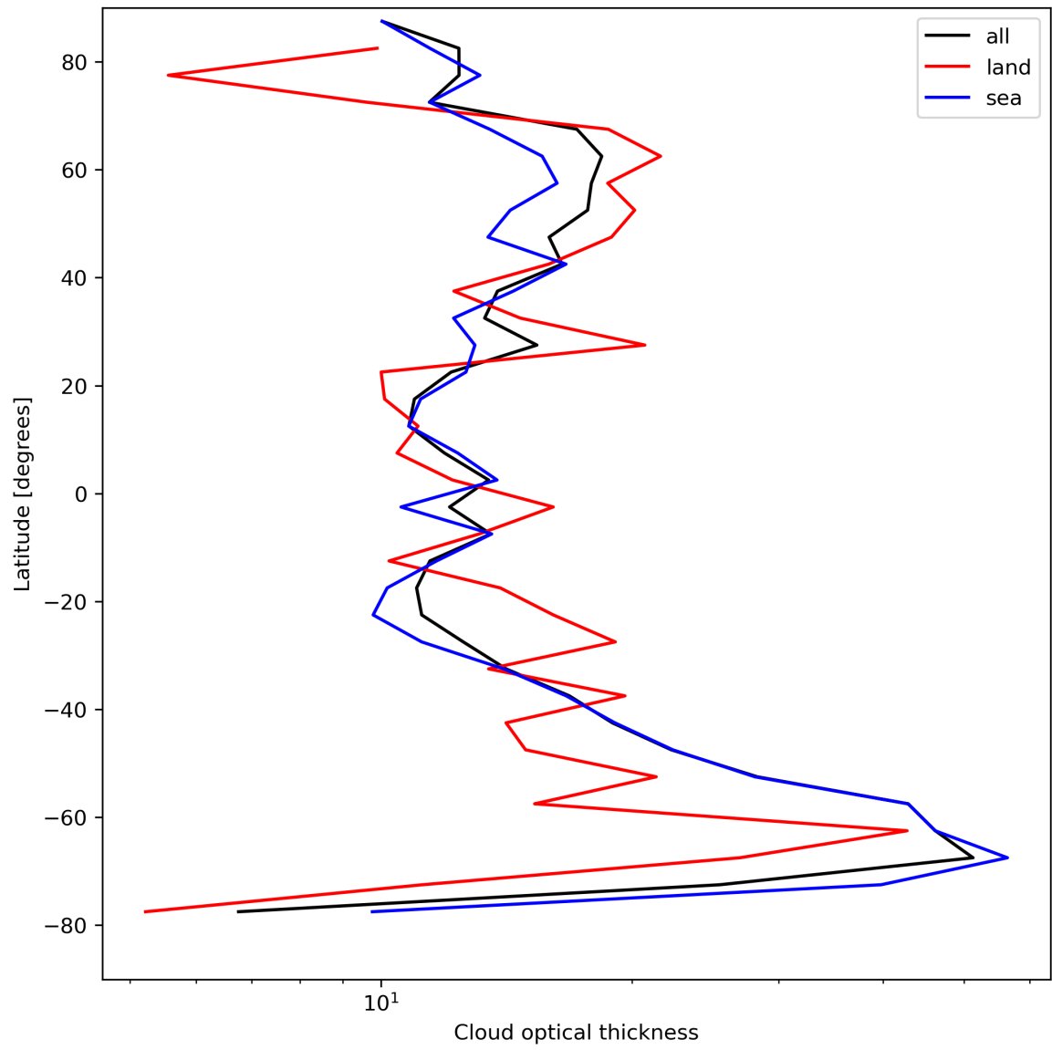
Figure 25: Zonal average of “Cloud optical thickness” for 2024-04-16 to 2024-04-17.
