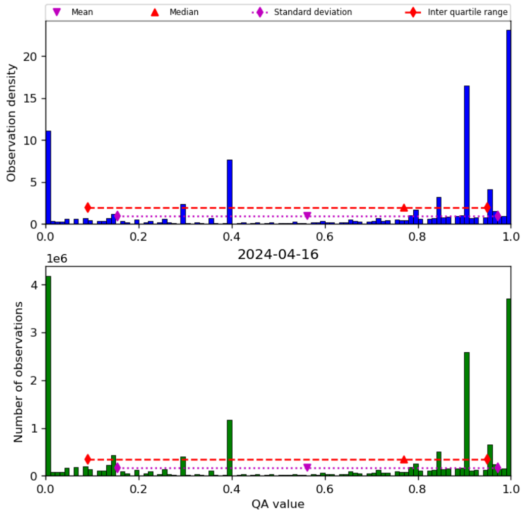
Figure 38: Histogram of “QA value” for 2024-04-16 to 2024-04-17
