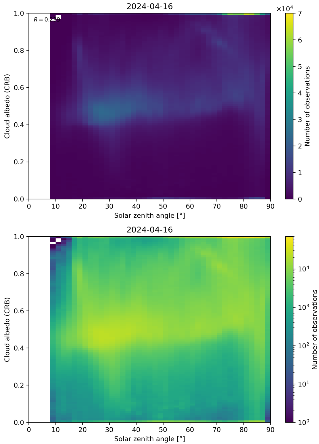
Figure 98: Scatter density plot of “Solar zenith angle” against “Cloud albedo (CRB)” for 2024-04-16 to 2024-04-17.
