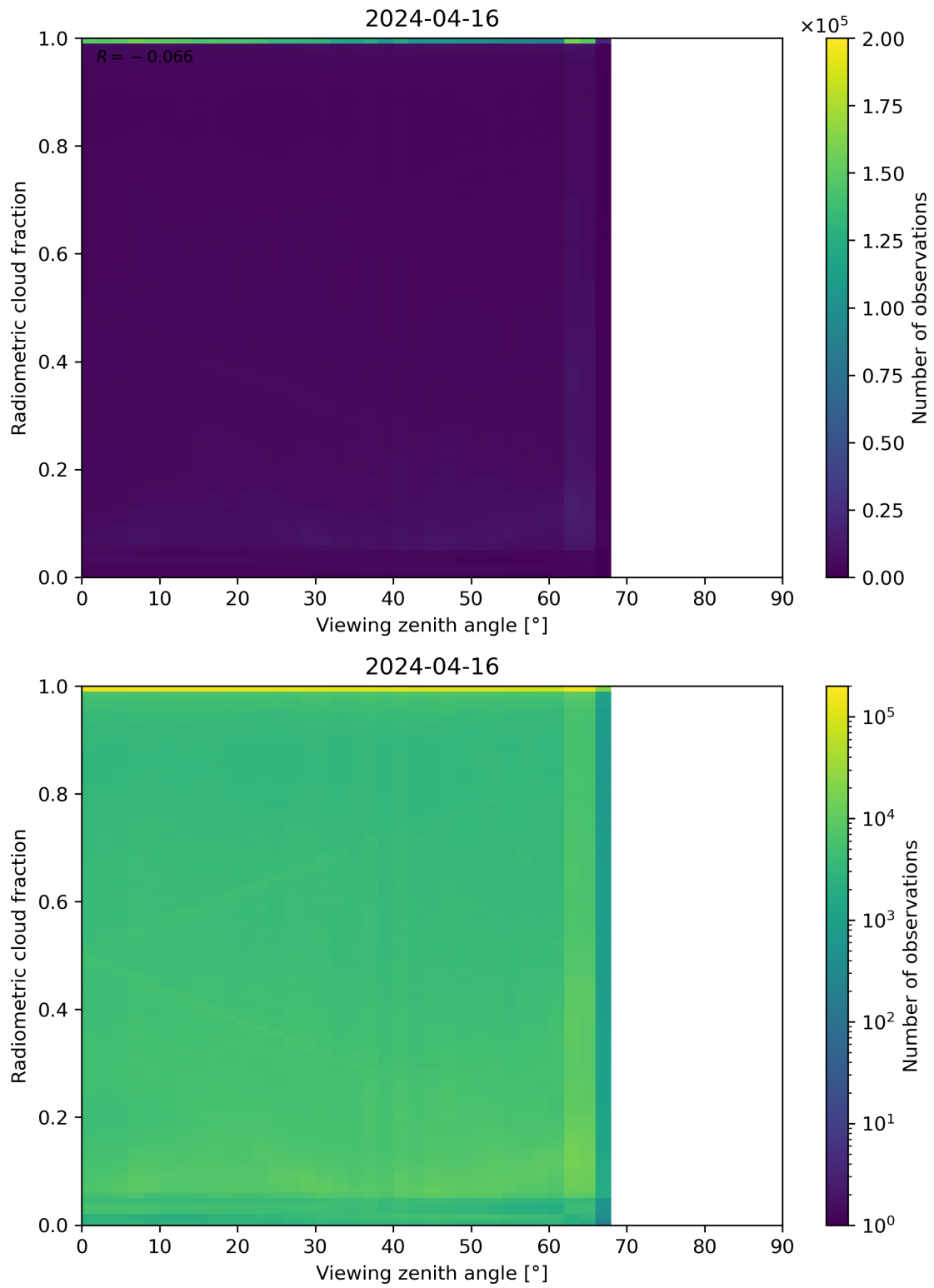
Figure 107: Scatter density plot of “Viewing zenith angle” against “Radiometric cloud fraction” for 2024-04-16 to 2024-04-17.
