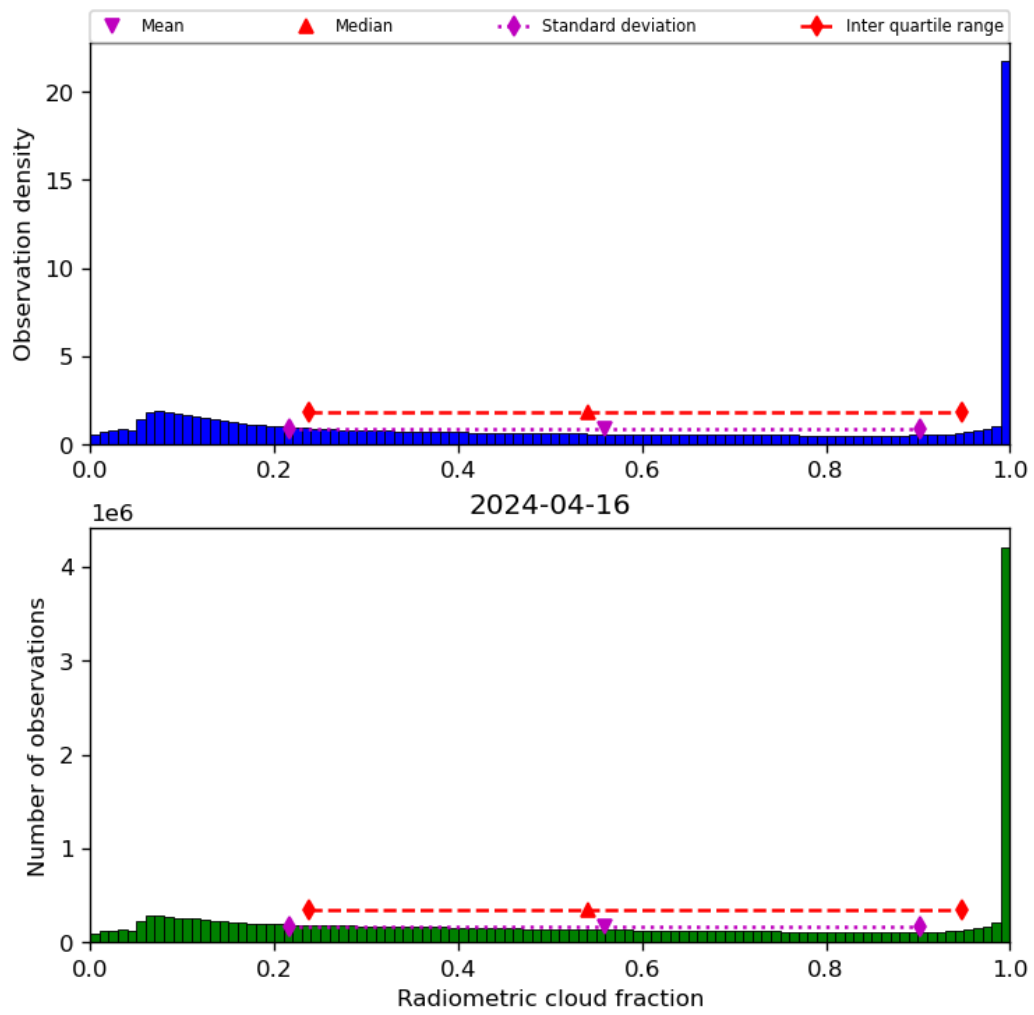
Figure 39: Histogram of “Radiometric cloud fraction” for 2024-04-16 to 2024-04-17
