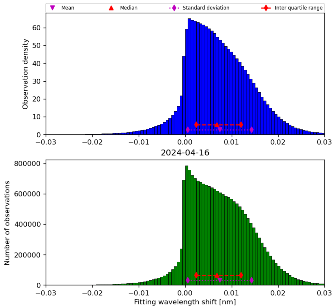
Figure 49: Histogram of “Fitting wavelength shift” for 2024-04-16 to 2024-04-17
