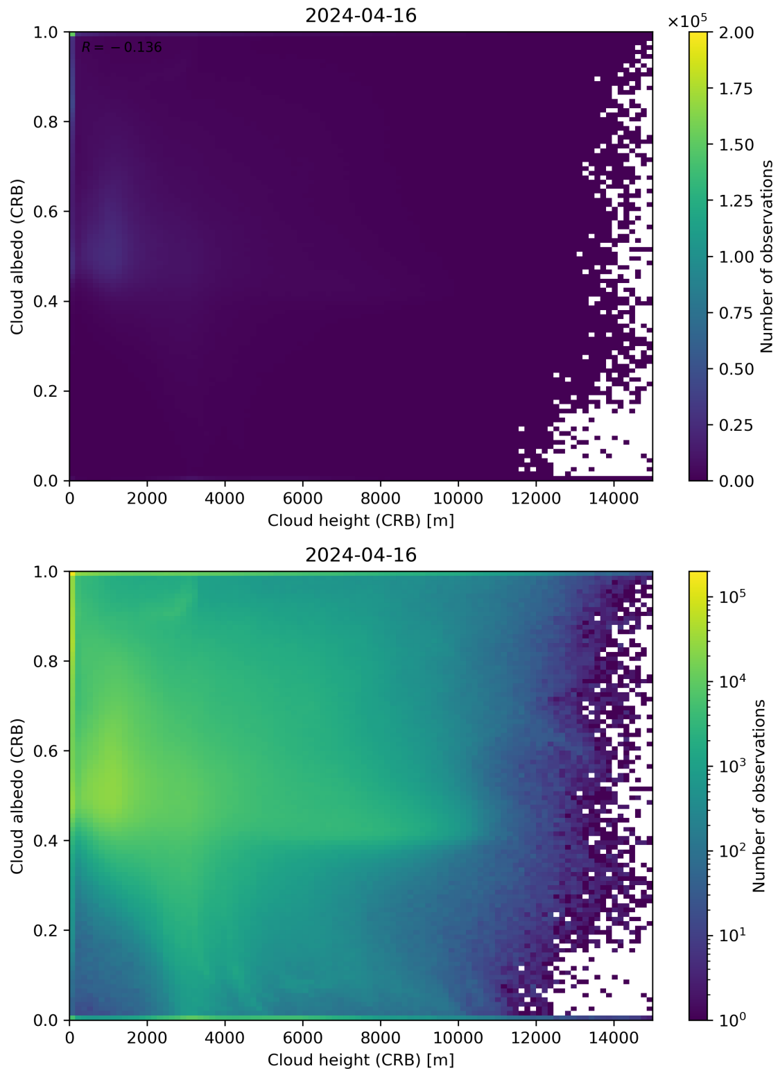
Figure 80: Scatter density plot of “Cloud height (CRB)” against “Cloud albedo (CRB)” for 2024-04-16 to 2024-04-17.
