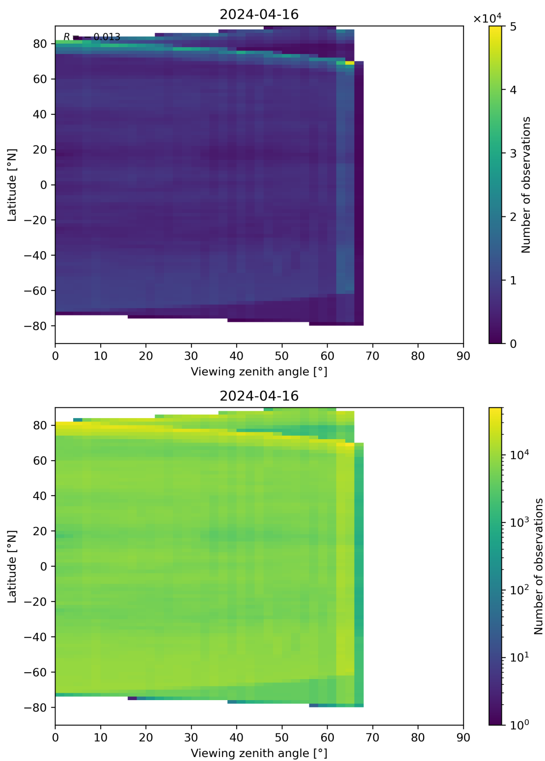
Figure 113: Scatter density plot of “Viewing zenith angle” against “Latitude” for 2024-04-16 to 2024-04-17.
