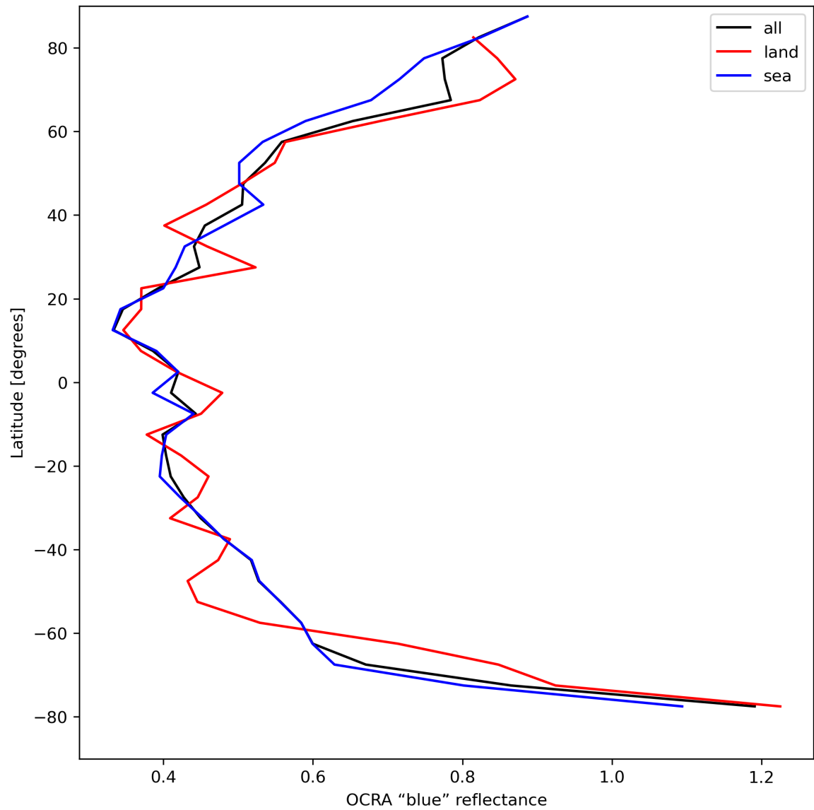
Figure 35: Zonal average of “OCRA “blue” reflectance” for 2024-04-16 to 2024-04-17.
