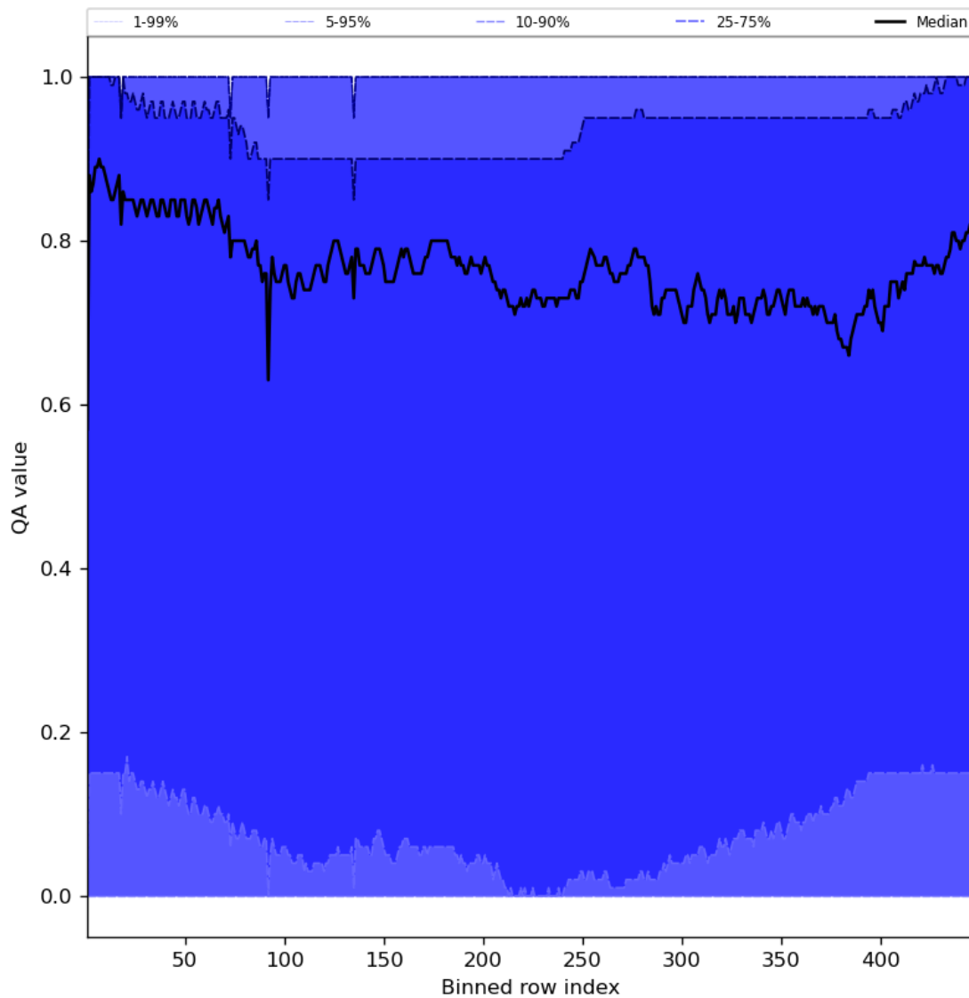
Figure 54: Along track statistics of “QA value” for 2024-04-16 to 2024-04-17
