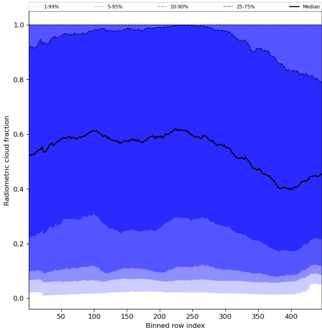
Figure 55: Along track statistics of “Radiometric cloud fraction” for 2024-04-16 to 2024-04-17
