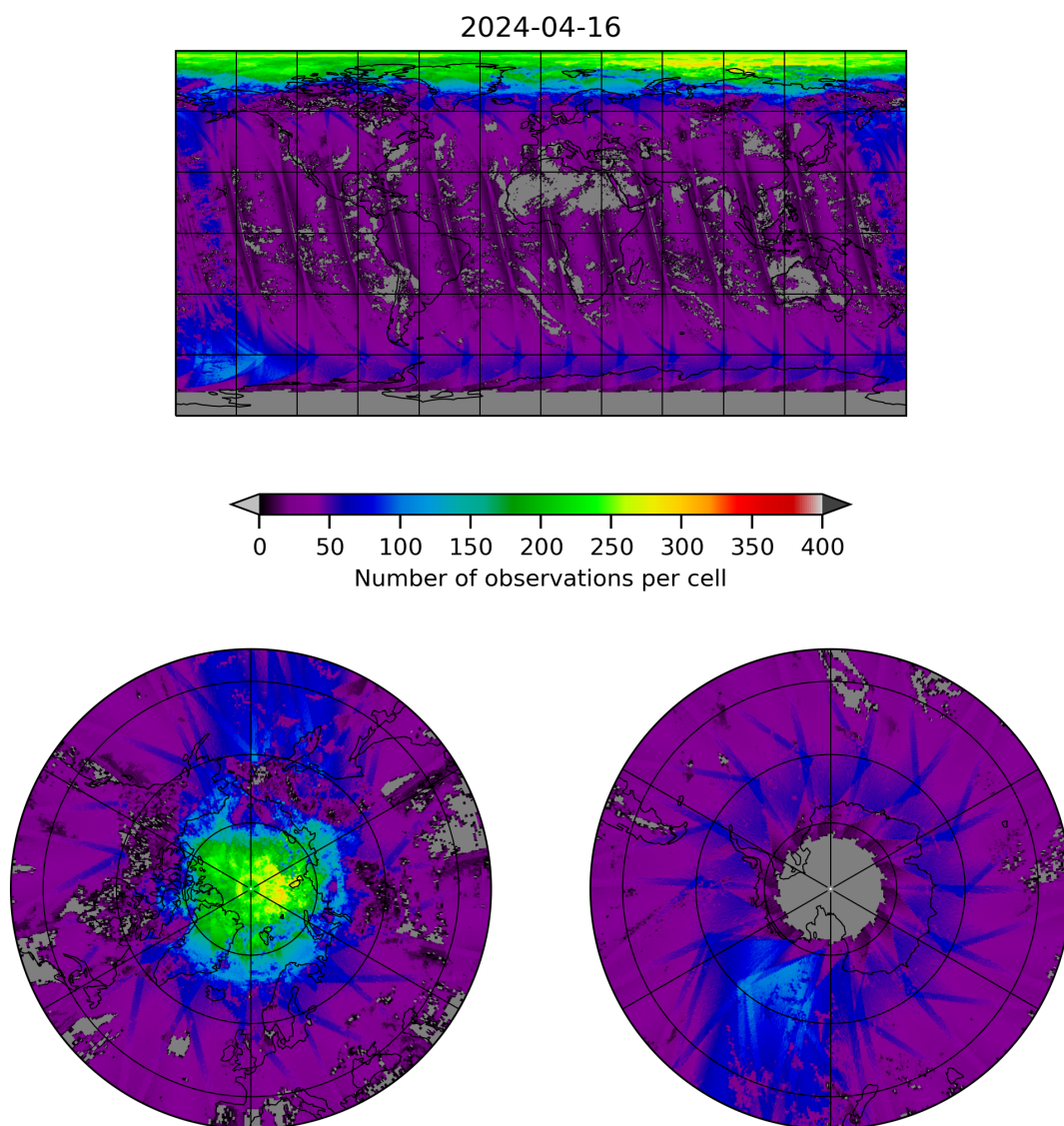
Figure 21: Map of the number of observations for 2024-04-16 to 2024-04-17
