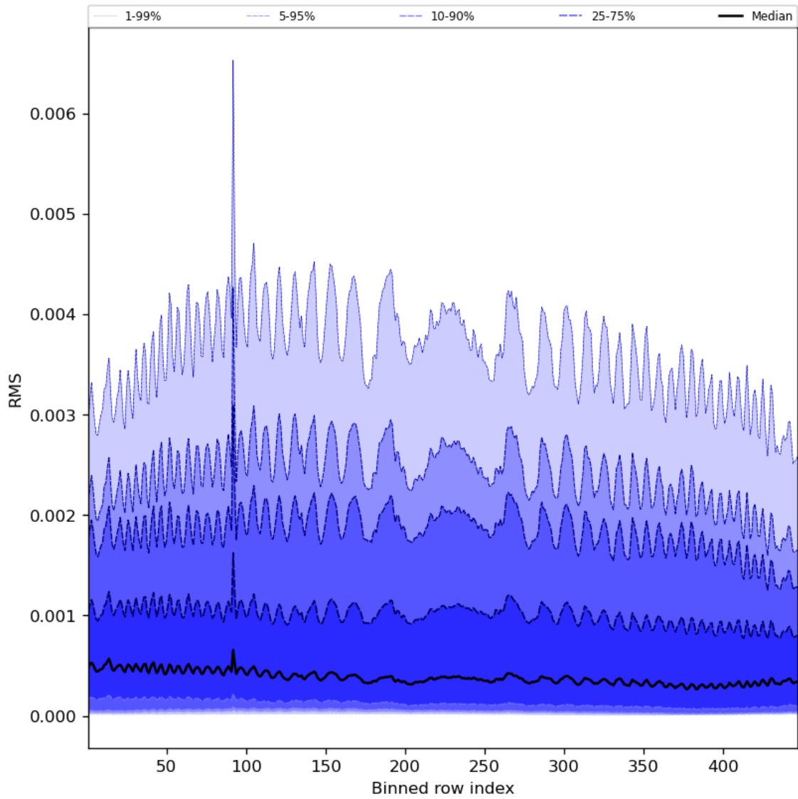
Figure 63: Along track statistics of “RMS” for 2024-04-16 to 2024-04-17
