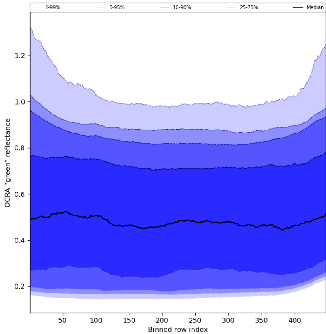
Figure 68: Along track statistics of “OCRA “green” reflectance” for 2024-04-16 to 2024-04-17
