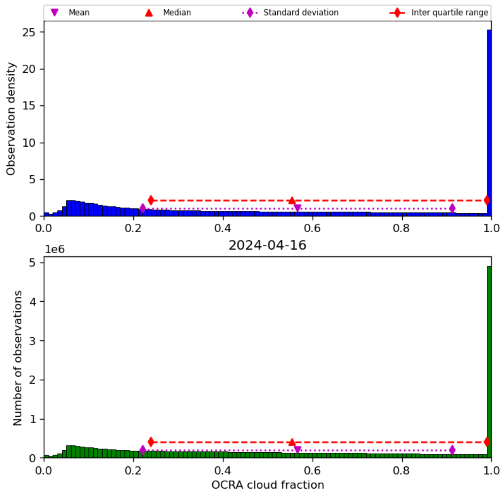
Figure 50: Histogram of “OCRA cloud fraction” for 2024-04-16 to 2024-04-17
