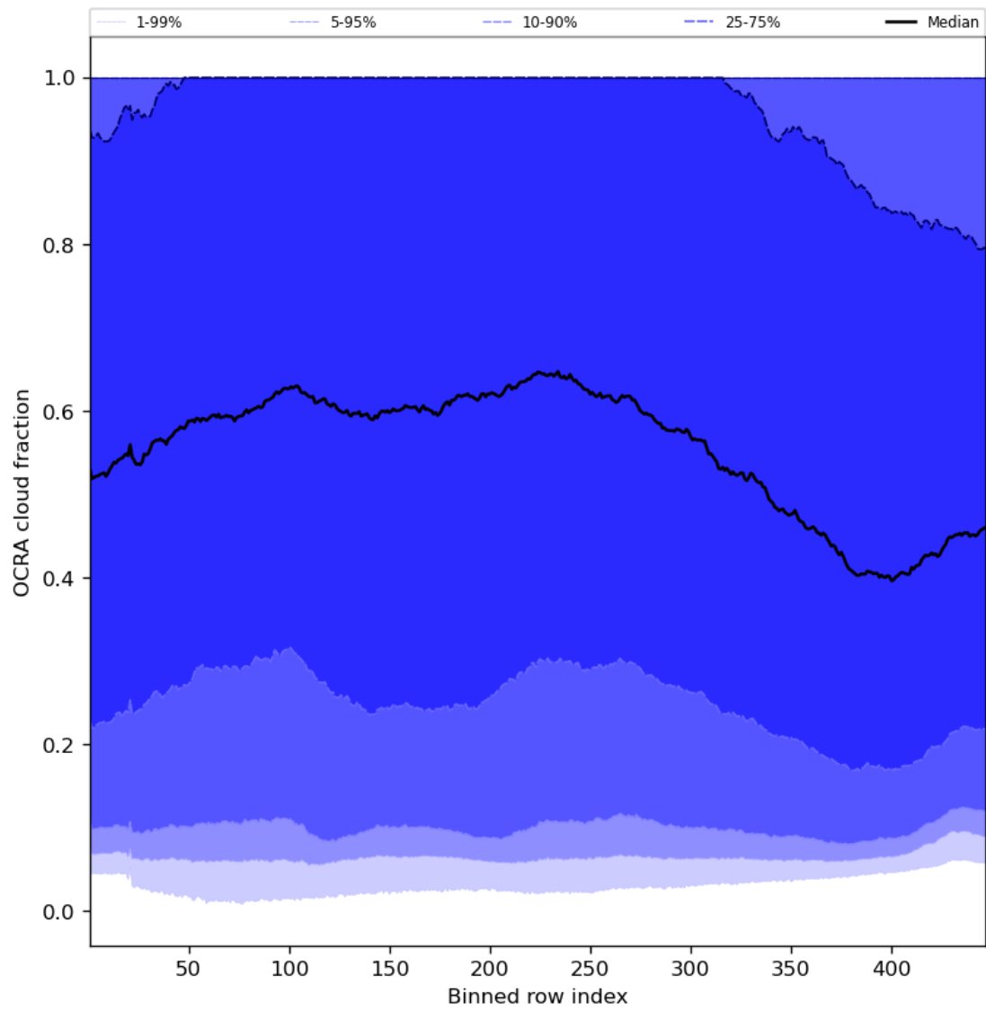
Figure 66: Along track statistics of “OCRA cloud fraction” for 2024-04-16 to 2024-04-17
