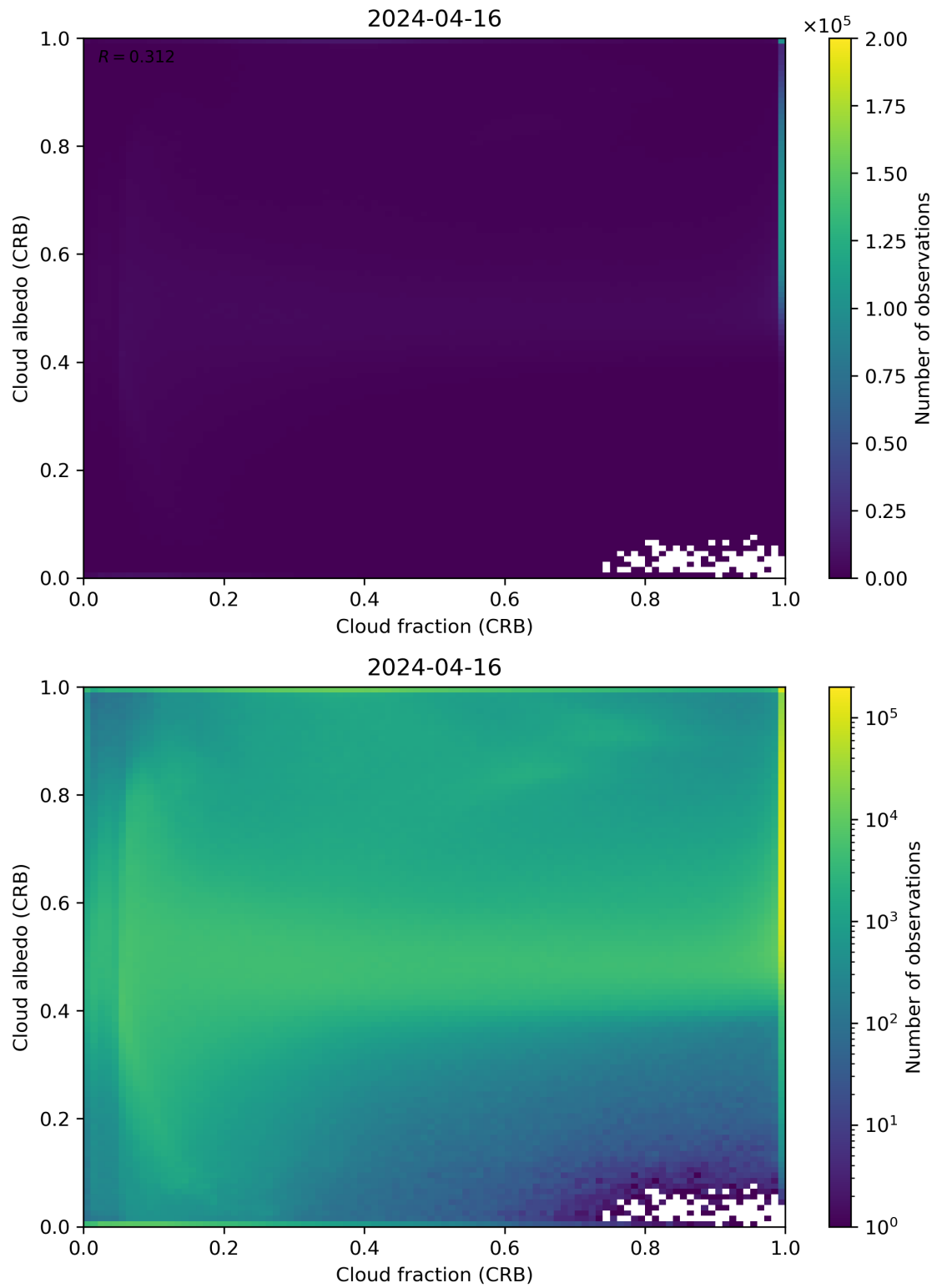
Figure 77: Scatter density plot of “Cloud fraction (CRB)” against “Cloud albedo (CRB)” for 2024-04-16 to 2024-04-17.
