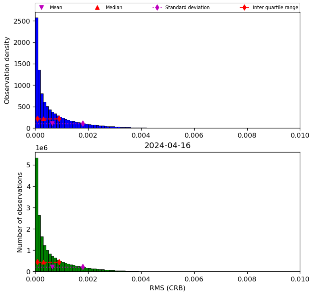
Figure 48: Histogram of “RMS (CRB)” for 2024-04-16 to 2024-04-17
