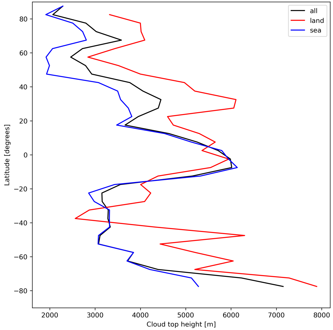
Figure 24: Zonal average of “Cloud top height” for 2024-04-16 to 2024-04-17.
