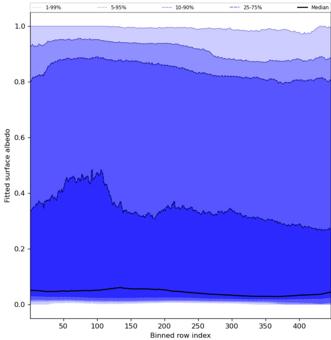
Figure 61: Along track statistics of “Fitted surface albedo” for 2024-04-16 to 2024-04-17
