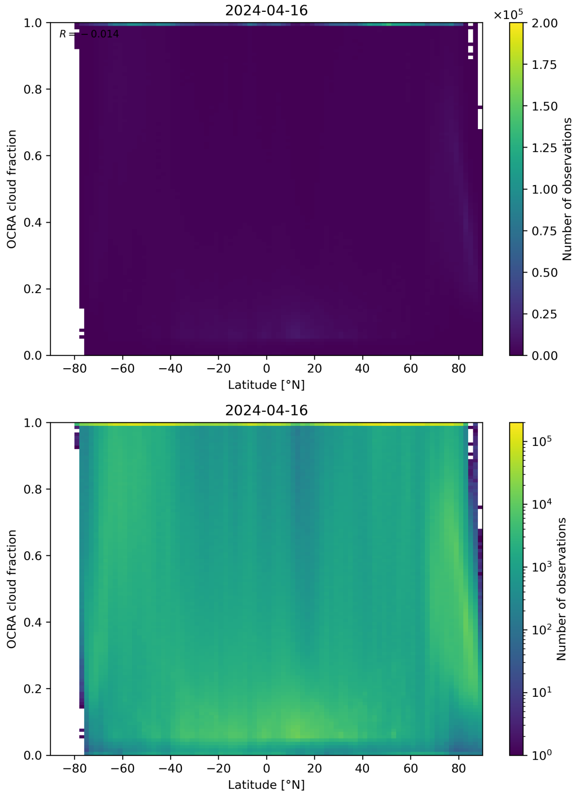
Figure 93: Scatter density plot of “Latitude” against “OCRA cloud fraction” for 2024-04-16 to 2024-04-17.
