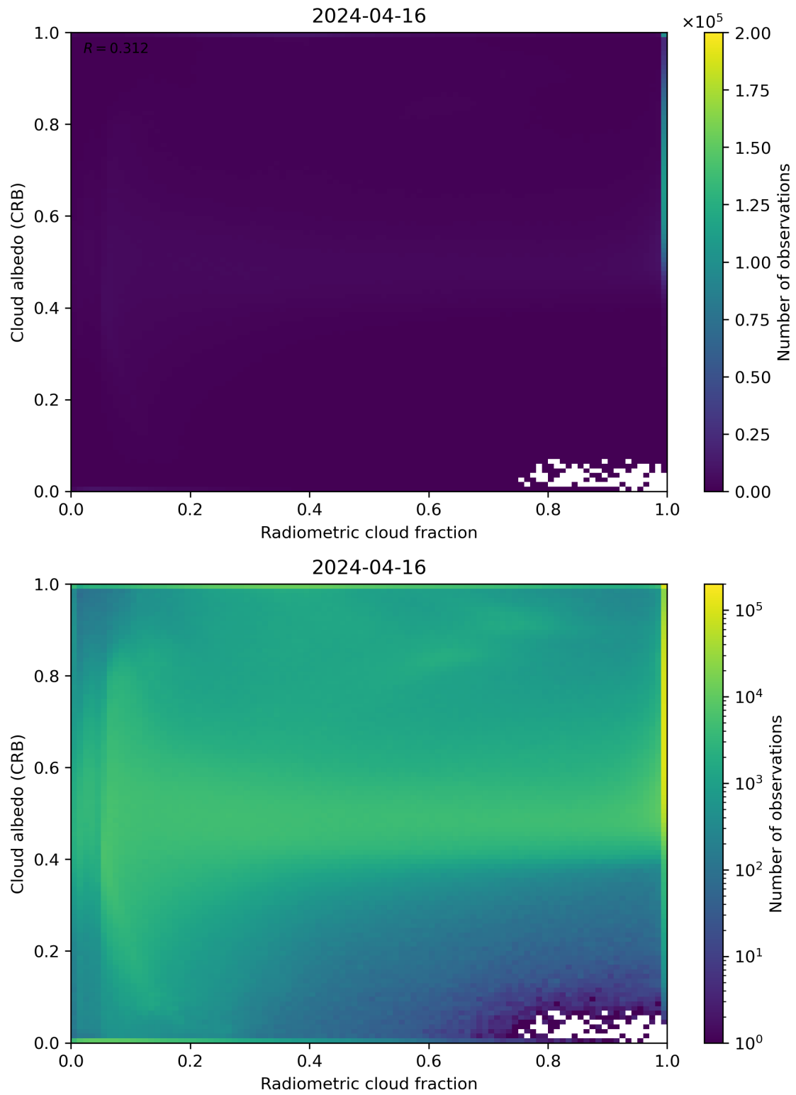
Figure 71: Scatter density plot of “Radiometric cloud fraction” against “Cloud albedo (CRB)” for 2024-04-16 to 2024-04-17.
