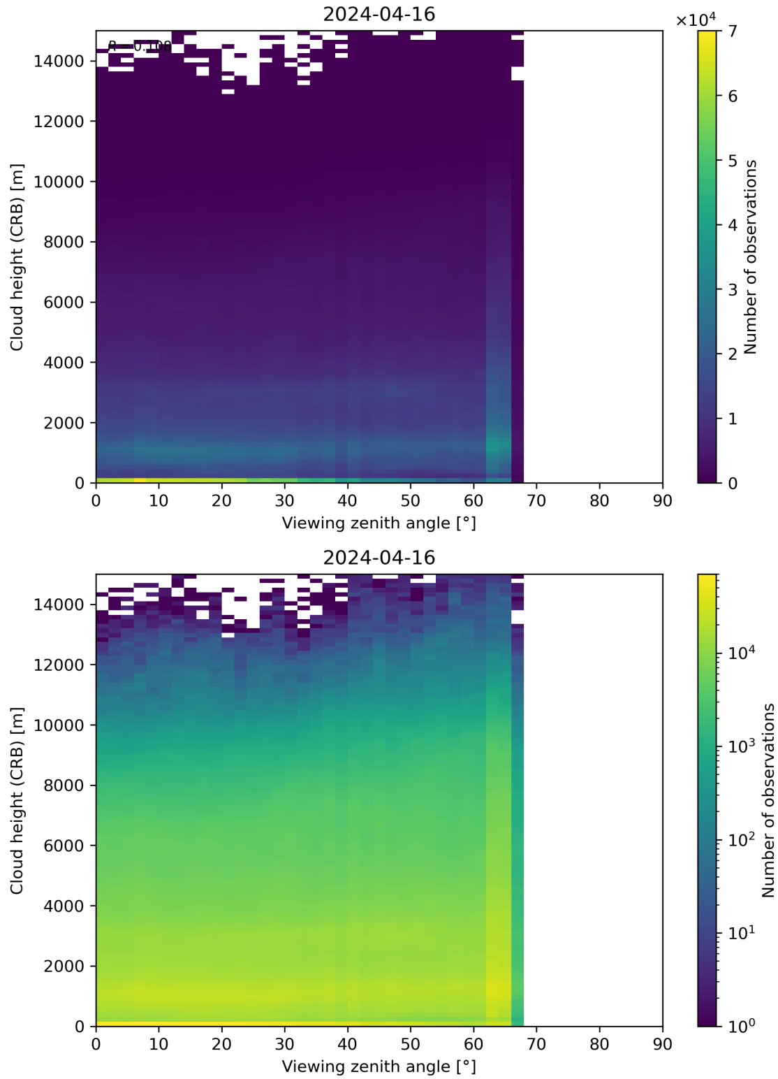
Figure 110: Scatter density plot of “Viewing zenith angle” against “Cloud height (CRB)” for 2024-04-16 to 2024-04-17.
