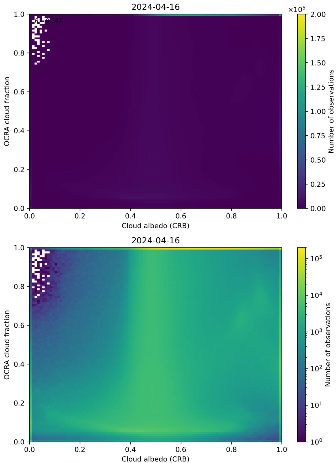
Figure 70: Scatter density plot of “Cloud albedo (CRB)” against “OCRA cloud fraction” for 2024-04-16 to 2024-04-17.
