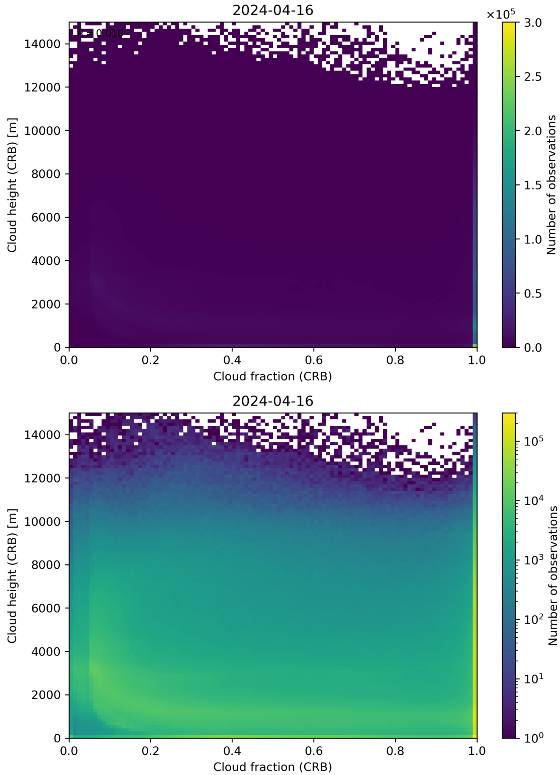
Figure 79: Scatter density plot of “Cloud fraction (CRB)” against “Cloud height (CRB)” for 2024-04-16 to 2024-04-17.
