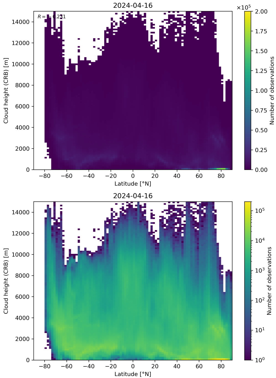
Figure 95: Scatter density plot of “Latitude” against “Cloud height (CRB)” for 2024-04-16 to 2024-04-17.
