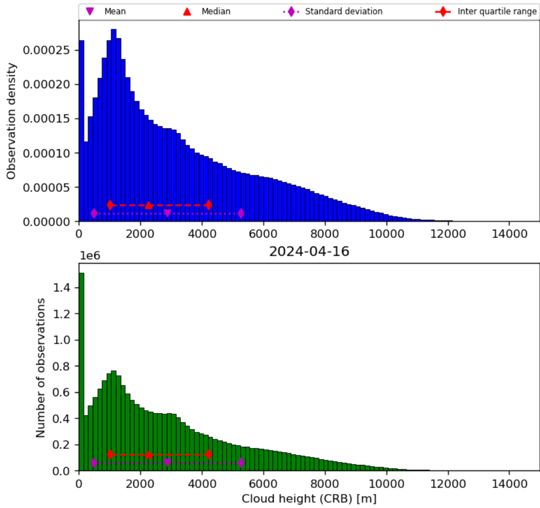
Figure 43: Histogram of “Cloud height (CRB)” for 2024-04-16 to 2024-04-17
