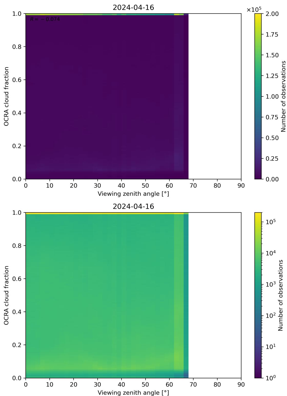
Figure 108: Scatter density plot of “Viewing zenith angle” against “OCRA cloud fraction” for 2024-04-16 to 2024-04-17.
