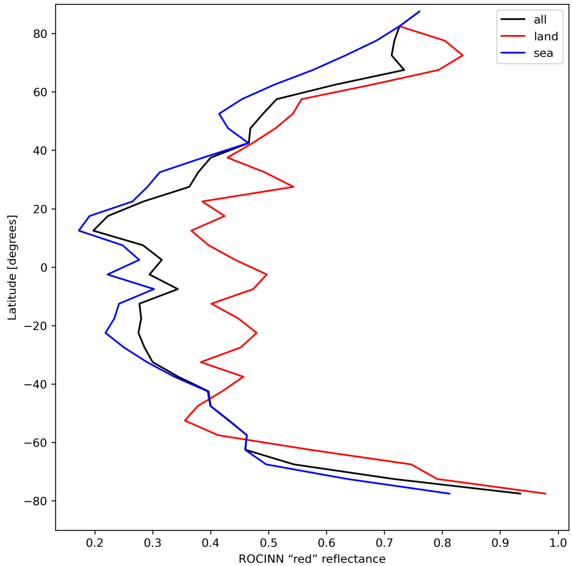
Figure 37: Zonal average of “ROCINN “red” reflectance” for 2024-04-16 to 2024-04-17.
