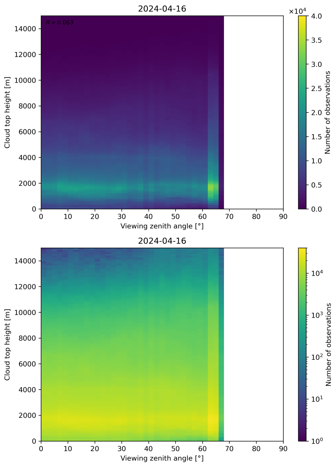
Figure 112: Scatter density plot of “Viewing zenith angle” against “Cloud top height” for 2024-04-16 to 2024-04-17.
