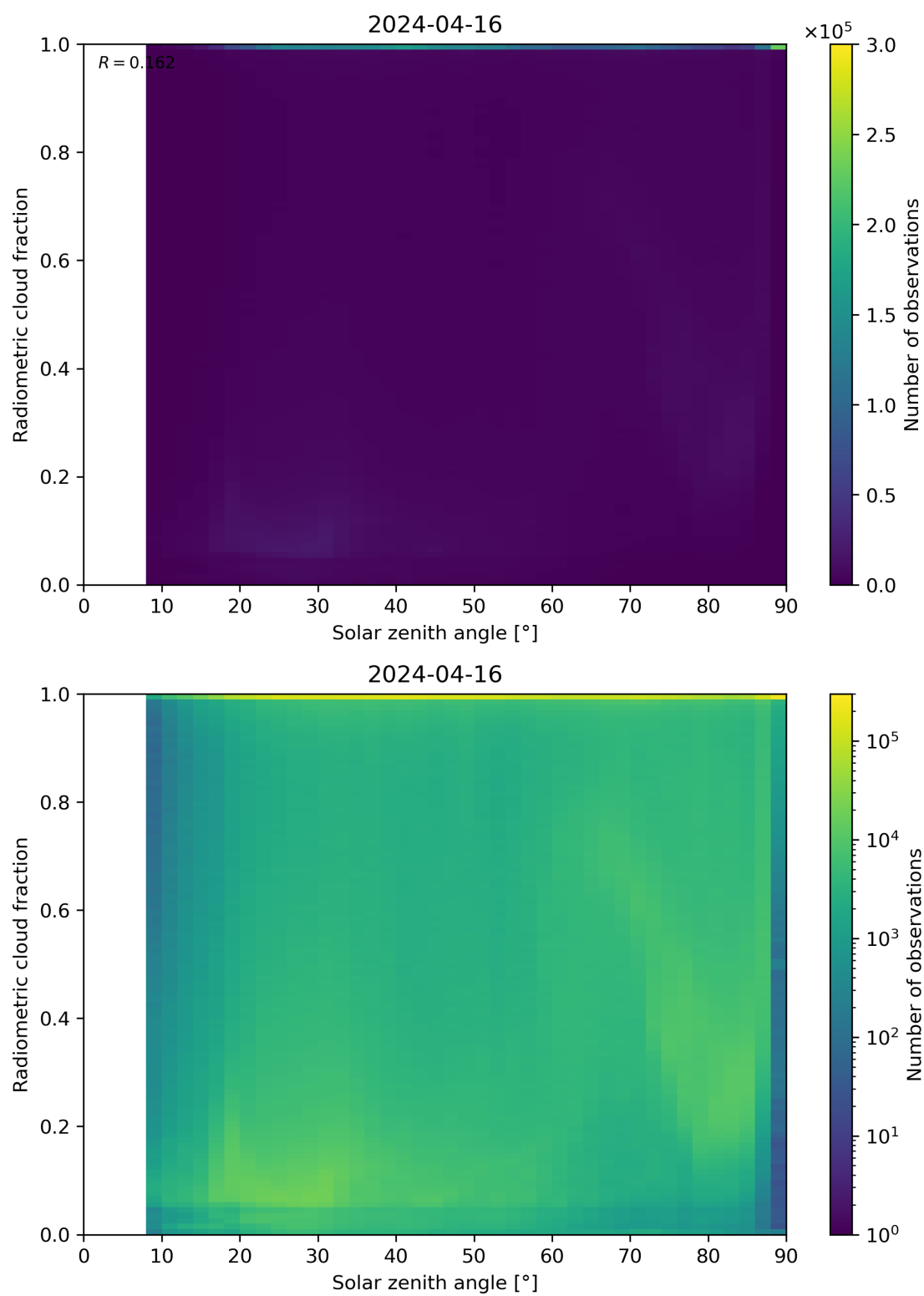
Figure 99: Scatter density plot of “Solar zenith angle” against “Radiometric cloud fraction” for 2024-04-16 to 2024-04-17.
