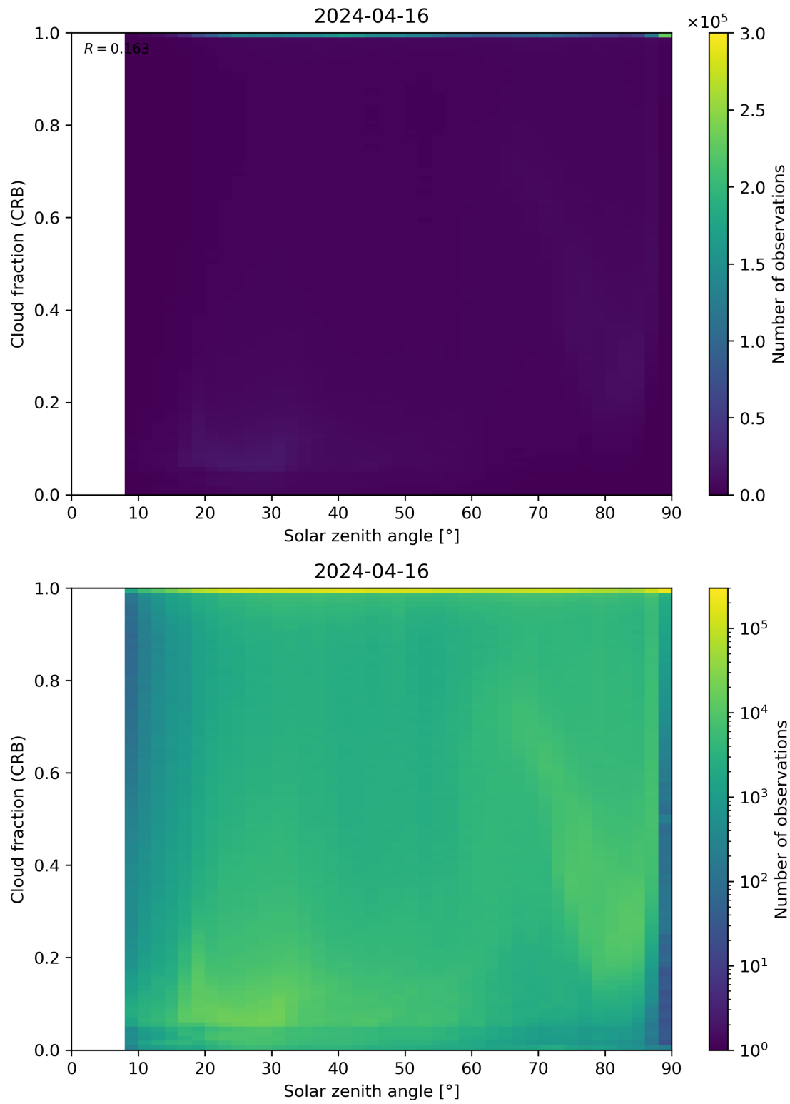
Figure 101: Scatter density plot of “Solar zenith angle” against “Cloud fraction (CRB)” for 2024-04-16 to 2024-04-17.
