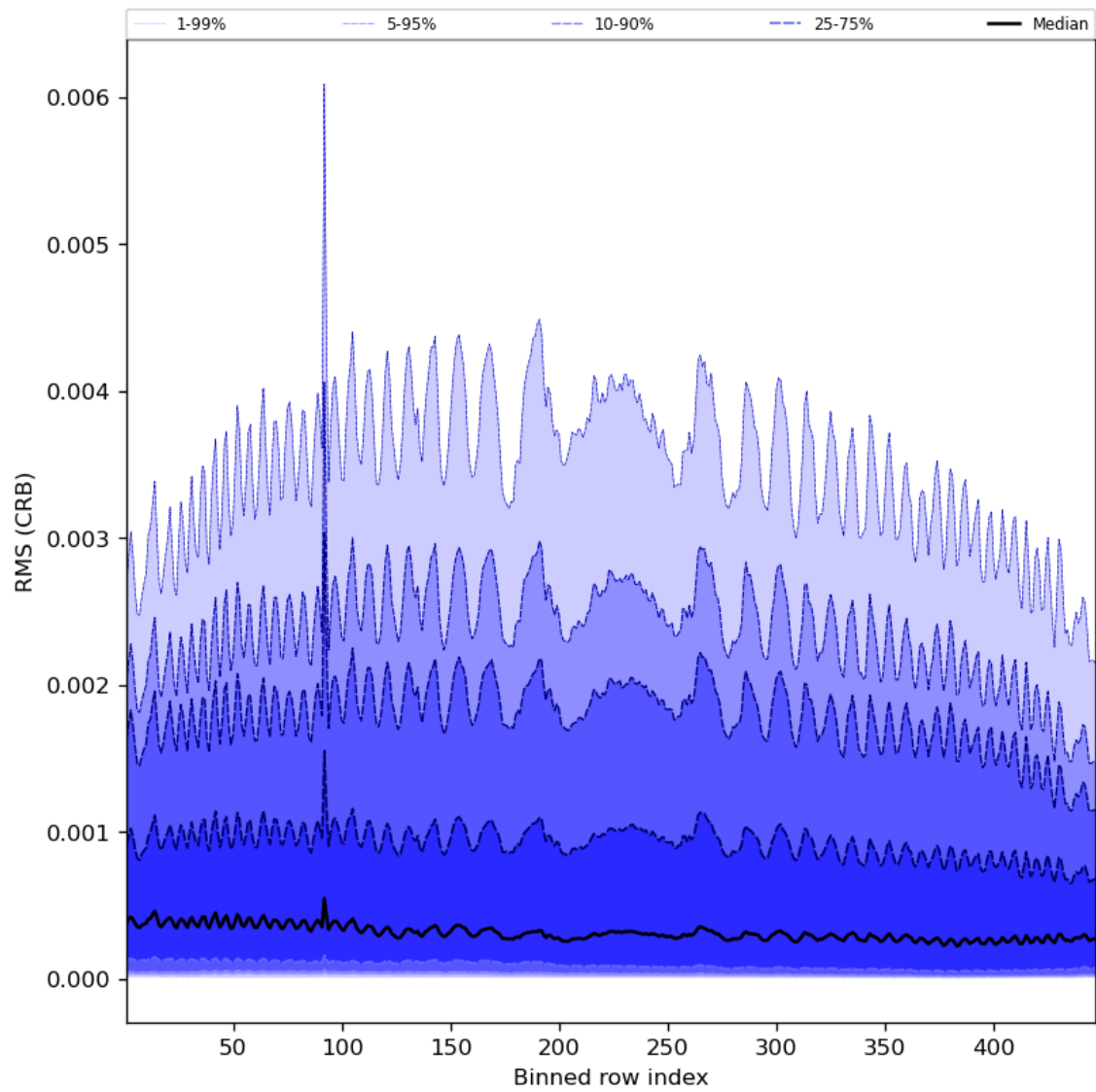
Figure 64: Along track statistics of “RMS (CRB)” for 2024-04-16 to 2024-04-17
