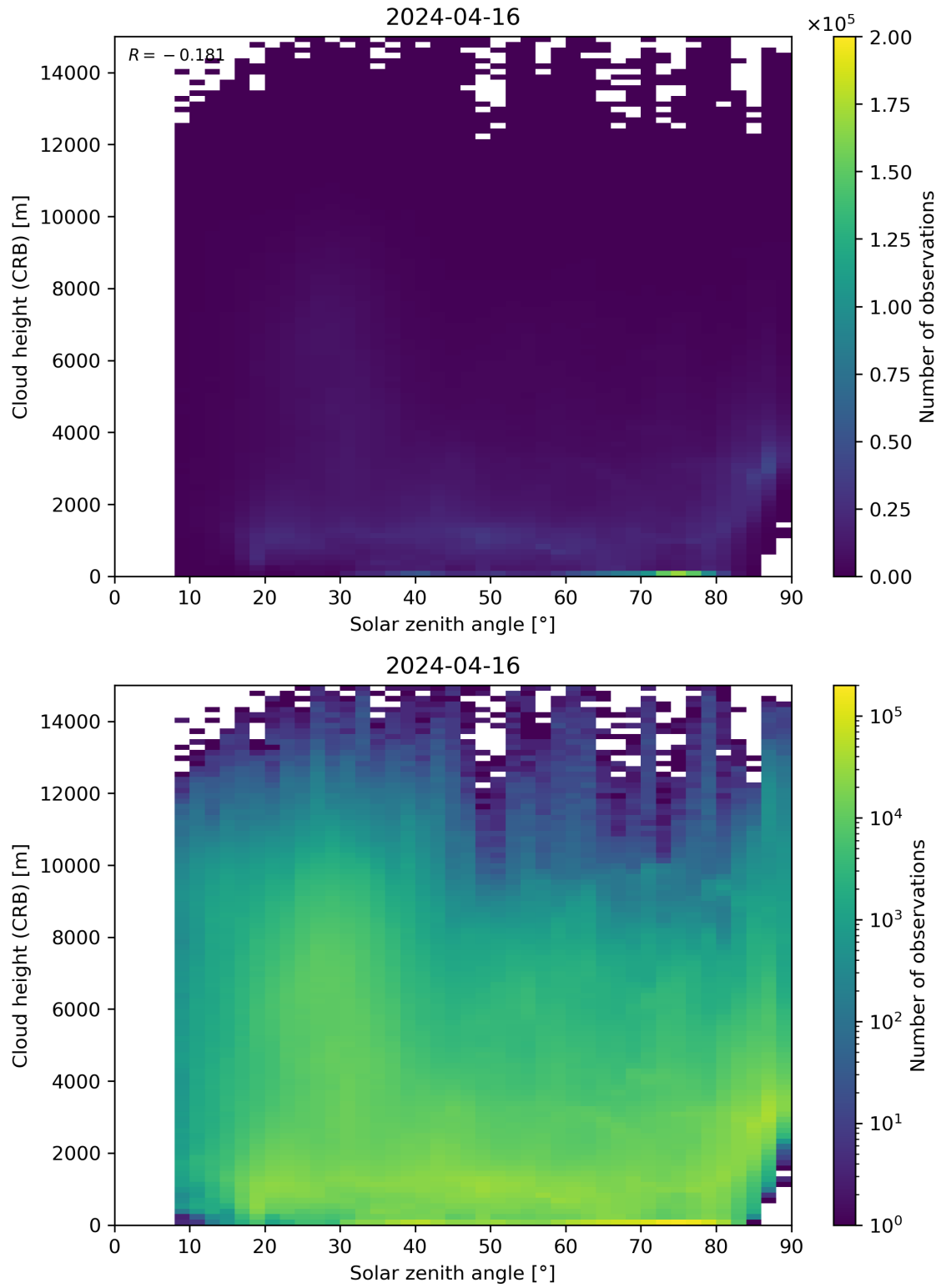
Figure 102: Scatter density plot of “Solar zenith angle” against “Cloud height (CRB)” for 2024-04-16 to 2024-04-17.
