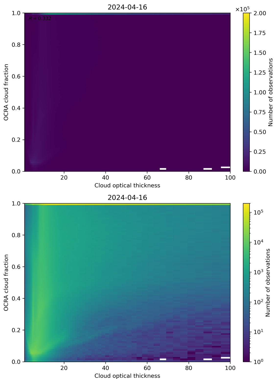
Figure 83: Scatter density plot of “Cloud optical thickness” against “OCRA cloud fraction” for 2024-04-16 to 2024-04-17.
