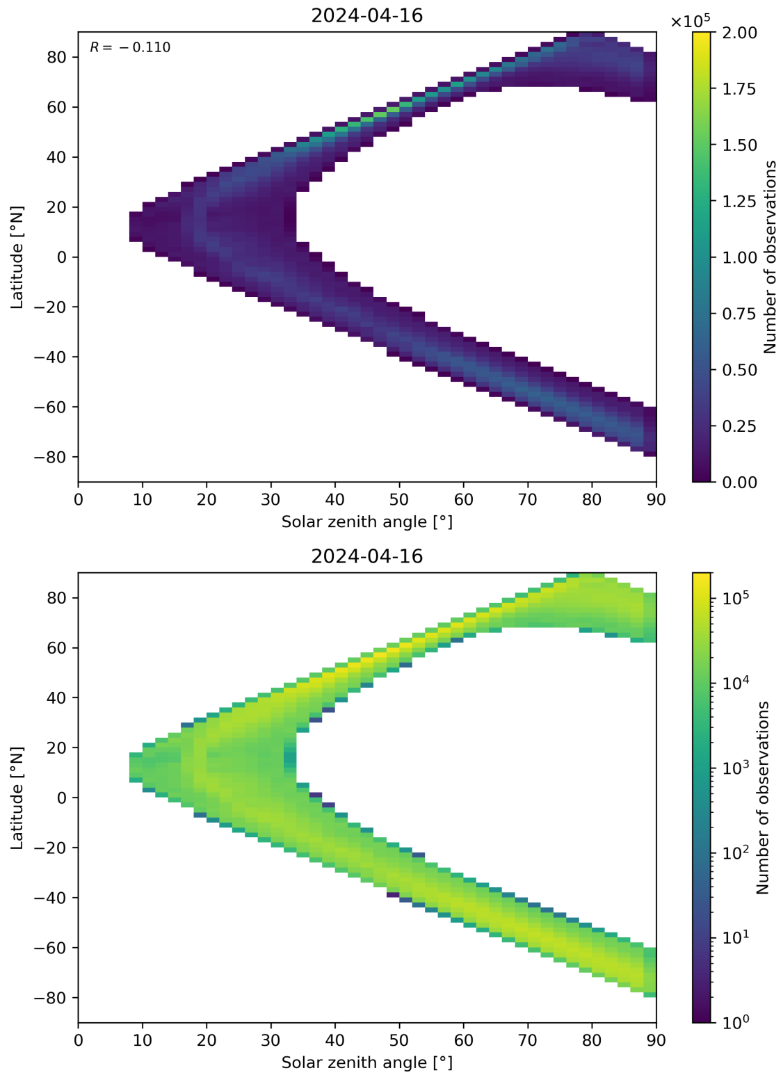
Figure 105: Scatter density plot of “Solar zenith angle” against “Latitude” for 2024-04-16 to 2024-04-17.
