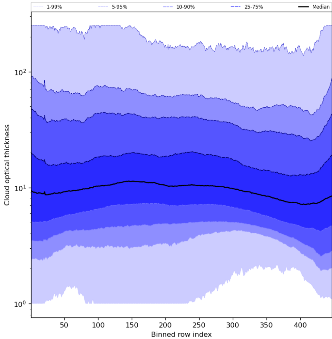
Figure 57: Along track statistics of “Cloud optical thickness” for 2024-04-16 to 2024-04-17
