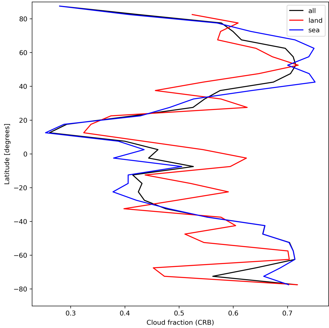
Figure 26: Zonal average of “Cloud fraction (CRB)” for 2024-04-16 to 2024-04-17.
