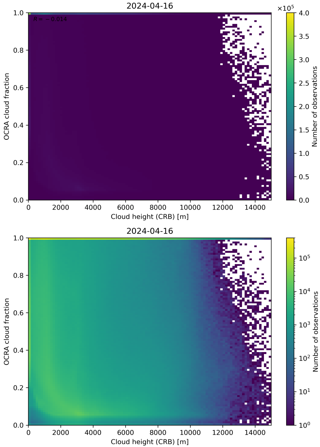
Figure 81: Scatter density plot of “Cloud height (CRB)” against “OCRA cloud fraction” for 2024-04-16 to 2024-04-17.
