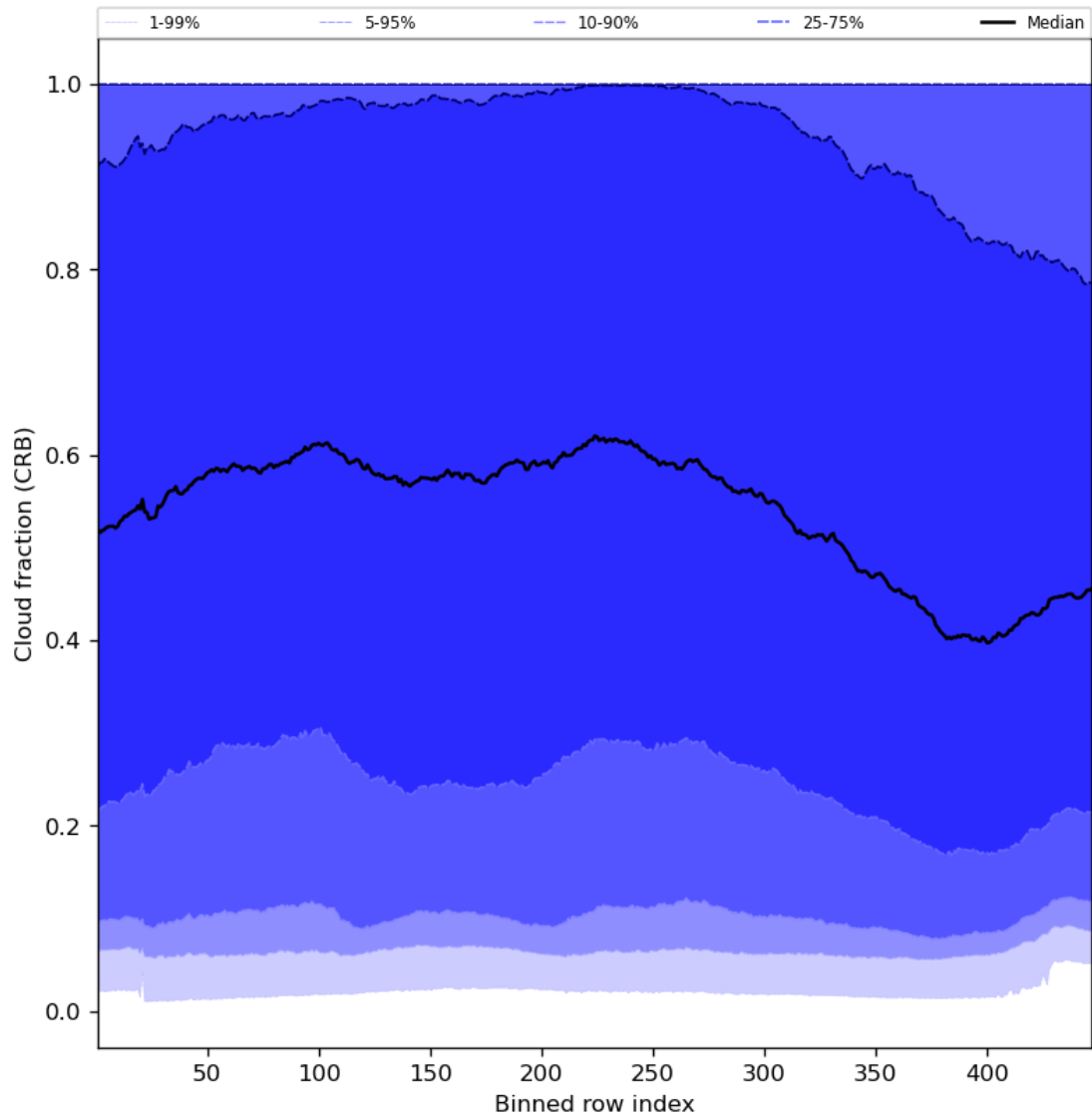
Figure 58: Along track statistics of “Cloud fraction (CRB)” for 2024-04-16 to 2024-04-17
