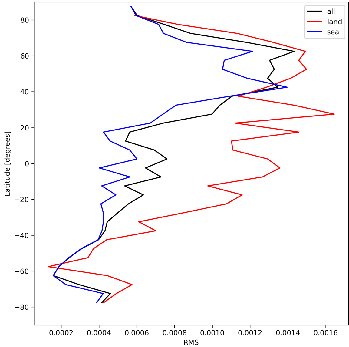
Figure 31: Zonal average of “RMS” for 2024-04-16 to 2024-04-17.
