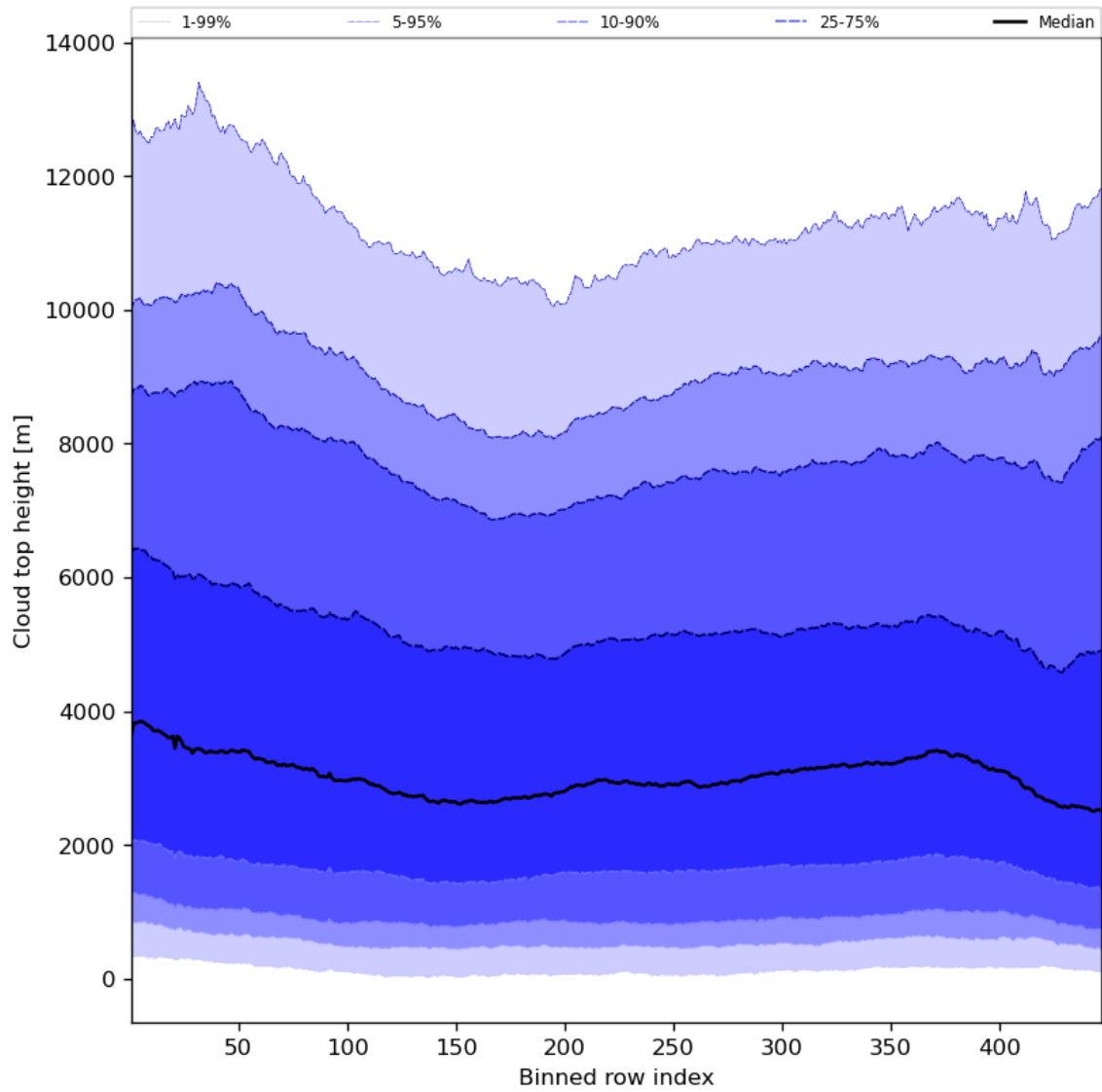
Figure 56: Along track statistics of “Cloud top height” for 2024-04-16 to 2024-04-17
