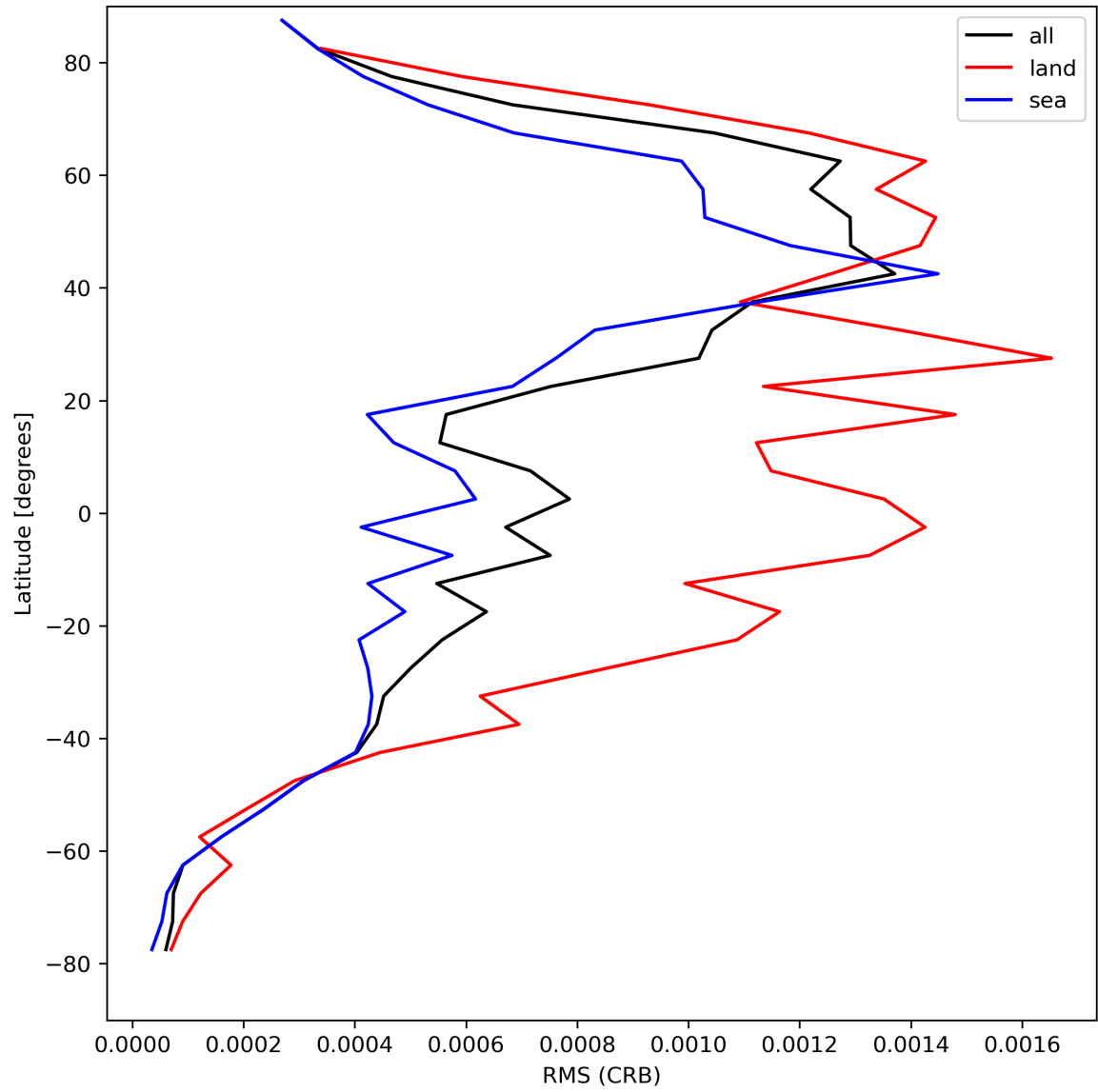
Figure 32: Zonal average of “RMS (CRB)” for 2024-04-16 to 2024-04-17.
