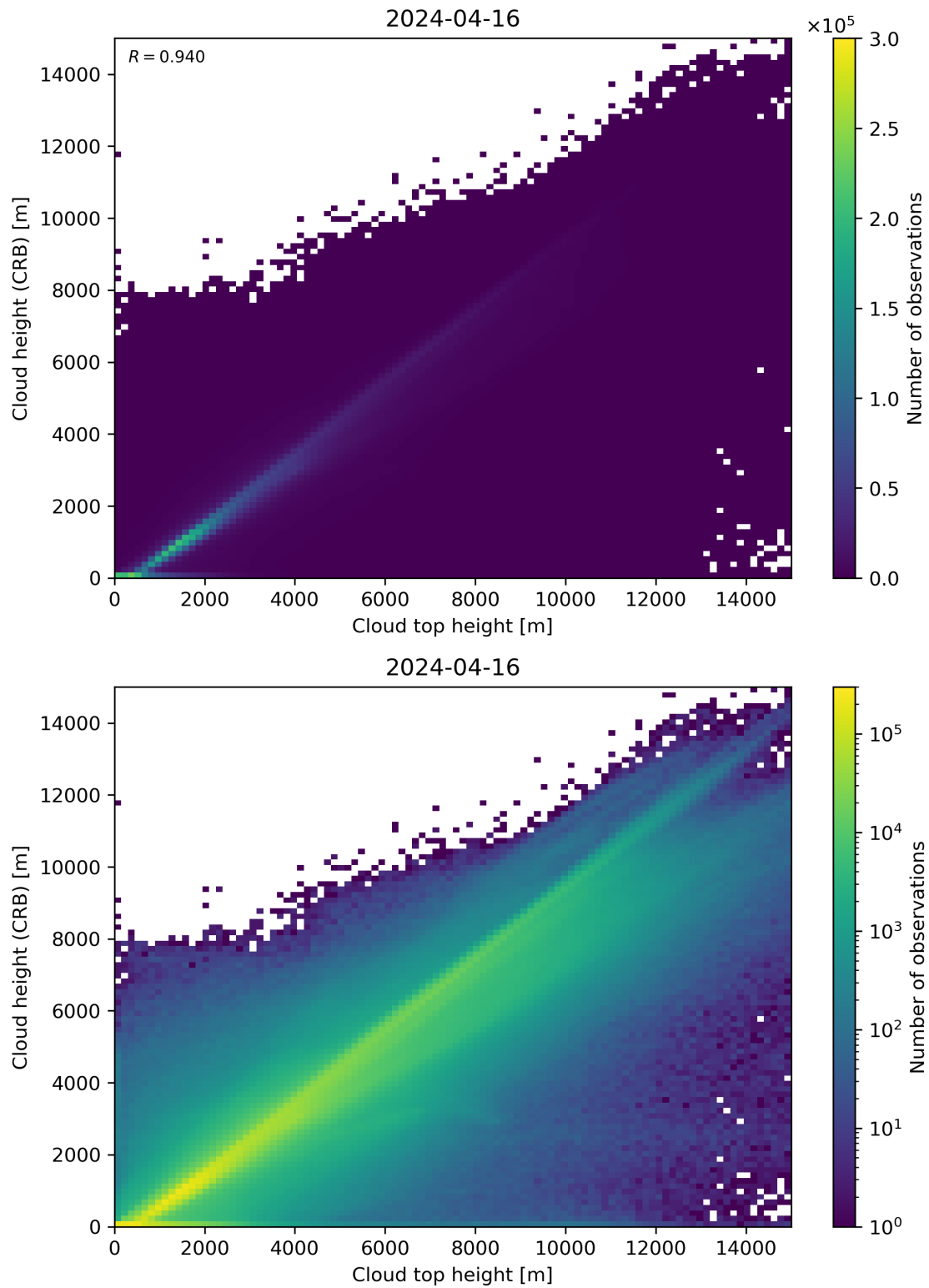
Figure 89: Scatter density plot of “Cloud top height” against “Cloud height (CRB)” for 2024-04-16 to 2024-04-17.
