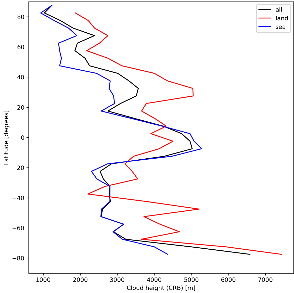
Figure 27: Zonal average of “Cloud height (CRB)” for 2024-04-16 to 2024-04-17.
