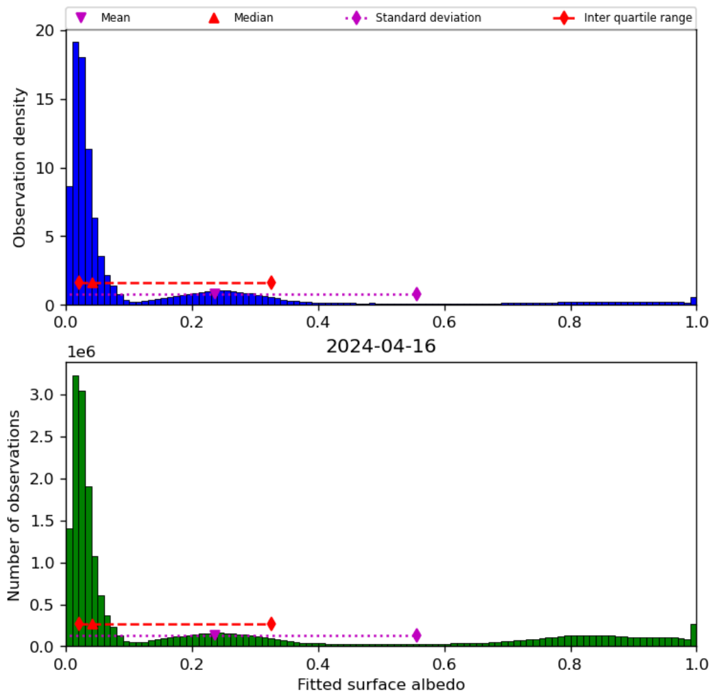
Figure 45: Histogram of “Fitted surface albedo” for 2024-04-16 to 2024-04-17
