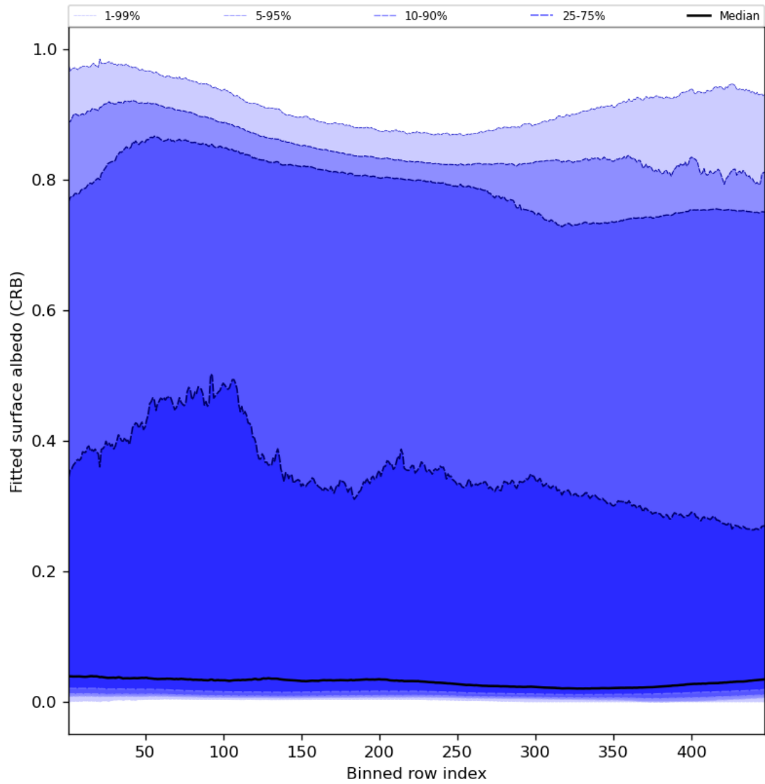
Figure 62: Along track statistics of “Fitted surface albedo (CRB)” for 2024-04-16 to 2024-04-17
