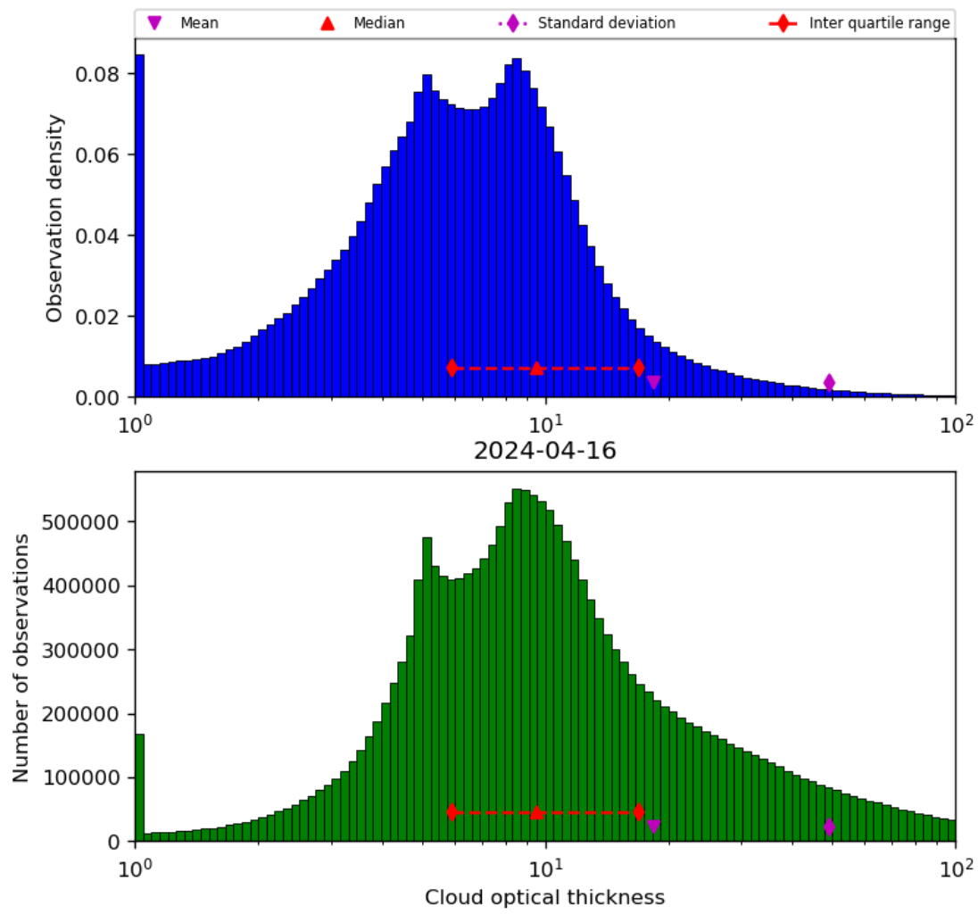
Figure 41: Histogram of “Cloud optical thickness” for 2024-04-16 to 2024-04-17
