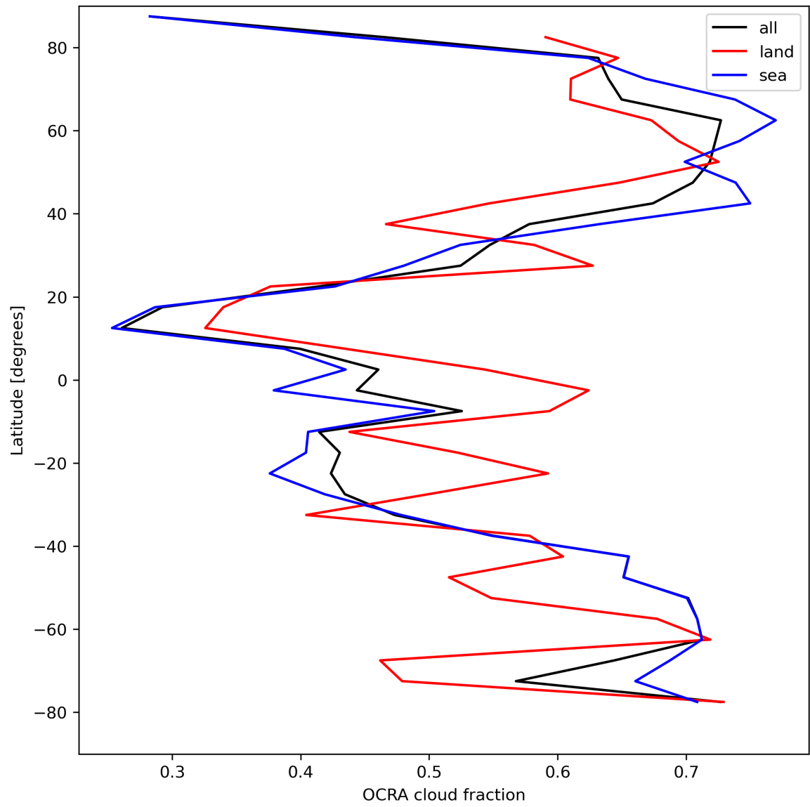
Figure 34: Zonal average of “OCRA cloud fraction” for 2024-04-16 to 2024-04-17.
