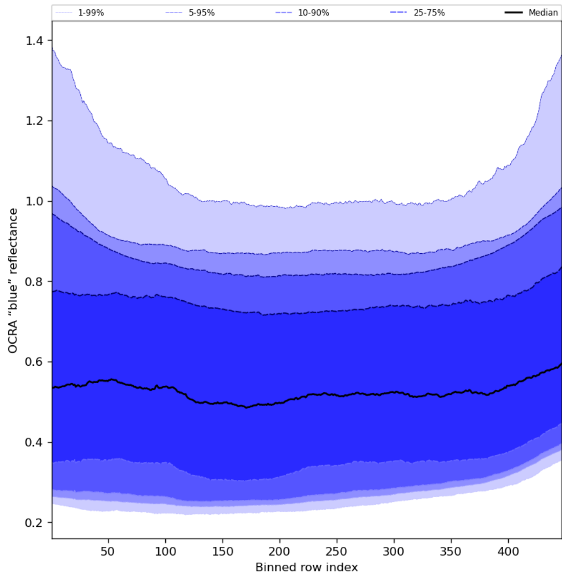
Figure 67: Along track statistics of “OCRA “blue” reflectance” for 2024-04-16 to 2024-04-17
