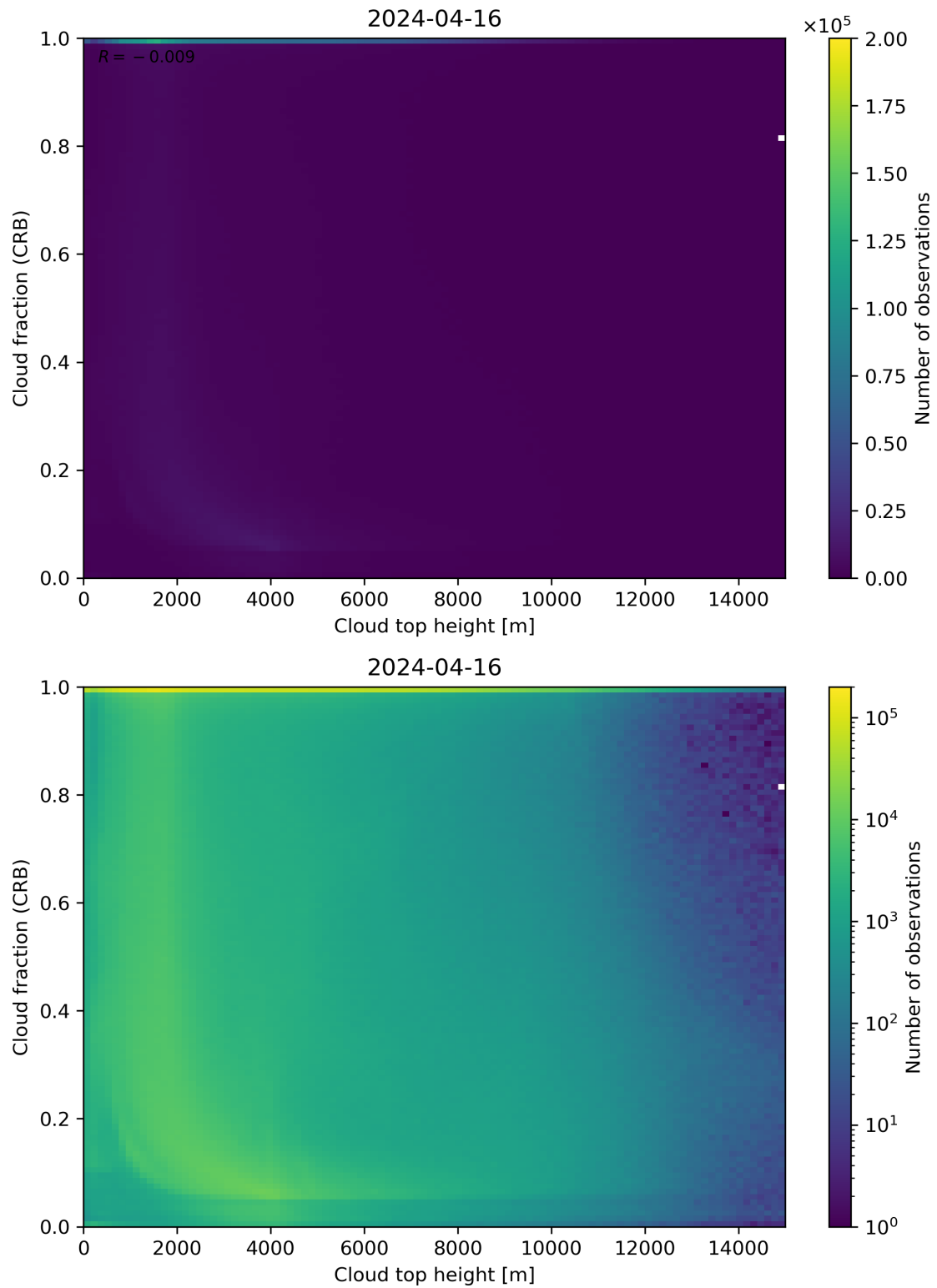
Figure 88: Scatter density plot of “Cloud top height” against “Cloud fraction (CRB)” for 2024-04-16 to 2024-04-17.
