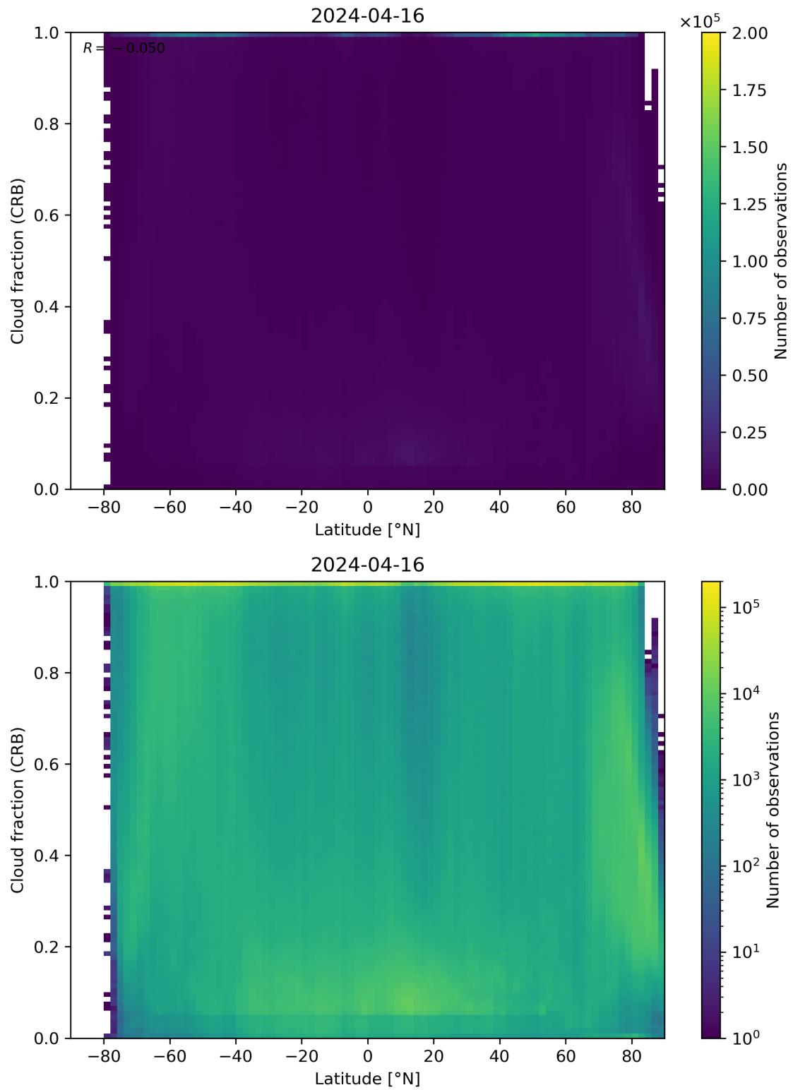
Figure 94: Scatter density plot of “Latitude” against “Cloud fraction (CRB)” for 2024-04-16 to 2024-04-17.
