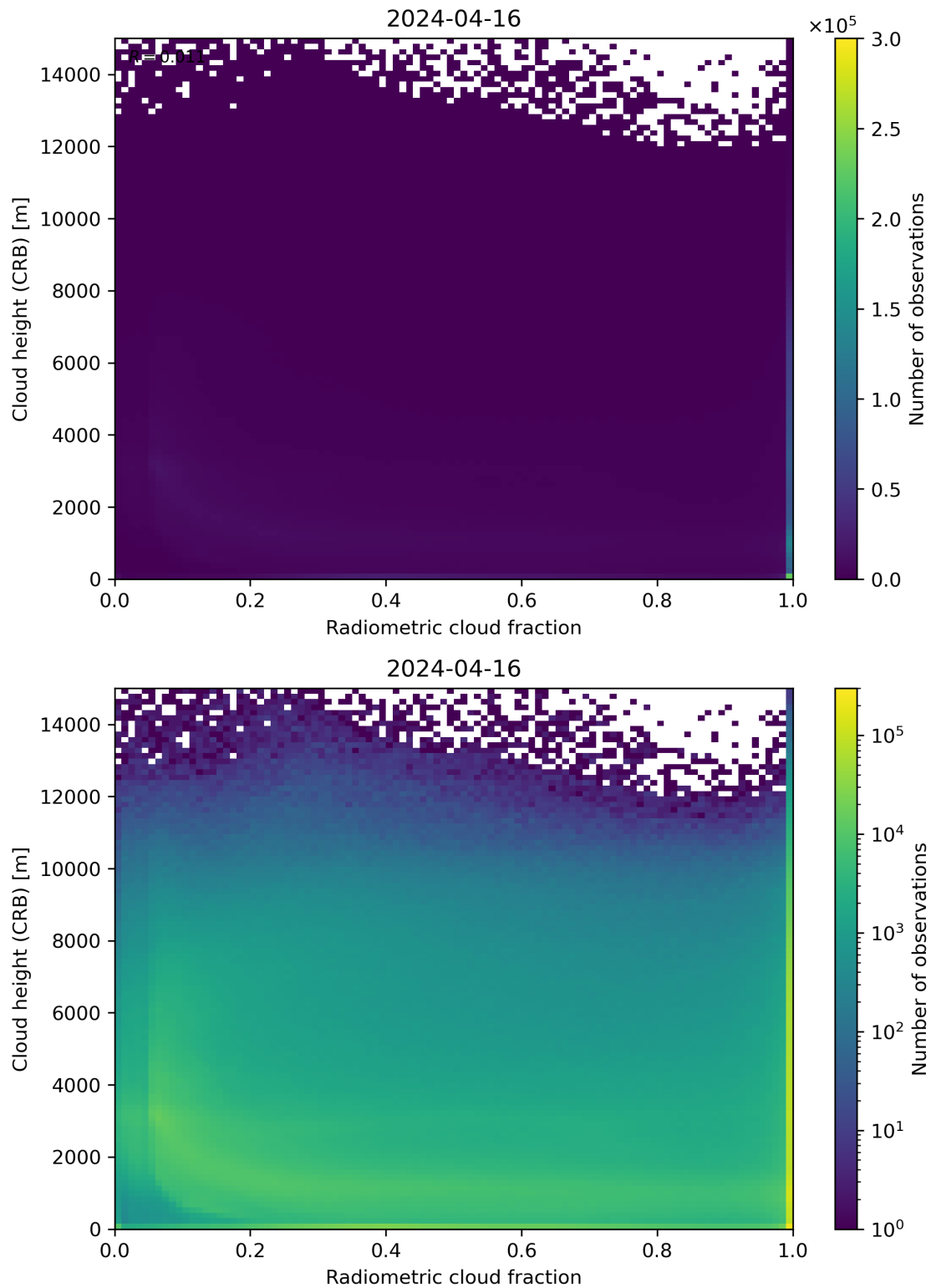
Figure 74: Scatter density plot of “Radiometric cloud fraction” against “Cloud height (CRB)” for 2024-04-16 to 2024-04-17.
