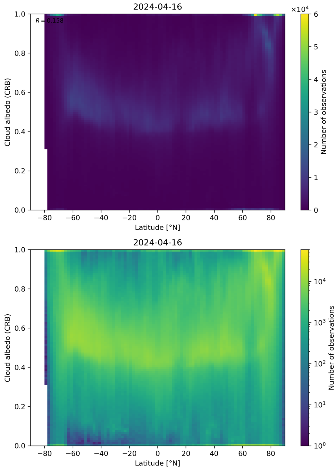
Figure 91: Scatter density plot of “Latitude” against “Cloud albedo (CRB)” for 2024-04-16 to 2024-04-17.
