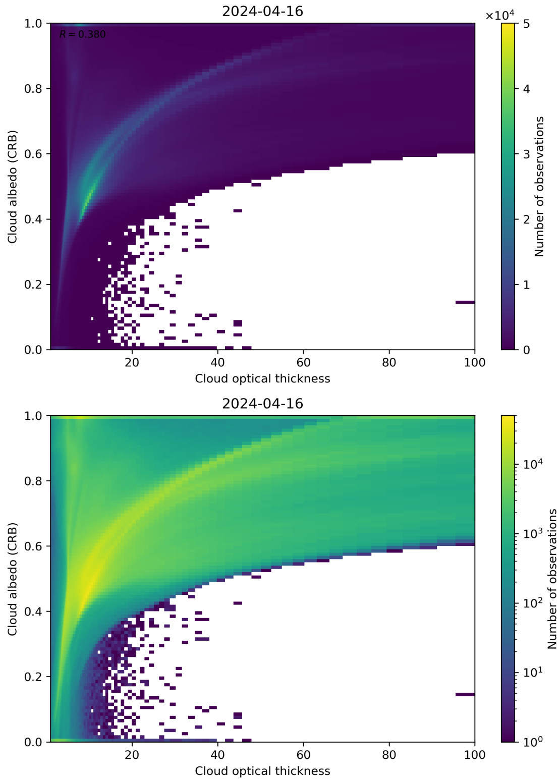
Figure 82: Scatter density plot of “Cloud optical thickness” against “Cloud albedo (CRB)” for 2024-04-16 to 2024-04-17.
