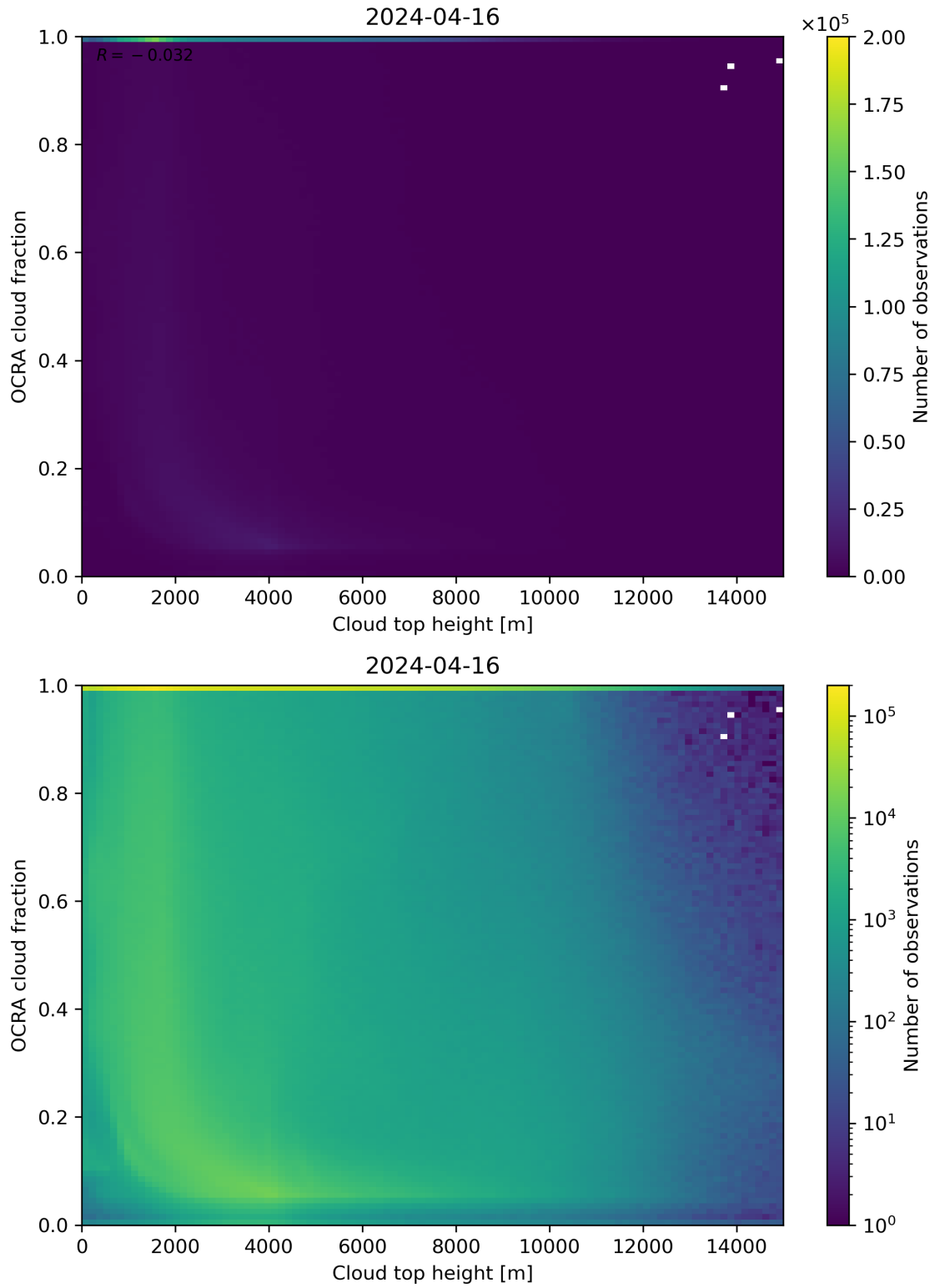
Figure 87: Scatter density plot of “Cloud top height” against “OCRA cloud fraction” for 2024-04-16 to 2024-04-17.
