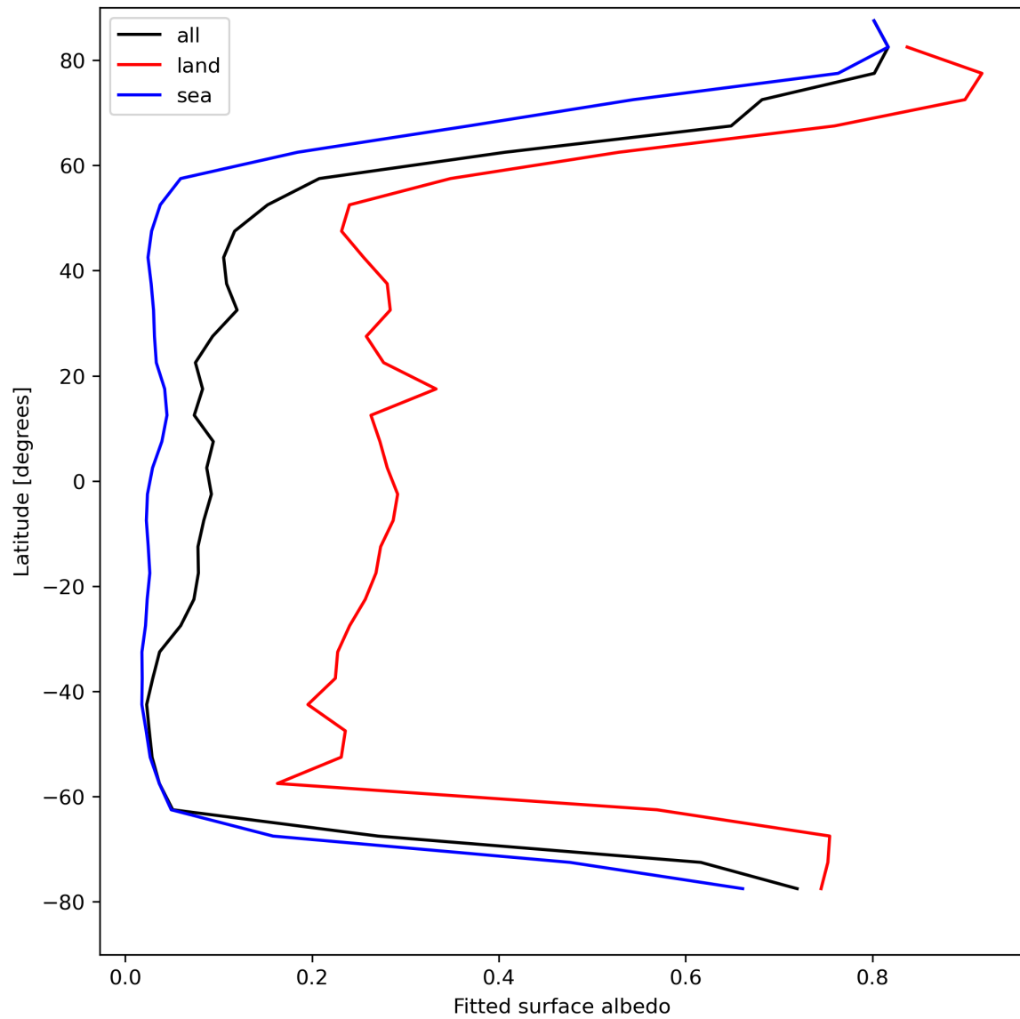
Figure 29: Zonal average of “Fitted surface albedo” for 2024-04-16 to 2024-04-17.
