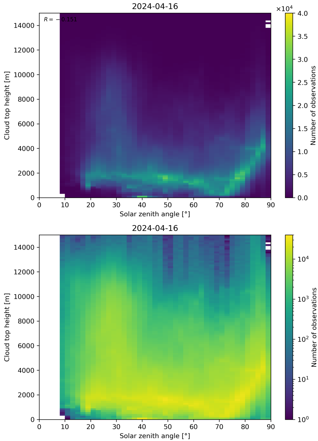
Figure 104: Scatter density plot of “Solar zenith angle” against “Cloud top height” for 2024-04-16 to 2024-04-17.
