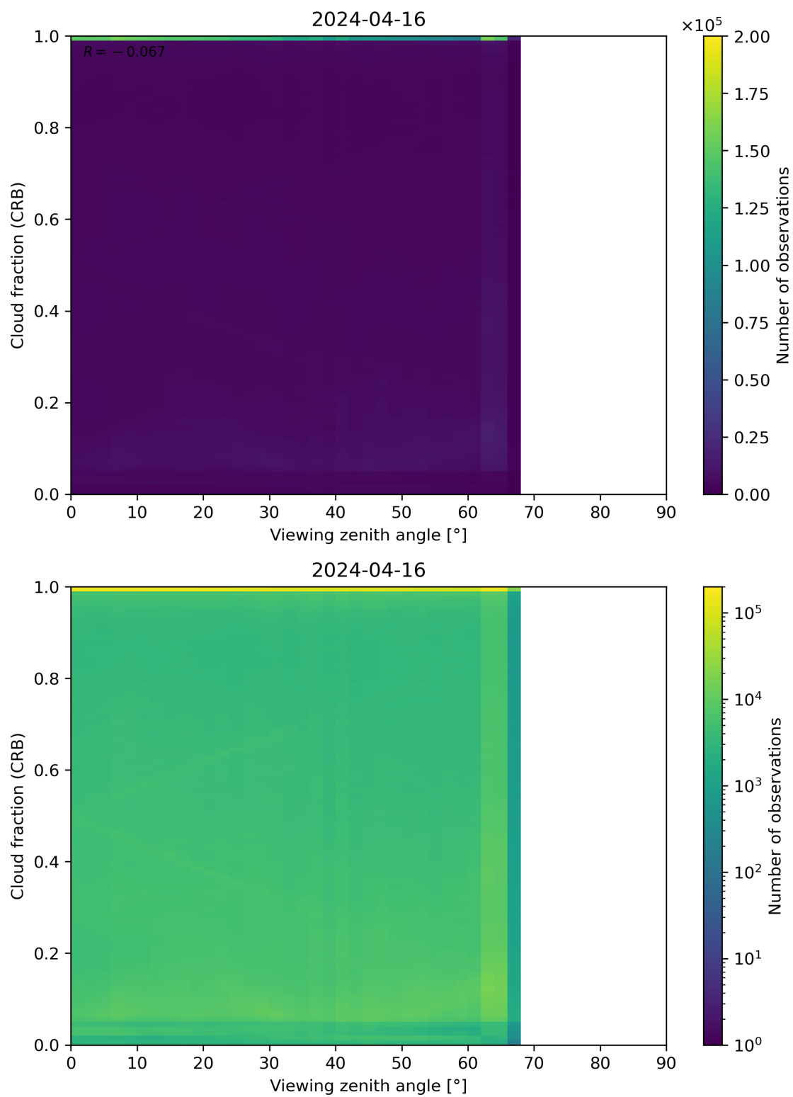
Figure 109: Scatter density plot of “Viewing zenith angle” against “Cloud fraction (CRB)” for 2024-04-16 to 2024-04-17.
