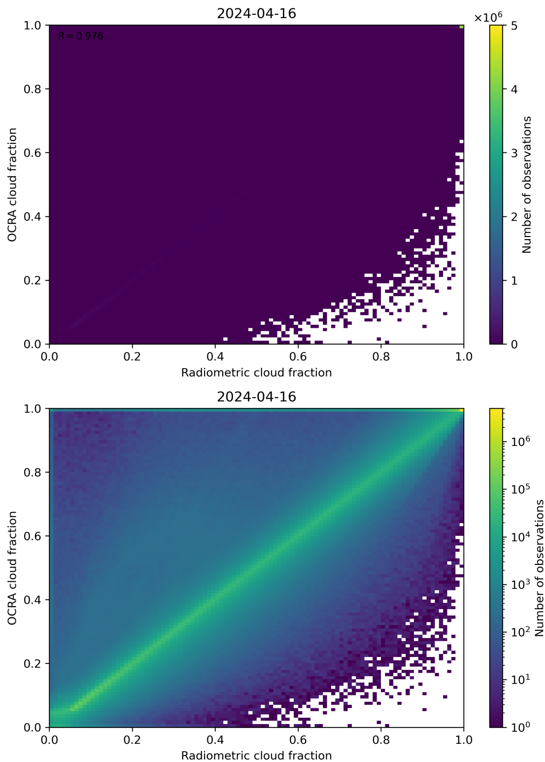
Figure 72: Scatter density plot of “Radiometric cloud fraction” against “OCRA cloud fraction” for 2024-04-16 to 2024-04-17.
