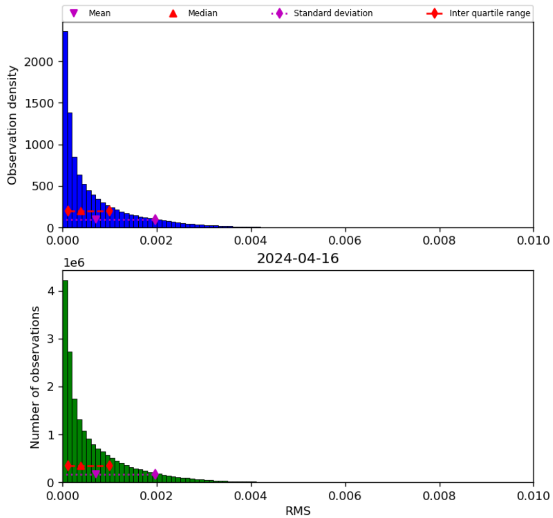
Figure 47: Histogram of “RMS” for 2024-04-16 to 2024-04-17
