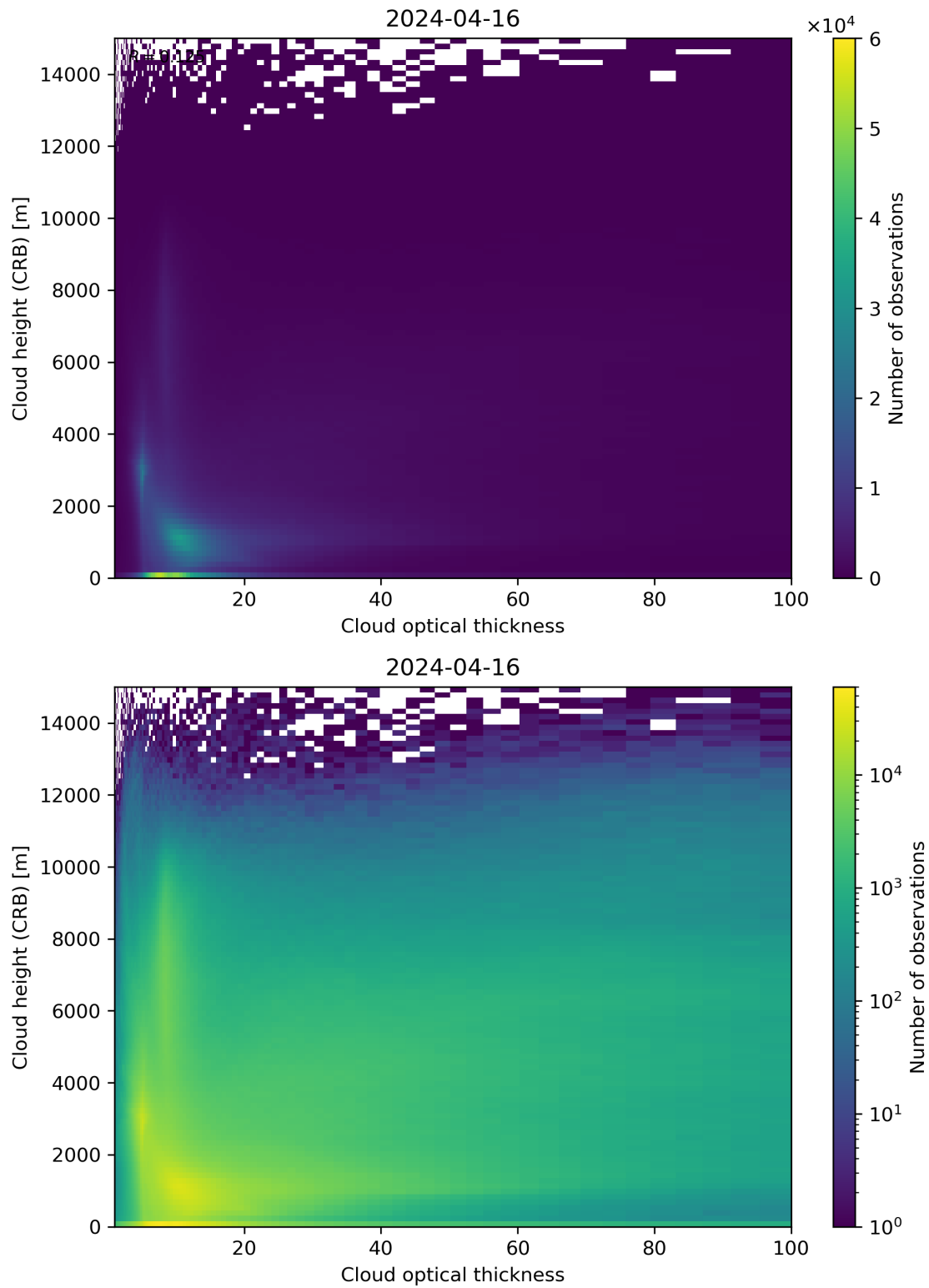
Figure 85: Scatter density plot of “Cloud optical thickness” against “Cloud height (CRB)” for 2024-04-16 to 2024-04-17.
