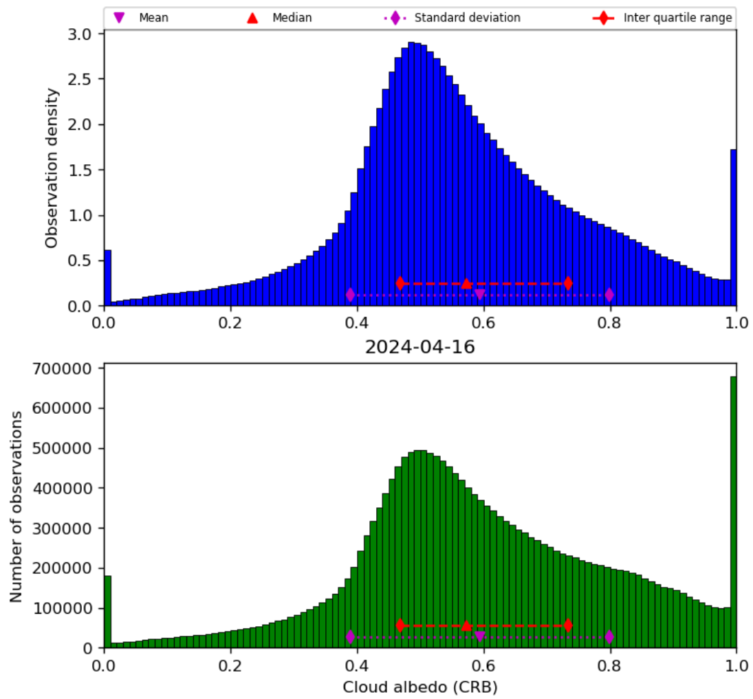
Figure 44: Histogram of “Cloud albedo (CRB)” for 2024-04-16 to 2024-04-17
