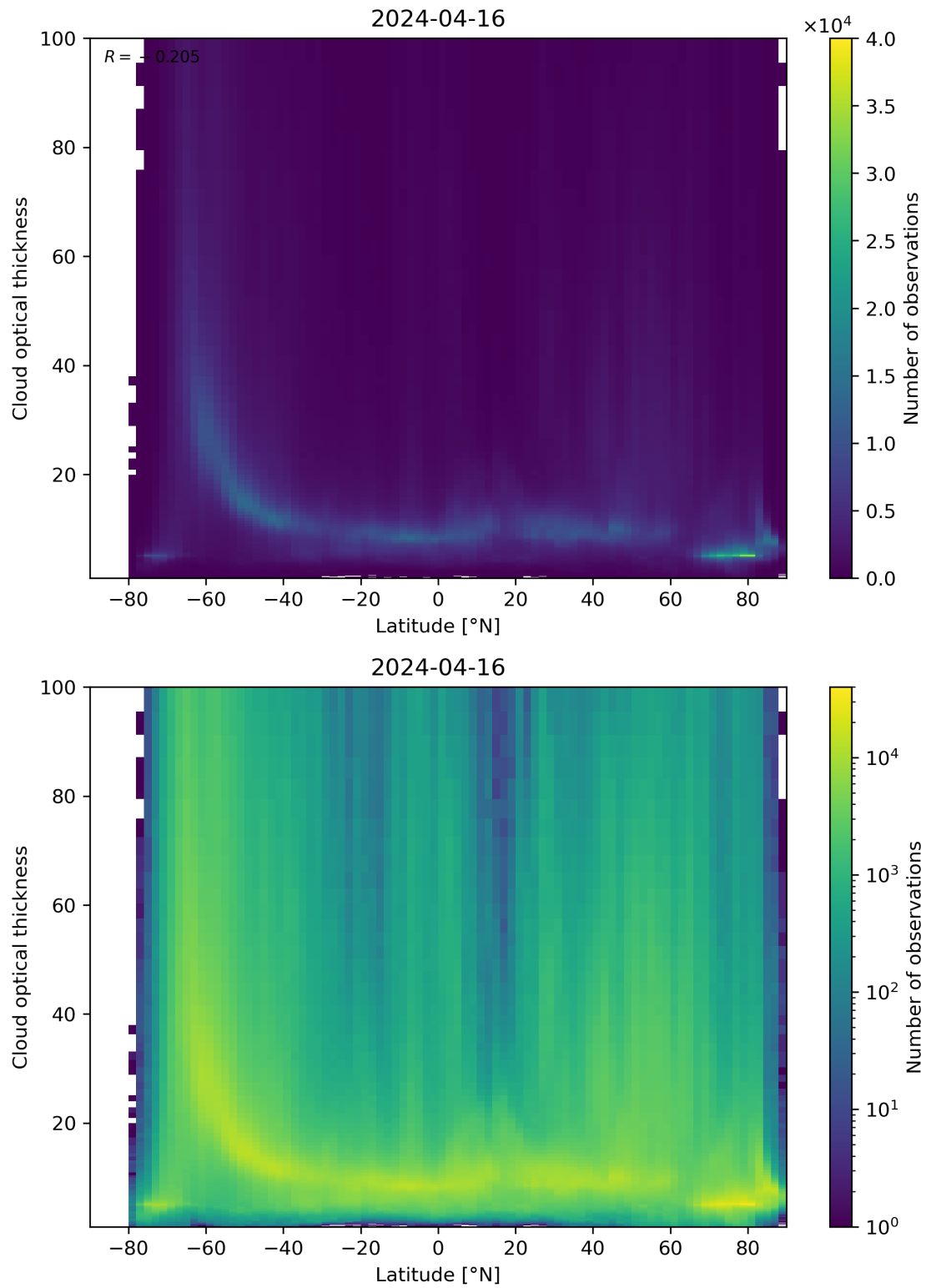
Figure 96: Scatter density plot of “Latitude” against “Cloud optical thickness” for 2024-04-16 to 2024-04-17.
