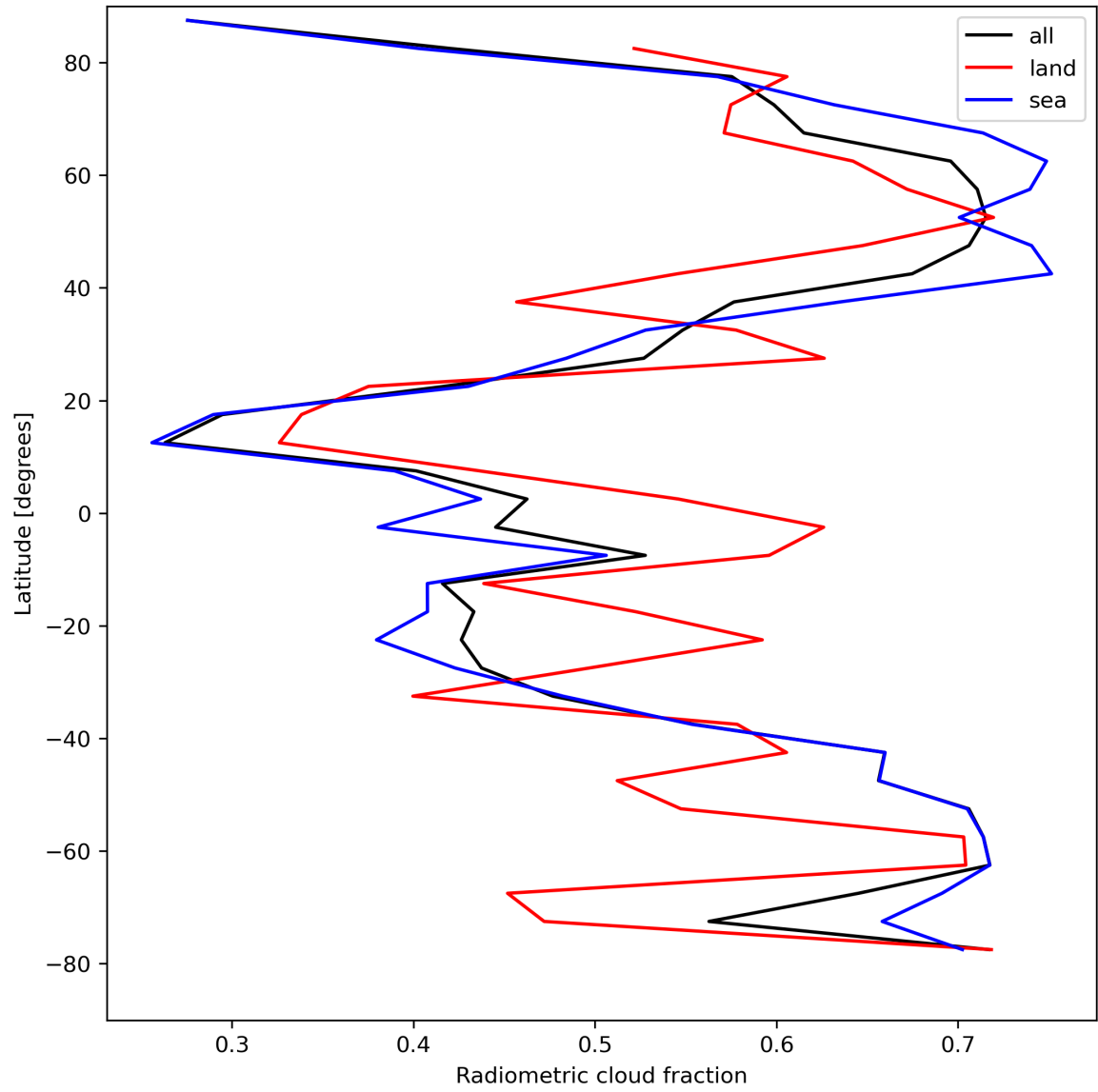
Figure 23: Zonal average of “Radiometric cloud fraction” for 2024-04-16 to 2024-04-17.
