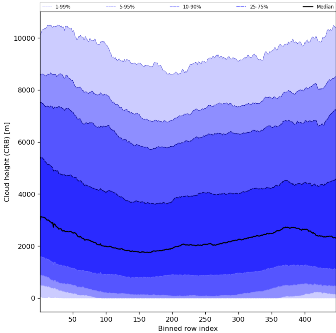
Figure 59: Along track statistics of “Cloud height (CRB)” for 2024-04-16 to 2024-04-17
