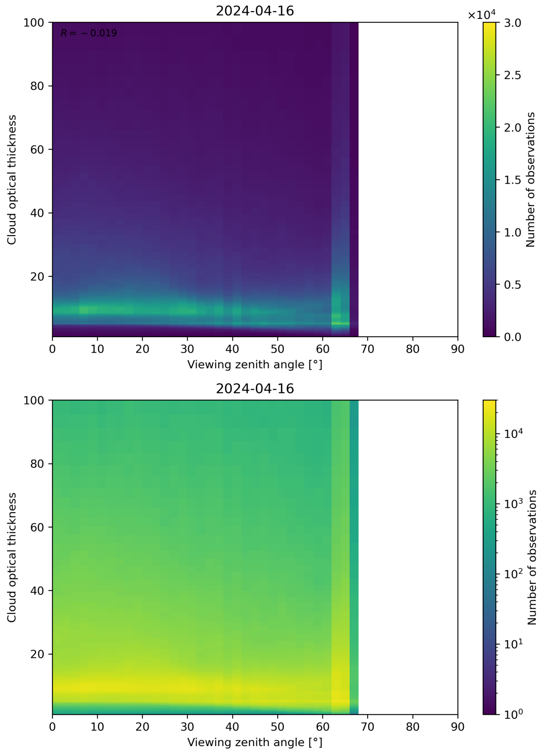
Figure 111: Scatter density plot of “Viewing zenith angle” against “Cloud optical thickness” for 2024-04-16 to 2024-04-17.
