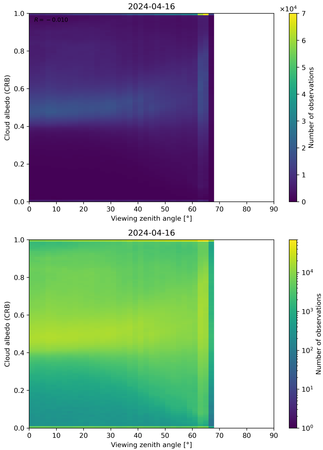
Figure 106: Scatter density plot of “Viewing zenith angle” against “Cloud albedo (CRB)” for 2024-04-16 to 2024-04-17.
