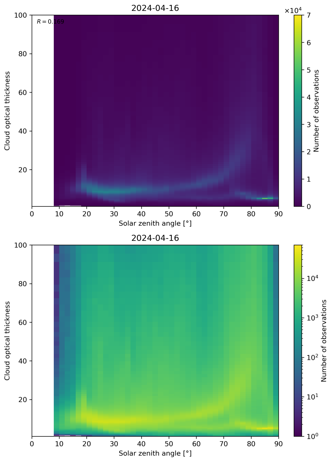
Figure 103: Scatter density plot of “Solar zenith angle” against “Cloud optical thickness” for 2024-04-16 to 2024-04-17.
