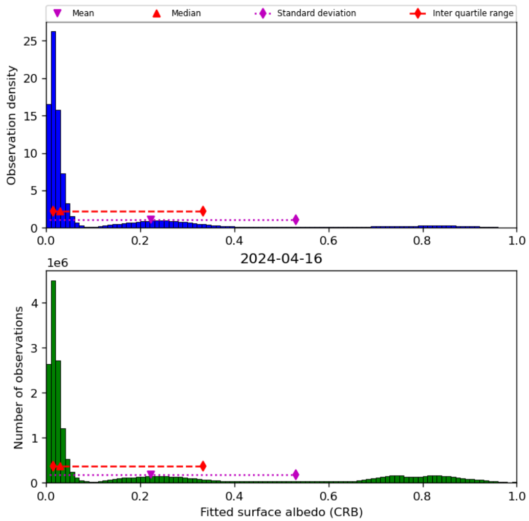
Figure 46: Histogram of “Fitted surface albedo (CRB)” for 2024-04-16 to 2024-04-17
