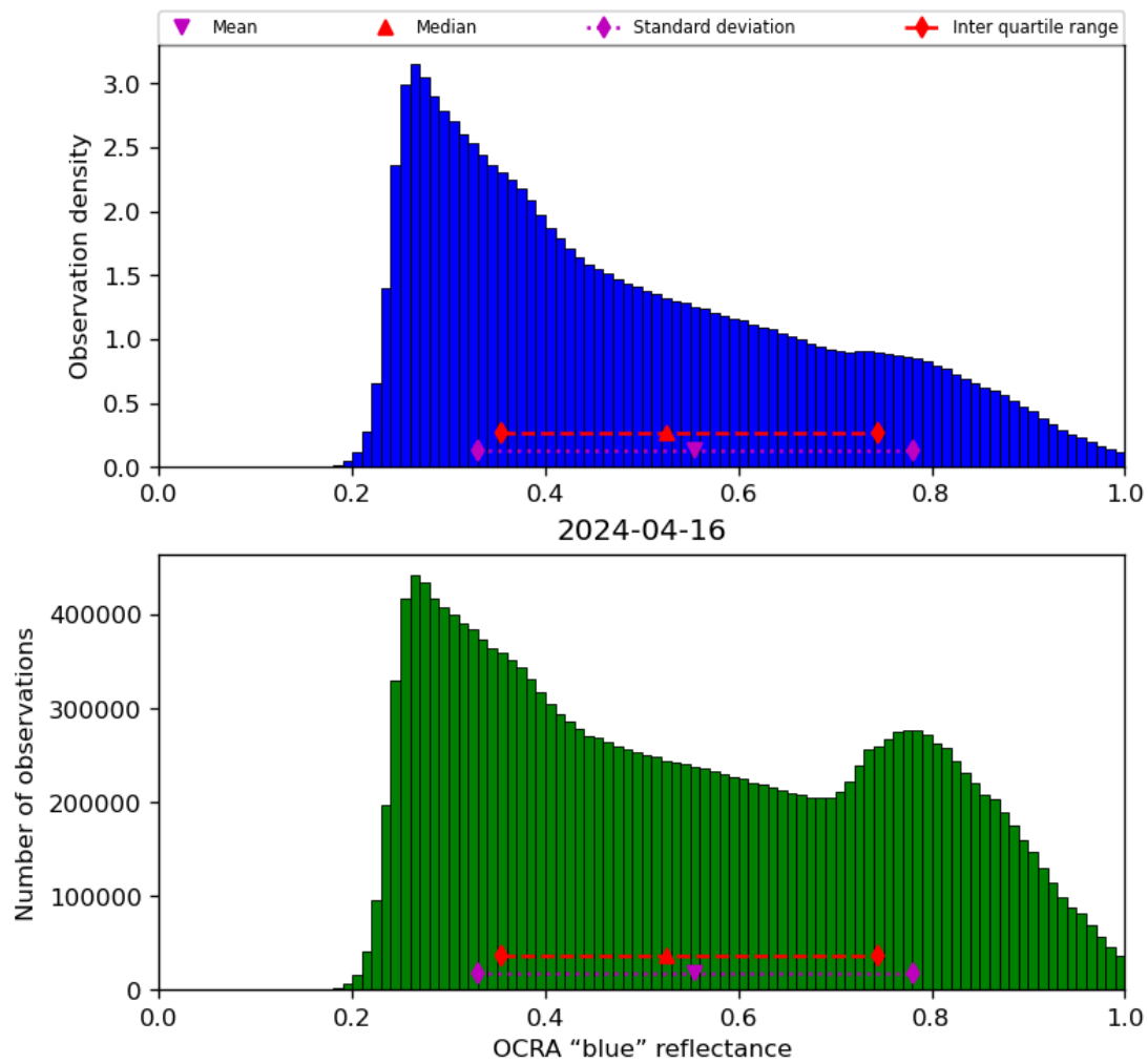
Figure 51: Histogram of “OCRA “blue” reflectance” for 2024-04-16 to 2024-04-17
