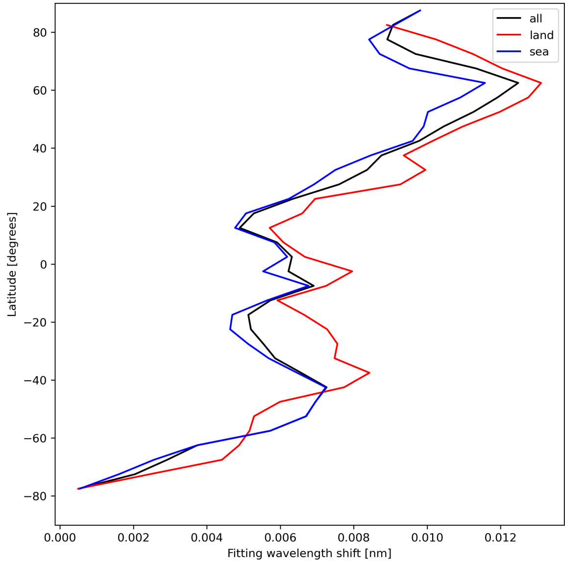
Figure 33: Zonal average of “Fitting wavelength shift” for 2024-04-16 to 2024-04-17.
