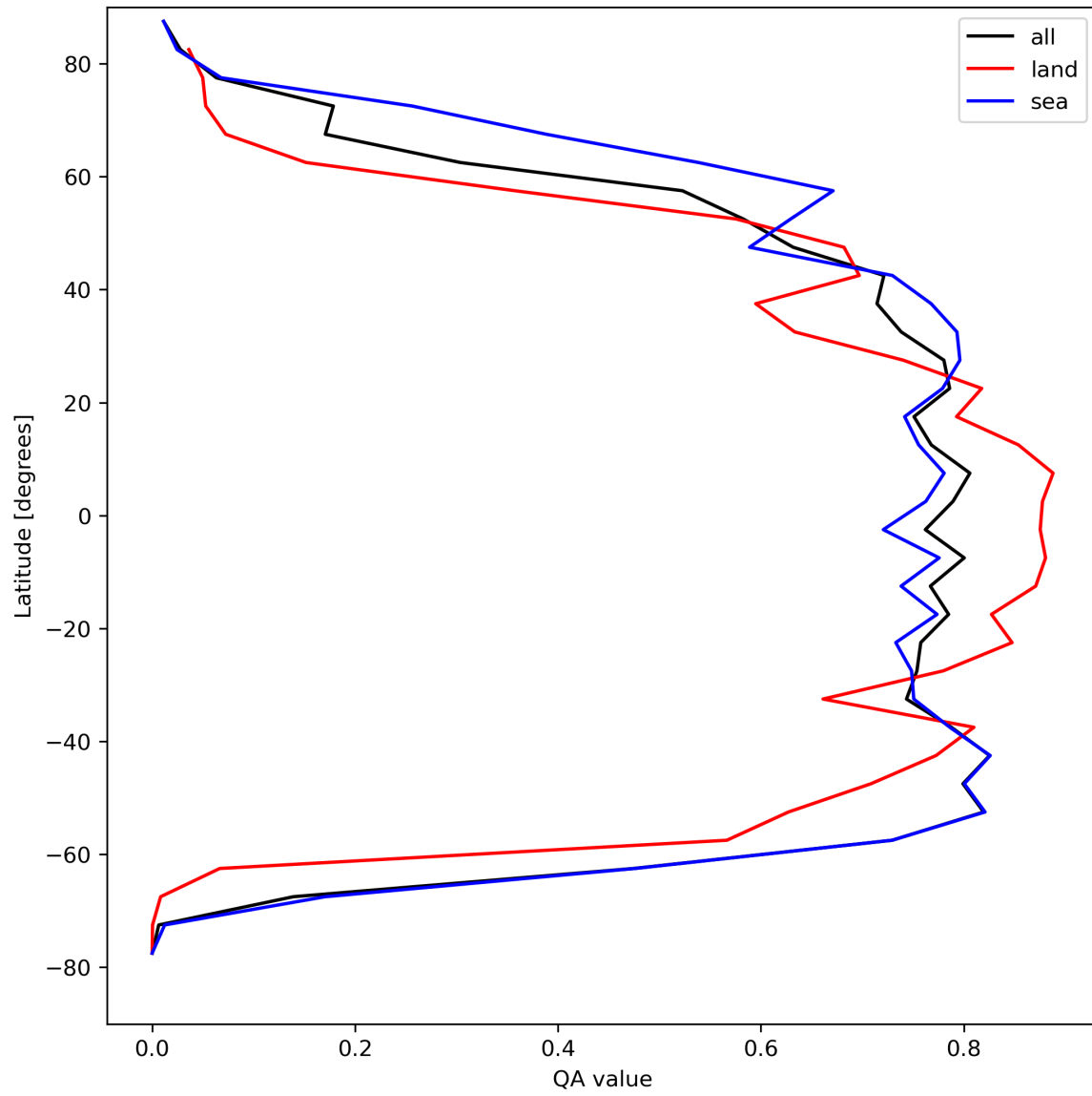
Figure 22: Zonal average of “QA value” for 2024-04-16 to 2024-04-17.
