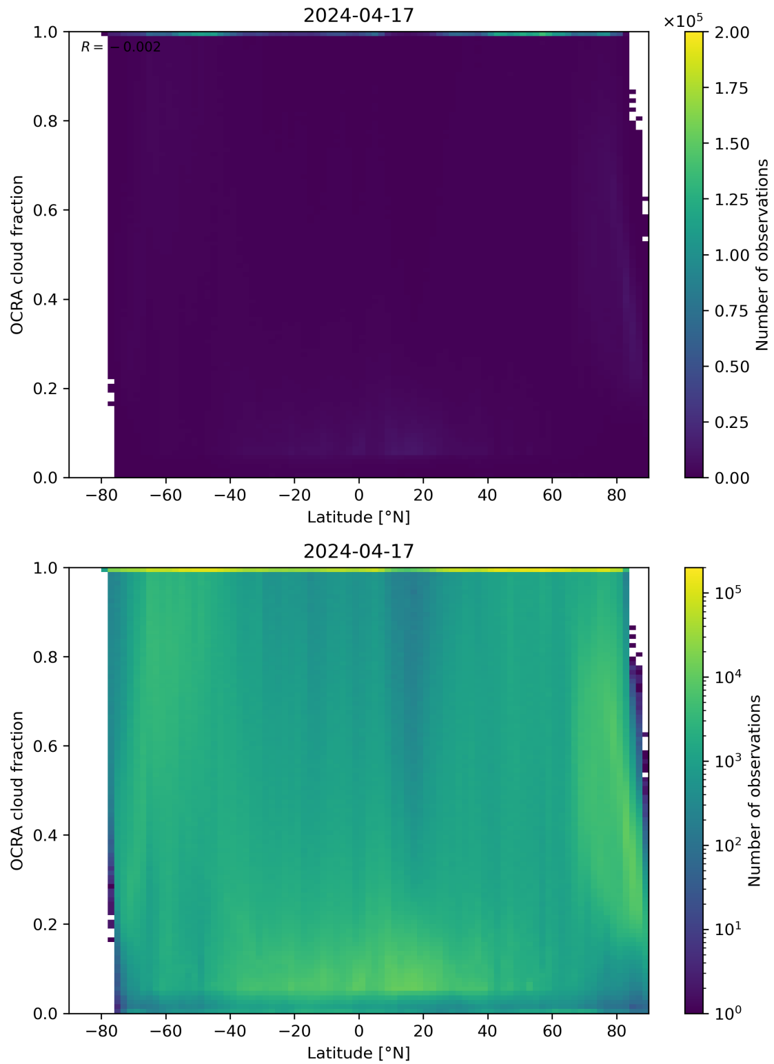
Figure 93: Scatter density plot of “Latitude” against “OCRA cloud fraction” for 2024-04-16 to 2024-04-18.
