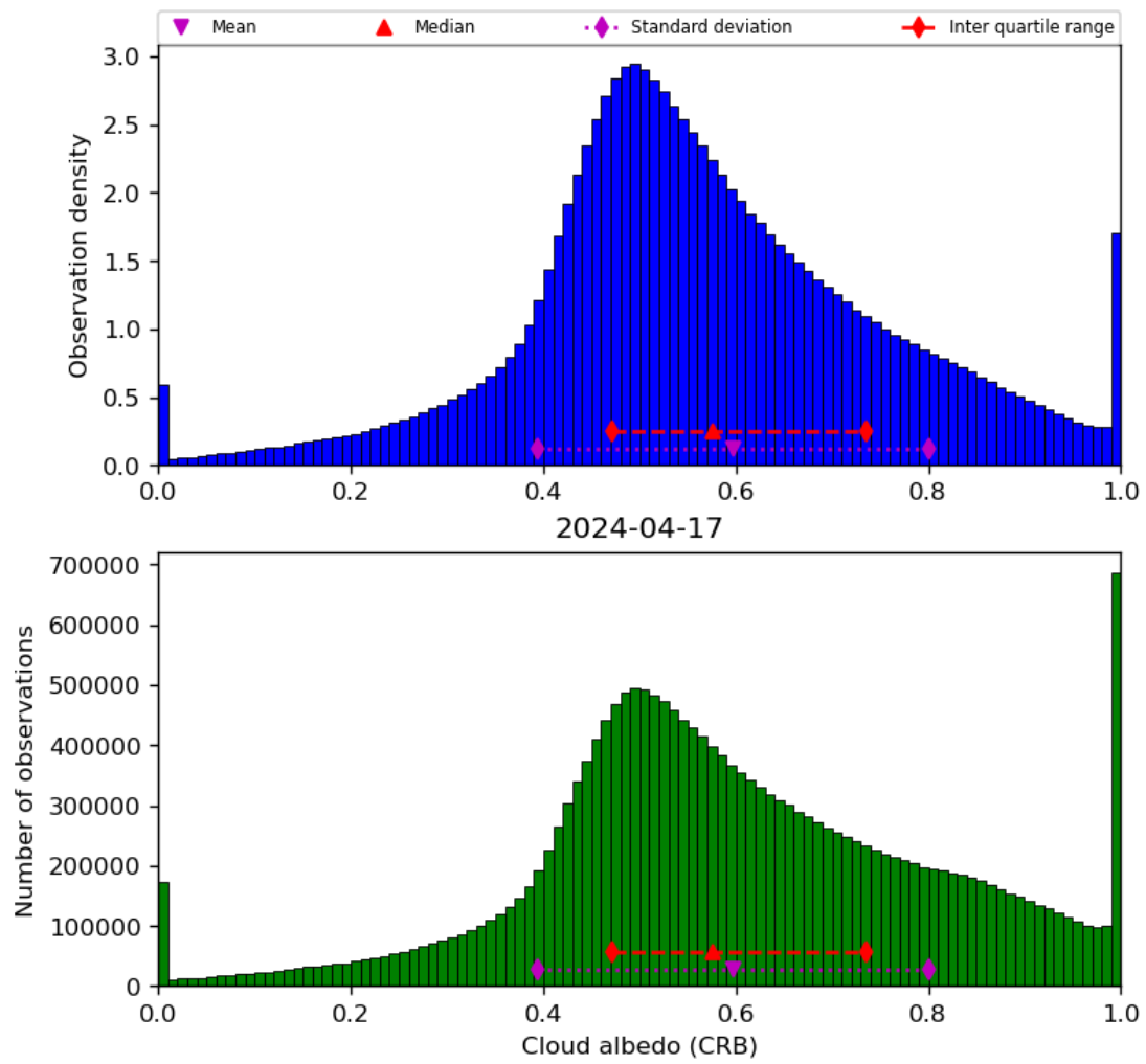
Figure 44: Histogram of “Cloud albedo (CRB)” for 2024-04-16 to 2024-04-18
