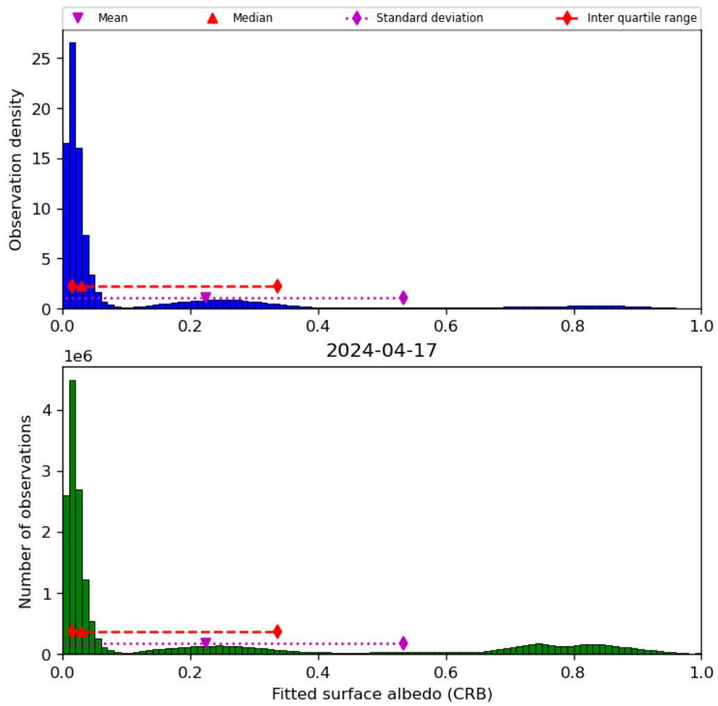
Figure 46: Histogram of “Fitted surface albedo (CRB)” for 2024-04-16 to 2024-04-18
