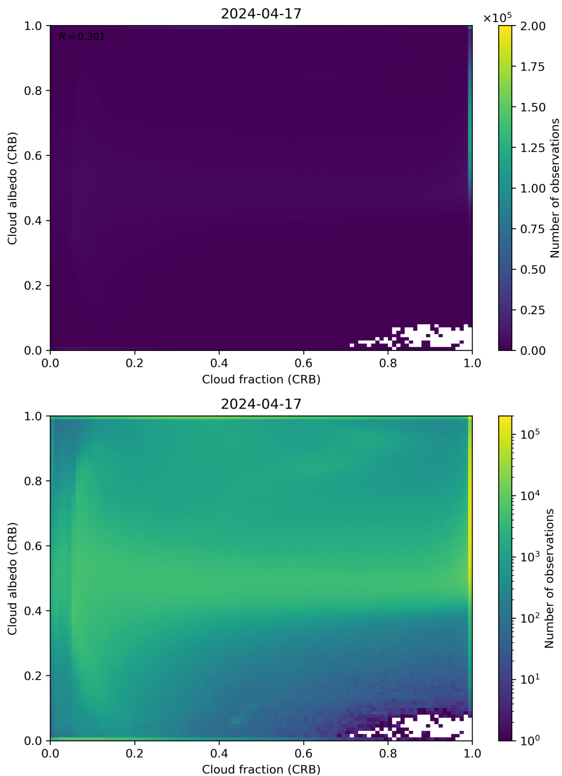
Figure 77: Scatter density plot of “Cloud fraction (CRB)” against “Cloud albedo (CRB)” for 2024-04-16 to 2024-04-18.
