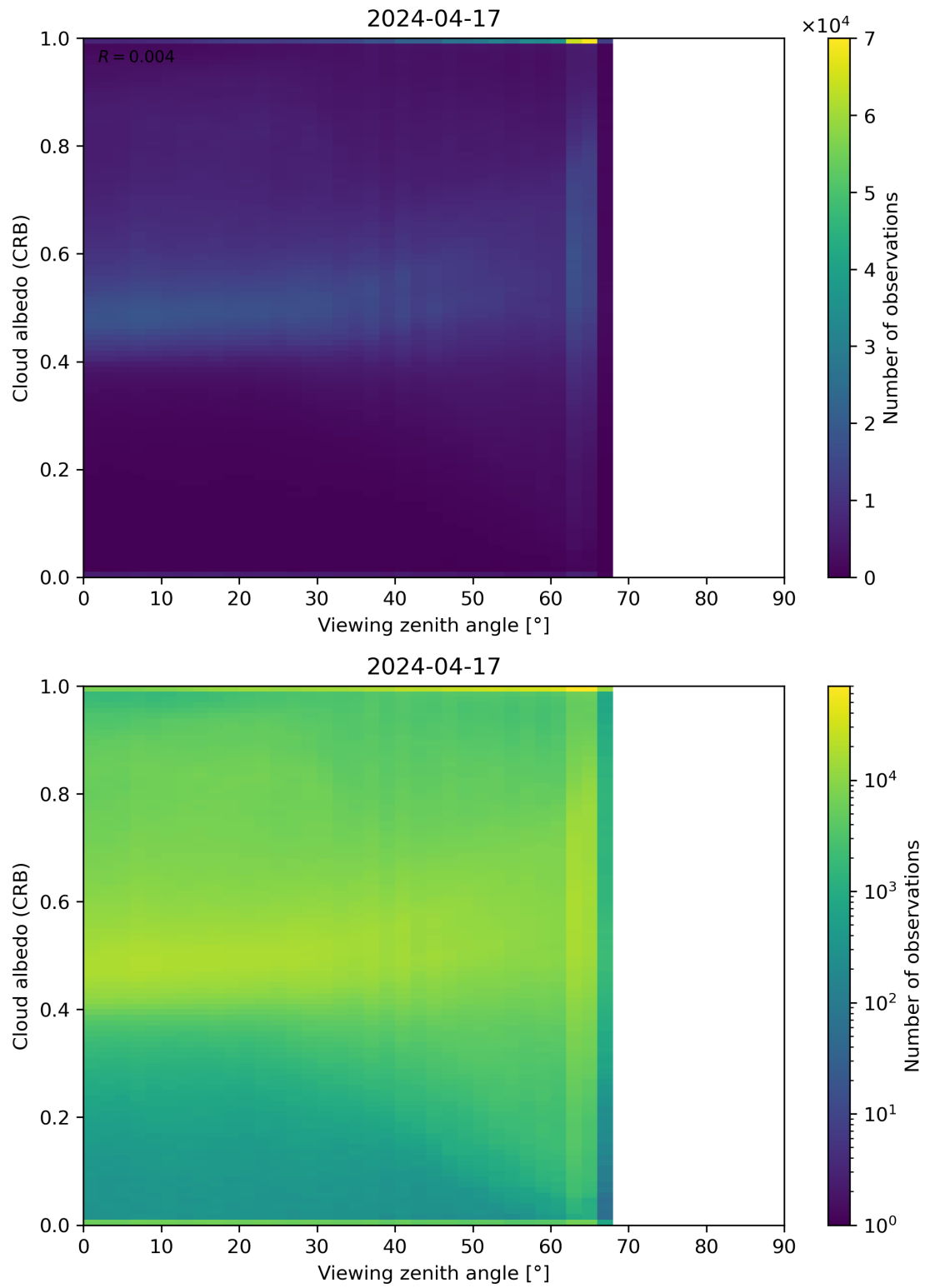
Figure 106: Scatter density plot of “Viewing zenith angle” against “Cloud albedo (CRB)” for 2024-04-16 to 2024-04-18.
