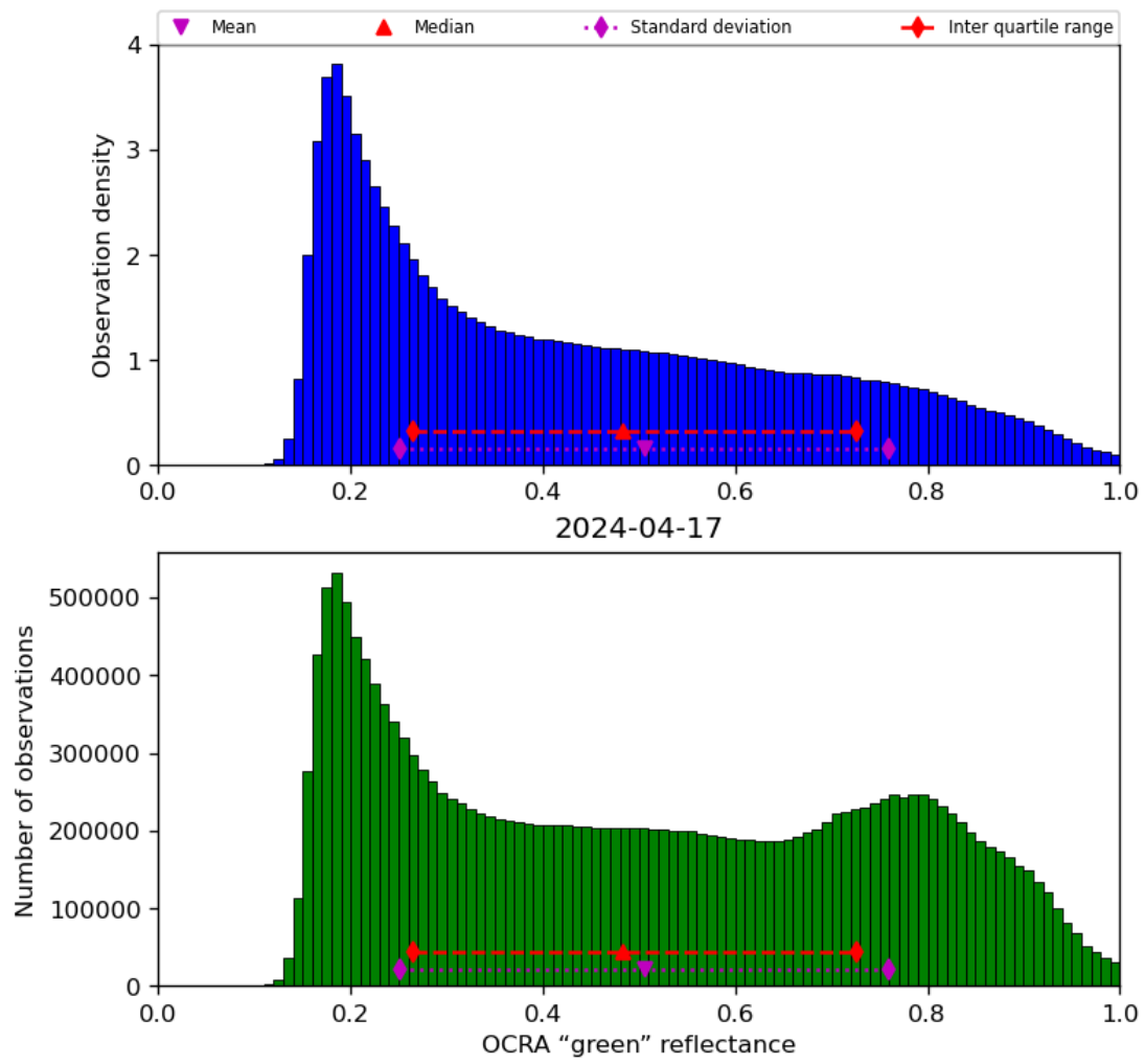
Figure 52: Histogram of “OCRA “green” reflectance” for 2024-04-16 to 2024-04-18
