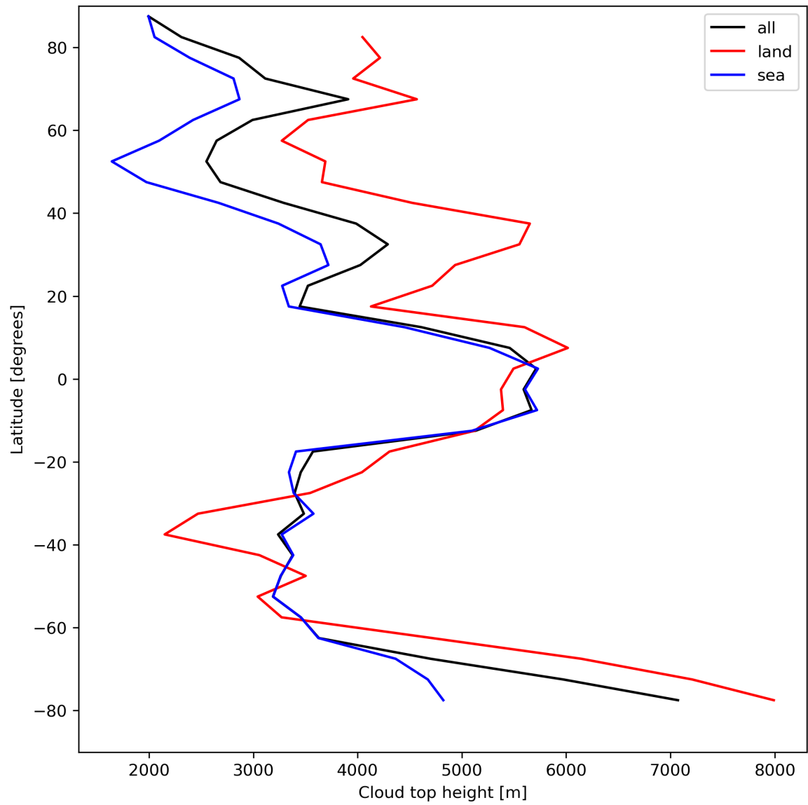
Figure 24: Zonal average of “Cloud top height” for 2024-04-16 to 2024-04-18.
