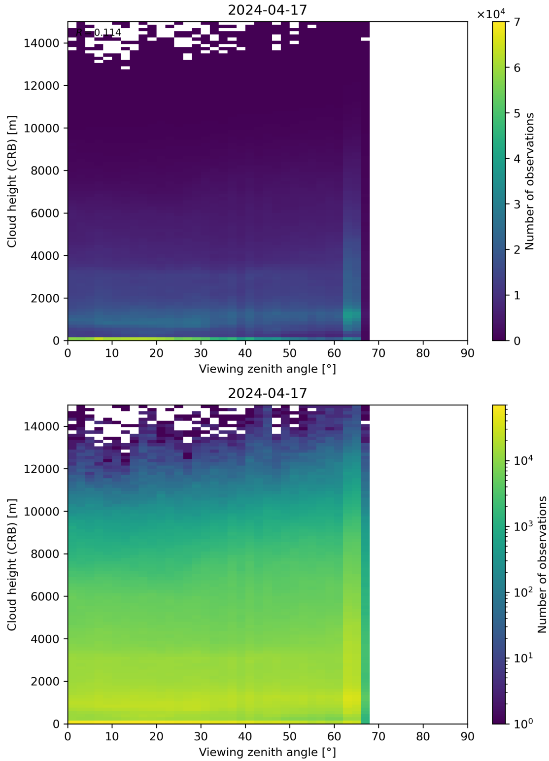
Figure 110: Scatter density plot of “Viewing zenith angle” against “Cloud height (CRB)” for 2024-04-16 to 2024-04-18.
