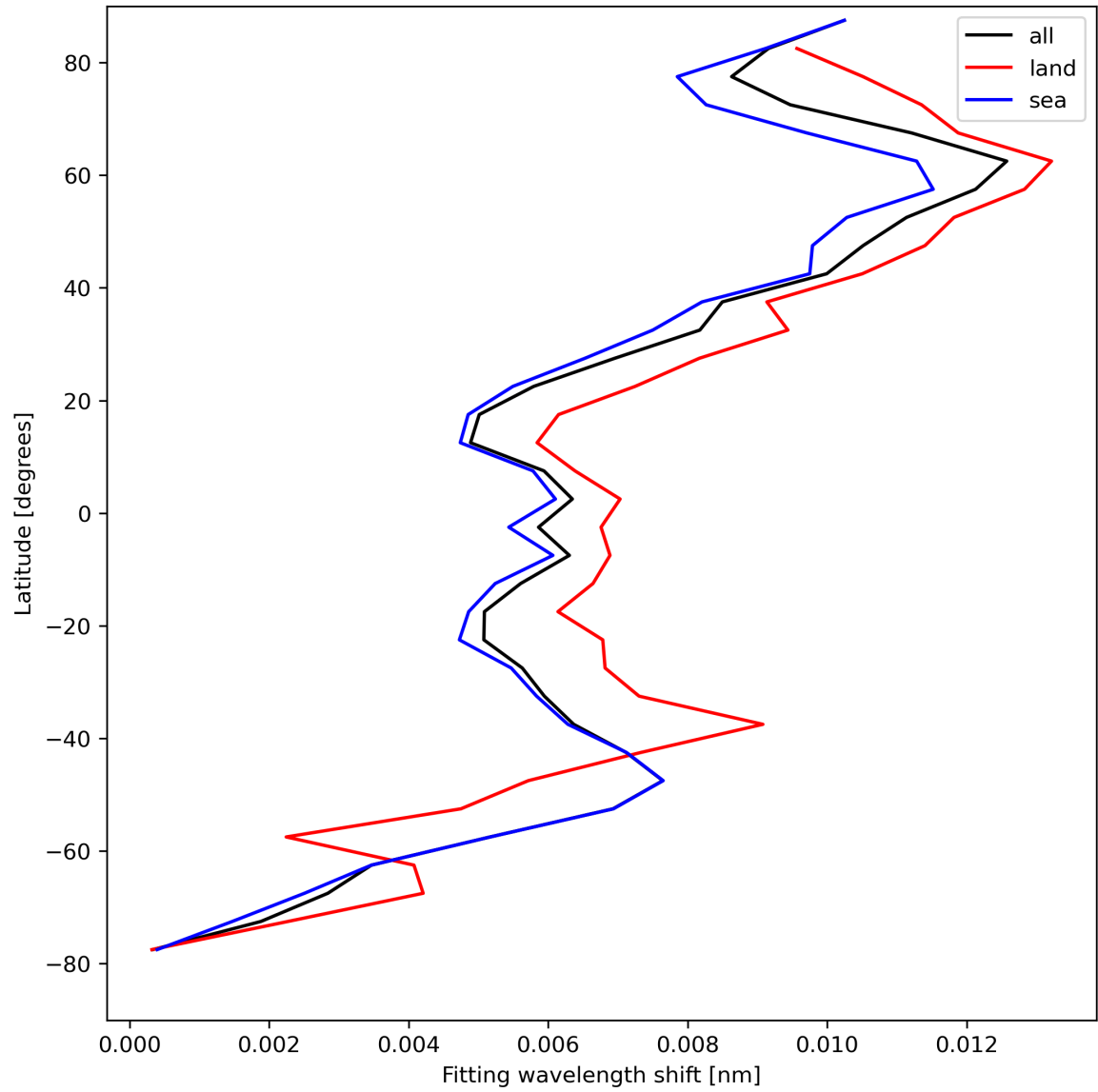
Figure 33: Zonal average of “Fitting wavelength shift” for 2024-04-16 to 2024-04-18.
