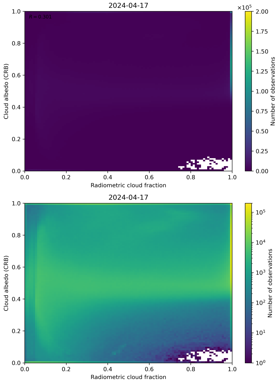
Figure 71: Scatter density plot of “Radiometric cloud fraction” against “Cloud albedo (CRB)” for 2024-04-16 to 2024-04-18.
