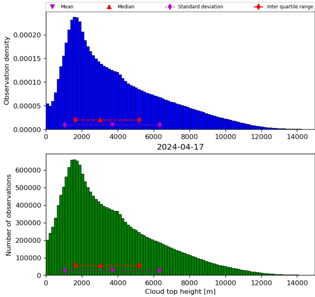
Figure 40: Histogram of “Cloud top height” for 2024-04-16 to 2024-04-18
