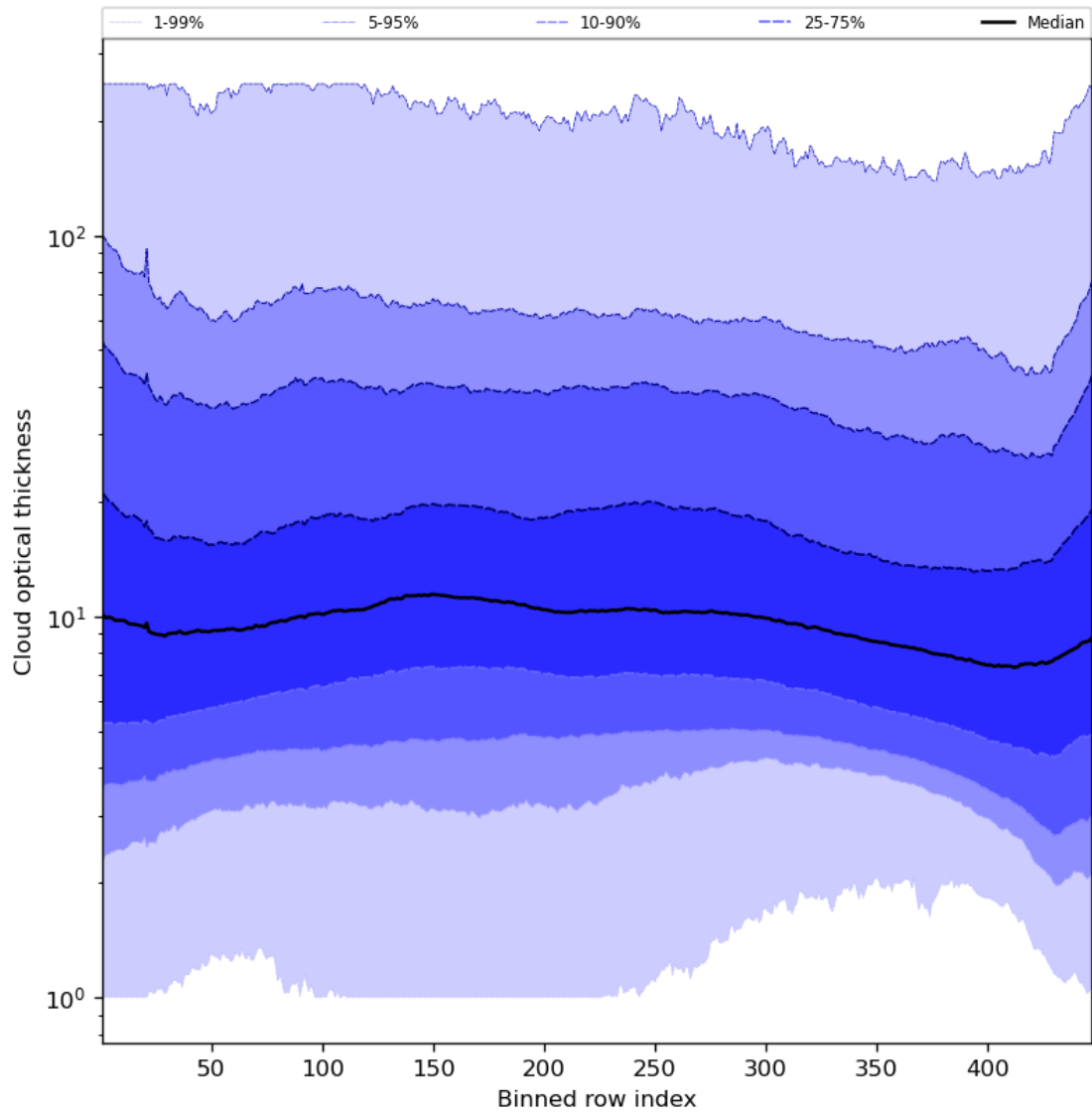
Figure 57: Along track statistics of “Cloud optical thickness” for 2024-04-16 to 2024-04-18
