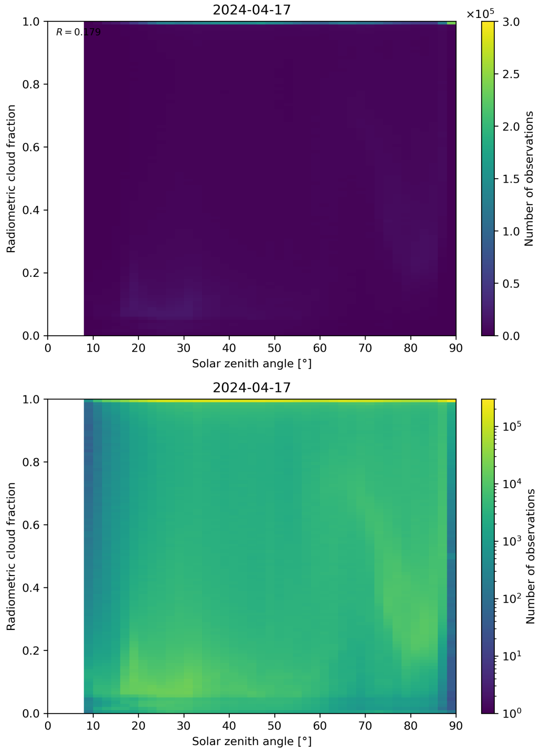
Figure 99: Scatter density plot of “Solar zenith angle” against “Radiometric cloud fraction” for 2024-04-16 to 2024-04-18.
