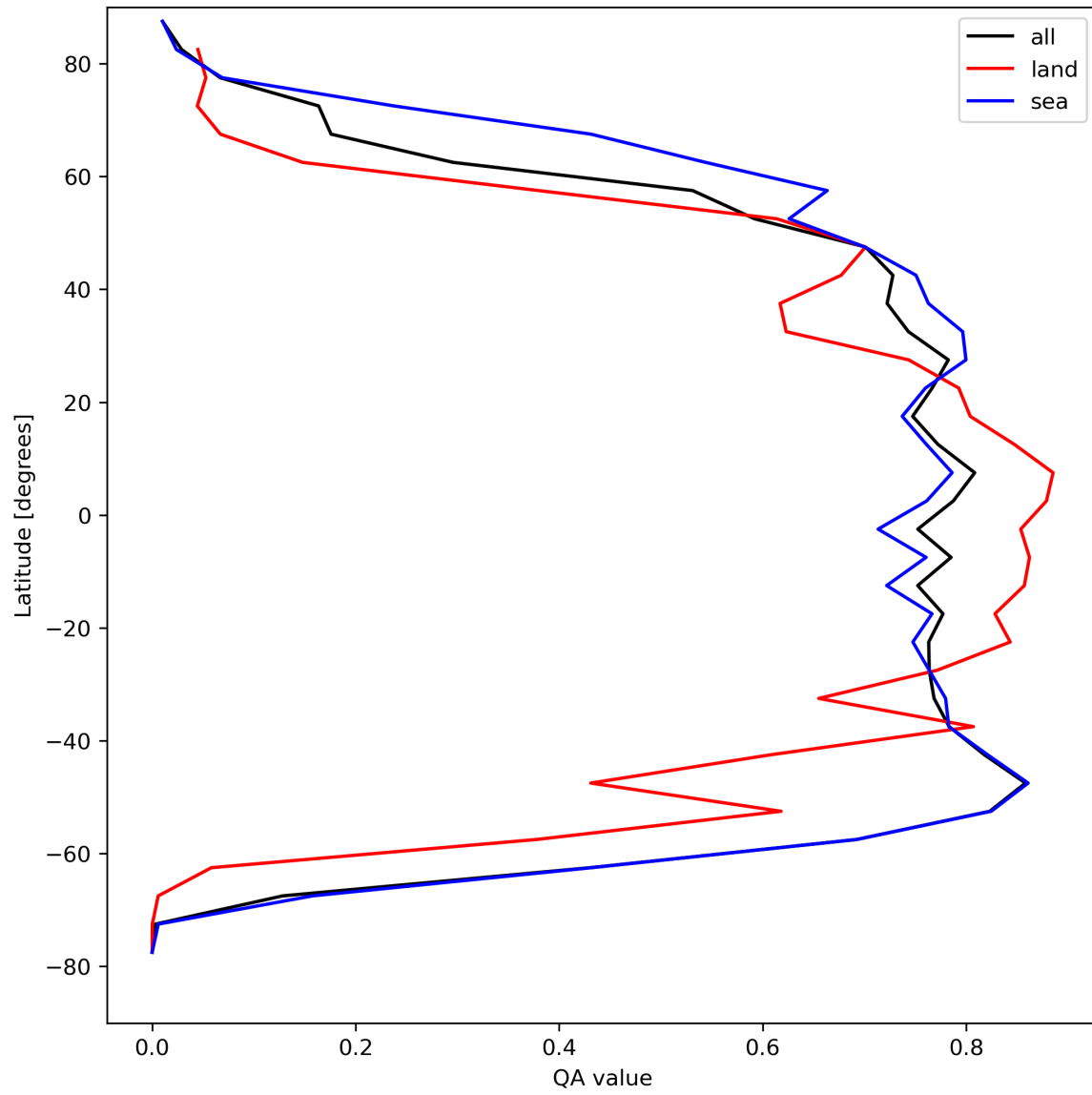
Figure 22: Zonal average of “QA value” for 2024-04-16 to 2024-04-18.
