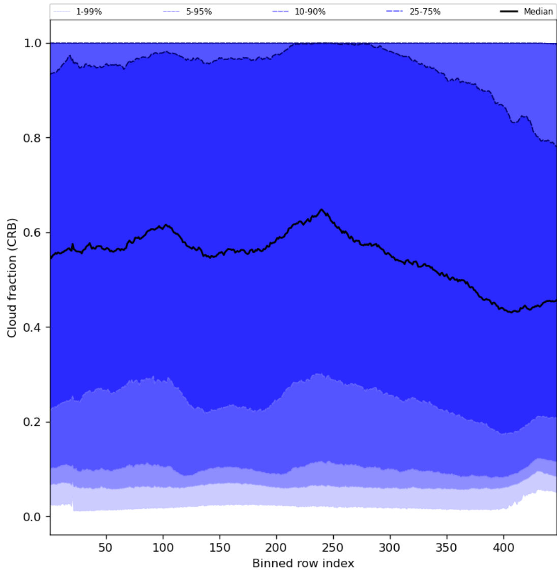
Figure 58: Along track statistics of “Cloud fraction (CRB)” for 2024-04-16 to 2024-04-18
