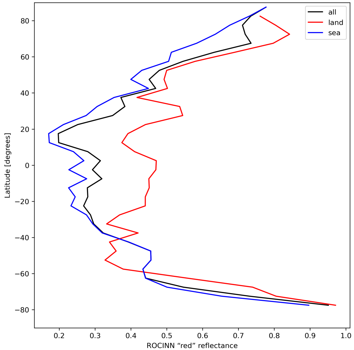
Figure 37: Zonal average of “ROCINN “red” reflectance” for 2024-04-16 to 2024-04-18.
