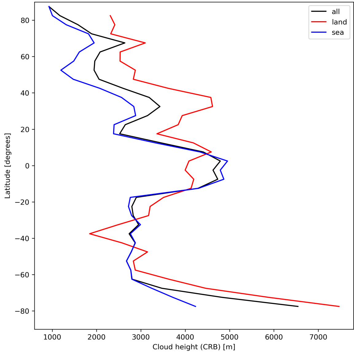
Figure 27: Zonal average of “Cloud height (CRB)” for 2024-04-16 to 2024-04-18.
