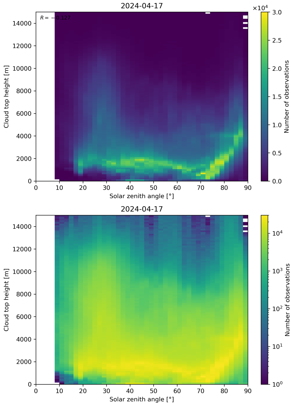
Figure 104: Scatter density plot of “Solar zenith angle” against “Cloud top height” for 2024-04-16 to 2024-04-18.
