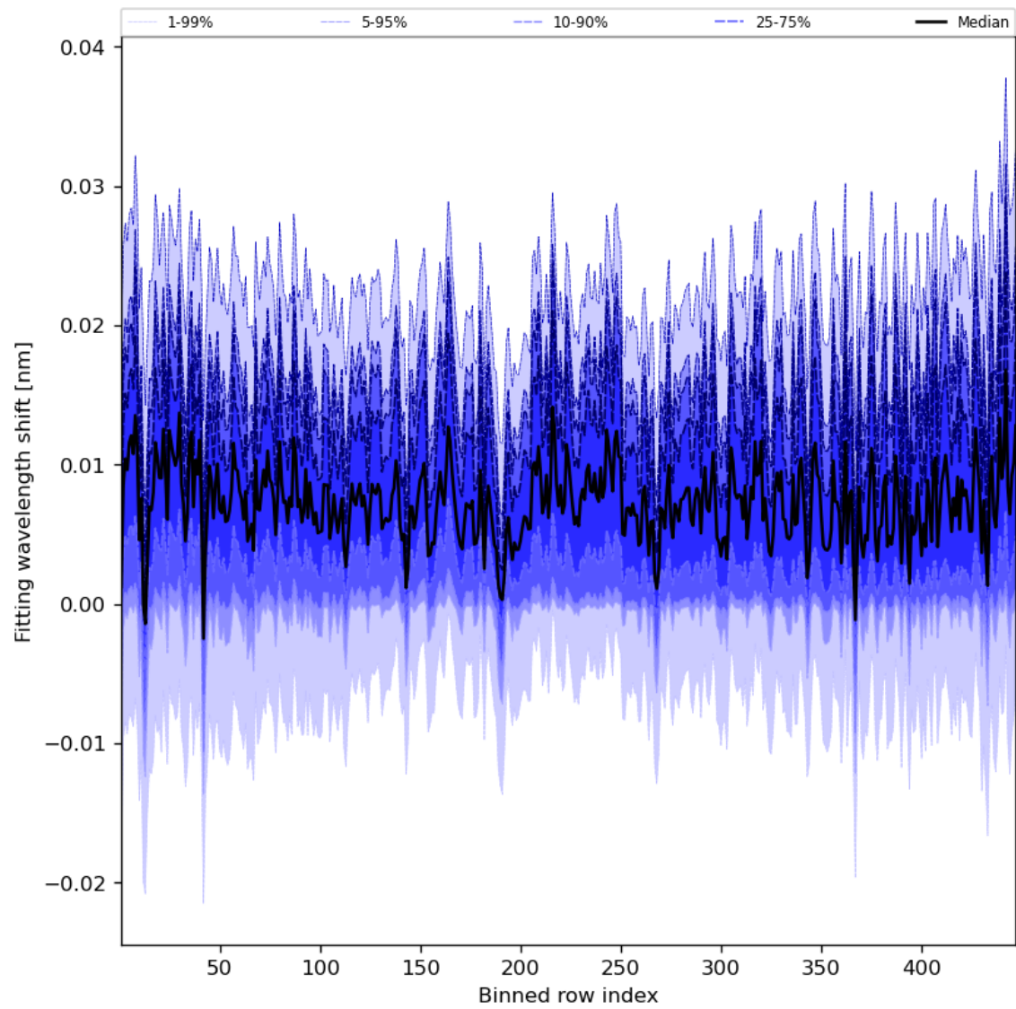
Figure 65: Along track statistics of “Fitting wavelength shift” for 2024-04-16 to 2024-04-18
