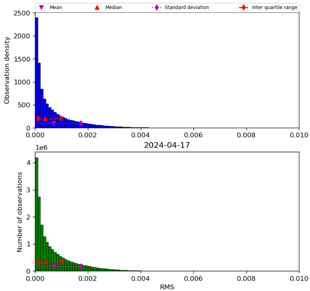
Figure 47: Histogram of “RMS” for 2024-04-16 to 2024-04-18
