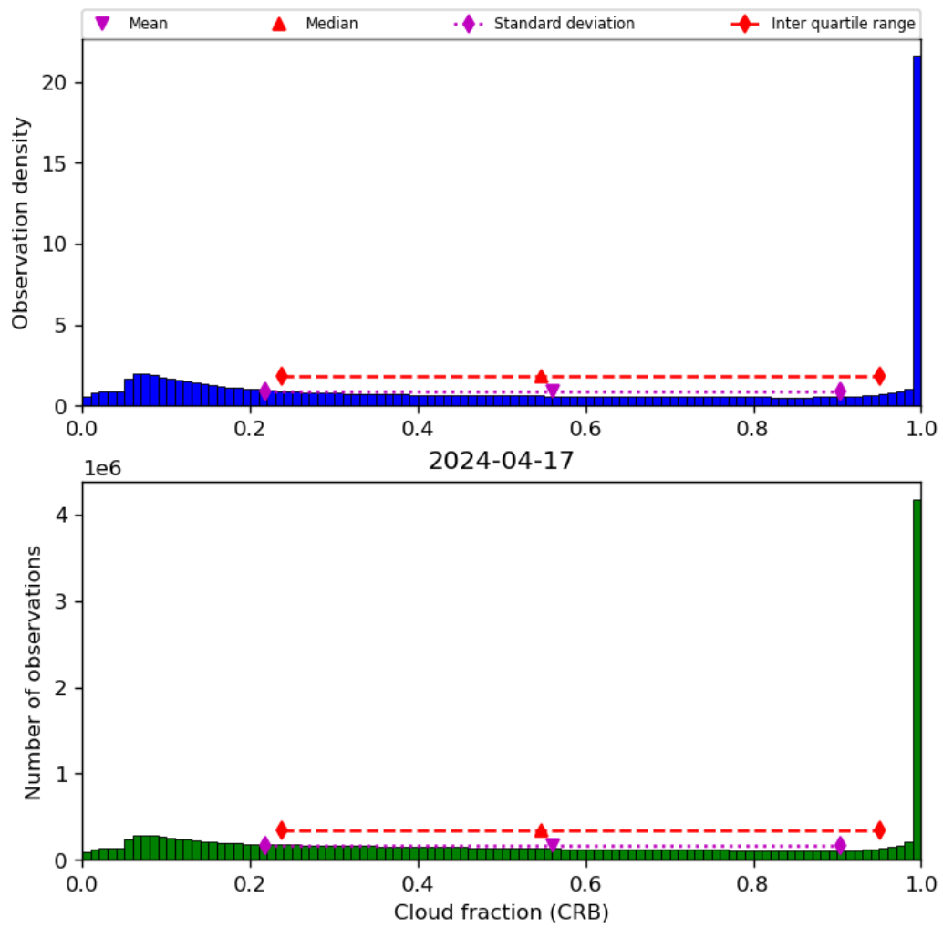
Figure 42: Histogram of “Cloud fraction (CRB)” for 2024-04-16 to 2024-04-18
