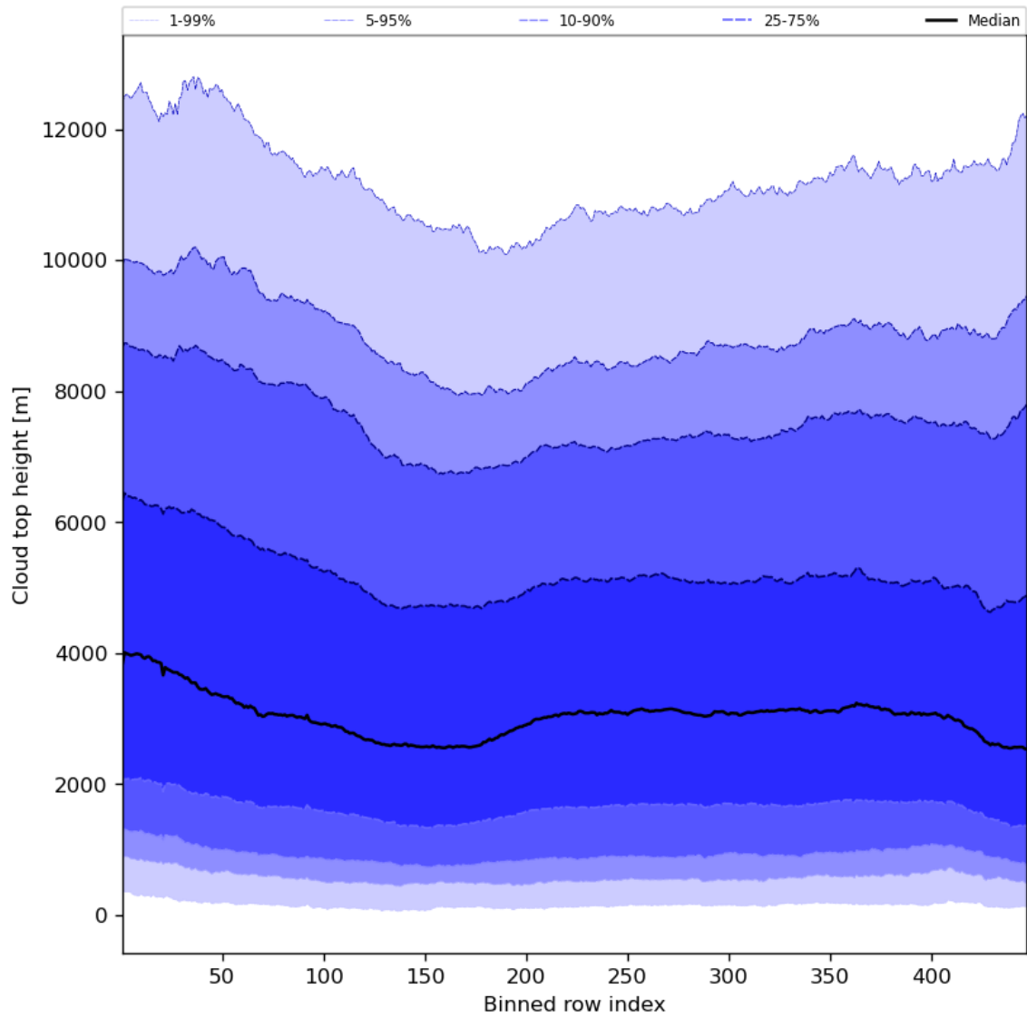
Figure 56: Along track statistics of “Cloud top height” for 2024-04-16 to 2024-04-18
