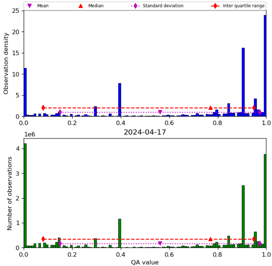
Figure 38: Histogram of “QA value” for 2024-04-16 to 2024-04-18
