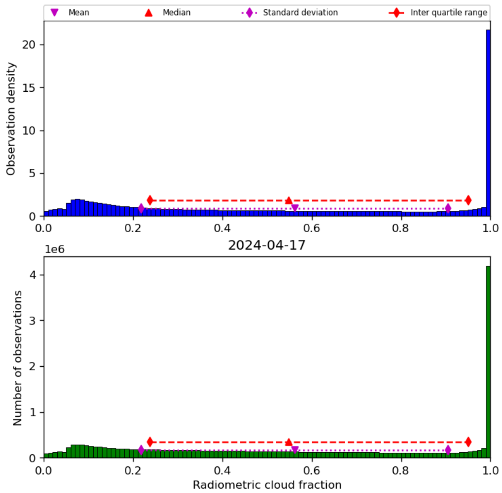
Figure 39: Histogram of “Radiometric cloud fraction” for 2024-04-16 to 2024-04-18
