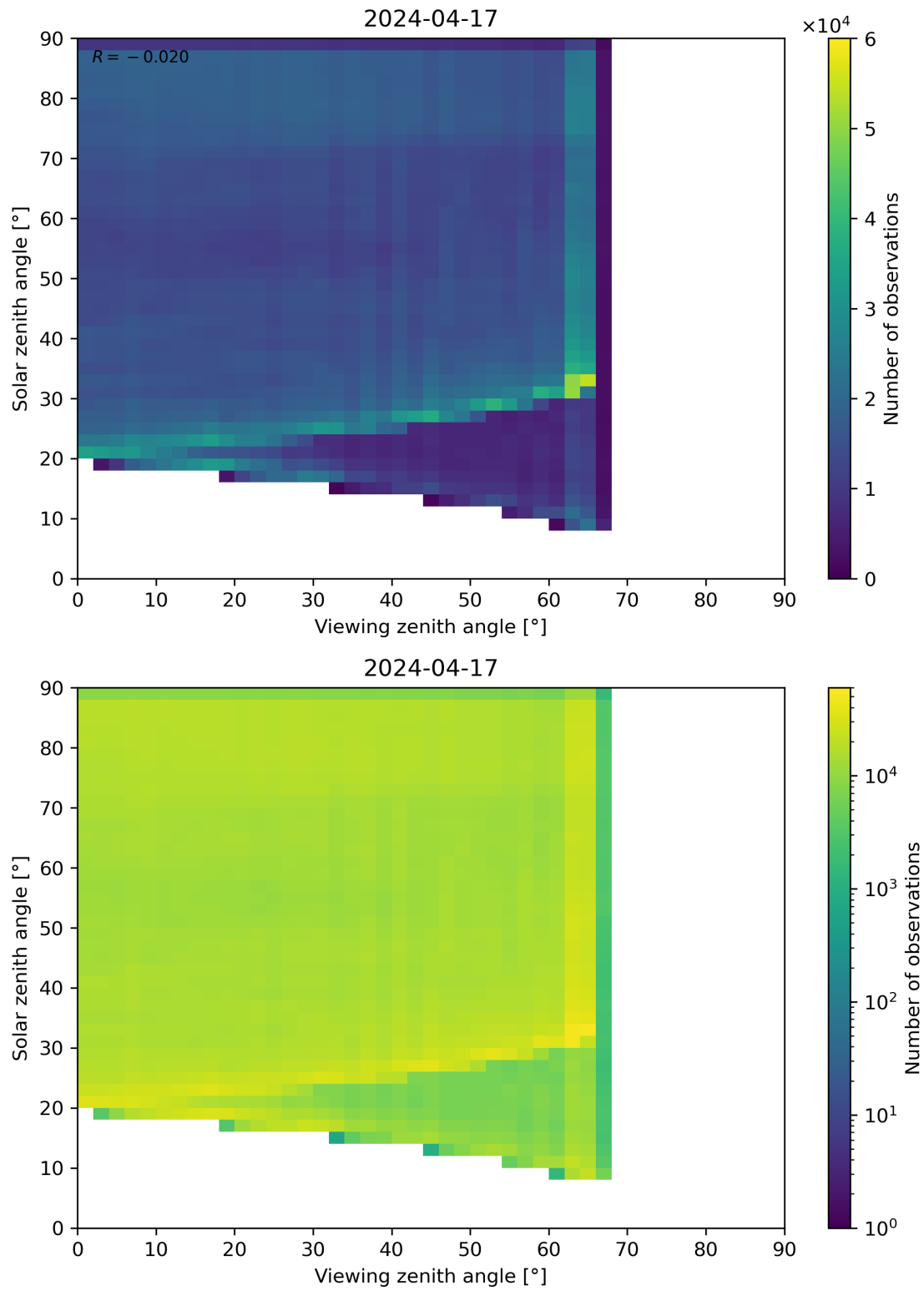
Figure 114: Scatter density plot of “Viewing zenith angle” against “Solar zenith angle” for 2024-04-16 to 2024-04-18.
