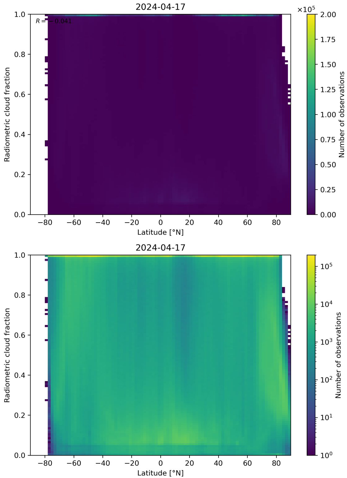
Figure 92: Scatter density plot of “Latitude” against “Radiometric cloud fraction” for 2024-04-16 to 2024-04-18.
