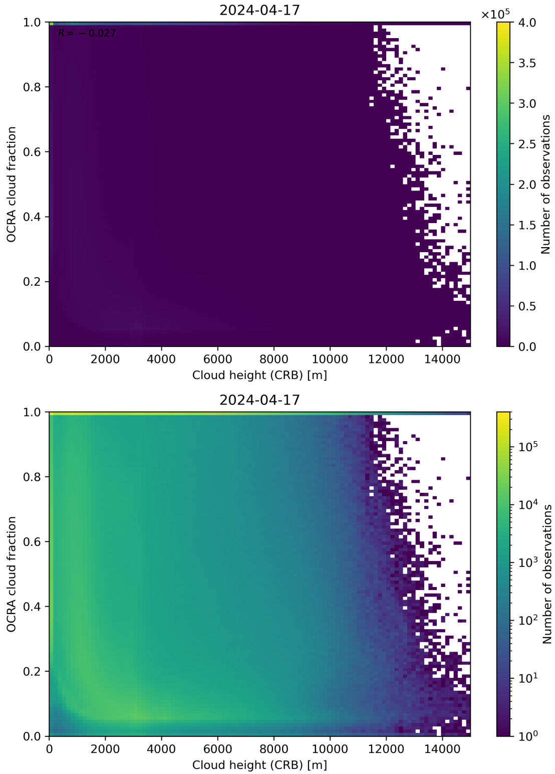
Figure 81: Scatter density plot of “Cloud height (CRB)” against “OCRA cloud fraction” for 2024-04-16 to 2024-04-18.
