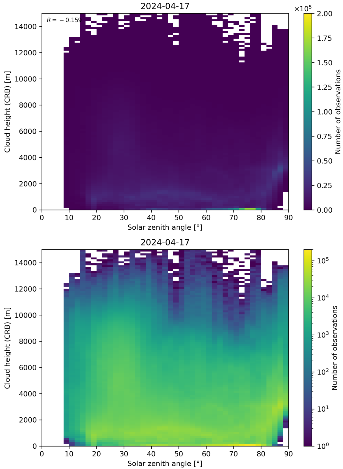
Figure 102: Scatter density plot of “Solar zenith angle” against “Cloud height (CRB)” for 2024-04-16 to 2024-04-18.
