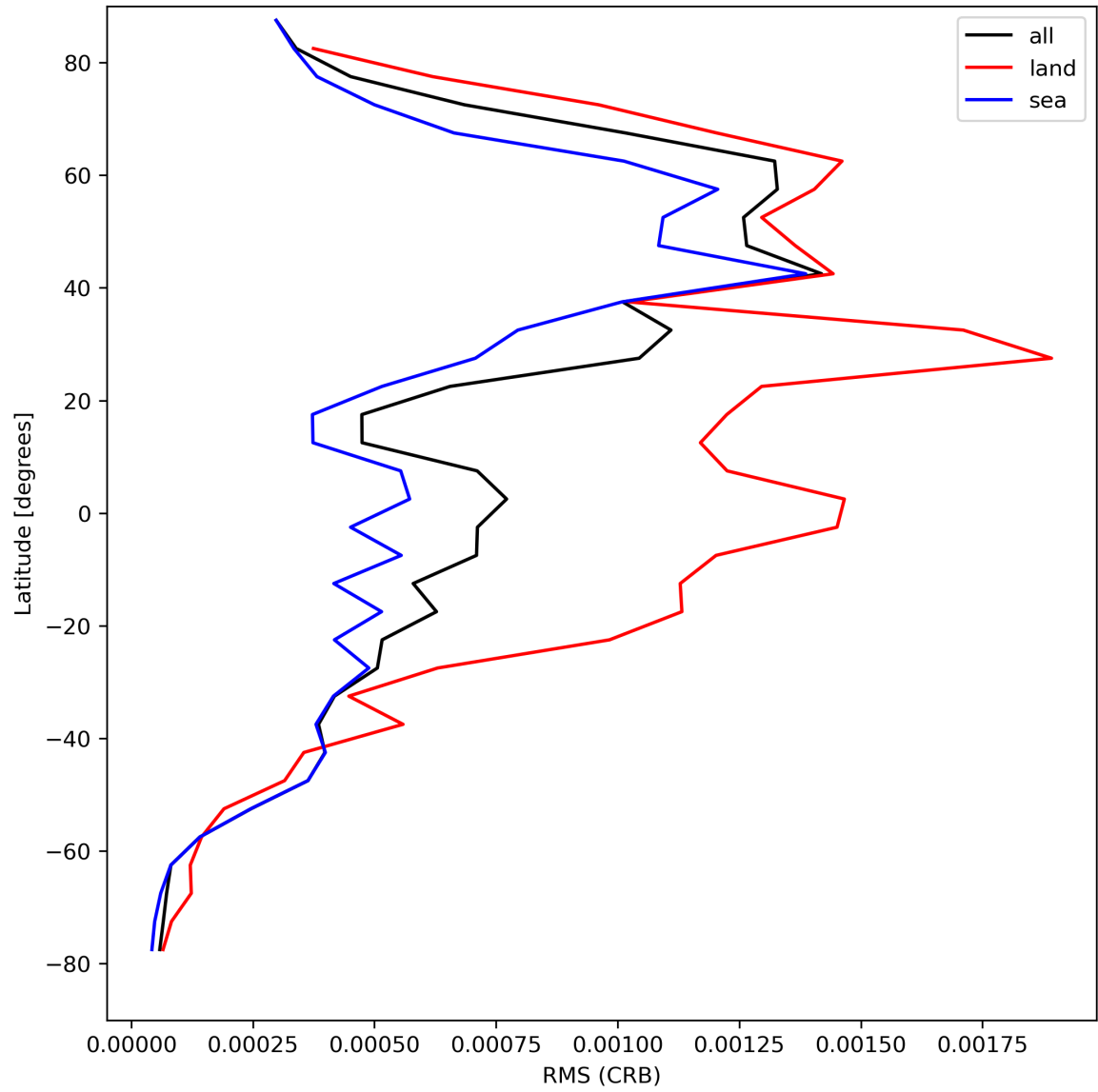
Figure 32: Zonal average of “RMS (CRB)” for 2024-04-16 to 2024-04-18.
