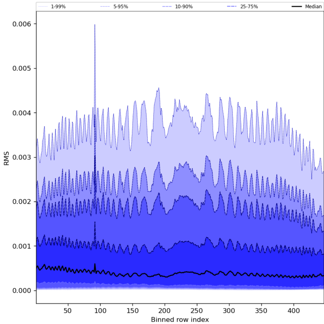
Figure 63: Along track statistics of “RMS” for 2024-04-16 to 2024-04-18
