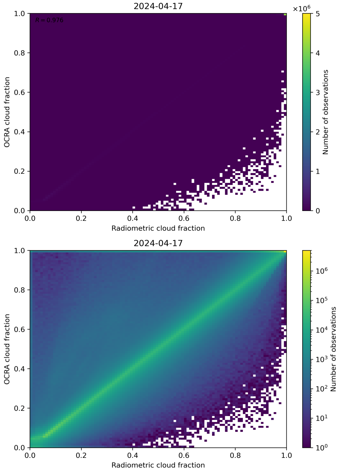
Figure 72: Scatter density plot of “Radiometric cloud fraction” against “OCRA cloud fraction” for 2024-04-16 to 2024-04-18.
