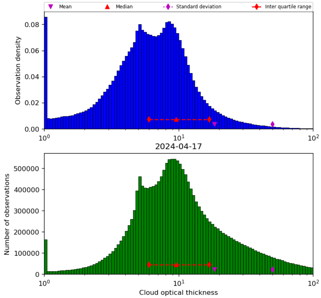
Figure 41: Histogram of “Cloud optical thickness” for 2024-04-16 to 2024-04-18
