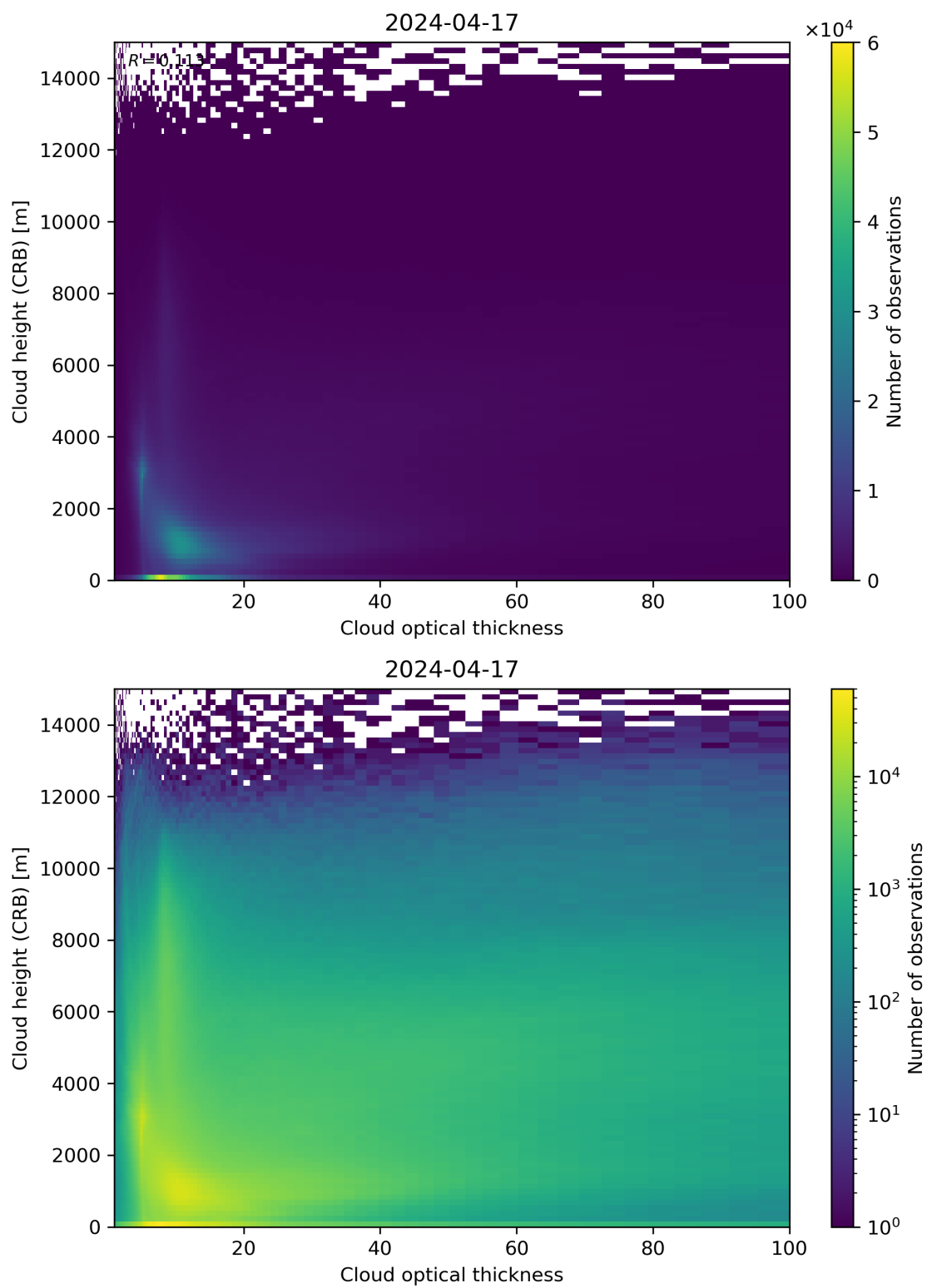
Figure 85: Scatter density plot of “Cloud optical thickness” against “Cloud height (CRB)” for 2024-04-16 to 2024-04-18.
