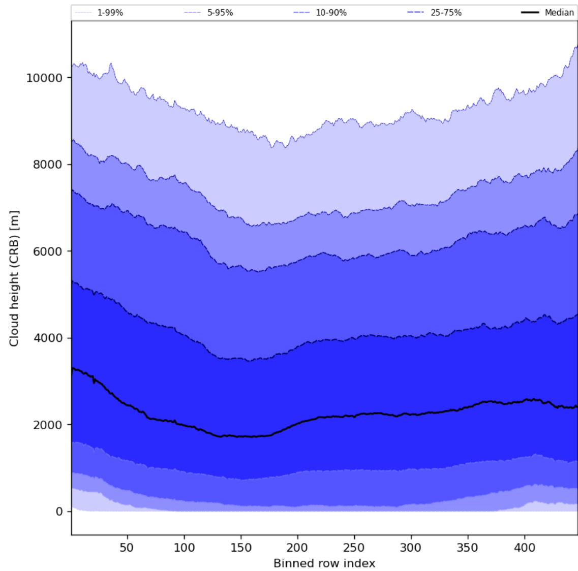
Figure 59: Along track statistics of “Cloud height (CRB)” for 2024-04-16 to 2024-04-18
