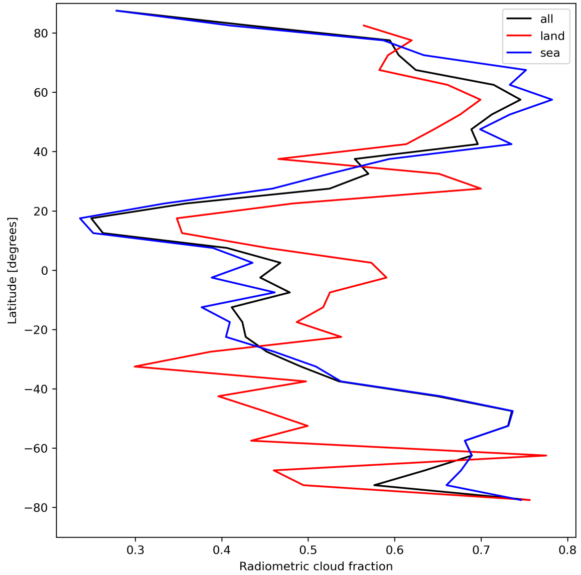
Figure 23: Zonal average of “Radiometric cloud fraction” for 2024-04-16 to 2024-04-18.
