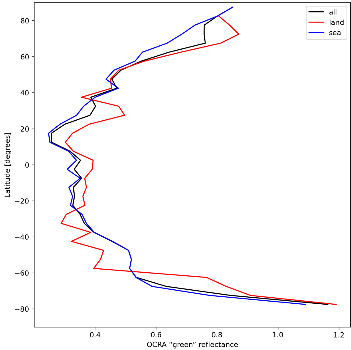
Figure 36: Zonal average of “OCRA “green” reflectance” for 2024-04-16 to 2024-04-18.
