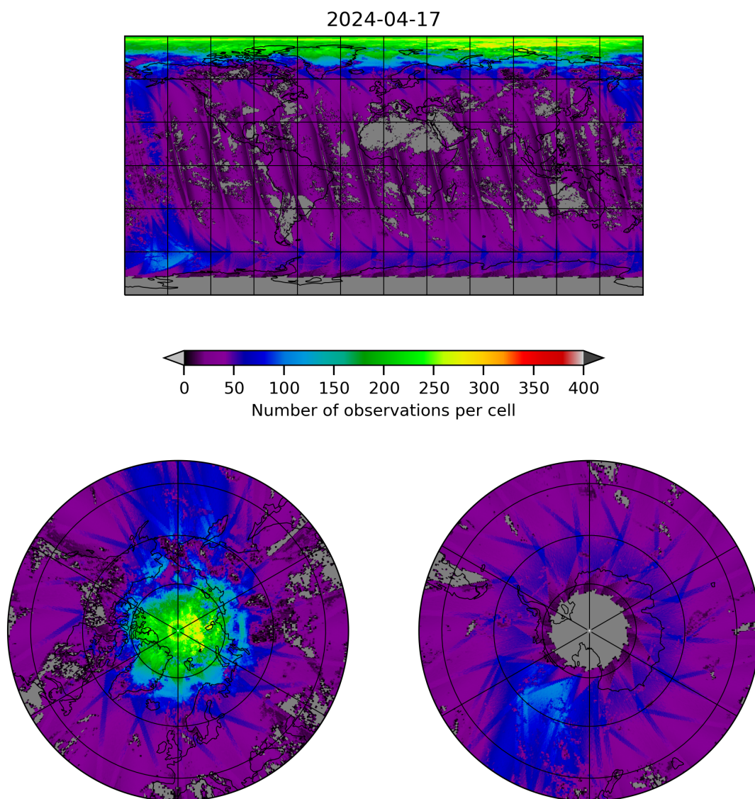
Figure 21: Map of the number of observations for 2024-04-16 to 2024-04-18
