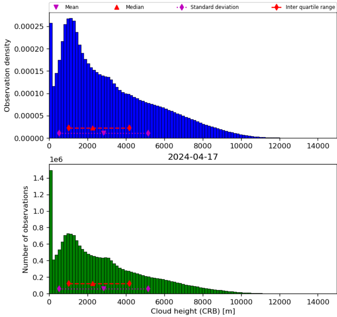
Figure 43: Histogram of “Cloud height (CRB)” for 2024-04-16 to 2024-04-18
