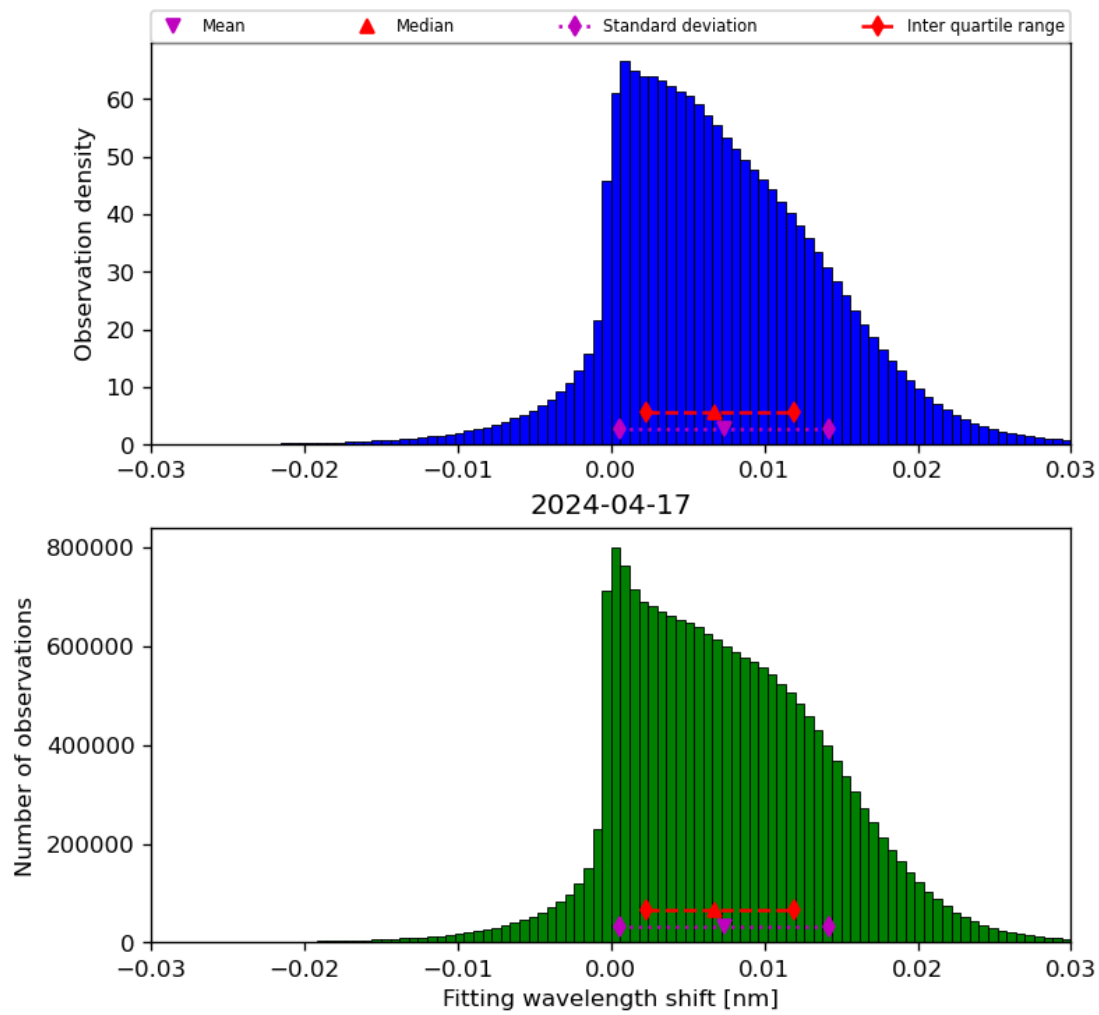
Figure 49: Histogram of “Fitting wavelength shift” for 2024-04-16 to 2024-04-18
