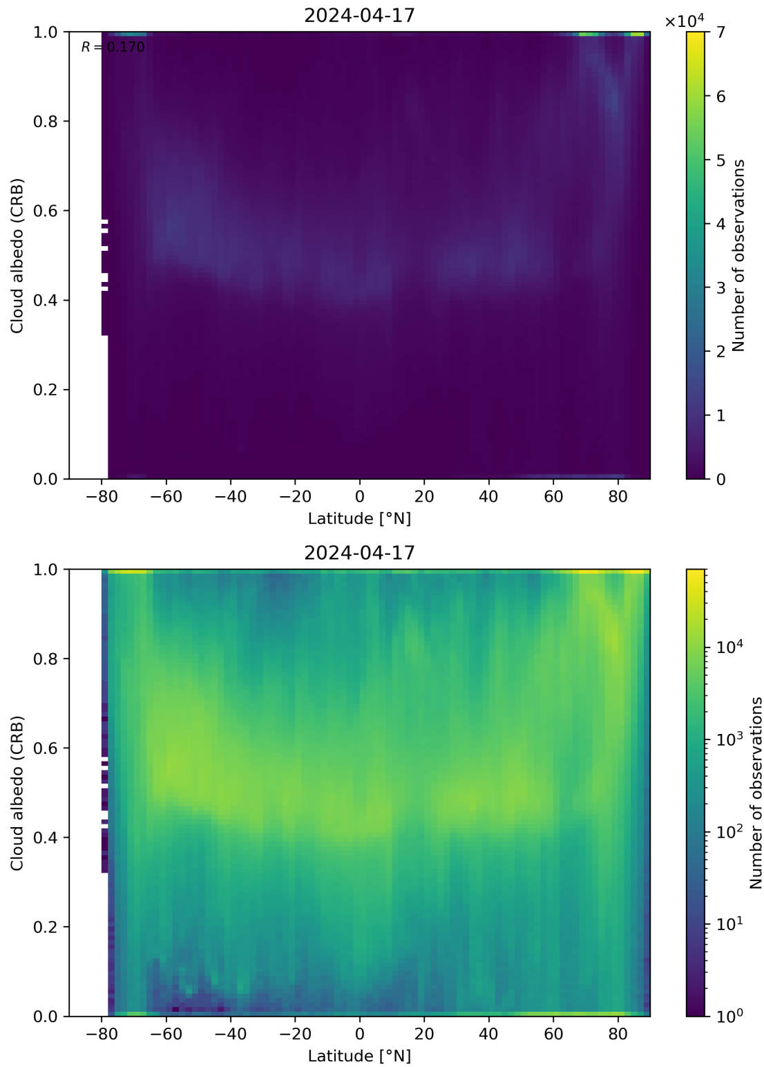
Figure 91: Scatter density plot of “Latitude” against “Cloud albedo (CRB)” for 2024-04-16 to 2024-04-18.
