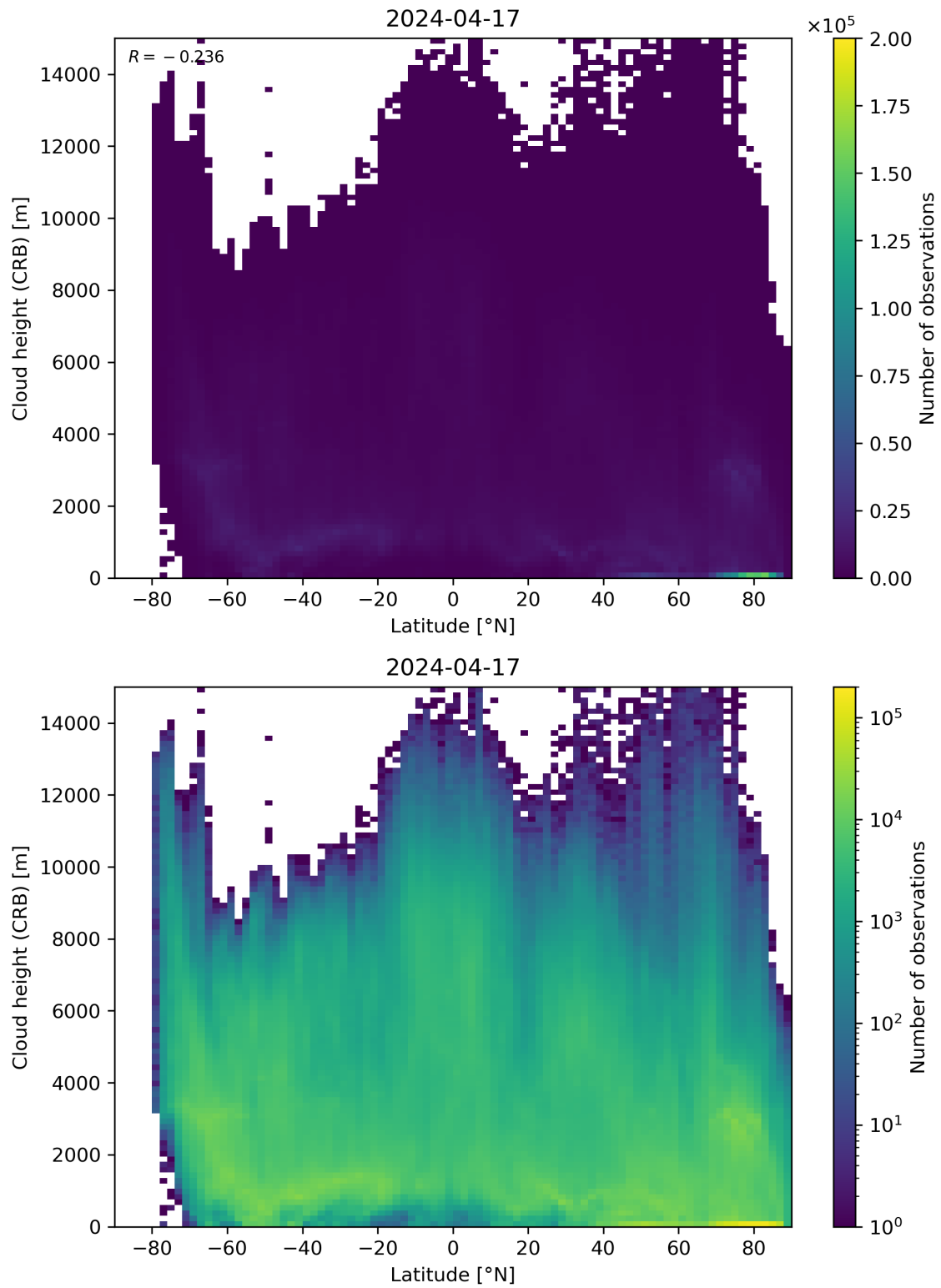
Figure 95: Scatter density plot of “Latitude” against “Cloud height (CRB)” for 2024-04-16 to 2024-04-18.
