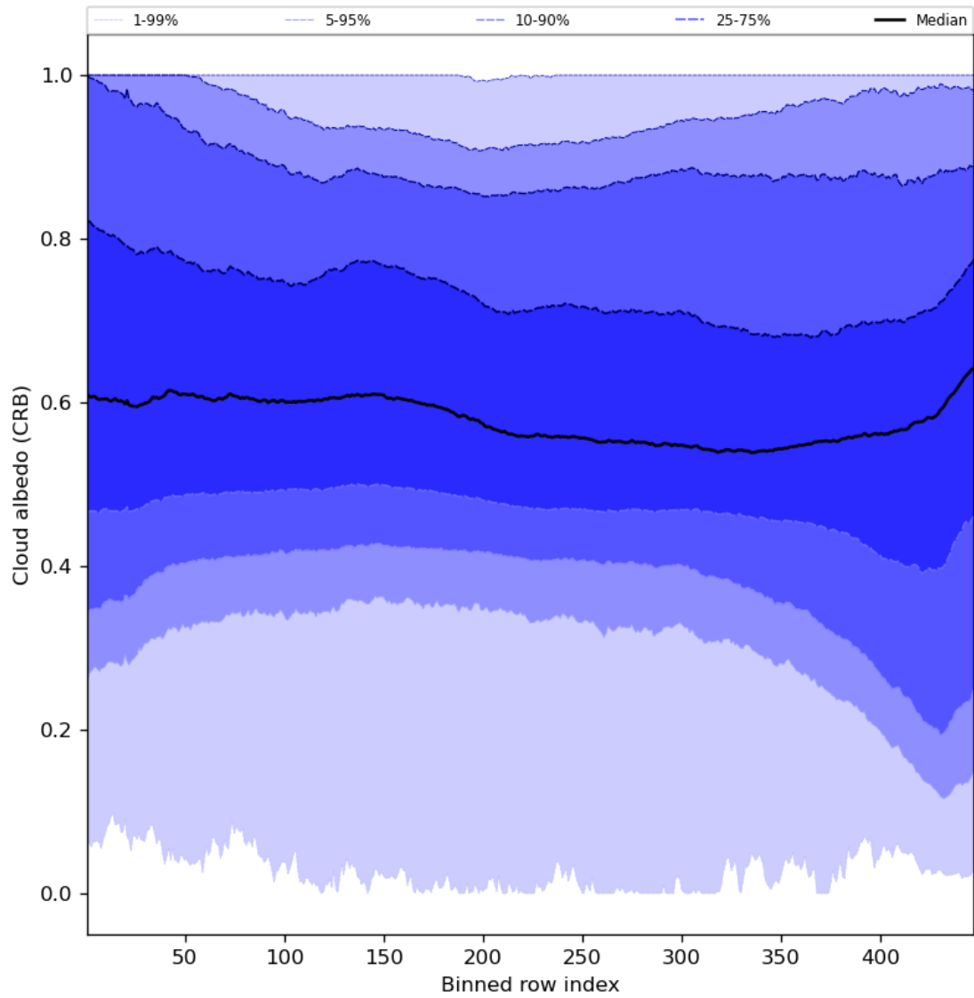
Figure 60: Along track statistics of “Cloud albedo (CRB)” for 2024-04-16 to 2024-04-18
