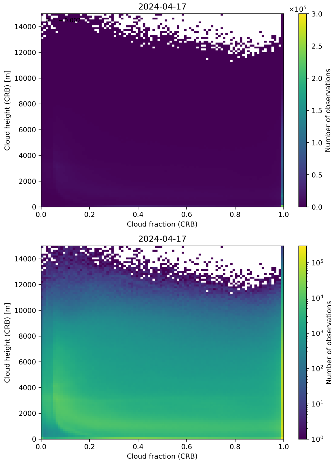
Figure 79: Scatter density plot of “Cloud fraction (CRB)” against “Cloud height (CRB)” for 2024-04-16 to 2024-04-18.
