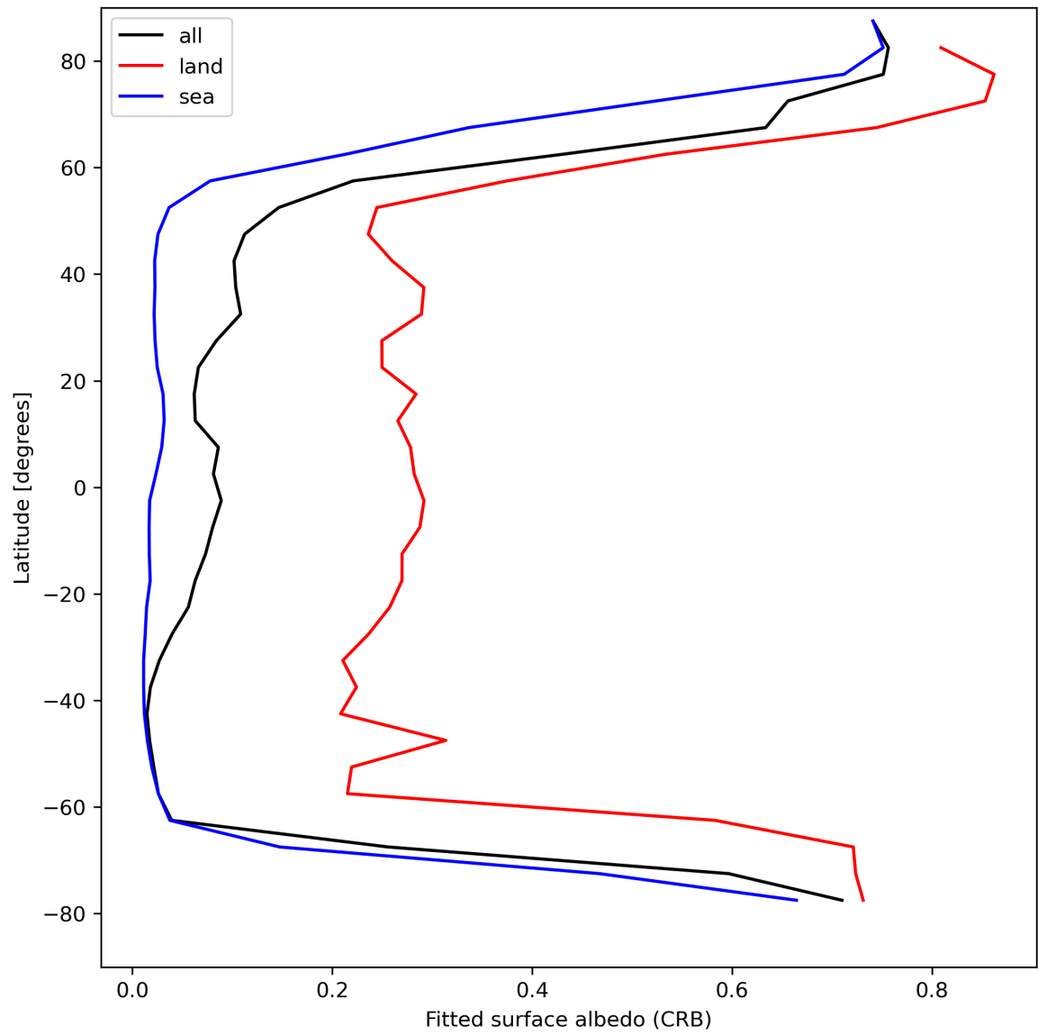
Figure 30: Zonal average of “Fitted surface albedo (CRB)” for 2024-04-16 to 2024-04-18.
