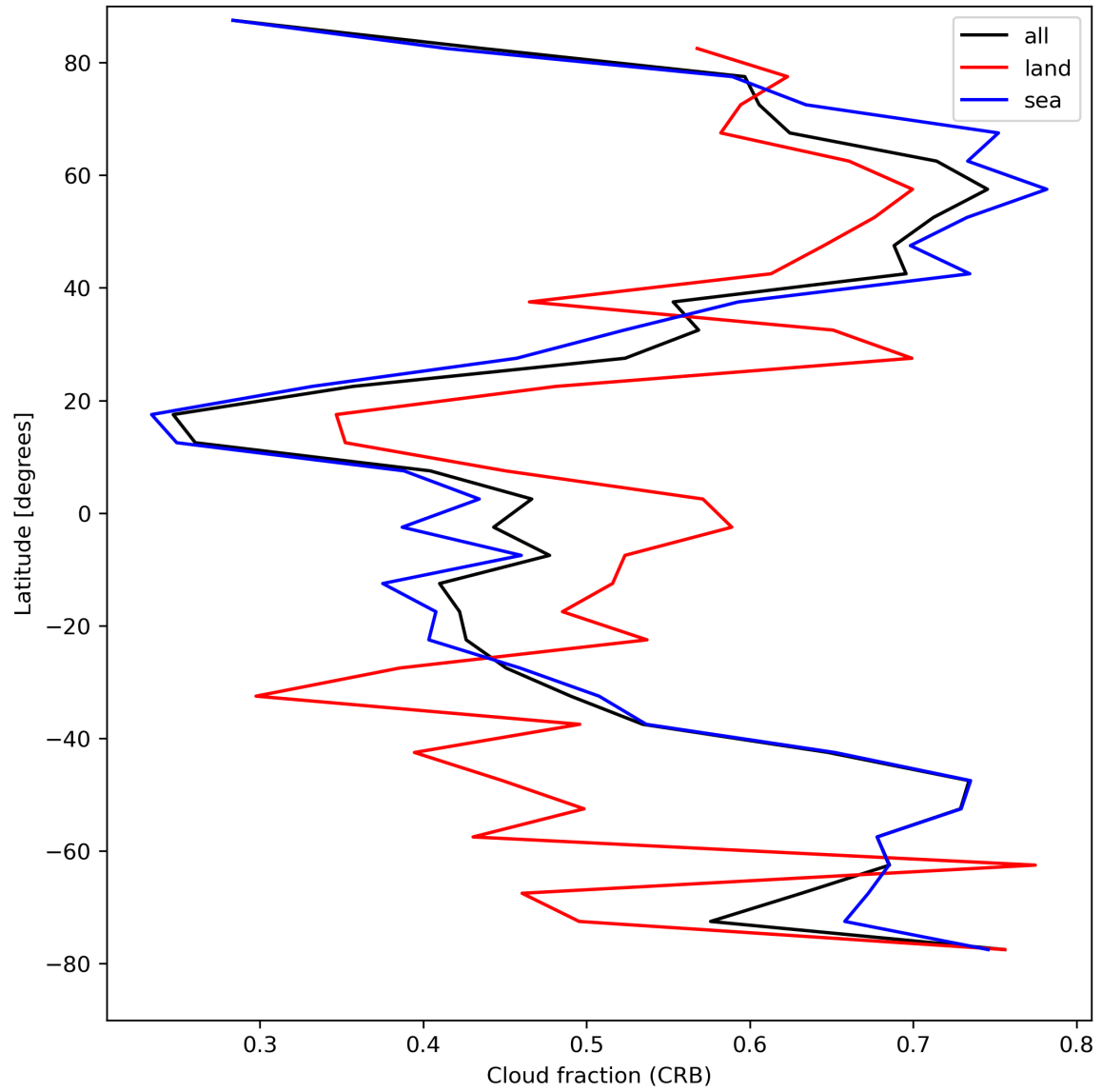
Figure 26: Zonal average of “Cloud fraction (CRB)” for 2024-04-16 to 2024-04-18.
