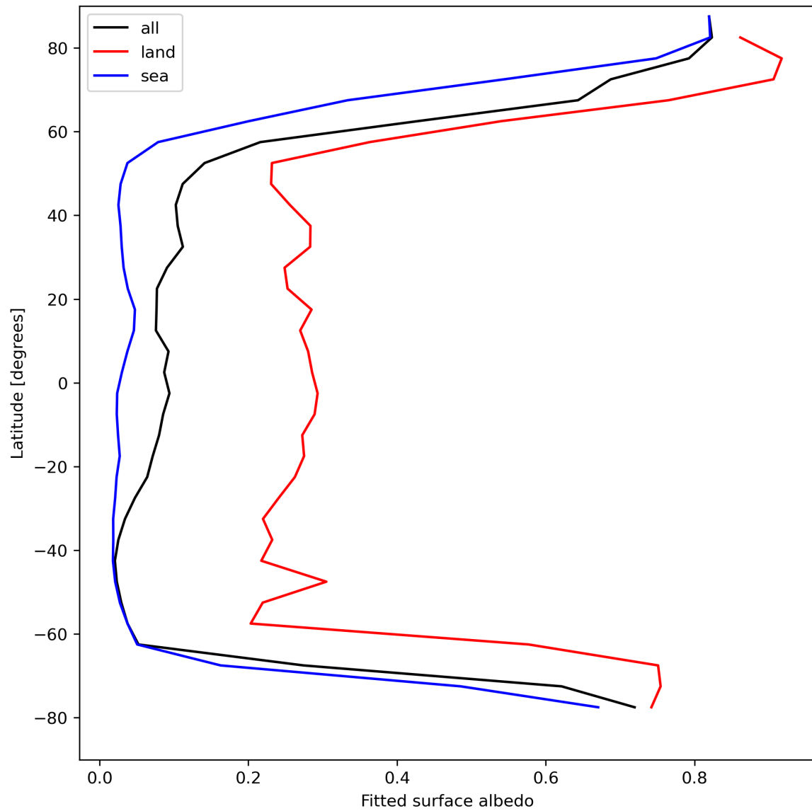
Figure 29: Zonal average of “Fitted surface albedo” for 2024-04-16 to 2024-04-18.
