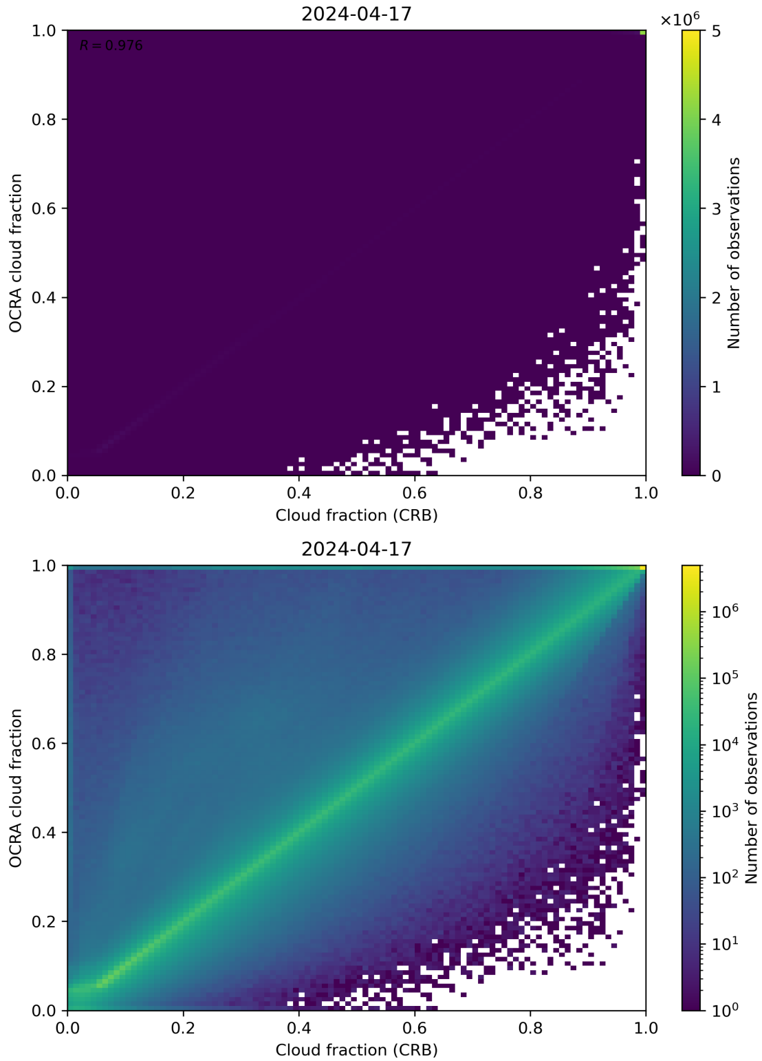
Figure 78: Scatter density plot of “Cloud fraction (CRB)” against “OCRA cloud fraction” for 2024-04-16 to 2024-04-18.
