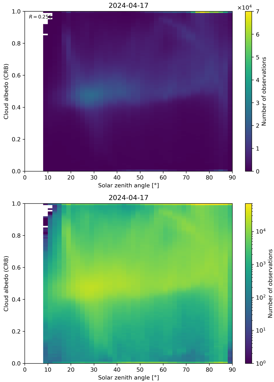
Figure 98: Scatter density plot of “Solar zenith angle” against “Cloud albedo (CRB)” for 2024-04-16 to 2024-04-18.
