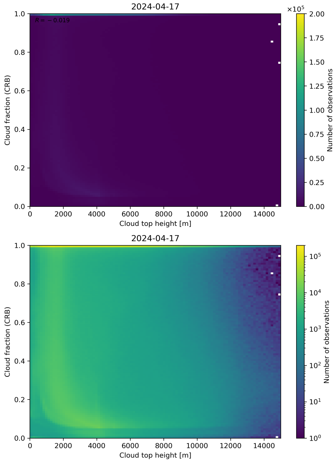
Figure 88: Scatter density plot of “Cloud top height” against “Cloud fraction (CRB)” for 2024-04-16 to 2024-04-18.
