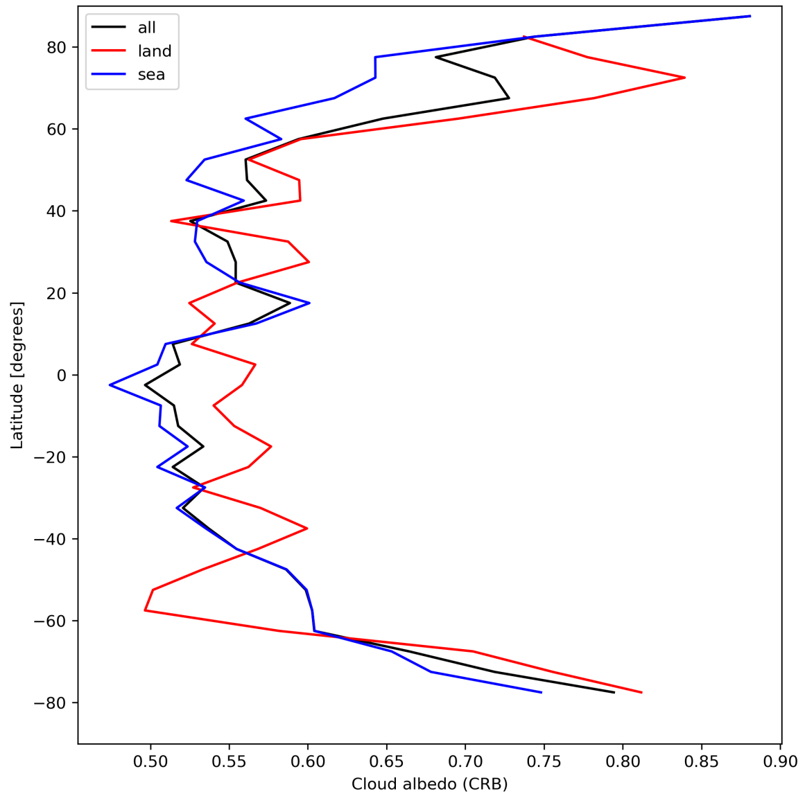
Figure 28: Zonal average of “Cloud albedo (CRB)” for 2024-04-16 to 2024-04-18.
