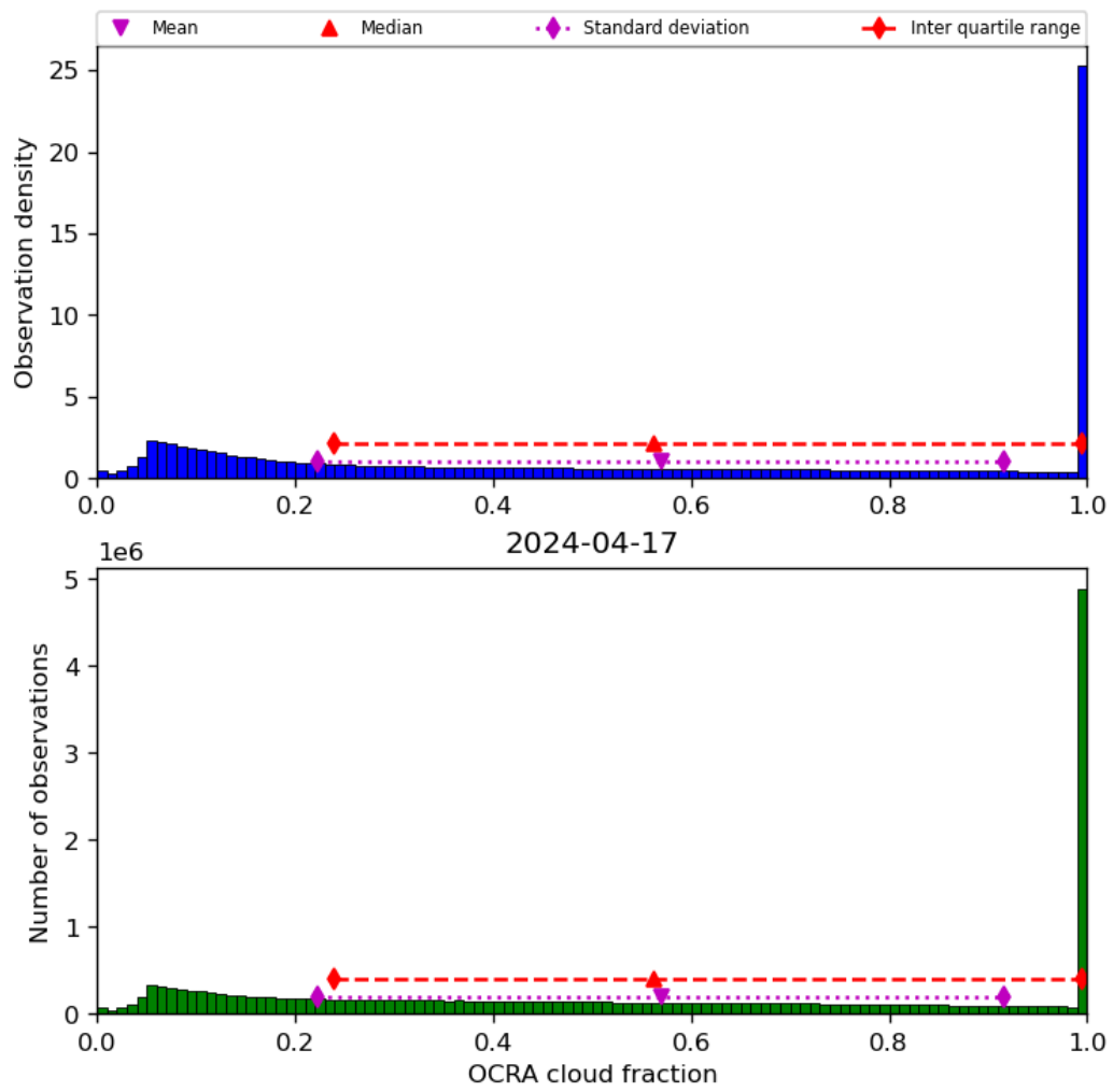
Figure 50: Histogram of “OCRA cloud fraction” for 2024-04-16 to 2024-04-18
