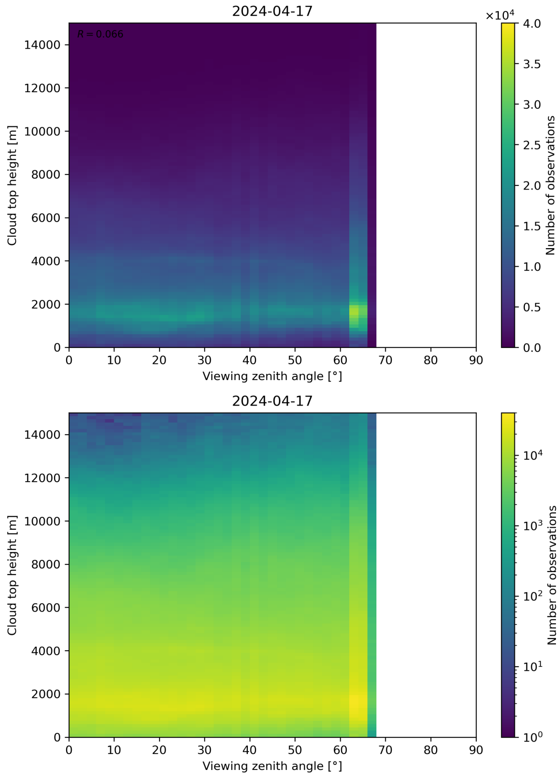
Figure 112: Scatter density plot of “Viewing zenith angle” against “Cloud top height” for 2024-04-16 to 2024-04-18.
