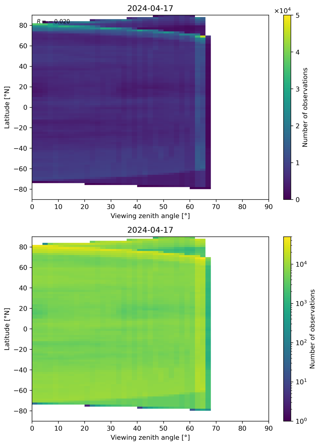
Figure 113: Scatter density plot of “Viewing zenith angle” against “Latitude” for 2024-04-16 to 2024-04-18.
