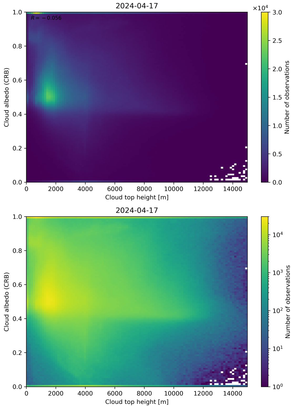
Figure 86: Scatter density plot of “Cloud top height” against “Cloud albedo (CRB)” for 2024-04-16 to 2024-04-18.
