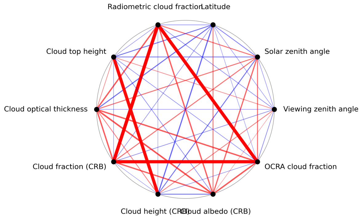
Figure 1: Map of correlation graph for 2024-04-16 to 2024-04-18.
