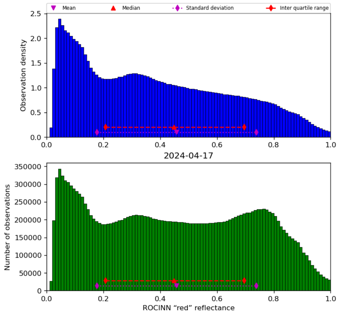
Figure 53: Histogram of “ROCINN “red” reflectance” for 2024-04-16 to 2024-04-18
