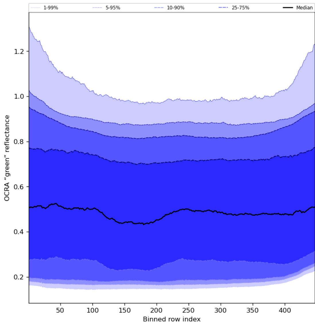
Figure 68: Along track statistics of “OCRA “green” reflectance” for 2024-04-16 to 2024-04-18
