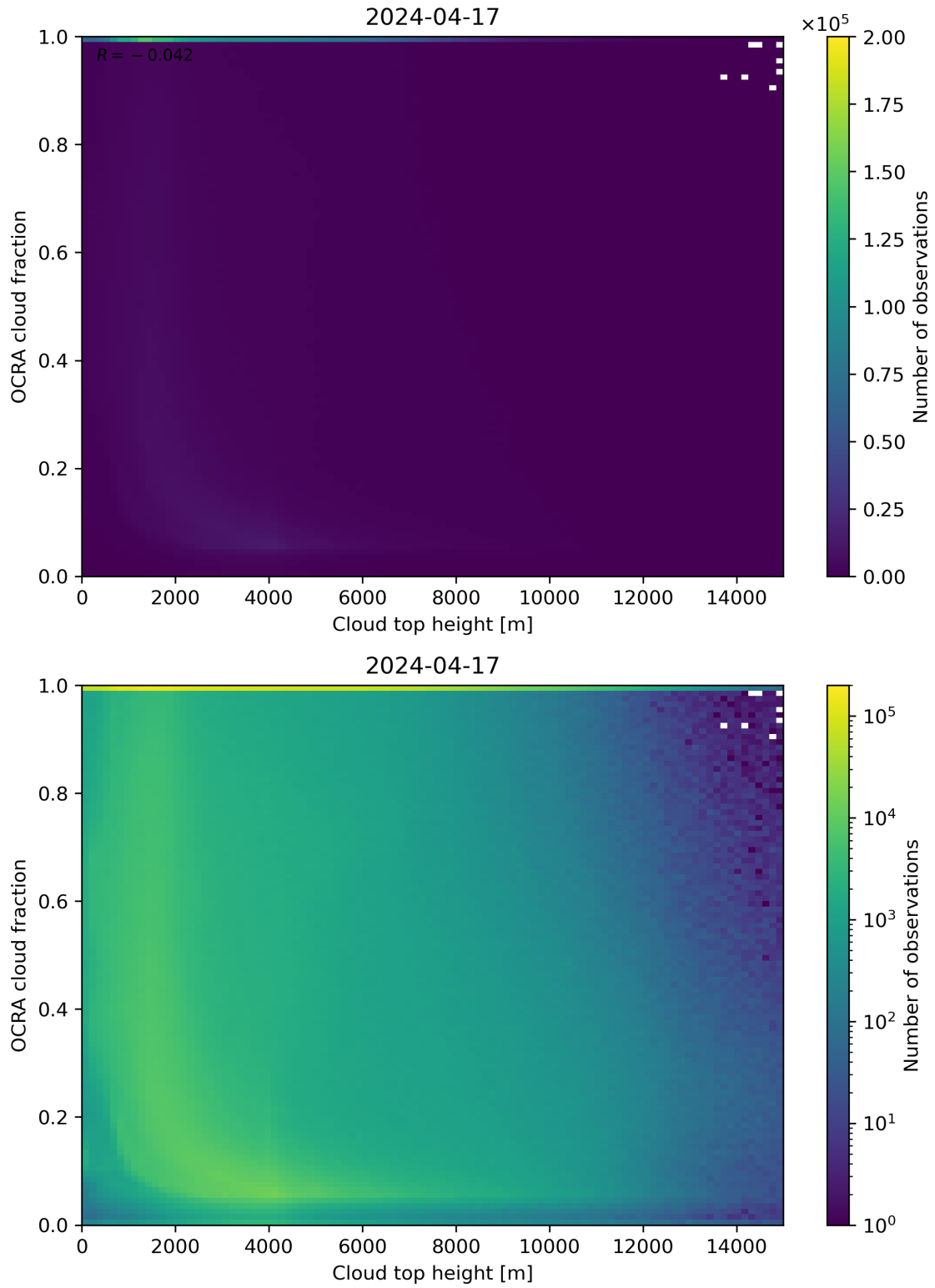
Figure 87: Scatter density plot of “Cloud top height” against “OCRA cloud fraction” for 2024-04-16 to 2024-04-18.
