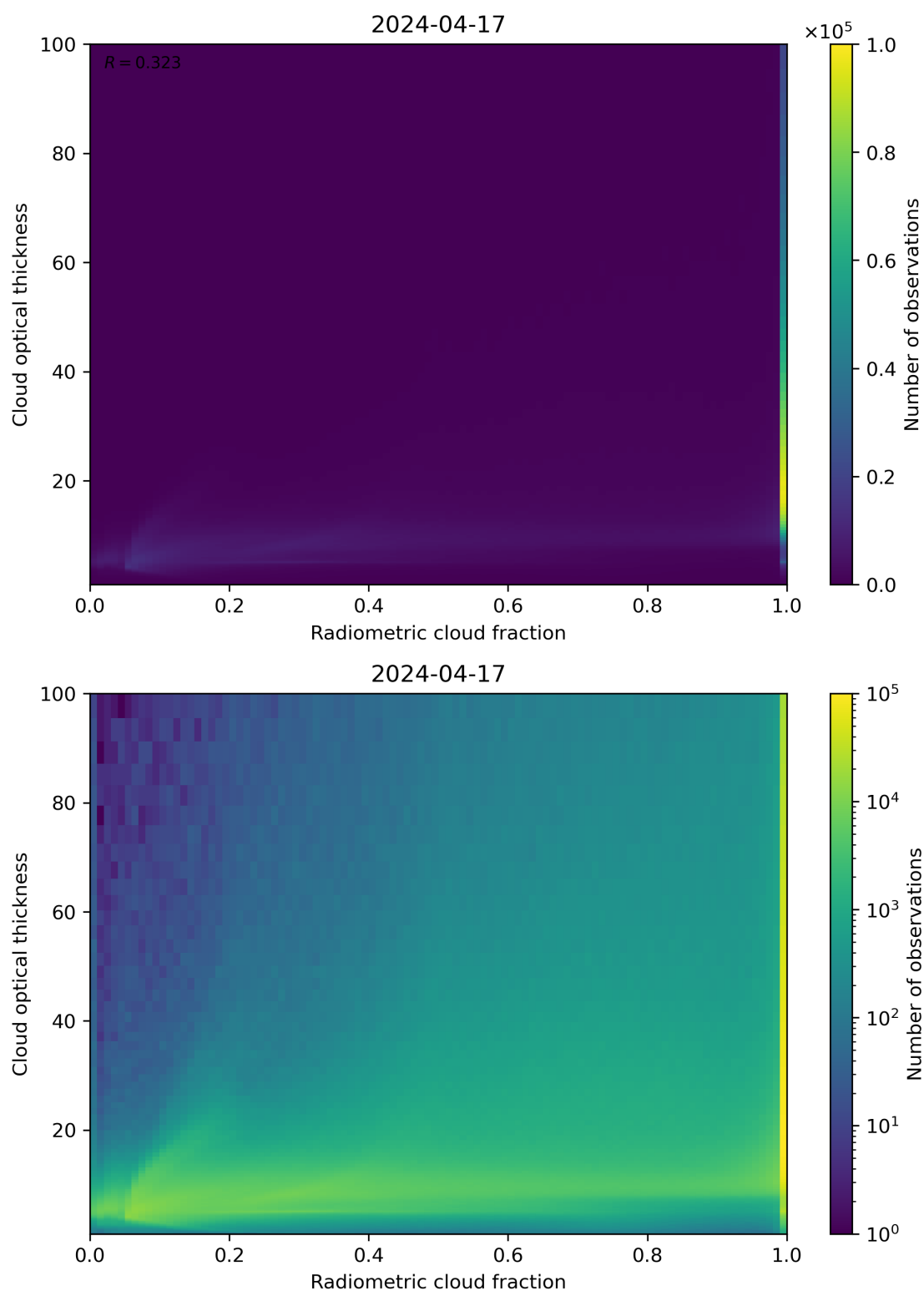
Figure 75: Scatter density plot of “Radiometric cloud fraction” against “Cloud optical thickness” for 2024-04-16 to 2024-04-18.
