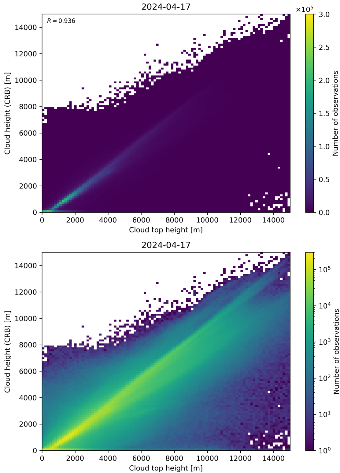
Figure 89: Scatter density plot of “Cloud top height” against “Cloud height (CRB)” for 2024-04-16 to 2024-04-18.
