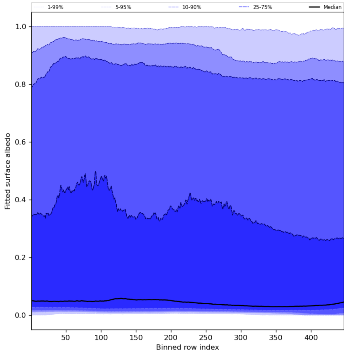
Figure 61: Along track statistics of “Fitted surface albedo” for 2024-04-16 to 2024-04-18
