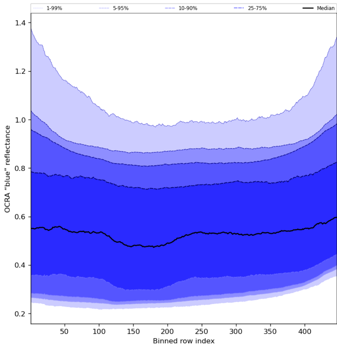
Figure 67: Along track statistics of “OCRA “blue” reflectance” for 2024-04-16 to 2024-04-18
