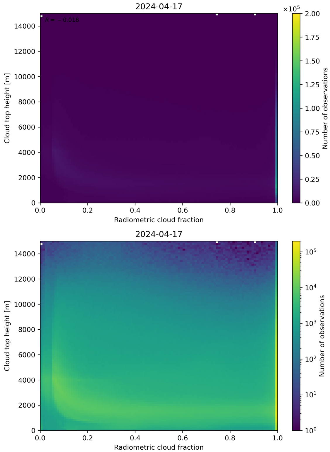
Figure 76: Scatter density plot of “Radiometric cloud fraction” against “Cloud top height” for 2024-04-16 to 2024-04-18.
