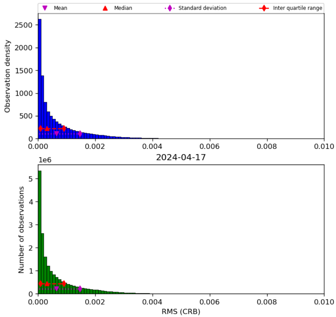
Figure 48: Histogram of “RMS (CRB)” for 2024-04-16 to 2024-04-18
