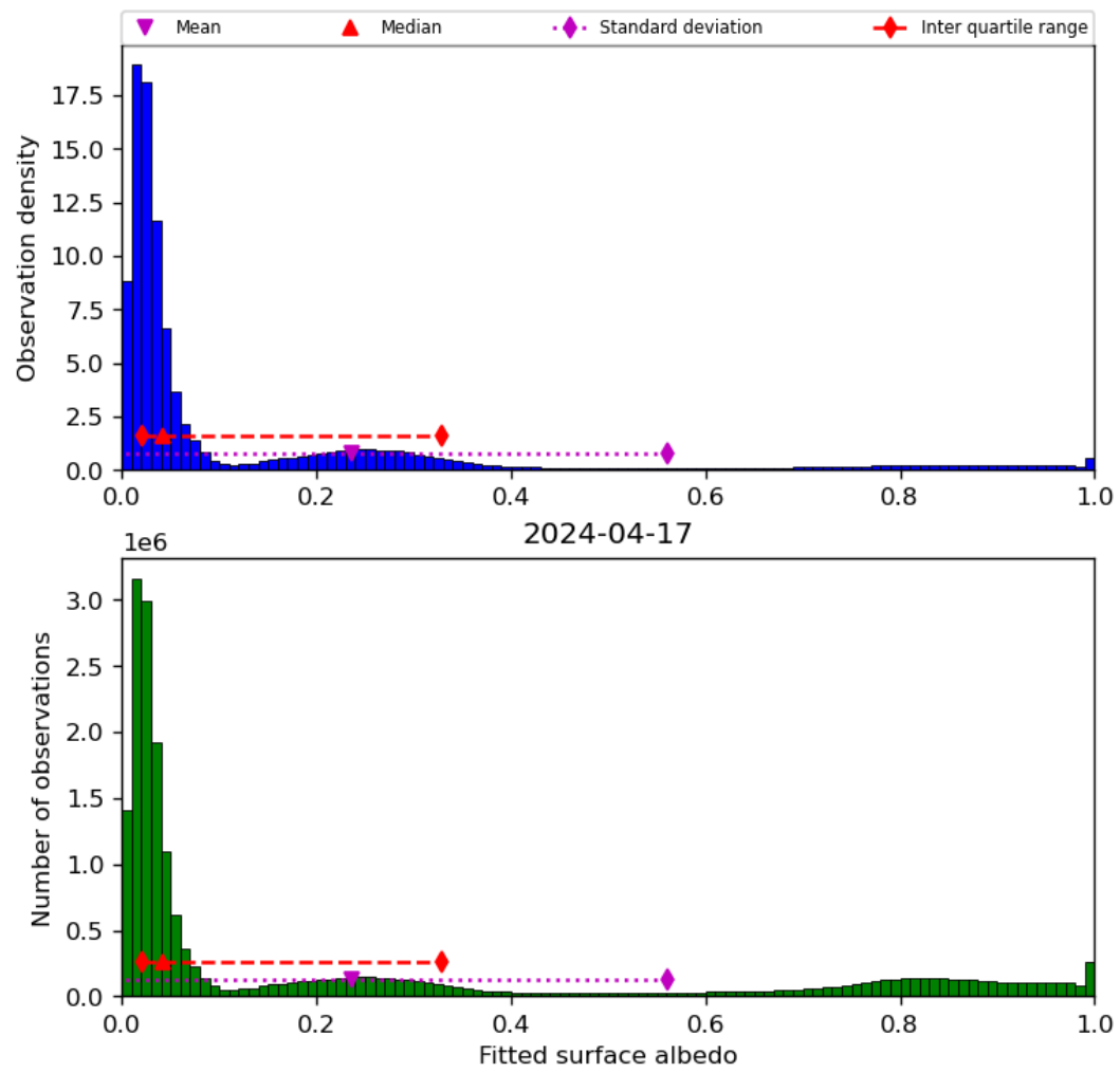
Figure 45: Histogram of “Fitted surface albedo” for 2024-04-16 to 2024-04-18
