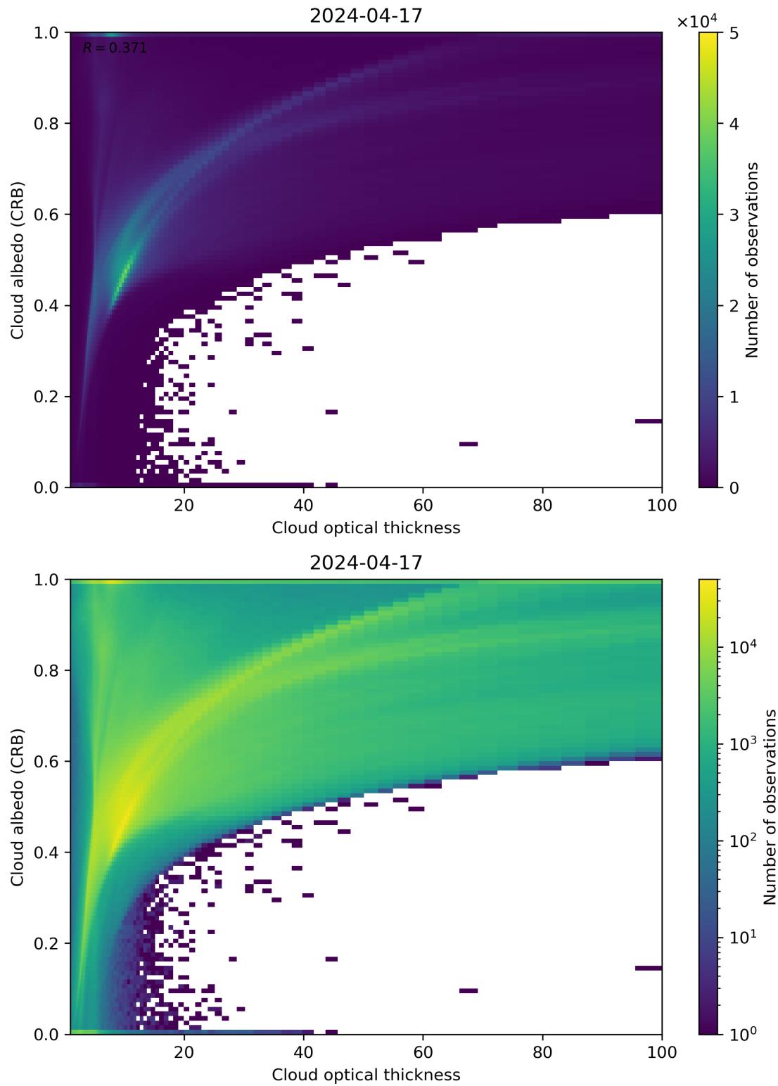
Figure 82: Scatter density plot of “Cloud optical thickness” against “Cloud albedo (CRB)” for 2024-04-16 to 2024-04-18.
