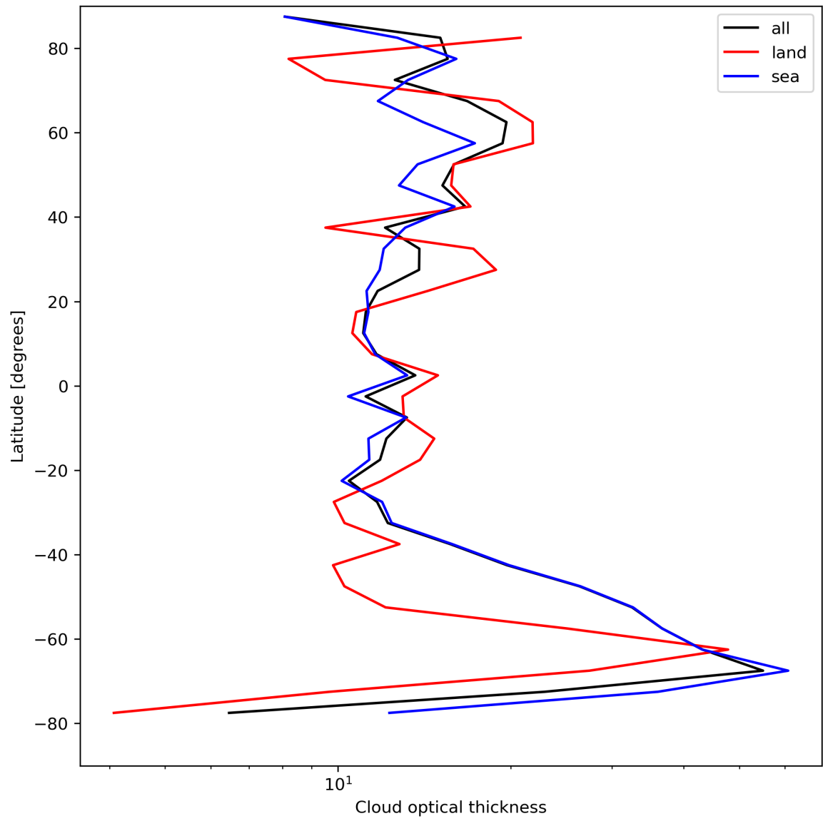
Figure 25: Zonal average of “Cloud optical thickness” for 2024-04-16 to 2024-04-18.
