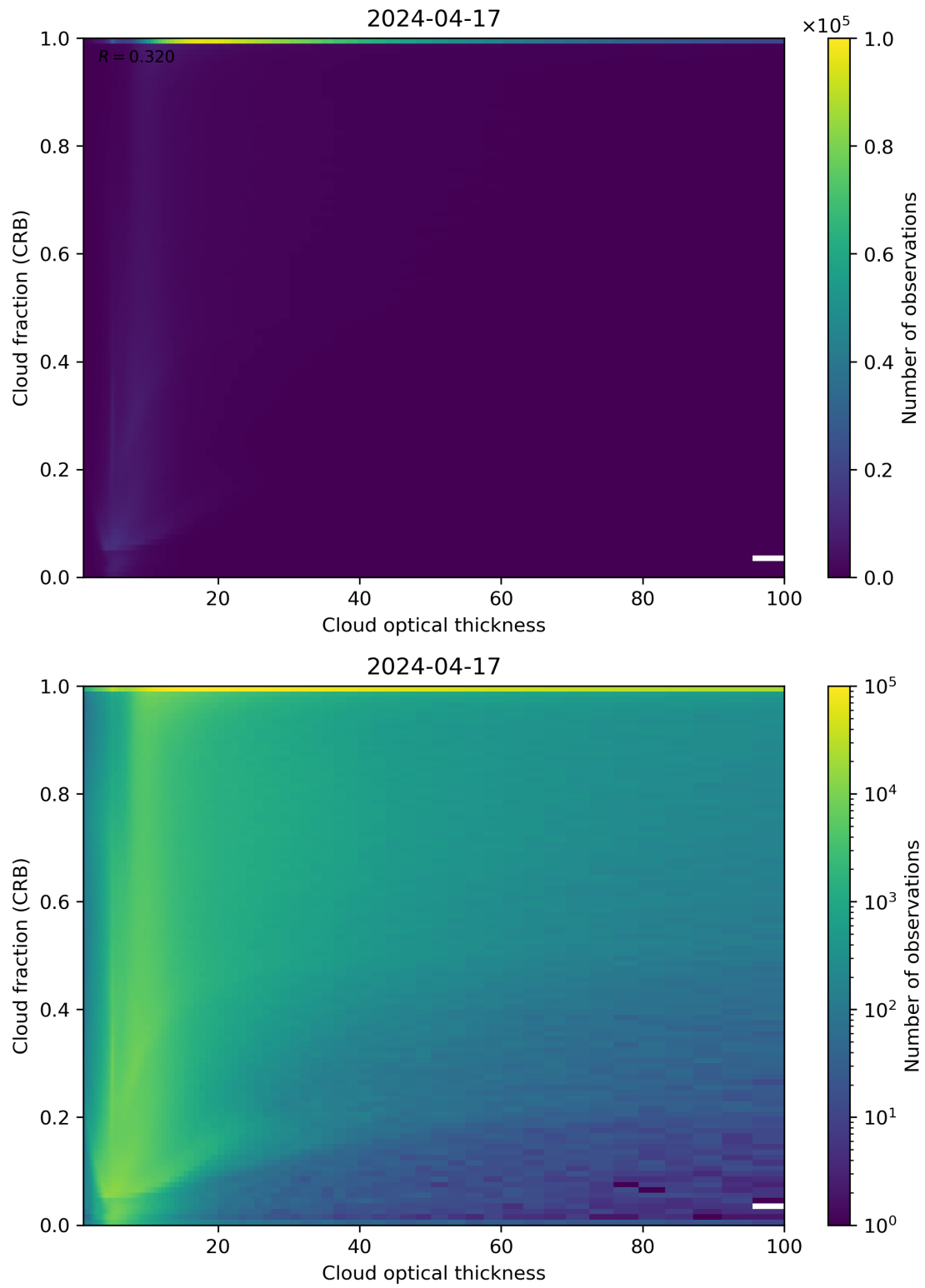
Figure 84: Scatter density plot of “Cloud optical thickness” against “Cloud fraction (CRB)” for 2024-04-16 to 2024-04-18.
