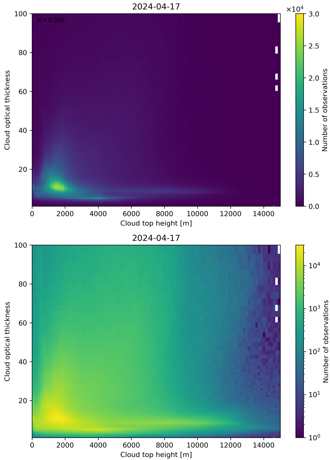
Figure 90: Scatter density plot of “Cloud top height” against “Cloud optical thickness” for 2024-04-16 to 2024-04-18.
