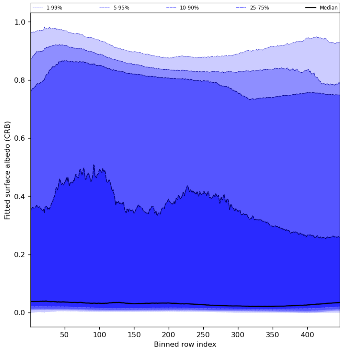
Figure 62: Along track statistics of “Fitted surface albedo (CRB)” for 2024-04-16 to 2024-04-18
