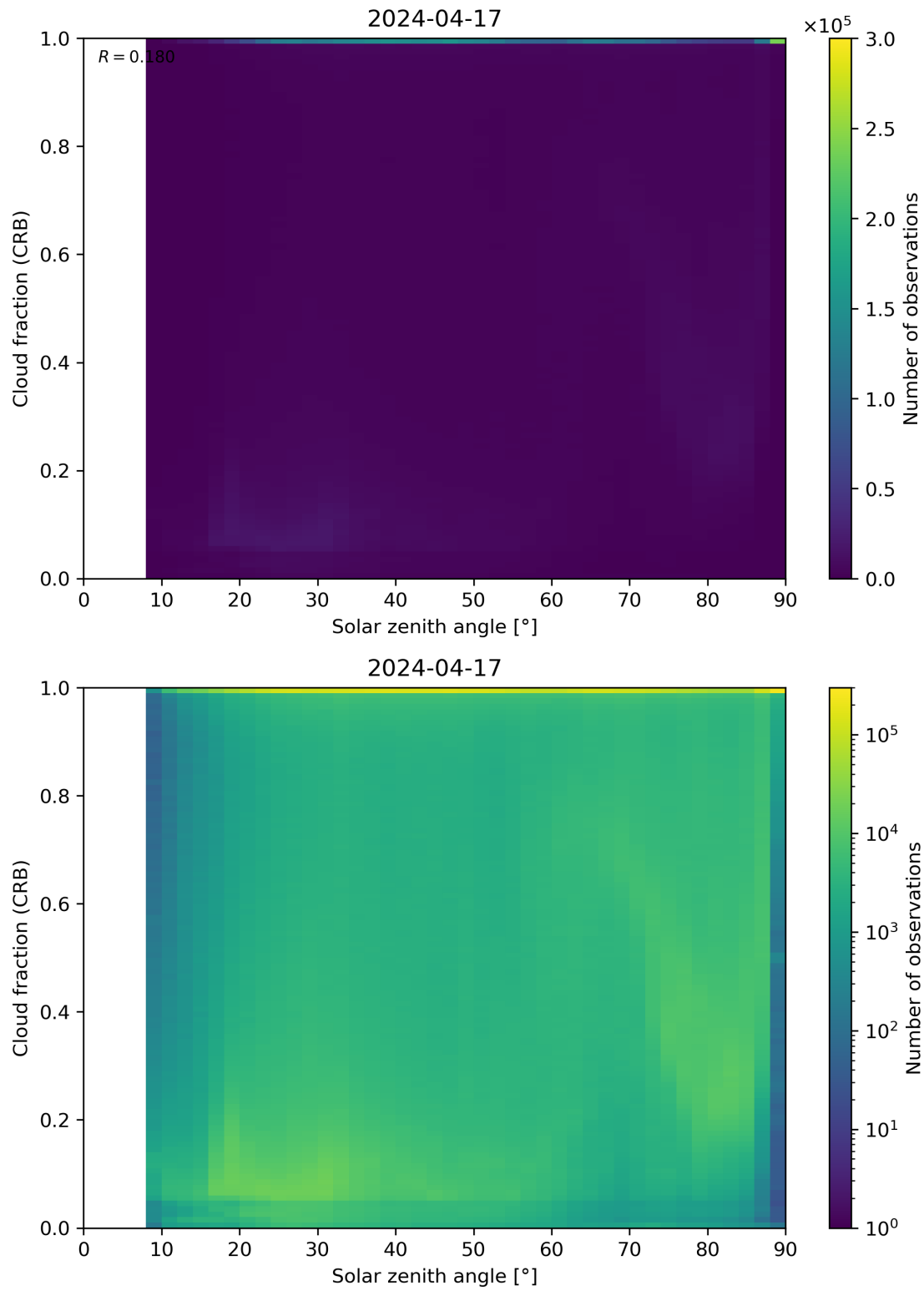
Figure 101: Scatter density plot of “Solar zenith angle” against “Cloud fraction (CRB)” for 2024-04-16 to 2024-04-18.
