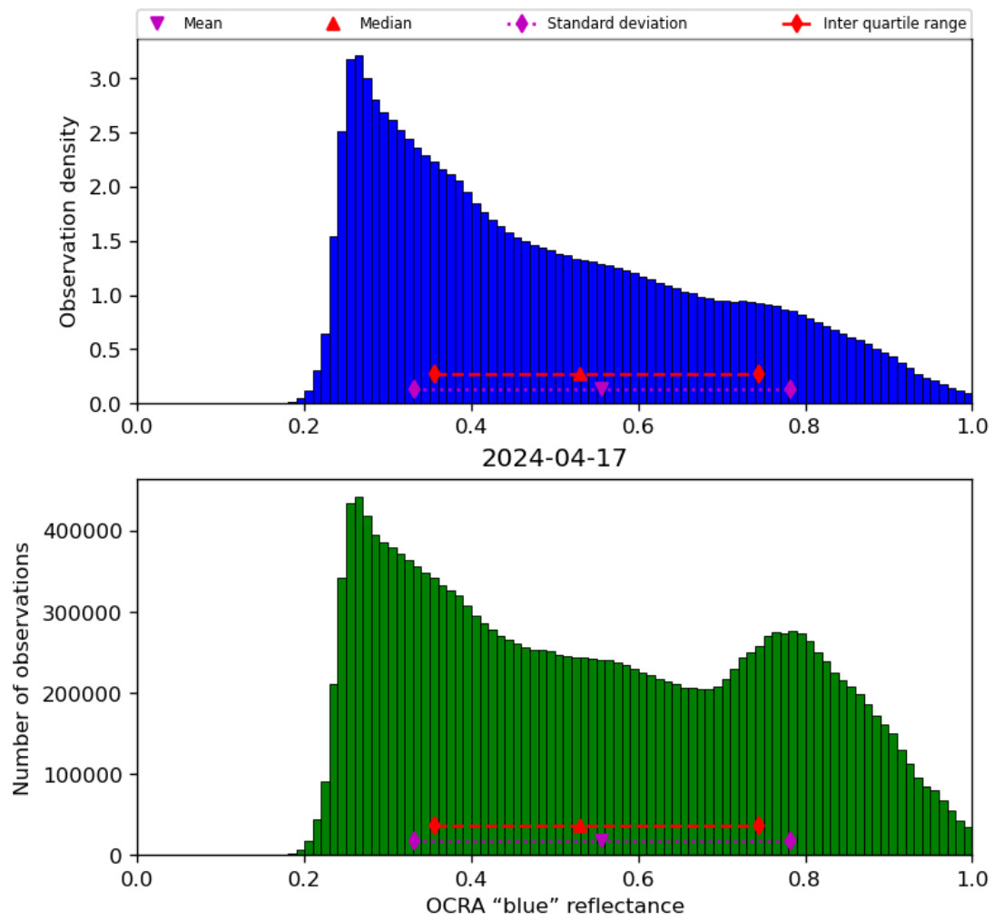
Figure 51: Histogram of “OCRA “blue” reflectance” for 2024-04-16 to 2024-04-18
