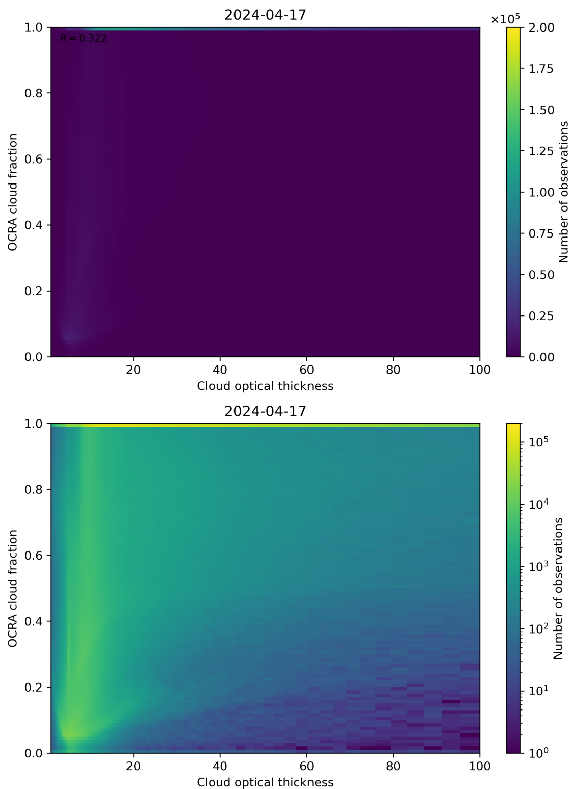
Figure 83: Scatter density plot of “Cloud optical thickness” against “OCRA cloud fraction” for 2024-04-16 to 2024-04-18.
