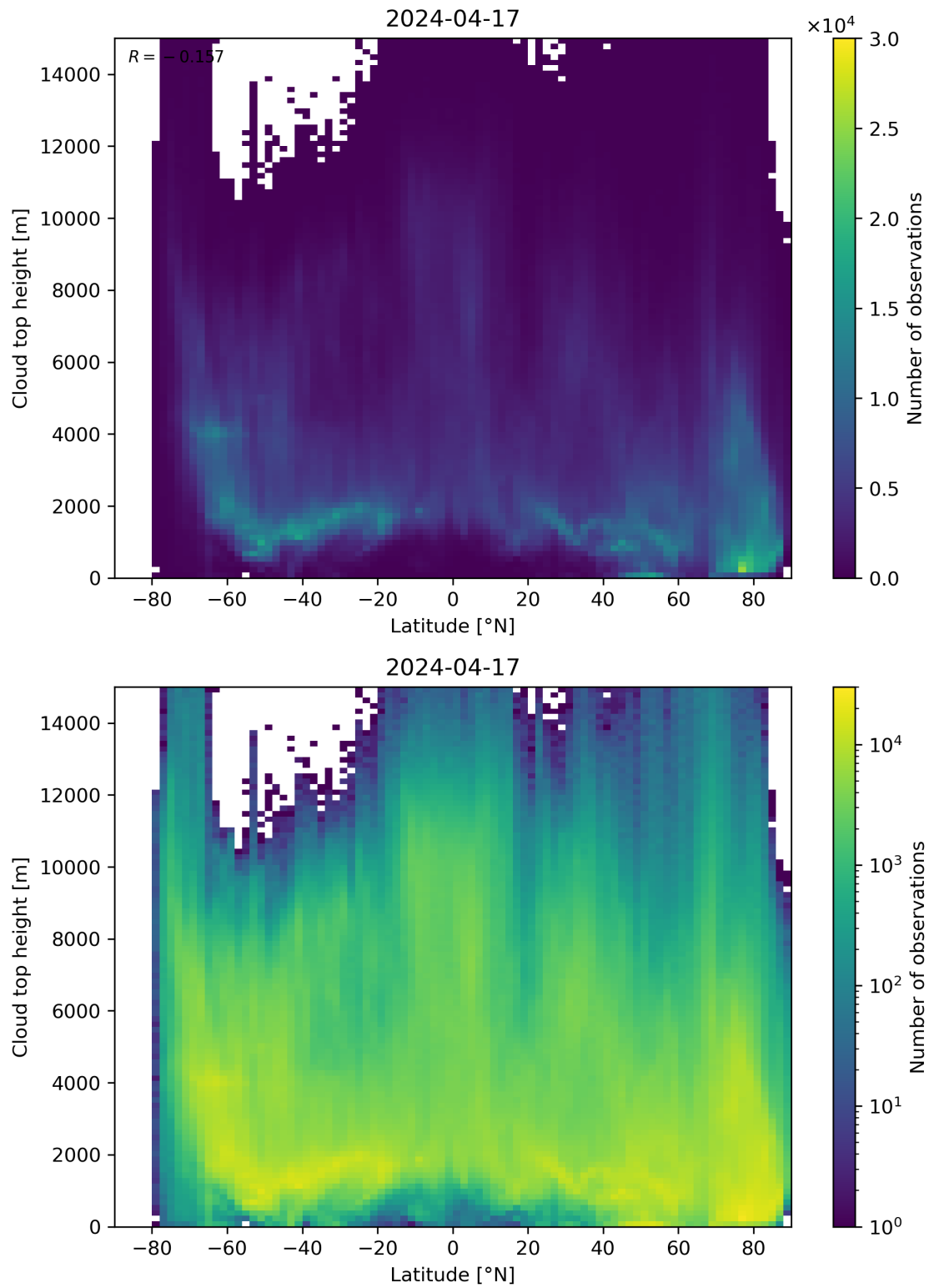
Figure 97: Scatter density plot of “Latitude” against “Cloud top height” for 2024-04-16 to 2024-04-18.
