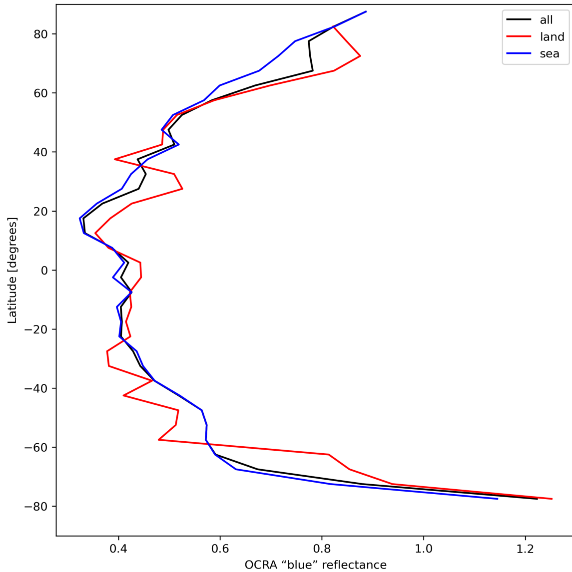
Figure 35: Zonal average of “OCRA “blue” reflectance” for 2024-04-16 to 2024-04-18.
