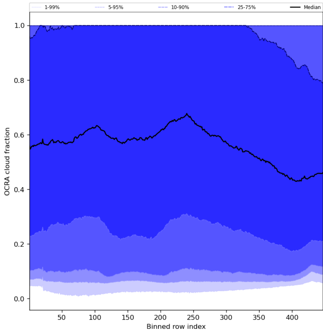
Figure 66: Along track statistics of “OCRA cloud fraction” for 2024-04-16 to 2024-04-18
