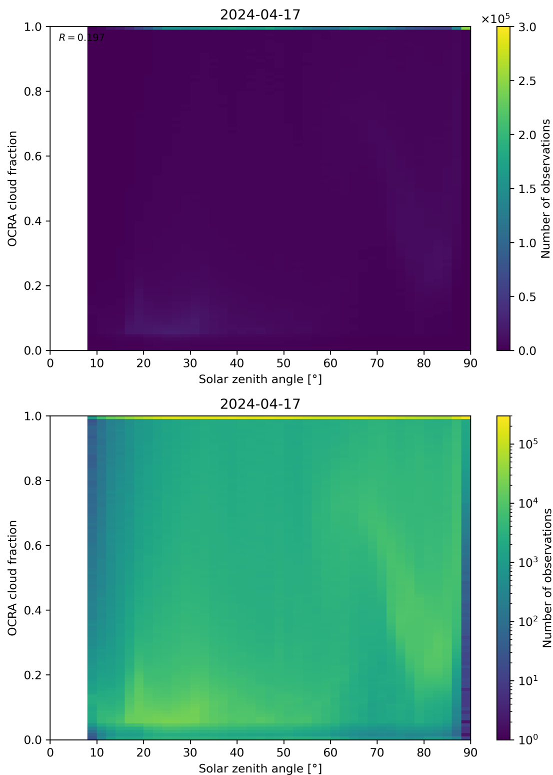
Figure 100: Scatter density plot of “Solar zenith angle” against “OCRA cloud fraction” for 2024-04-16 to 2024-04-18.
