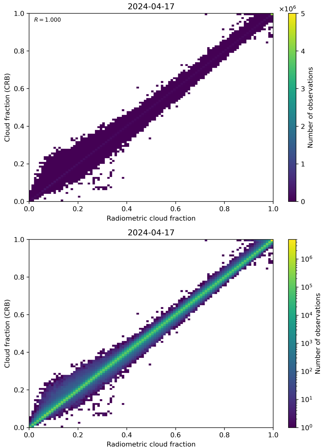
Figure 73: Scatter density plot of “Radiometric cloud fraction” against “Cloud fraction (CRB)” for 2024-04-16 to 2024-04-18.
