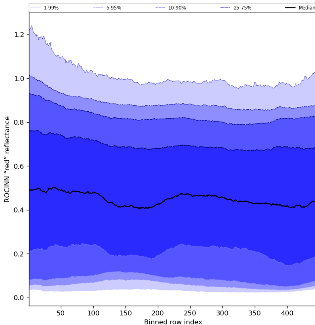
Figure 69: Along track statistics of "ROCINN "red" reflectance" for 2024-04-16 to 2024-04-18
