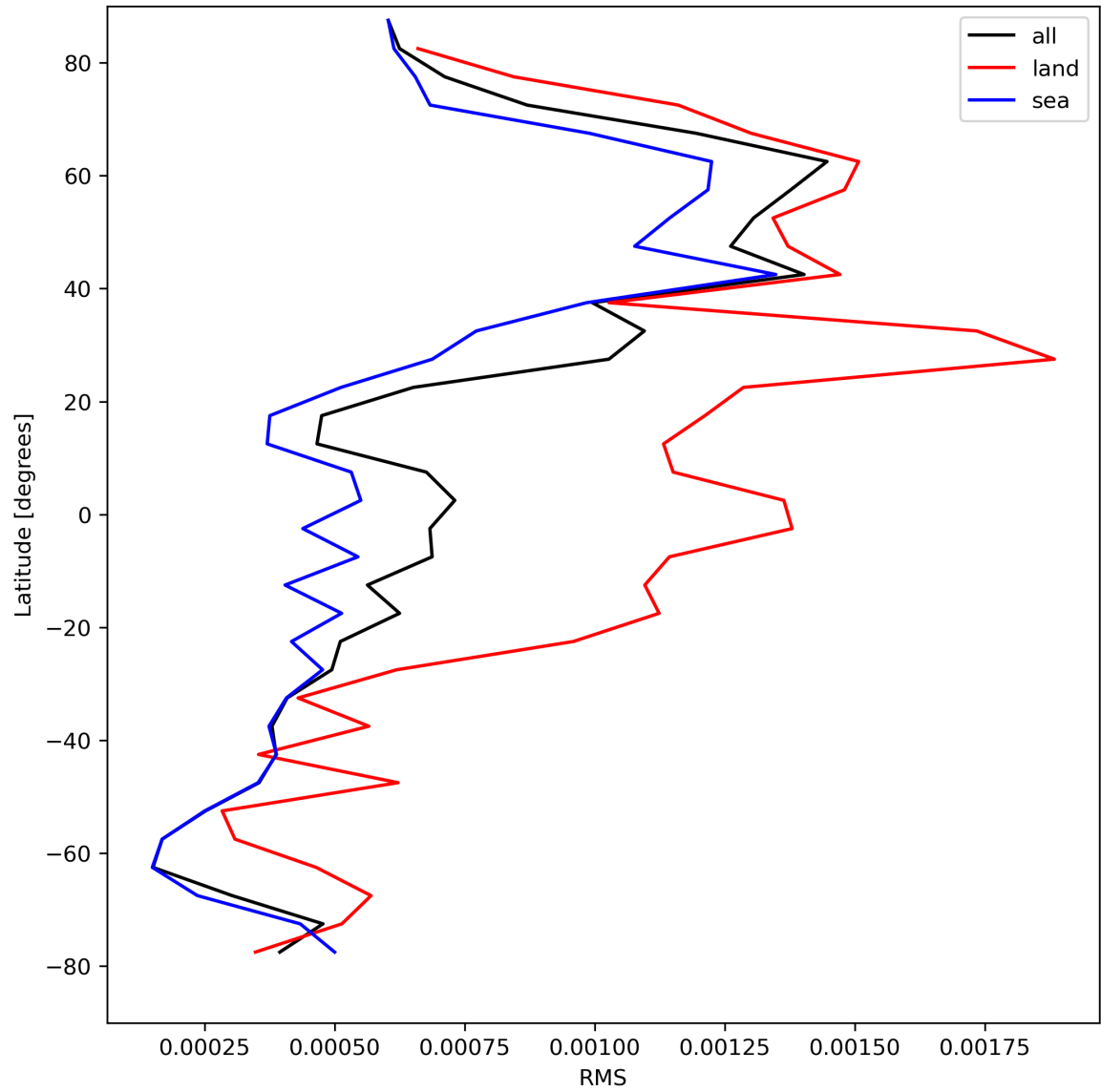
Figure 31: Zonal average of “RMS” for 2024-04-16 to 2024-04-18.
