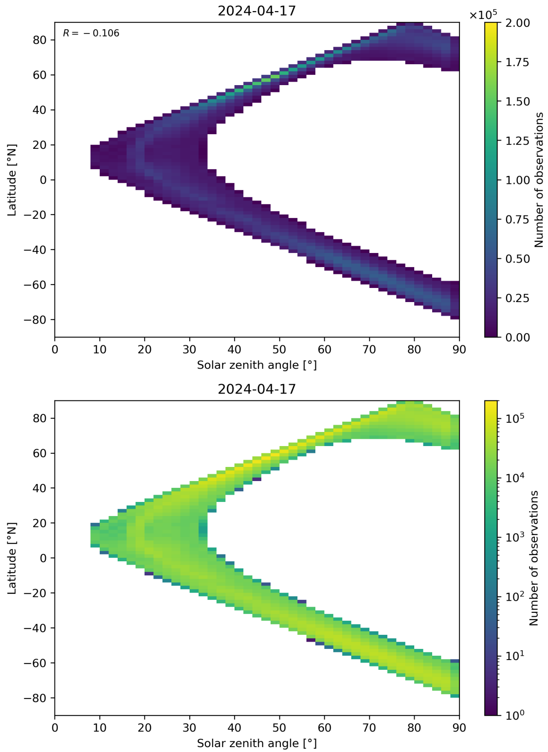
Figure 105: Scatter density plot of “Solar zenith angle” against “Latitude” for 2024-04-16 to 2024-04-18.
