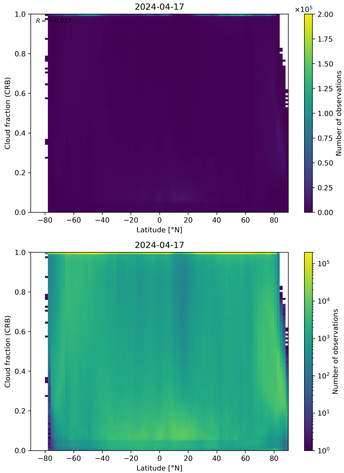
Figure 94: Scatter density plot of “Latitude” against “Cloud fraction (CRB)” for 2024-04-16 to 2024-04-18.
