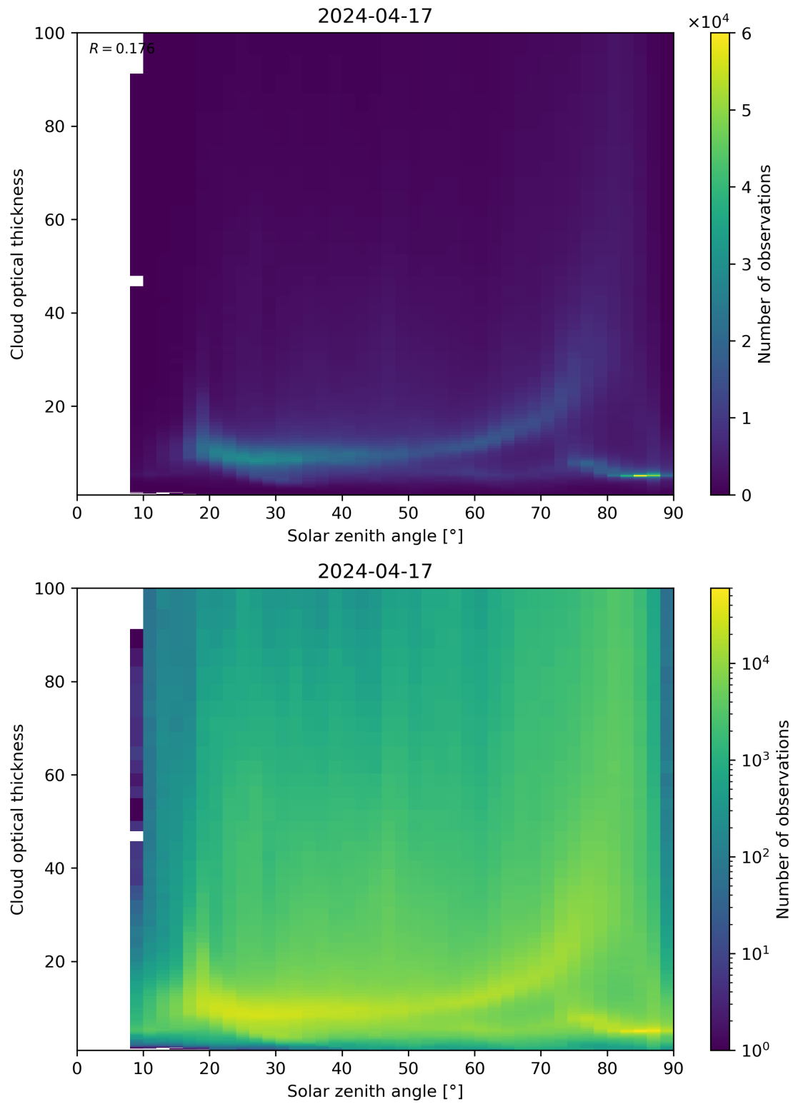
Figure 103: Scatter density plot of “Solar zenith angle” against “Cloud optical thickness” for 2024-04-16 to 2024-04-18.
