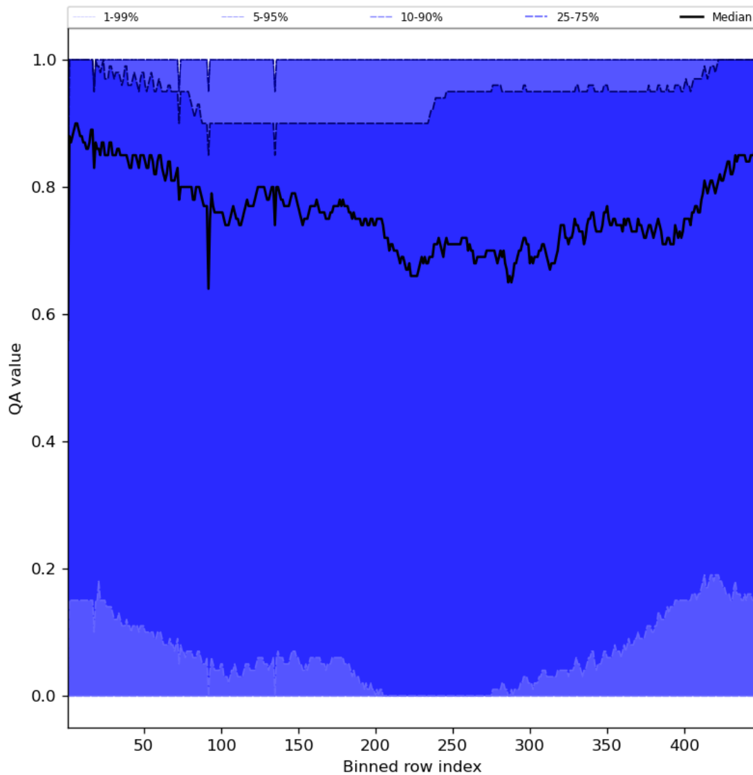
Figure 54: Along track statistics of “QA value” for 2024-04-16 to 2024-04-18
