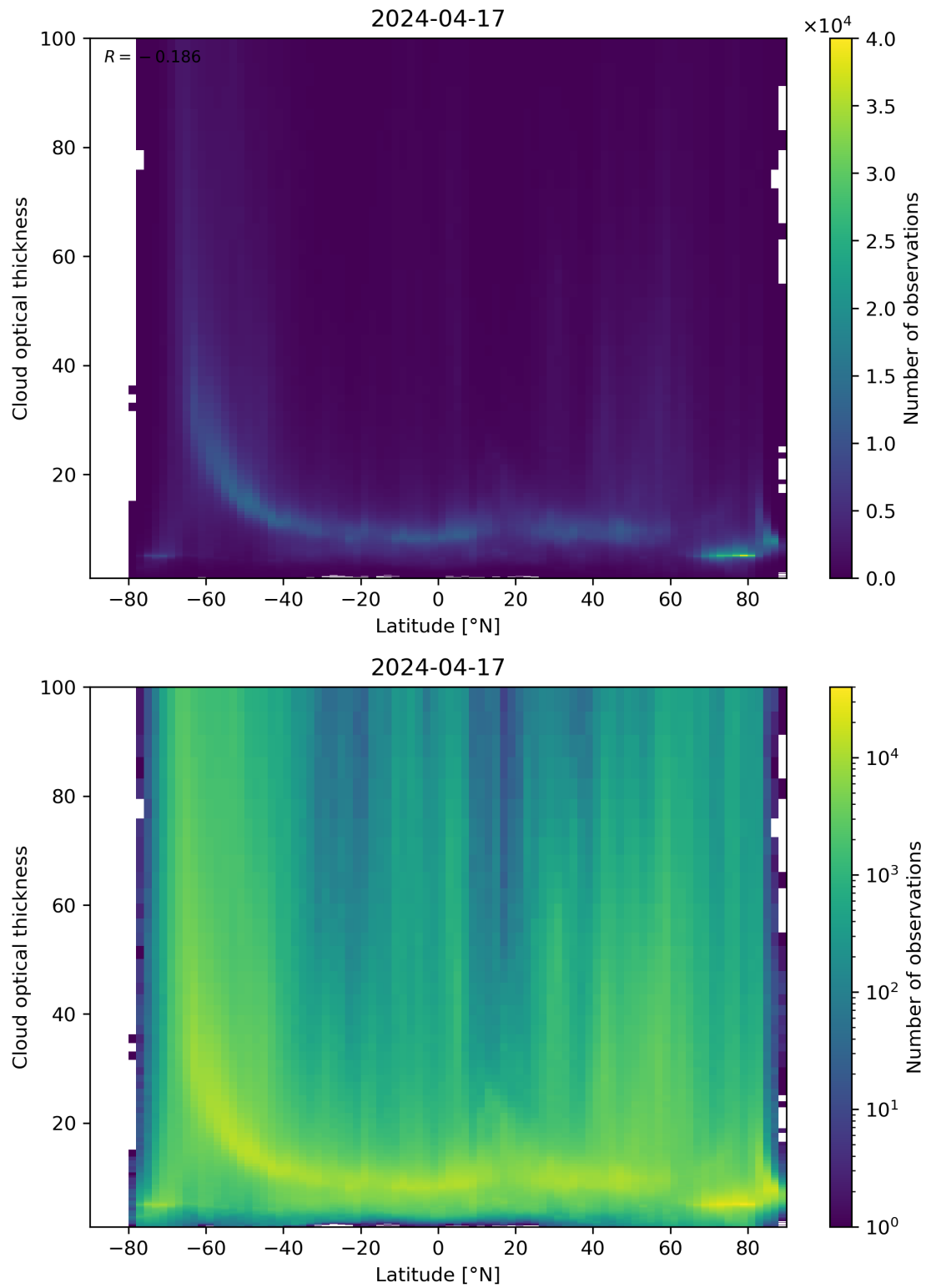
Figure 96: Scatter density plot of “Latitude” against “Cloud optical thickness” for 2024-04-16 to 2024-04-18.
