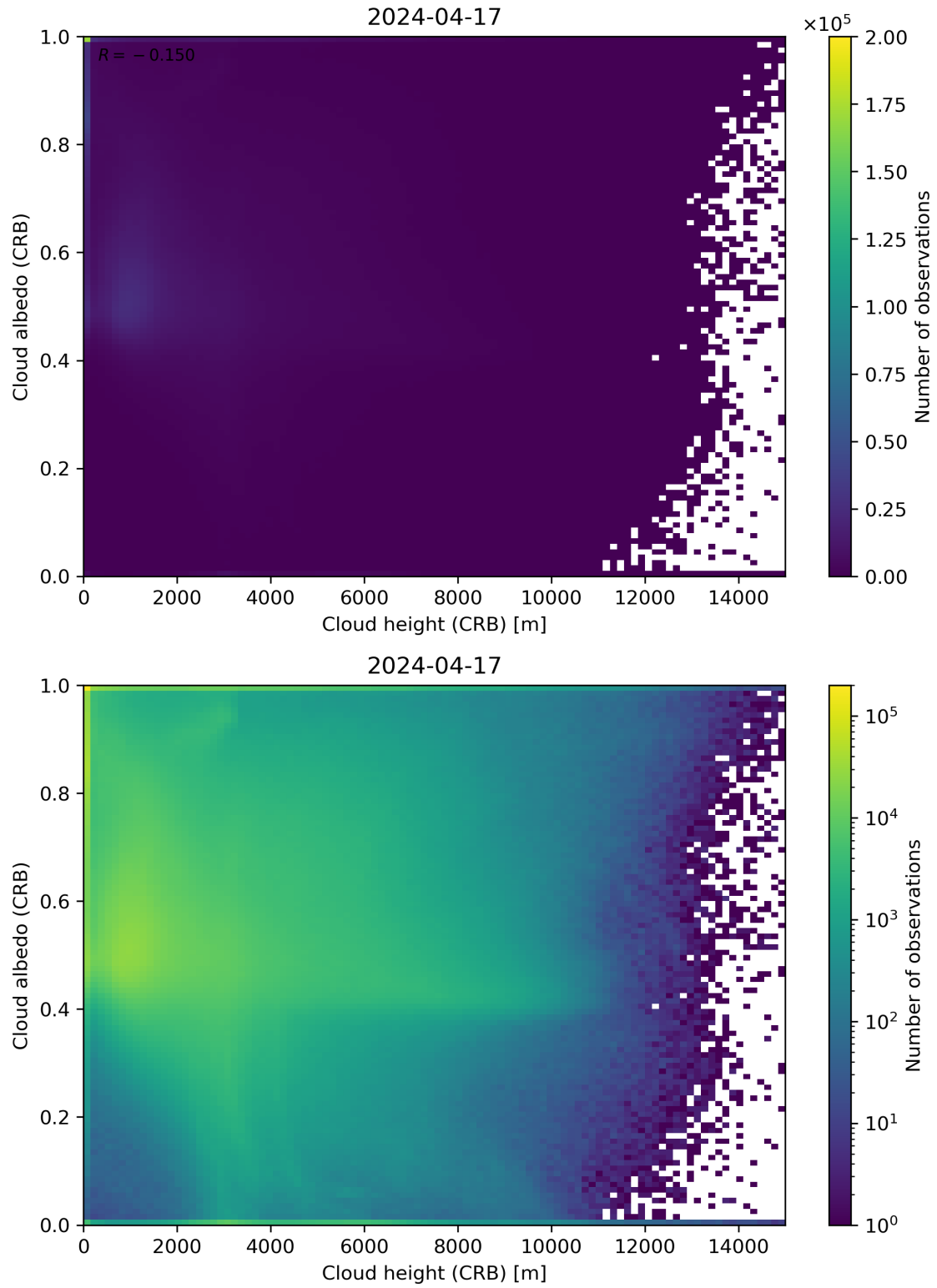
Figure 80: Scatter density plot of “Cloud height (CRB)” against “Cloud albedo (CRB)” for 2024-04-16 to 2024-04-18.
