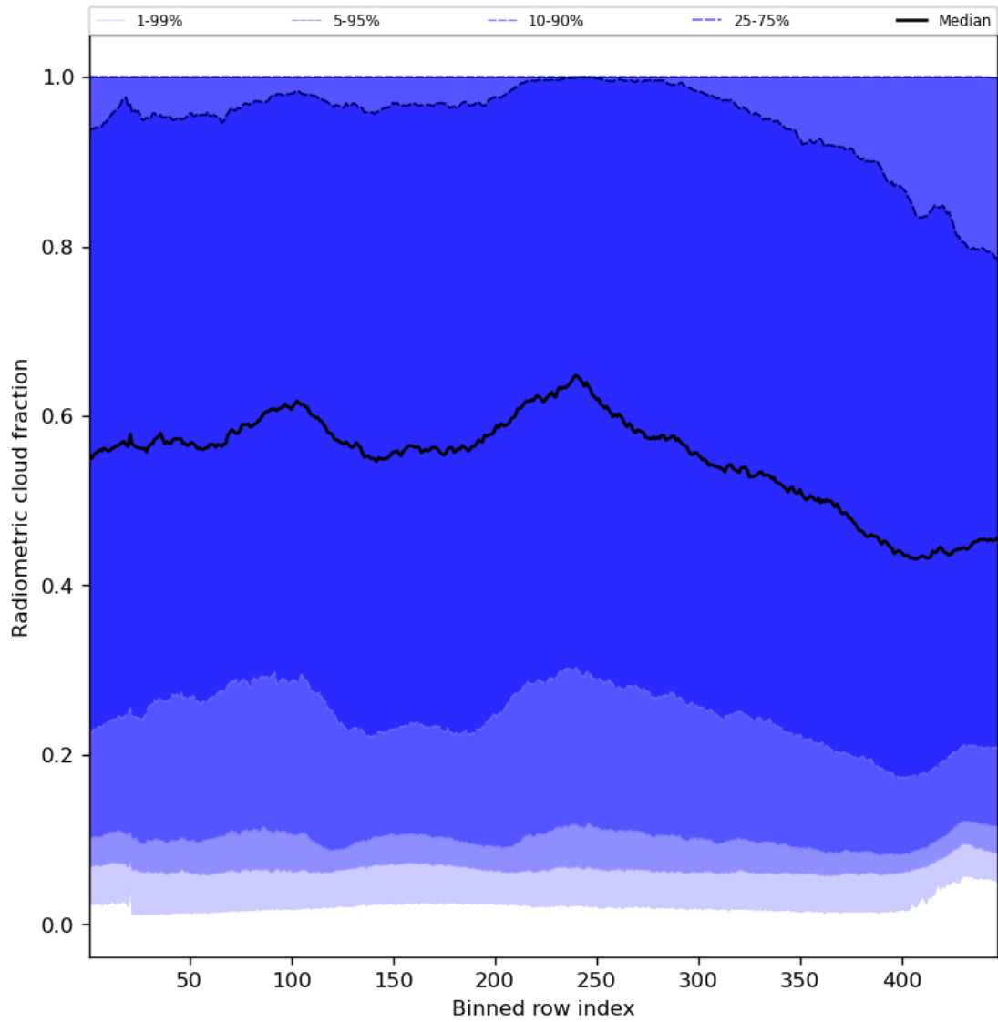
Figure 55: Along track statistics of “Radiometric cloud fraction” for 2024-04-16 to 2024-04-18
