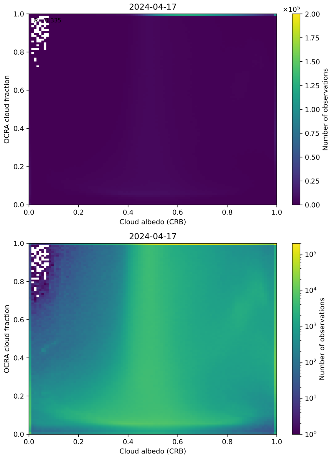
Figure 70: Scatter density plot of “Cloud albedo (CRB)” against “OCRA cloud fraction” for 2024-04-16 to 2024-04-18.
