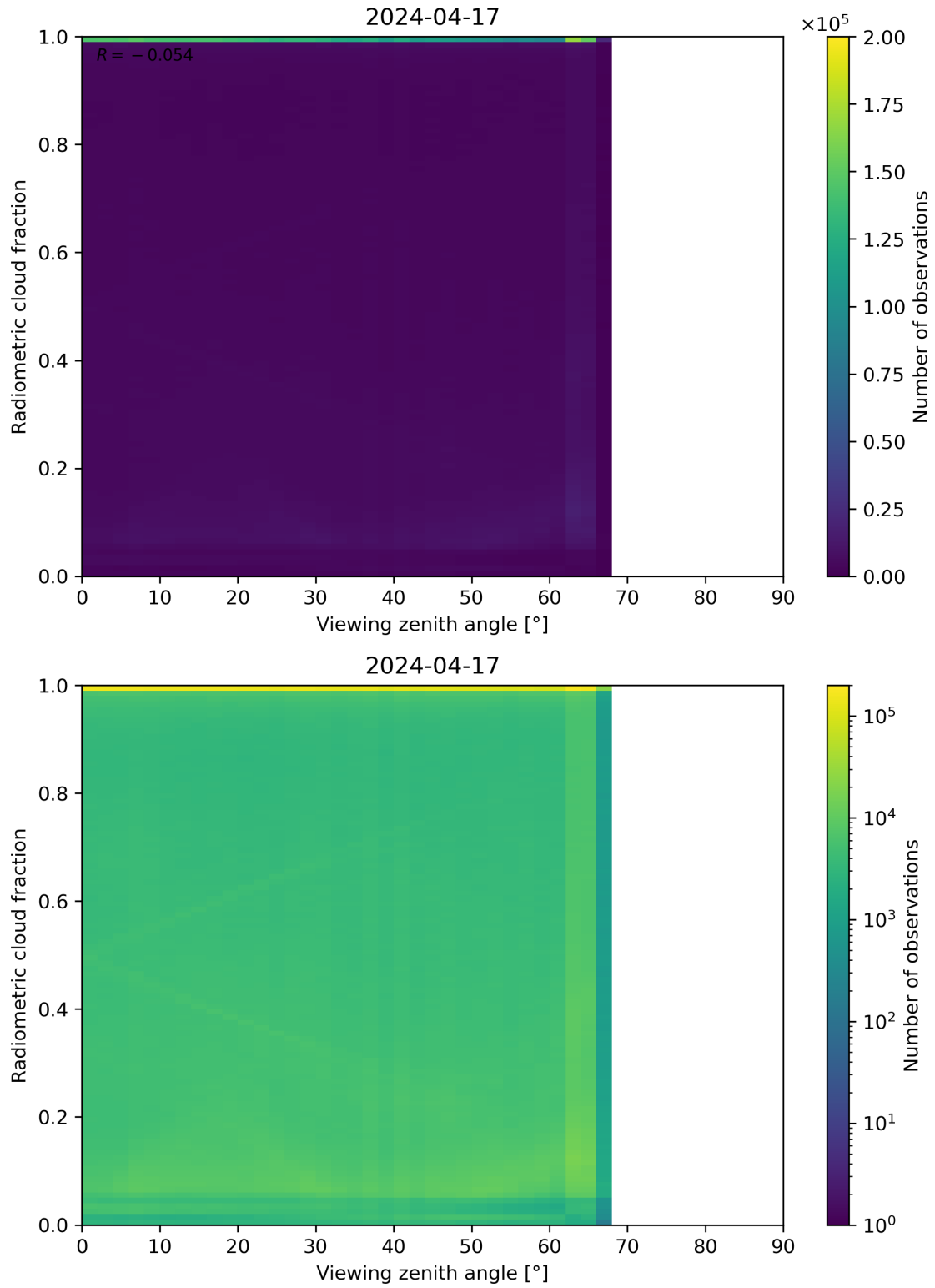
Figure 107: Scatter density plot of “Viewing zenith angle” against “Radiometric cloud fraction” for 2024-04-16 to 2024-04-18.
