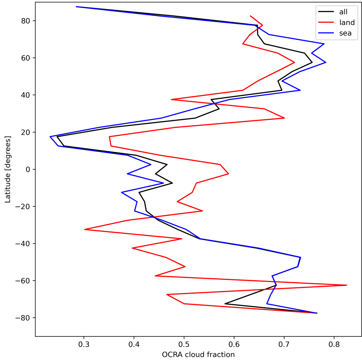
Figure 34: Zonal average of “OCRA cloud fraction” for 2024-04-16 to 2024-04-18.
