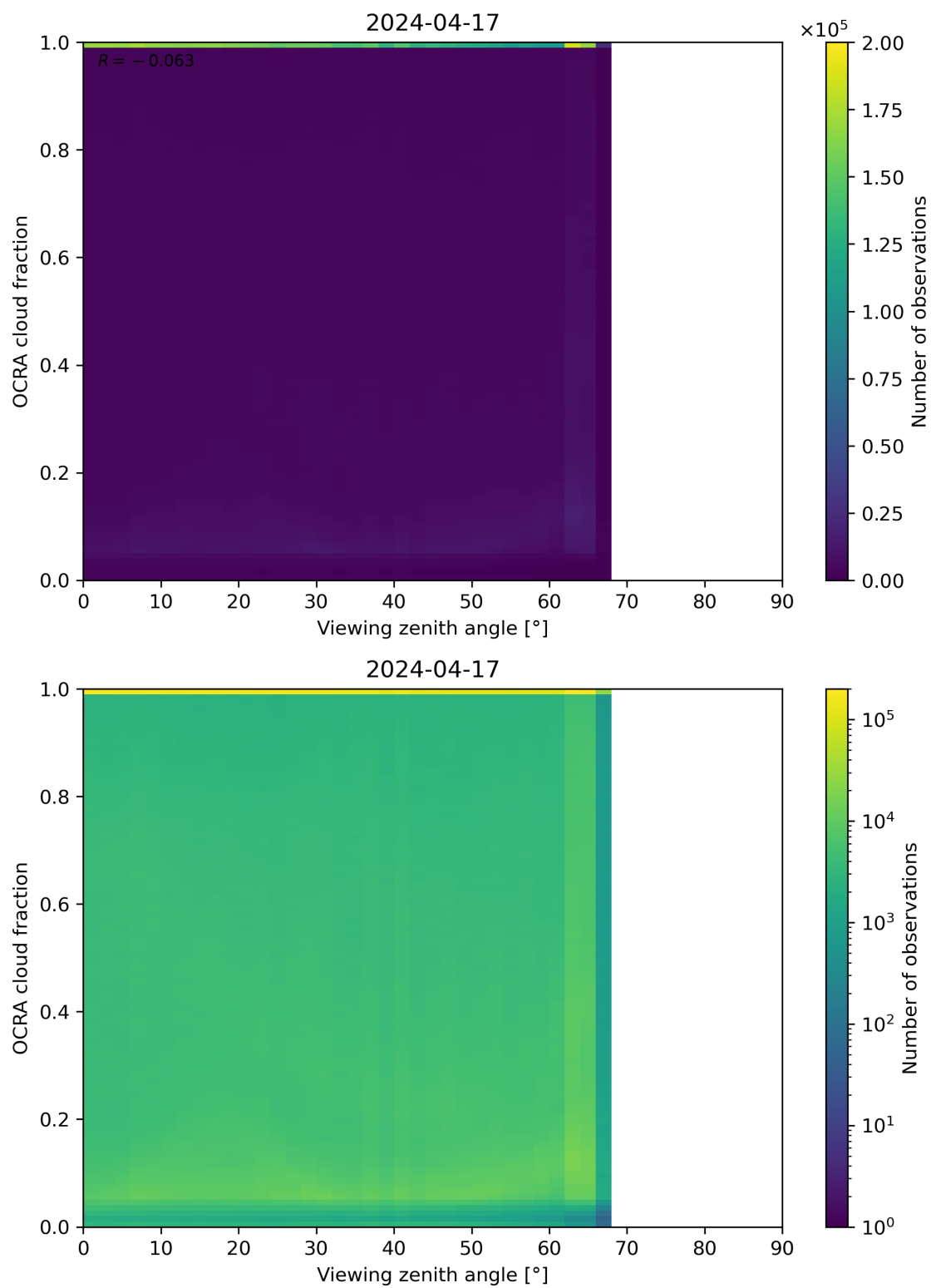
Figure 108: Scatter density plot of “Viewing zenith angle” against “OCRA cloud fraction” for 2024-04-16 to 2024-04-18.
