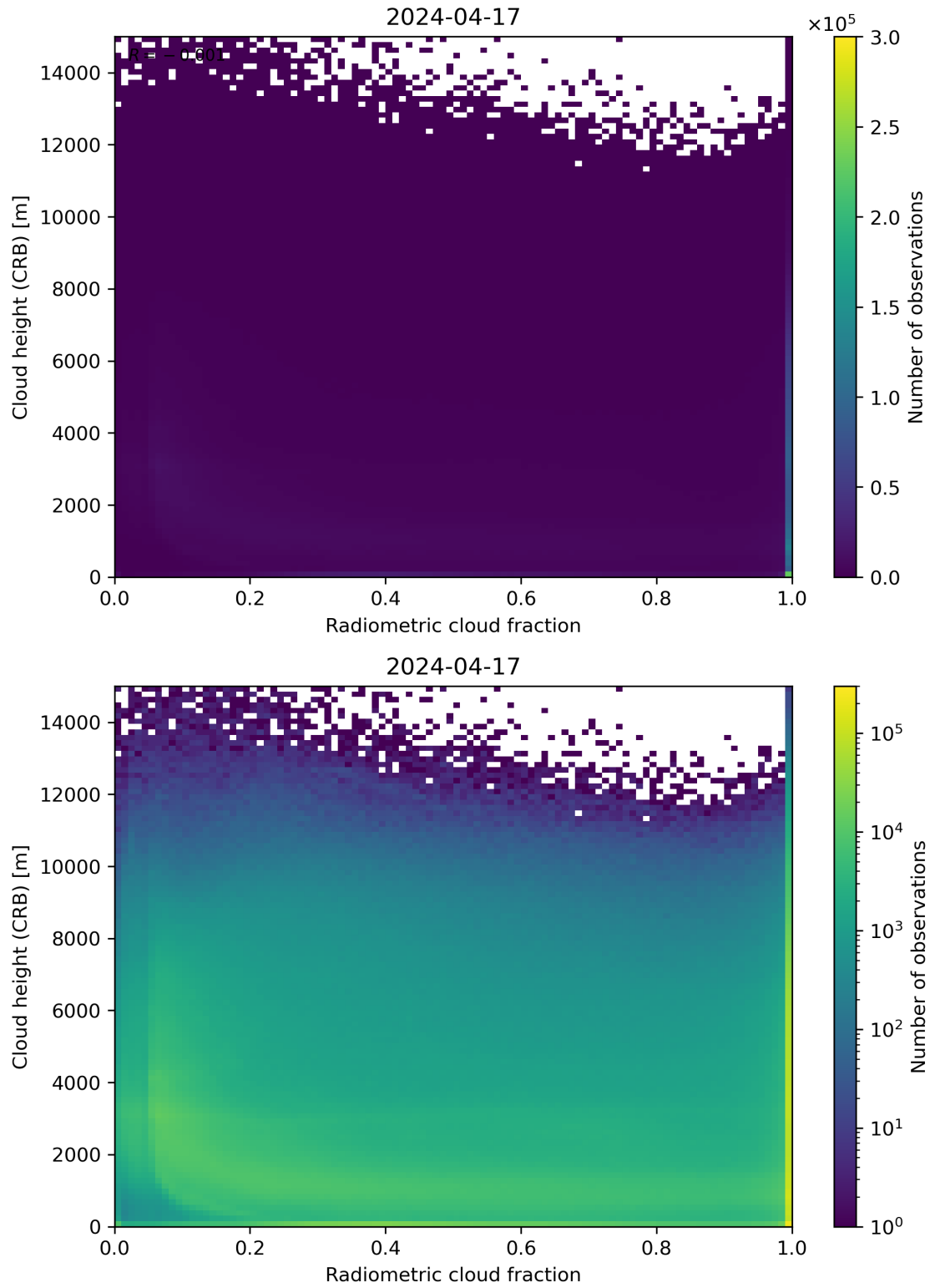
Figure 74: Scatter density plot of “Radiometric cloud fraction” against “Cloud height (CRB)” for 2024-04-16 to 2024-04-18.
