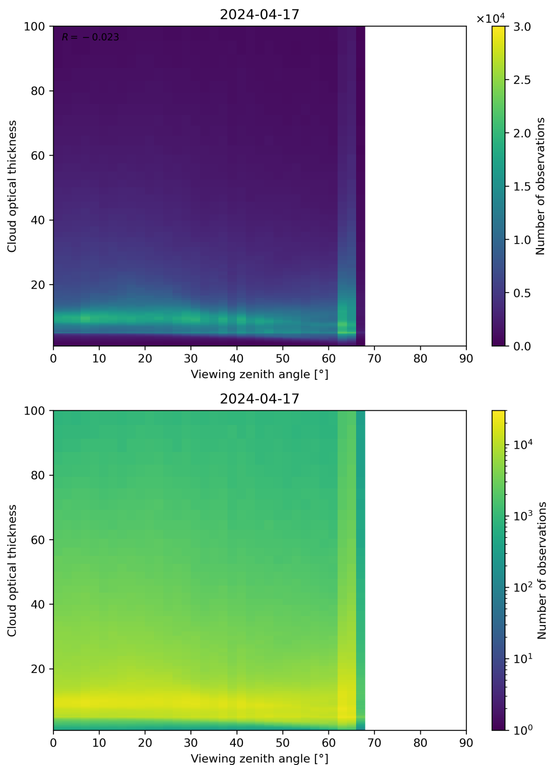
Figure 111: Scatter density plot of “Viewing zenith angle” against “Cloud optical thickness” for 2024-04-16 to 2024-04-18.
