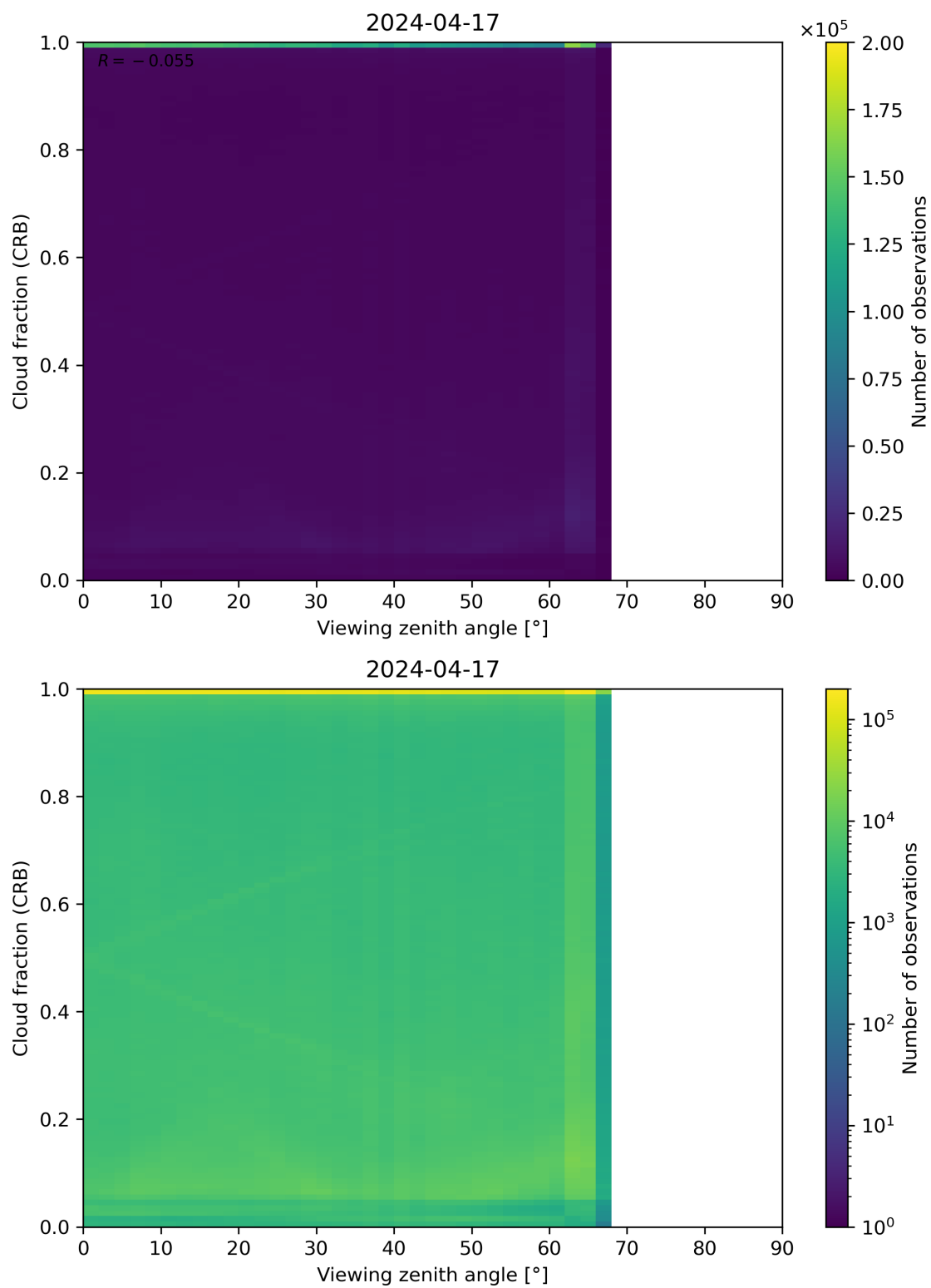
Figure 109: Scatter density plot of “Viewing zenith angle” against “Cloud fraction (CRB)” for 2024-04-16 to 2024-04-18.
