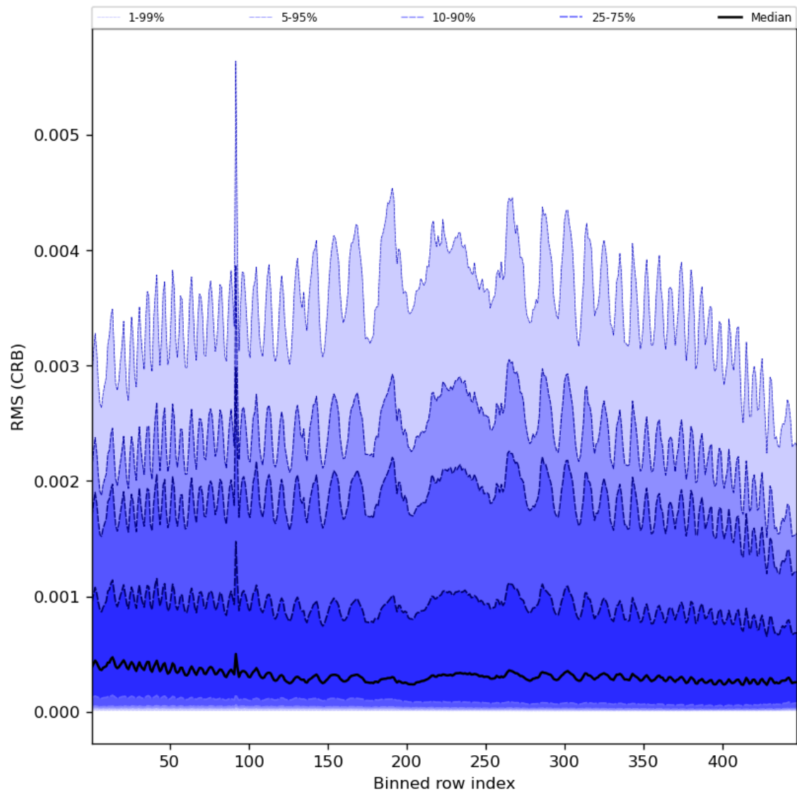
Figure 64: Along track statistics of “RMS (CRB)” for 2024-04-16 to 2024-04-18
