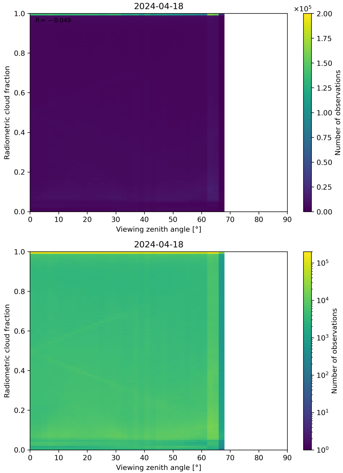
Figure 107: Scatter density plot of “Viewing zenith angle” against “Radiometric cloud fraction” for 2024-04-17 to 2024-04-19.
