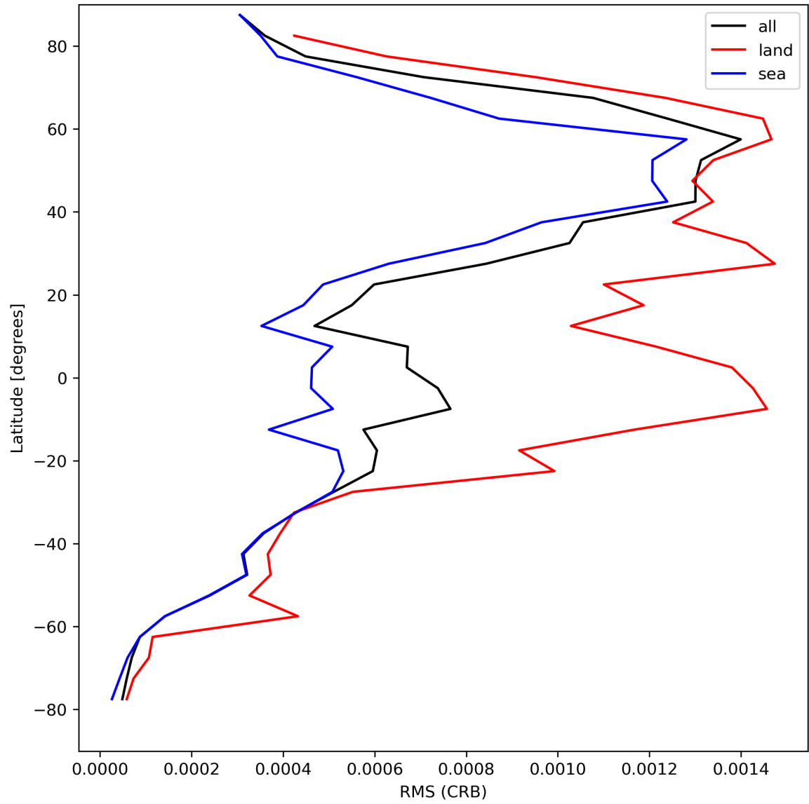
Figure 32: Zonal average of “RMS (CRB)” for 2024-04-17 to 2024-04-19.
