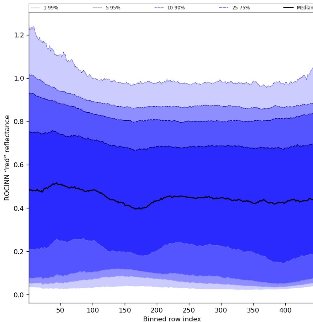
Figure 69: Along track statistics of “ROCINN “red” reflectance” for 2024-04-17 to 2024-04-19
