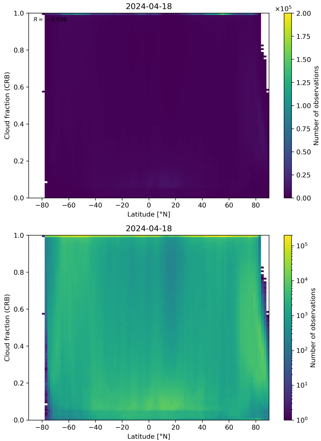
Figure 94: Scatter density plot of “Latitude” against “Cloud fraction (CRB)” for 2024-04-17 to 2024-04-19.
