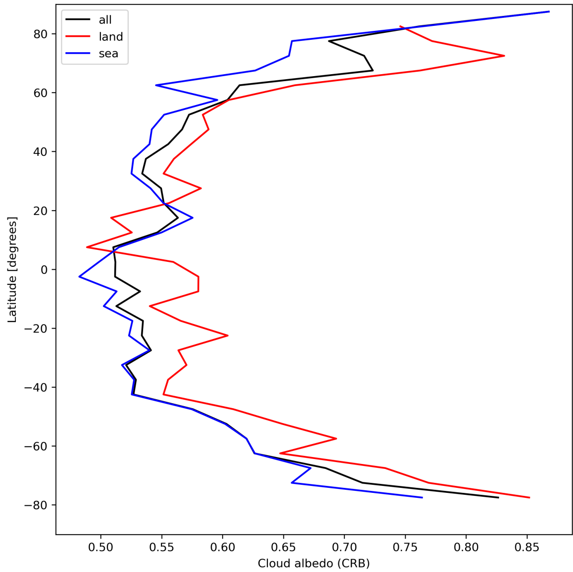
Figure 28: Zonal average of “Cloud albedo (CRB)” for 2024-04-17 to 2024-04-19.
