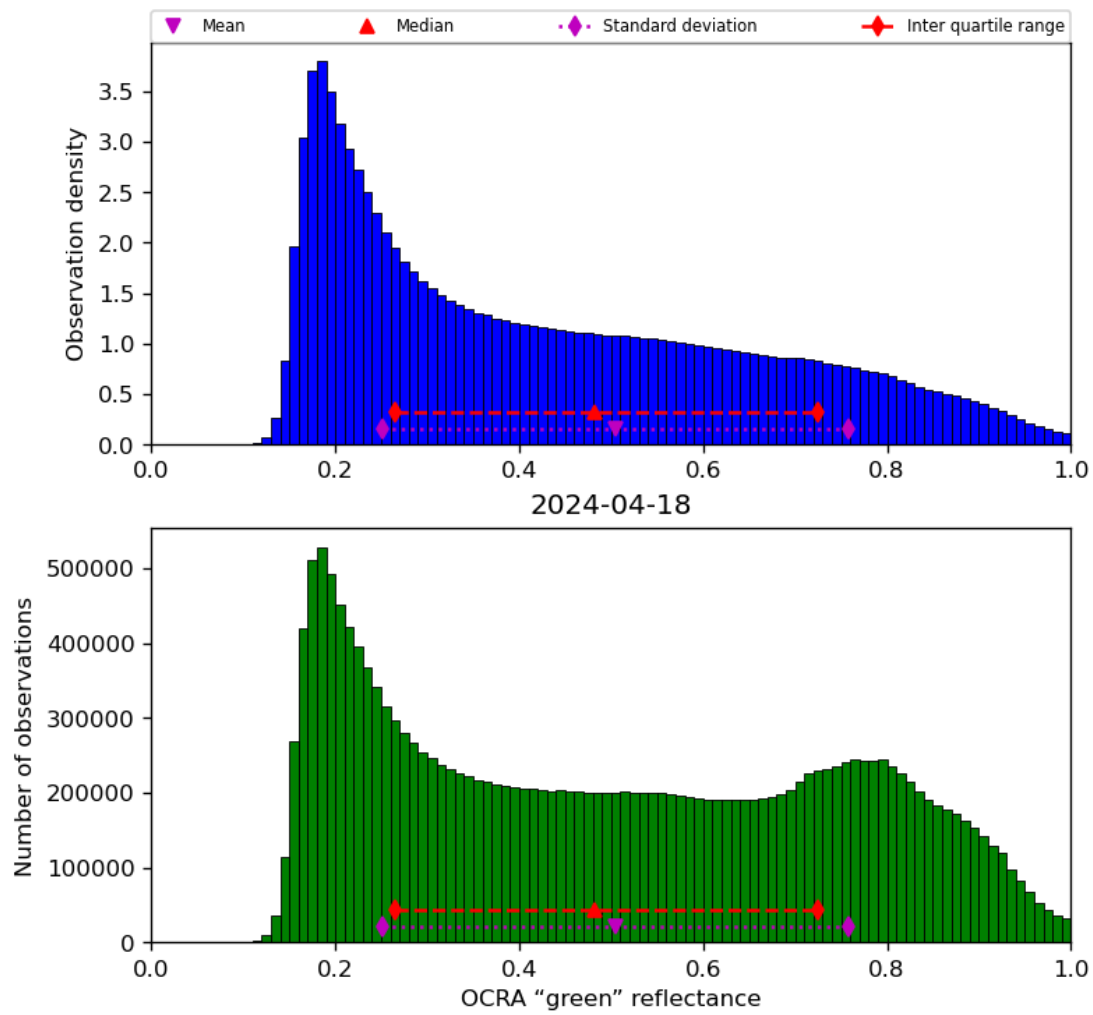
Figure 52: Histogram of “OCRA “green” reflectance” for 2024-04-17 to 2024-04-19
