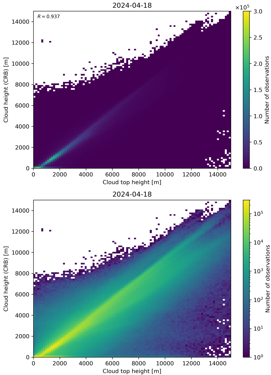
Figure 89: Scatter density plot of “Cloud top height” against “Cloud height (CRB)” for 2024-04-17 to 2024-04-19.
