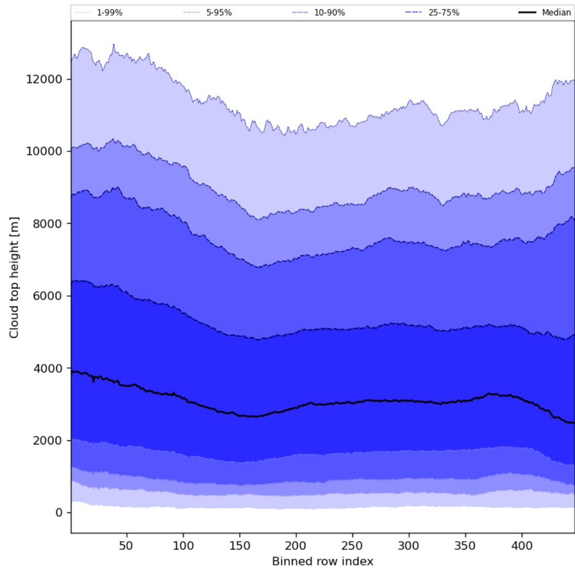
Figure 56: Along track statistics of “Cloud top height” for 2024-04-17 to 2024-04-19
