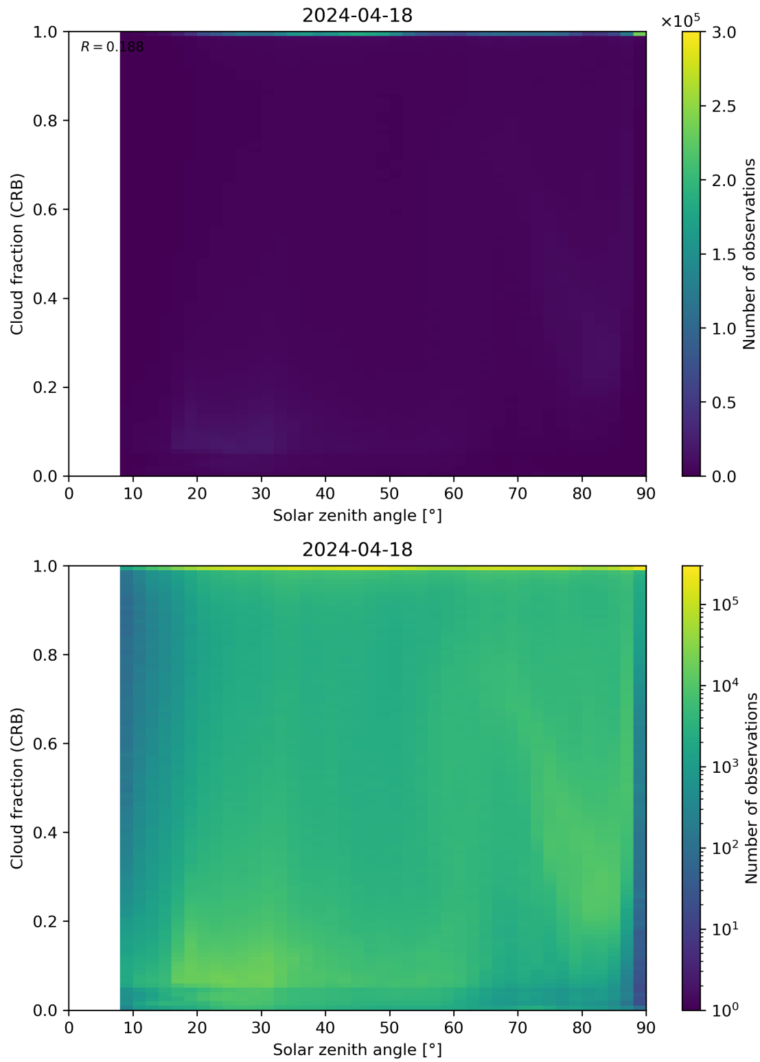
Figure 101: Scatter density plot of “Solar zenith angle” against “Cloud fraction (CRB)” for 2024-04-17 to 2024-04-19.
