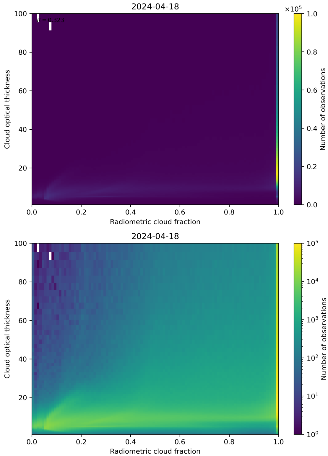
Figure 75: Scatter density plot of “Radiometric cloud fraction” against “Cloud optical thickness” for 2024-04-17 to 2024-04-19.
