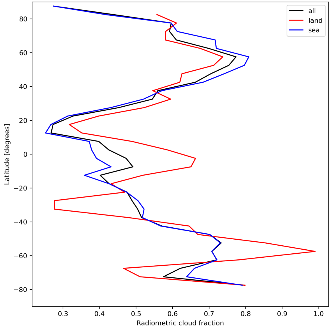
Figure 23: Zonal average of “Radiometric cloud fraction” for 2024-04-17 to 2024-04-19.
