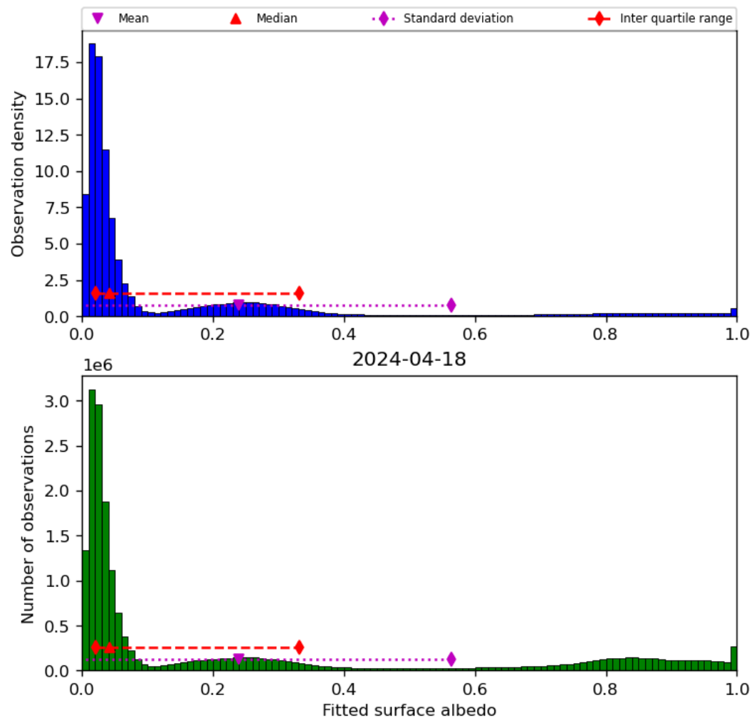
Figure 45: Histogram of “Fitted surface albedo” for 2024-04-17 to 2024-04-19
