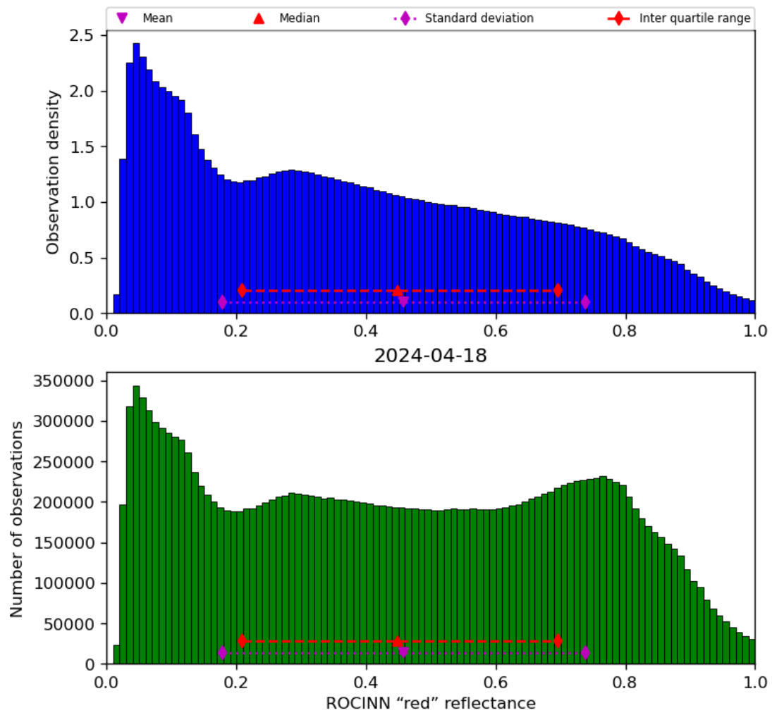
Figure 53: Histogram of “ROCINN “red” reflectance” for 2024-04-17 to 2024-04-19
