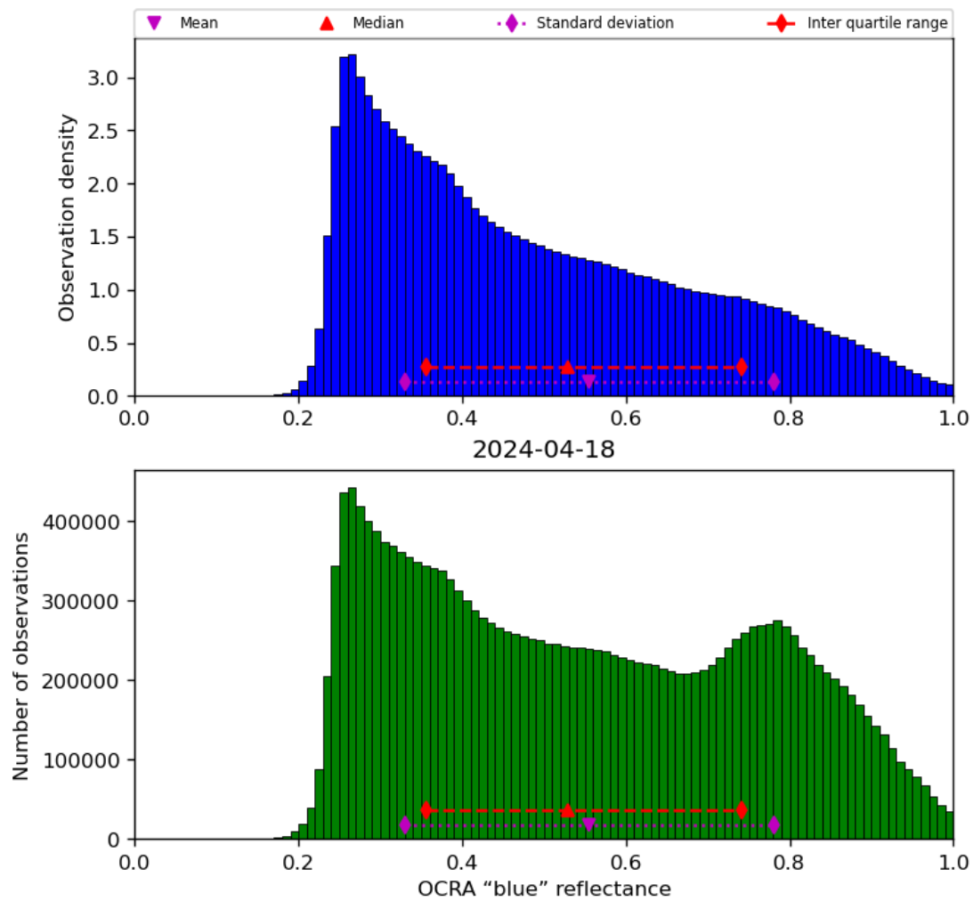
Figure 51: Histogram of “OCRA “blue” reflectance” for 2024-04-17 to 2024-04-19
