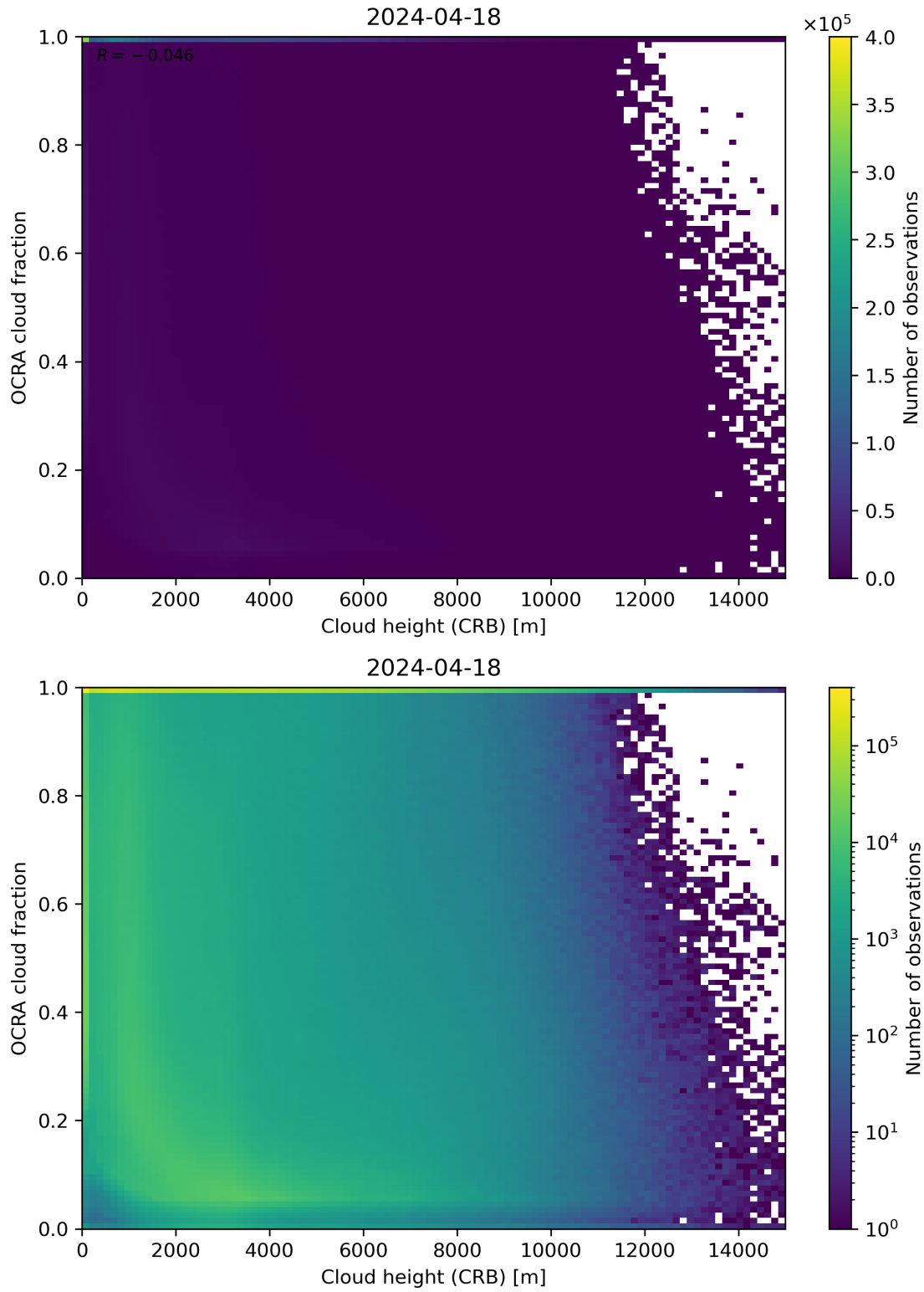
Figure 81: Scatter density plot of “Cloud height (CRB)” against “OCRA cloud fraction” for 2024-04-17 to 2024-04-19.
