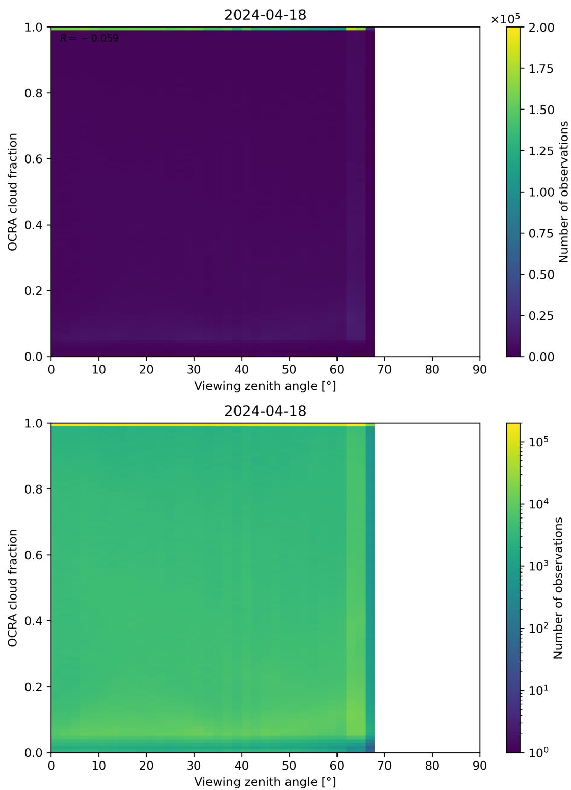
Figure 108: Scatter density plot of “Viewing zenith angle” against “OCRA cloud fraction” for 2024-04-17 to 2024-04-19.
