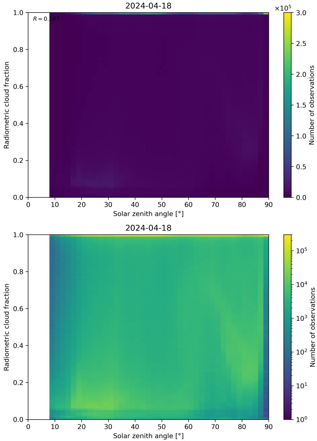
Figure 99: Scatter density plot of “Solar zenith angle” against “Radiometric cloud fraction” for 2024-04-17 to 2024-04-19.
