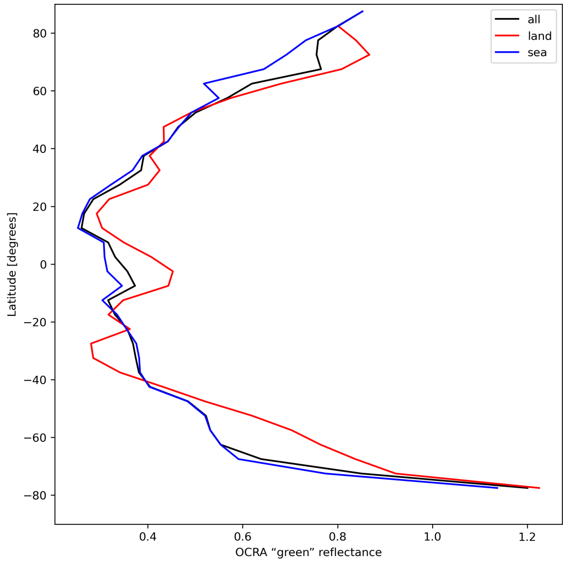
Figure 36: Zonal average of “OCRA “green” reflectance” for 2024-04-17 to 2024-04-19.
