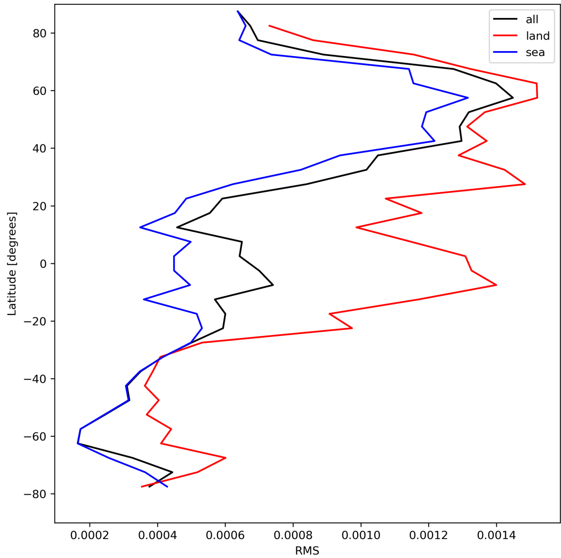
Figure 31: Zonal average of “RMS” for 2024-04-17 to 2024-04-19.
