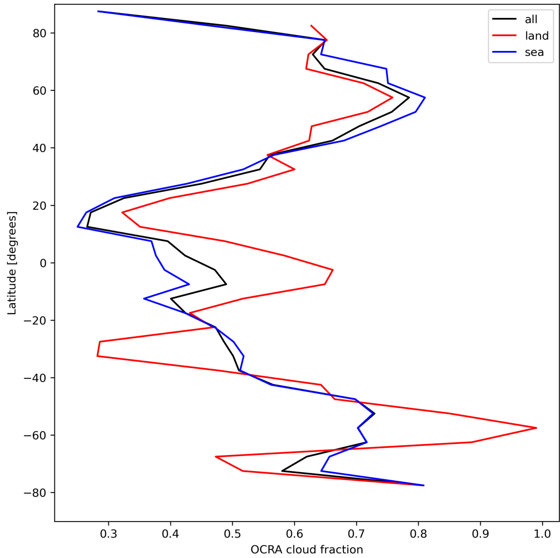
Figure 34: Zonal average of “OCRA cloud fraction” for 2024-04-17 to 2024-04-19.
