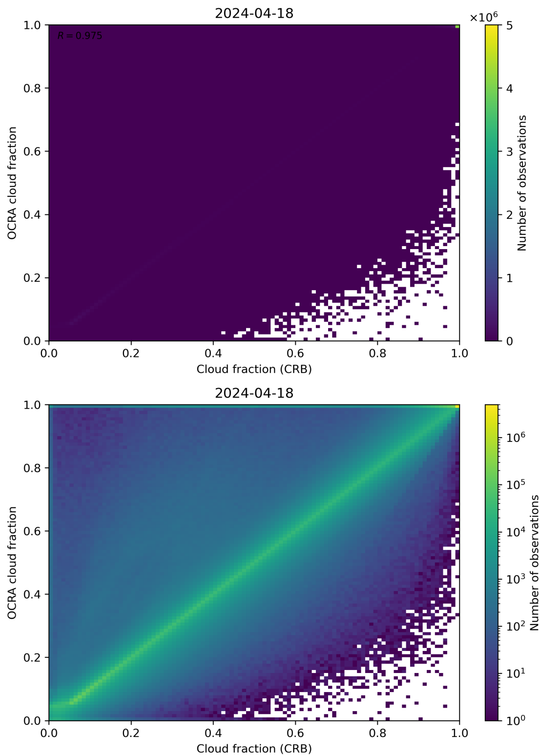
Figure 78: Scatter density plot of “Cloud fraction (CRB)” against “OCRA cloud fraction” for 2024-04-17 to 2024-04-19.
