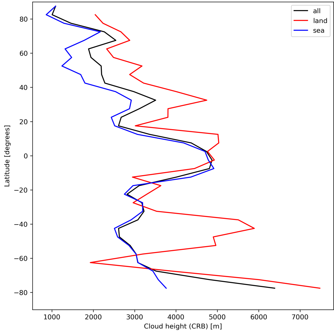
Figure 27: Zonal average of “Cloud height (CRB)” for 2024-04-17 to 2024-04-19.
