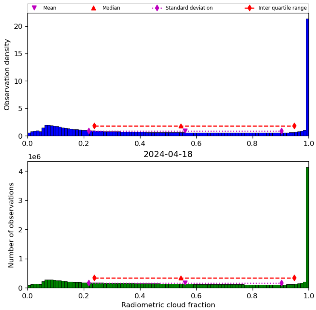
Figure 39: Histogram of “Radiometric cloud fraction” for 2024-04-17 to 2024-04-19
