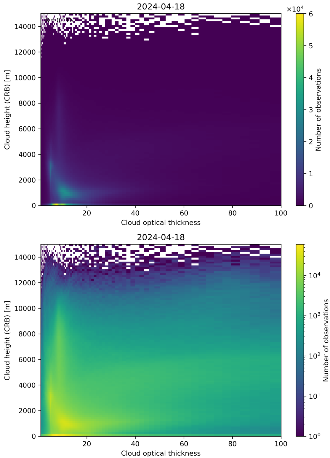
Figure 85: Scatter density plot of “Cloud optical thickness” against “Cloud height (CRB)” for 2024-04-17 to 2024-04-19.
