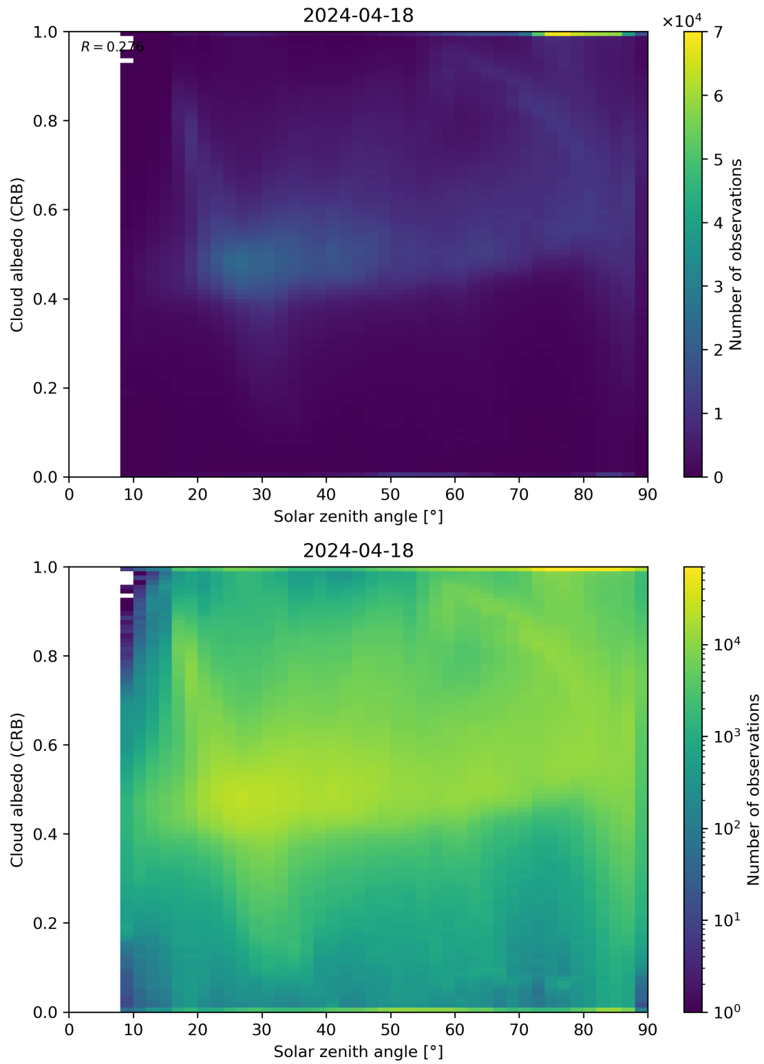
Figure 98: Scatter density plot of “Solar zenith angle” against “Cloud albedo (CRB)” for 2024-04-17 to 2024-04-19.
