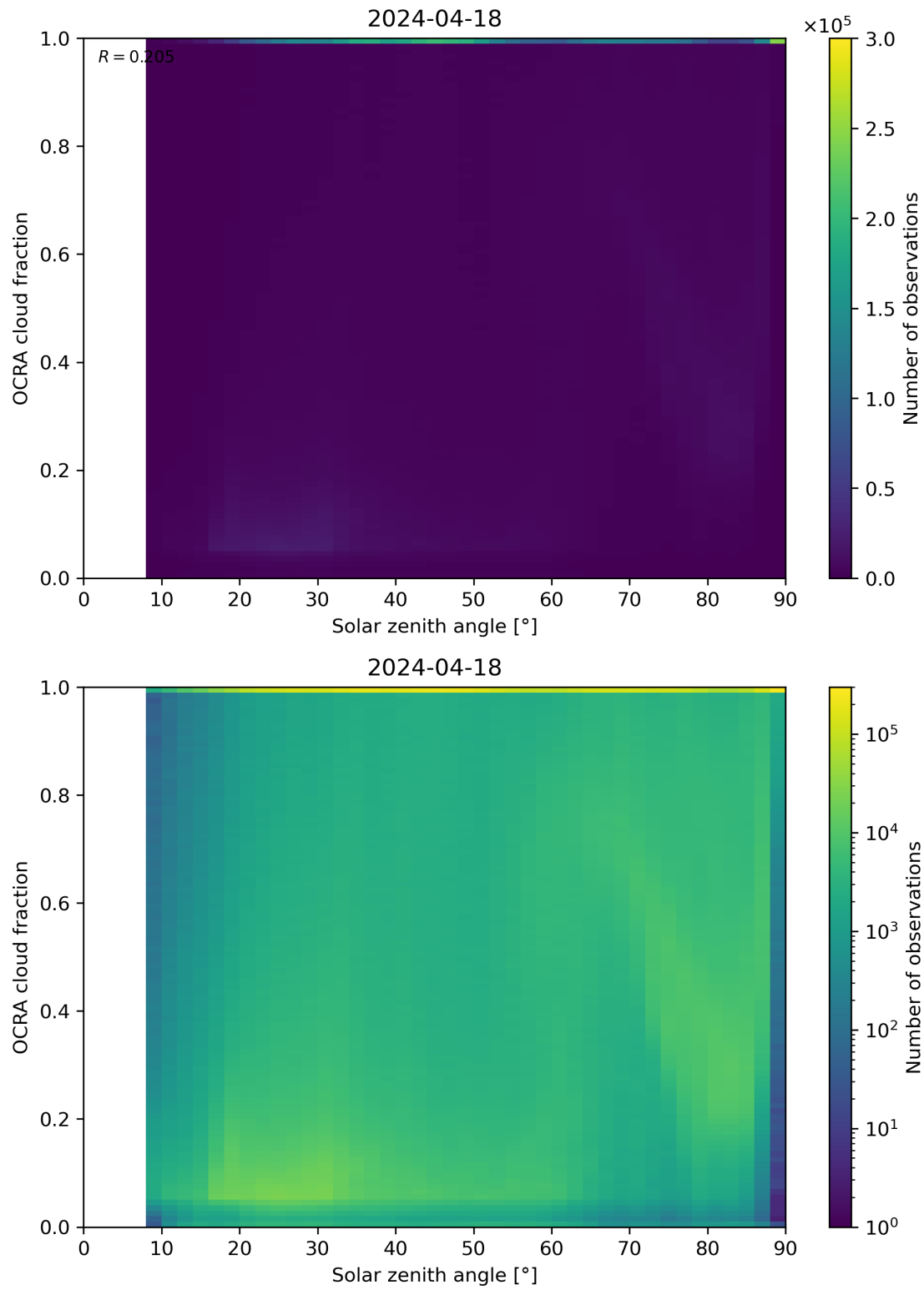
Figure 100: Scatter density plot of “Solar zenith angle” against “OCRA cloud fraction” for 2024-04-17 to 2024-04-19.
