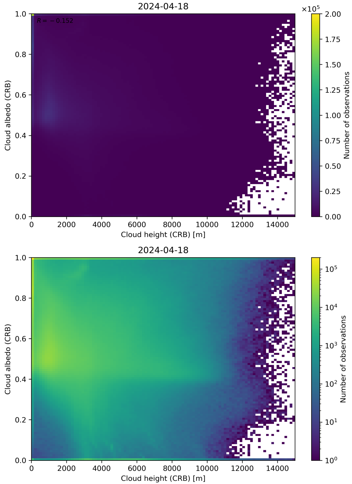
Figure 80: Scatter density plot of “Cloud height (CRB)” against “Cloud albedo (CRB)” for 2024-04-17 to 2024-04-19.
