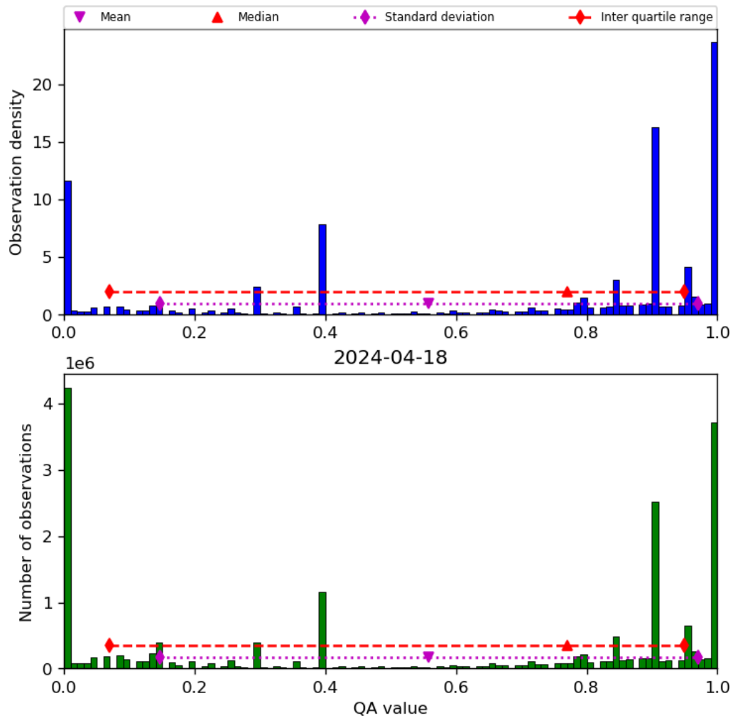
Figure 38: Histogram of “QA value” for 2024-04-17 to 2024-04-19
