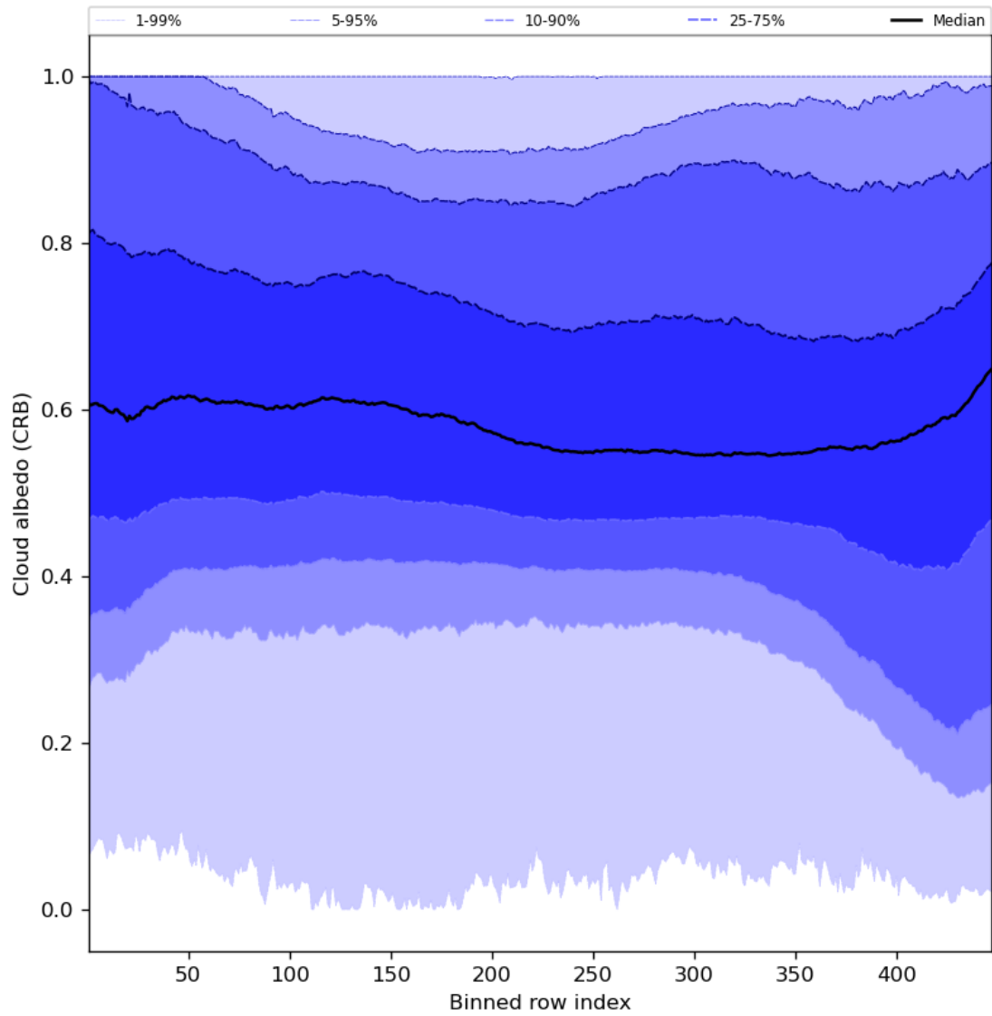
Figure 60: Along track statistics of “Cloud albedo (CRB)” for 2024-04-17 to 2024-04-19
