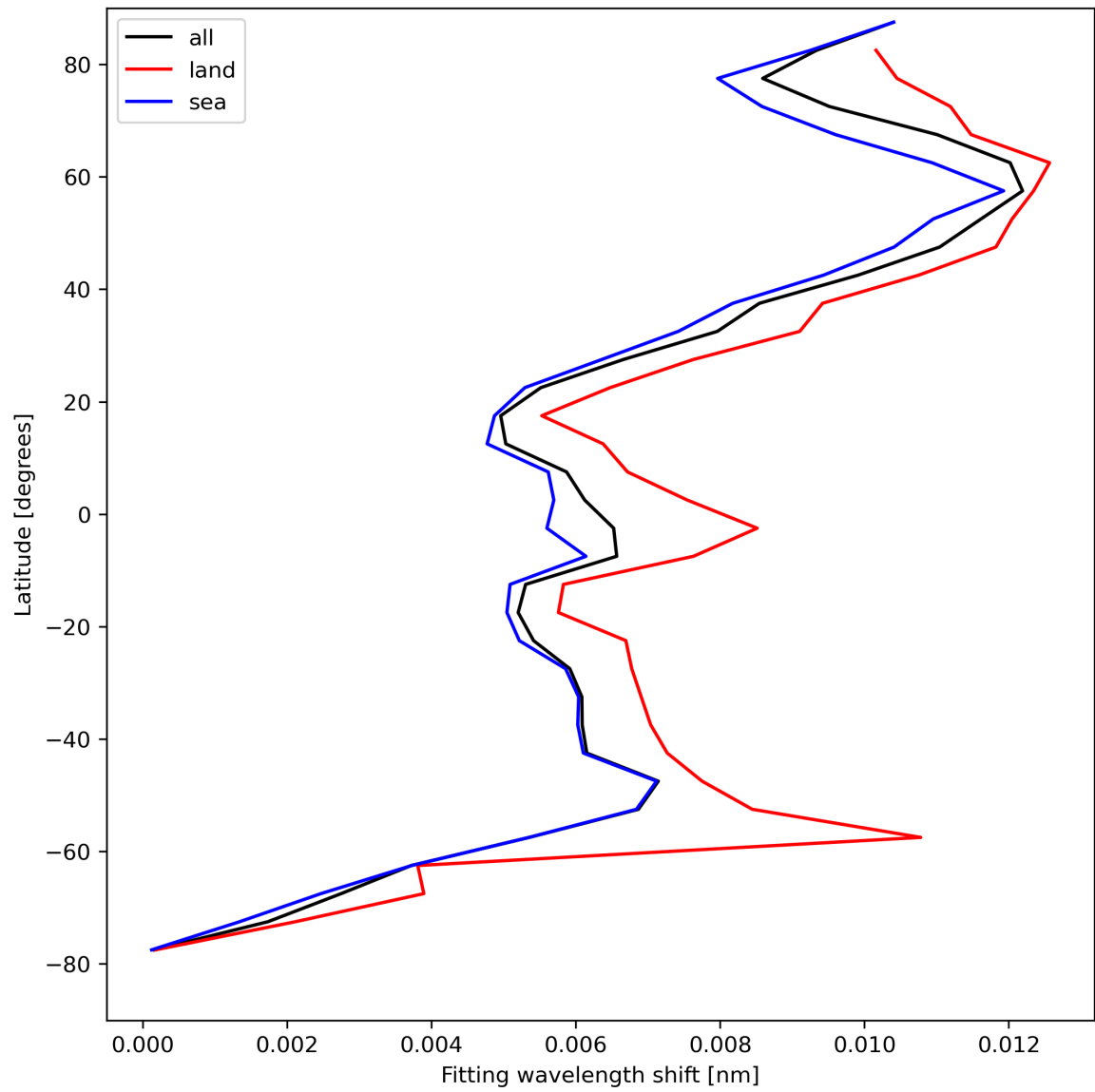
Figure 33: Zonal average of “Fitting wavelength shift” for 2024-04-17 to 2024-04-19.
