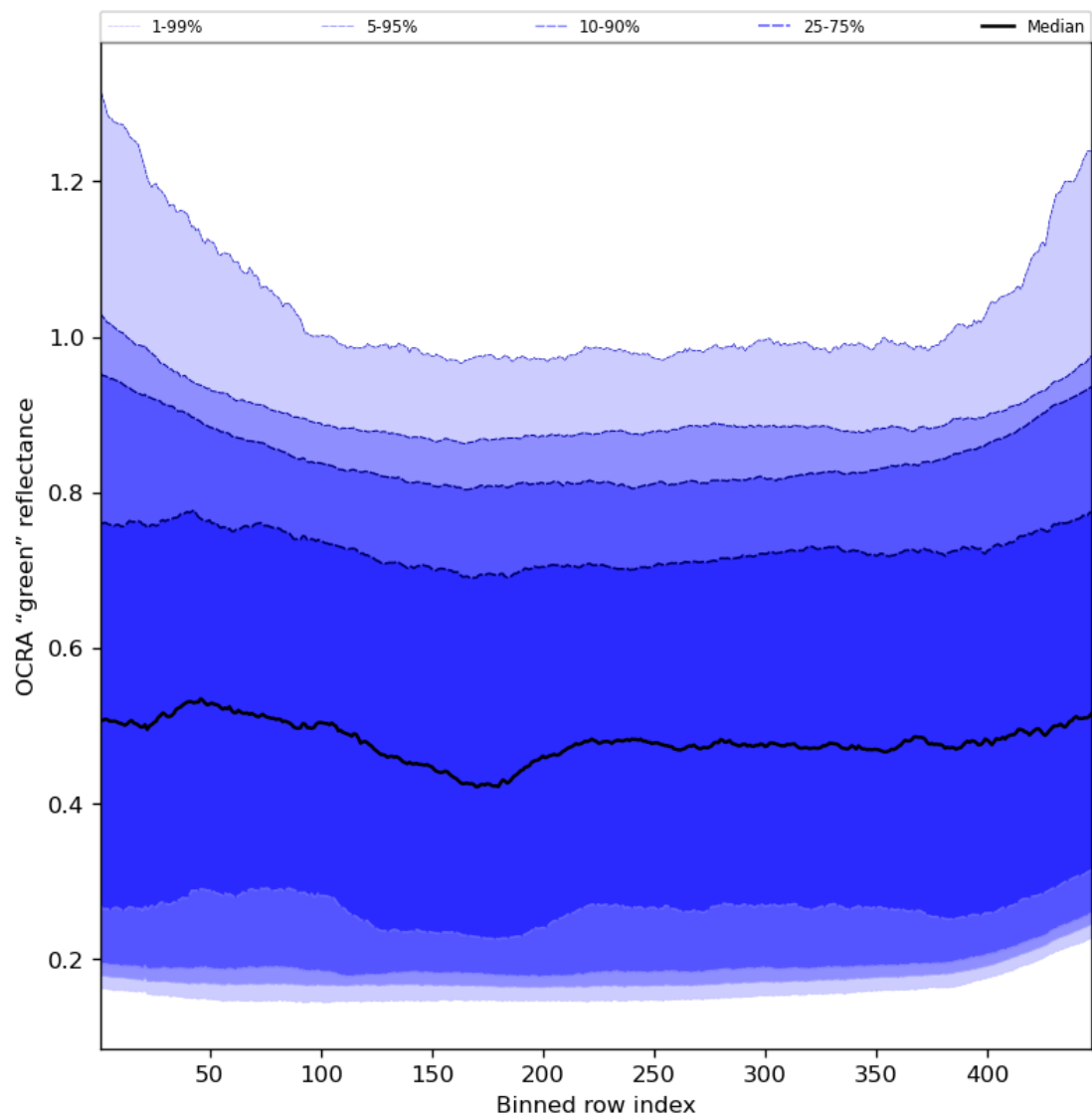
Figure 68: Along track statistics of “OCRA “green” reflectance” for 2024-04-17 to 2024-04-19
