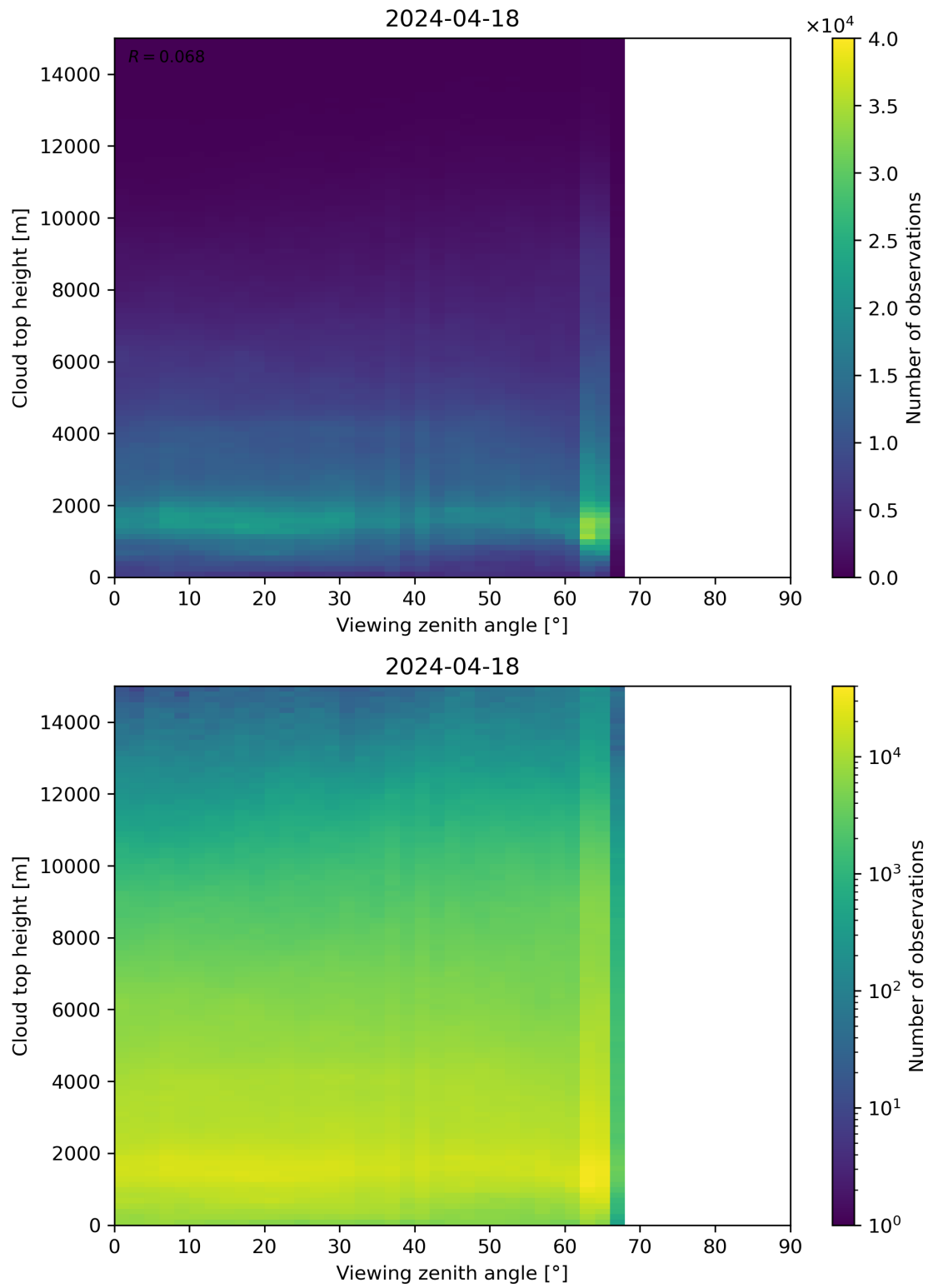
Figure 112: Scatter density plot of “Viewing zenith angle” against “Cloud top height” for 2024-04-17 to 2024-04-19.
