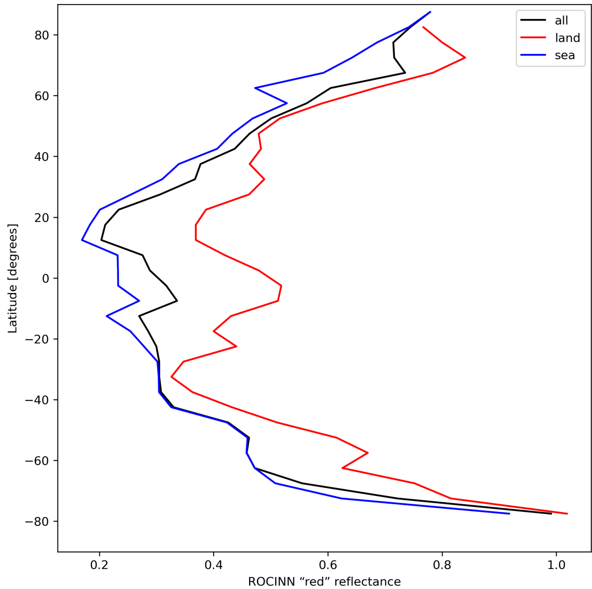
Figure 37: Zonal average of “ROCINN “red” reflectance” for 2024-04-17 to 2024-04-19.
