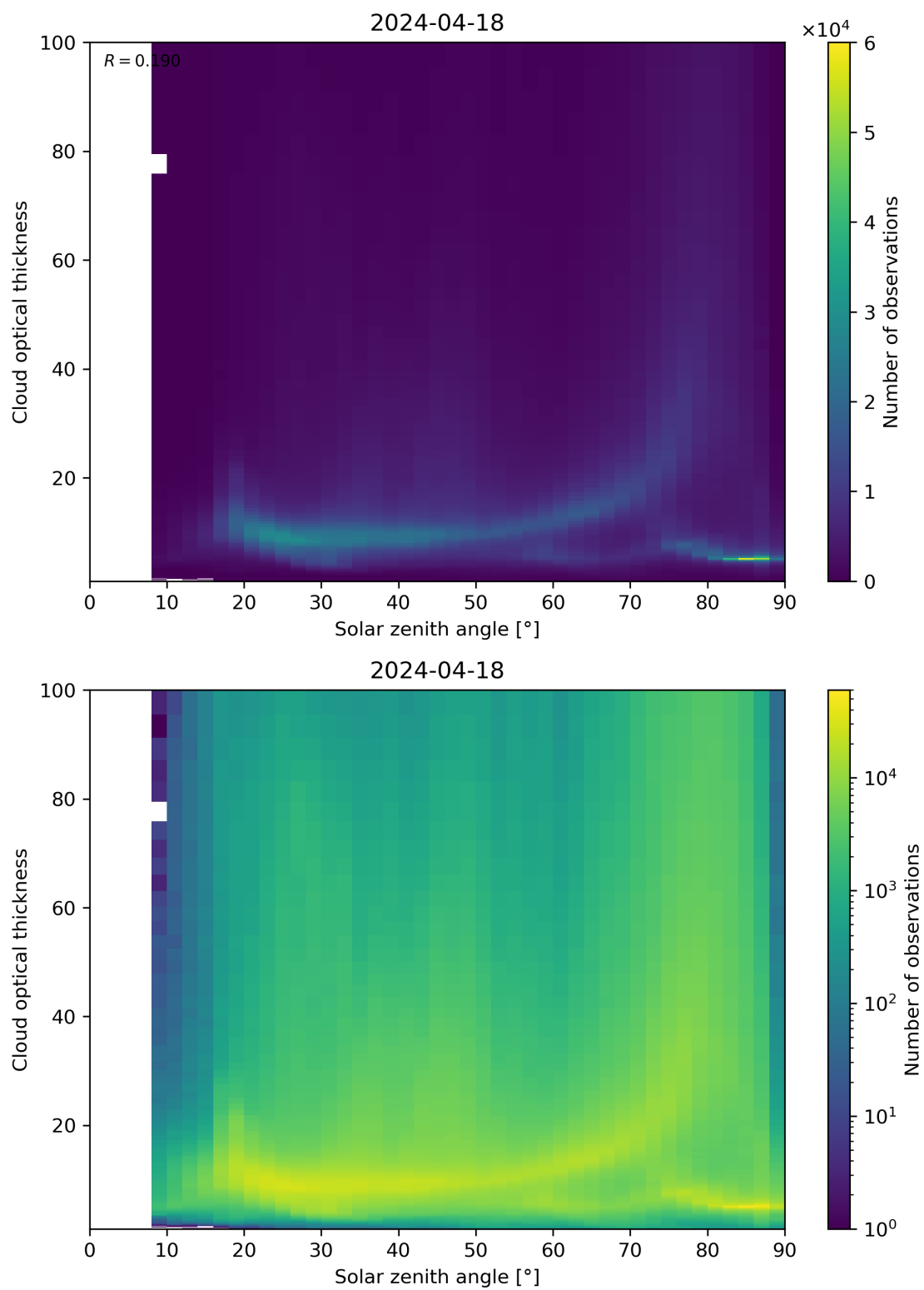
Figure 103: Scatter density plot of “Solar zenith angle” against “Cloud optical thickness” for 2024-04-17 to 2024-04-19.
