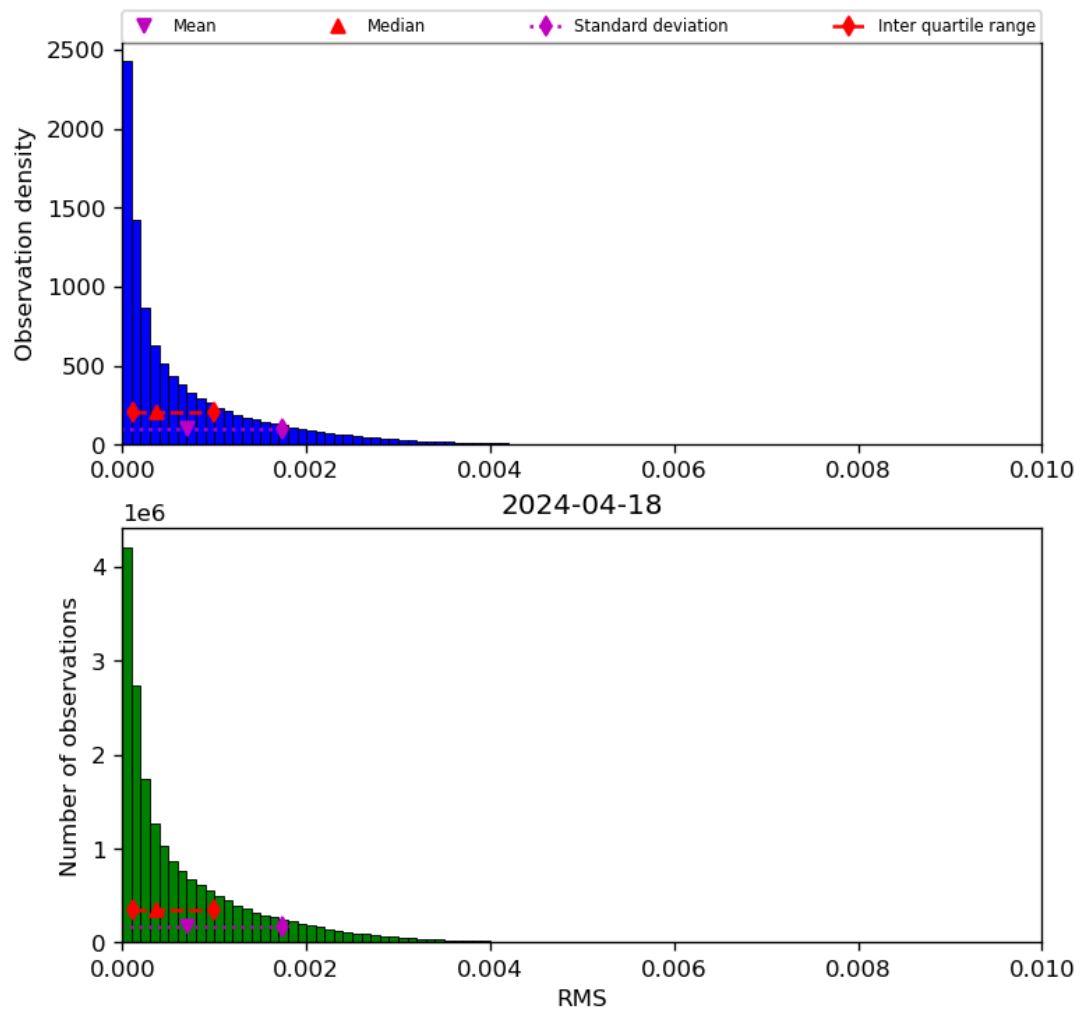
Figure 47: Histogram of “RMS” for 2024-04-17 to 2024-04-19
