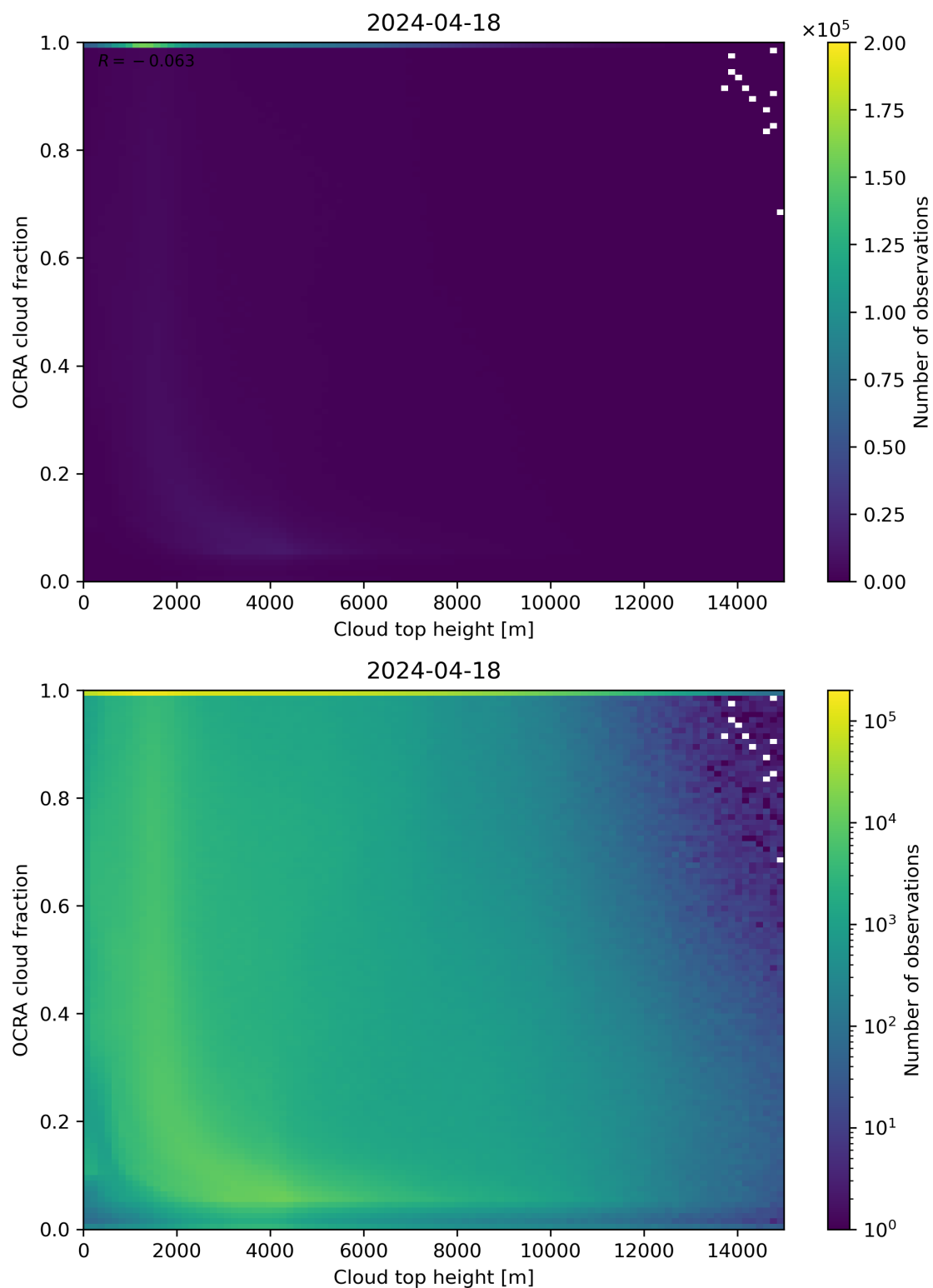
Figure 87: Scatter density plot of “Cloud top height” against “OCRA cloud fraction” for 2024-04-17 to 2024-04-19.
