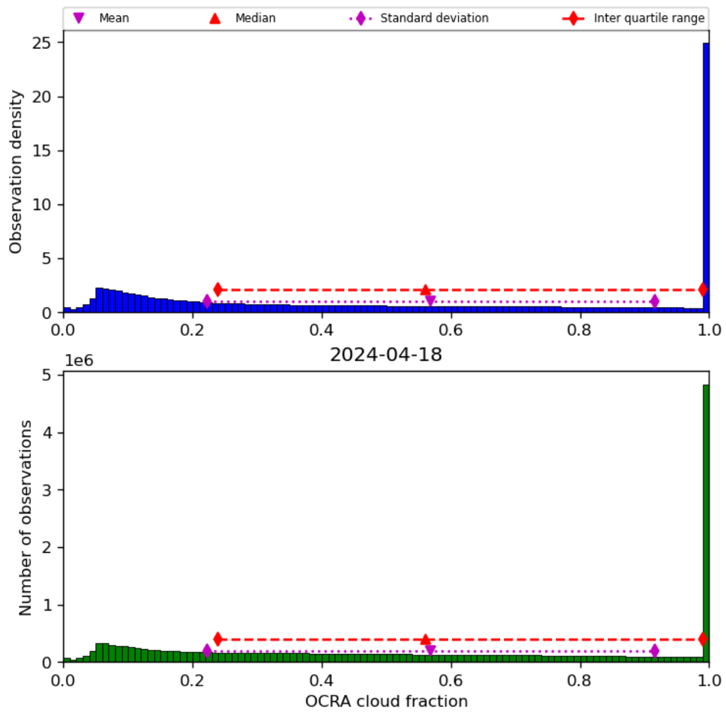
Figure 50: Histogram of “OCRA cloud fraction” for 2024-04-17 to 2024-04-19
