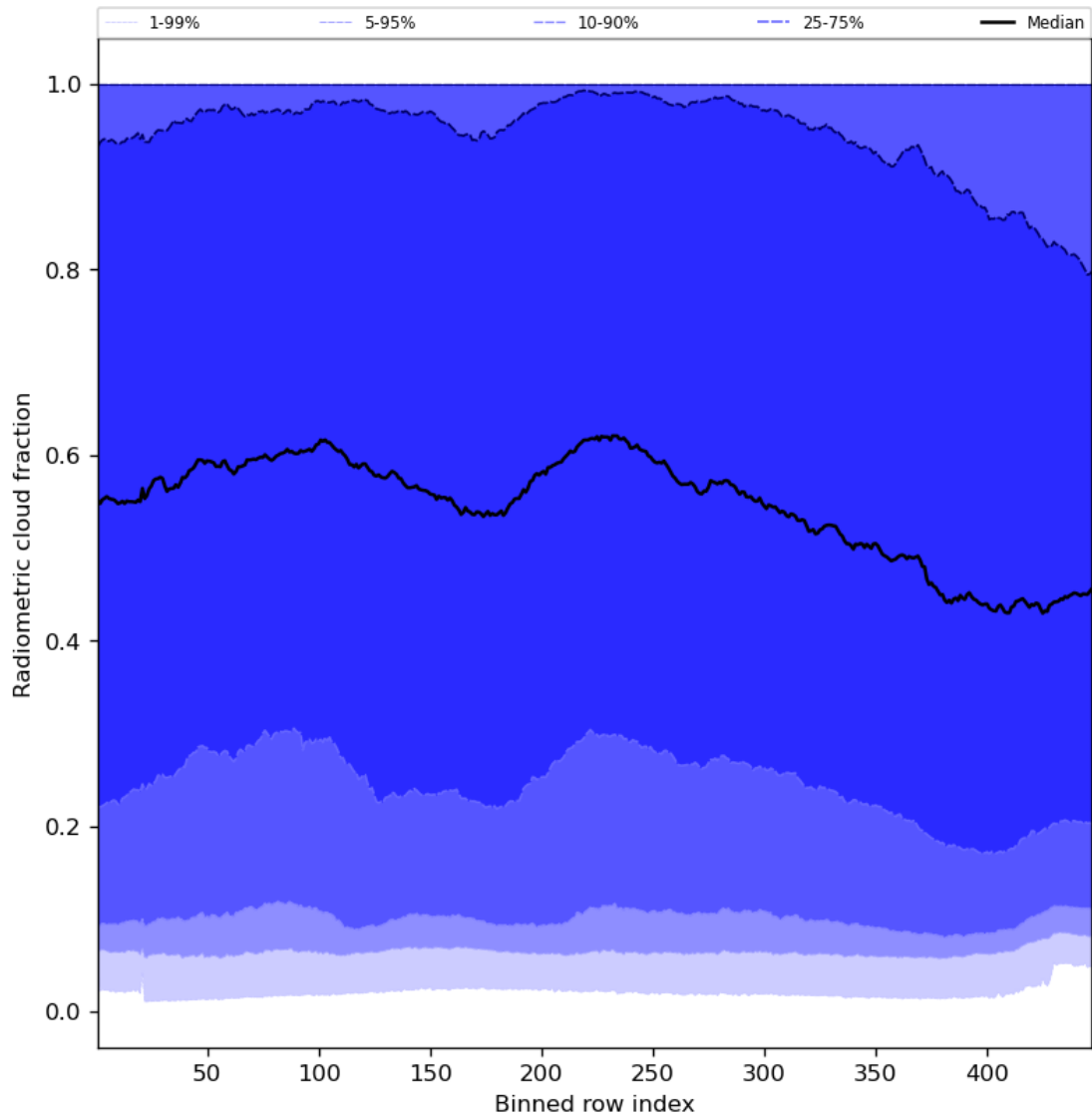
Figure 55: Along track statistics of “Radiometric cloud fraction” for 2024-04-17 to 2024-04-19
