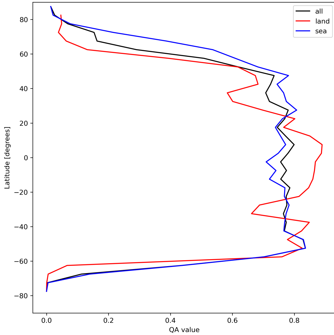
Figure 22: Zonal average of “QA value” for 2024-04-17 to 2024-04-19.
