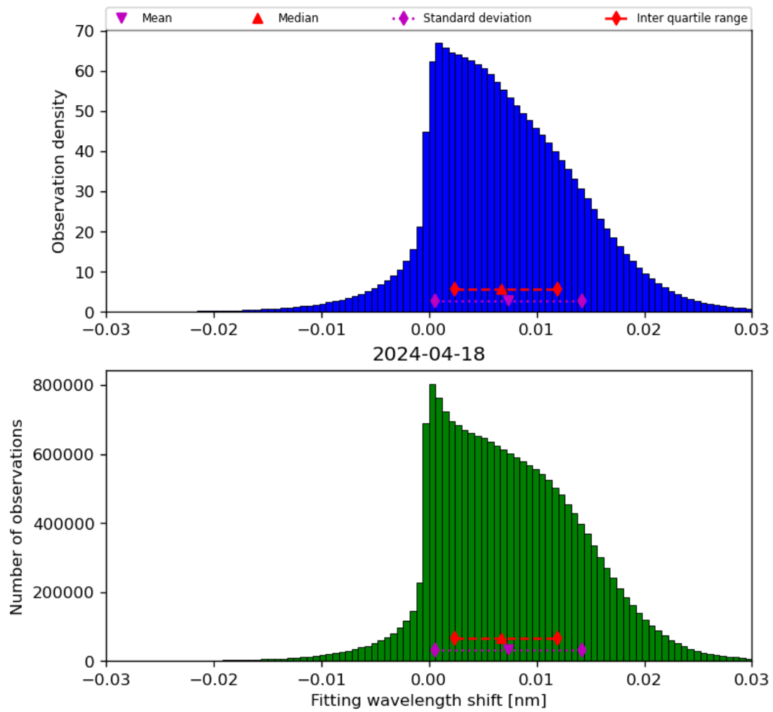
Figure 49: Histogram of “Fitting wavelength shift” for 2024-04-17 to 2024-04-19
