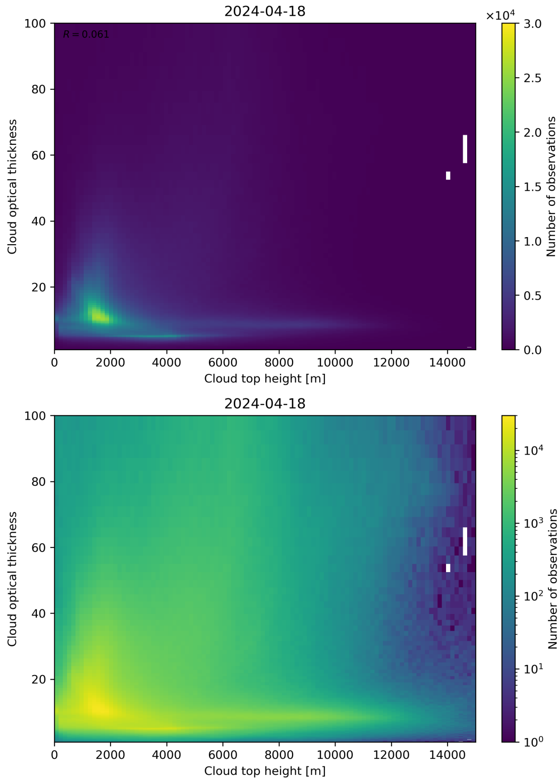
Figure 90: Scatter density plot of “Cloud top height” against “Cloud optical thickness” for 2024-04-17 to 2024-04-19.
