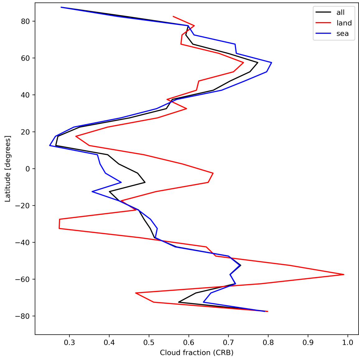
Figure 26: Zonal average of “Cloud fraction (CRB)” for 2024-04-17 to 2024-04-19.
