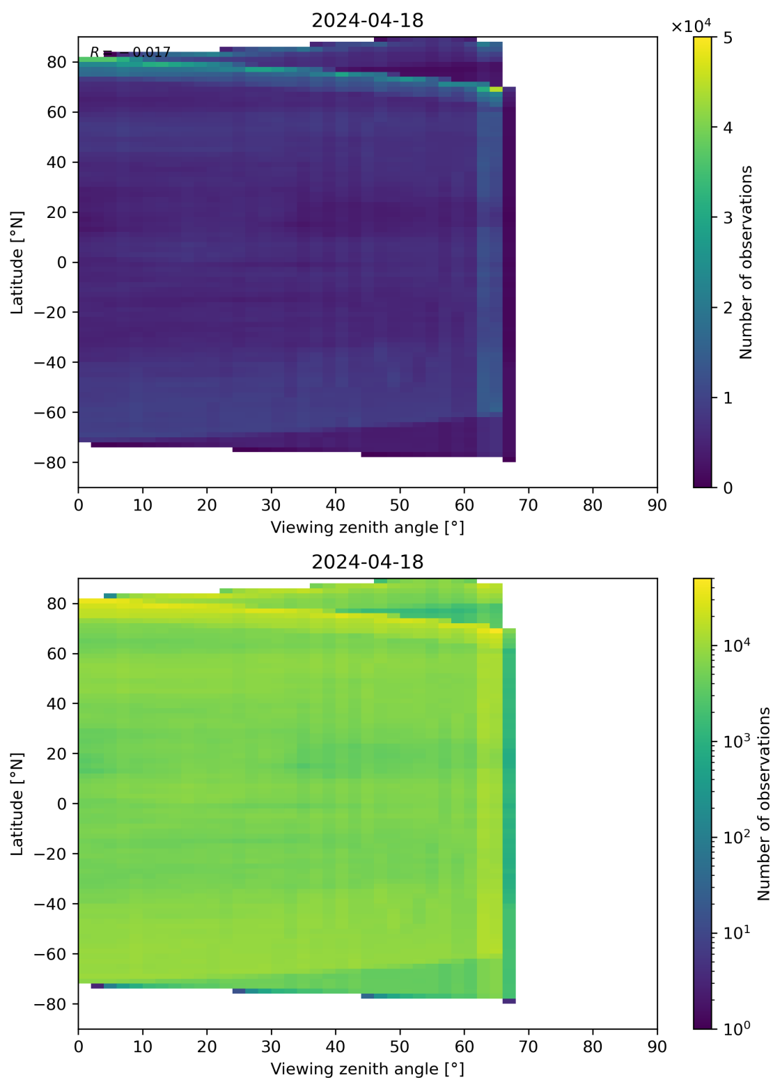
Figure 113: Scatter density plot of “Viewing zenith angle” against “Latitude” for 2024-04-17 to 2024-04-19.
