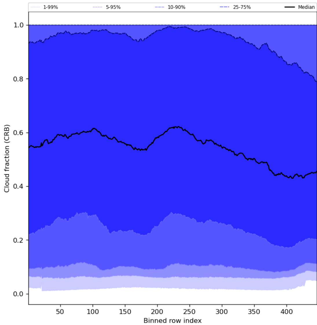
Figure 58: Along track statistics of “Cloud fraction (CRB)” for 2024-04-17 to 2024-04-19
