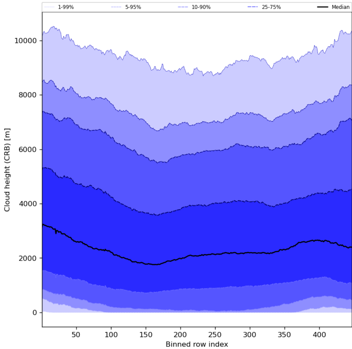
Figure 59: Along track statistics of “Cloud height (CRB)” for 2024-04-17 to 2024-04-19
