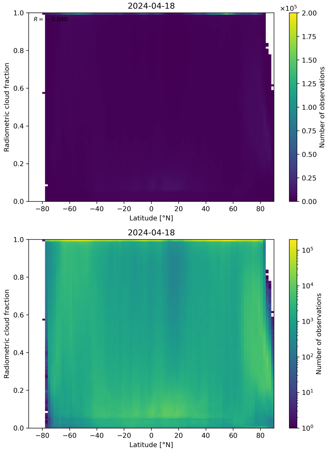
Figure 92: Scatter density plot of “Latitude” against “Radiometric cloud fraction” for 2024-04-17 to 2024-04-19.
