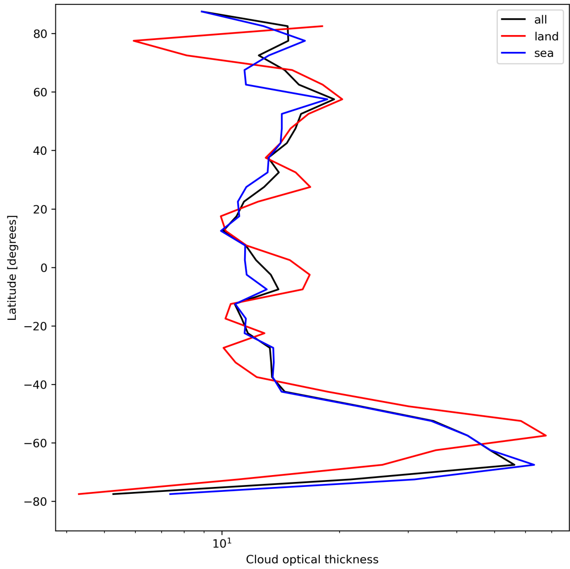
Figure 25: Zonal average of “Cloud optical thickness” for 2024-04-17 to 2024-04-19.
