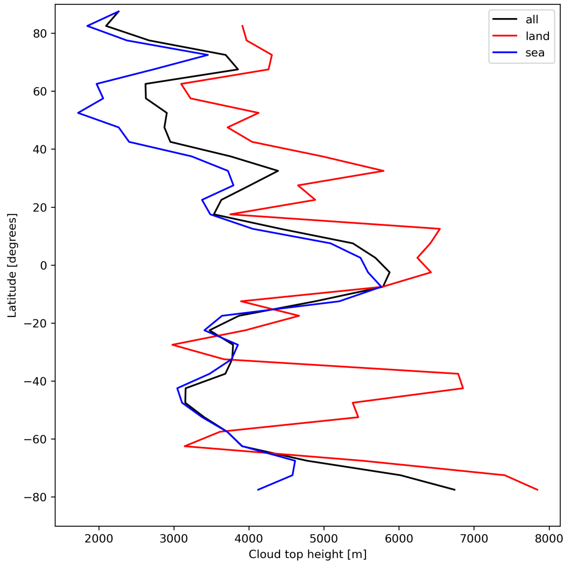
Figure 24: Zonal average of “Cloud top height” for 2024-04-17 to 2024-04-19.
