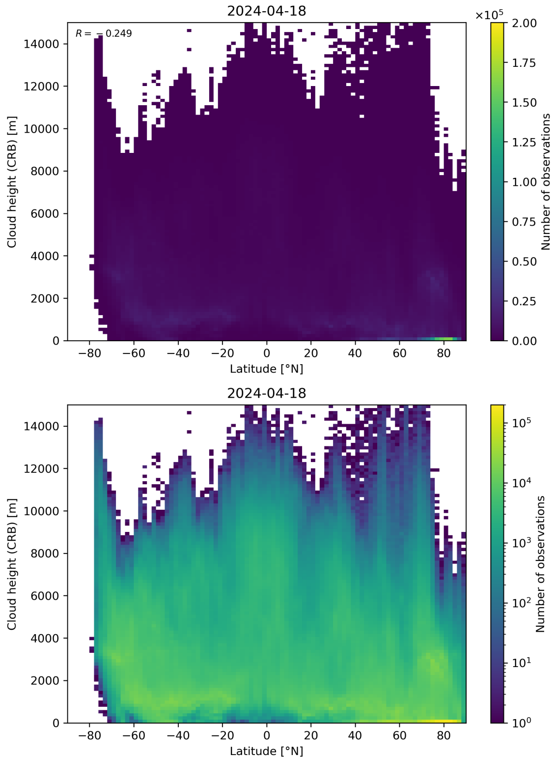
Figure 95: Scatter density plot of “Latitude” against “Cloud height (CRB)” for 2024-04-17 to 2024-04-19.
