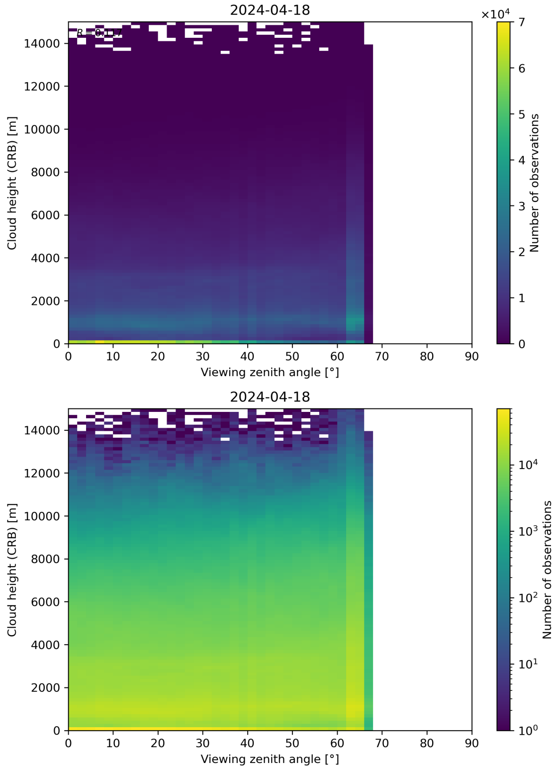
Figure 110: Scatter density plot of “Viewing zenith angle” against “Cloud height (CRB)” for 2024-04-17 to 2024-04-19.
