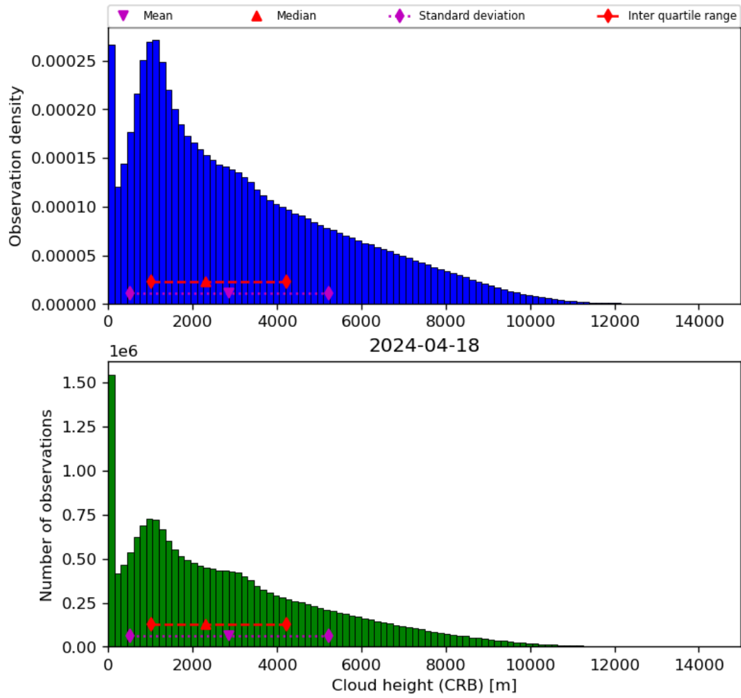
Figure 43: Histogram of “Cloud height (CRB)” for 2024-04-17 to 2024-04-19
