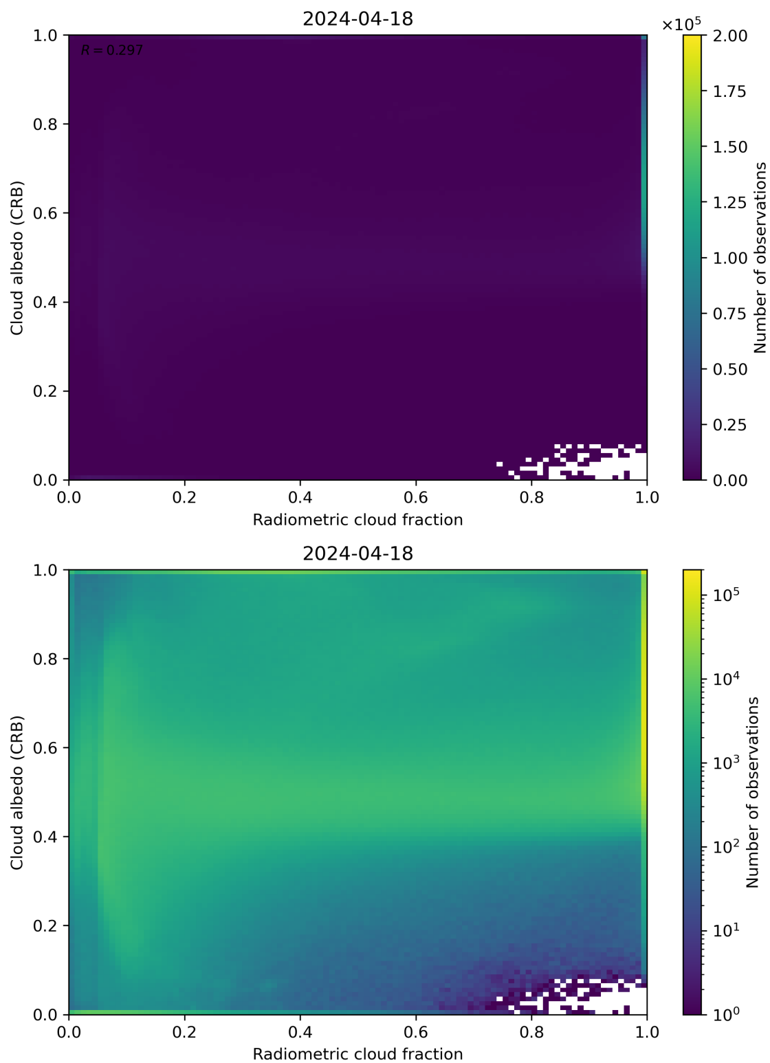
Figure 71: Scatter density plot of “Radiometric cloud fraction” against “Cloud albedo (CRB)” for 2024-04-17 to 2024-04-19.
