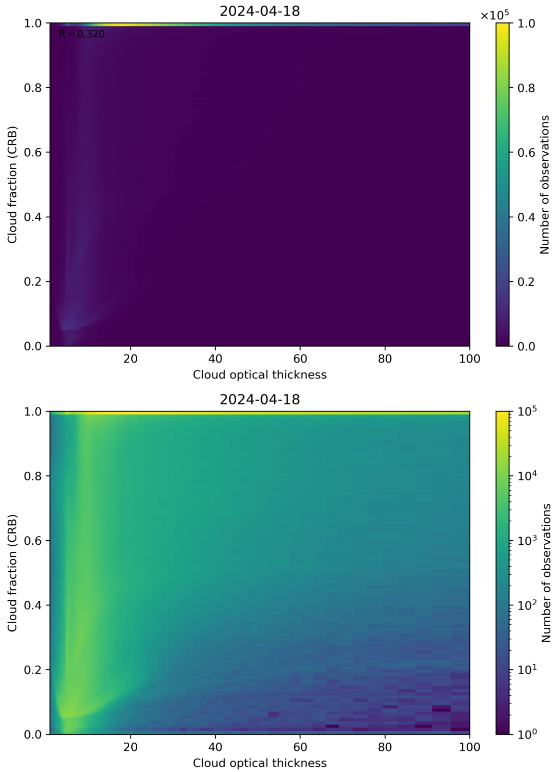
Figure 84: Scatter density plot of “Cloud optical thickness” against “Cloud fraction (CRB)” for 2024-04-17 to 2024-04-19.
