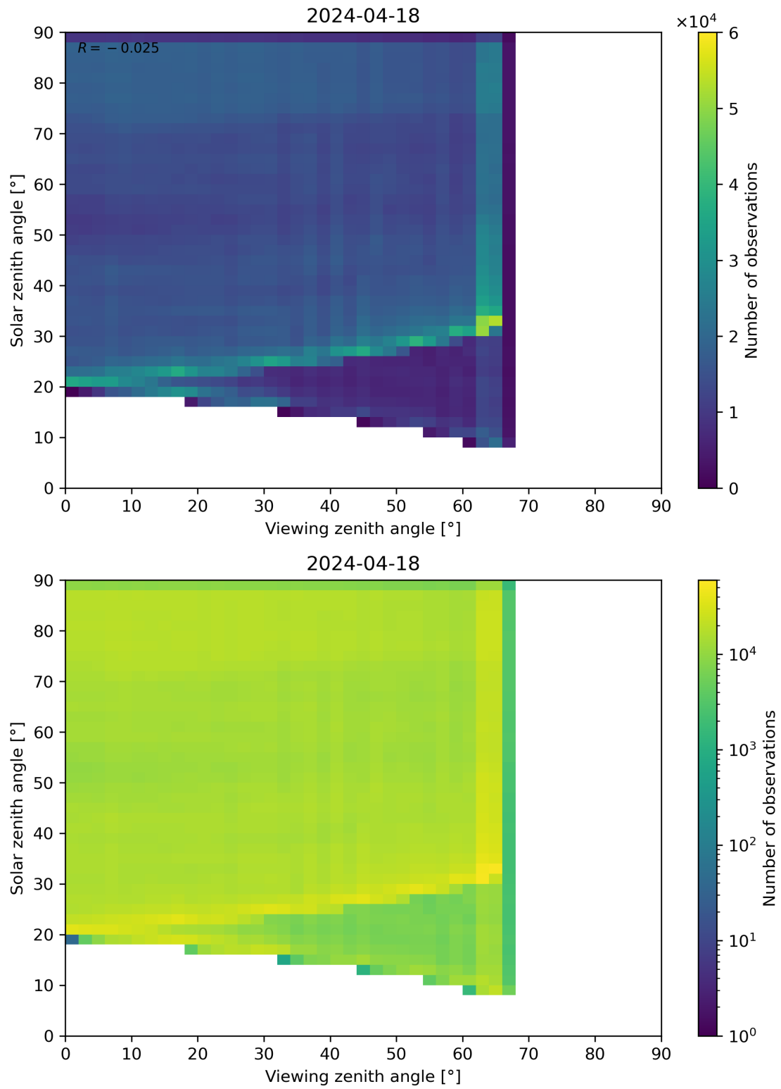
Figure 114: Scatter density plot of “Viewing zenith angle” against “Solar zenith angle” for 2024-04-17 to 2024-04-19.
