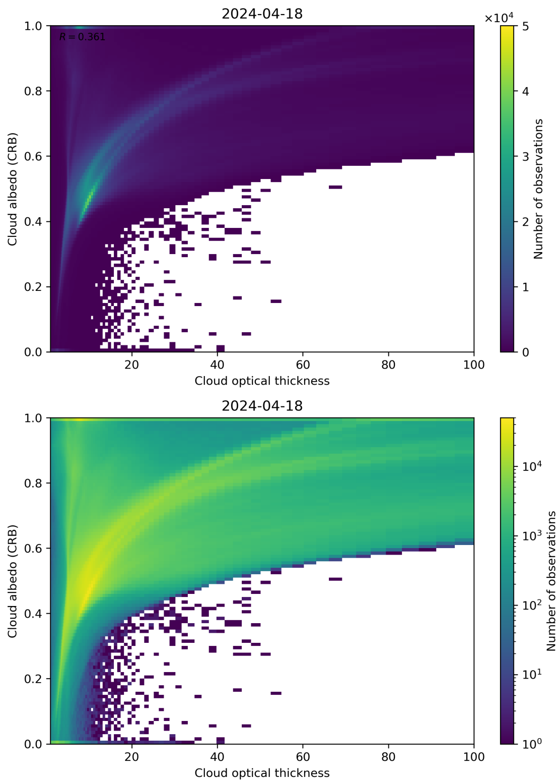
Figure 82: Scatter density plot of “Cloud optical thickness” against “Cloud albedo (CRB)” for 2024-04-17 to 2024-04-19.
