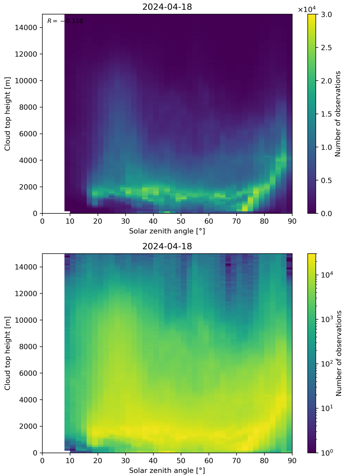
Figure 104: Scatter density plot of “Solar zenith angle” against “Cloud top height” for 2024-04-17 to 2024-04-19.
