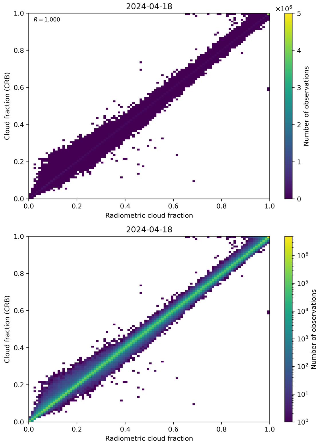
Figure 73: Scatter density plot of “Radiometric cloud fraction” against “Cloud fraction (CRB)” for 2024-04-17 to 2024-04-19.
