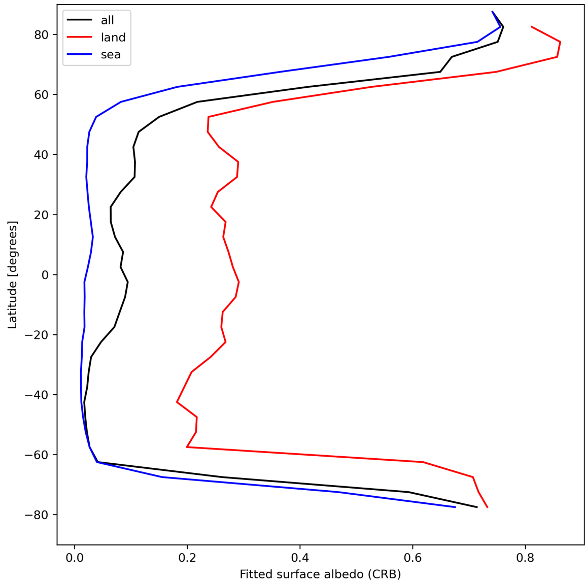
Figure 30: Zonal average of “Fitted surface albedo (CRB)” for 2024-04-17 to 2024-04-19.
