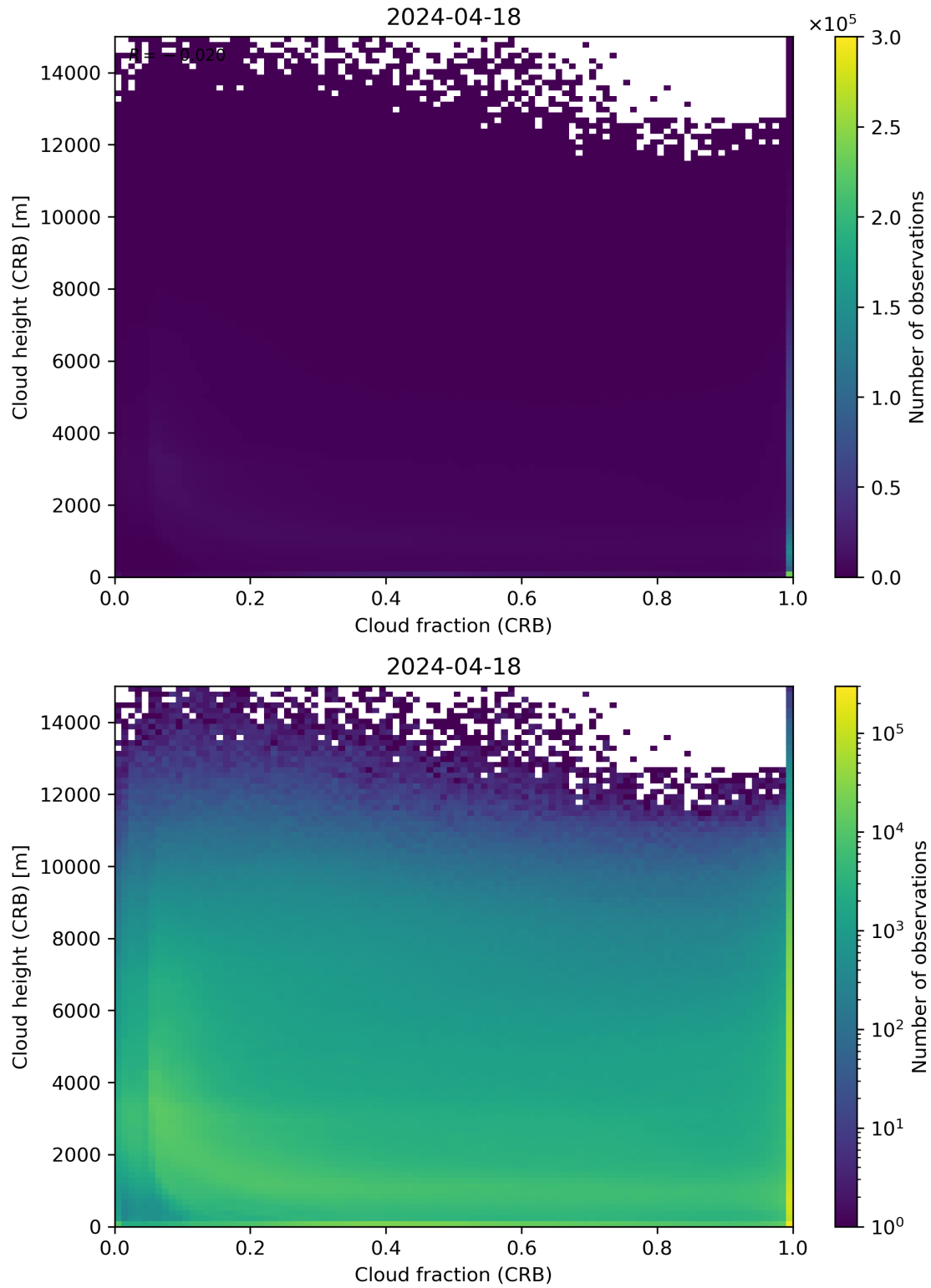
Figure 79: Scatter density plot of “Cloud fraction (CRB)” against “Cloud height (CRB)” for 2024-04-17 to 2024-04-19.
