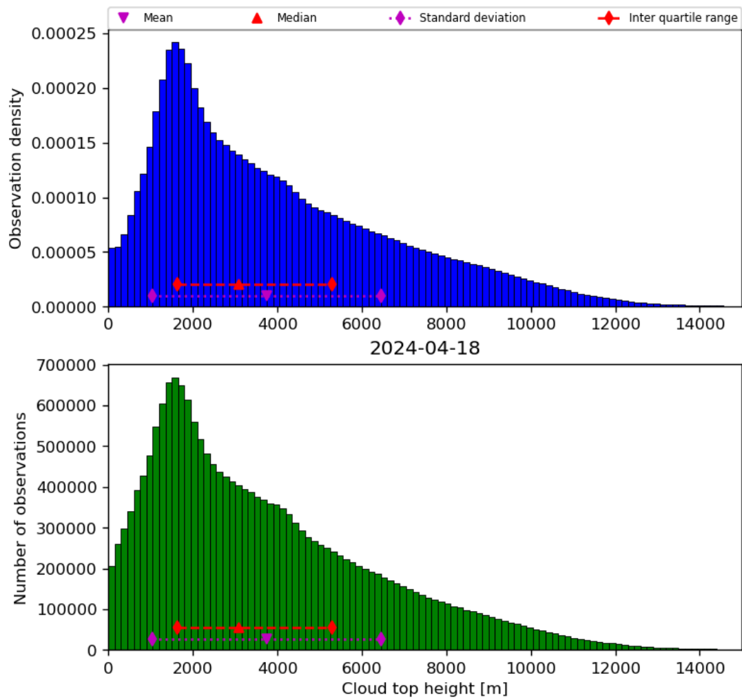
Figure 40: Histogram of “Cloud top height” for 2024-04-17 to 2024-04-19
