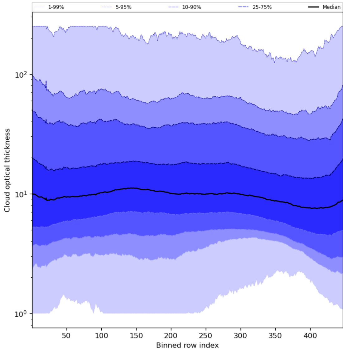
Figure 57: Along track statistics of “Cloud optical thickness” for 2024-04-17 to 2024-04-19
