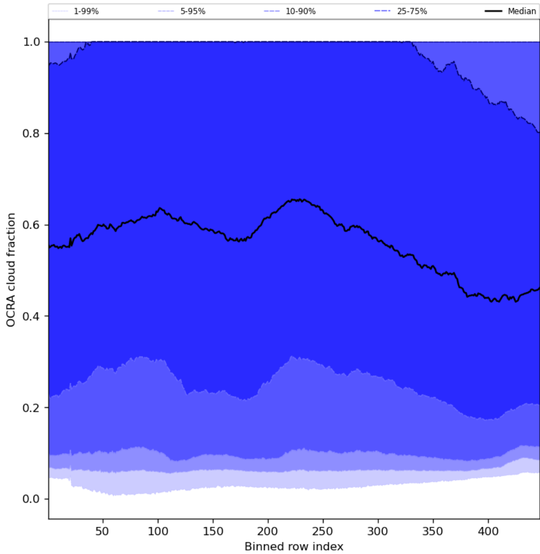
Figure 66: Along track statistics of “OCRA cloud fraction” for 2024-04-17 to 2024-04-19
