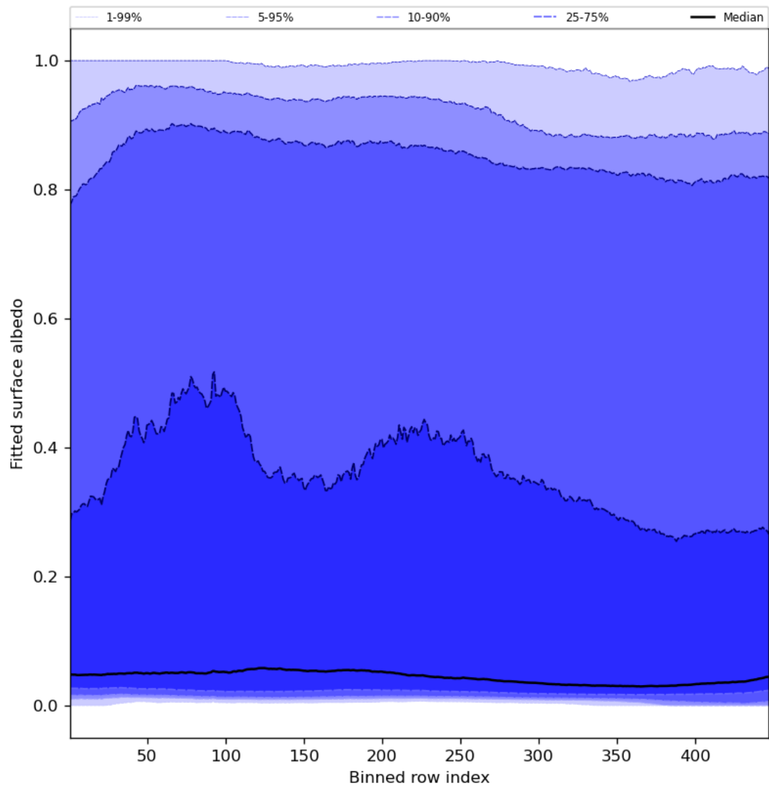
Figure 61: Along track statistics of “Fitted surface albedo” for 2024-04-17 to 2024-04-19
