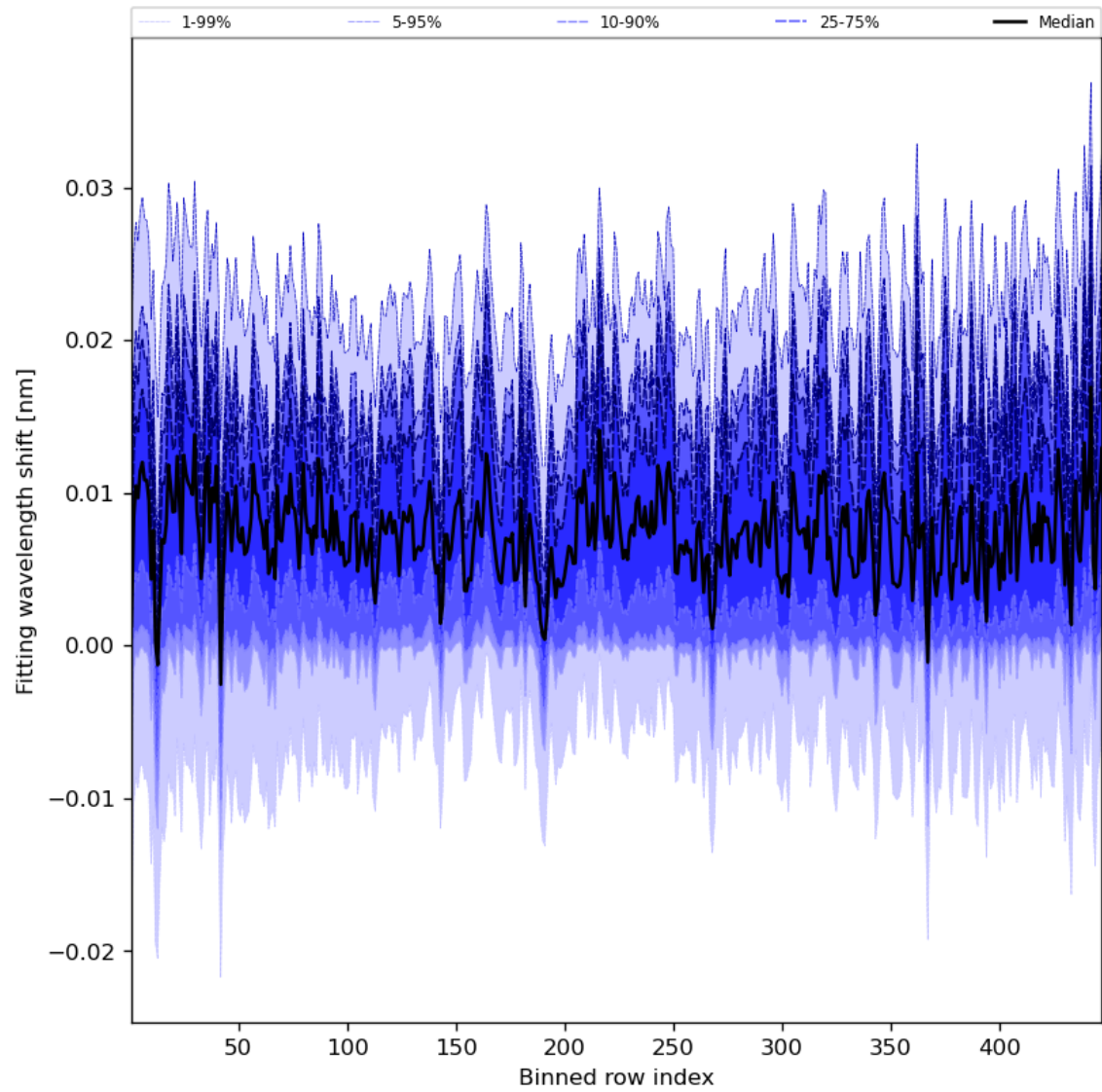
Figure 65: Along track statistics of “Fitting wavelength shift” for 2024-04-17 to 2024-04-19
