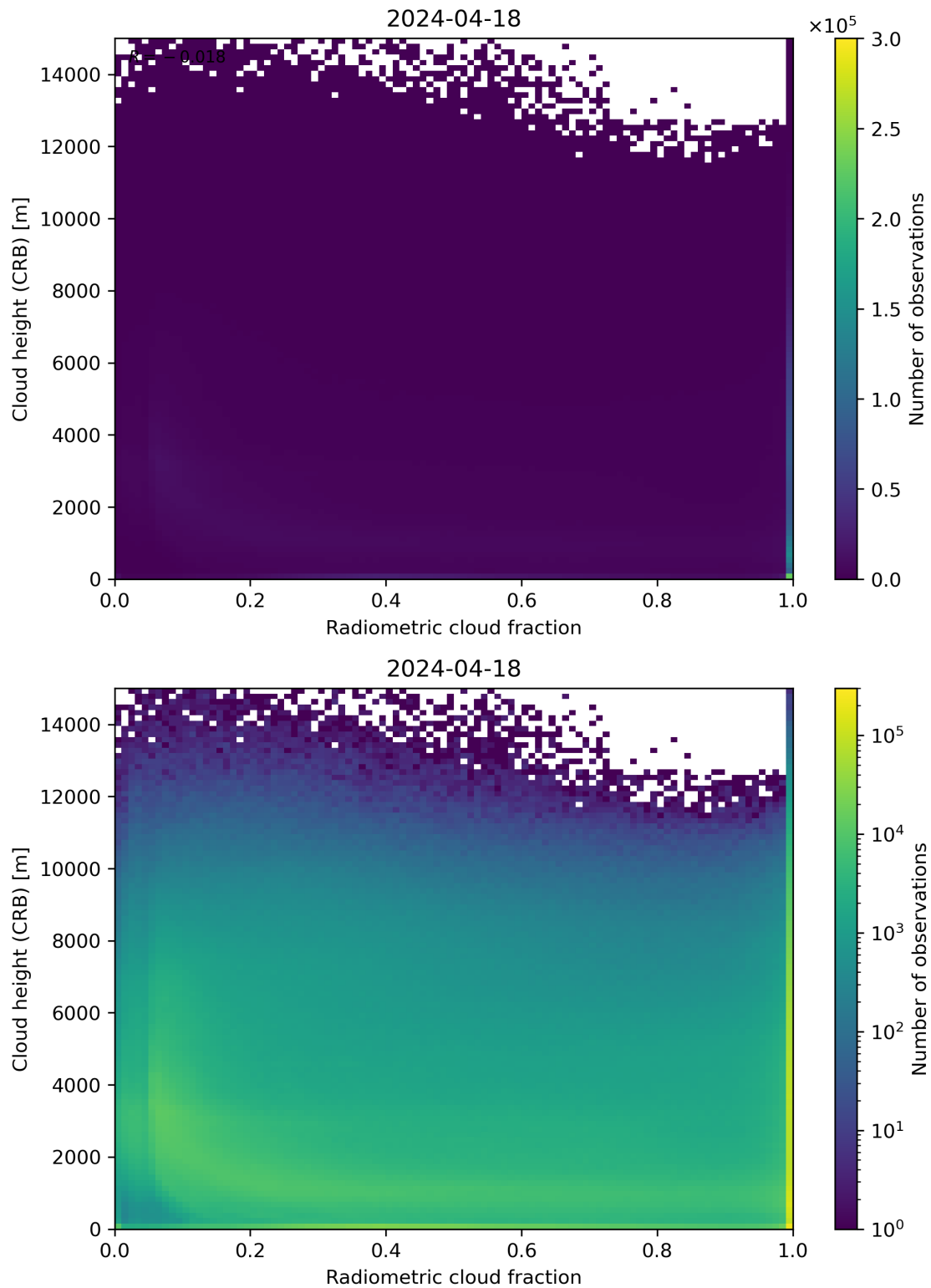
Figure 74: Scatter density plot of “Radiometric cloud fraction” against “Cloud height (CRB)” for 2024-04-17 to 2024-04-19.
