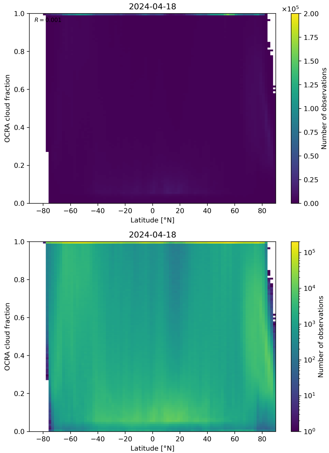
Figure 93: Scatter density plot of “Latitude” against “OCRA cloud fraction” for 2024-04-17 to 2024-04-19.
