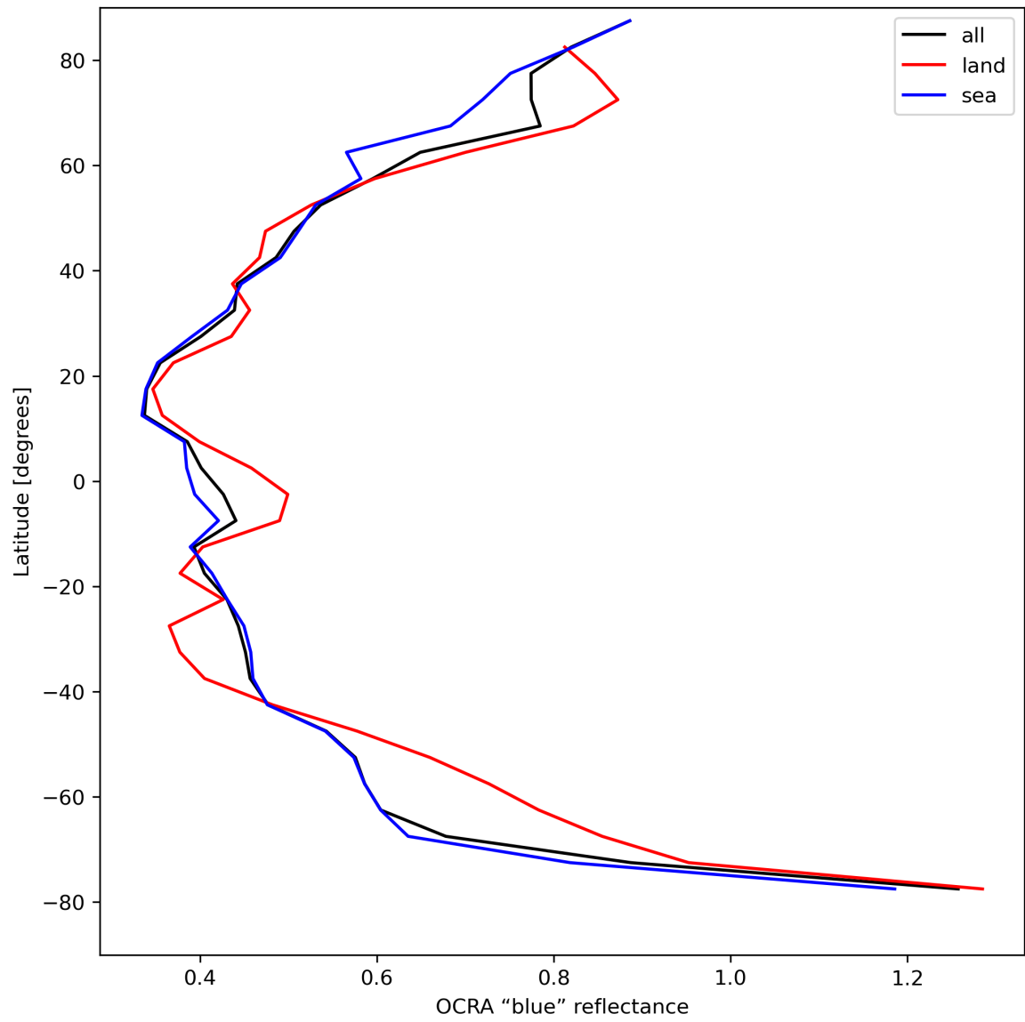
Figure 35: Zonal average of “OCRA “blue” reflectance” for 2024-04-17 to 2024-04-19.
