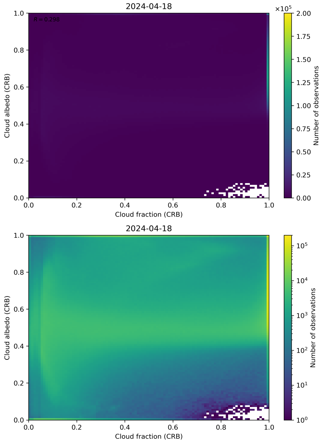
Figure 77: Scatter density plot of “Cloud fraction (CRB)” against “Cloud albedo (CRB)” for 2024-04-17 to 2024-04-19.
