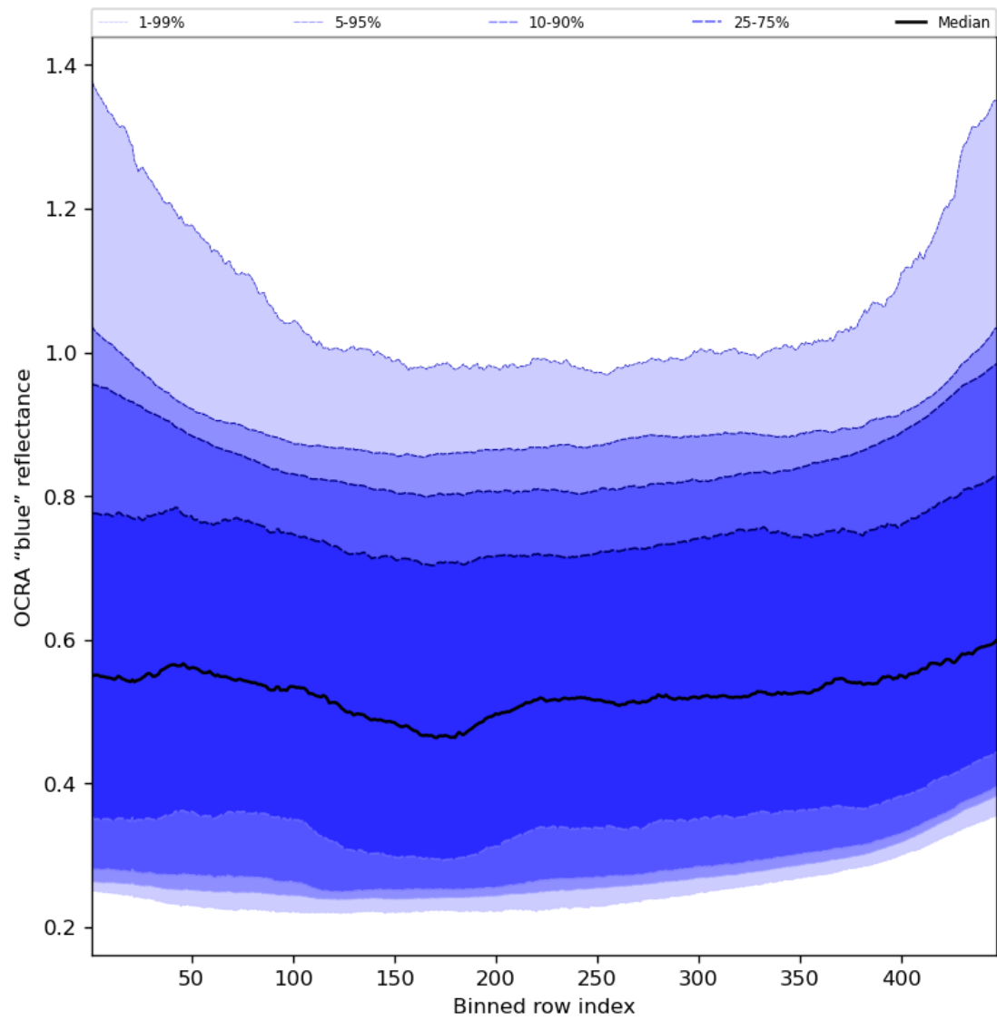
Figure 67: Along track statistics of “OCRA “blue” reflectance” for 2024-04-17 to 2024-04-19
