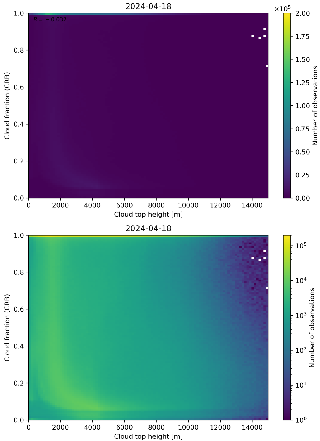
Figure 88: Scatter density plot of “Cloud top height” against “Cloud fraction (CRB)” for 2024-04-17 to 2024-04-19.
