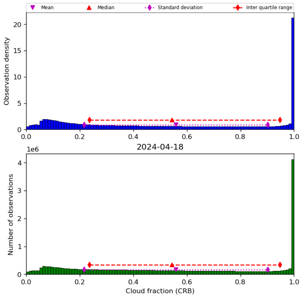
Figure 42: Histogram of “Cloud fraction (CRB)” for 2024-04-17 to 2024-04-19
