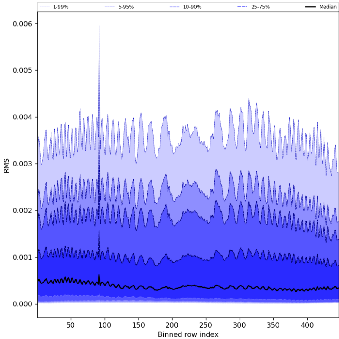
Figure 63: Along track statistics of “RMS” for 2024-04-17 to 2024-04-19
