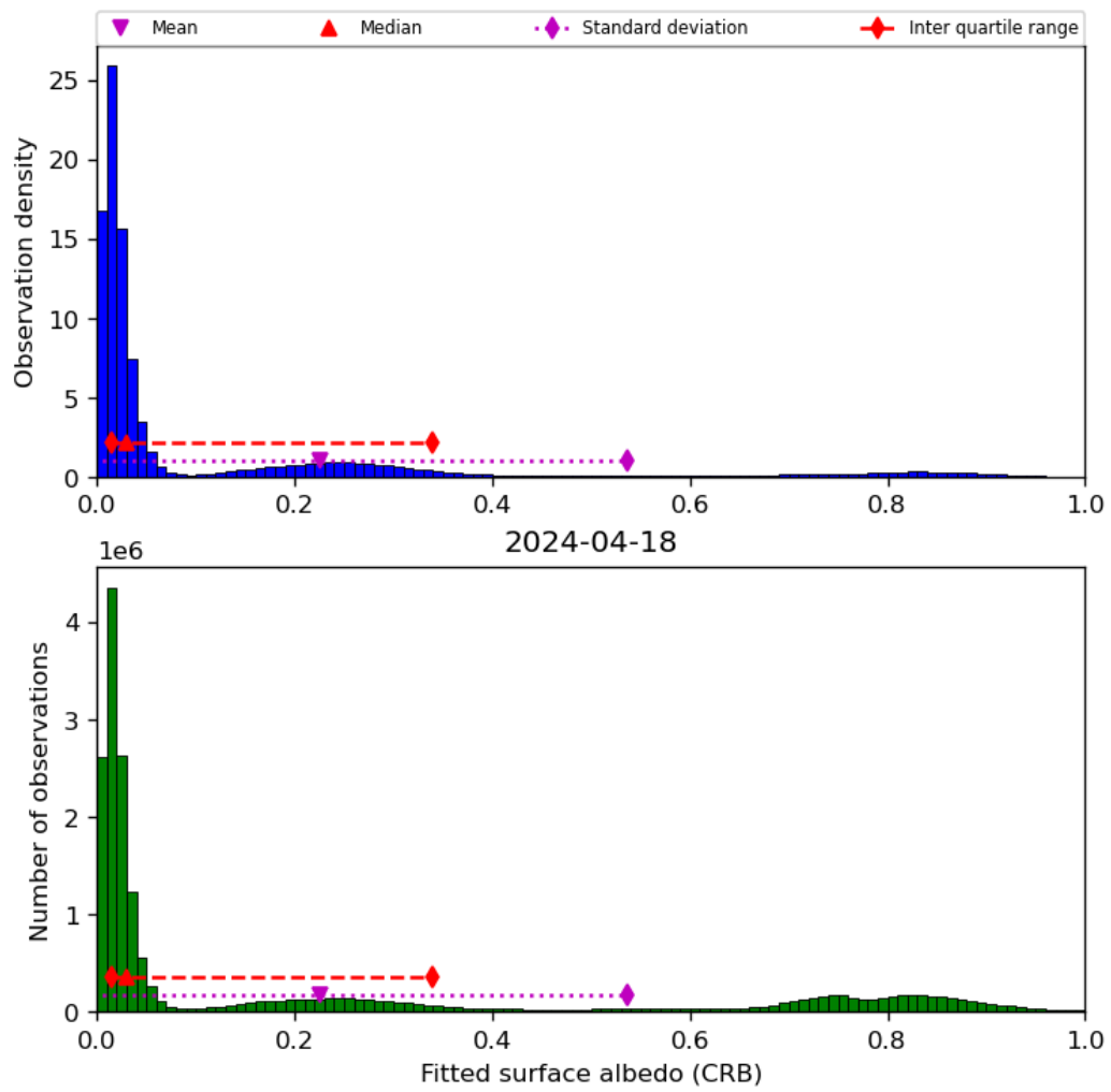
Figure 46: Histogram of “Fitted surface albedo (CRB)” for 2024-04-17 to 2024-04-19
