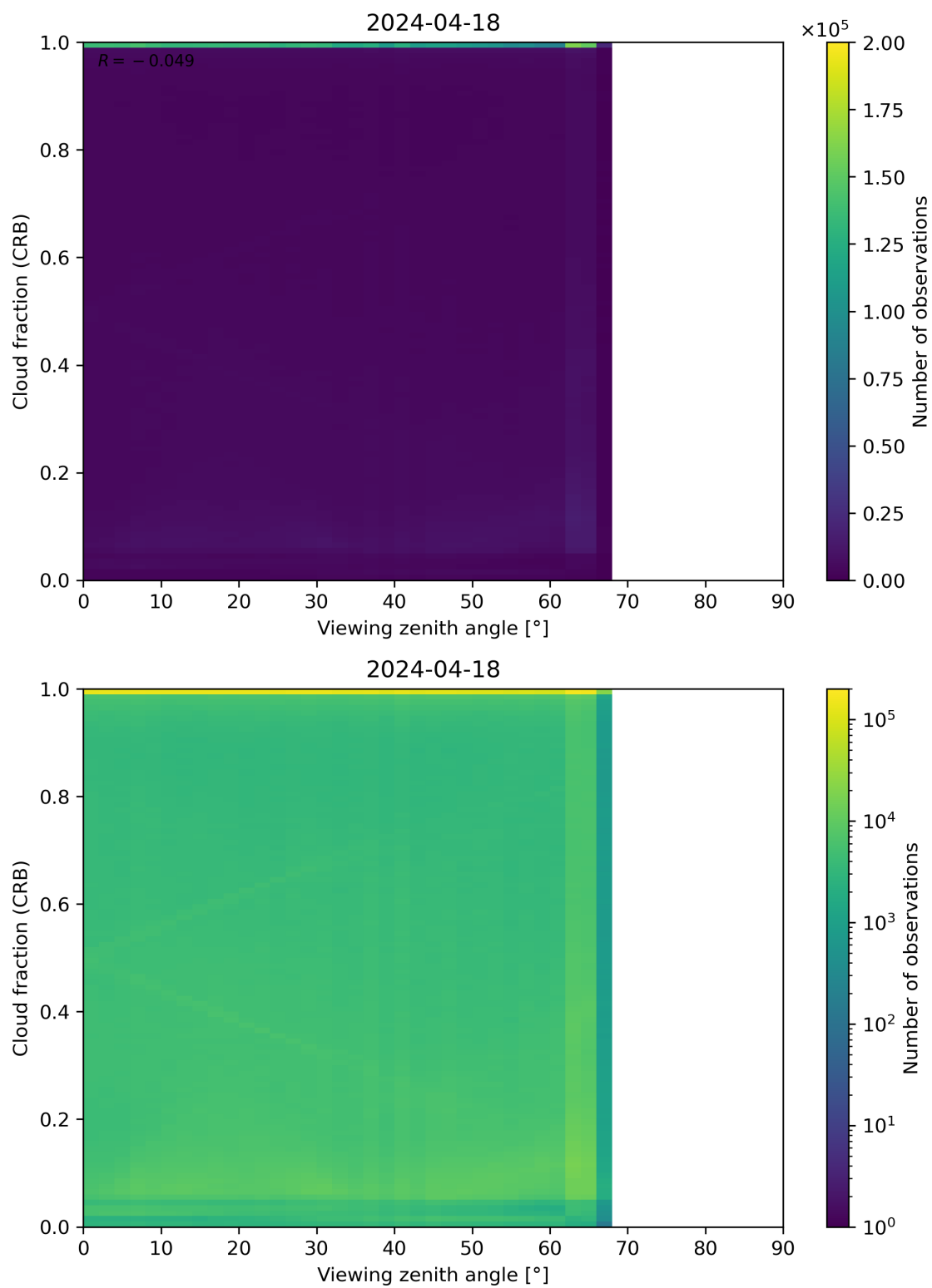
Figure 109: Scatter density plot of “Viewing zenith angle” against “Cloud fraction (CRB)” for 2024-04-17 to 2024-04-19.
