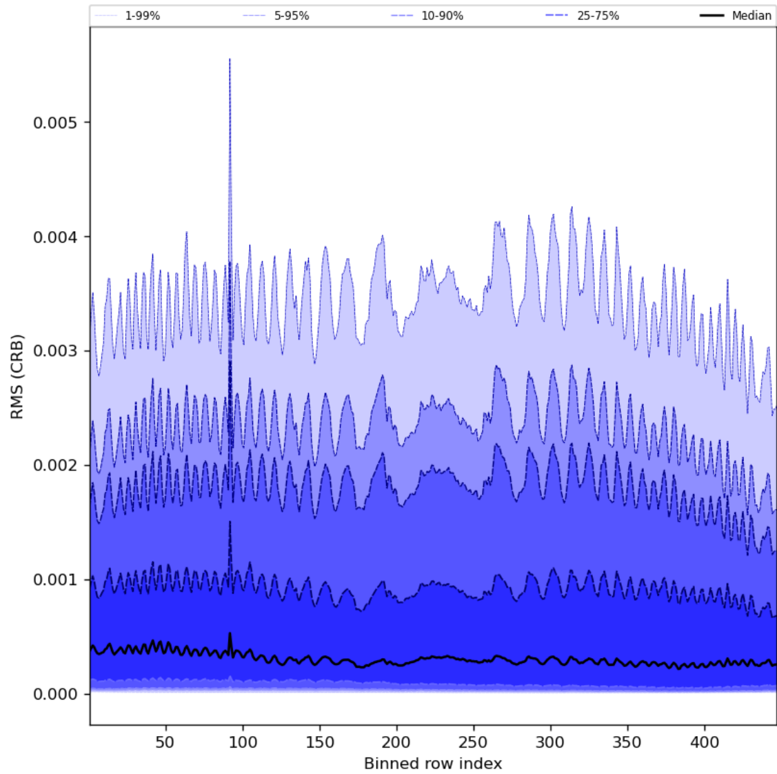
Figure 64: Along track statistics of “RMS (CRB)” for 2024-04-17 to 2024-04-19
