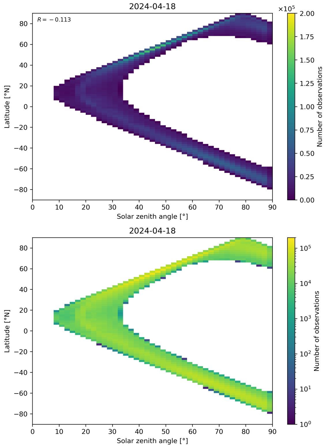
Figure 105: Scatter density plot of “Solar zenith angle” against “Latitude” for 2024-04-17 to 2024-04-19.
