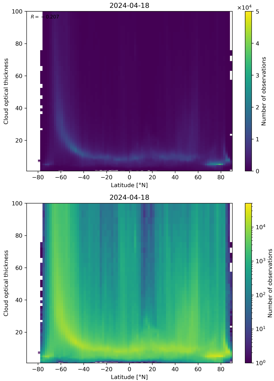
Figure 96: Scatter density plot of “Latitude” against “Cloud optical thickness” for 2024-04-17 to 2024-04-19.
