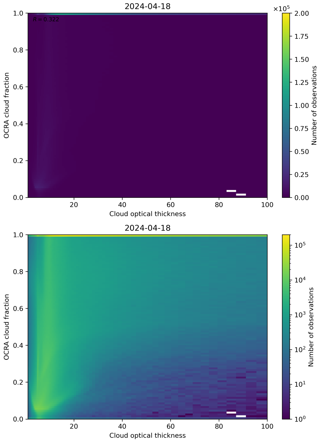
Figure 83: Scatter density plot of “Cloud optical thickness” against “OCRA cloud fraction” for 2024-04-17 to 2024-04-19.
