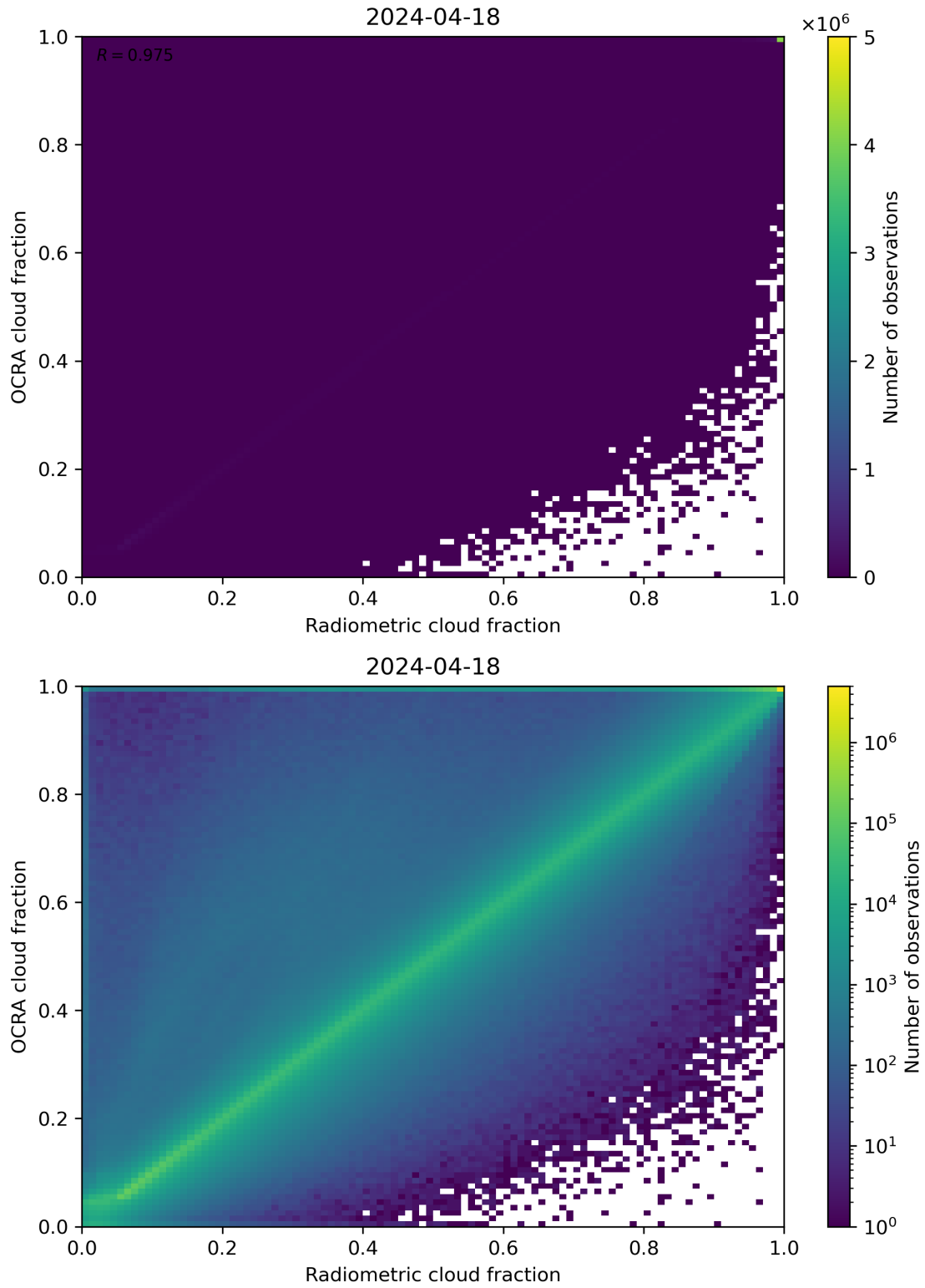
Figure 72: Scatter density plot of “Radiometric cloud fraction” against “OCRA cloud fraction” for 2024-04-17 to 2024-04-19.
