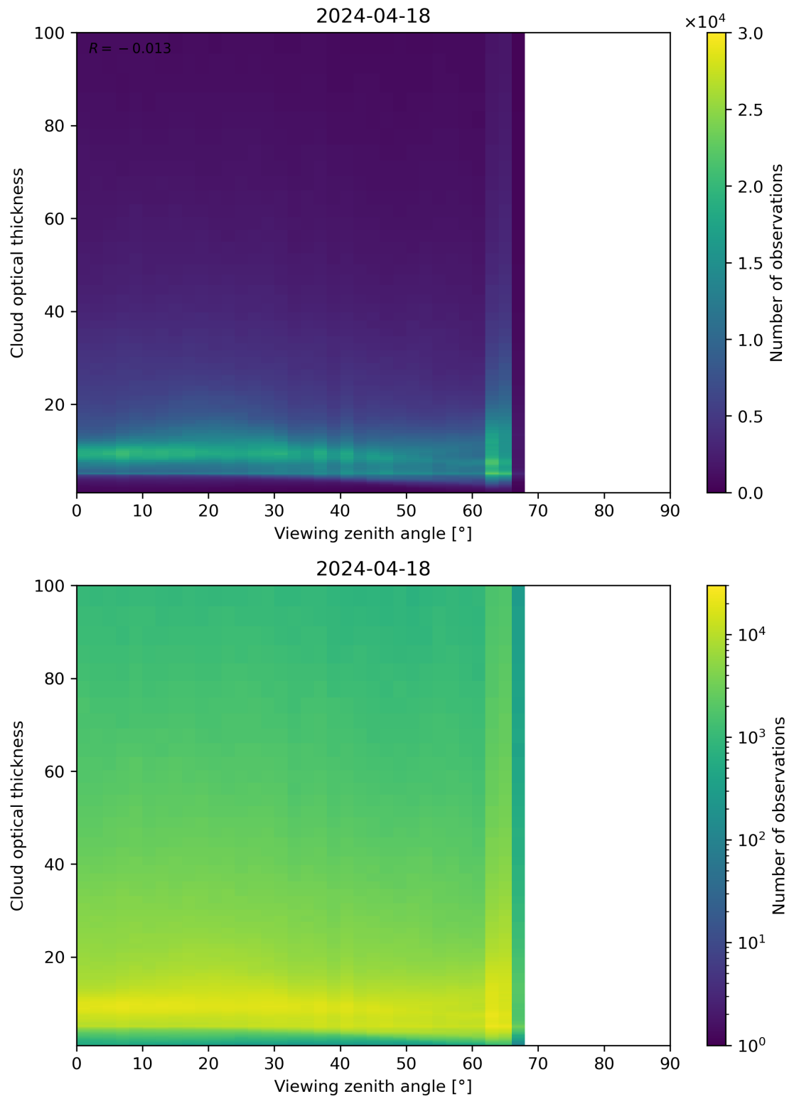
Figure 111: Scatter density plot of “Viewing zenith angle” against “Cloud optical thickness” for 2024-04-17 to 2024-04-19.
