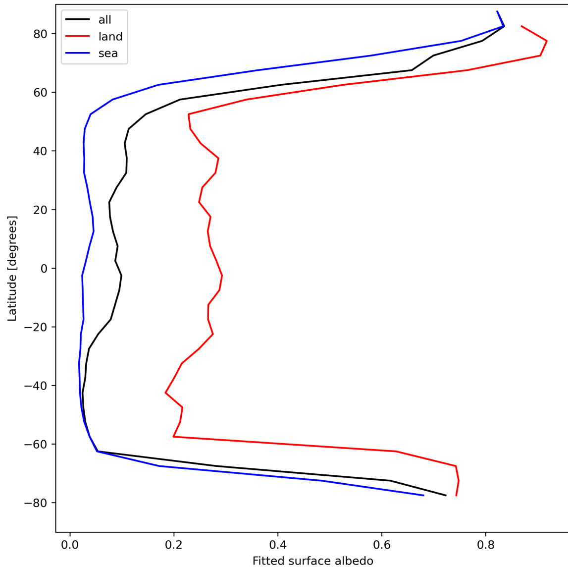
Figure 29: Zonal average of “Fitted surface albedo” for 2024-04-17 to 2024-04-19.
