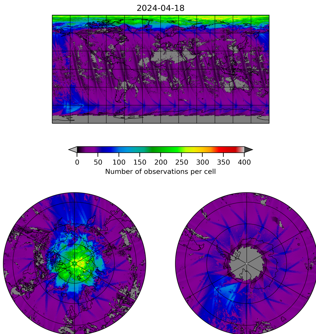
Figure 21: Map of the number of observations for 2024-04-17 to 2024-04-19
