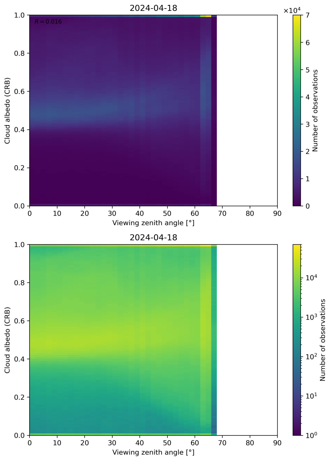
Figure 106: Scatter density plot of “Viewing zenith angle” against “Cloud albedo (CRB)” for 2024-04-17 to 2024-04-19.
