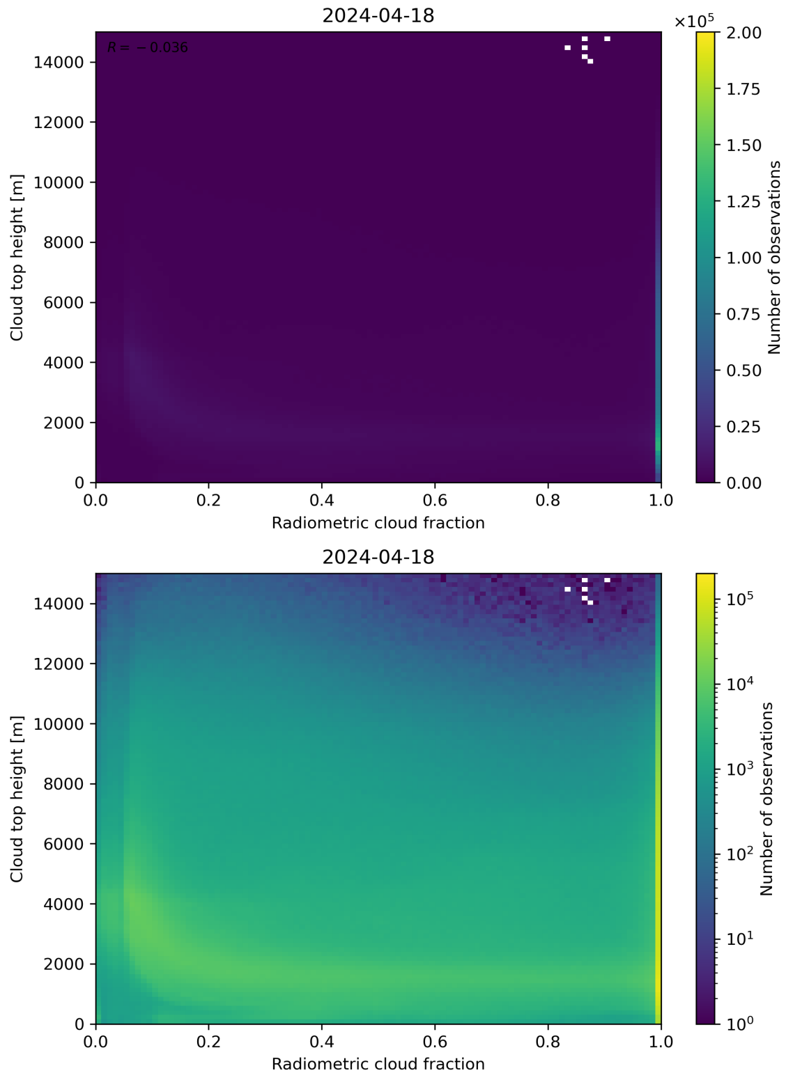
Figure 76: Scatter density plot of “Radiometric cloud fraction” against “Cloud top height” for 2024-04-17 to 2024-04-19.
