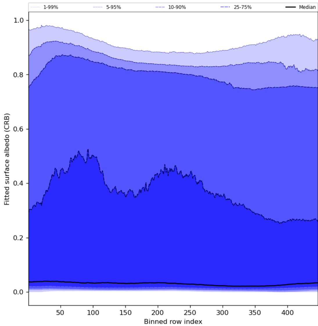
Figure 62: Along track statistics of “Fitted surface albedo (CRB)” for 2024-04-17 to 2024-04-19
