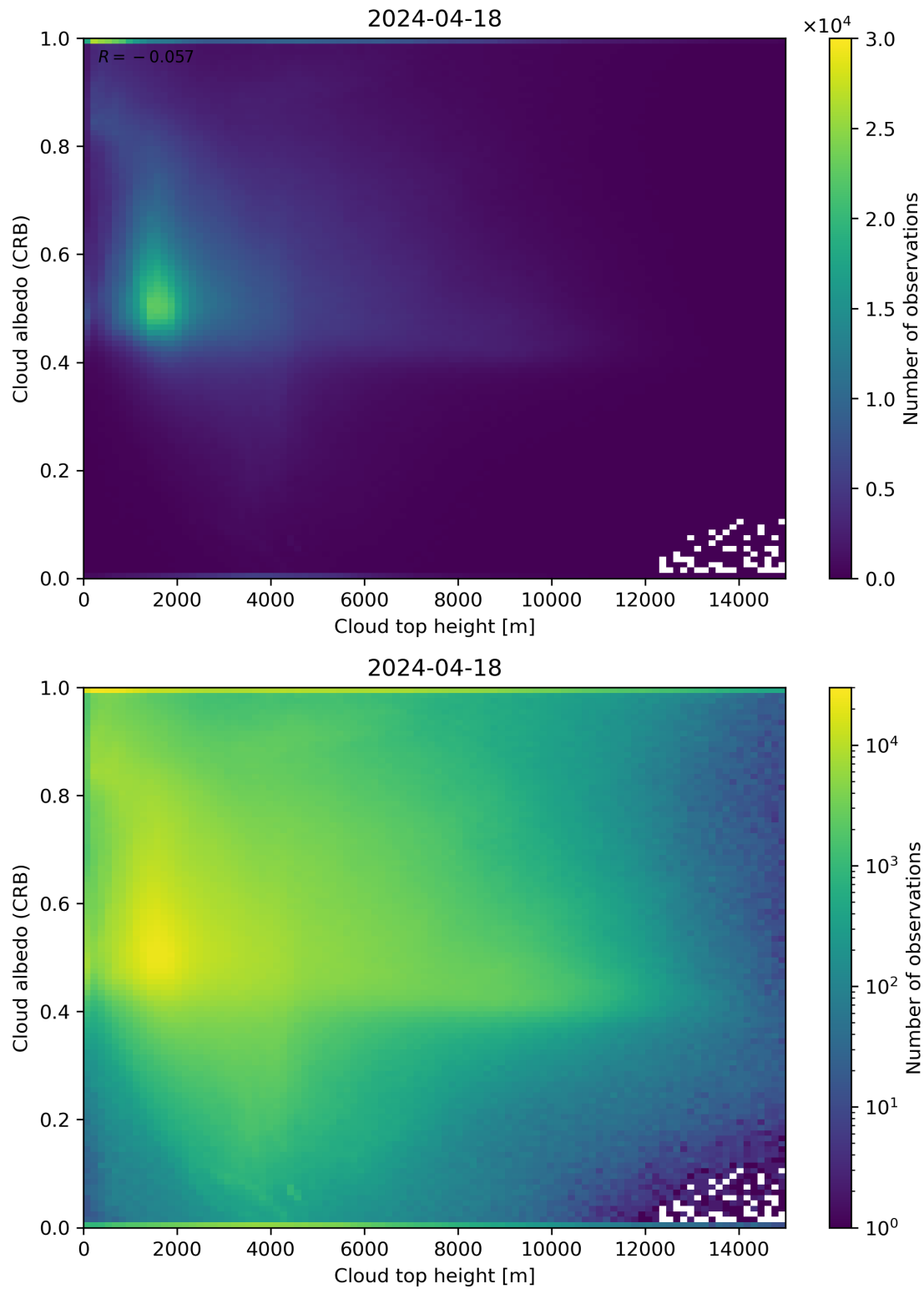
Figure 86: Scatter density plot of “Cloud top height” against “Cloud albedo (CRB)” for 2024-04-17 to 2024-04-19.
