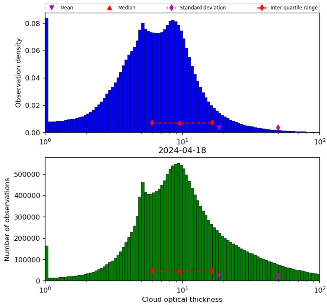
Figure 41: Histogram of “Cloud optical thickness” for 2024-04-17 to 2024-04-19
