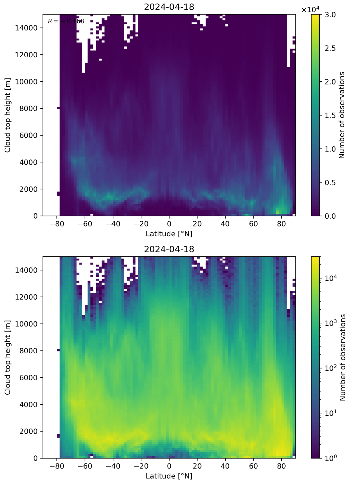
Figure 97: Scatter density plot of “Latitude” against “Cloud top height” for 2024-04-17 to 2024-04-19.
