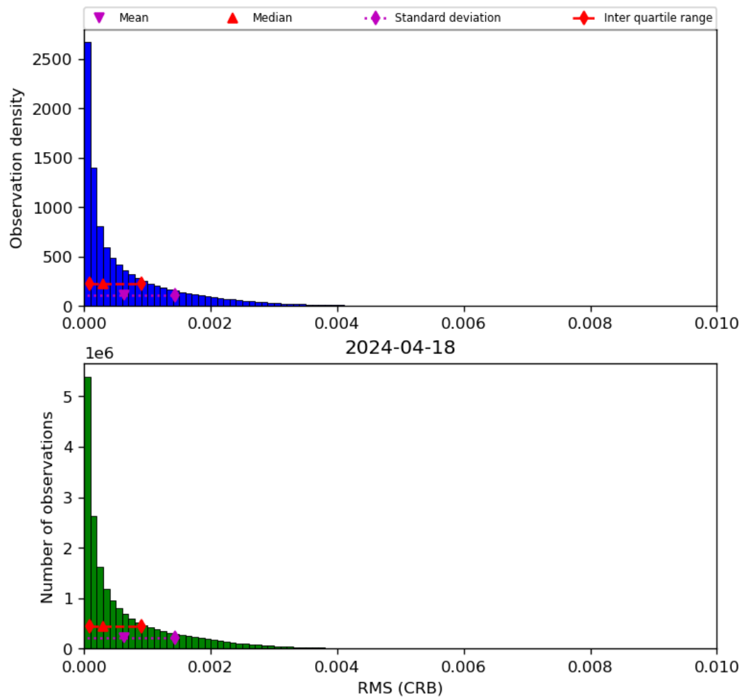
Figure 48: Histogram of “RMS (CRB)” for 2024-04-17 to 2024-04-19
