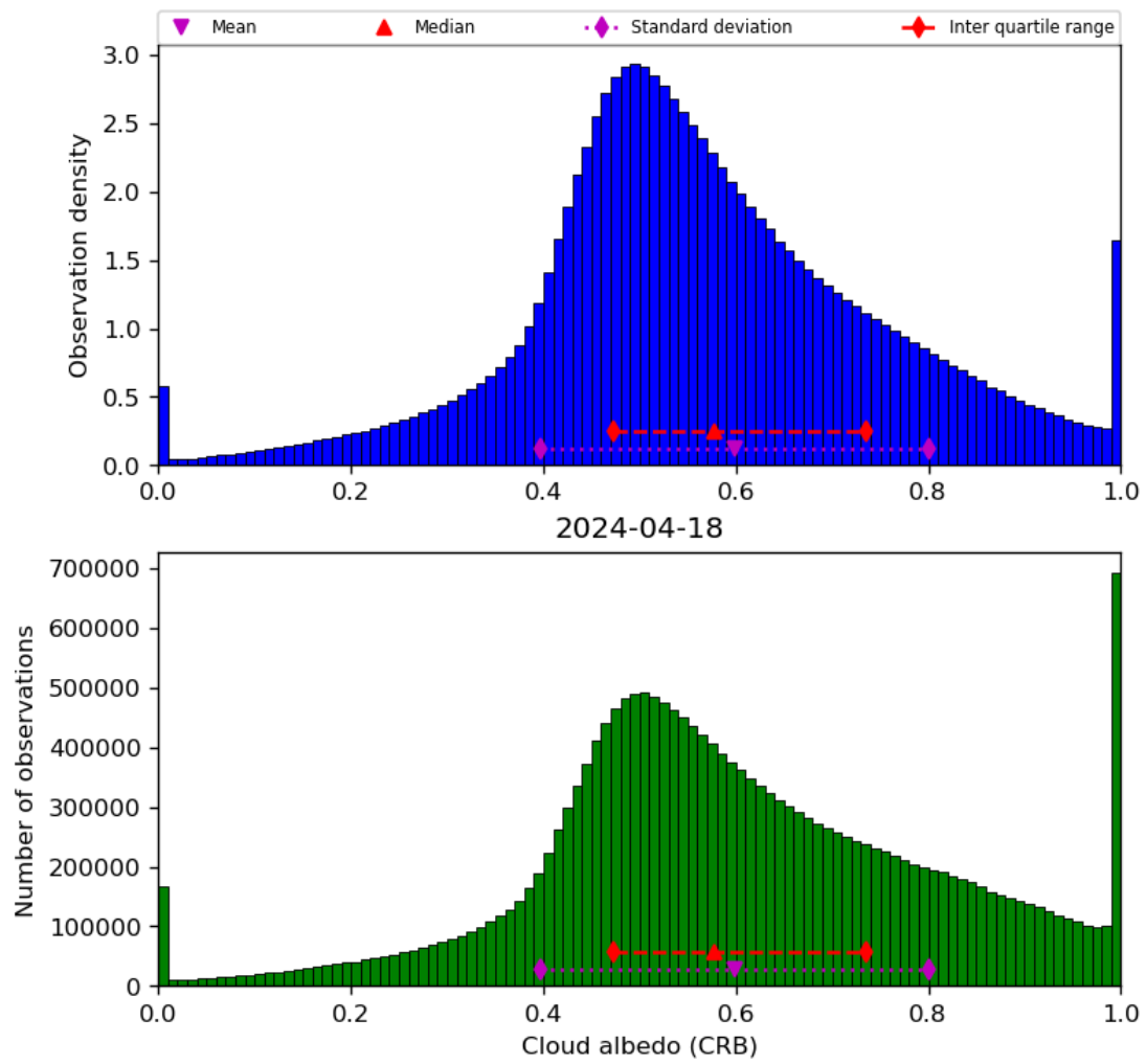
Figure 44: Histogram of “Cloud albedo (CRB)” for 2024-04-17 to 2024-04-19
