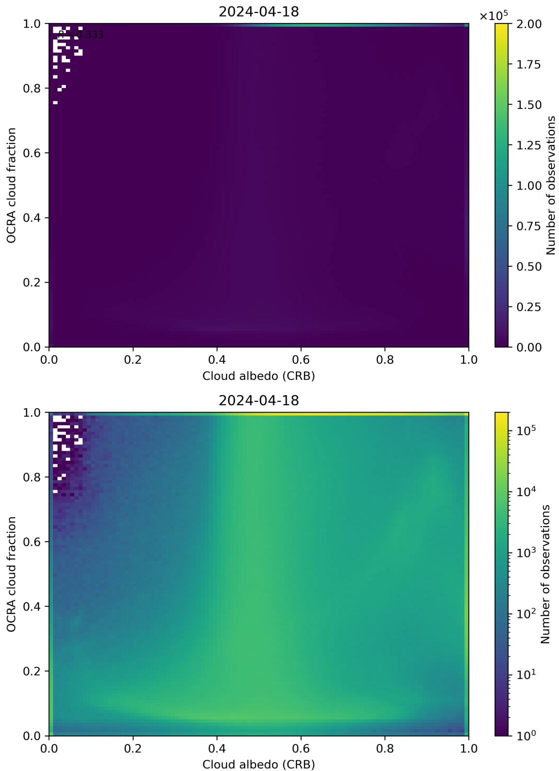
Figure 70: Scatter density plot of “Cloud albedo (CRB)” against “OCRA cloud fraction” for 2024-04-17 to 2024-04-19.
