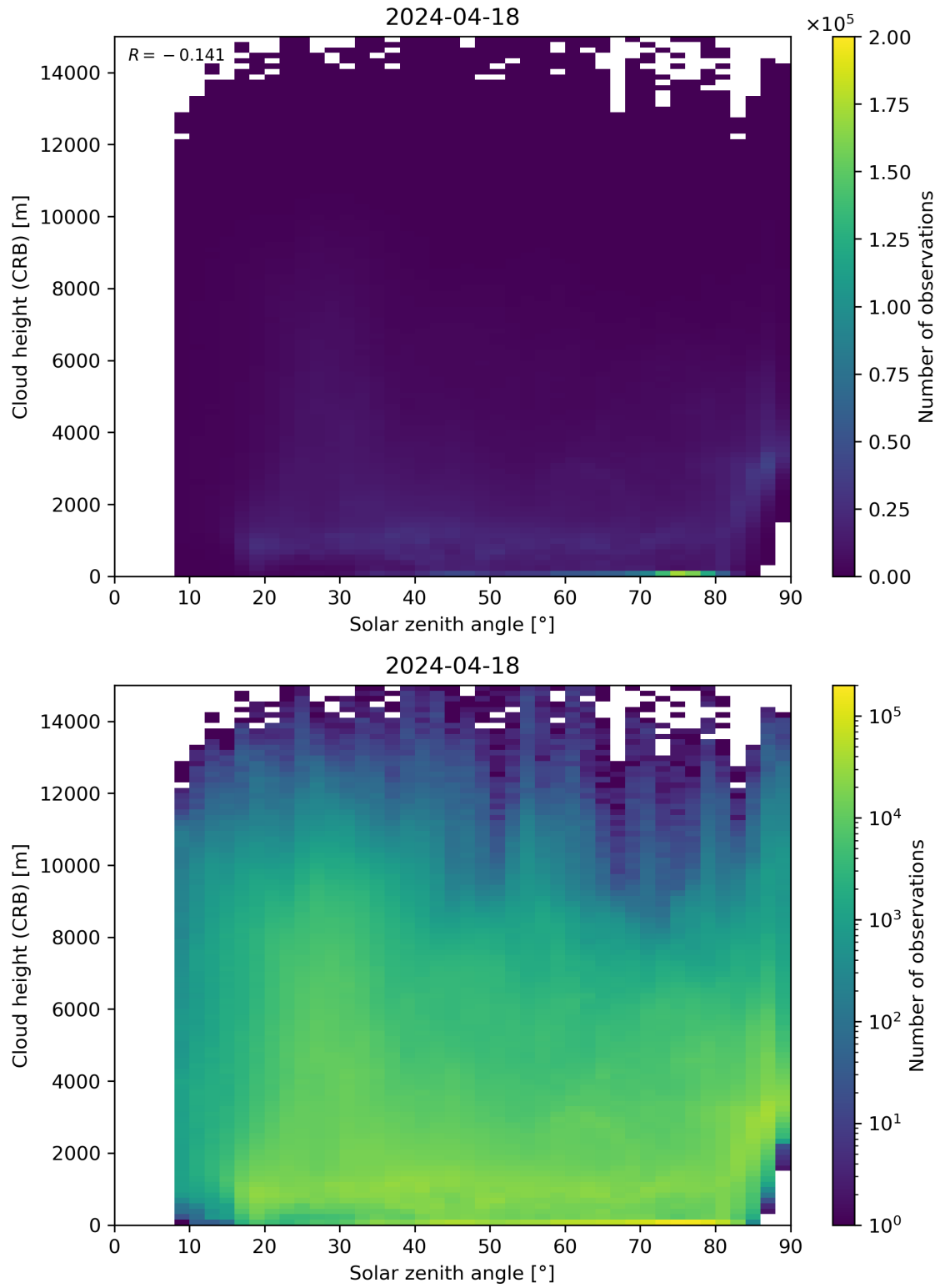
Figure 102: Scatter density plot of “Solar zenith angle” against “Cloud height (CRB)” for 2024-04-17 to 2024-04-19.
