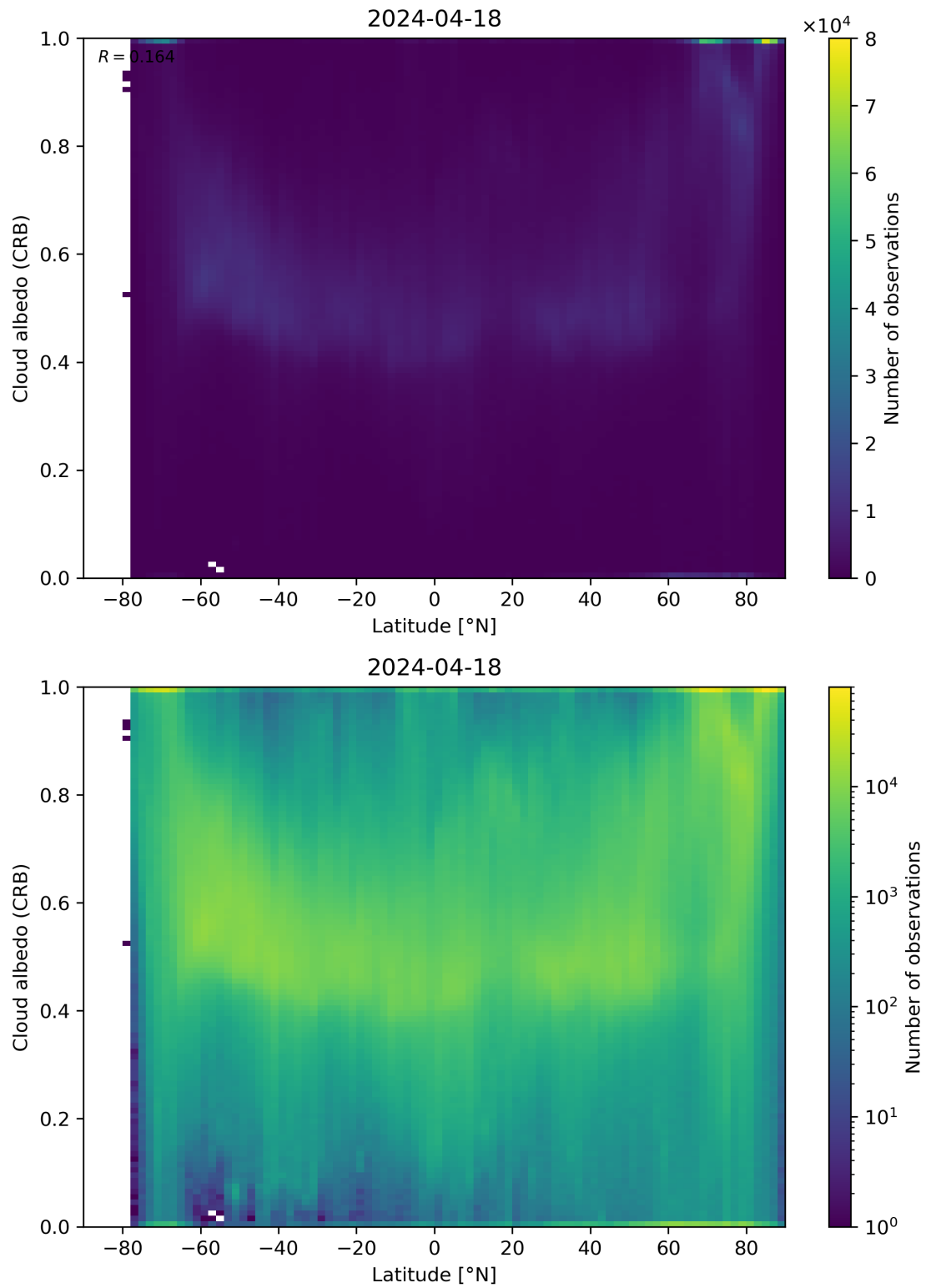
Figure 91: Scatter density plot of “Latitude” against “Cloud albedo (CRB)” for 2024-04-17 to 2024-04-19.
