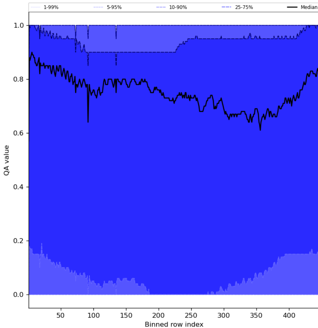
Figure 54: Along track statistics of “QA value” for 2024-04-17 to 2024-04-19
