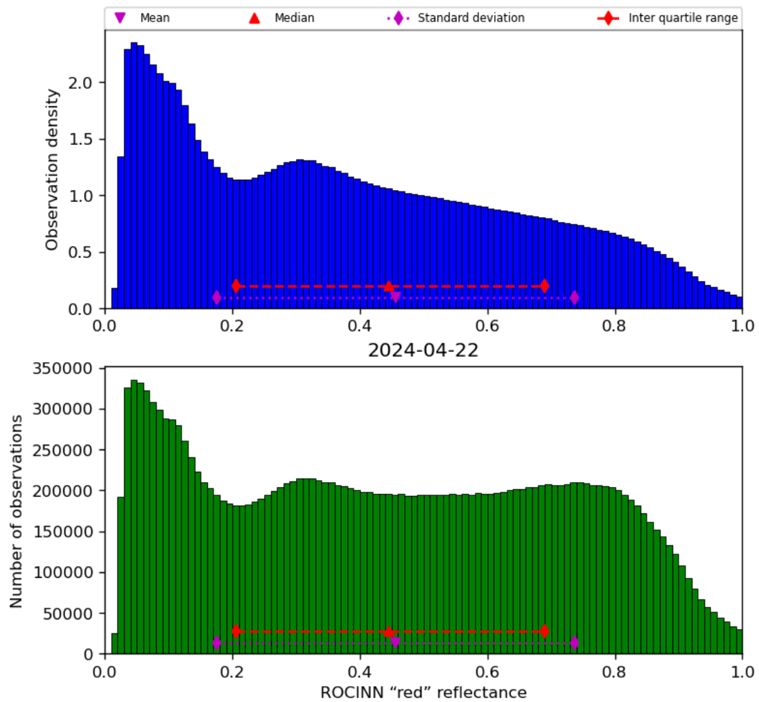
Figure 53: Histogram of “ROCINN “red” reflectance” for 2024-04-21 to 2024-04-23
