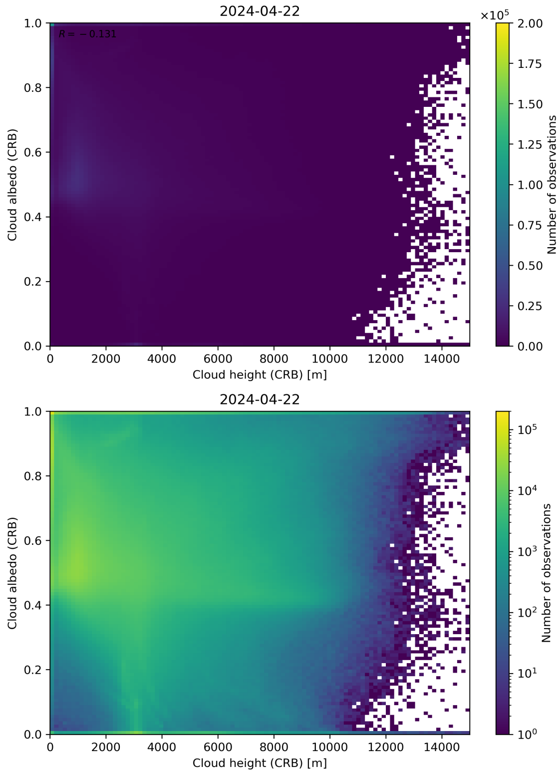
Figure 80: Scatter density plot of “Cloud height (CRB)” against “Cloud albedo (CRB)” for 2024-04-21 to 2024-04-23.
