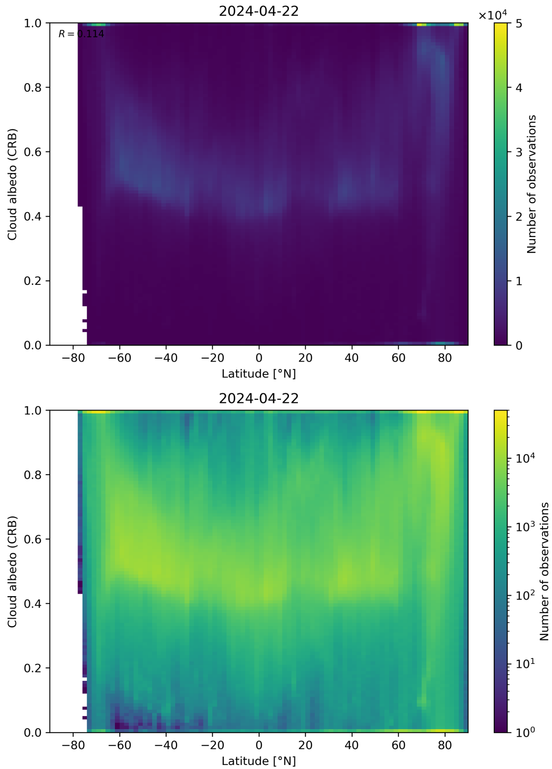
Figure 91: Scatter density plot of “Latitude” against “Cloud albedo (CRB)” for 2024-04-21 to 2024-04-23.
