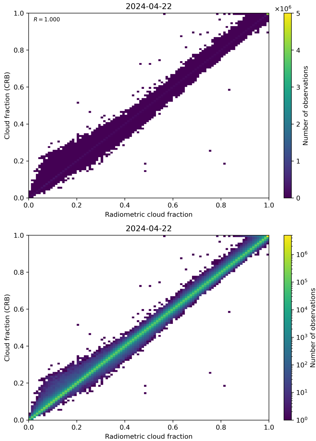
Figure 73: Scatter density plot of “Radiometric cloud fraction” against “Cloud fraction (CRB)” for 2024-04-21 to 2024-04-23.
