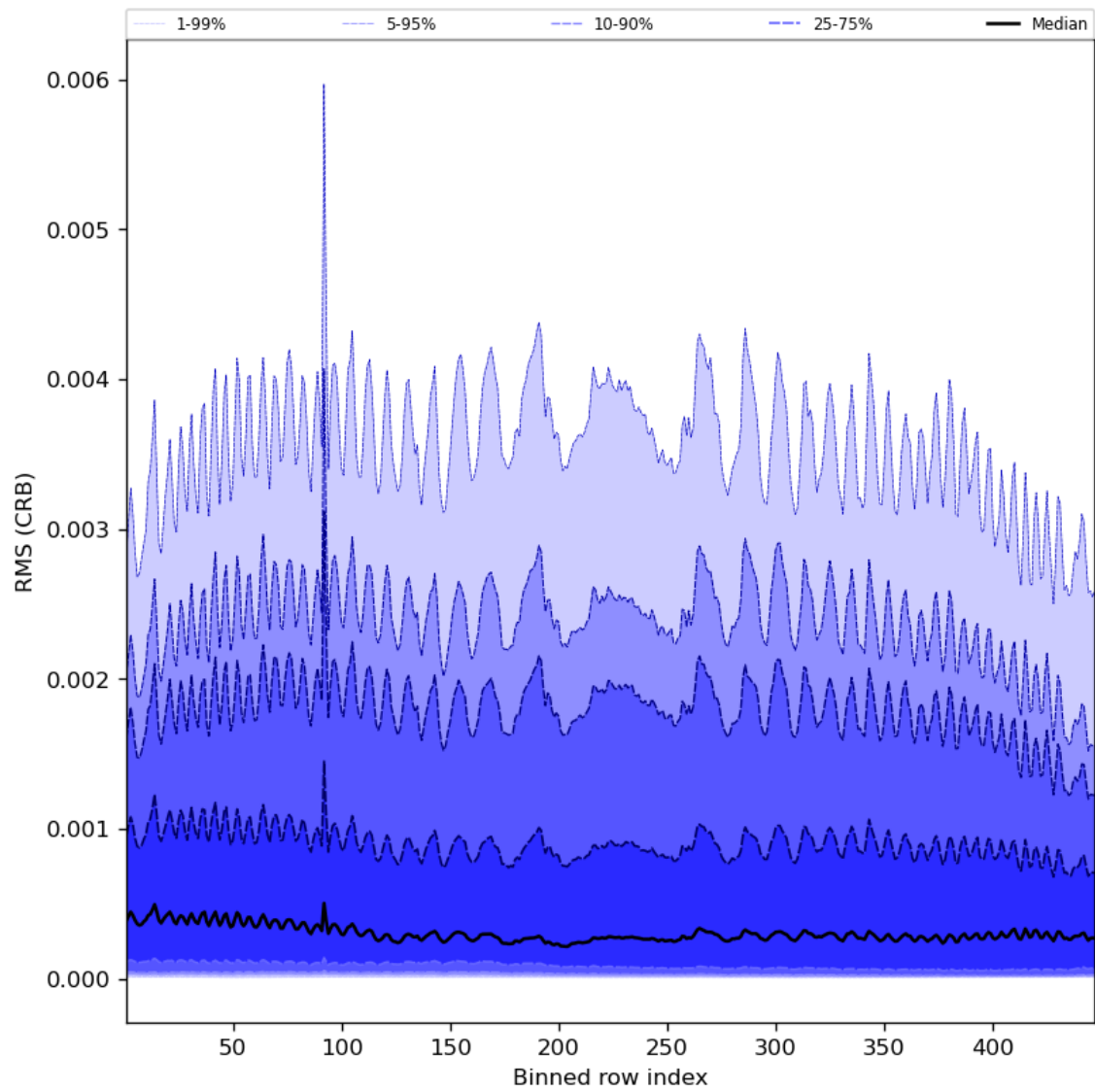
Figure 64: Along track statistics of “RMS (CRB)” for 2024-04-21 to 2024-04-23
