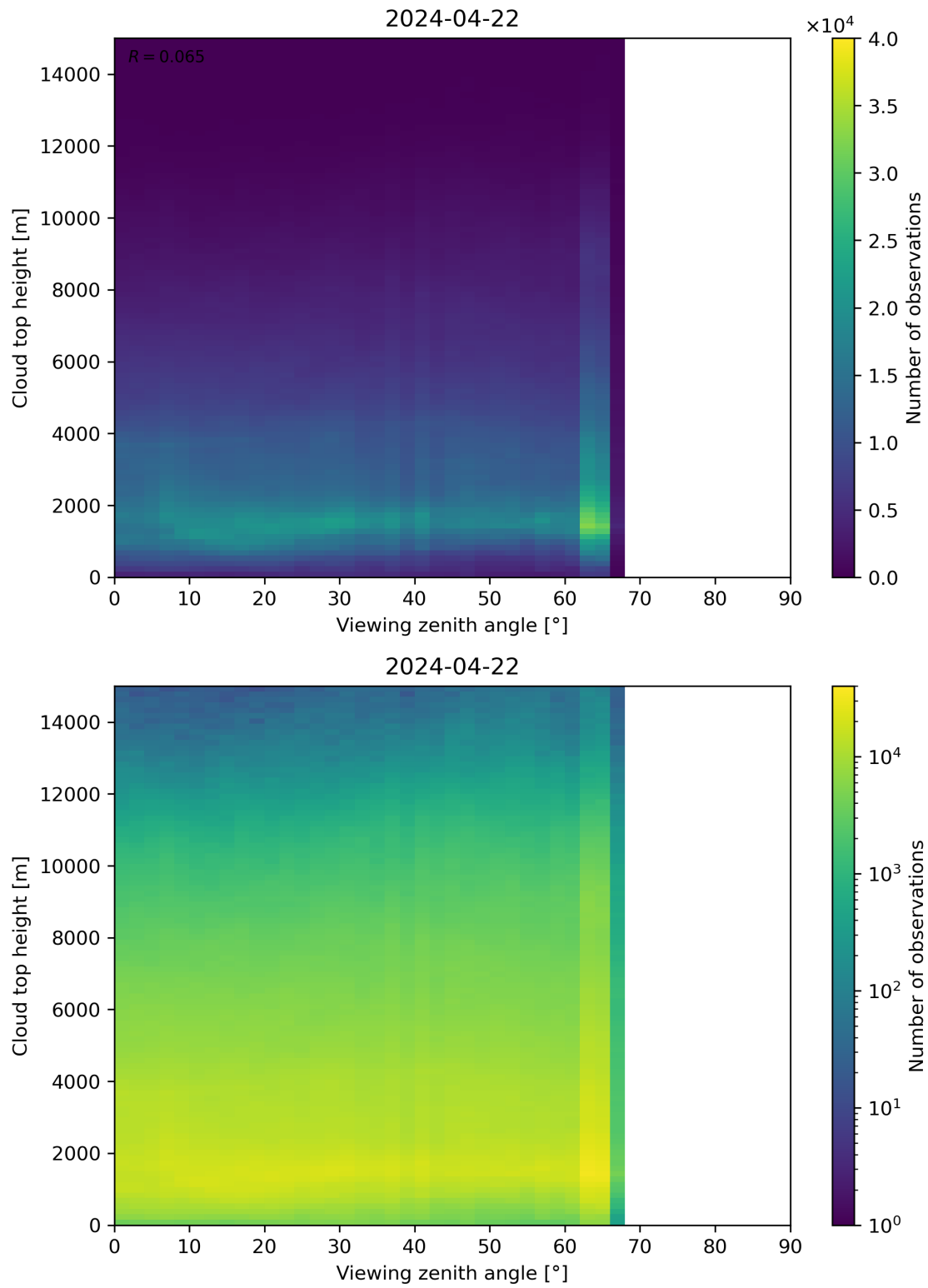
Figure 112: Scatter density plot of “Viewing zenith angle” against “Cloud top height” for 2024-04-21 to 2024-04-23.
