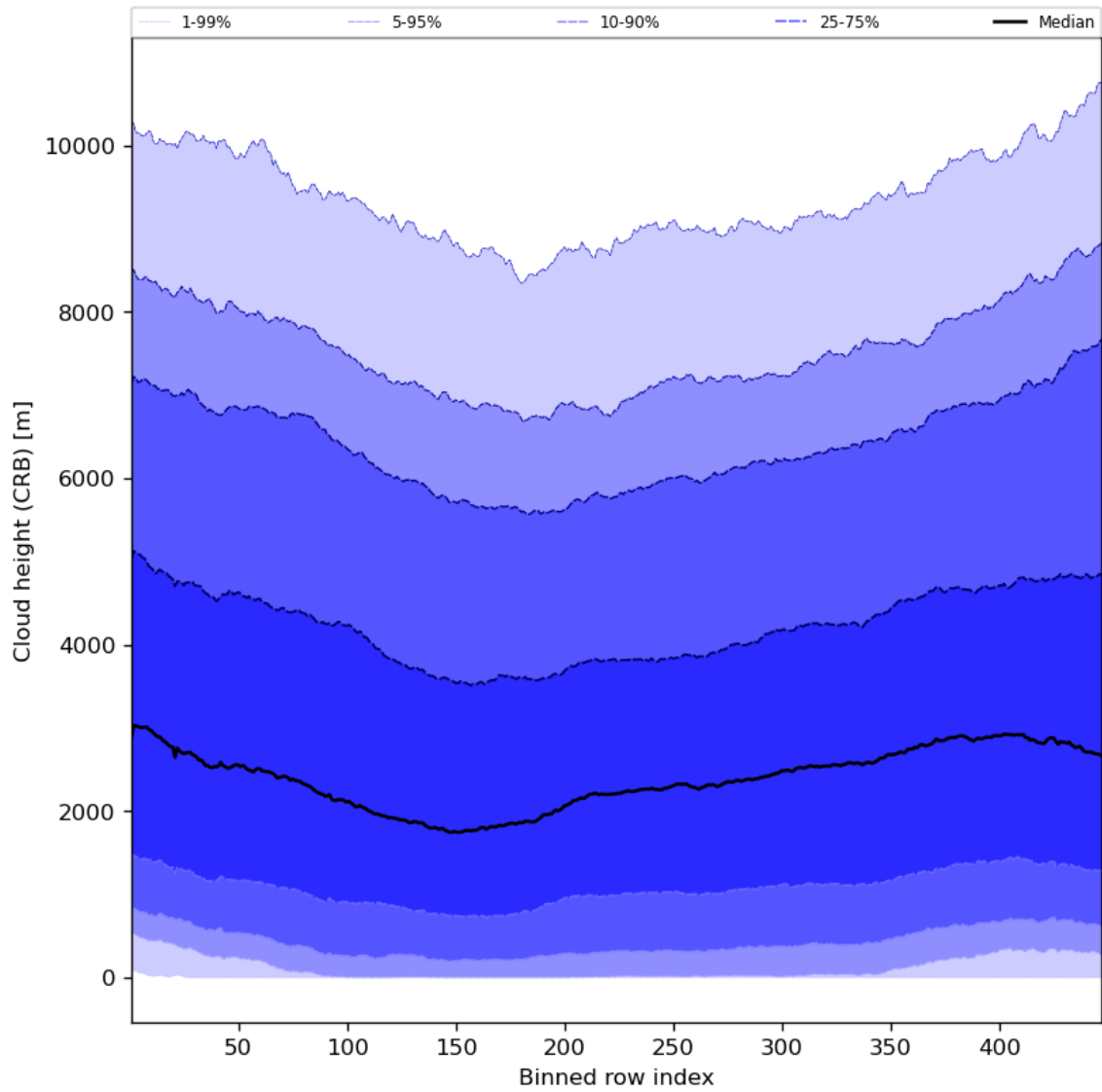
Figure 59: Along track statistics of “Cloud height (CRB)” for 2024-04-21 to 2024-04-23
