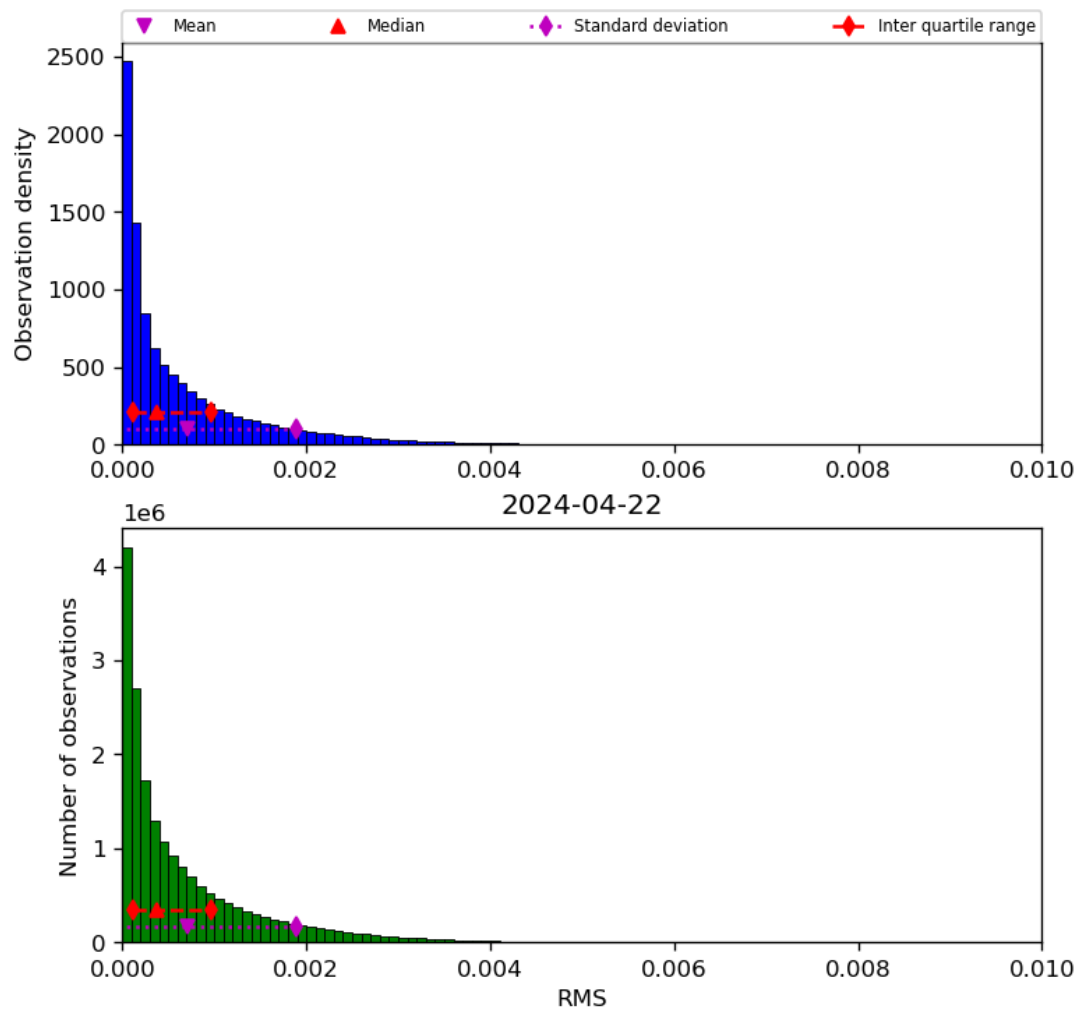
Figure 47: Histogram of “RMS” for 2024-04-21 to 2024-04-23
