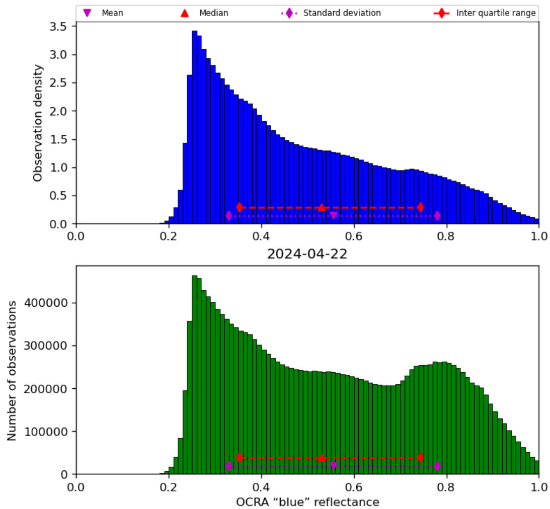
Figure 51: Histogram of “OCRA “blue” reflectance” for 2024-04-21 to 2024-04-23
