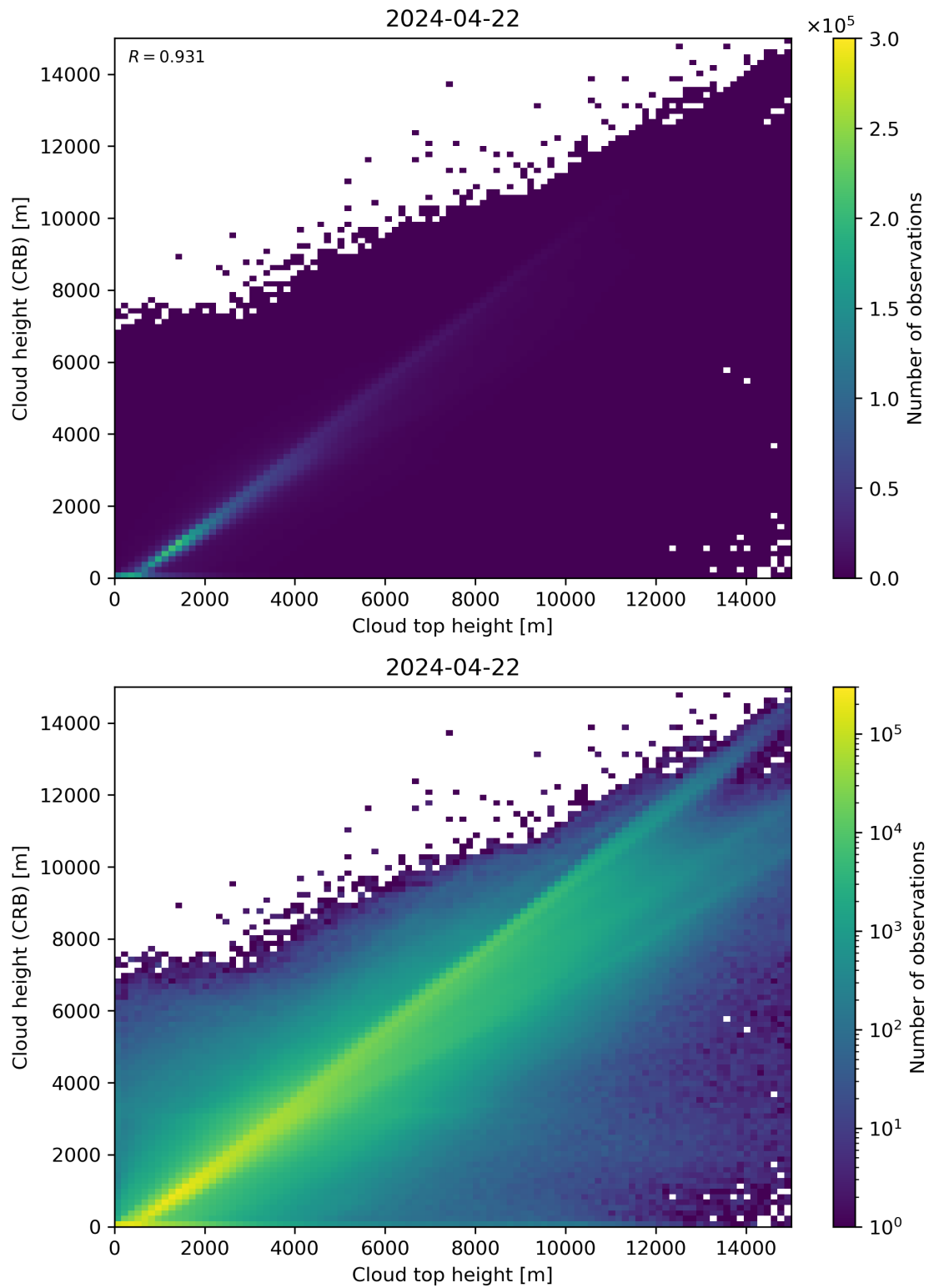
Figure 89: Scatter density plot of “Cloud top height” against “Cloud height (CRB)” for 2024-04-21 to 2024-04-23.
