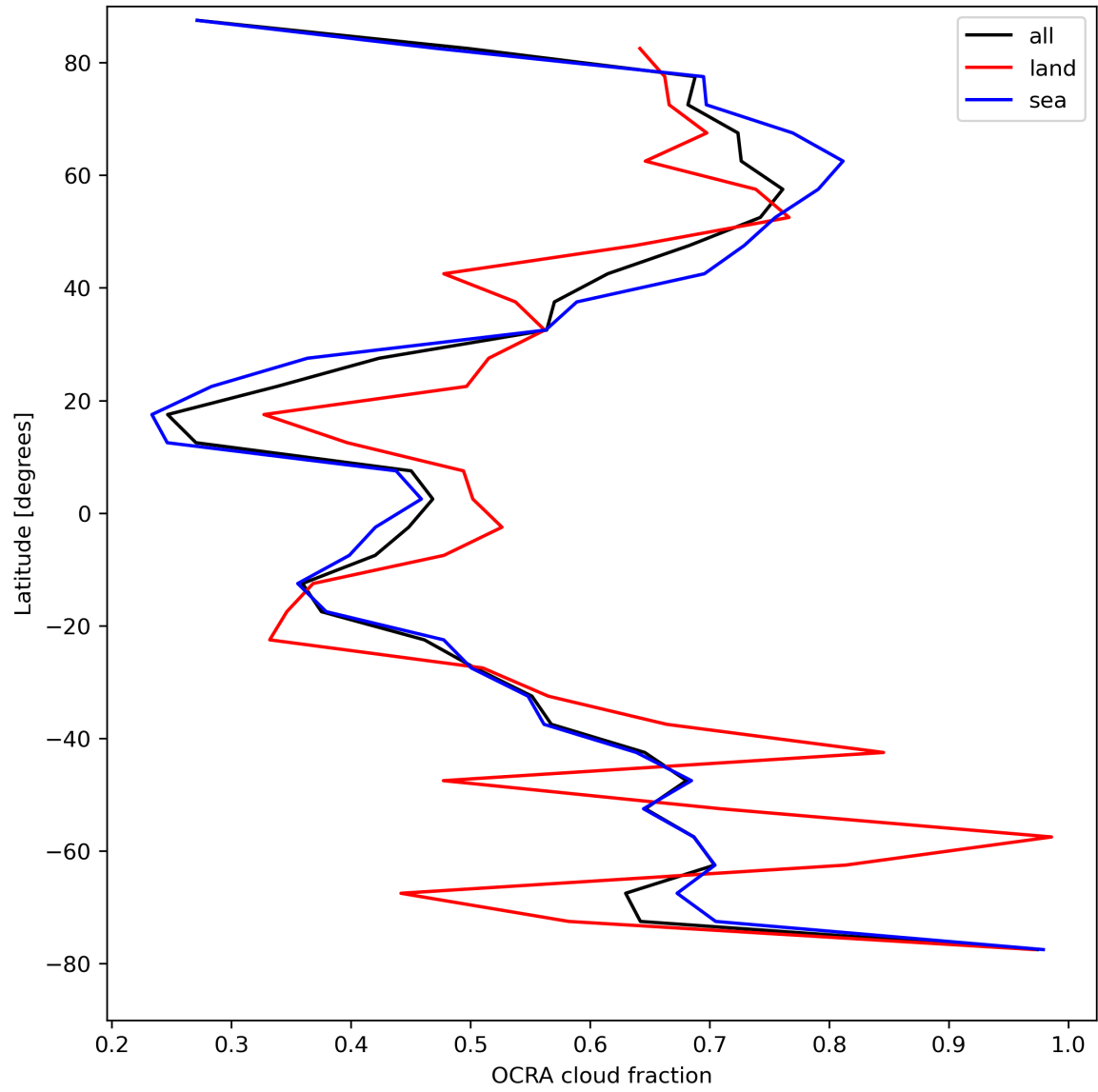
Figure 34: Zonal average of “OCRA cloud fraction” for 2024-04-21 to 2024-04-23.
