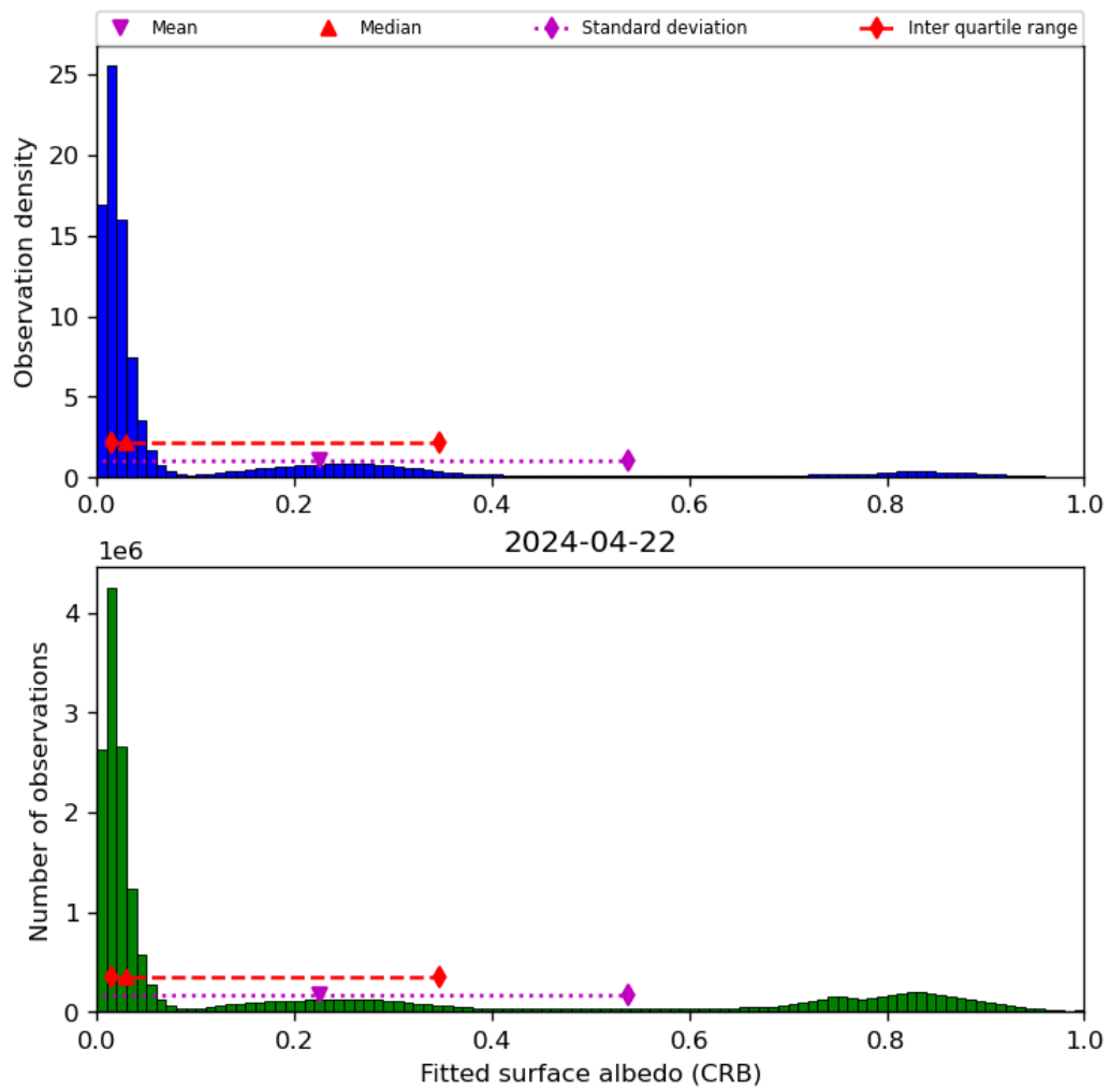
Figure 46: Histogram of “Fitted surface albedo (CRB)” for 2024-04-21 to 2024-04-23
