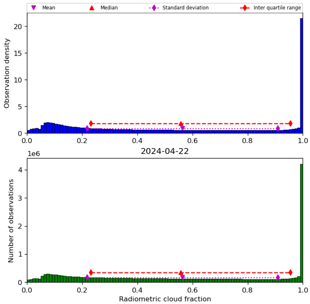
Figure 39: Histogram of “Radiometric cloud fraction” for 2024-04-21 to 2024-04-23
