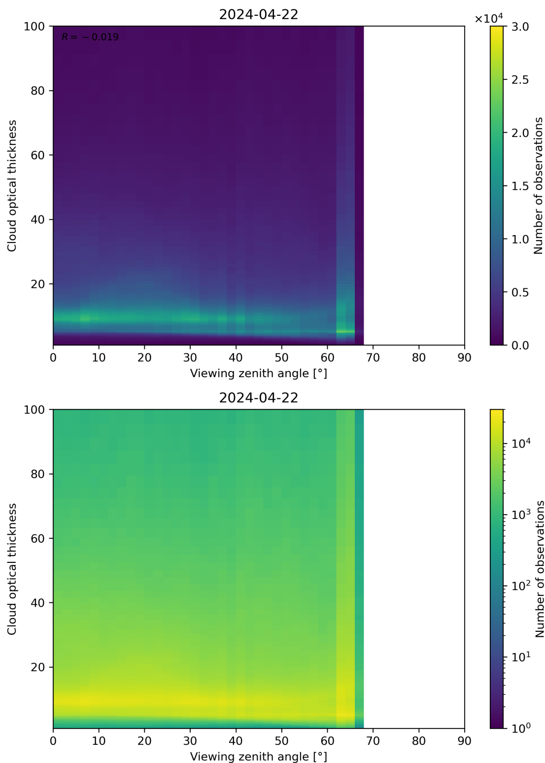
Figure 111: Scatter density plot of “Viewing zenith angle” against “Cloud optical thickness” for 2024-04-21 to 2024-04-23.
