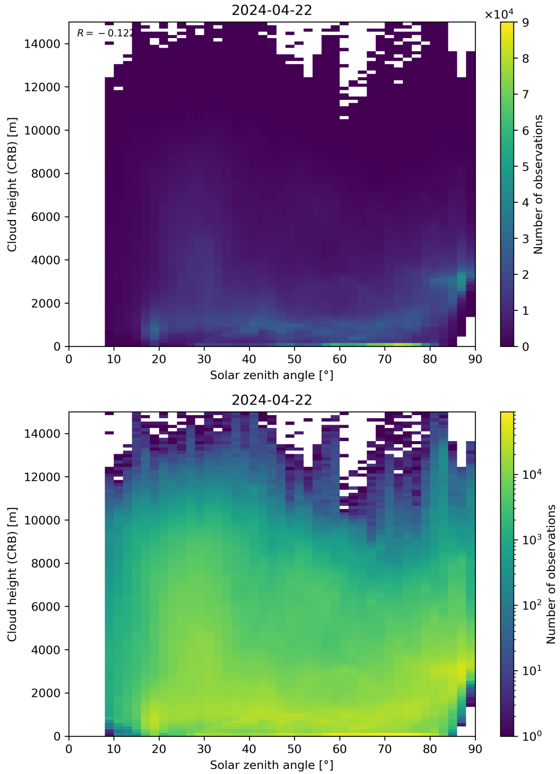
Figure 102: Scatter density plot of “Solar zenith angle” against “Cloud height (CRB)” for 2024-04-21 to 2024-04-23.
