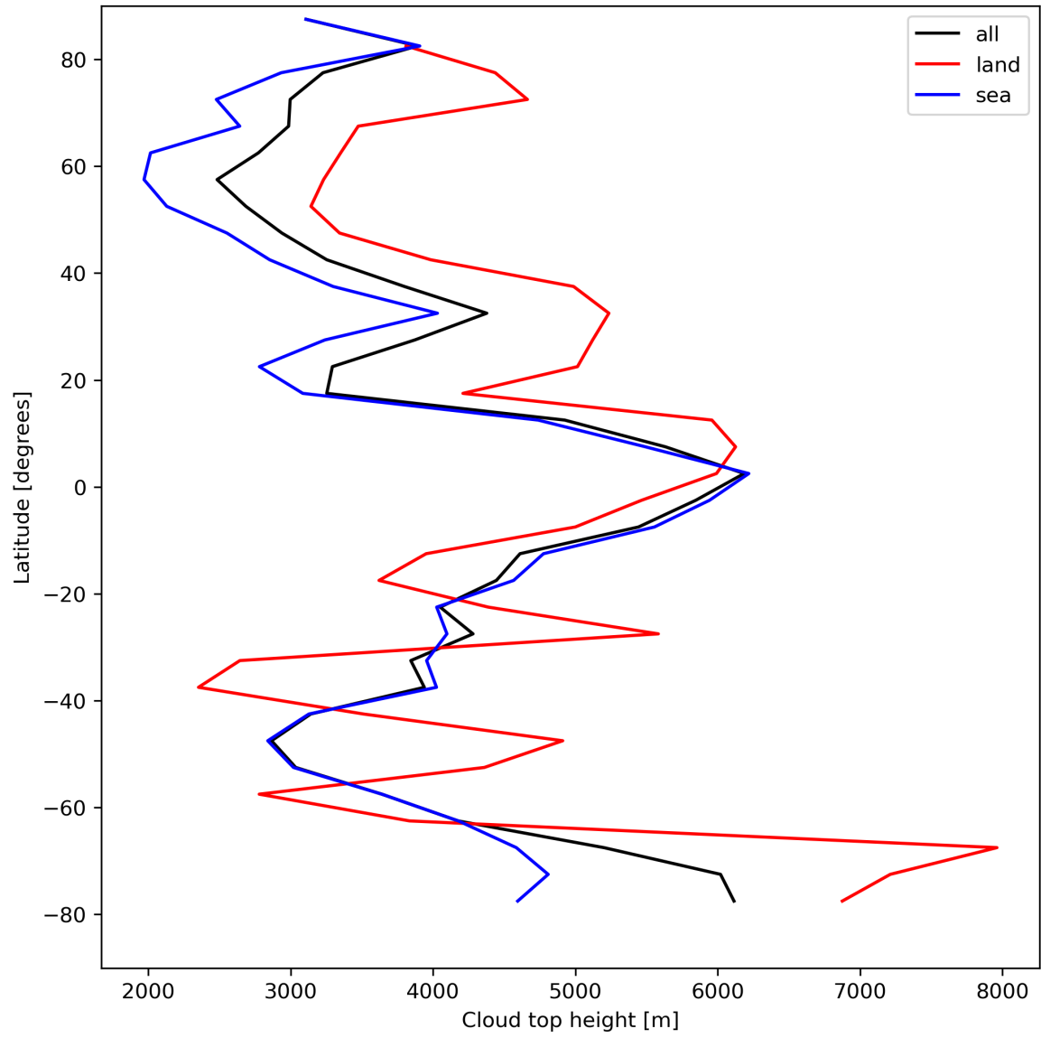
Figure 24: Zonal average of “Cloud top height” for 2024-04-21 to 2024-04-23.
