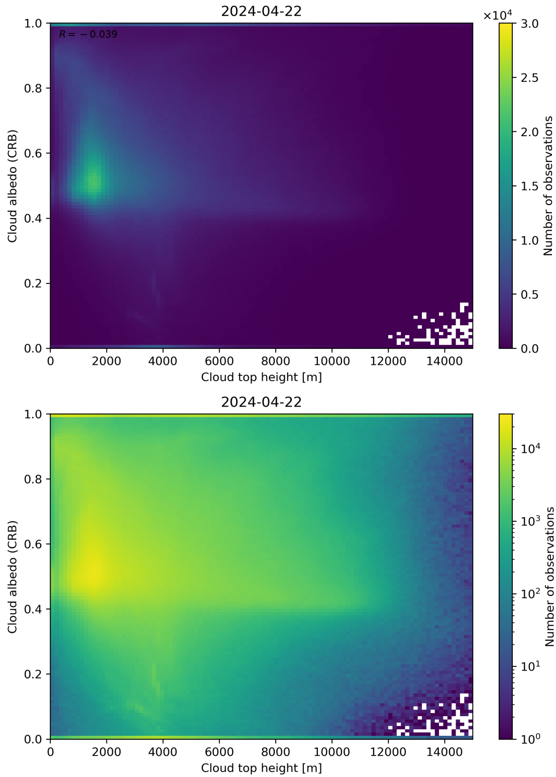
Figure 86: Scatter density plot of “Cloud top height” against “Cloud albedo (CRB)” for 2024-04-21 to 2024-04-23.
