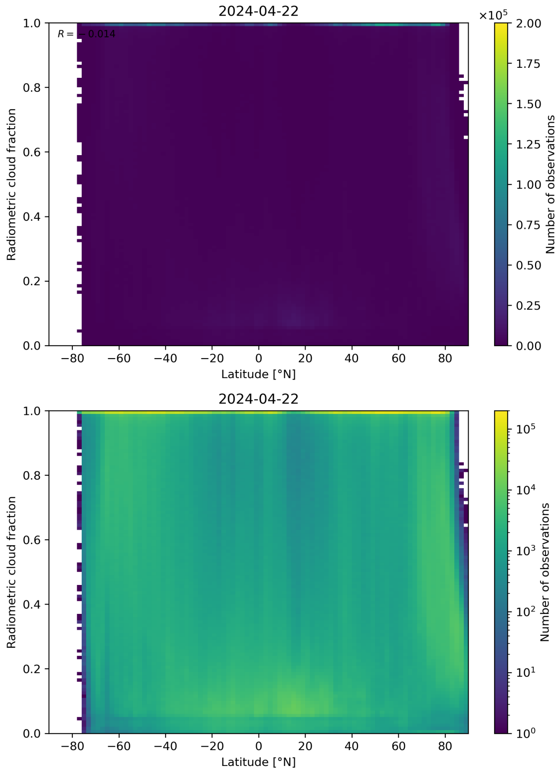
Figure 92: Scatter density plot of “Latitude” against “Radiometric cloud fraction” for 2024-04-21 to 2024-04-23.
