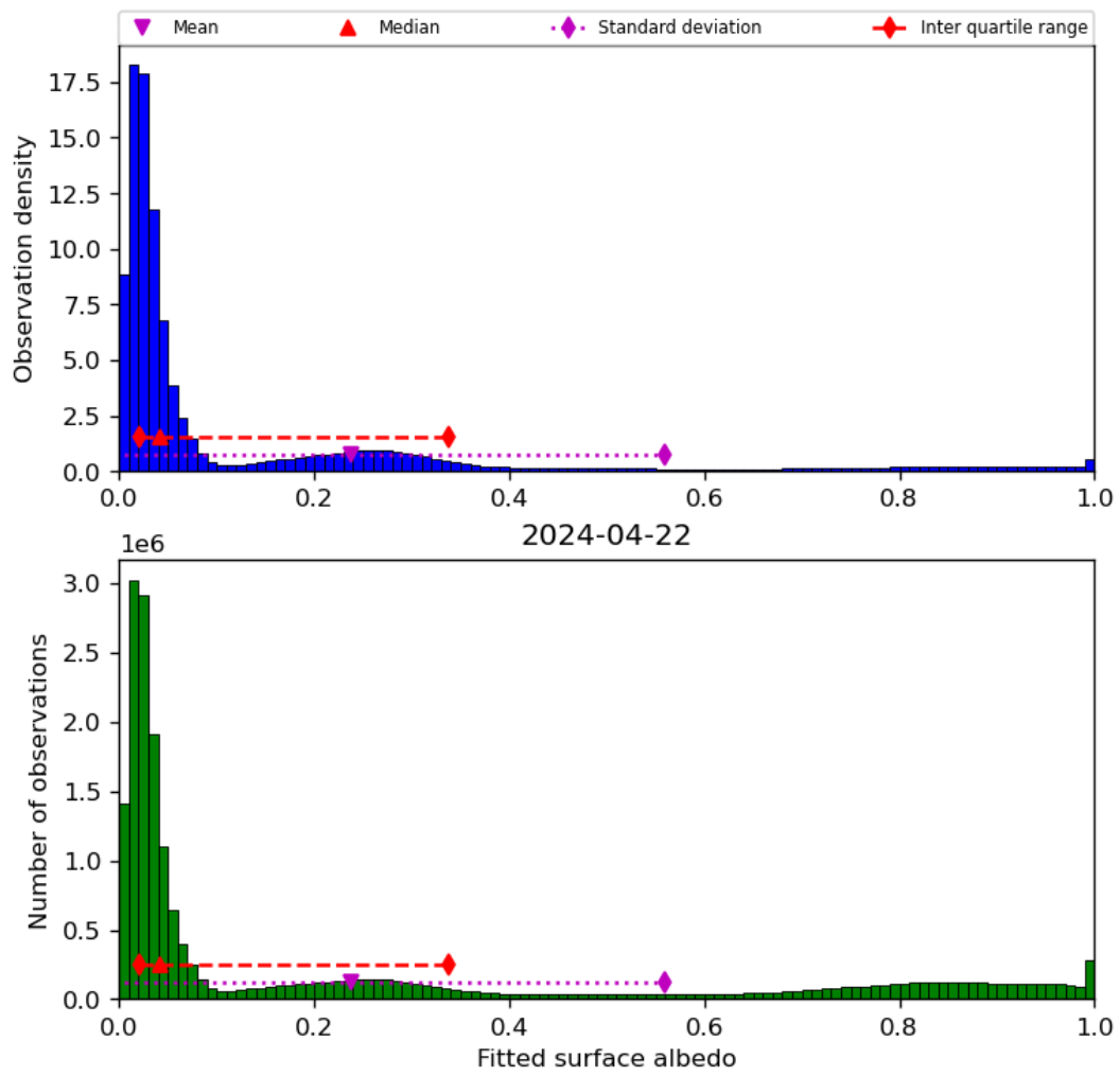
Figure 45: Histogram of “Fitted surface albedo” for 2024-04-21 to 2024-04-23
