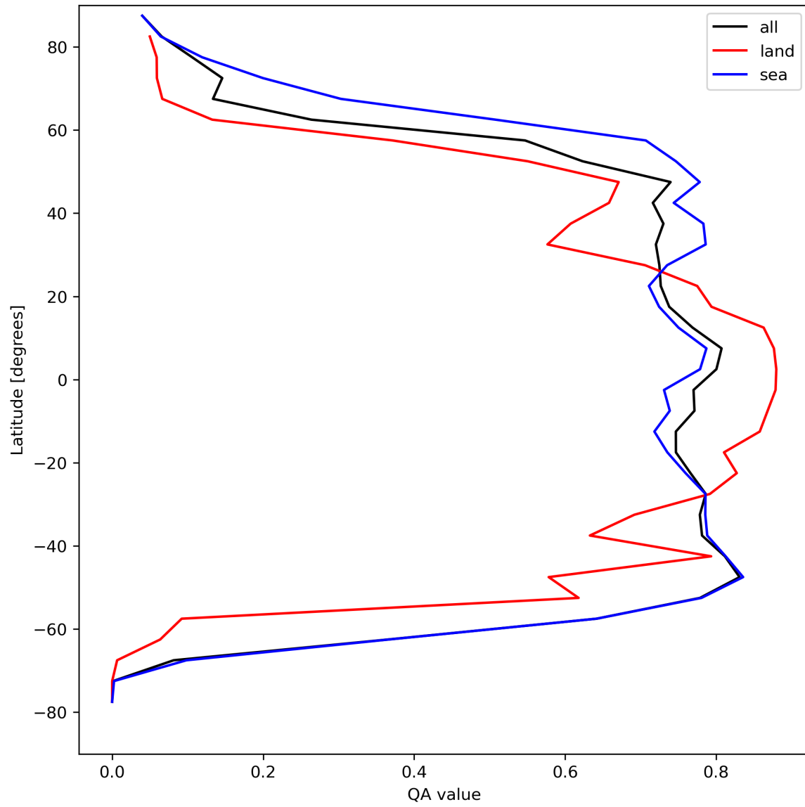
Figure 22: Zonal average of “QA value” for 2024-04-21 to 2024-04-23.
