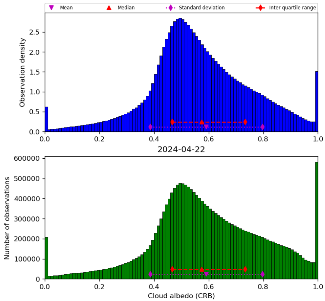
Figure 44: Histogram of “Cloud albedo (CRB)” for 2024-04-21 to 2024-04-23
