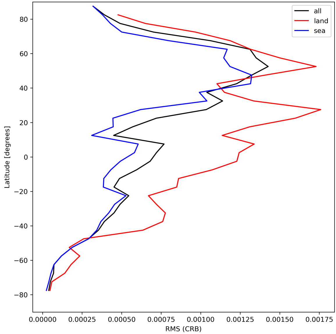
Figure 32: Zonal average of “RMS (CRB)” for 2024-04-21 to 2024-04-23.
