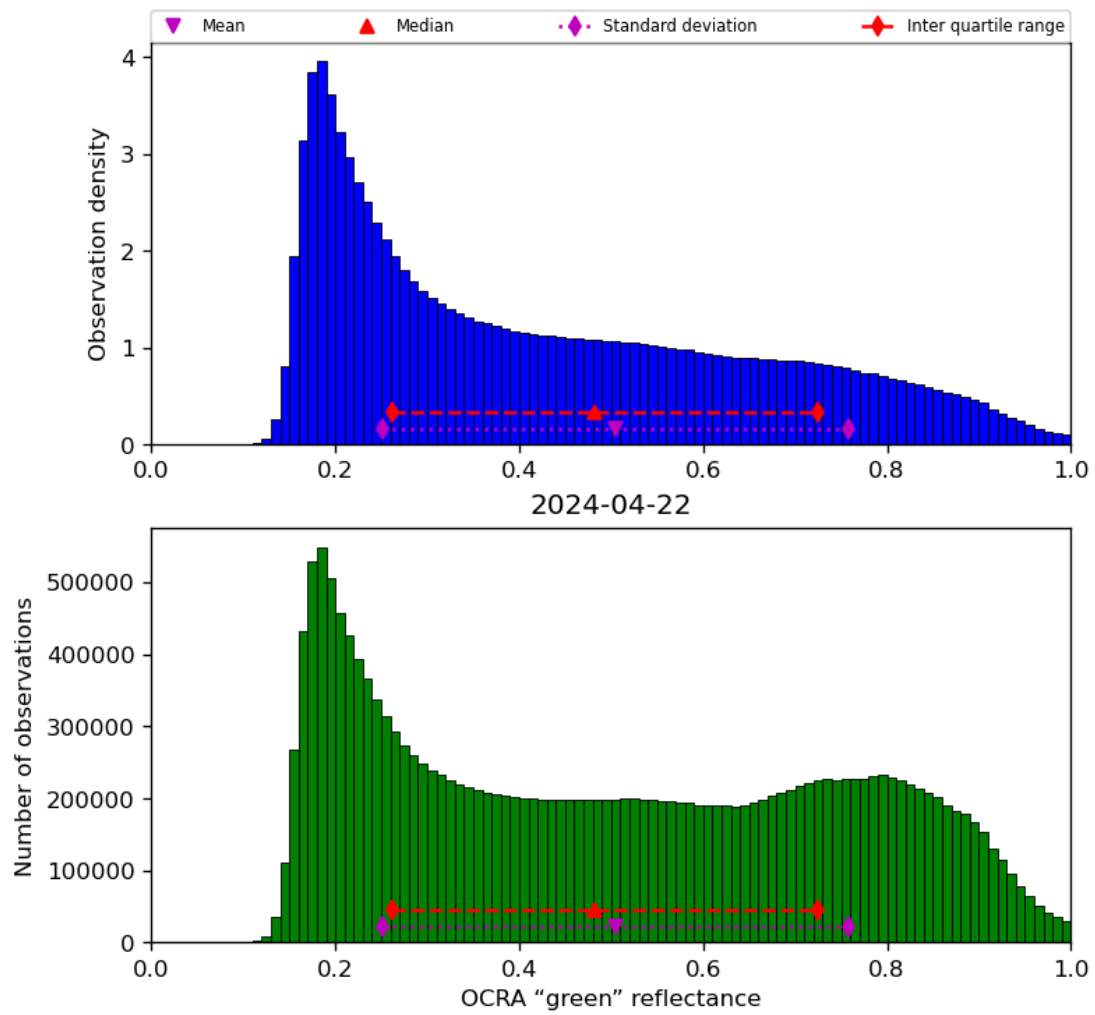
Figure 52: Histogram of “OCRA “green” reflectance” for 2024-04-21 to 2024-04-23
