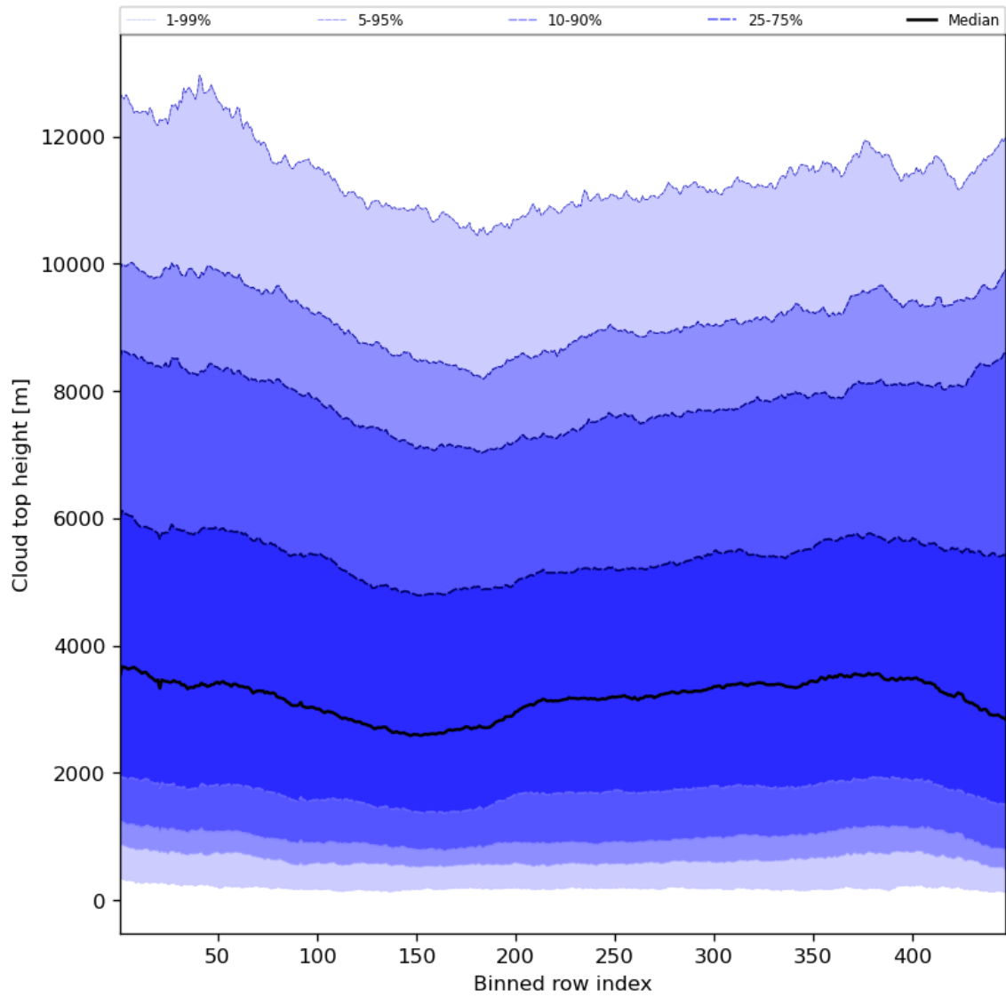
Figure 56: Along track statistics of “Cloud top height” for 2024-04-21 to 2024-04-23
