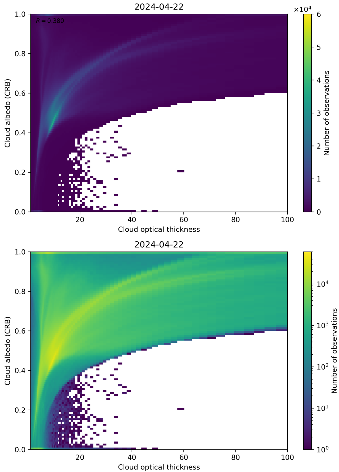
Figure 82: Scatter density plot of “Cloud optical thickness” against “Cloud albedo (CRB)” for 2024-04-21 to 2024-04-23.
