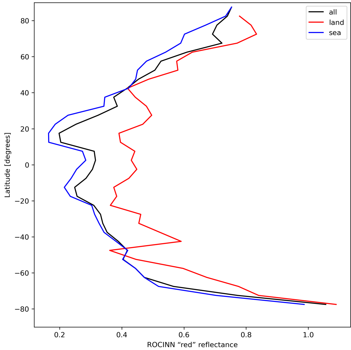
Figure 37: Zonal average of “ROCINN “red” reflectance” for 2024-04-21 to 2024-04-23.
