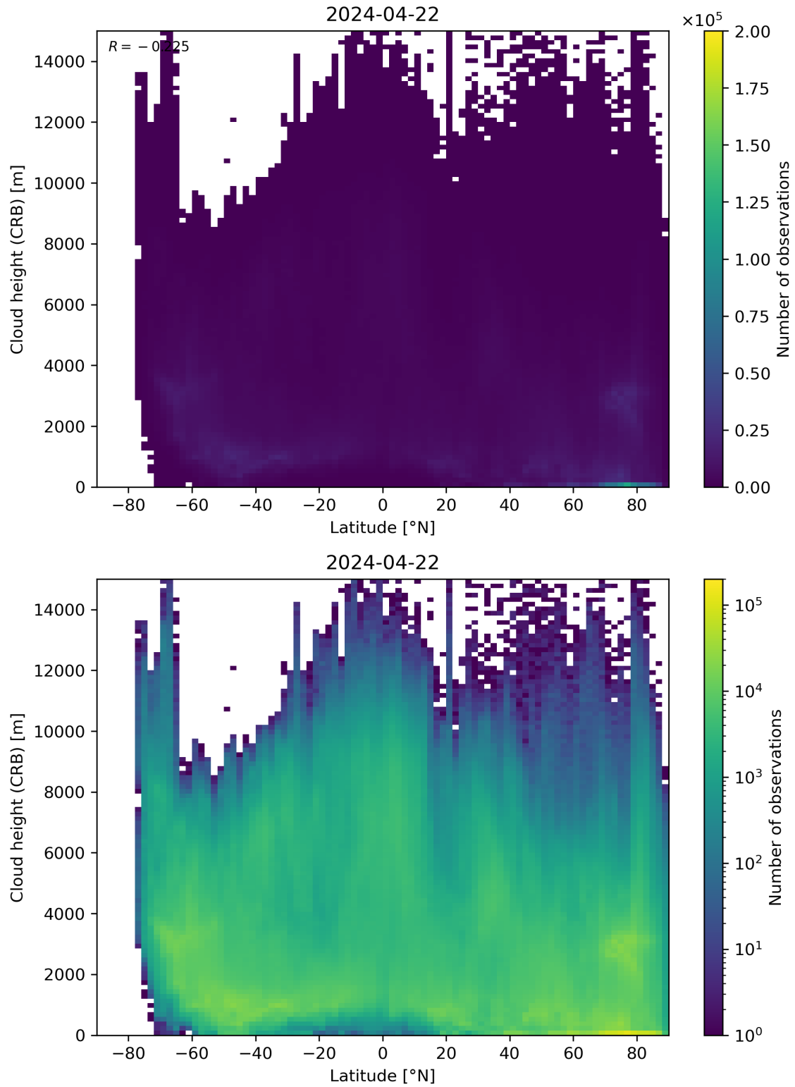
Figure 95: Scatter density plot of “Latitude” against “Cloud height (CRB)” for 2024-04-21 to 2024-04-23.
