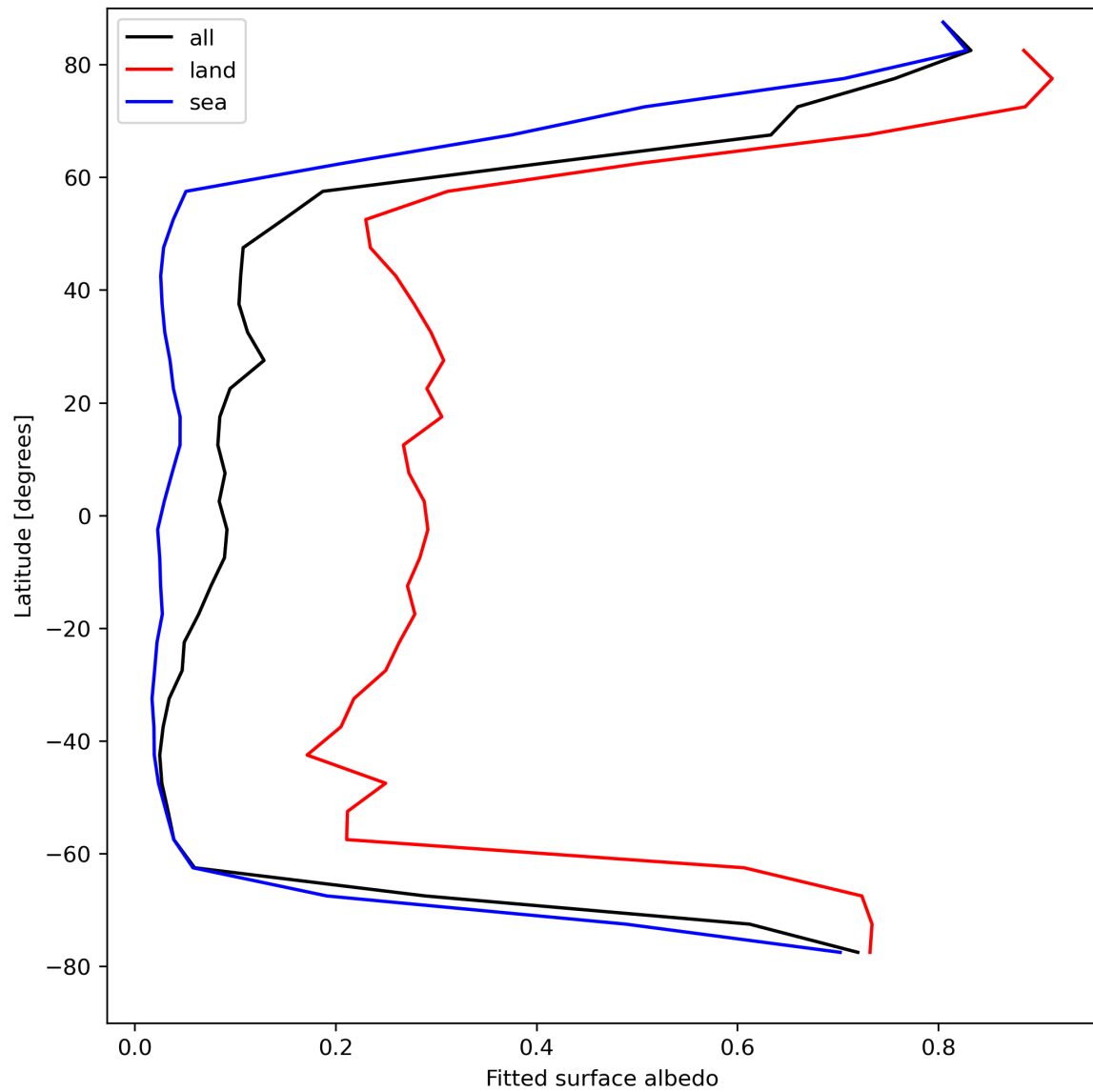
Figure 29: Zonal average of “Fitted surface albedo” for 2024-04-21 to 2024-04-23.
