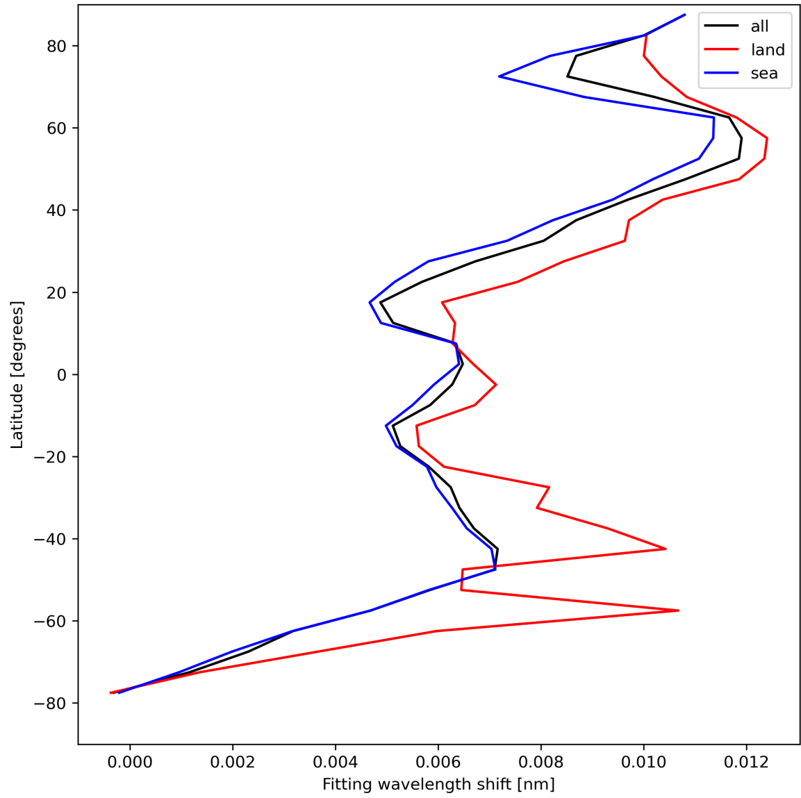
Figure 33: Zonal average of “Fitting wavelength shift” for 2024-04-21 to 2024-04-23.
