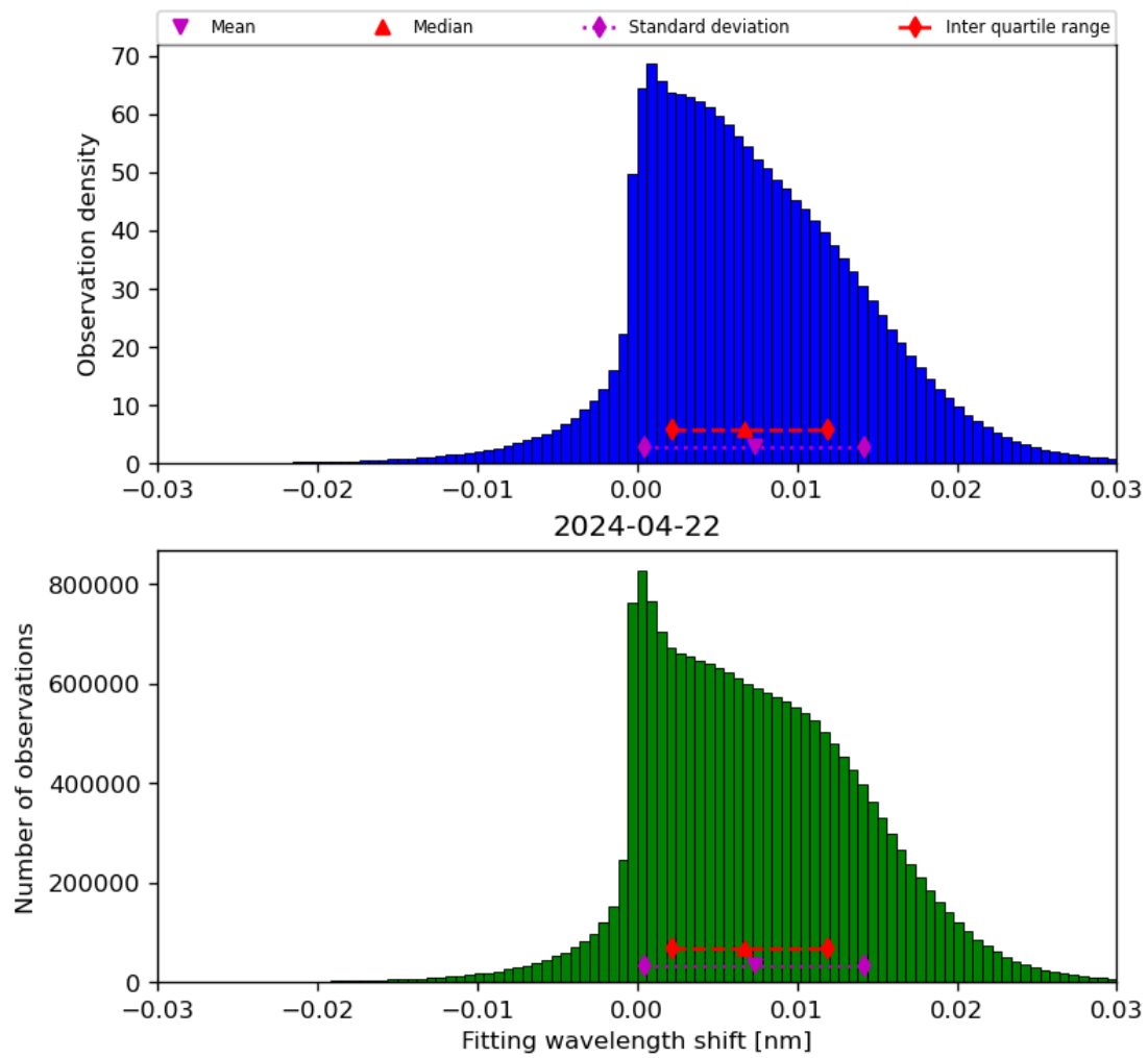
Figure 49: Histogram of “Fitting wavelength shift” for 2024-04-21 to 2024-04-23
