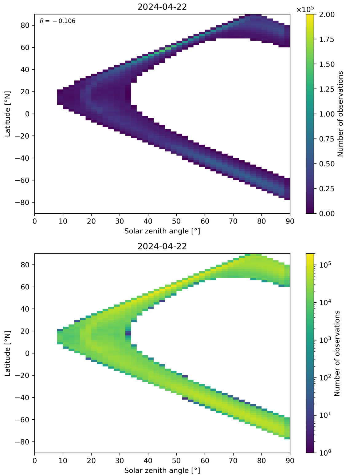
Figure 105: Scatter density plot of “Solar zenith angle” against “Latitude” for 2024-04-21 to 2024-04-23.
