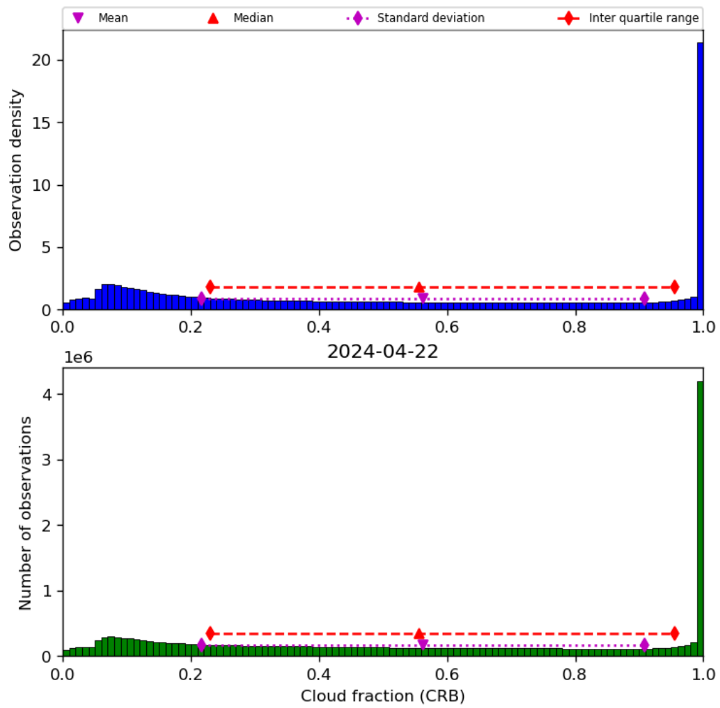
Figure 42: Histogram of “Cloud fraction (CRB)” for 2024-04-21 to 2024-04-23
