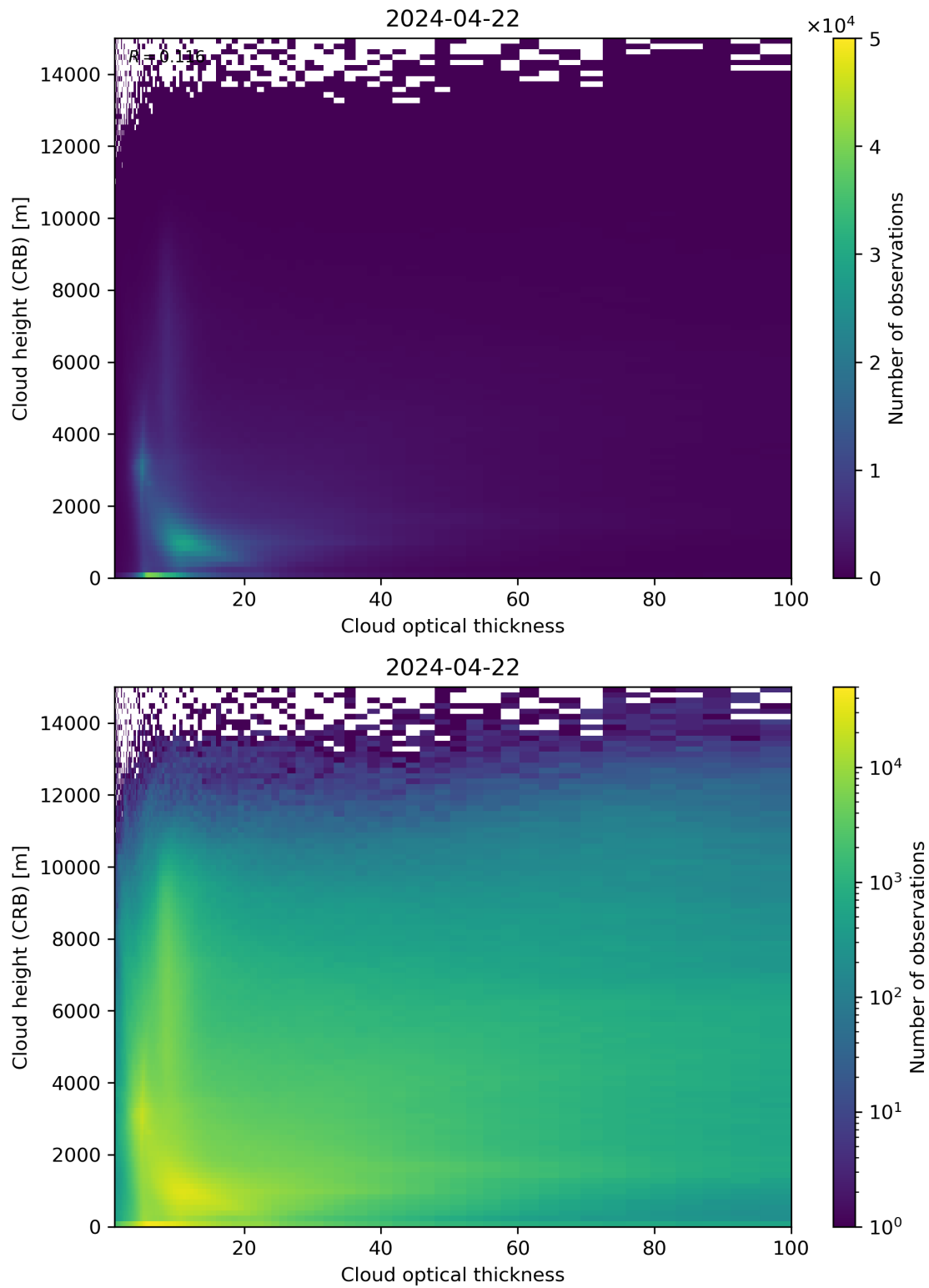
Figure 85: Scatter density plot of “Cloud optical thickness” against “Cloud height (CRB)” for 2024-04-21 to 2024-04-23.
