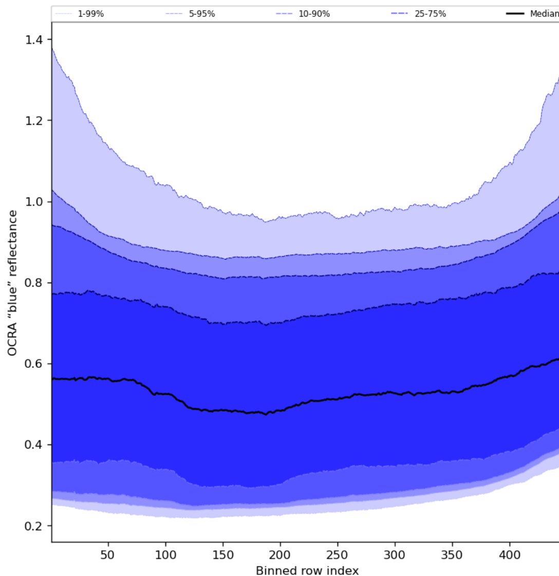
Figure 67: Along track statistics of “OCRA “blue” reflectance” for 2024-04-21 to 2024-04-23
