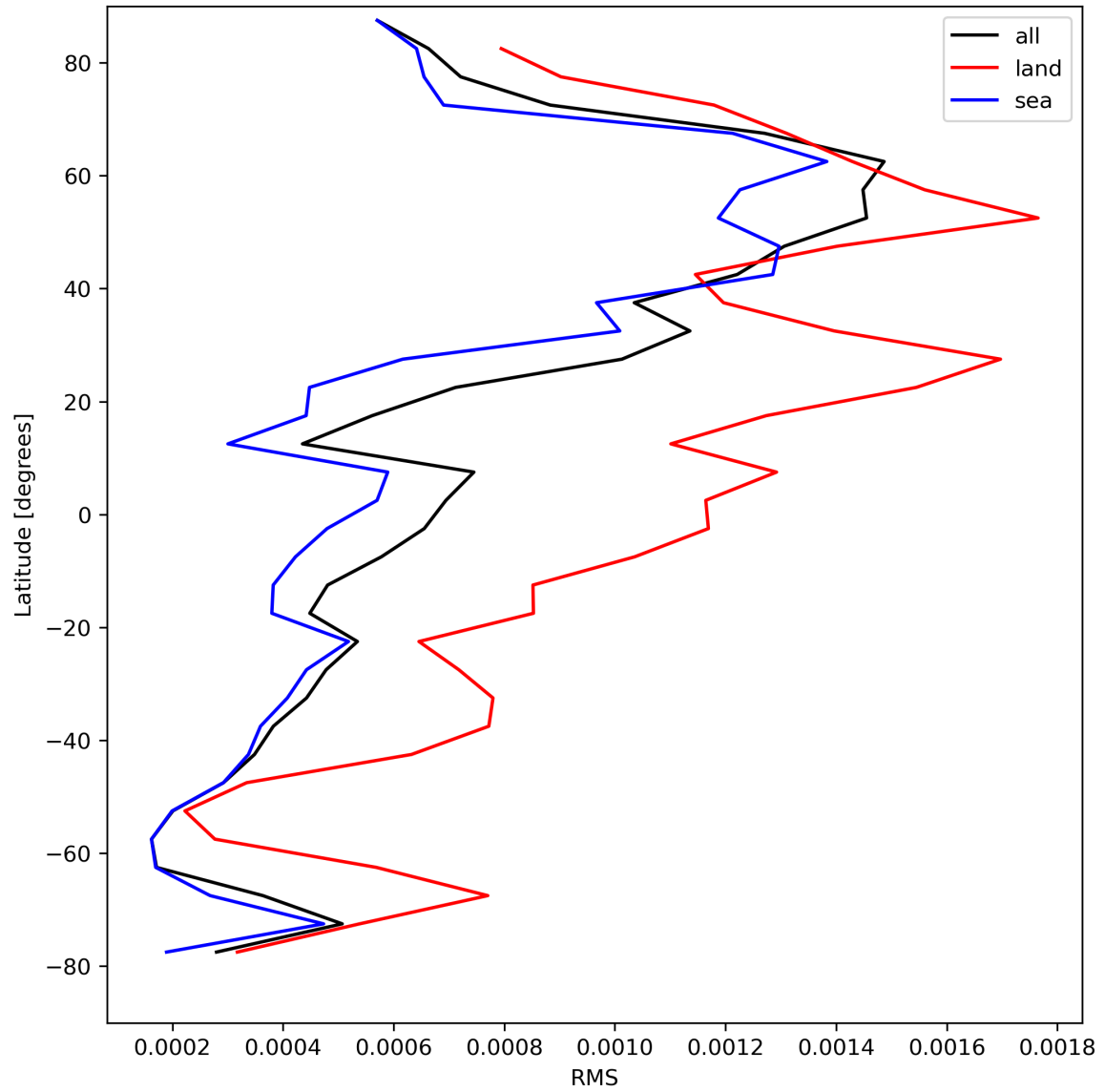
Figure 31: Zonal average of “RMS” for 2024-04-21 to 2024-04-23.
