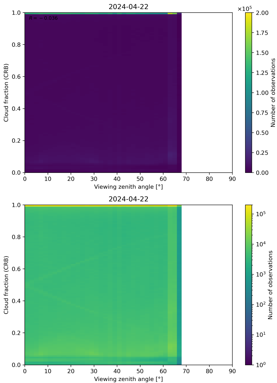
Figure 109: Scatter density plot of “Viewing zenith angle” against “Cloud fraction (CRB)” for 2024-04-21 to 2024-04-23.
