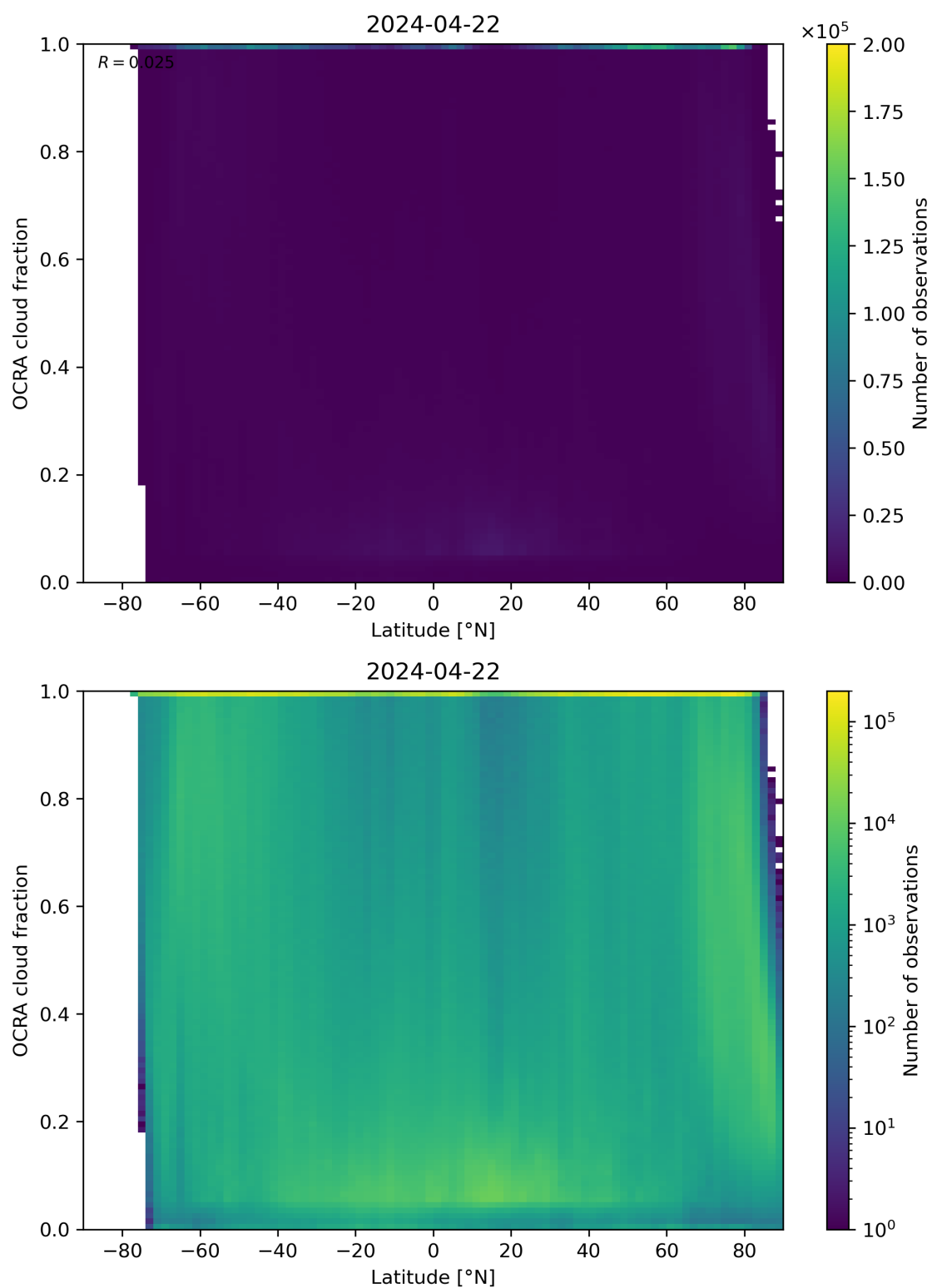
Figure 93: Scatter density plot of “Latitude” against “OCRA cloud fraction” for 2024-04-21 to 2024-04-23.
