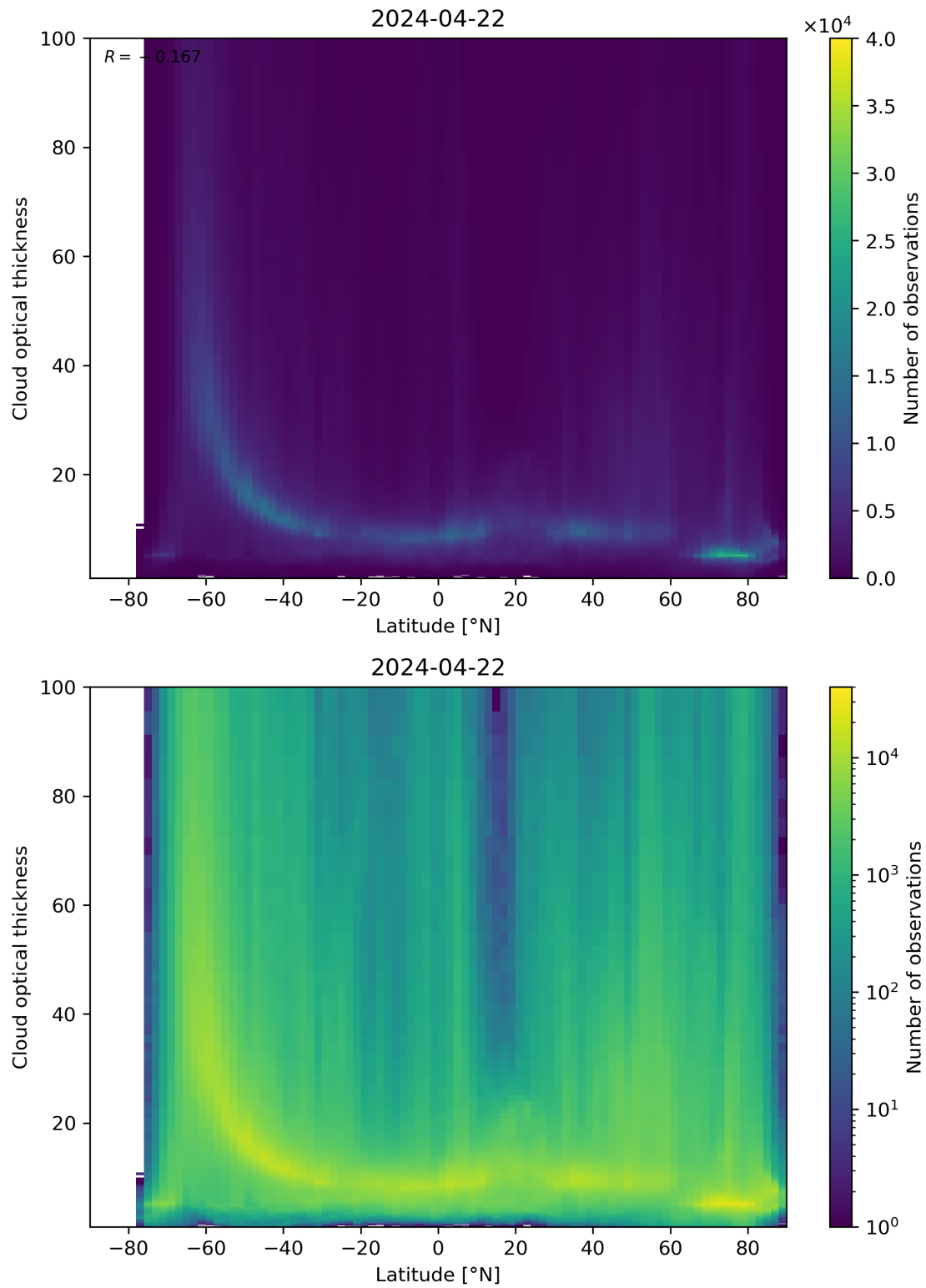
Figure 96: Scatter density plot of “Latitude” against “Cloud optical thickness” for 2024-04-21 to 2024-04-23.
