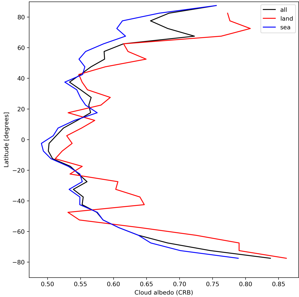
Figure 28: Zonal average of “Cloud albedo (CRB)” for 2024-04-21 to 2024-04-23.
