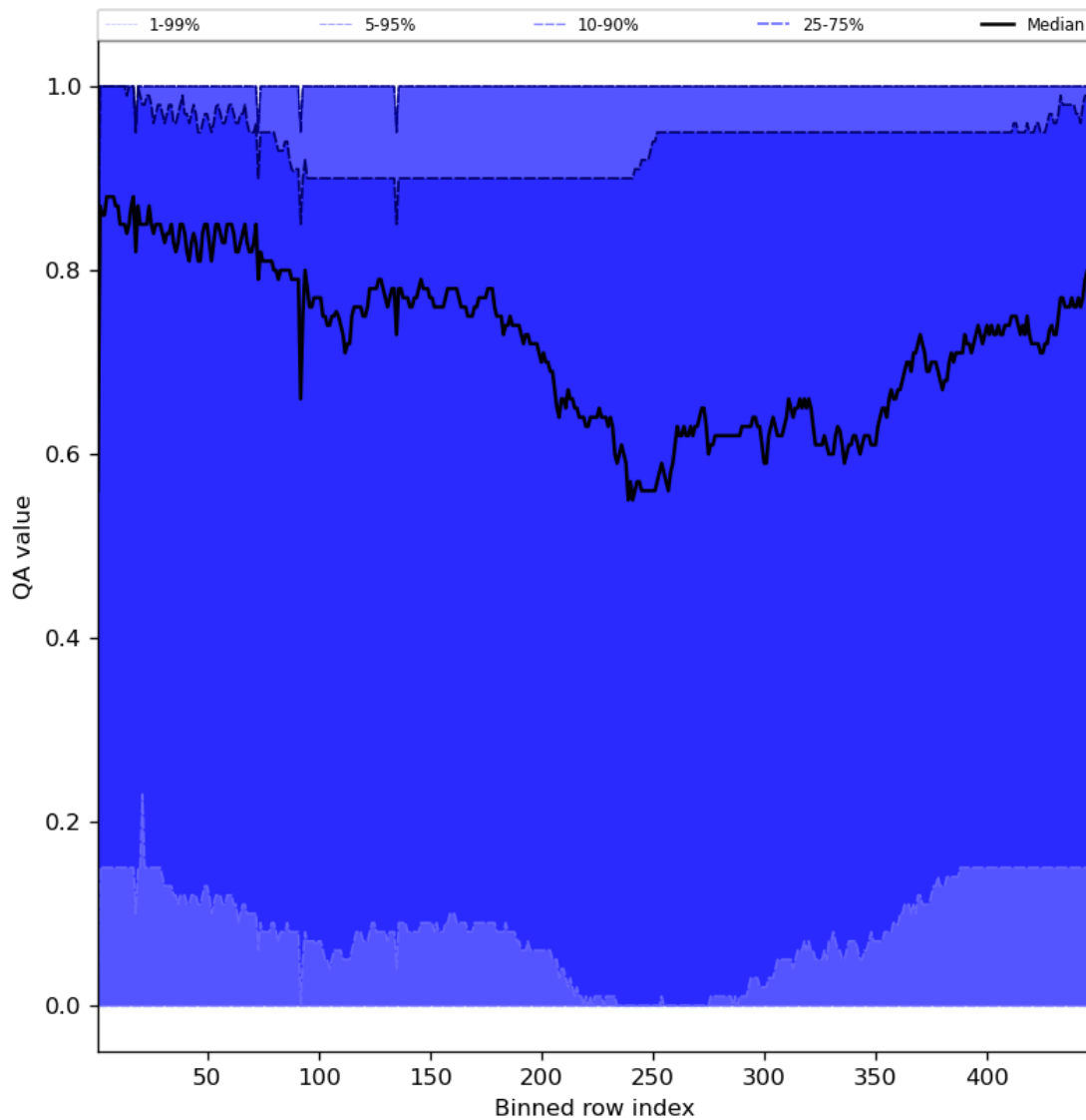
Figure 54: Along track statistics of “QA value” for 2024-04-21 to 2024-04-23
