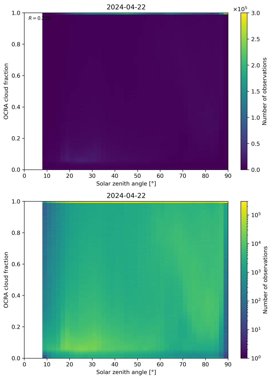
Figure 100: Scatter density plot of “Solar zenith angle” against “OCRA cloud fraction” for 2024-04-21 to 2024-04-23.
