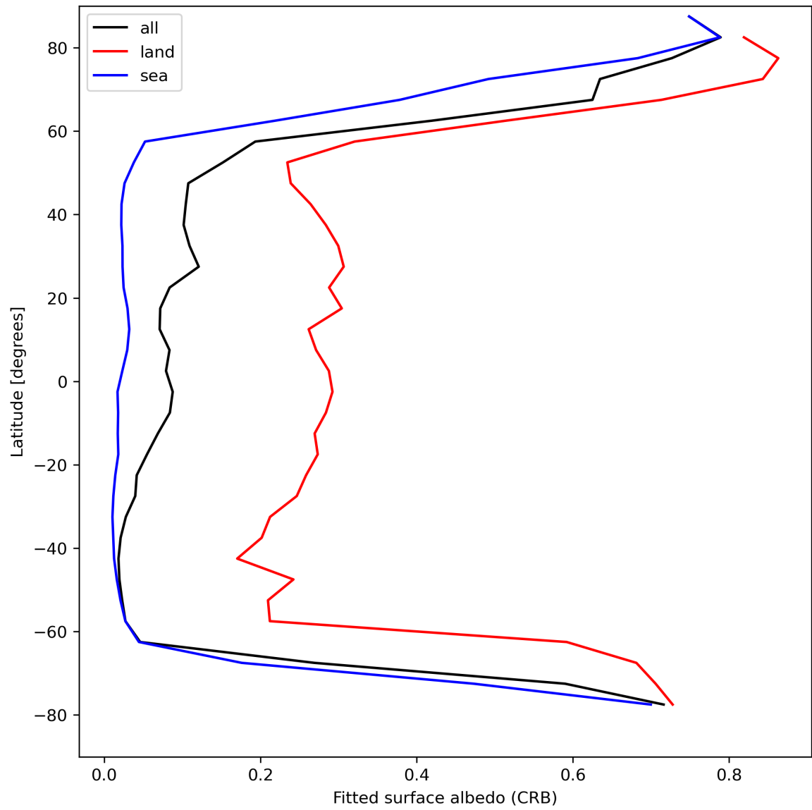
Figure 30: Zonal average of “Fitted surface albedo (CRB)” for 2024-04-21 to 2024-04-23.
