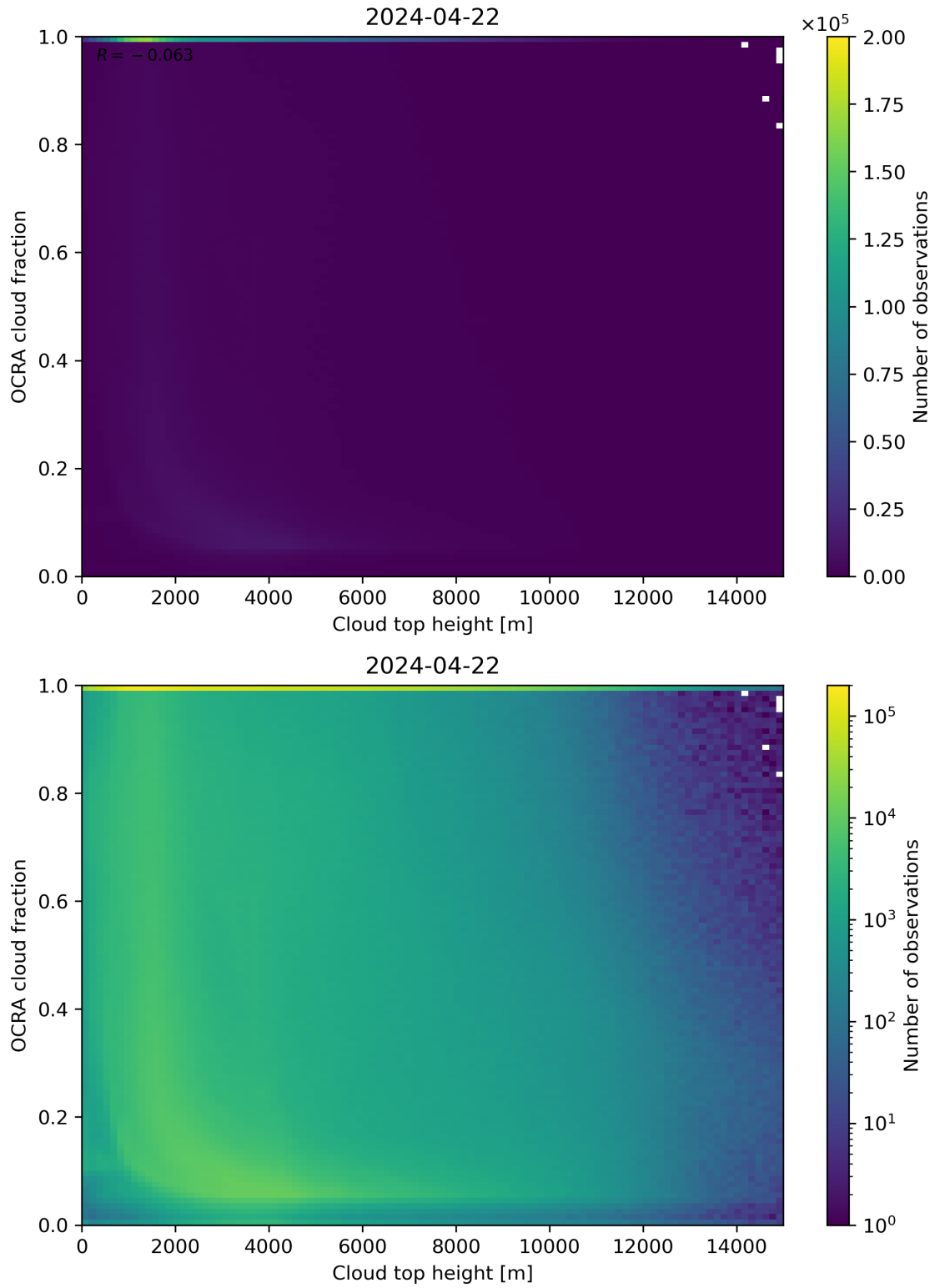
Figure 87: Scatter density plot of “Cloud top height” against “OCRA cloud fraction” for 2024-04-21 to 2024-04-23.
