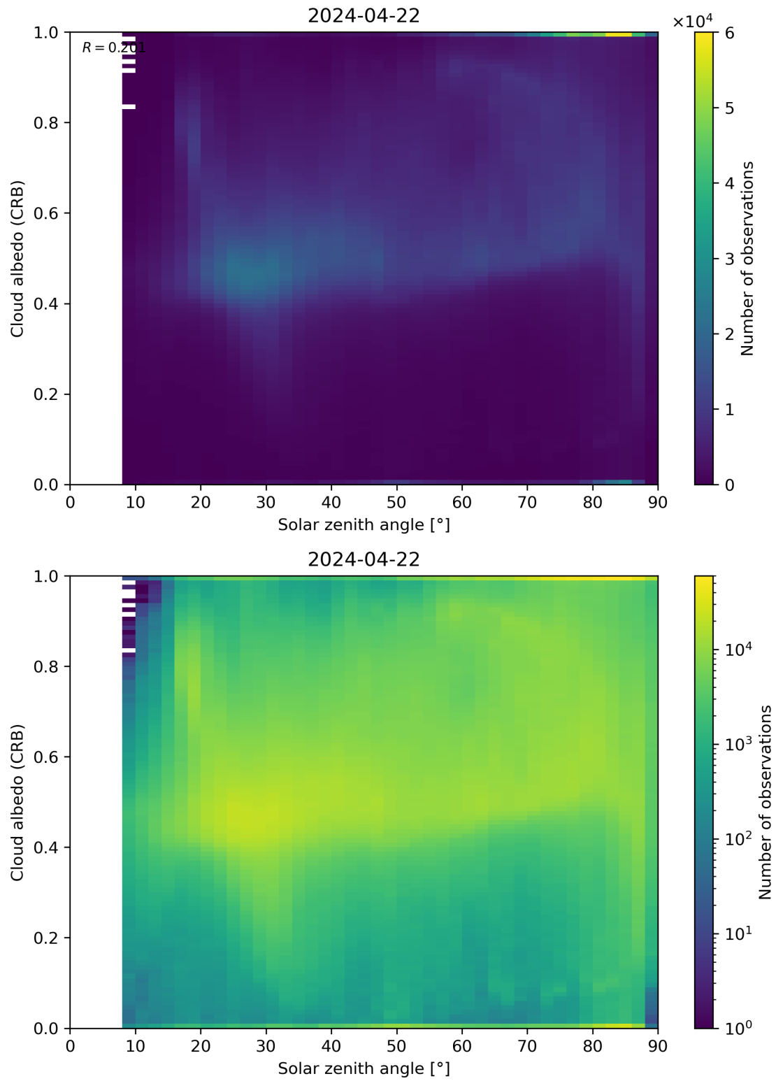
Figure 98: Scatter density plot of “Solar zenith angle” against “Cloud albedo (CRB)” for 2024-04-21 to 2024-04-23.
