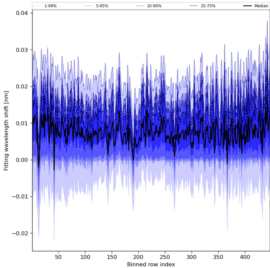
Figure 65: Along track statistics of “Fitting wavelength shift” for 2024-04-21 to 2024-04-23
