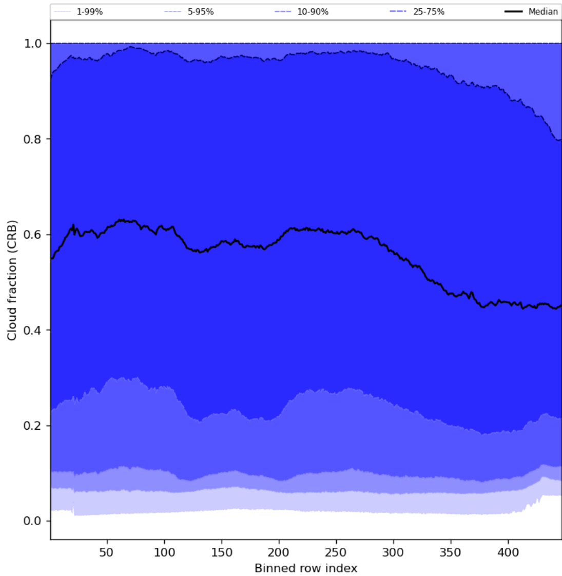
Figure 58: Along track statistics of “Cloud fraction (CRB)” for 2024-04-21 to 2024-04-23
