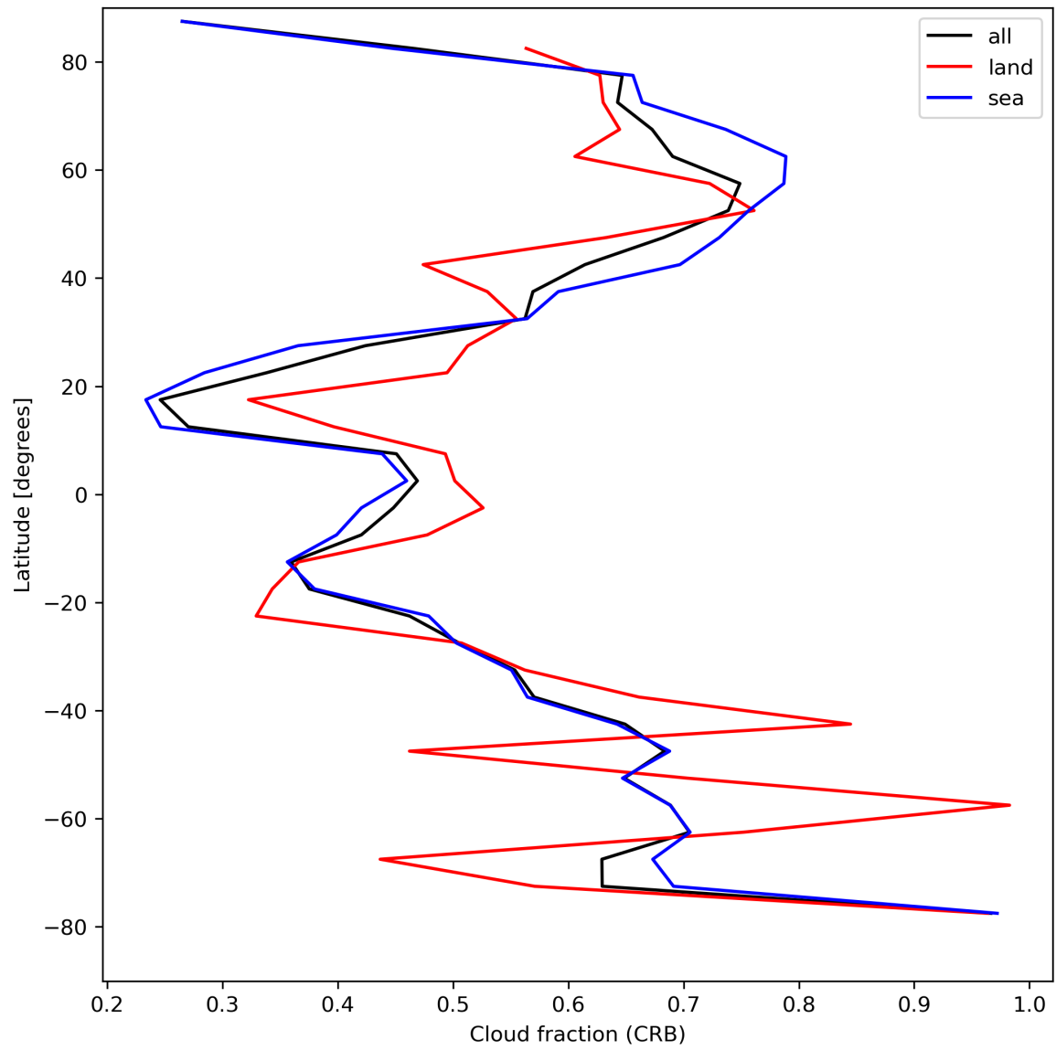
Figure 26: Zonal average of “Cloud fraction (CRB)” for 2024-04-21 to 2024-04-23.
