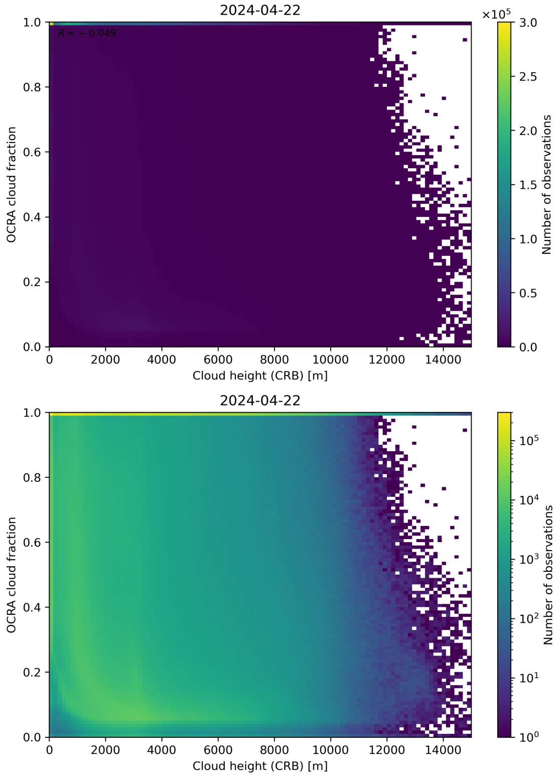
Figure 81: Scatter density plot of “Cloud height (CRB)” against “OCRA cloud fraction” for 2024-04-21 to 2024-04-23.
