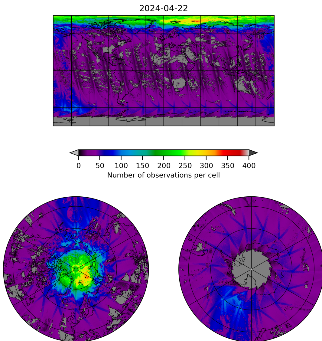
Figure 21: Map of the number of observations for 2024-04-21 to 2024-04-23
