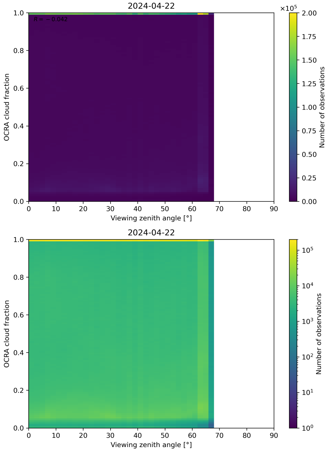
Figure 108: Scatter density plot of “Viewing zenith angle” against “OCRA cloud fraction” for 2024-04-21 to 2024-04-23.
