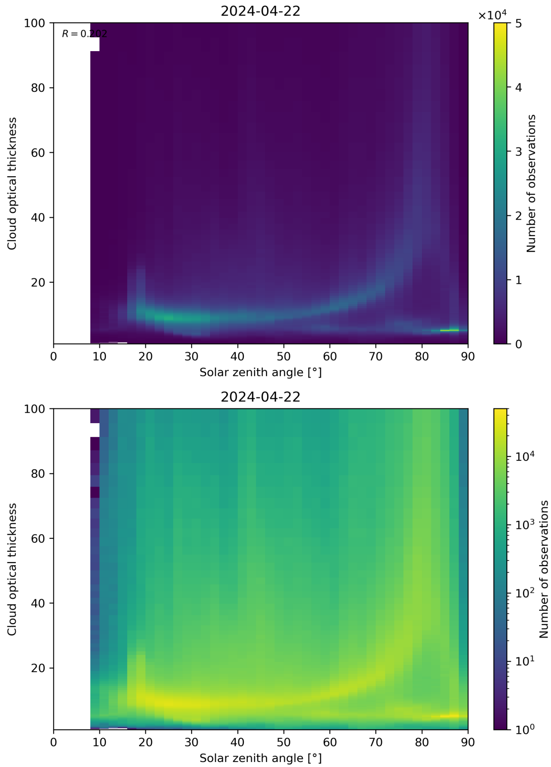
Figure 103: Scatter density plot of “Solar zenith angle” against “Cloud optical thickness” for 2024-04-21 to 2024-04-23.
