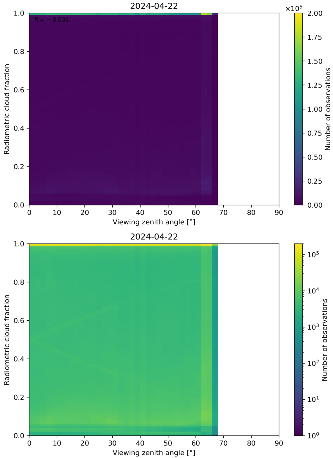
Figure 107: Scatter density plot of “Viewing zenith angle” against “Radiometric cloud fraction” for 2024-04-21 to 2024-04-23.
