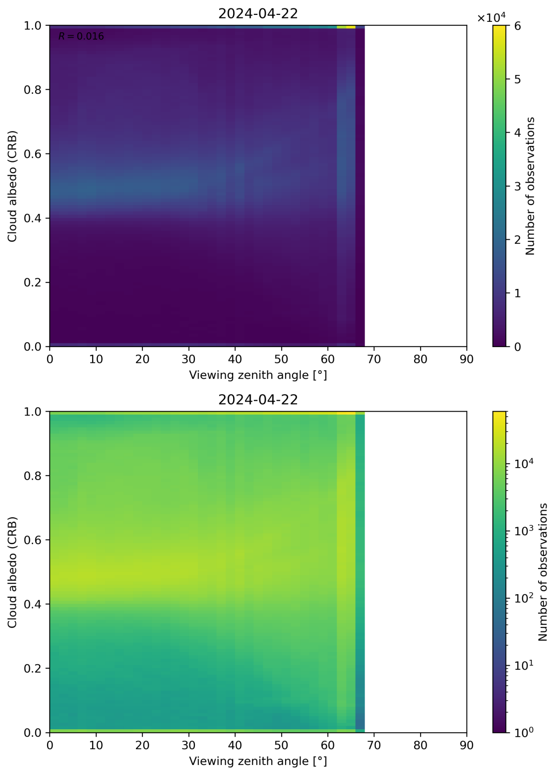
Figure 106: Scatter density plot of “Viewing zenith angle” against “Cloud albedo (CRB)” for 2024-04-21 to 2024-04-23.
