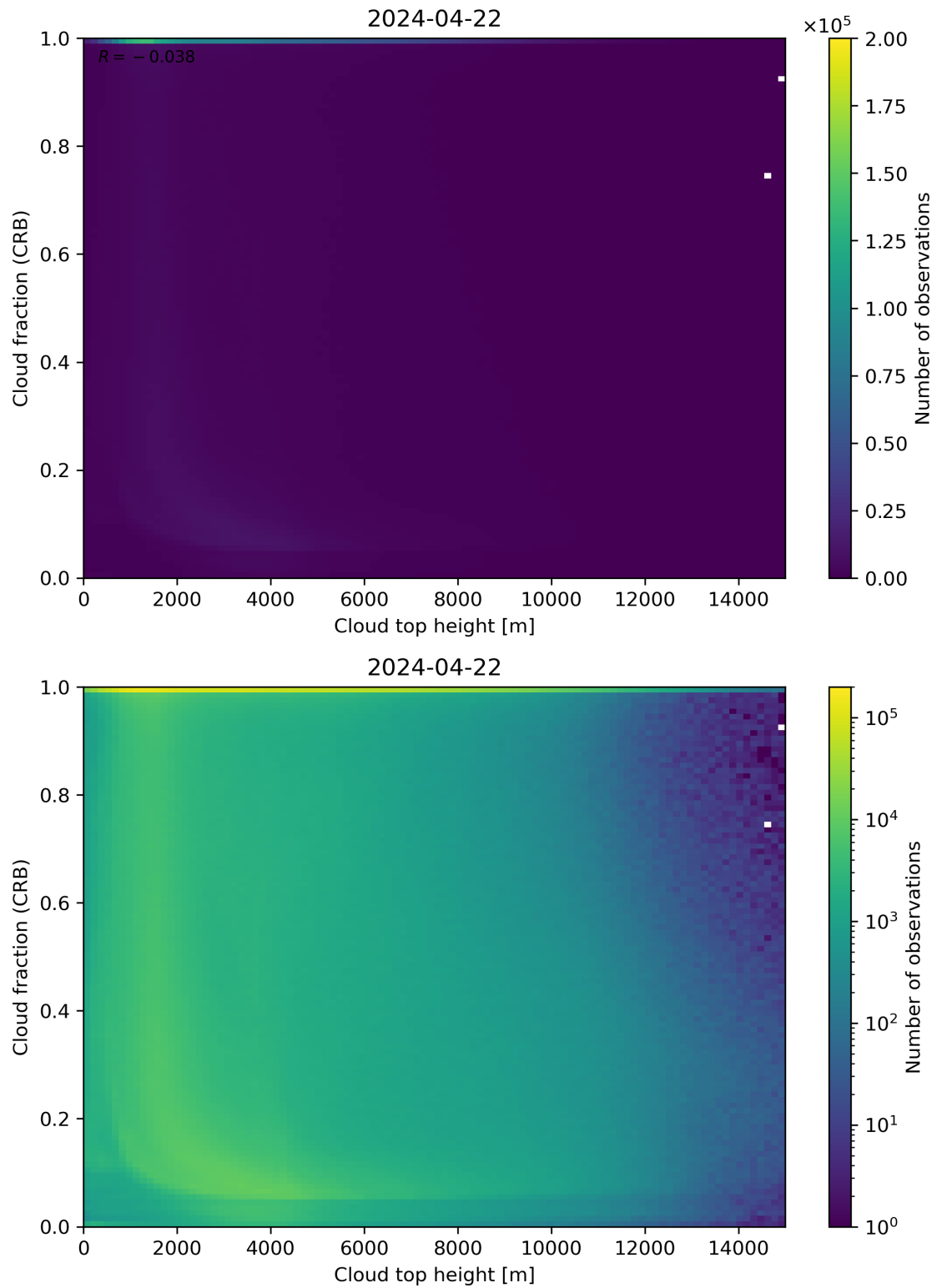
Figure 88: Scatter density plot of “Cloud top height” against “Cloud fraction (CRB)” for 2024-04-21 to 2024-04-23.
