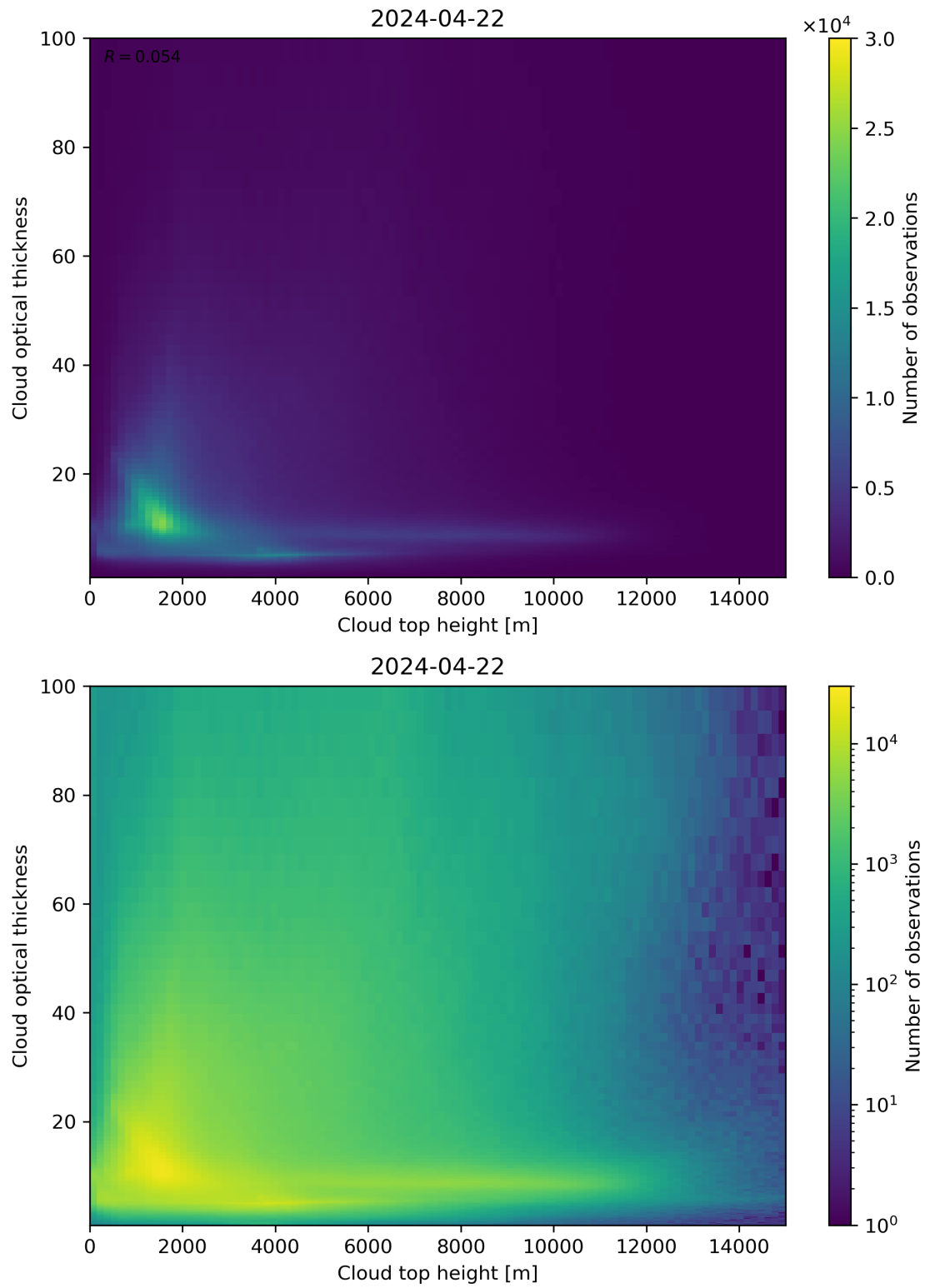
Figure 90: Scatter density plot of “Cloud top height” against “Cloud optical thickness” for 2024-04-21 to 2024-04-23.
