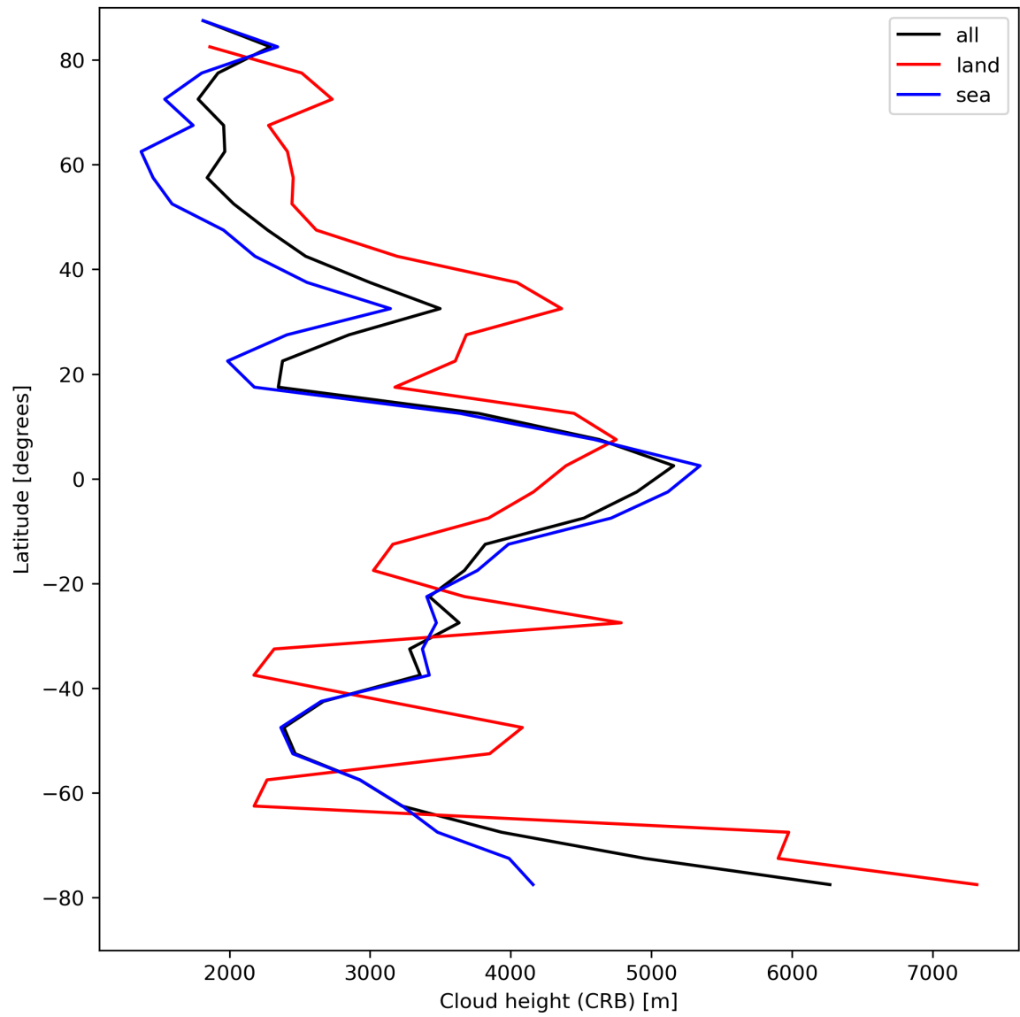
Figure 27: Zonal average of “Cloud height (CRB)” for 2024-04-21 to 2024-04-23.
