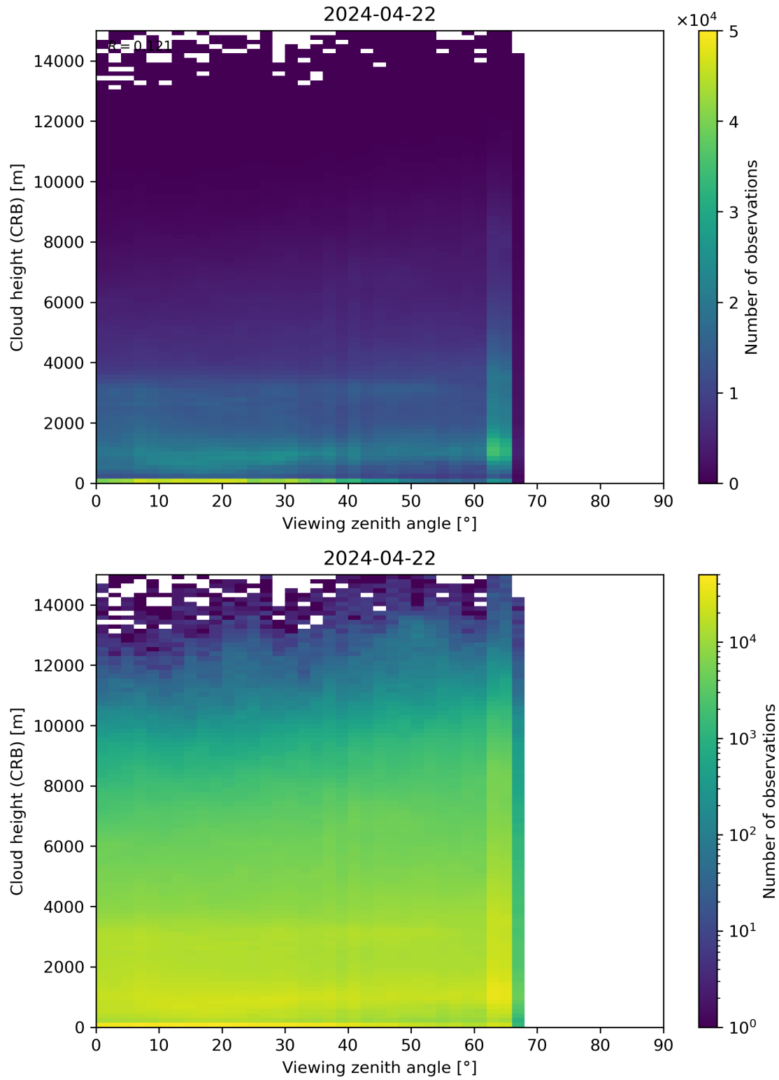
Figure 110: Scatter density plot of “Viewing zenith angle” against “Cloud height (CRB)” for 2024-04-21 to 2024-04-23.
