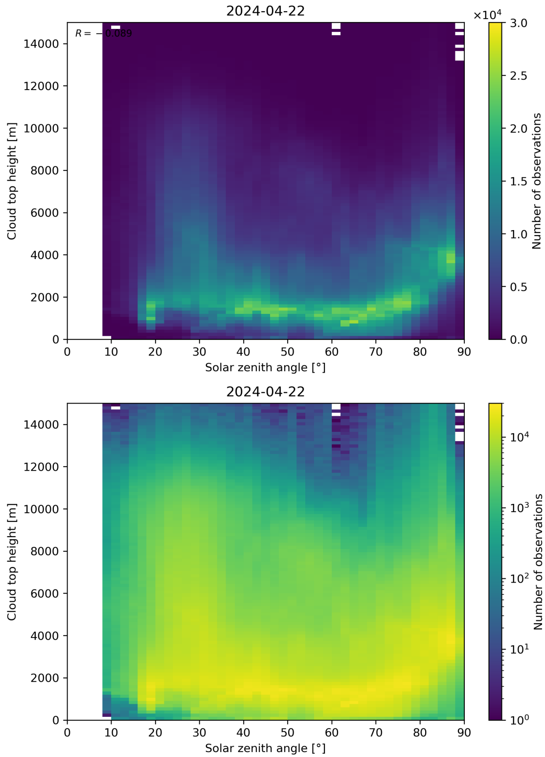
Figure 104: Scatter density plot of “Solar zenith angle” against “Cloud top height” for 2024-04-21 to 2024-04-23.
