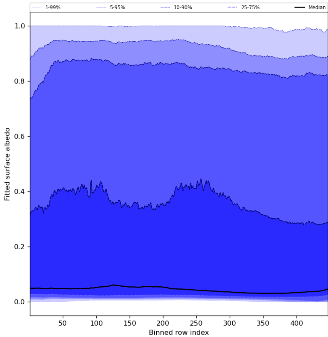
Figure 61: Along track statistics of “Fitted surface albedo” for 2024-04-21 to 2024-04-23
