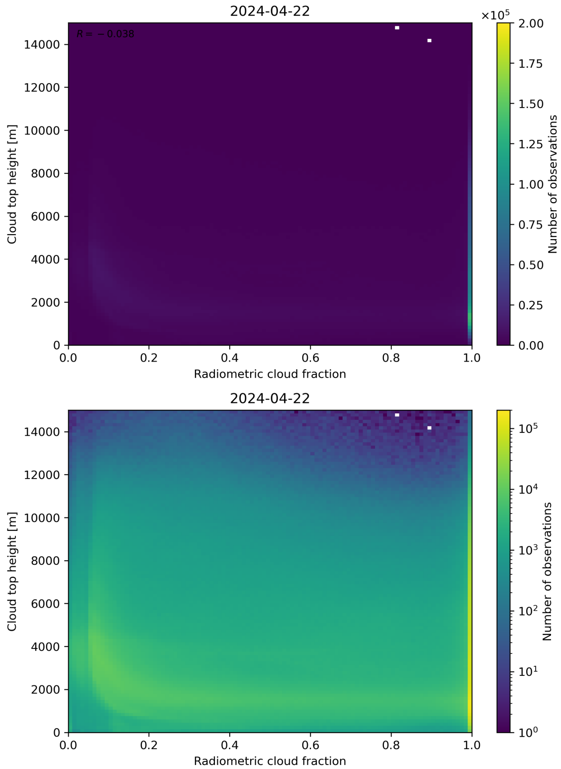
Figure 76: Scatter density plot of “Radiometric cloud fraction” against “Cloud top height” for 2024-04-21 to 2024-04-23.
