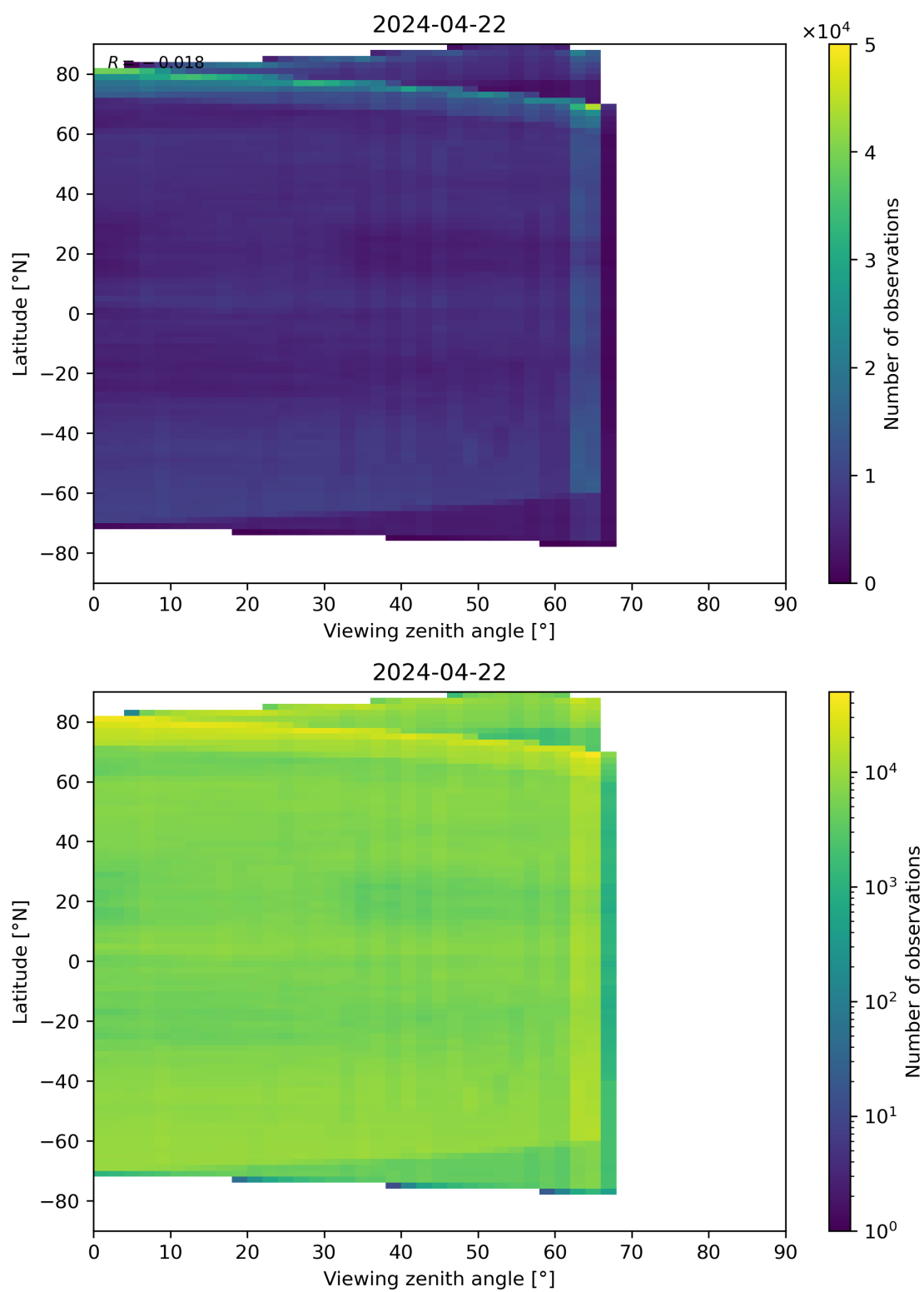
Figure 113: Scatter density plot of “Viewing zenith angle” against “Latitude” for 2024-04-21 to 2024-04-23.
