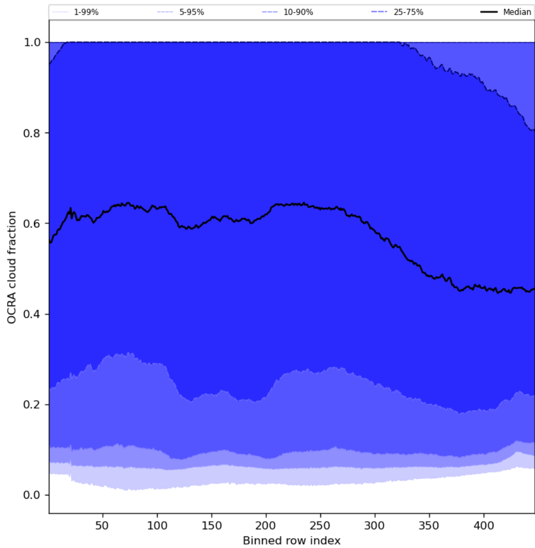
Figure 66: Along track statistics of “OCRA cloud fraction” for 2024-04-21 to 2024-04-23
