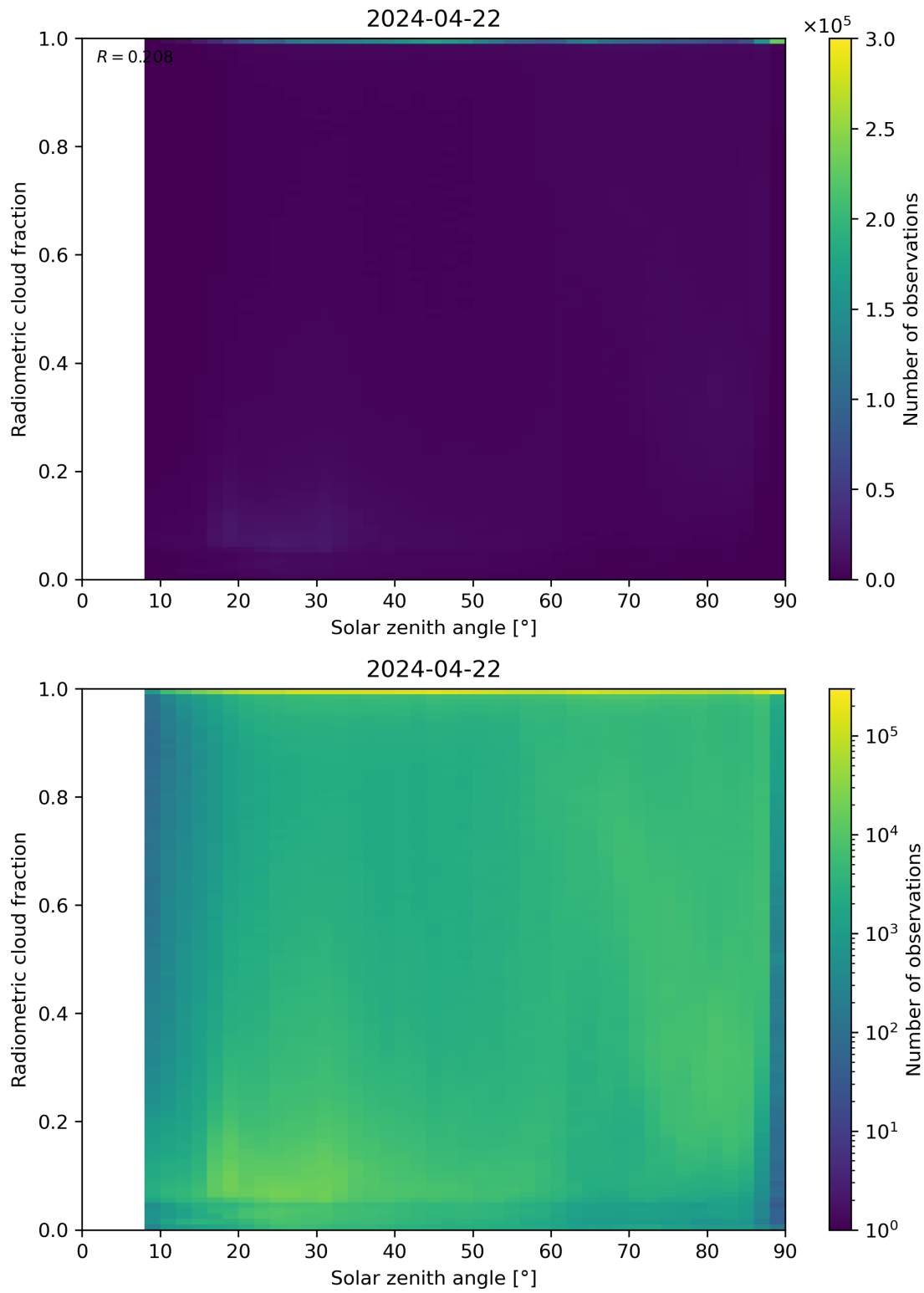
Figure 99: Scatter density plot of “Solar zenith angle” against “Radiometric cloud fraction” for 2024-04-21 to 2024-04-23.
