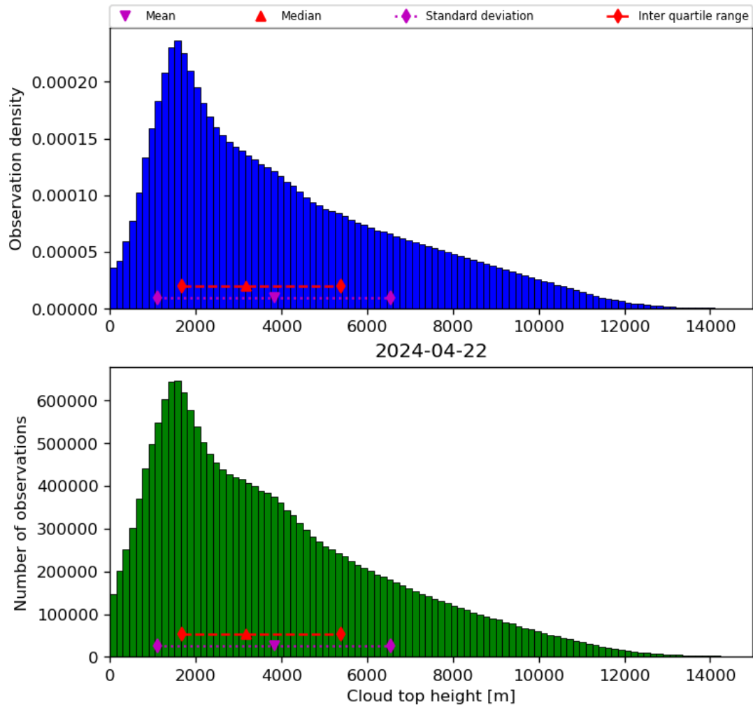
Figure 40: Histogram of “Cloud top height” for 2024-04-21 to 2024-04-23
