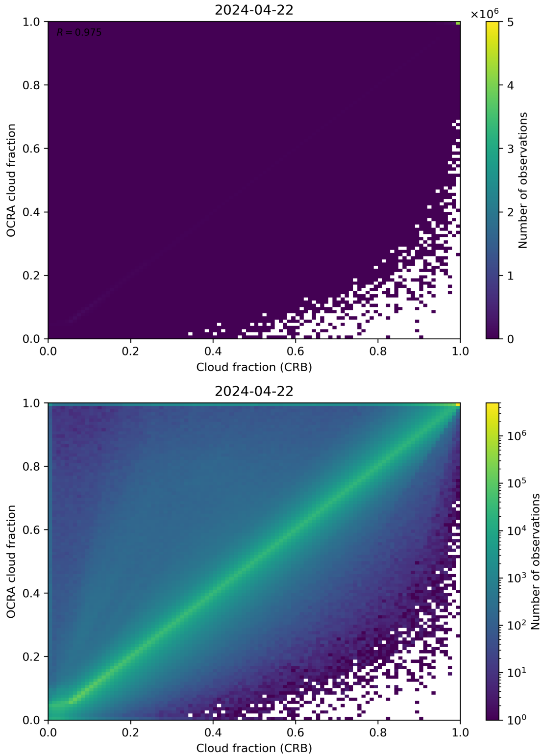
Figure 78: Scatter density plot of “Cloud fraction (CRB)” against “OCRA cloud fraction” for 2024-04-21 to 2024-04-23.
