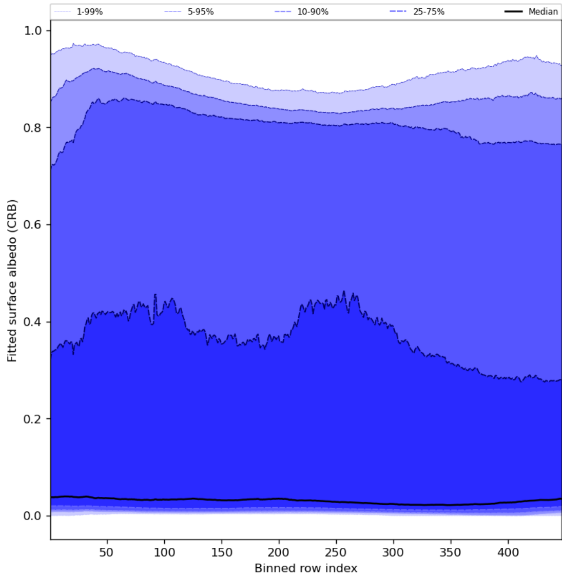
Figure 62: Along track statistics of “Fitted surface albedo (CRB)” for 2024-04-21 to 2024-04-23
