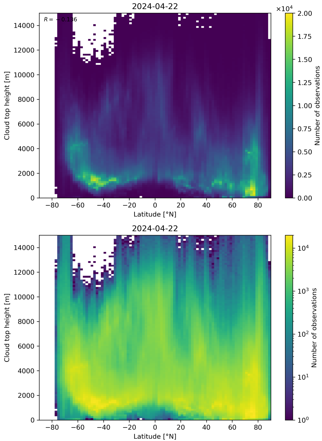
Figure 97: Scatter density plot of “Latitude” against “Cloud top height” for 2024-04-21 to 2024-04-23.
