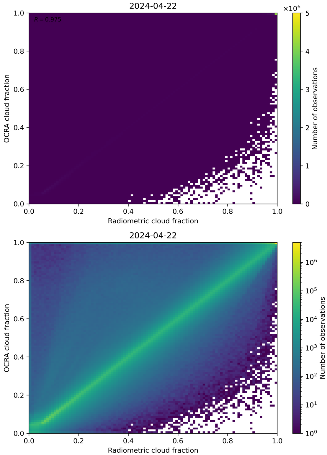
Figure 72: Scatter density plot of “Radiometric cloud fraction” against “OCRA cloud fraction” for 2024-04-21 to 2024-04-23.
