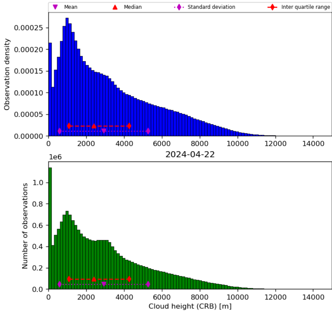
Figure 43: Histogram of “Cloud height (CRB)” for 2024-04-21 to 2024-04-23
