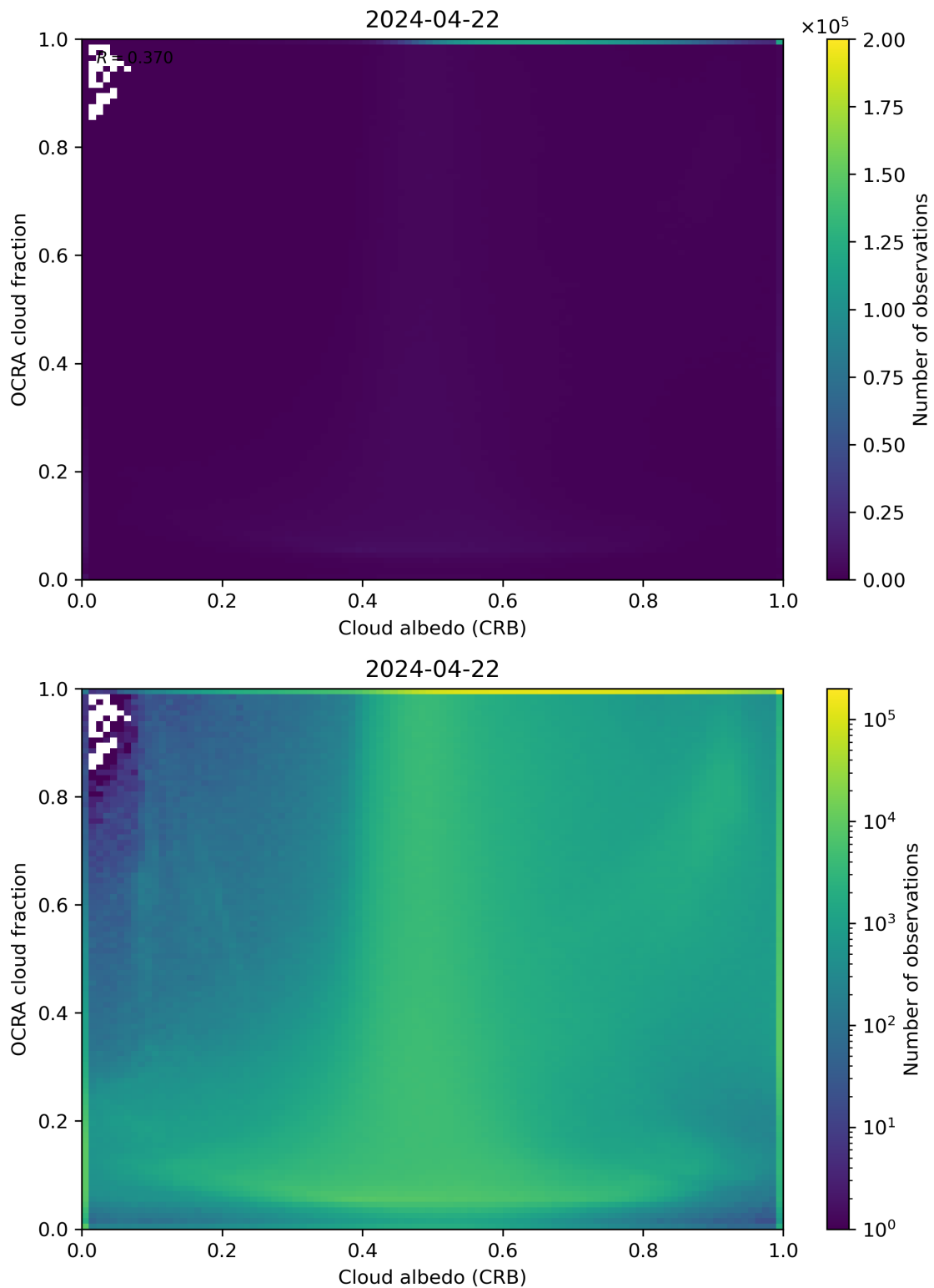
Figure 70: Scatter density plot of “Cloud albedo (CRB)” against “OCRA cloud fraction” for 2024-04-21 to 2024-04-23.
