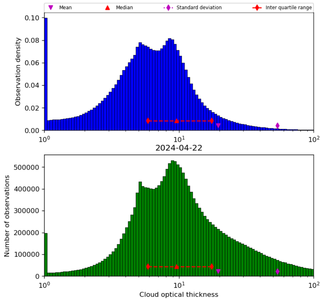
Figure 41: Histogram of “Cloud optical thickness” for 2024-04-21 to 2024-04-23
