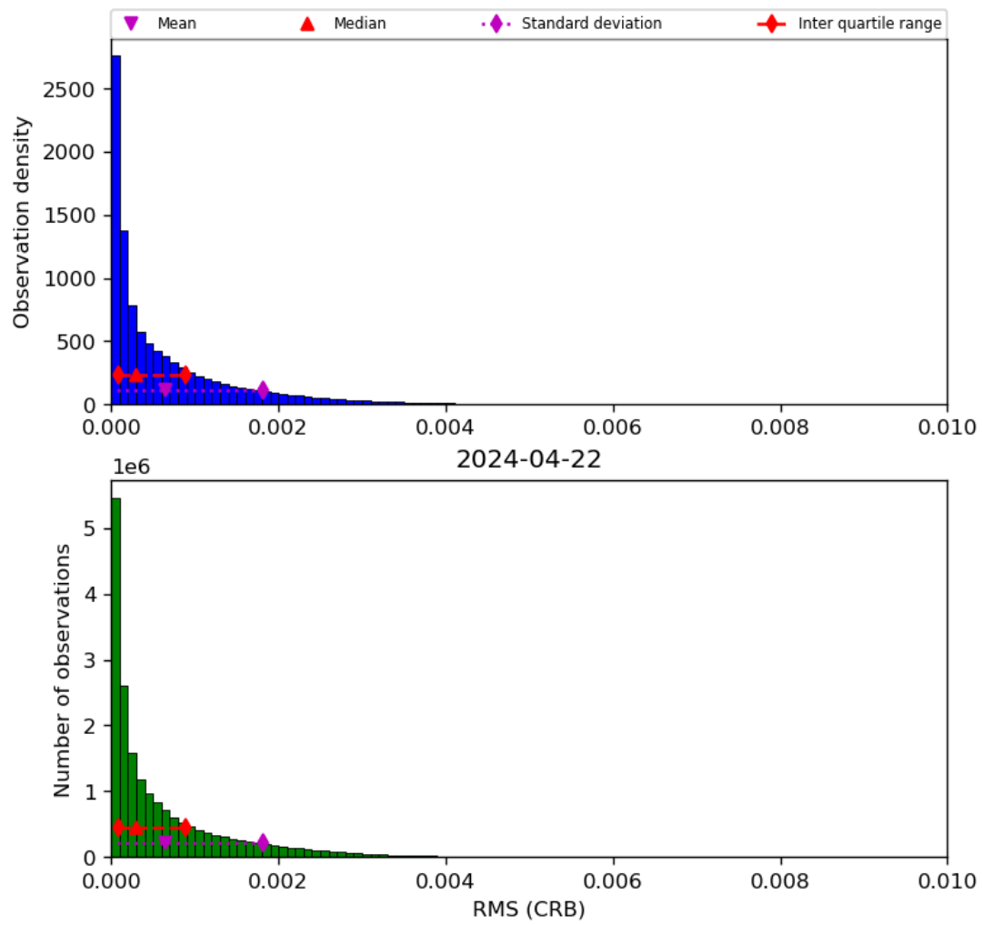
Figure 48: Histogram of “RMS (CRB)” for 2024-04-21 to 2024-04-23
