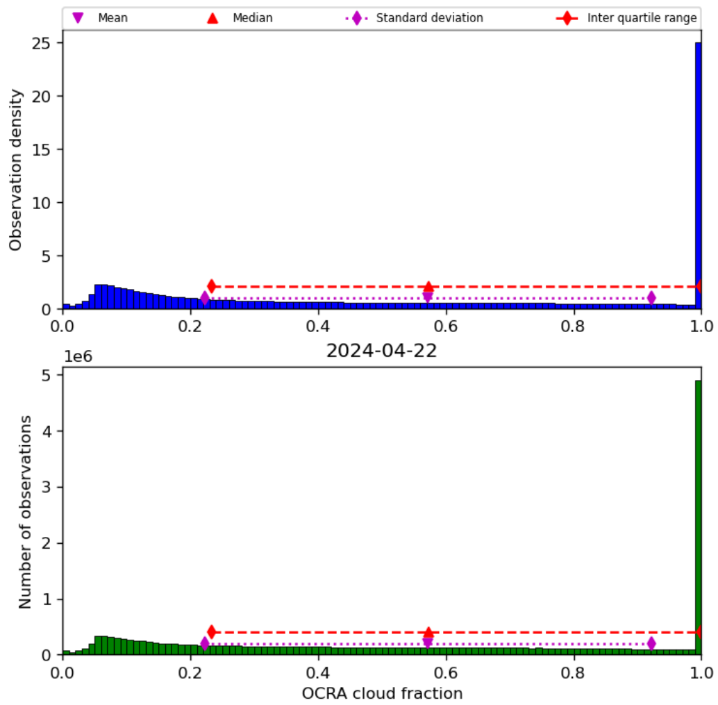
Figure 50: Histogram of “OCRA cloud fraction” for 2024-04-21 to 2024-04-23
