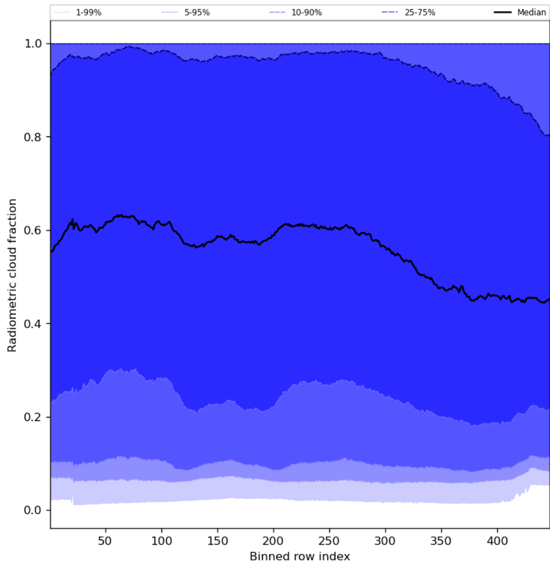
Figure 55: Along track statistics of “Radiometric cloud fraction” for 2024-04-21 to 2024-04-23
