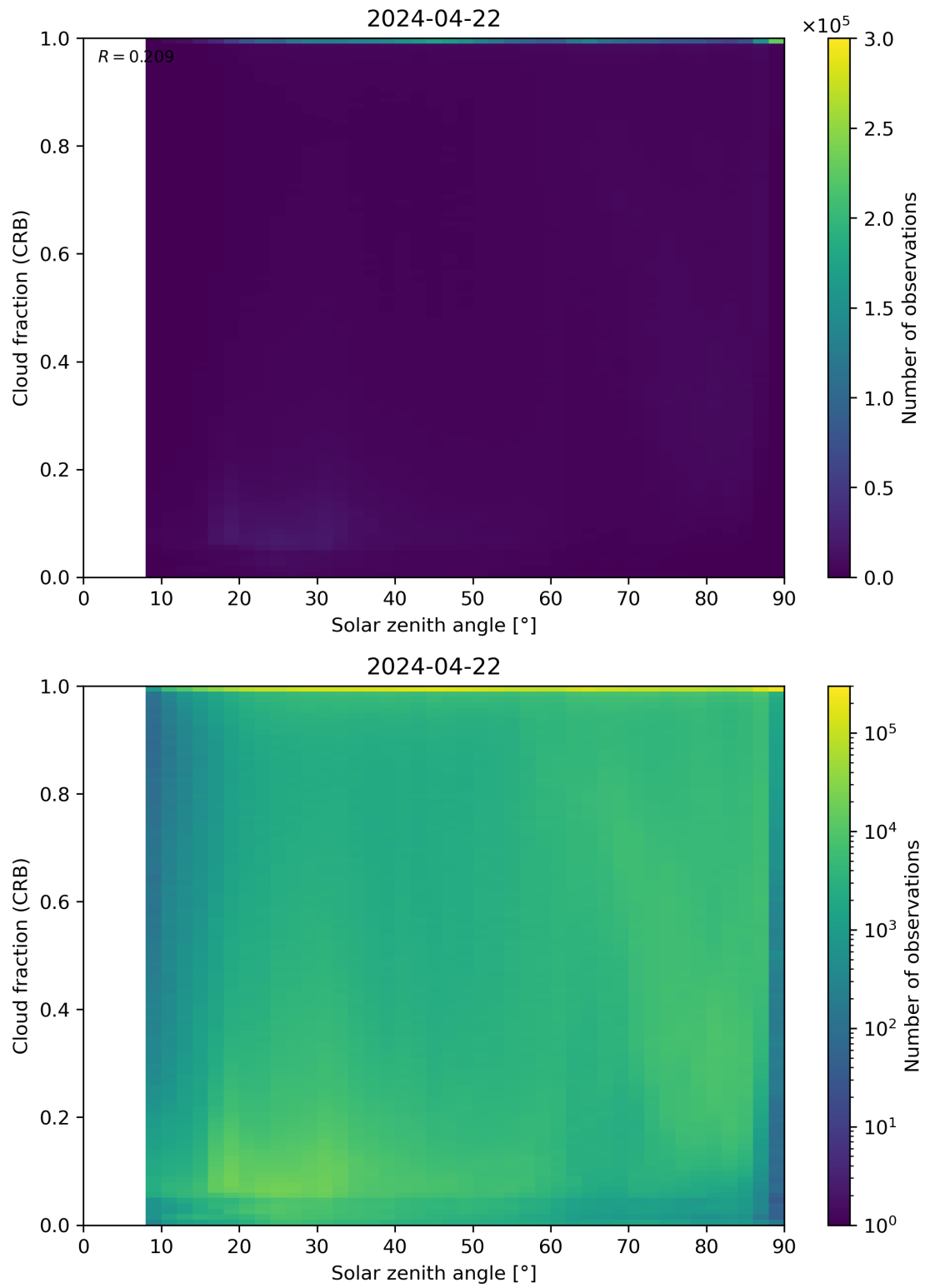
Figure 101: Scatter density plot of “Solar zenith angle” against “Cloud fraction (CRB)” for 2024-04-21 to 2024-04-23.
