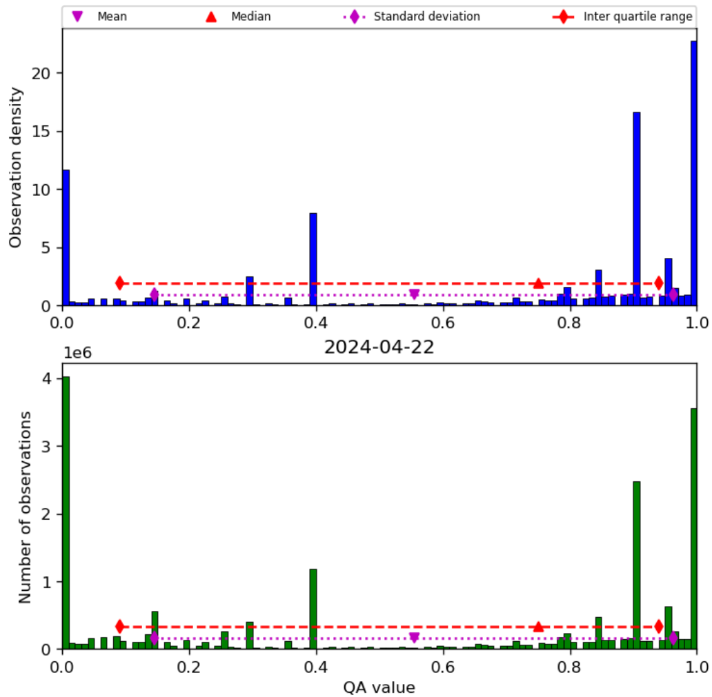
Figure 38: Histogram of “QA value” for 2024-04-21 to 2024-04-23
