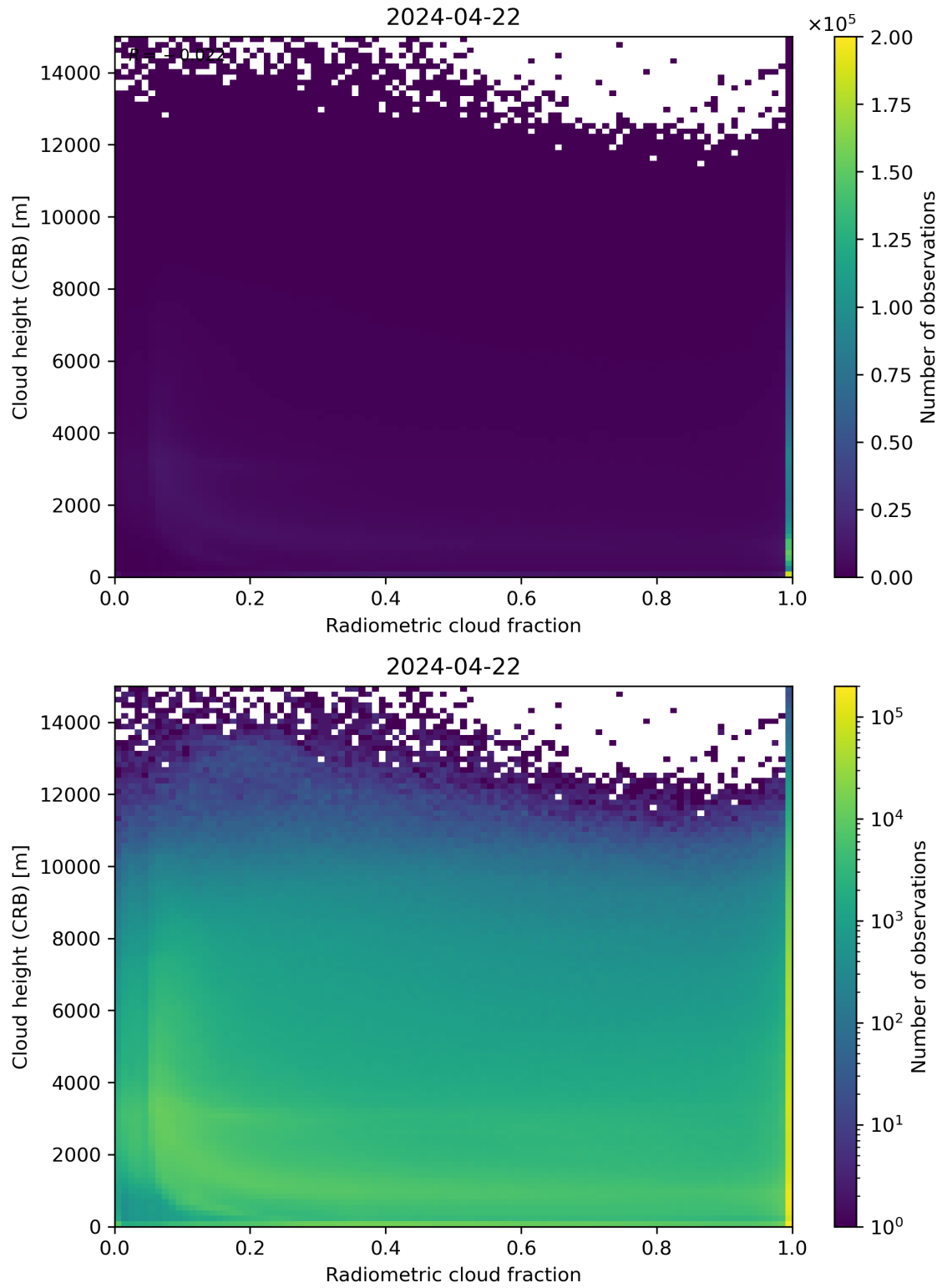
Figure 74: Scatter density plot of “Radiometric cloud fraction” against “Cloud height (CRB)” for 2024-04-21 to 2024-04-23.
