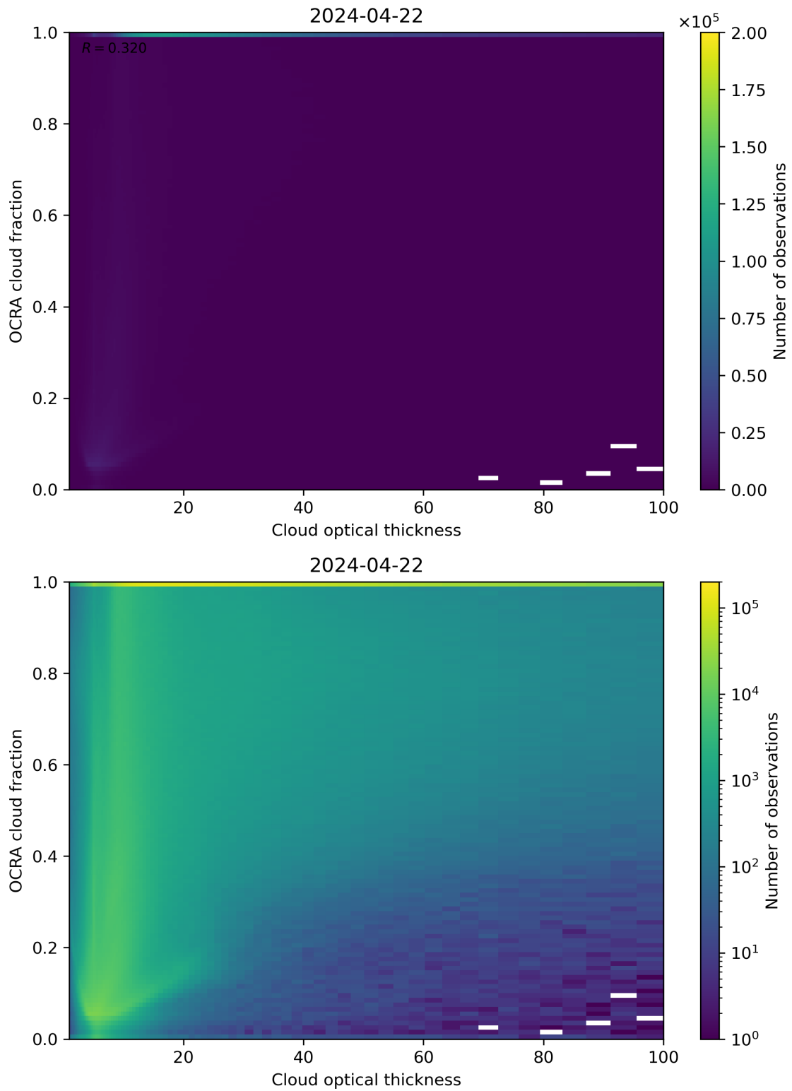
Figure 83: Scatter density plot of “Cloud optical thickness” against “OCRA cloud fraction” for 2024-04-21 to 2024-04-23.
