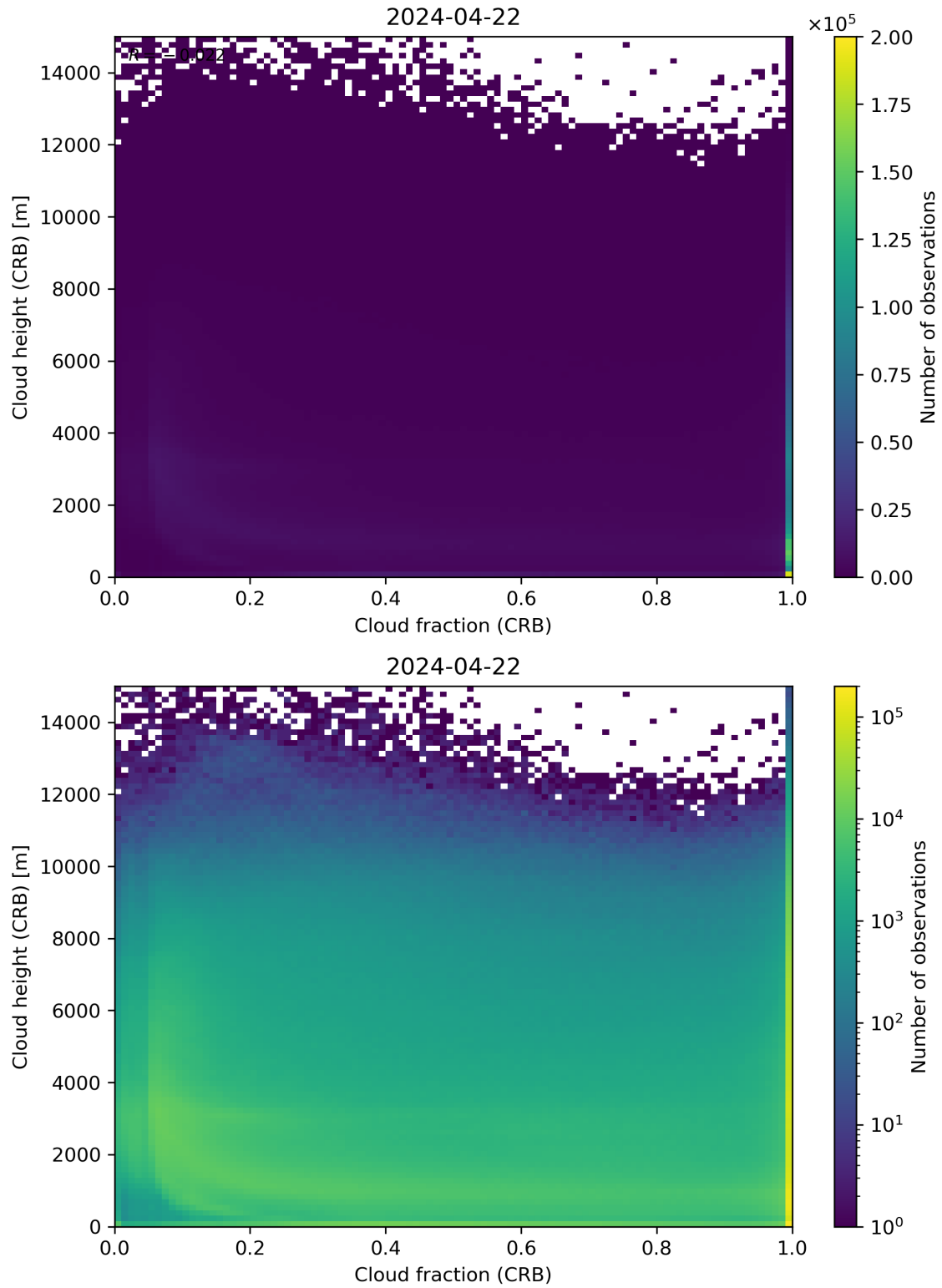
Figure 79: Scatter density plot of “Cloud fraction (CRB)” against “Cloud height (CRB)” for 2024-04-21 to 2024-04-23.
