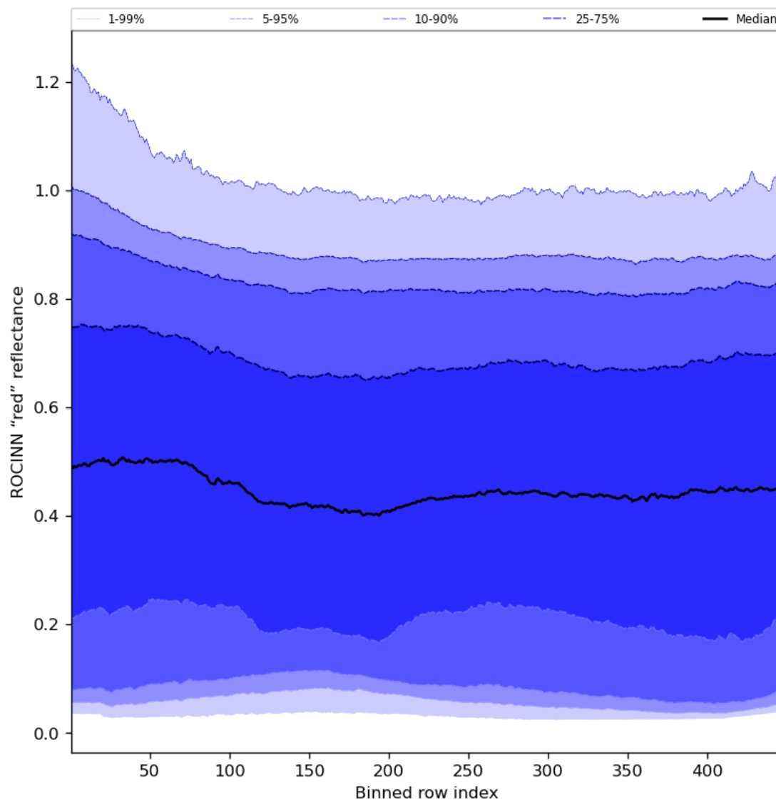
Figure 69: Along track statistics of “ROCINN “red” reflectance” for 2024-04-21 to 2024-04-23
