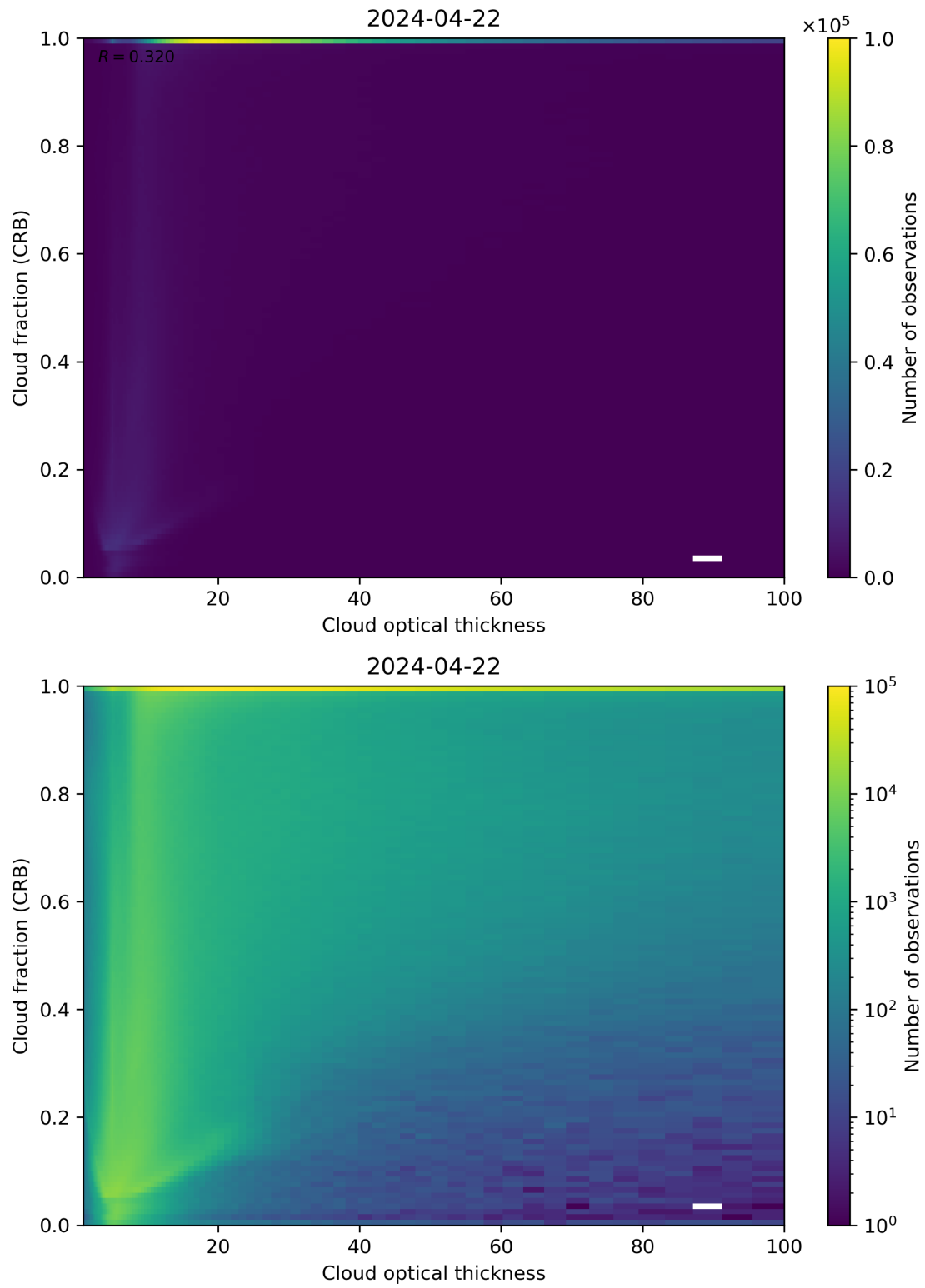
Figure 84: Scatter density plot of “Cloud optical thickness” against “Cloud fraction (CRB)” for 2024-04-21 to 2024-04-23.
