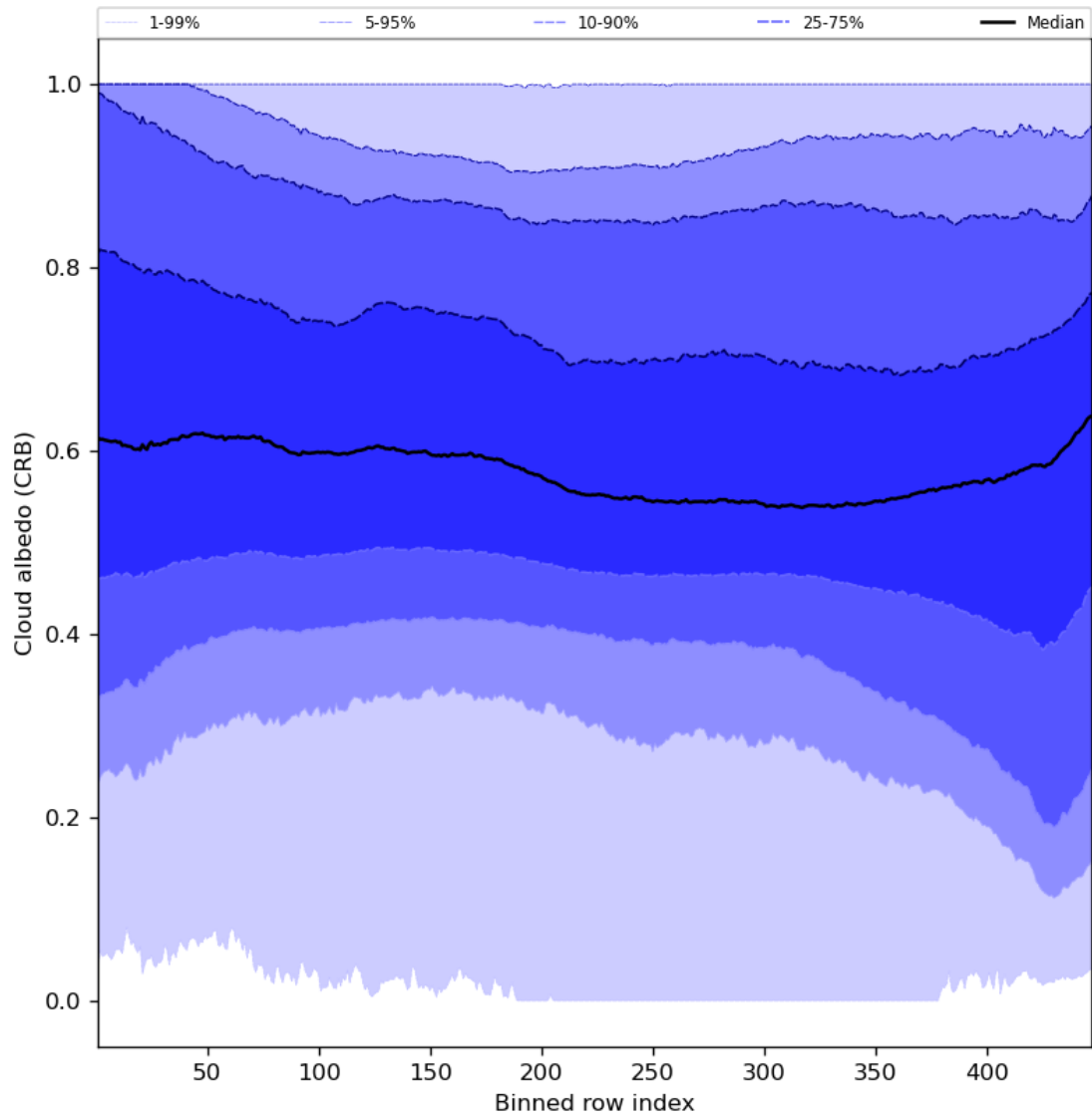
Figure 60: Along track statistics of “Cloud albedo (CRB)” for 2024-04-21 to 2024-04-23
