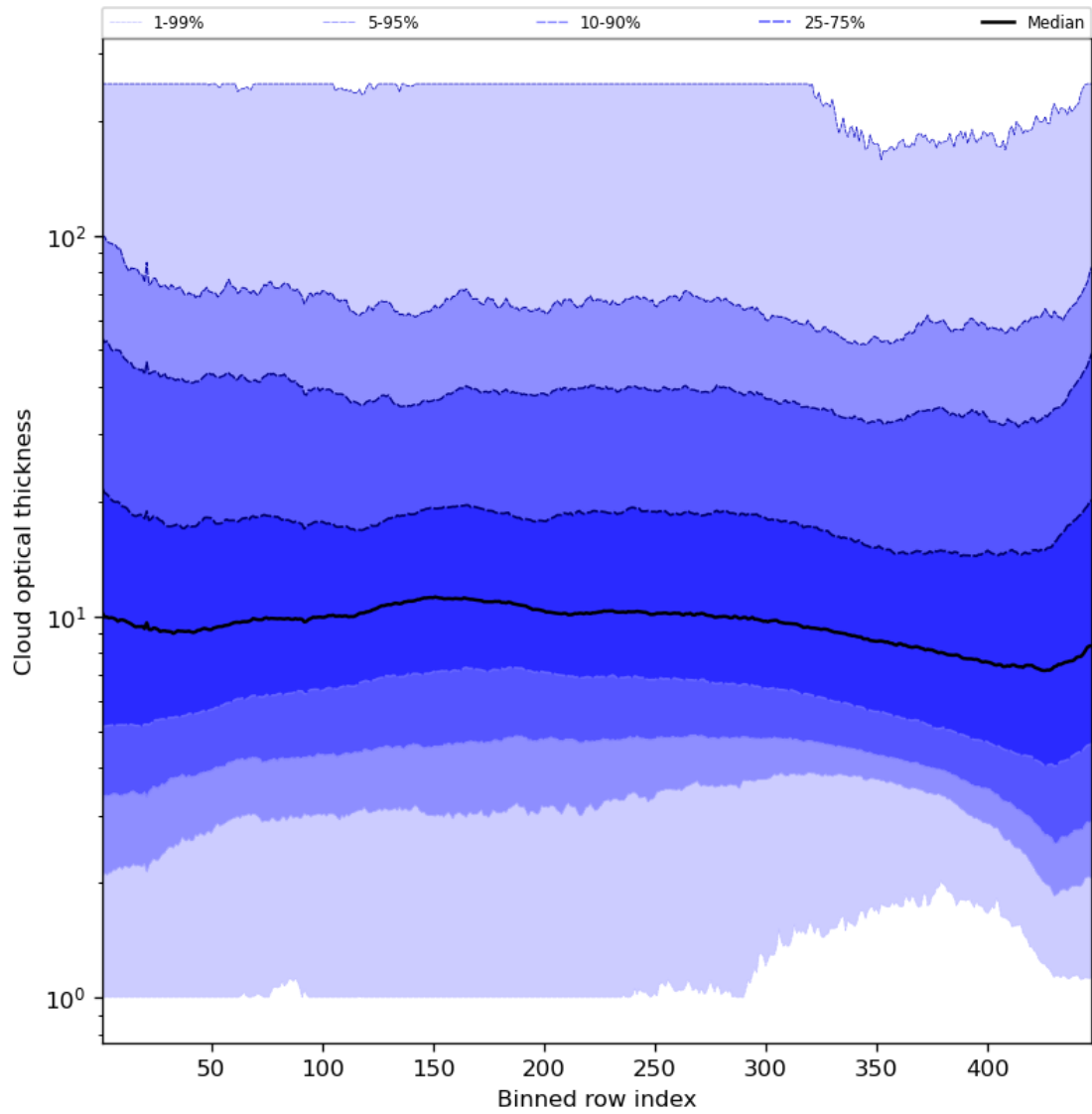
Figure 57: Along track statistics of “Cloud optical thickness” for 2024-04-21 to 2024-04-23
