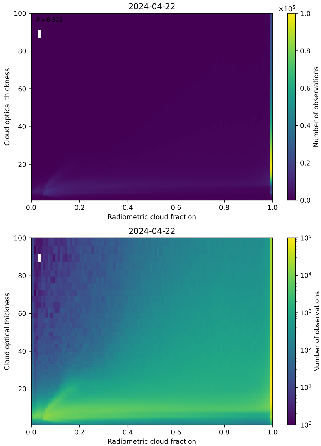
Figure 75: Scatter density plot of “Radiometric cloud fraction” against “Cloud optical thickness” for 2024-04-21 to 2024-04-23.
