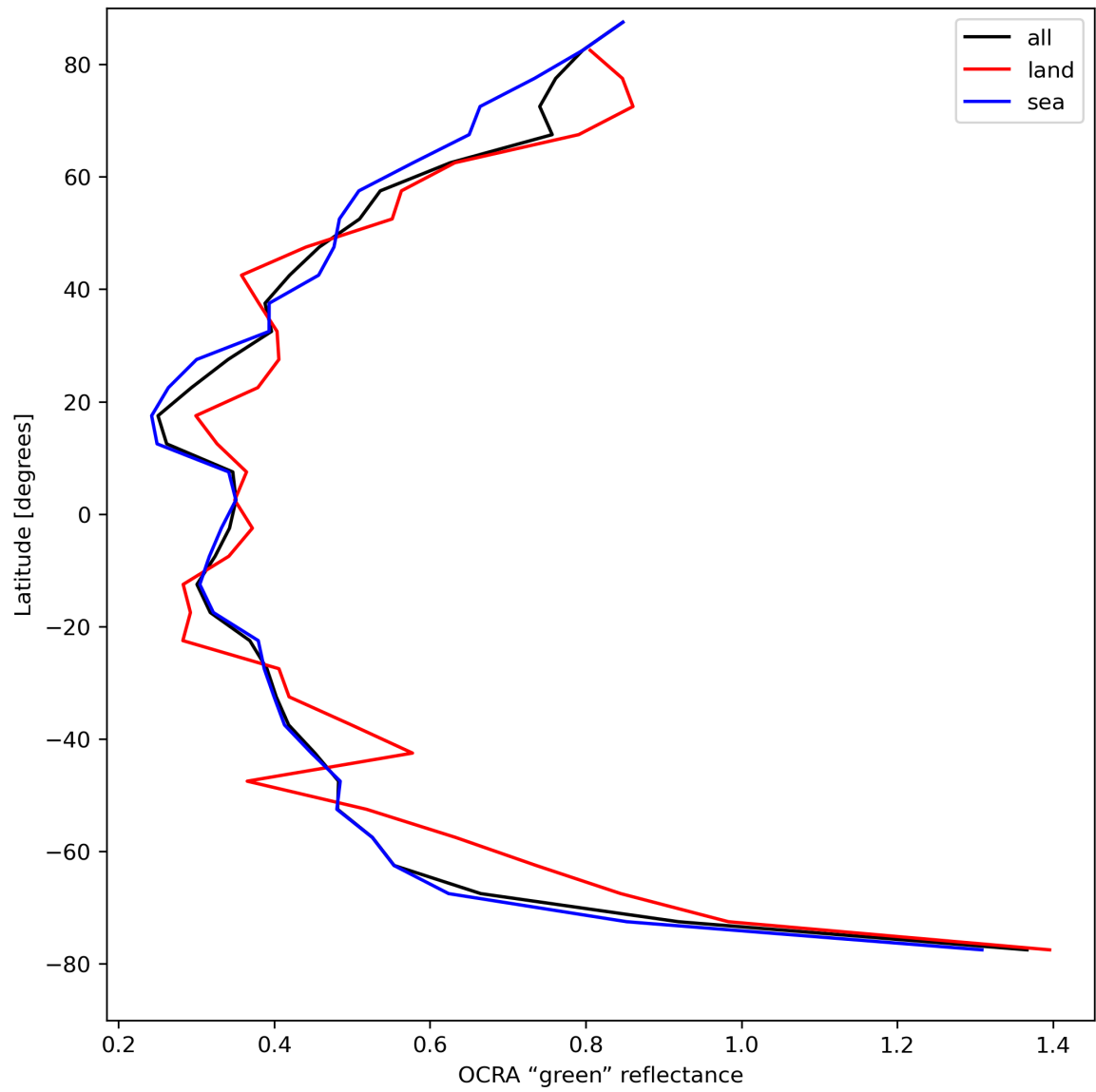
Figure 36: Zonal average of “OCRA “green” reflectance” for 2024-04-21 to 2024-04-23.
