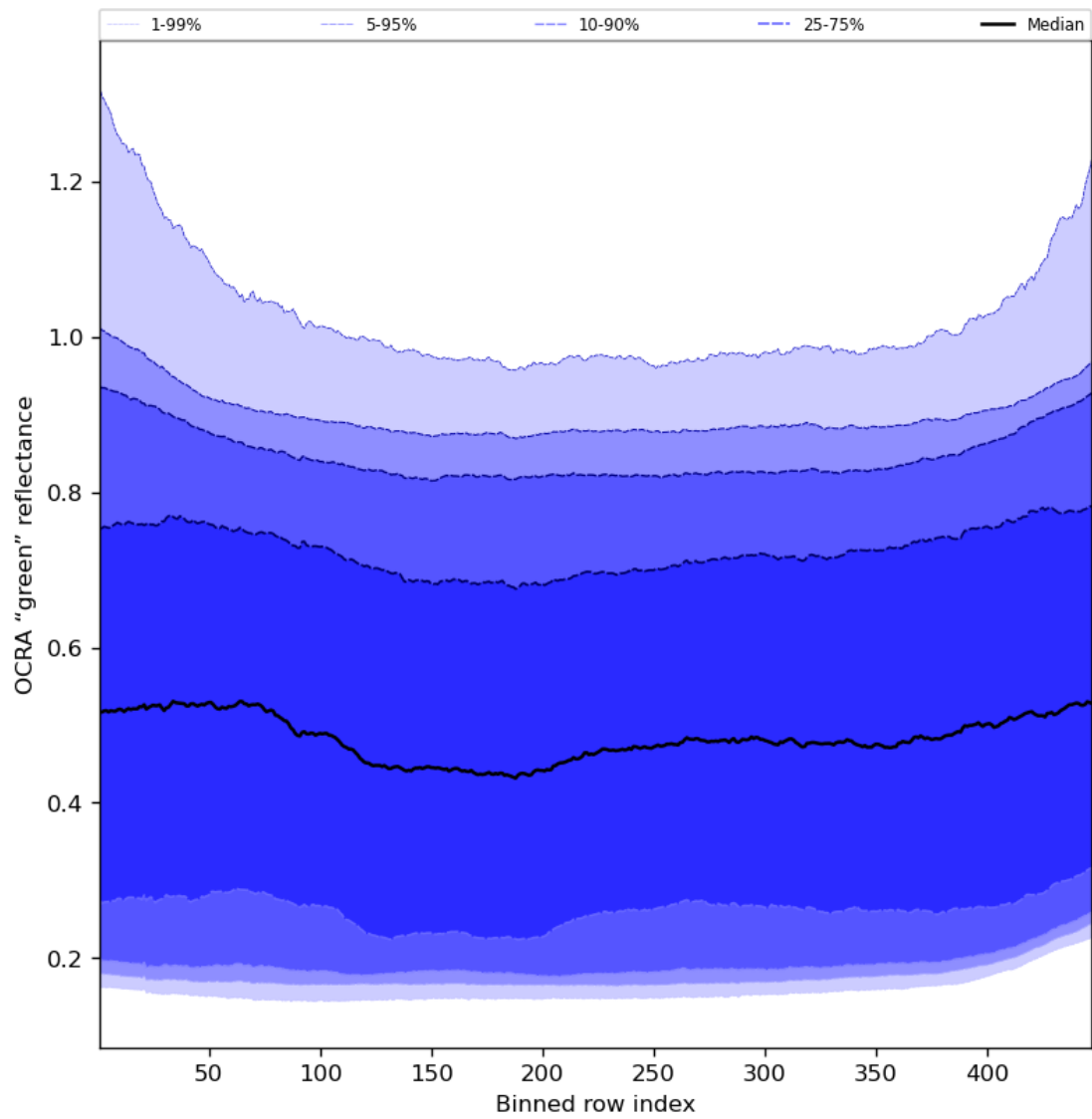
Figure 68: Along track statistics of “OCRA “green” reflectance” for 2024-04-21 to 2024-04-23
