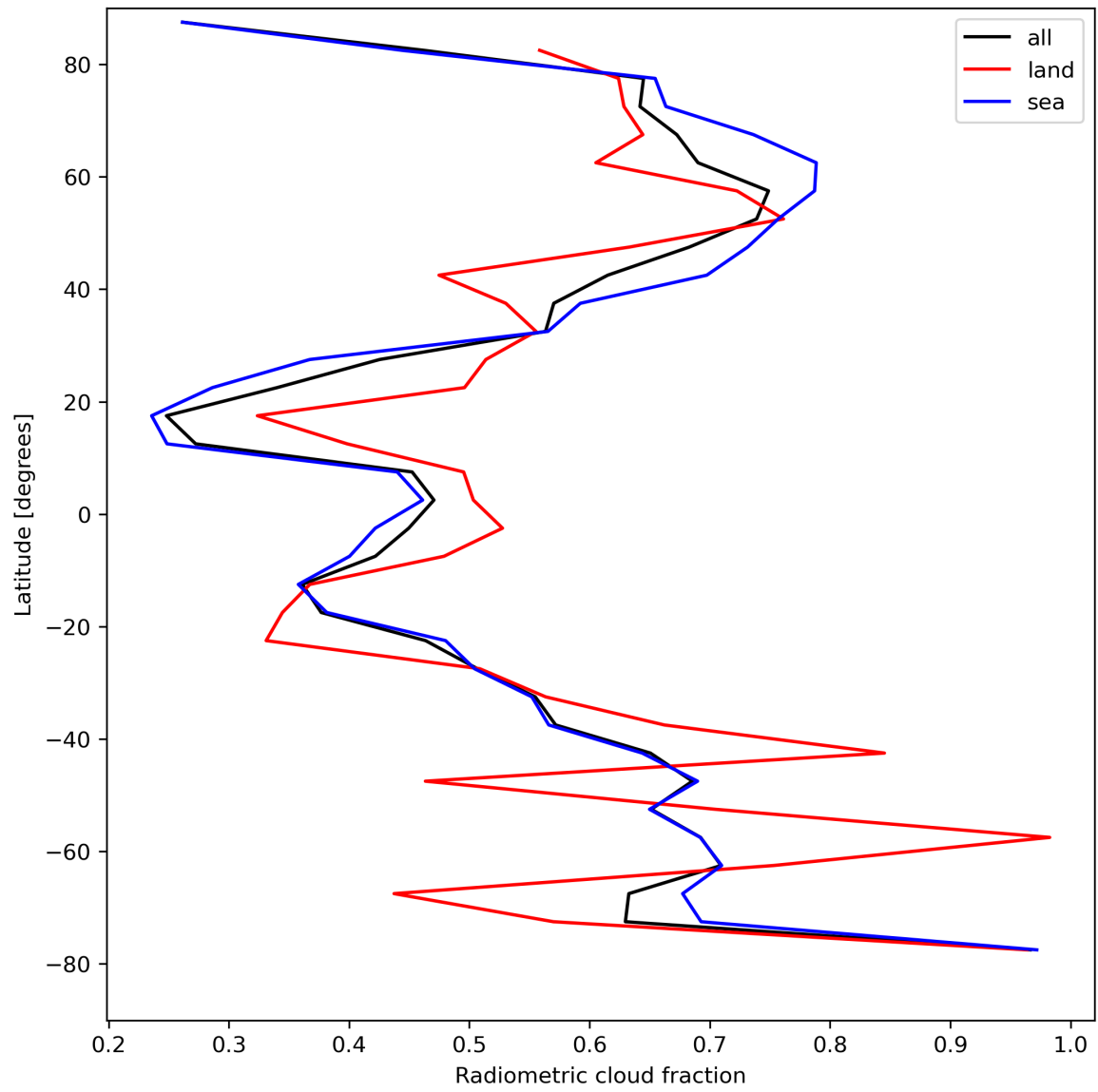
Figure 23: Zonal average of “Radiometric cloud fraction” for 2024-04-21 to 2024-04-23.
