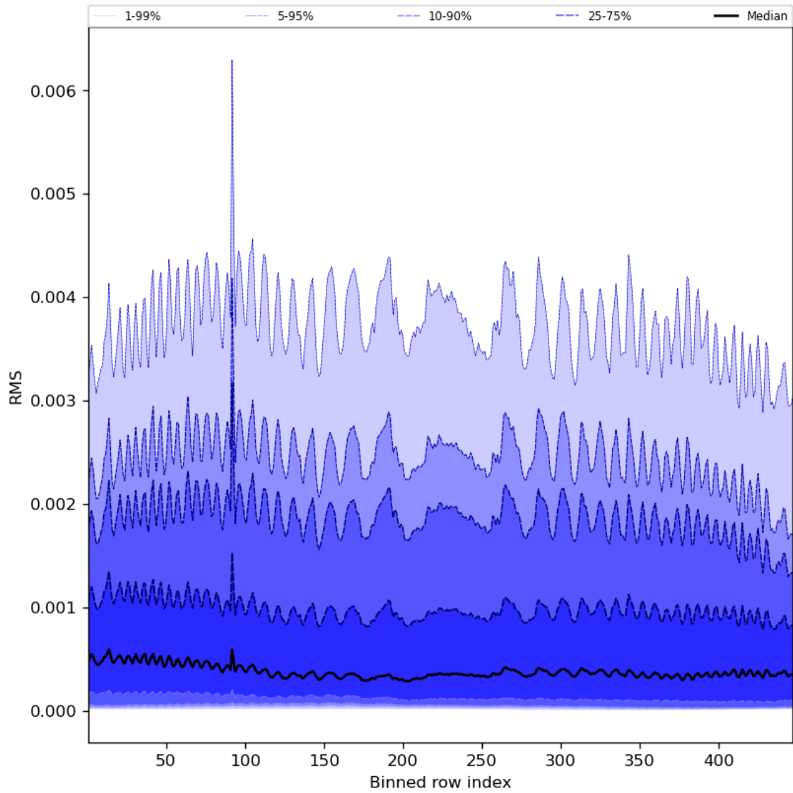
Figure 63: Along track statistics of “RMS” for 2024-04-21 to 2024-04-23
