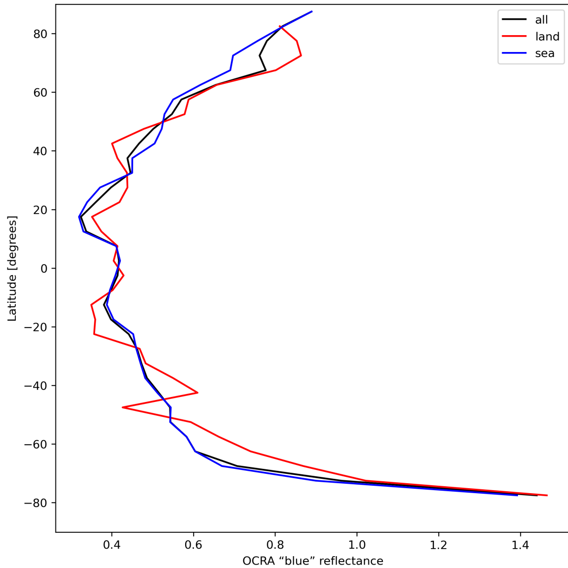
Figure 35: Zonal average of "OCRA "blue" reflectance" for 2024-04-21 to 2024-04-23.
