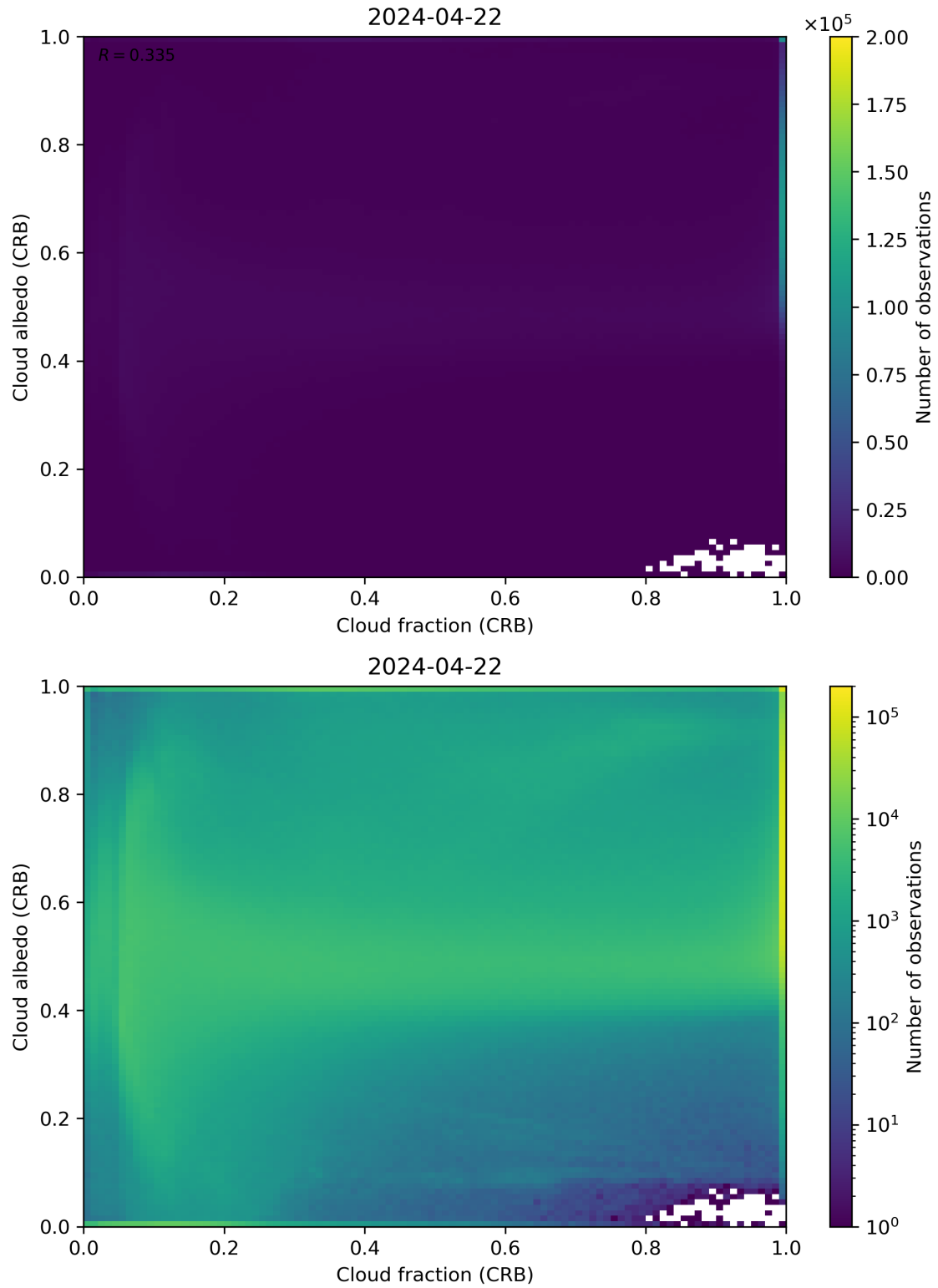
Figure 77: Scatter density plot of “Cloud fraction (CRB)” against “Cloud albedo (CRB)” for 2024-04-21 to 2024-04-23.
