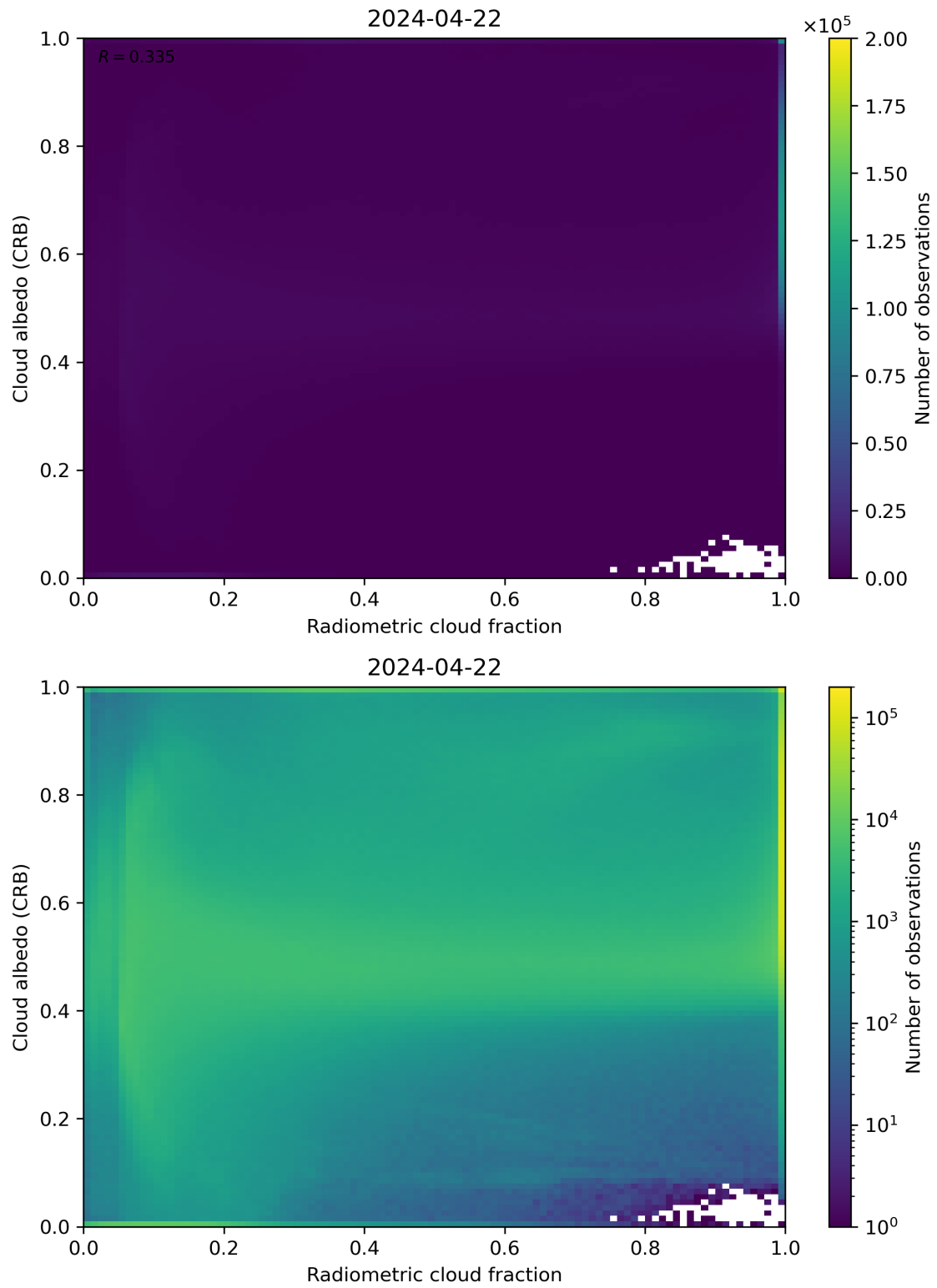
Figure 71: Scatter density plot of “Radiometric cloud fraction” against “Cloud albedo (CRB)” for 2024-04-21 to 2024-04-23.
