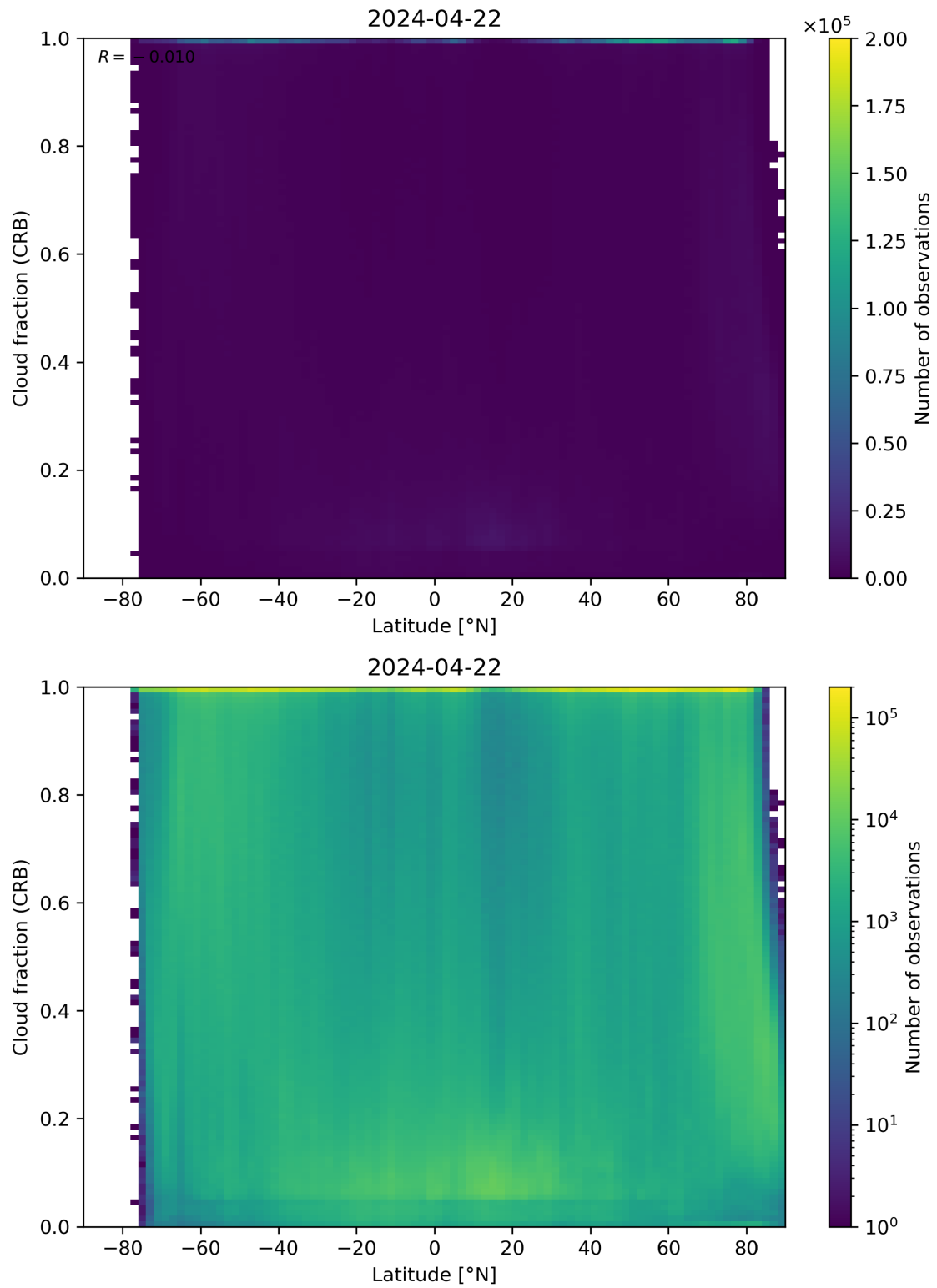
Figure 94: Scatter density plot of “Latitude” against “Cloud fraction (CRB)” for 2024-04-21 to 2024-04-23.
