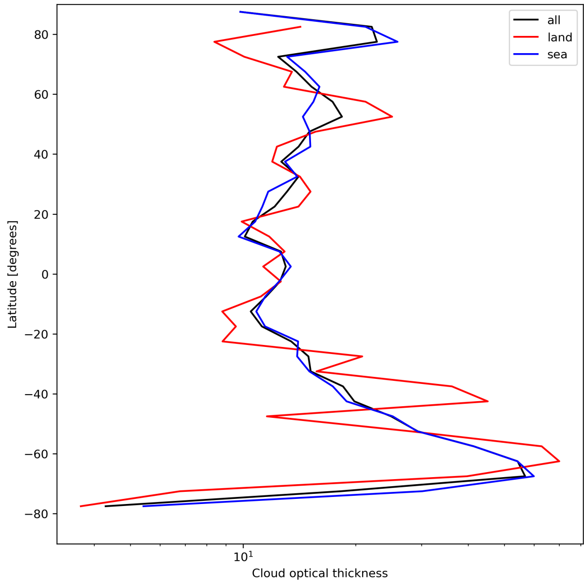
Figure 25: Zonal average of “Cloud optical thickness” for 2024-04-21 to 2024-04-23.
