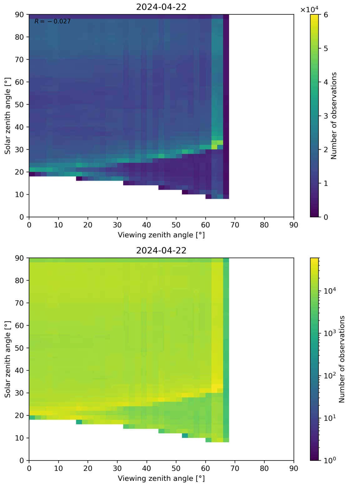
Figure 114: Scatter density plot of “Viewing zenith angle” against “Solar zenith angle” for 2024-04-21 to 2024-04-23.
