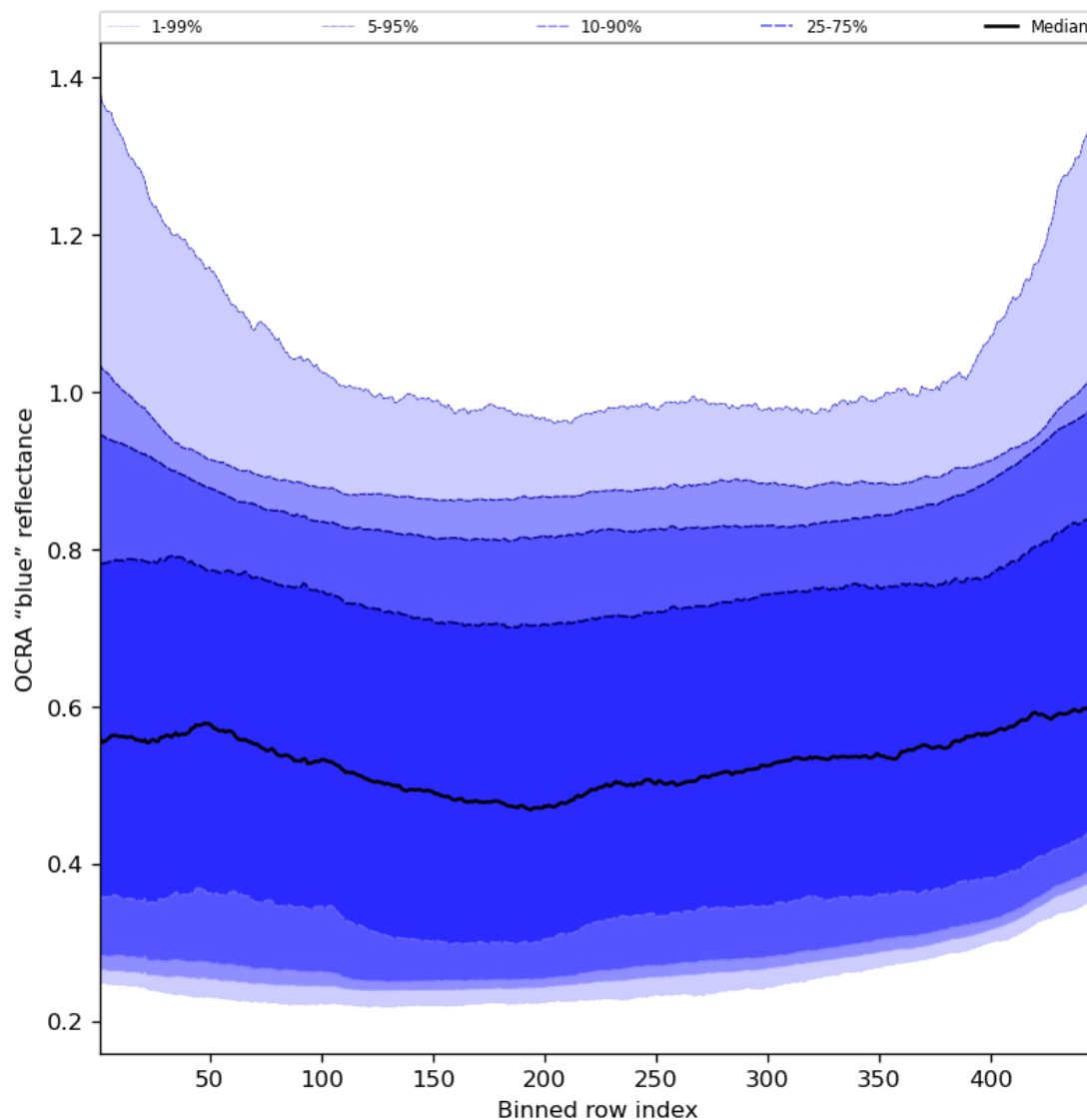
Figure 67: Along track statistics of “OCRA “blue” reflectance” for 2024-04-22 to 2024-04-24
