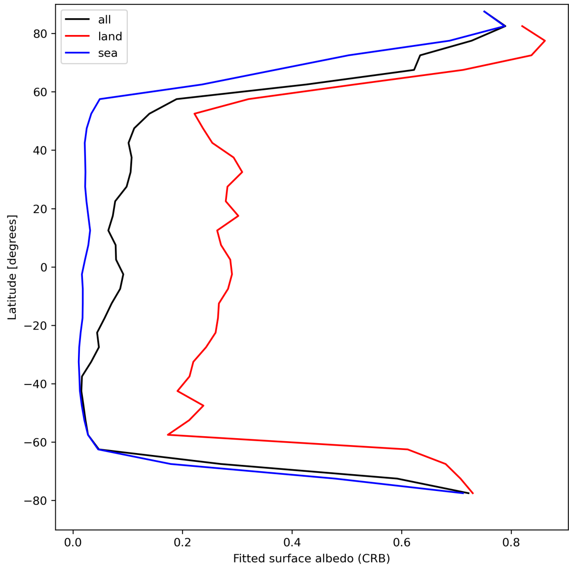
Figure 30: Zonal average of “Fitted surface albedo (CRB)” for 2024-04-22 to 2024-04-24.
