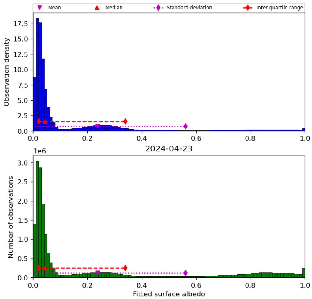
Figure 45: Histogram of “Fitted surface albedo” for 2024-04-22 to 2024-04-24
