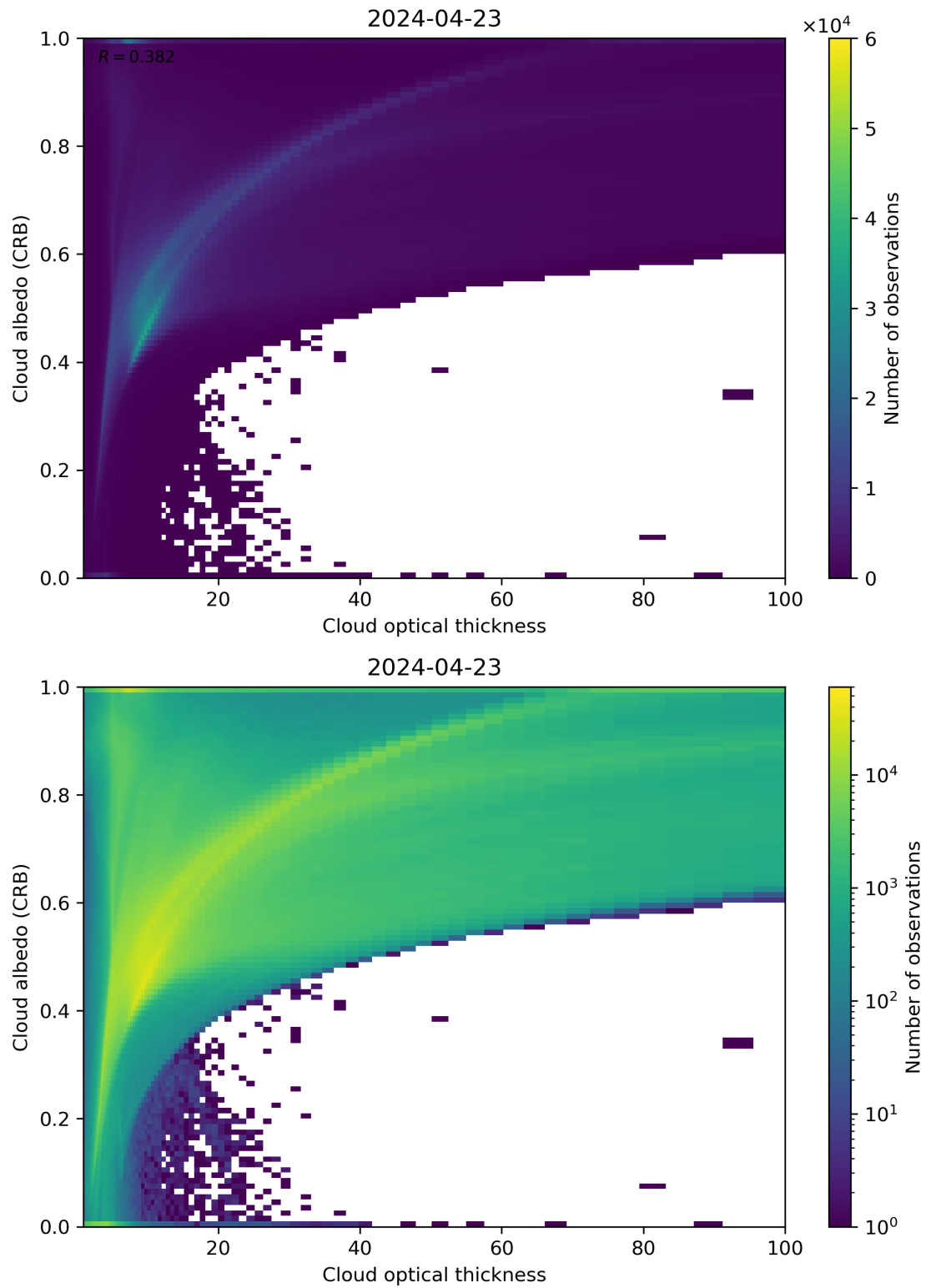
Figure 82: Scatter density plot of “Cloud optical thickness” against “Cloud albedo (CRB)” for 2024-04-22 to 2024-04-24.
