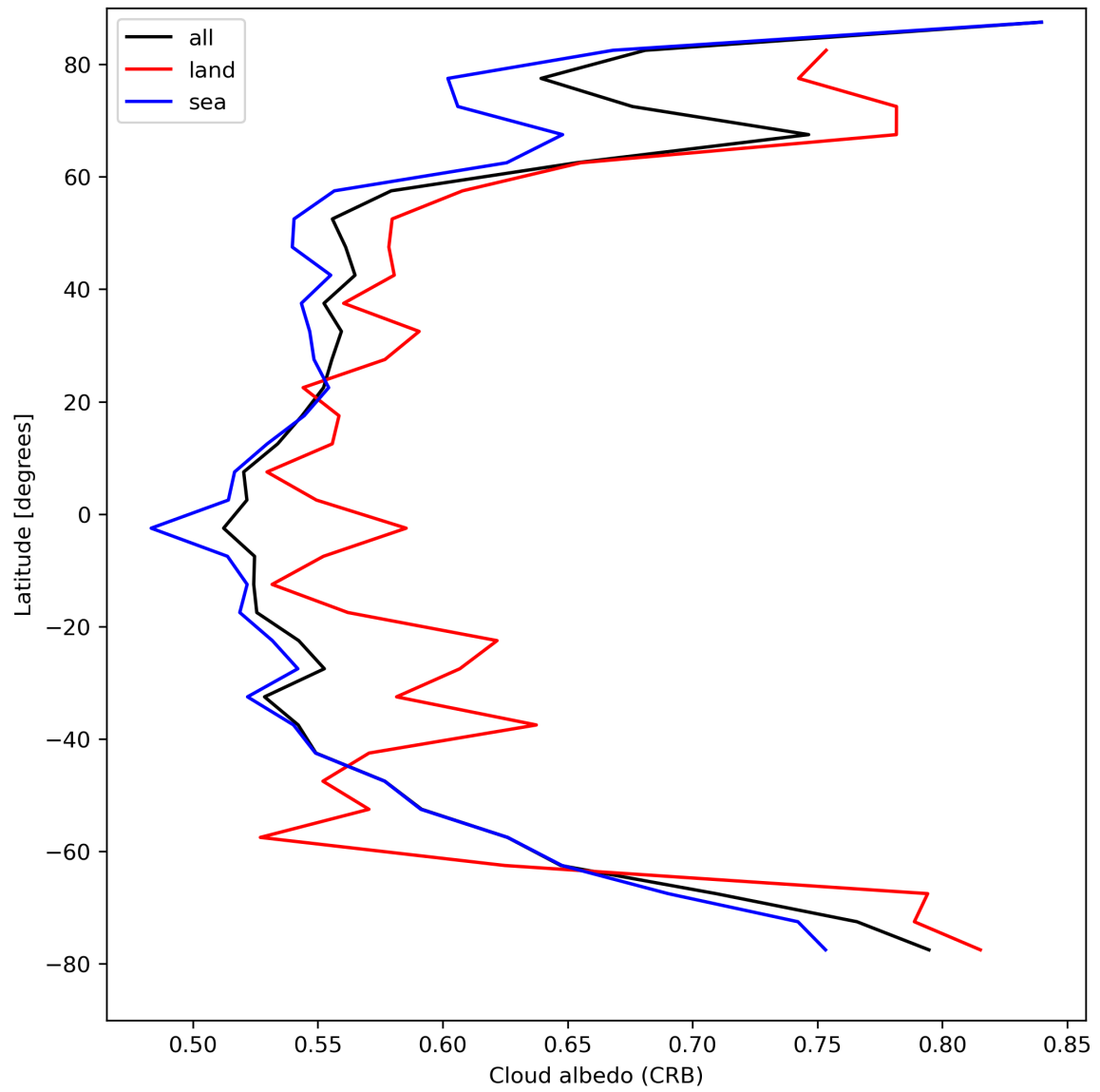
Figure 28: Zonal average of “Cloud albedo (CRB)” for 2024-04-22 to 2024-04-24.
