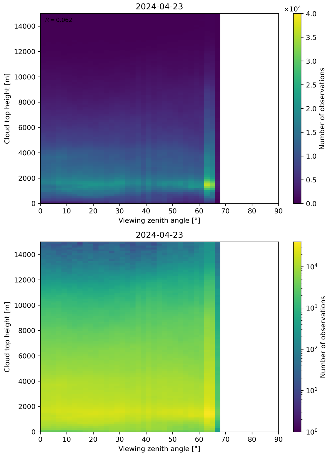
Figure 112: Scatter density plot of “Viewing zenith angle” against “Cloud top height” for 2024-04-22 to 2024-04-24.
