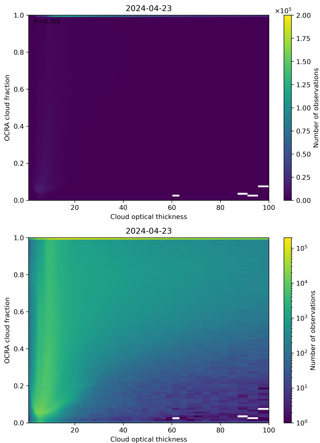
Figure 83: Scatter density plot of “Cloud optical thickness” against “OCRA cloud fraction” for 2024-04-22 to 2024-04-24.
