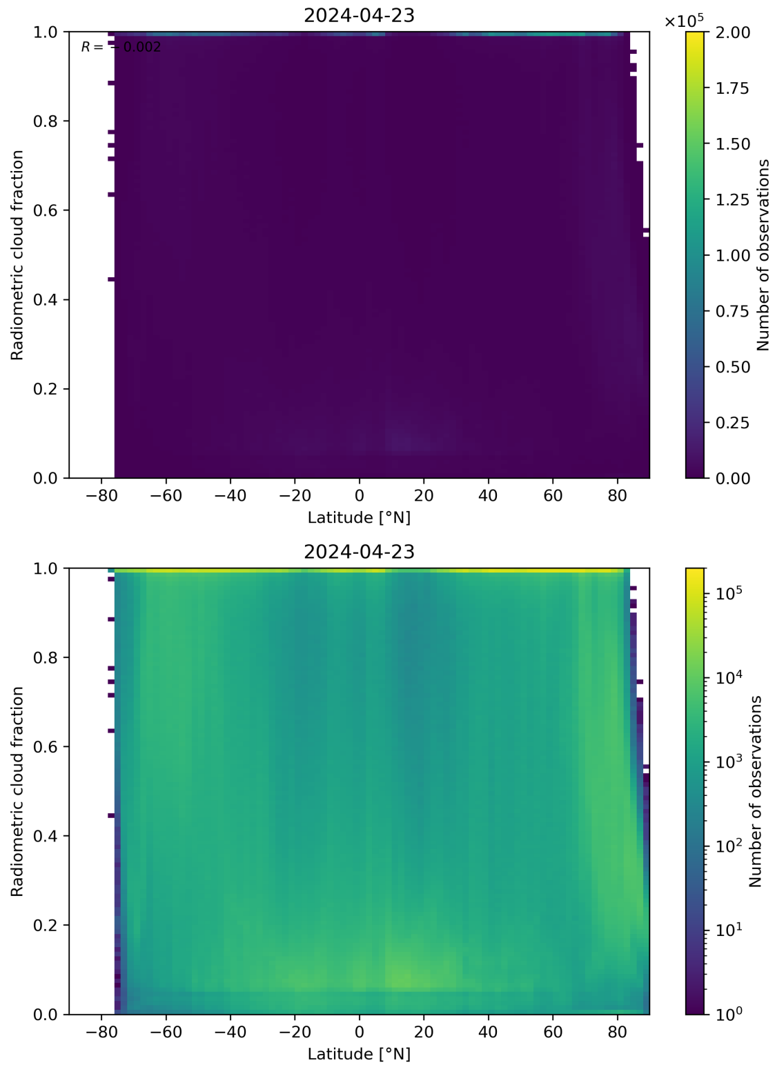
Figure 92: Scatter density plot of “Latitude” against “Radiometric cloud fraction” for 2024-04-22 to 2024-04-24.
