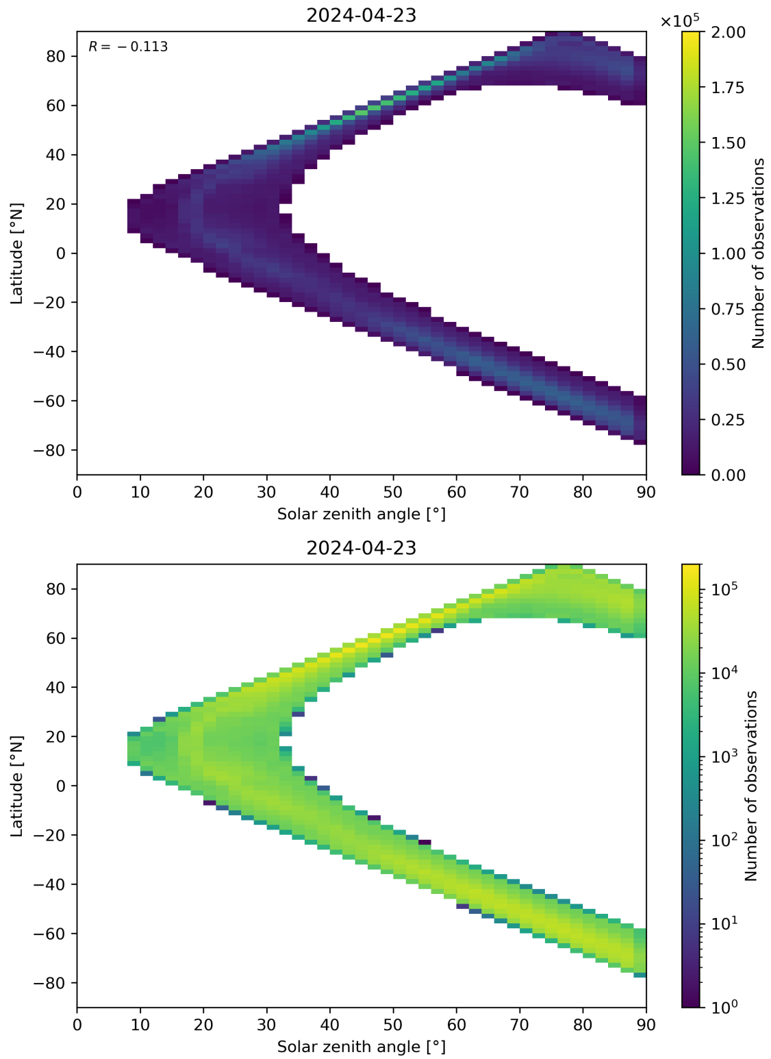
Figure 105: Scatter density plot of “Solar zenith angle” against “Latitude” for 2024-04-22 to 2024-04-24.
