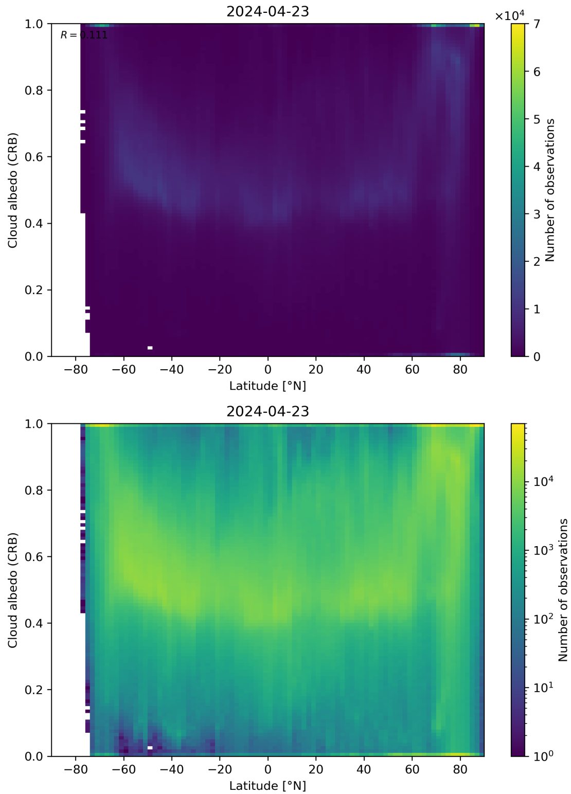
Figure 91: Scatter density plot of “Latitude” against “Cloud albedo (CRB)” for 2024-04-22 to 2024-04-24.
