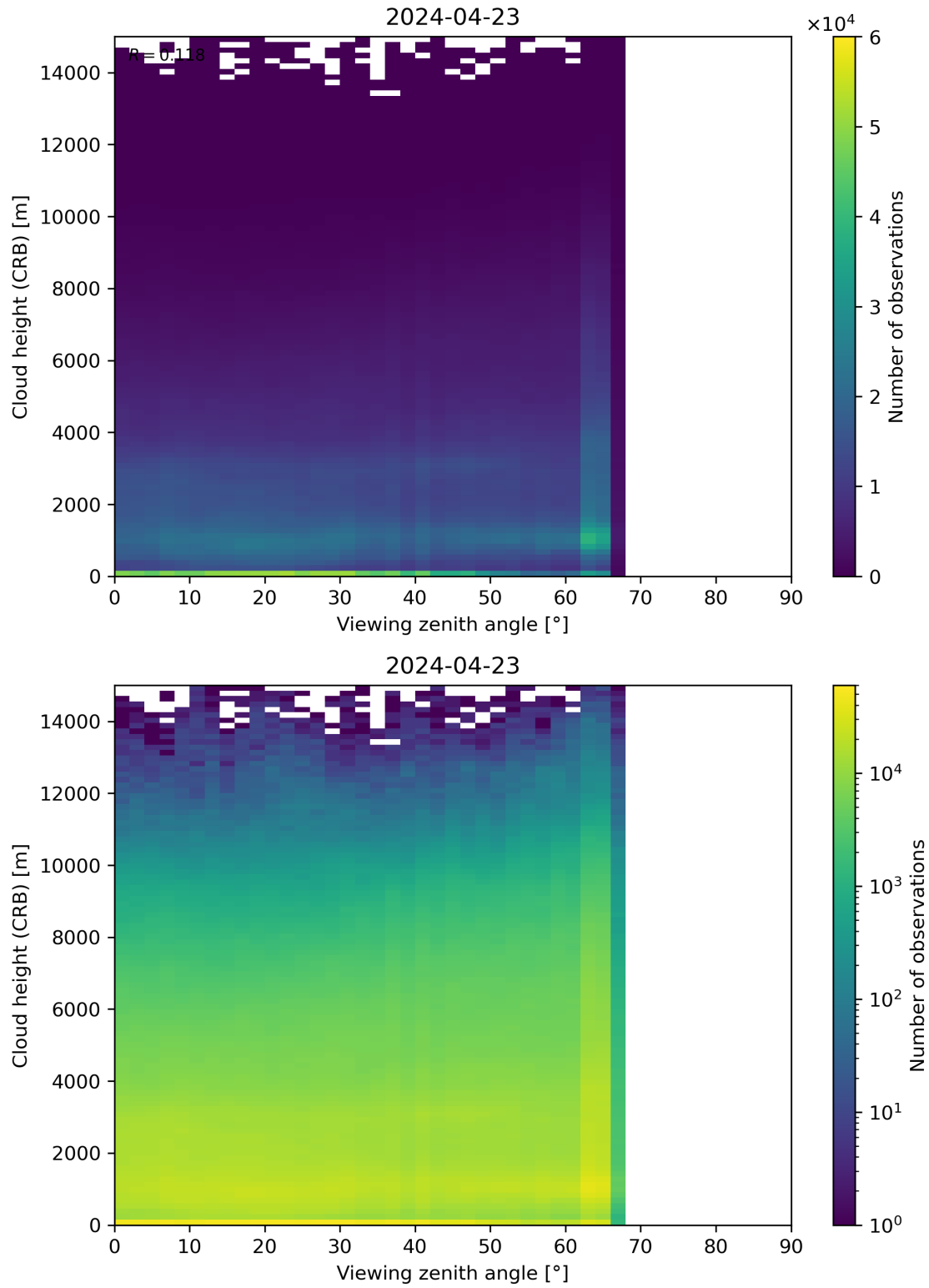
Figure 110: Scatter density plot of “Viewing zenith angle” against “Cloud height (CRB)” for 2024-04-22 to 2024-04-24.
