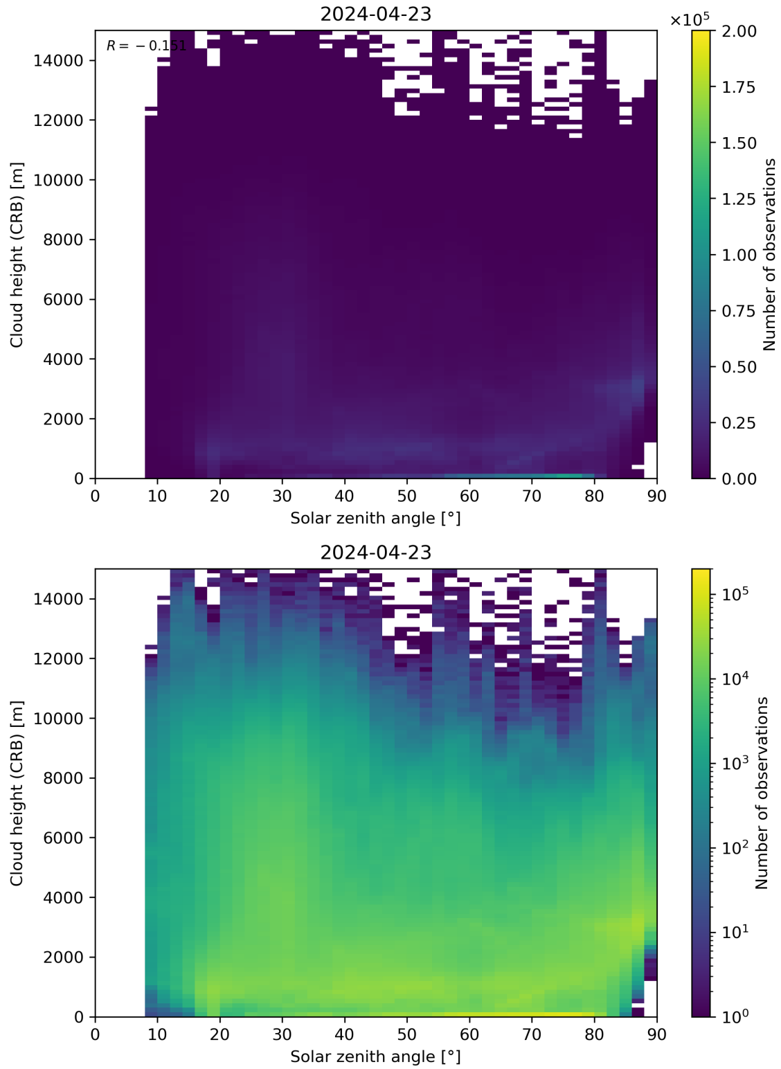
Figure 102: Scatter density plot of “Solar zenith angle” against “Cloud height (CRB)” for 2024-04-22 to 2024-04-24.
