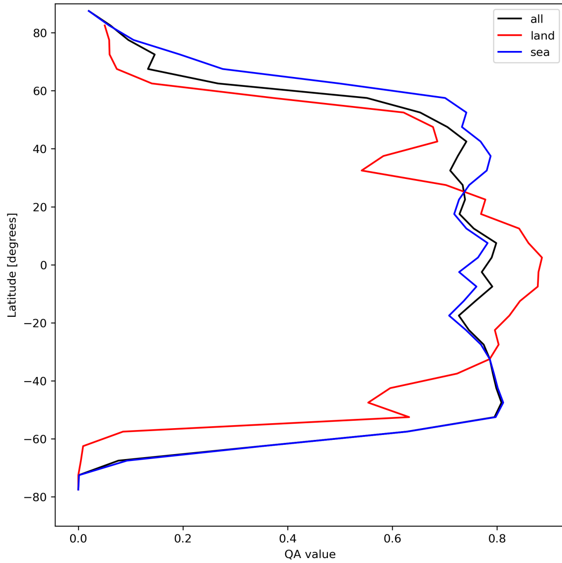
Figure 22: Zonal average of “QA value” for 2024-04-22 to 2024-04-24.
