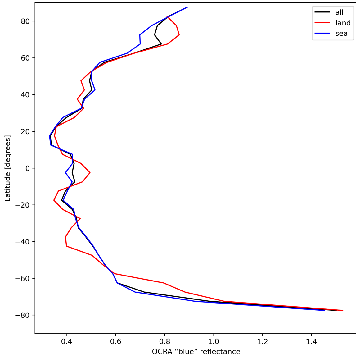
Figure 35: Zonal average of “OCRA “blue” reflectance” for 2024-04-22 to 2024-04-24.
