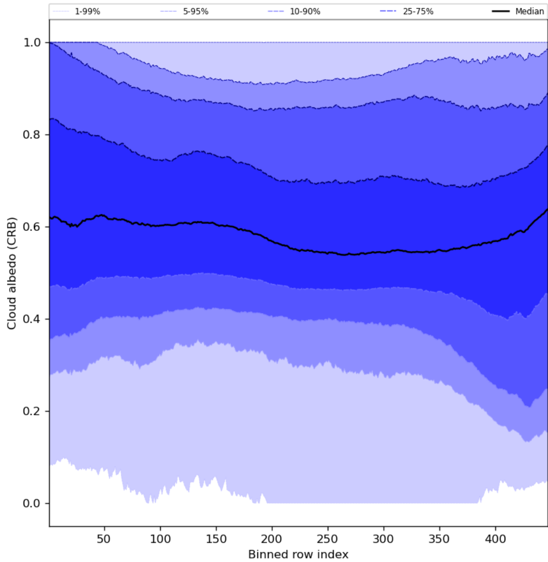
Figure 60: Along track statistics of “Cloud albedo (CRB)” for 2024-04-22 to 2024-04-24
