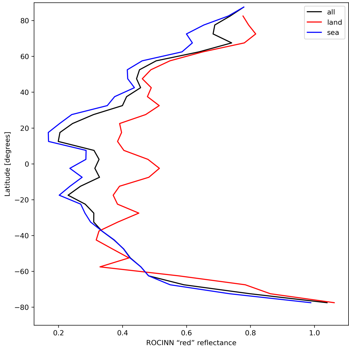
Figure 37: Zonal average of “ROCINN “red” reflectance” for 2024-04-22 to 2024-04-24.
