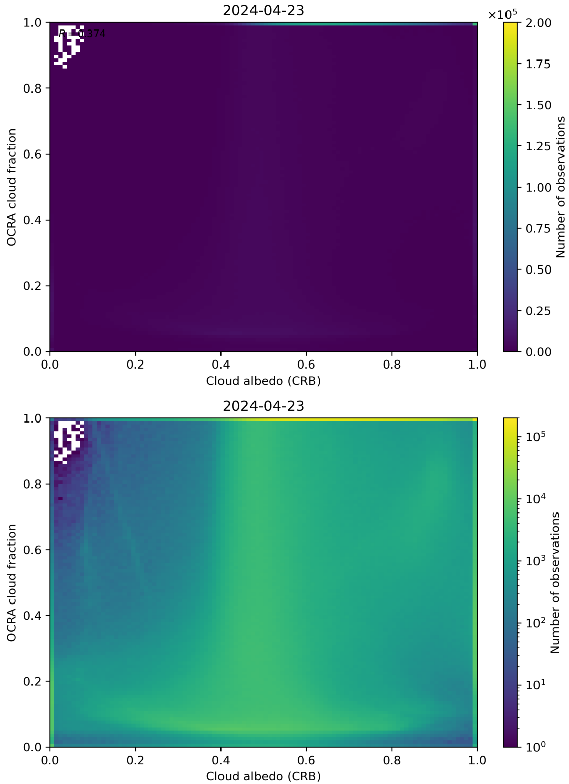
Figure 70: Scatter density plot of “Cloud albedo (CRB)” against “OCRA cloud fraction” for 2024-04-22 to 2024-04-24.
