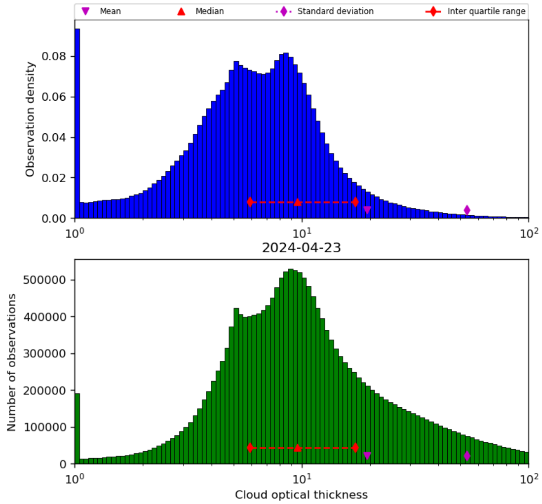
Figure 41: Histogram of “Cloud optical thickness” for 2024-04-22 to 2024-04-24
