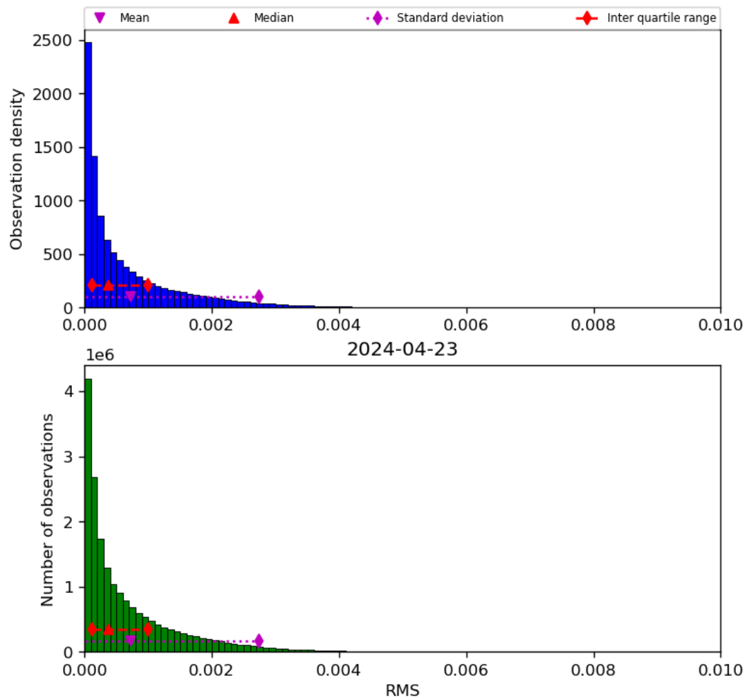
Figure 47: Histogram of “RMS” for 2024-04-22 to 2024-04-24
