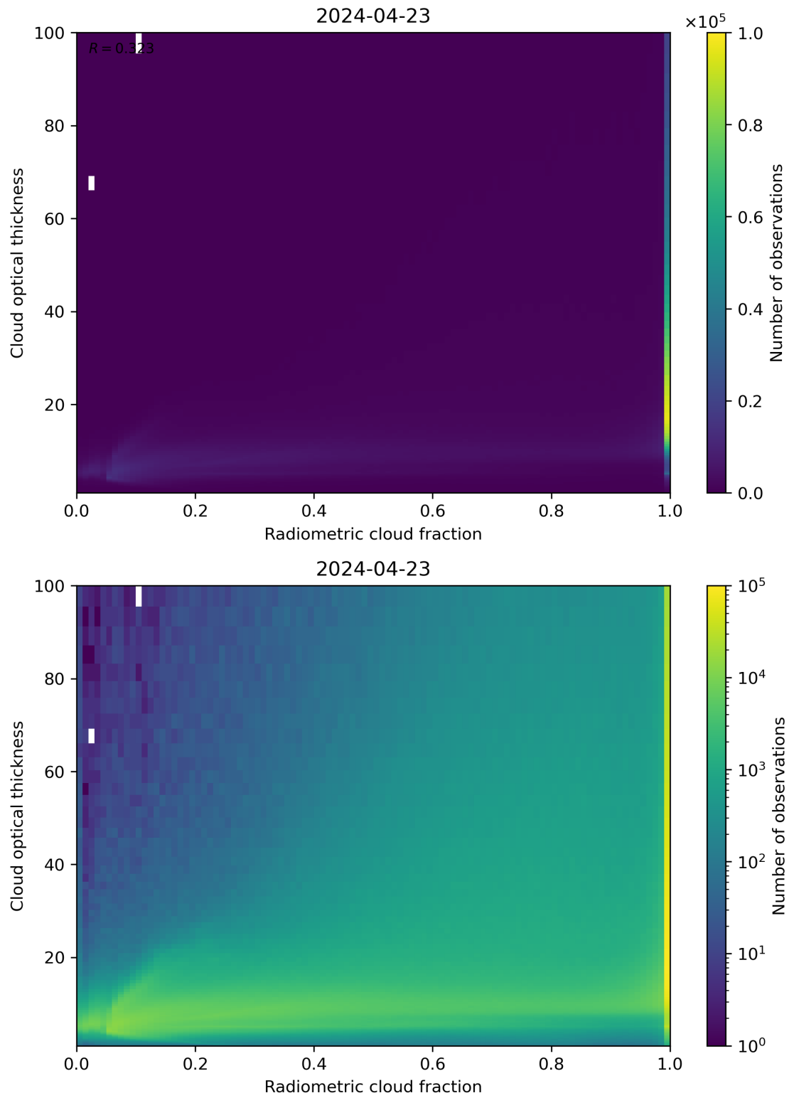
Figure 75: Scatter density plot of “Radiometric cloud fraction” against “Cloud optical thickness” for 2024-04-22 to 2024-04-24.
