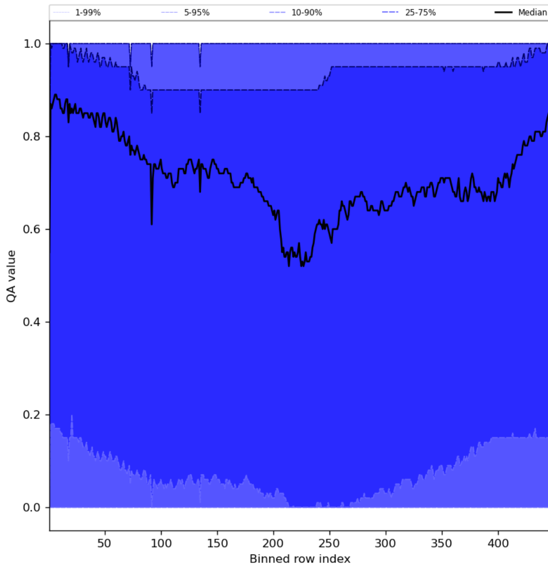
Figure 54: Along track statistics of “QA value” for 2024-04-22 to 2024-04-24
