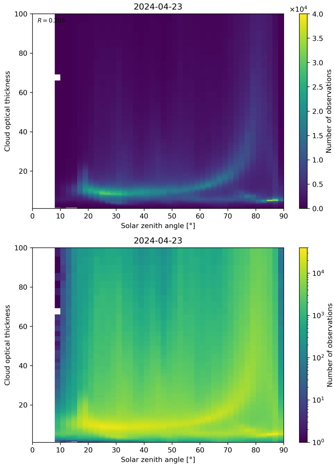
Figure 103: Scatter density plot of “Solar zenith angle” against “Cloud optical thickness” for 2024-04-22 to 2024-04-24.
