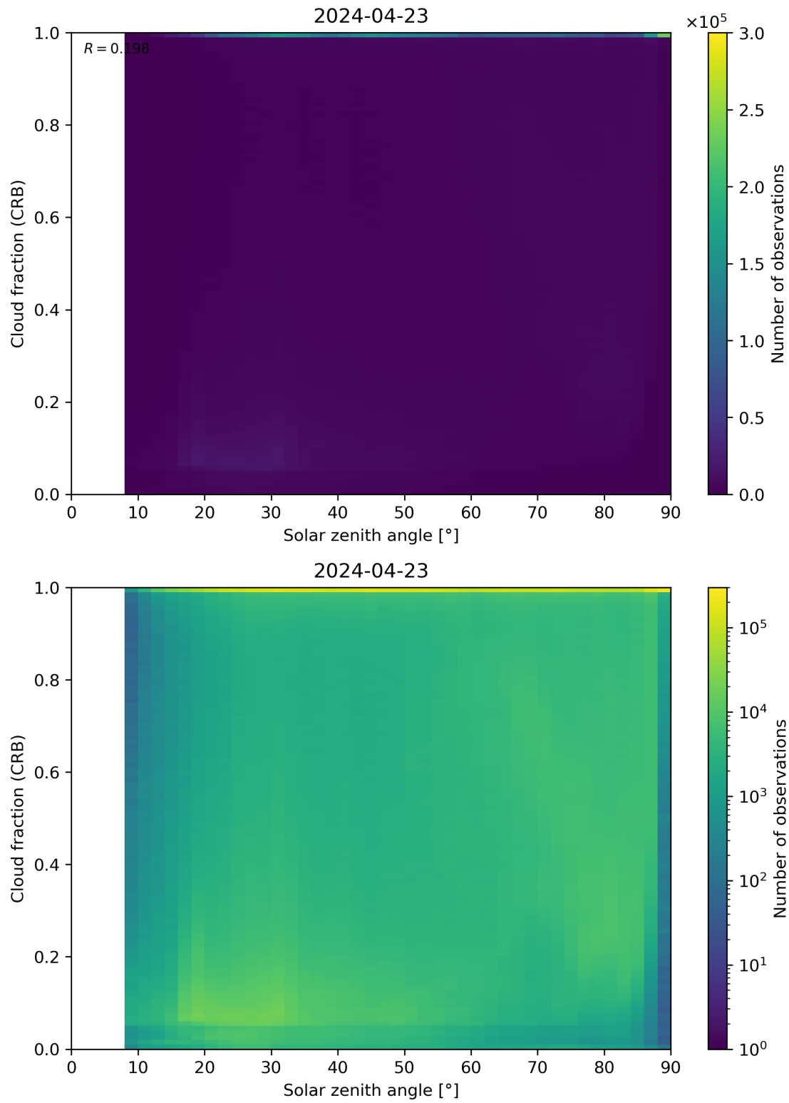
Figure 101: Scatter density plot of “Solar zenith angle” against “Cloud fraction (CRB)” for 2024-04-22 to 2024-04-24.
