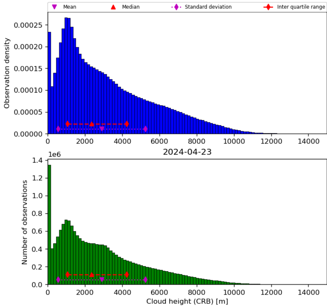
Figure 43: Histogram of “Cloud height (CRB)” for 2024-04-22 to 2024-04-24
