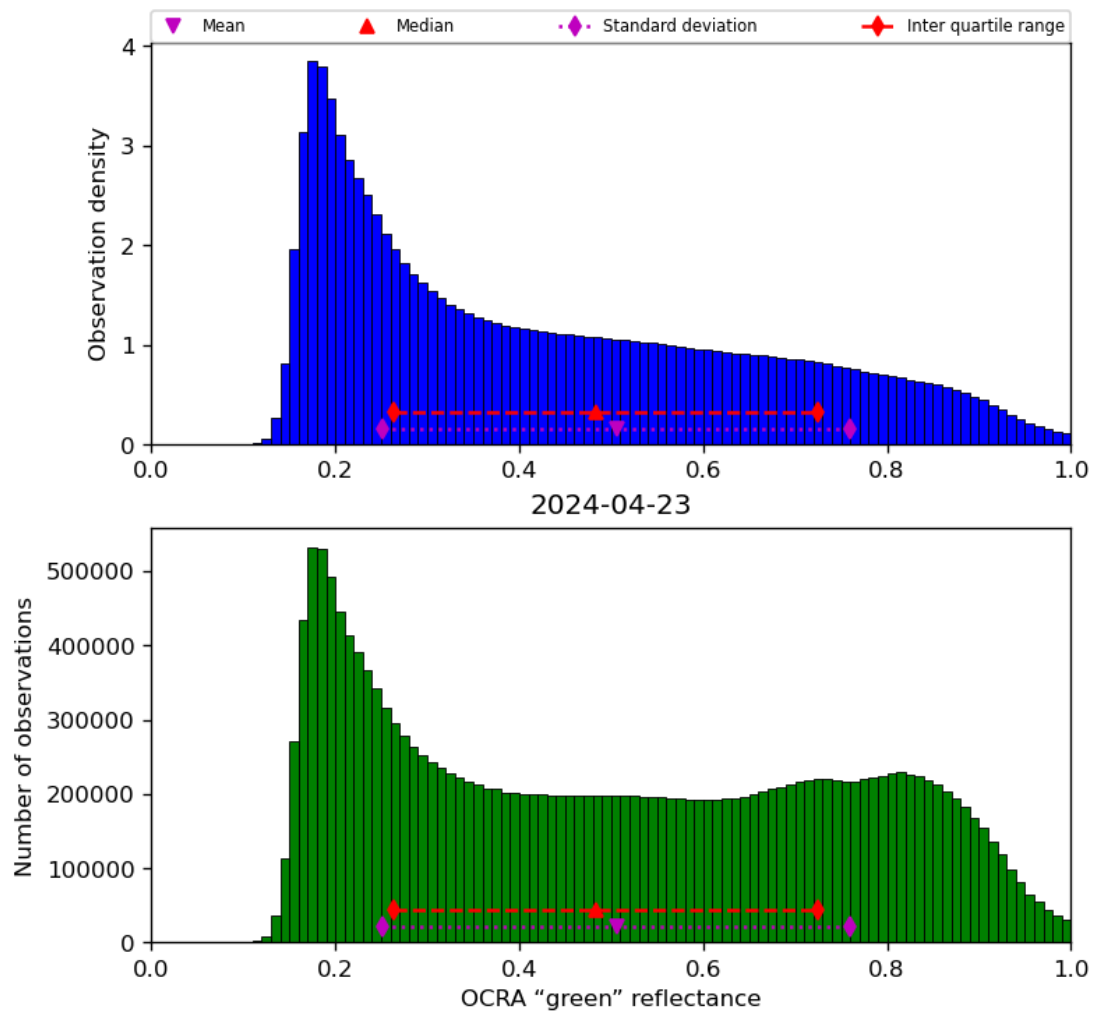
Figure 52: Histogram of “OCRA “green” reflectance” for 2024-04-22 to 2024-04-24
