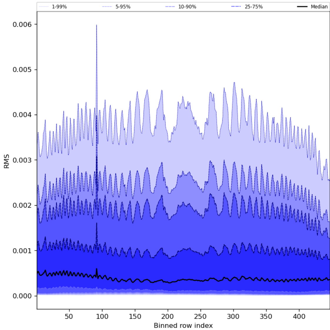
Figure 63: Along track statistics of “RMS” for 2024-04-22 to 2024-04-24
