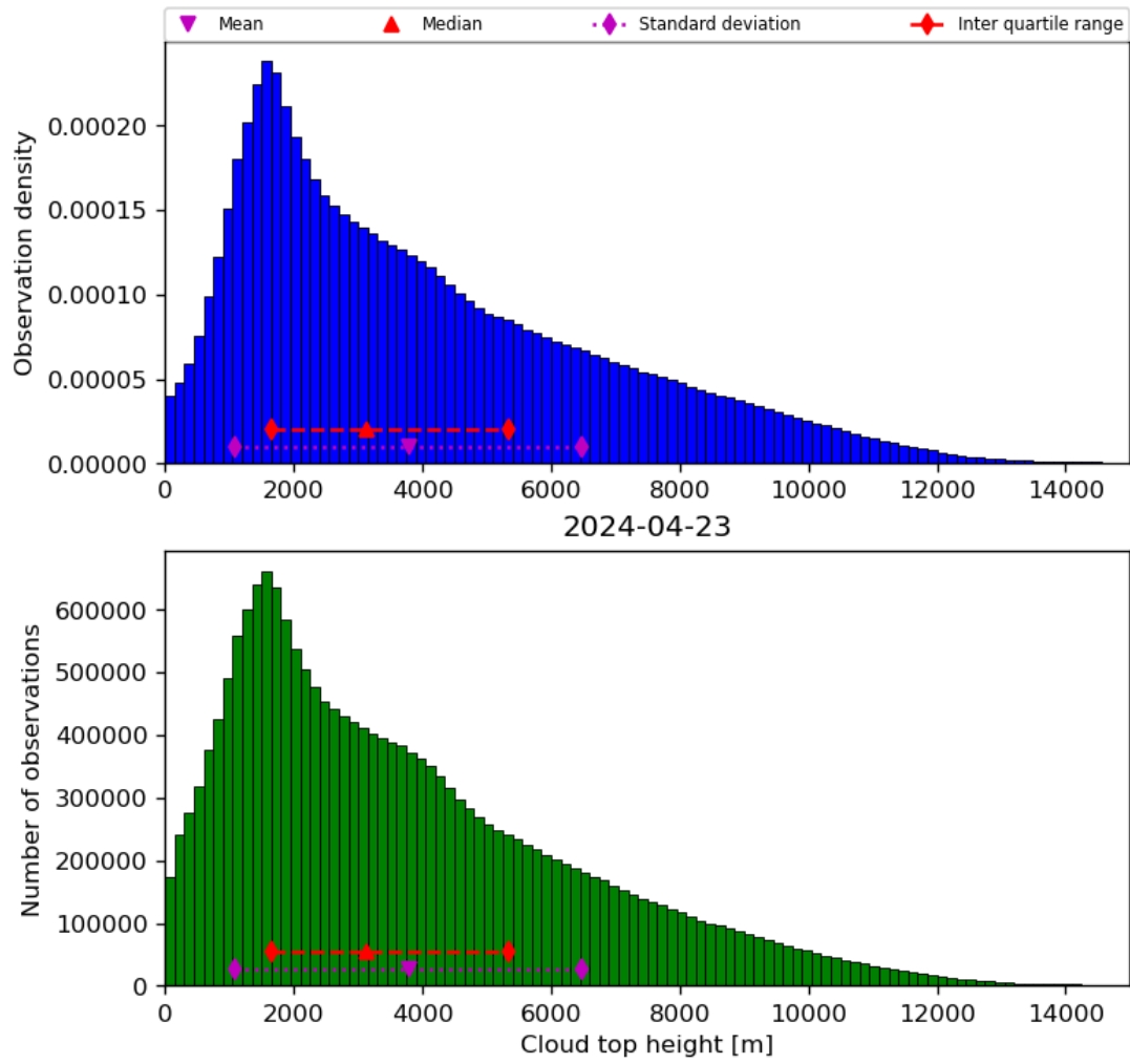
Figure 40: Histogram of “Cloud top height” for 2024-04-22 to 2024-04-24
