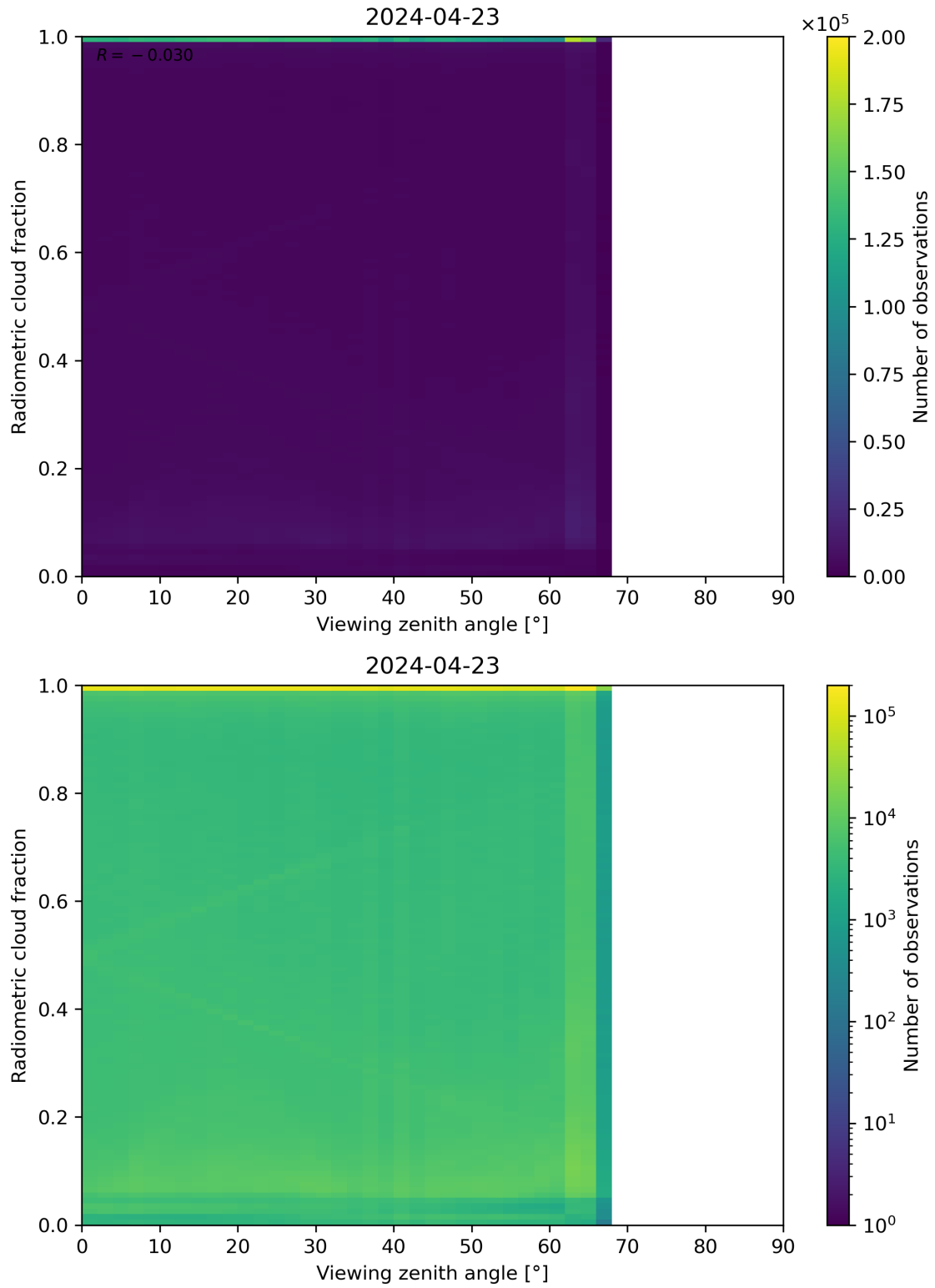
Figure 107: Scatter density plot of “Viewing zenith angle” against “Radiometric cloud fraction” for 2024-04-22 to 2024-04-24.
