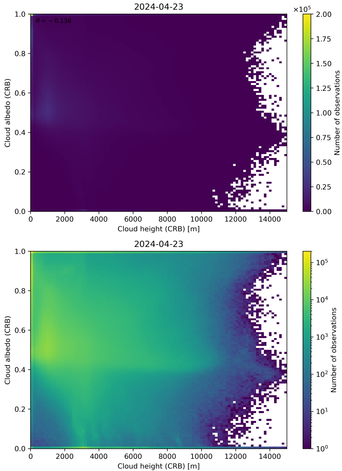
Figure 80: Scatter density plot of “Cloud height (CRB)” against “Cloud albedo (CRB)” for 2024-04-22 to 2024-04-24.
