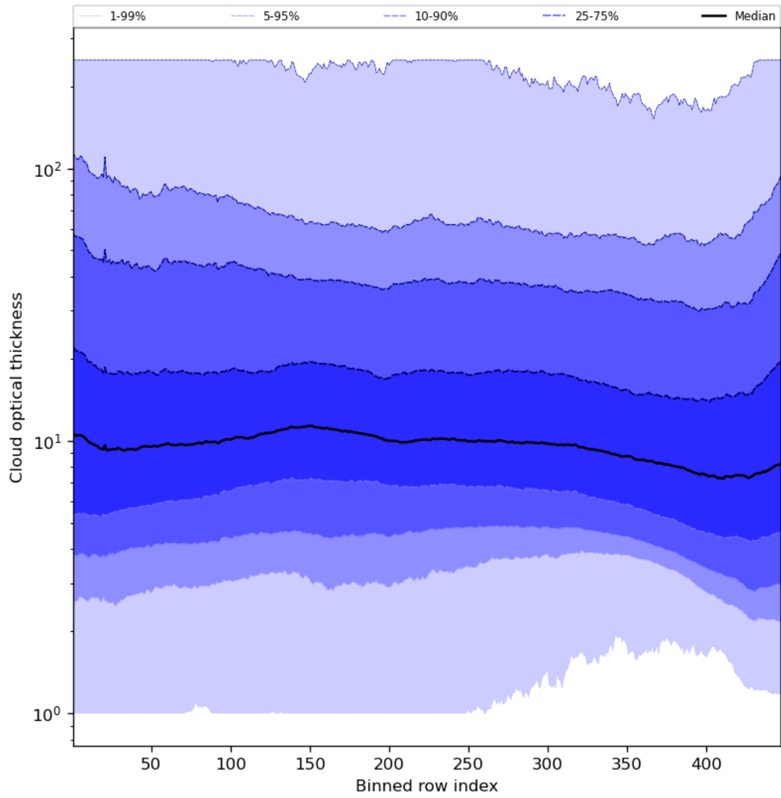
Figure 57: Along track statistics of “Cloud optical thickness” for 2024-04-22 to 2024-04-24
