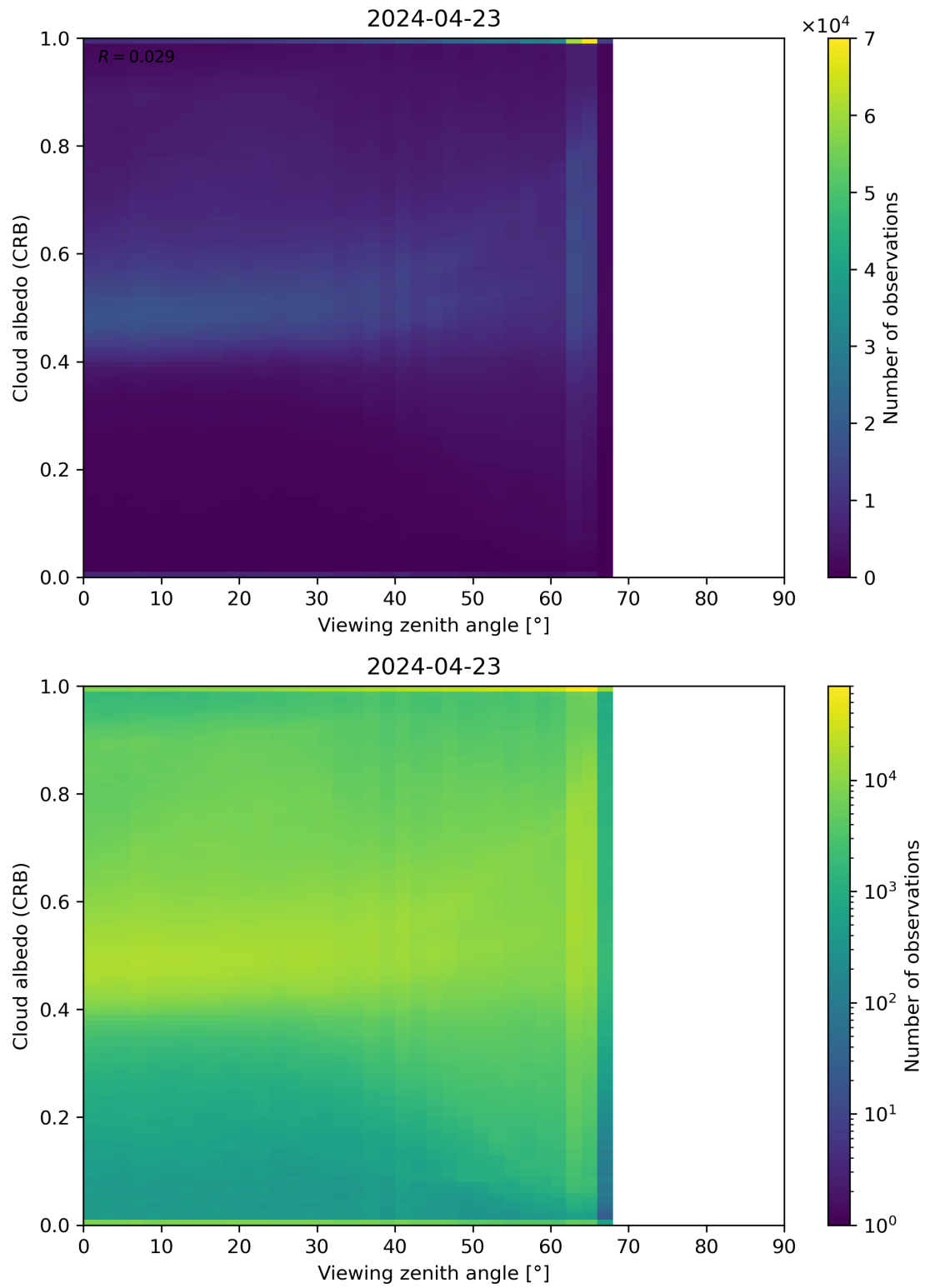
Figure 106: Scatter density plot of “Viewing zenith angle” against “Cloud albedo (CRB)” for 2024-04-22 to 2024-04-24.
