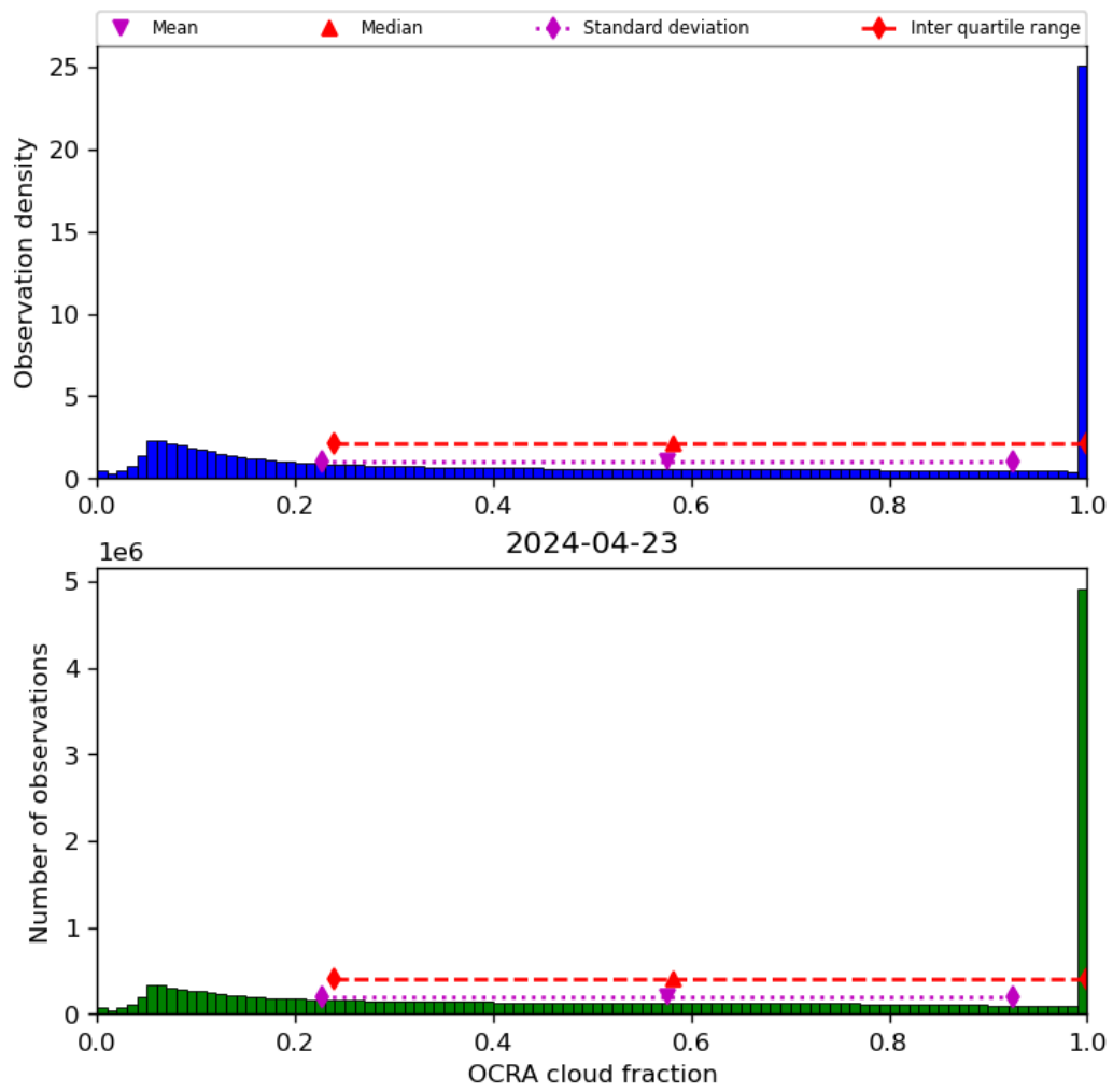
Figure 50: Histogram of “OCRA cloud fraction” for 2024-04-22 to 2024-04-24
