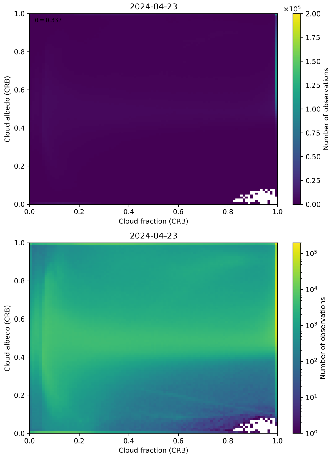
Figure 77: Scatter density plot of “Cloud fraction (CRB)” against “Cloud albedo (CRB)” for 2024-04-22 to 2024-04-24.
