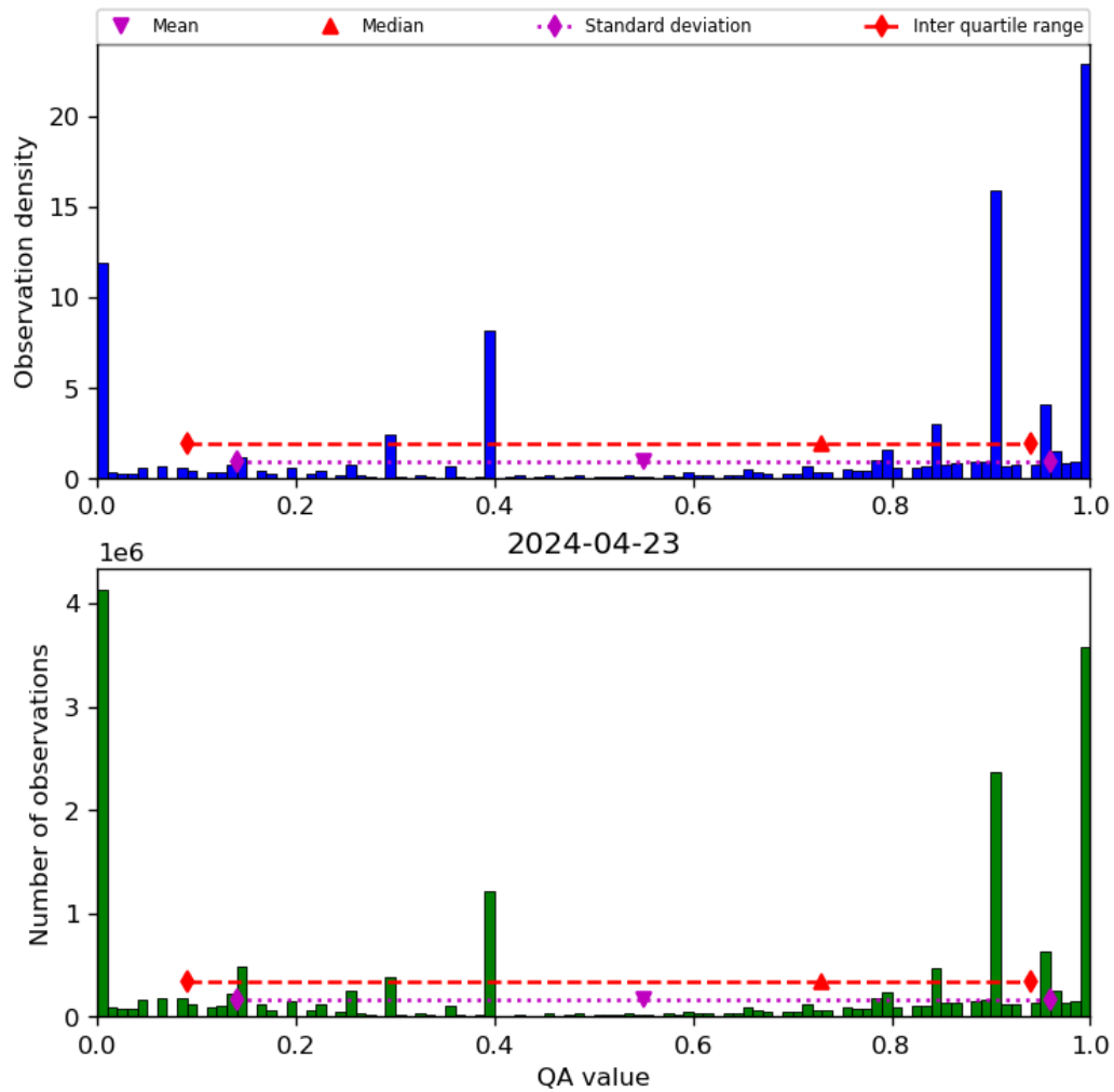
Figure 38: Histogram of “QA value” for 2024-04-22 to 2024-04-24
