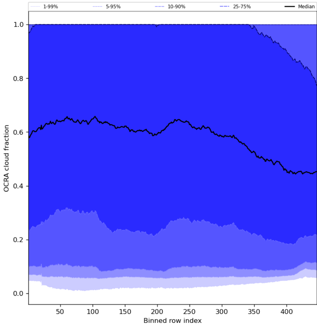
Figure 66: Along track statistics of “OCRA cloud fraction” for 2024-04-22 to 2024-04-24
