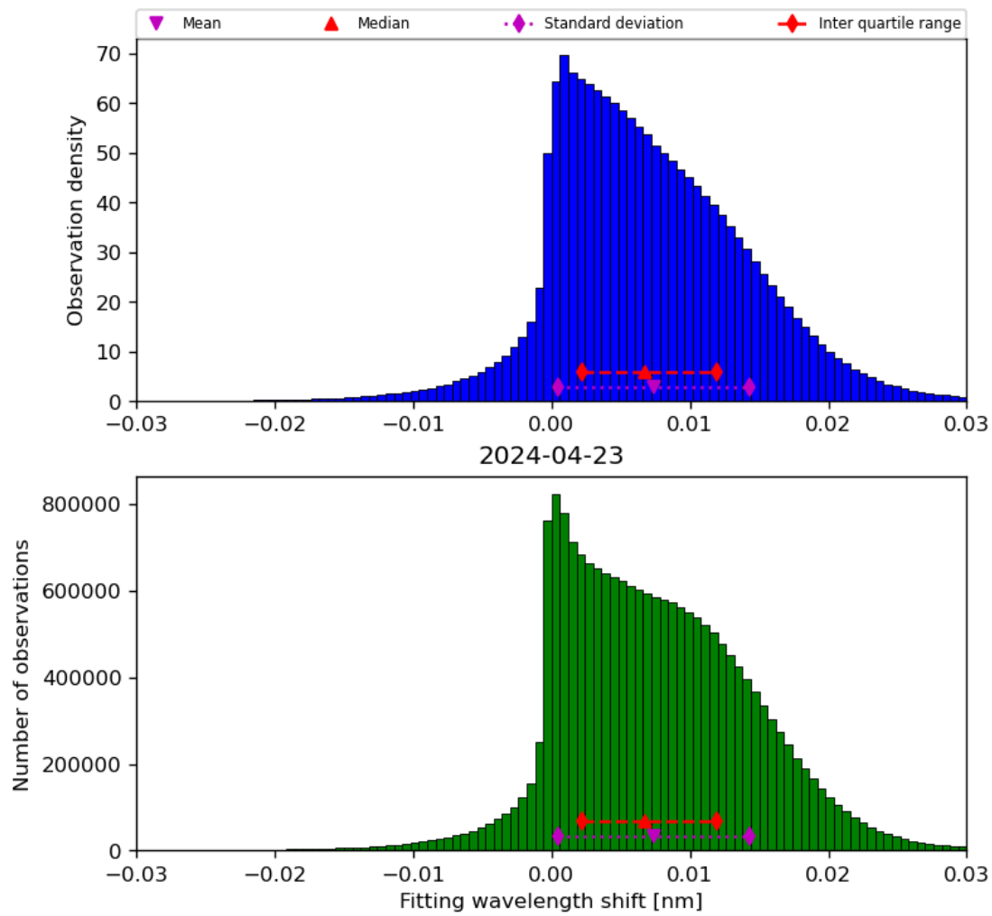
Figure 49: Histogram of “Fitting wavelength shift” for 2024-04-22 to 2024-04-24
