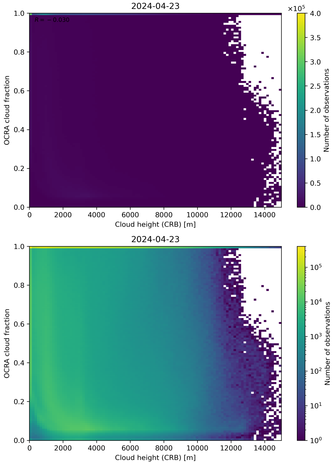
Figure 81: Scatter density plot of “Cloud height (CRB)” against “OCRA cloud fraction” for 2024-04-22 to 2024-04-24.
