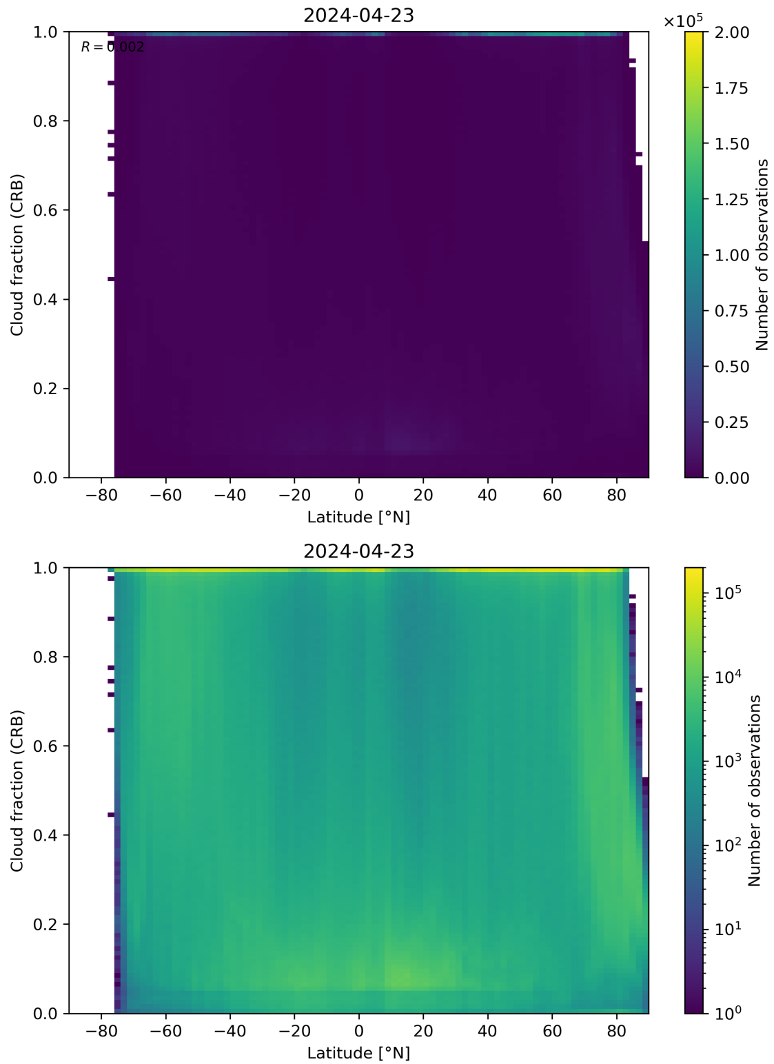
Figure 94: Scatter density plot of “Latitude” against “Cloud fraction (CRB)” for 2024-04-22 to 2024-04-24.
