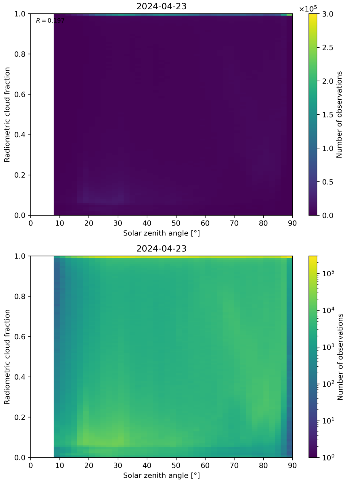
Figure 99: Scatter density plot of “Solar zenith angle” against “Radiometric cloud fraction” for 2024-04-22 to 2024-04-24.
