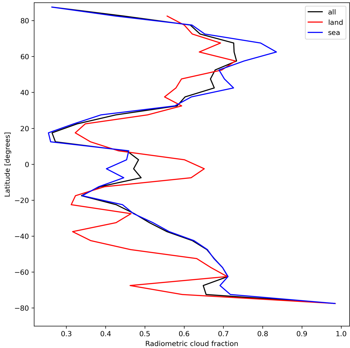
Figure 23: Zonal average of “Radiometric cloud fraction” for 2024-04-22 to 2024-04-24.
