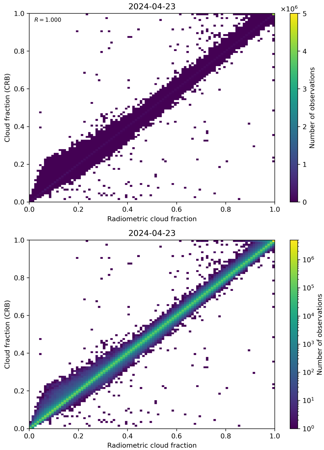
Figure 73: Scatter density plot of “Radiometric cloud fraction” against “Cloud fraction (CRB)” for 2024-04-22 to 2024-04-24.
