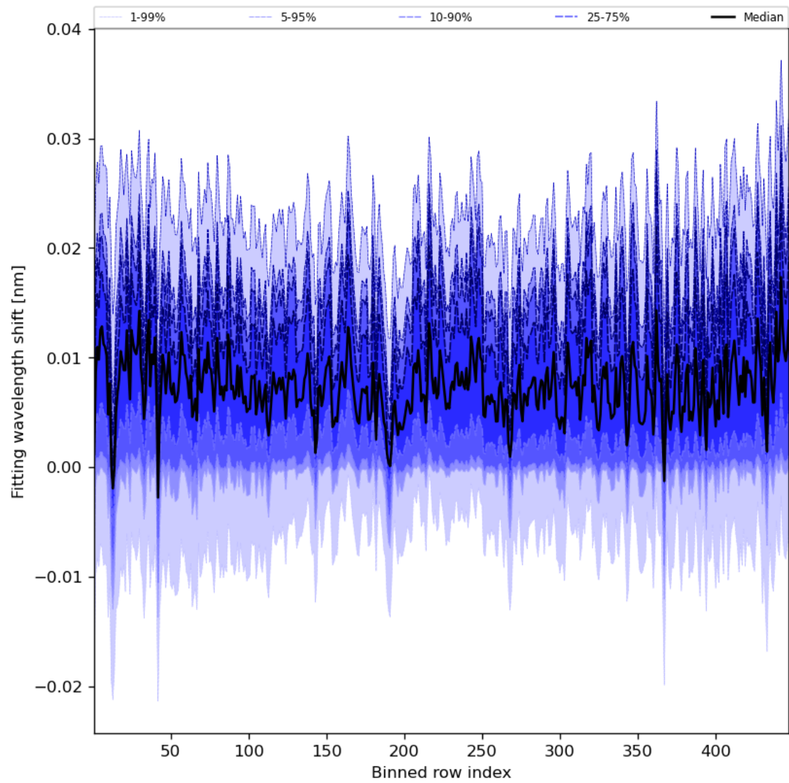
Figure 65: Along track statistics of “Fitting wavelength shift” for 2024-04-22 to 2024-04-24
