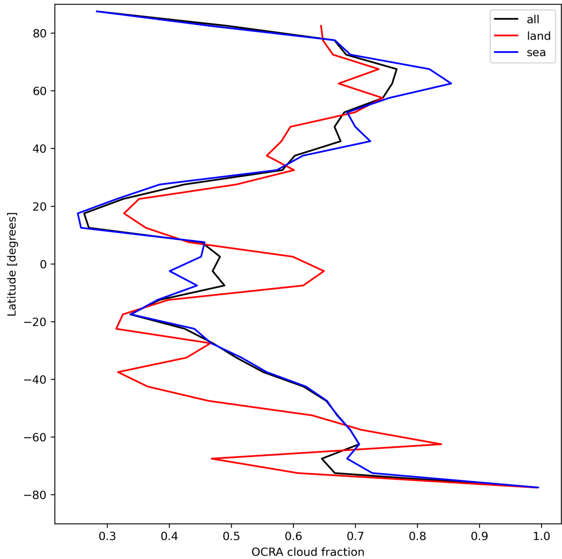
Figure 34: Zonal average of “OCRA cloud fraction” for 2024-04-22 to 2024-04-24.
