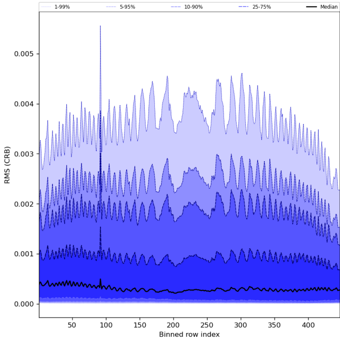
Figure 64: Along track statistics of “RMS (CRB)” for 2024-04-22 to 2024-04-24
