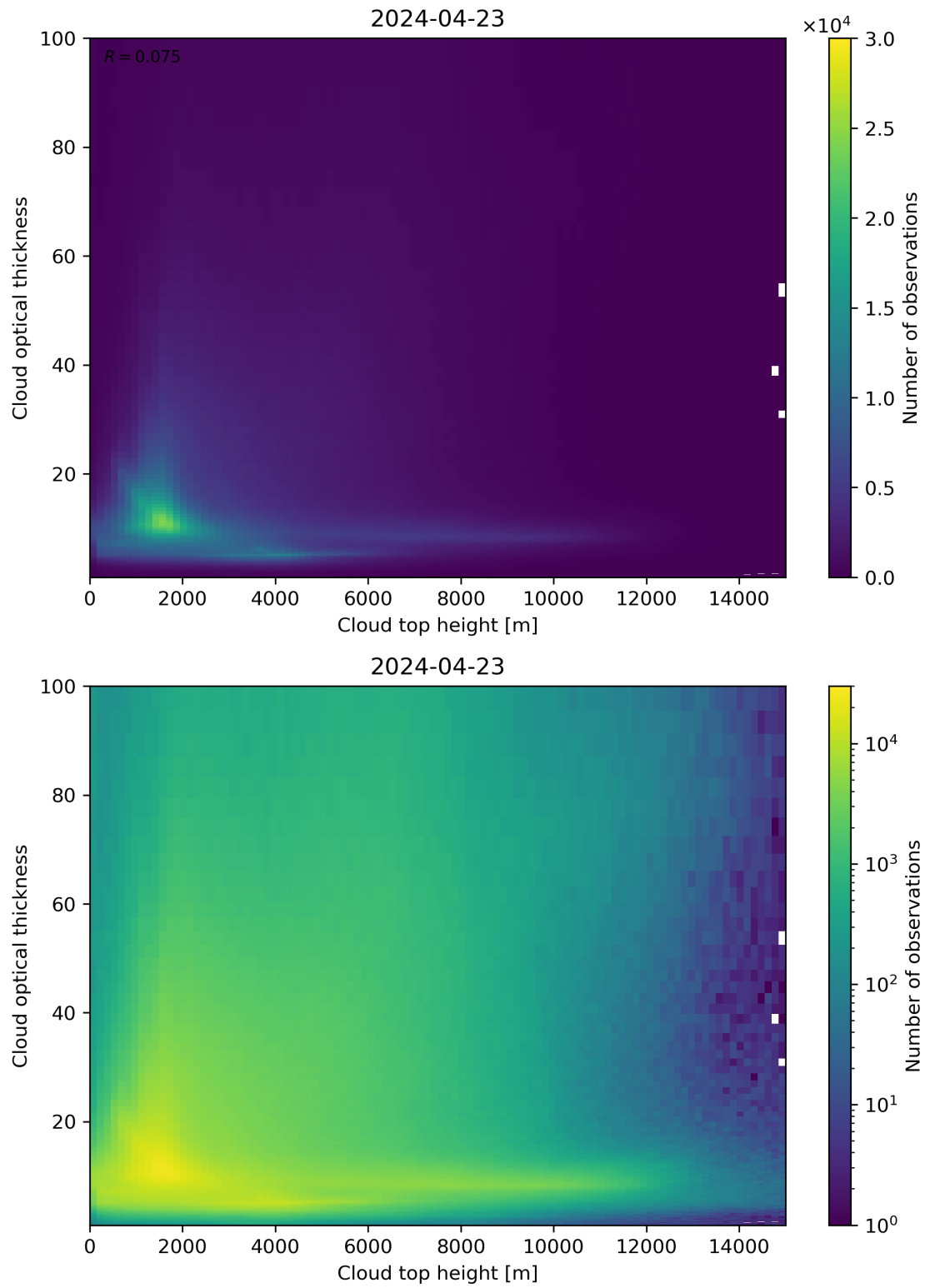
Figure 90: Scatter density plot of “Cloud top height” against “Cloud optical thickness” for 2024-04-22 to 2024-04-24.
