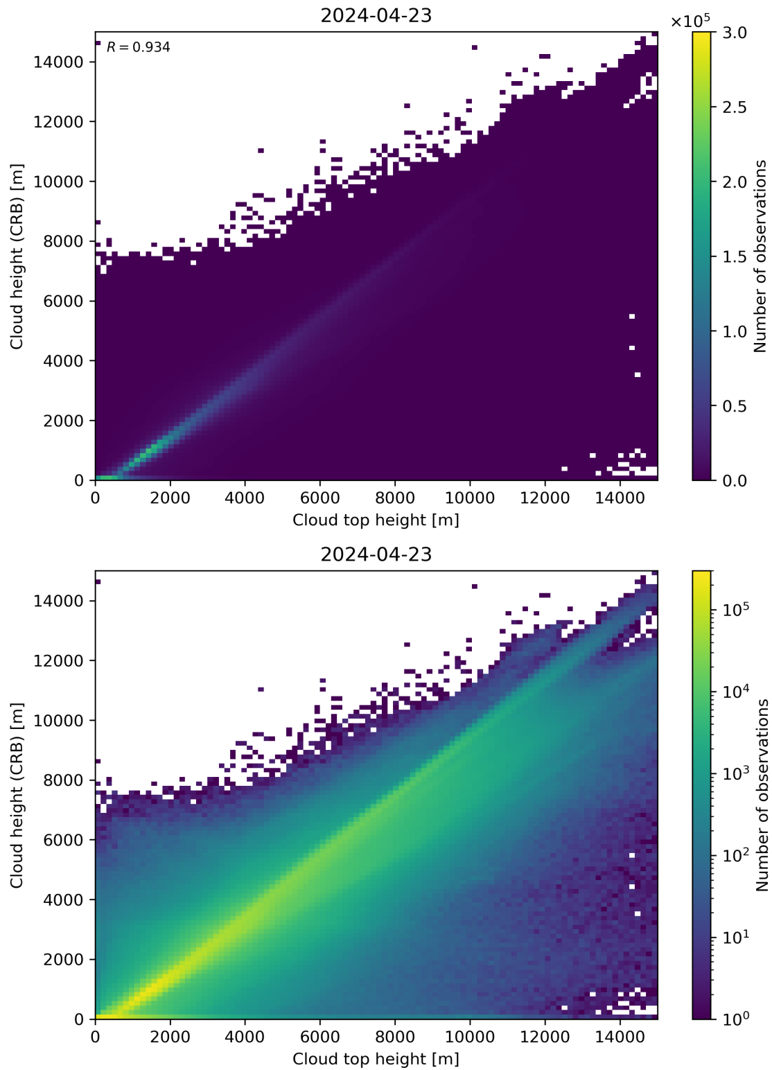
Figure 89: Scatter density plot of “Cloud top height” against “Cloud height (CRB)” for 2024-04-22 to 2024-04-24.
