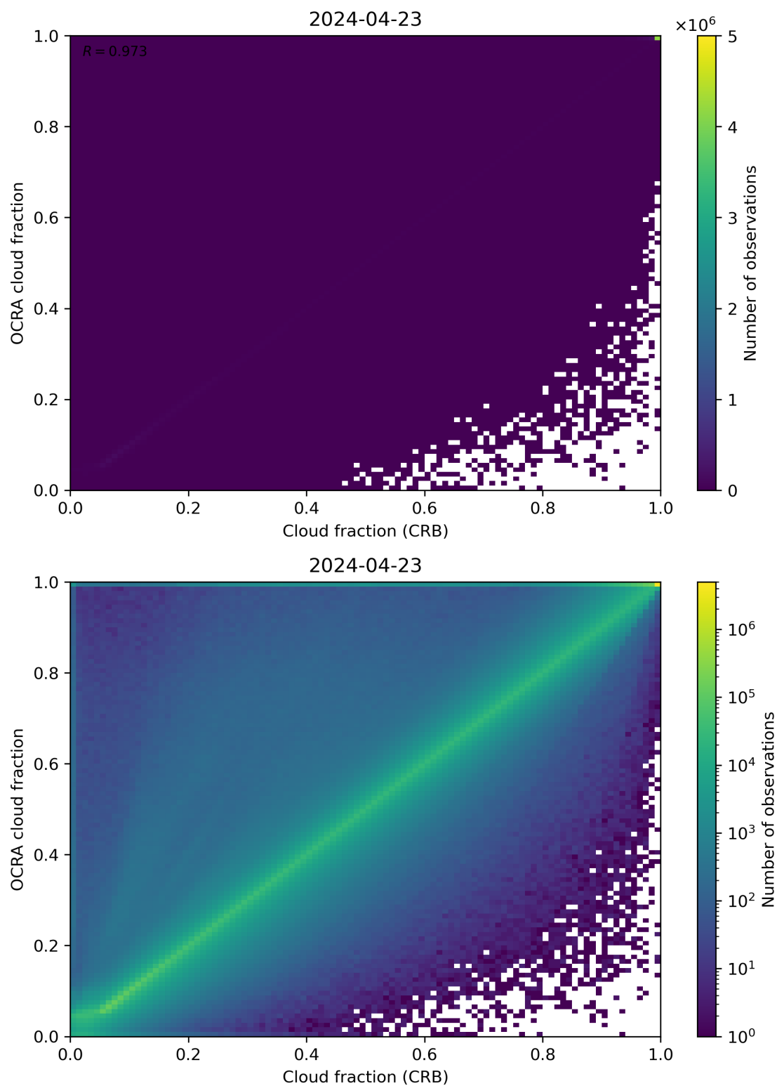
Figure 78: Scatter density plot of “Cloud fraction (CRB)” against “OCRA cloud fraction” for 2024-04-22 to 2024-04-24.
