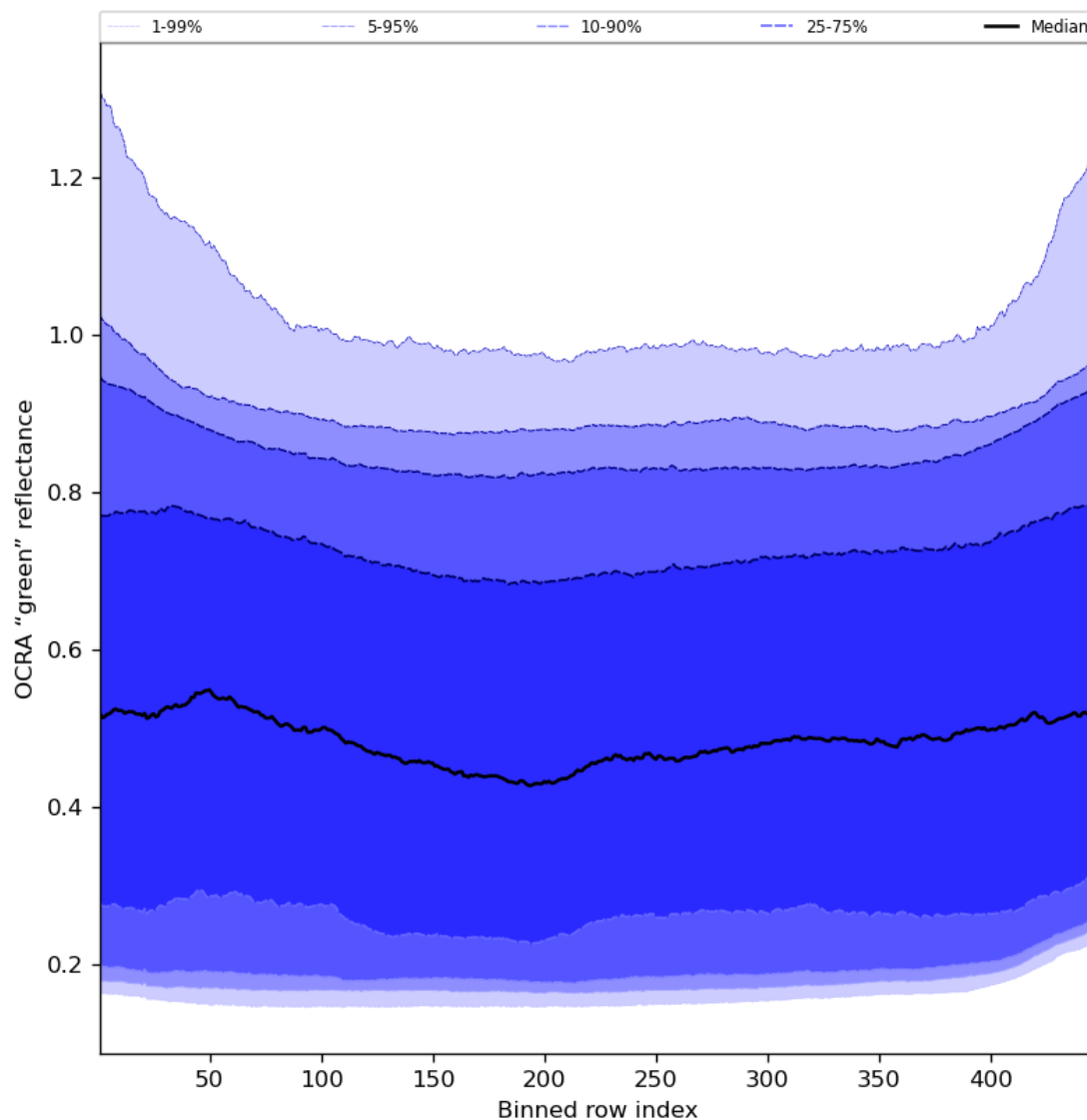
Figure 68: Along track statistics of “OCRA “green” reflectance” for 2024-04-22 to 2024-04-24
