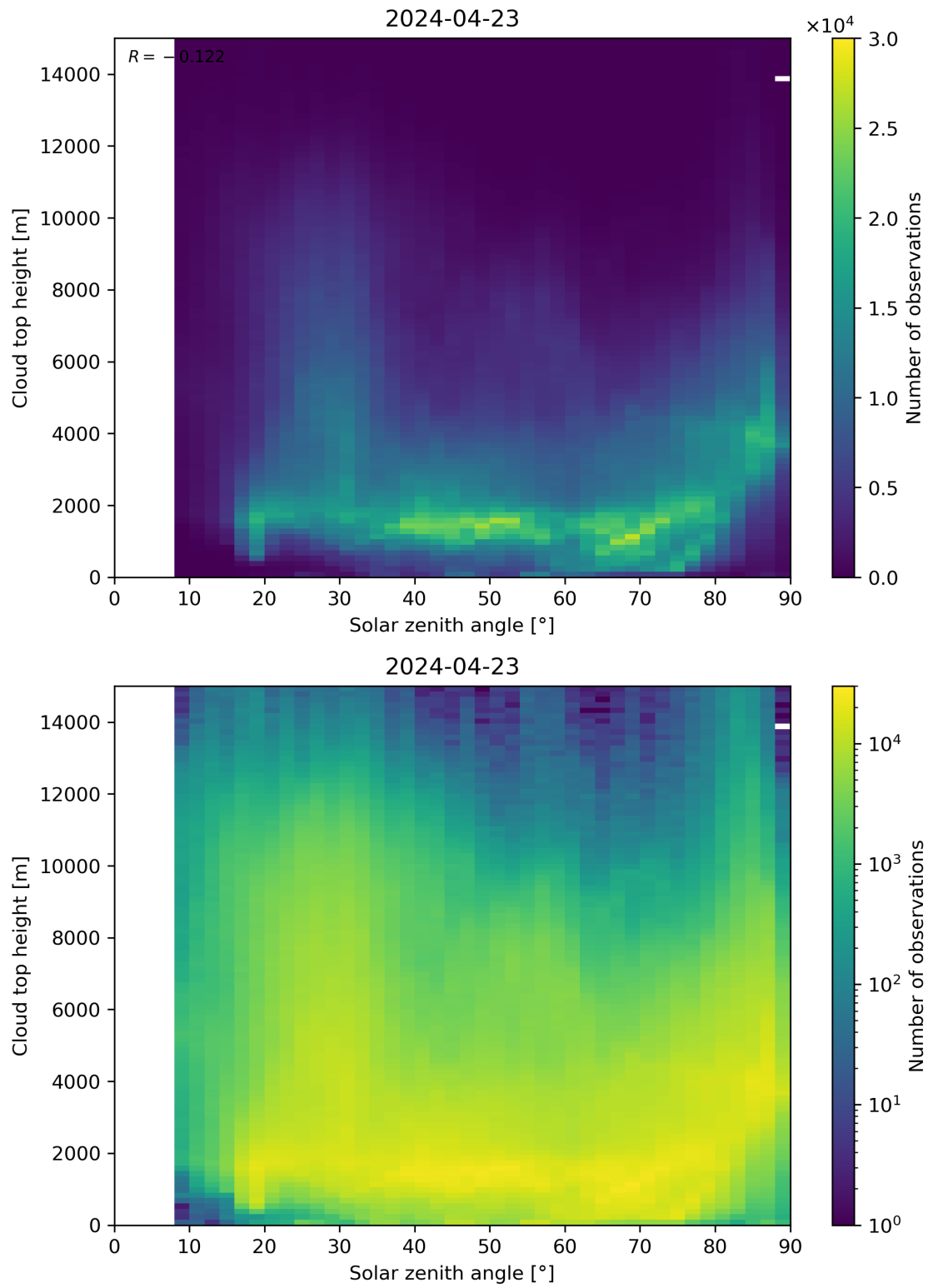
Figure 104: Scatter density plot of “Solar zenith angle” against “Cloud top height” for 2024-04-22 to 2024-04-24.
