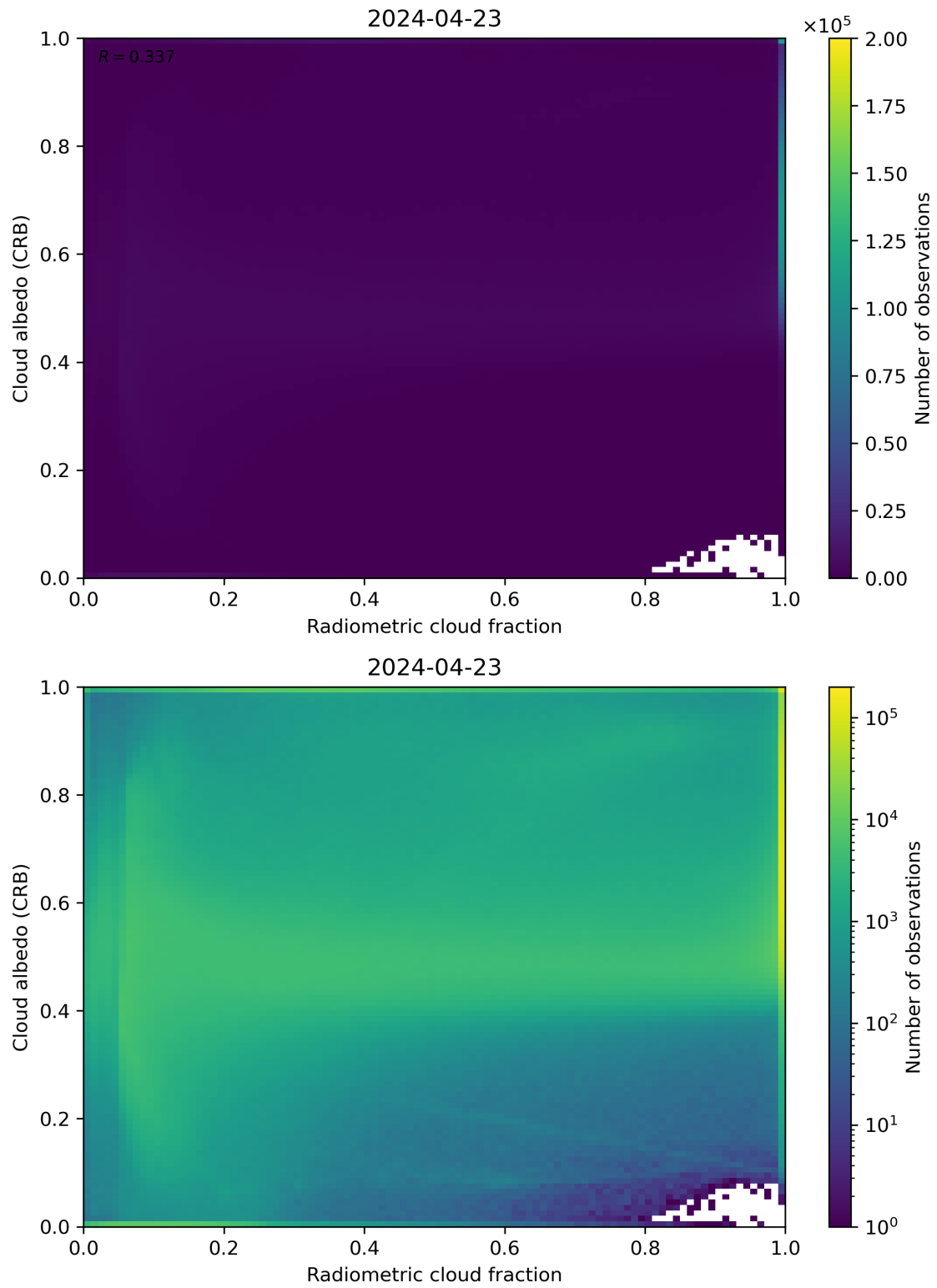
Figure 71: Scatter density plot of “Radiometric cloud fraction” against “Cloud albedo (CRB)” for 2024-04-22 to 2024-04-24.
