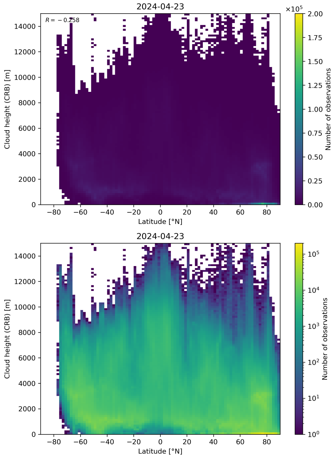
Figure 95: Scatter density plot of “Latitude” against “Cloud height (CRB)” for 2024-04-22 to 2024-04-24.
