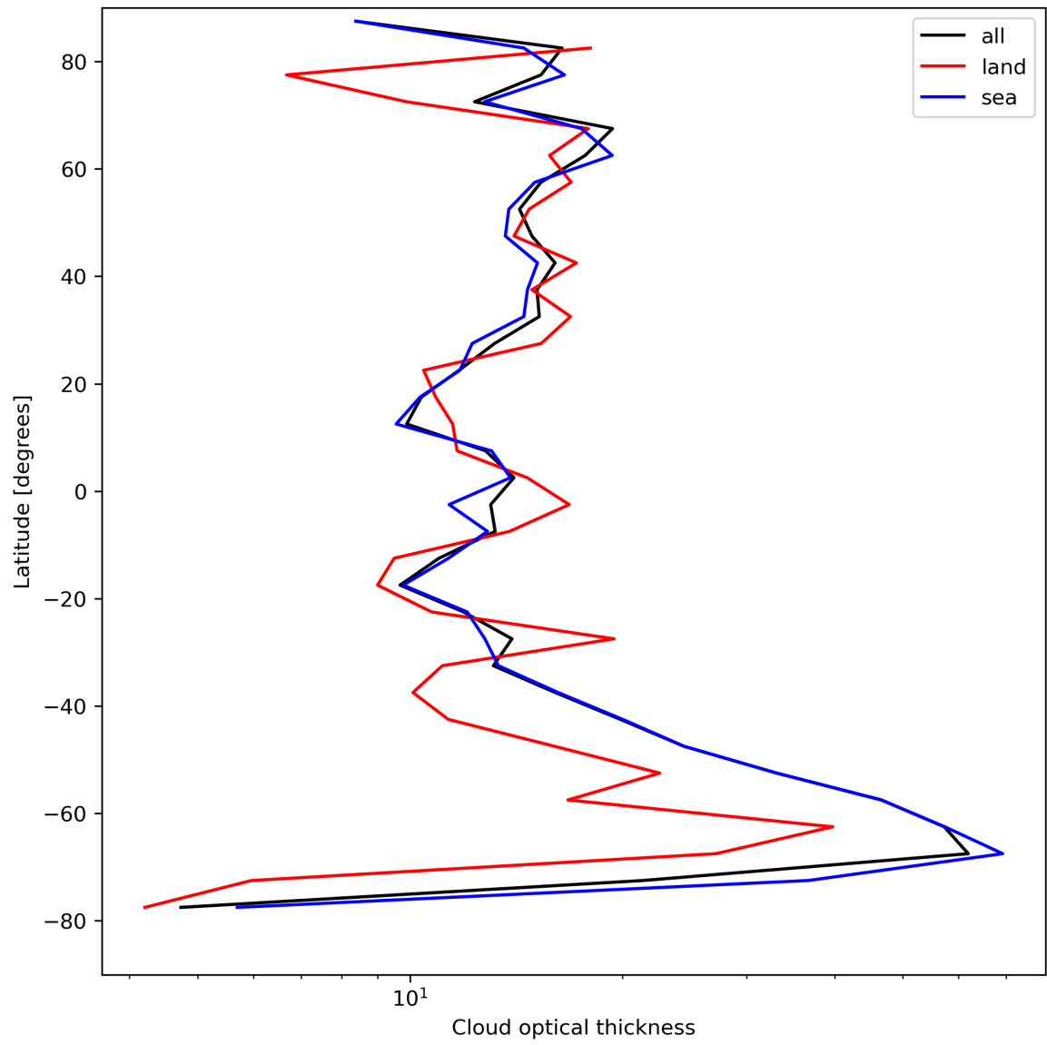
Figure 25: Zonal average of “Cloud optical thickness” for 2024-04-22 to 2024-04-24.
