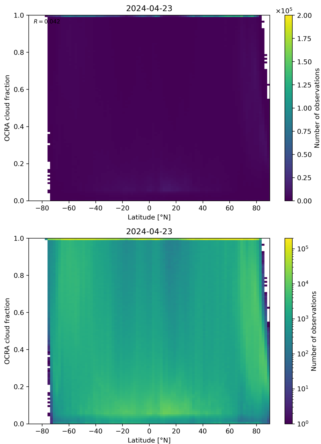
Figure 93: Scatter density plot of “Latitude” against “OCRA cloud fraction” for 2024-04-22 to 2024-04-24.
