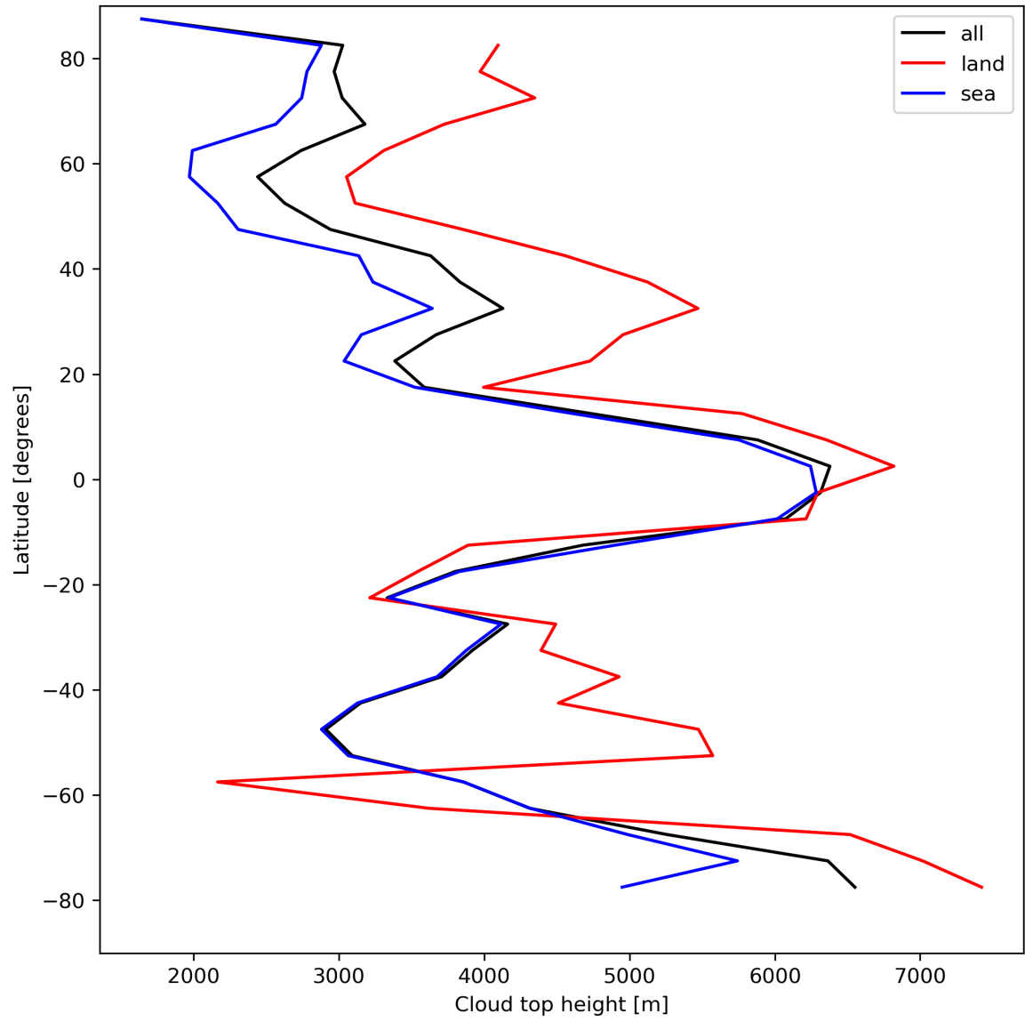
Figure 24: Zonal average of “Cloud top height” for 2024-04-22 to 2024-04-24.
