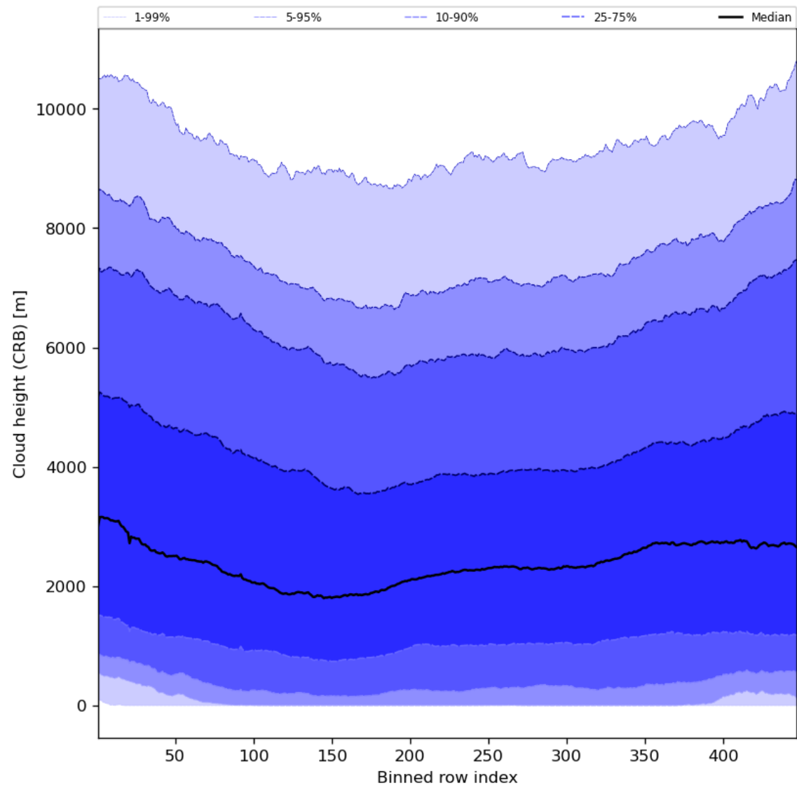
Figure 59: Along track statistics of “Cloud height (CRB)” for 2024-04-22 to 2024-04-24
