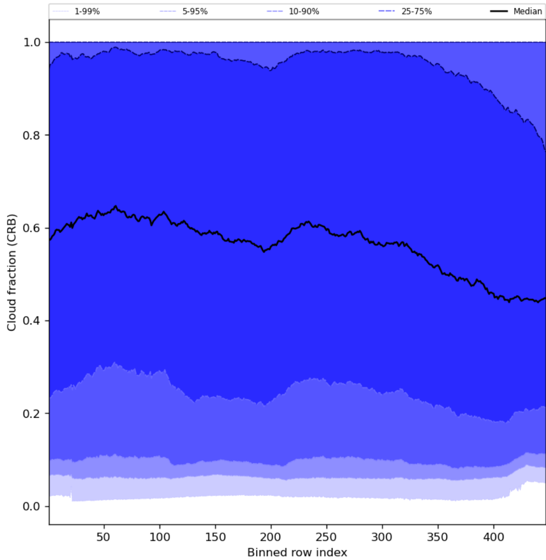
Figure 58: Along track statistics of “Cloud fraction (CRB)” for 2024-04-22 to 2024-04-24
