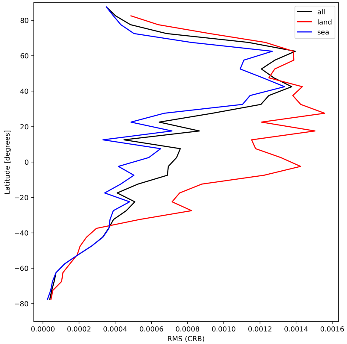
Figure 32: Zonal average of “RMS (CRB)” for 2024-04-22 to 2024-04-24.
