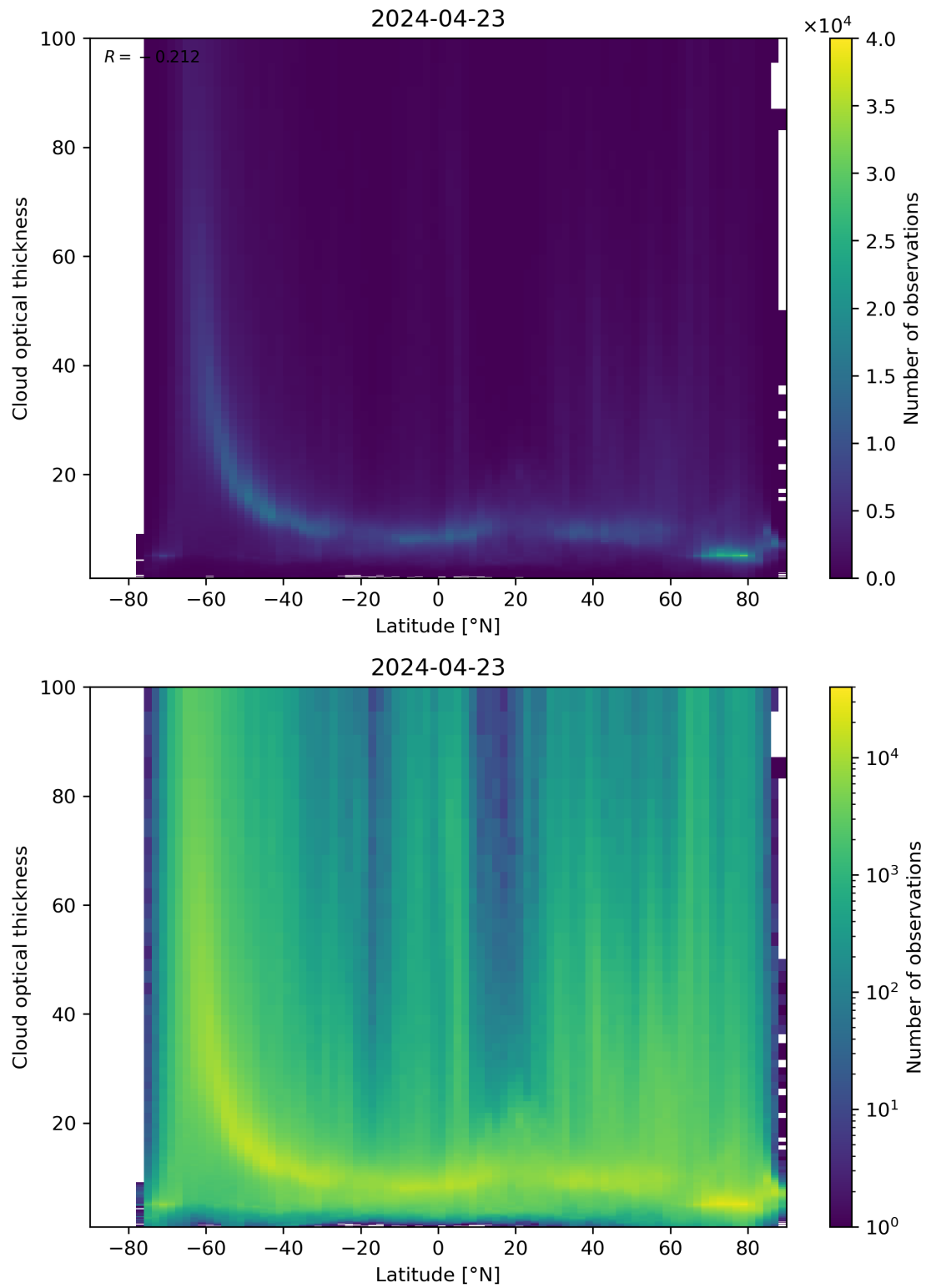
Figure 96: Scatter density plot of “Latitude” against “Cloud optical thickness” for 2024-04-22 to 2024-04-24.
