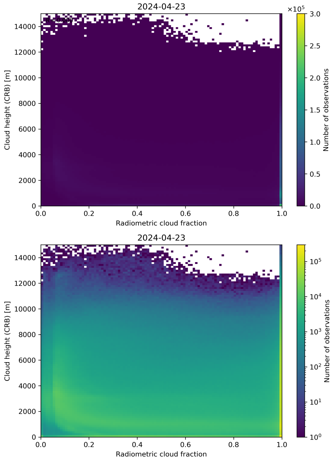
Figure 74: Scatter density plot of “Radiometric cloud fraction” against “Cloud height (CRB)” for 2024-04-22 to 2024-04-24.
