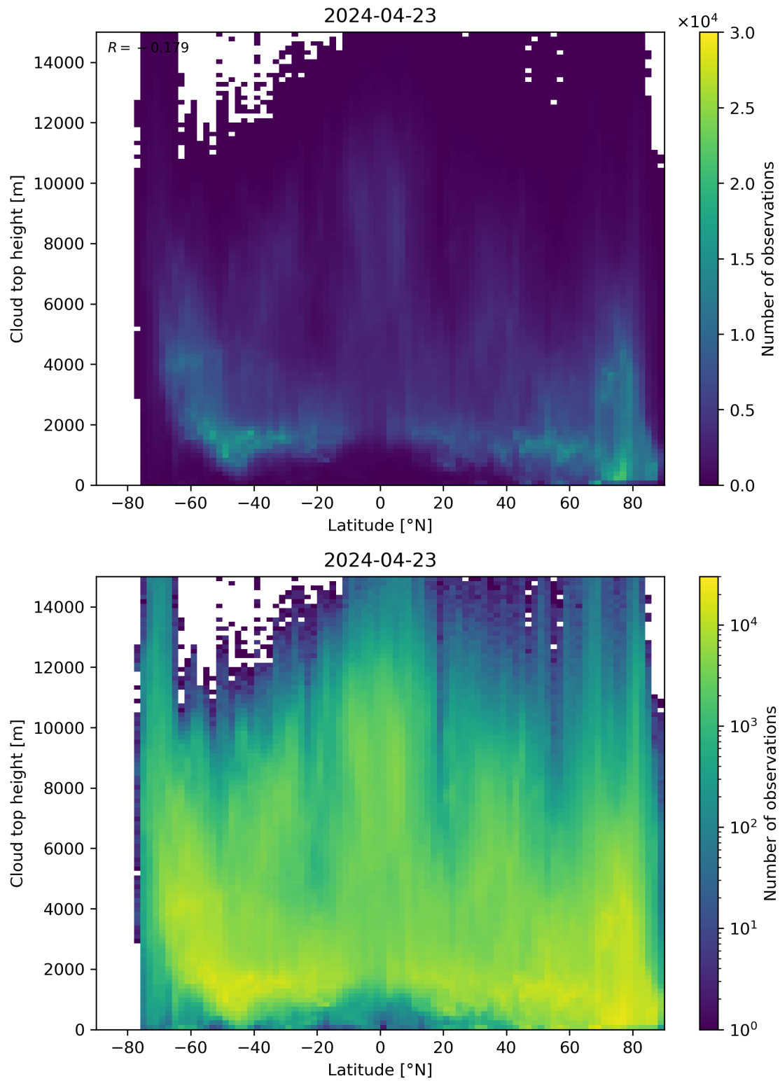
Figure 97: Scatter density plot of “Latitude” against “Cloud top height” for 2024-04-22 to 2024-04-24.
