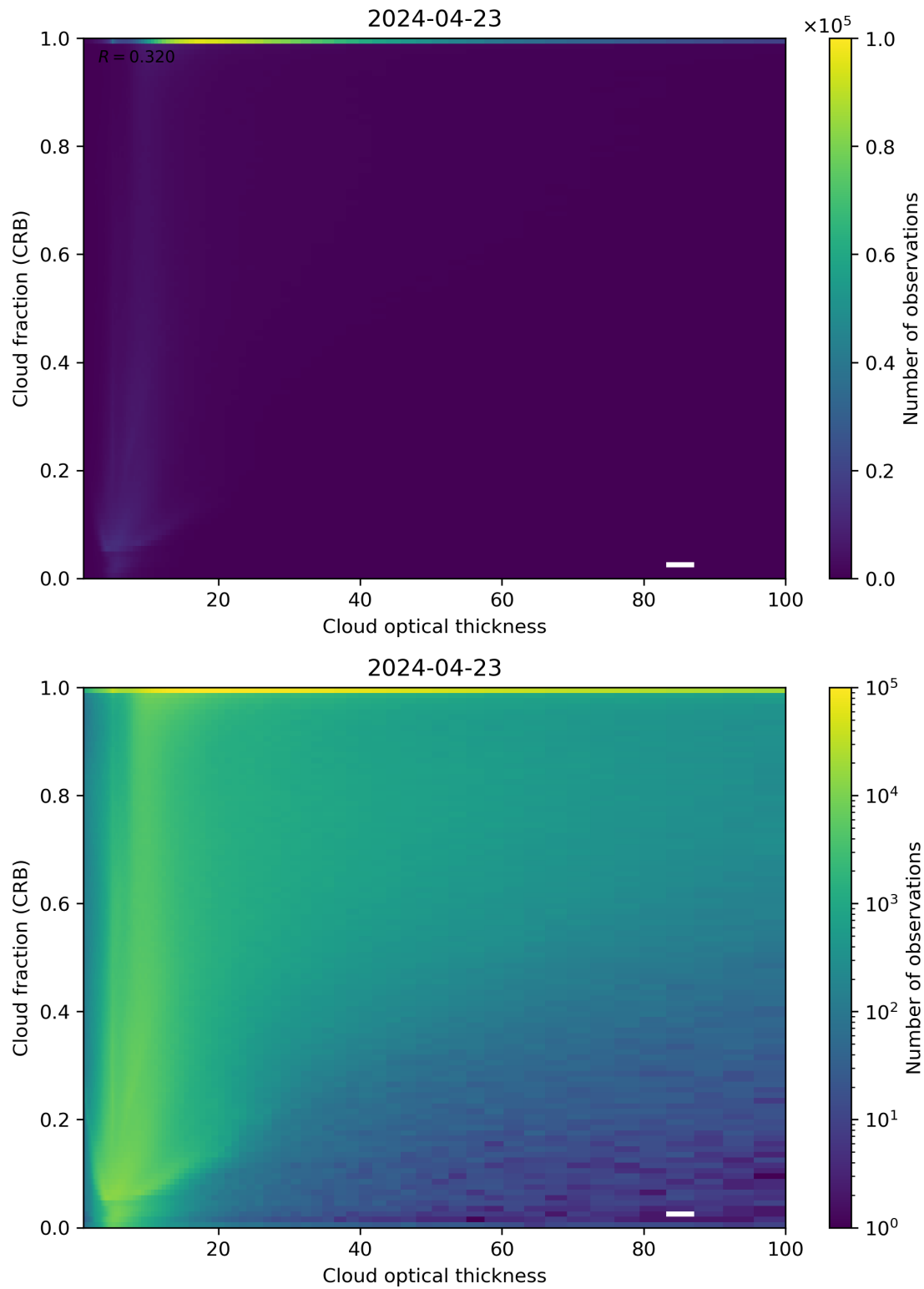
Figure 84: Scatter density plot of “Cloud optical thickness” against “Cloud fraction (CRB)” for 2024-04-22 to 2024-04-24.
