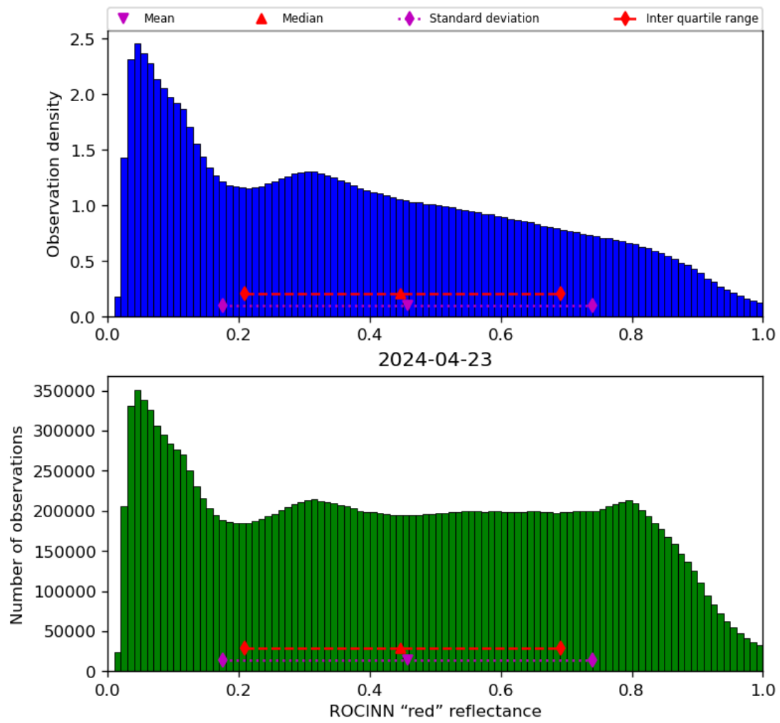
Figure 53: Histogram of “ROCINN “red” reflectance” for 2024-04-22 to 2024-04-24
