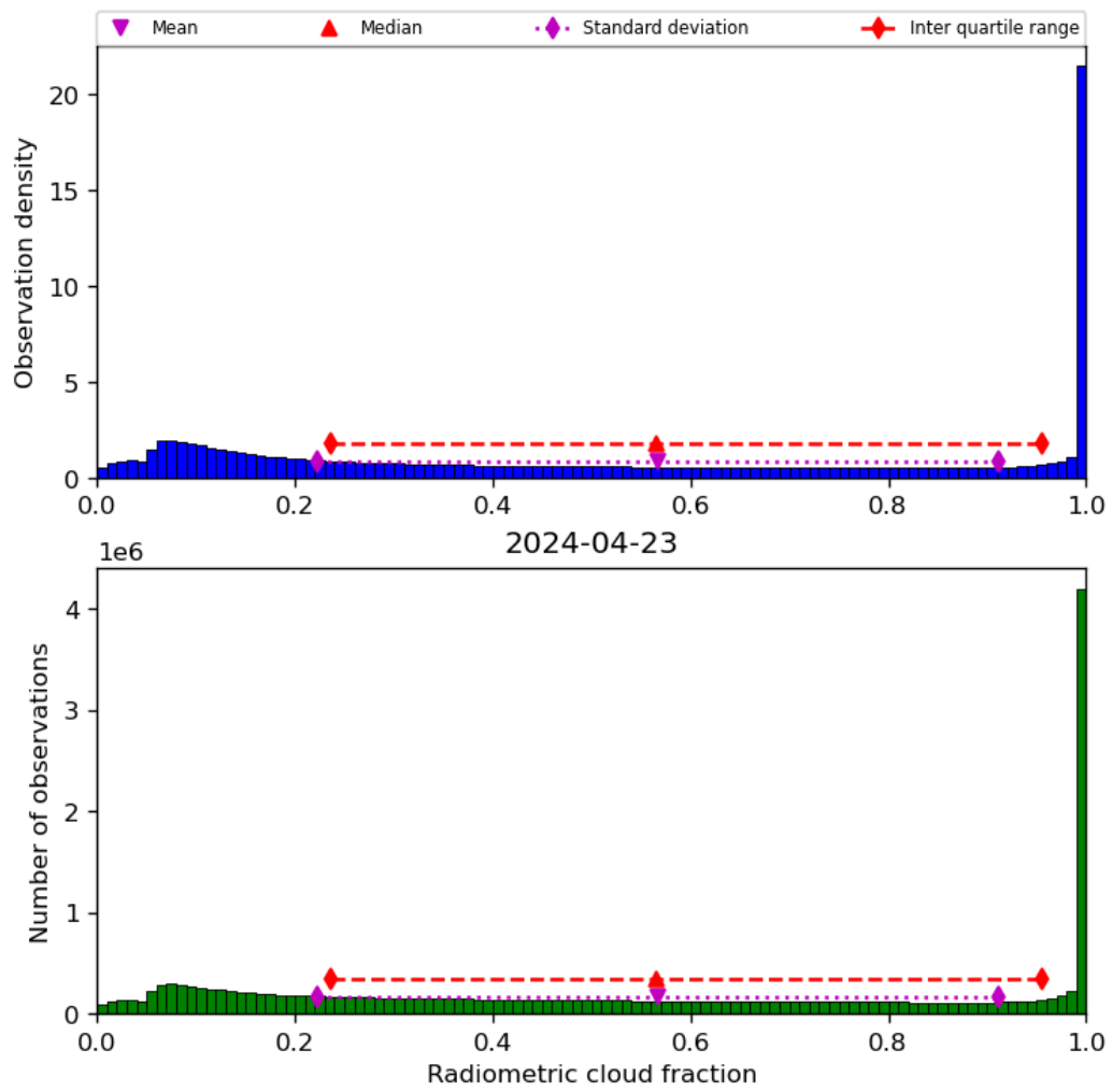
Figure 39: Histogram of “Radiometric cloud fraction” for 2024-04-22 to 2024-04-24
