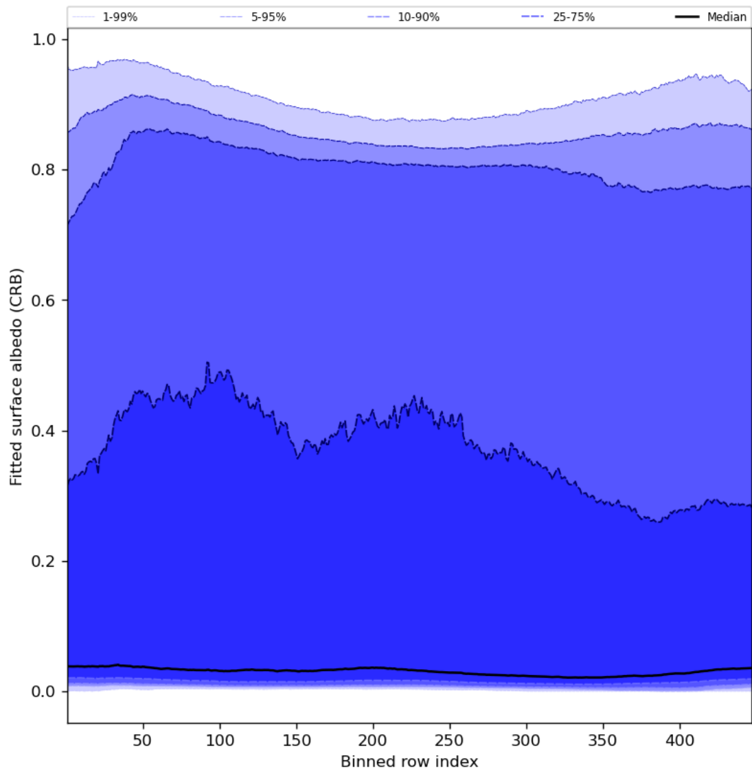
Figure 62: Along track statistics of “Fitted surface albedo (CRB)” for 2024-04-22 to 2024-04-24
