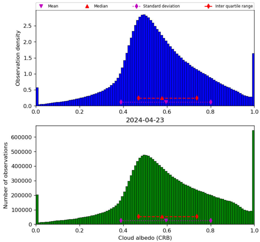
Figure 44: Histogram of “Cloud albedo (CRB)” for 2024-04-22 to 2024-04-24
