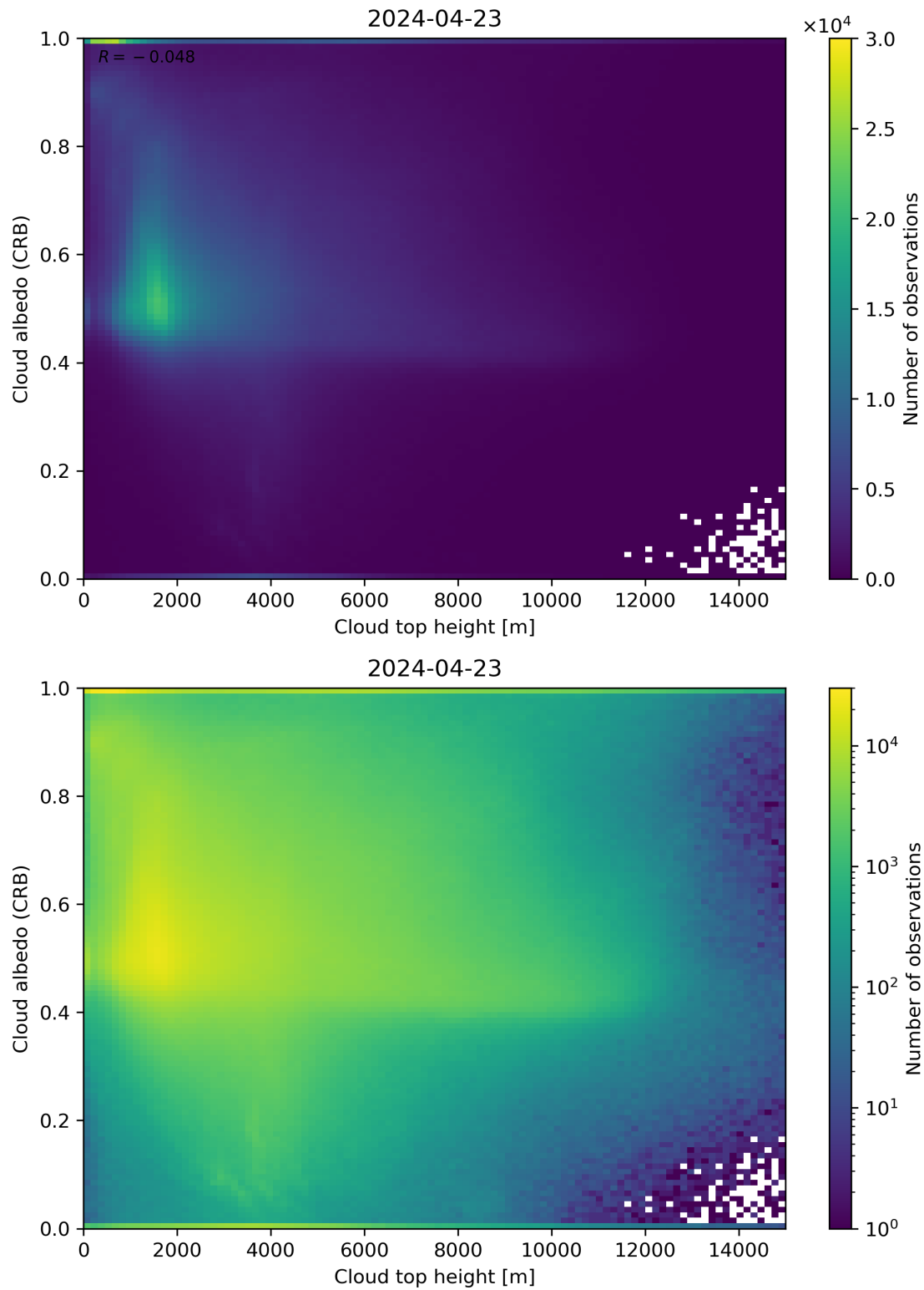
Figure 86: Scatter density plot of “Cloud top height” against “Cloud albedo (CRB)” for 2024-04-22 to 2024-04-24.
