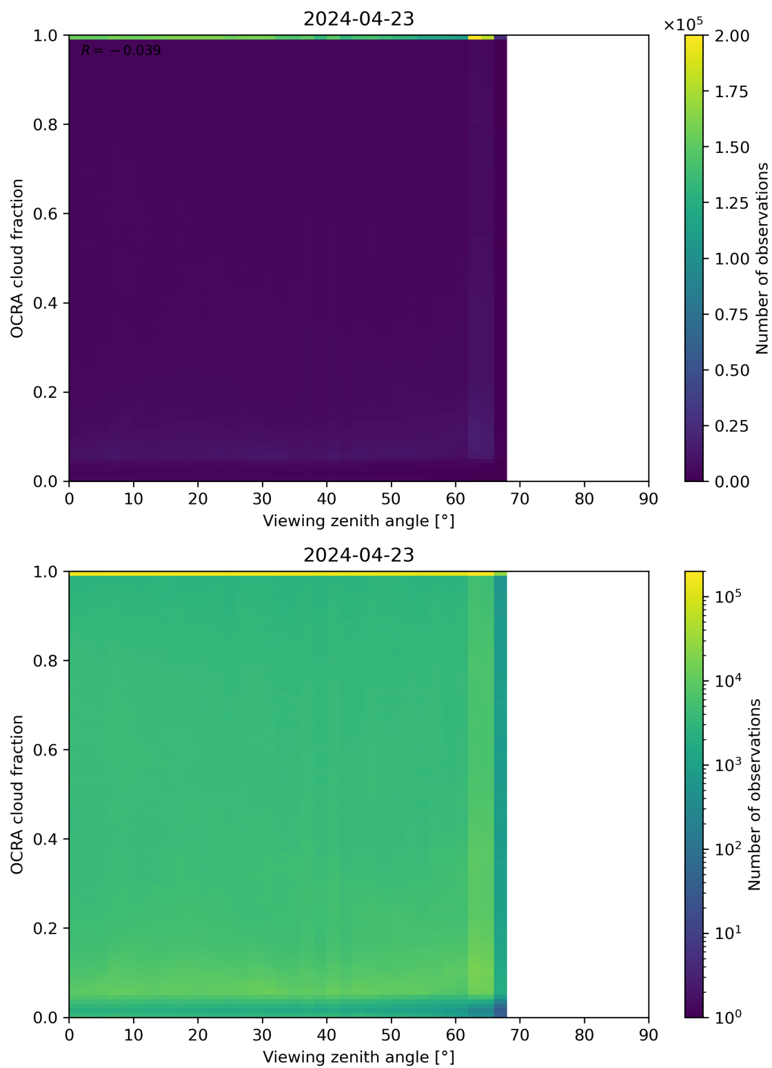
Figure 108: Scatter density plot of “Viewing zenith angle” against “OCRA cloud fraction” for 2024-04-22 to 2024-04-24.
