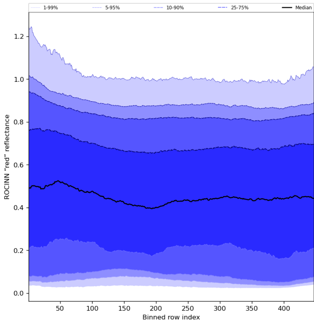
Figure 69: Along track statistics of “ROCINN “red” reflectance” for 2024-04-22 to 2024-04-24
