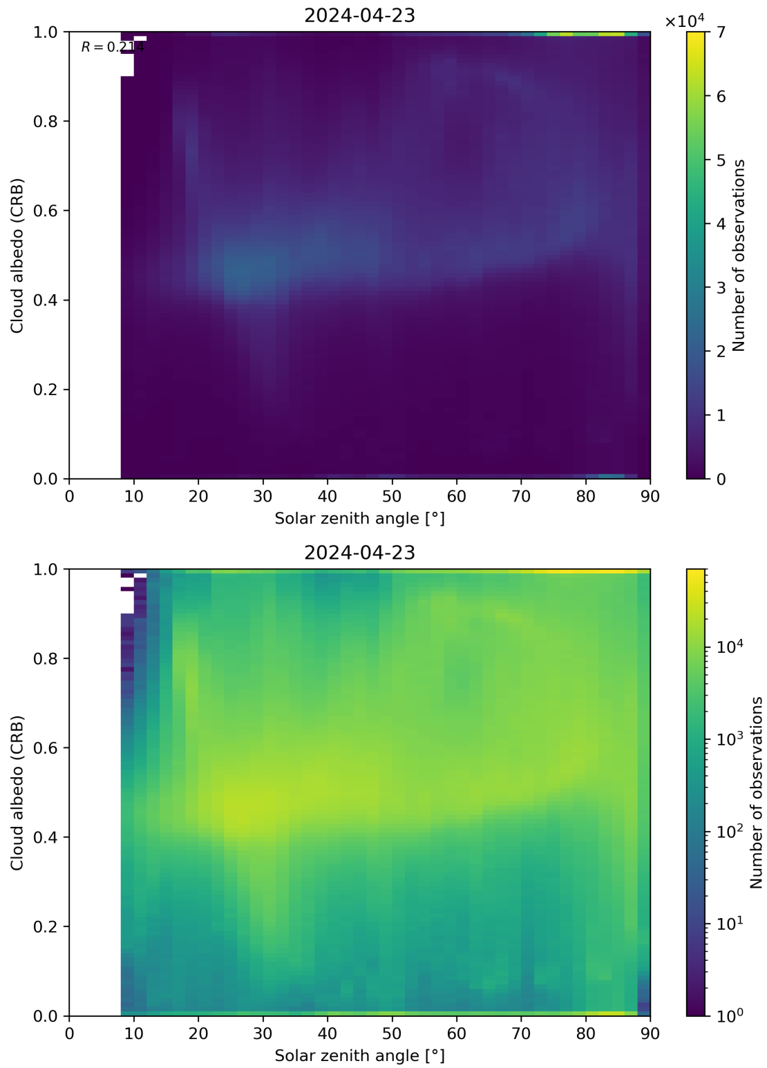
Figure 98: Scatter density plot of “Solar zenith angle” against “Cloud albedo (CRB)” for 2024-04-22 to 2024-04-24.
