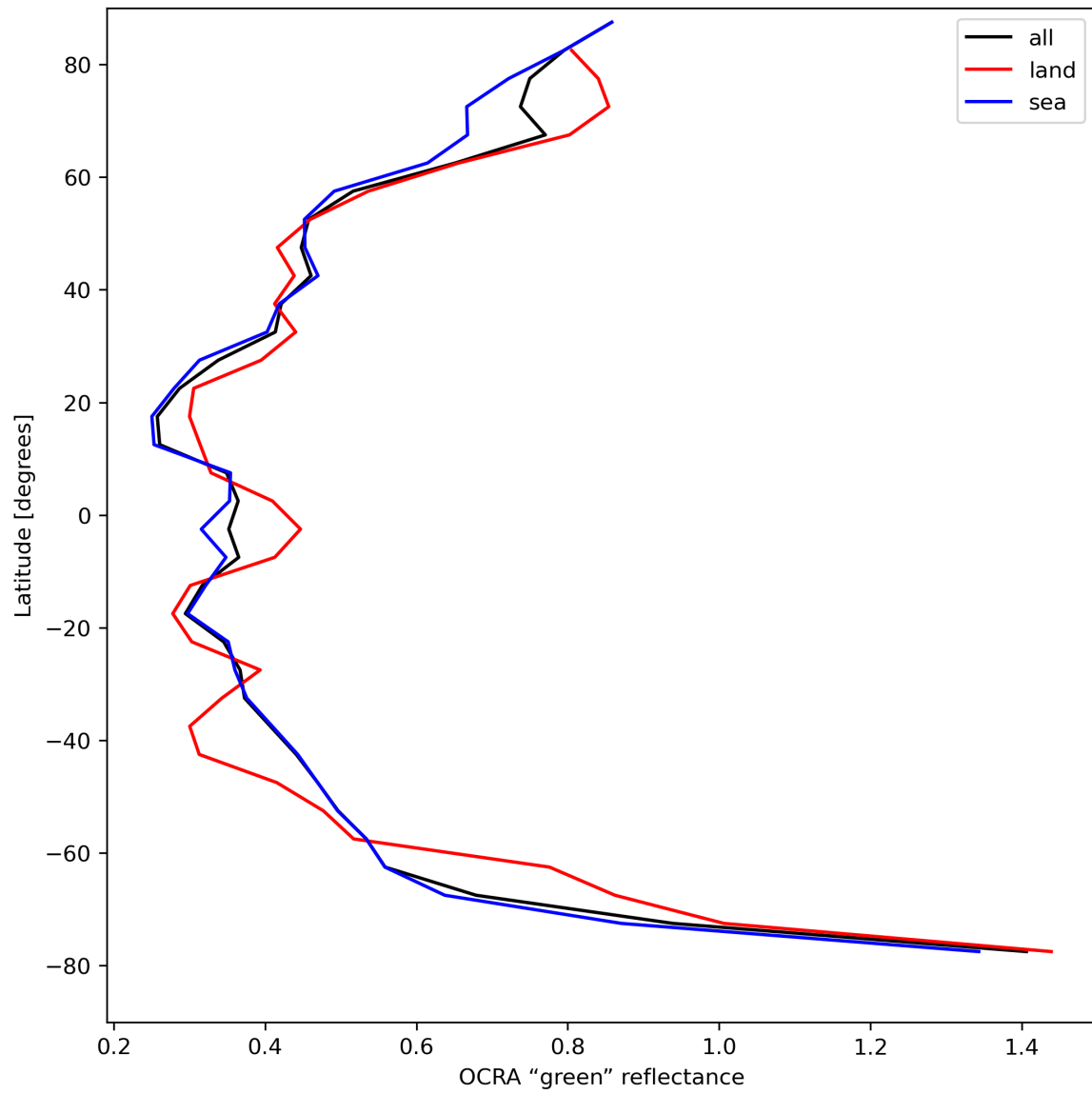
Figure 36: Zonal average of “OCRA “green” reflectance” for 2024-04-22 to 2024-04-24.
