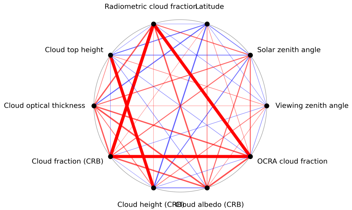
Figure 1: Map of correlation graph for 2024-04-22 to 2024-04-24.
