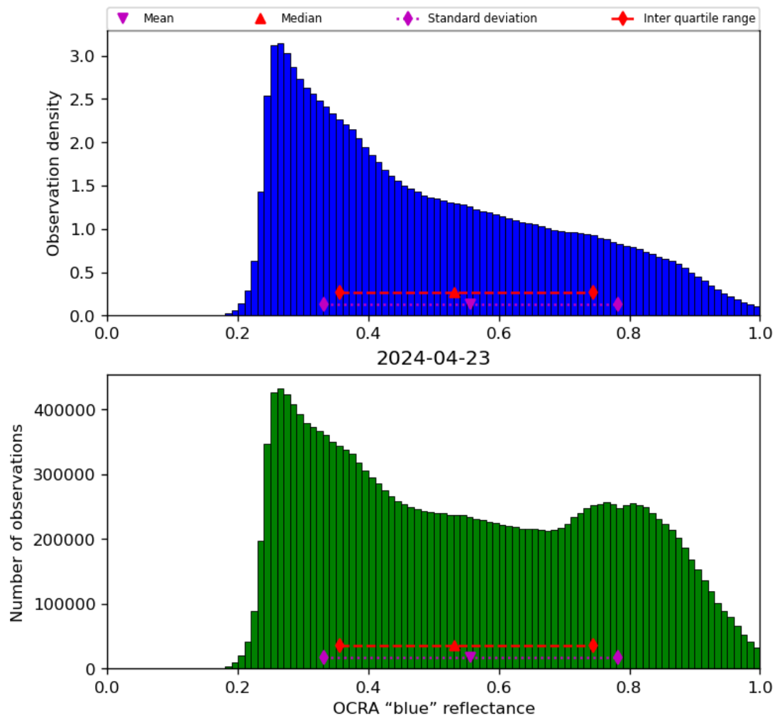
Figure 51: Histogram of “OCRA “blue” reflectance” for 2024-04-22 to 2024-04-24
