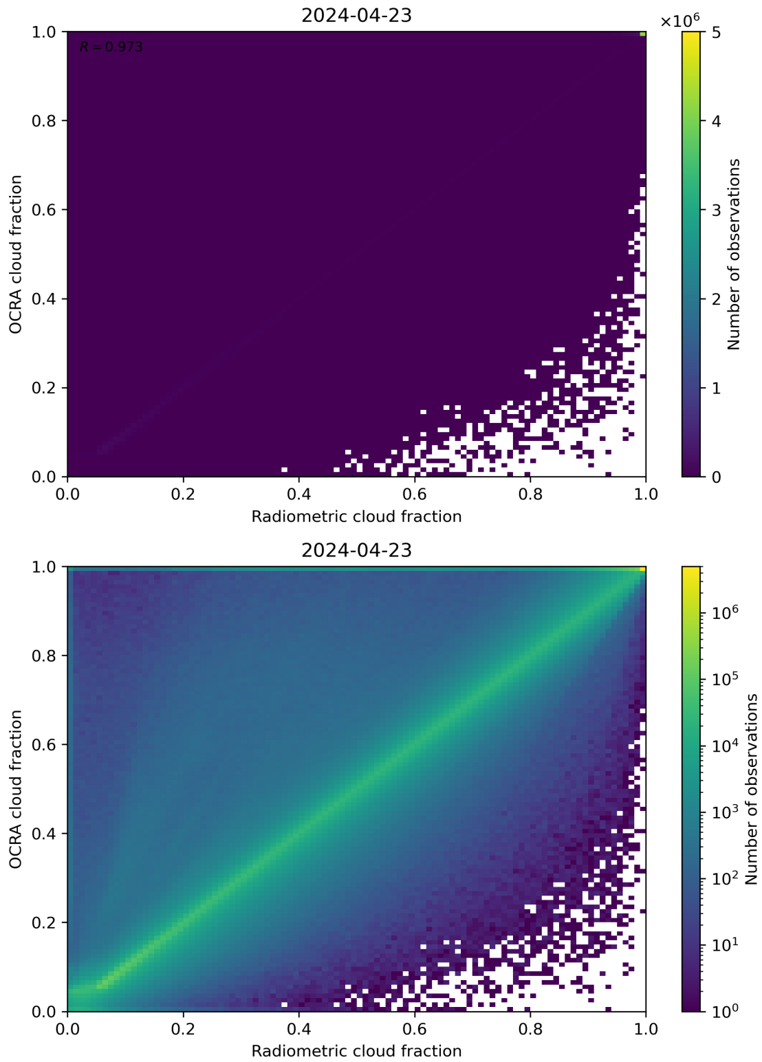
Figure 72: Scatter density plot of “Radiometric cloud fraction” against “OCRA cloud fraction” for 2024-04-22 to 2024-04-24.
