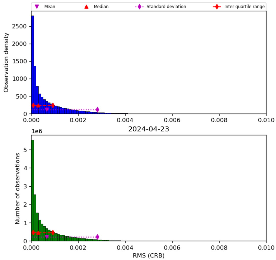
Figure 48: Histogram of “RMS (CRB)” for 2024-04-22 to 2024-04-24
