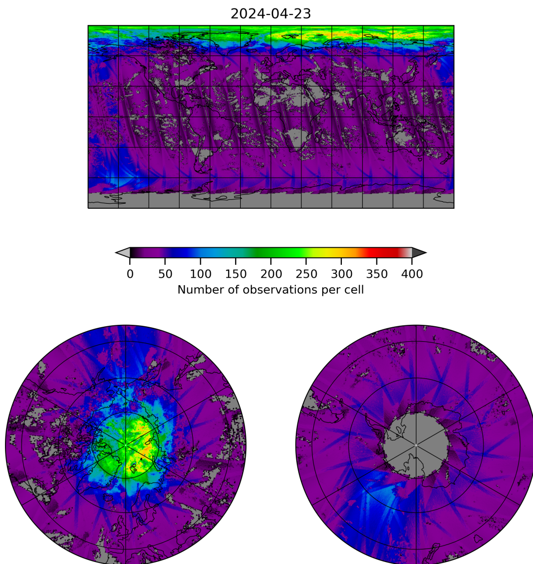
Figure 21: Map of the number of observations for 2024-04-22 to 2024-04-24
