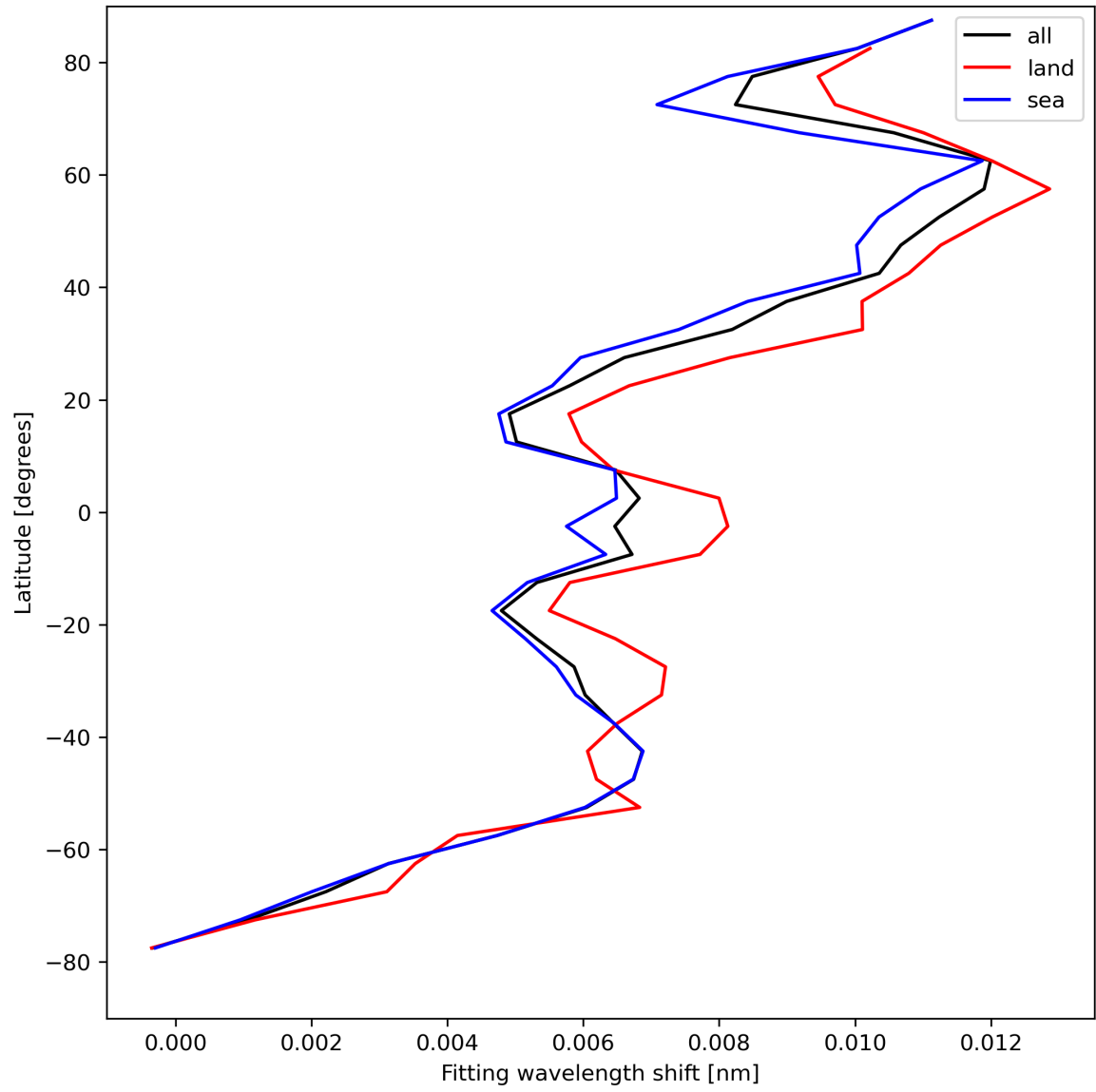
Figure 33: Zonal average of “Fitting wavelength shift” for 2024-04-22 to 2024-04-24.
