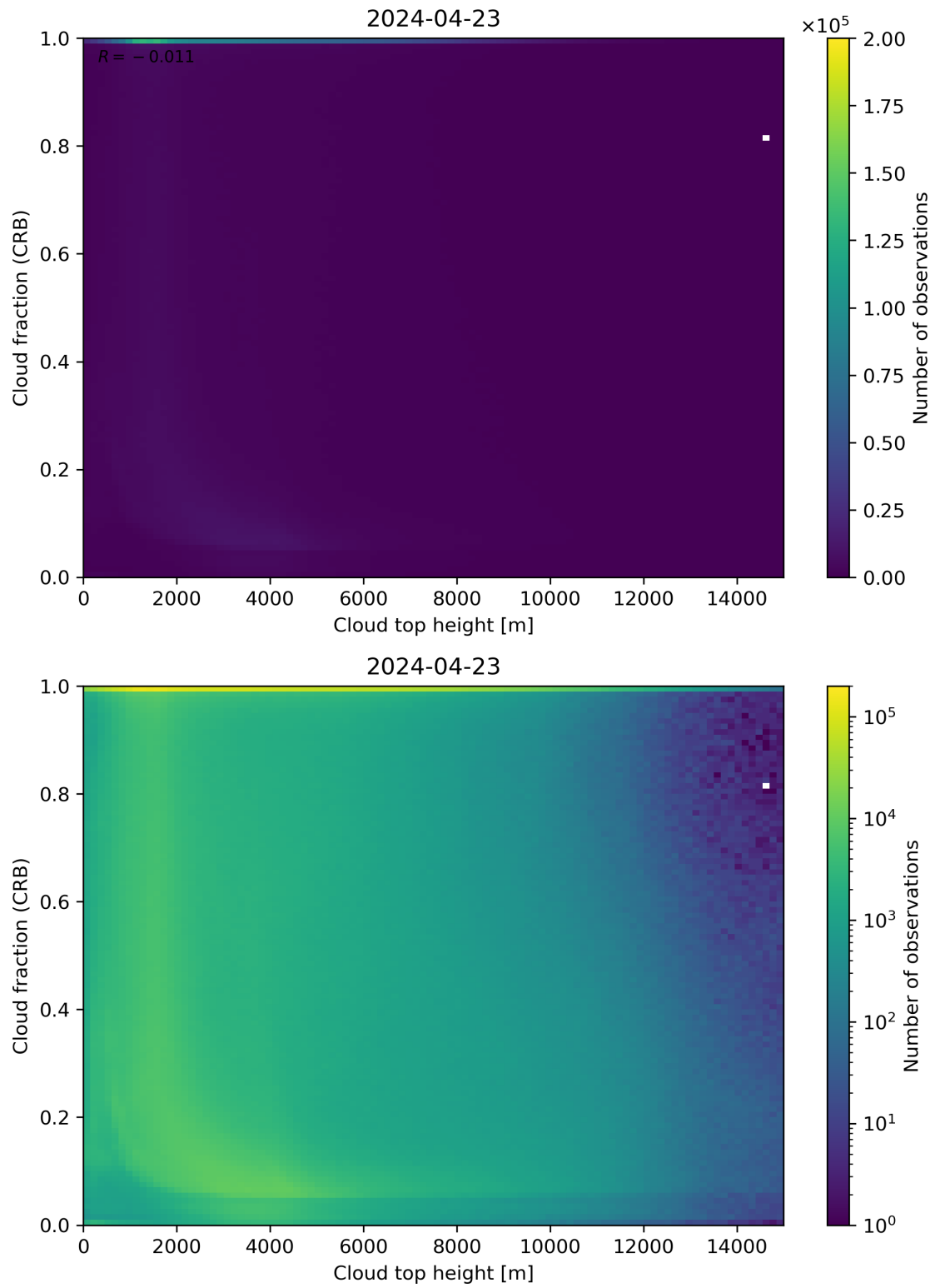
Figure 88: Scatter density plot of “Cloud top height” against “Cloud fraction (CRB)” for 2024-04-22 to 2024-04-24.
