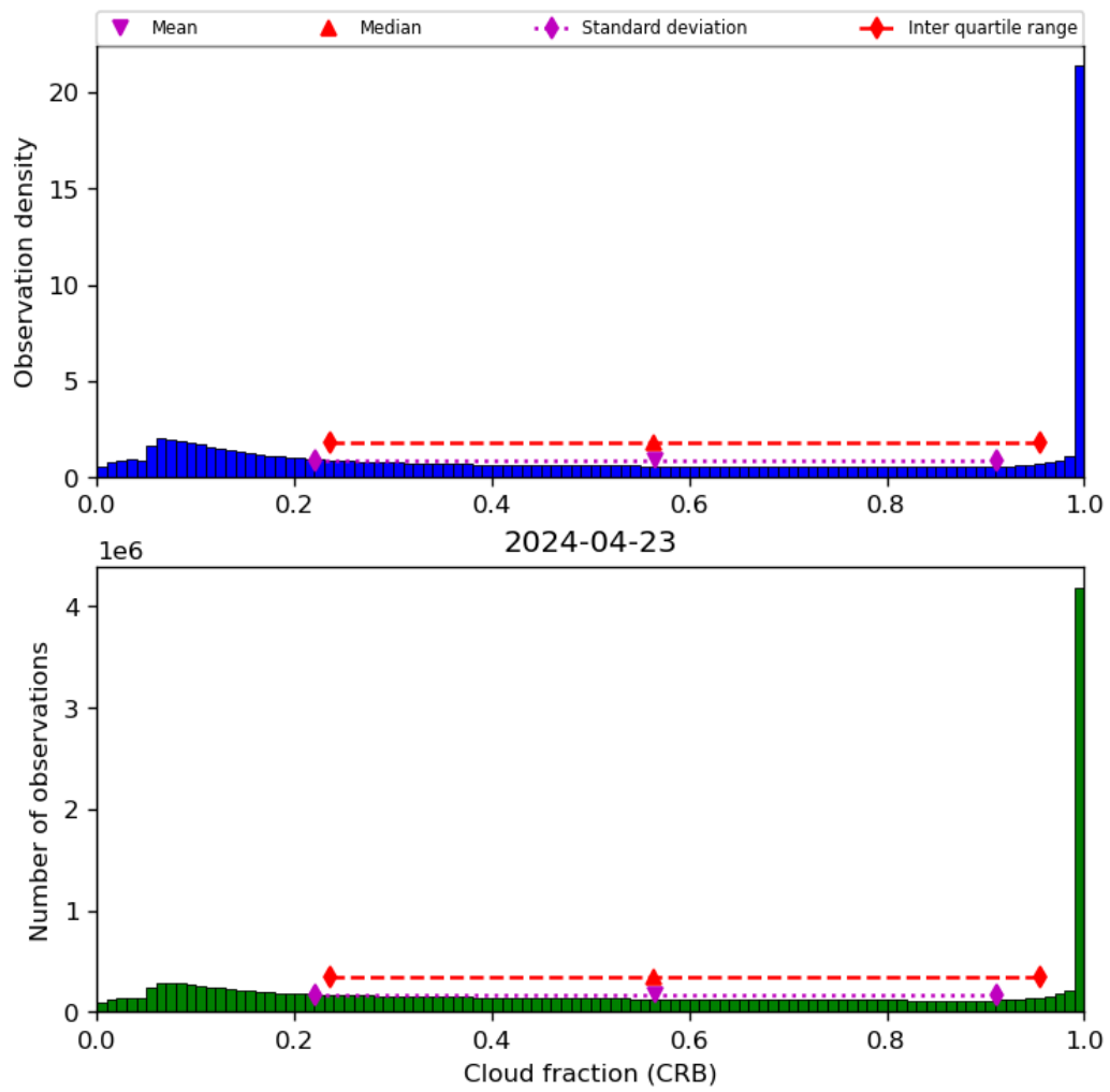
Figure 42: Histogram of “Cloud fraction (CRB)” for 2024-04-22 to 2024-04-24
