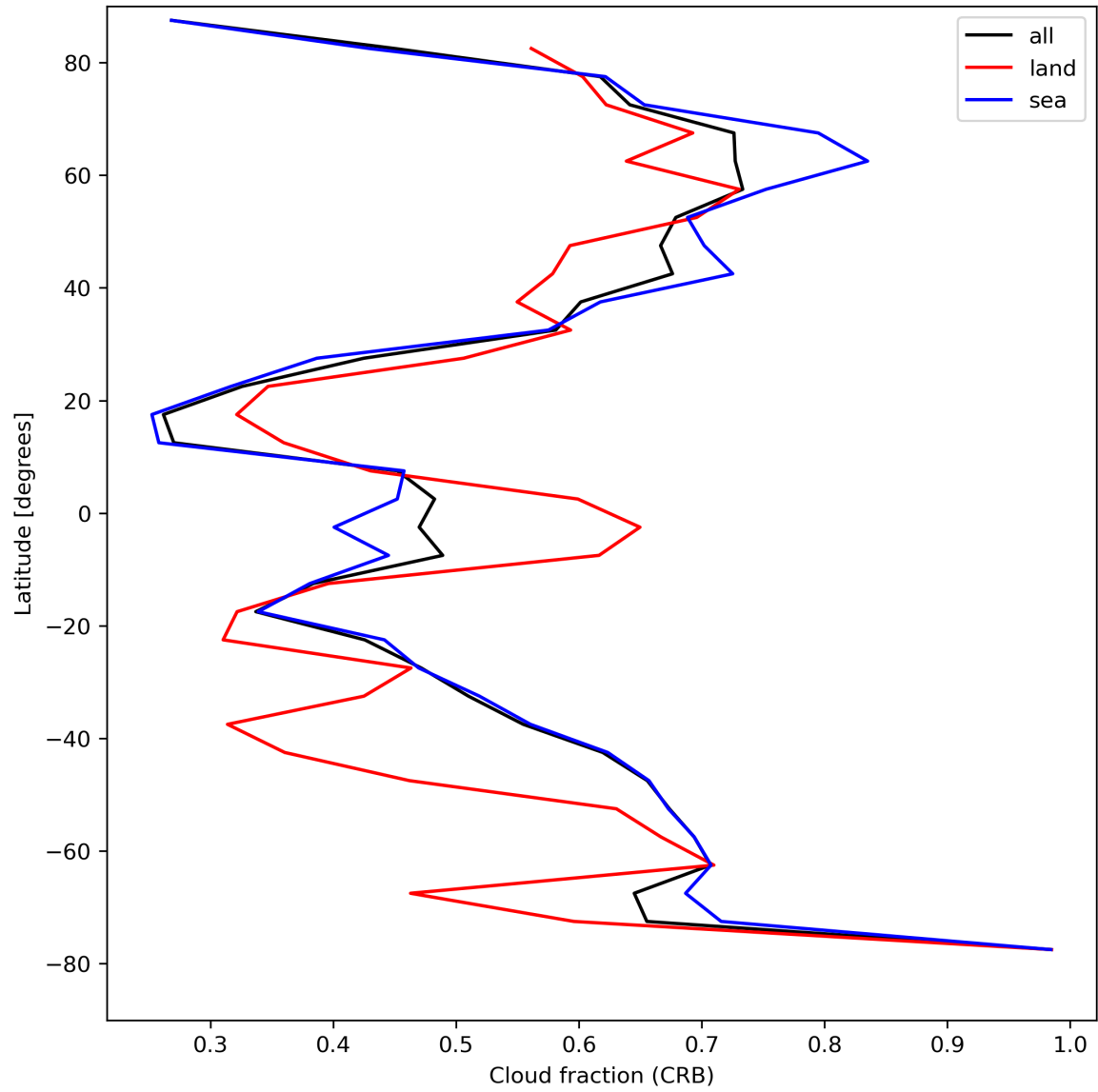
Figure 26: Zonal average of “Cloud fraction (CRB)” for 2024-04-22 to 2024-04-24.
