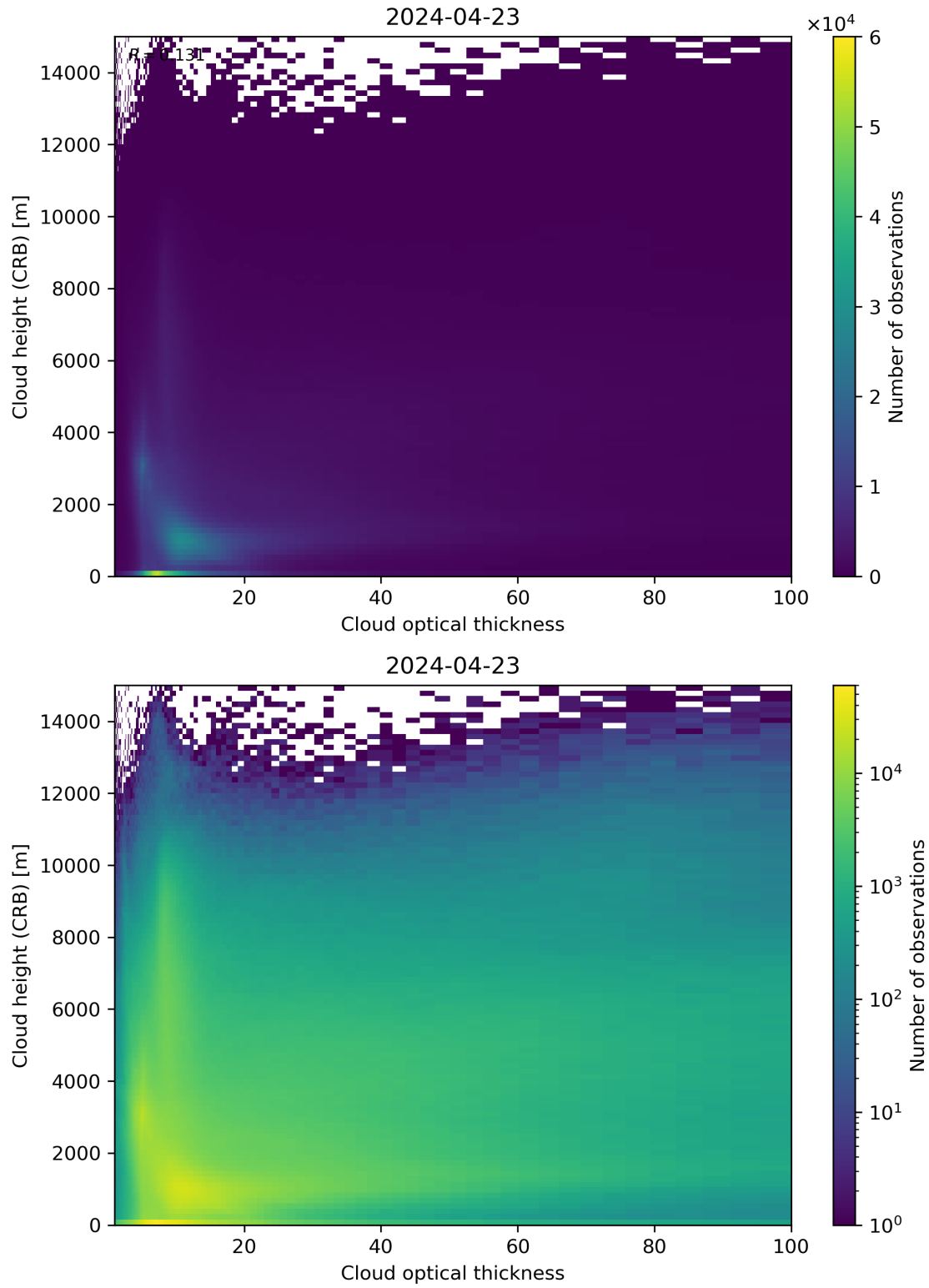
Figure 85: Scatter density plot of “Cloud optical thickness” against “Cloud height (CRB)” for 2024-04-22 to 2024-04-24.
