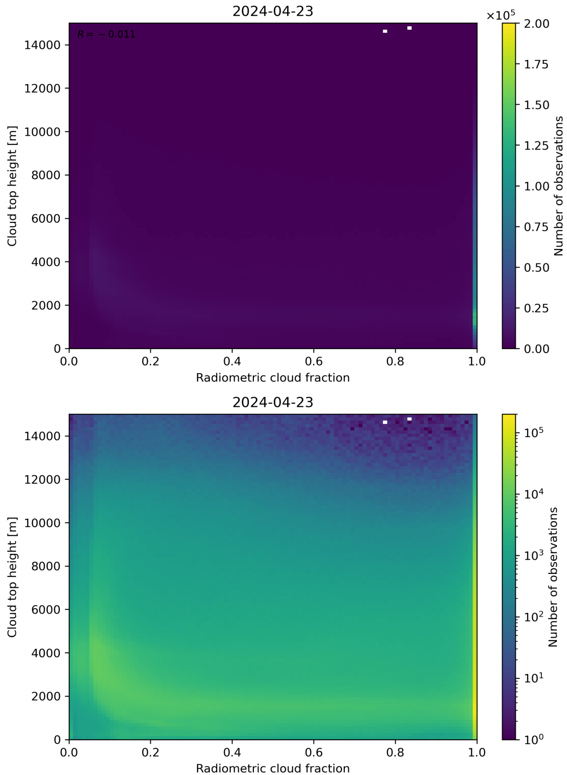
Figure 76: Scatter density plot of “Radiometric cloud fraction” against “Cloud top height” for 2024-04-22 to 2024-04-24.
