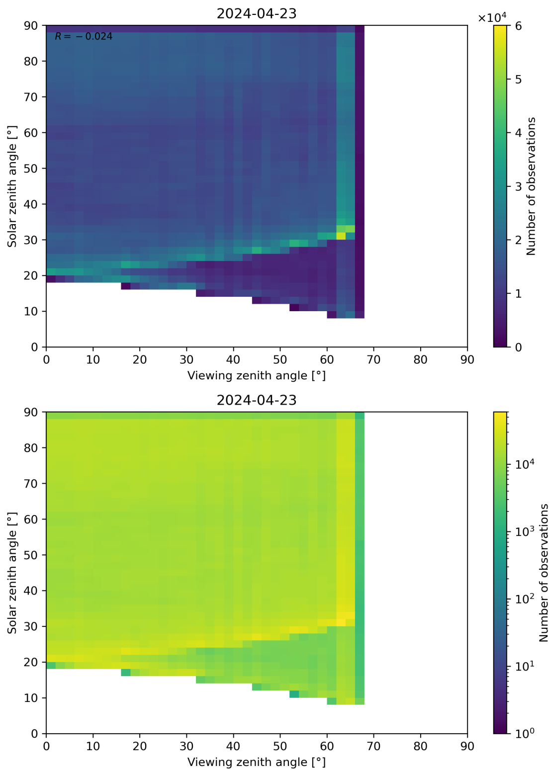
Figure 114: Scatter density plot of “Viewing zenith angle” against “Solar zenith angle” for 2024-04-22 to 2024-04-24.
