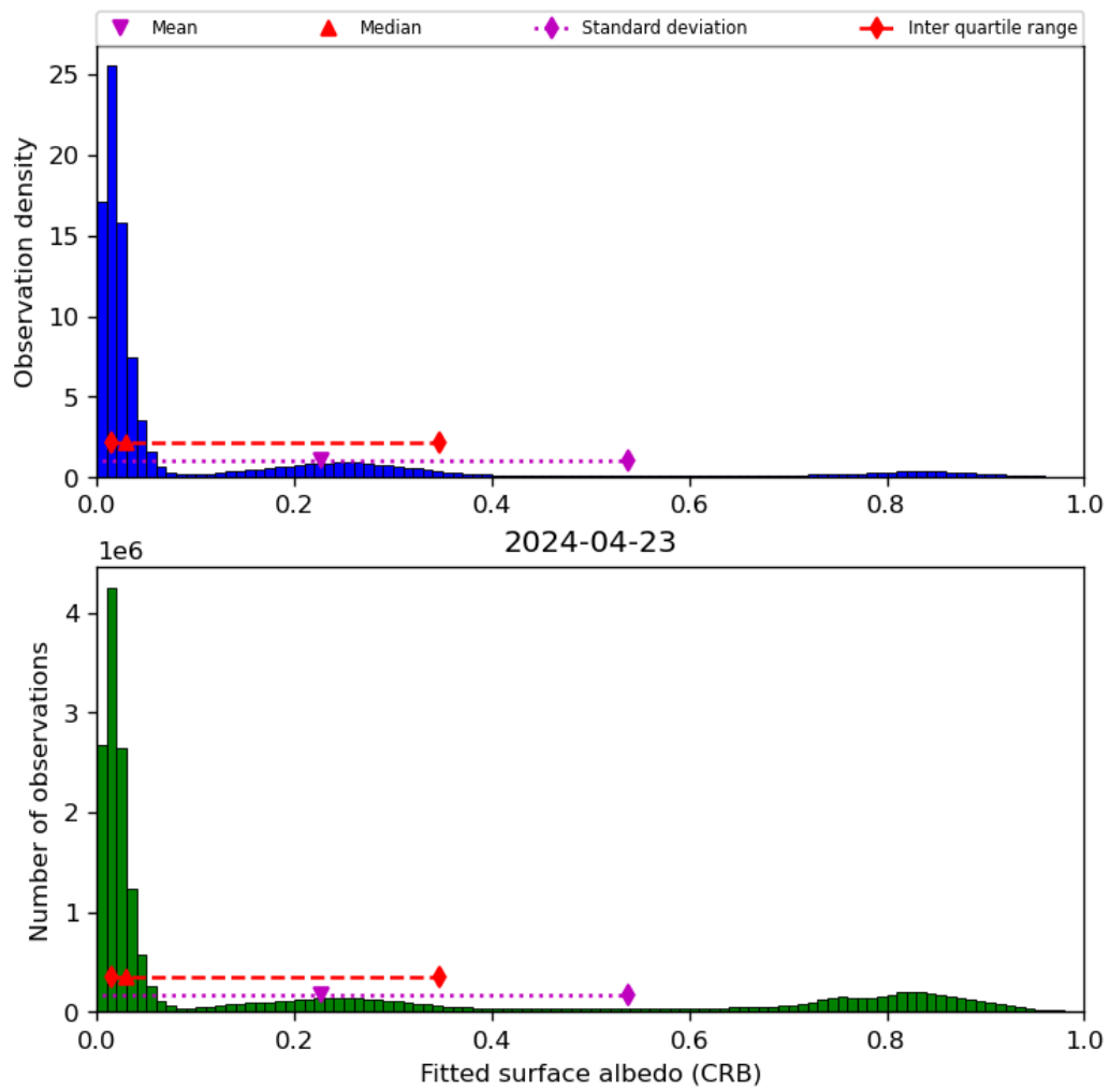
Figure 46: Histogram of “Fitted surface albedo (CRB)” for 2024-04-22 to 2024-04-24
