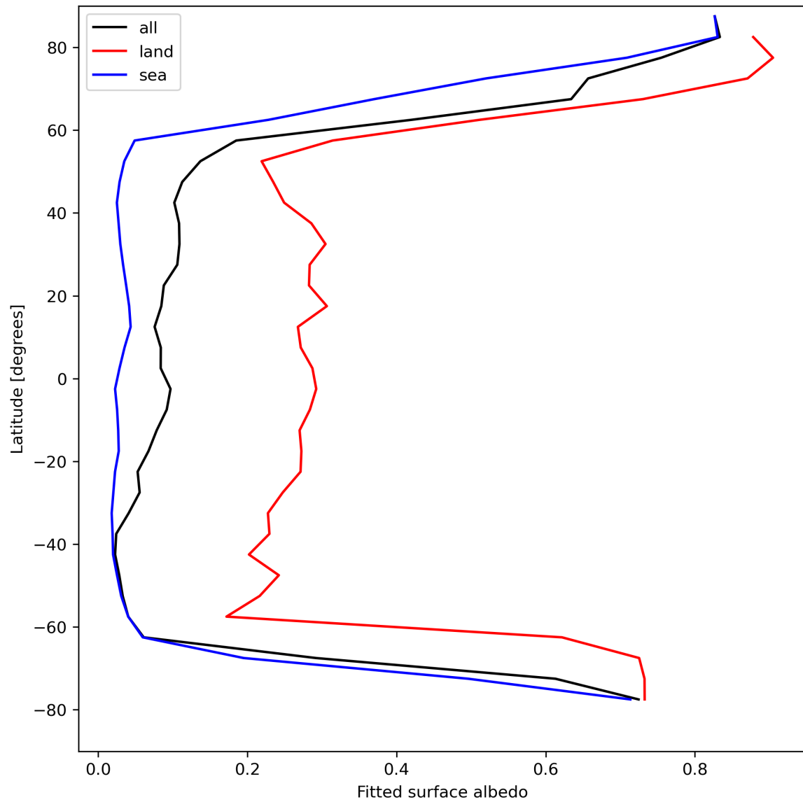
Figure 29: Zonal average of “Fitted surface albedo” for 2024-04-22 to 2024-04-24.
