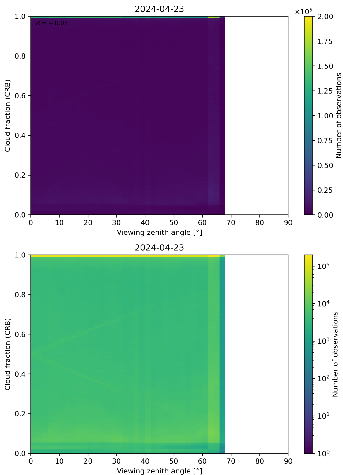
Figure 109: Scatter density plot of “Viewing zenith angle” against “Cloud fraction (CRB)” for 2024-04-22 to 2024-04-24.
