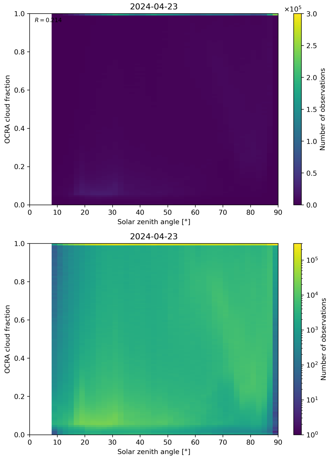
Figure 100: Scatter density plot of “Solar zenith angle” against “OCRA cloud fraction” for 2024-04-22 to 2024-04-24.
