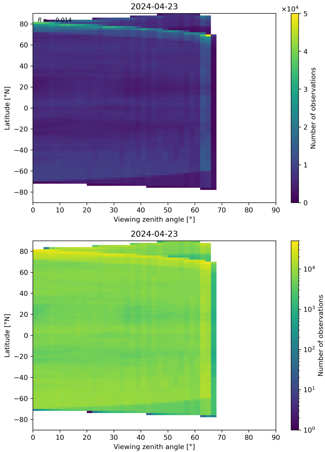
Figure 113: Scatter density plot of “Viewing zenith angle” against “Latitude” for 2024-04-22 to 2024-04-24.
