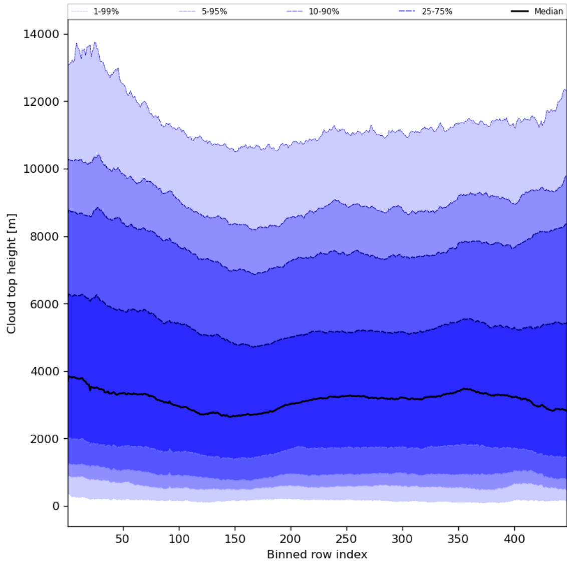
Figure 56: Along track statistics of “Cloud top height” for 2024-04-22 to 2024-04-24
