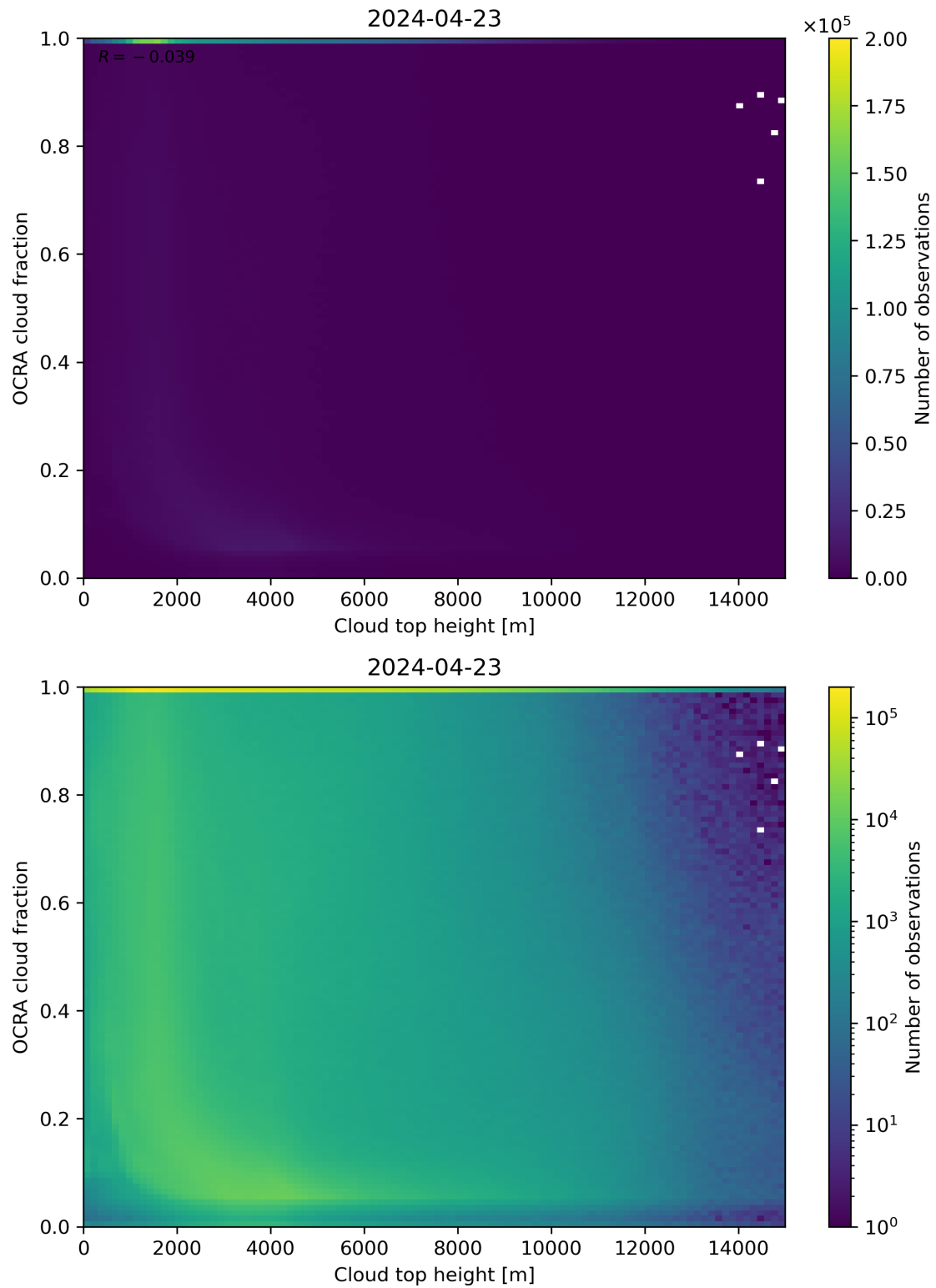
Figure 87: Scatter density plot of “Cloud top height” against “OCRA cloud fraction” for 2024-04-22 to 2024-04-24.
