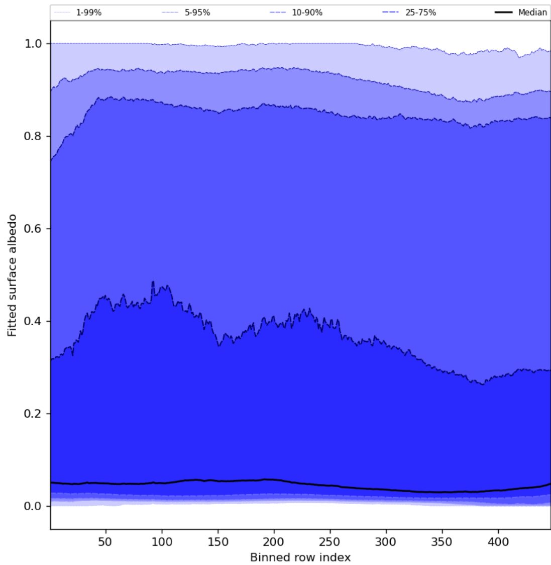
Figure 61: Along track statistics of “Fitted surface albedo” for 2024-04-22 to 2024-04-24
