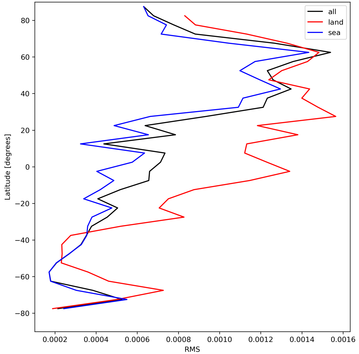
Figure 31: Zonal average of “RMS” for 2024-04-22 to 2024-04-24.
