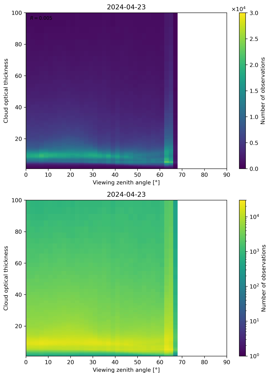
Figure 111: Scatter density plot of “Viewing zenith angle” against “Cloud optical thickness” for 2024-04-22 to 2024-04-24.
