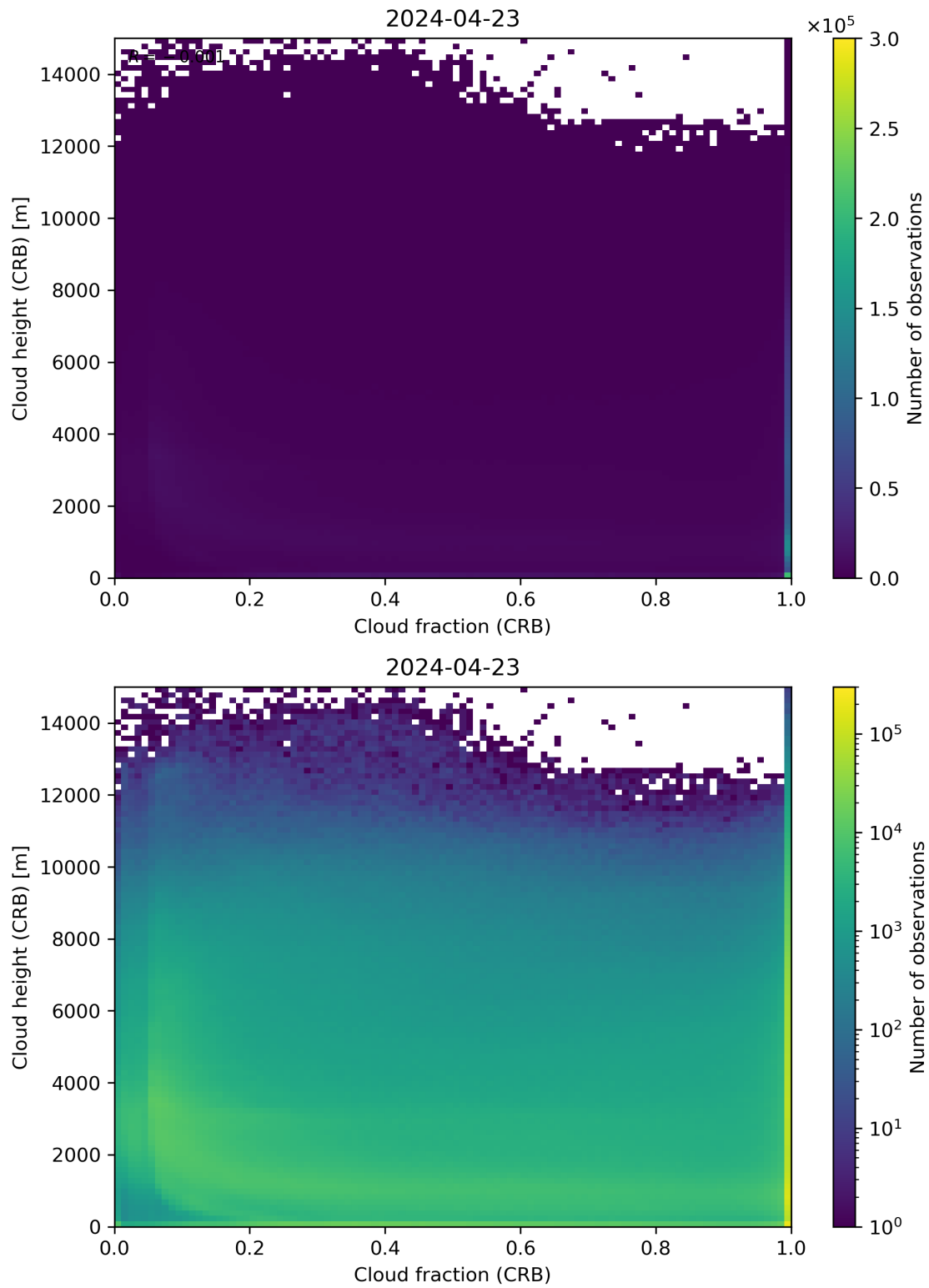
Figure 79: Scatter density plot of “Cloud fraction (CRB)” against “Cloud height (CRB)” for 2024-04-22 to 2024-04-24.
