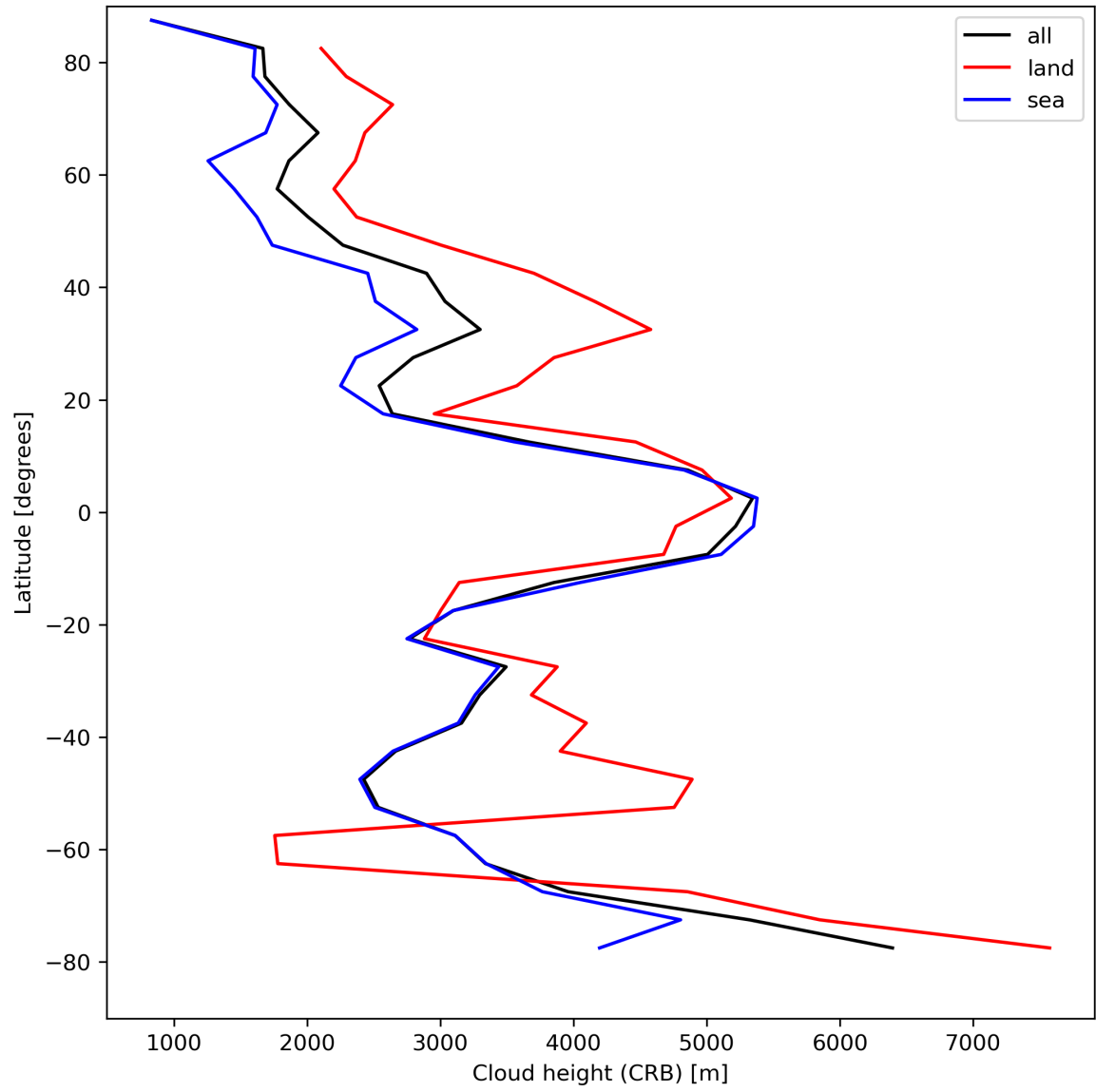
Figure 27: Zonal average of “Cloud height (CRB)” for 2024-04-22 to 2024-04-24.
