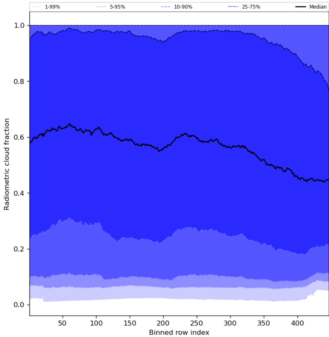
Figure 55: Along track statistics of “Radiometric cloud fraction” for 2024-04-22 to 2024-04-24
