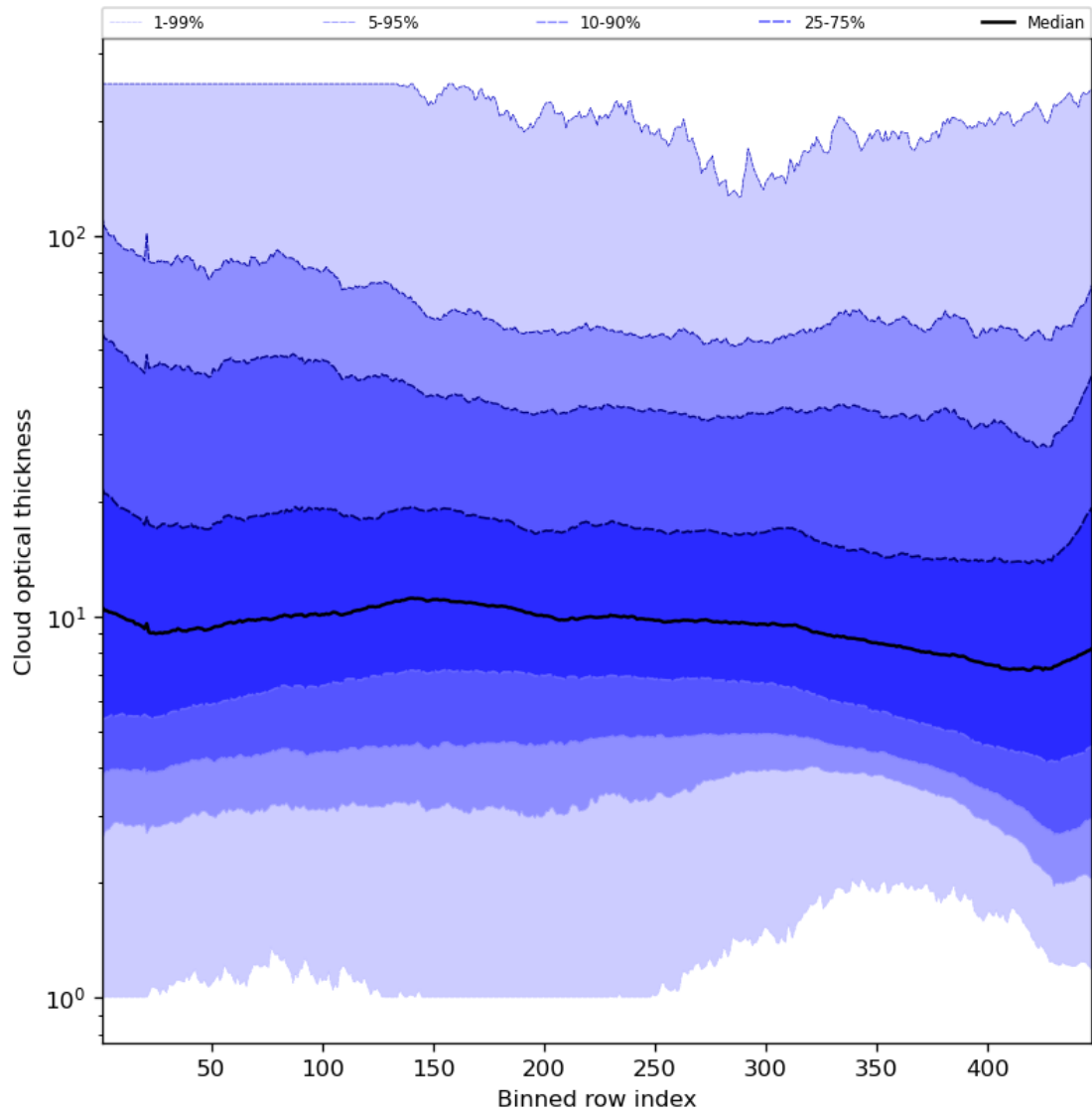
Figure 57: Along track statistics of “Cloud optical thickness” for 2024-04-23 to 2024-04-25
