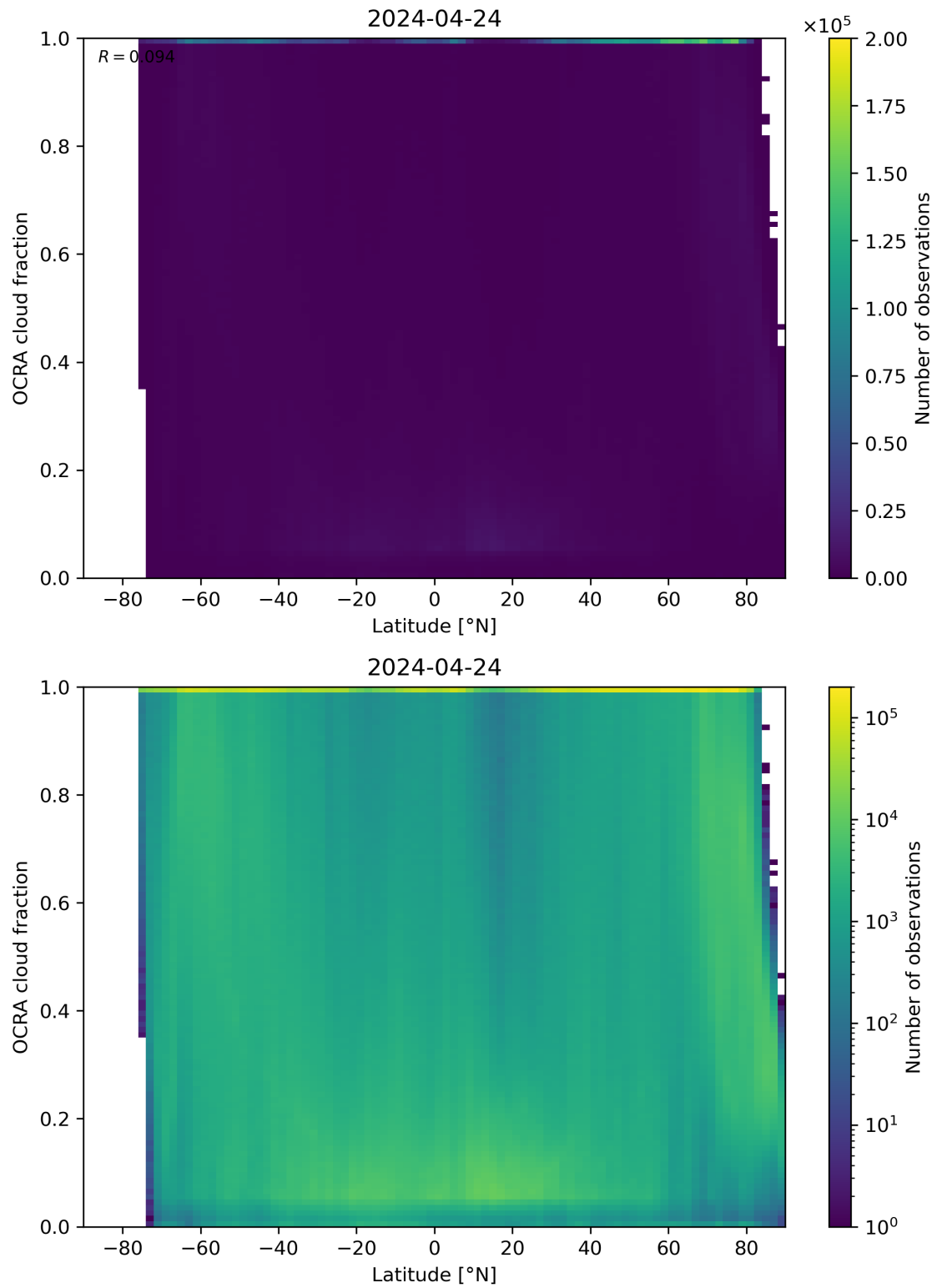
Figure 93: Scatter density plot of “Latitude” against “OCRA cloud fraction” for 2024-04-23 to 2024-04-25.
