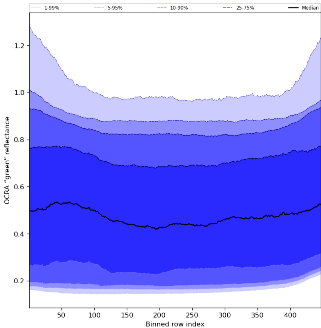
Figure 68: Along track statistics of “OCRA “green” reflectance” for 2024-04-23 to 2024-04-25
