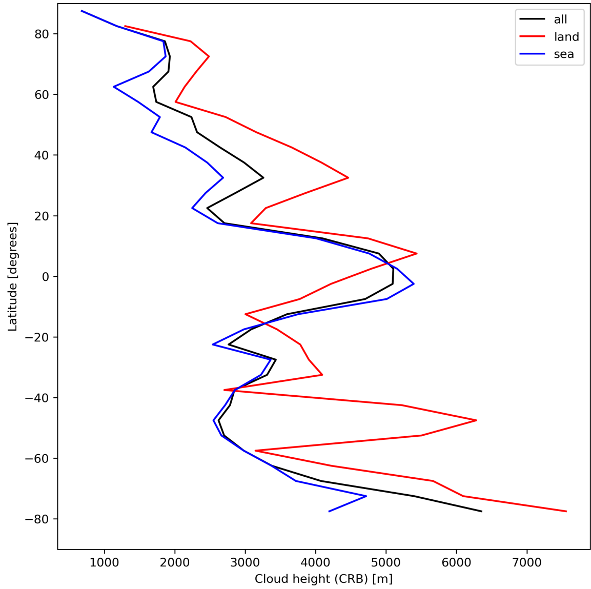
Figure 27: Zonal average of “Cloud height (CRB)” for 2024-04-23 to 2024-04-25.
