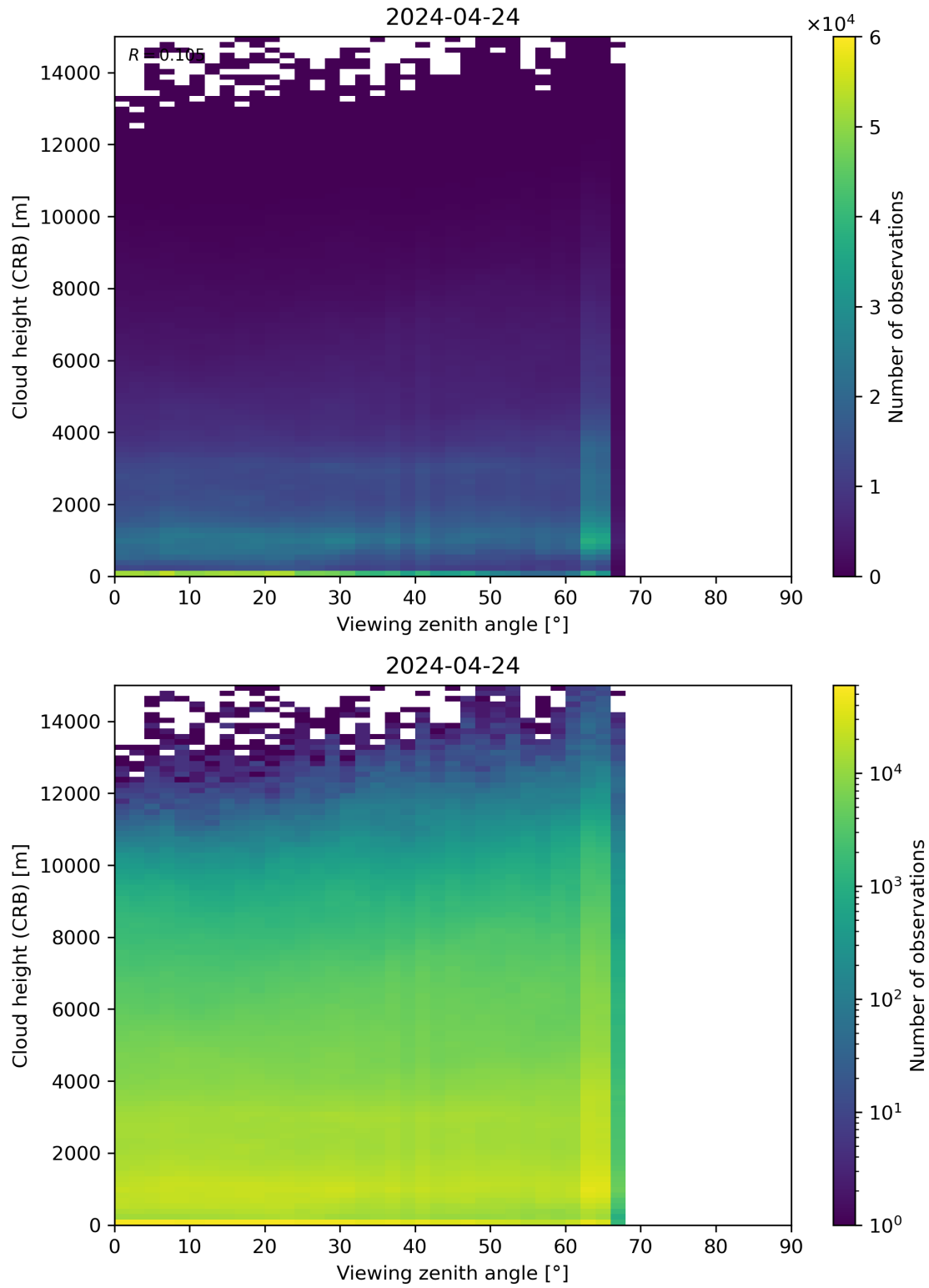
Figure 110: Scatter density plot of “Viewing zenith angle” against “Cloud height (CRB)” for 2024-04-23 to 2024-04-25.
