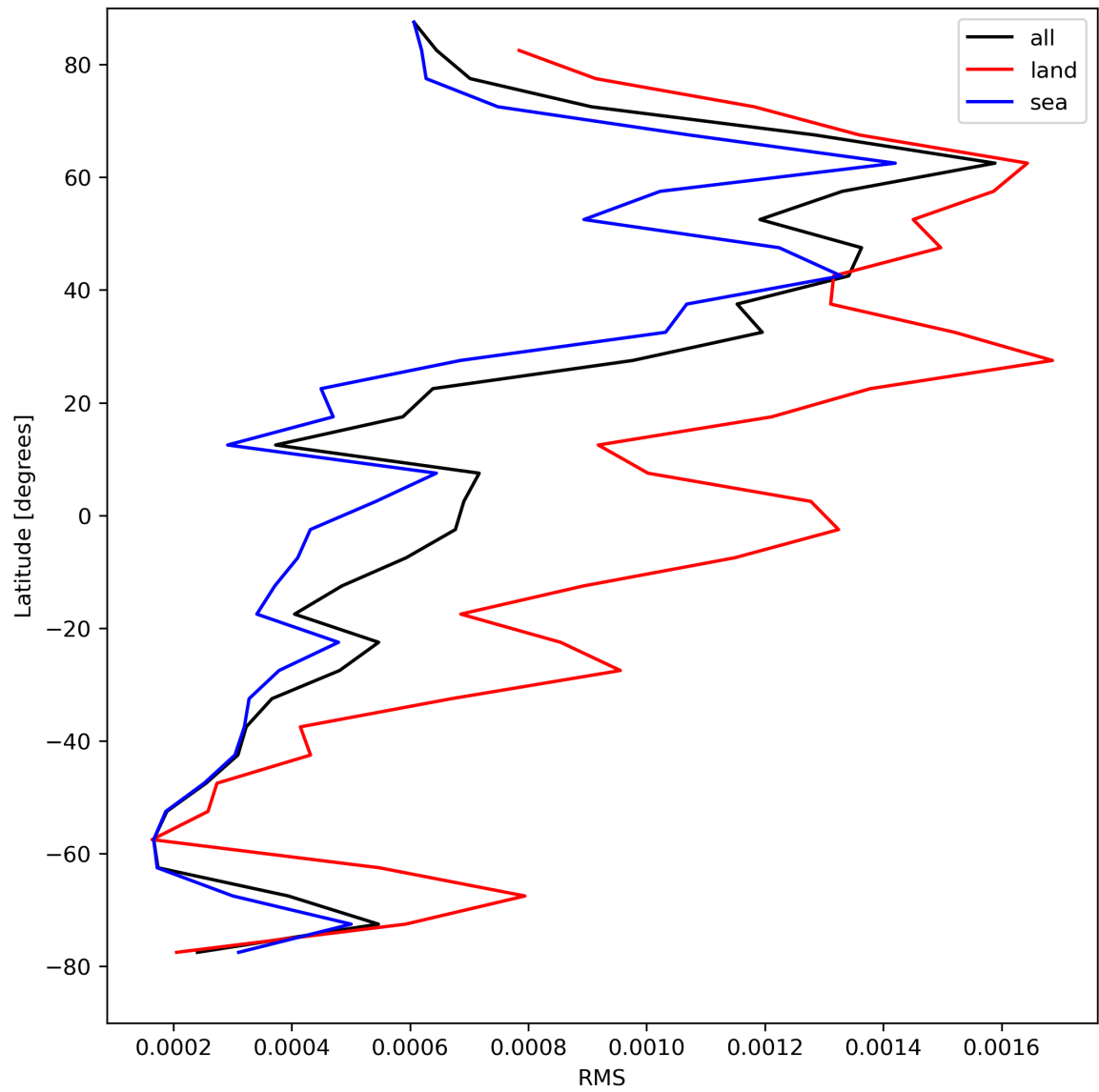
Figure 31: Zonal average of “RMS” for 2024-04-23 to 2024-04-25.
