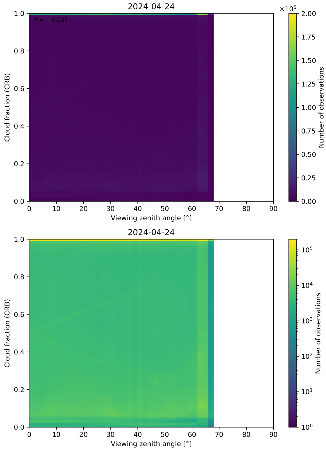
Figure 109: Scatter density plot of “Viewing zenith angle” against “Cloud fraction (CRB)” for 2024-04-23 to 2024-04-25.
