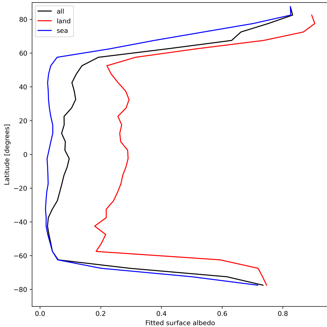
Figure 29: Zonal average of “Fitted surface albedo” for 2024-04-23 to 2024-04-25.
