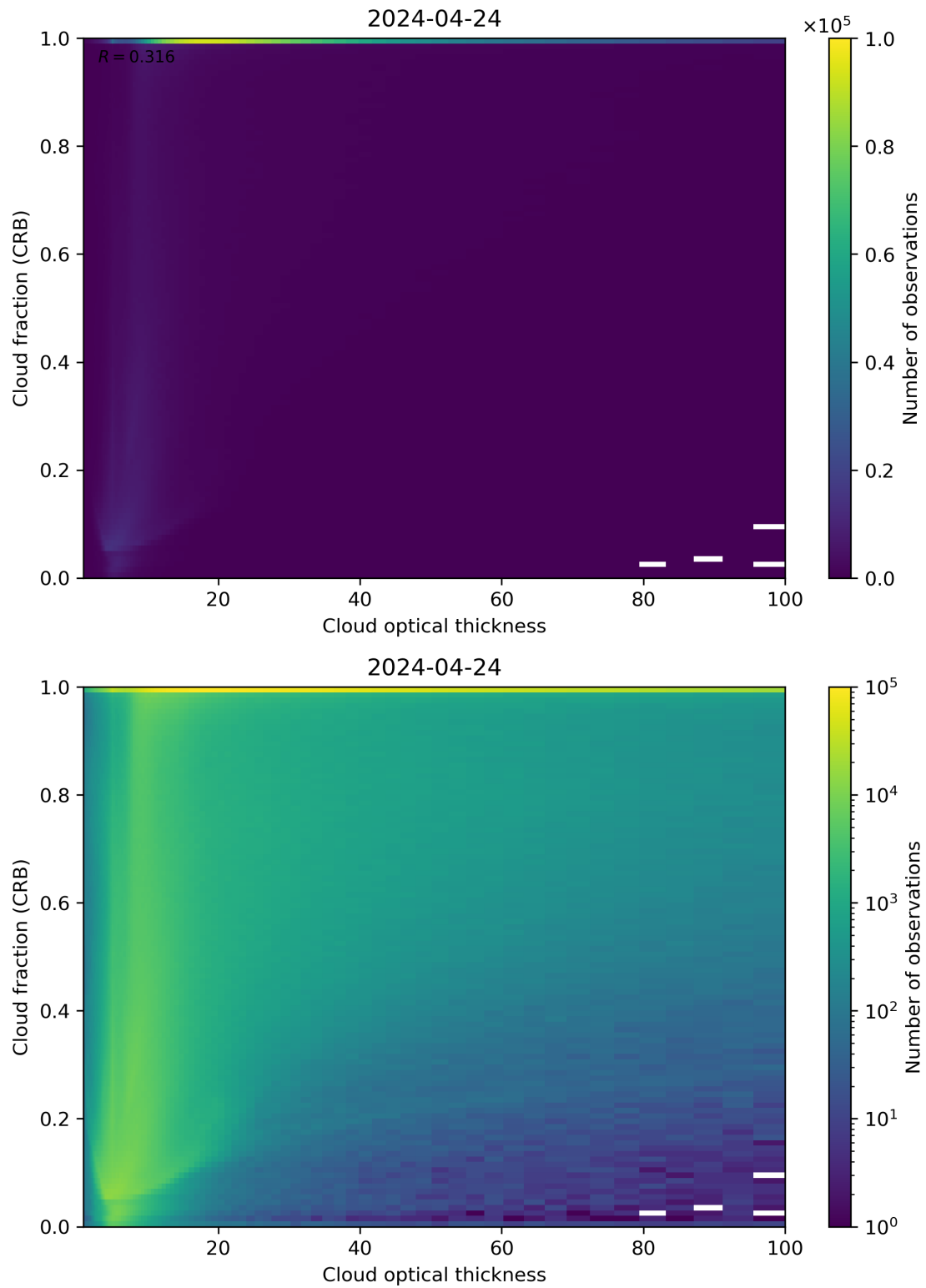
Figure 84: Scatter density plot of “Cloud optical thickness” against “Cloud fraction (CRB)” for 2024-04-23 to 2024-04-25.
