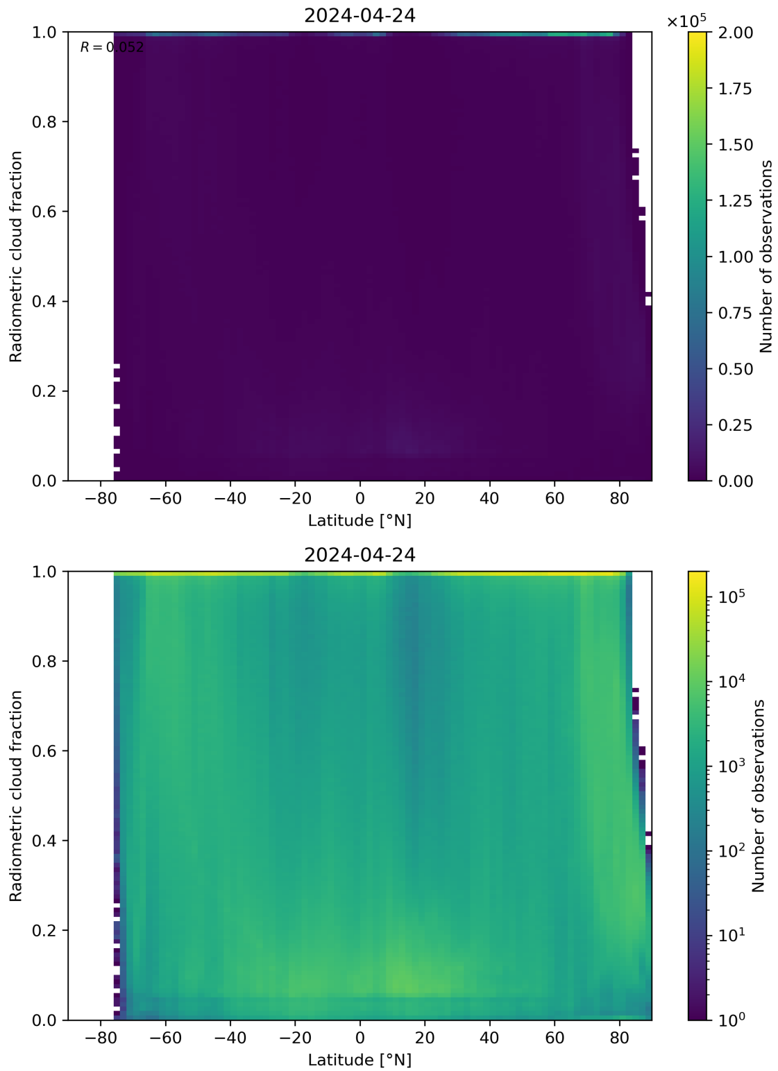
Figure 92: Scatter density plot of “Latitude” against “Radiometric cloud fraction” for 2024-04-23 to 2024-04-25.
