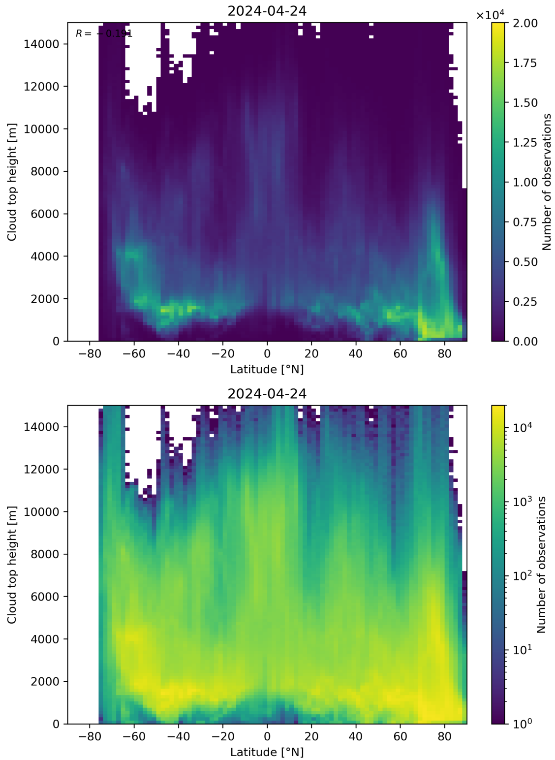
Figure 97: Scatter density plot of “Latitude” against “Cloud top height” for 2024-04-23 to 2024-04-25.
