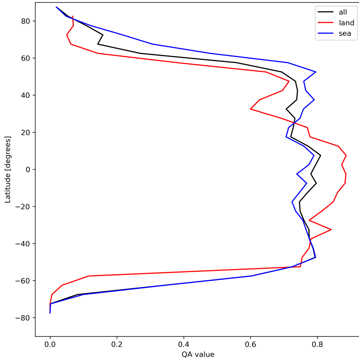
Figure 22: Zonal average of “QA value” for 2024-04-23 to 2024-04-25.
