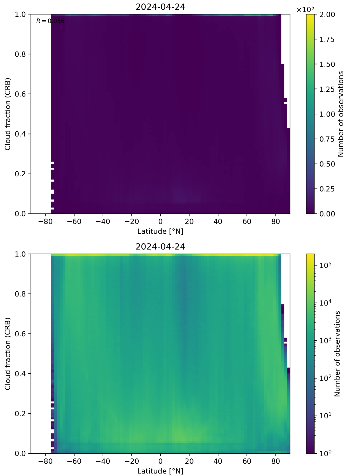
Figure 94: Scatter density plot of “Latitude” against “Cloud fraction (CRB)” for 2024-04-23 to 2024-04-25.
