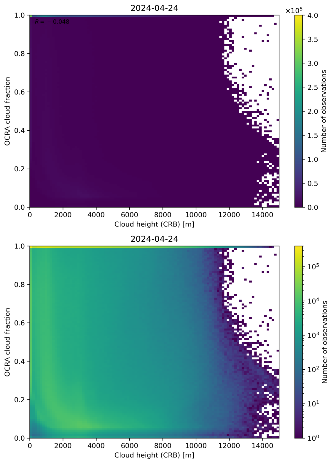
Figure 81: Scatter density plot of “Cloud height (CRB)” against “OCRA cloud fraction” for 2024-04-23 to 2024-04-25.
