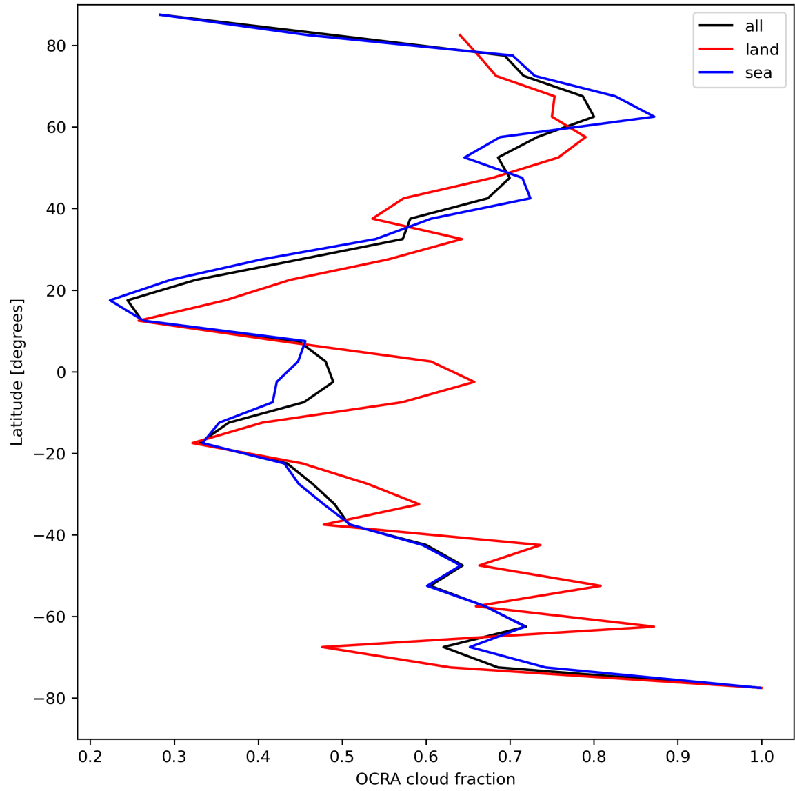
Figure 34: Zonal average of “OCRA cloud fraction” for 2024-04-23 to 2024-04-25.
