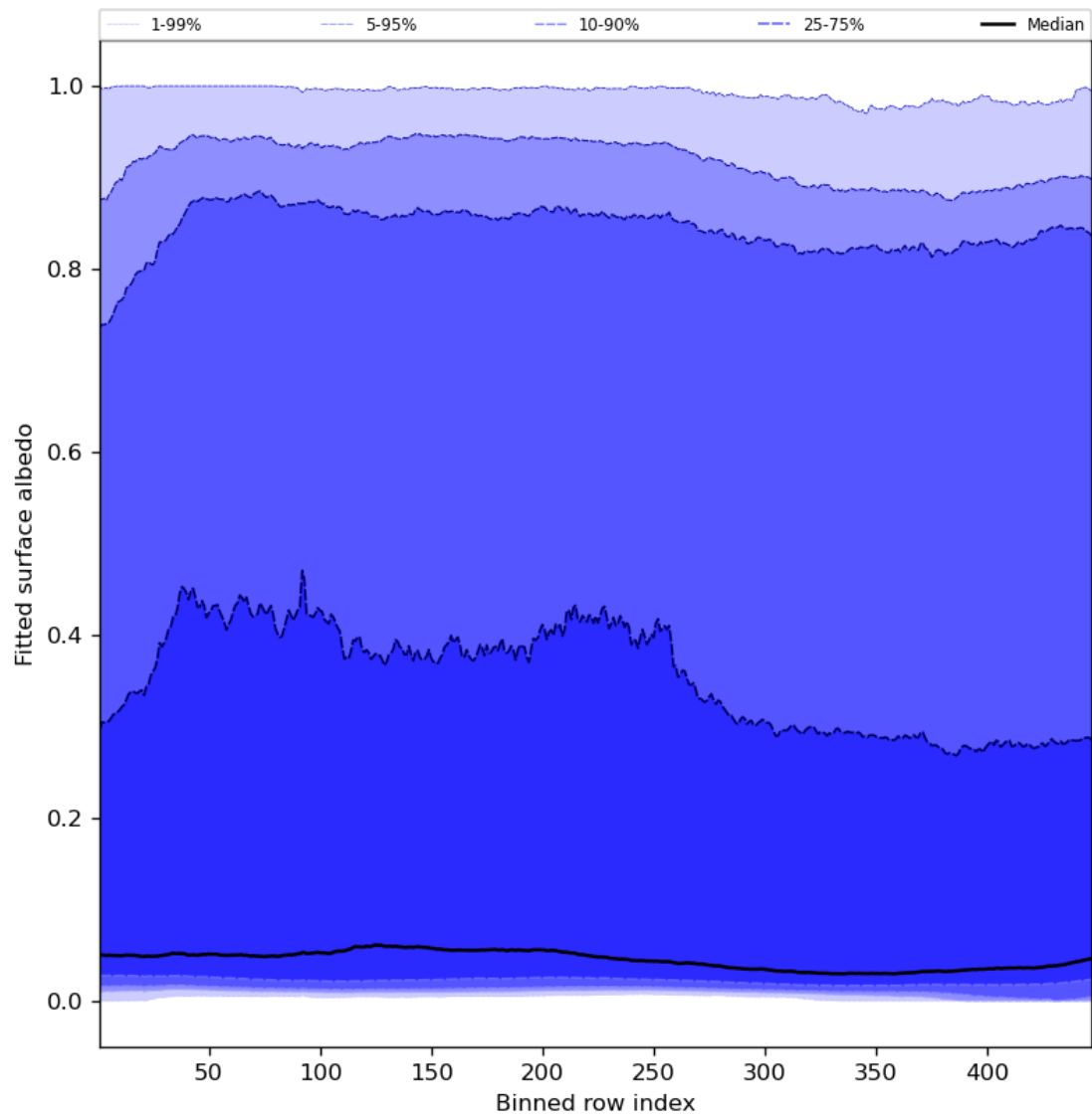
Figure 61: Along track statistics of “Fitted surface albedo” for 2024-04-23 to 2024-04-25
