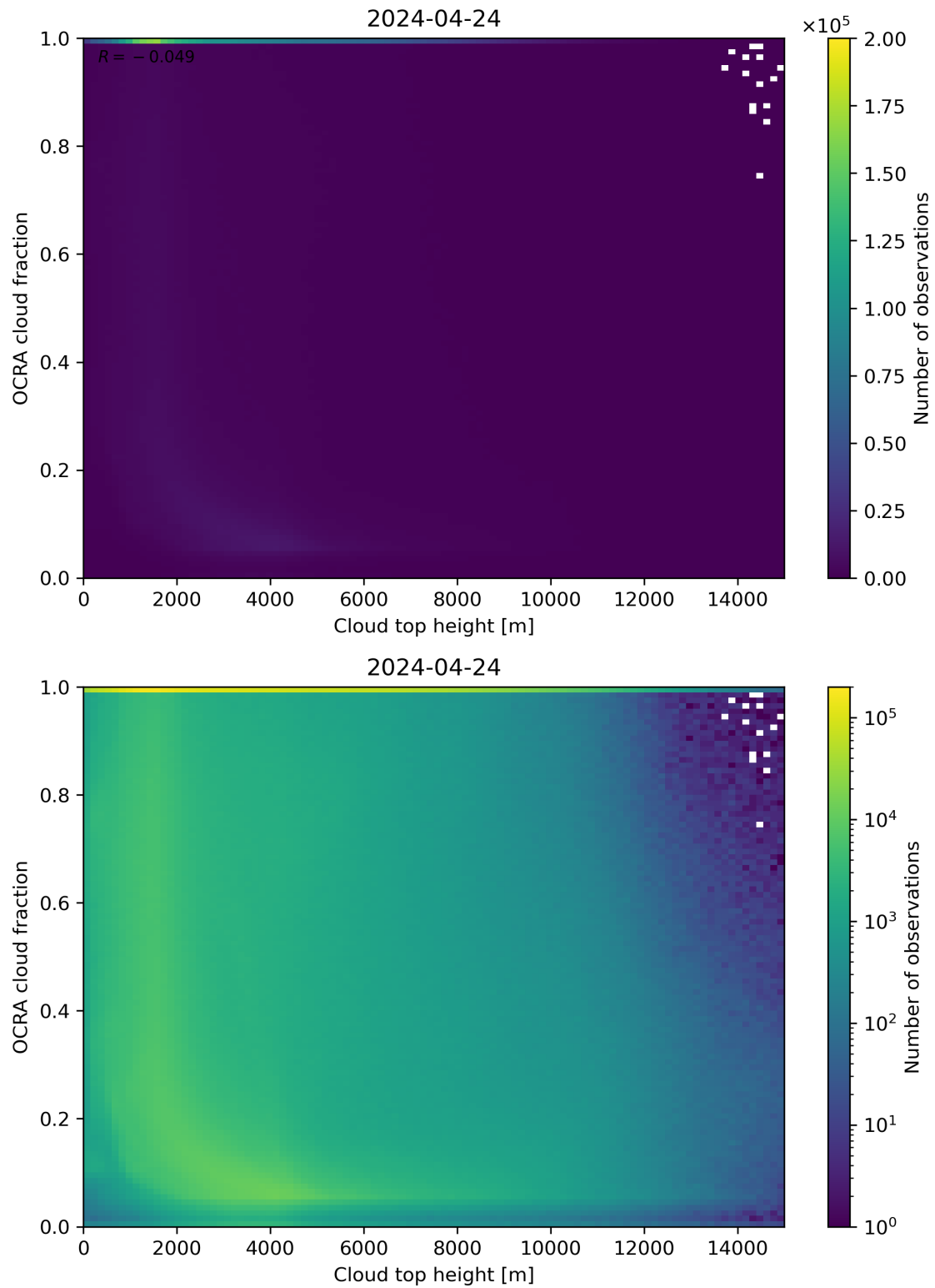
Figure 87: Scatter density plot of “Cloud top height” against “OCRA cloud fraction” for 2024-04-23 to 2024-04-25.
