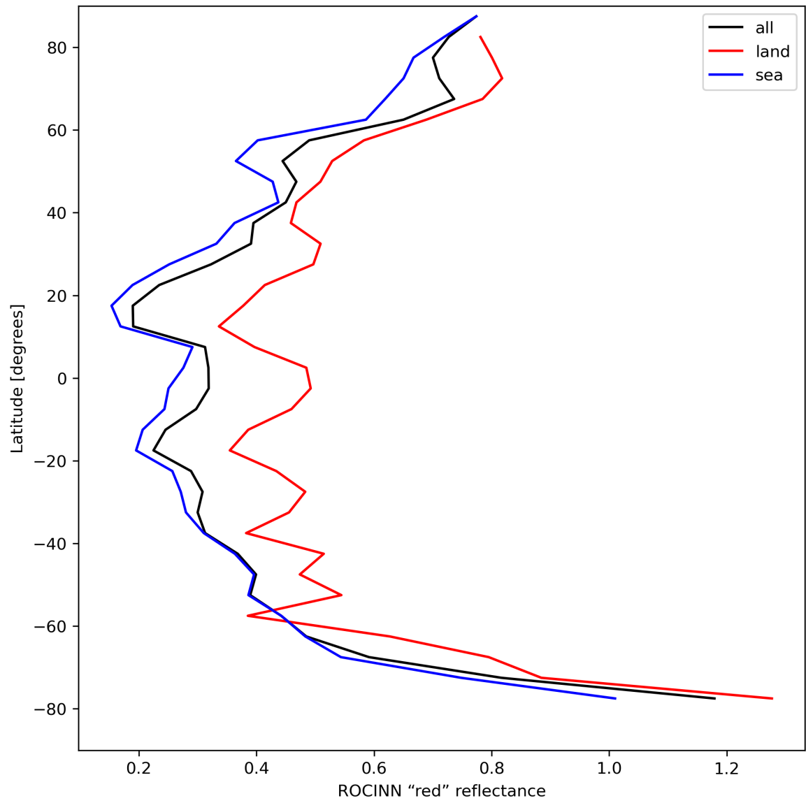
Figure 37: Zonal average of “ROCINN “red” reflectance” for 2024-04-23 to 2024-04-25.
