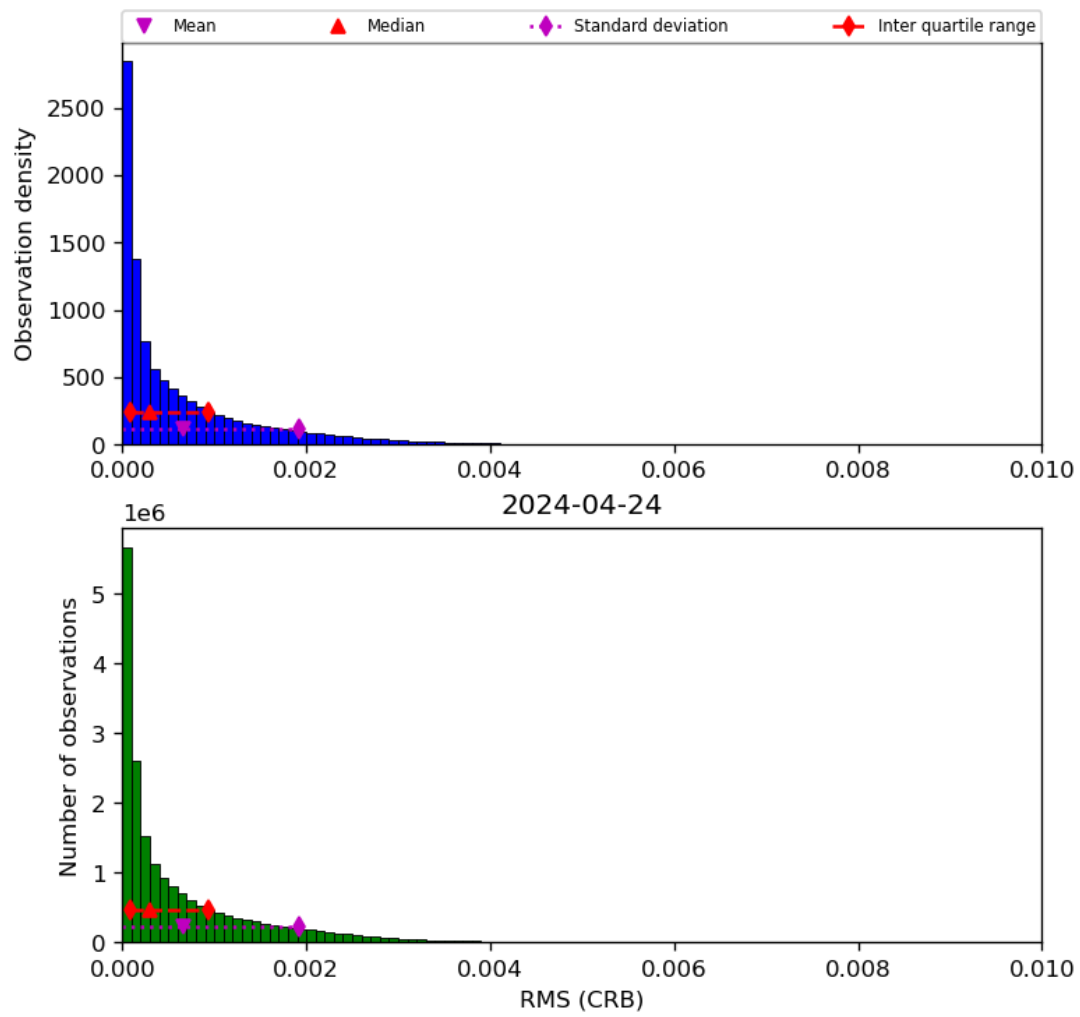
Figure 48: Histogram of “RMS (CRB)” for 2024-04-23 to 2024-04-25
