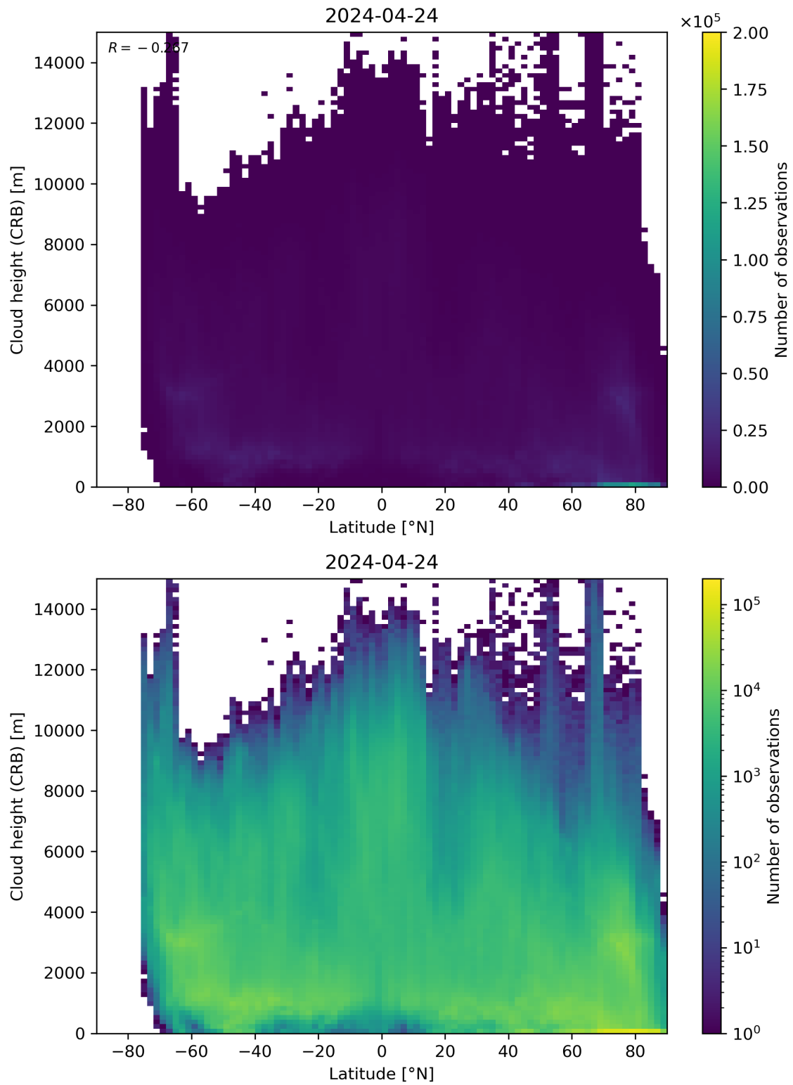
Figure 95: Scatter density plot of “Latitude” against “Cloud height (CRB)” for 2024-04-23 to 2024-04-25.
