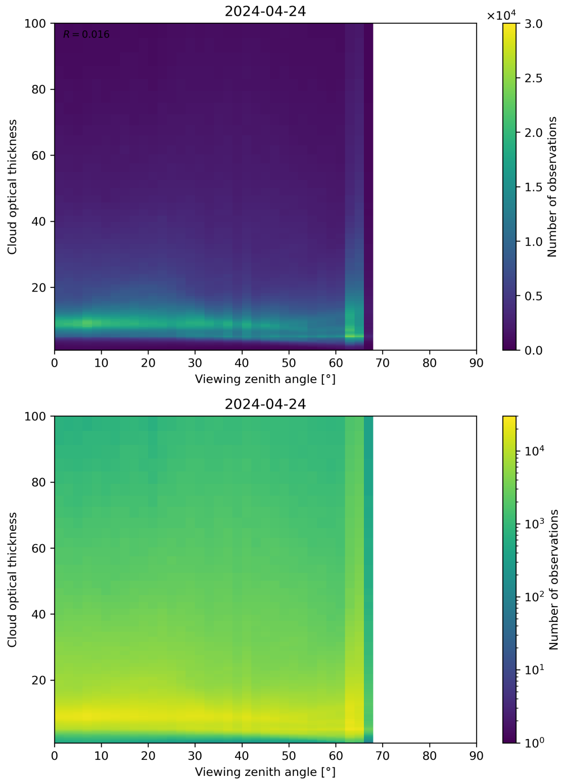
Figure 111: Scatter density plot of “Viewing zenith angle” against “Cloud optical thickness” for 2024-04-23 to 2024-04-25.
