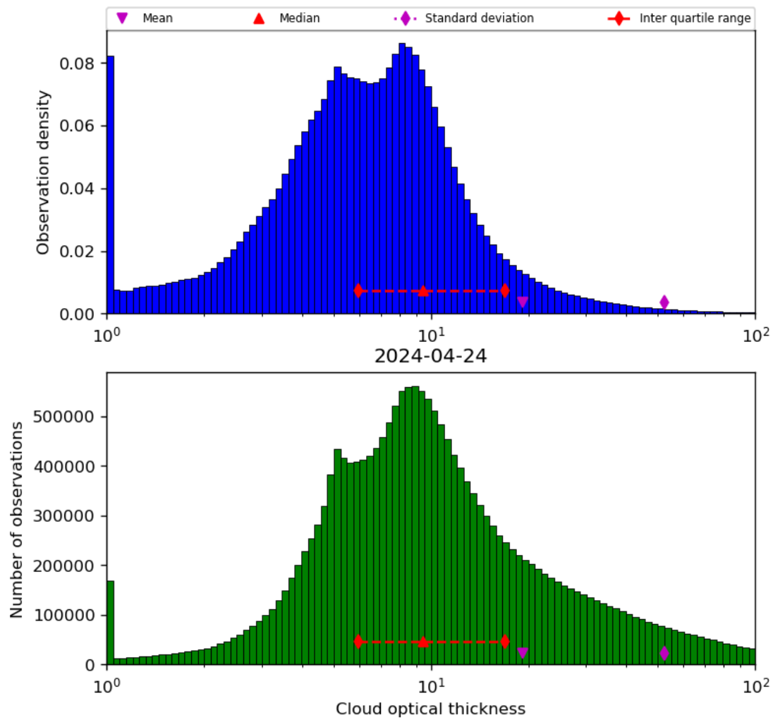
Figure 41: Histogram of “Cloud optical thickness” for 2024-04-23 to 2024-04-25
