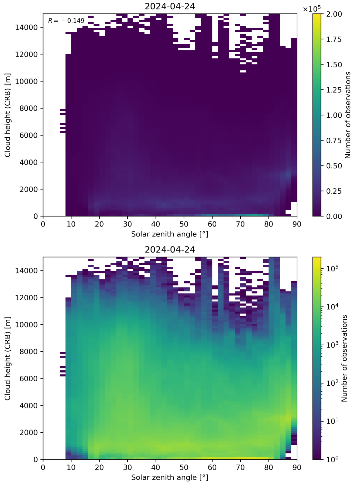
Figure 102: Scatter density plot of “Solar zenith angle” against “Cloud height (CRB)” for 2024-04-23 to 2024-04-25.
