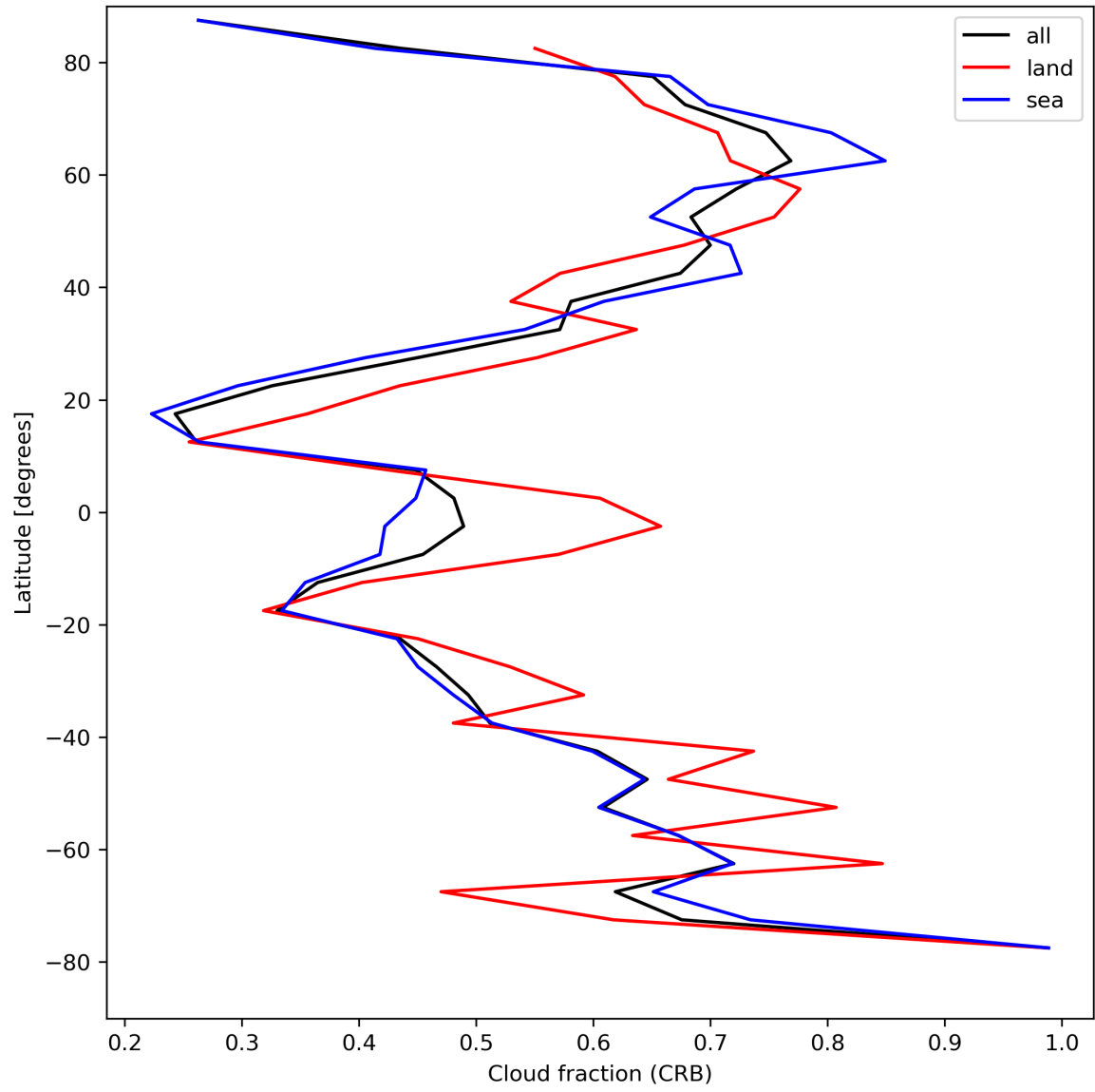
Figure 26: Zonal average of “Cloud fraction (CRB)” for 2024-04-23 to 2024-04-25.
