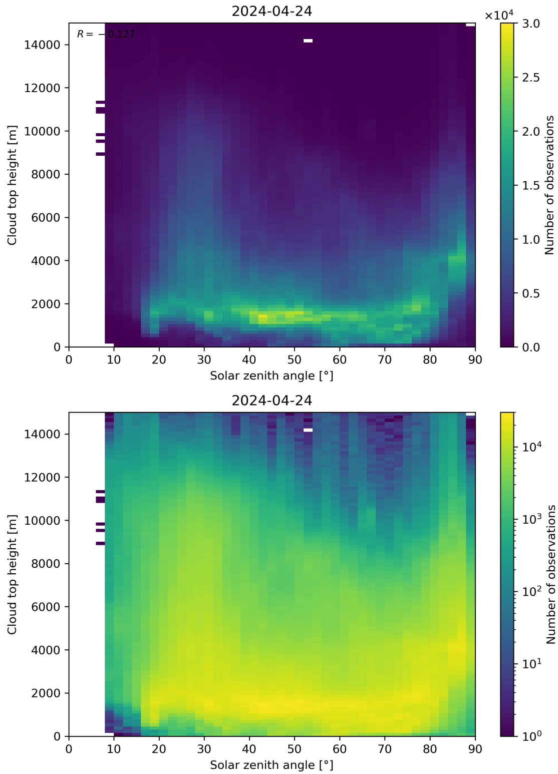
Figure 104: Scatter density plot of “Solar zenith angle” against “Cloud top height” for 2024-04-23 to 2024-04-25.
