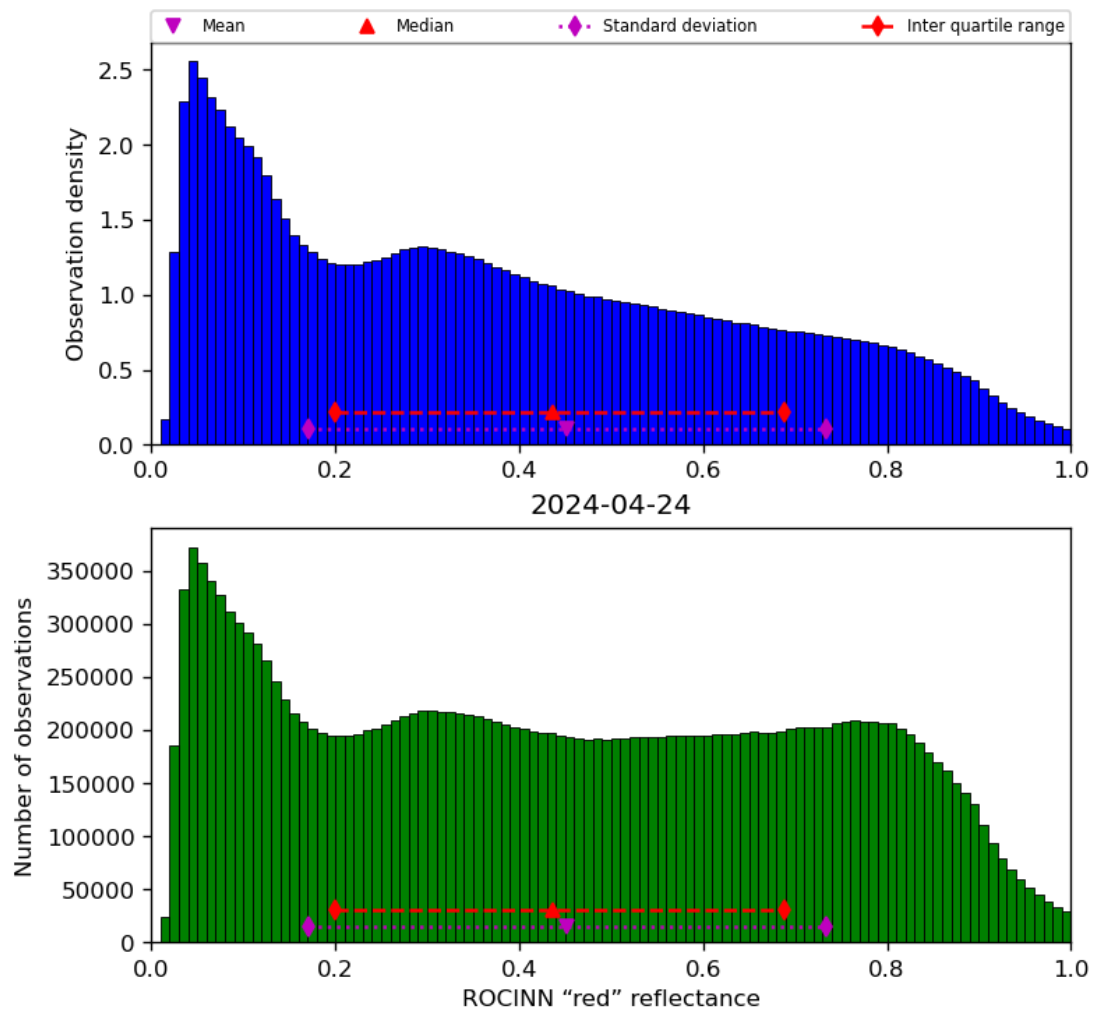
Figure 53: Histogram of “ROCINN “red” reflectance” for 2024-04-23 to 2024-04-25
