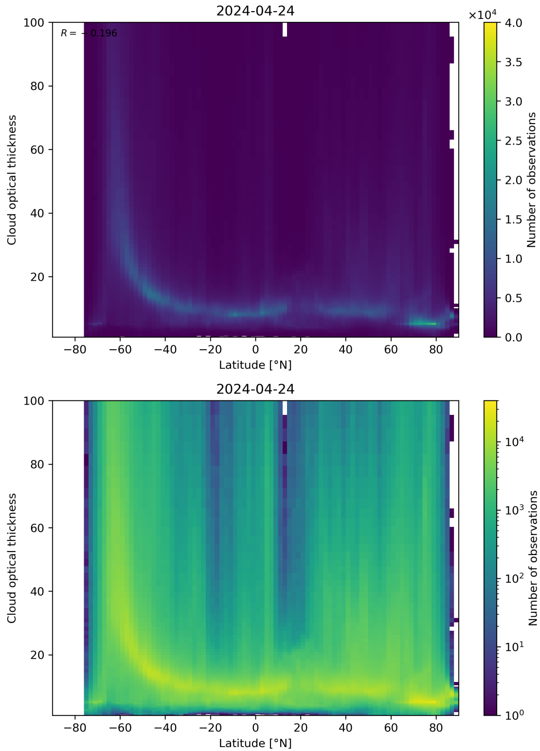
Figure 96: Scatter density plot of “Latitude” against “Cloud optical thickness” for 2024-04-23 to 2024-04-25.
