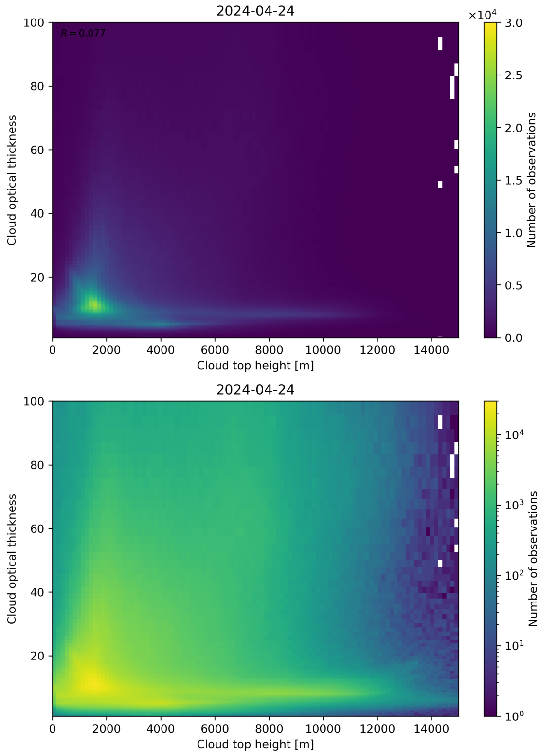
Figure 90: Scatter density plot of “Cloud top height” against “Cloud optical thickness” for 2024-04-23 to 2024-04-25.
