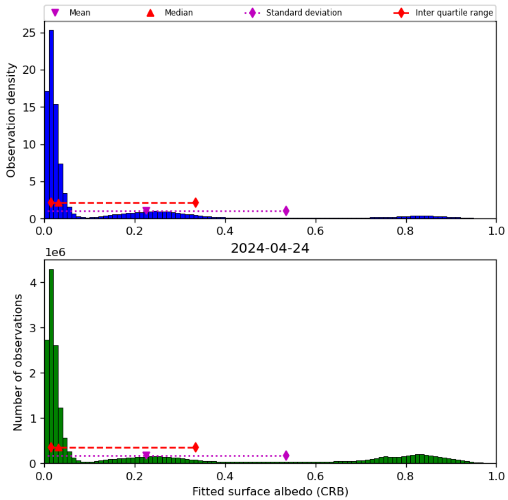
Figure 46: Histogram of “Fitted surface albedo (CRB)” for 2024-04-23 to 2024-04-25
