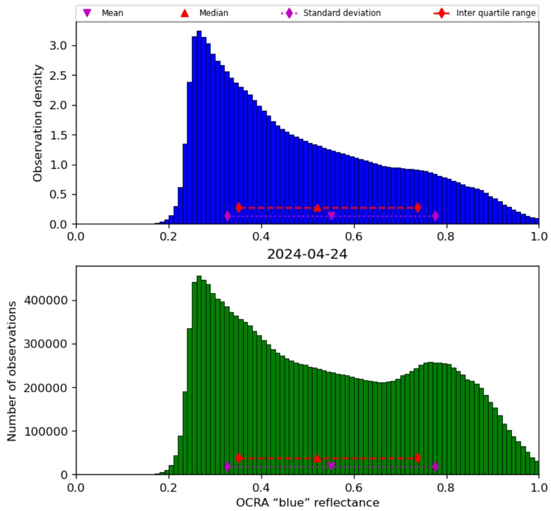
Figure 51: Histogram of “OCRA “blue” reflectance” for 2024-04-23 to 2024-04-25
