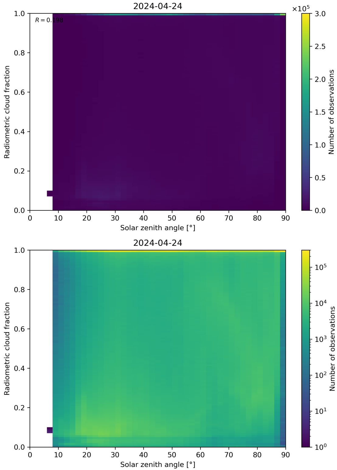
Figure 99: Scatter density plot of “Solar zenith angle” against “Radiometric cloud fraction” for 2024-04-23 to 2024-04-25.
