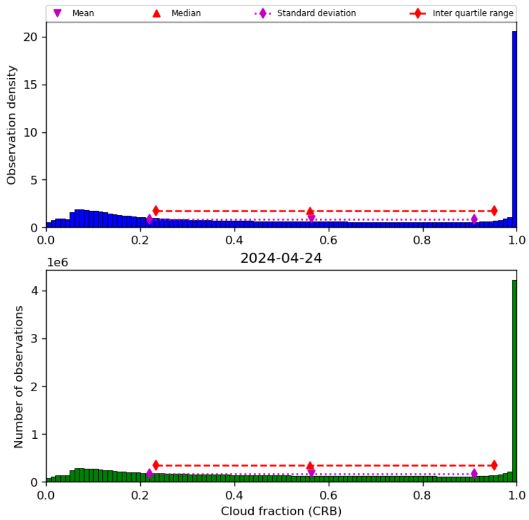
Figure 42: Histogram of “Cloud fraction (CRB)” for 2024-04-23 to 2024-04-25
