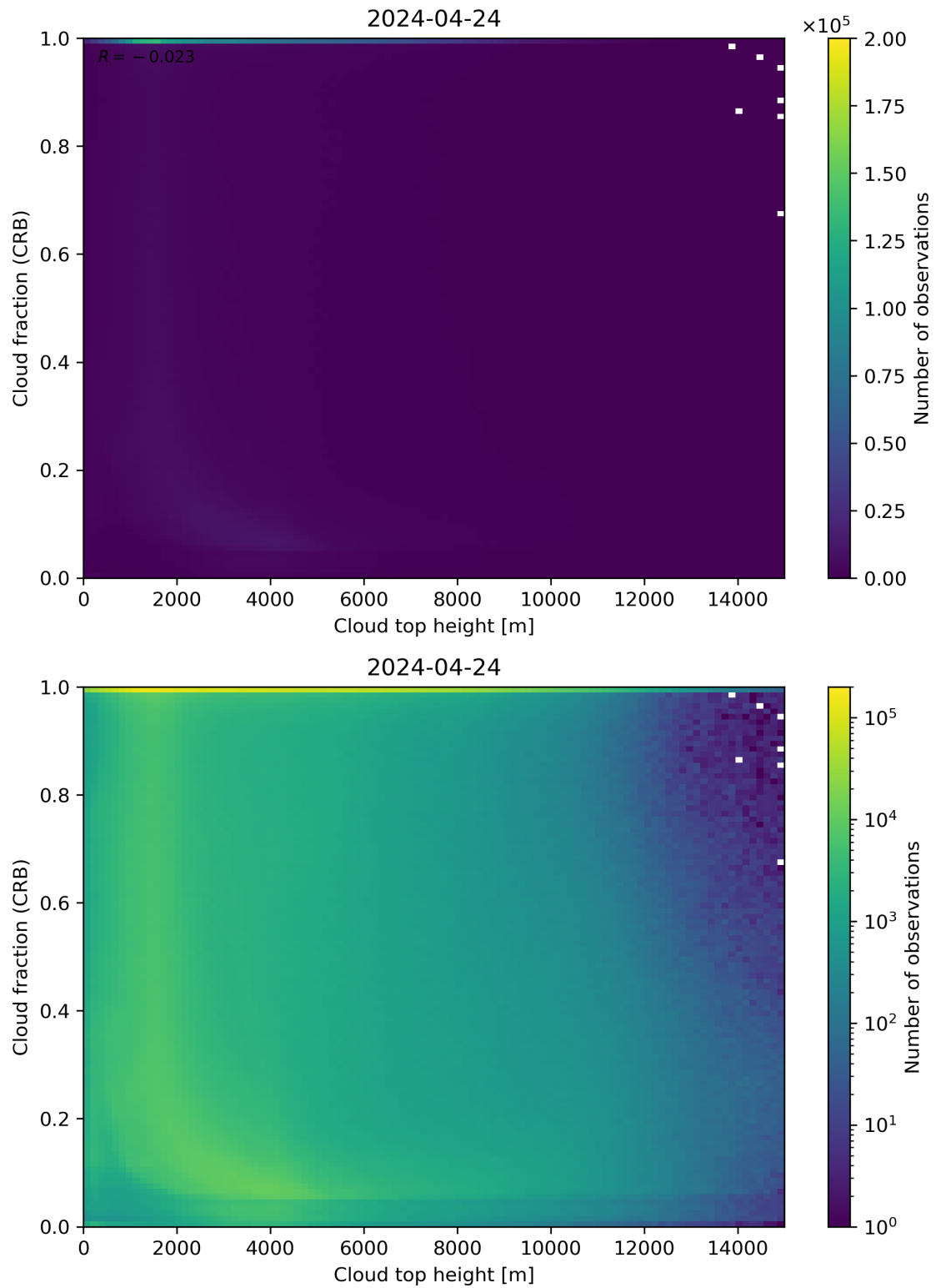
Figure 88: Scatter density plot of “Cloud top height” against “Cloud fraction (CRB)” for 2024-04-23 to 2024-04-25.
