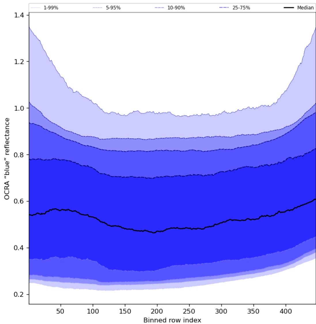
Figure 67: Along track statistics of “OCRA “blue” reflectance” for 2024-04-23 to 2024-04-25
