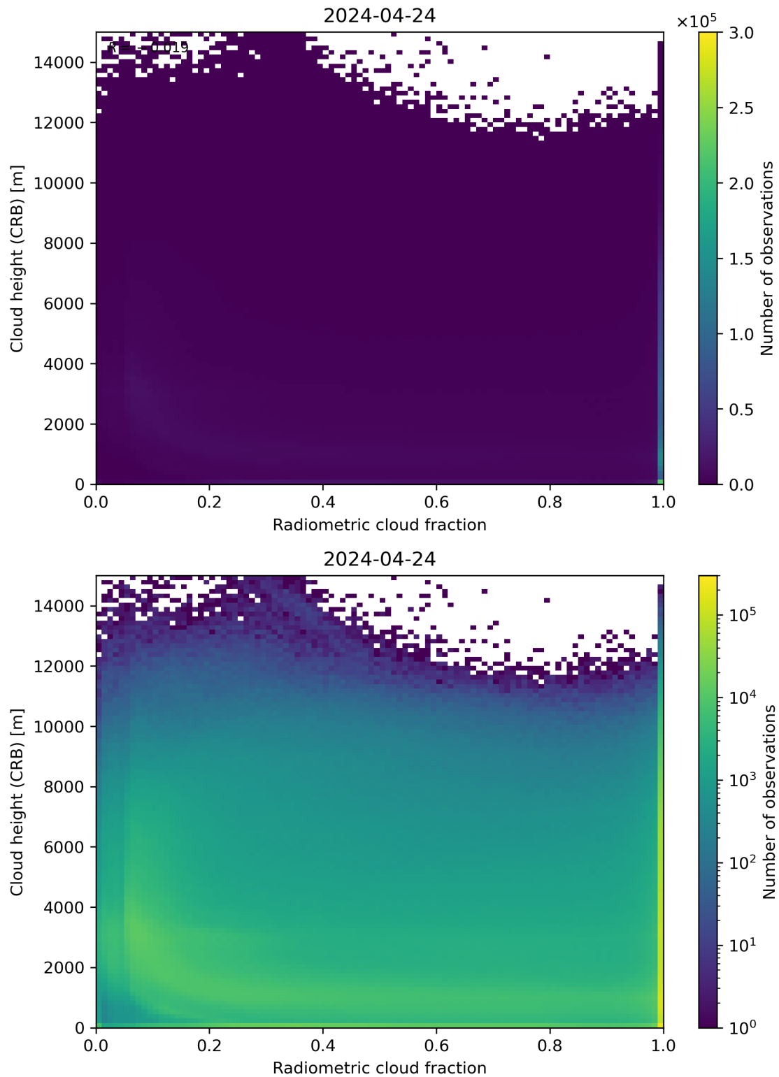
Figure 74: Scatter density plot of “Radiometric cloud fraction” against “Cloud height (CRB)” for 2024-04-23 to 2024-04-25.
