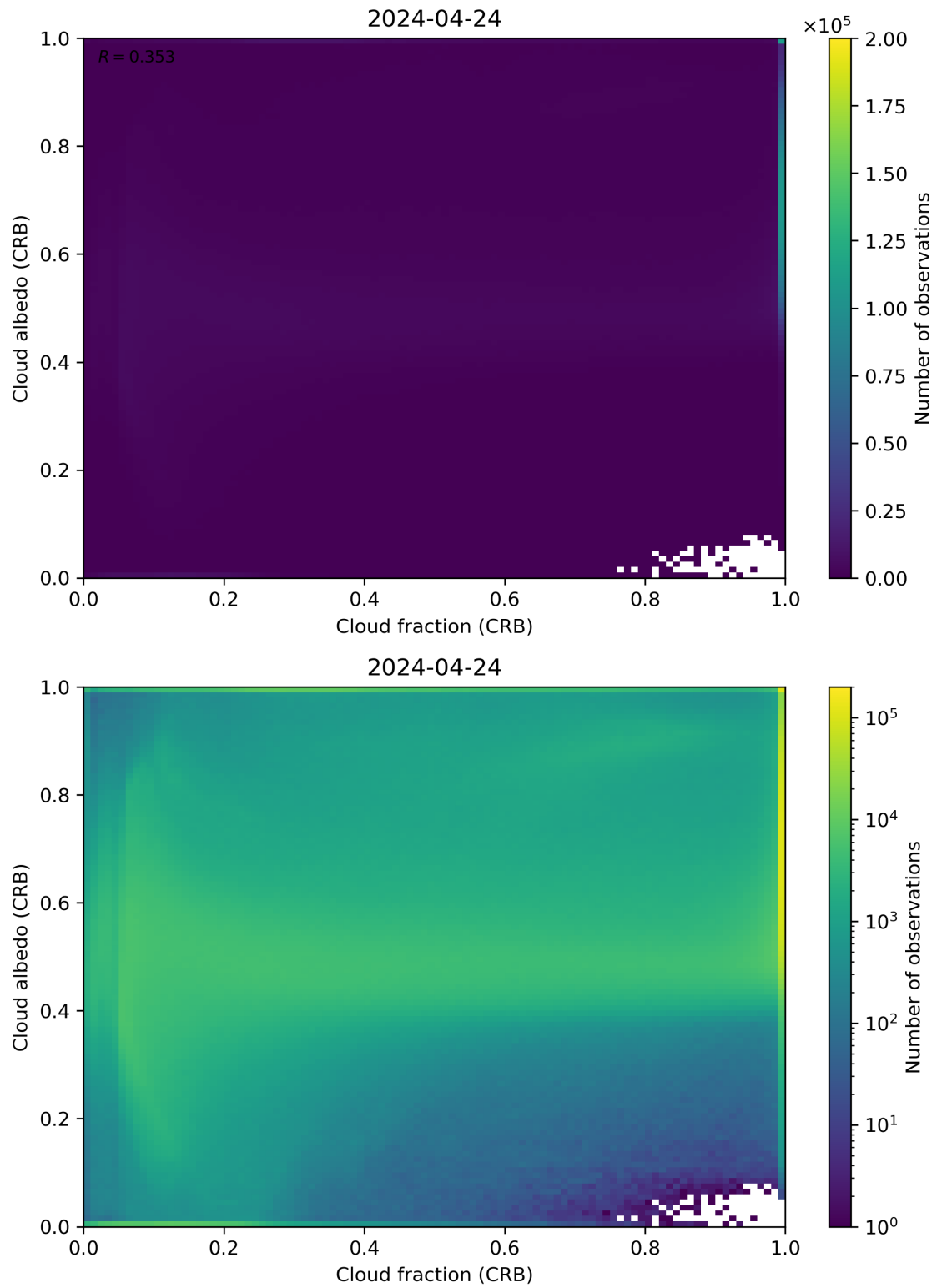
Figure 77: Scatter density plot of “Cloud fraction (CRB)” against “Cloud albedo (CRB)” for 2024-04-23 to 2024-04-25.
