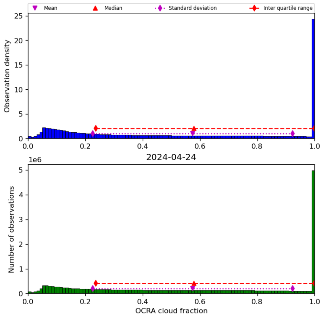
Figure 50: Histogram of “OCRA cloud fraction” for 2024-04-23 to 2024-04-25
