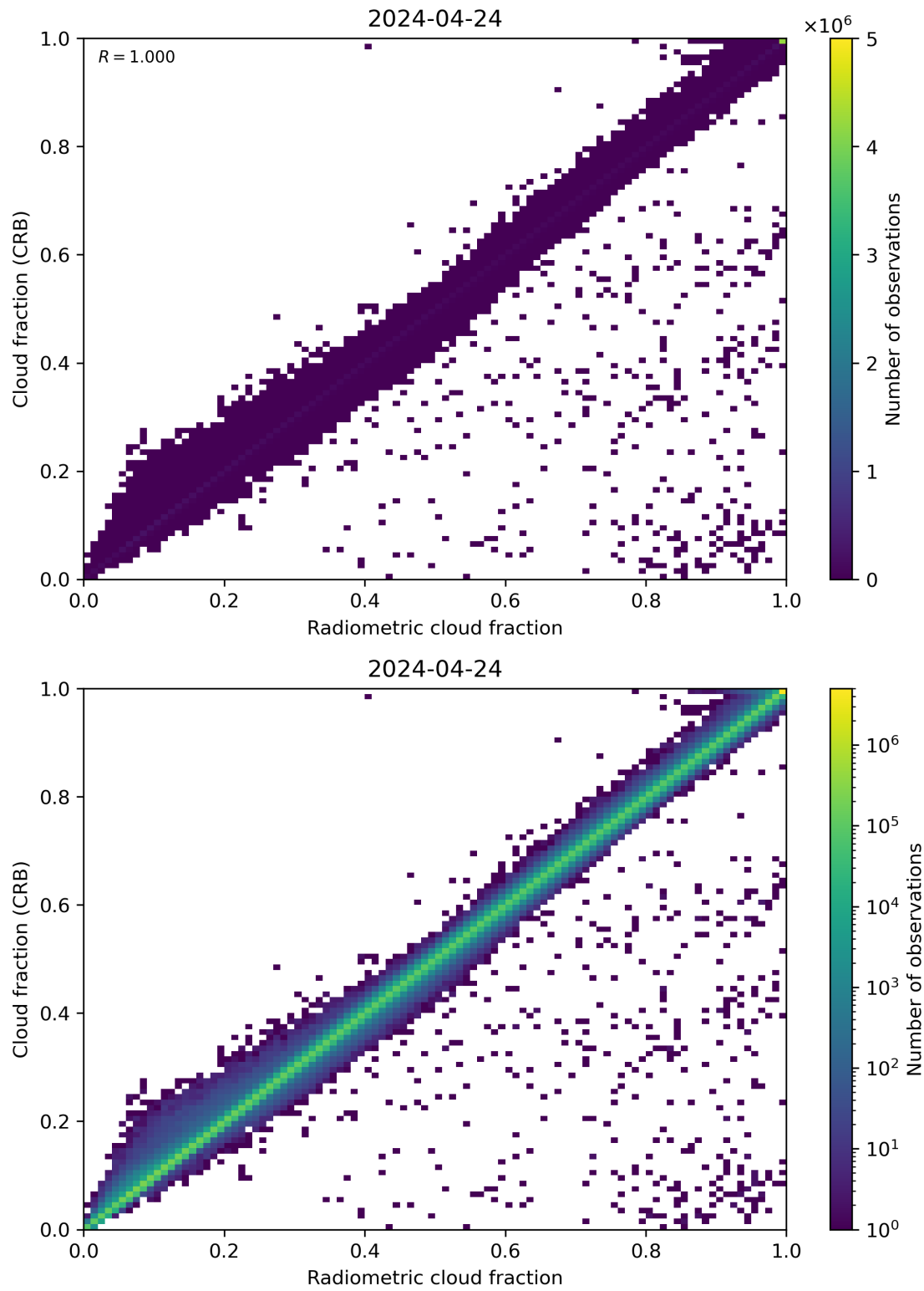
Figure 73: Scatter density plot of “Radiometric cloud fraction” against “Cloud fraction (CRB)” for 2024-04-23 to 2024-04-25.
