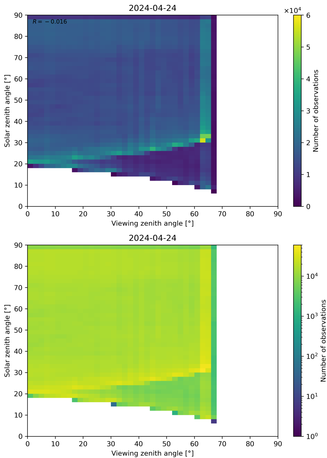
Figure 114: Scatter density plot of “Viewing zenith angle” against “Solar zenith angle” for 2024-04-23 to 2024-04-25.
