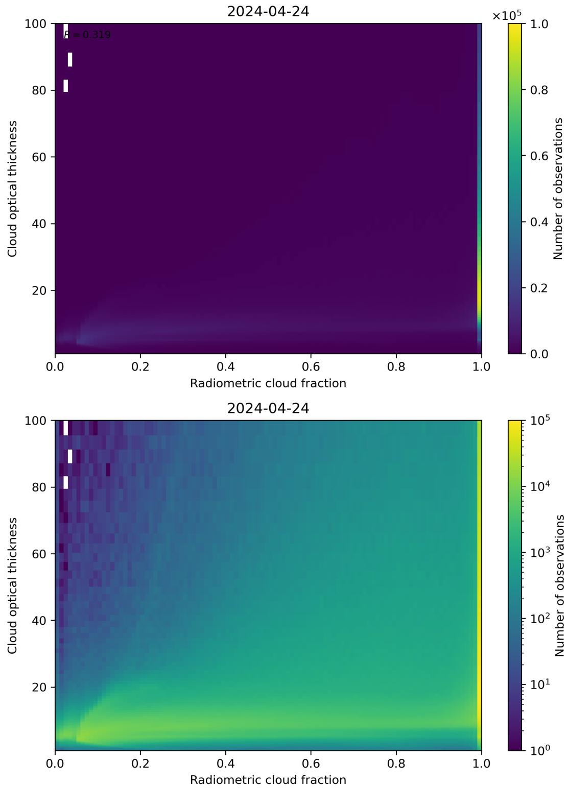
Figure 75: Scatter density plot of “Radiometric cloud fraction” against “Cloud optical thickness” for 2024-04-23 to 2024-04-25.
