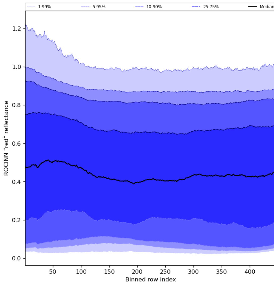
Figure 69: Along track statistics of “ROCINN “red” reflectance” for 2024-04-23 to 2024-04-25
