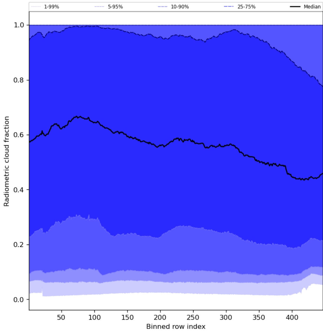
Figure 55: Along track statistics of “Radiometric cloud fraction” for 2024-04-23 to 2024-04-25
