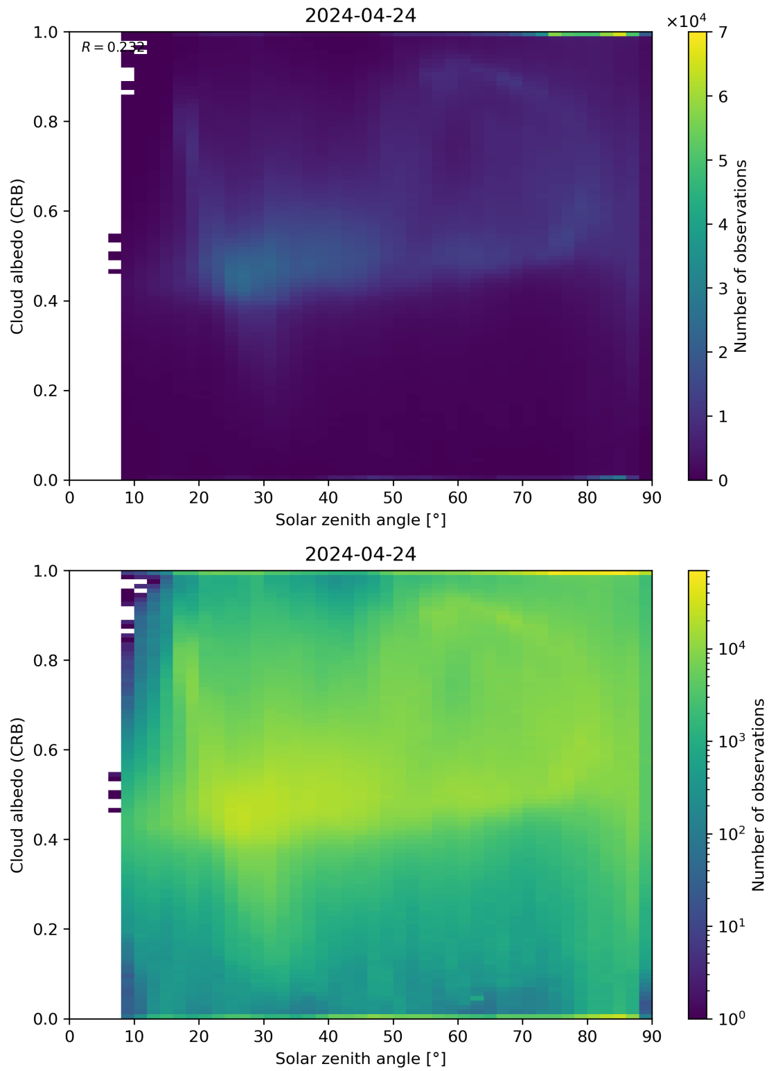
Figure 98: Scatter density plot of “Solar zenith angle” against “Cloud albedo (CRB)” for 2024-04-23 to 2024-04-25.
