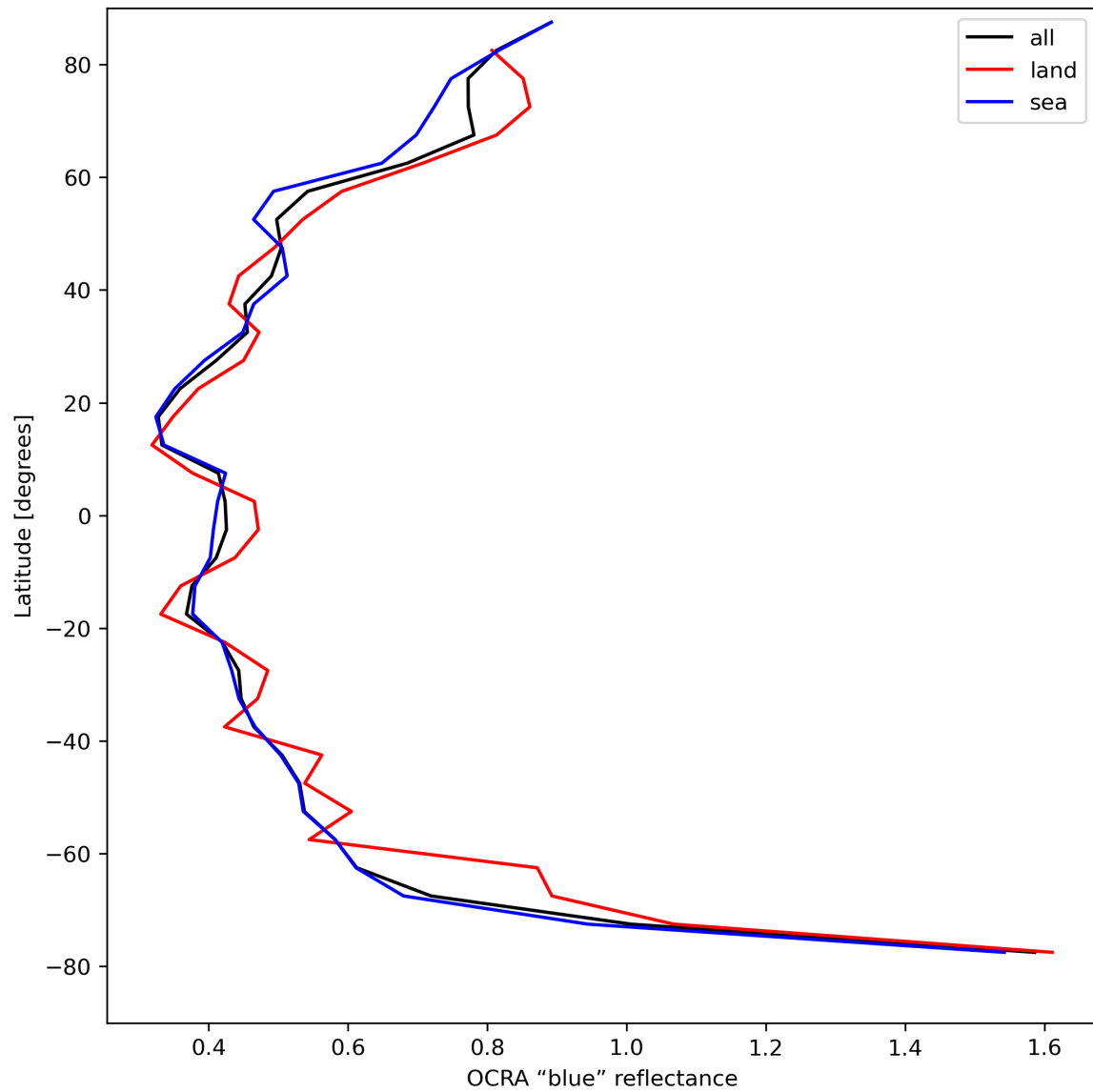
Figure 35: Zonal average of “OCRA “blue” reflectance” for 2024-04-23 to 2024-04-25.
