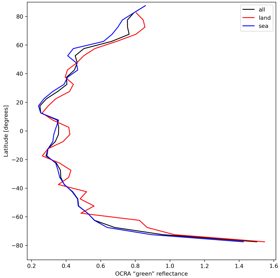
Figure 36: Zonal average of “OCRA “green” reflectance” for 2024-04-23 to 2024-04-25.
