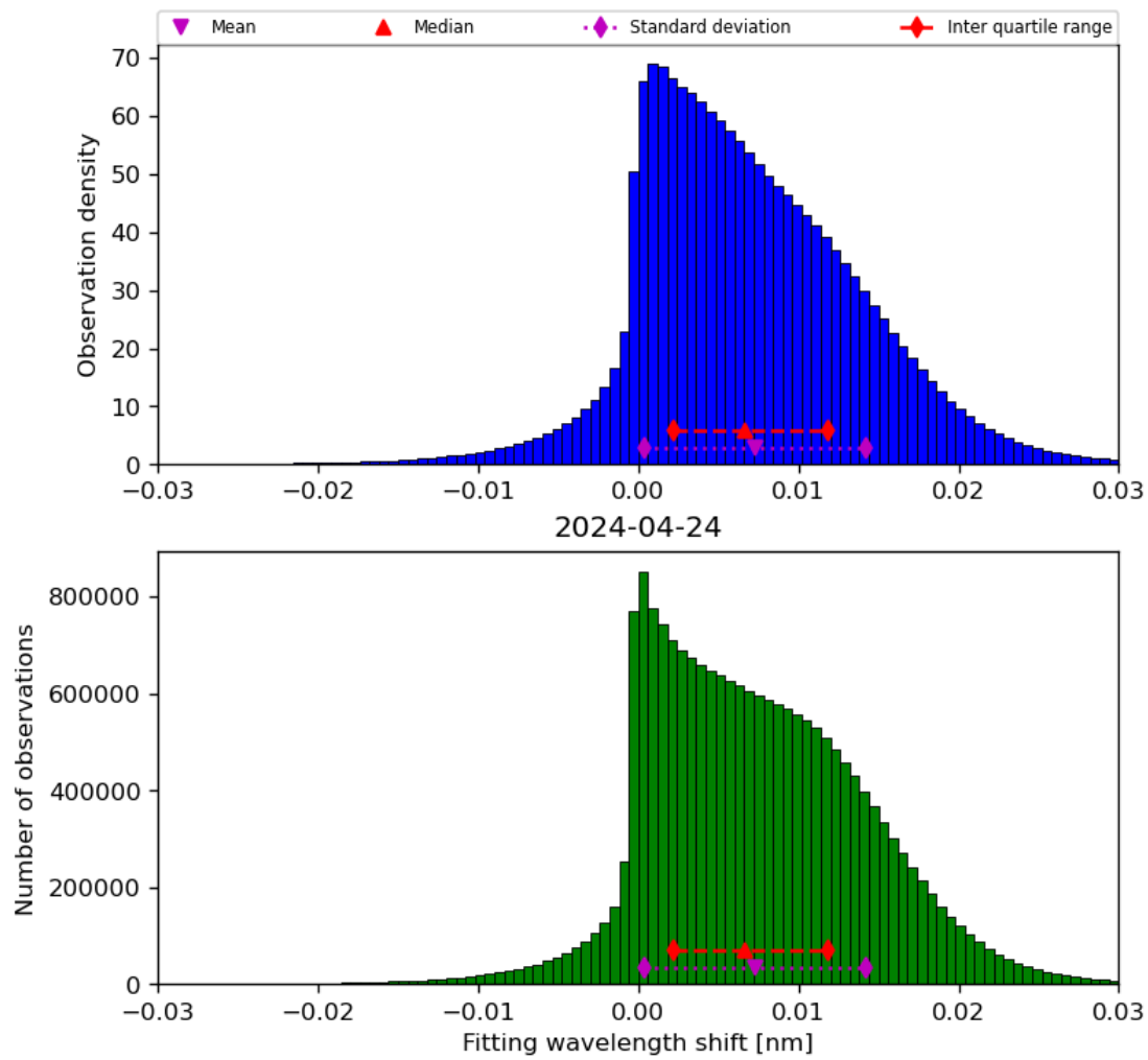
Figure 49: Histogram of “Fitting wavelength shift” for 2024-04-23 to 2024-04-25
