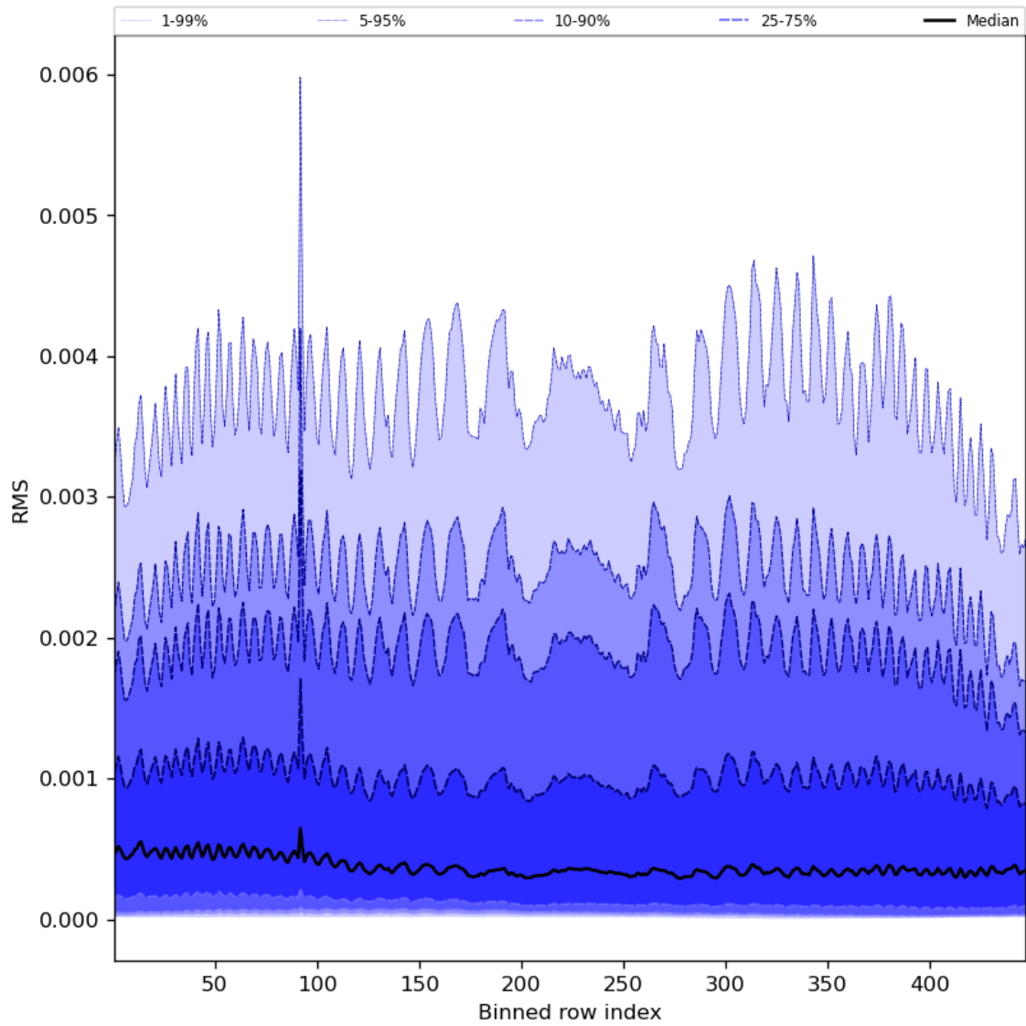
Figure 63: Along track statistics of “RMS” for 2024-04-23 to 2024-04-25
