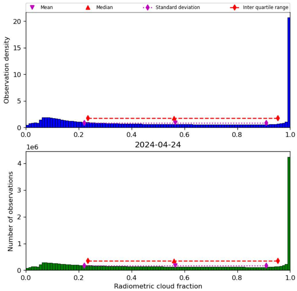
Figure 39: Histogram of “Radiometric cloud fraction” for 2024-04-23 to 2024-04-25
