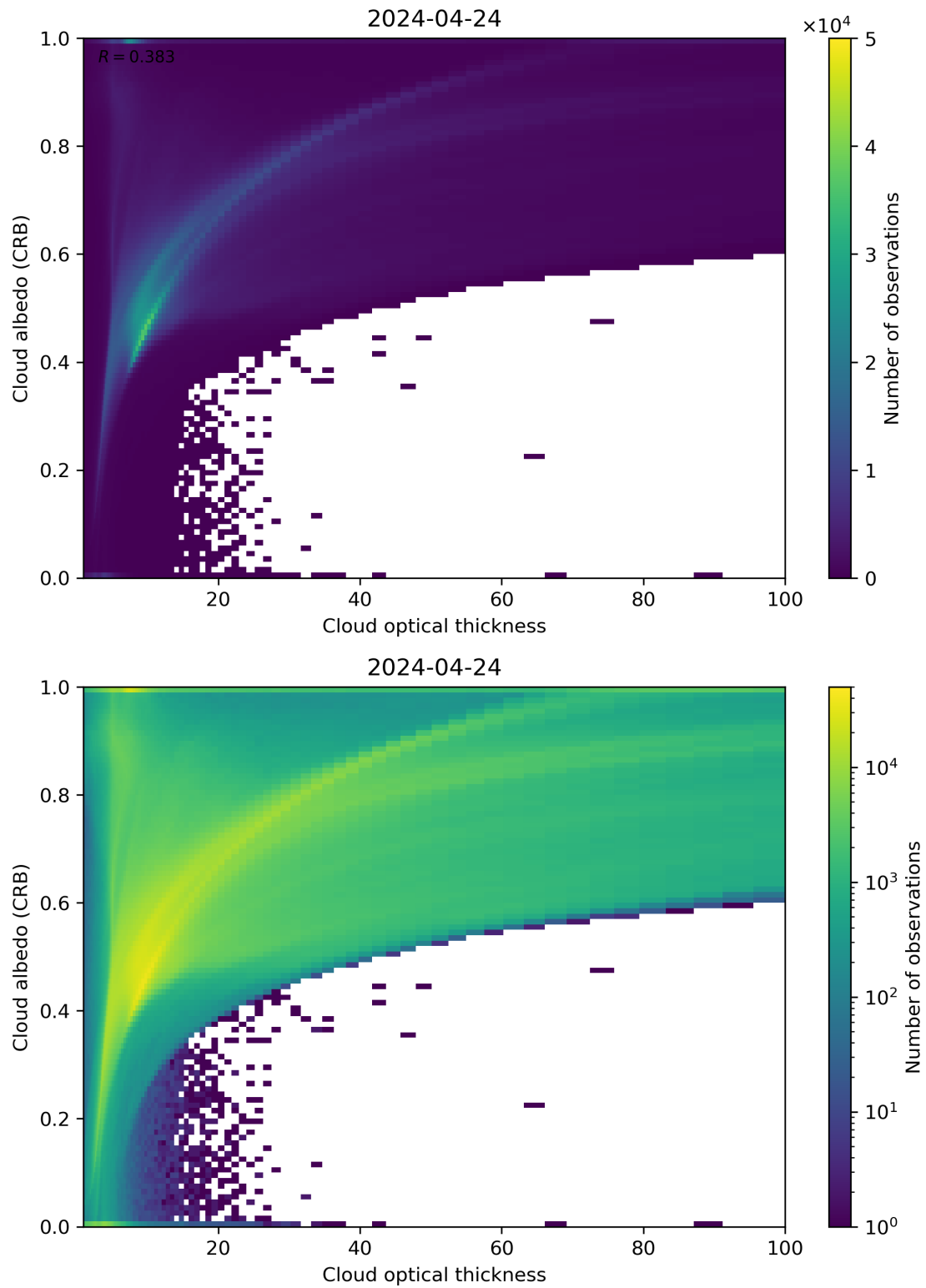
Figure 82: Scatter density plot of “Cloud optical thickness” against “Cloud albedo (CRB)” for 2024-04-23 to 2024-04-25.
