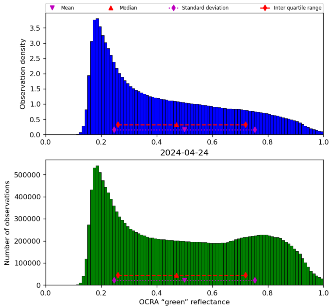
Figure 52: Histogram of “OCRA “green” reflectance” for 2024-04-23 to 2024-04-25
