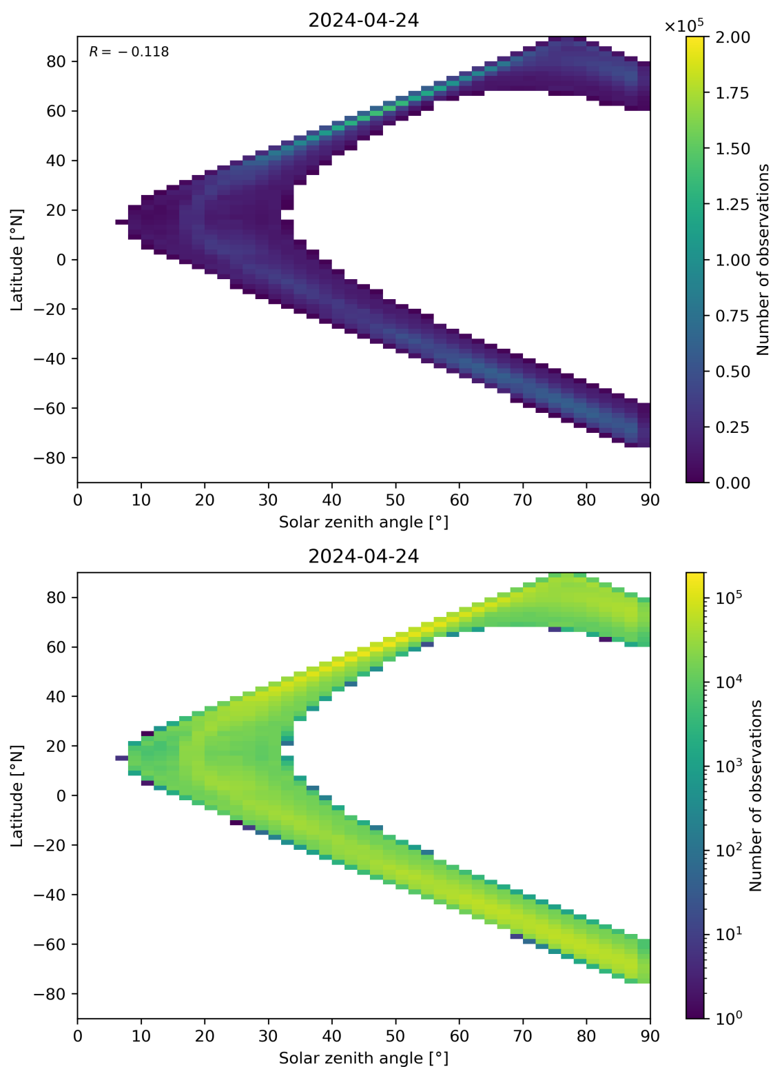
Figure 105: Scatter density plot of “Solar zenith angle” against “Latitude” for 2024-04-23 to 2024-04-25.
