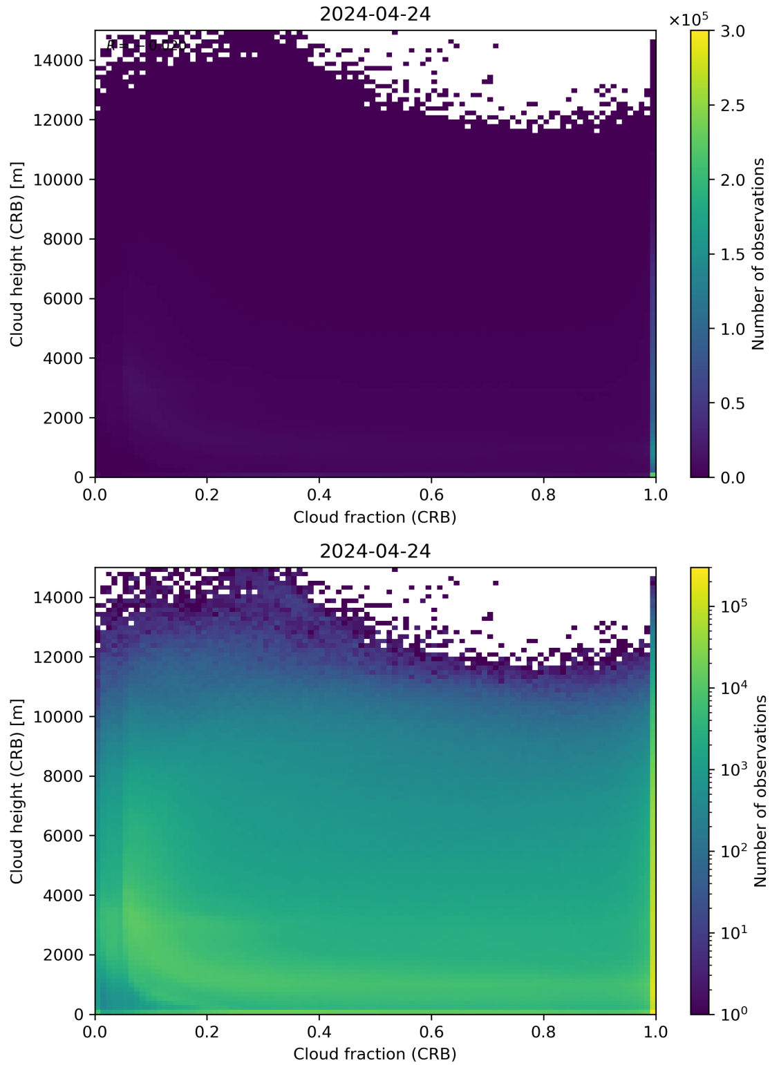
Figure 79: Scatter density plot of “Cloud fraction (CRB)” against “Cloud height (CRB)” for 2024-04-23 to 2024-04-25.
