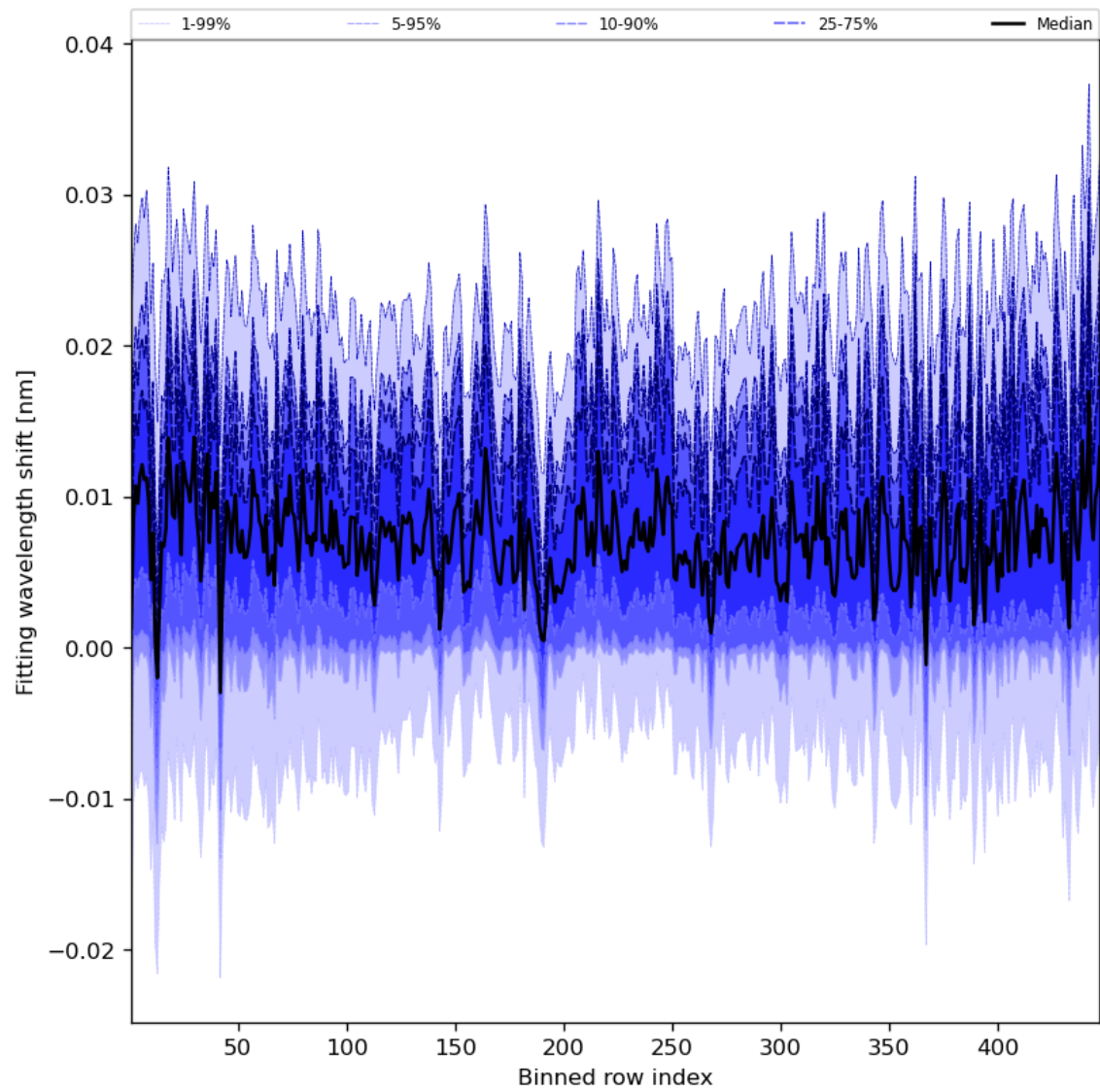
Figure 65: Along track statistics of “Fitting wavelength shift” for 2024-04-23 to 2024-04-25
