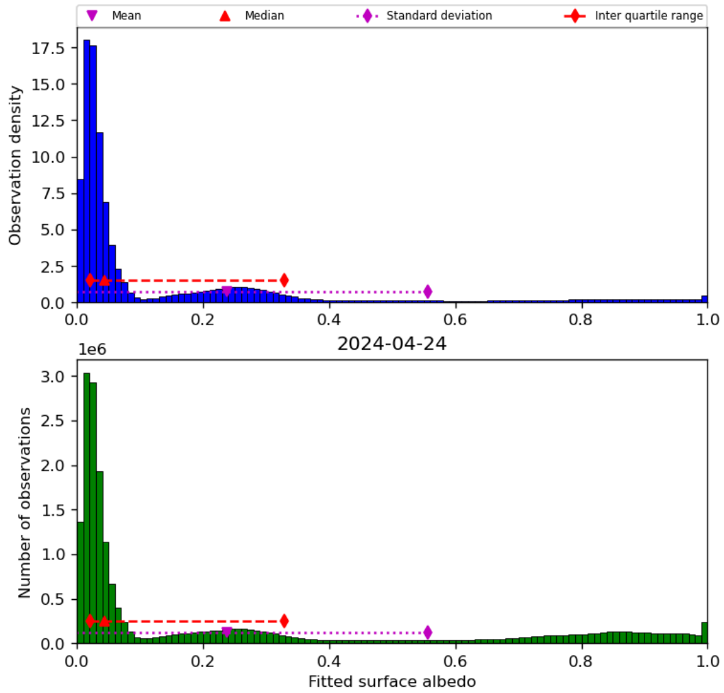
Figure 45: Histogram of “Fitted surface albedo” for 2024-04-23 to 2024-04-25
