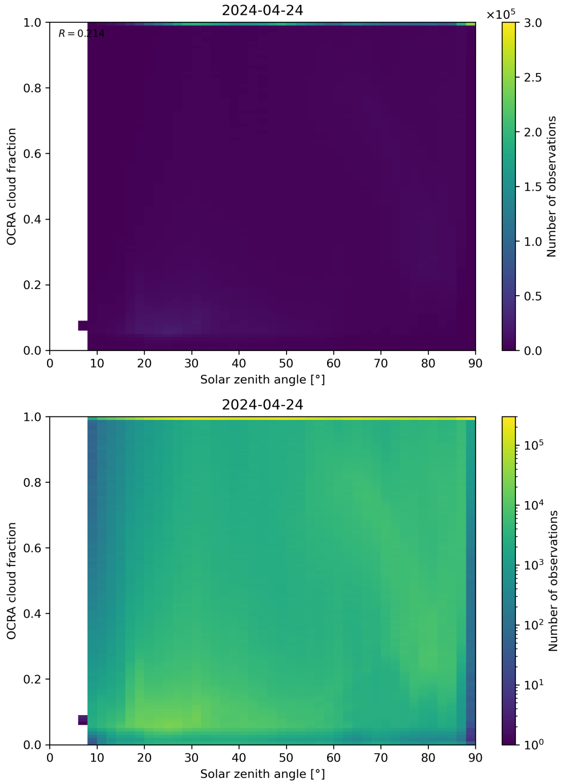
Figure 100: Scatter density plot of “Solar zenith angle” against “OCRA cloud fraction” for 2024-04-23 to 2024-04-25.
