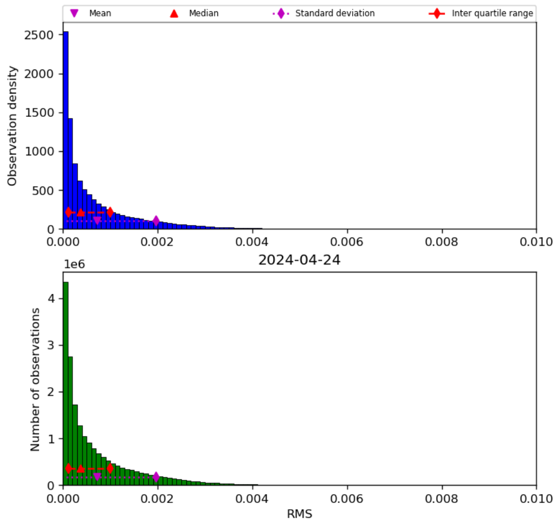
Figure 47: Histogram of “RMS” for 2024-04-23 to 2024-04-25
