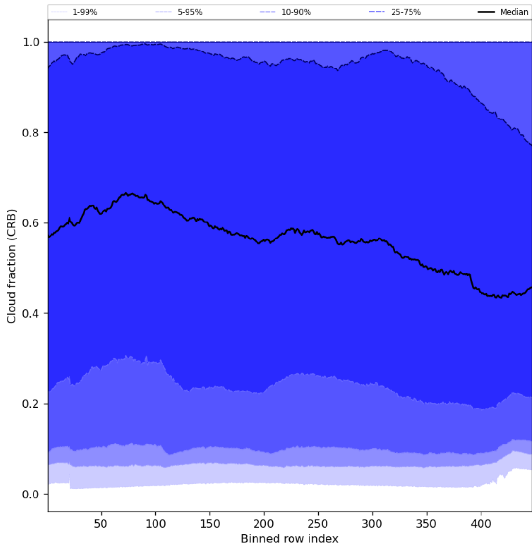
Figure 58: Along track statistics of “Cloud fraction (CRB)” for 2024-04-23 to 2024-04-25
