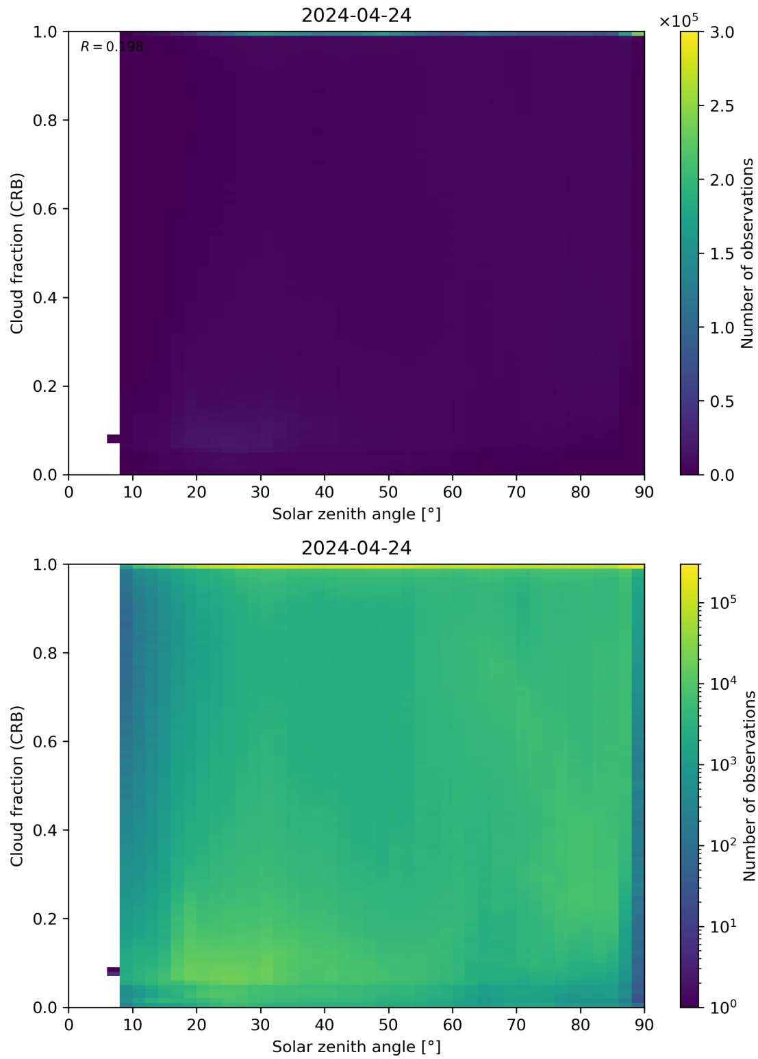
Figure 101: Scatter density plot of “Solar zenith angle” against “Cloud fraction (CRB)” for 2024-04-23 to 2024-04-25.
