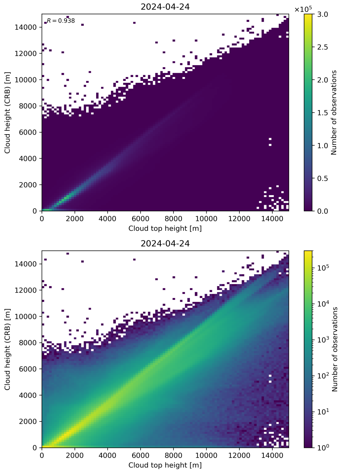
Figure 89: Scatter density plot of “Cloud top height” against “Cloud height (CRB)” for 2024-04-23 to 2024-04-25.
