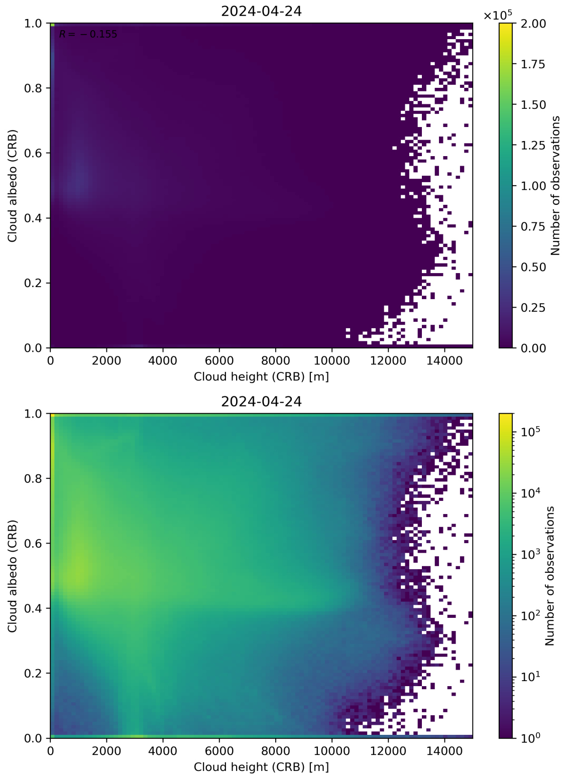
Figure 80: Scatter density plot of “Cloud height (CRB)” against “Cloud albedo (CRB)” for 2024-04-23 to 2024-04-25.
