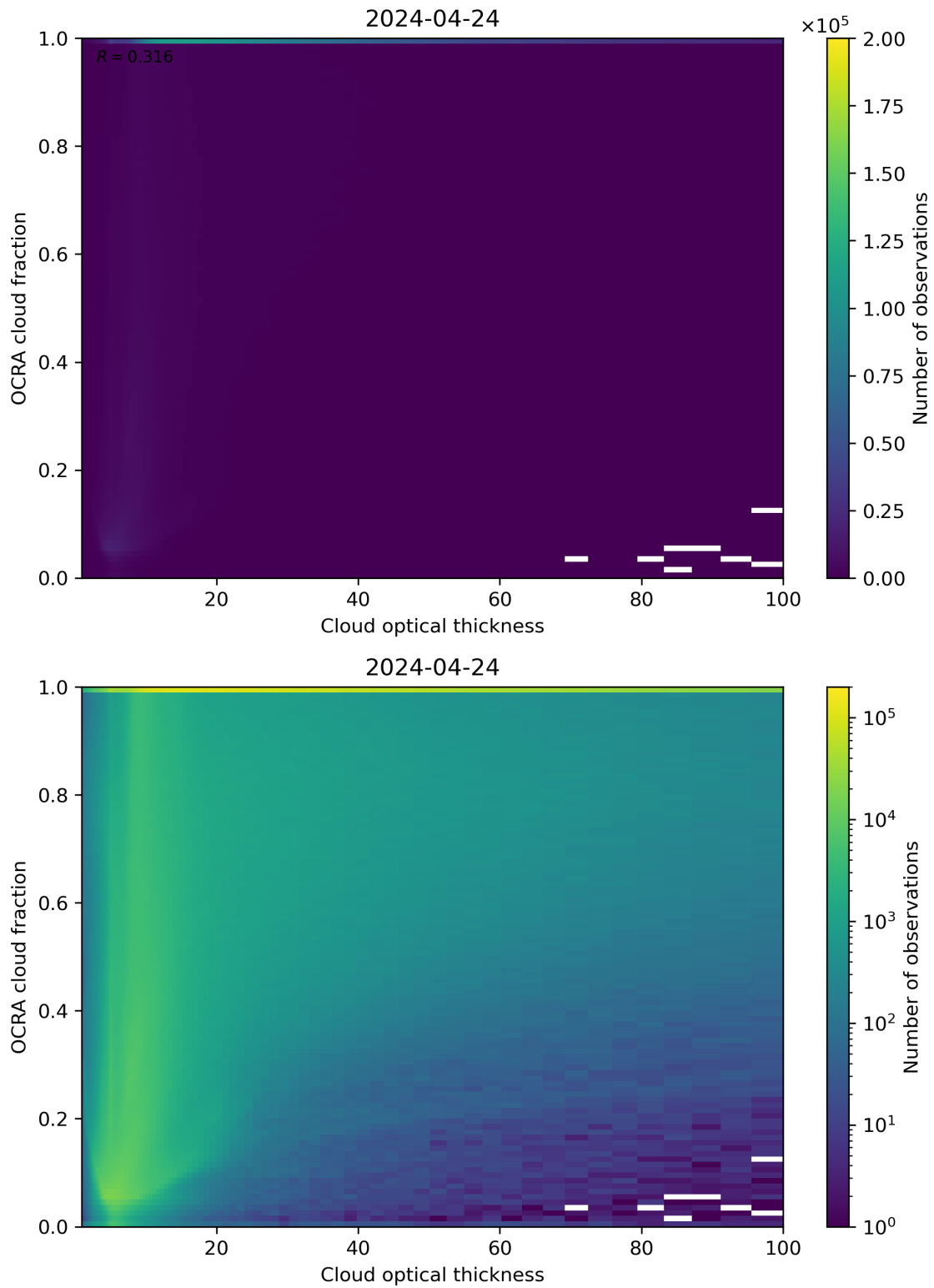
Figure 83: Scatter density plot of “Cloud optical thickness” against “OCRA cloud fraction” for 2024-04-23 to 2024-04-25.
