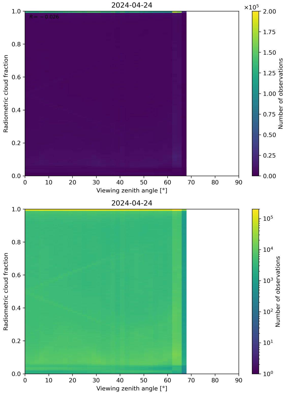
Figure 107: Scatter density plot of “Viewing zenith angle” against “Radiometric cloud fraction” for 2024-04-23 to 2024-04-25.
