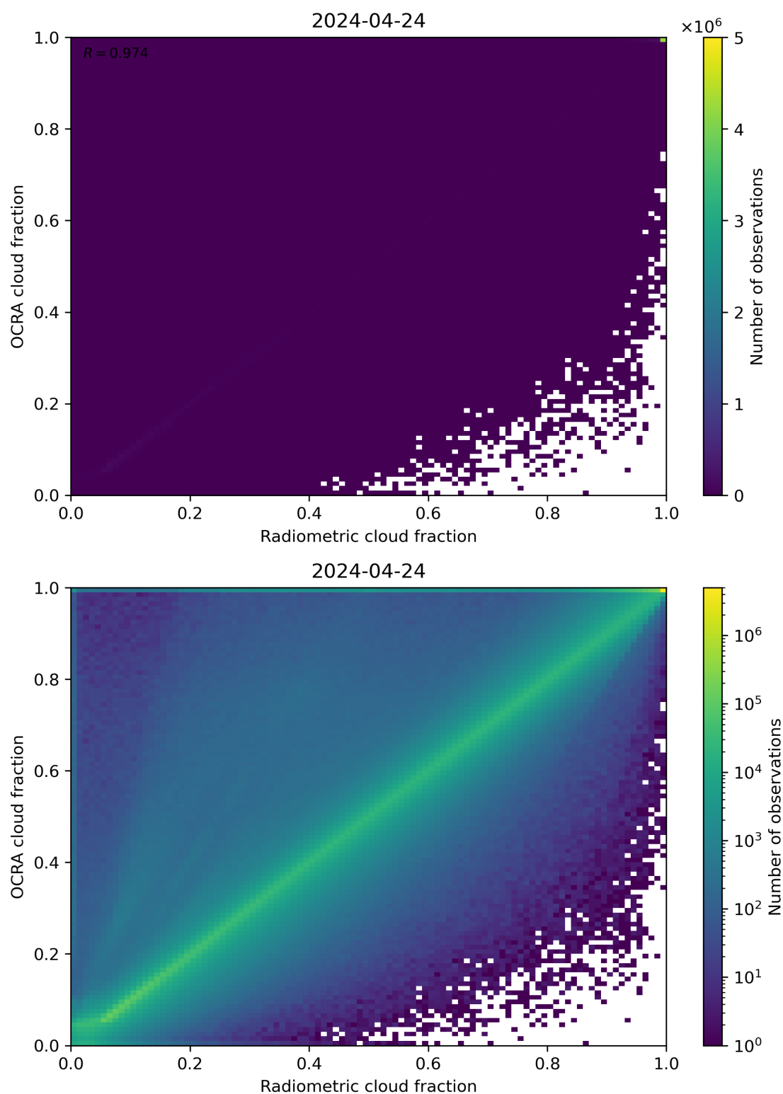
Figure 72: Scatter density plot of “Radiometric cloud fraction” against “OCRA cloud fraction” for 2024-04-23 to 2024-04-25.
