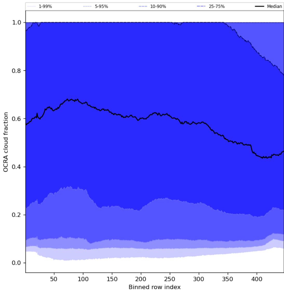
Figure 66: Along track statistics of “OCRA cloud fraction” for 2024-04-23 to 2024-04-25
