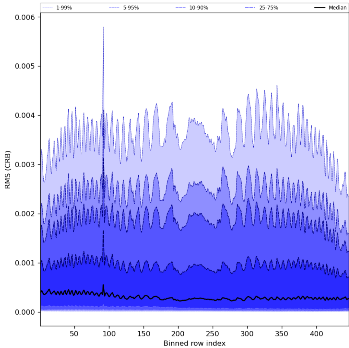
Figure 64: Along track statistics of “RMS (CRB)” for 2024-04-23 to 2024-04-25
