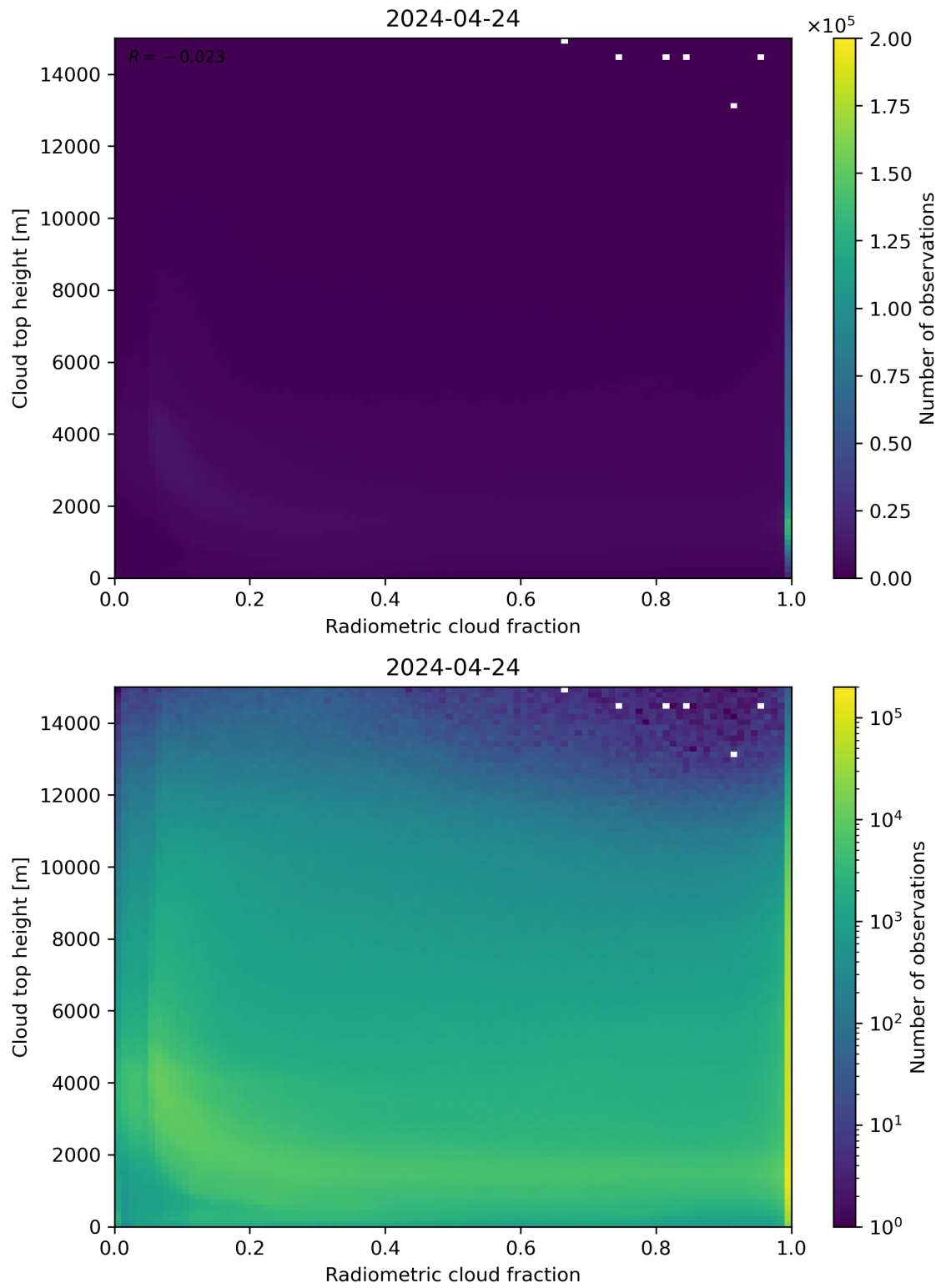
Figure 76: Scatter density plot of “Radiometric cloud fraction” against “Cloud top height” for 2024-04-23 to 2024-04-25.
