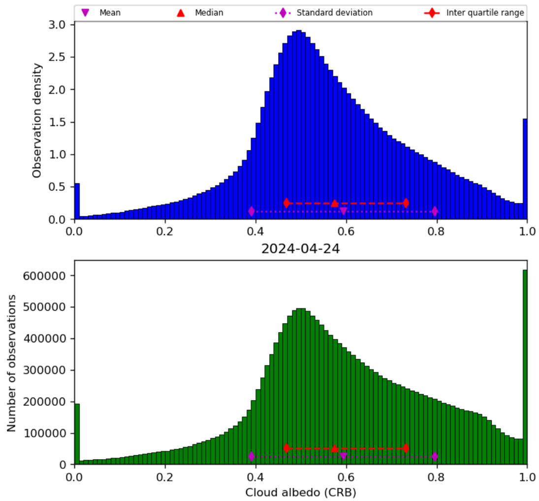
Figure 44: Histogram of “Cloud albedo (CRB)” for 2024-04-23 to 2024-04-25
