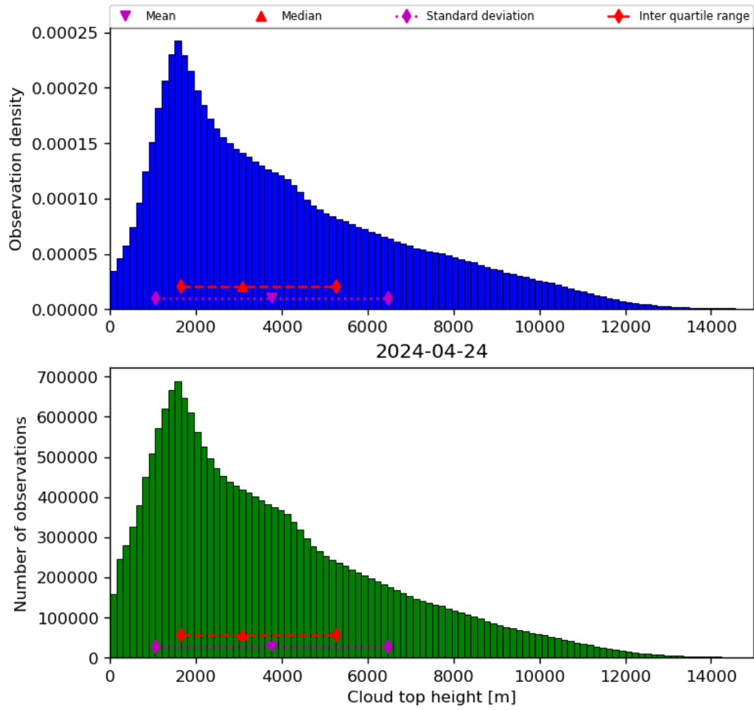
Figure 40: Histogram of “Cloud top height” for 2024-04-23 to 2024-04-25
