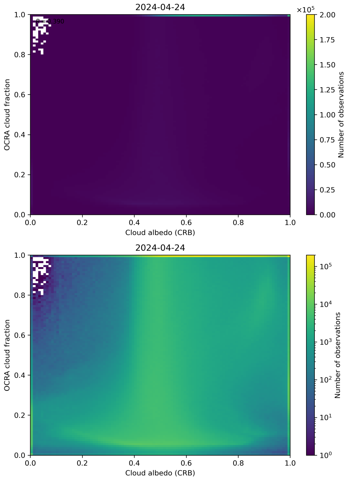
Figure 70: Scatter density plot of “Cloud albedo (CRB)” against “OCRA cloud fraction” for 2024-04-23 to 2024-04-25.
