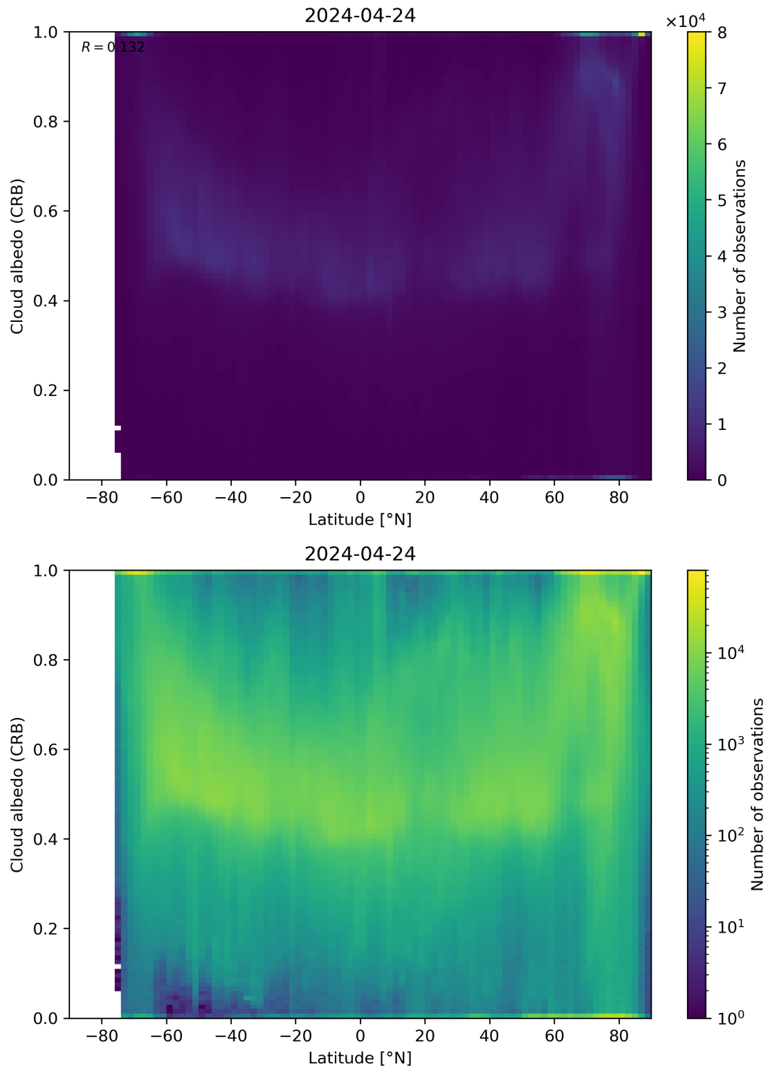
Figure 91: Scatter density plot of “Latitude” against “Cloud albedo (CRB)” for 2024-04-23 to 2024-04-25.
