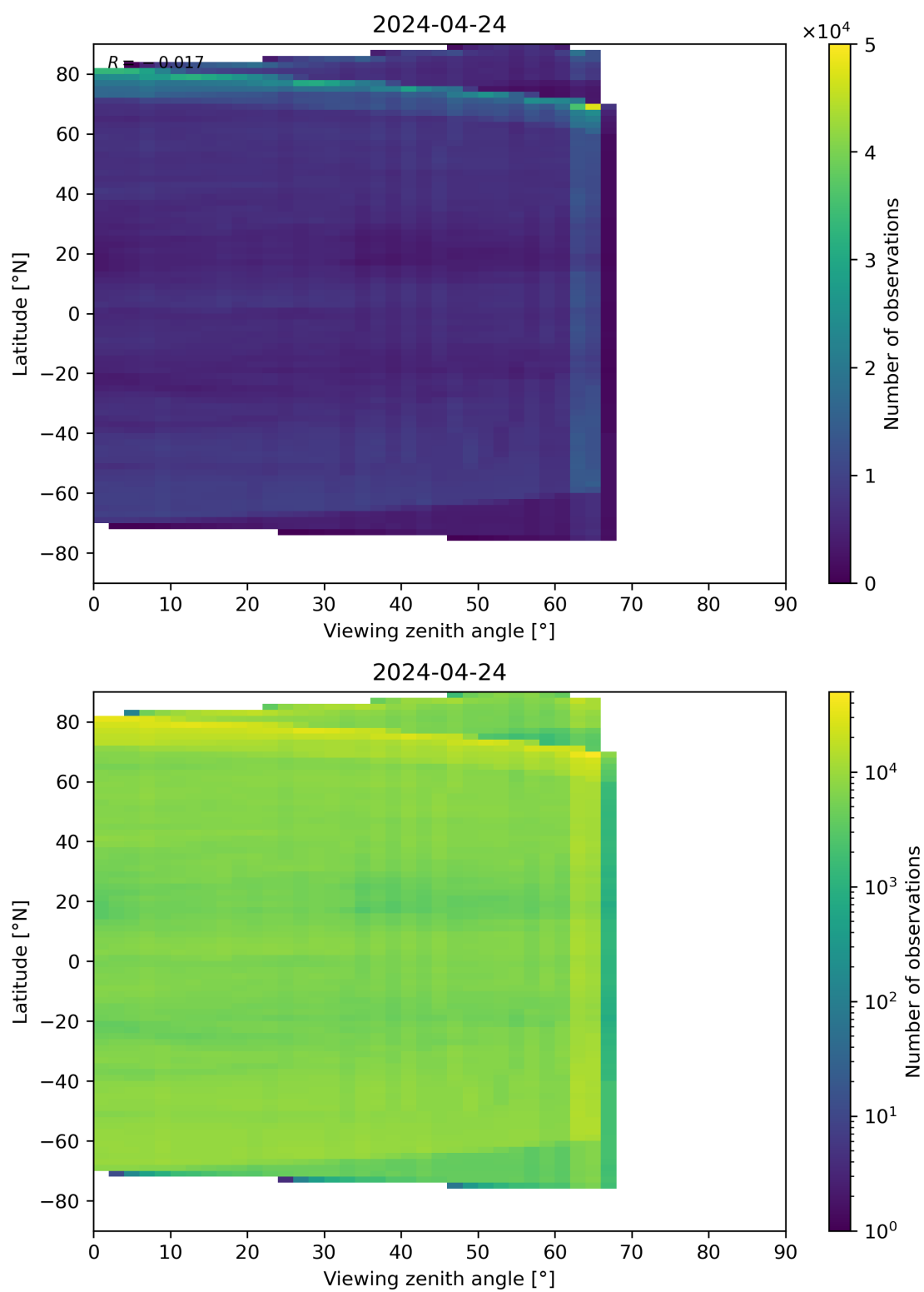
Figure 113: Scatter density plot of “Viewing zenith angle” against “Latitude” for 2024-04-23 to 2024-04-25.
