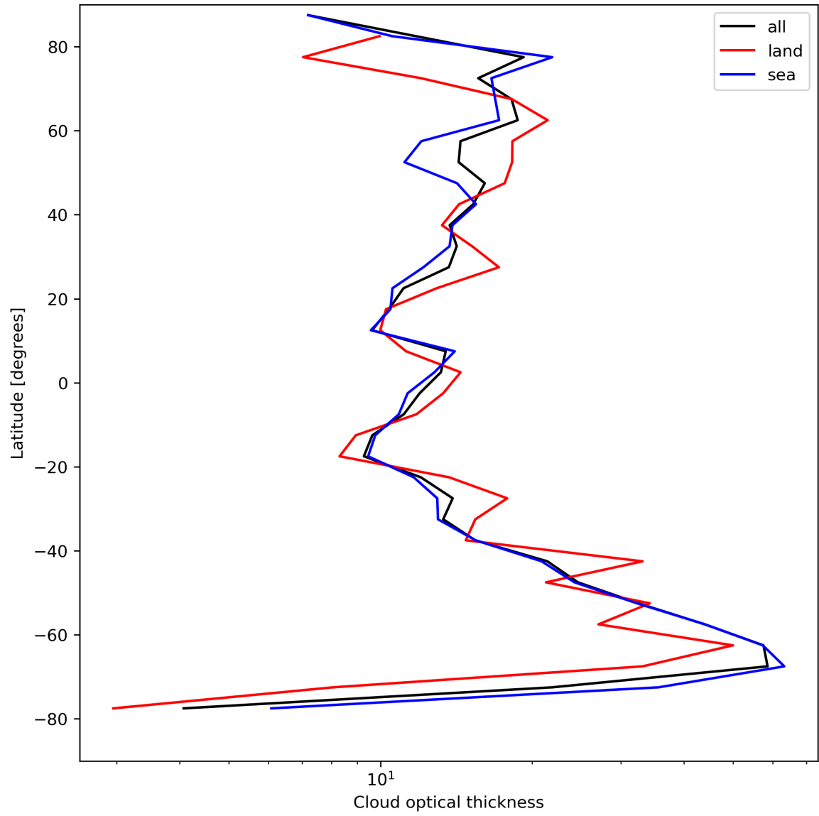
Figure 25: Zonal average of “Cloud optical thickness” for 2024-04-23 to 2024-04-25.
