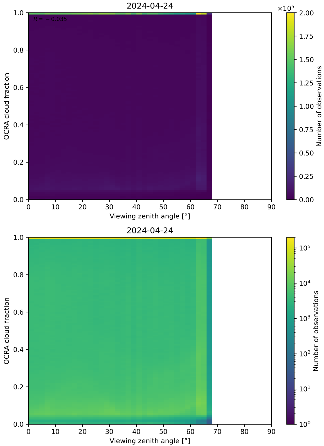
Figure 108: Scatter density plot of “Viewing zenith angle” against “OCRA cloud fraction” for 2024-04-23 to 2024-04-25.
