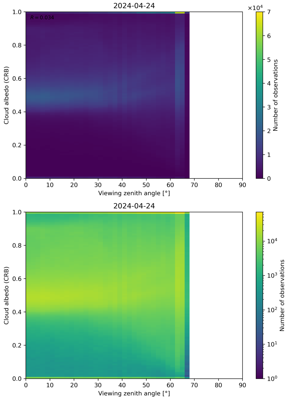
Figure 106: Scatter density plot of “Viewing zenith angle” against “Cloud albedo (CRB)” for 2024-04-23 to 2024-04-25.
