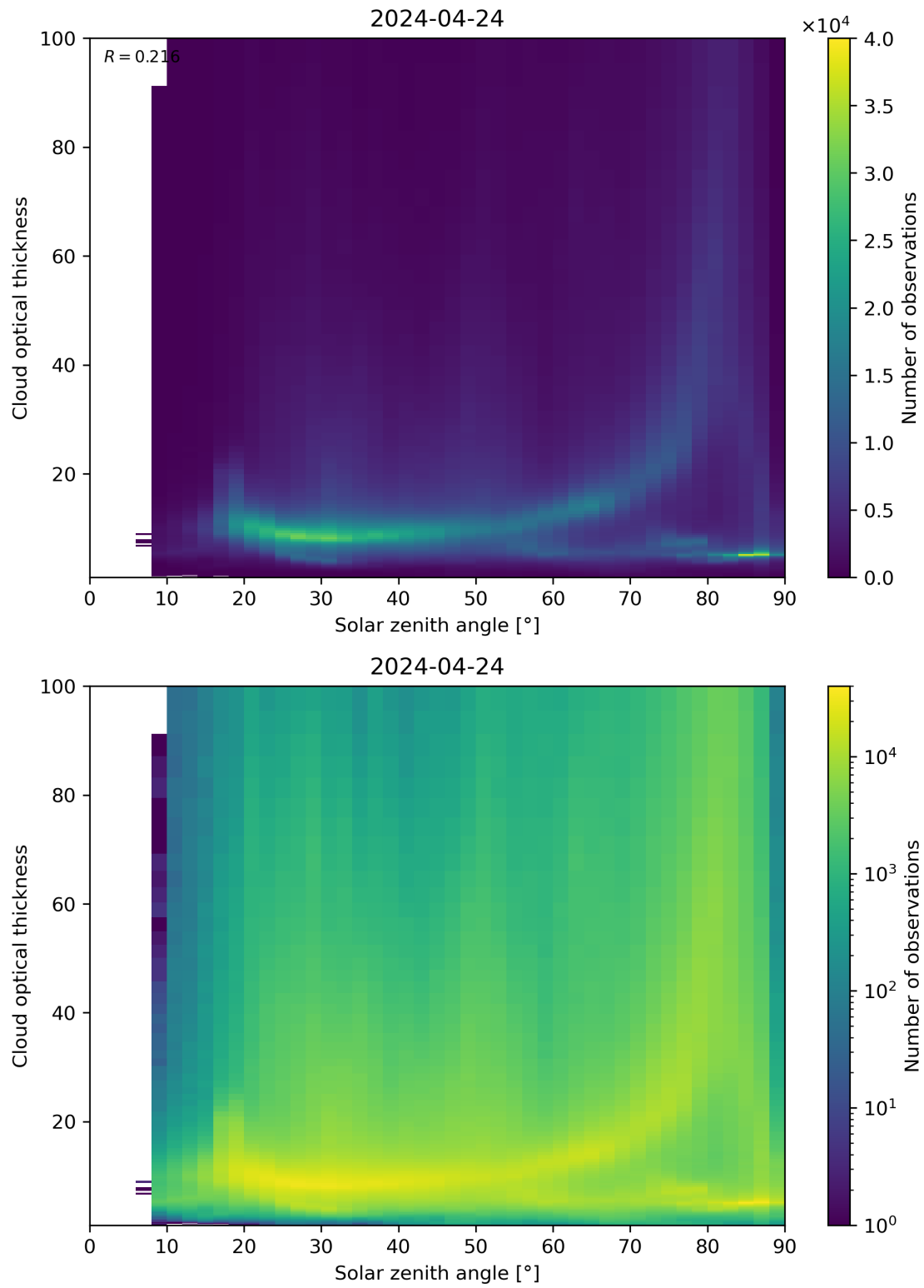
Figure 103: Scatter density plot of “Solar zenith angle” against “Cloud optical thickness” for 2024-04-23 to 2024-04-25.
