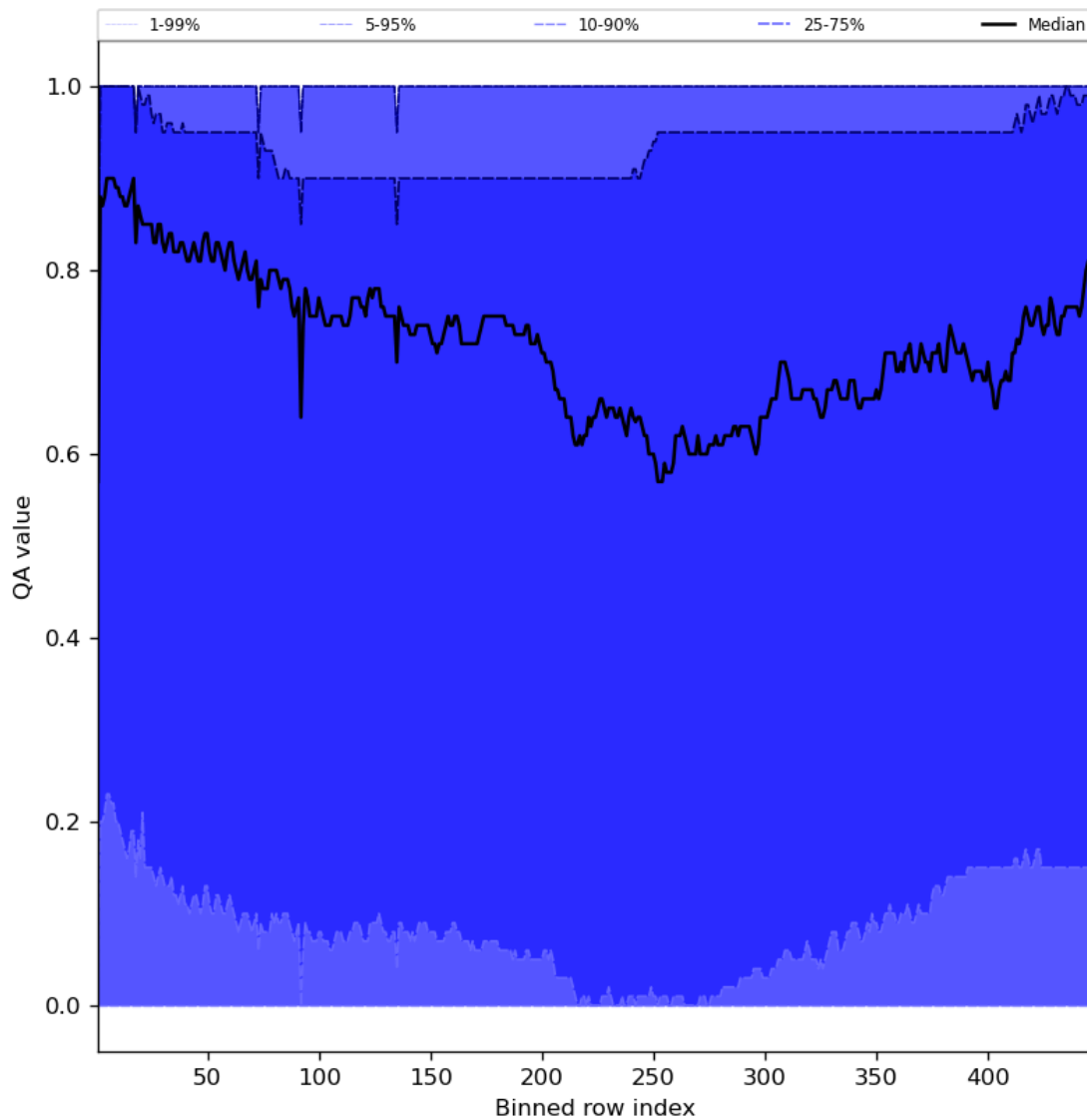
Figure 54: Along track statistics of “QA value” for 2024-04-23 to 2024-04-25
