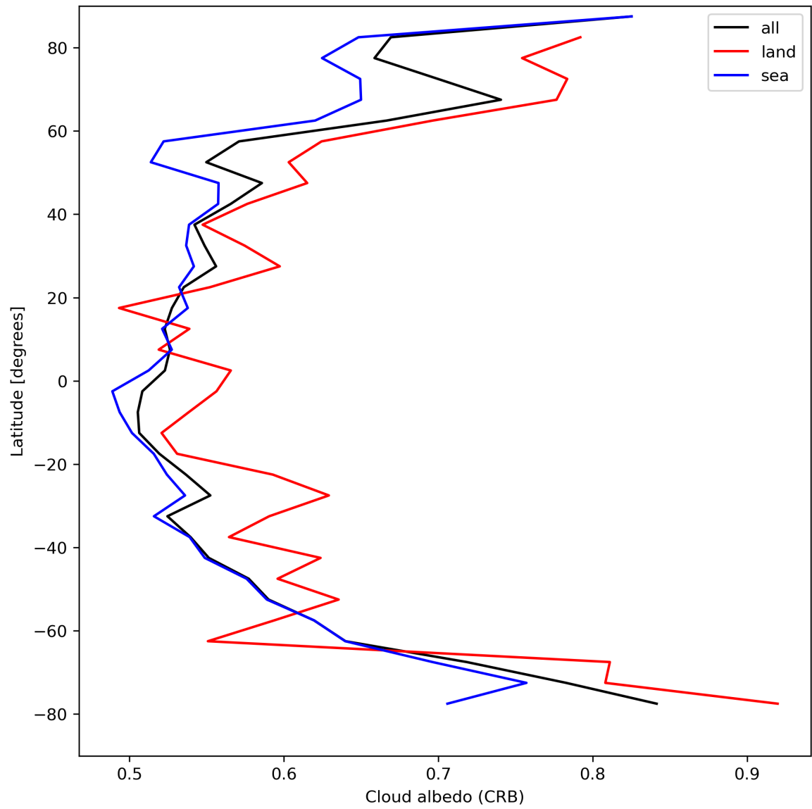
Figure 28: Zonal average of “Cloud albedo (CRB)” for 2024-04-23 to 2024-04-25.
