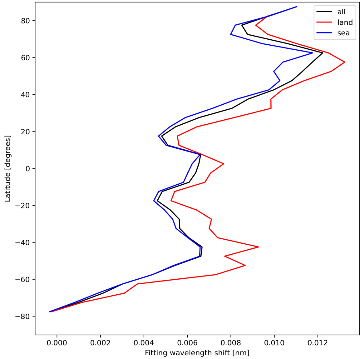
Figure 33: Zonal average of “Fitting wavelength shift” for 2024-04-23 to 2024-04-25.
