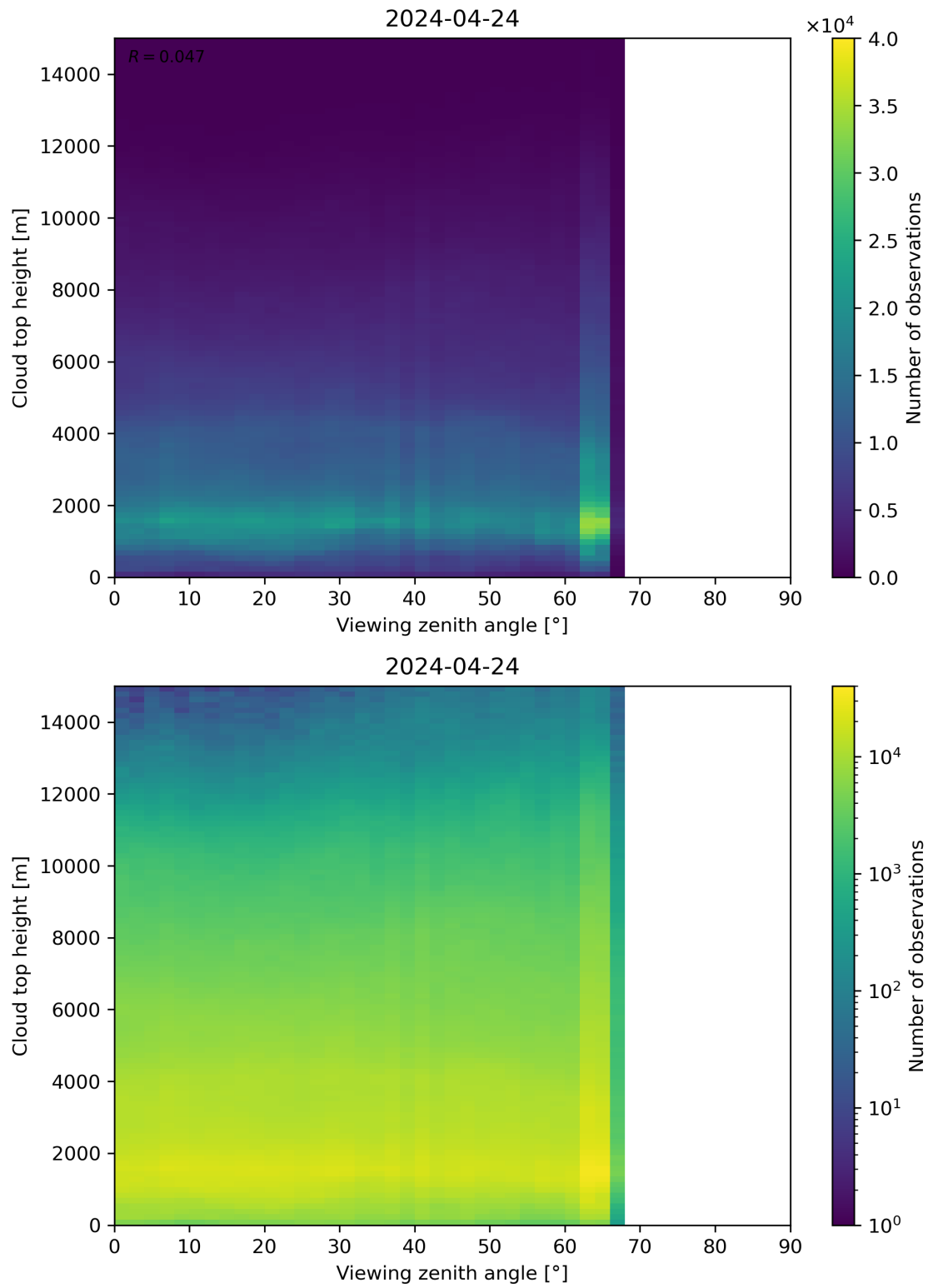
Figure 112: Scatter density plot of “Viewing zenith angle” against “Cloud top height” for 2024-04-23 to 2024-04-25.
