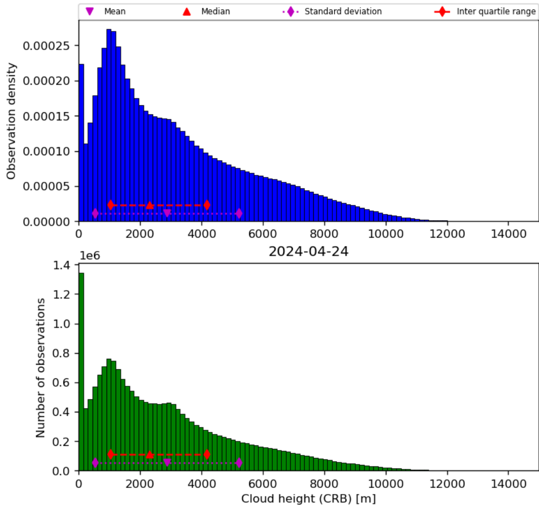
Figure 43: Histogram of “Cloud height (CRB)” for 2024-04-23 to 2024-04-25
