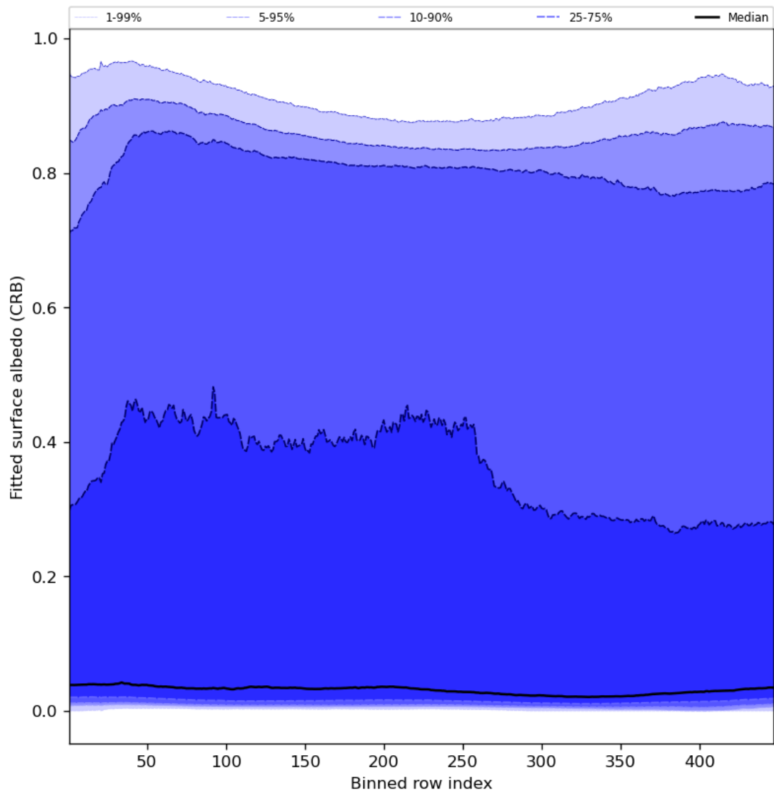
Figure 62: Along track statistics of “Fitted surface albedo (CRB)” for 2024-04-23 to 2024-04-25
