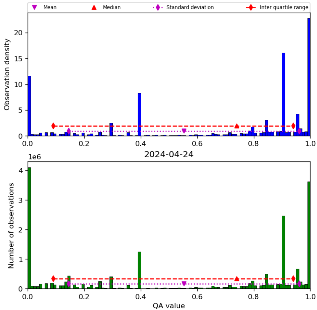
Figure 38: Histogram of “QA value” for 2024-04-23 to 2024-04-25
