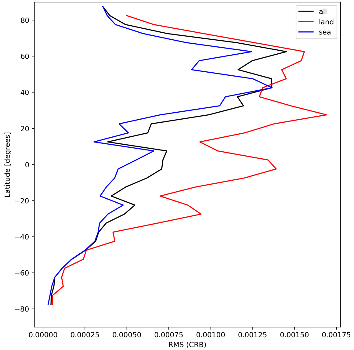
Figure 32: Zonal average of “RMS (CRB)” for 2024-04-23 to 2024-04-25.
