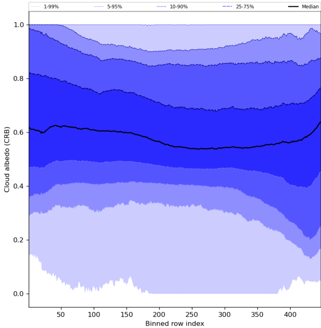
Figure 60: Along track statistics of “Cloud albedo (CRB)” for 2024-04-23 to 2024-04-25
