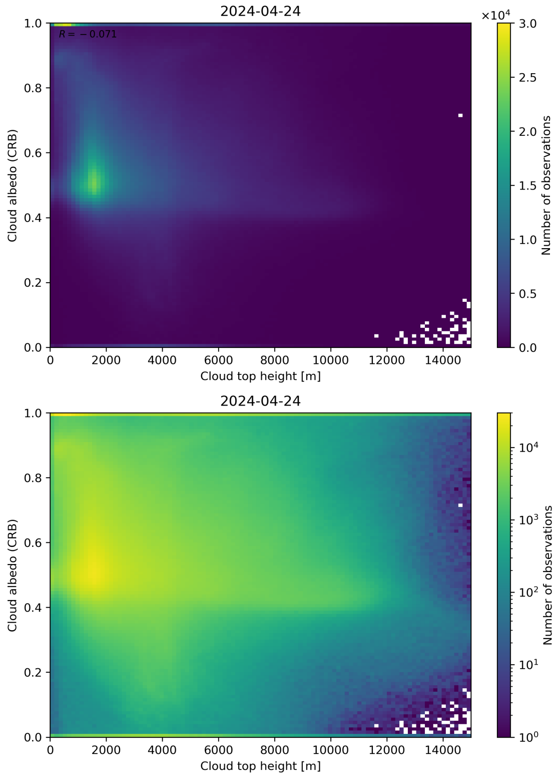
Figure 86: Scatter density plot of “Cloud top height” against “Cloud albedo (CRB)” for 2024-04-23 to 2024-04-25.
