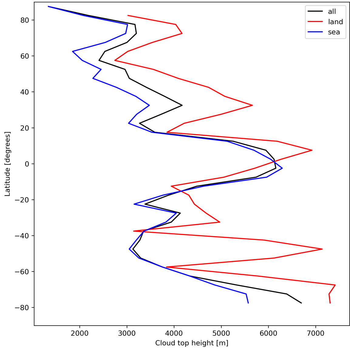
Figure 24: Zonal average of “Cloud top height” for 2024-04-23 to 2024-04-25.
