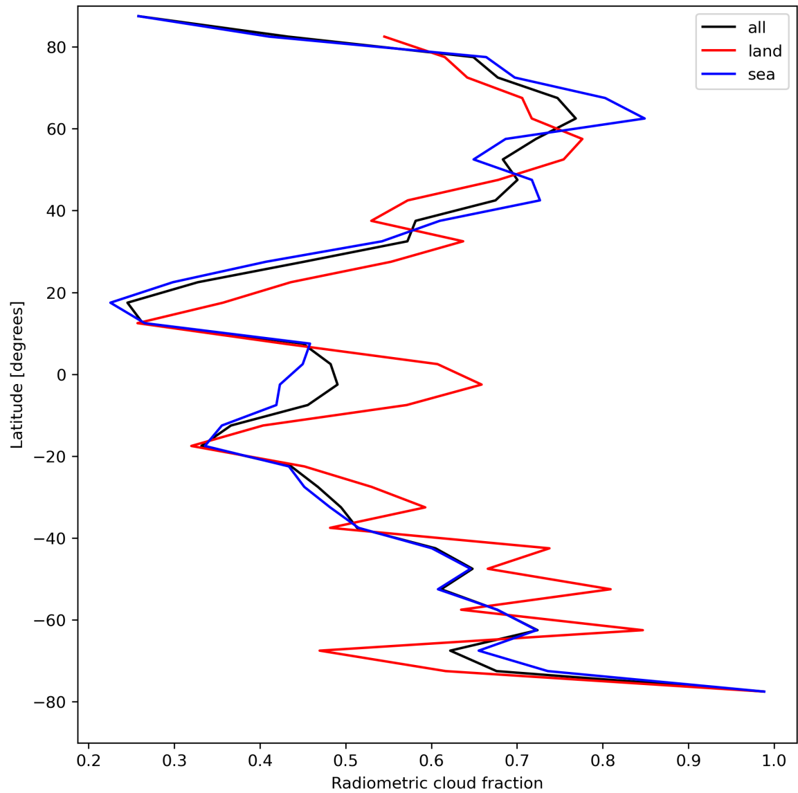
Figure 23: Zonal average of “Radiometric cloud fraction” for 2024-04-23 to 2024-04-25.
