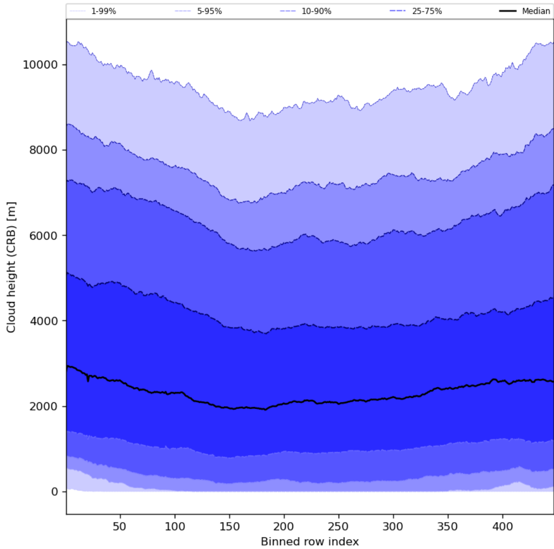
Figure 59: Along track statistics of “Cloud height (CRB)” for 2024-04-23 to 2024-04-25
