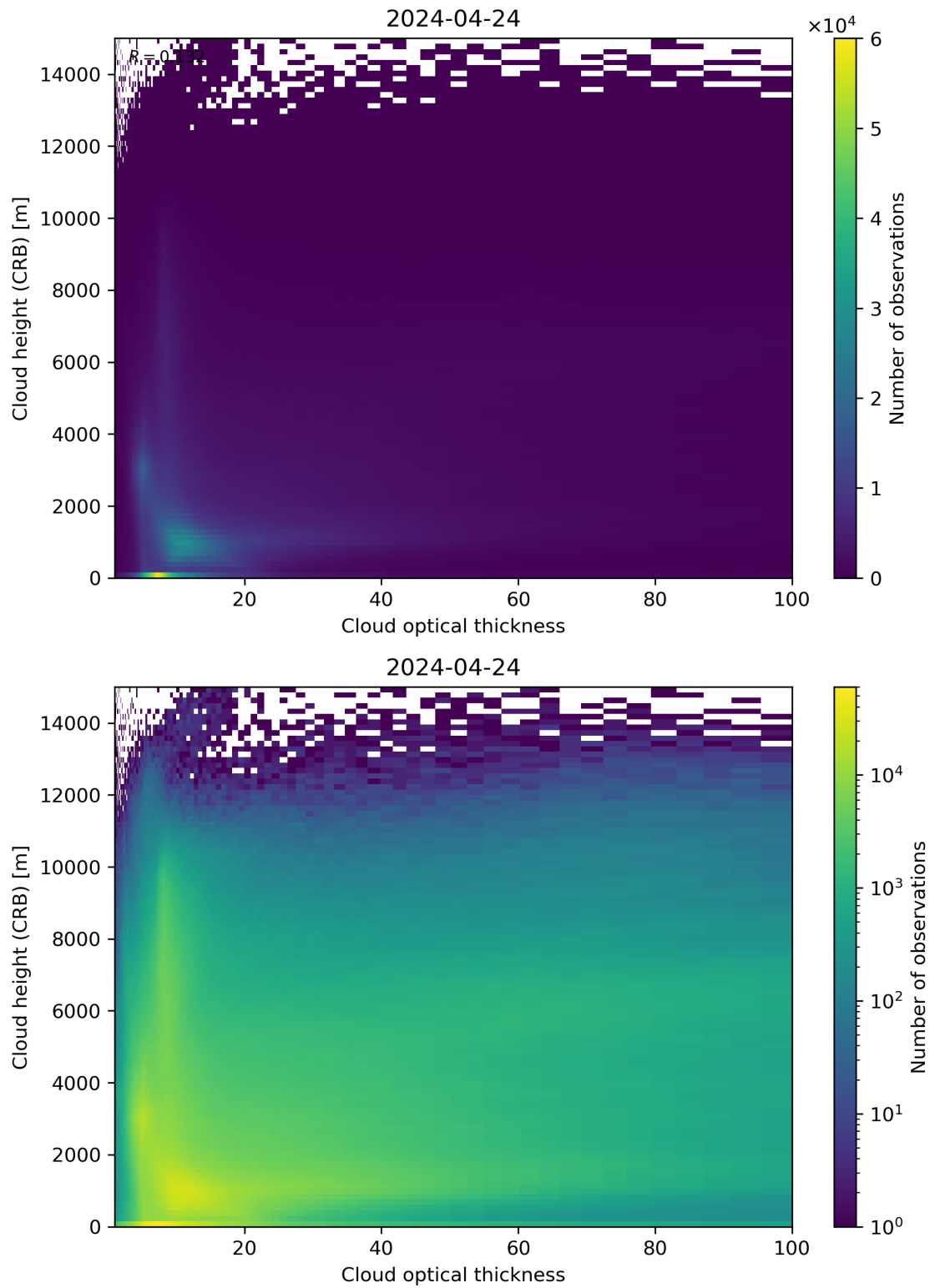
Figure 85: Scatter density plot of “Cloud optical thickness” against “Cloud height (CRB)” for 2024-04-23 to 2024-04-25.
