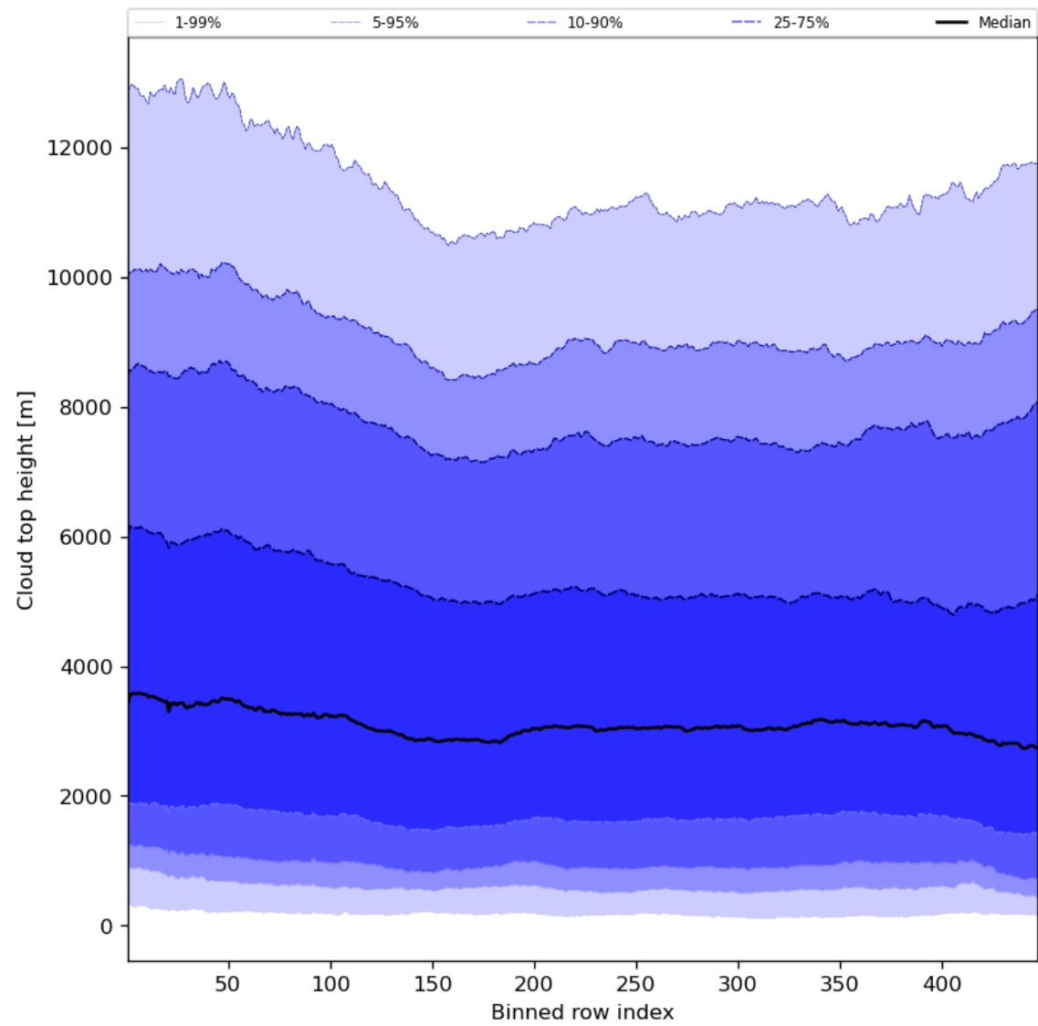
Figure 56: Along track statistics of “Cloud top height” for 2024-04-23 to 2024-04-25
