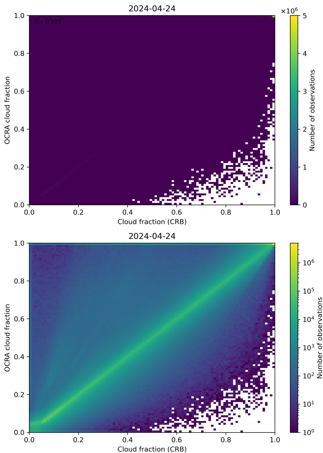
Figure 78: Scatter density plot of “Cloud fraction (CRB)” against “OCRA cloud fraction” for 2024-04-23 to 2024-04-25.
