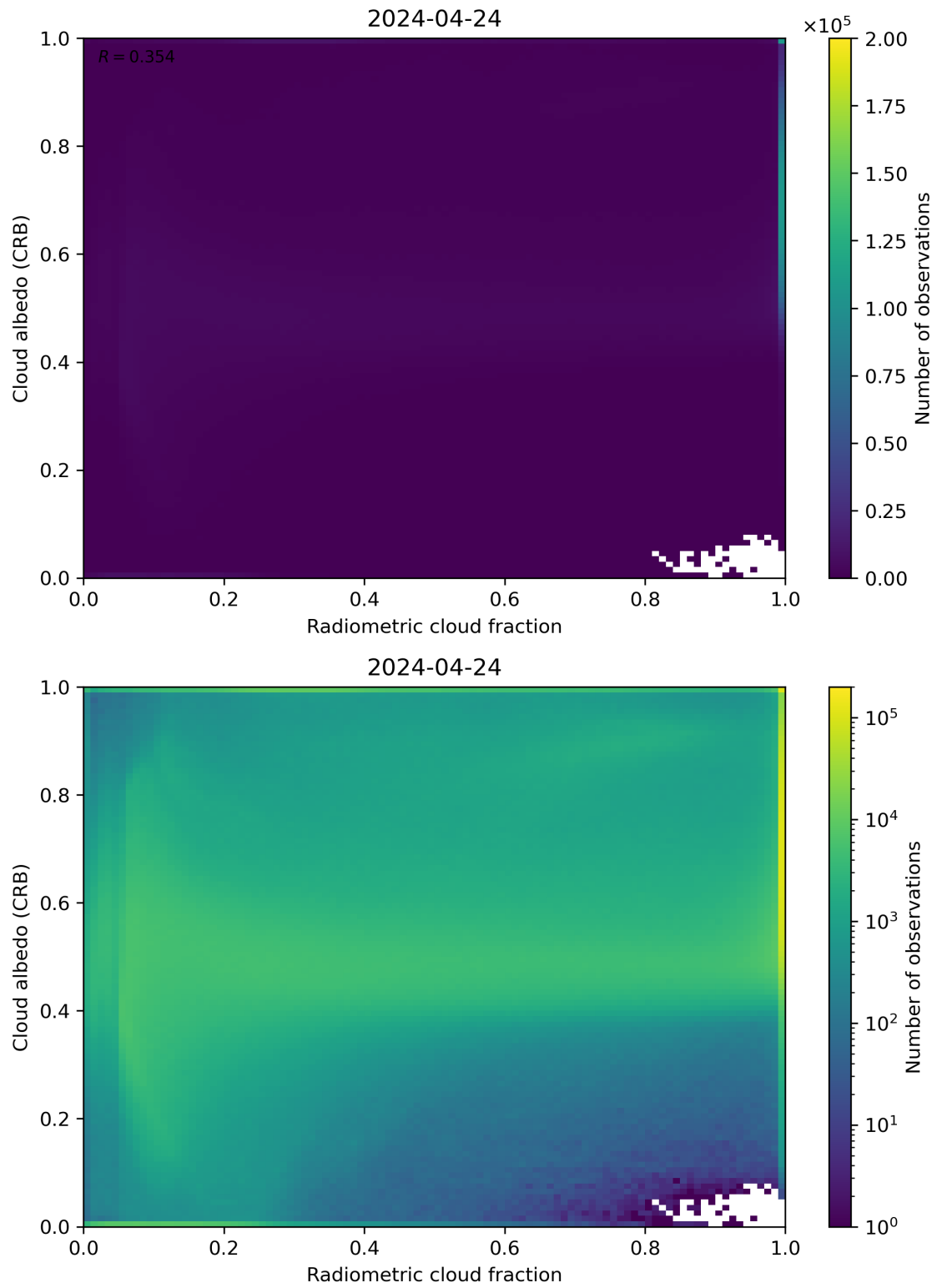
Figure 71: Scatter density plot of “Radiometric cloud fraction” against “Cloud albedo (CRB)” for 2024-04-23 to 2024-04-25.
