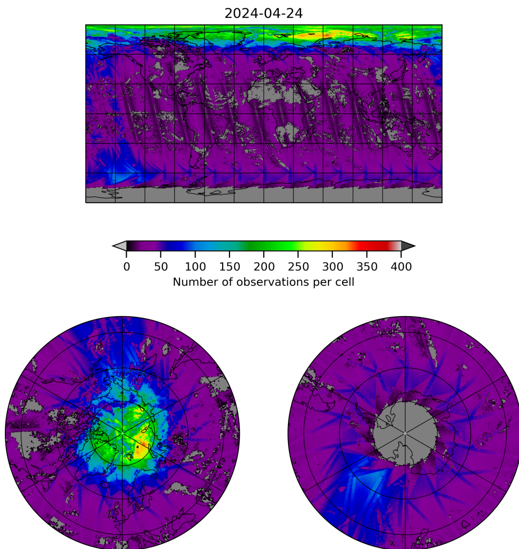
Figure 21: Map of the number of observations for 2024-04-23 to 2024-04-25
