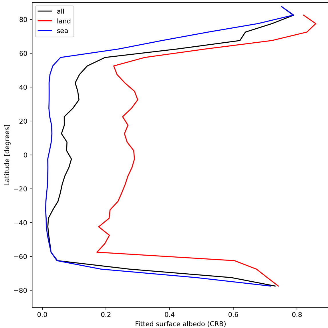
Figure 30: Zonal average of “Fitted surface albedo (CRB)” for 2024-04-23 to 2024-04-25.
