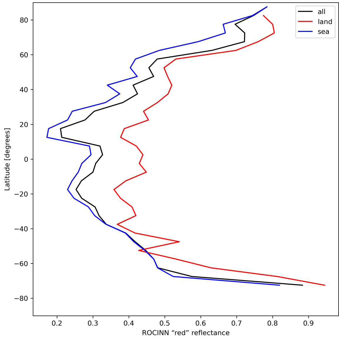
Figure 37: Zonal average of “ROCINN “red” reflectance” for 2024-04-26 to 2024-04-28.
