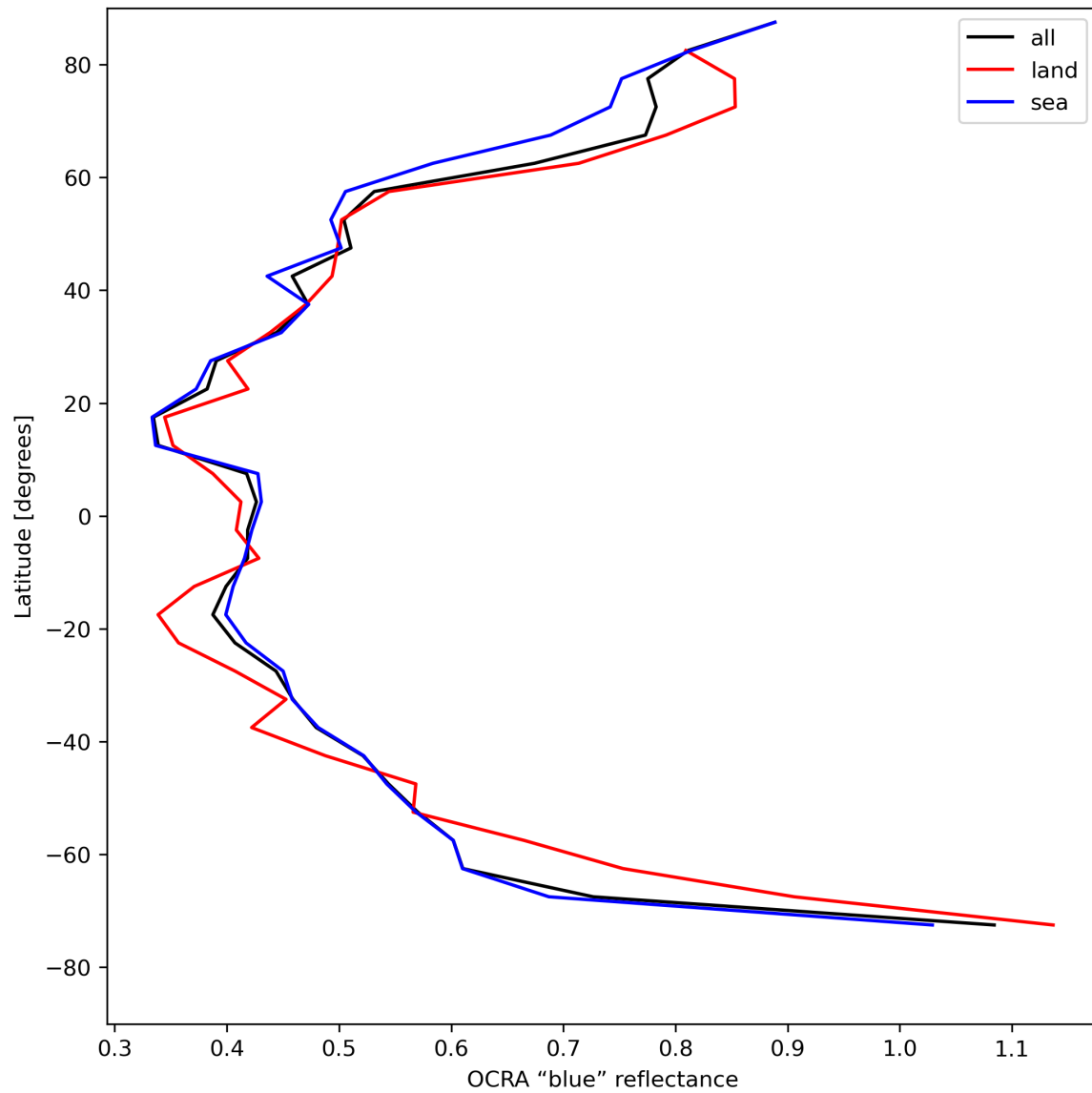
Figure 35: Zonal average of “OCRA “blue” reflectance” for 2024-04-26 to 2024-04-28.
