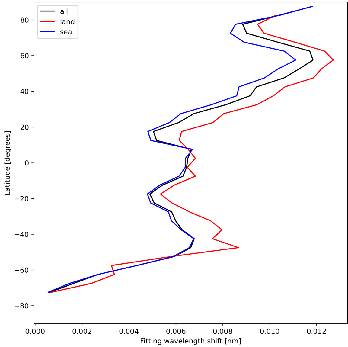
Figure 33: Zonal average of “Fitting wavelength shift” for 2024-04-26 to 2024-04-28.
