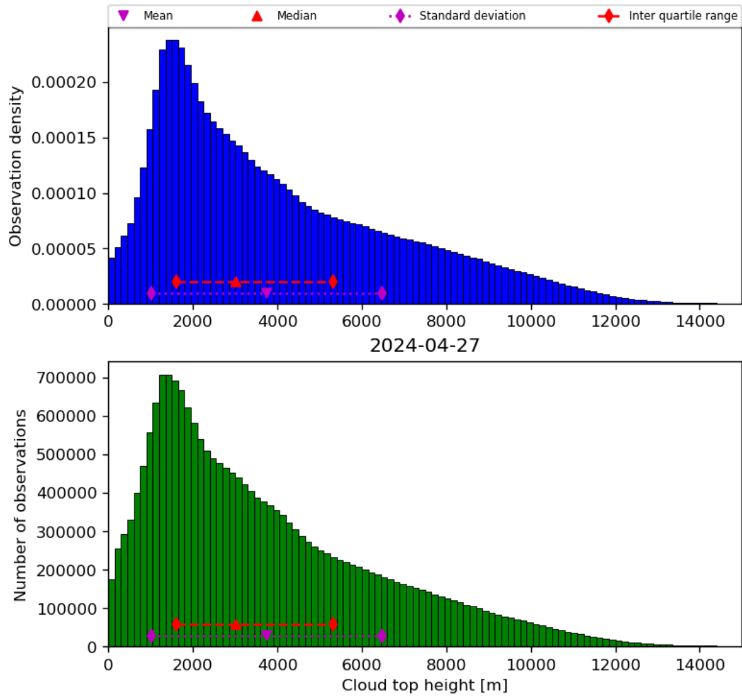
Figure 40: Histogram of “Cloud top height” for 2024-04-26 to 2024-04-28
