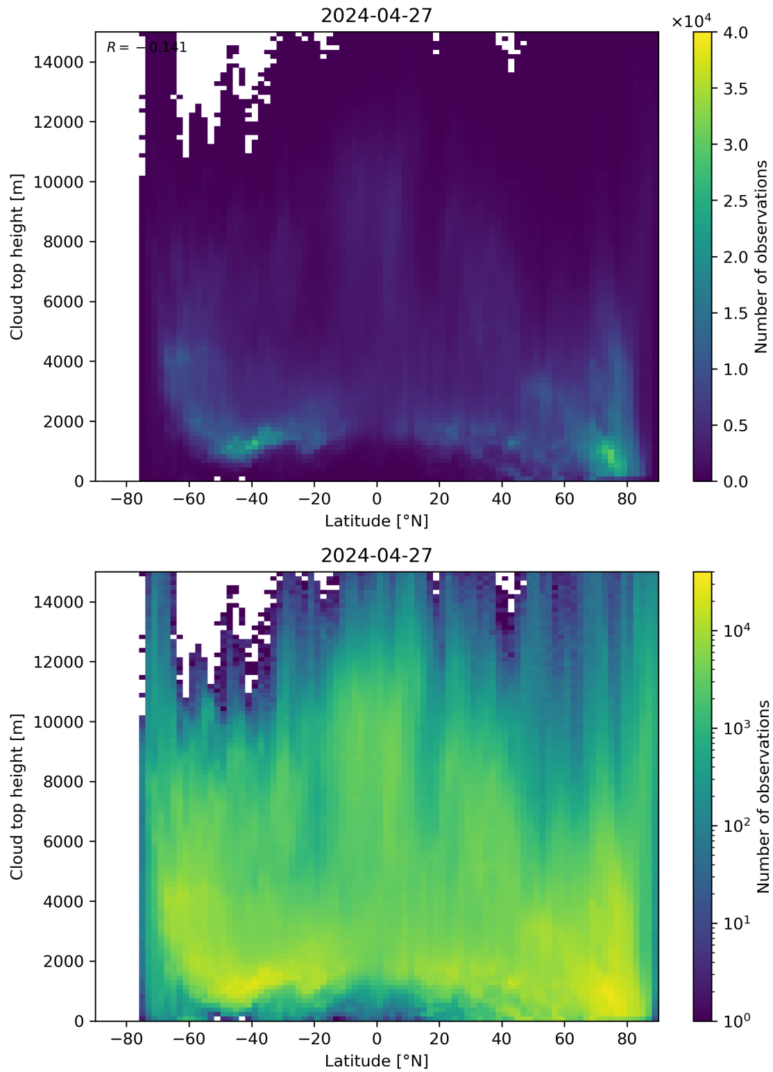
Figure 97: Scatter density plot of “Latitude” against “Cloud top height” for 2024-04-26 to 2024-04-28.
