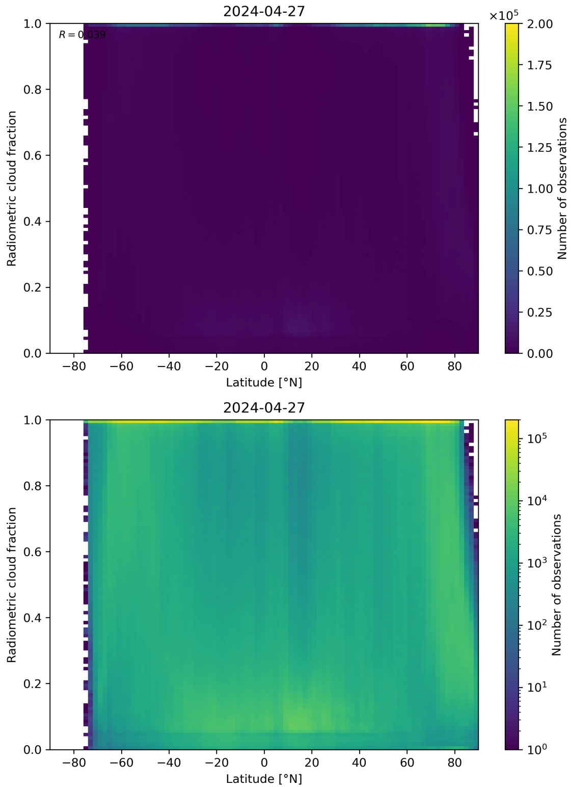
Figure 92: Scatter density plot of “Latitude” against “Radiometric cloud fraction” for 2024-04-26 to 2024-04-28.
