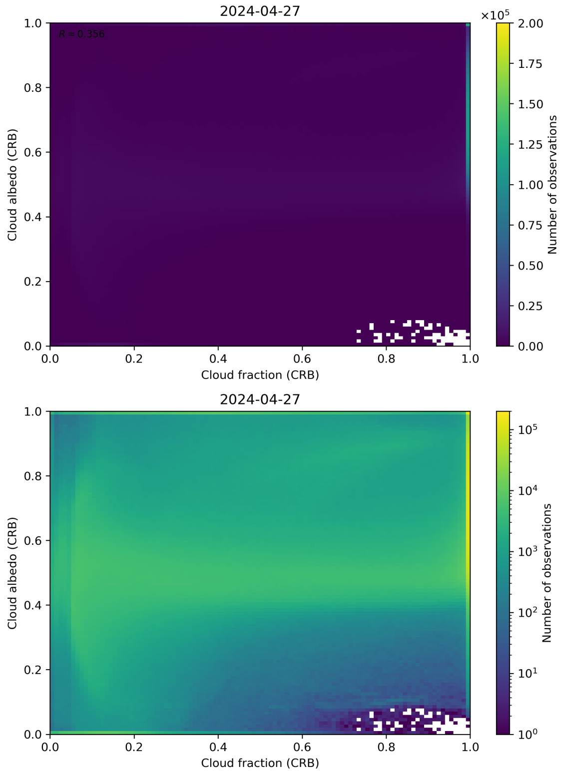
Figure 77: Scatter density plot of “Cloud fraction (CRB)” against “Cloud albedo (CRB)” for 2024-04-26 to 2024-04-28.
