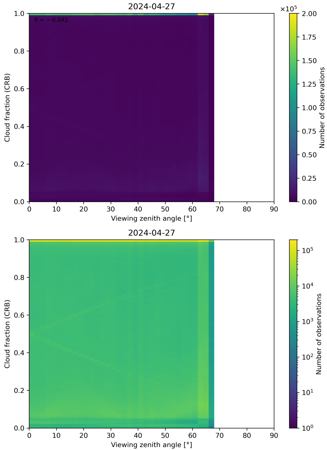
Figure 109: Scatter density plot of “Viewing zenith angle” against “Cloud fraction (CRB)” for 2024-04-26 to 2024-04-28.
