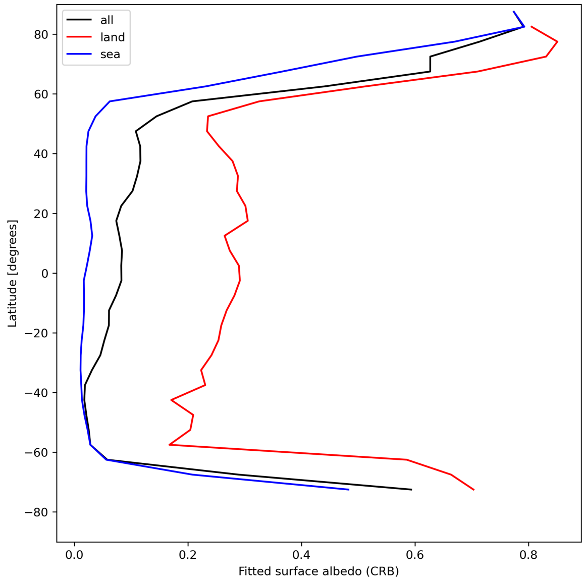
Figure 30: Zonal average of “Fitted surface albedo (CRB)” for 2024-04-26 to 2024-04-28.
