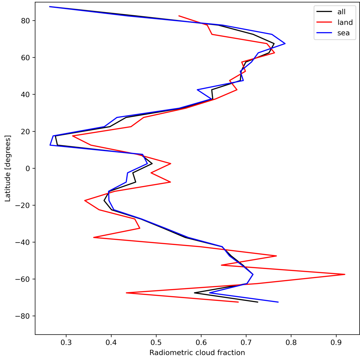
Figure 23: Zonal average of “Radiometric cloud fraction” for 2024-04-26 to 2024-04-28.
