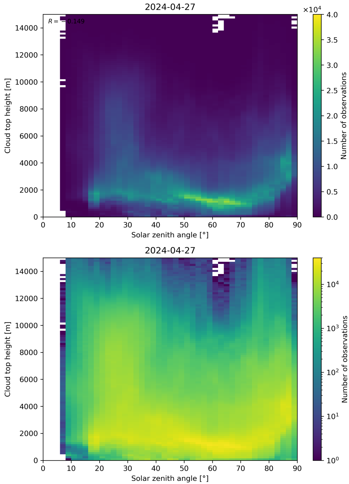
Figure 104: Scatter density plot of “Solar zenith angle” against “Cloud top height” for 2024-04-26 to 2024-04-28.
