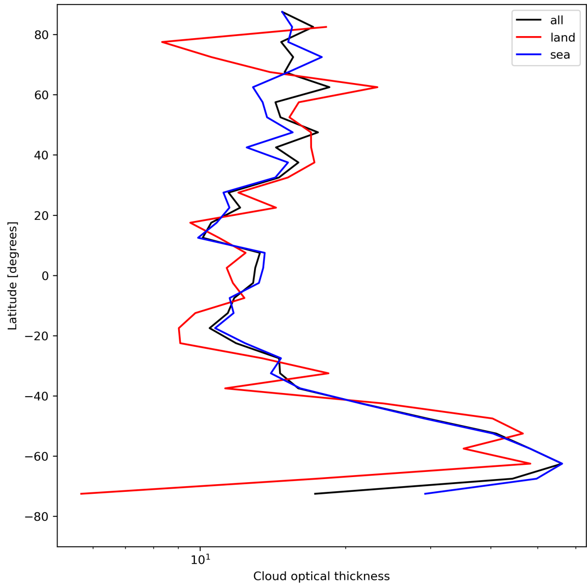
Figure 25: Zonal average of “Cloud optical thickness” for 2024-04-26 to 2024-04-28.
