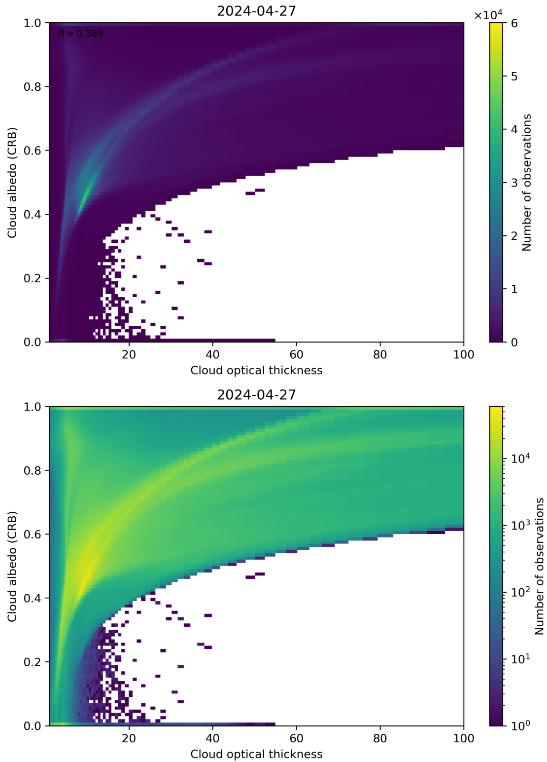
Figure 82: Scatter density plot of “Cloud optical thickness” against “Cloud albedo (CRB)” for 2024-04-26 to 2024-04-28.
