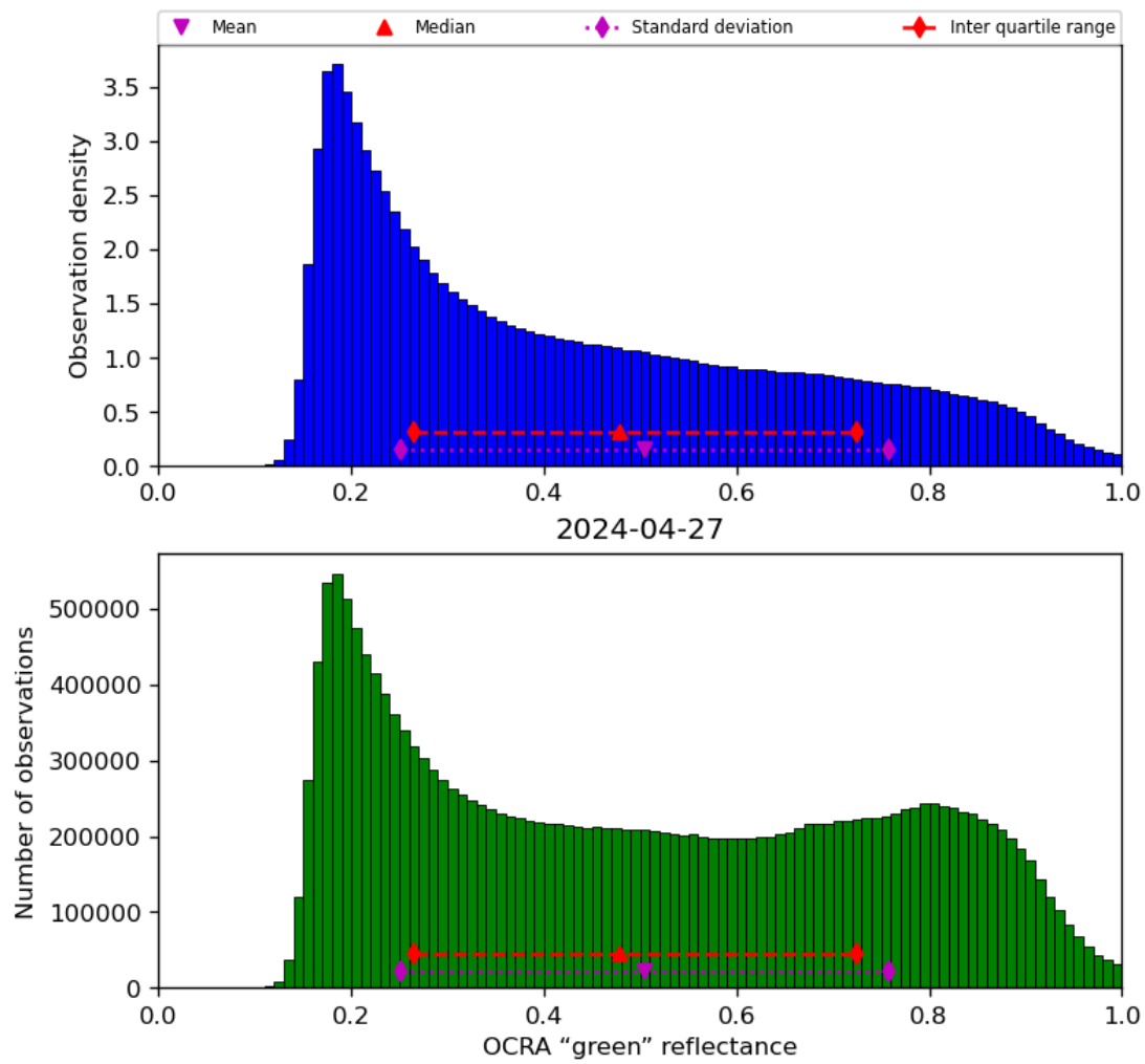
Figure 52: Histogram of “OCRA “green” reflectance” for 2024-04-26 to 2024-04-28
