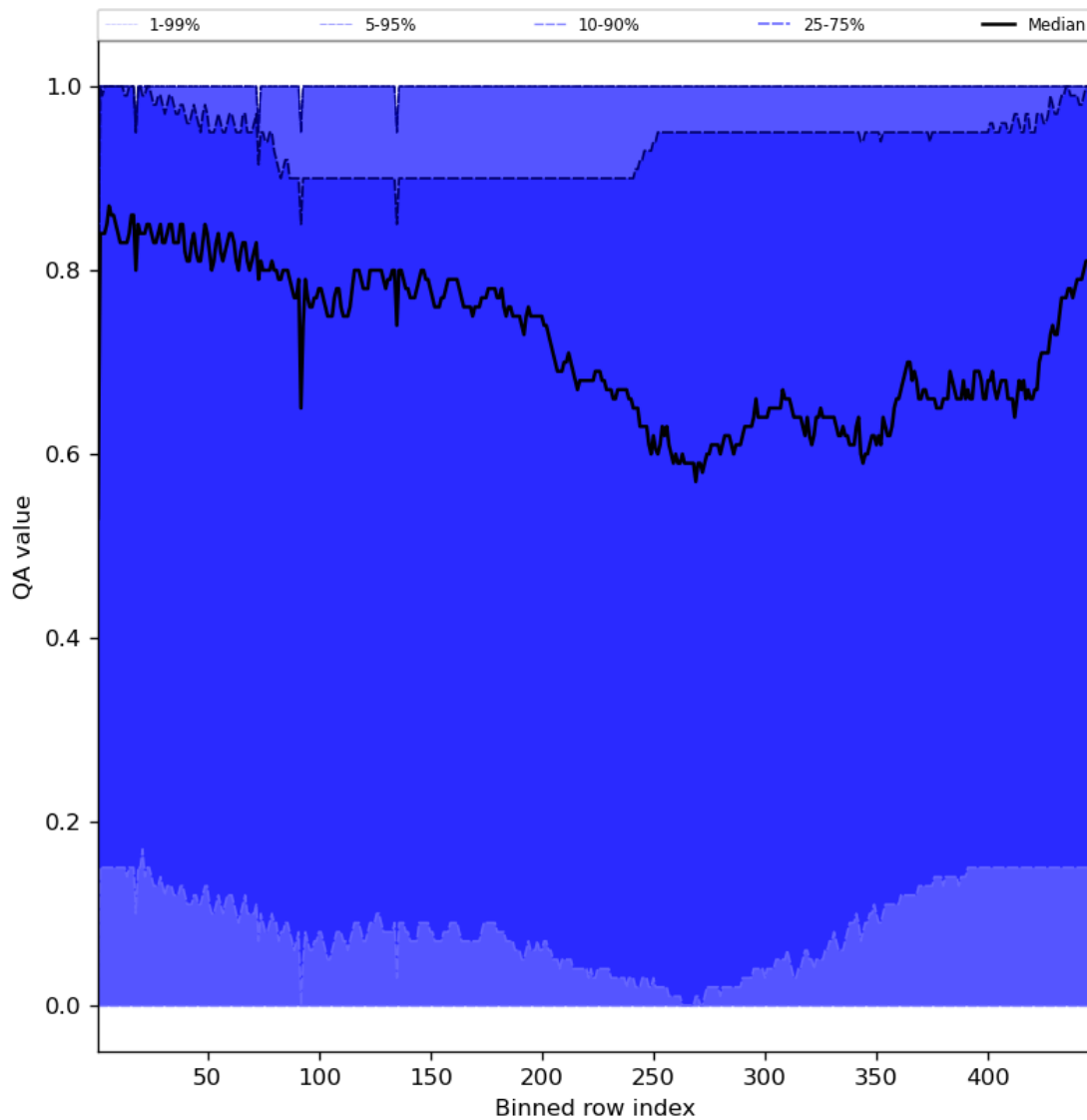
Figure 54: Along track statistics of “QA value” for 2024-04-26 to 2024-04-28
