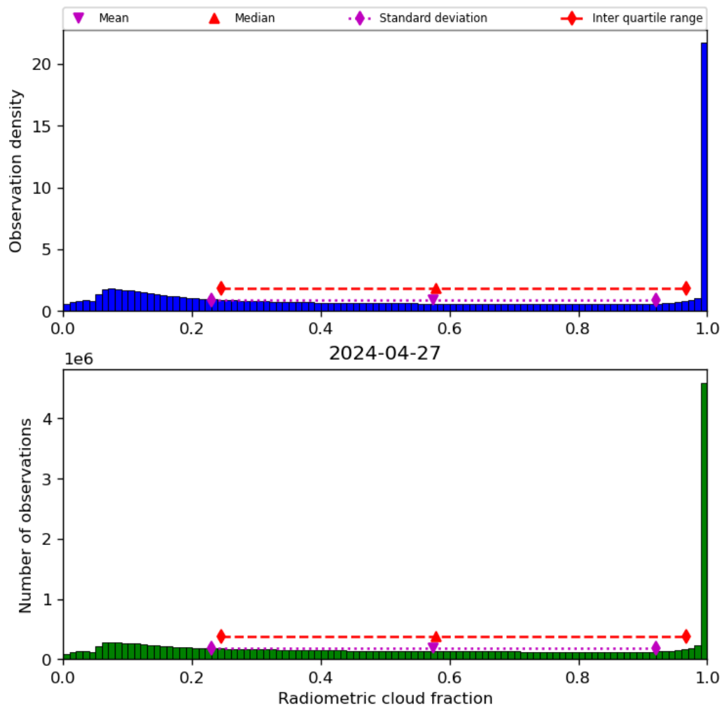
Figure 39: Histogram of “Radiometric cloud fraction” for 2024-04-26 to 2024-04-28
