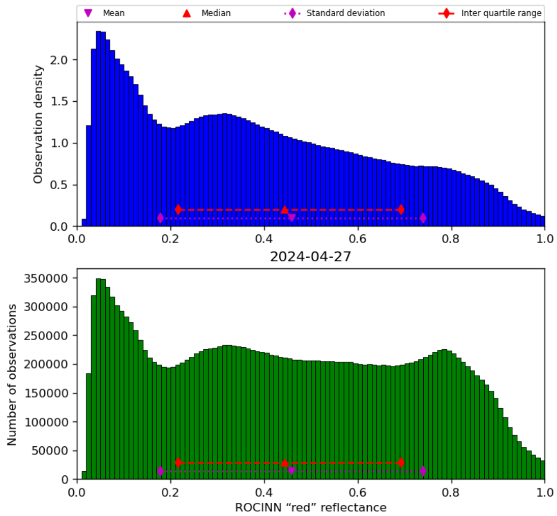
Figure 53: Histogram of “ROCINN “red” reflectance” for 2024-04-26 to 2024-04-28
