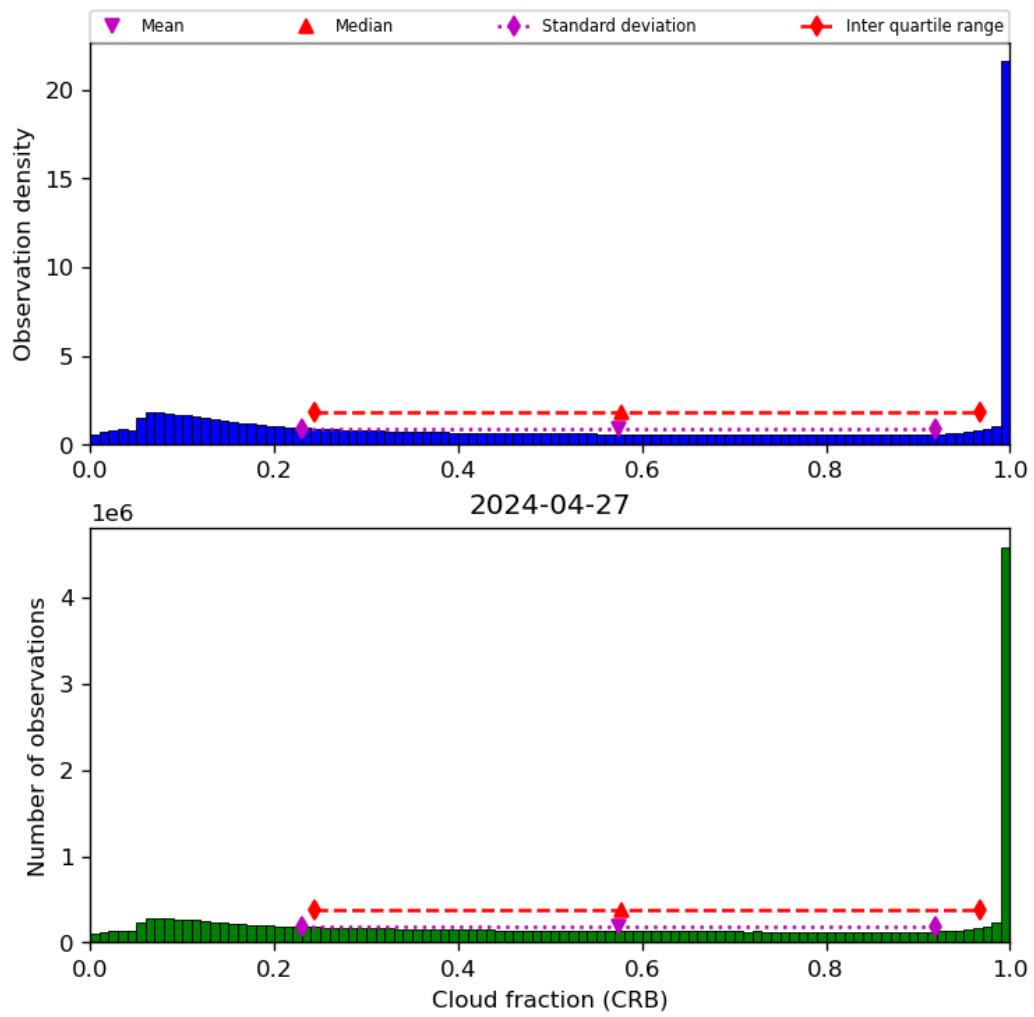
Figure 42: Histogram of “Cloud fraction (CRB)” for 2024-04-26 to 2024-04-28
