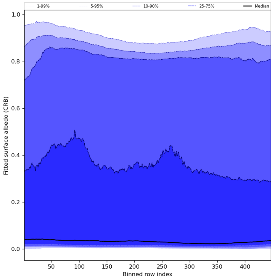
Figure 62: Along track statistics of “Fitted surface albedo (CRB)” for 2024-04-26 to 2024-04-28
