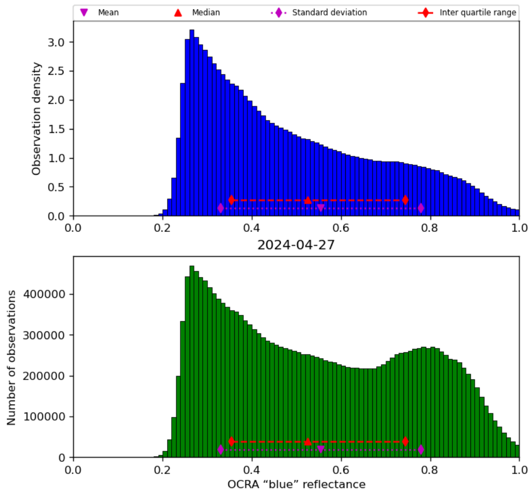
Figure 51: Histogram of “OCRA “blue” reflectance” for 2024-04-26 to 2024-04-28
