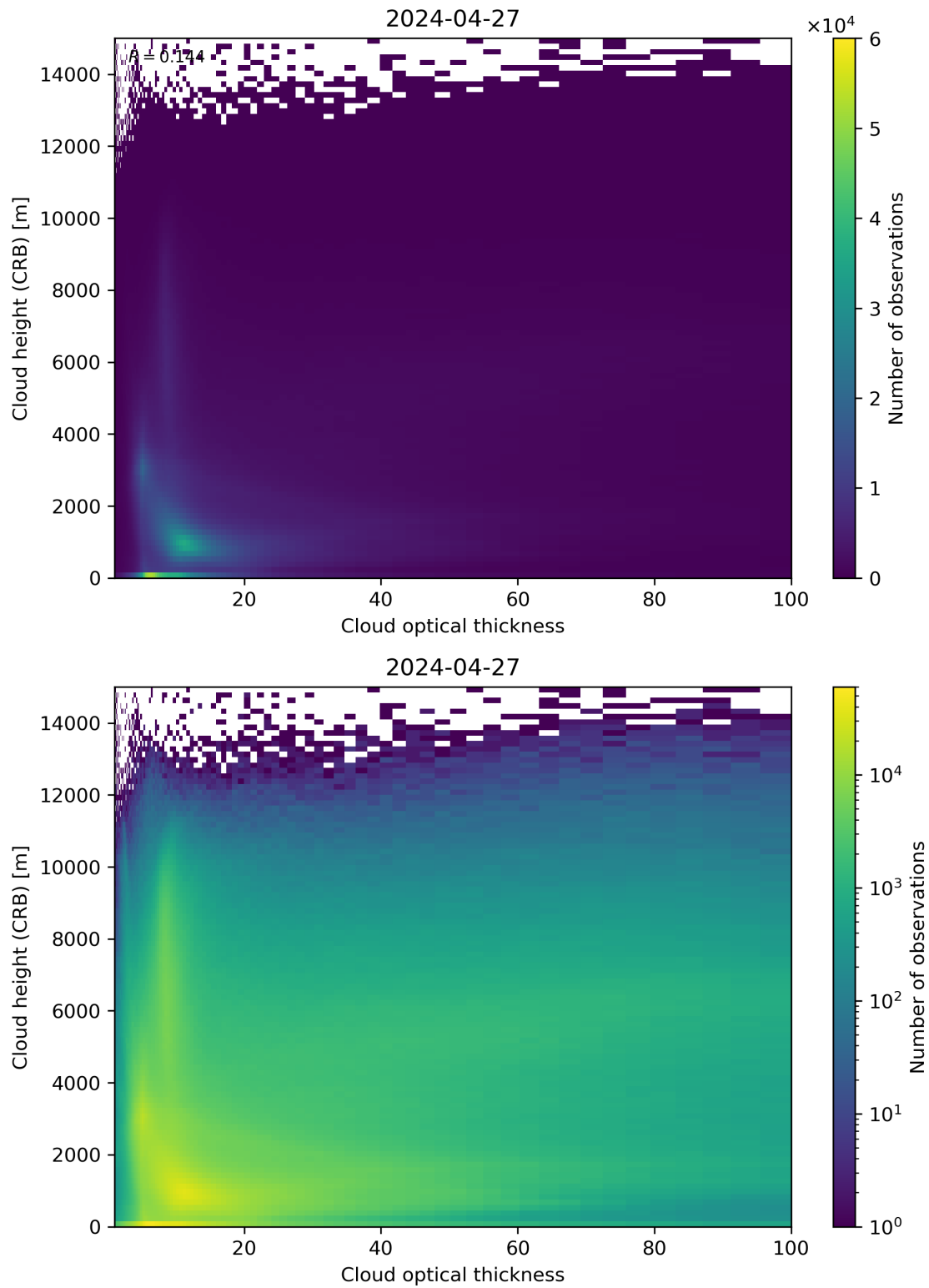
Figure 85: Scatter density plot of “Cloud optical thickness” against “Cloud height (CRB)” for 2024-04-26 to 2024-04-28.
