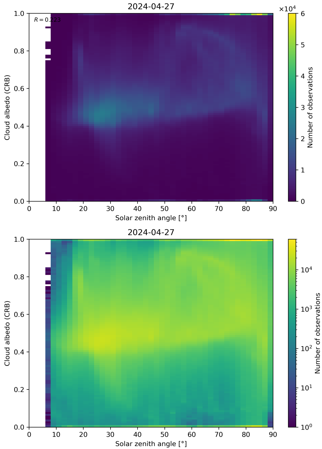
Figure 98: Scatter density plot of “Solar zenith angle” against “Cloud albedo (CRB)” for 2024-04-26 to 2024-04-28.
