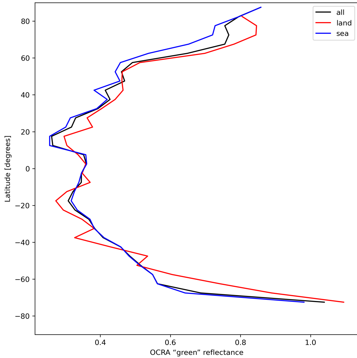
Figure 36: Zonal average of “OCRA “green” reflectance” for 2024-04-26 to 2024-04-28.
