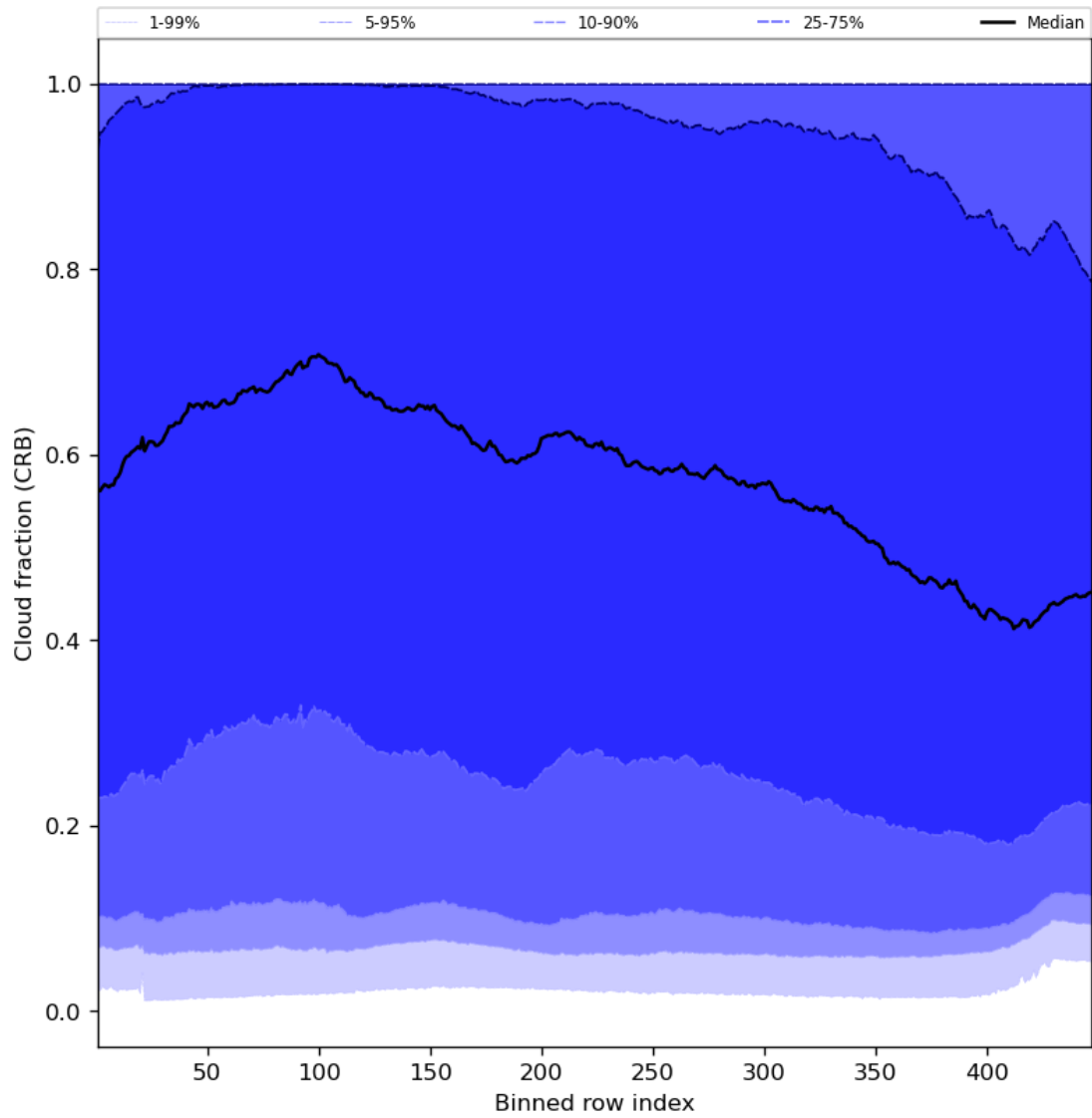
Figure 58: Along track statistics of “Cloud fraction (CRB)” for 2024-04-26 to 2024-04-28
