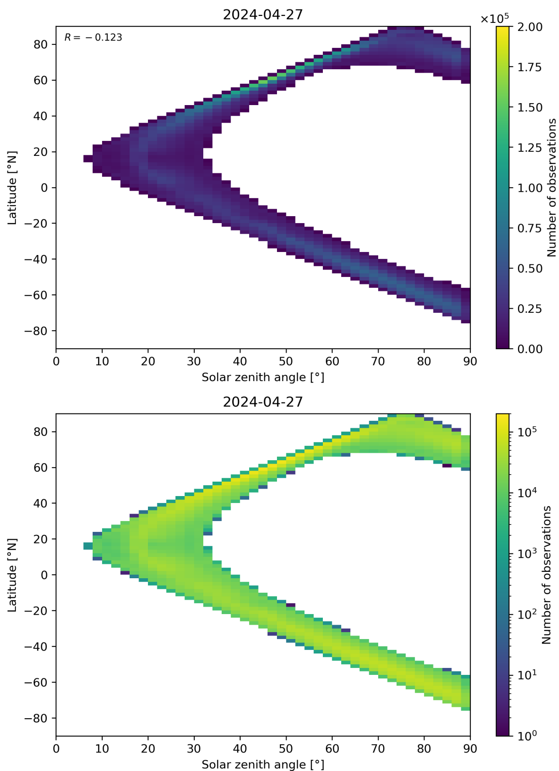
Figure 105: Scatter density plot of “Solar zenith angle” against “Latitude” for 2024-04-26 to 2024-04-28.
