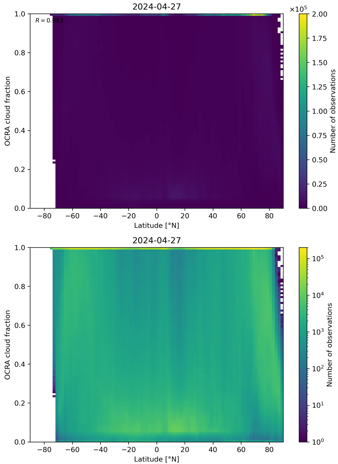
Figure 93: Scatter density plot of “Latitude” against “OCRA cloud fraction” for 2024-04-26 to 2024-04-28.
