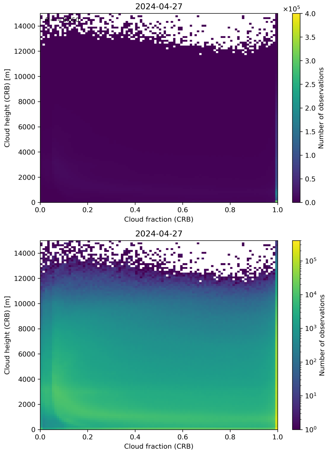
Figure 79: Scatter density plot of “Cloud fraction (CRB)” against “Cloud height (CRB)” for 2024-04-26 to 2024-04-28.
