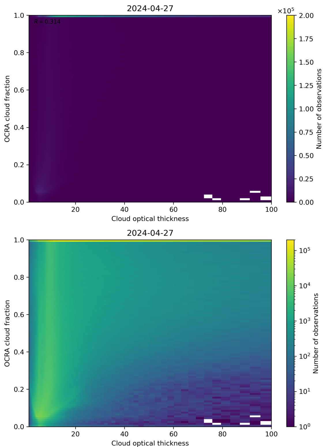
Figure 83: Scatter density plot of “Cloud optical thickness” against “OCRA cloud fraction” for 2024-04-26 to 2024-04-28.
