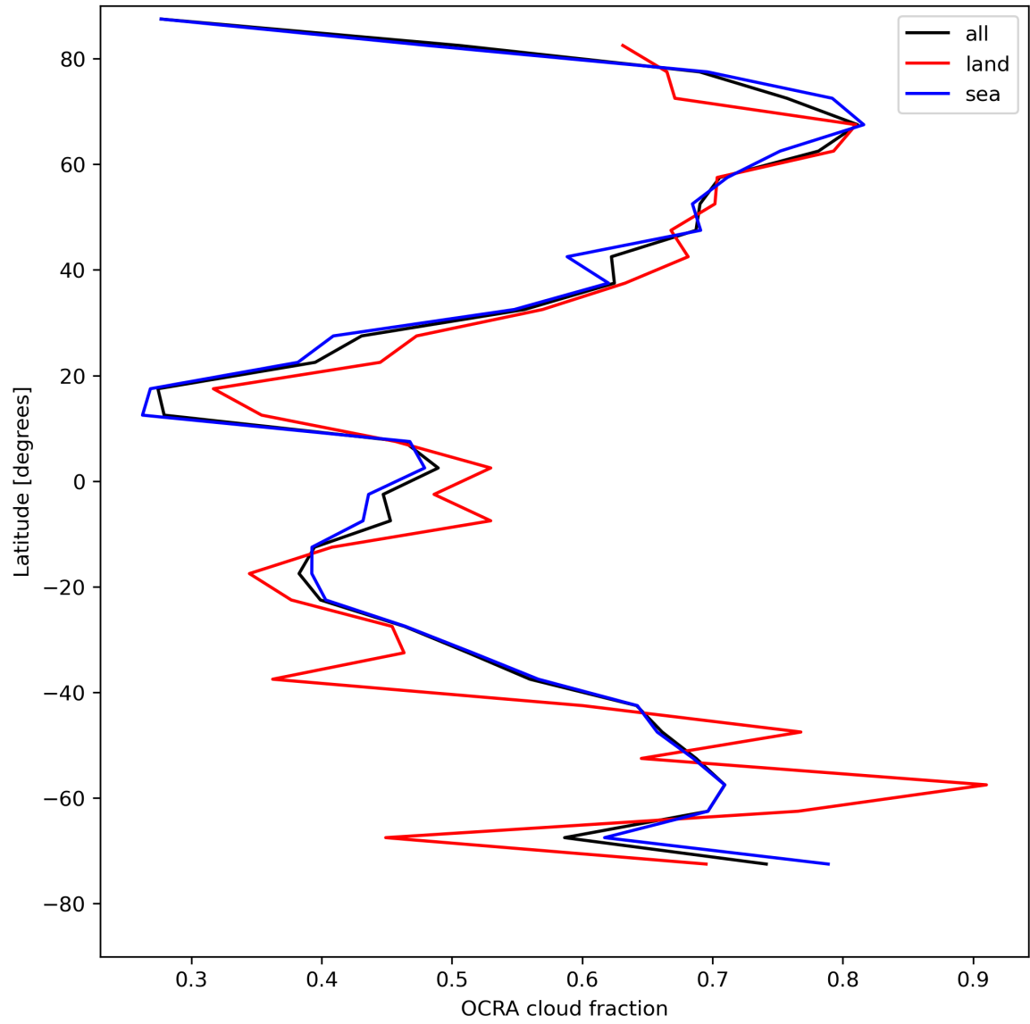
Figure 34: Zonal average of “OCRA cloud fraction” for 2024-04-26 to 2024-04-28.
