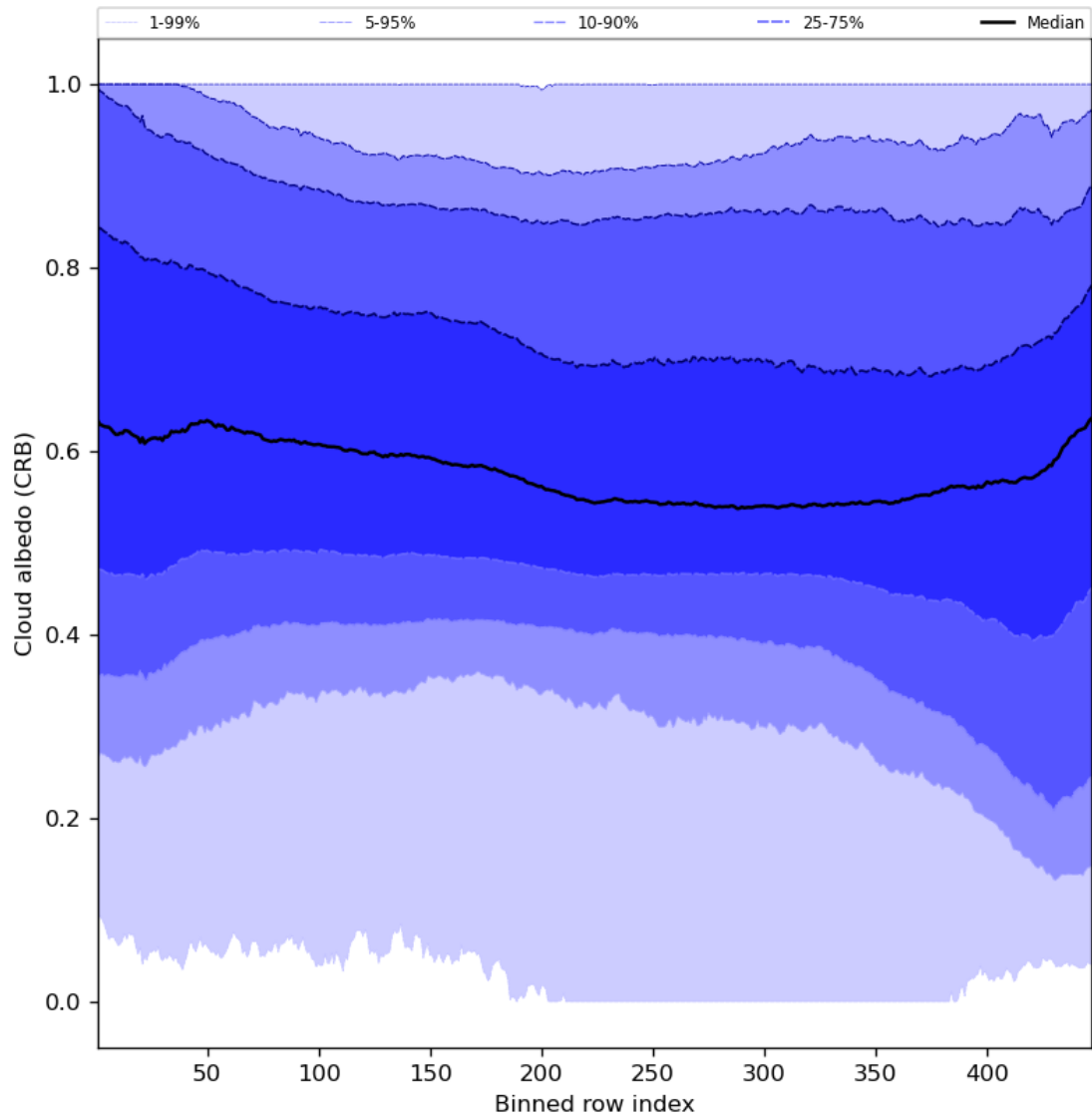
Figure 60: Along track statistics of “Cloud albedo (CRB)” for 2024-04-26 to 2024-04-28
