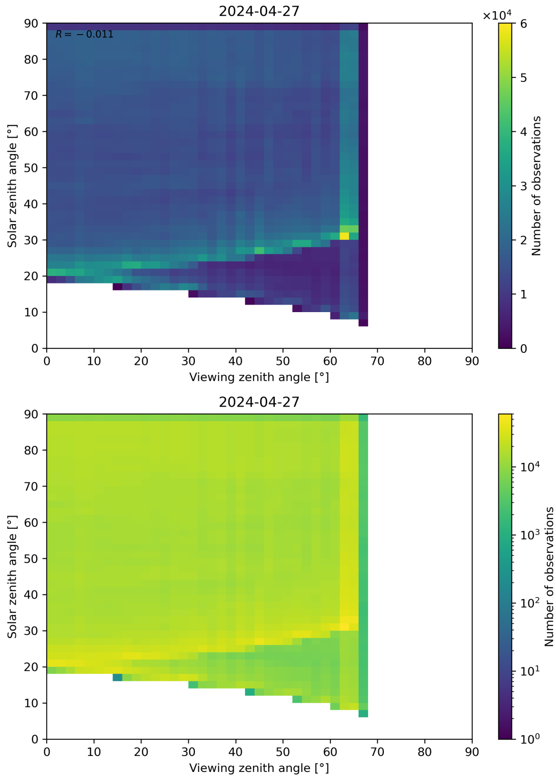
Figure 114: Scatter density plot of “Viewing zenith angle” against “Solar zenith angle” for 2024-04-26 to 2024-04-28.
