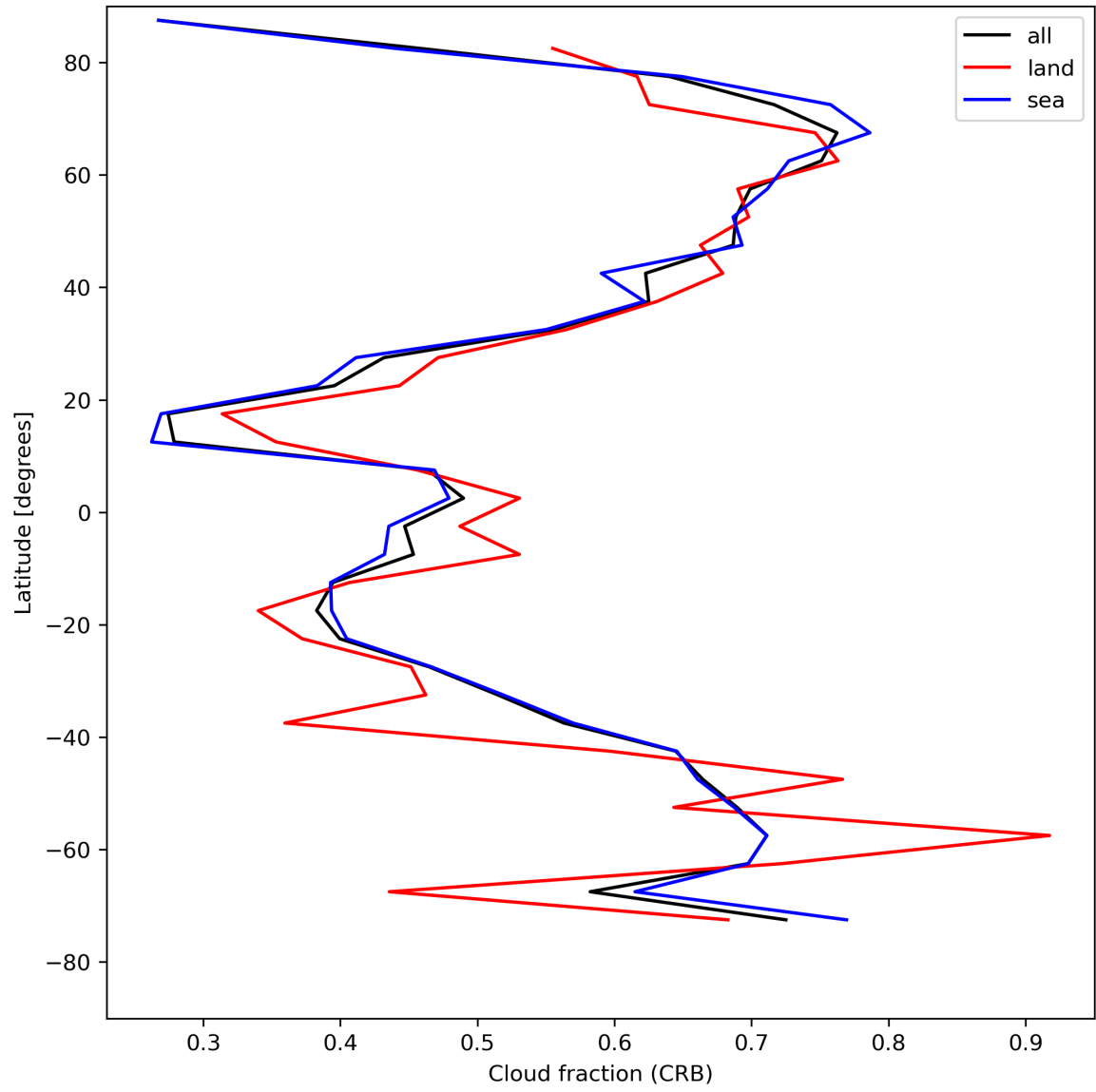
Figure 26: Zonal average of “Cloud fraction (CRB)” for 2024-04-26 to 2024-04-28.
