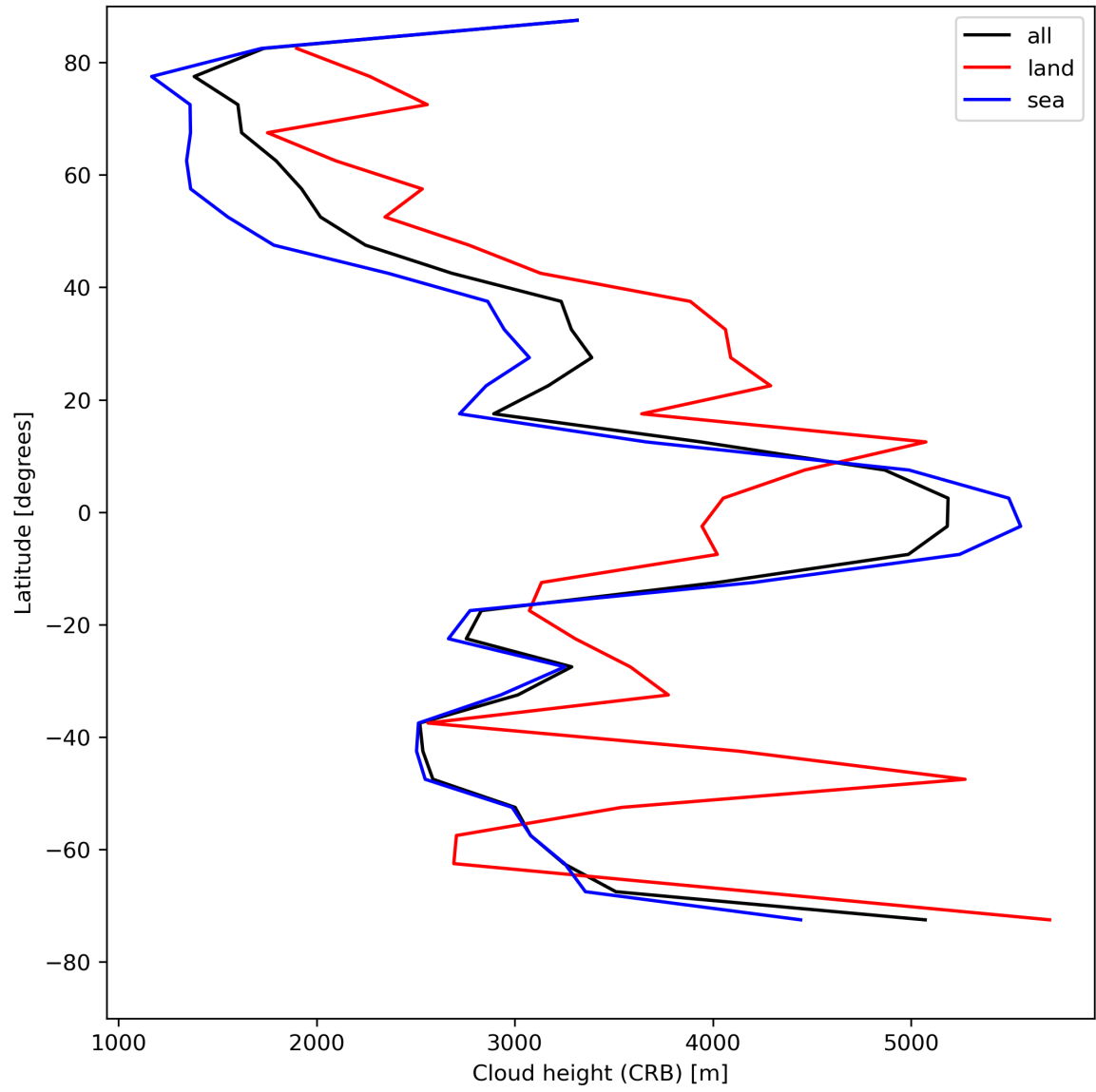
Figure 27: Zonal average of “Cloud height (CRB)” for 2024-04-26 to 2024-04-28.
