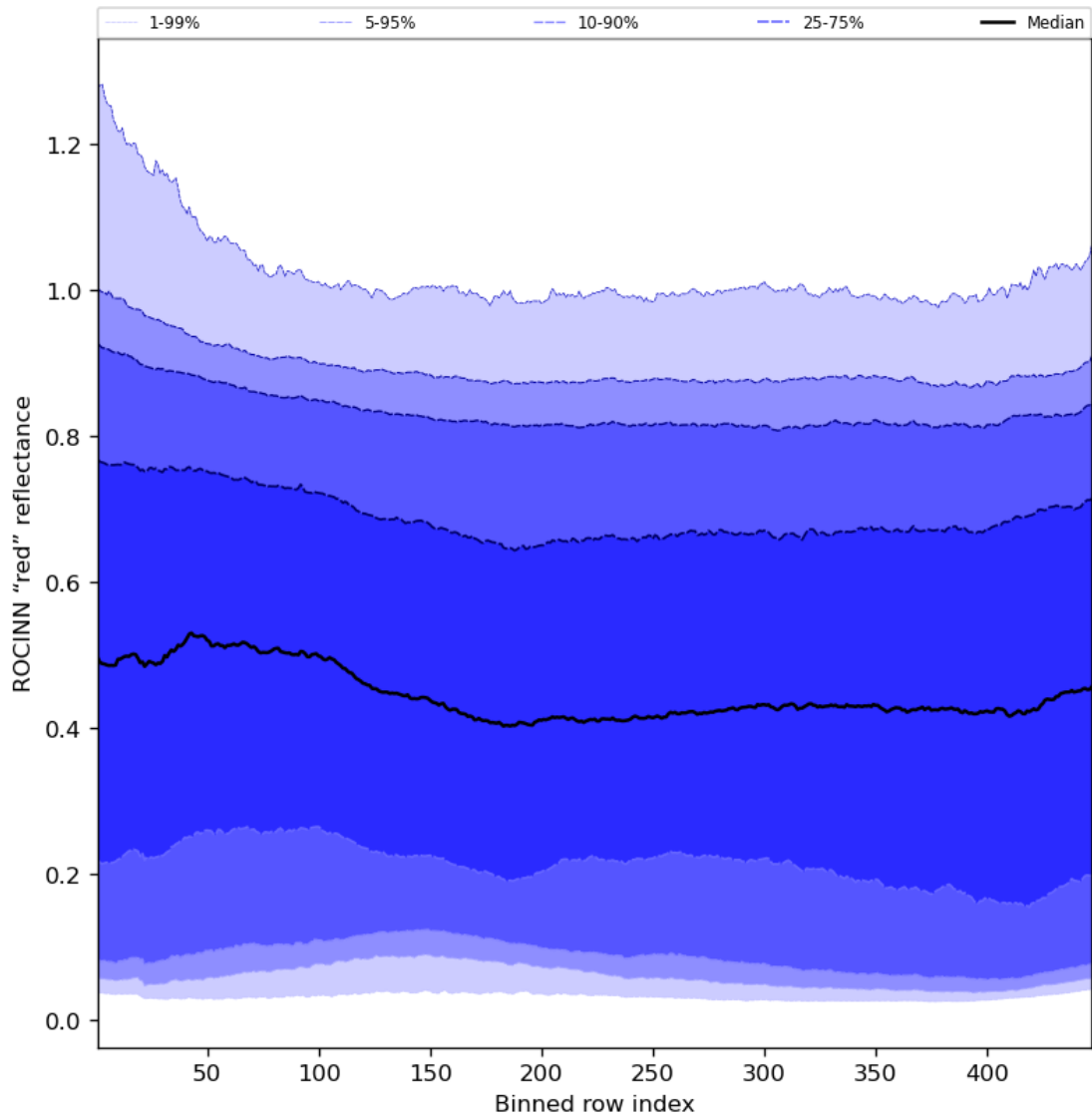
Figure 69: Along track statistics of “ROCINN “red” reflectance” for 2024-04-26 to 2024-04-28
