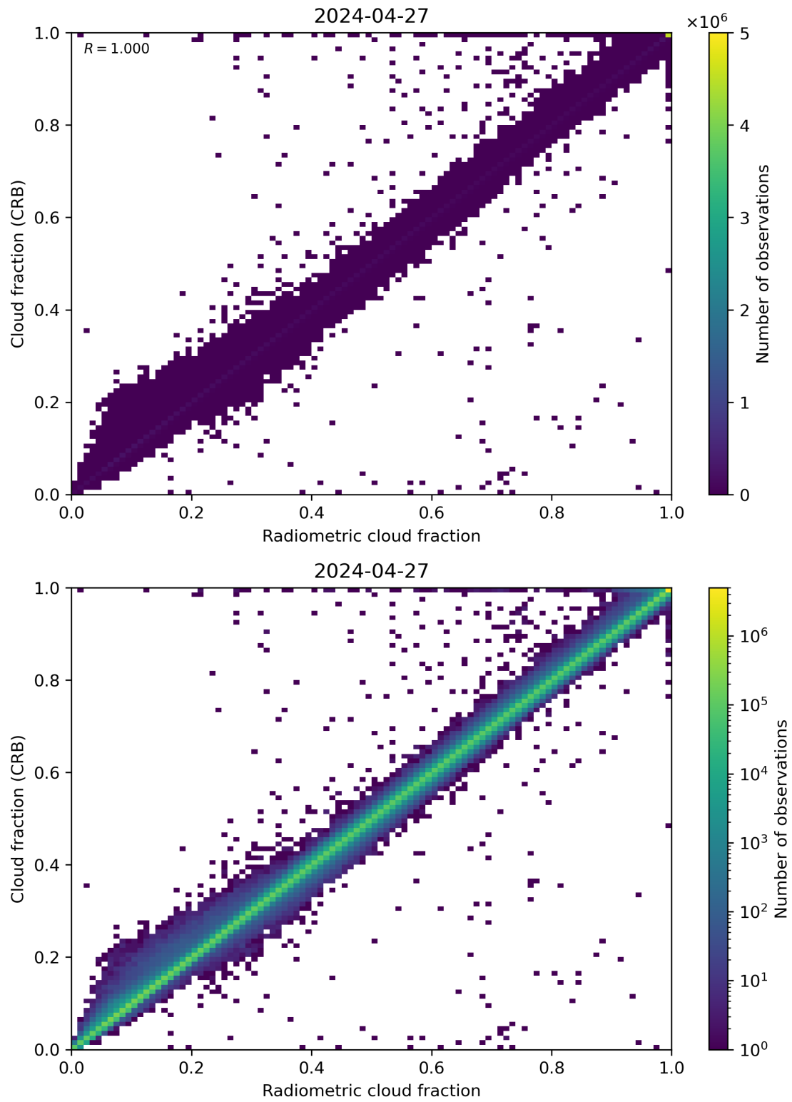
Figure 73: Scatter density plot of “Radiometric cloud fraction” against “Cloud fraction (CRB)” for 2024-04-26 to 2024-04-28.
