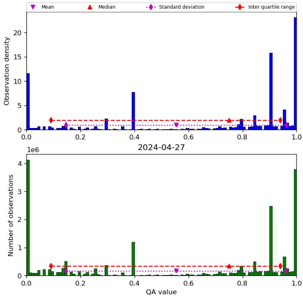
Figure 38: Histogram of “QA value” for 2024-04-26 to 2024-04-28
