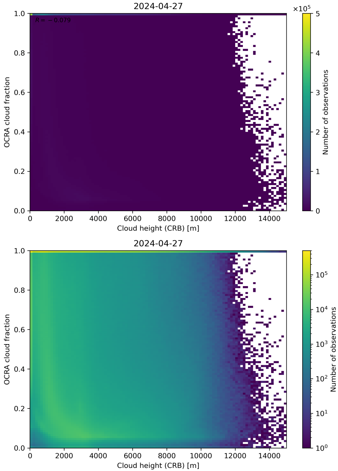
Figure 81: Scatter density plot of “Cloud height (CRB)” against “OCRA cloud fraction” for 2024-04-26 to 2024-04-28.
