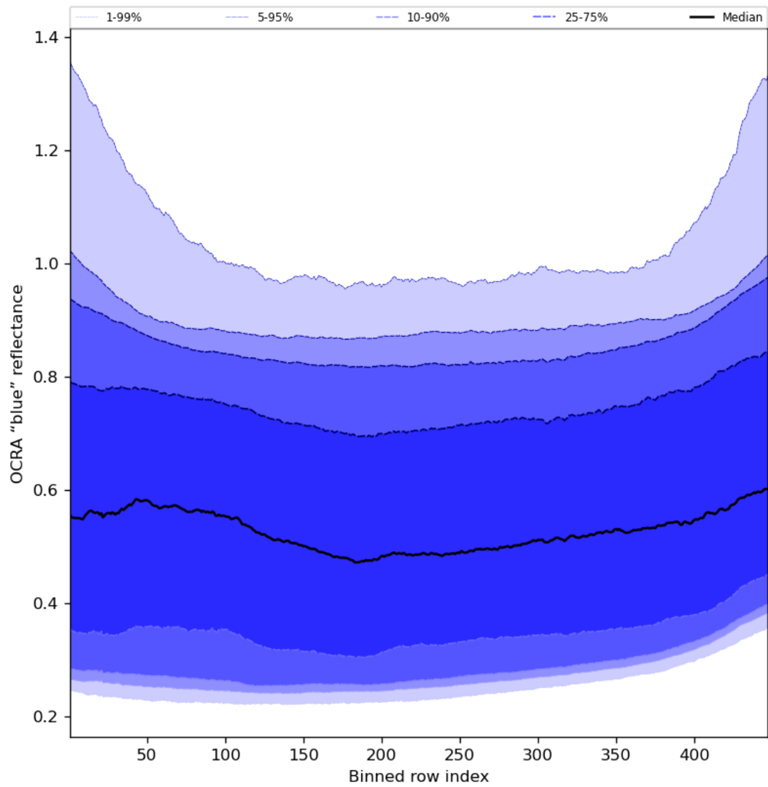
Figure 67: Along track statistics of “OCRA “blue” reflectance” for 2024-04-26 to 2024-04-28
