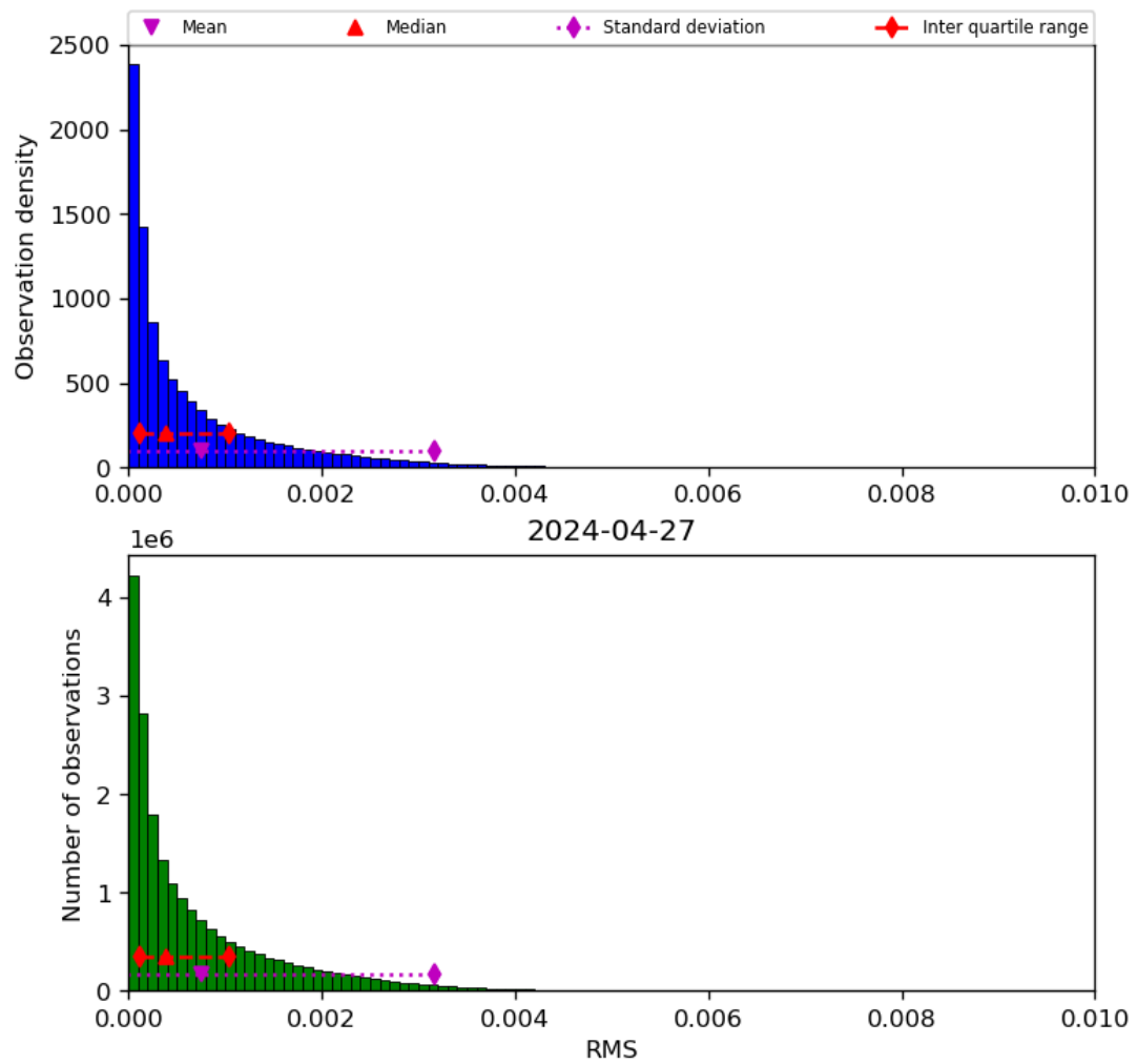
Figure 47: Histogram of “RMS” for 2024-04-26 to 2024-04-28
