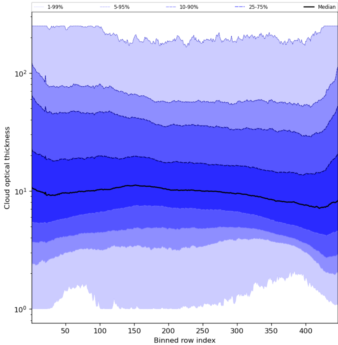
Figure 57: Along track statistics of “Cloud optical thickness” for 2024-04-26 to 2024-04-28
