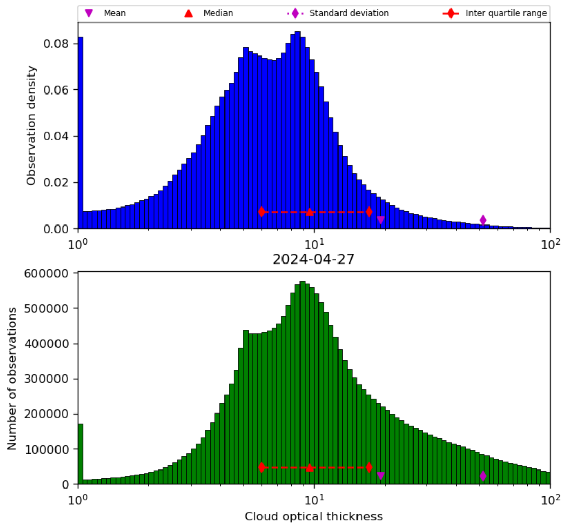
Figure 41: Histogram of “Cloud optical thickness” for 2024-04-26 to 2024-04-28
