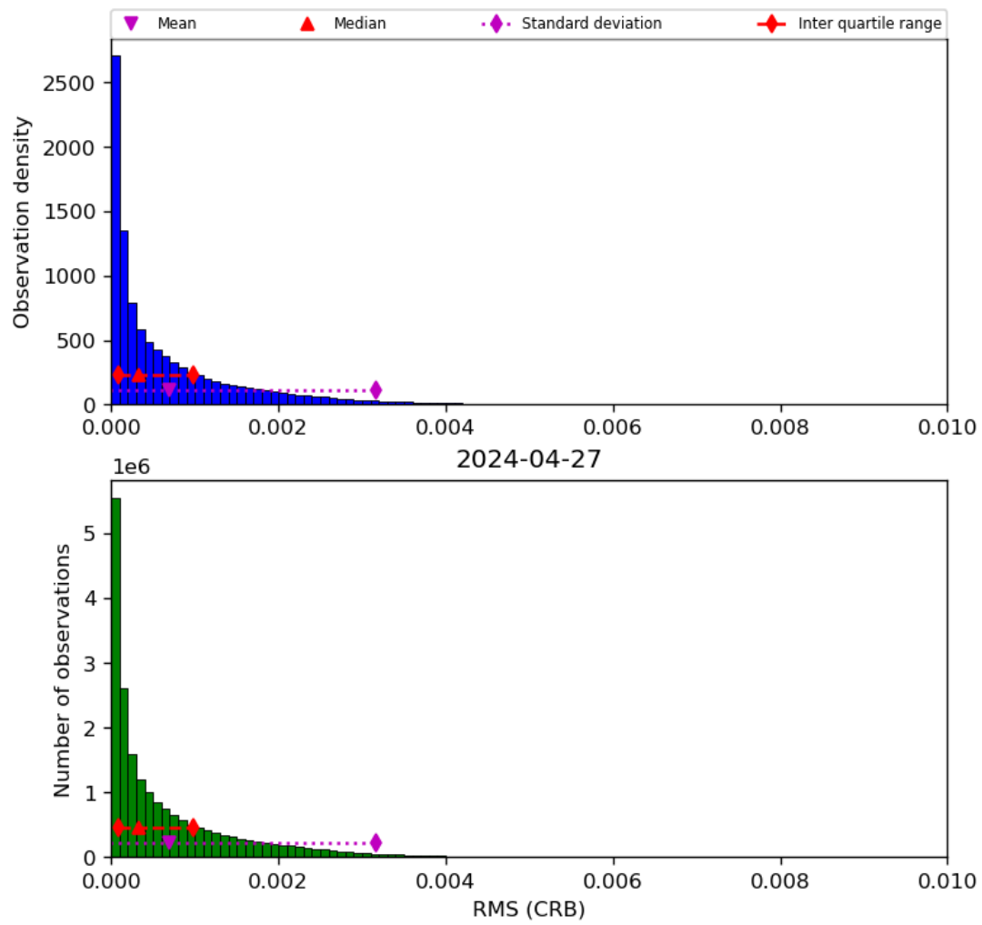
Figure 48: Histogram of “RMS (CRB)” for 2024-04-26 to 2024-04-28
