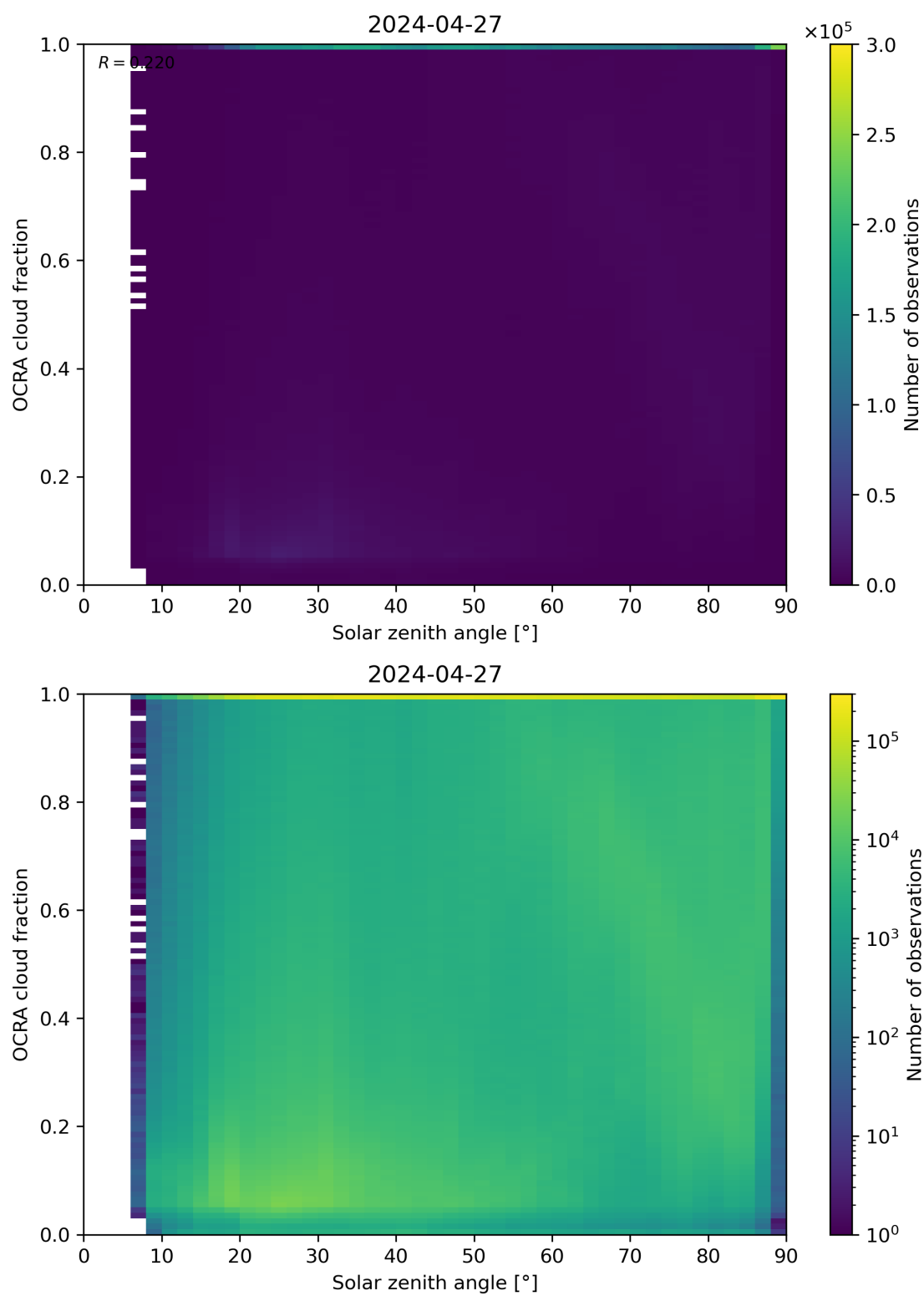
Figure 100: Scatter density plot of “Solar zenith angle” against “OCRA cloud fraction” for 2024-04-26 to 2024-04-28.
