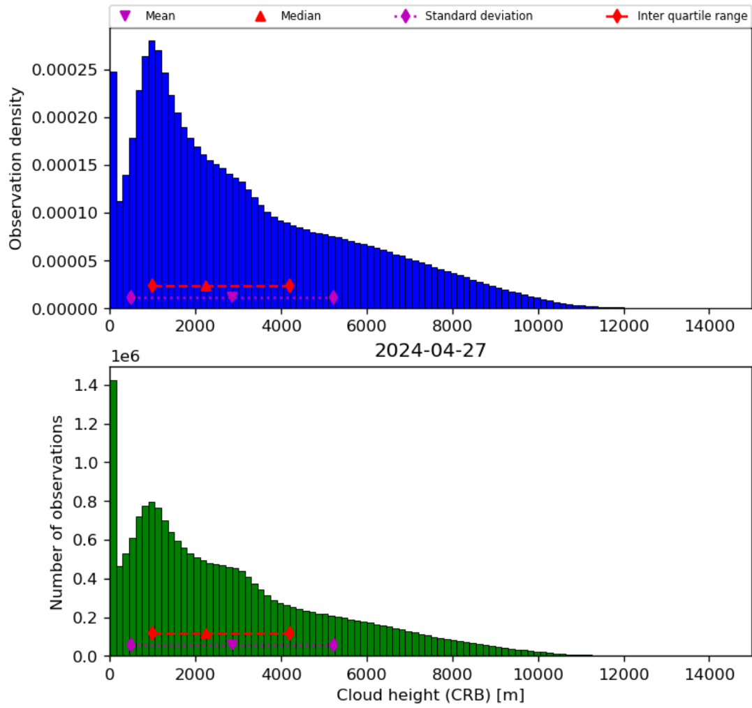
Figure 43: Histogram of “Cloud height (CRB)” for 2024-04-26 to 2024-04-28
