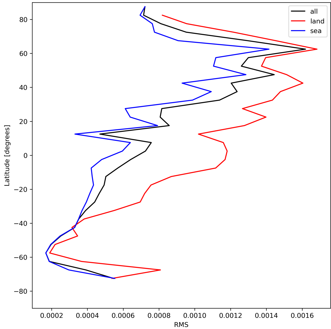
Figure 31: Zonal average of “RMS” for 2024-04-26 to 2024-04-28.
