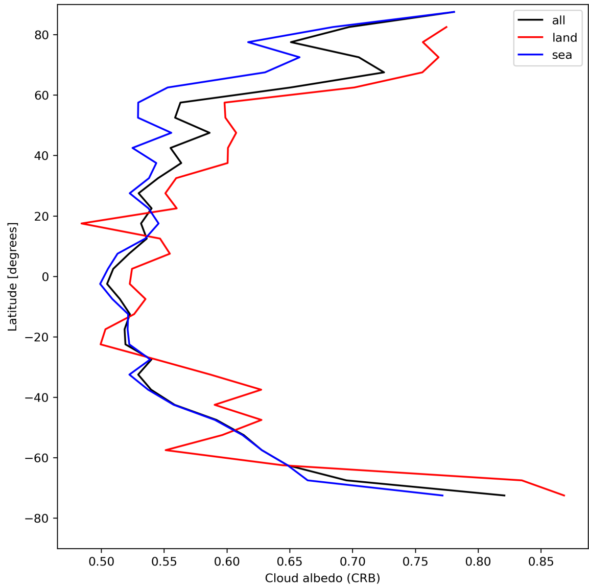
Figure 28: Zonal average of “Cloud albedo (CRB)” for 2024-04-26 to 2024-04-28.
