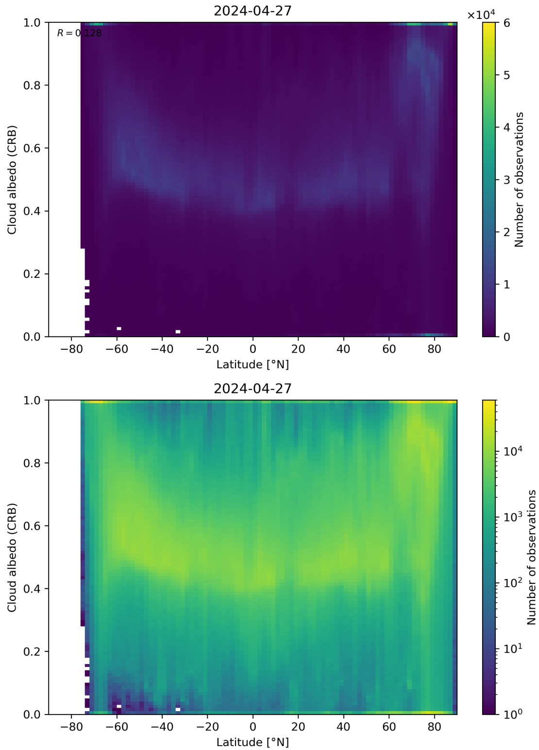
Figure 91: Scatter density plot of “Latitude” against “Cloud albedo (CRB)” for 2024-04-26 to 2024-04-28.
