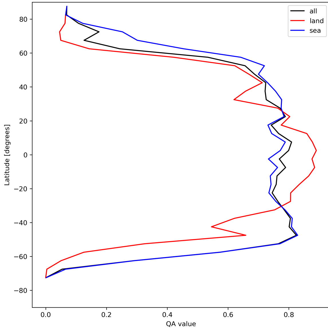
Figure 22: Zonal average of “QA value” for 2024-04-26 to 2024-04-28.
