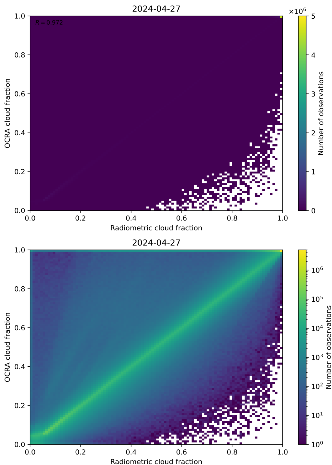
Figure 72: Scatter density plot of “Radiometric cloud fraction” against “OCRA cloud fraction” for 2024-04-26 to 2024-04-28.
