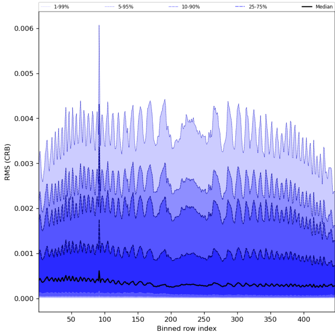
Figure 64: Along track statistics of “RMS (CRB)” for 2024-04-26 to 2024-04-28
