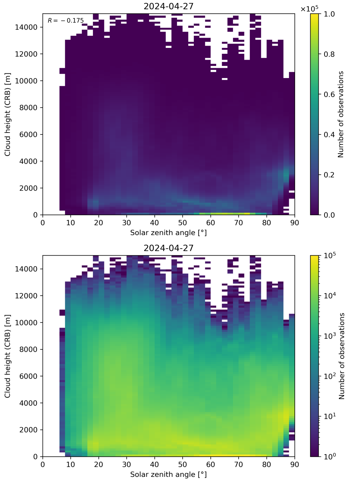
Figure 102: Scatter density plot of “Solar zenith angle” against “Cloud height (CRB)” for 2024-04-26 to 2024-04-28.
