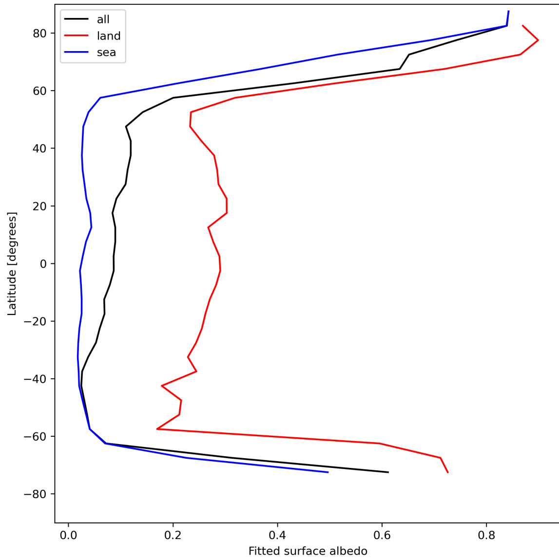
Figure 29: Zonal average of “Fitted surface albedo” for 2024-04-26 to 2024-04-28.
