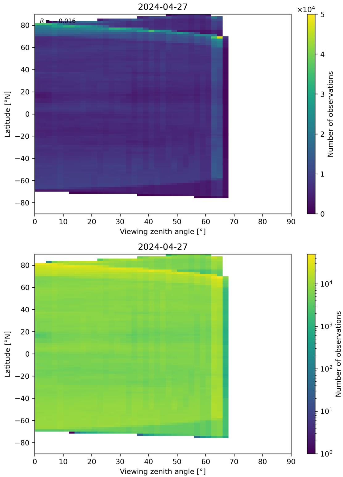
Figure 113: Scatter density plot of “Viewing zenith angle” against “Latitude” for 2024-04-26 to 2024-04-28.
