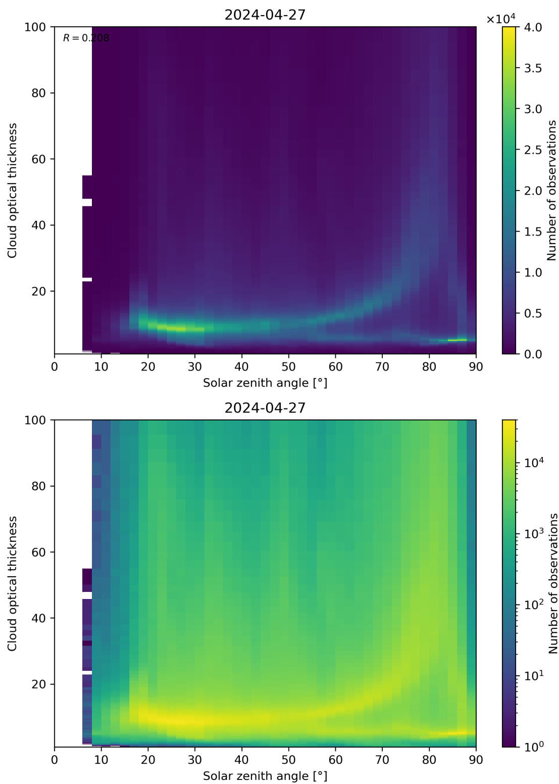
Figure 103: Scatter density plot of “Solar zenith angle” against “Cloud optical thickness” for 2024-04-26 to 2024-04-28.
