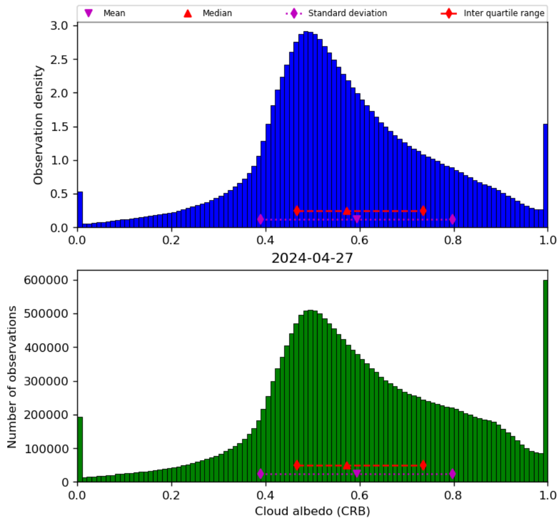
Figure 44: Histogram of “Cloud albedo (CRB)” for 2024-04-26 to 2024-04-28
