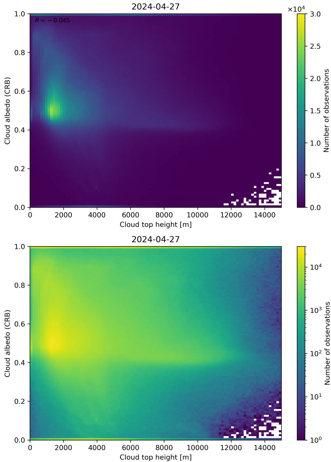
Figure 86: Scatter density plot of “Cloud top height” against “Cloud albedo (CRB)” for 2024-04-26 to 2024-04-28.
