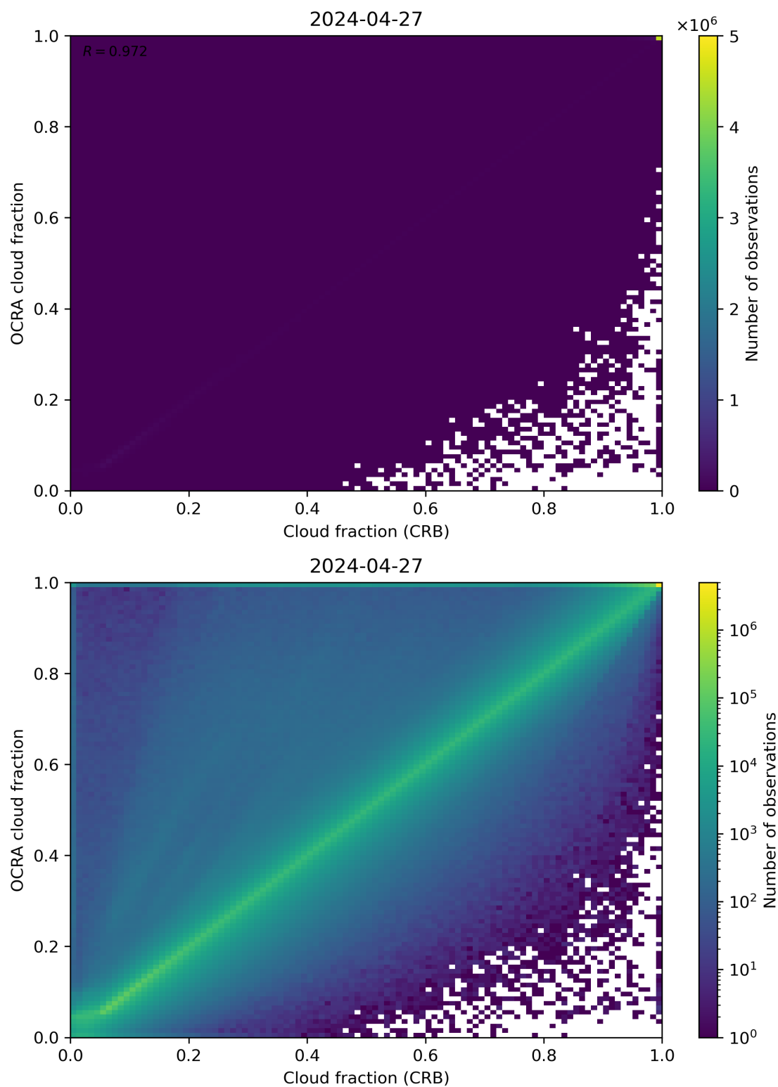
Figure 78: Scatter density plot of “Cloud fraction (CRB)” against “OCRA cloud fraction” for 2024-04-26 to 2024-04-28.
