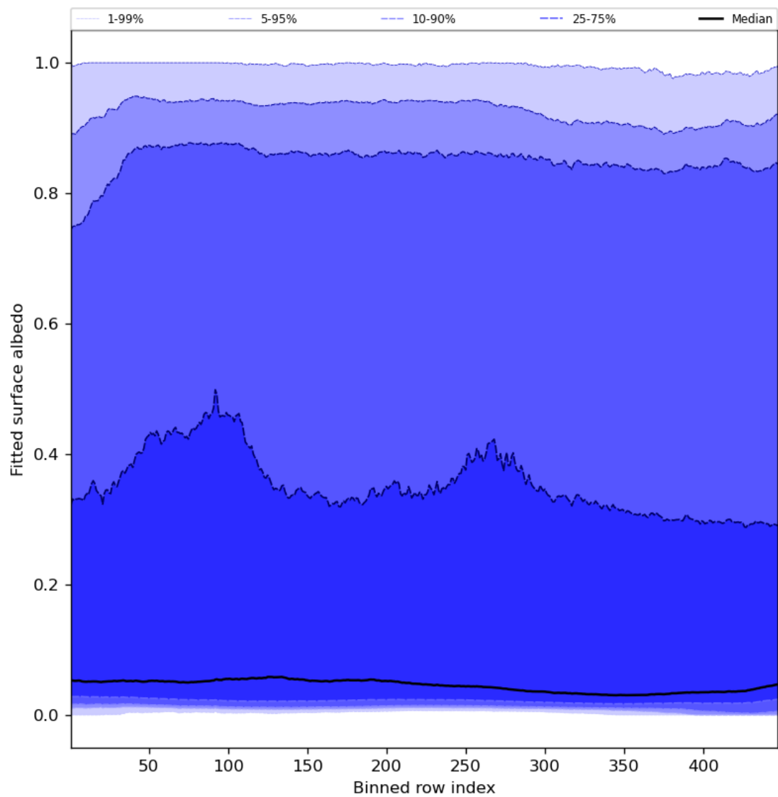
Figure 61: Along track statistics of “Fitted surface albedo” for 2024-04-26 to 2024-04-28
