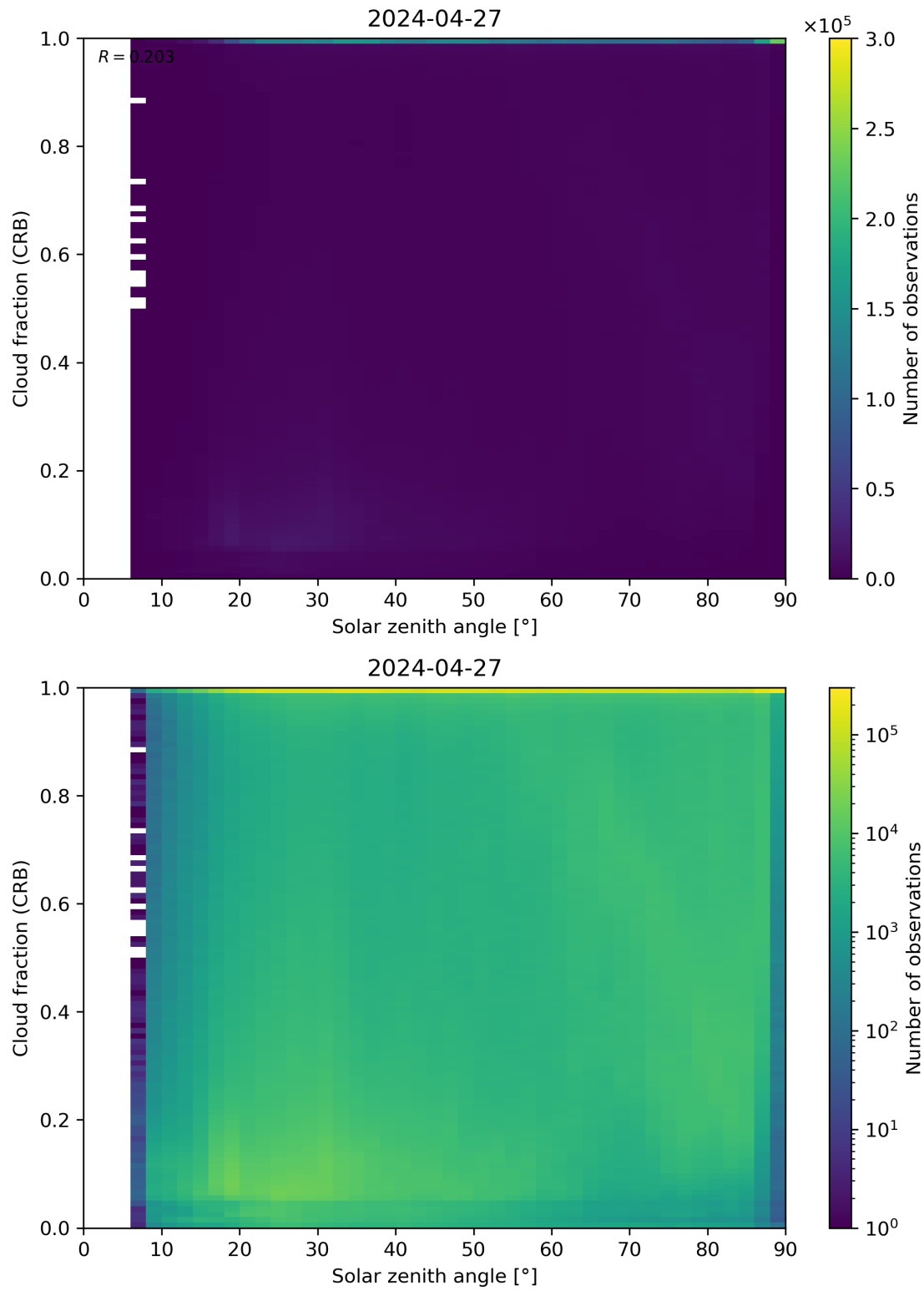
Figure 101: Scatter density plot of “Solar zenith angle” against “Cloud fraction (CRB)” for 2024-04-26 to 2024-04-28.
