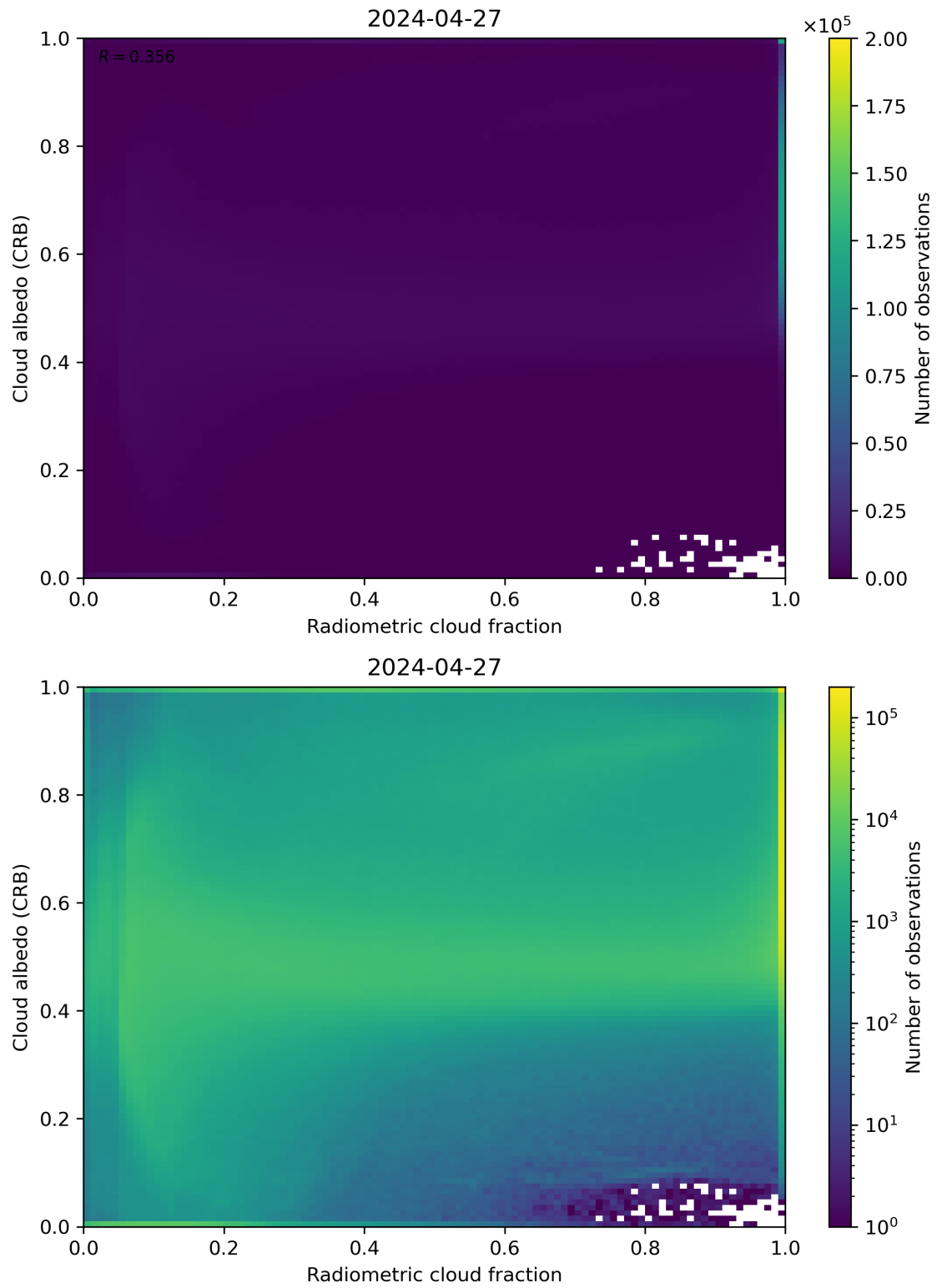
Figure 71: Scatter density plot of “Radiometric cloud fraction” against “Cloud albedo (CRB)” for 2024-04-26 to 2024-04-28.
