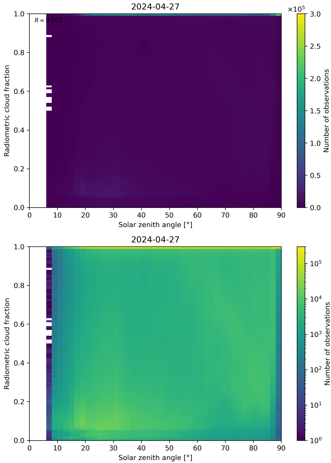
Figure 99: Scatter density plot of “Solar zenith angle” against “Radiometric cloud fraction” for 2024-04-26 to 2024-04-28.
