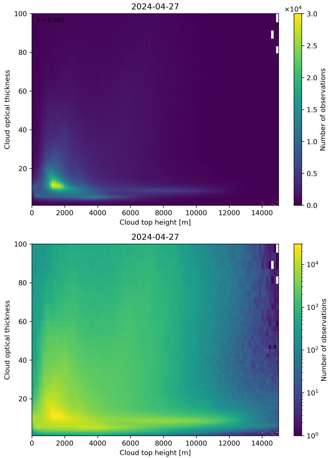
Figure 90: Scatter density plot of “Cloud top height” against “Cloud optical thickness” for 2024-04-26 to 2024-04-28.
