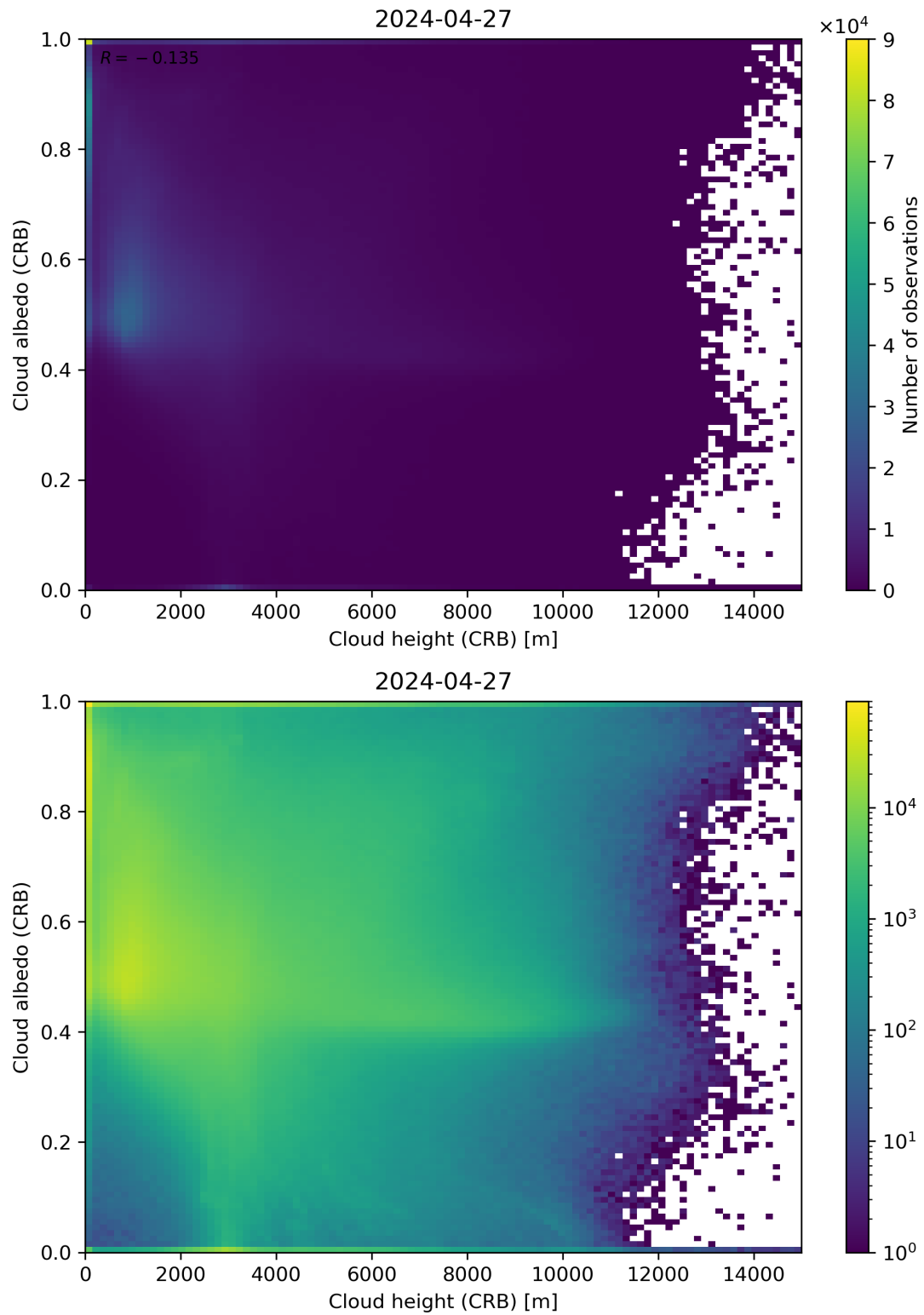
Figure 80: Scatter density plot of “Cloud height (CRB)” against “Cloud albedo (CRB)” for 2024-04-26 to 2024-04-28.
