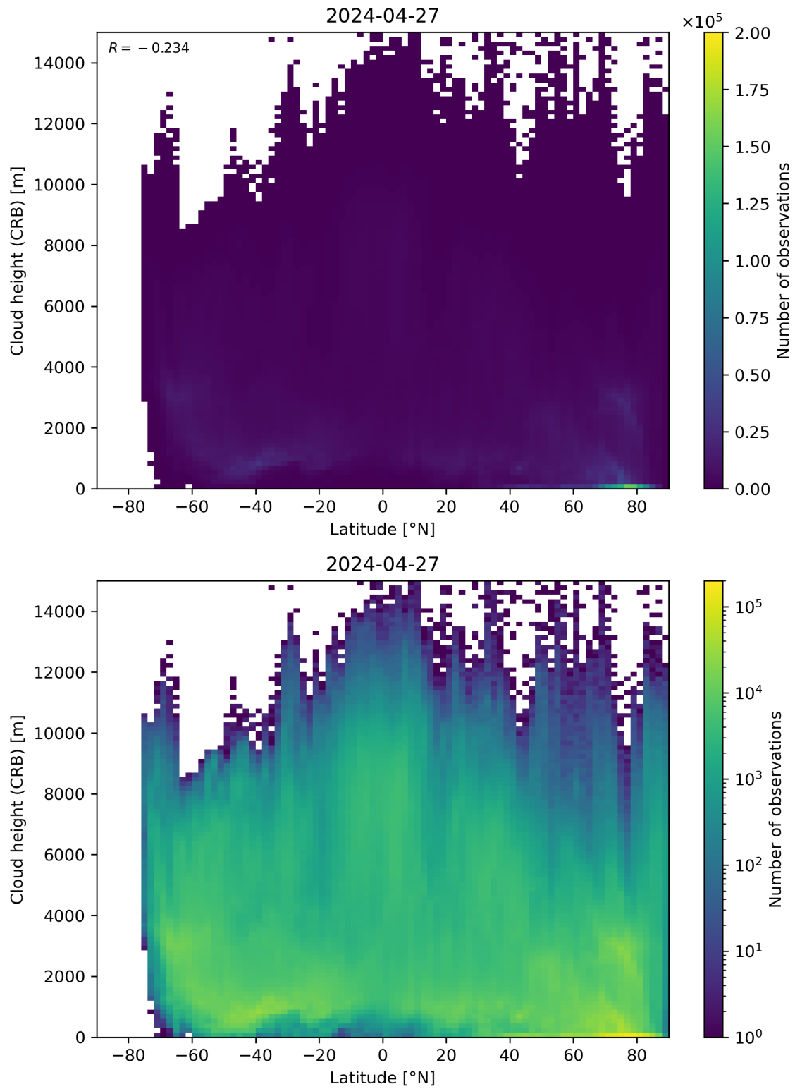
Figure 95: Scatter density plot of “Latitude” against “Cloud height (CRB)” for 2024-04-26 to 2024-04-28.
