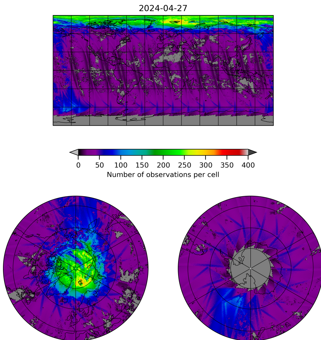
Figure 21: Map of the number of observations for 2024-04-26 to 2024-04-28
