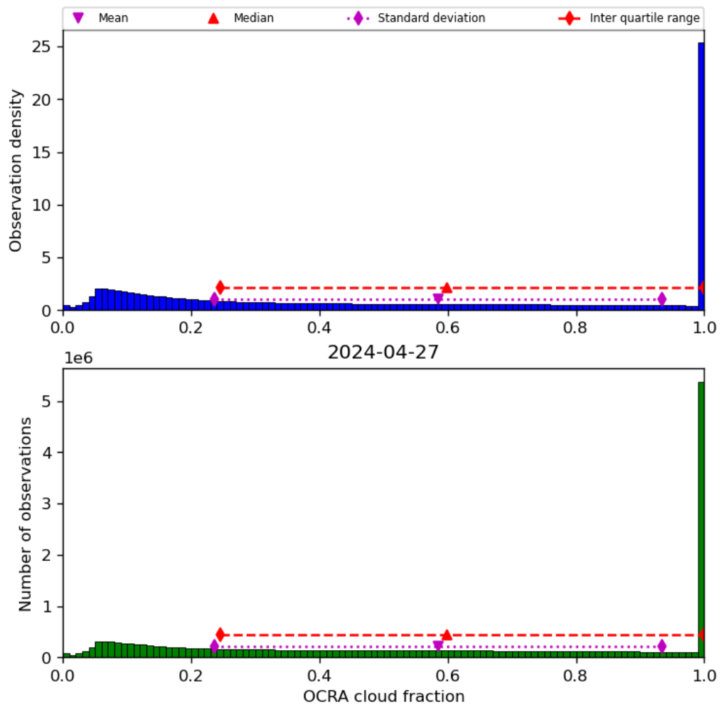
Figure 50: Histogram of “OCRA cloud fraction” for 2024-04-26 to 2024-04-28
