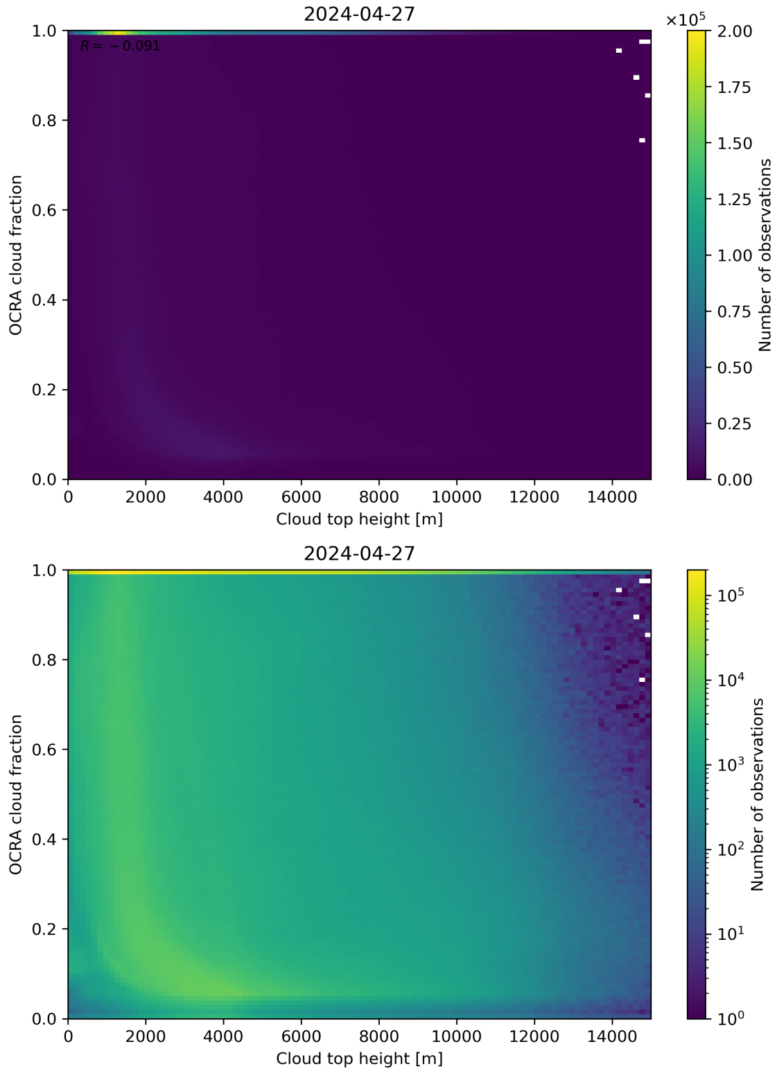
Figure 87: Scatter density plot of “Cloud top height” against “OCRA cloud fraction” for 2024-04-26 to 2024-04-28.
