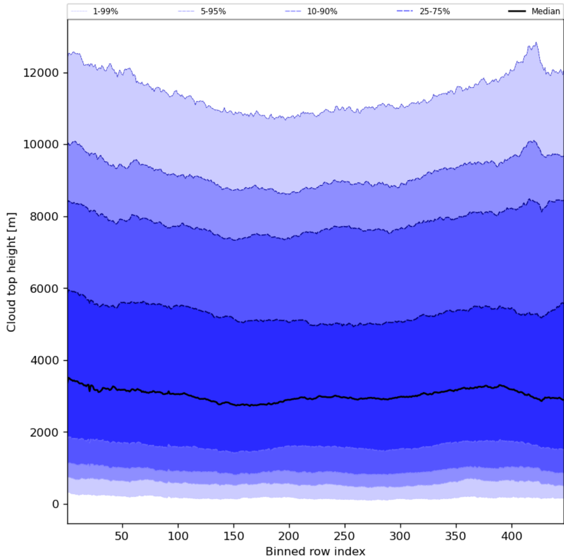
Figure 56: Along track statistics of “Cloud top height” for 2024-04-26 to 2024-04-28
