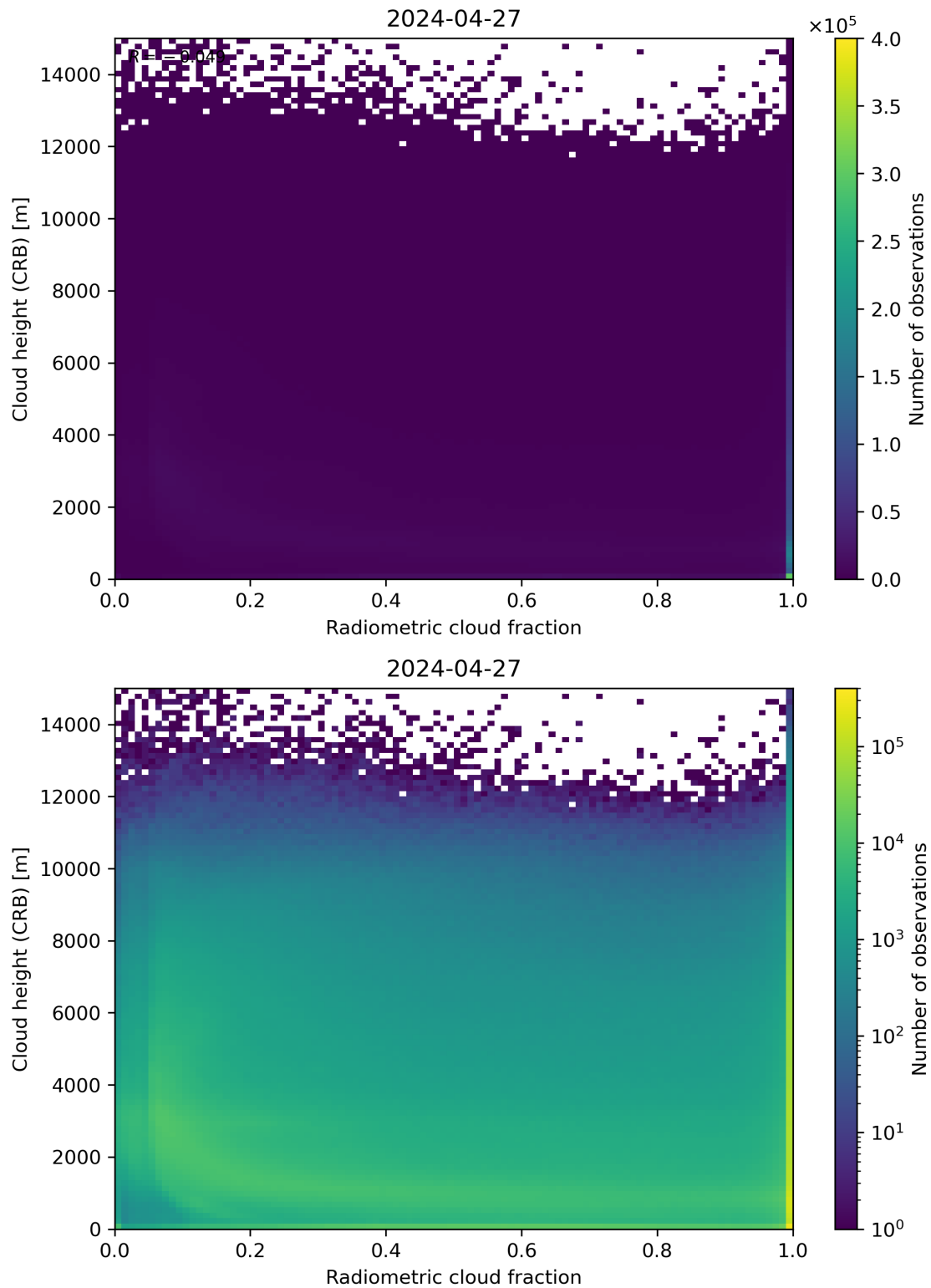
Figure 74: Scatter density plot of “Radiometric cloud fraction” against “Cloud height (CRB)” for 2024-04-26 to 2024-04-28.
