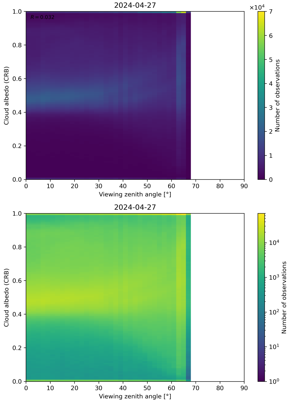
Figure 106: Scatter density plot of “Viewing zenith angle” against “Cloud albedo (CRB)” for 2024-04-26 to 2024-04-28.
