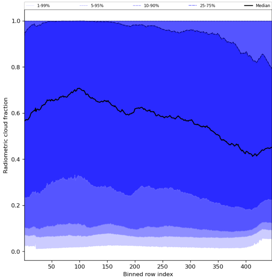
Figure 55: Along track statistics of “Radiometric cloud fraction” for 2024-04-26 to 2024-04-28
