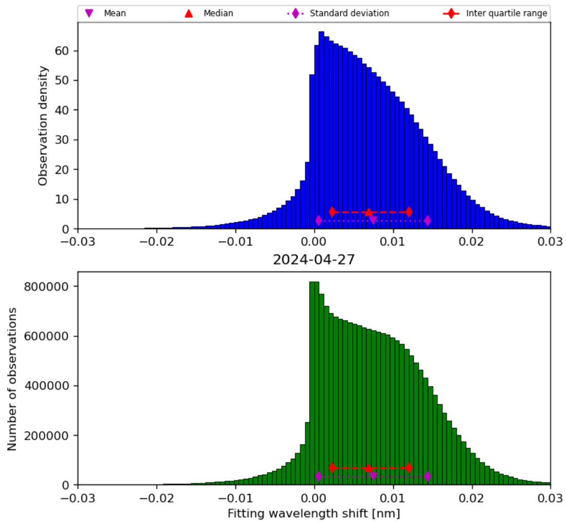
Figure 49: Histogram of “Fitting wavelength shift” for 2024-04-26 to 2024-04-28
