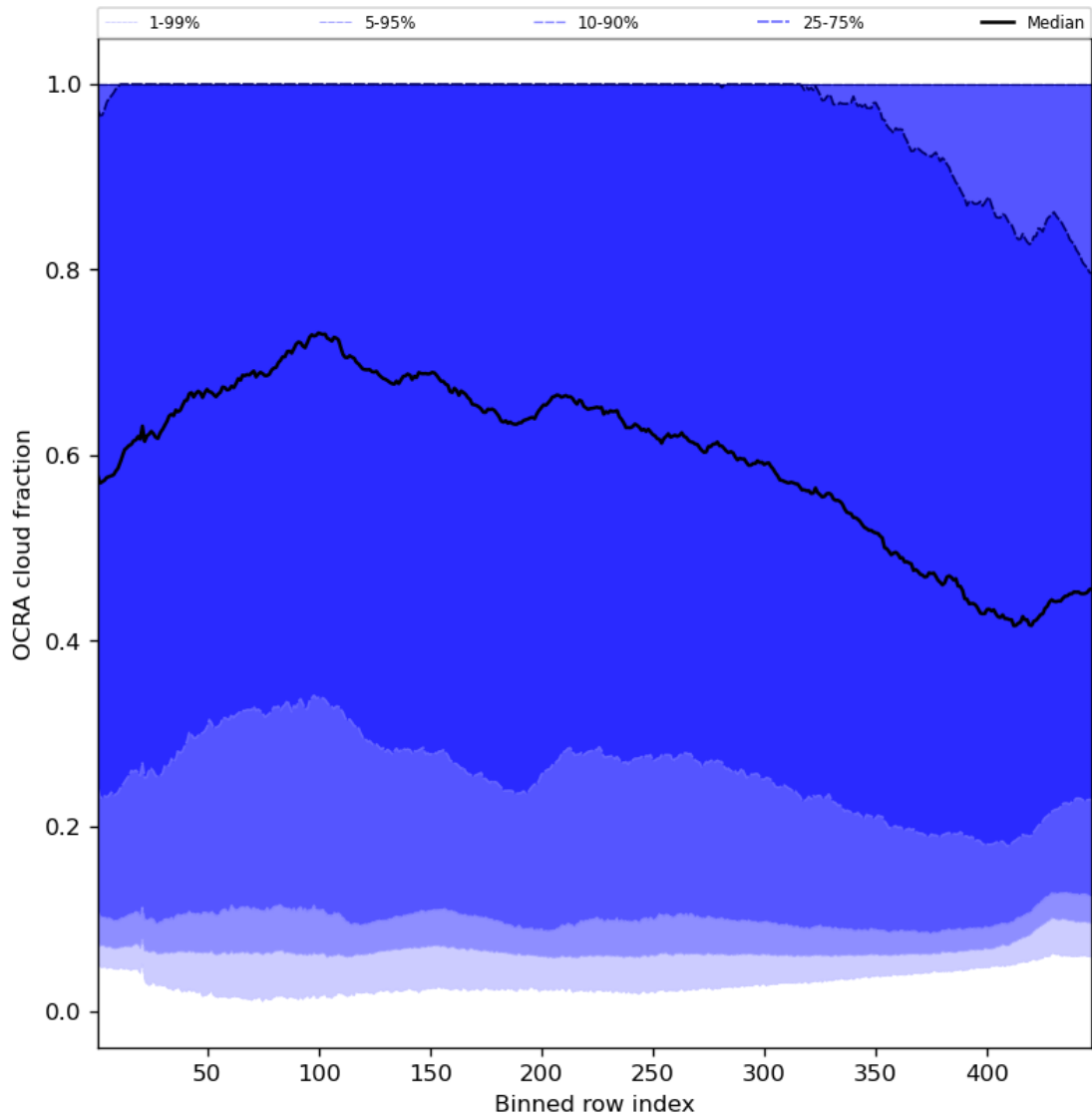
Figure 66: Along track statistics of “OCRA cloud fraction” for 2024-04-26 to 2024-04-28
