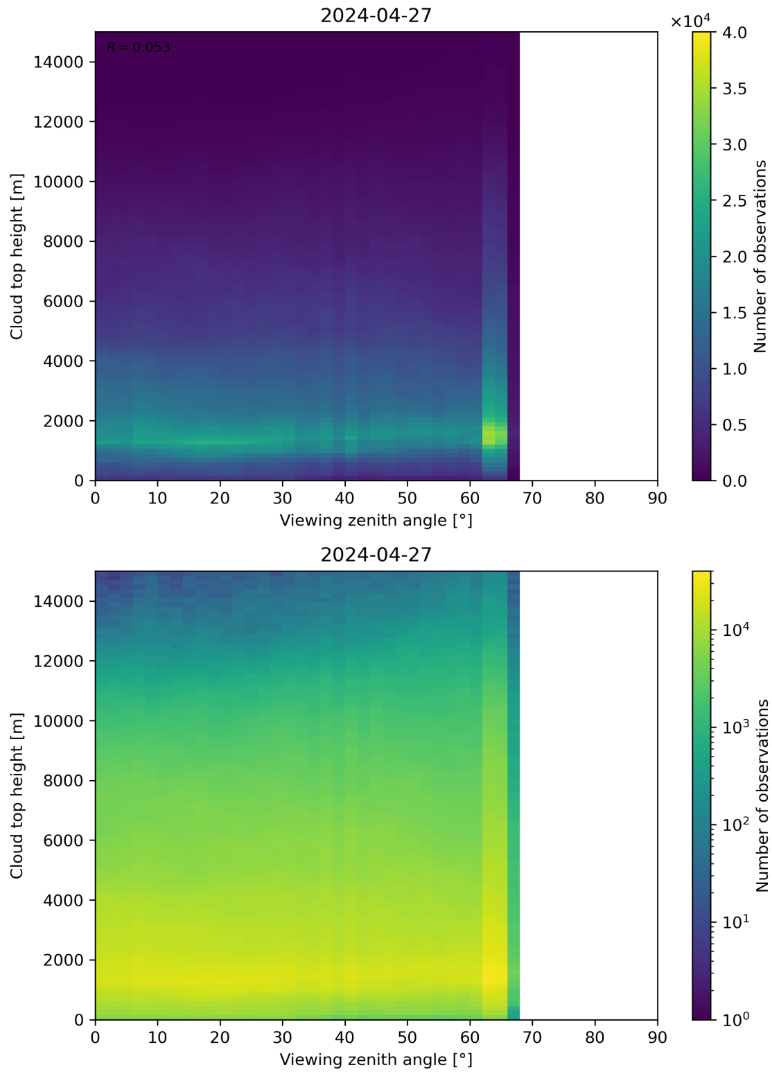
Figure 112: Scatter density plot of “Viewing zenith angle” against “Cloud top height” for 2024-04-26 to 2024-04-28.
