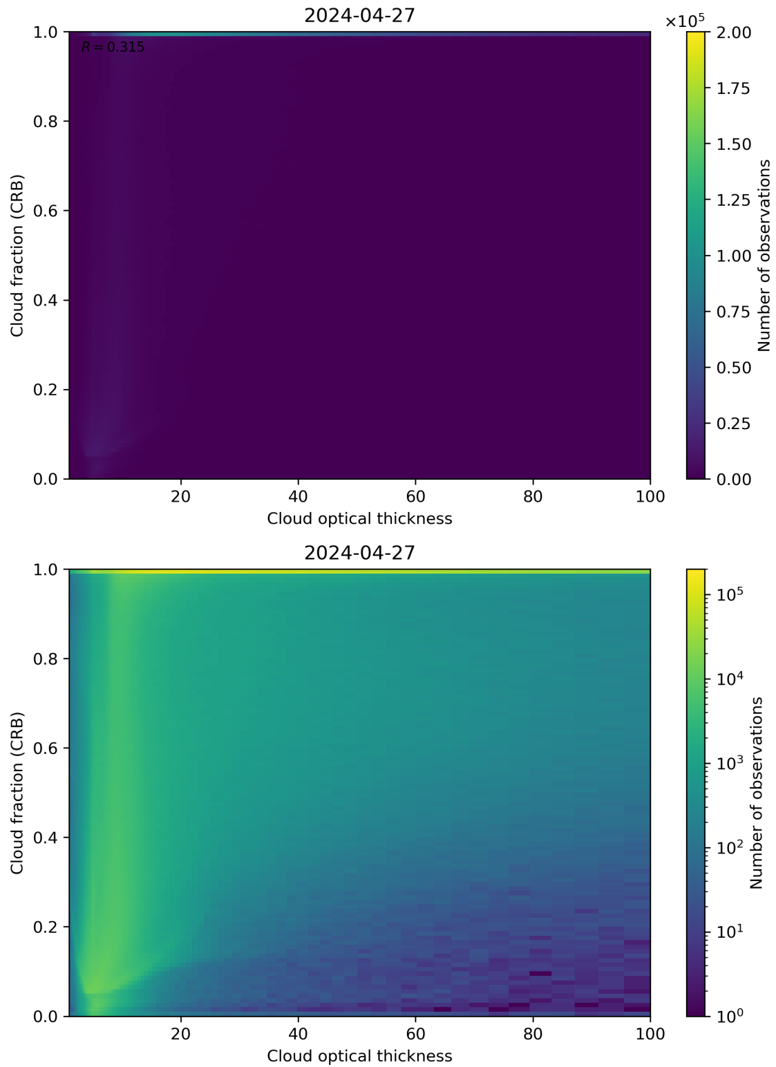
Figure 84: Scatter density plot of “Cloud optical thickness” against “Cloud fraction (CRB)” for 2024-04-26 to 2024-04-28.
