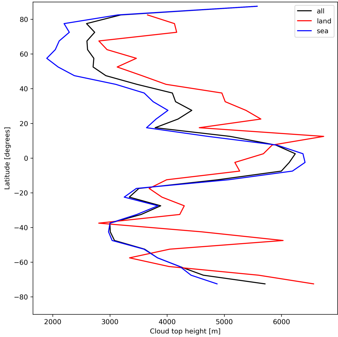
Figure 24: Zonal average of “Cloud top height” for 2024-04-26 to 2024-04-28.
