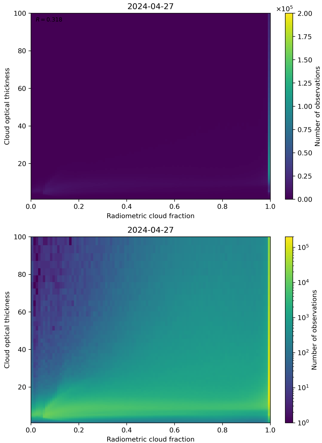
Figure 75: Scatter density plot of “Radiometric cloud fraction” against “Cloud optical thickness” for 2024-04-26 to 2024-04-28.
