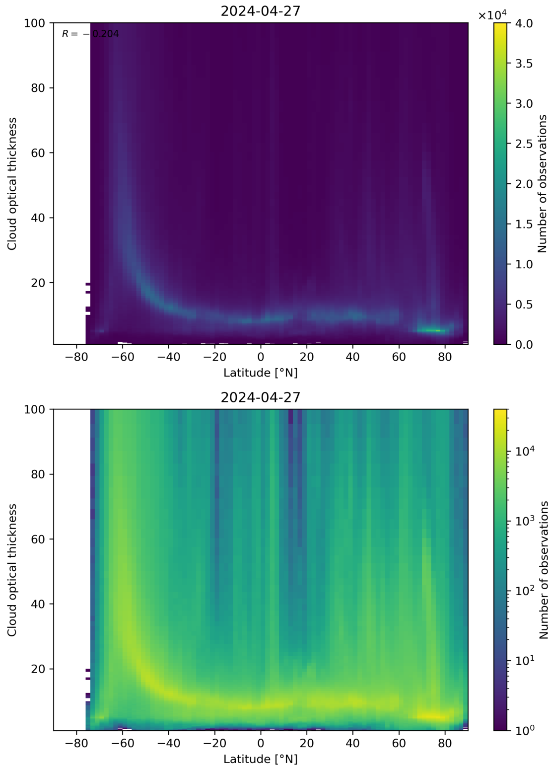
Figure 96: Scatter density plot of “Latitude” against “Cloud optical thickness” for 2024-04-26 to 2024-04-28.
