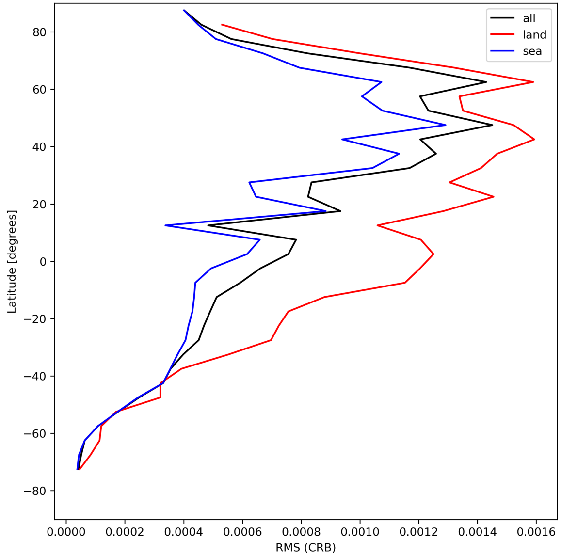
Figure 32: Zonal average of “RMS (CRB)” for 2024-04-26 to 2024-04-28.
