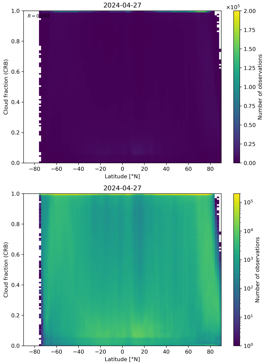
Figure 94: Scatter density plot of “Latitude” against “Cloud fraction (CRB)” for 2024-04-26 to 2024-04-28.
