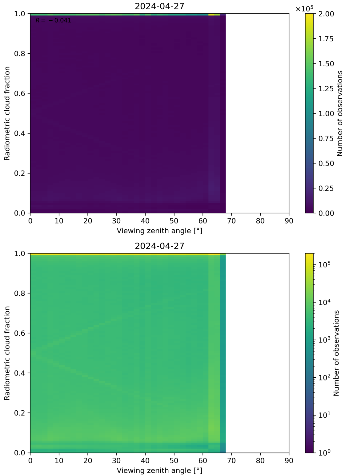
Figure 107: Scatter density plot of “Viewing zenith angle” against “Radiometric cloud fraction” for 2024-04-26 to 2024-04-28.
