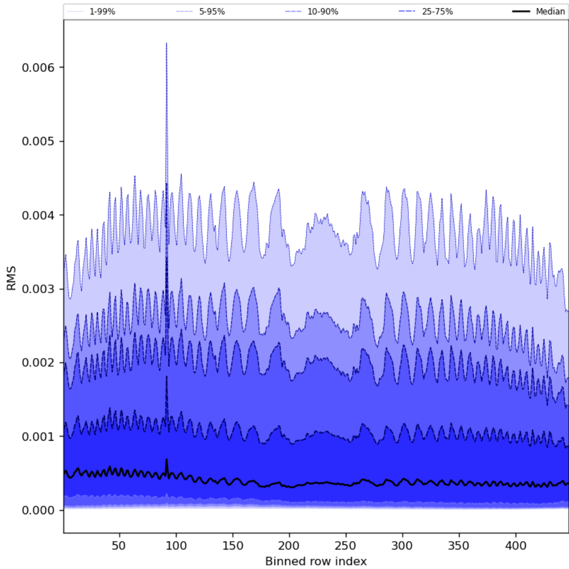
Figure 63: Along track statistics of “RMS” for 2024-04-26 to 2024-04-28
