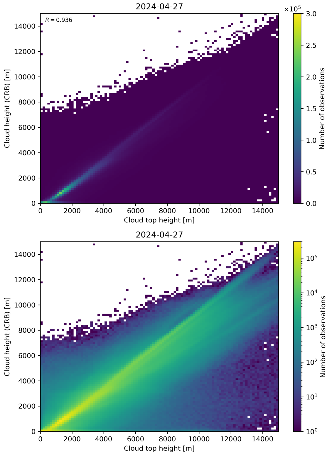
Figure 89: Scatter density plot of “Cloud top height” against “Cloud height (CRB)” for 2024-04-26 to 2024-04-28.
