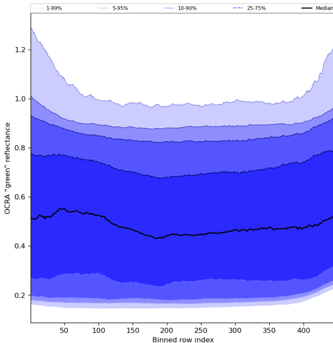
Figure 68: Along track statistics of "OCRA "green" reflectance" for 2024-04-26 to 2024-04-28
