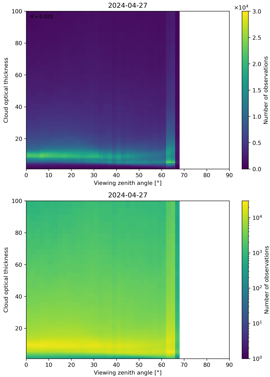
Figure 111: Scatter density plot of “Viewing zenith angle” against “Cloud optical thickness” for 2024-04-26 to 2024-04-28.
