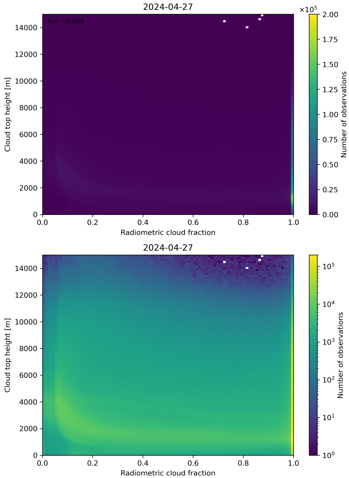
Figure 76: Scatter density plot of “Radiometric cloud fraction” against “Cloud top height” for 2024-04-26 to 2024-04-28.
