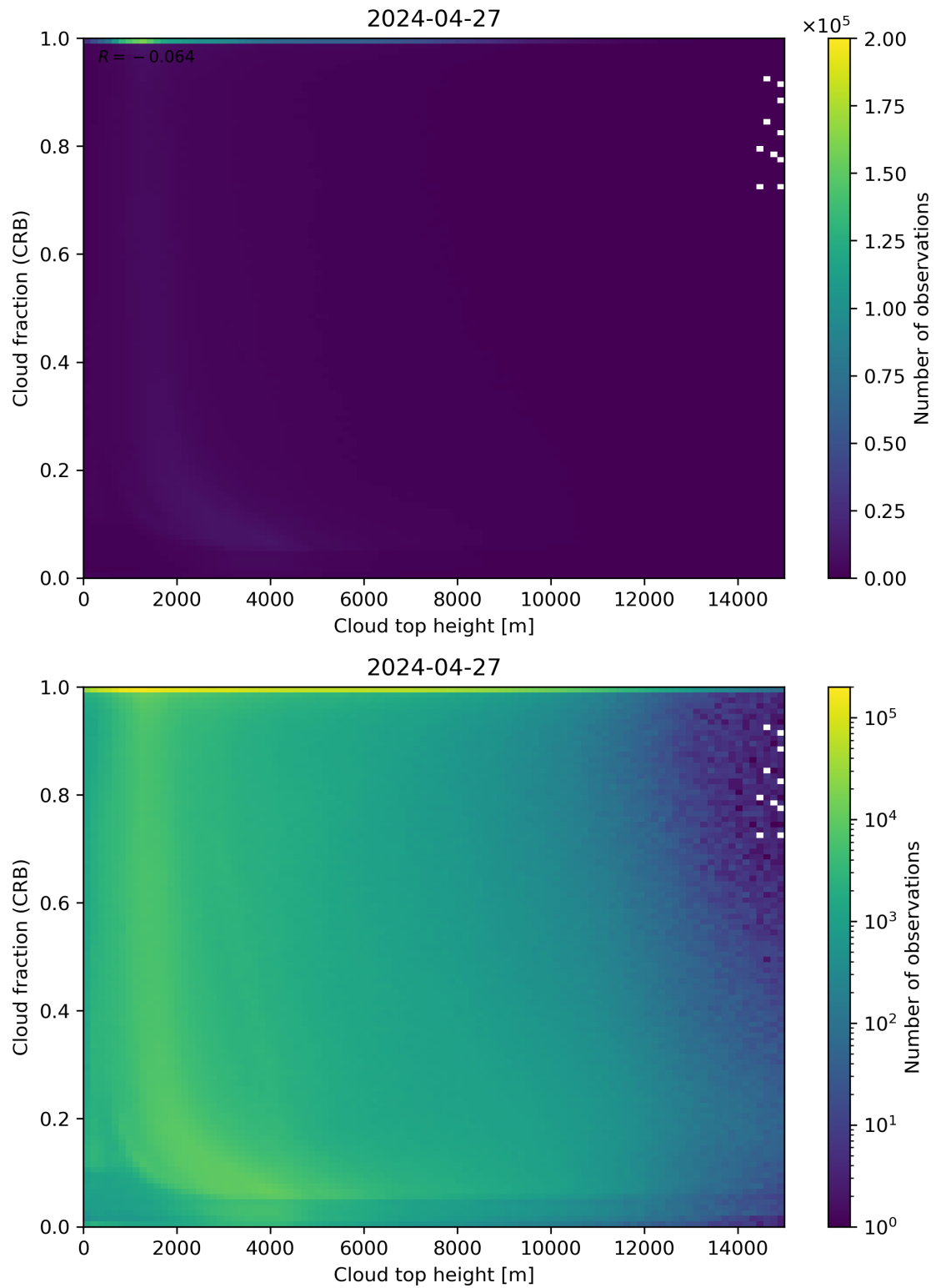
Figure 88: Scatter density plot of “Cloud top height” against “Cloud fraction (CRB)” for 2024-04-26 to 2024-04-28.
