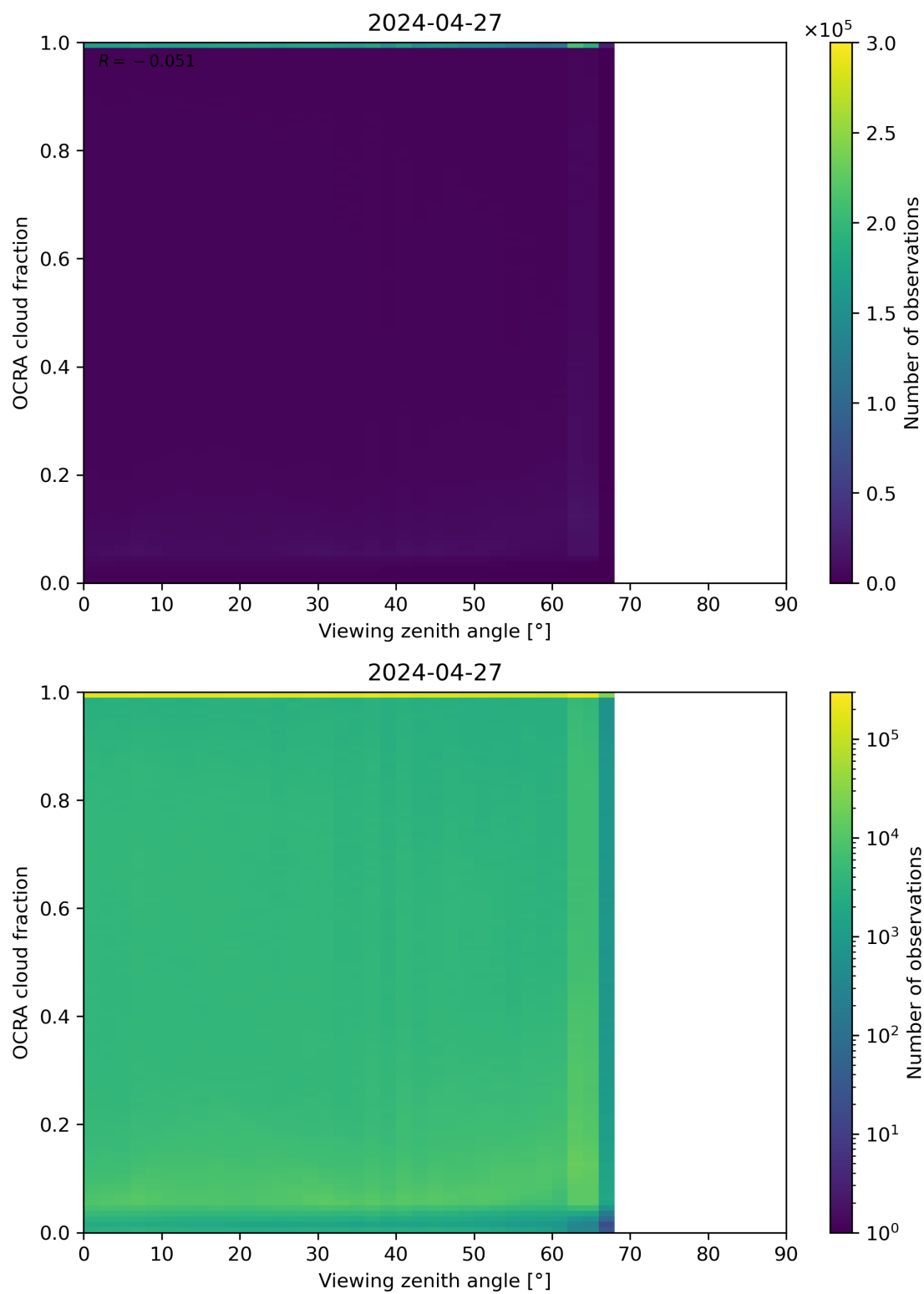
Figure 108: Scatter density plot of “Viewing zenith angle” against “OCRA cloud fraction” for 2024-04-26 to 2024-04-28.
