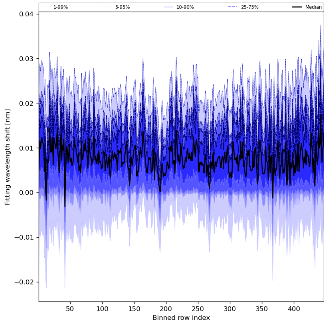
Figure 65: Along track statistics of “Fitting wavelength shift” for 2024-04-26 to 2024-04-28
