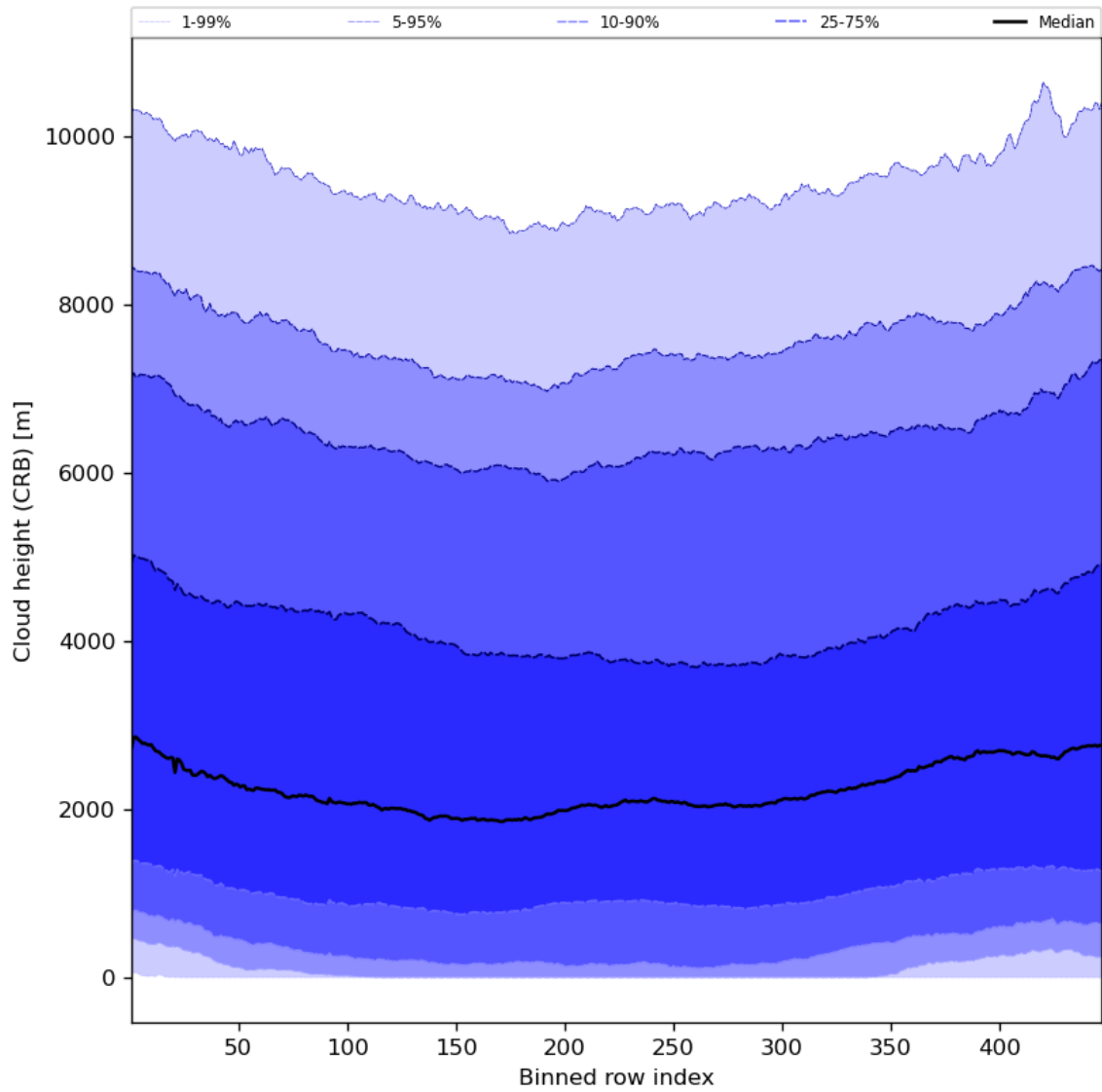
Figure 59: Along track statistics of “Cloud height (CRB)” for 2024-04-26 to 2024-04-28
