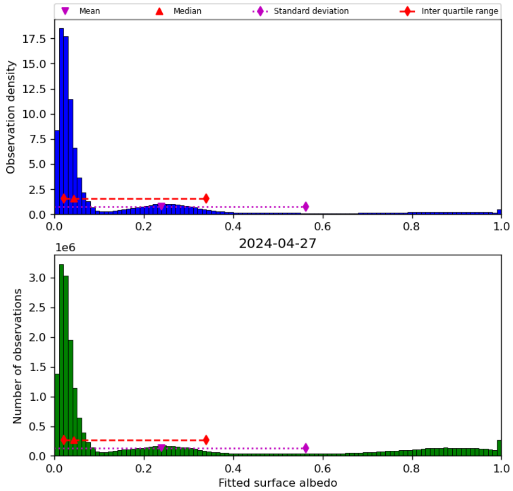
Figure 45: Histogram of “Fitted surface albedo” for 2024-04-26 to 2024-04-28
