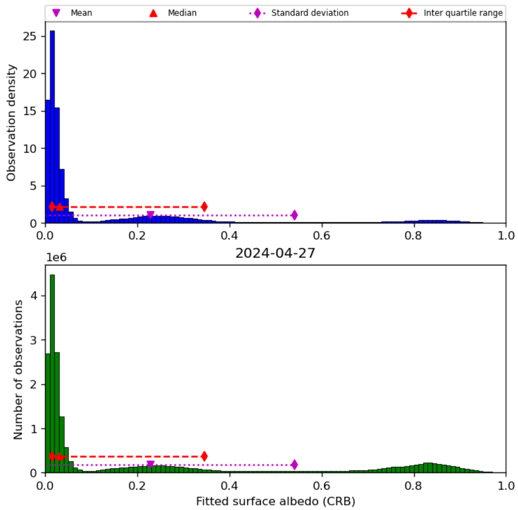
Figure 46: Histogram of “Fitted surface albedo (CRB)” for 2024-04-26 to 2024-04-28
