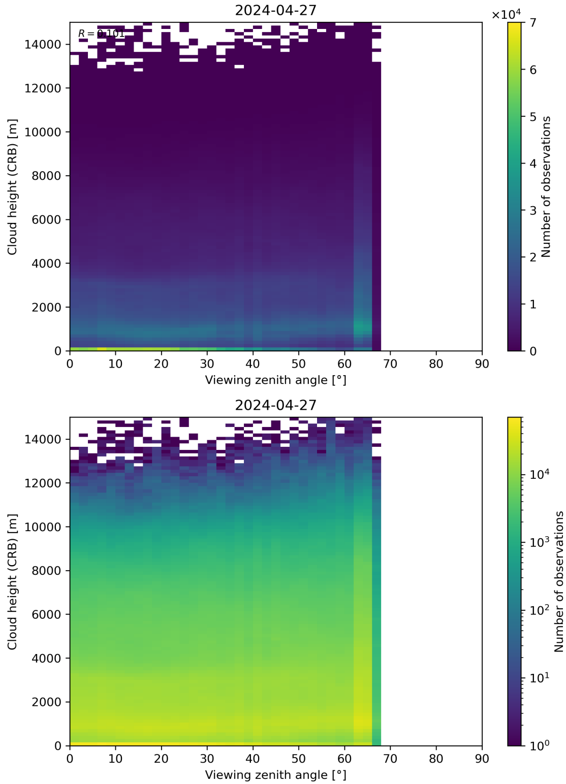
Figure 110: Scatter density plot of “Viewing zenith angle” against “Cloud height (CRB)” for 2024-04-26 to 2024-04-28.
