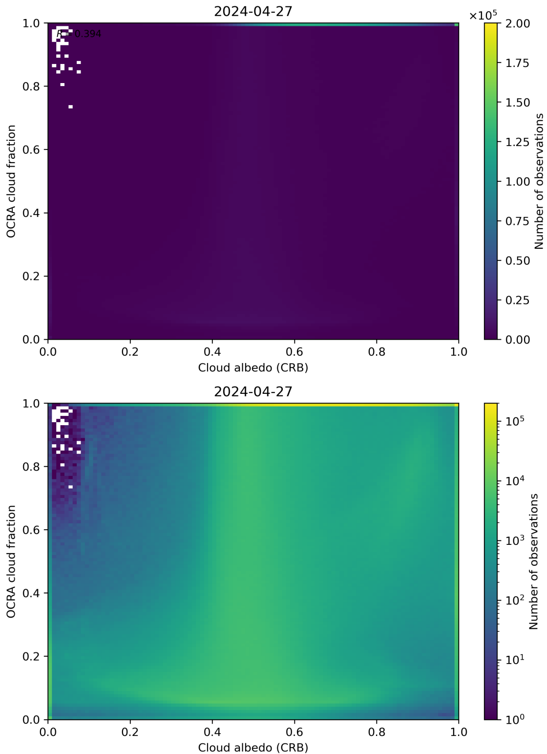
Figure 70: Scatter density plot of “Cloud albedo (CRB)” against “OCRA cloud fraction” for 2024-04-26 to 2024-04-28.
