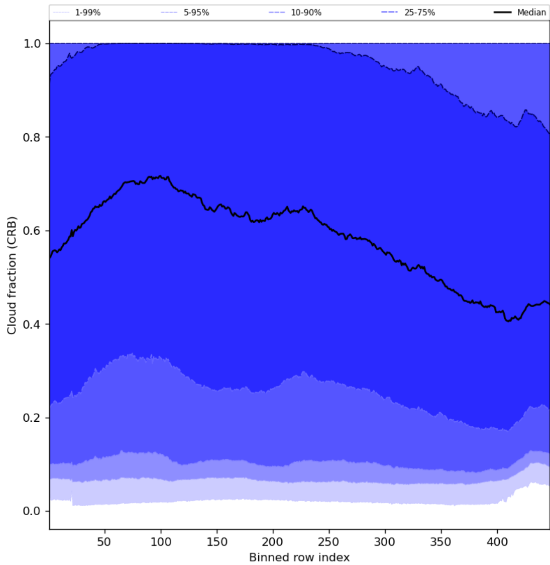
Figure 58: Along track statistics of “Cloud fraction (CRB)” for 2024-04-27 to 2024-04-29
