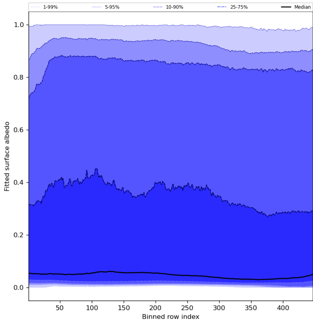
Figure 61: Along track statistics of “Fitted surface albedo” for 2024-04-27 to 2024-04-29
