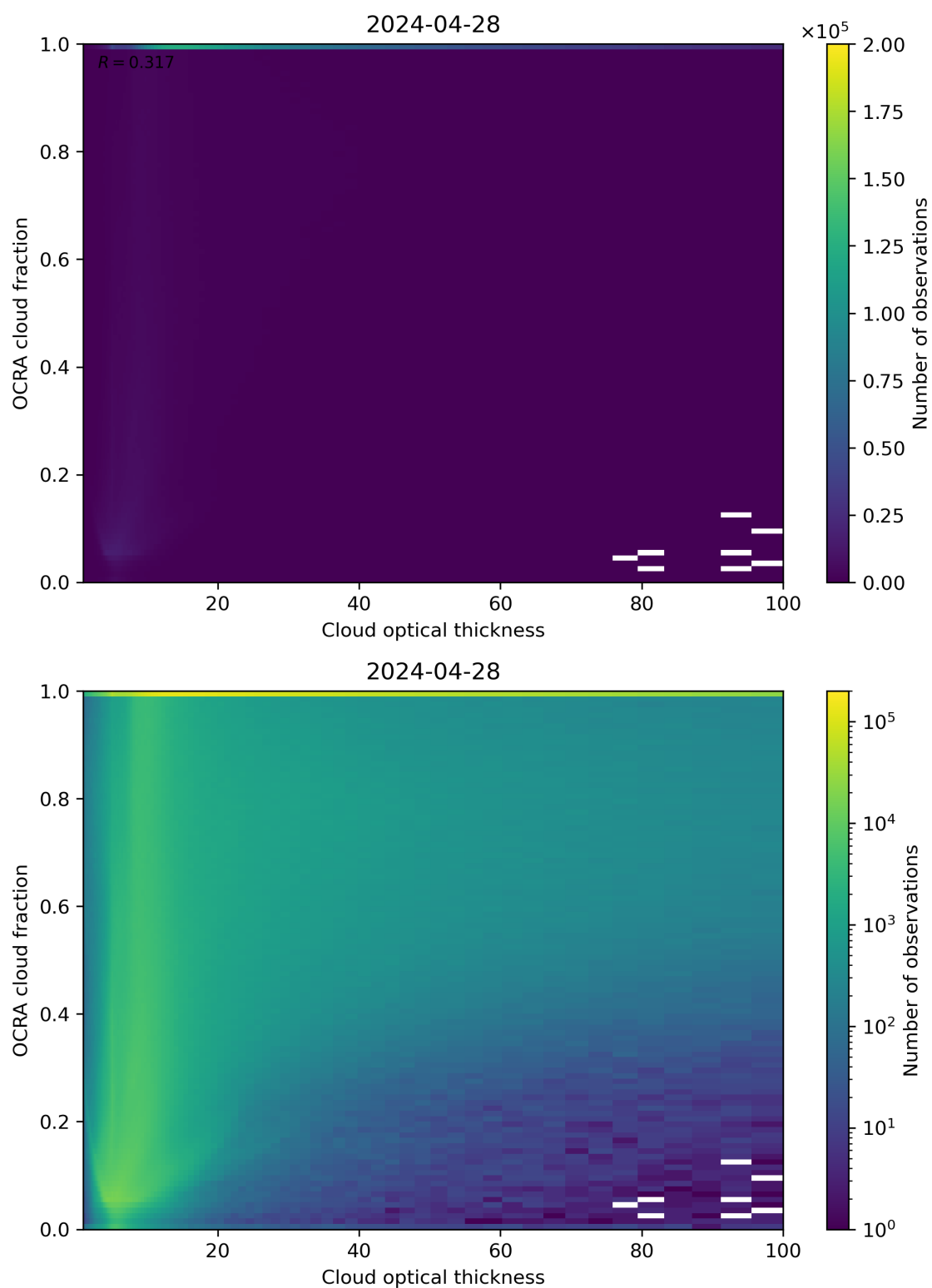
Figure 83: Scatter density plot of “Cloud optical thickness” against “OCRA cloud fraction” for 2024-04-27 to 2024-04-29.
