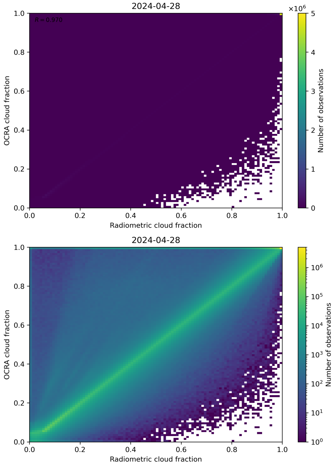
Figure 72: Scatter density plot of “Radiometric cloud fraction” against “OCRA cloud fraction” for 2024-04-27 to 2024-04-29.
