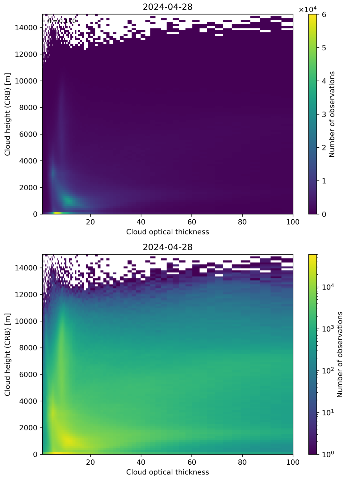
Figure 85: Scatter density plot of “Cloud optical thickness” against “Cloud height (CRB)” for 2024-04-27 to 2024-04-29.
