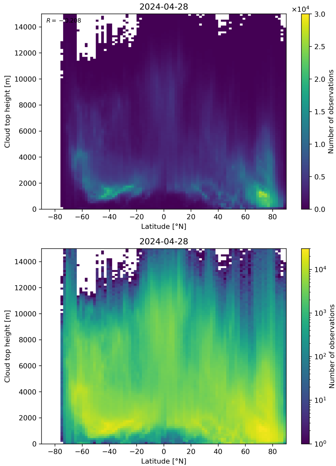
Figure 97: Scatter density plot of “Latitude” against “Cloud top height” for 2024-04-27 to 2024-04-29.
