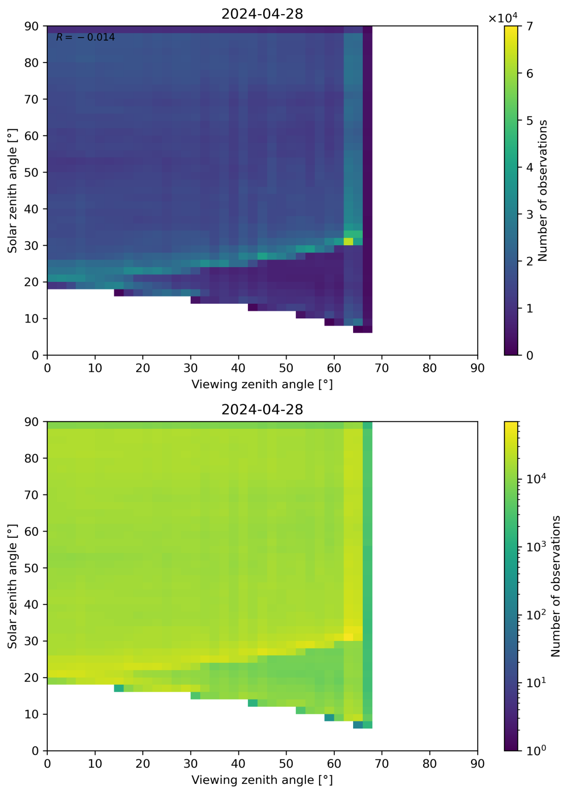
Figure 114: Scatter density plot of “Viewing zenith angle” against “Solar zenith angle” for 2024-04-27 to 2024-04-29.
