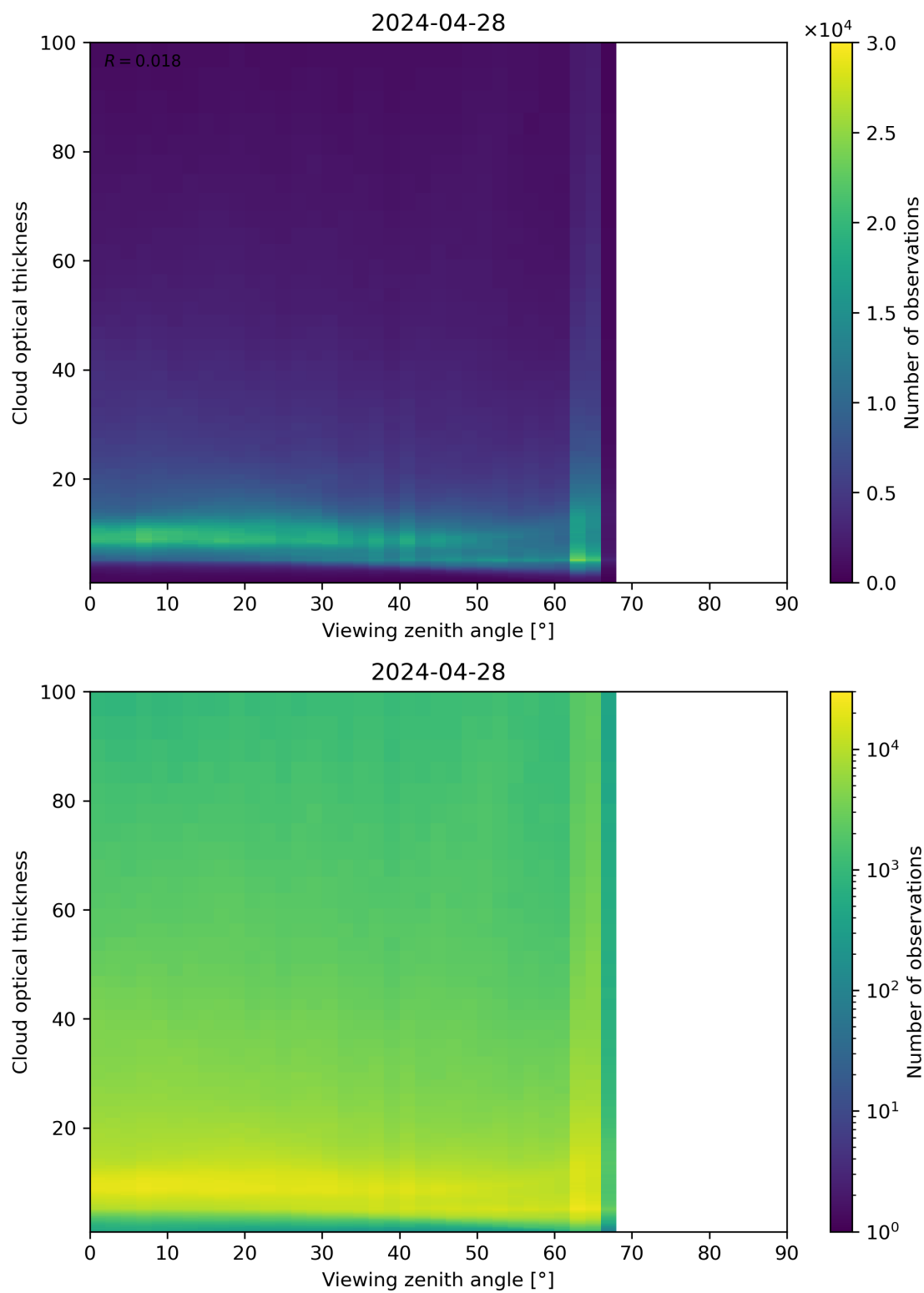
Figure 111: Scatter density plot of “Viewing zenith angle” against “Cloud optical thickness” for 2024-04-27 to 2024-04-29.
