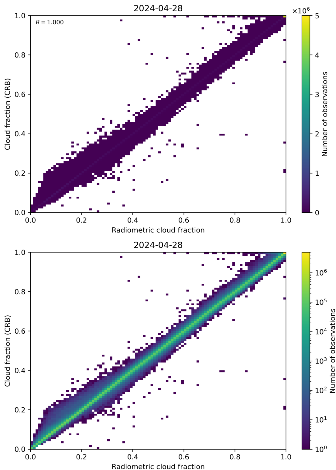
Figure 73: Scatter density plot of “Radiometric cloud fraction” against “Cloud fraction (CRB)” for 2024-04-27 to 2024-04-29.
