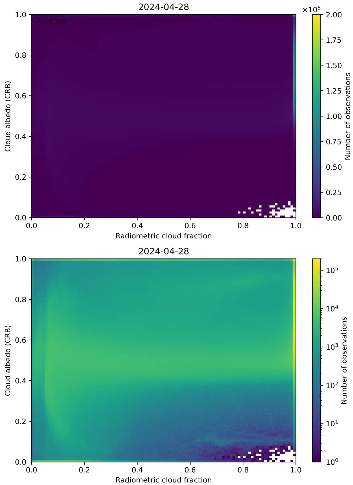
Figure 71: Scatter density plot of “Radiometric cloud fraction” against “Cloud albedo (CRB)” for 2024-04-27 to 2024-04-29.
