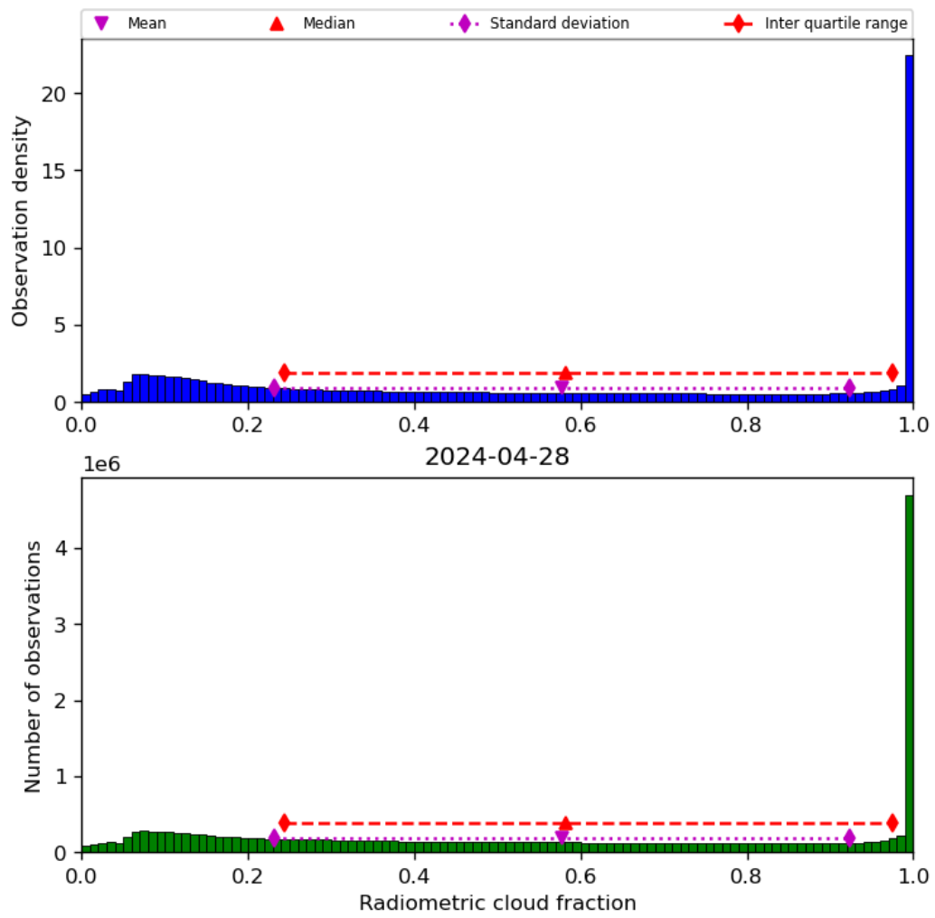
Figure 39: Histogram of “Radiometric cloud fraction” for 2024-04-27 to 2024-04-29
