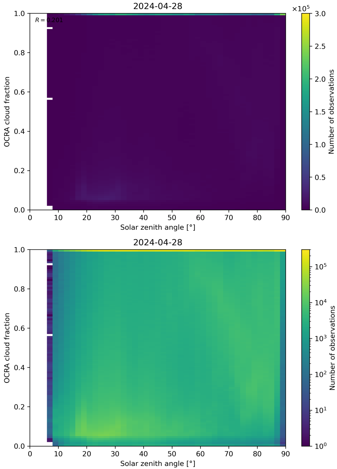
Figure 100: Scatter density plot of “Solar zenith angle” against “OCRA cloud fraction” for 2024-04-27 to 2024-04-29.
