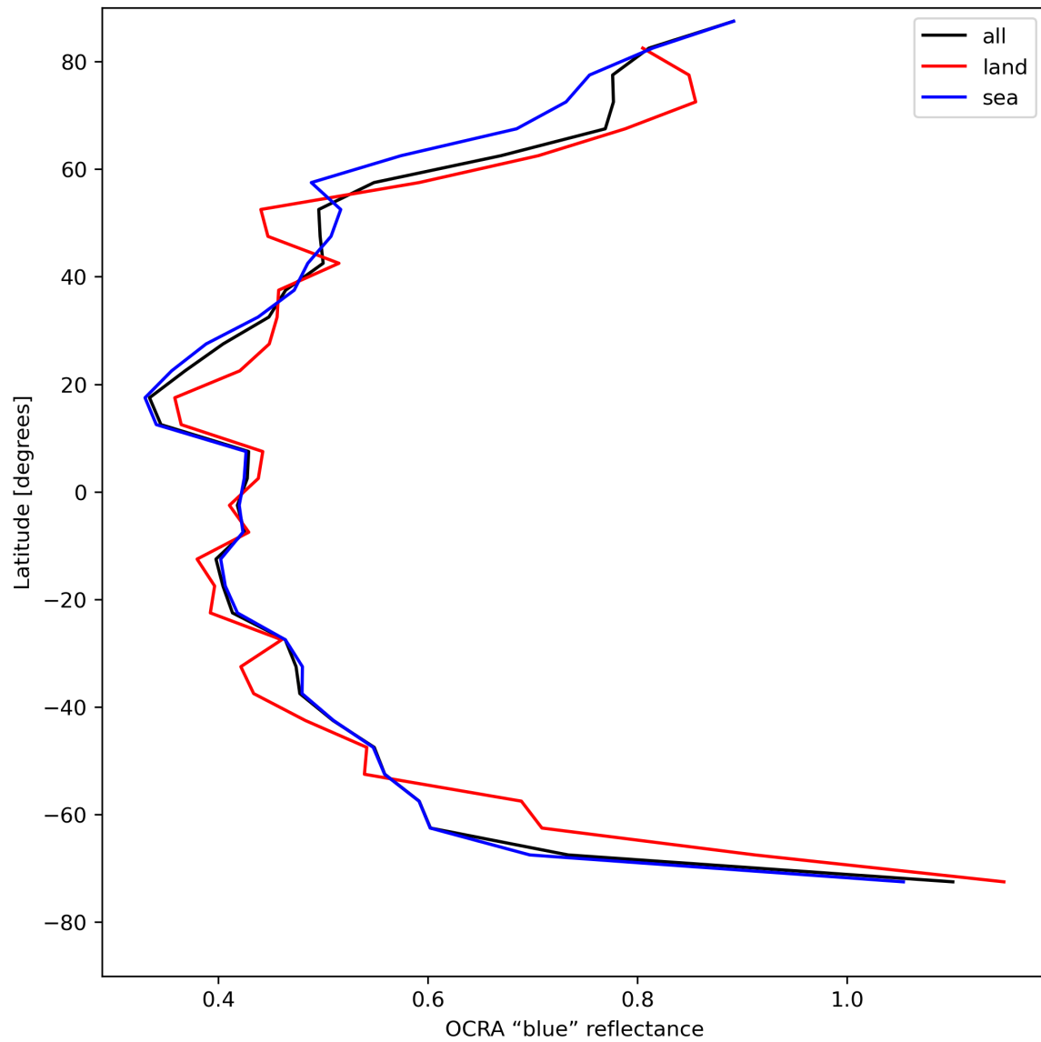
Figure 35: Zonal average of “OCRA “blue” reflectance” for 2024-04-27 to 2024-04-29.
