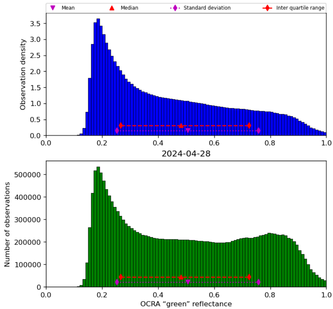
Figure 52: Histogram of “OCRA “green” reflectance” for 2024-04-27 to 2024-04-29
