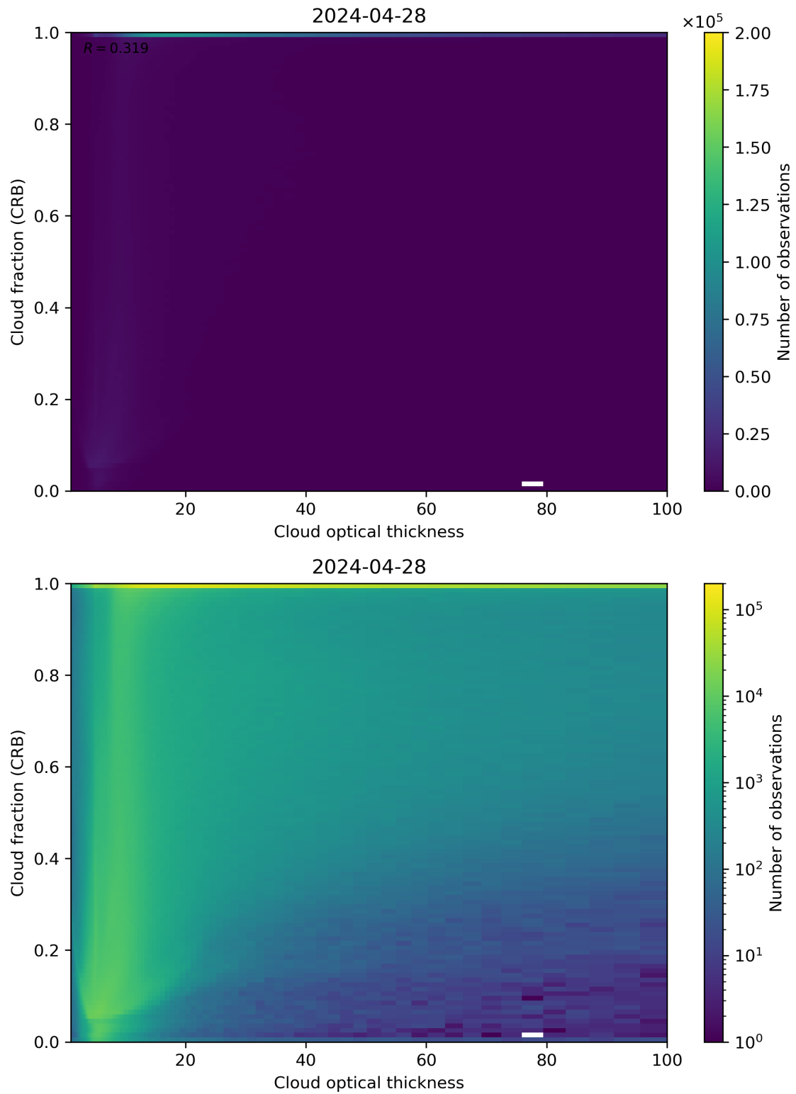
Figure 84: Scatter density plot of “Cloud optical thickness” against “Cloud fraction (CRB)” for 2024-04-27 to 2024-04-29.
