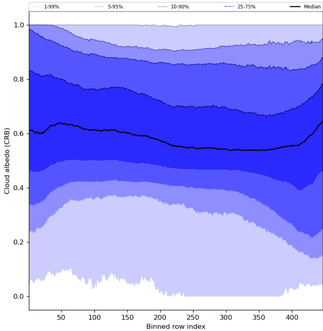
Figure 60: Along track statistics of “Cloud albedo (CRB)” for 2024-04-27 to 2024-04-29
