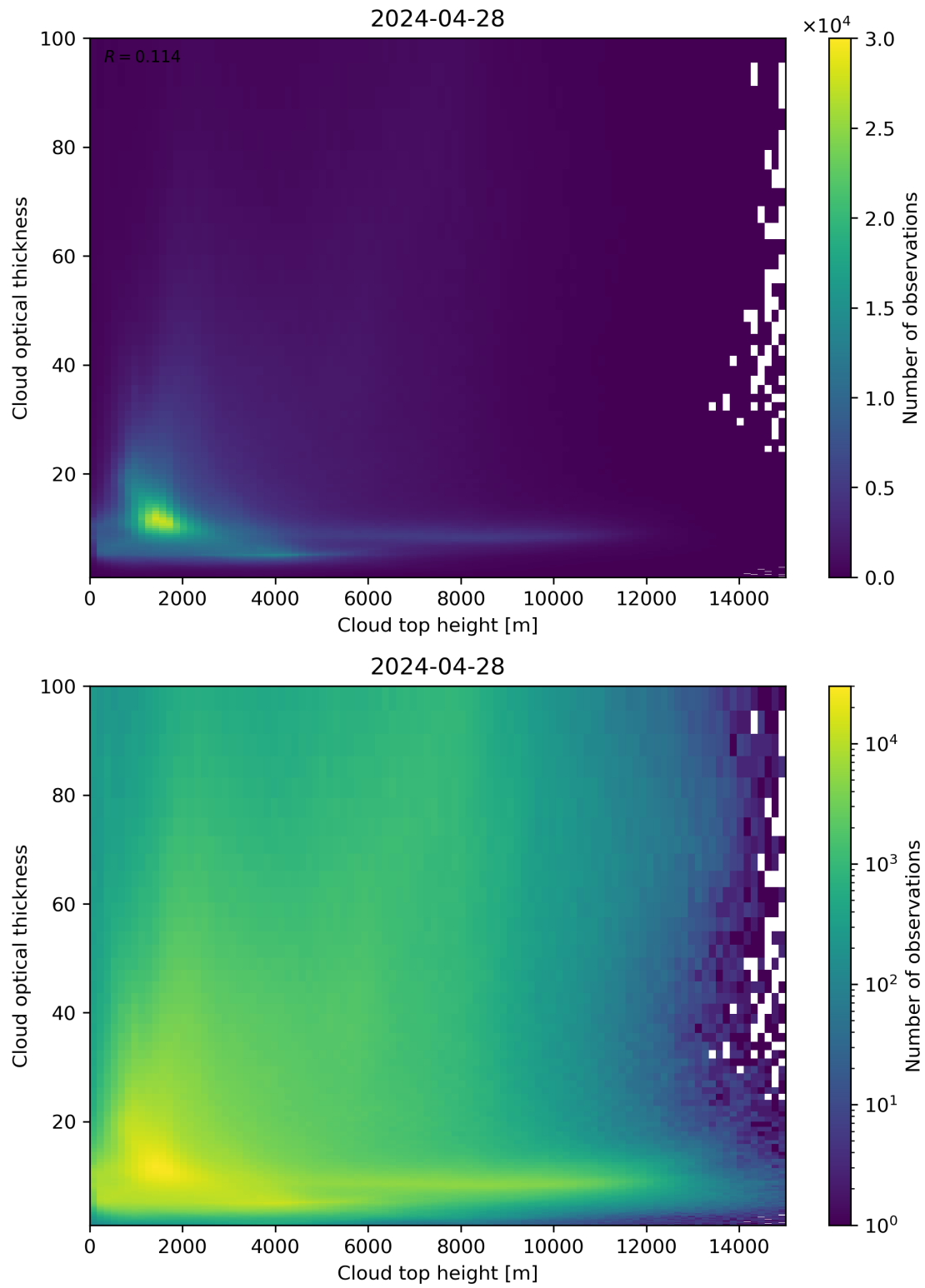
Figure 90: Scatter density plot of “Cloud top height” against “Cloud optical thickness” for 2024-04-27 to 2024-04-29.
