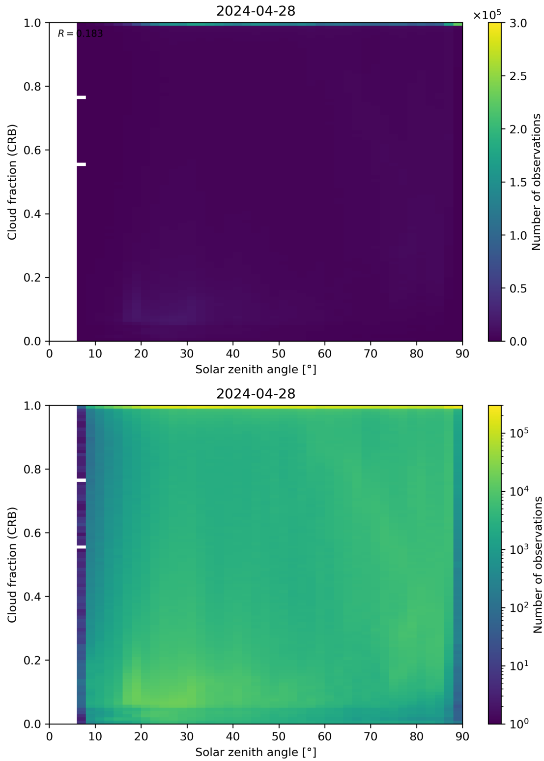
Figure 101: Scatter density plot of “Solar zenith angle” against “Cloud fraction (CRB)” for 2024-04-27 to 2024-04-29.
