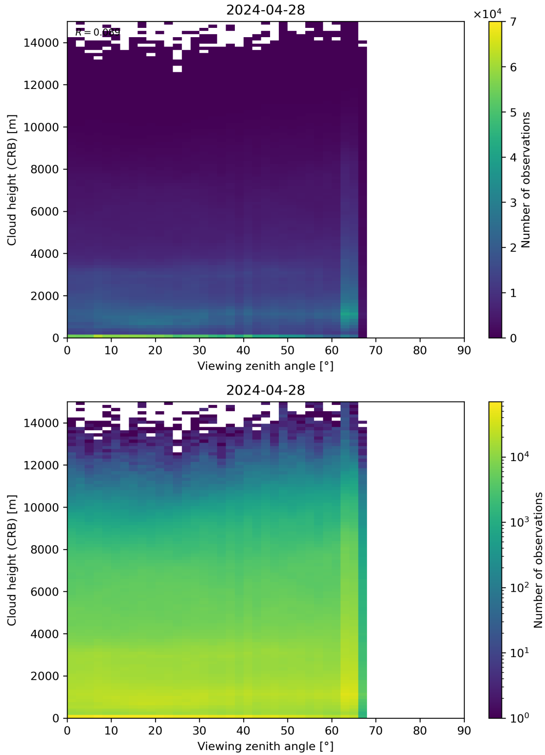
Figure 110: Scatter density plot of “Viewing zenith angle” against “Cloud height (CRB)” for 2024-04-27 to 2024-04-29.
