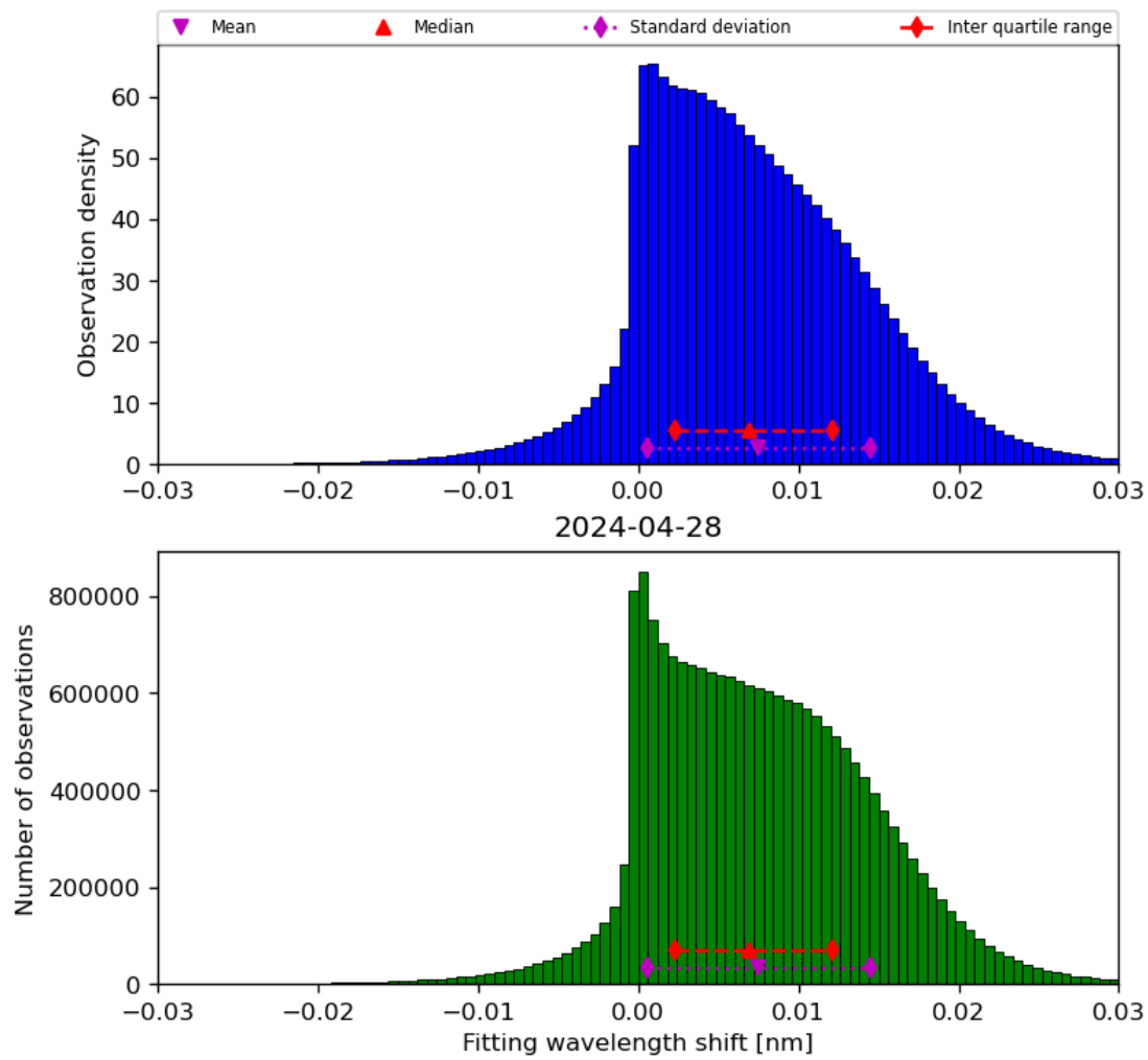
Figure 49: Histogram of “Fitting wavelength shift” for 2024-04-27 to 2024-04-29
