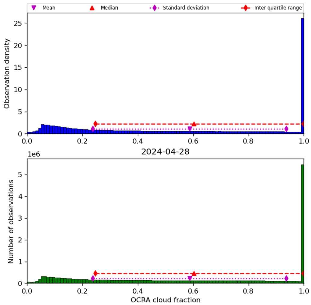
Figure 50: Histogram of “OCRA cloud fraction” for 2024-04-27 to 2024-04-29
