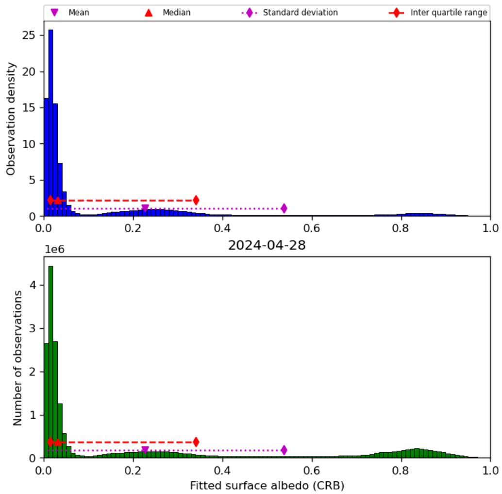
Figure 46: Histogram of “Fitted surface albedo (CRB)” for 2024-04-27 to 2024-04-29
