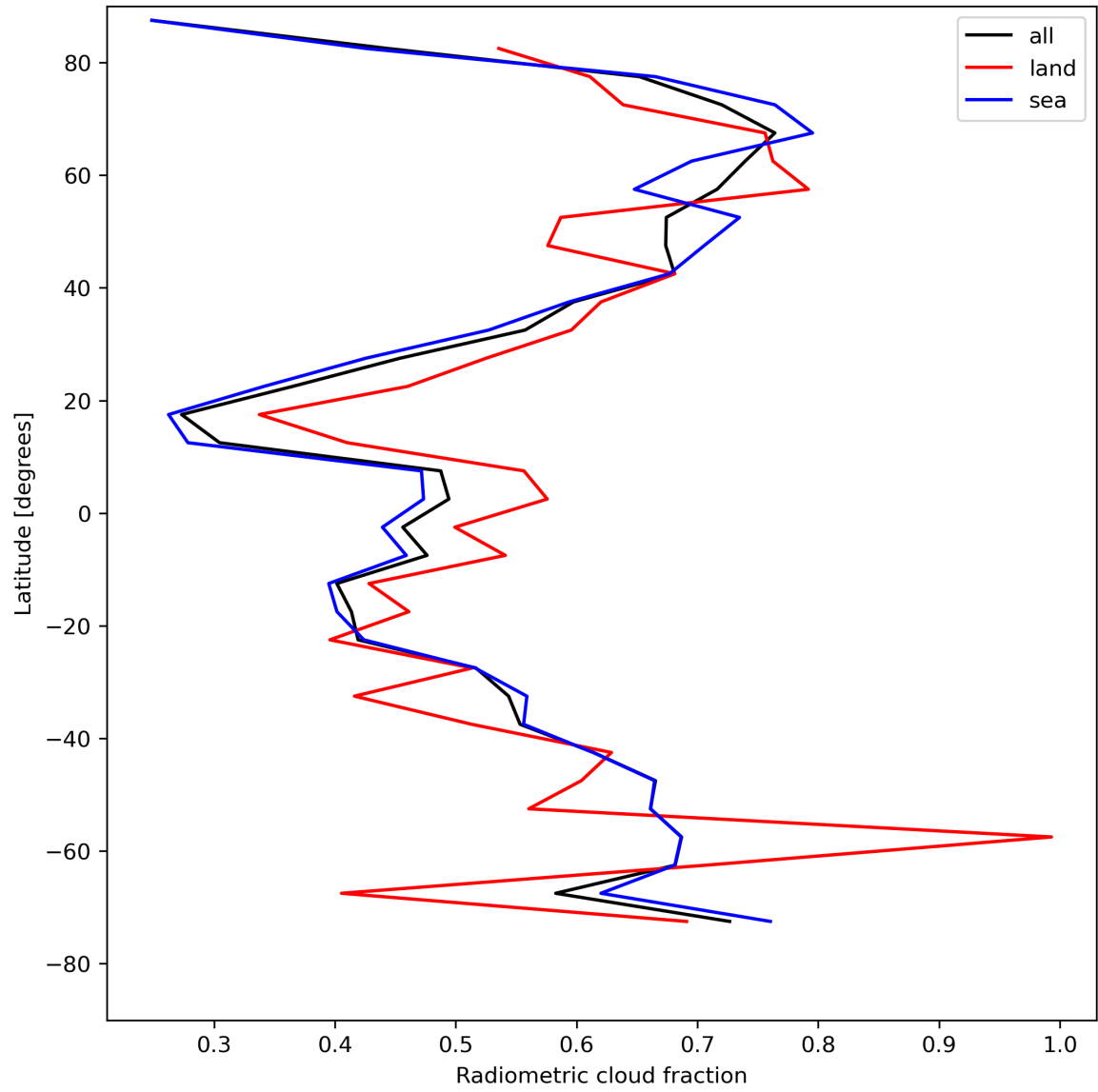
Figure 23: Zonal average of “Radiometric cloud fraction” for 2024-04-27 to 2024-04-29.
