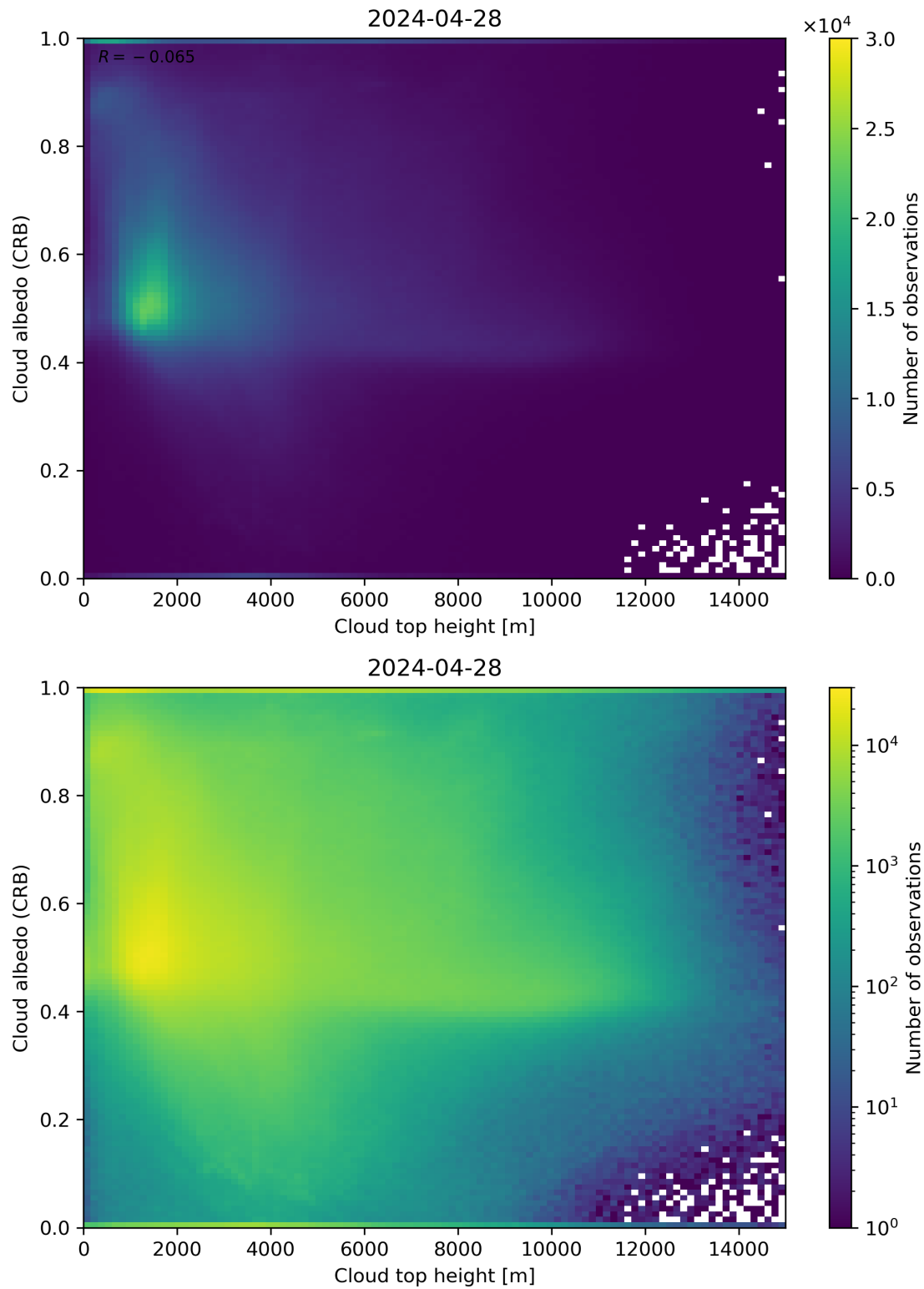
Figure 86: Scatter density plot of “Cloud top height” against “Cloud albedo (CRB)” for 2024-04-27 to 2024-04-29.
