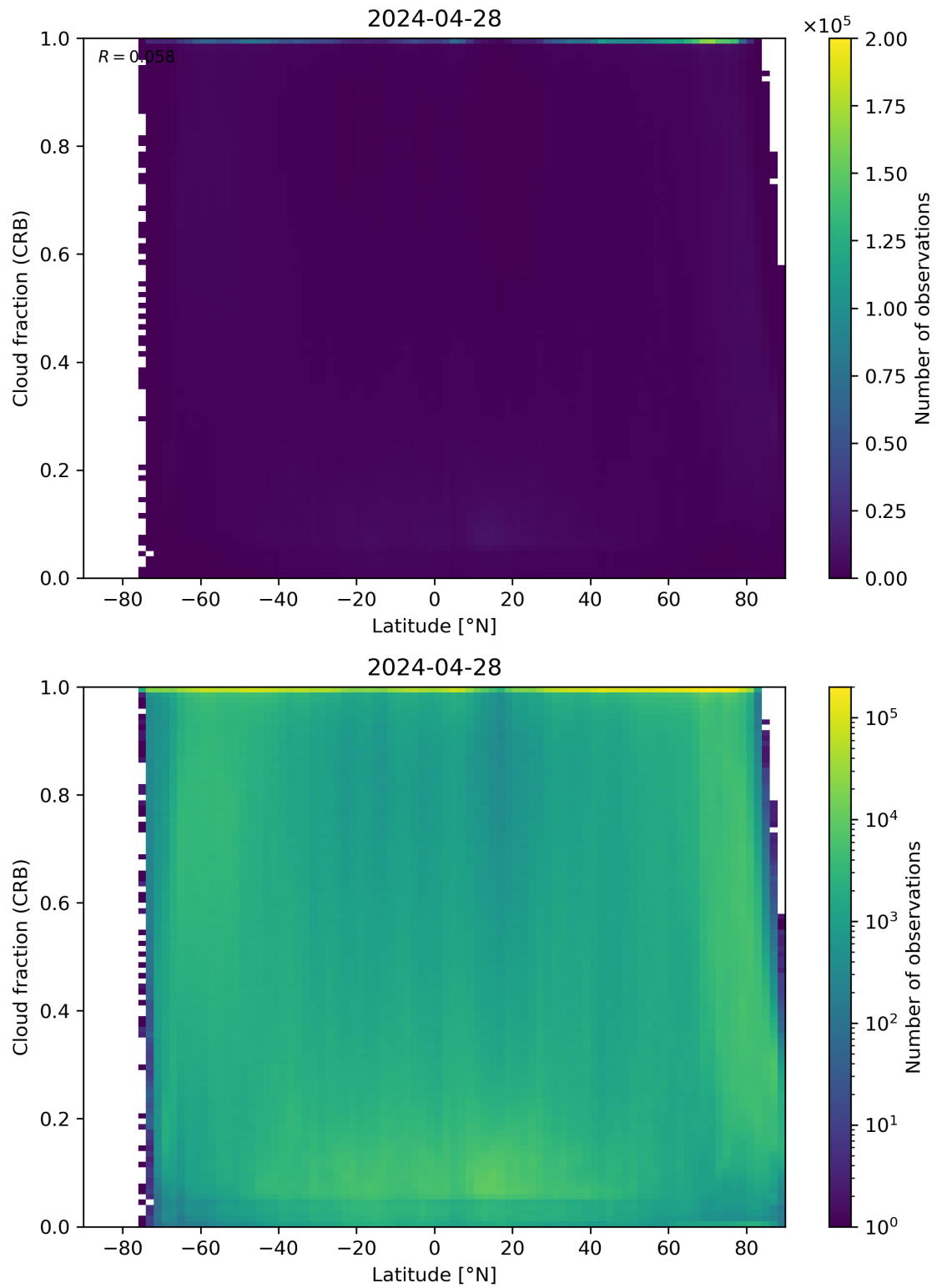
Figure 94: Scatter density plot of “Latitude” against “Cloud fraction (CRB)” for 2024-04-27 to 2024-04-29.
