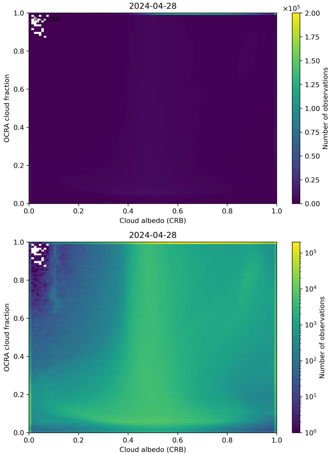
Figure 70: Scatter density plot of “Cloud albedo (CRB)” against “OCRA cloud fraction” for 2024-04-27 to 2024-04-29.
