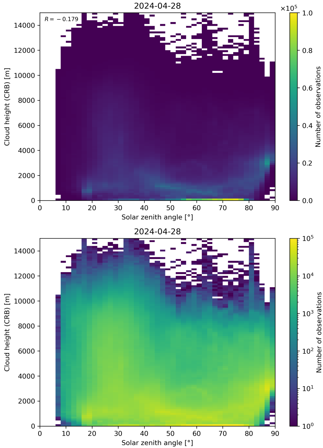
Figure 102: Scatter density plot of “Solar zenith angle” against “Cloud height (CRB)” for 2024-04-27 to 2024-04-29.
