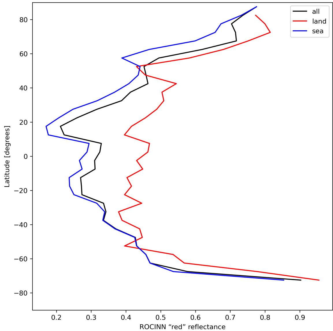
Figure 37: Zonal average of “ROCINN “red” reflectance” for 2024-04-27 to 2024-04-29.
