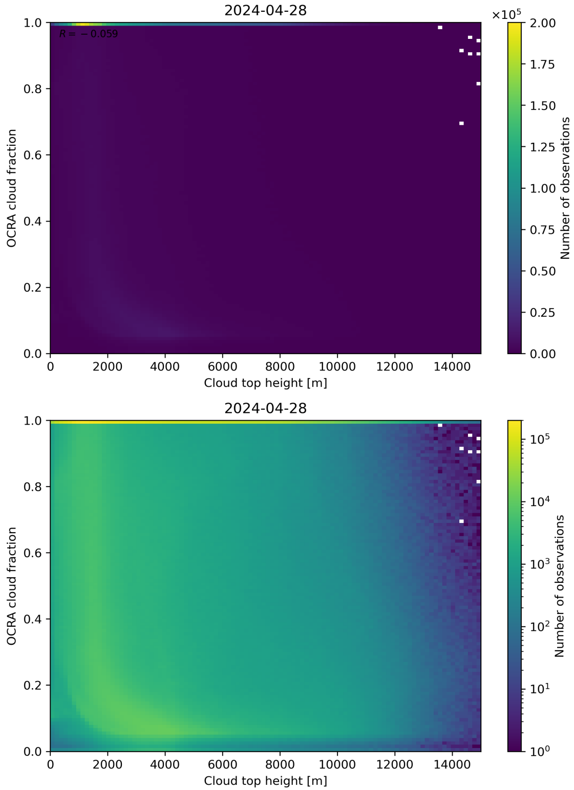
Figure 87: Scatter density plot of “Cloud top height” against “OCRA cloud fraction” for 2024-04-27 to 2024-04-29.
