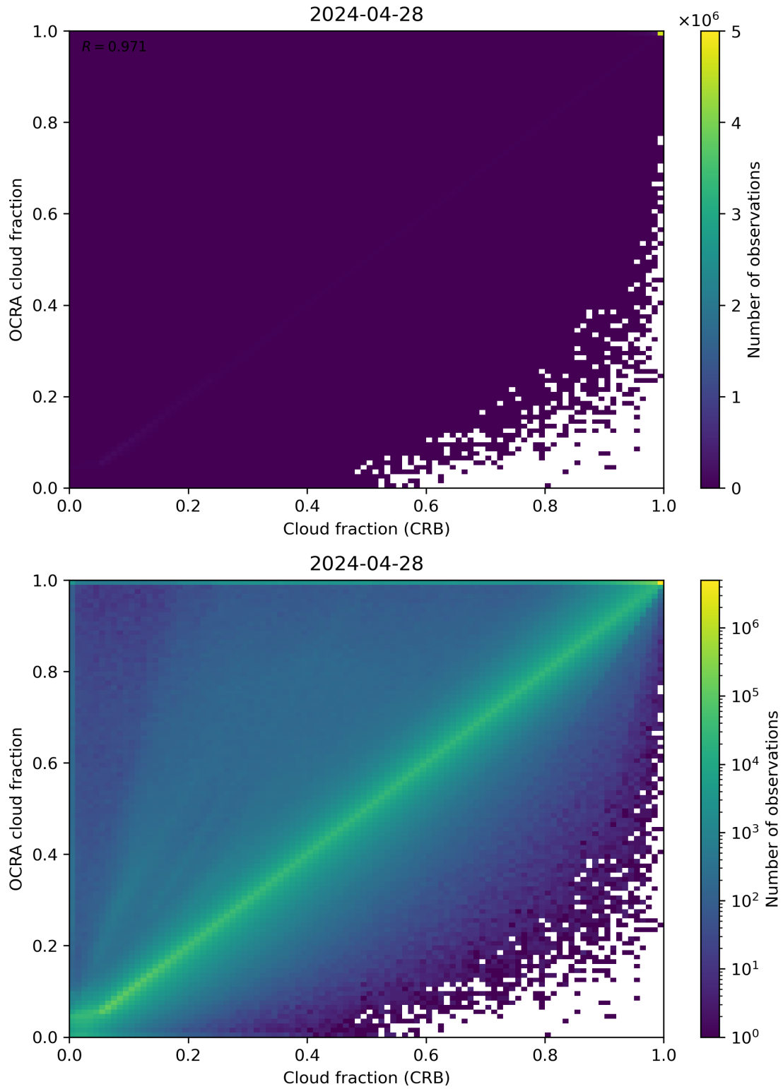
Figure 78: Scatter density plot of “Cloud fraction (CRB)” against “OCRA cloud fraction” for 2024-04-27 to 2024-04-29.
