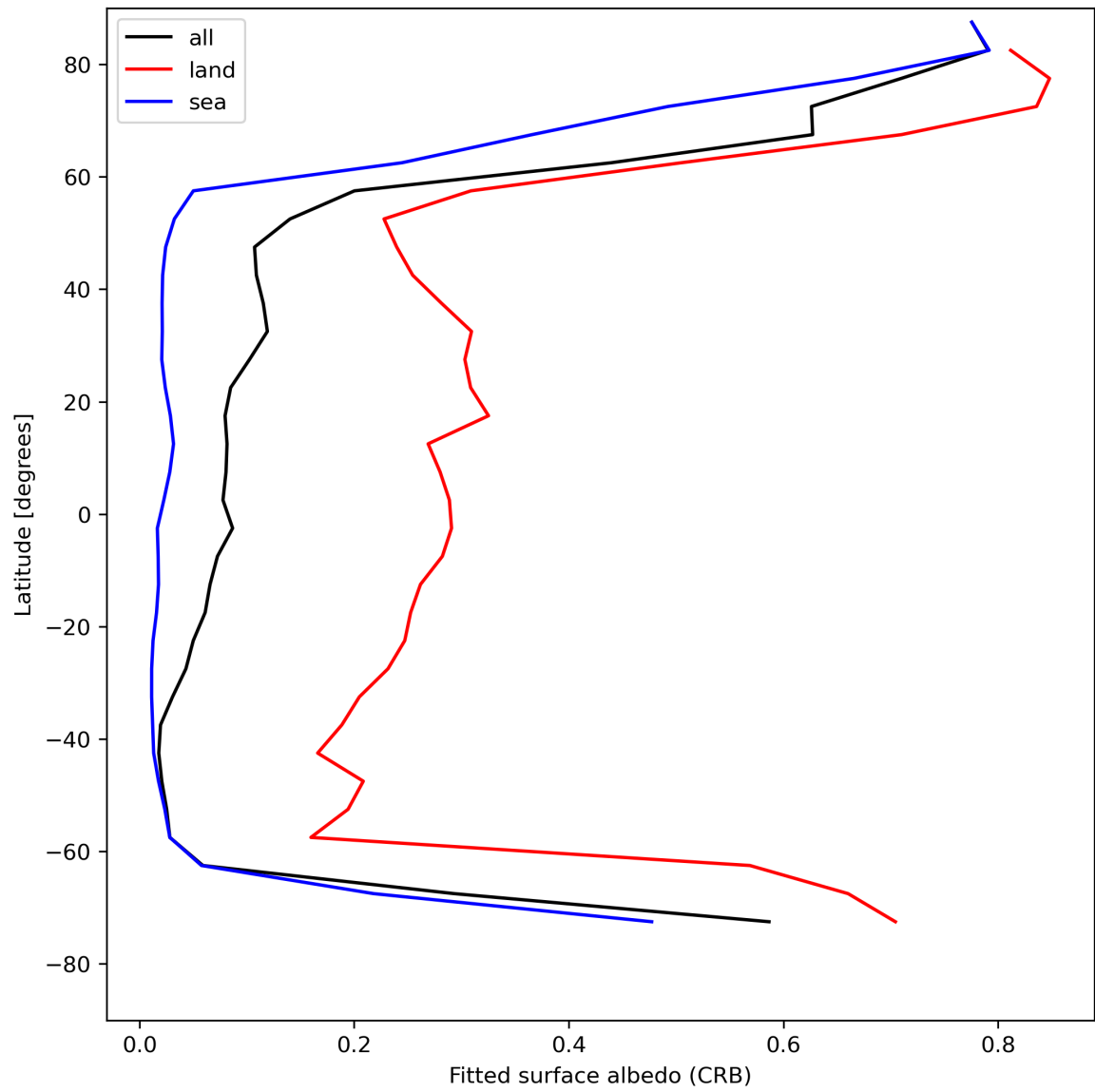
Figure 30: Zonal average of “Fitted surface albedo (CRB)” for 2024-04-27 to 2024-04-29.
