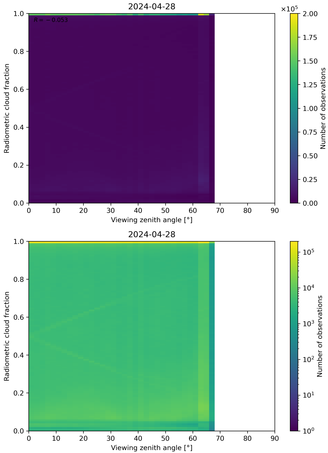
Figure 107: Scatter density plot of “Viewing zenith angle” against “Radiometric cloud fraction” for 2024-04-27 to 2024-04-29.
