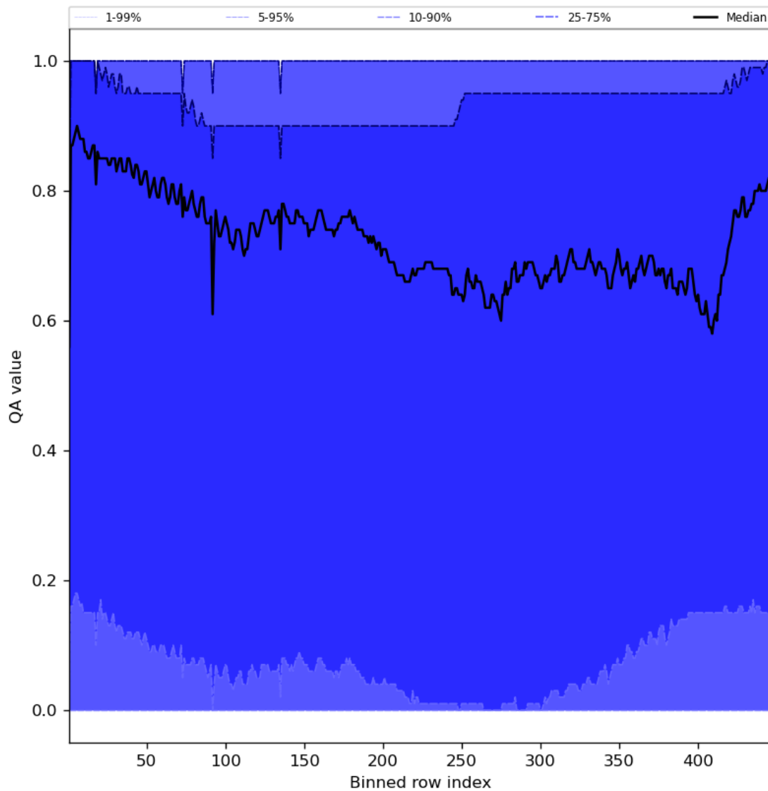
Figure 54: Along track statistics of “QA value” for 2024-04-27 to 2024-04-29
