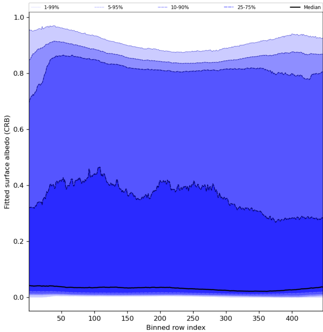
Figure 62: Along track statistics of “Fitted surface albedo (CRB)” for 2024-04-27 to 2024-04-29
