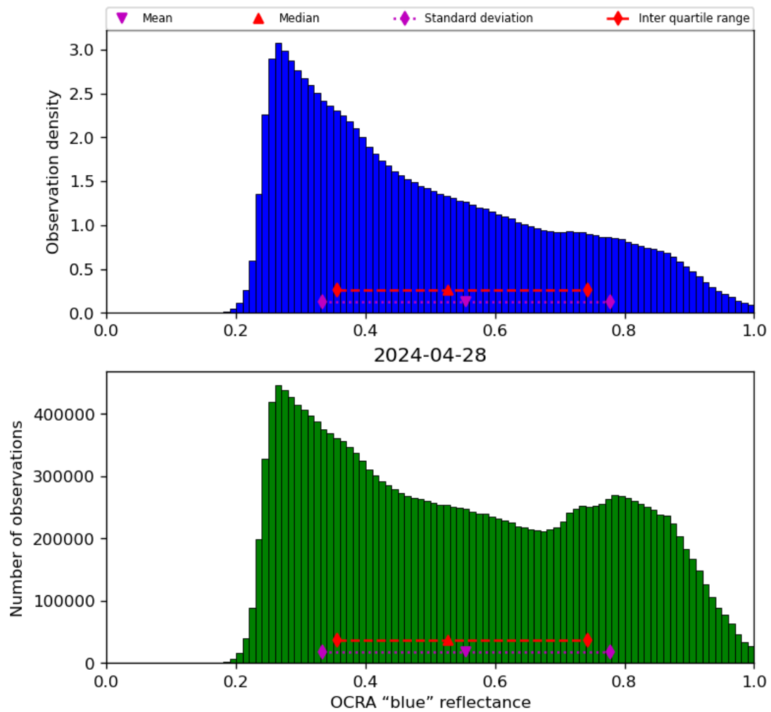
Figure 51: Histogram of “OCRA “blue” reflectance” for 2024-04-27 to 2024-04-29
