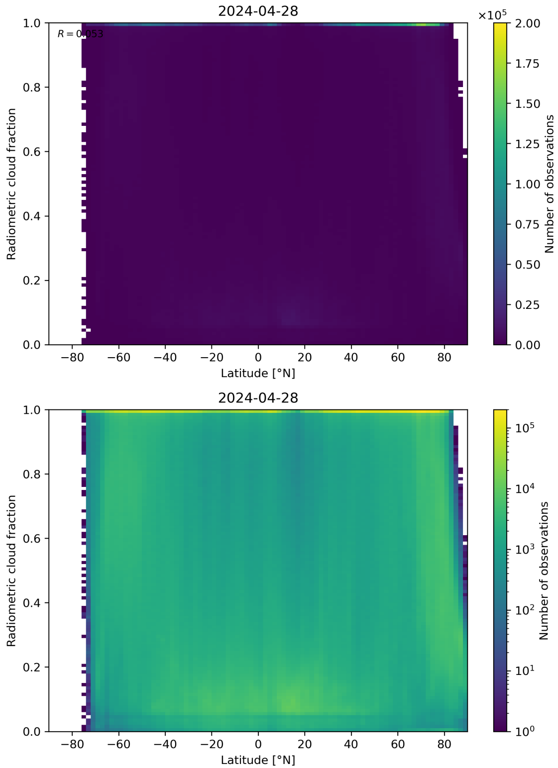
Figure 92: Scatter density plot of “Latitude” against “Radiometric cloud fraction” for 2024-04-27 to 2024-04-29.
