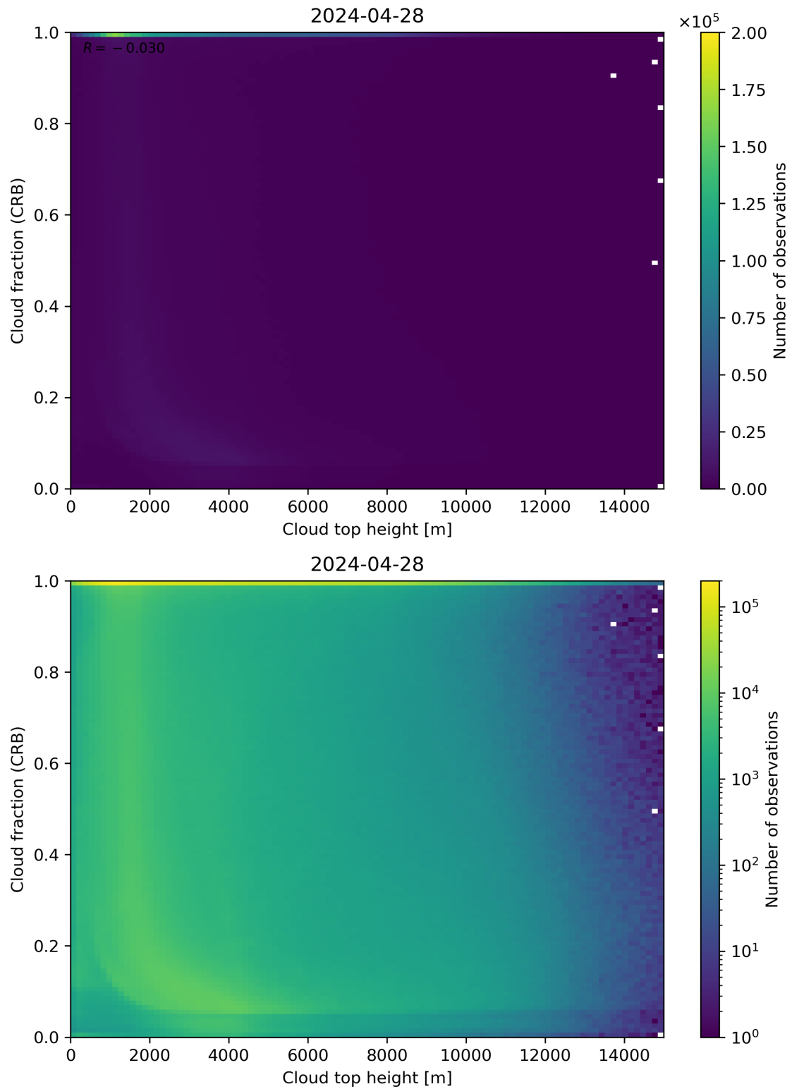
Figure 88: Scatter density plot of “Cloud top height” against “Cloud fraction (CRB)” for 2024-04-27 to 2024-04-29.
