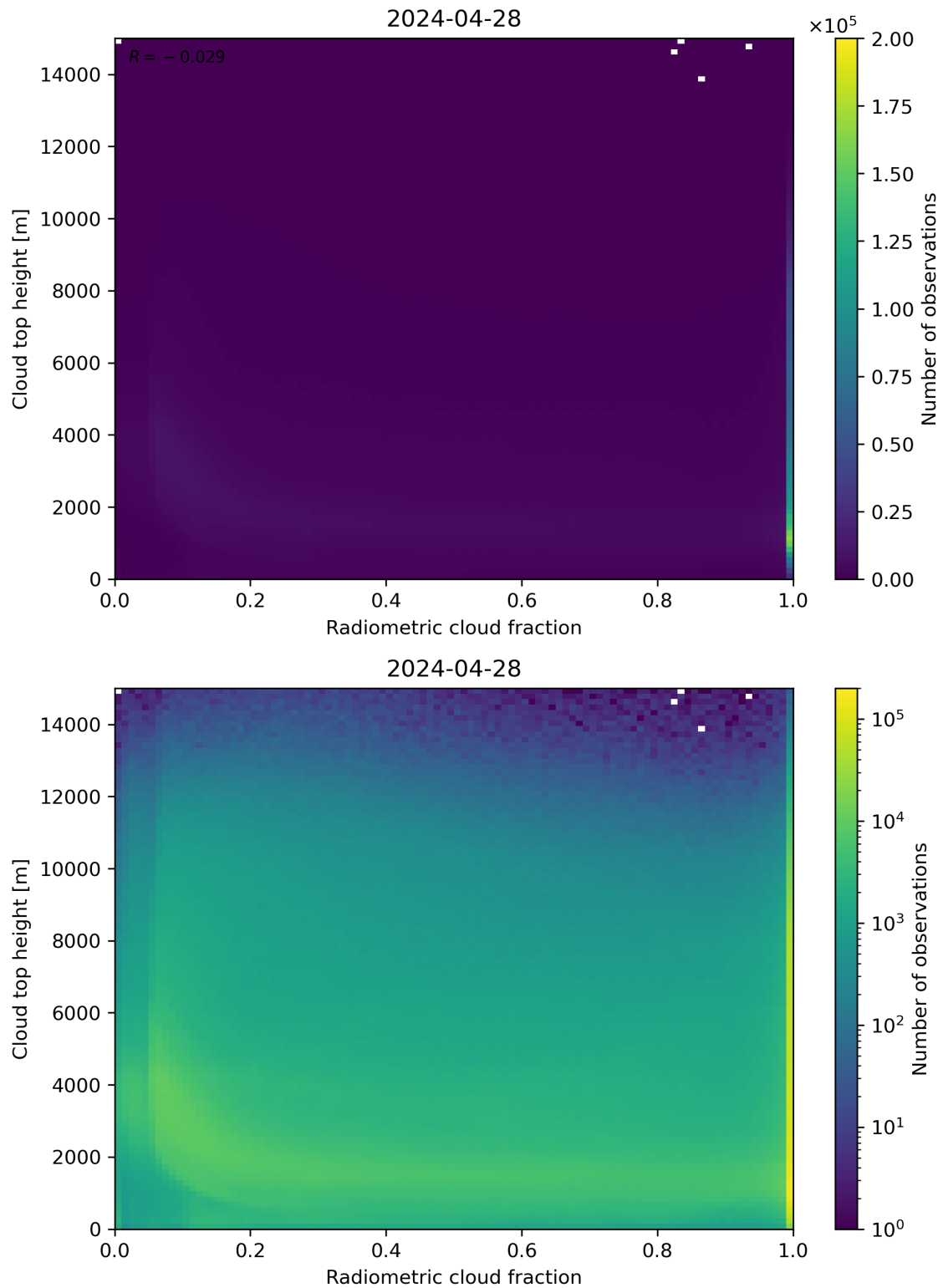
Figure 76: Scatter density plot of “Radiometric cloud fraction” against “Cloud top height” for 2024-04-27 to 2024-04-29.
