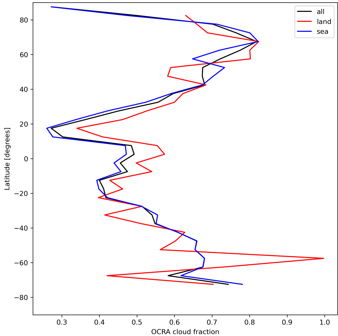
Figure 34: Zonal average of “OCRA cloud fraction” for 2024-04-27 to 2024-04-29.
