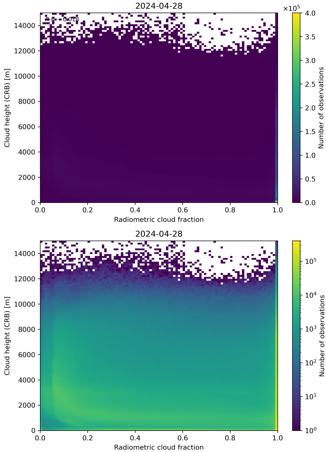
Figure 74: Scatter density plot of “Radiometric cloud fraction” against “Cloud height (CRB)” for 2024-04-27 to 2024-04-29.
