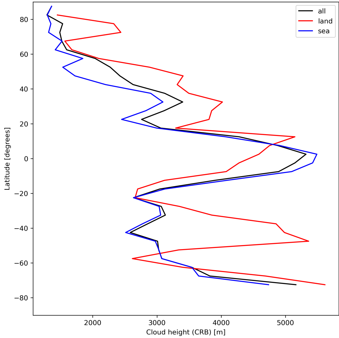
Figure 27: Zonal average of “Cloud height (CRB)” for 2024-04-27 to 2024-04-29.
