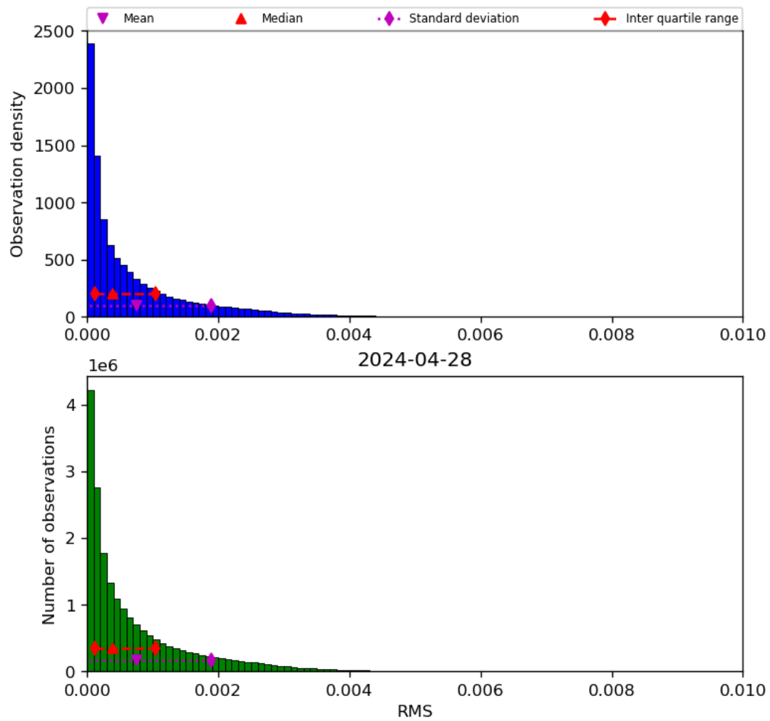
Figure 47: Histogram of “RMS” for 2024-04-27 to 2024-04-29
