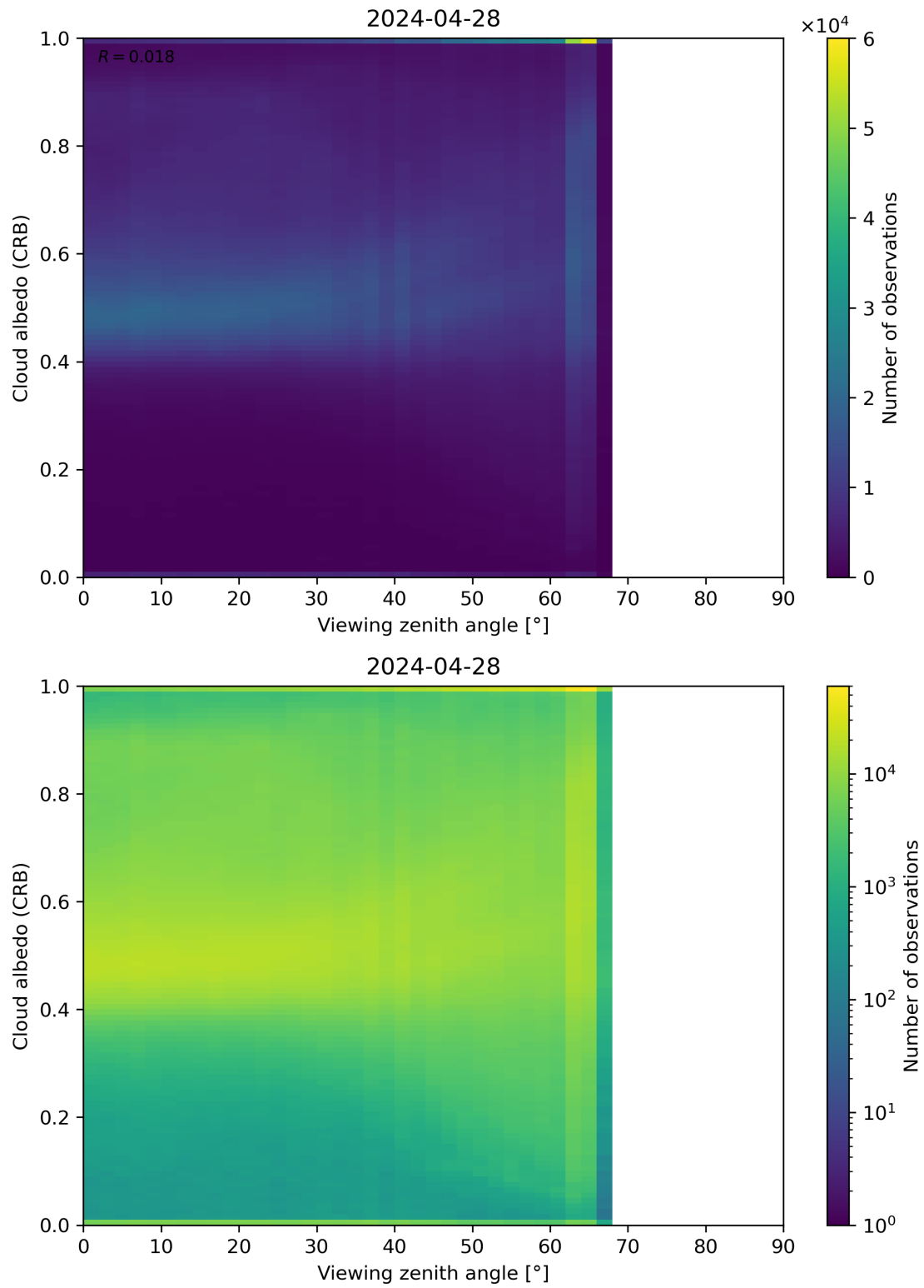
Figure 106: Scatter density plot of “Viewing zenith angle” against “Cloud albedo (CRB)” for 2024-04-27 to 2024-04-29.
