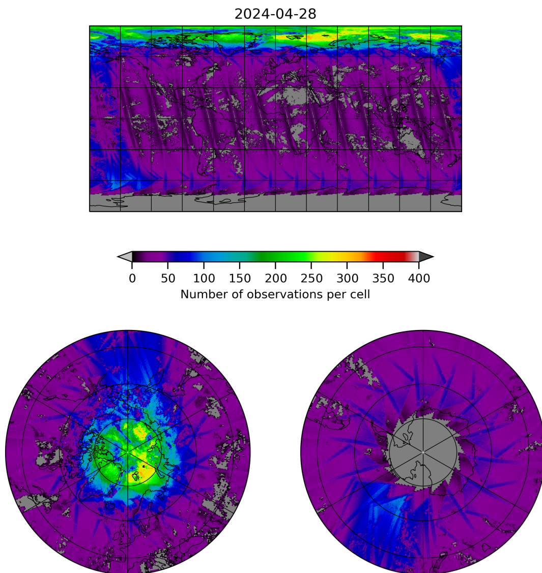
Figure 21: Map of the number of observations for 2024-04-27 to 2024-04-29
