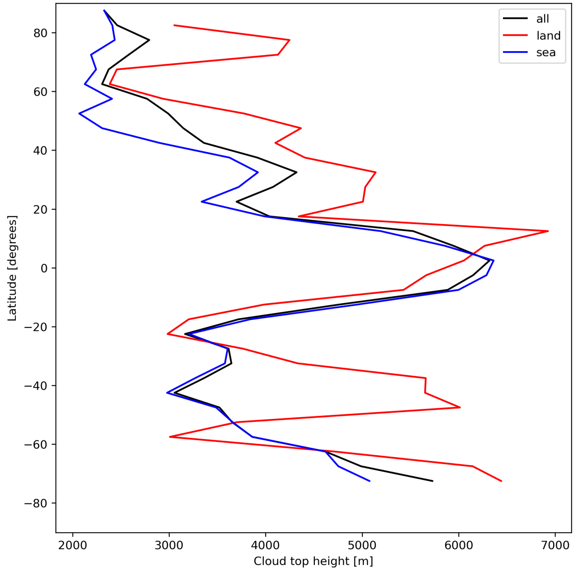
Figure 24: Zonal average of “Cloud top height” for 2024-04-27 to 2024-04-29.
