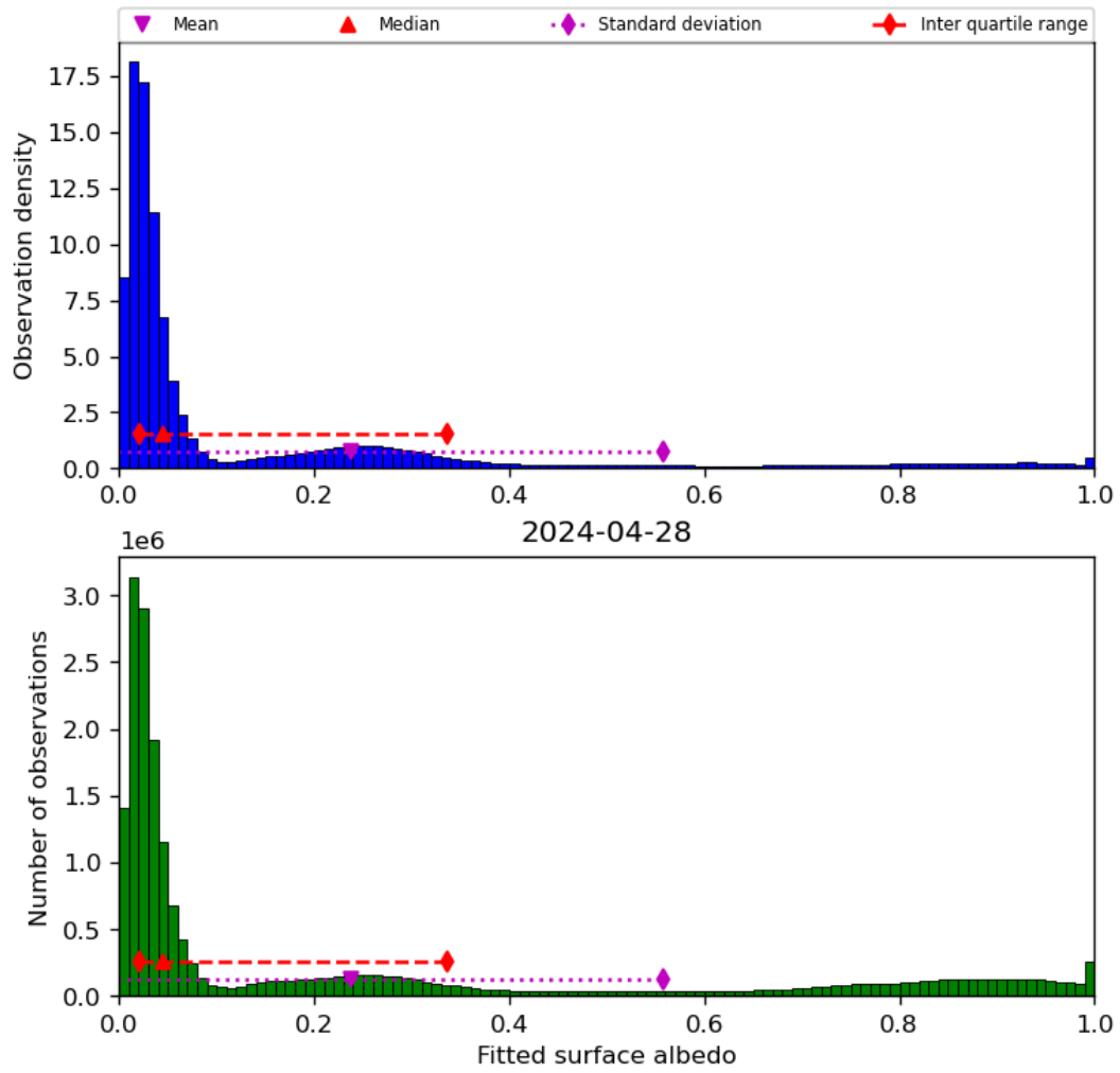
Figure 45: Histogram of “Fitted surface albedo” for 2024-04-27 to 2024-04-29
