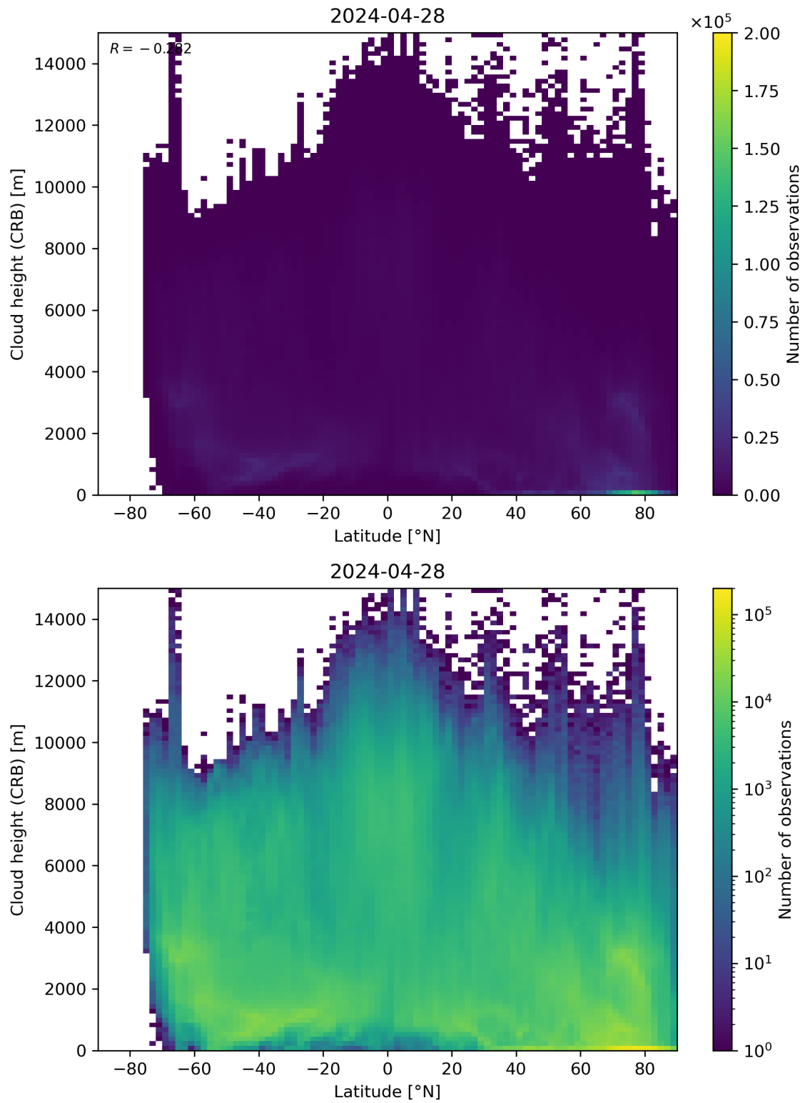
Figure 95: Scatter density plot of “Latitude” against “Cloud height (CRB)” for 2024-04-27 to 2024-04-29.
