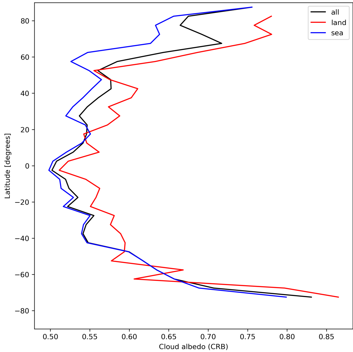
Figure 28: Zonal average of “Cloud albedo (CRB)” for 2024-04-27 to 2024-04-29.
