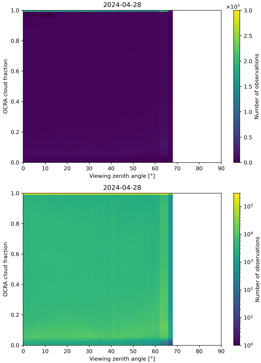
Figure 108: Scatter density plot of “Viewing zenith angle” against “OCRA cloud fraction” for 2024-04-27 to 2024-04-29.
