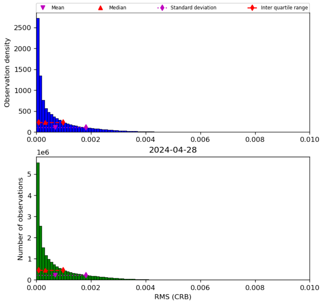
Figure 48: Histogram of "RMS (CRB)" for 2024-04-27 to 2024-04-29
