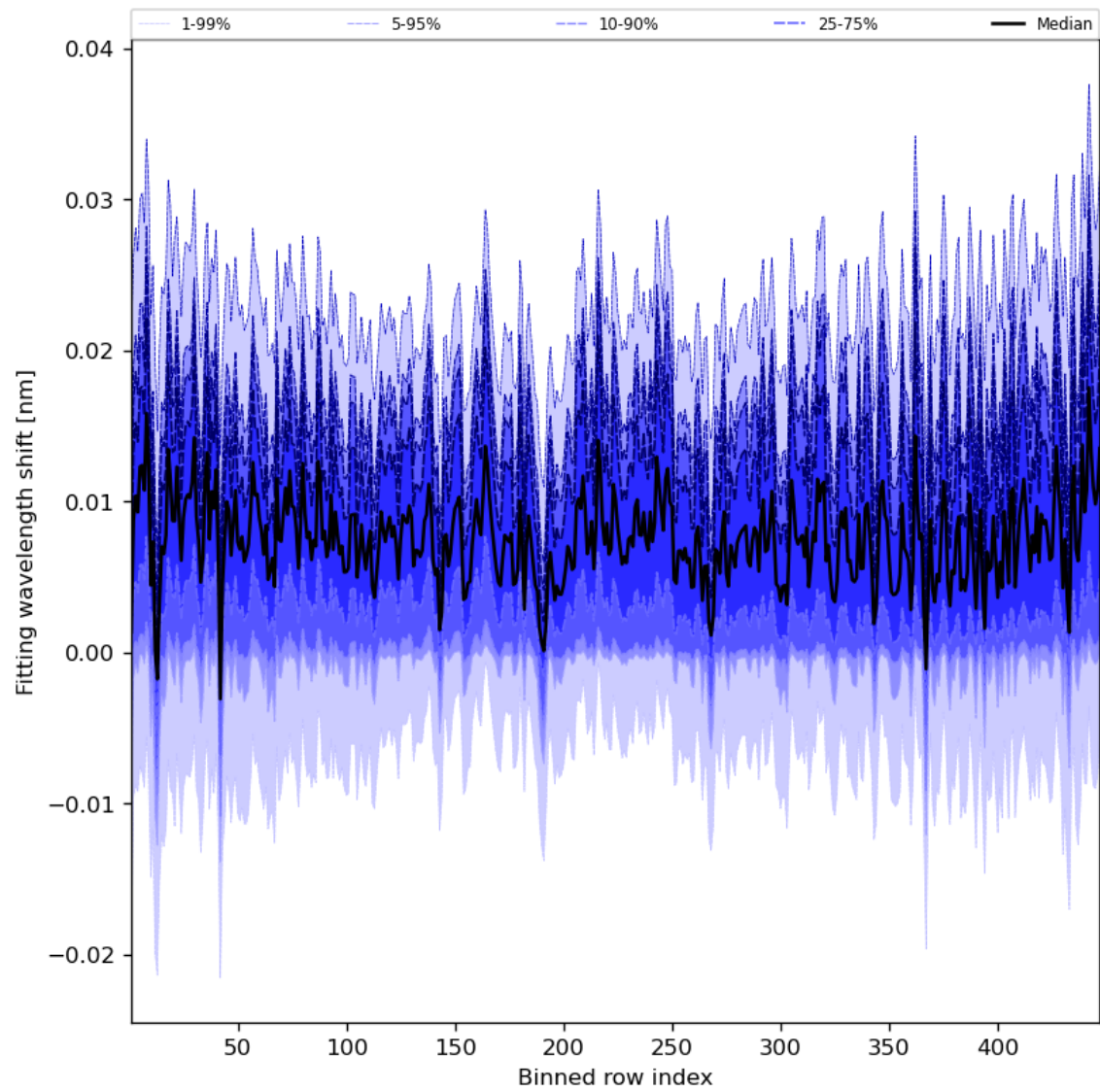
Figure 65: Along track statistics of “Fitting wavelength shift” for 2024-04-27 to 2024-04-29
