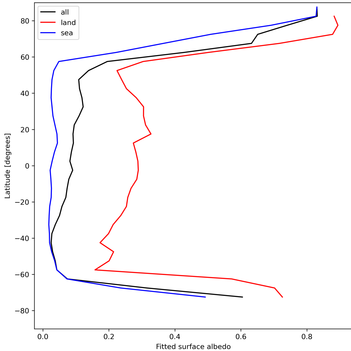
Figure 29: Zonal average of “Fitted surface albedo” for 2024-04-27 to 2024-04-29.
