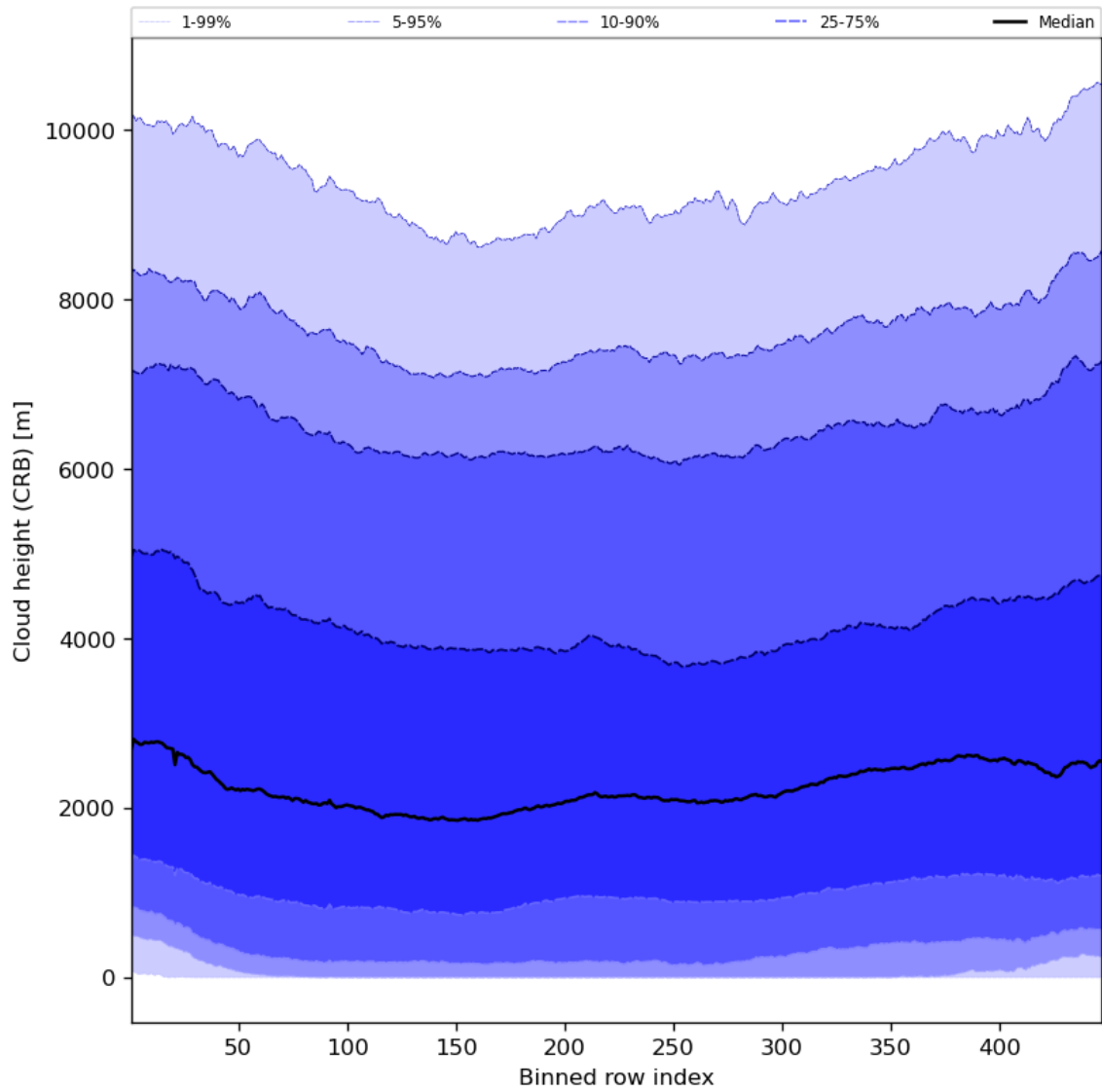
Figure 59: Along track statistics of “Cloud height (CRB)” for 2024-04-27 to 2024-04-29
