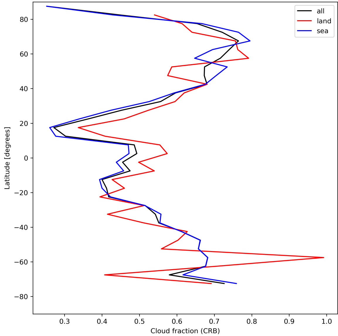
Figure 26: Zonal average of “Cloud fraction (CRB)” for 2024-04-27 to 2024-04-29.
