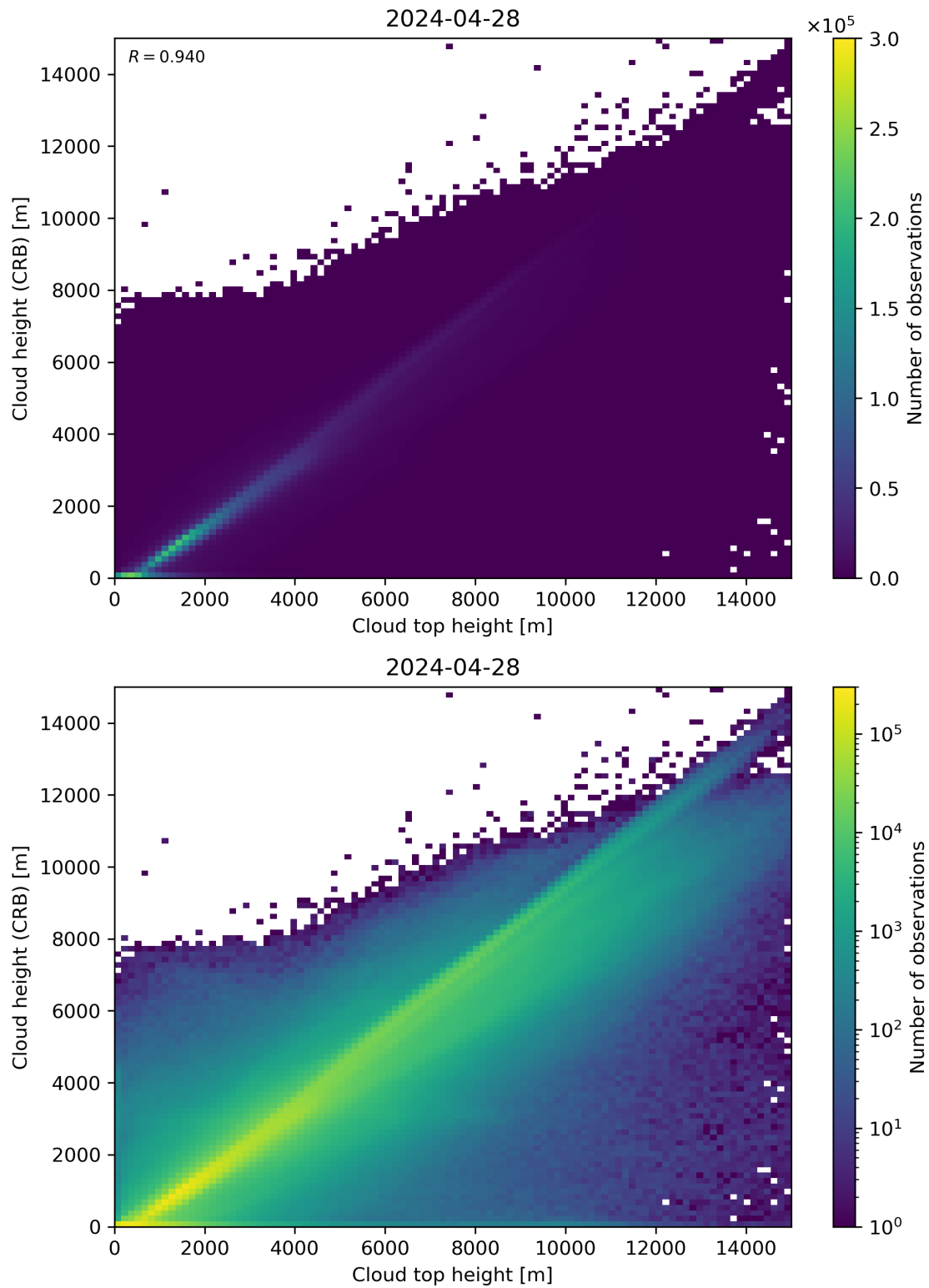
Figure 89: Scatter density plot of “Cloud top height” against “Cloud height (CRB)” for 2024-04-27 to 2024-04-29.
