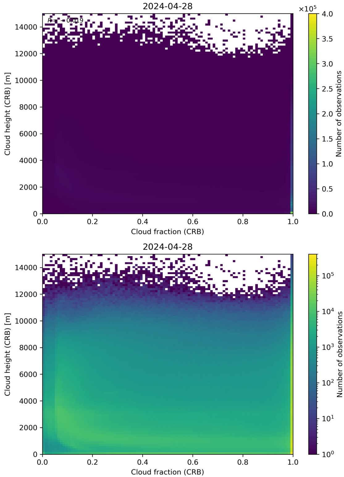
Figure 79: Scatter density plot of “Cloud fraction (CRB)” against “Cloud height (CRB)” for 2024-04-27 to 2024-04-29.
