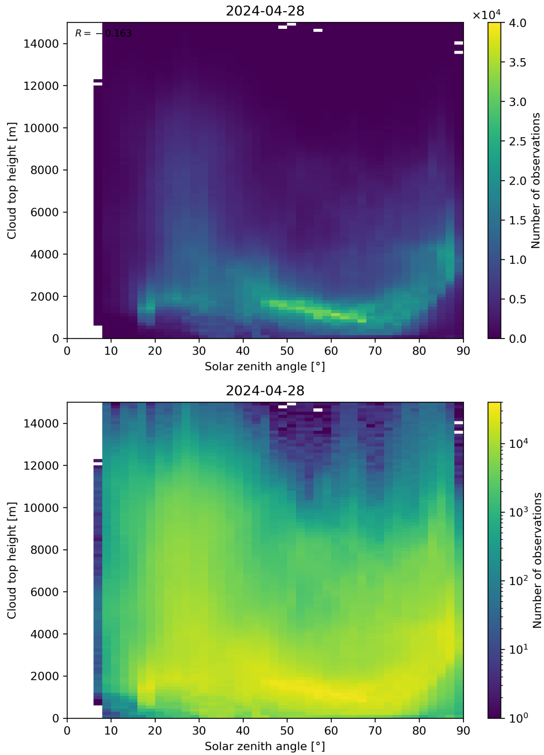
Figure 104: Scatter density plot of “Solar zenith angle” against “Cloud top height” for 2024-04-27 to 2024-04-29.
