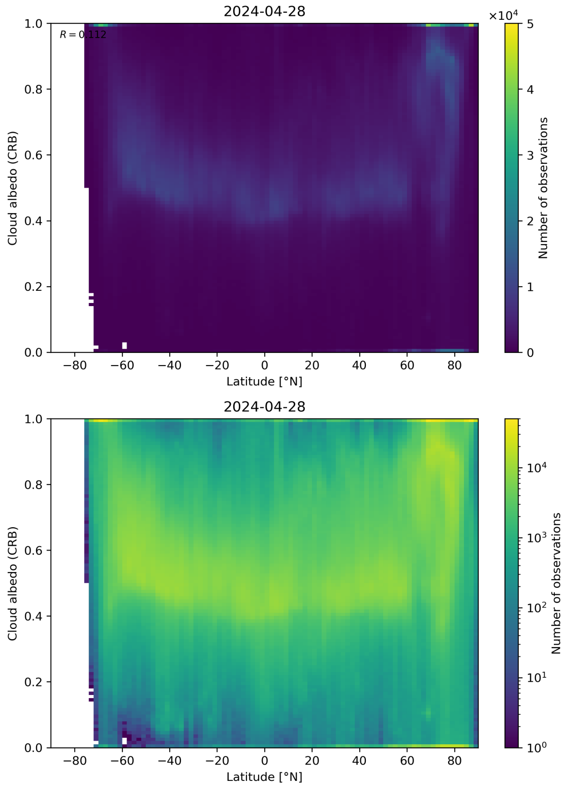
Figure 91: Scatter density plot of “Latitude” against “Cloud albedo (CRB)” for 2024-04-27 to 2024-04-29.
