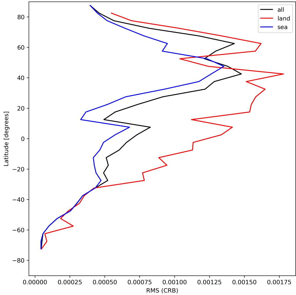
Figure 32: Zonal average of “RMS (CRB)” for 2024-04-27 to 2024-04-29.
