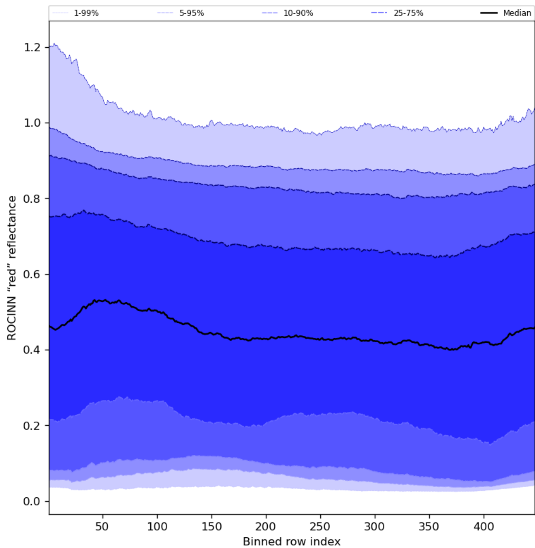
Figure 69: Along track statistics of “ROCINN “red” reflectance” for 2024-04-27 to 2024-04-29
