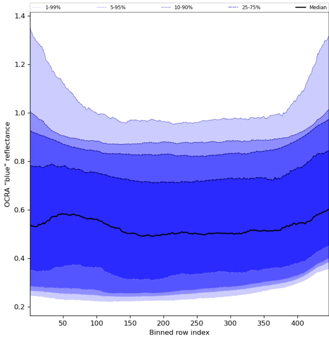
Figure 67: Along track statistics of “OCRA “blue” reflectance” for 2024-04-27 to 2024-04-29
