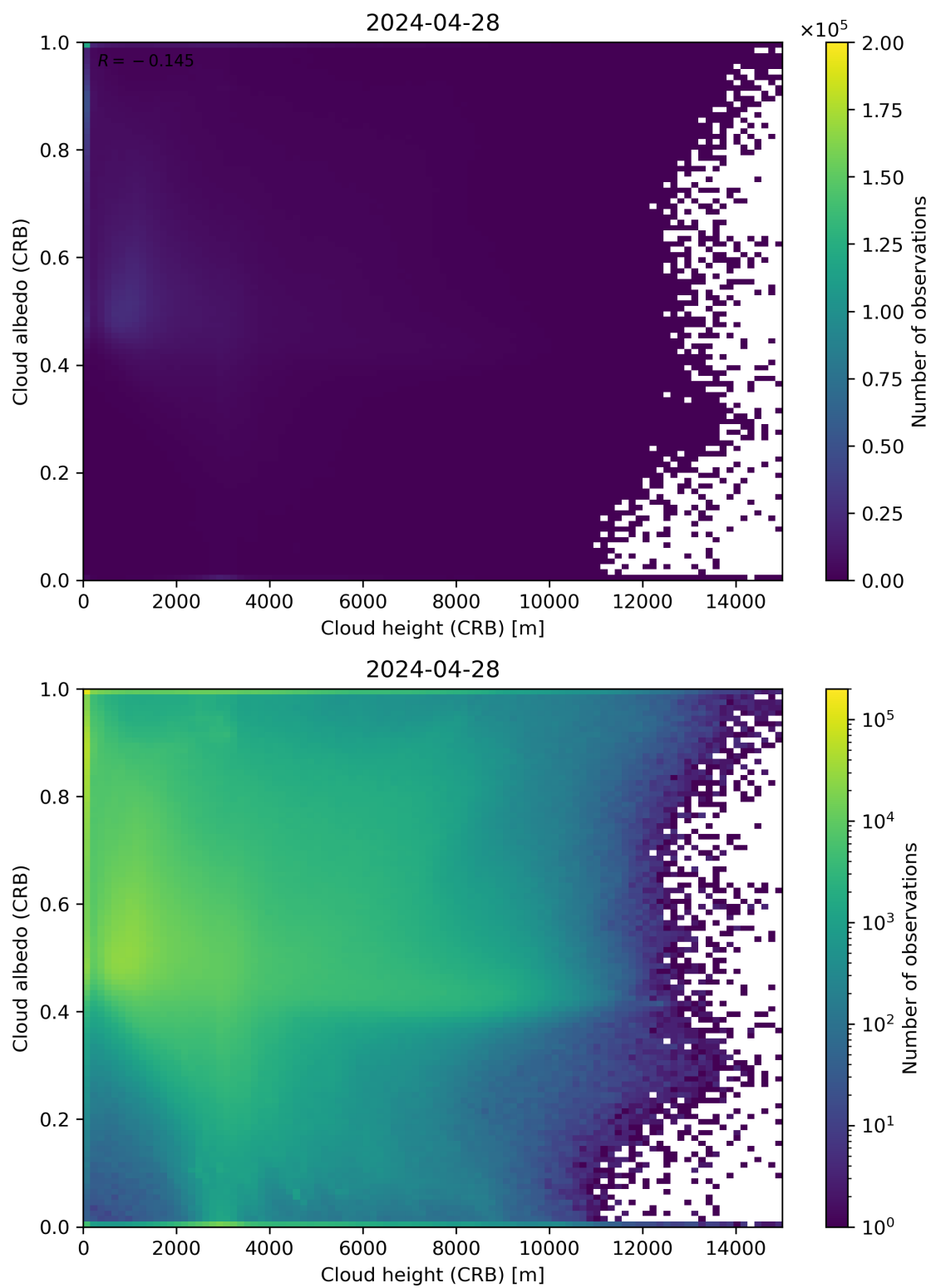
Figure 80: Scatter density plot of “Cloud height (CRB)” against “Cloud albedo (CRB)” for 2024-04-27 to 2024-04-29.
