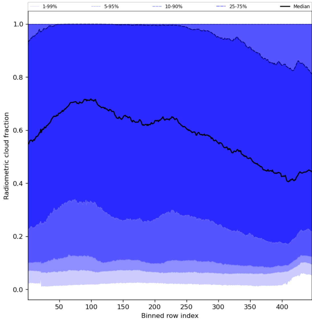
Figure 55: Along track statistics of “Radiometric cloud fraction” for 2024-04-27 to 2024-04-29
