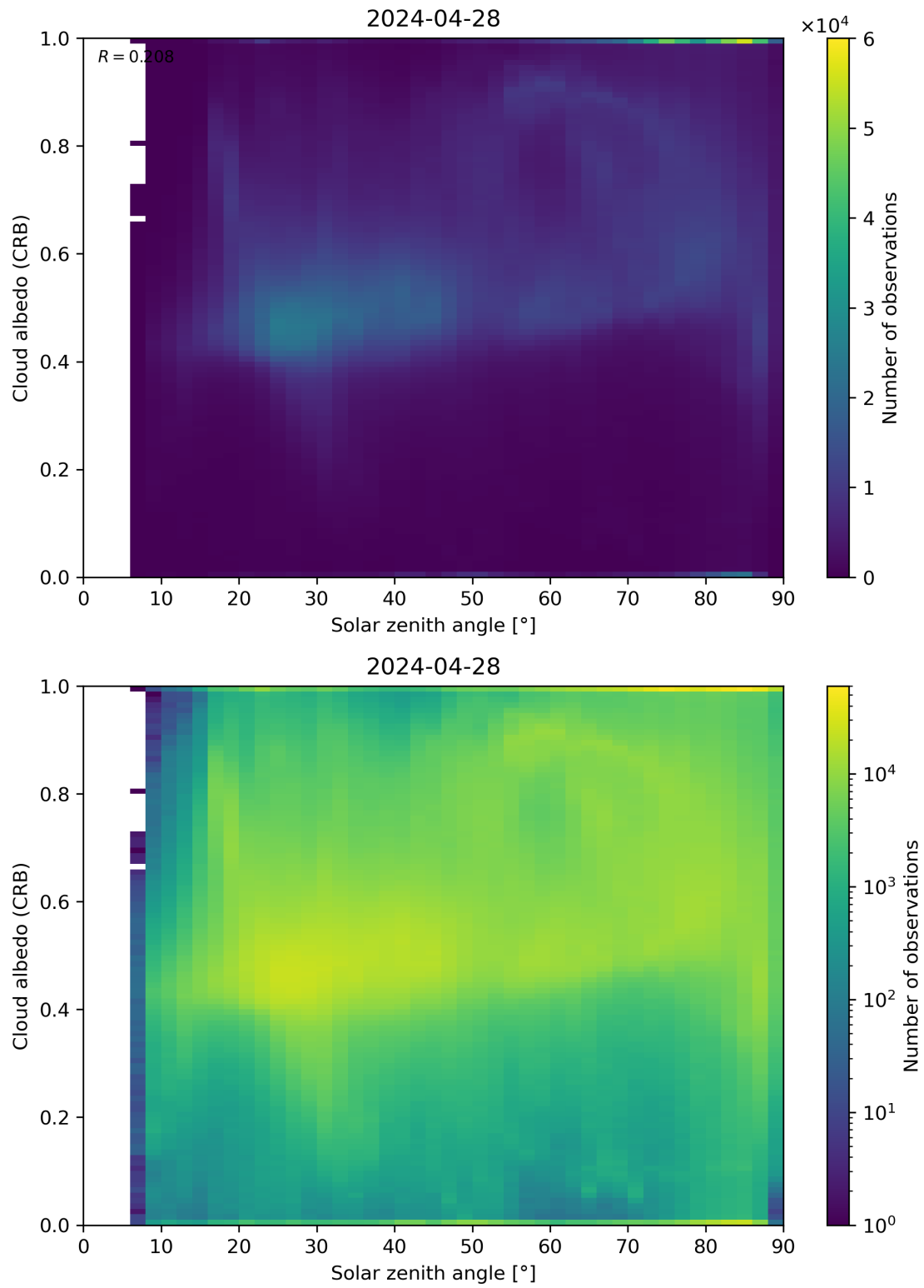
Figure 98: Scatter density plot of “Solar zenith angle” against “Cloud albedo (CRB)” for 2024-04-27 to 2024-04-29.
