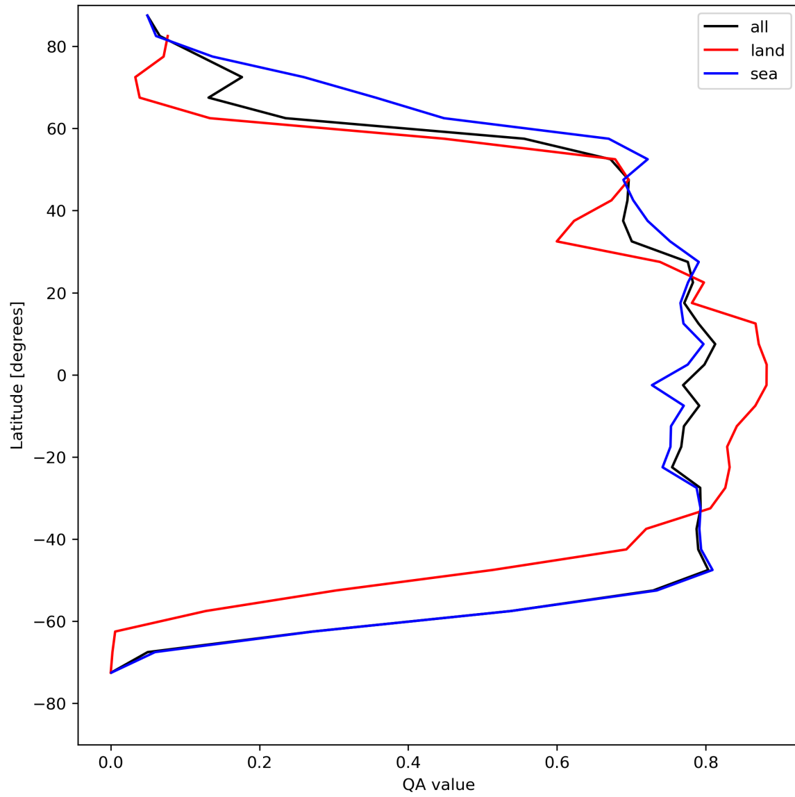
Figure 22: Zonal average of “QA value” for 2024-04-27 to 2024-04-29.
