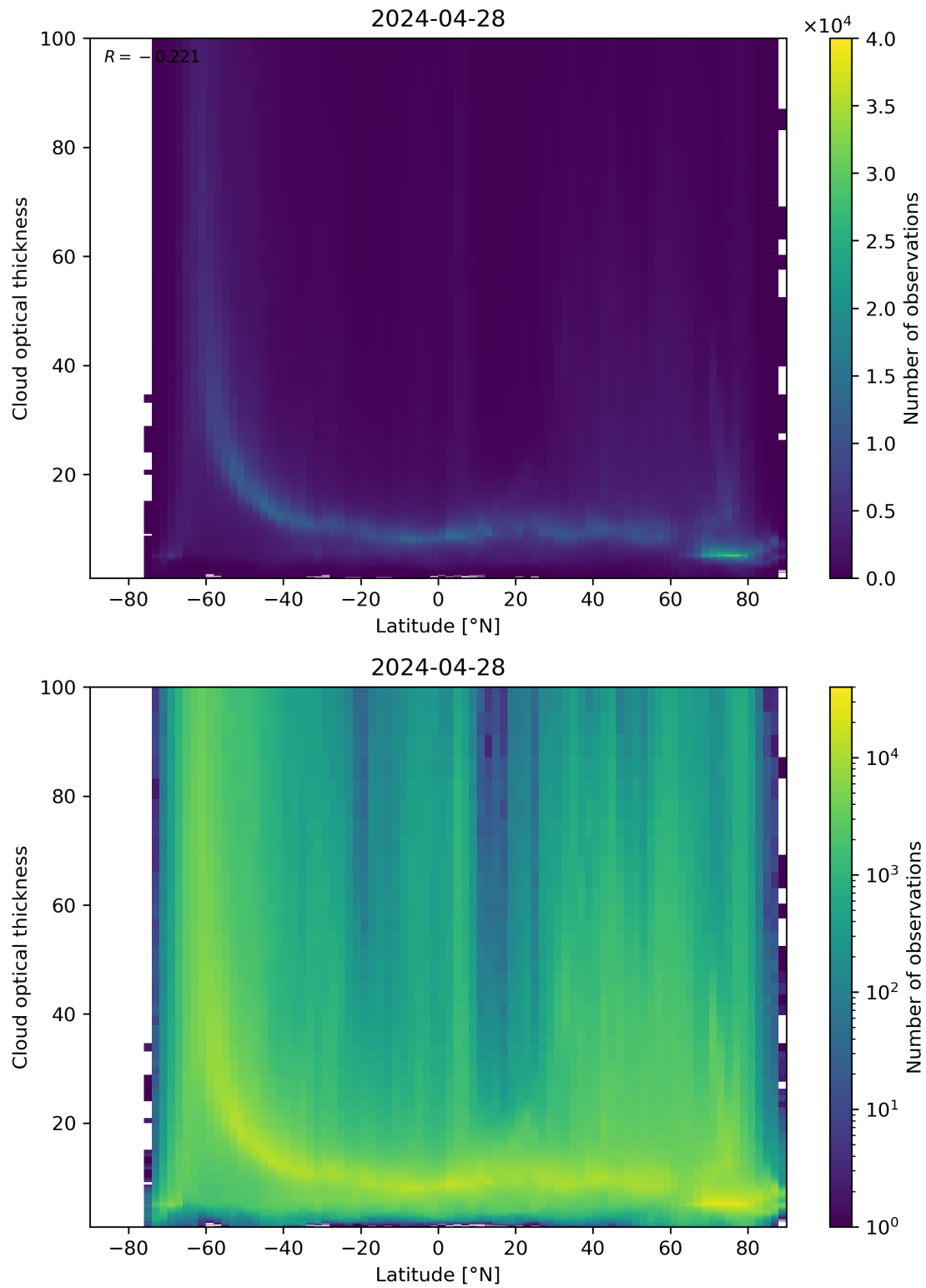
Figure 96: Scatter density plot of “Latitude” against “Cloud optical thickness” for 2024-04-27 to 2024-04-29.
