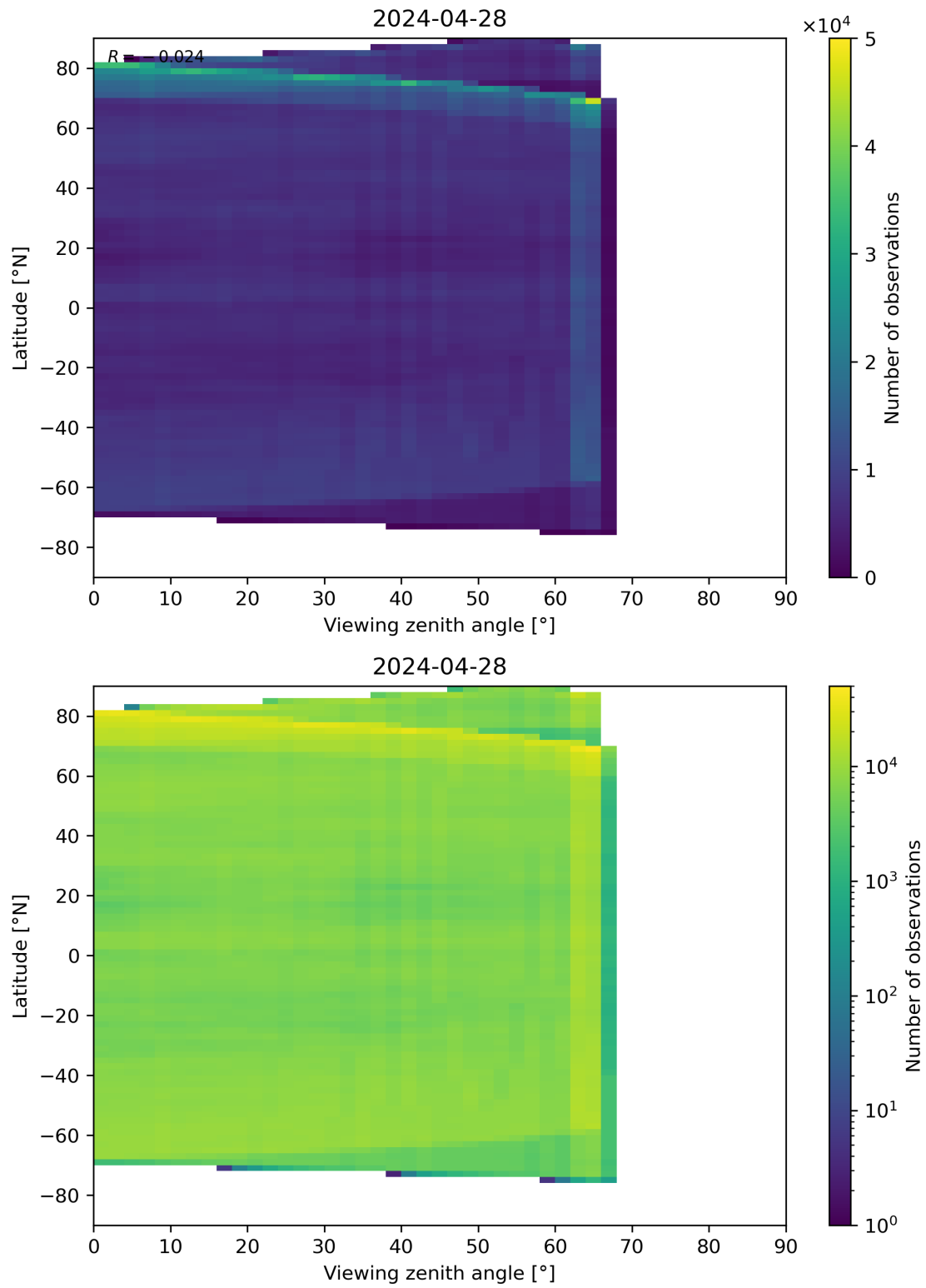
Figure 113: Scatter density plot of “Viewing zenith angle” against “Latitude” for 2024-04-27 to 2024-04-29.
