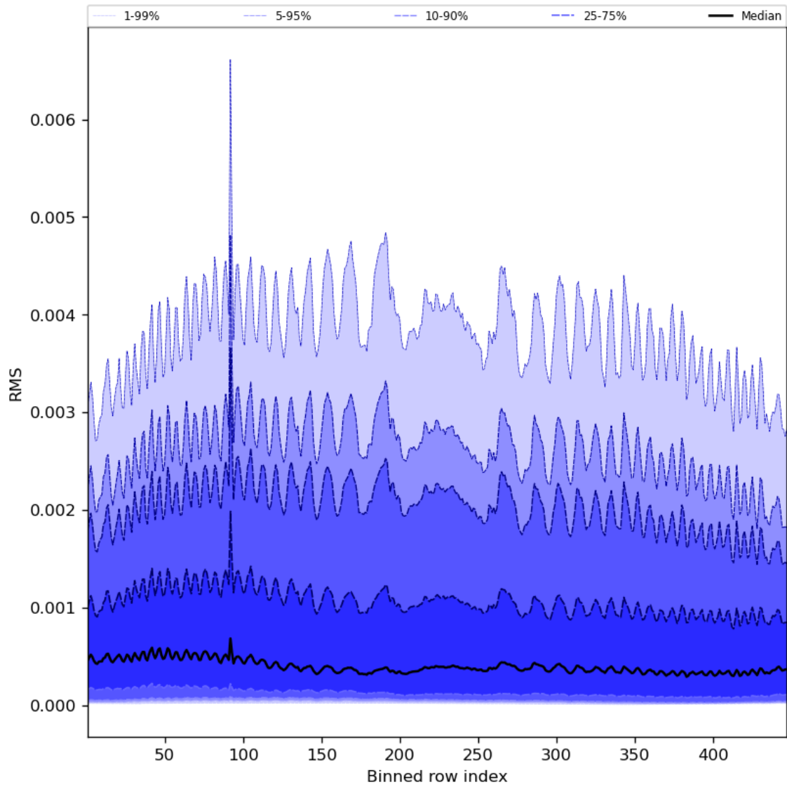
Figure 63: Along track statistics of “RMS” for 2024-04-27 to 2024-04-29
