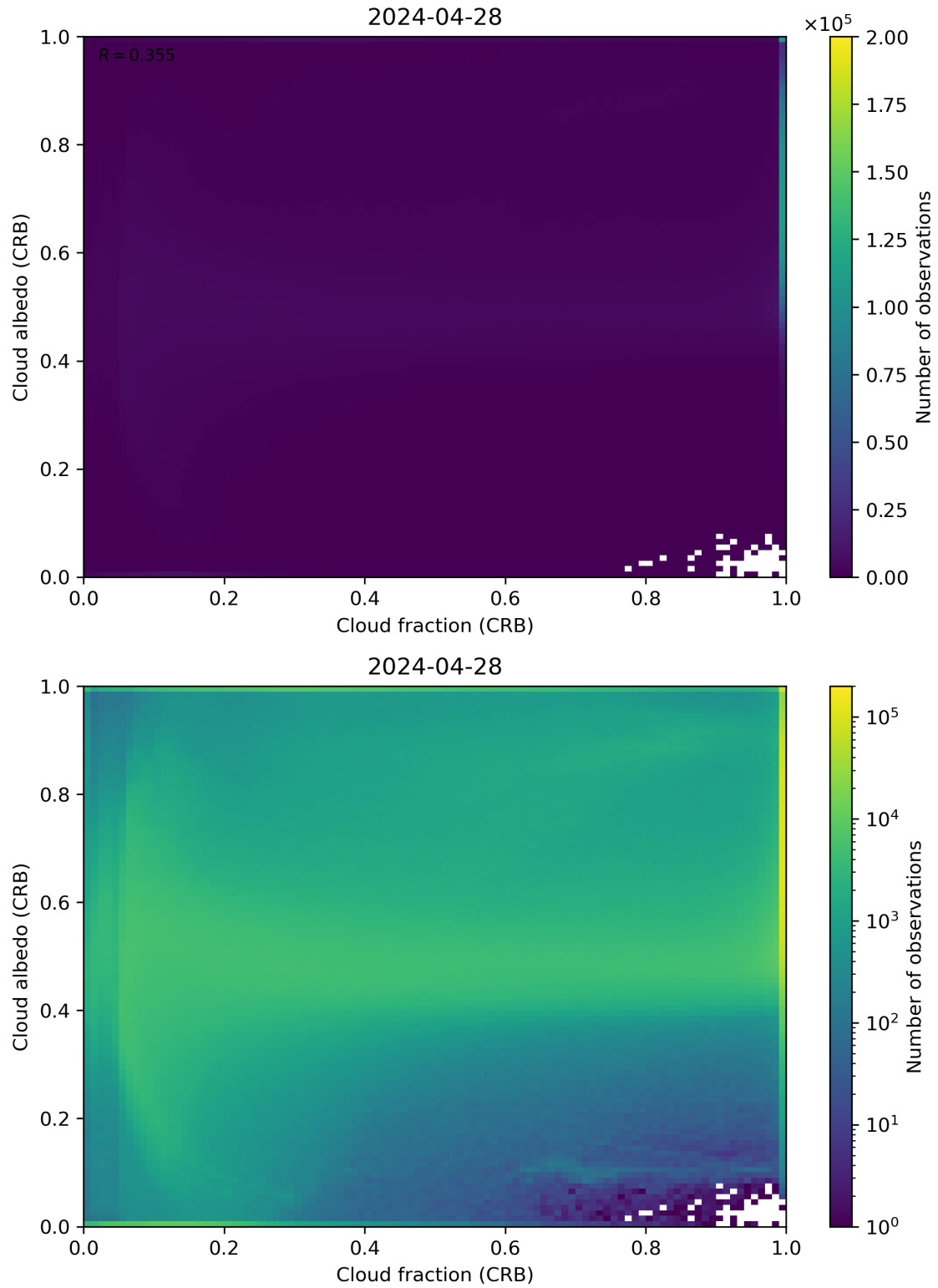
Figure 77: Scatter density plot of “Cloud fraction (CRB)” against “Cloud albedo (CRB)” for 2024-04-27 to 2024-04-29.
