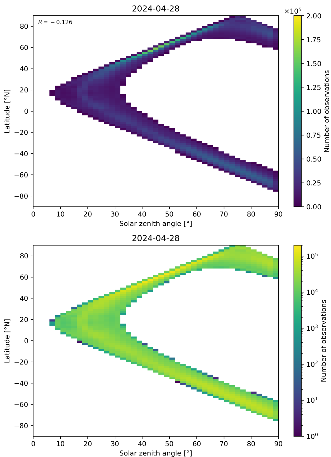
Figure 105: Scatter density plot of “Solar zenith angle” against “Latitude” for 2024-04-27 to 2024-04-29.
