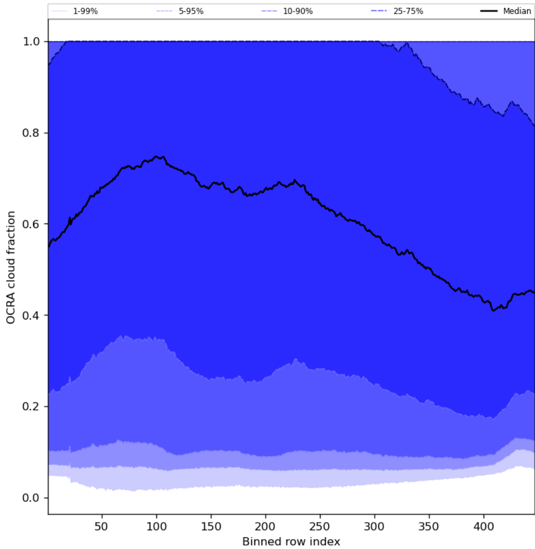
Figure 66: Along track statistics of “OCRA cloud fraction” for 2024-04-27 to 2024-04-29
