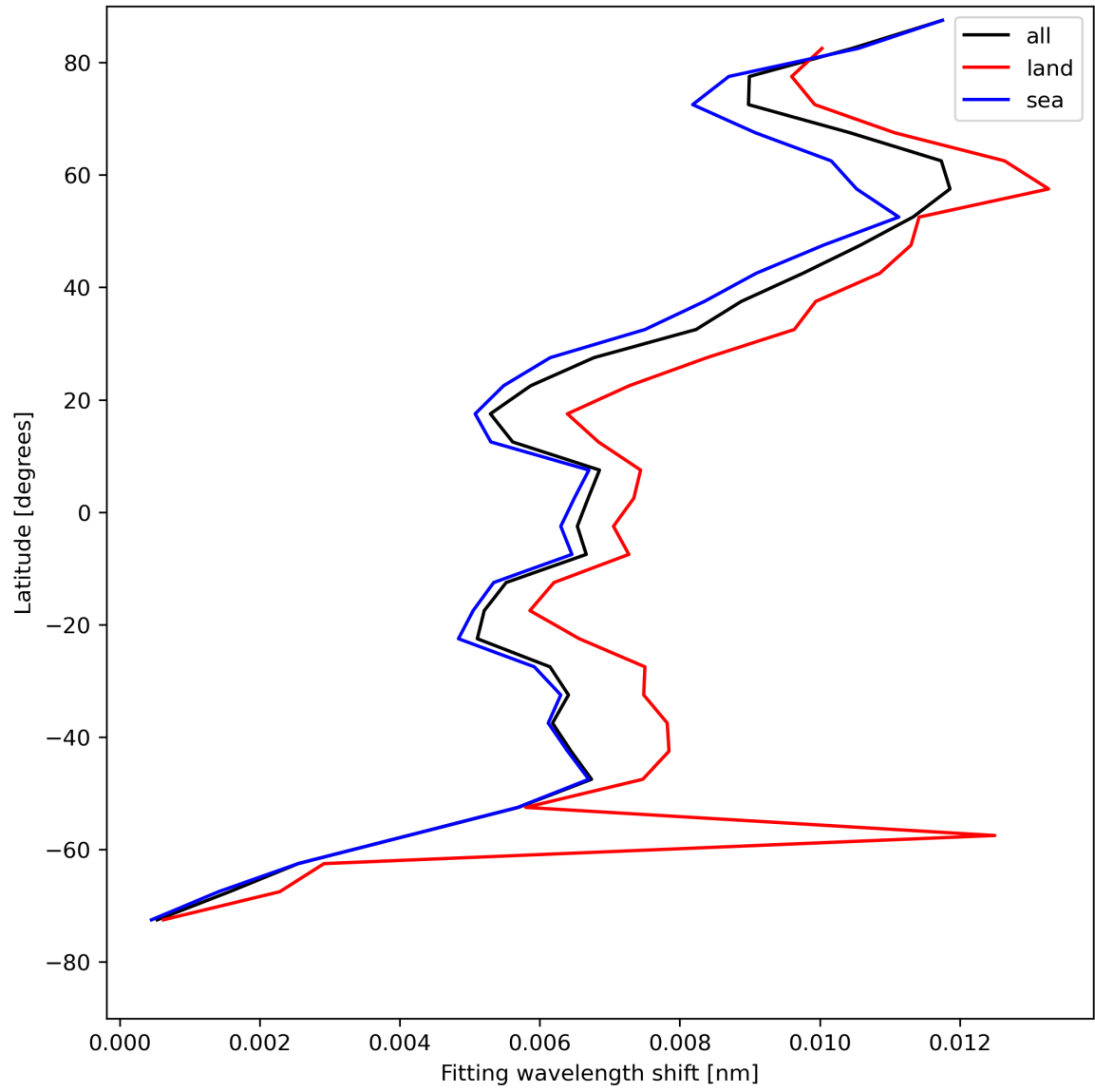
Figure 33: Zonal average of “Fitting wavelength shift” for 2024-04-27 to 2024-04-29.
