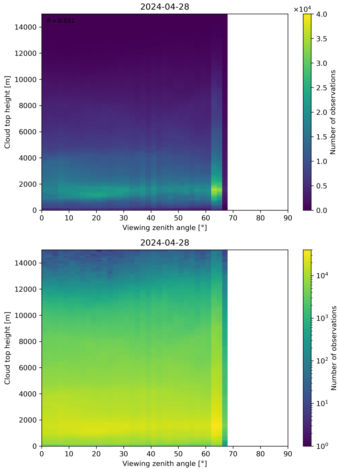
Figure 112: Scatter density plot of “Viewing zenith angle” against “Cloud top height” for 2024-04-27 to 2024-04-29.
