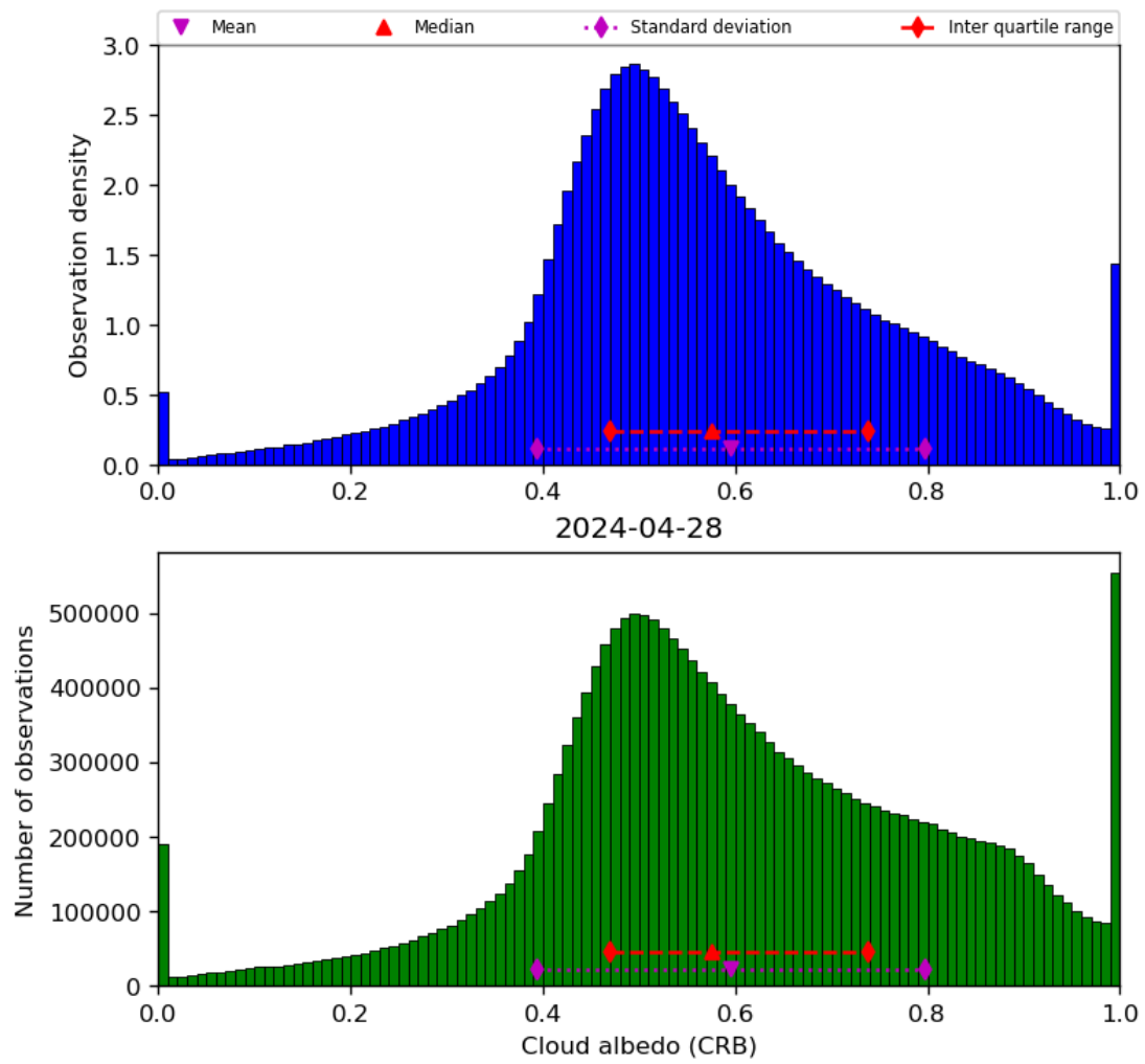
Figure 44: Histogram of “Cloud albedo (CRB)” for 2024-04-27 to 2024-04-29
