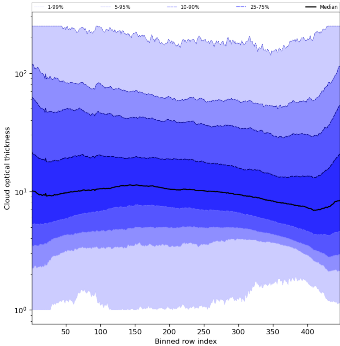
Figure 57: Along track statistics of “Cloud optical thickness” for 2024-04-27 to 2024-04-29
