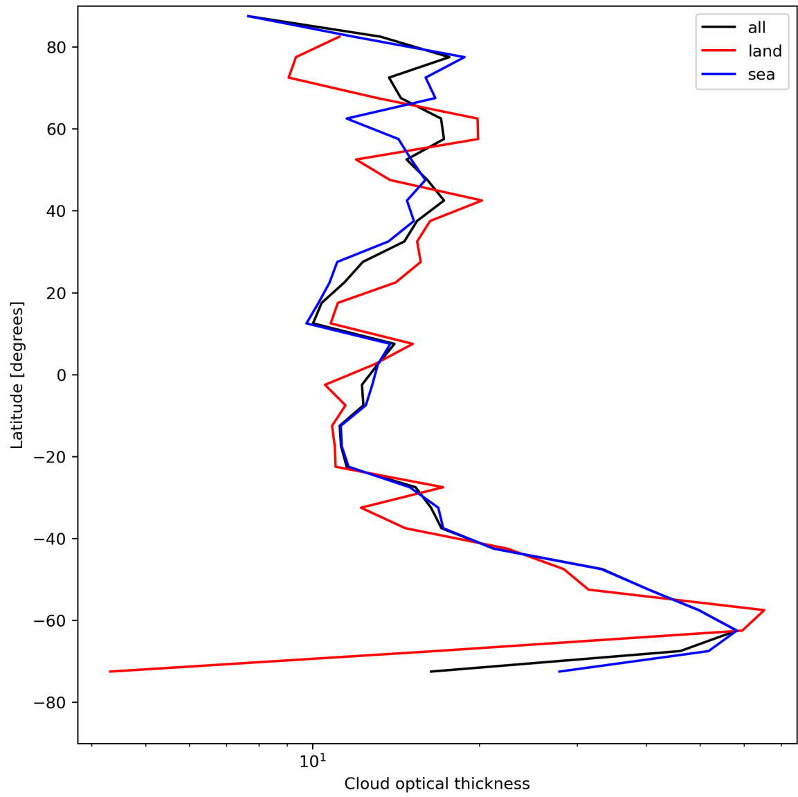
Figure 25: Zonal average of “Cloud optical thickness” for 2024-04-27 to 2024-04-29.
