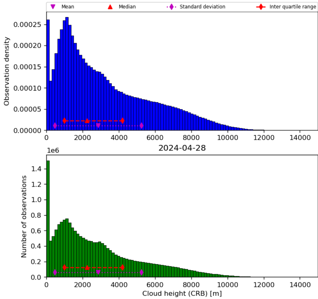
Figure 43: Histogram of “Cloud height (CRB)” for 2024-04-27 to 2024-04-29
