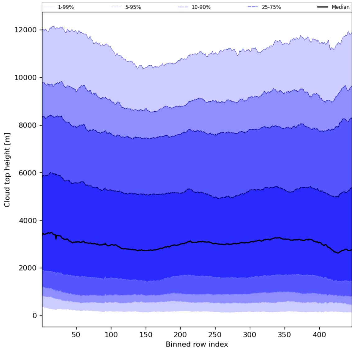
Figure 56: Along track statistics of “Cloud top height” for 2024-04-27 to 2024-04-29
