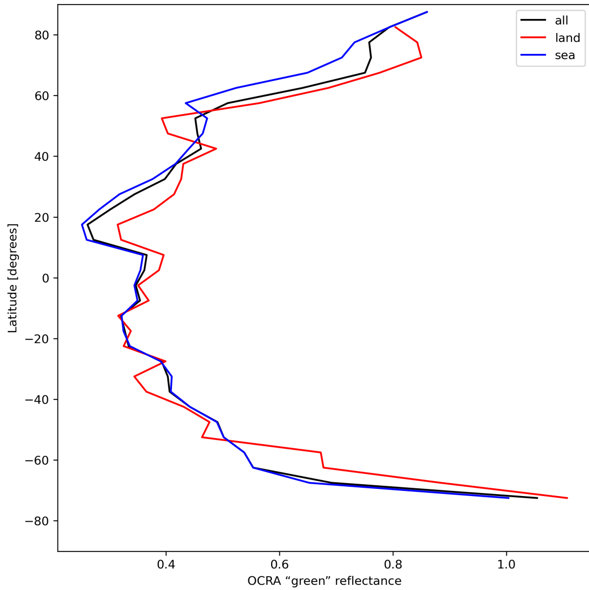
Figure 36: Zonal average of “OCRA “green” reflectance” for 2024-04-27 to 2024-04-29.
