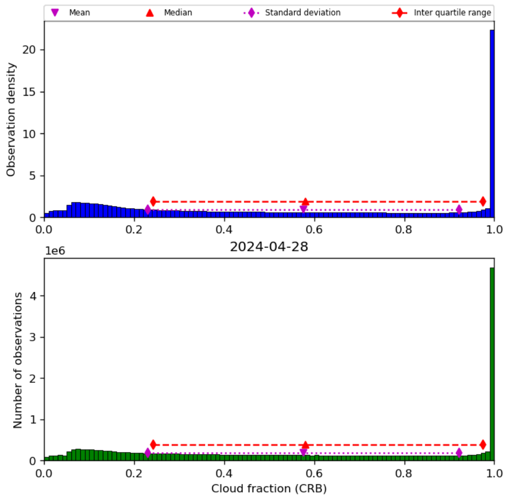
Figure 42: Histogram of “Cloud fraction (CRB)” for 2024-04-27 to 2024-04-29
