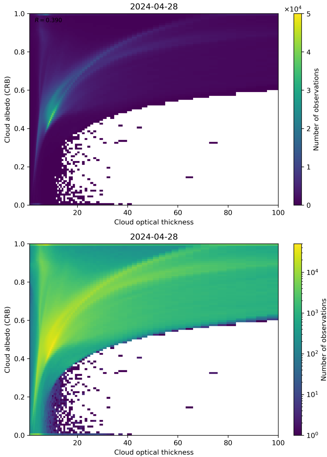
Figure 82: Scatter density plot of “Cloud optical thickness” against “Cloud albedo (CRB)” for 2024-04-27 to 2024-04-29.
