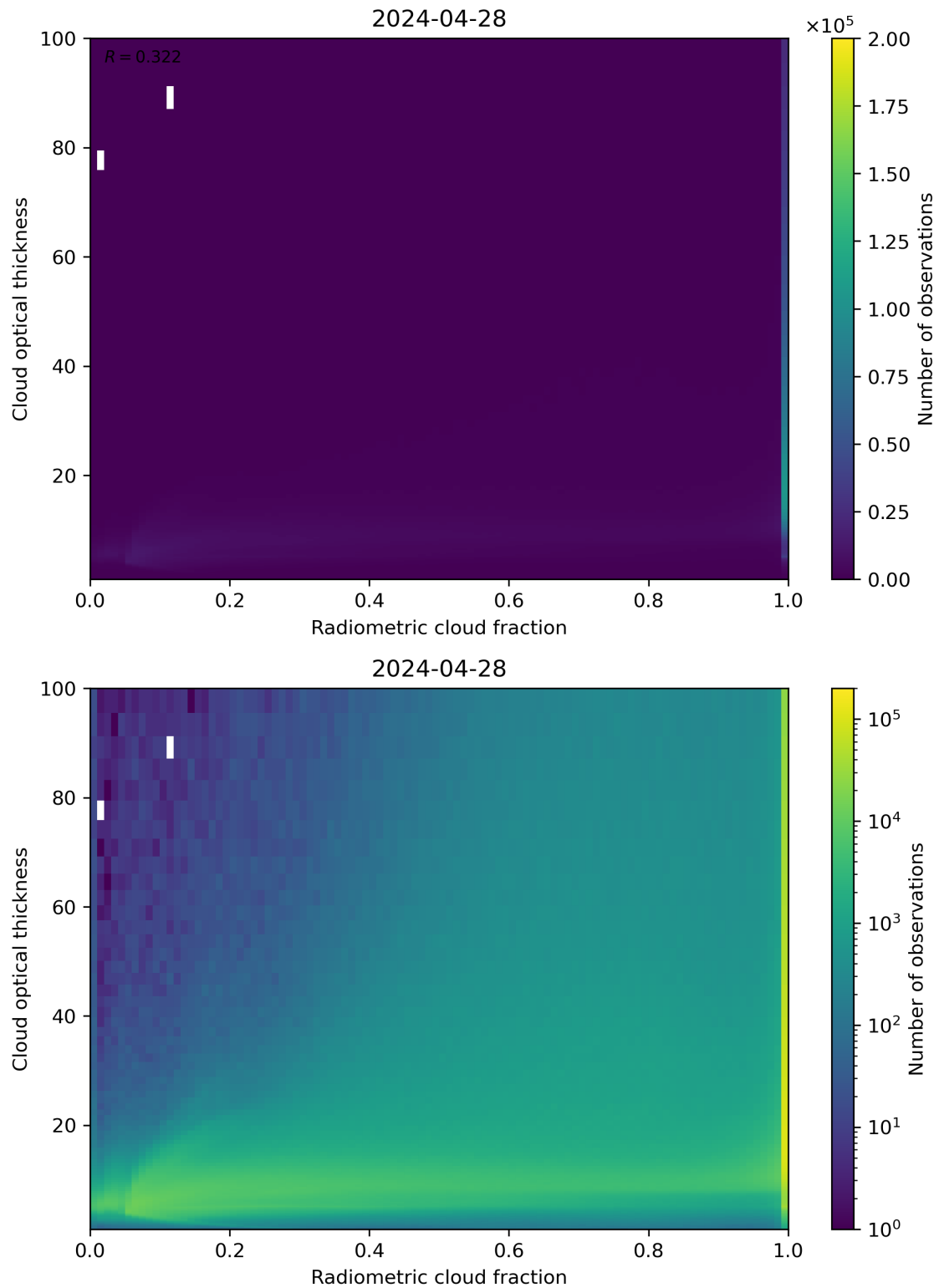
Figure 75: Scatter density plot of “Radiometric cloud fraction” against “Cloud optical thickness” for 2024-04-27 to 2024-04-29.
