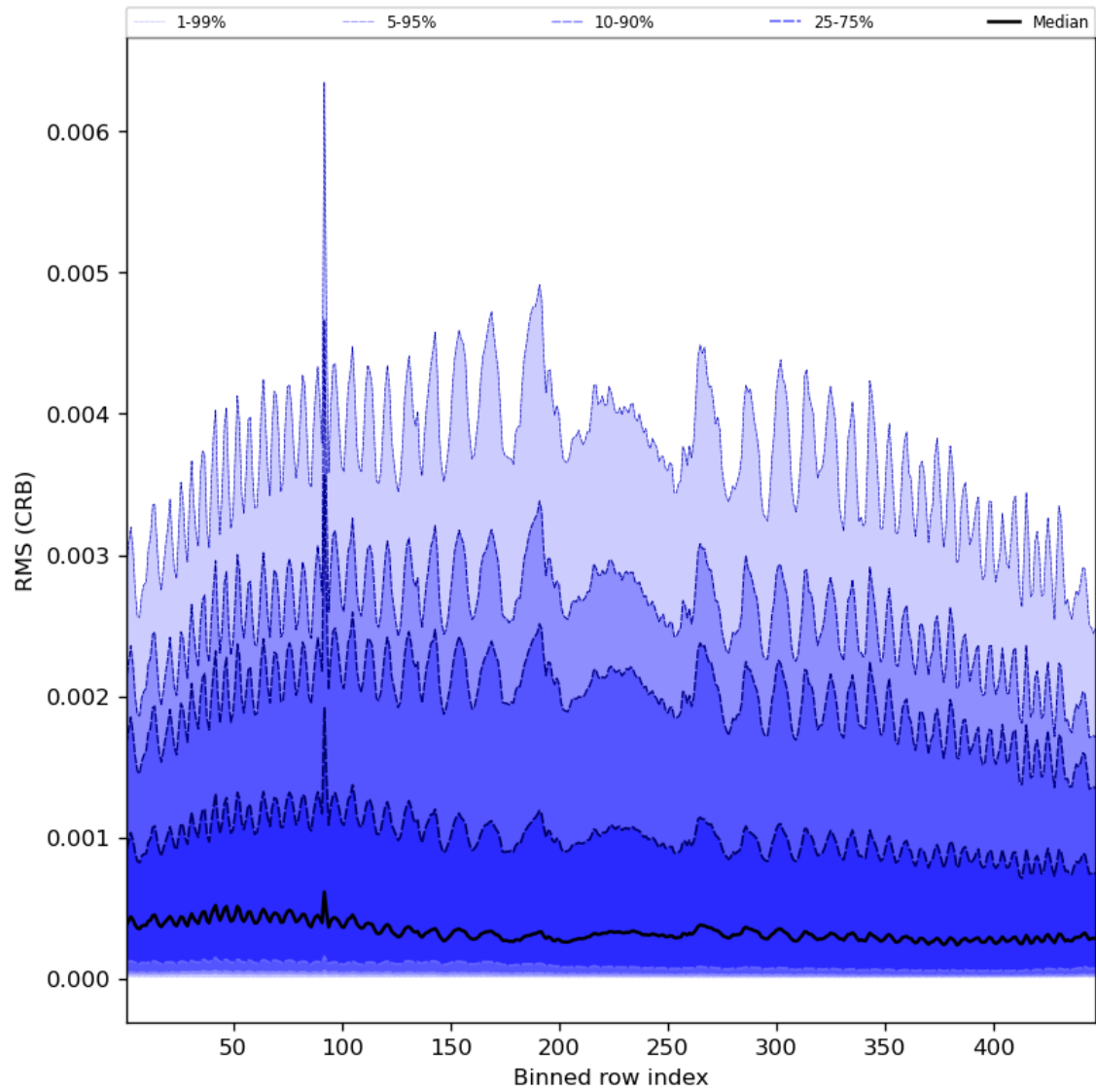
Figure 64: Along track statistics of “RMS (CRB)” for 2024-04-27 to 2024-04-29
