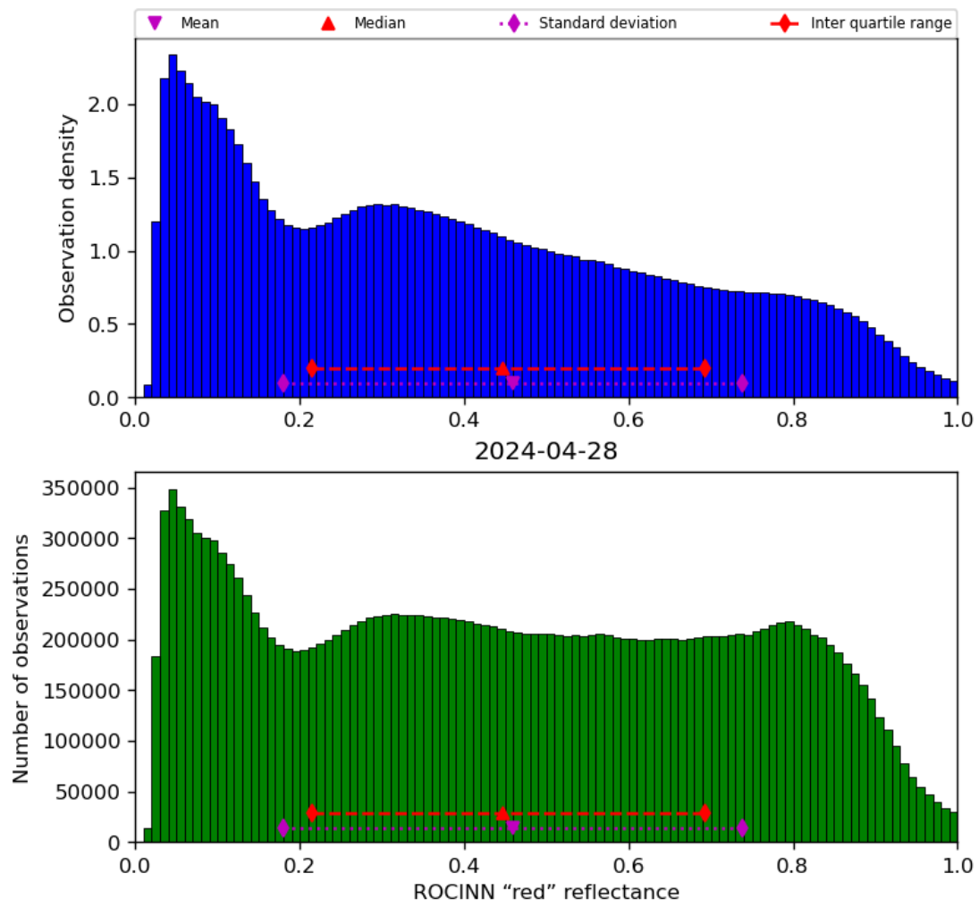
Figure 53: Histogram of “ROCINN “red” reflectance” for 2024-04-27 to 2024-04-29
