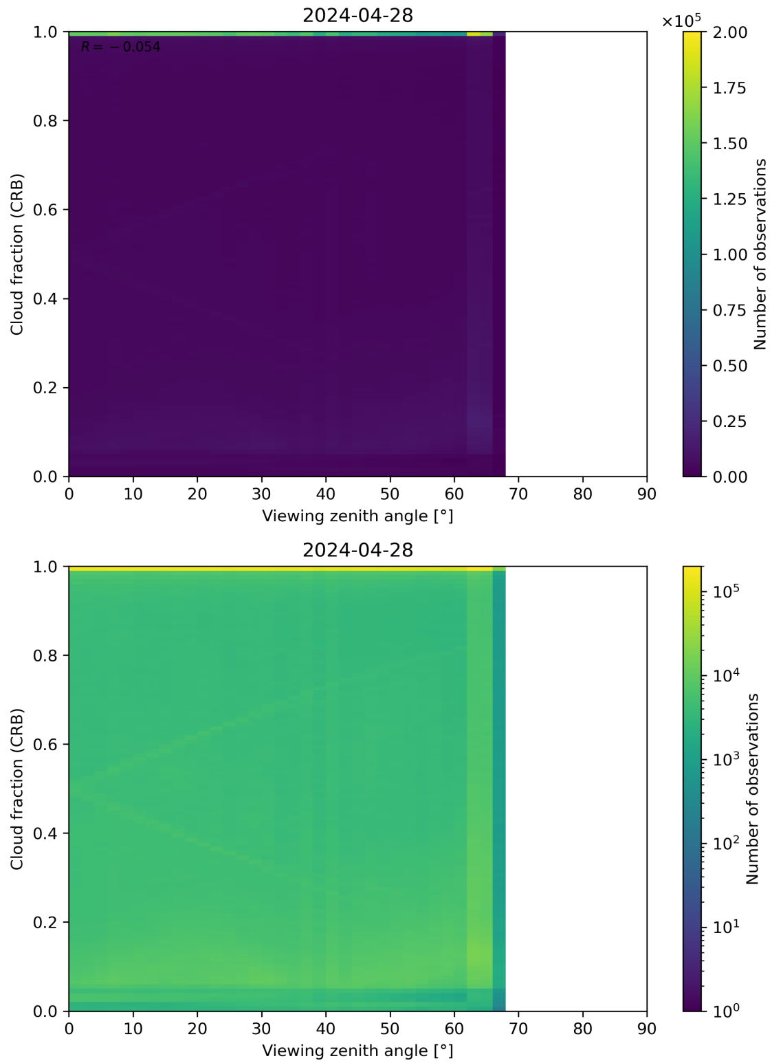
Figure 109: Scatter density plot of “Viewing zenith angle” against “Cloud fraction (CRB)” for 2024-04-27 to 2024-04-29.
