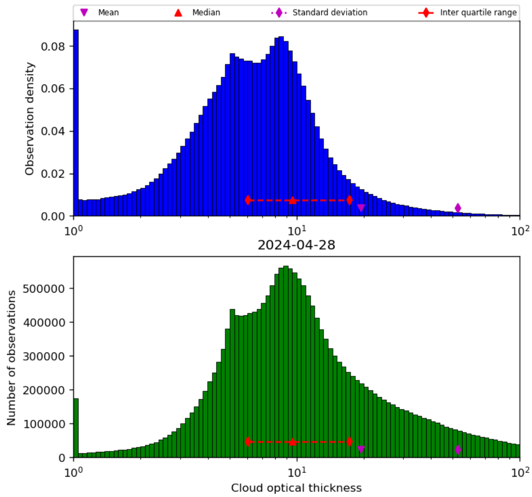
Figure 41: Histogram of “Cloud optical thickness” for 2024-04-27 to 2024-04-29
