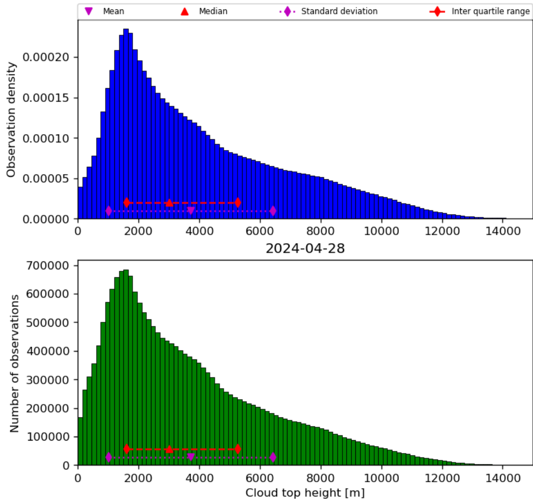
Figure 40: Histogram of “Cloud top height” for 2024-04-27 to 2024-04-29
