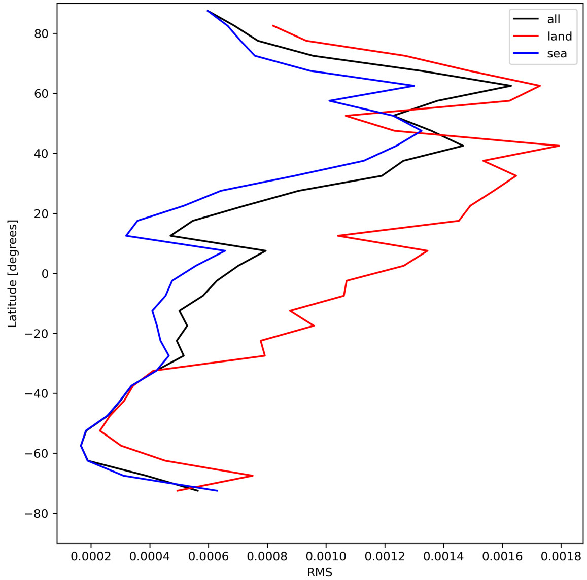
Figure 31: Zonal average of “RMS” for 2024-04-27 to 2024-04-29.
