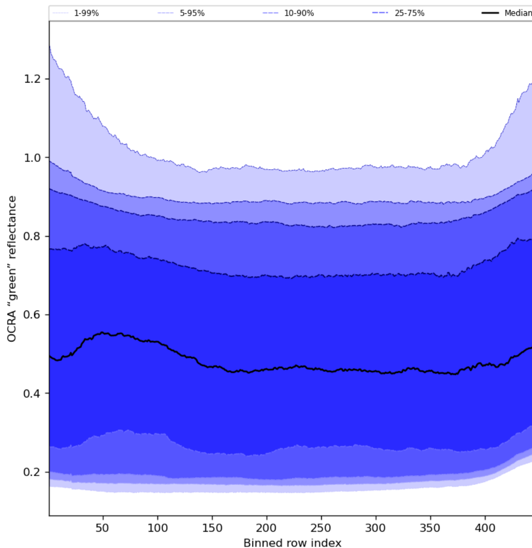
Figure 68: Along track statistics of "OCRA "green" reflectance" for 2024-04-27 to 2024-04-29
