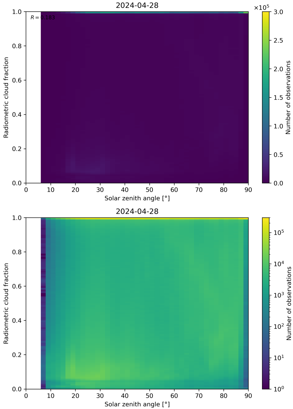
Figure 99: Scatter density plot of “Solar zenith angle” against “Radiometric cloud fraction” for 2024-04-27 to 2024-04-29.
