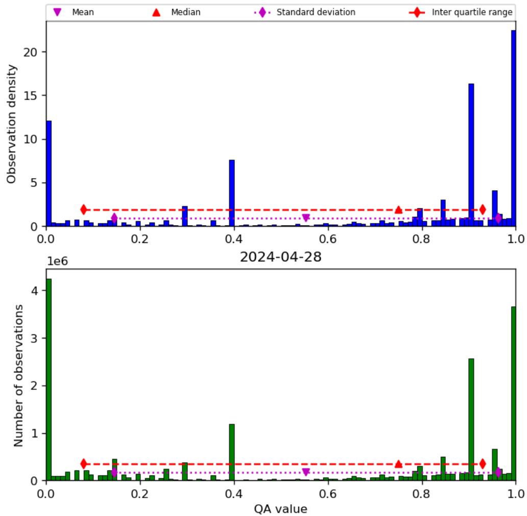
Figure 38: Histogram of “QA value” for 2024-04-27 to 2024-04-29
