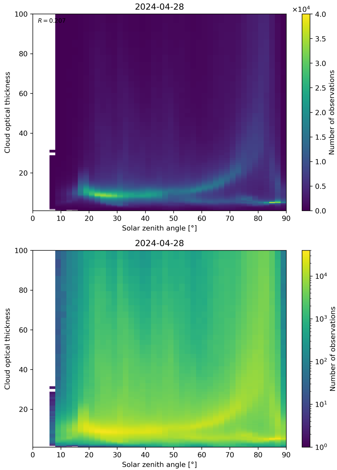
Figure 103: Scatter density plot of “Solar zenith angle” against “Cloud optical thickness” for 2024-04-27 to 2024-04-29.
