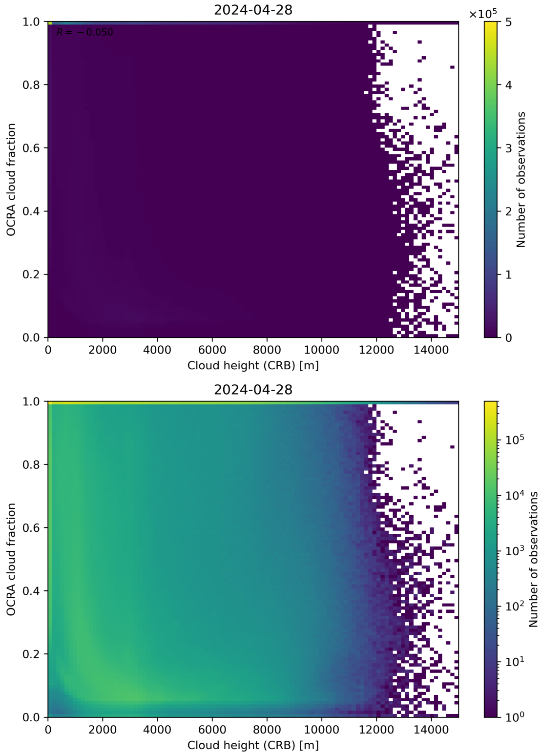
Figure 81: Scatter density plot of “Cloud height (CRB)” against “OCRA cloud fraction” for 2024-04-27 to 2024-04-29.
