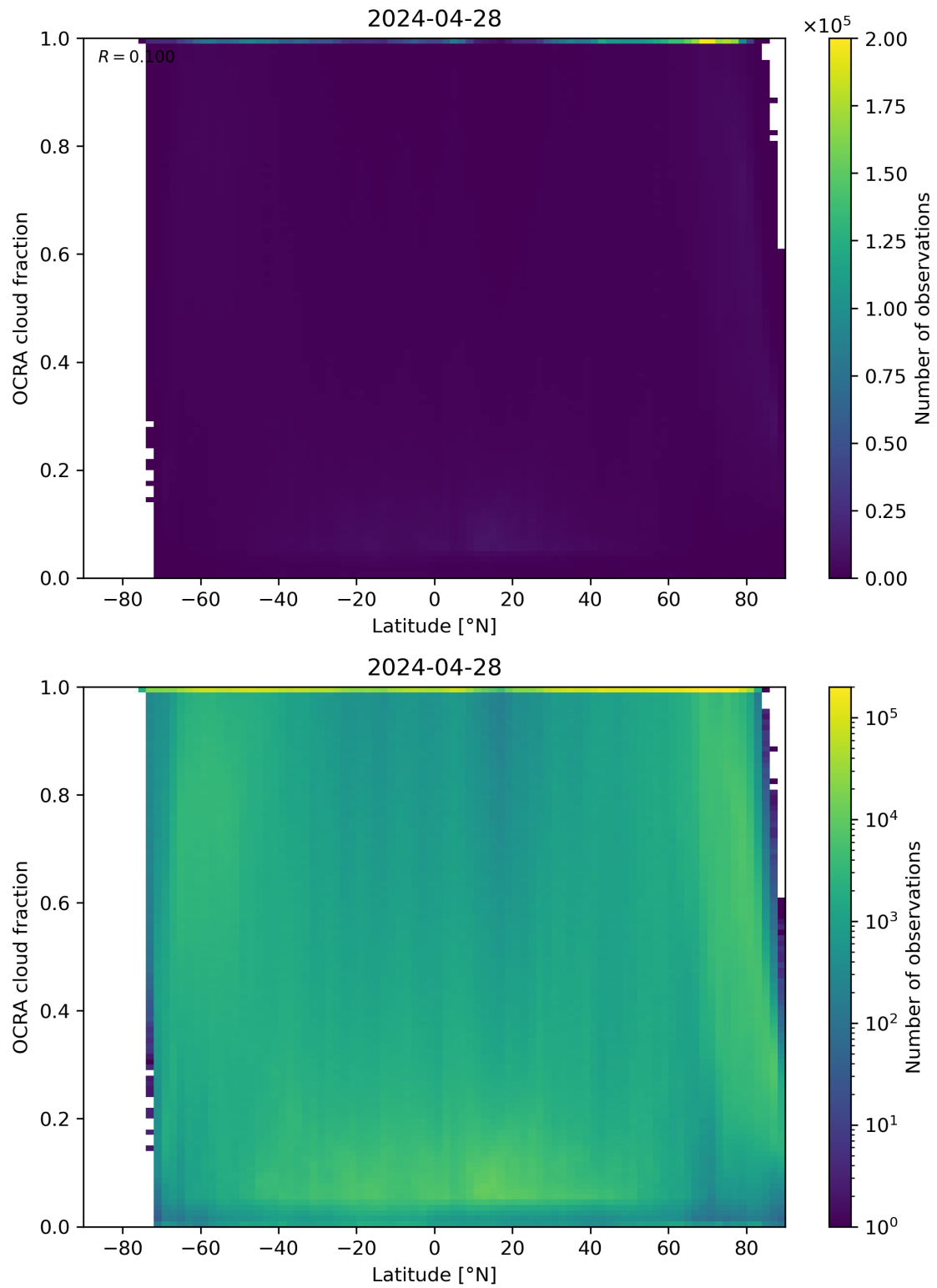
Figure 93: Scatter density plot of “Latitude” against “OCRA cloud fraction” for 2024-04-27 to 2024-04-29.
