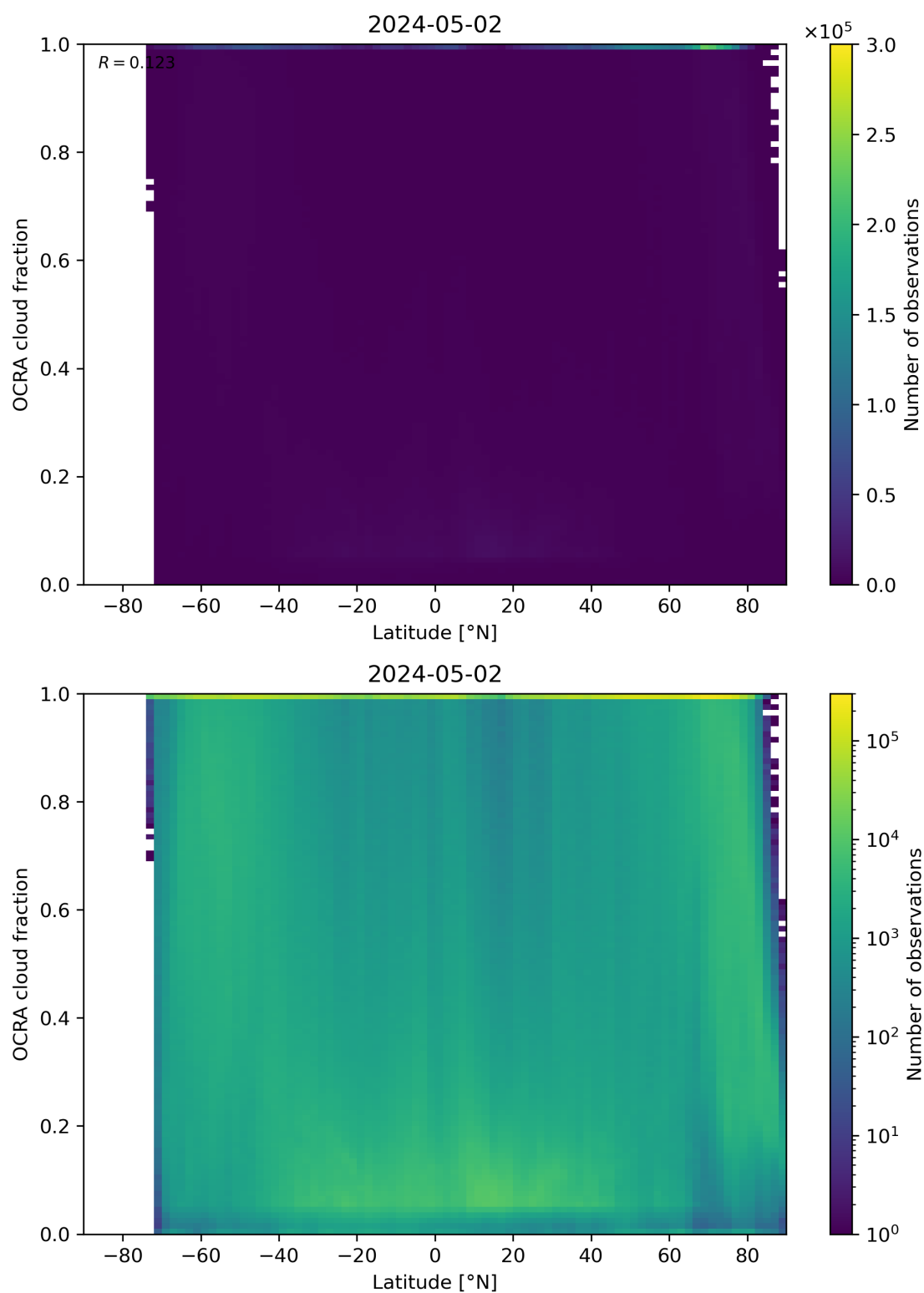
Figure 93: Scatter density plot of “Latitude” against “OCRA cloud fraction” for 2024-05-02 to 2024-05-03.
