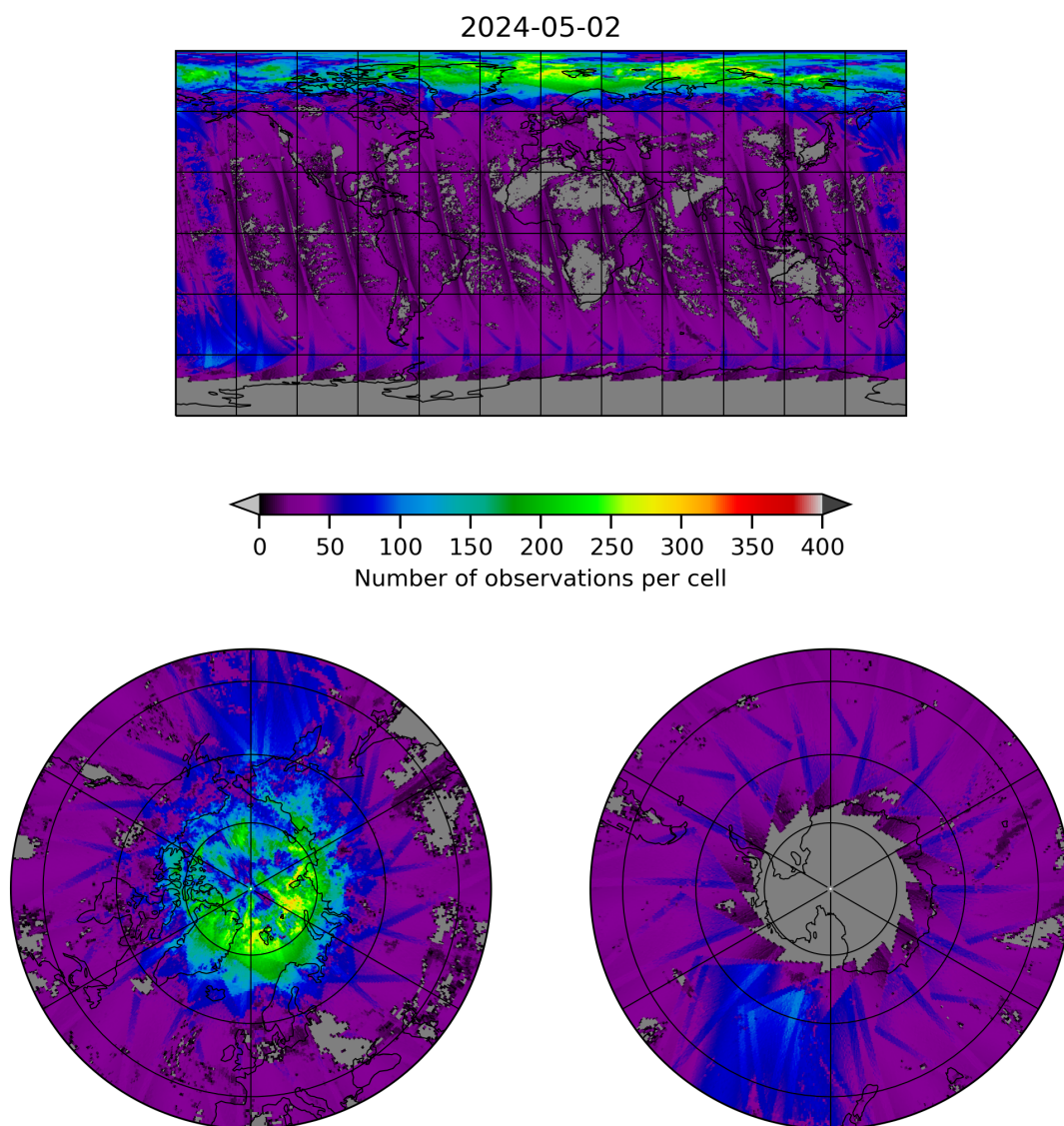
Figure 21: Map of the number of observations for 2024-05-02 to 2024-05-03
