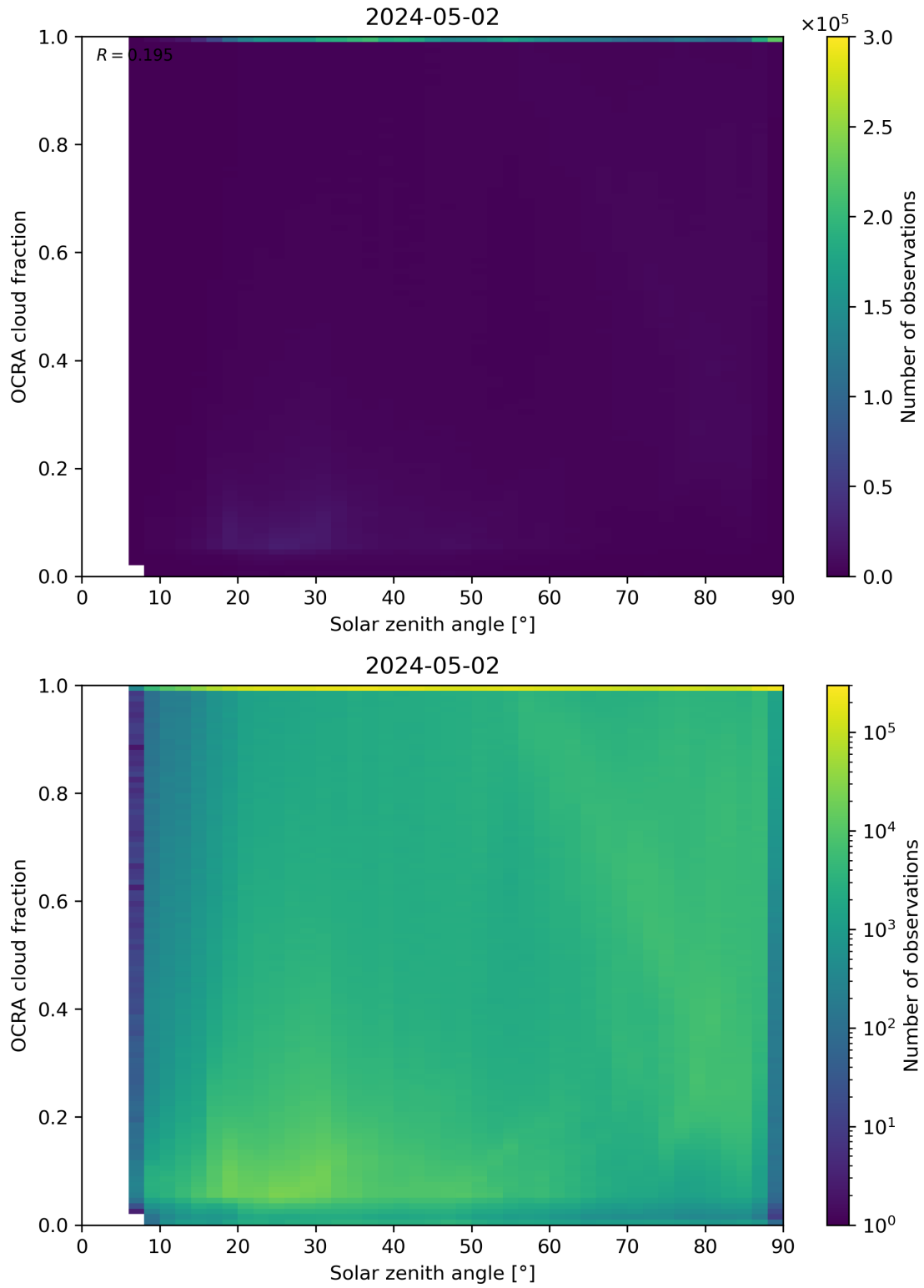
Figure 100: Scatter density plot of “Solar zenith angle” against “OCRA cloud fraction” for 2024-05-02 to 2024-05-03.
