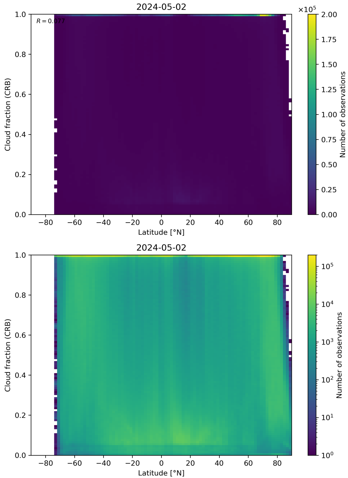
Figure 94: Scatter density plot of “Latitude” against “Cloud fraction (CRB)” for 2024-05-02 to 2024-05-03.
