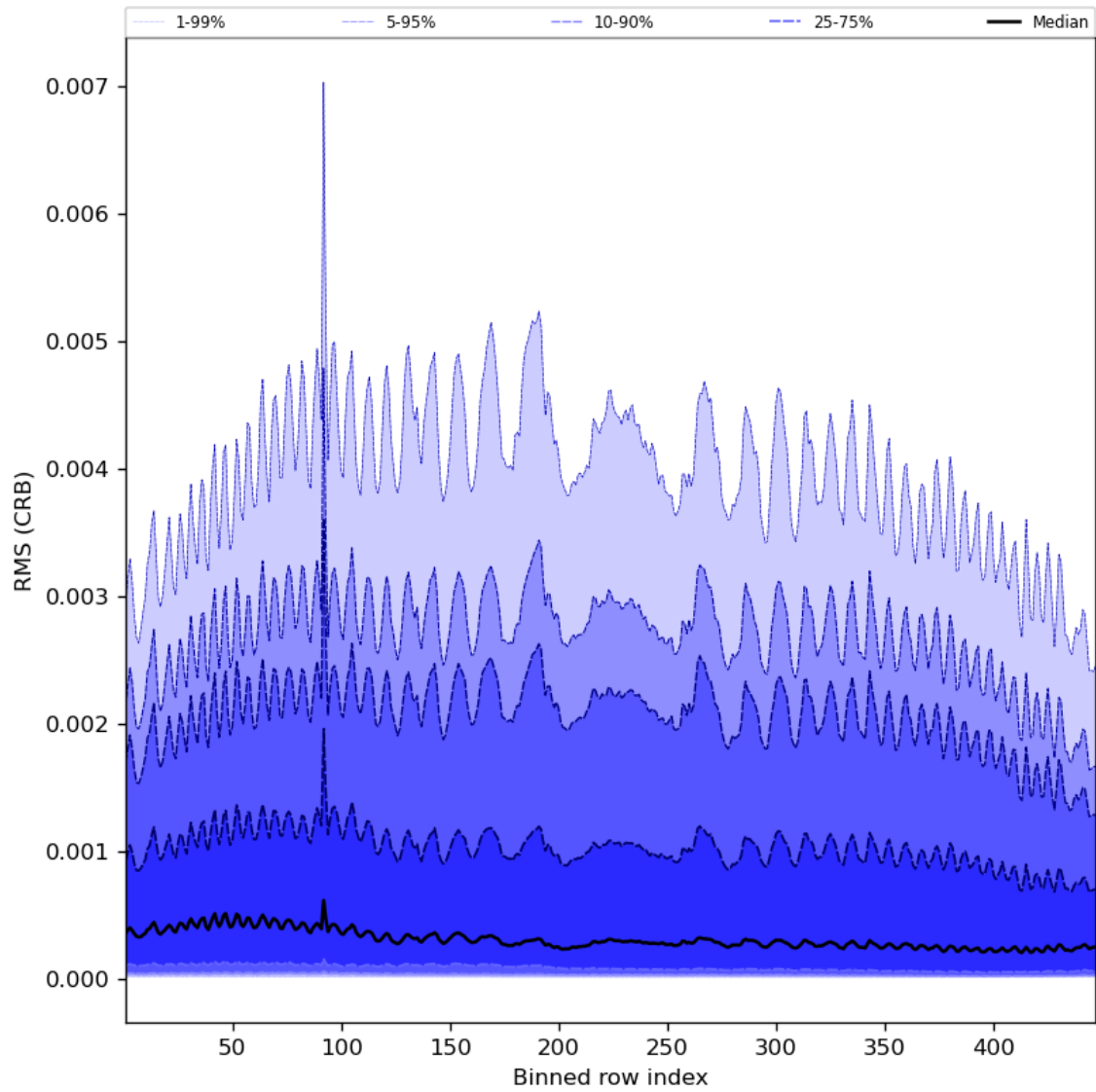
Figure 64: Along track statistics of “RMS (CRB)” for 2024-05-02 to 2024-05-03
