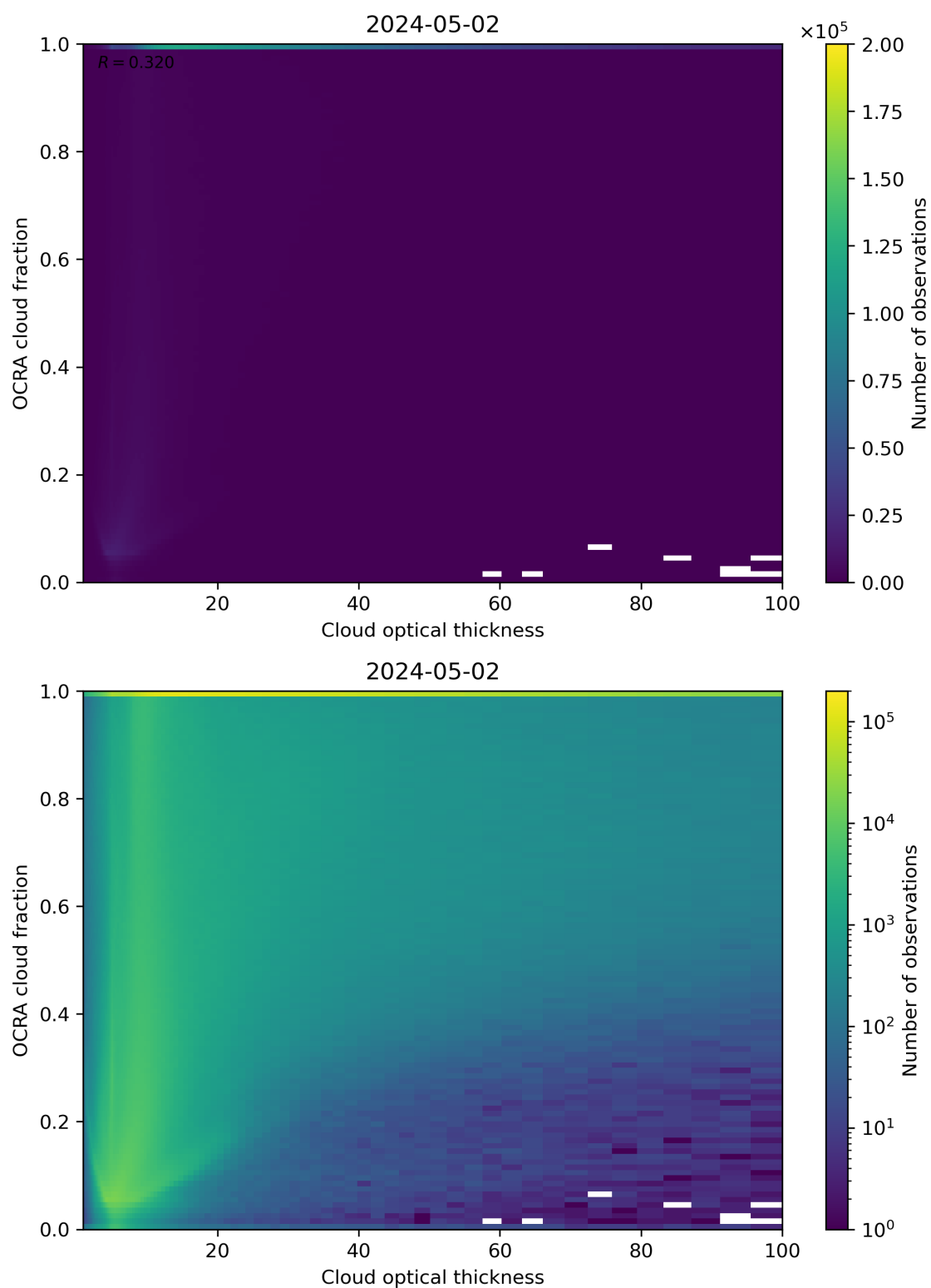
Figure 83: Scatter density plot of “Cloud optical thickness” against “OCRA cloud fraction” for 2024-05-02 to 2024-05-03.
