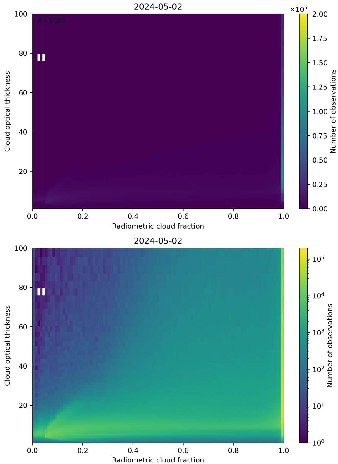
Figure 75: Scatter density plot of “Radiometric cloud fraction” against “Cloud optical thickness” for 2024-05-02 to 2024-05-03.
