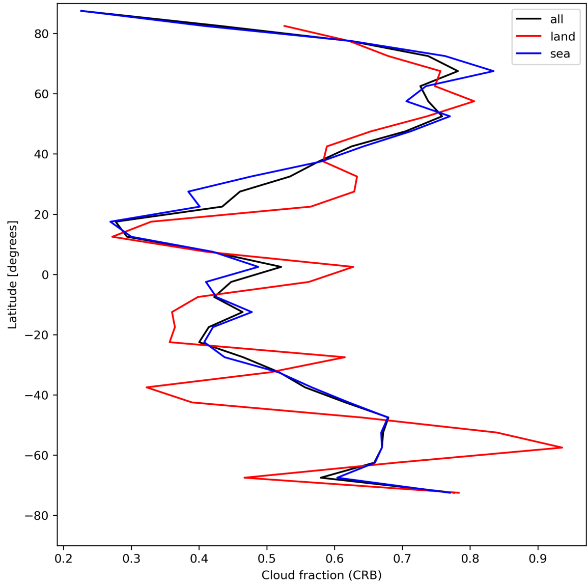
Figure 26: Zonal average of “Cloud fraction (CRB)” for 2024-05-02 to 2024-05-03.
