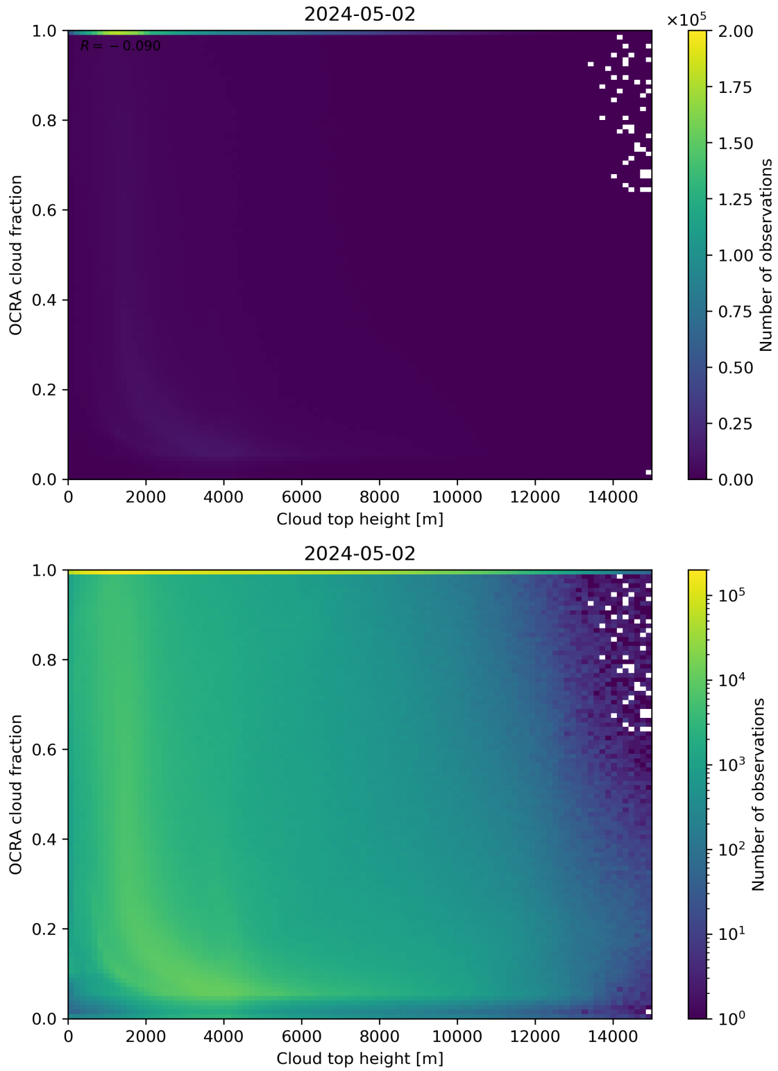
Figure 87: Scatter density plot of “Cloud top height” against “OCRA cloud fraction” for 2024-05-02 to 2024-05-03.
