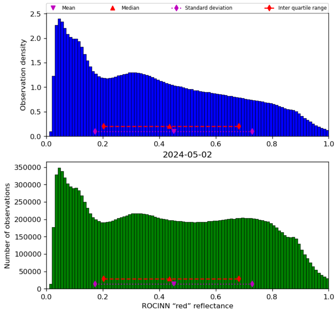
Figure 53: Histogram of “ROCINN “red” reflectance” for 2024-05-02 to 2024-05-03
