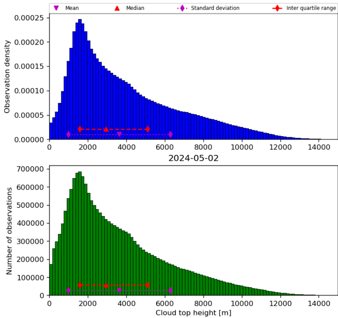
Figure 40: Histogram of “Cloud top height” for 2024-05-02 to 2024-05-03
