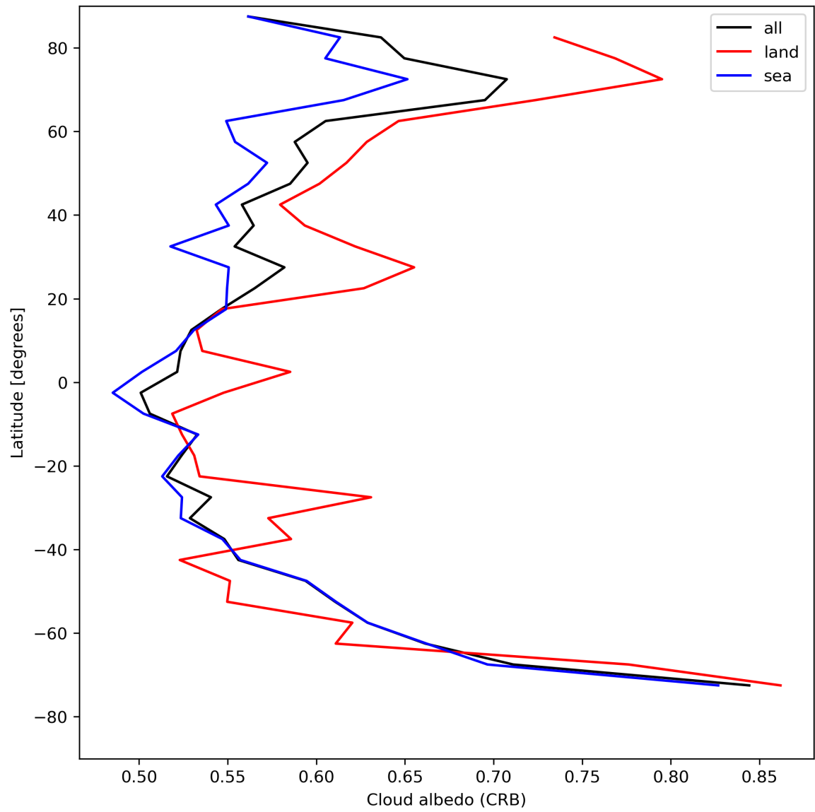
Figure 28: Zonal average of “Cloud albedo (CRB)” for 2024-05-02 to 2024-05-03.
