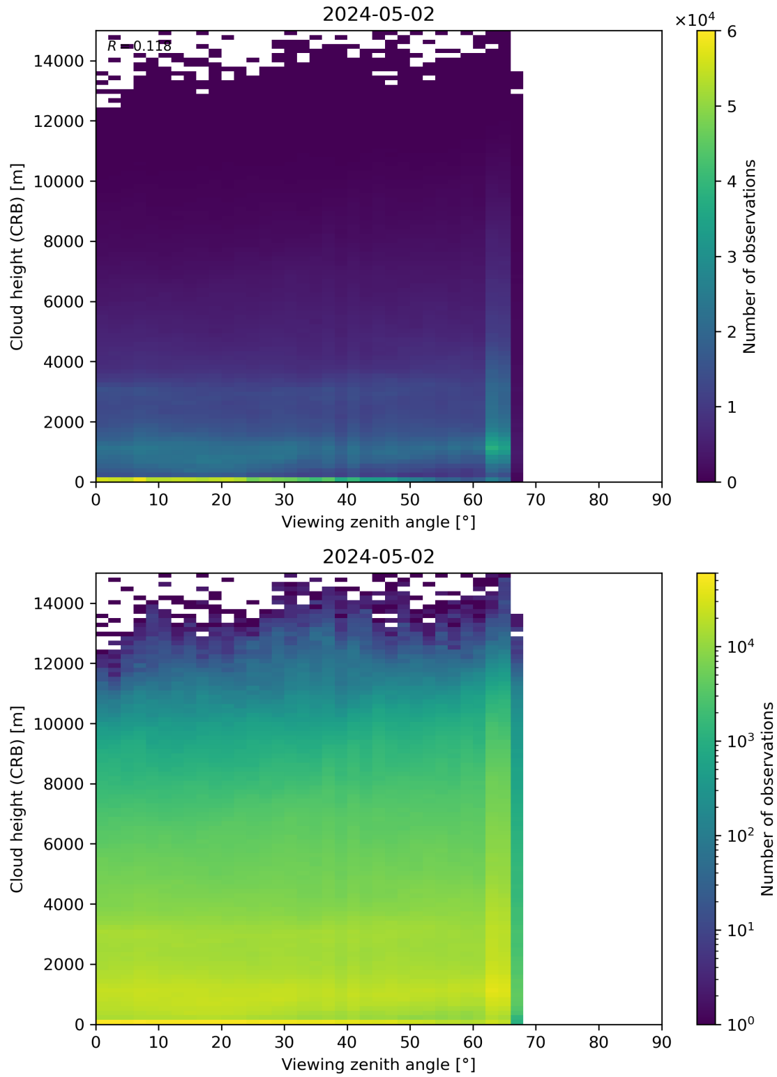
Figure 110: Scatter density plot of “Viewing zenith angle” against “Cloud height (CRB)” for 2024-05-02 to 2024-05-03.
