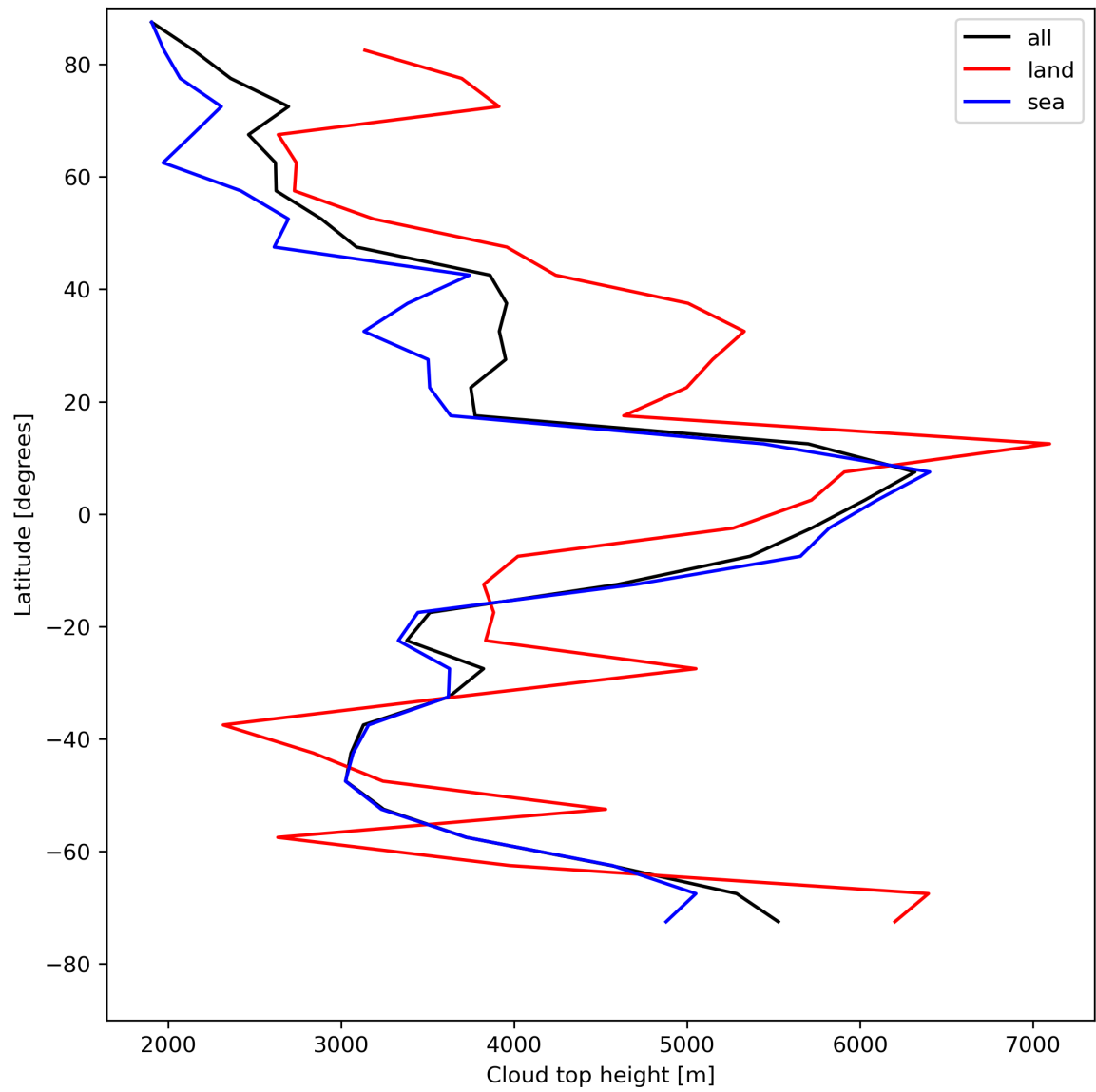
Figure 24: Zonal average of “Cloud top height” for 2024-05-02 to 2024-05-03.
