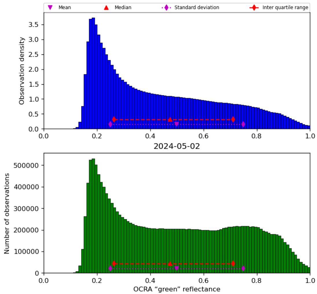
Figure 52: Histogram of “OCRA “green” reflectance” for 2024-05-02 to 2024-05-03
