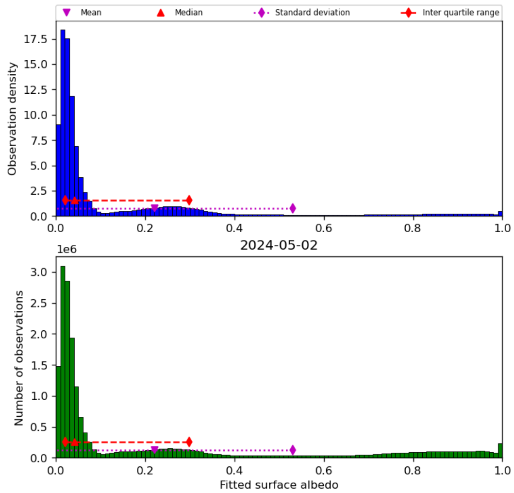
Figure 45: Histogram of “Fitted surface albedo” for 2024-05-02 to 2024-05-03
