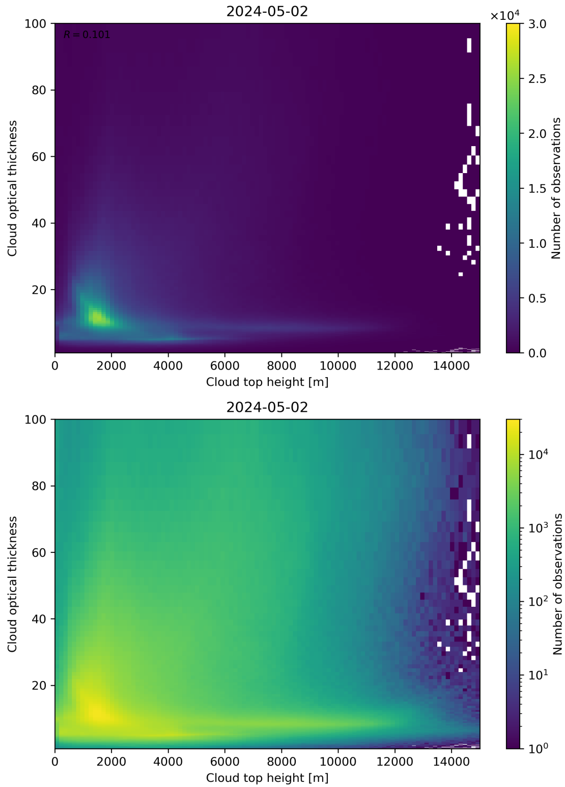
Figure 90: Scatter density plot of “Cloud top height” against “Cloud optical thickness” for 2024-05-02 to 2024-05-03.
