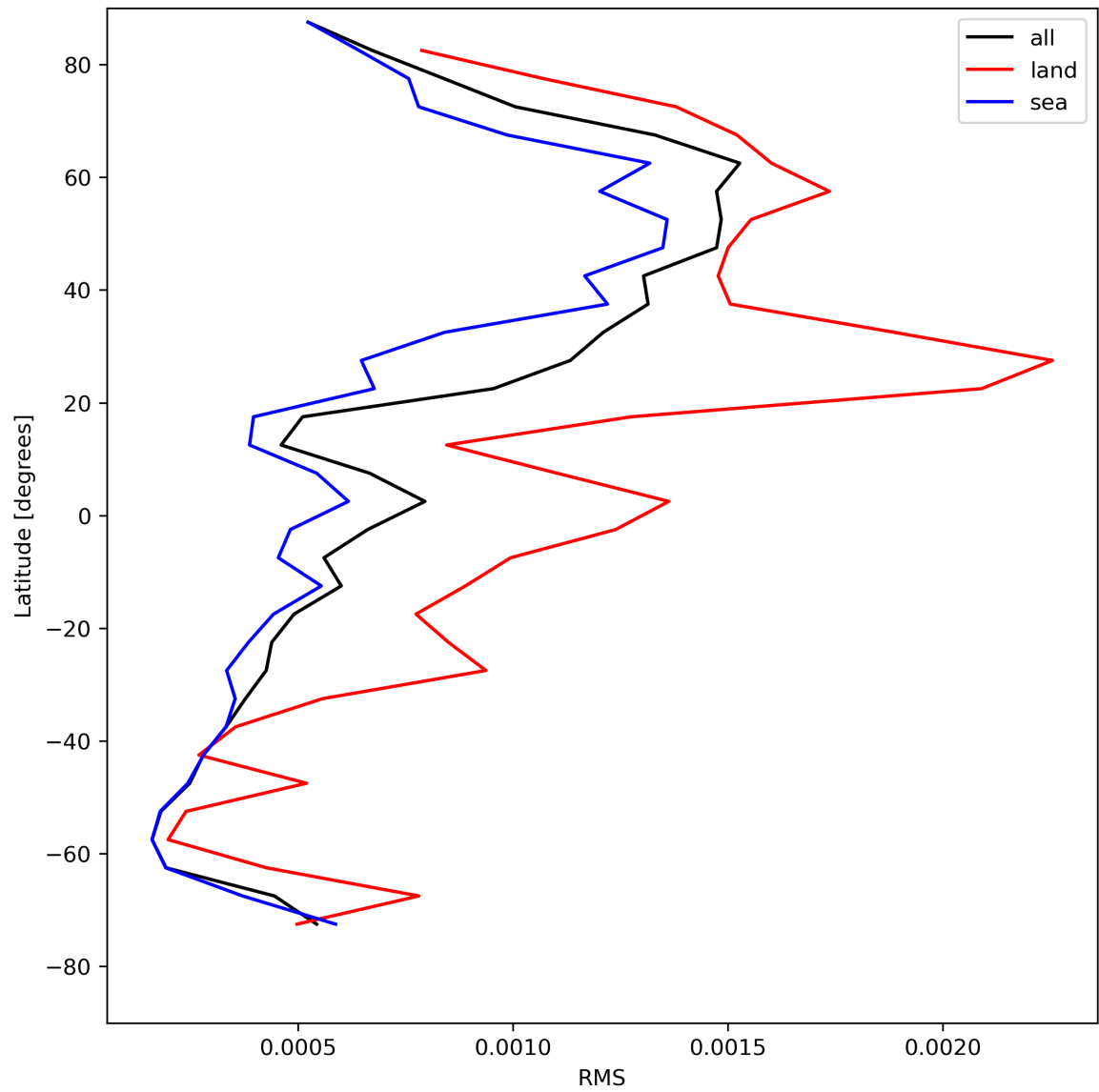
Figure 31: Zonal average of “RMS” for 2024-05-02 to 2024-05-03.
