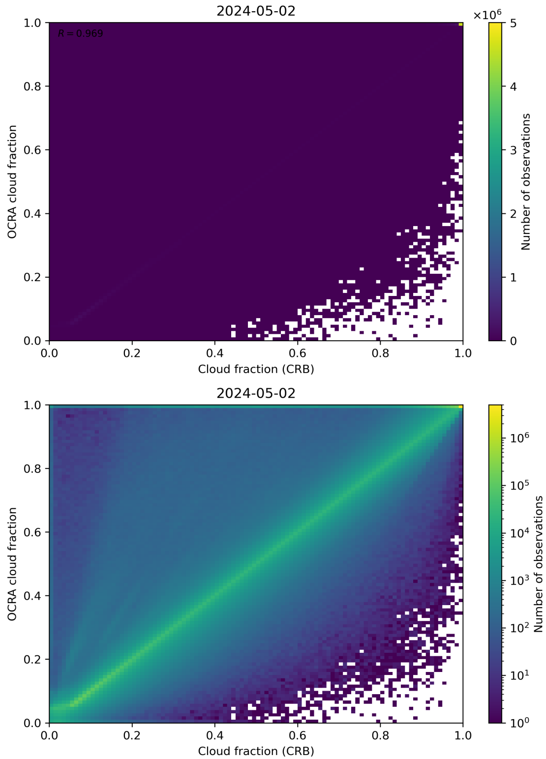
Figure 78: Scatter density plot of “Cloud fraction (CRB)” against “OCRA cloud fraction” for 2024-05-02 to 2024-05-03.
