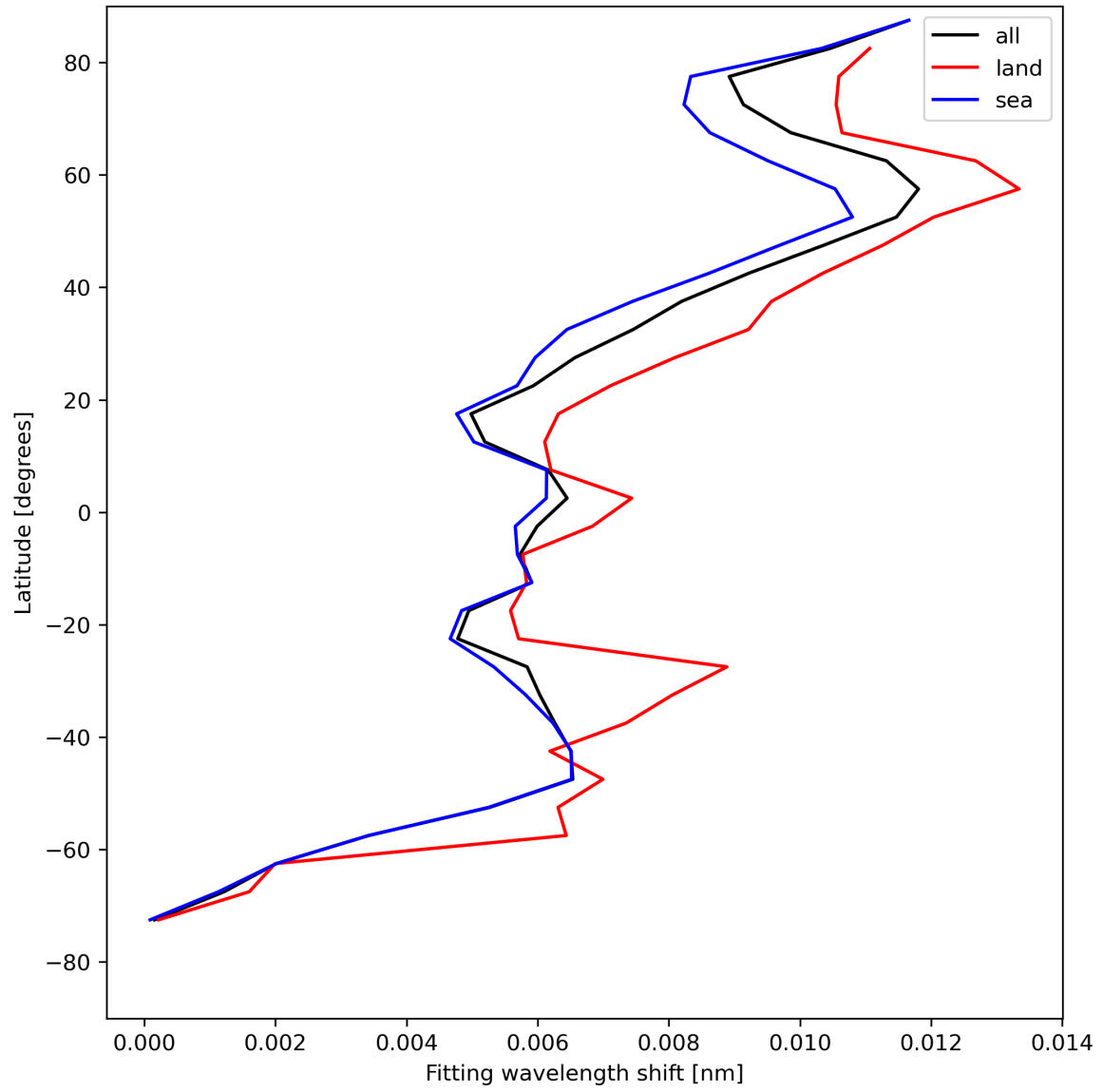
Figure 33: Zonal average of “Fitting wavelength shift” for 2024-05-02 to 2024-05-03.
