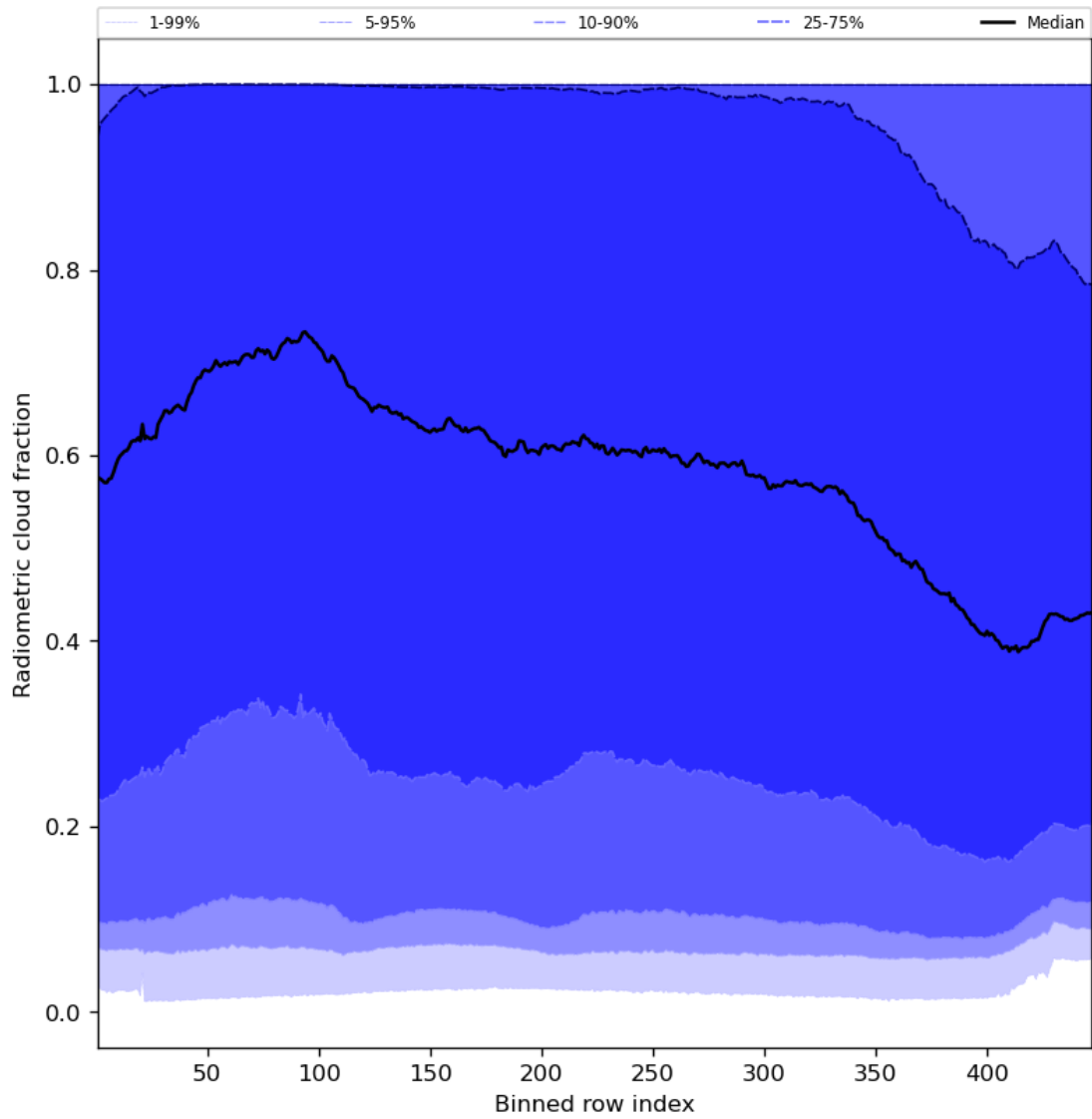
Figure 55: Along track statistics of “Radiometric cloud fraction” for 2024-05-02 to 2024-05-03
