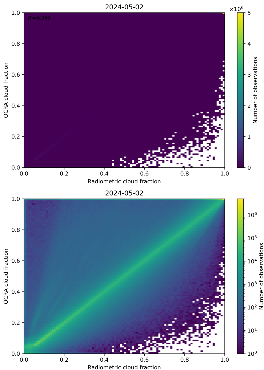
Figure 72: Scatter density plot of “Radiometric cloud fraction” against “OCRA cloud fraction” for 2024-05-02 to 2024-05-03.
