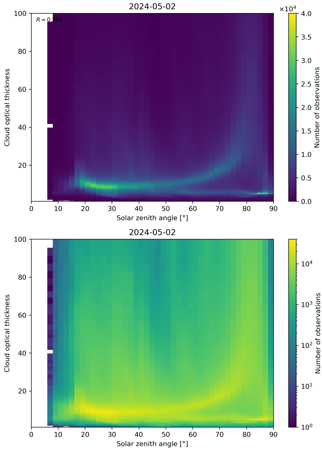
Figure 103: Scatter density plot of “Solar zenith angle” against “Cloud optical thickness” for 2024-05-02 to 2024-05-03.
