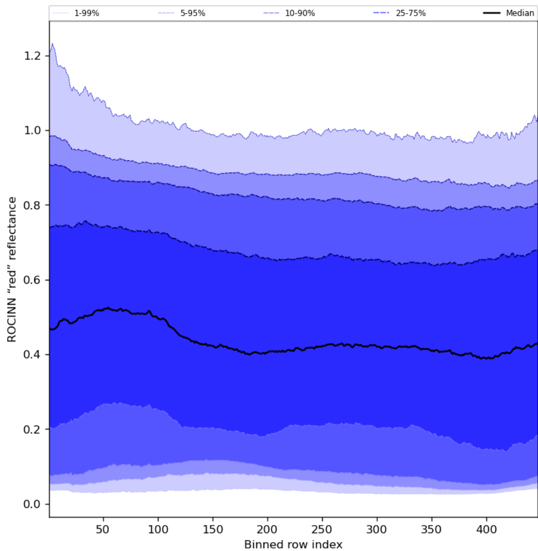
Figure 69: Along track statistics of “ROCINN “red” reflectance” for 2024-05-02 to 2024-05-03
