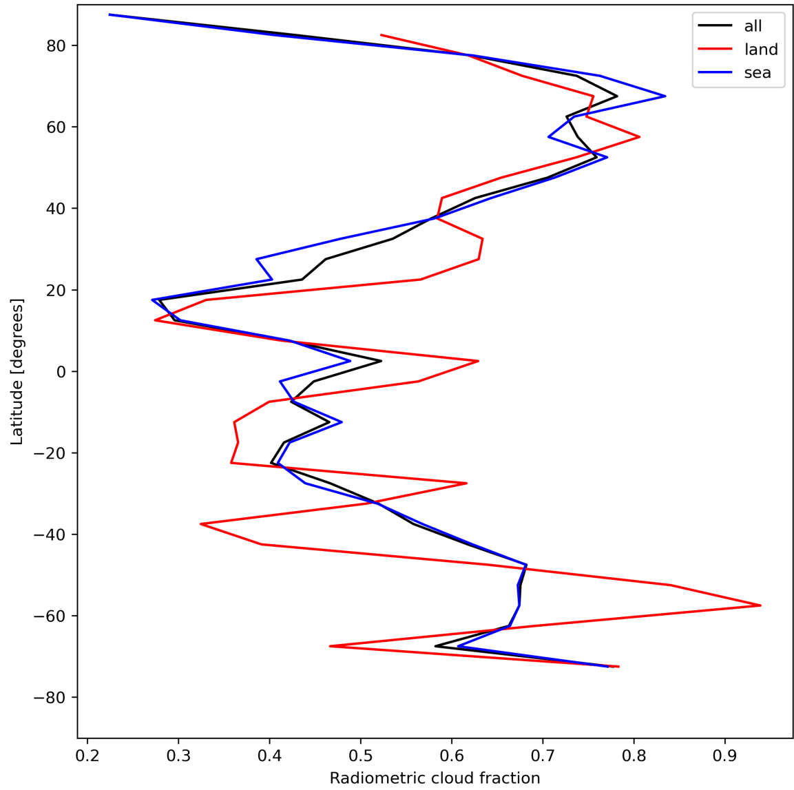
Figure 23: Zonal average of “Radiometric cloud fraction” for 2024-05-02 to 2024-05-03.
