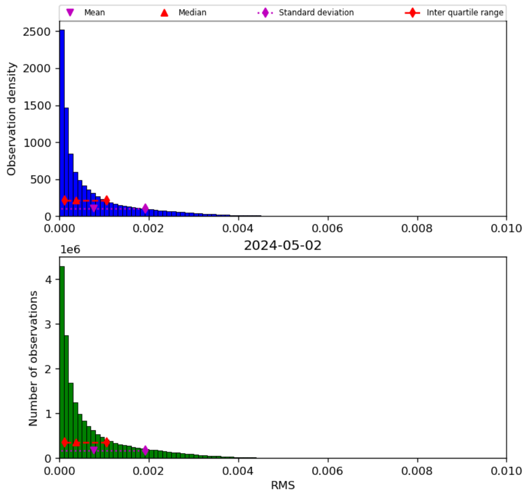
Figure 47: Histogram of “RMS” for 2024-05-02 to 2024-05-03
