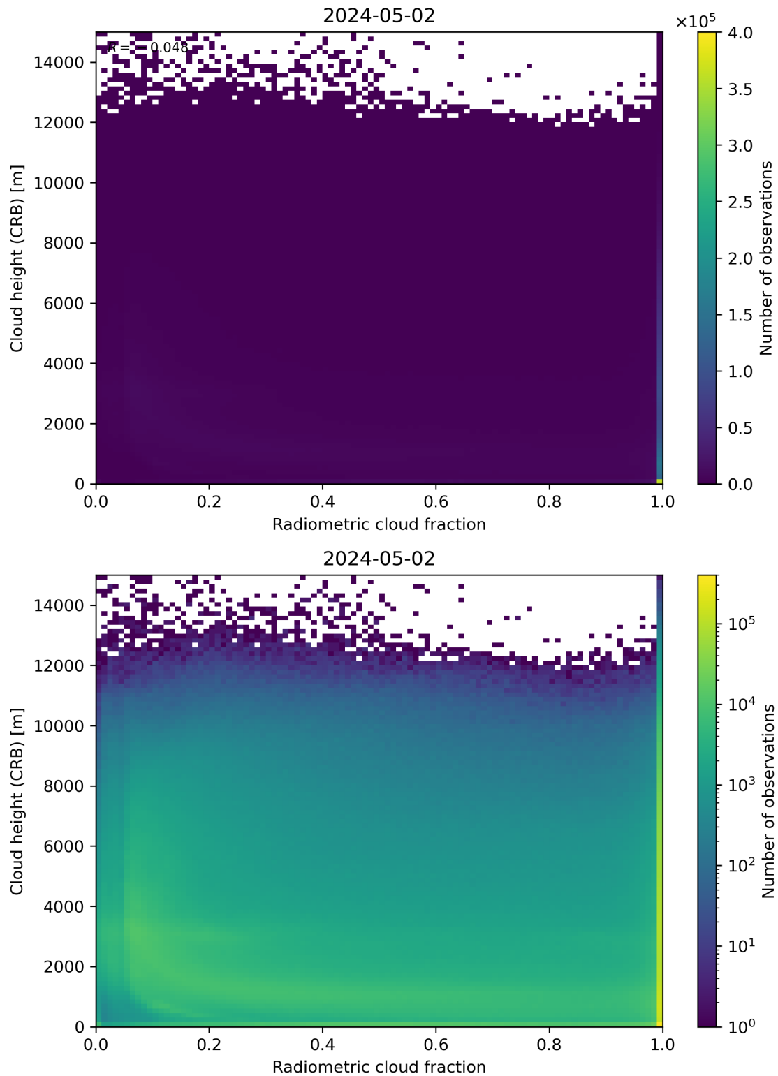
Figure 74: Scatter density plot of “Radiometric cloud fraction” against “Cloud height (CRB)” for 2024-05-02 to 2024-05-03.
