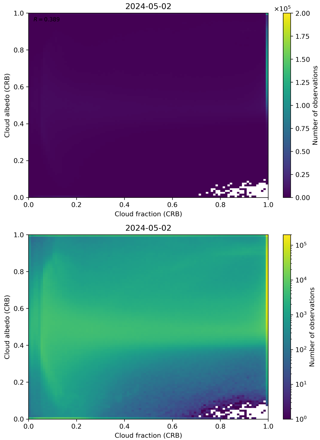
Figure 77: Scatter density plot of “Cloud fraction (CRB)” against “Cloud albedo (CRB)” for 2024-05-02 to 2024-05-03.
