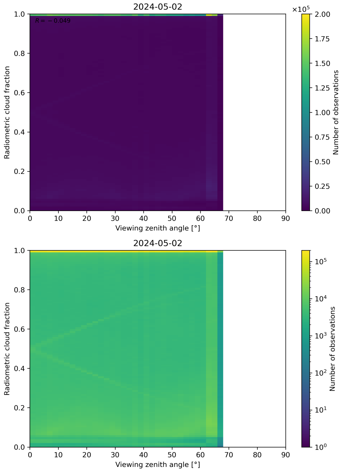
Figure 107: Scatter density plot of “Viewing zenith angle” against “Radiometric cloud fraction” for 2024-05-02 to 2024-05-03.
