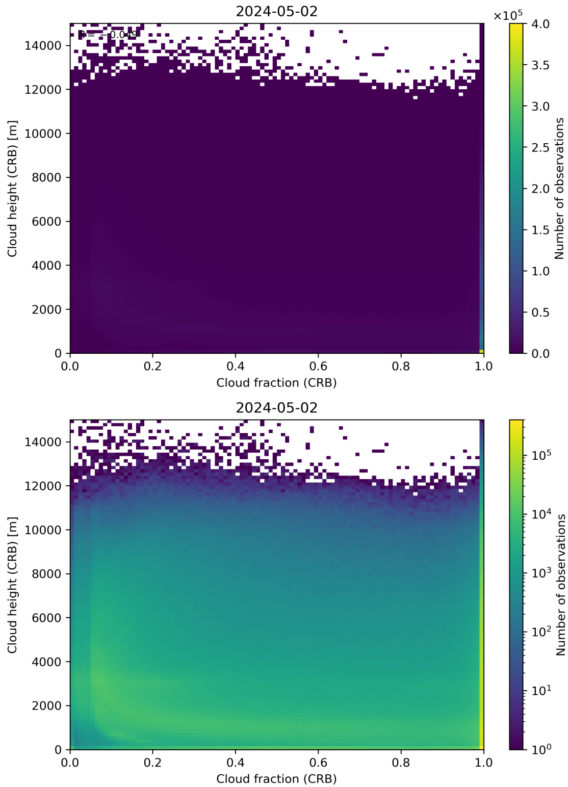
Figure 79: Scatter density plot of “Cloud fraction (CRB)” against “Cloud height (CRB)” for 2024-05-02 to 2024-05-03.
