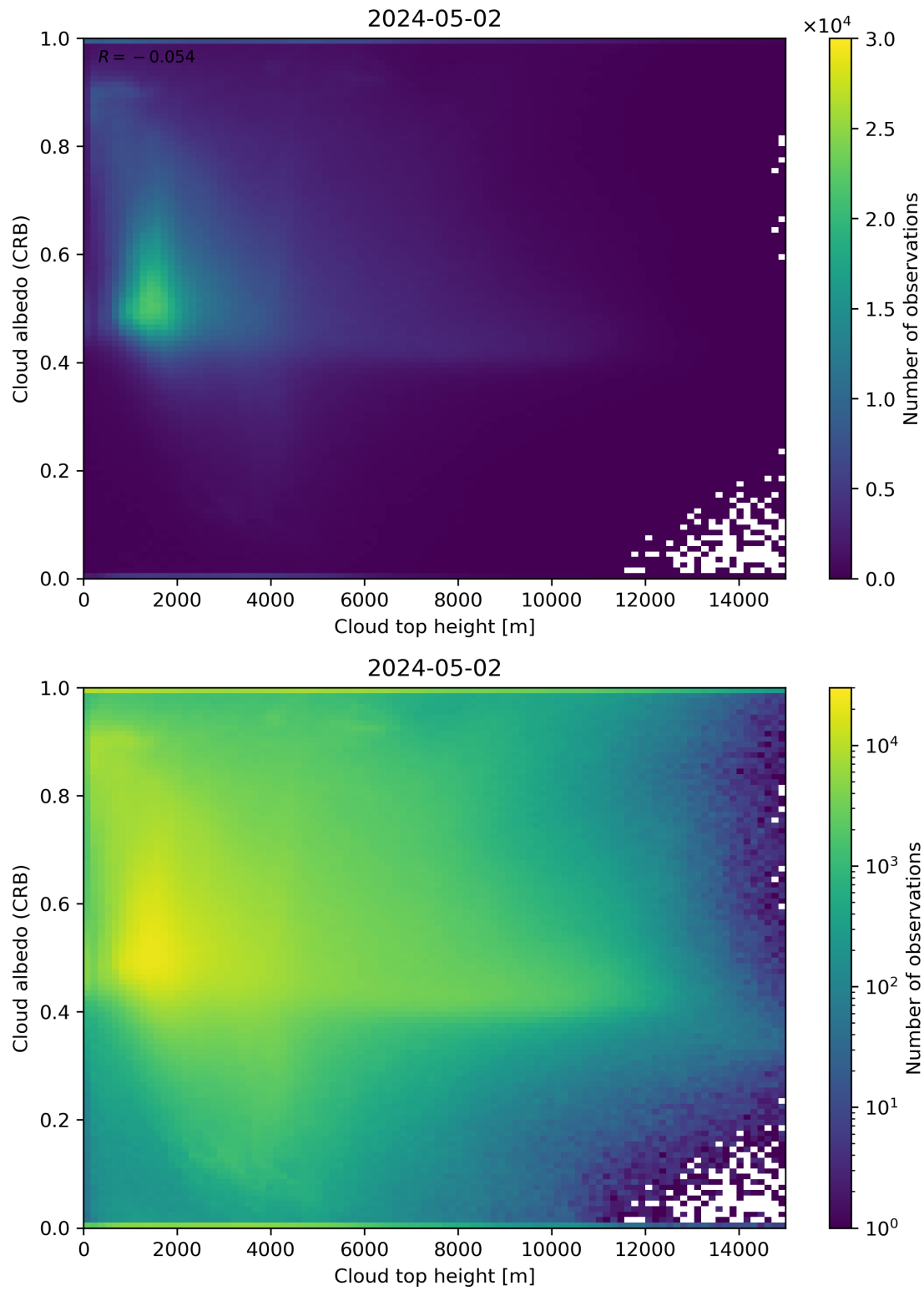
Figure 86: Scatter density plot of “Cloud top height” against “Cloud albedo (CRB)” for 2024-05-02 to 2024-05-03.
