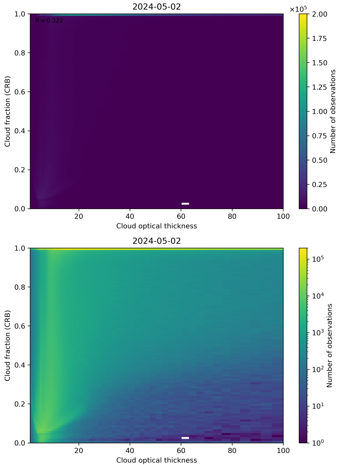
Figure 84: Scatter density plot of “Cloud optical thickness” against “Cloud fraction (CRB)” for 2024-05-02 to 2024-05-03.
