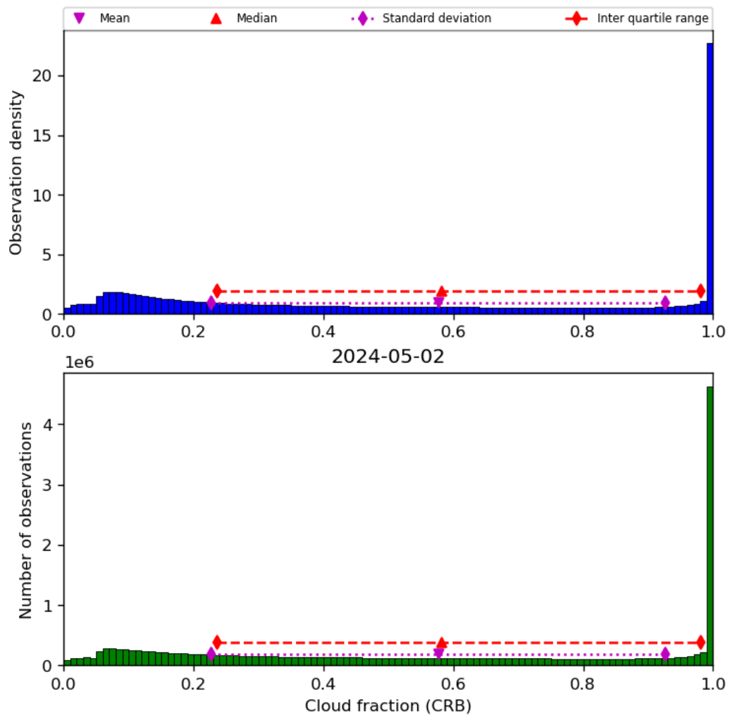
Figure 42: Histogram of “Cloud fraction (CRB)” for 2024-05-02 to 2024-05-03
