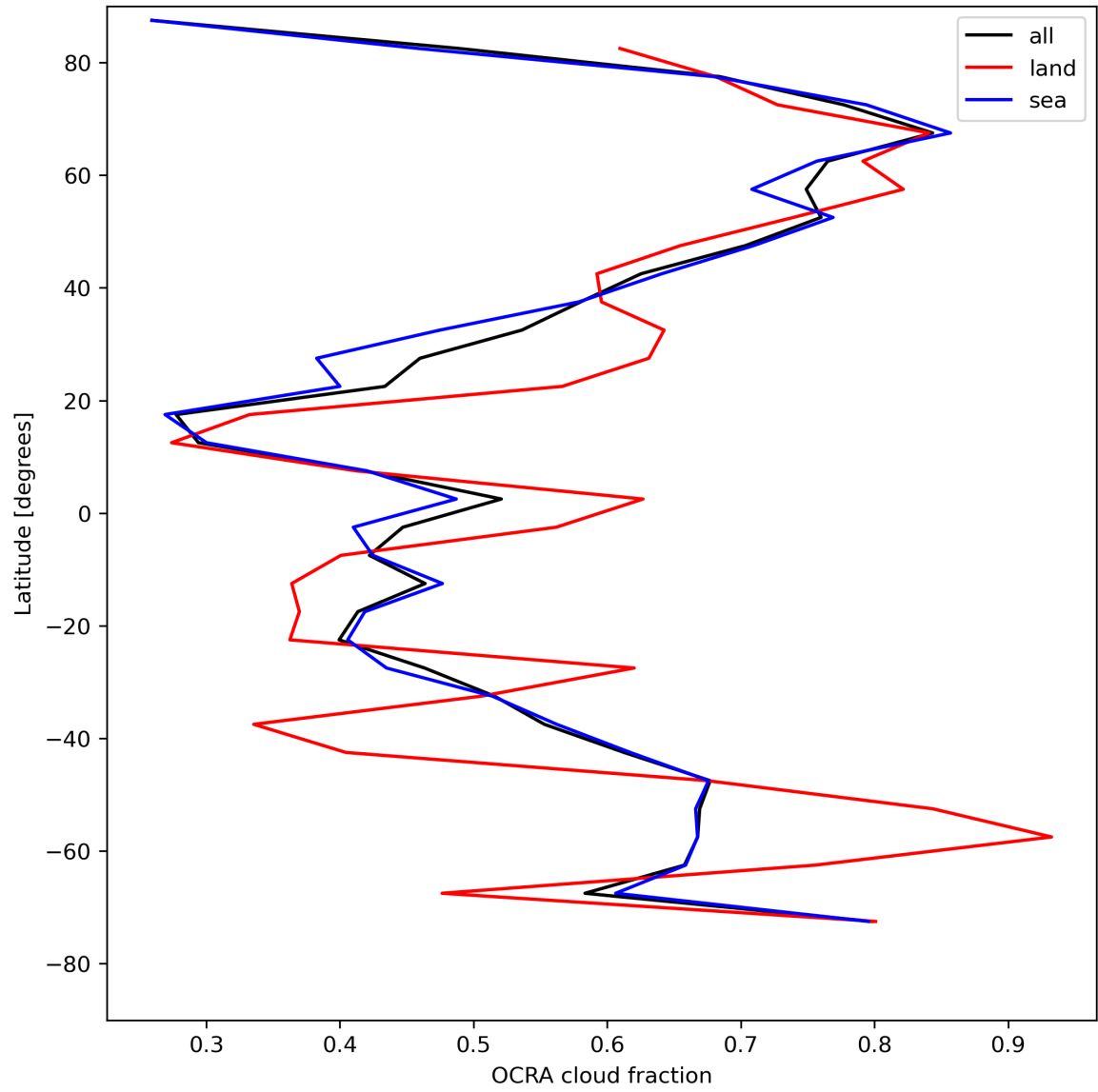
Figure 34: Zonal average of “OCRA cloud fraction” for 2024-05-02 to 2024-05-03.
