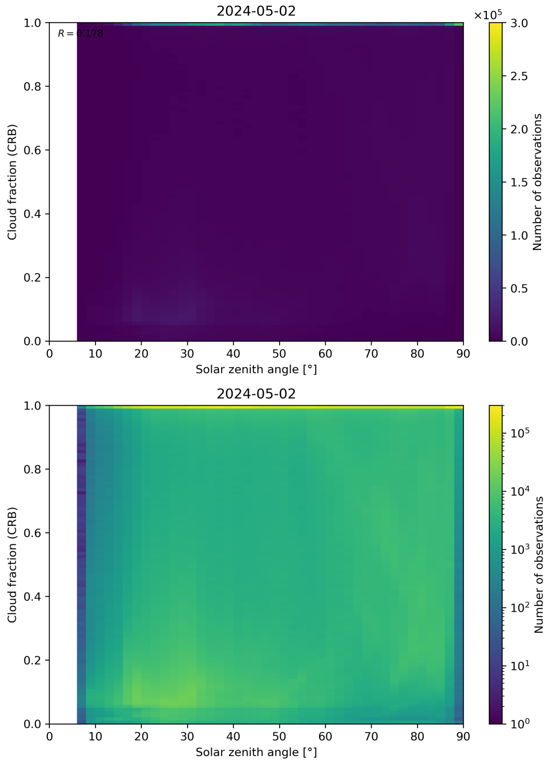
Figure 101: Scatter density plot of “Solar zenith angle” against “Cloud fraction (CRB)” for 2024-05-02 to 2024-05-03.
