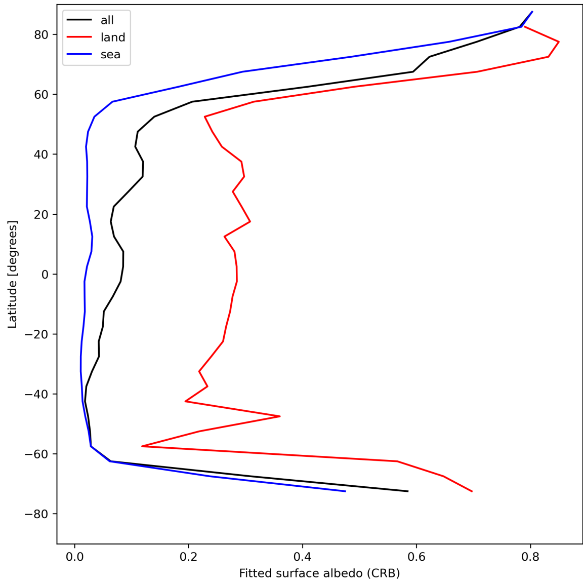
Figure 30: Zonal average of “Fitted surface albedo (CRB)” for 2024-05-02 to 2024-05-03.
