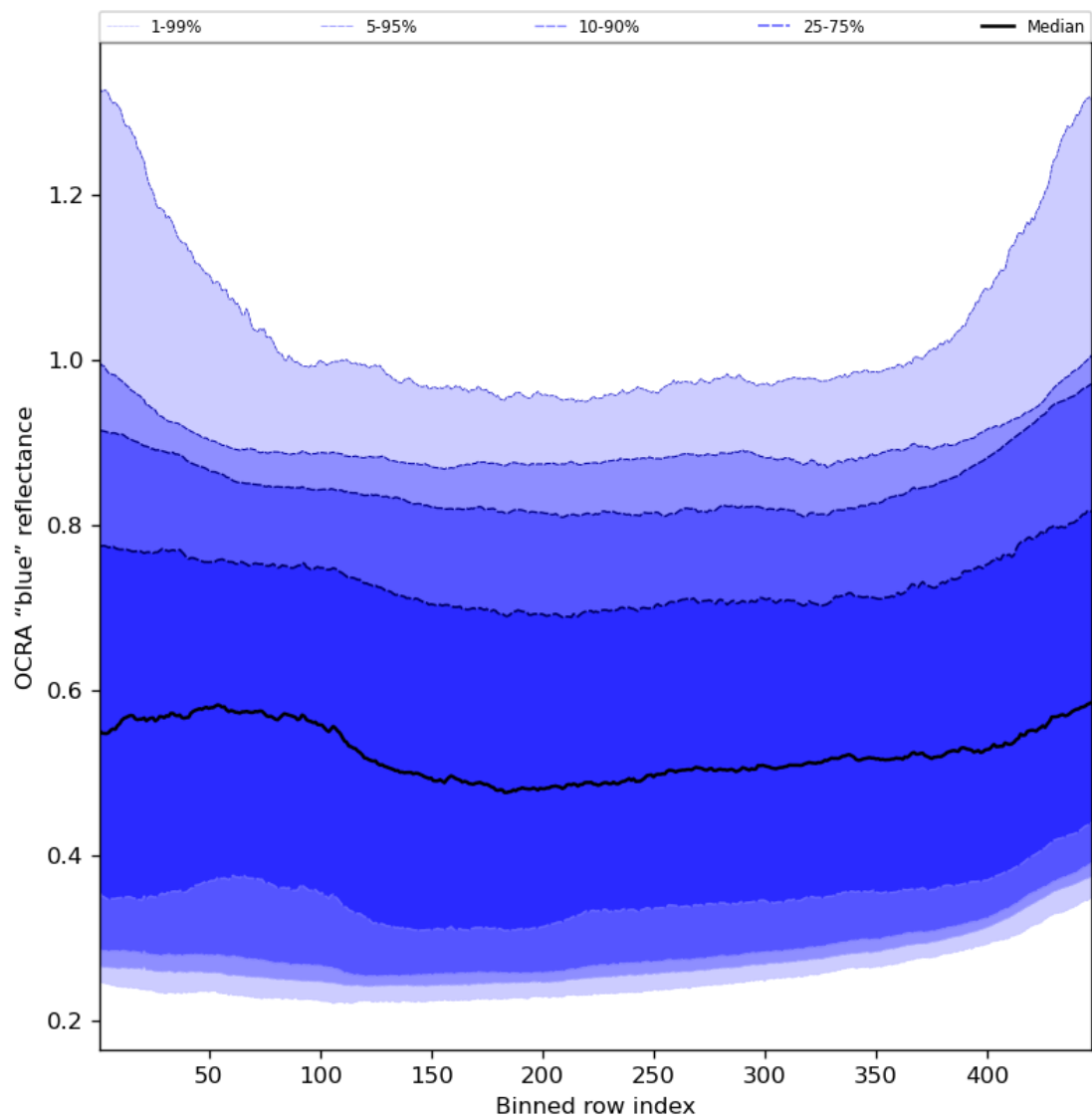
Figure 67: Along track statistics of “OCRA “blue” reflectance” for 2024-05-02 to 2024-05-03
