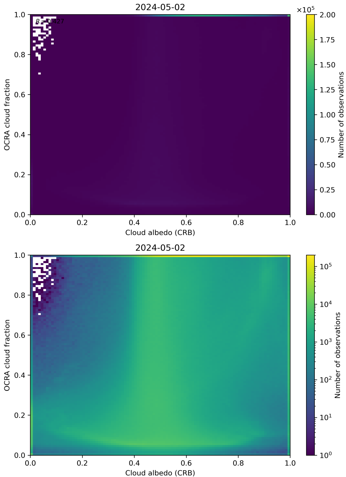
Figure 70: Scatter density plot of “Cloud albedo (CRB)” against “OCRA cloud fraction” for 2024-05-02 to 2024-05-03.
