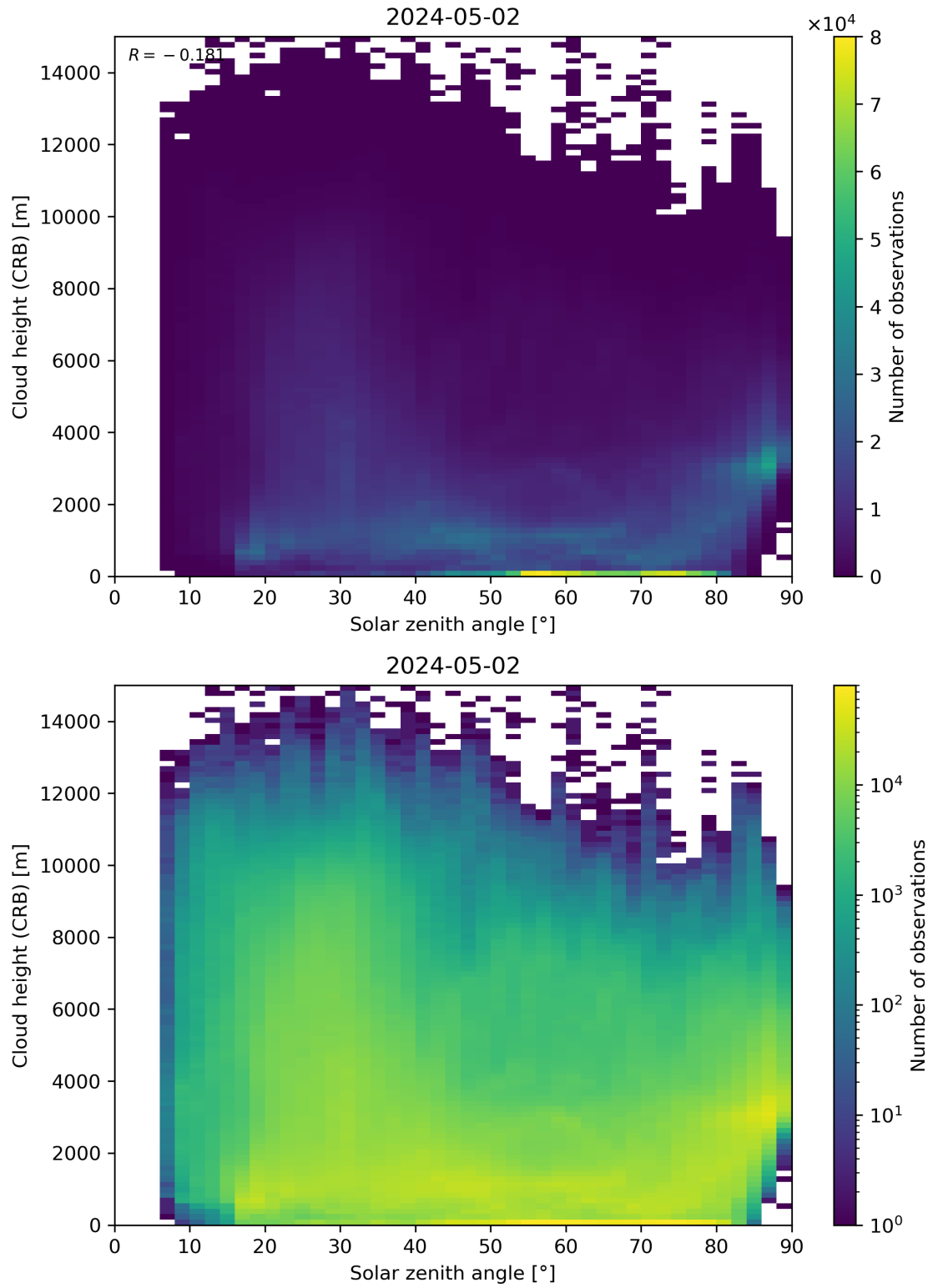
Figure 102: Scatter density plot of “Solar zenith angle” against “Cloud height (CRB)” for 2024-05-02 to 2024-05-03.
