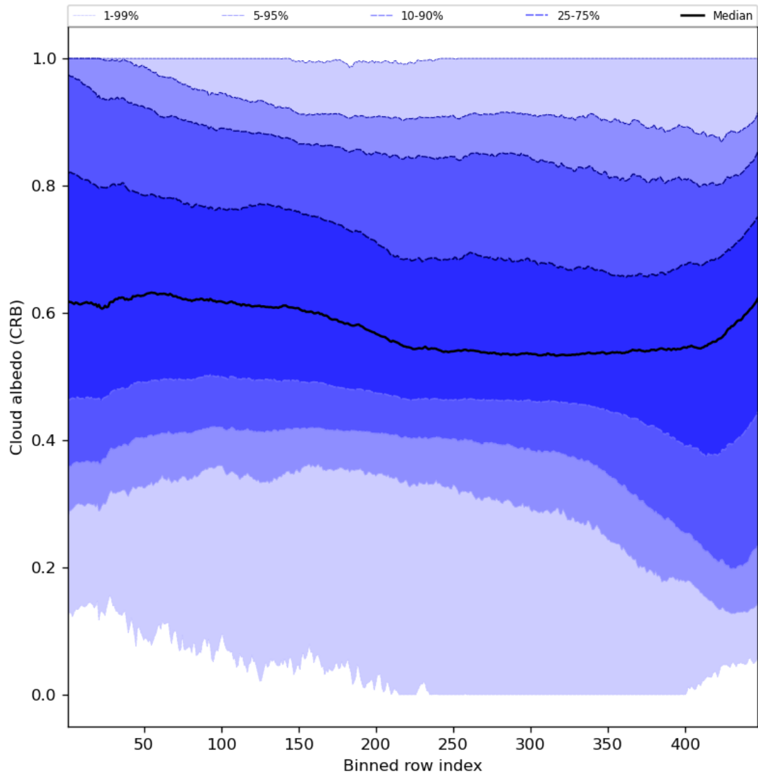
Figure 60: Along track statistics of “Cloud albedo (CRB)” for 2024-05-02 to 2024-05-03
