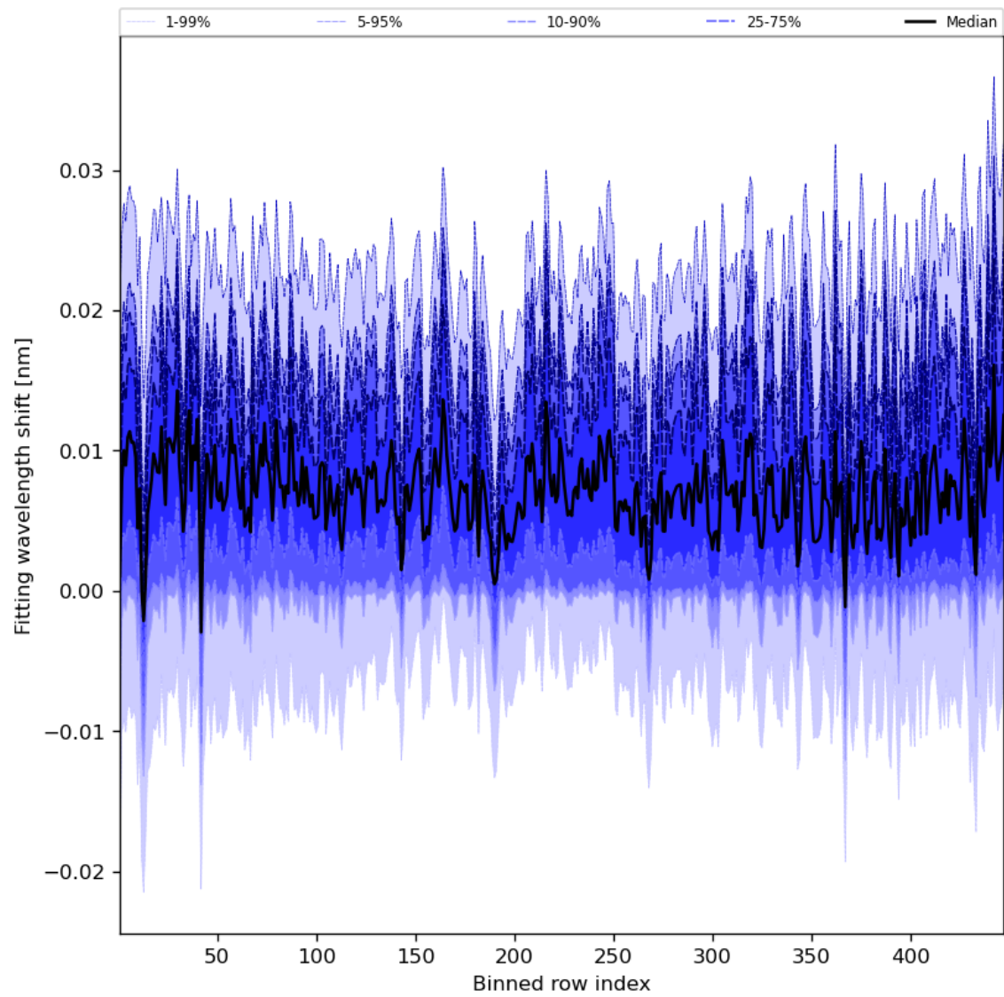
Figure 65: Along track statistics of “Fitting wavelength shift” for 2024-05-02 to 2024-05-03
