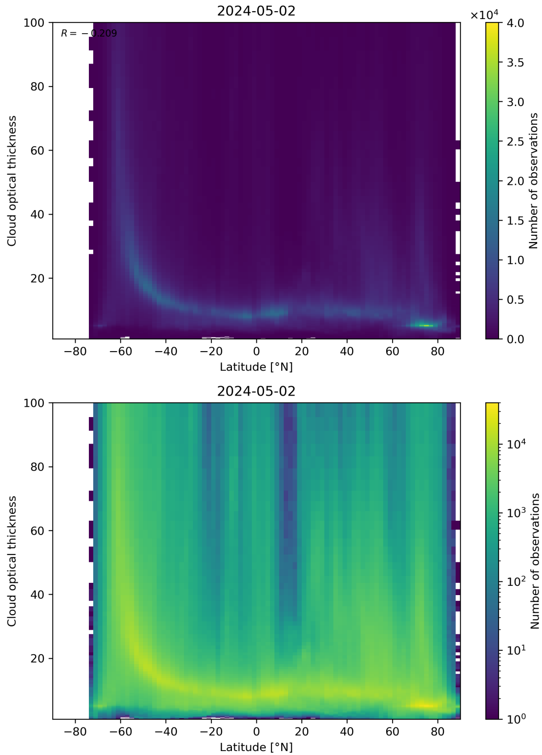
Figure 96: Scatter density plot of “Latitude” against “Cloud optical thickness” for 2024-05-02 to 2024-05-03.
