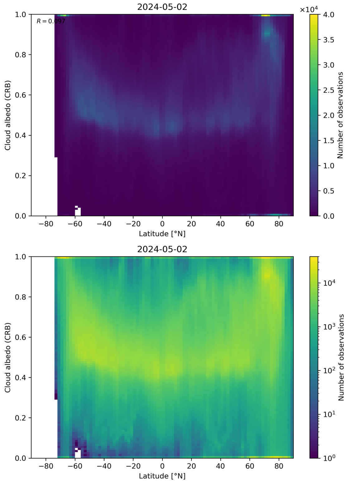
Figure 91: Scatter density plot of “Latitude” against “Cloud albedo (CRB)” for 2024-05-02 to 2024-05-03.
