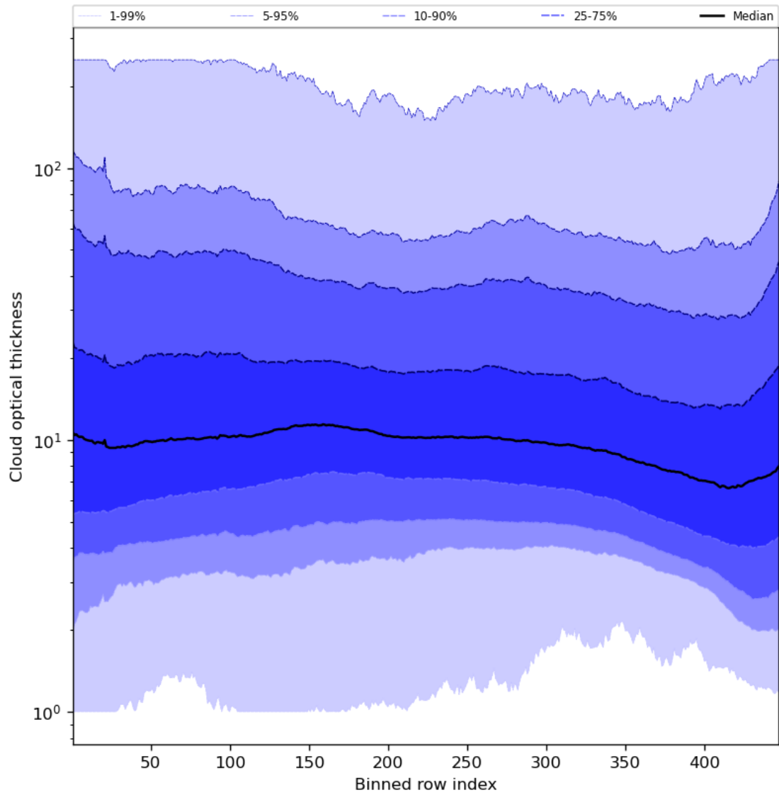
Figure 57: Along track statistics of “Cloud optical thickness” for 2024-05-02 to 2024-05-03
