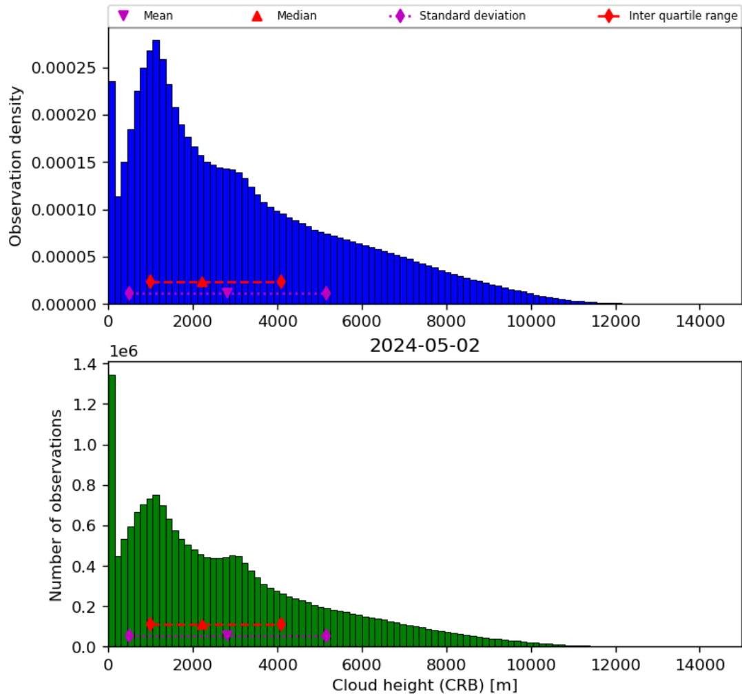
Figure 43: Histogram of “Cloud height (CRB)” for 2024-05-02 to 2024-05-03
