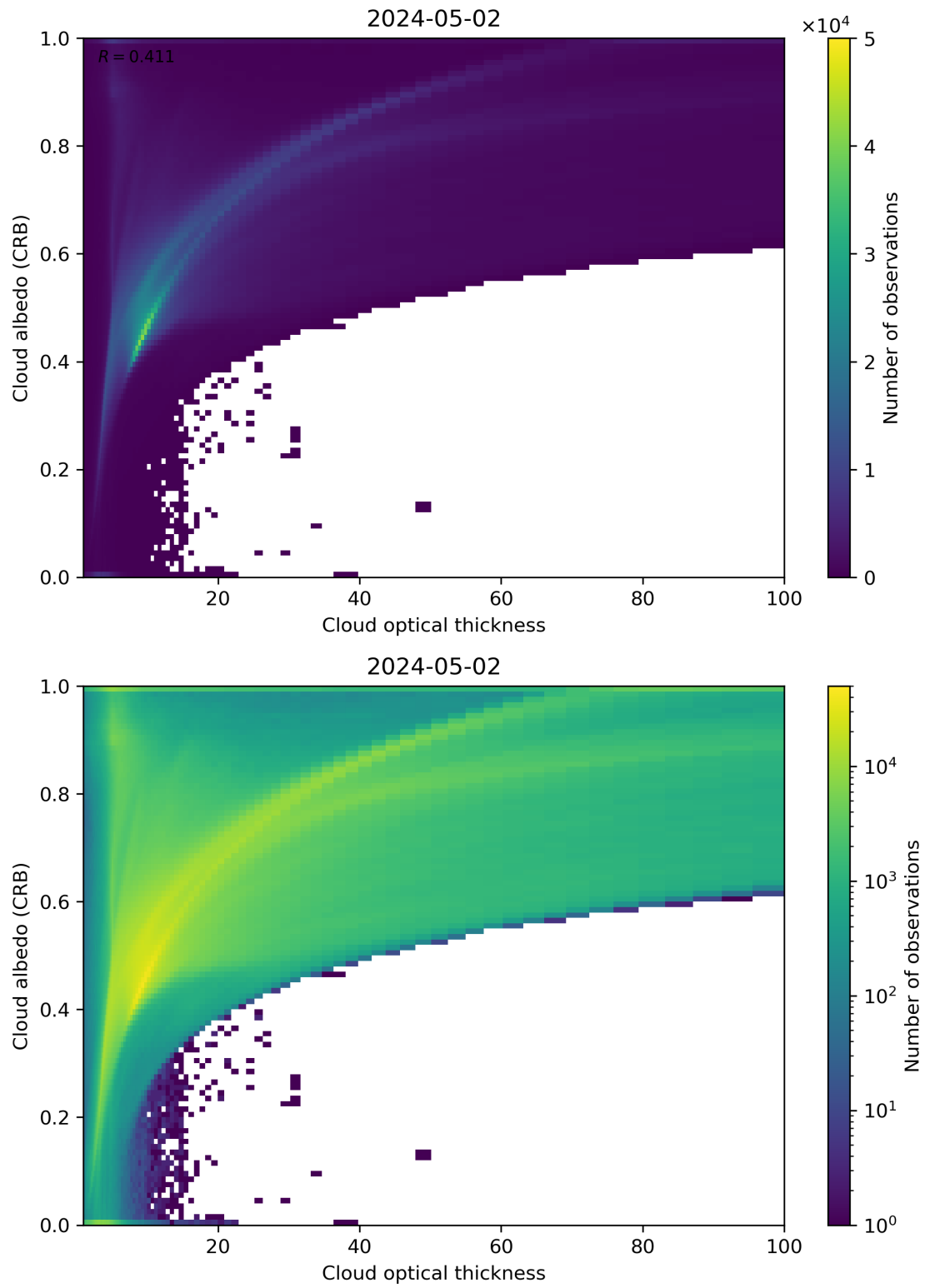
Figure 82: Scatter density plot of “Cloud optical thickness” against “Cloud albedo (CRB)” for 2024-05-02 to 2024-05-03.
