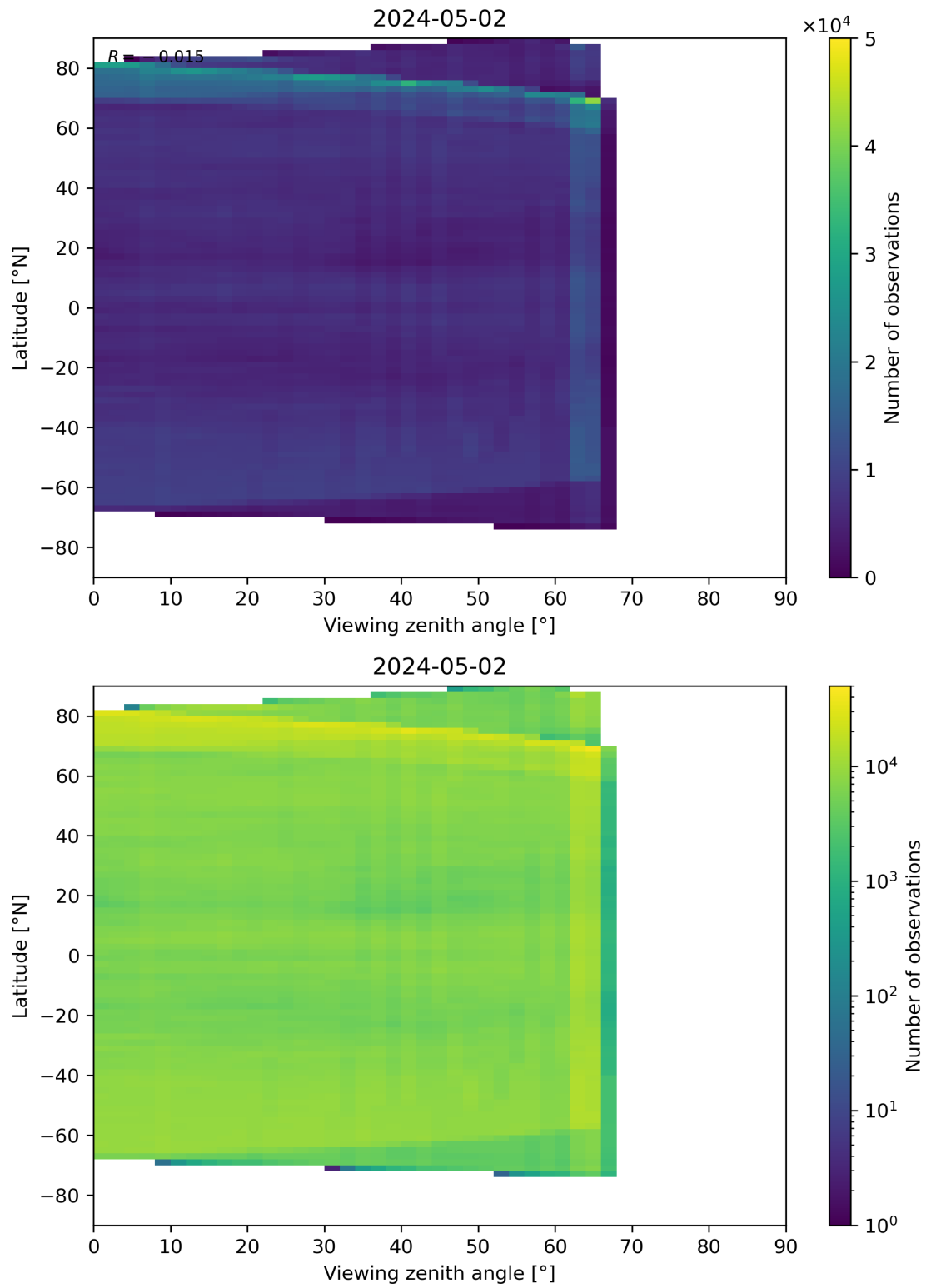
Figure 113: Scatter density plot of “Viewing zenith angle” against “Latitude” for 2024-05-02 to 2024-05-03.
