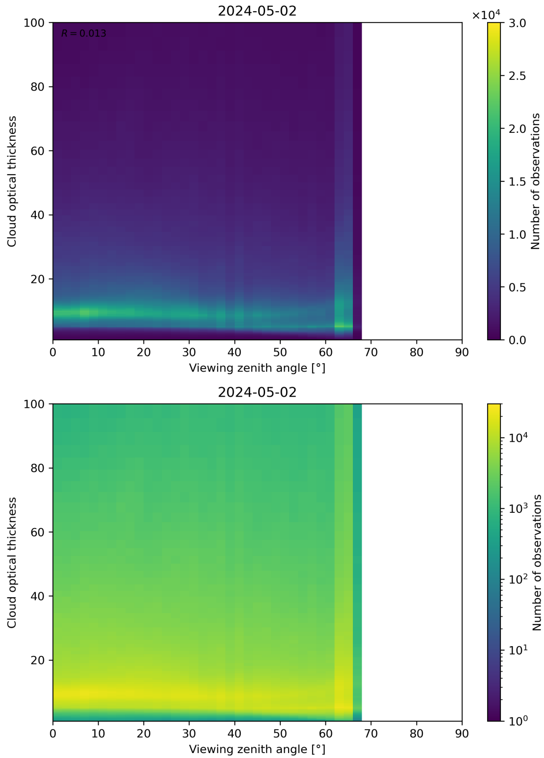
Figure 111: Scatter density plot of “Viewing zenith angle” against “Cloud optical thickness” for 2024-05-02 to 2024-05-03.
