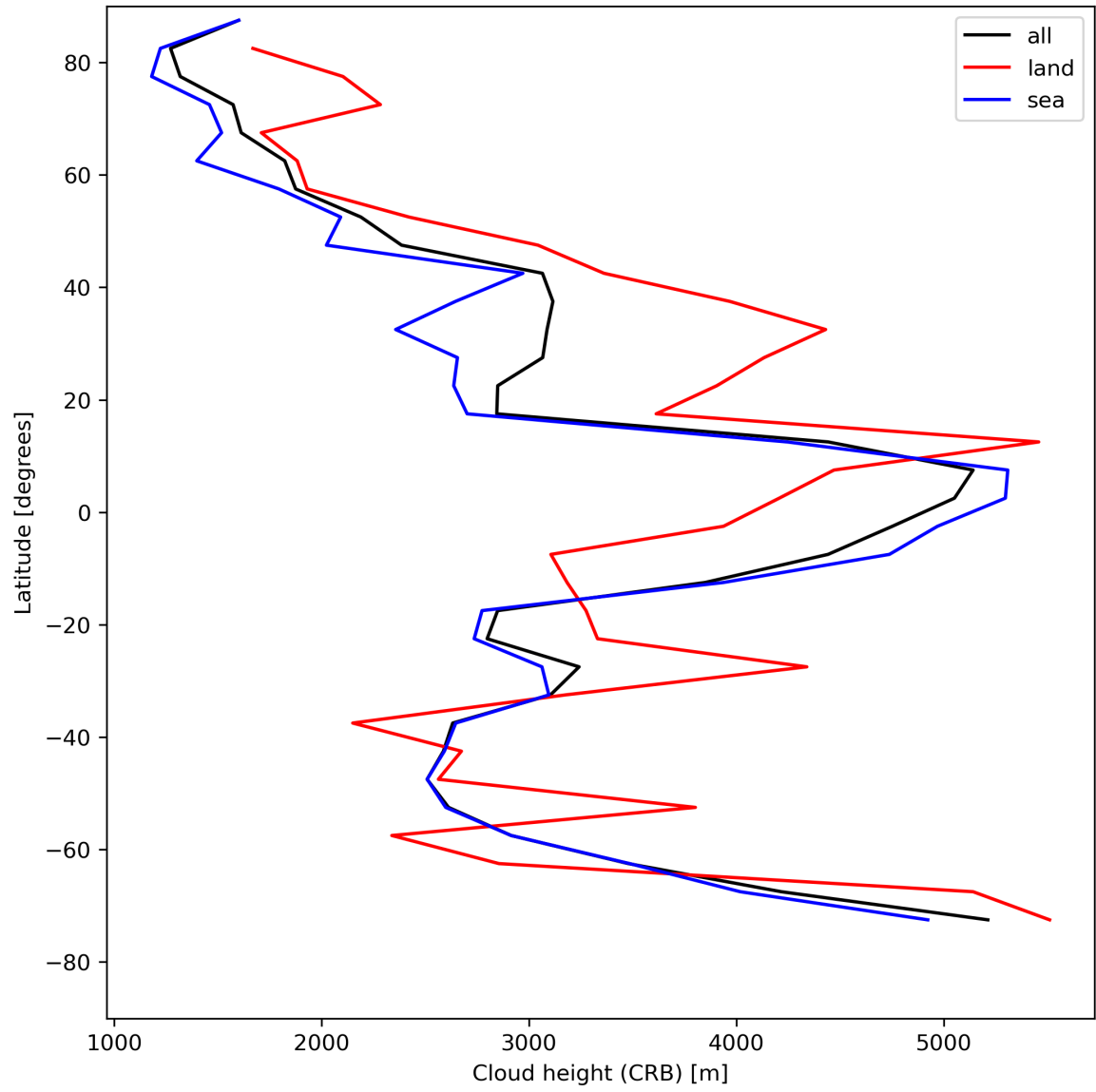
Figure 27: Zonal average of “Cloud height (CRB)” for 2024-05-02 to 2024-05-03.
