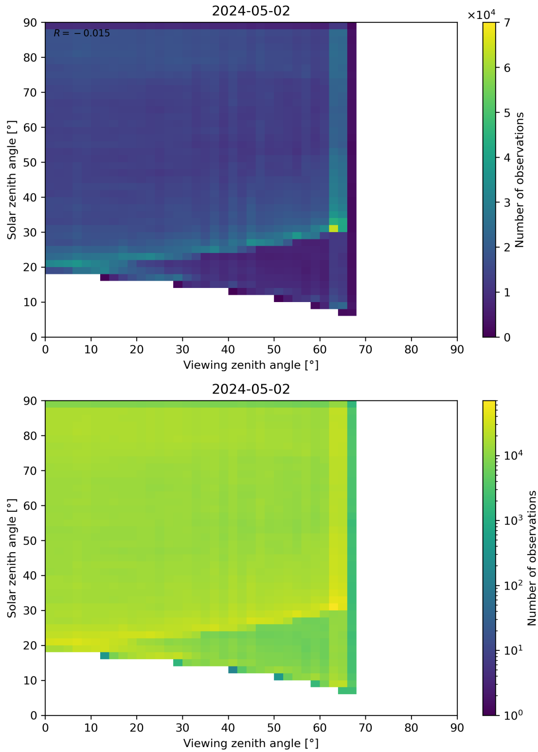
Figure 114: Scatter density plot of “Viewing zenith angle” against “Solar zenith angle” for 2024-05-02 to 2024-05-03.
