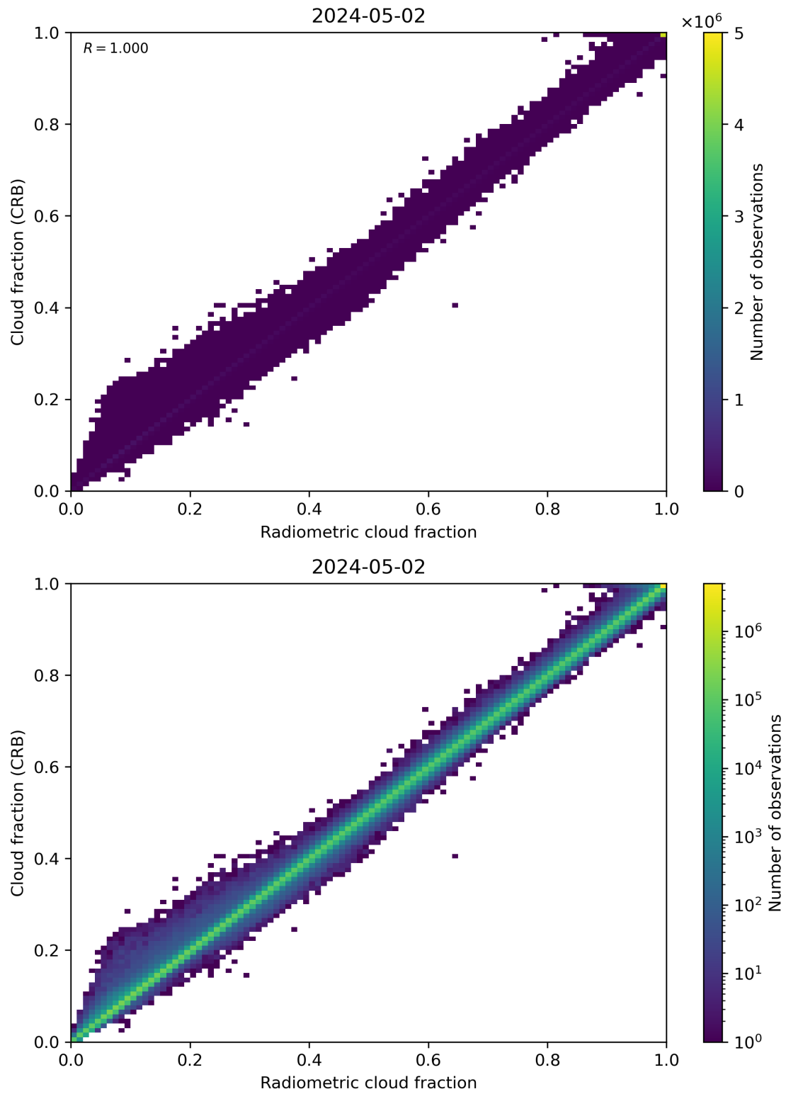
Figure 73: Scatter density plot of “Radiometric cloud fraction” against “Cloud fraction (CRB)” for 2024-05-02 to 2024-05-03.
