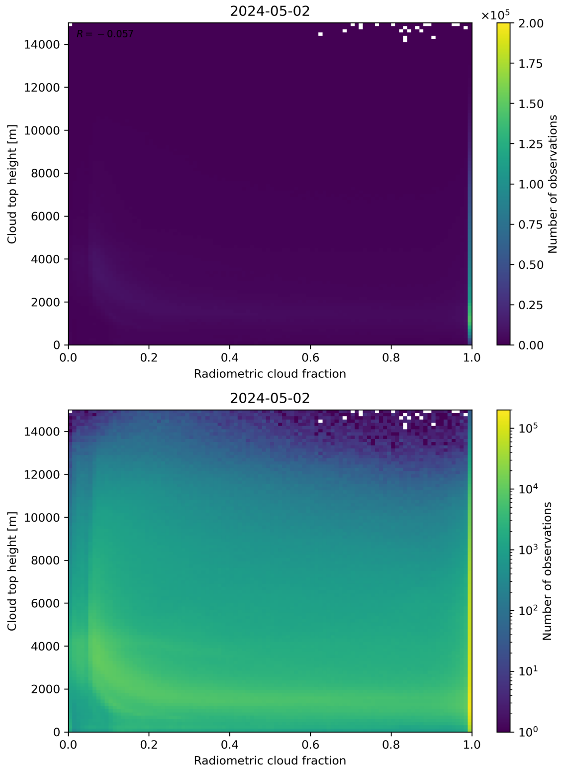
Figure 76: Scatter density plot of “Radiometric cloud fraction” against “Cloud top height” for 2024-05-02 to 2024-05-03.
