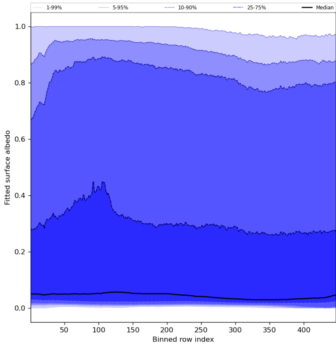
Figure 61: Along track statistics of “Fitted surface albedo” for 2024-05-02 to 2024-05-03
