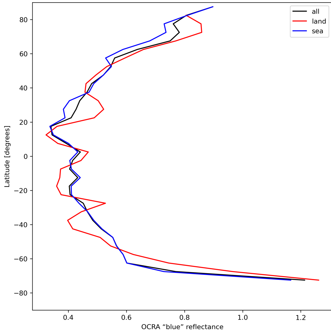
Figure 35: Zonal average of "OCRA "blue" reflectance" for 2024-05-02 to 2024-05-03.
