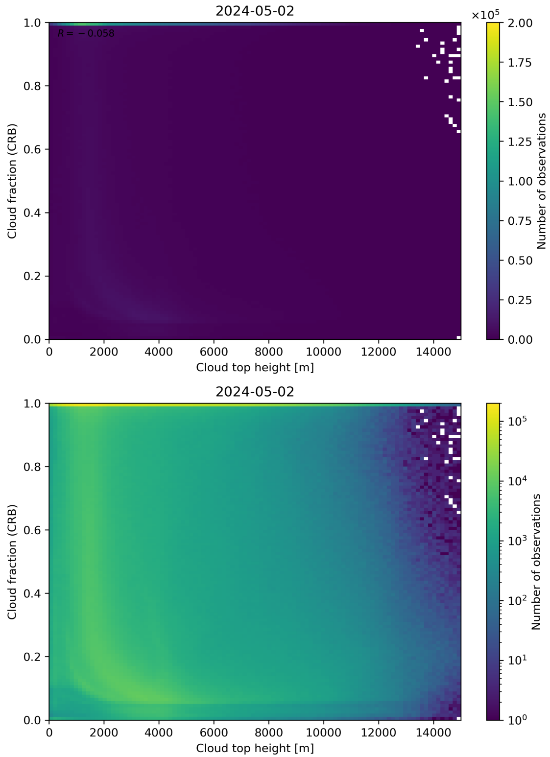
Figure 88: Scatter density plot of “Cloud top height” against “Cloud fraction (CRB)” for 2024-05-02 to 2024-05-03.
