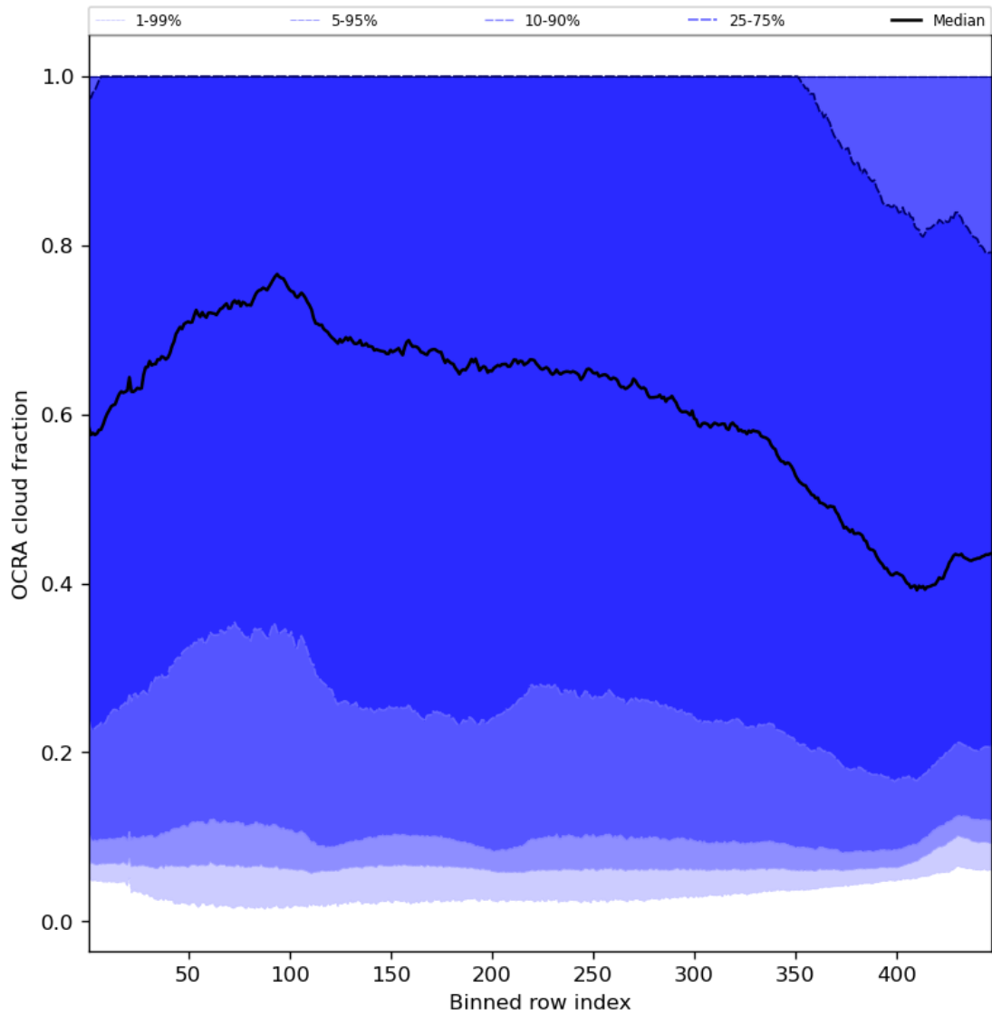
Figure 66: Along track statistics of “OCRA cloud fraction” for 2024-05-02 to 2024-05-03
