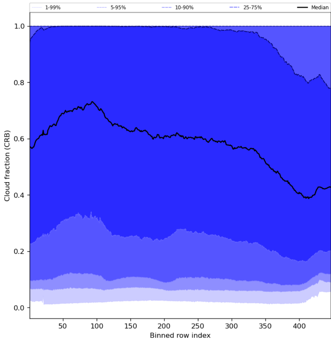
Figure 58: Along track statistics of “Cloud fraction (CRB)” for 2024-05-02 to 2024-05-03
