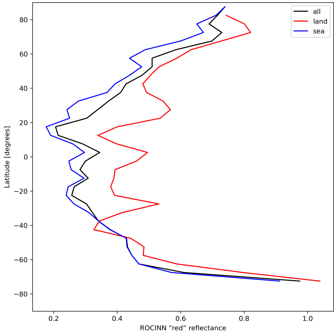
Figure 37: Zonal average of “ROCINN “red” reflectance” for 2024-05-02 to 2024-05-03.
