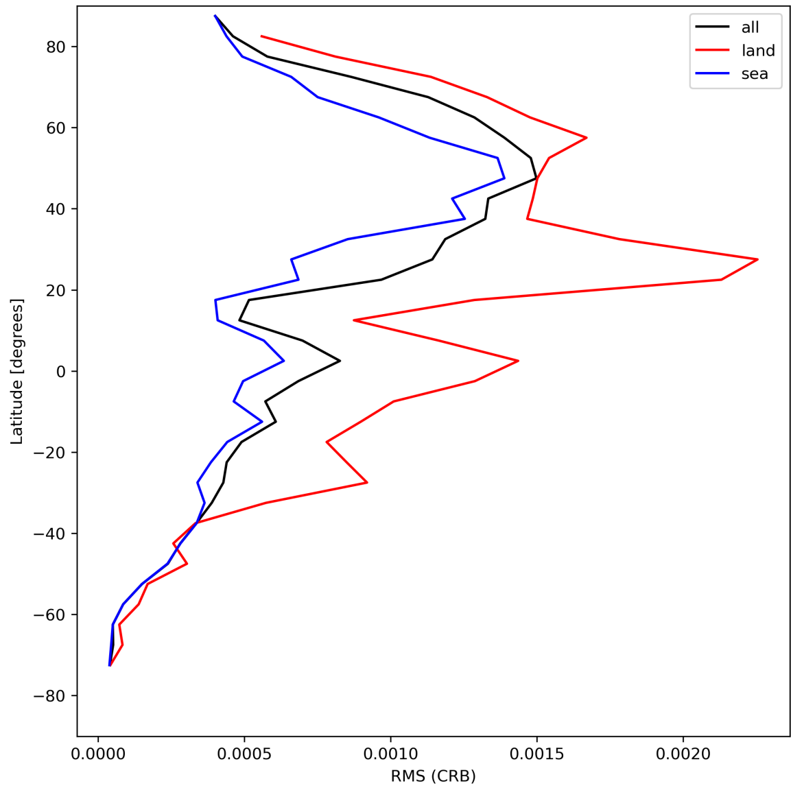
Figure 32: Zonal average of “RMS (CRB)” for 2024-05-02 to 2024-05-03.
