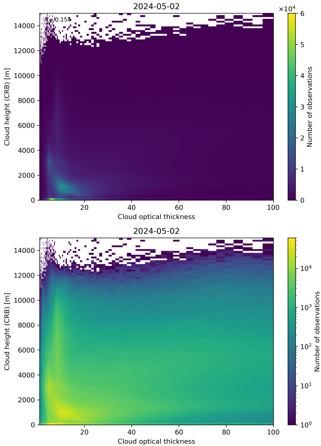
Figure 85: Scatter density plot of “Cloud optical thickness” against “Cloud height (CRB)” for 2024-05-02 to 2024-05-03.
