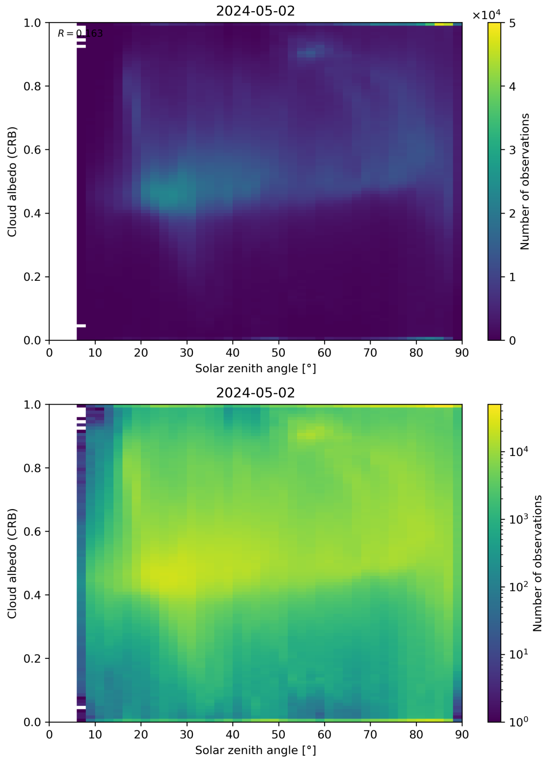
Figure 98: Scatter density plot of “Solar zenith angle” against “Cloud albedo (CRB)” for 2024-05-02 to 2024-05-03.
