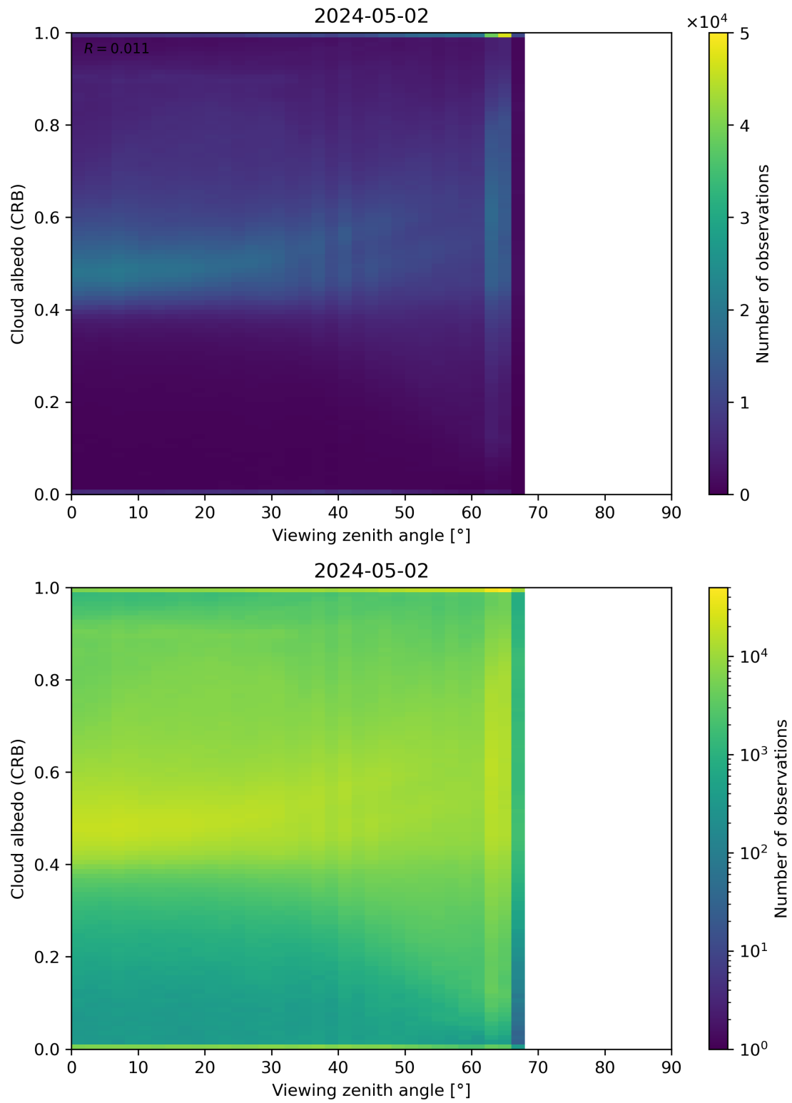
Figure 106: Scatter density plot of “Viewing zenith angle” against “Cloud albedo (CRB)” for 2024-05-02 to 2024-05-03.
