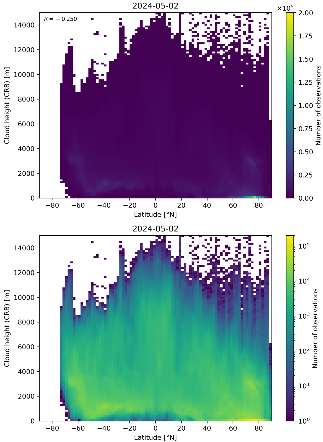
Figure 95: Scatter density plot of “Latitude” against “Cloud height (CRB)” for 2024-05-02 to 2024-05-03.
