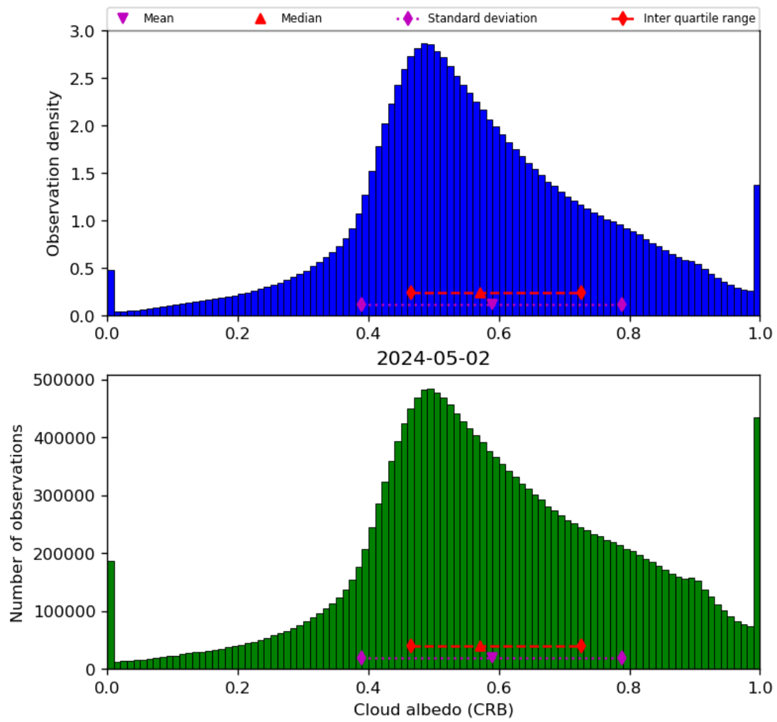
Figure 44: Histogram of “Cloud albedo (CRB)” for 2024-05-02 to 2024-05-03
