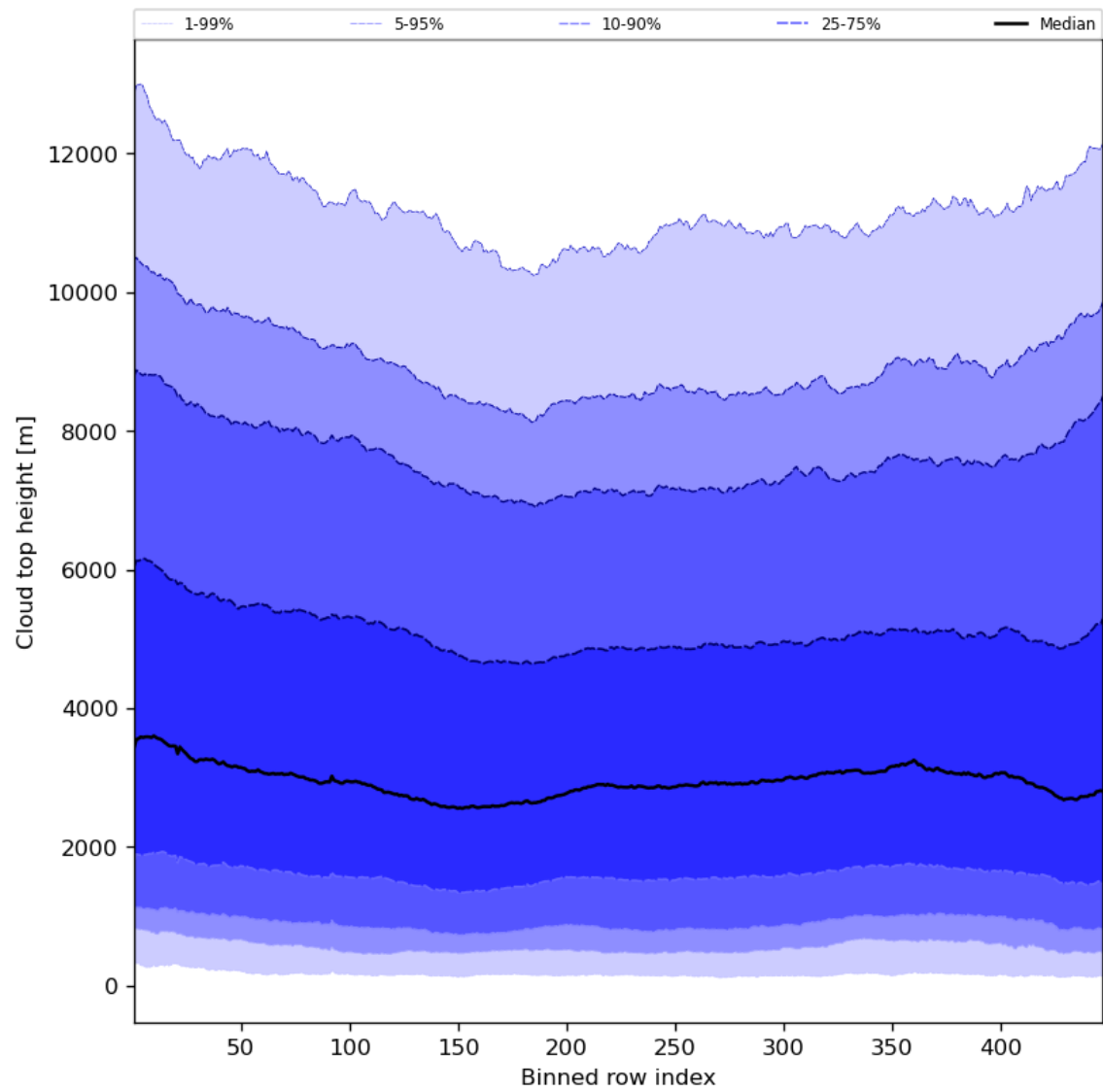
Figure 56: Along track statistics of “Cloud top height” for 2024-05-02 to 2024-05-03
