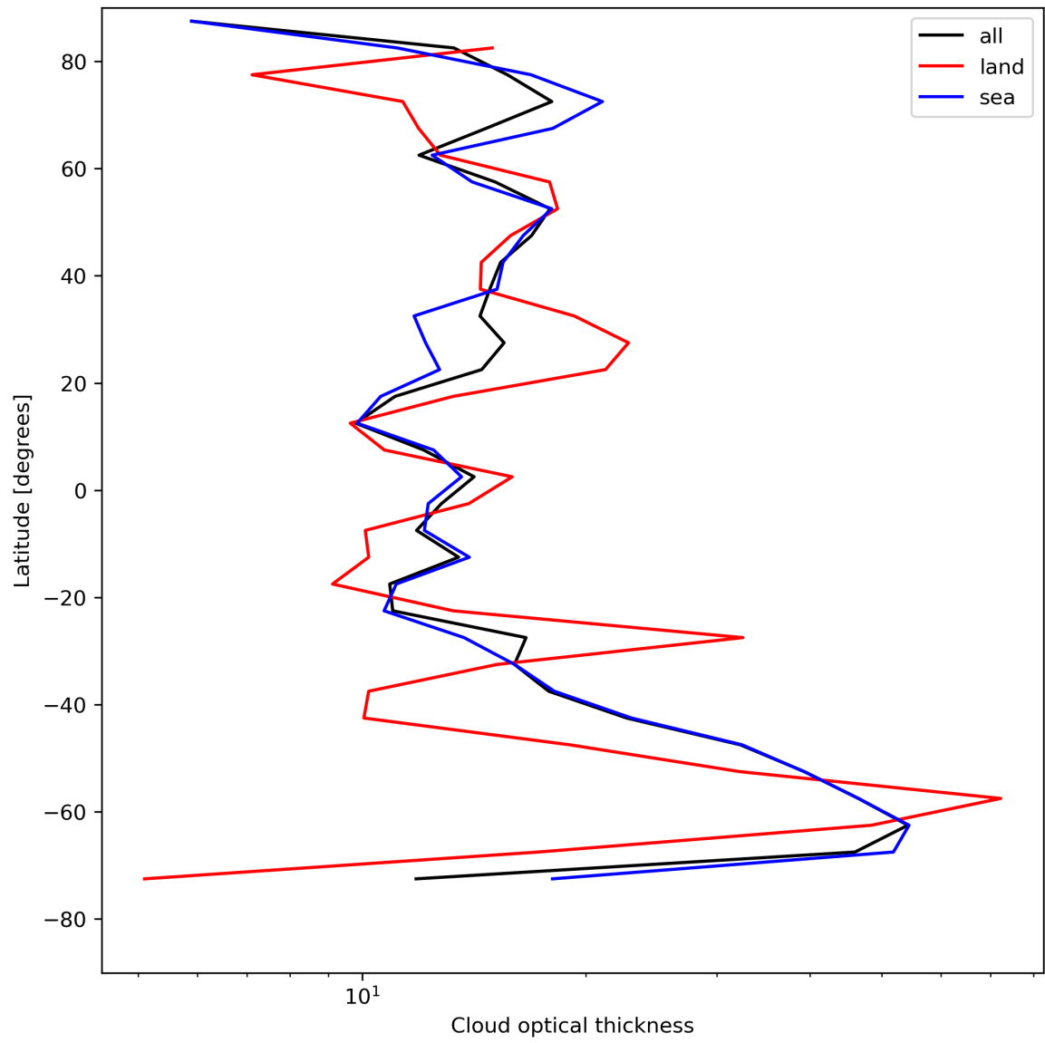
Figure 25: Zonal average of “Cloud optical thickness” for 2024-05-02 to 2024-05-03.
