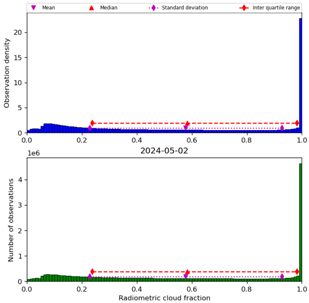
Figure 39: Histogram of “Radiometric cloud fraction” for 2024-05-02 to 2024-05-03
