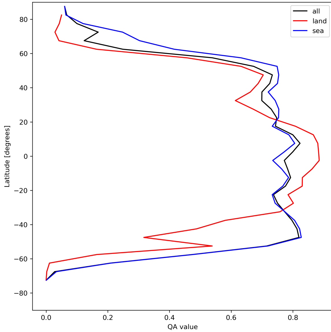
Figure 22: Zonal average of “QA value” for 2024-05-02 to 2024-05-03.
