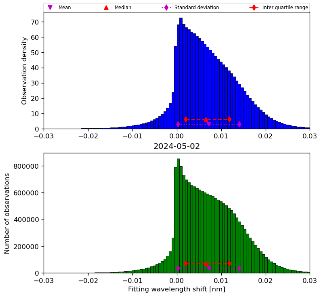
Figure 49: Histogram of “Fitting wavelength shift” for 2024-05-02 to 2024-05-03
