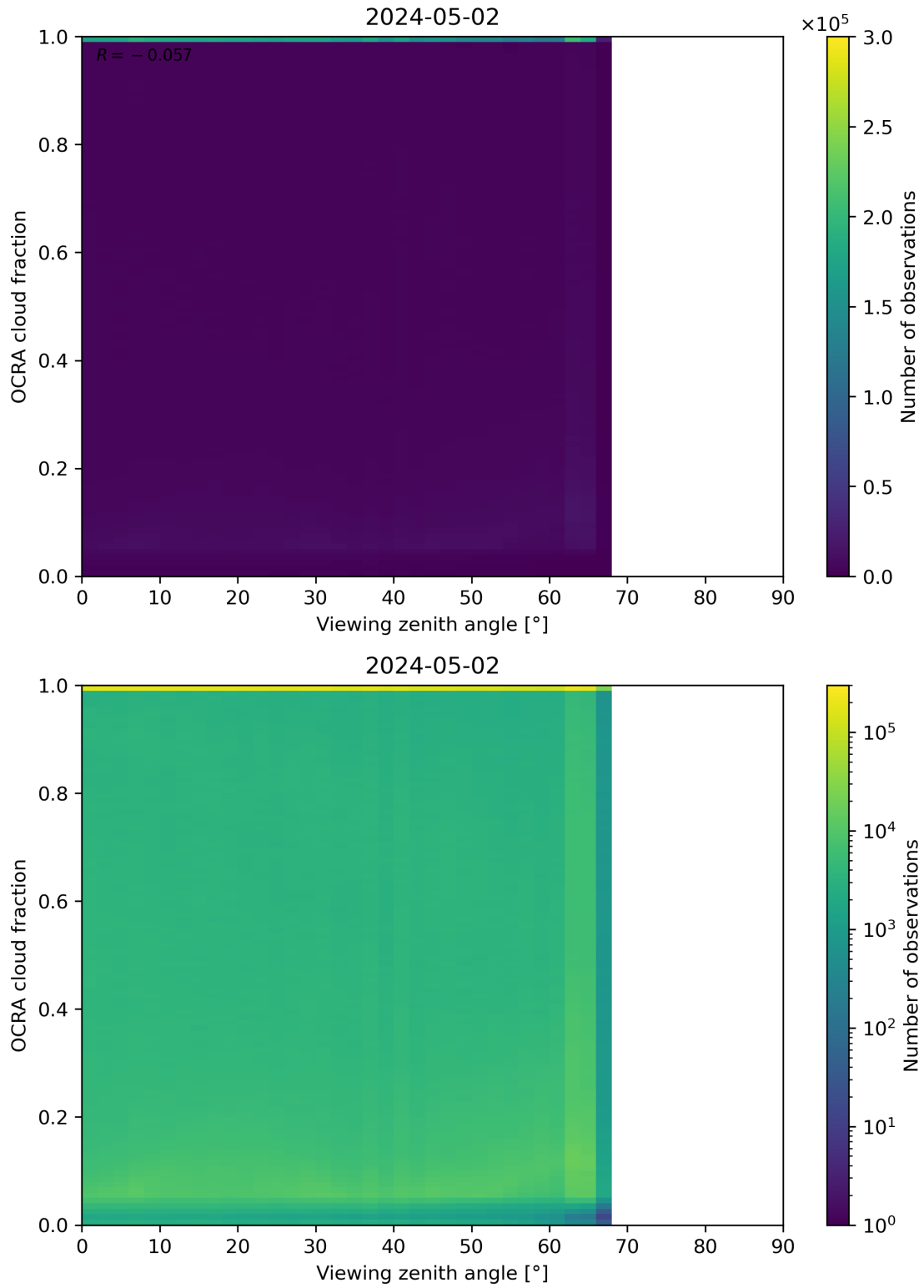
Figure 108: Scatter density plot of “Viewing zenith angle” against “OCRA cloud fraction” for 2024-05-02 to 2024-05-03.
