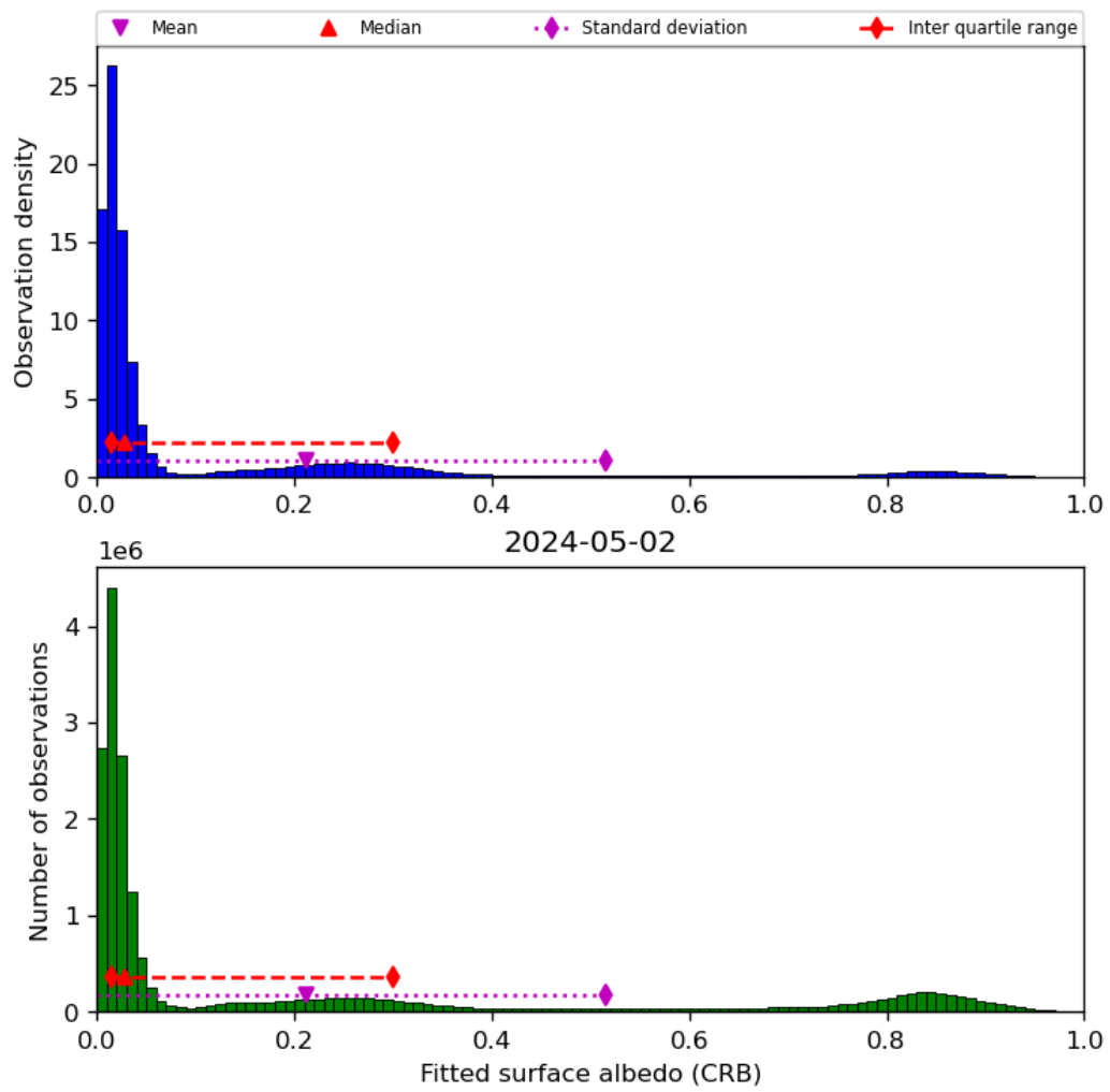
Figure 46: Histogram of “Fitted surface albedo (CRB)” for 2024-05-02 to 2024-05-03
