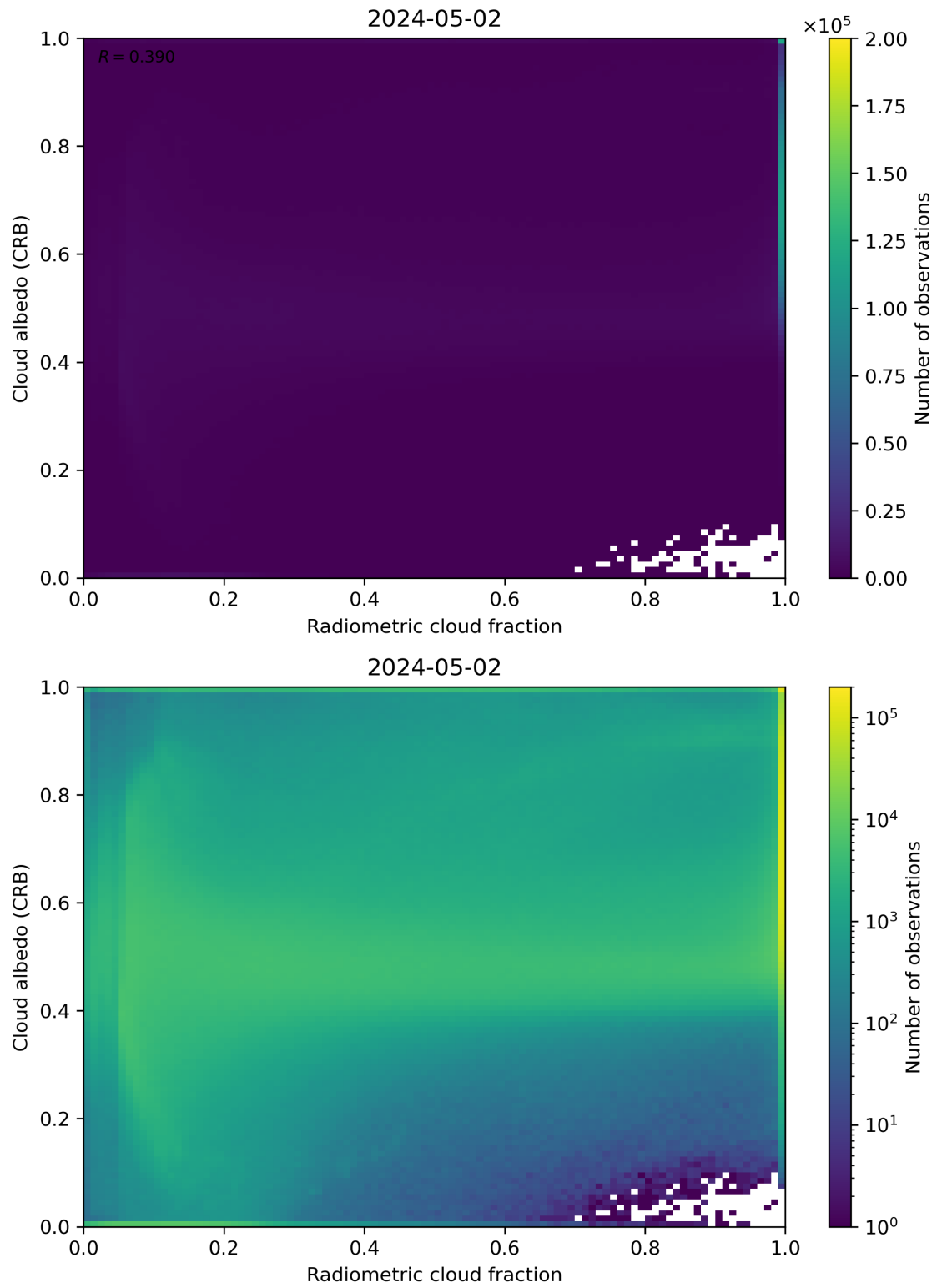
Figure 71: Scatter density plot of “Radiometric cloud fraction” against “Cloud albedo (CRB)” for 2024-05-02 to 2024-05-03.
