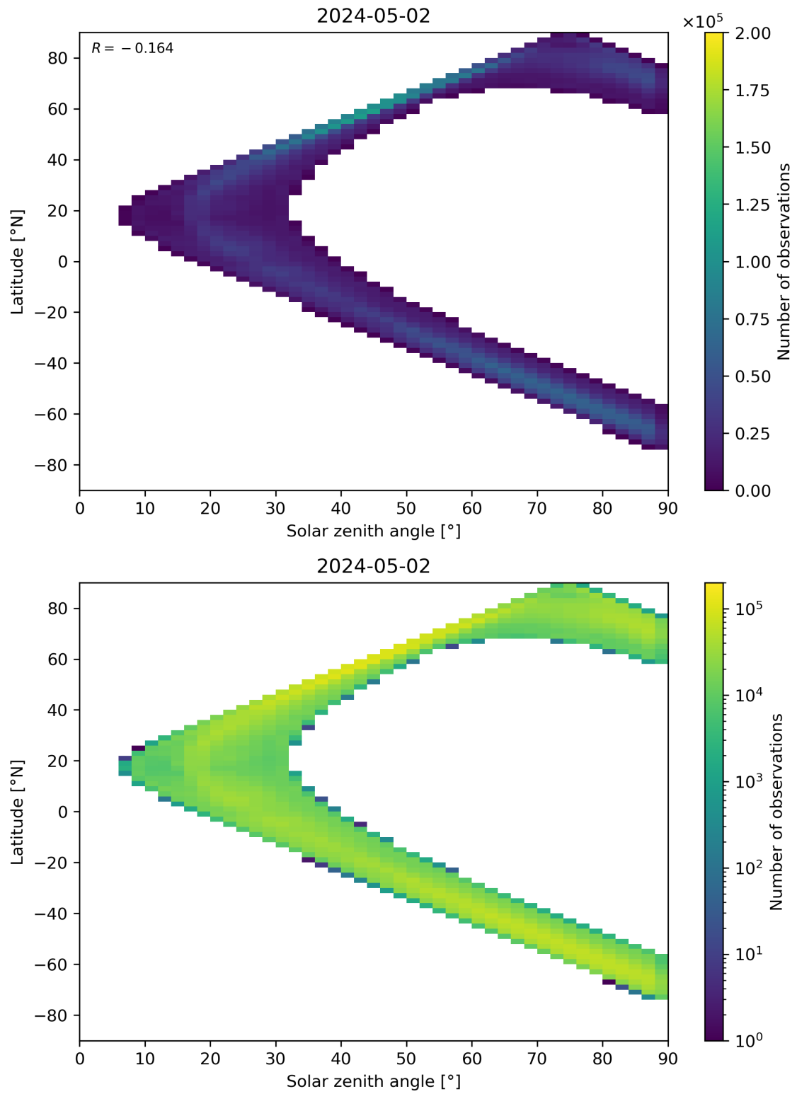
Figure 105: Scatter density plot of “Solar zenith angle” against “Latitude” for 2024-05-02 to 2024-05-03.
