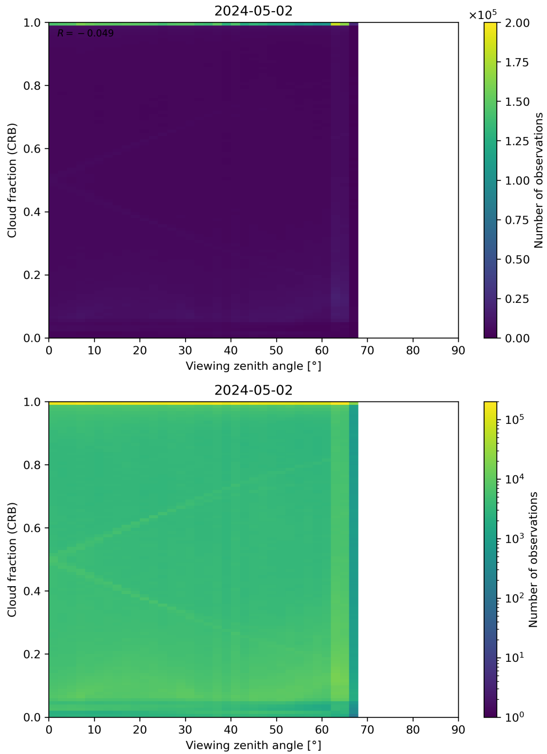
Figure 109: Scatter density plot of “Viewing zenith angle” against “Cloud fraction (CRB)” for 2024-05-02 to 2024-05-03.
