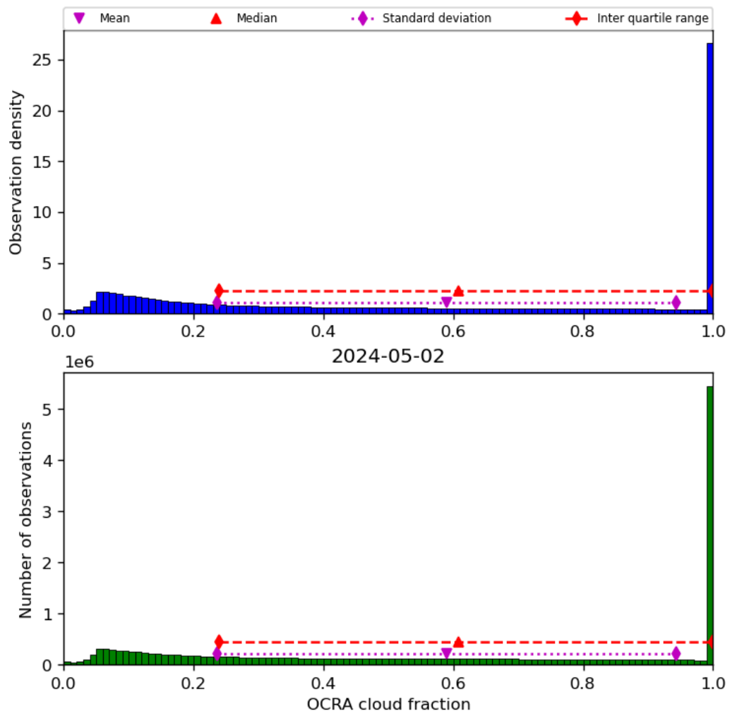
Figure 50: Histogram of “OCRA cloud fraction” for 2024-05-02 to 2024-05-03
