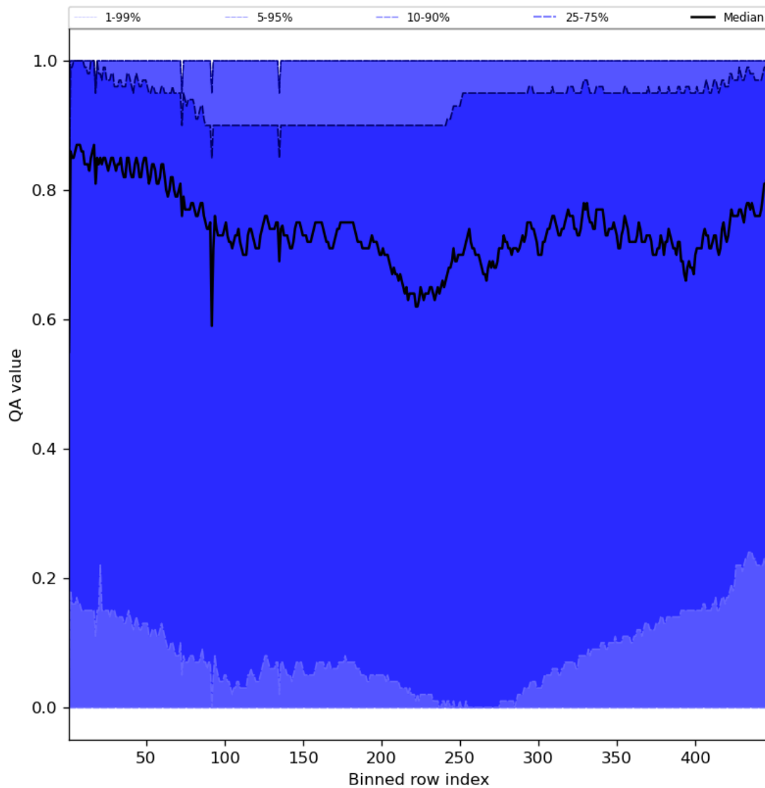
Figure 54: Along track statistics of “QA value” for 2024-05-02 to 2024-05-03
