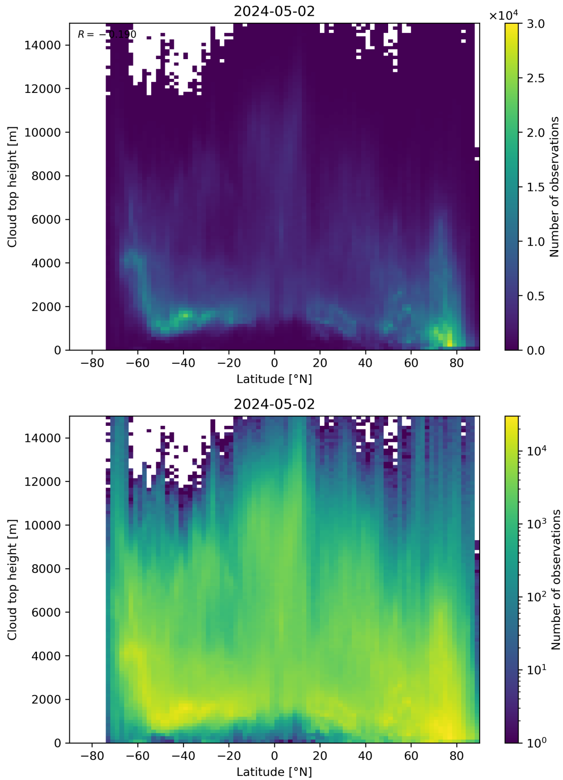
Figure 97: Scatter density plot of “Latitude” against “Cloud top height” for 2024-05-02 to 2024-05-03.
