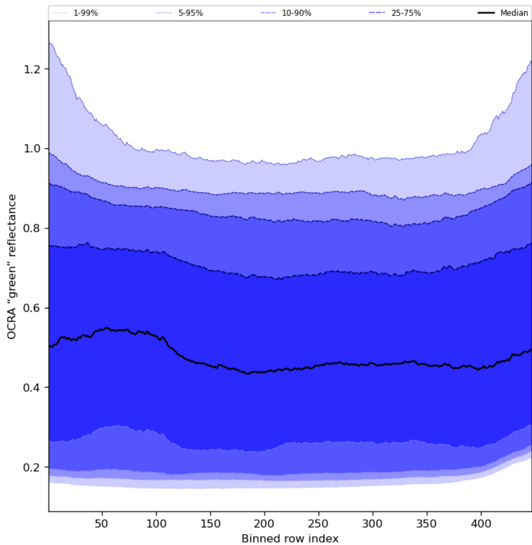
Figure 68: Along track statistics of "OCRA "green" reflectance" for 2024-05-02 to 2024-05-03
