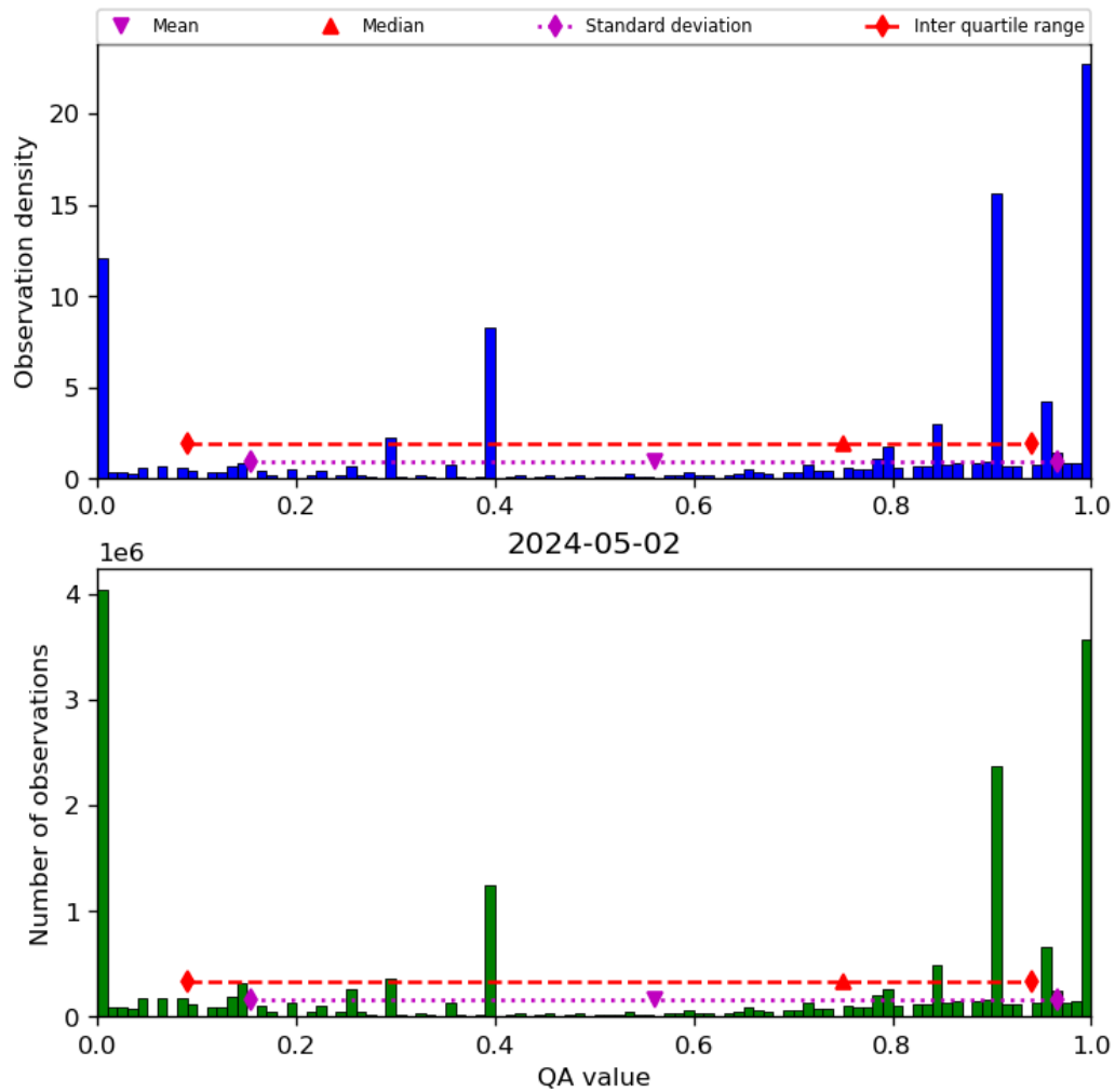
Figure 38: Histogram of “QA value” for 2024-05-02 to 2024-05-03
