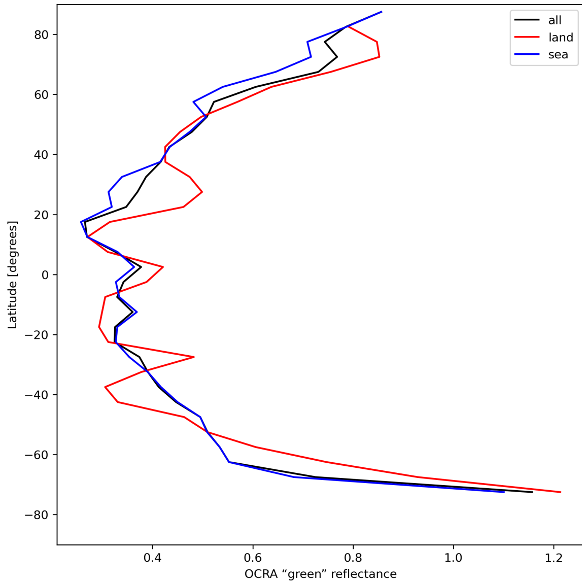
Figure 36: Zonal average of “OCRA “green” reflectance” for 2024-05-02 to 2024-05-03.
