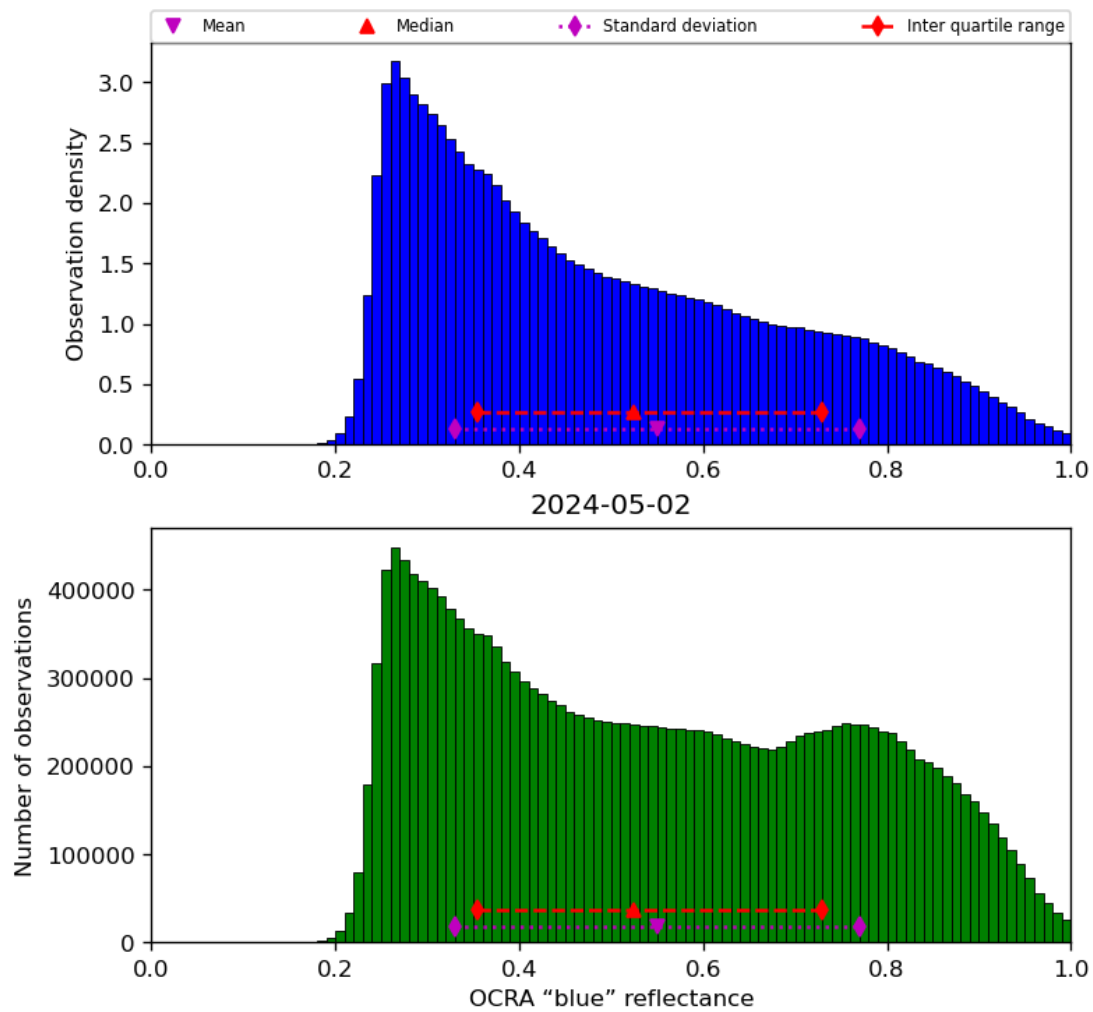
Figure 51: Histogram of “OCRA “blue” reflectance” for 2024-05-02 to 2024-05-03
