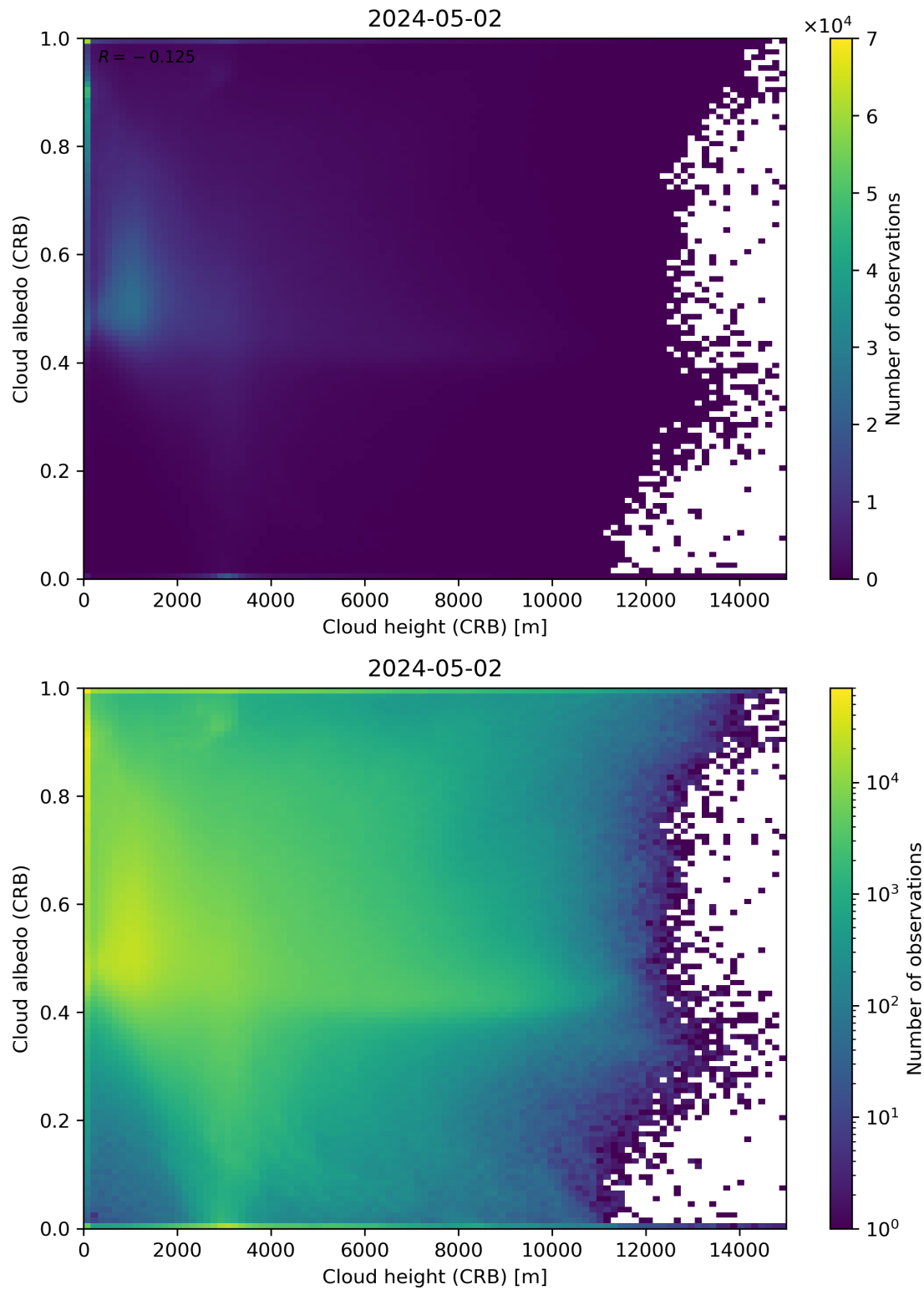
Figure 80: Scatter density plot of “Cloud height (CRB)” against “Cloud albedo (CRB)” for 2024-05-02 to 2024-05-03.
