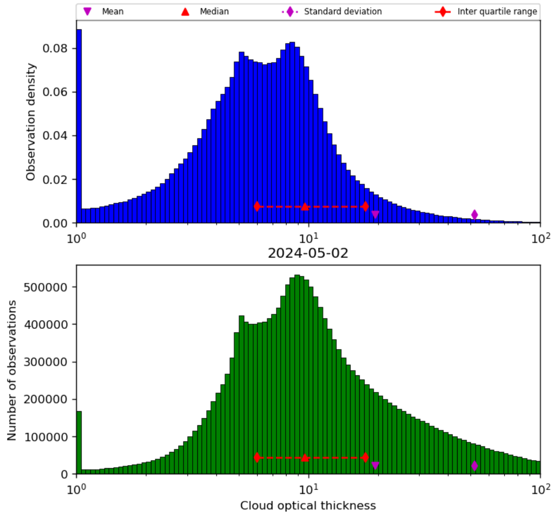
Figure 41: Histogram of “Cloud optical thickness” for 2024-05-02 to 2024-05-03
