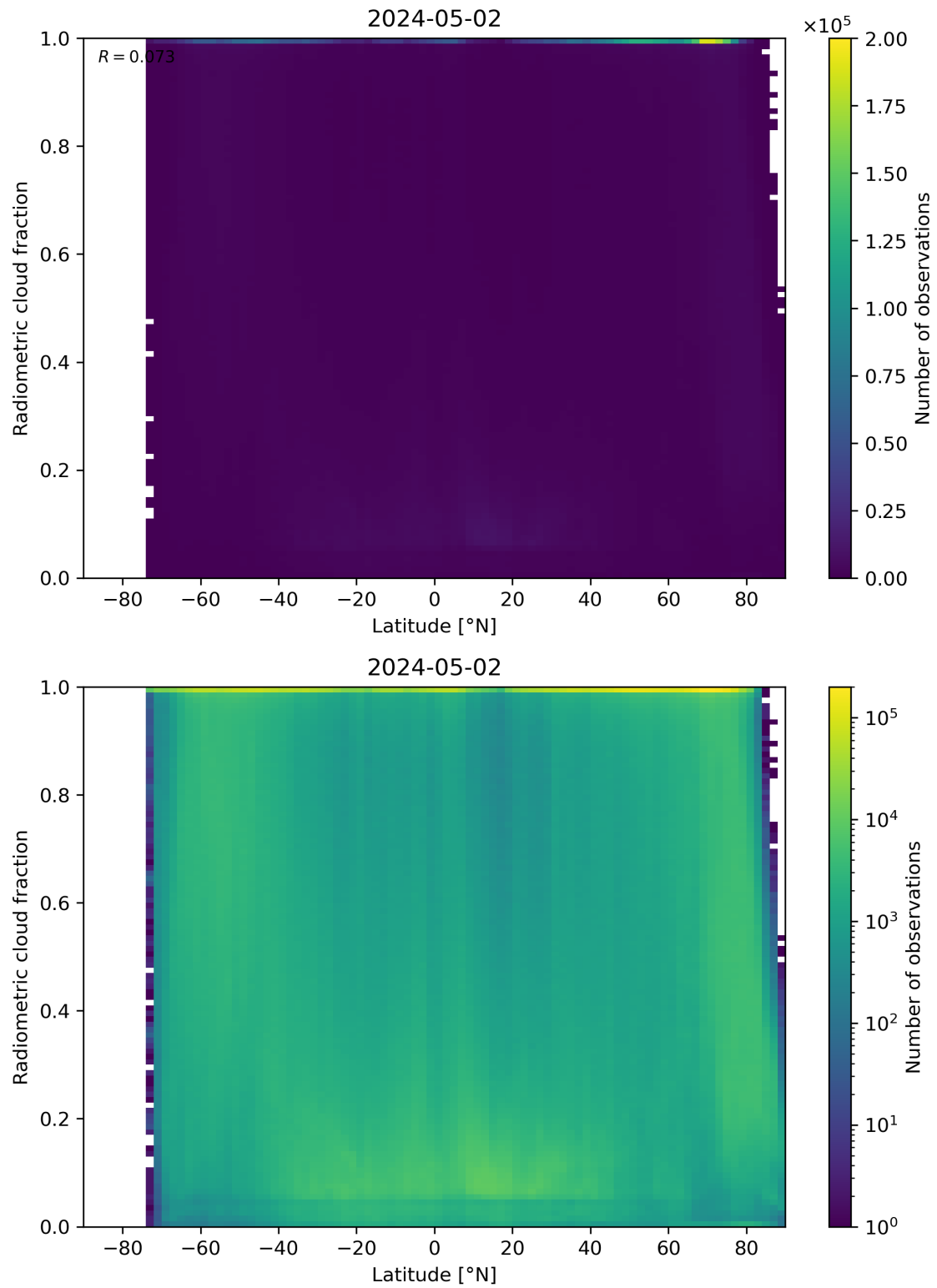
Figure 92: Scatter density plot of “Latitude” against “Radiometric cloud fraction” for 2024-05-02 to 2024-05-03.
