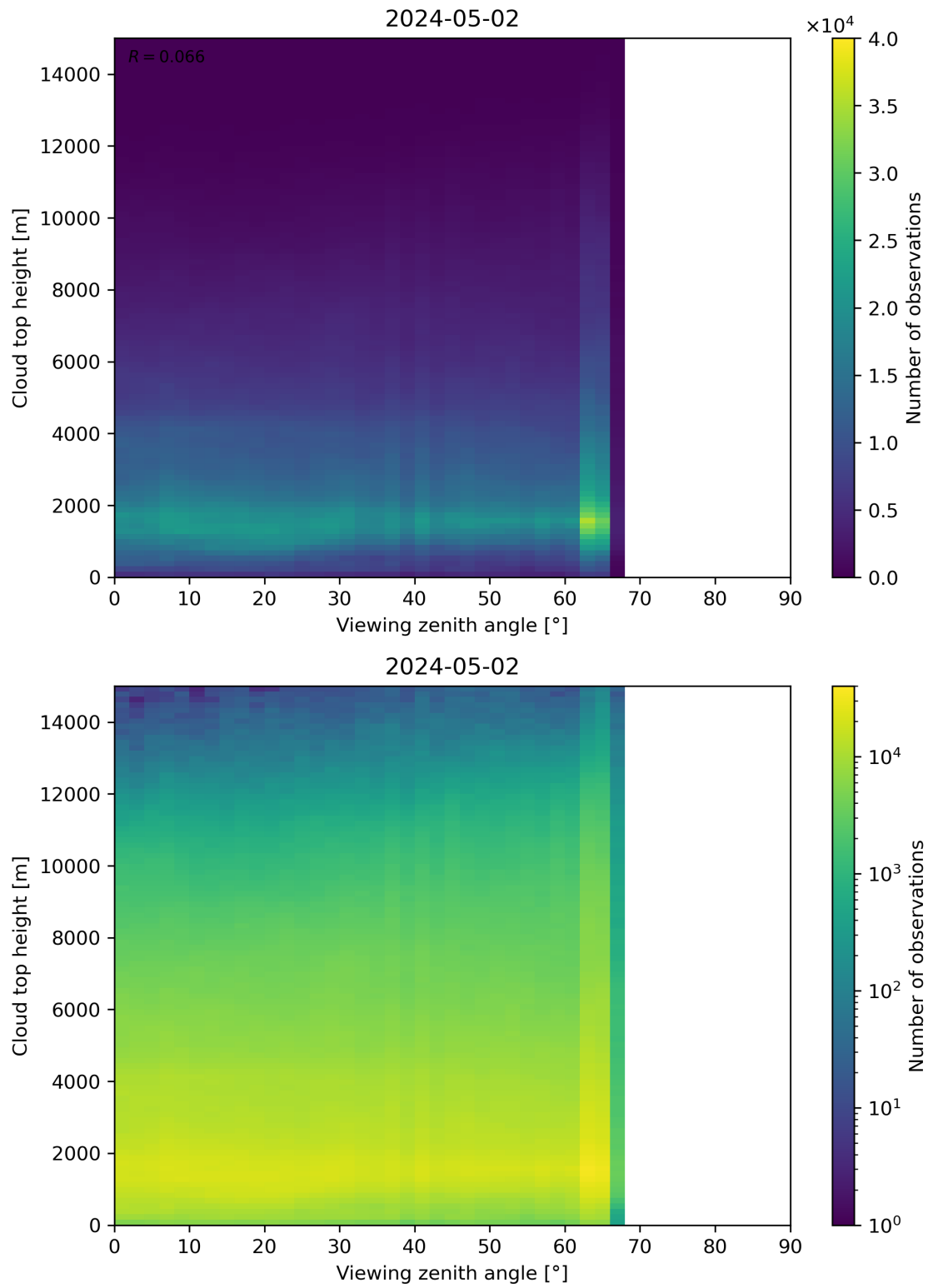
Figure 112: Scatter density plot of “Viewing zenith angle” against “Cloud top height” for 2024-05-02 to 2024-05-03.
