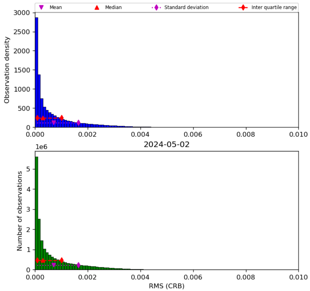
Figure 48: Histogram of “RMS (CRB)” for 2024-05-02 to 2024-05-03
