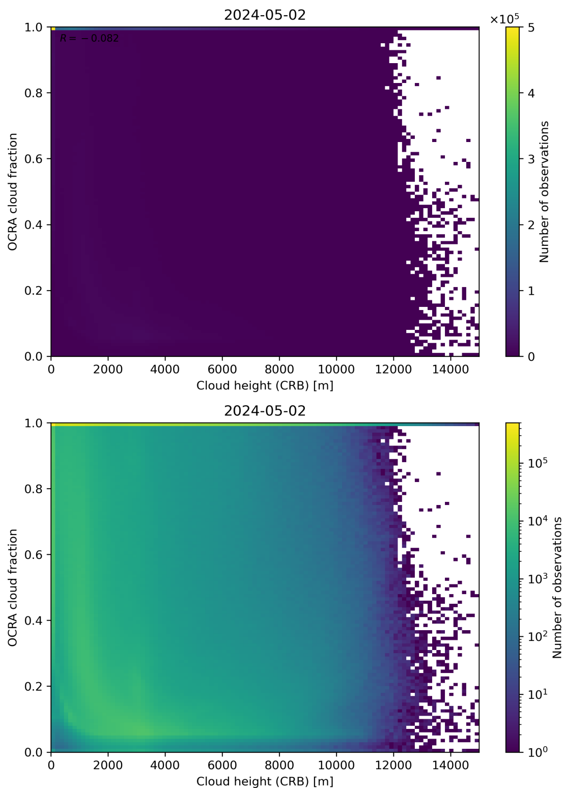
Figure 81: Scatter density plot of “Cloud height (CRB)” against “OCRA cloud fraction” for 2024-05-02 to 2024-05-03.
