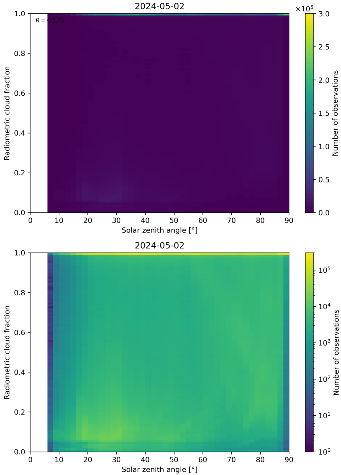
Figure 99: Scatter density plot of “Solar zenith angle” against “Radiometric cloud fraction” for 2024-05-02 to 2024-05-03.
