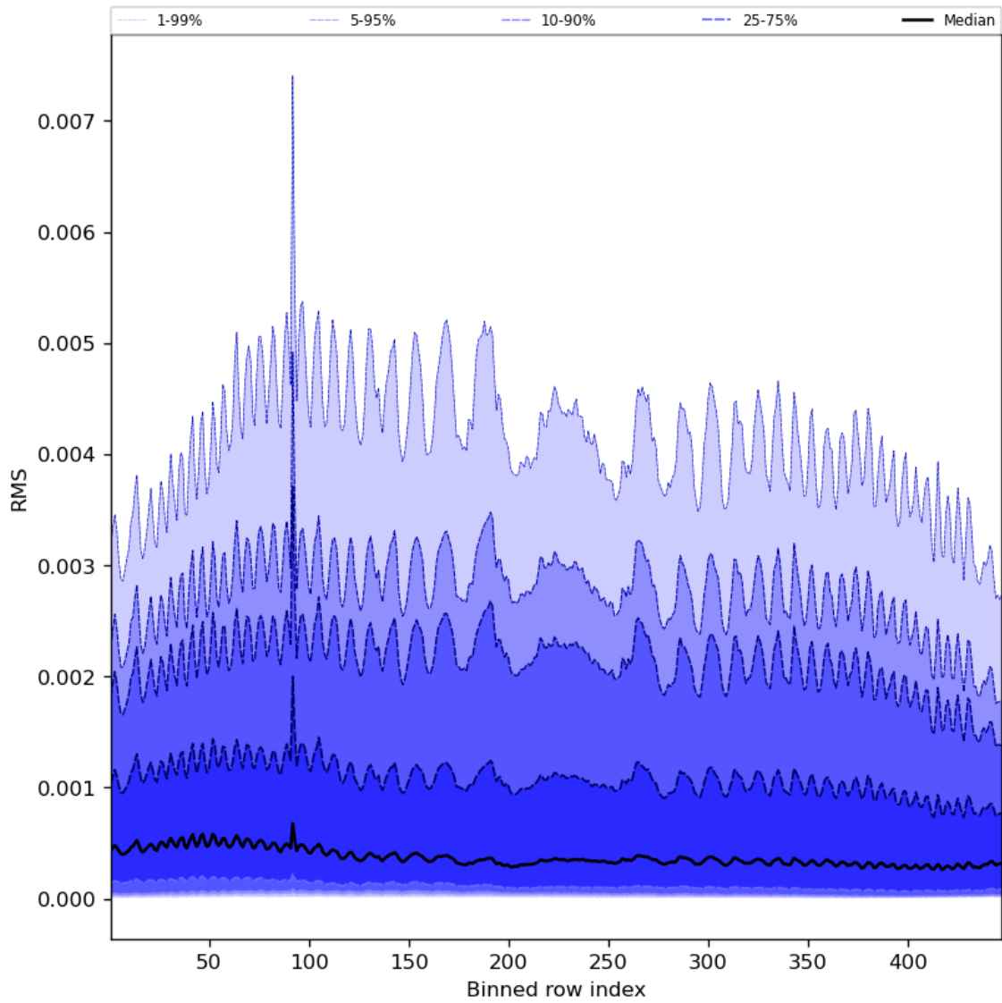
Figure 63: Along track statistics of “RMS” for 2024-05-02 to 2024-05-03
