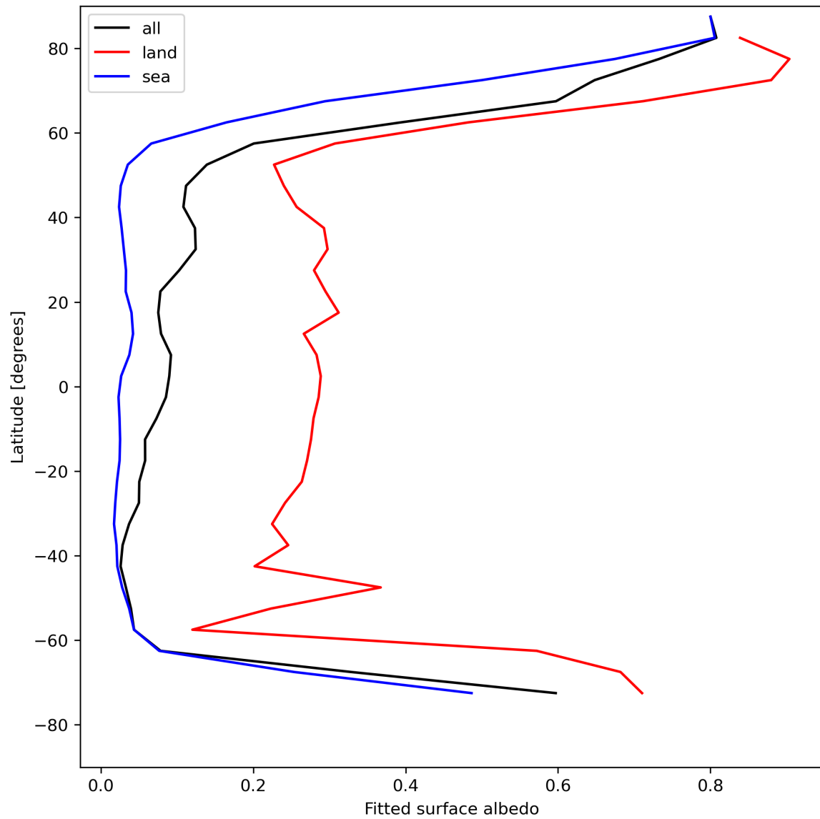
Figure 29: Zonal average of “Fitted surface albedo” for 2024-05-02 to 2024-05-03.
