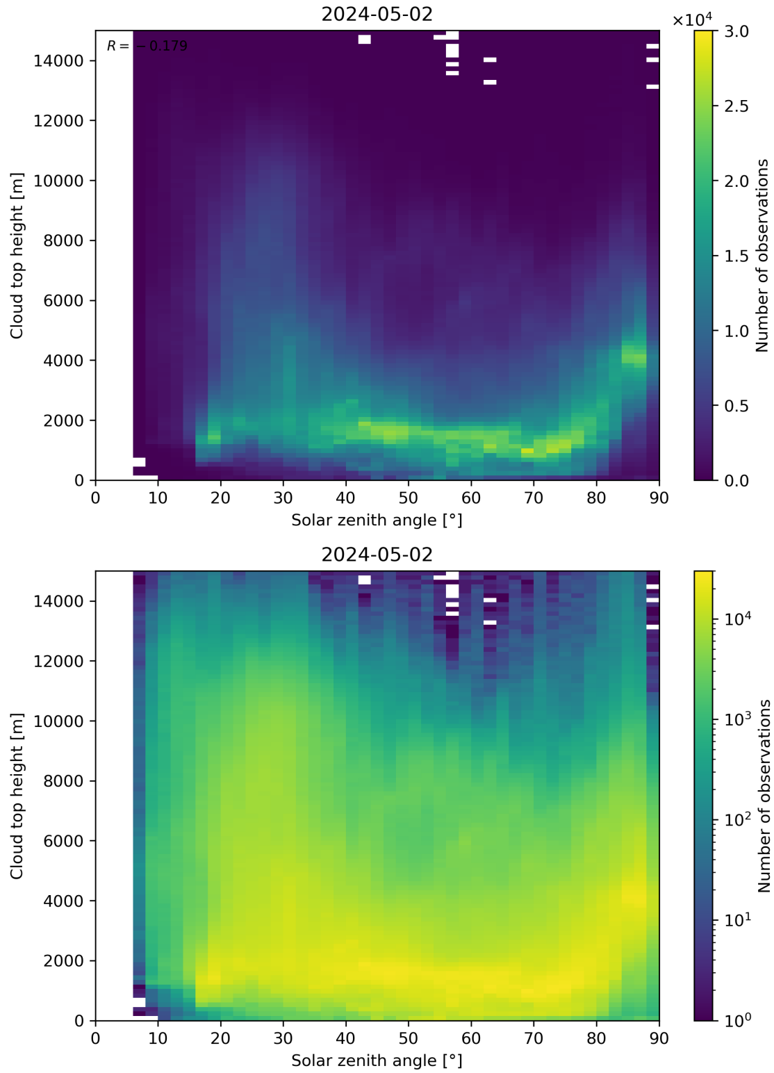
Figure 104: Scatter density plot of “Solar zenith angle” against “Cloud top height” for 2024-05-02 to 2024-05-03.
