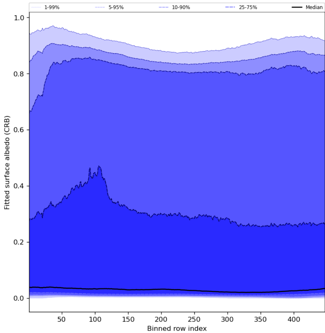
Figure 62: Along track statistics of “Fitted surface albedo (CRB)” for 2024-05-02 to 2024-05-03
