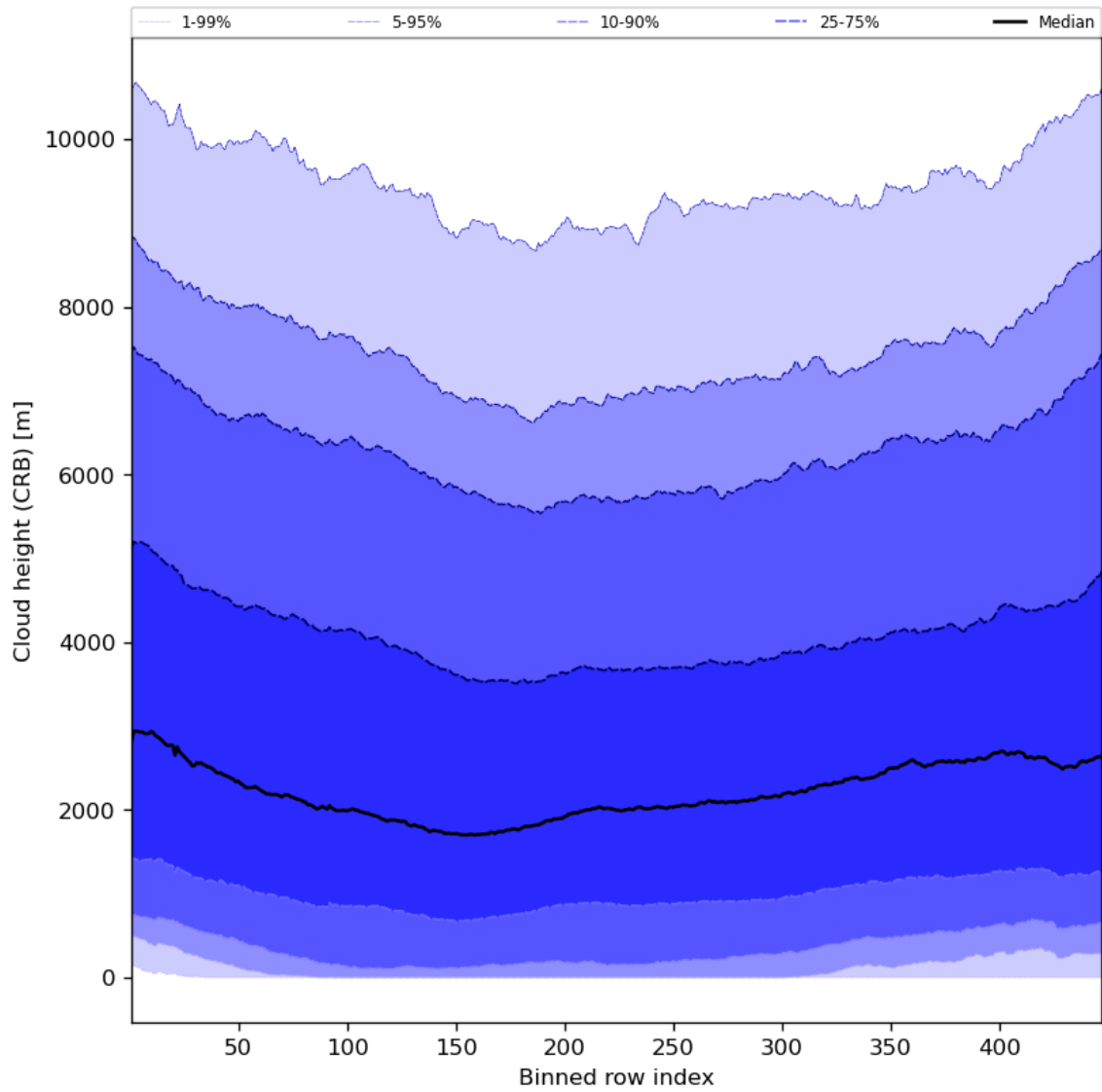
Figure 59: Along track statistics of “Cloud height (CRB)” for 2024-05-02 to 2024-05-03
