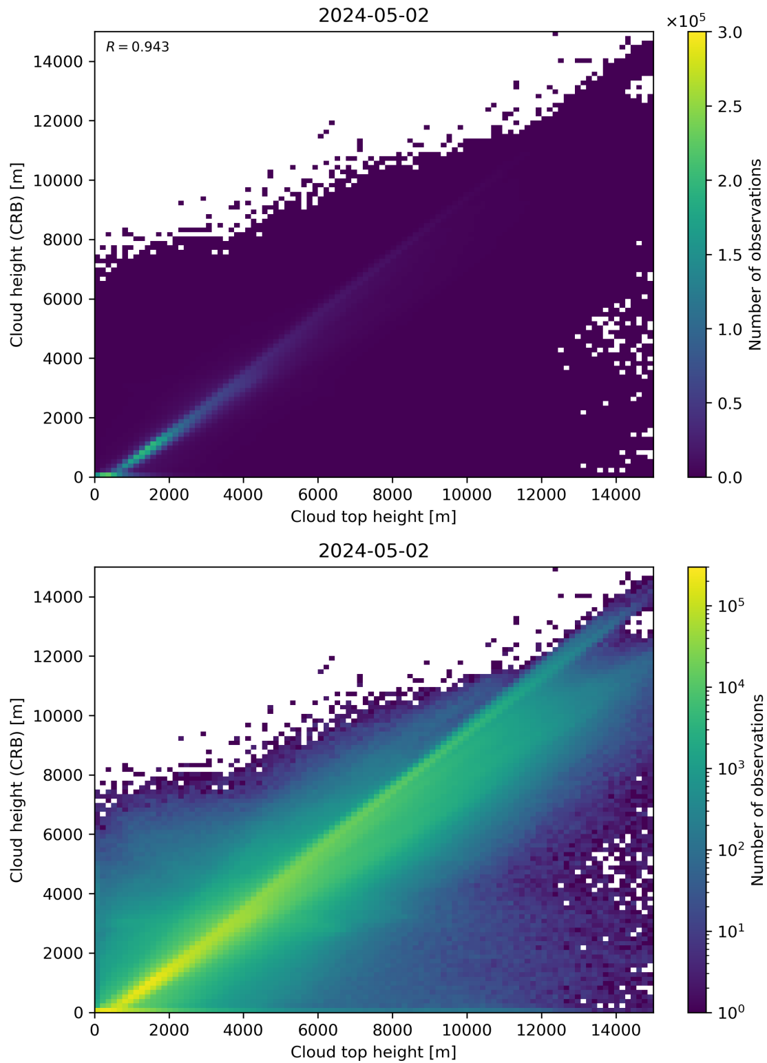
Figure 89: Scatter density plot of “Cloud top height” against “Cloud height (CRB)” for 2024-05-02 to 2024-05-03.
