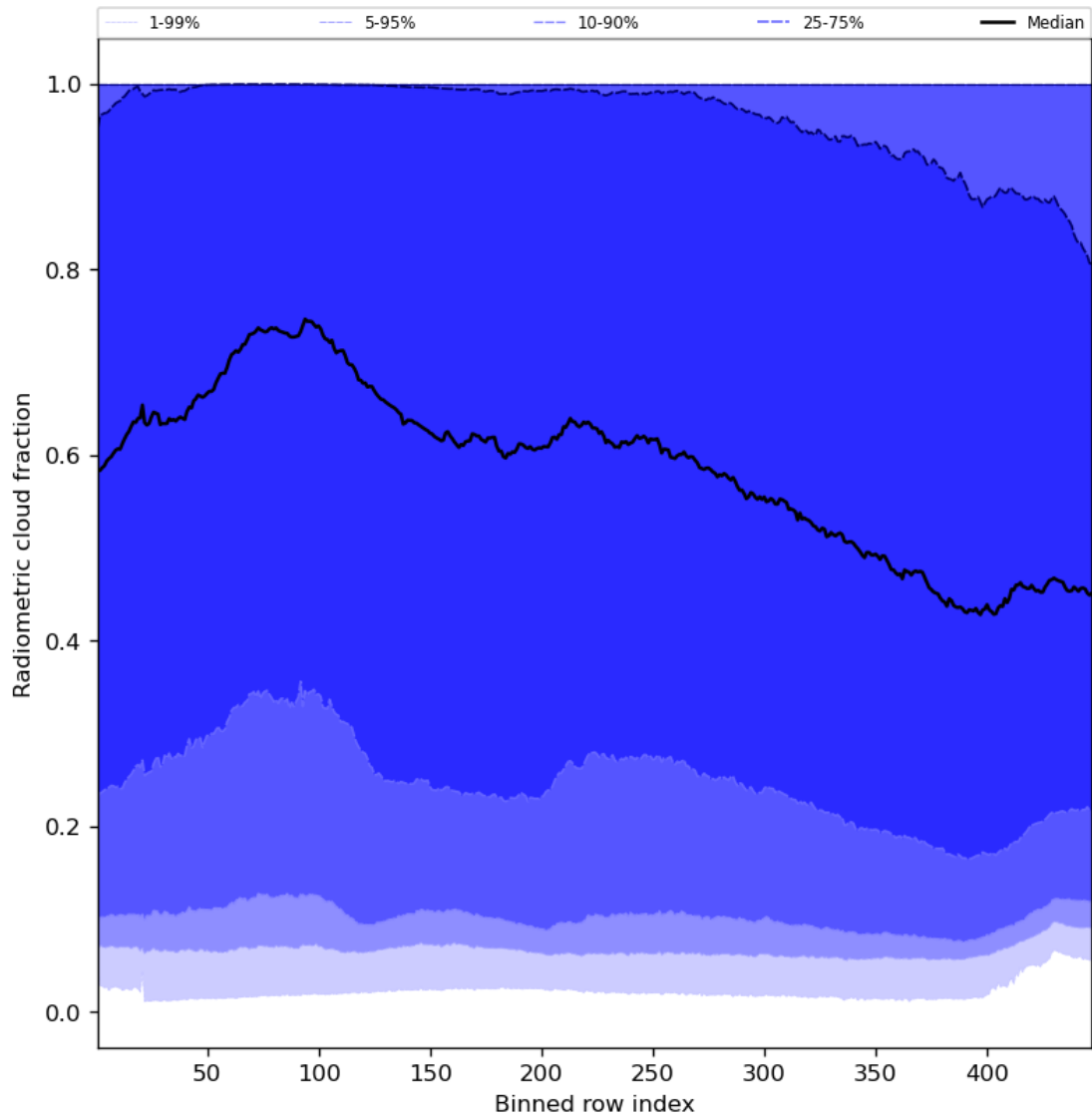
Figure 55: Along track statistics of “Radiometric cloud fraction” for 2024-05-02 to 2024-05-04
