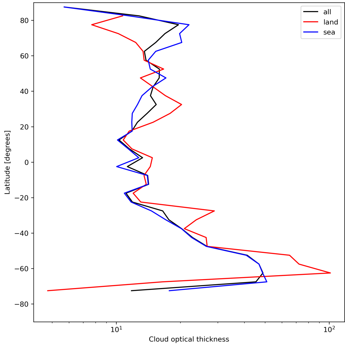
Figure 25: Zonal average of “Cloud optical thickness” for 2024-05-02 to 2024-05-04.
