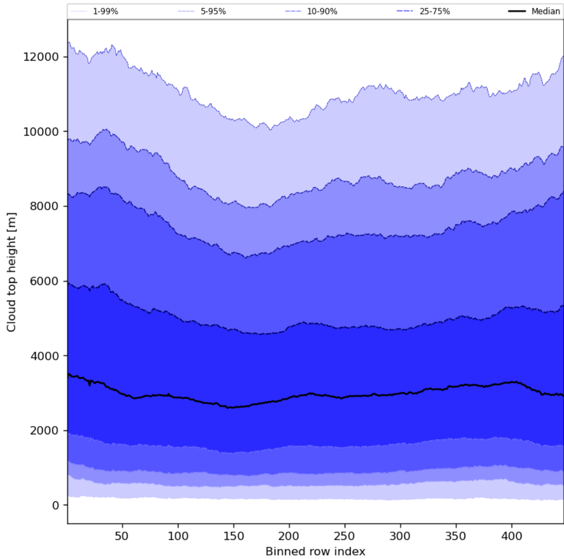
Figure 56: Along track statistics of “Cloud top height” for 2024-05-02 to 2024-05-04
