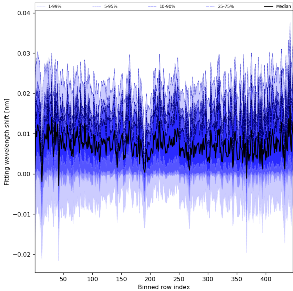
Figure 65: Along track statistics of “Fitting wavelength shift” for 2024-05-02 to 2024-05-04
