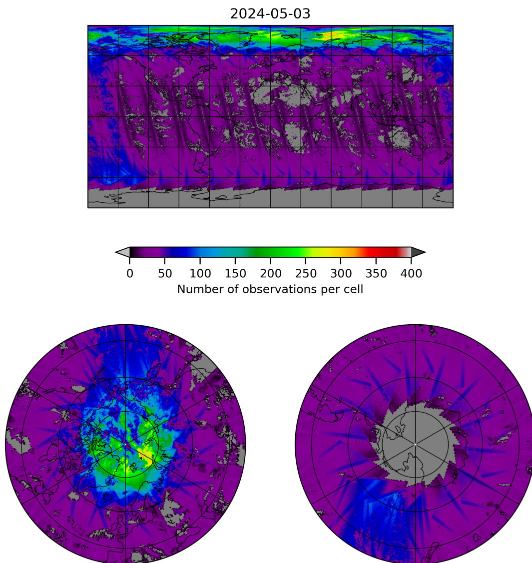
Figure 21: Map of the number of observations for 2024-05-02 to 2024-05-04
