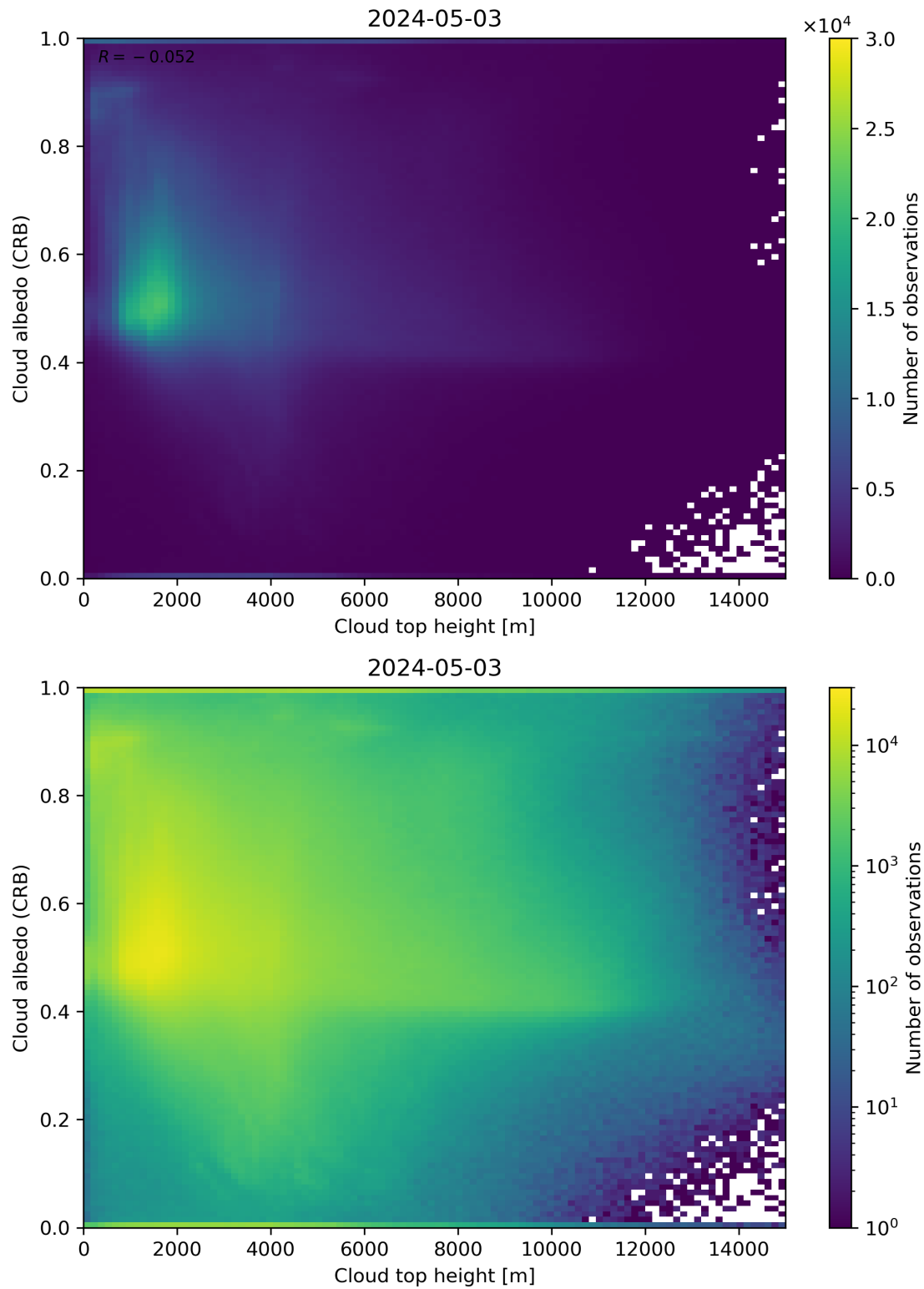
Figure 86: Scatter density plot of “Cloud top height” against “Cloud albedo (CRB)” for 2024-05-02 to 2024-05-04.
