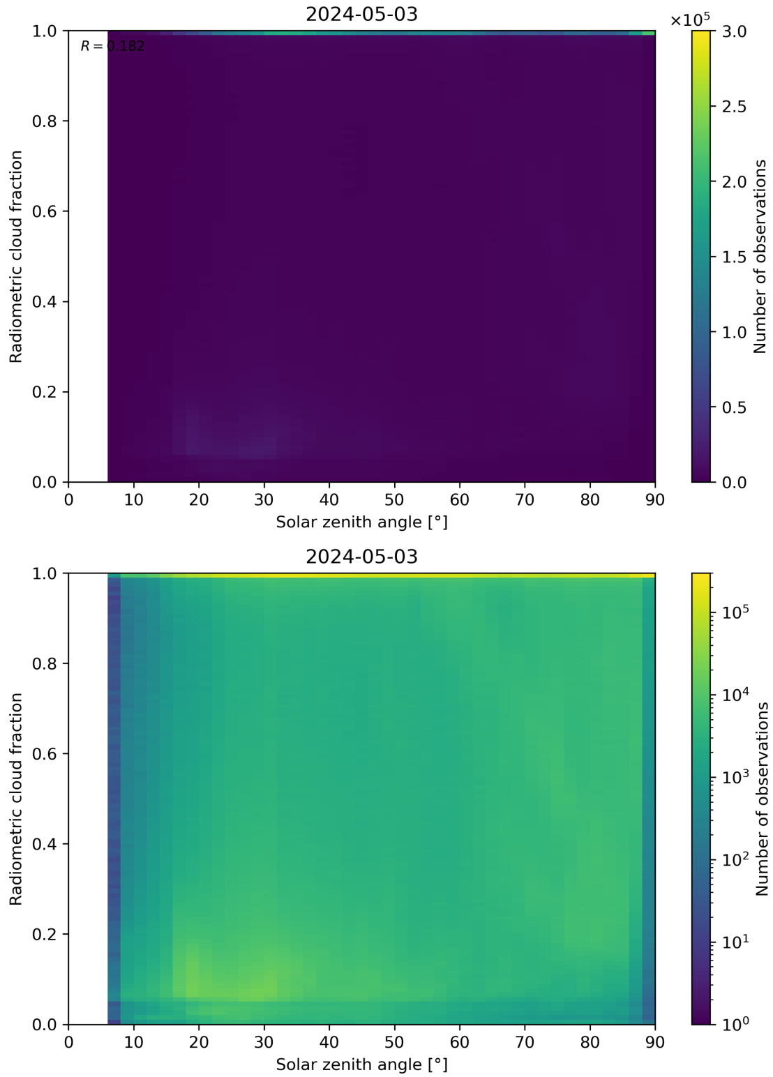
Figure 99: Scatter density plot of “Solar zenith angle” against “Radiometric cloud fraction” for 2024-05-02 to 2024-05-04.
