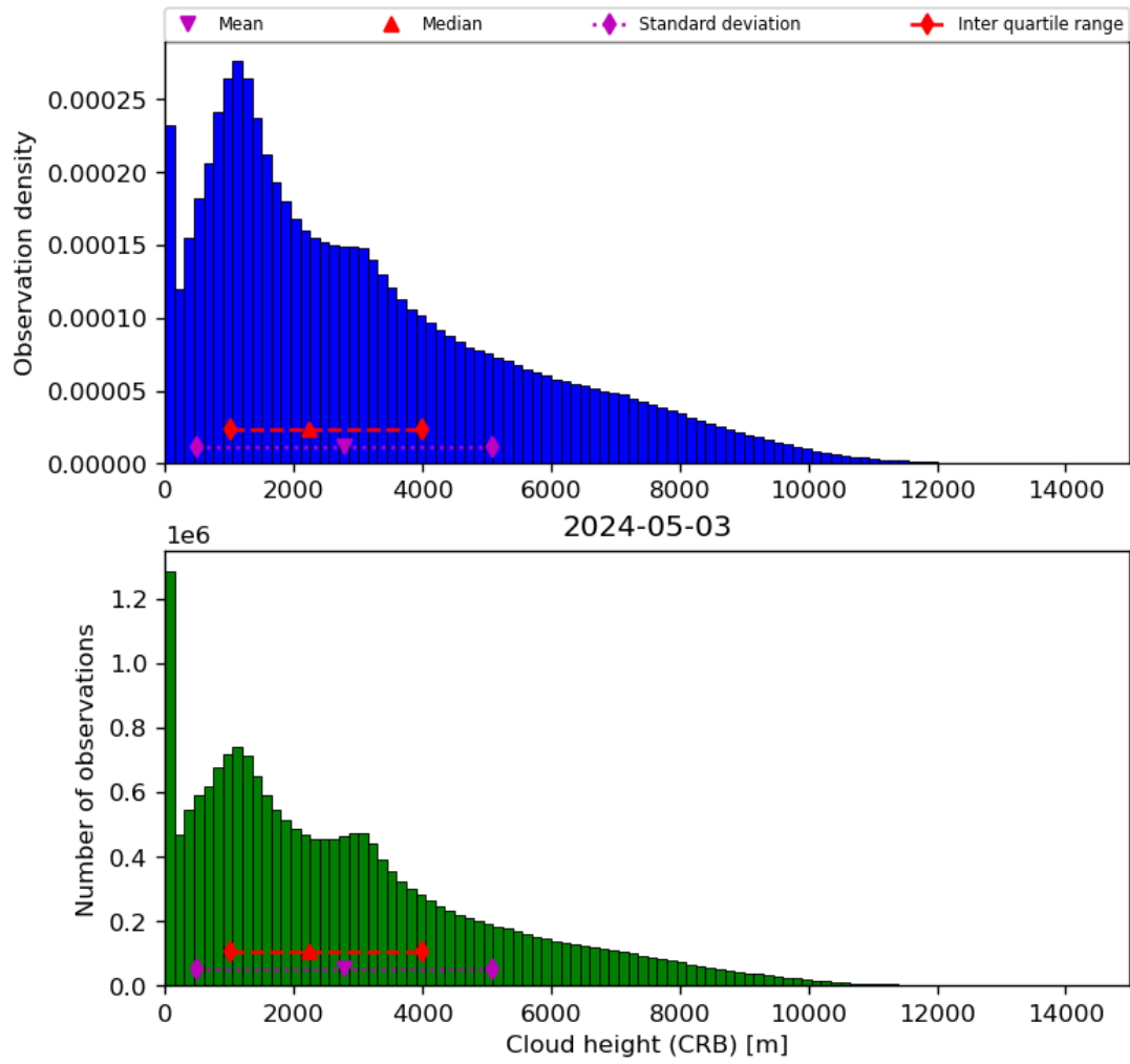
Figure 43: Histogram of “Cloud height (CRB)” for 2024-05-02 to 2024-05-04
