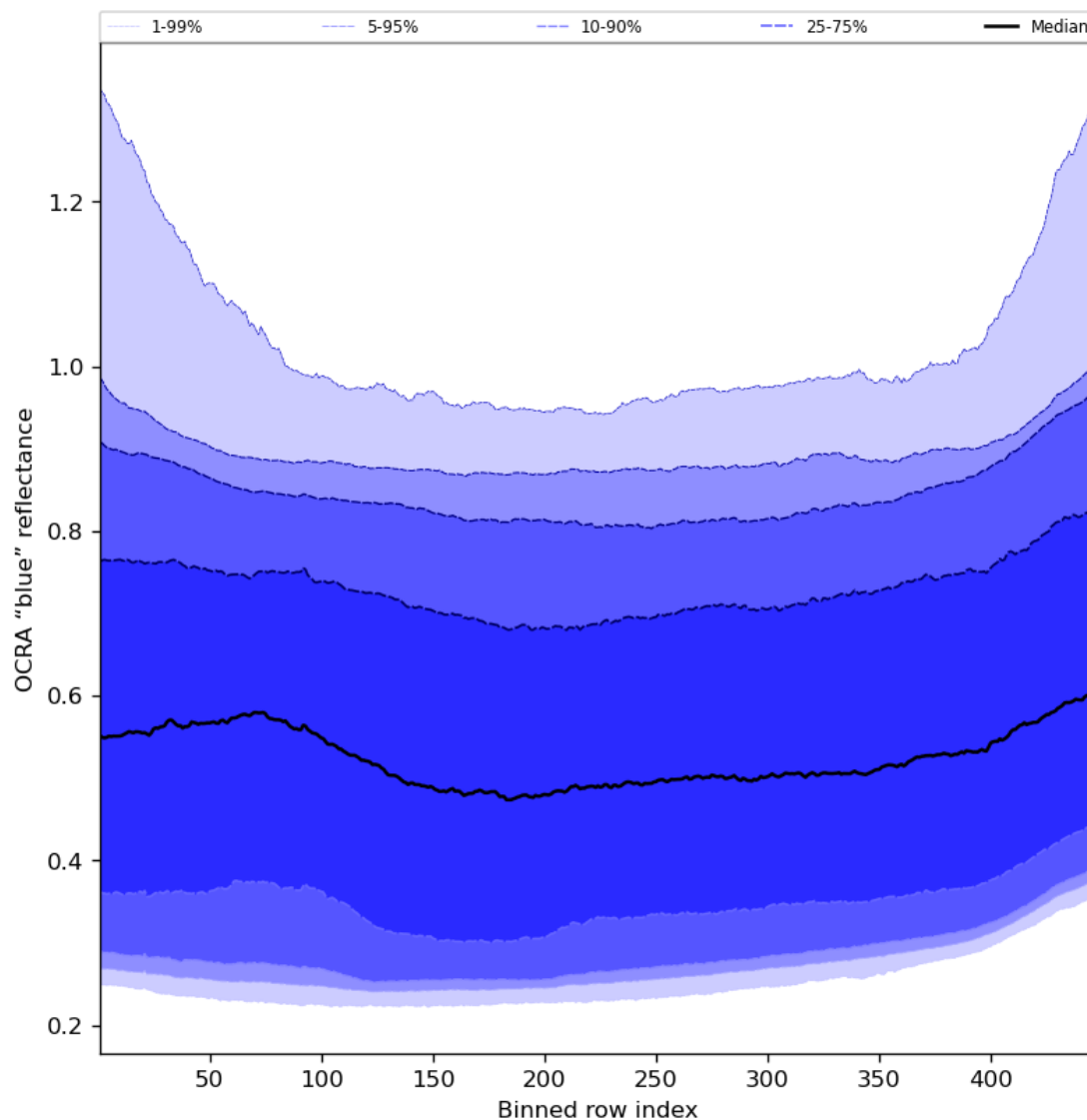
Figure 67: Along track statistics of “OCRA “blue” reflectance” for 2024-05-02 to 2024-05-04
