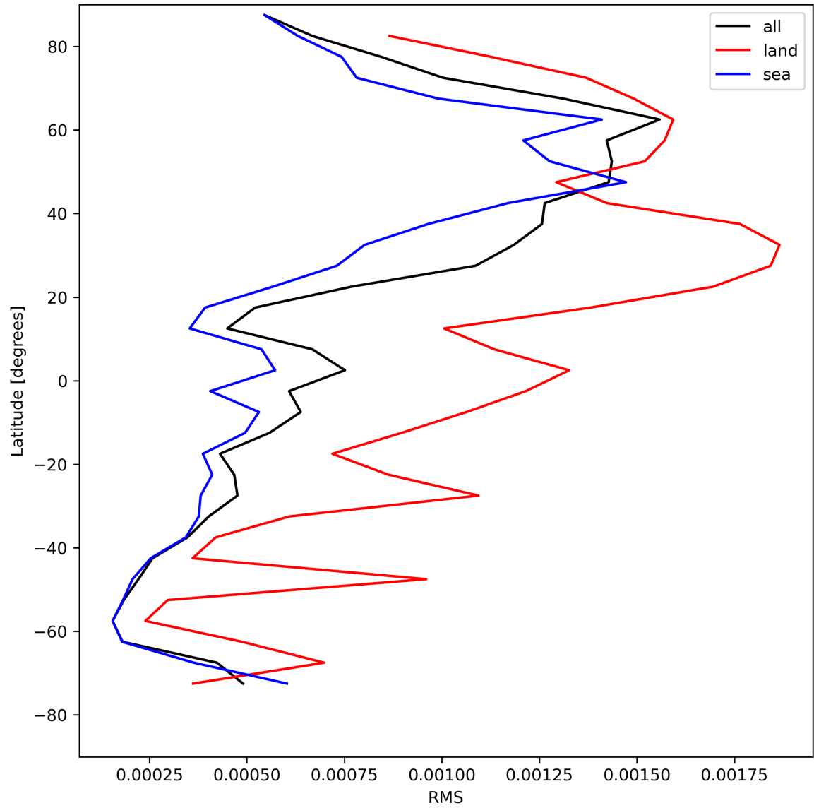
Figure 31: Zonal average of “RMS” for 2024-05-02 to 2024-05-04.
