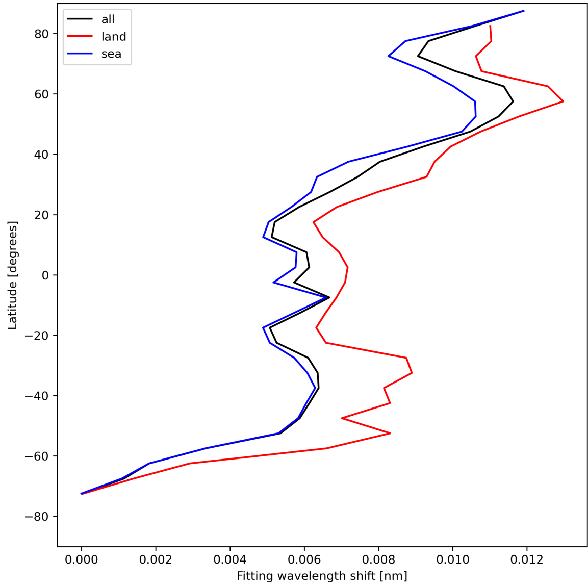
Figure 33: Zonal average of “Fitting wavelength shift” for 2024-05-02 to 2024-05-04.
