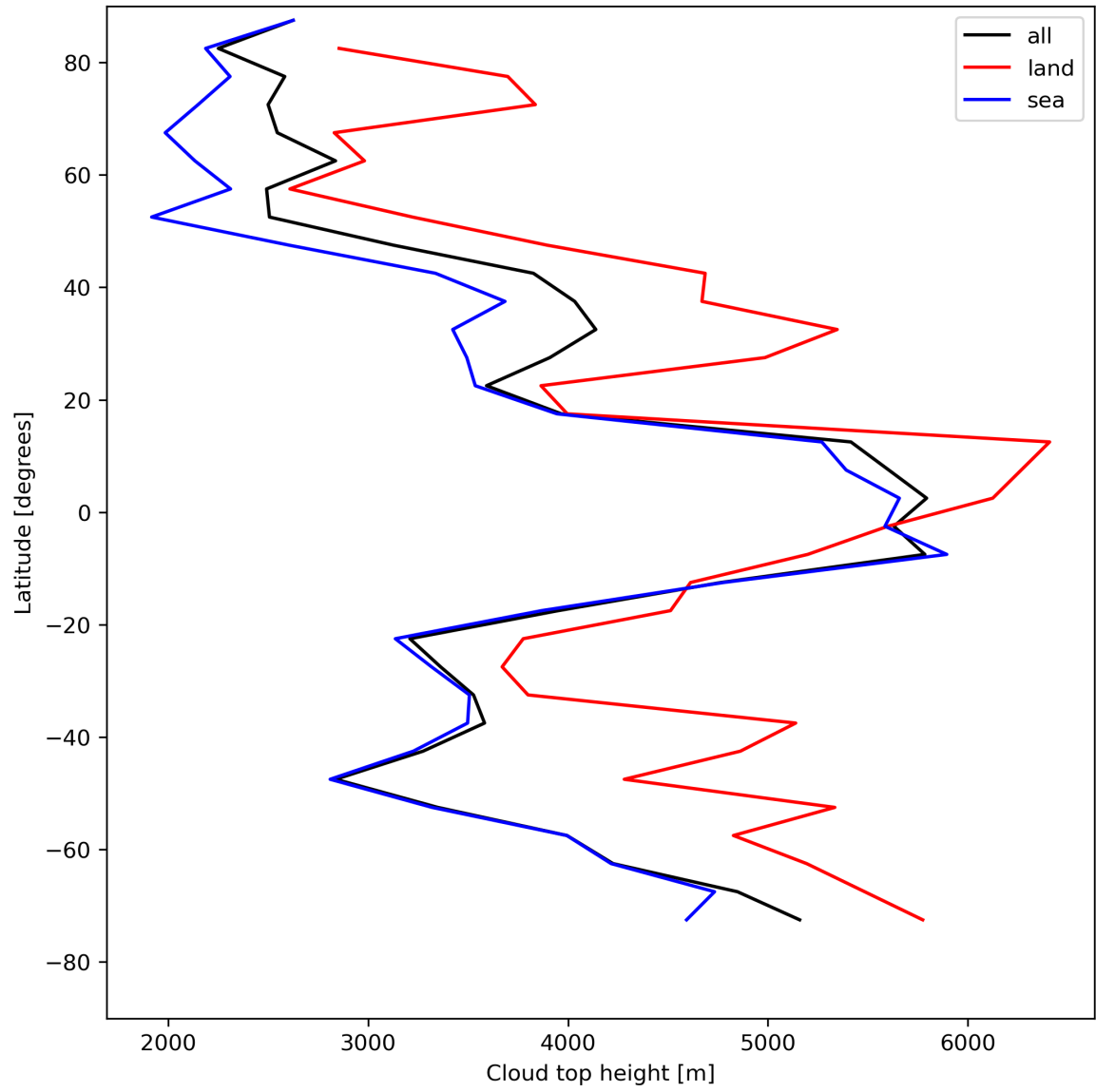
Figure 24: Zonal average of “Cloud top height” for 2024-05-02 to 2024-05-04.
