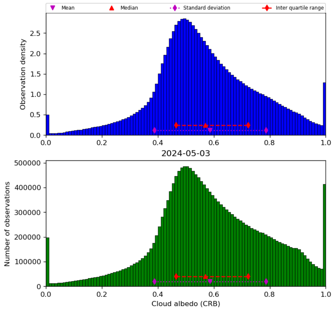
Figure 44: Histogram of “Cloud albedo (CRB)” for 2024-05-02 to 2024-05-04
