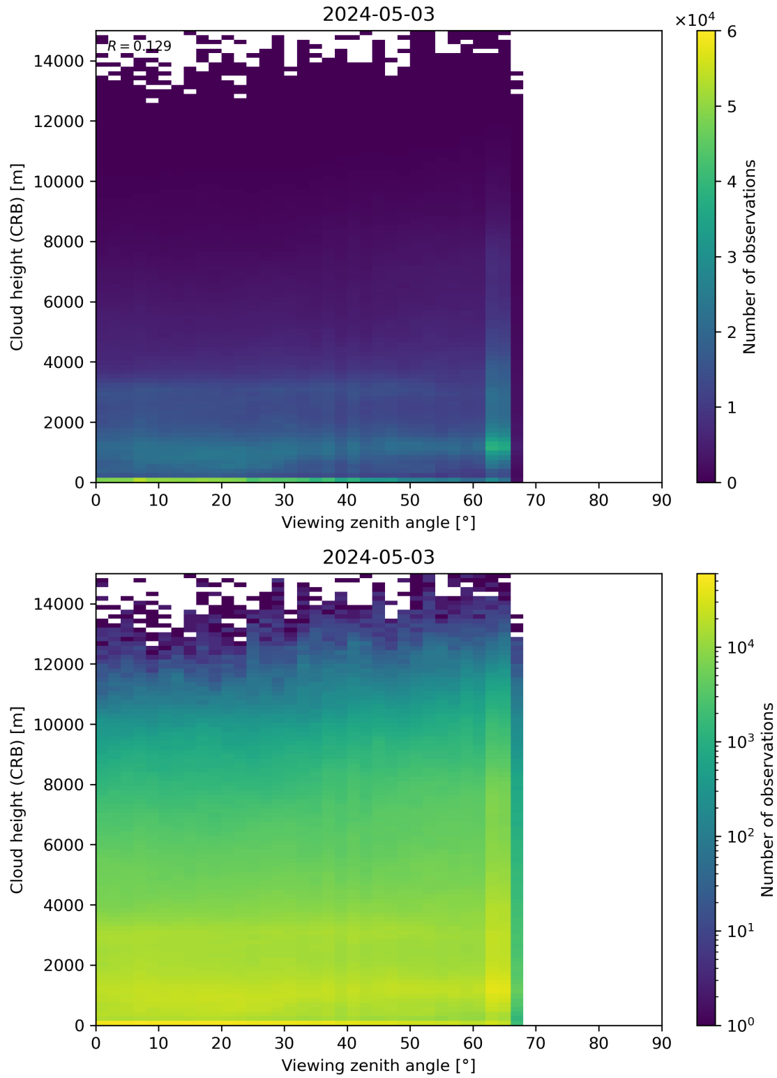
Figure 110: Scatter density plot of “Viewing zenith angle” against “Cloud height (CRB)” for 2024-05-02 to 2024-05-04.
