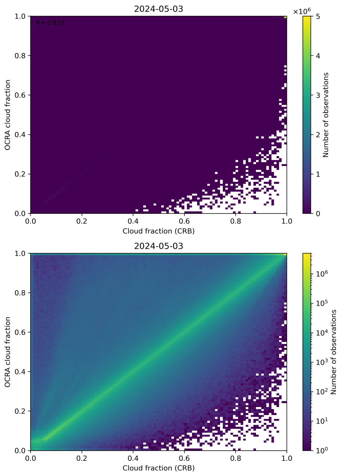
Figure 78: Scatter density plot of “Cloud fraction (CRB)” against “OCRA cloud fraction” for 2024-05-02 to 2024-05-04.
