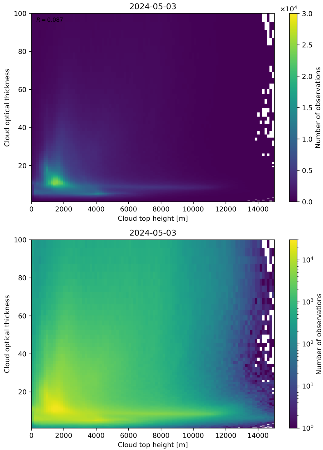
Figure 90: Scatter density plot of “Cloud top height” against “Cloud optical thickness” for 2024-05-02 to 2024-05-04.
