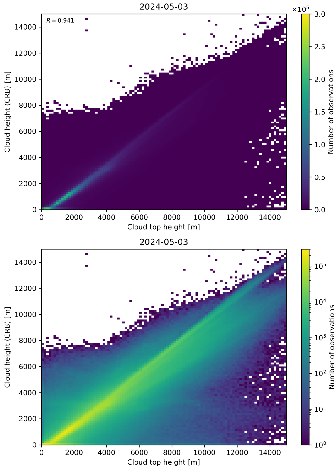
Figure 89: Scatter density plot of “Cloud top height” against “Cloud height (CRB)” for 2024-05-02 to 2024-05-04.
