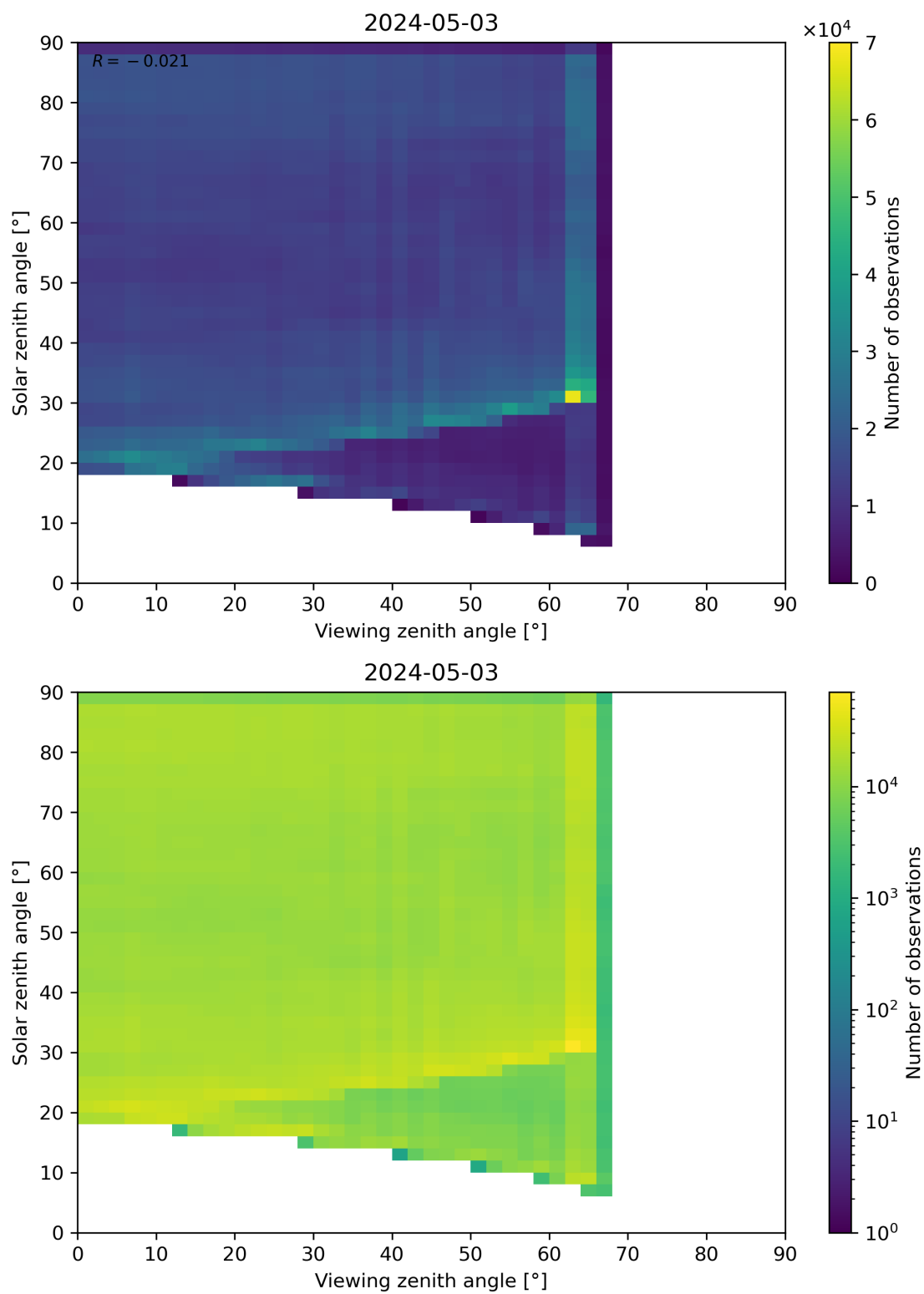
Figure 114: Scatter density plot of “Viewing zenith angle” against “Solar zenith angle” for 2024-05-02 to 2024-05-04.
