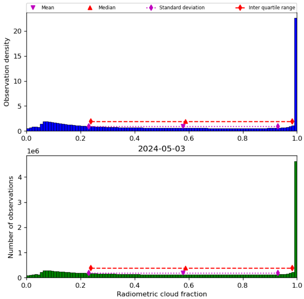
Figure 39: Histogram of “Radiometric cloud fraction” for 2024-05-02 to 2024-05-04
