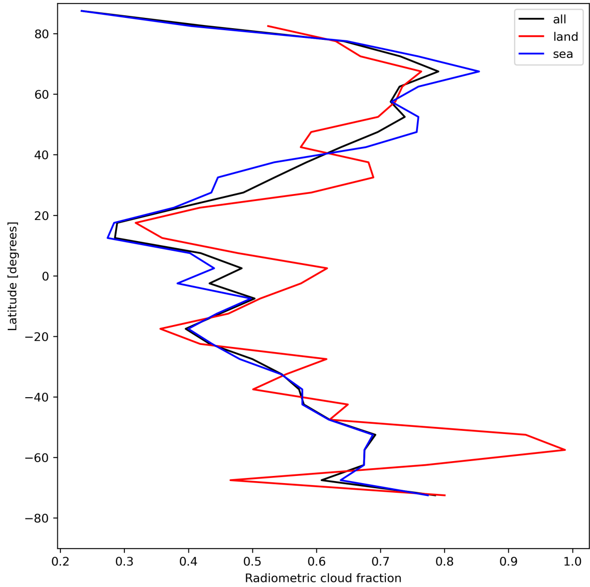
Figure 23: Zonal average of “Radiometric cloud fraction” for 2024-05-02 to 2024-05-04.
