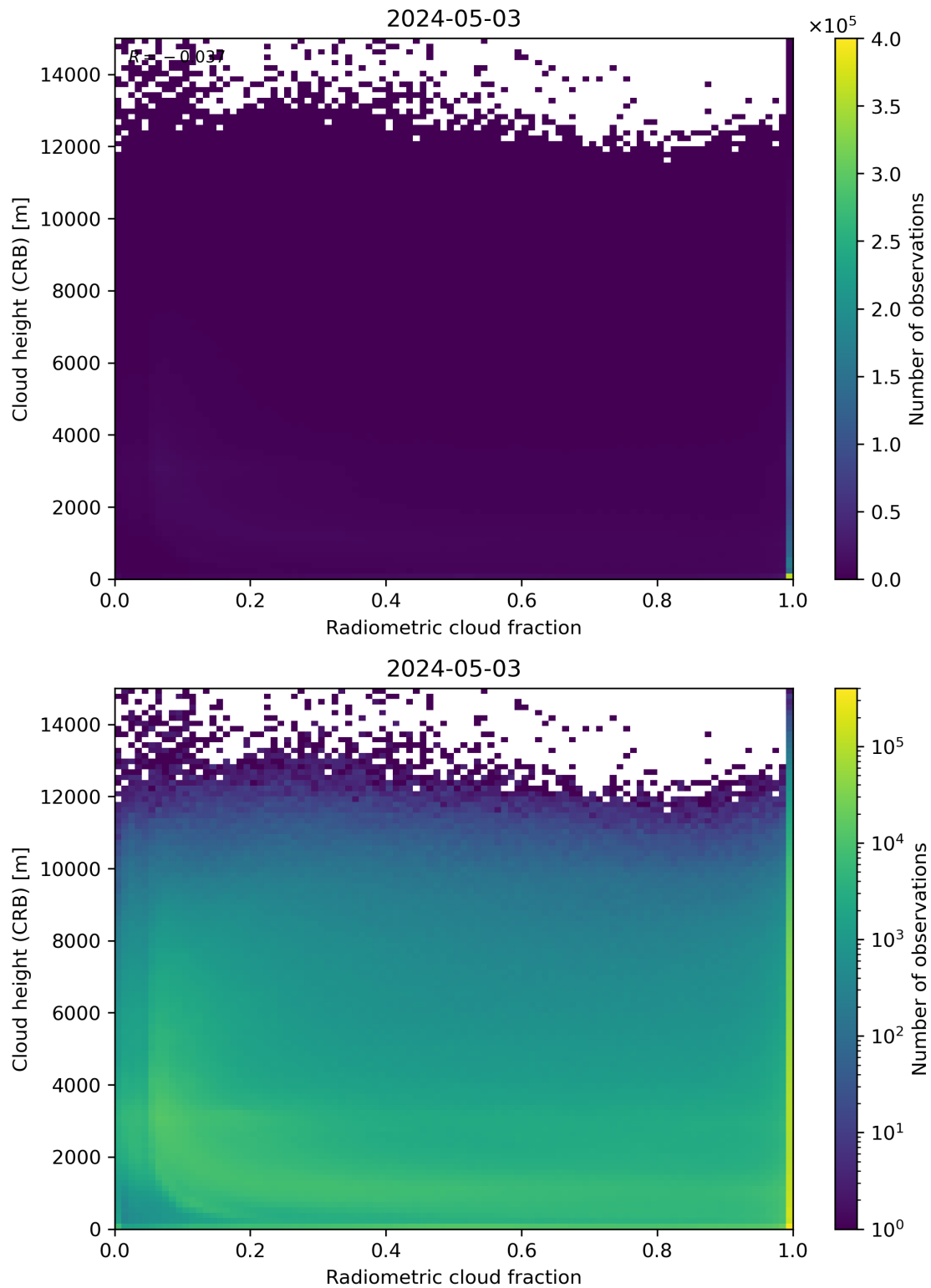
Figure 74: Scatter density plot of “Radiometric cloud fraction” against “Cloud height (CRB)” for 2024-05-02 to 2024-05-04.
