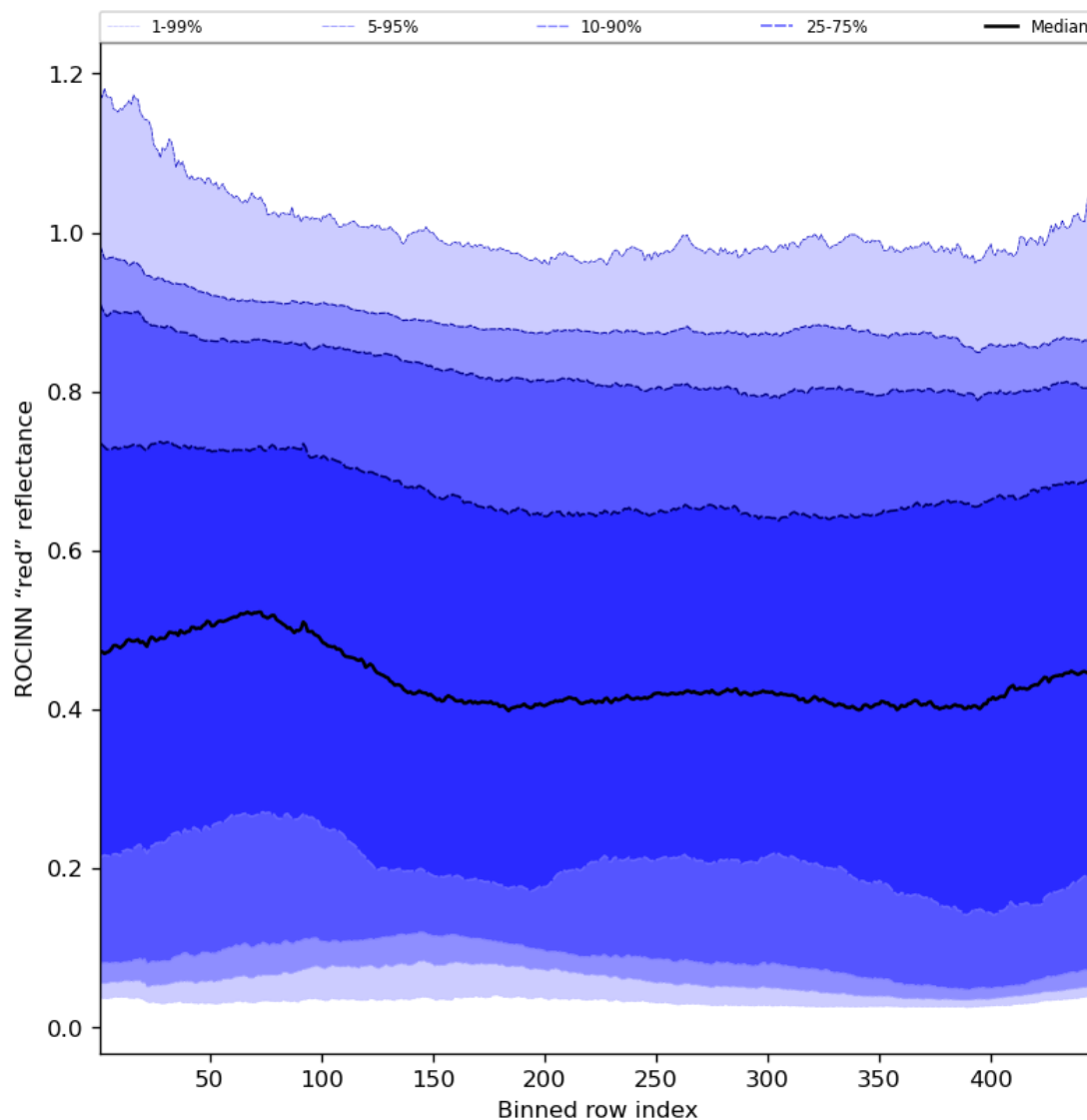
Figure 69: Along track statistics of “ROCINN “red” reflectance” for 2024-05-02 to 2024-05-04
