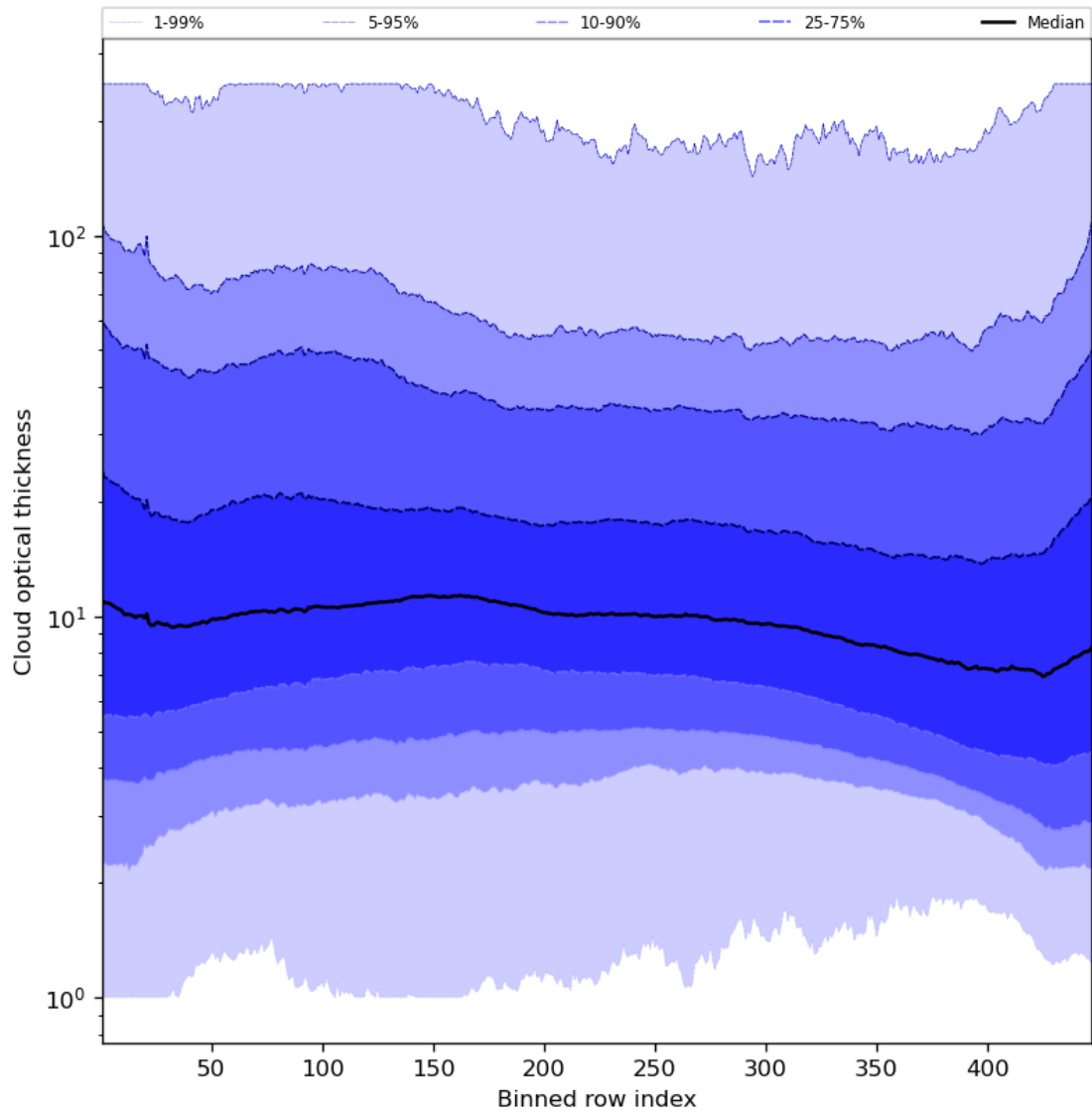
Figure 57: Along track statistics of “Cloud optical thickness” for 2024-05-02 to 2024-05-04
