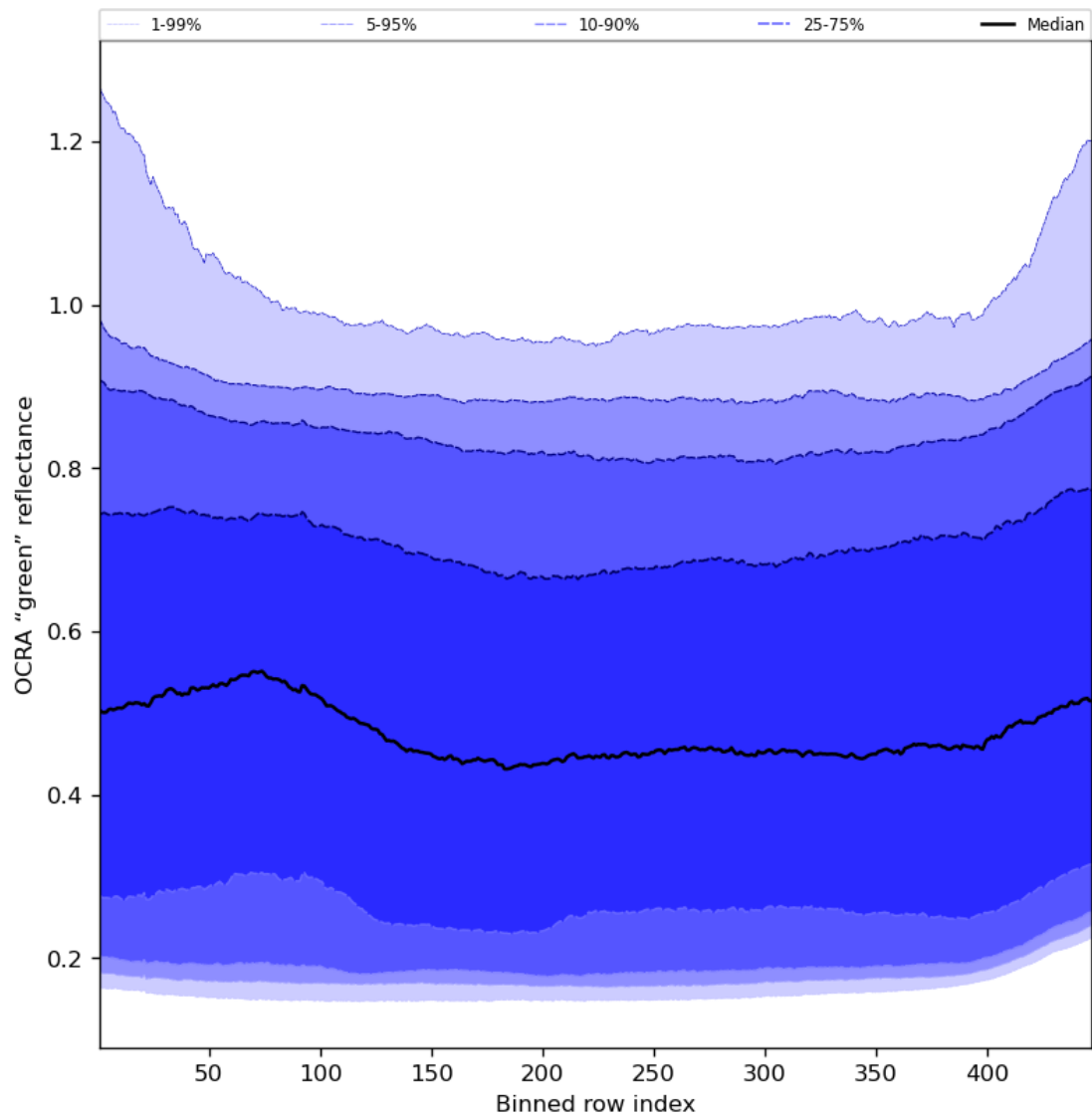
Figure 68: Along track statistics of "OCRA "green" reflectance" for 2024-05-02 to 2024-05-04
