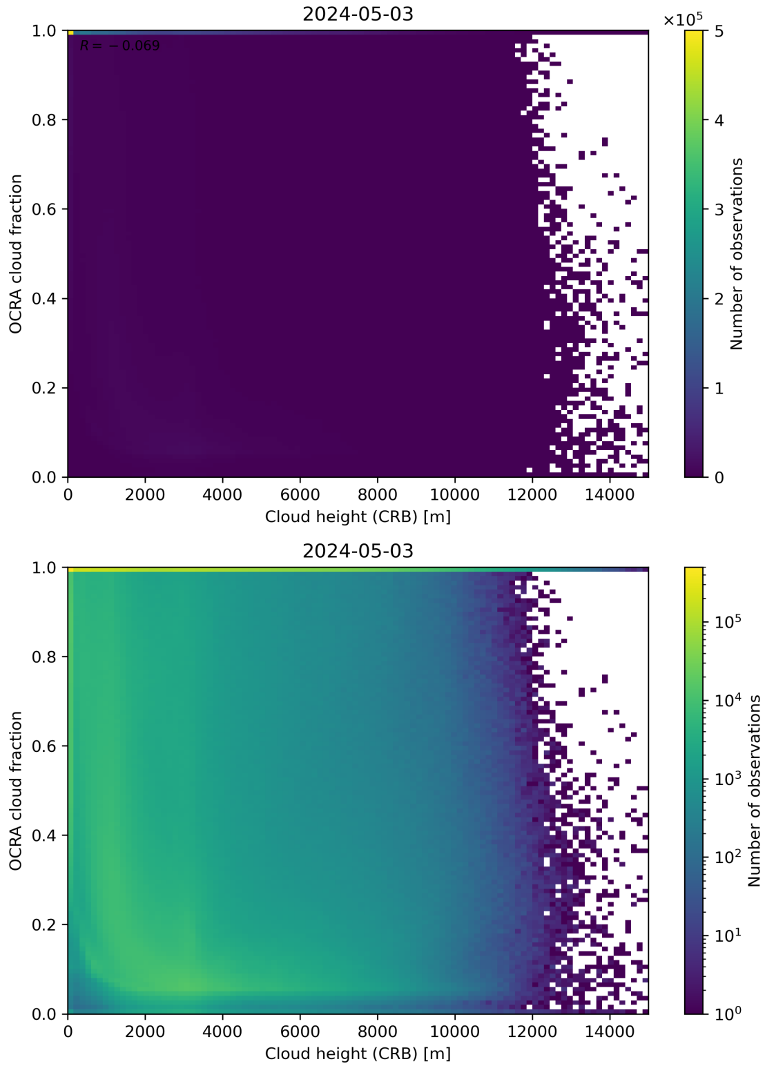
Figure 81: Scatter density plot of “Cloud height (CRB)” against “OCRA cloud fraction” for 2024-05-02 to 2024-05-04.
