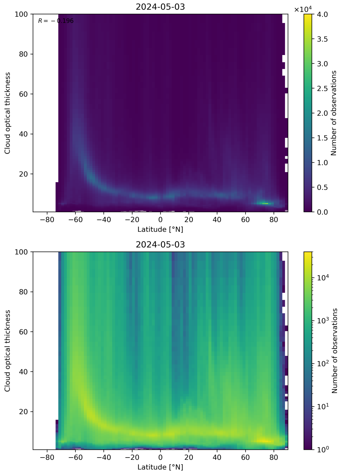
Figure 96: Scatter density plot of “Latitude” against “Cloud optical thickness” for 2024-05-02 to 2024-05-04.
