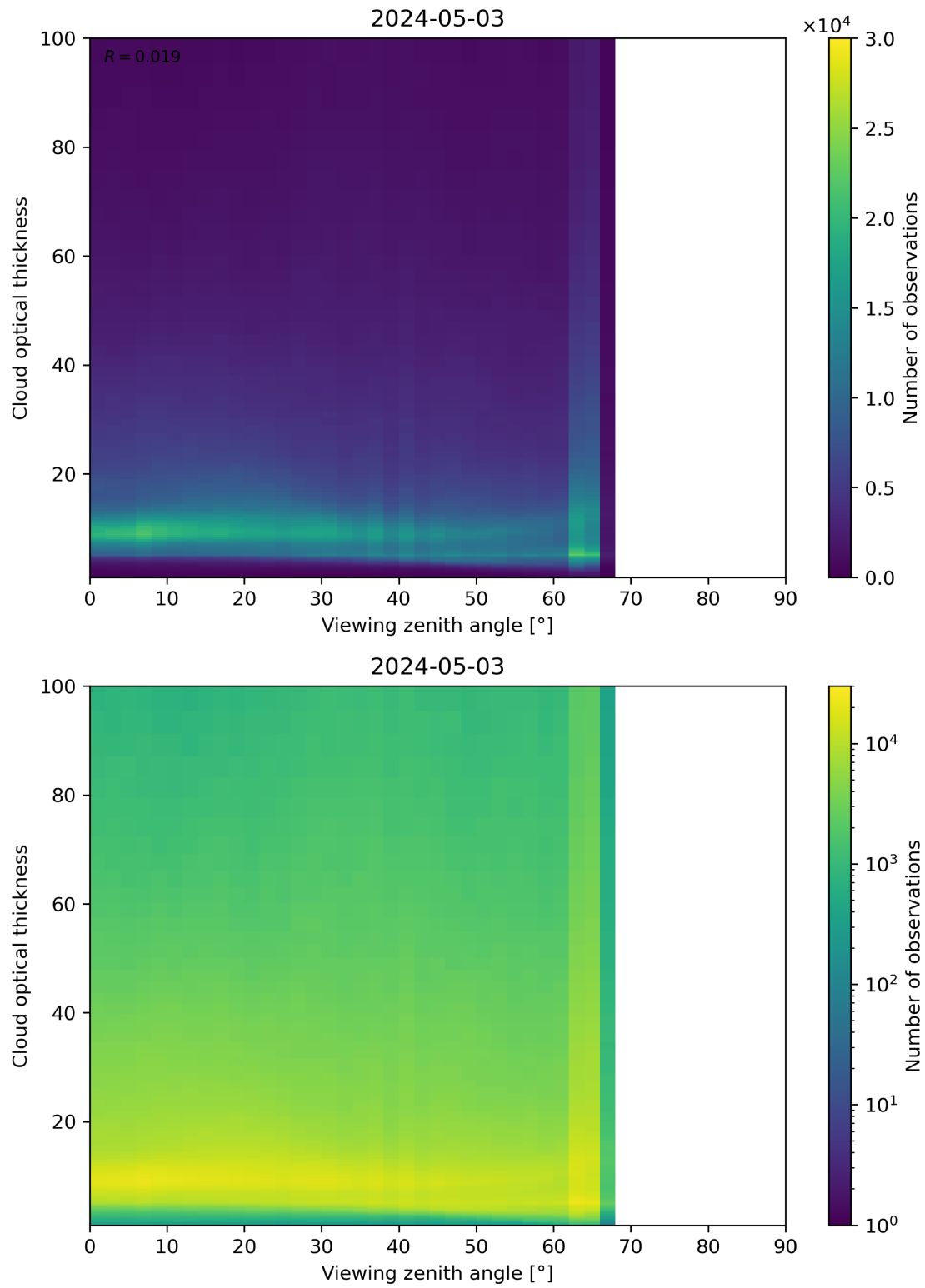
Figure 111: Scatter density plot of “Viewing zenith angle” against “Cloud optical thickness” for 2024-05-02 to 2024-05-04.
