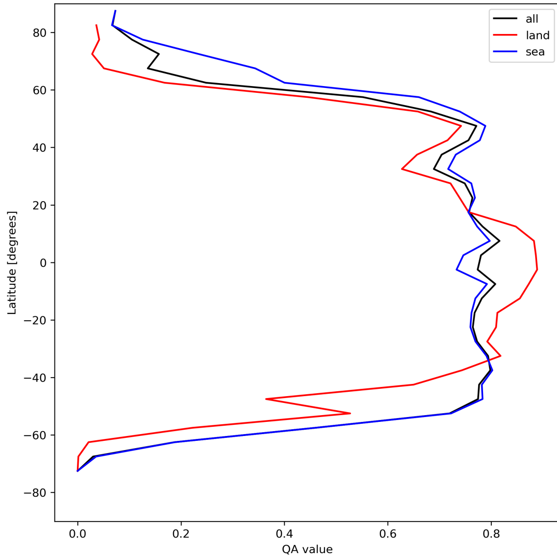
Figure 22: Zonal average of “QA value” for 2024-05-02 to 2024-05-04.
