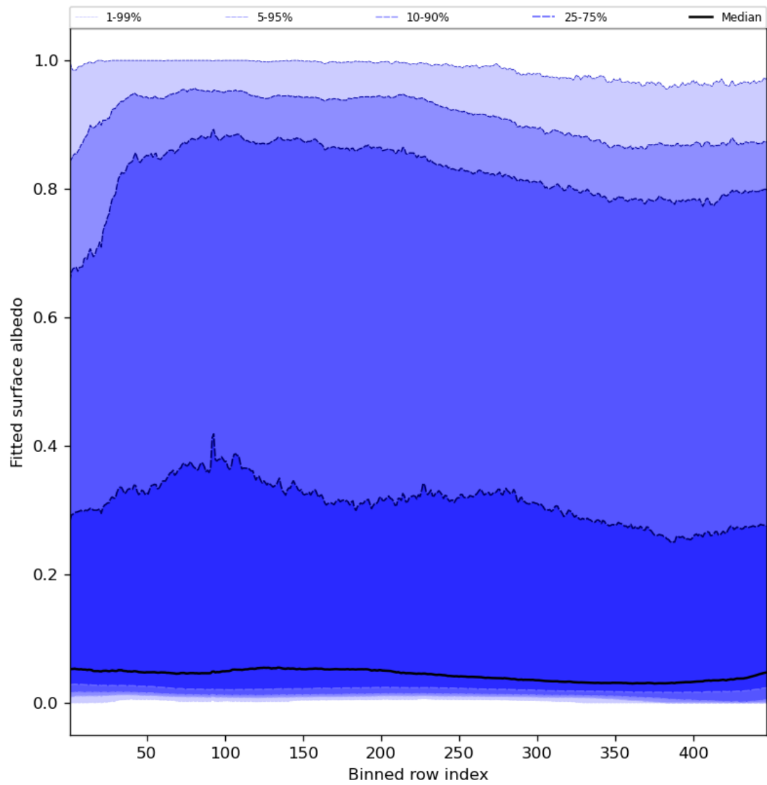
Figure 61: Along track statistics of “Fitted surface albedo” for 2024-05-02 to 2024-05-04
