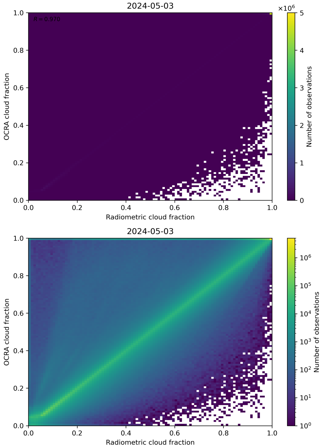
Figure 72: Scatter density plot of “Radiometric cloud fraction” against “OCRA cloud fraction” for 2024-05-02 to 2024-05-04.
