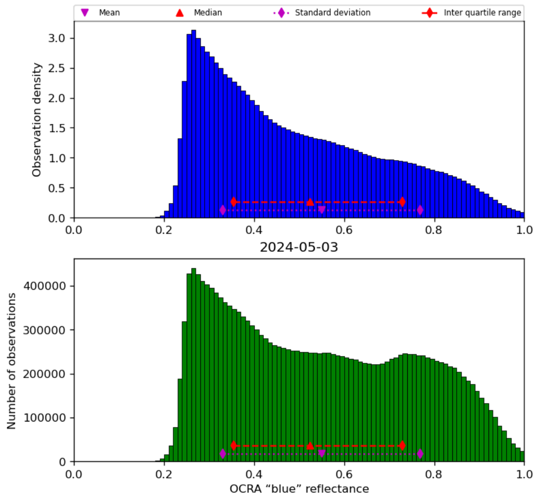
Figure 51: Histogram of “OCRA “blue” reflectance” for 2024-05-02 to 2024-05-04
