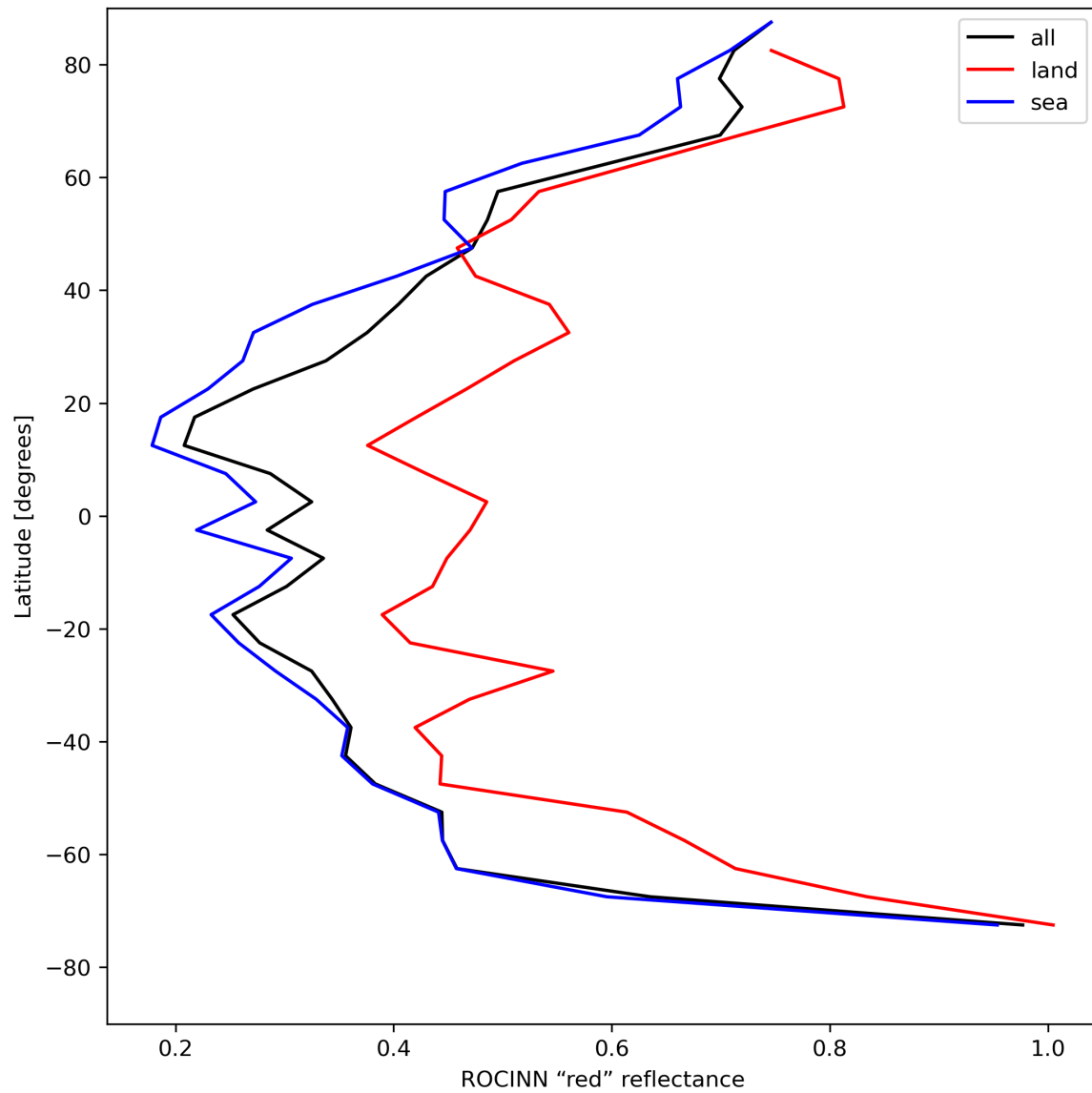
Figure 37: Zonal average of “ROCINN “red” reflectance” for 2024-05-02 to 2024-05-04.
