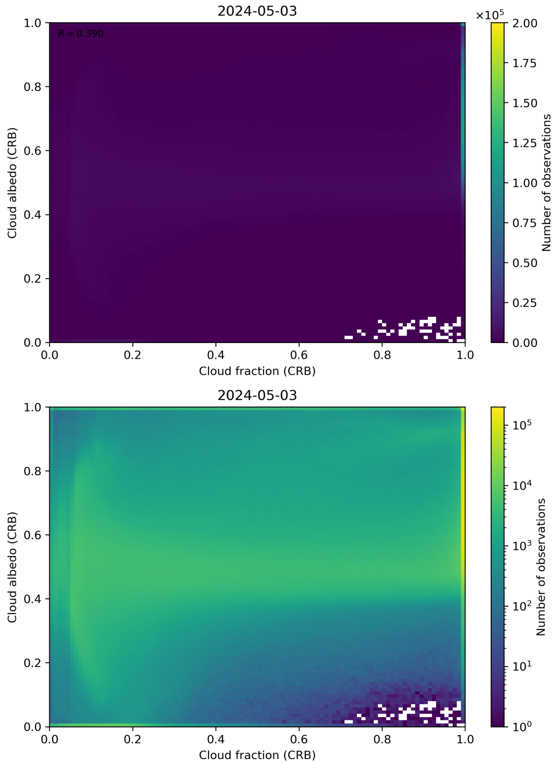
Figure 77: Scatter density plot of “Cloud fraction (CRB)” against “Cloud albedo (CRB)” for 2024-05-02 to 2024-05-04.
