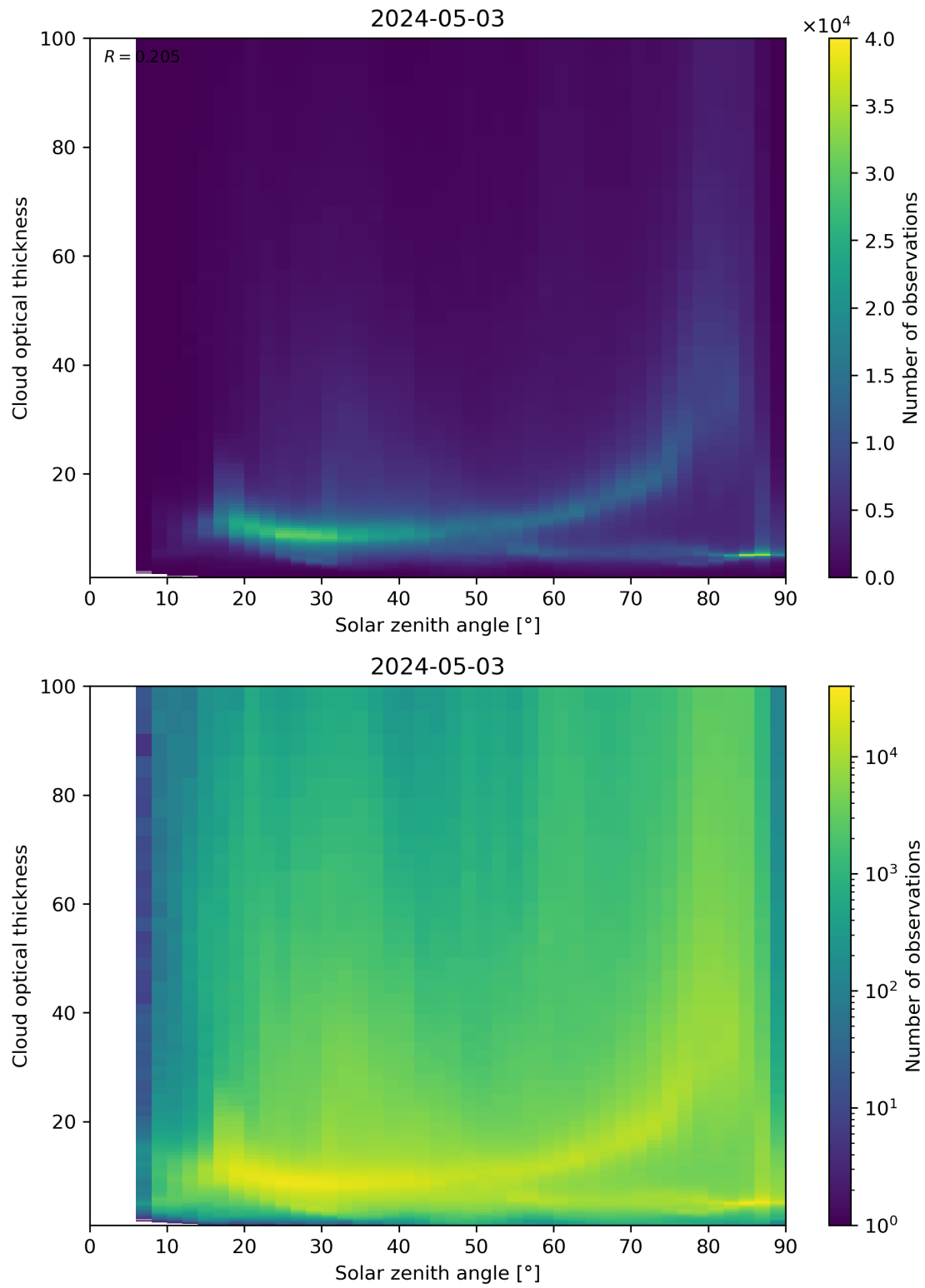
Figure 103: Scatter density plot of “Solar zenith angle” against “Cloud optical thickness” for 2024-05-02 to 2024-05-04.
