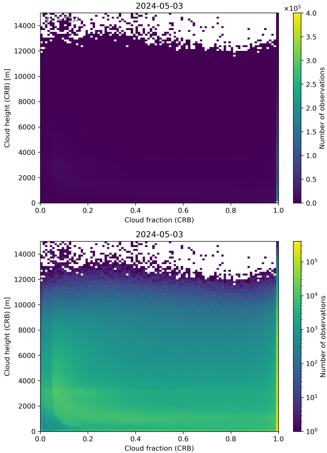
Figure 79: Scatter density plot of “Cloud fraction (CRB)” against “Cloud height (CRB)” for 2024-05-02 to 2024-05-04.
