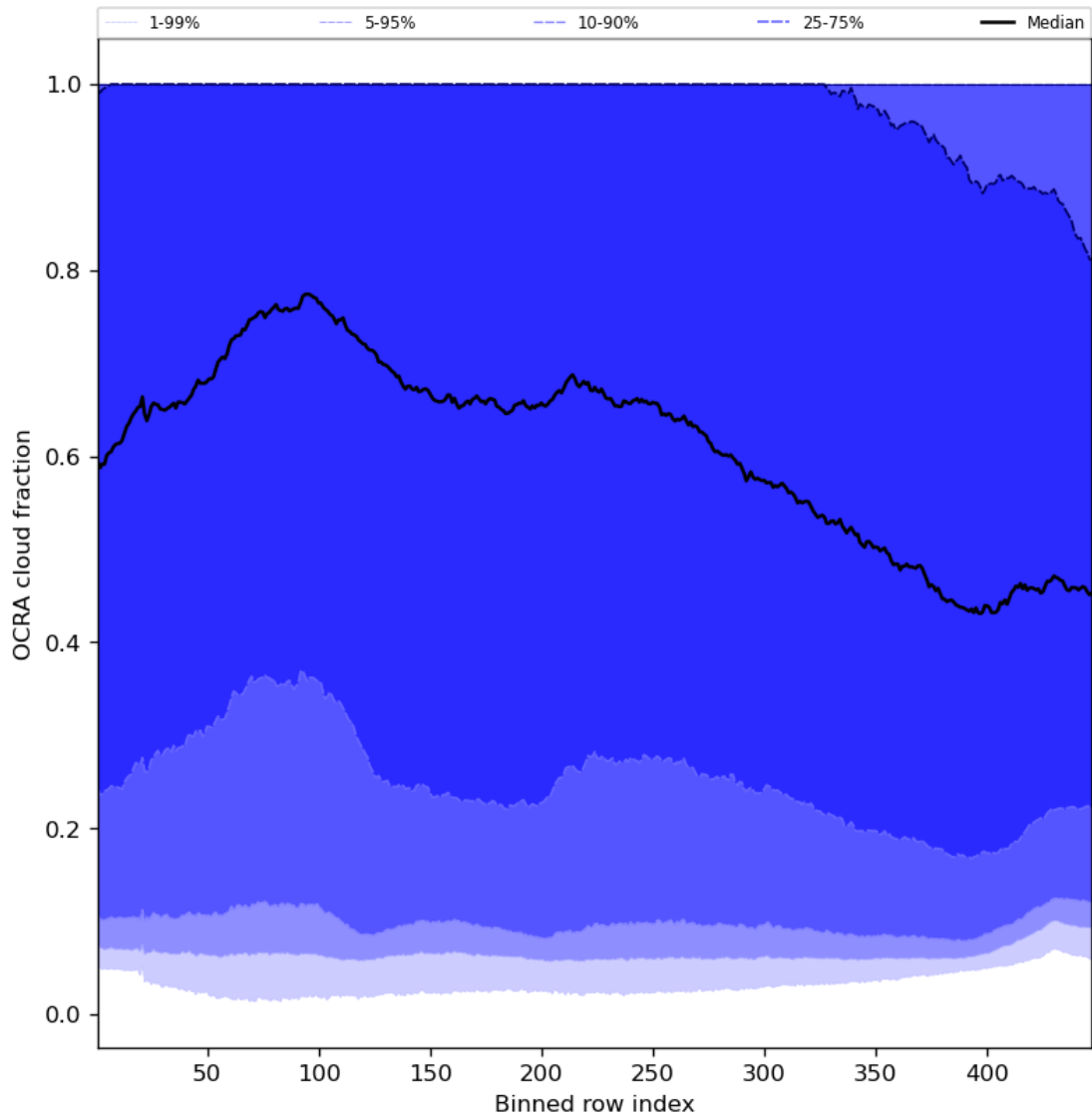
Figure 66: Along track statistics of “OCRA cloud fraction” for 2024-05-02 to 2024-05-04
