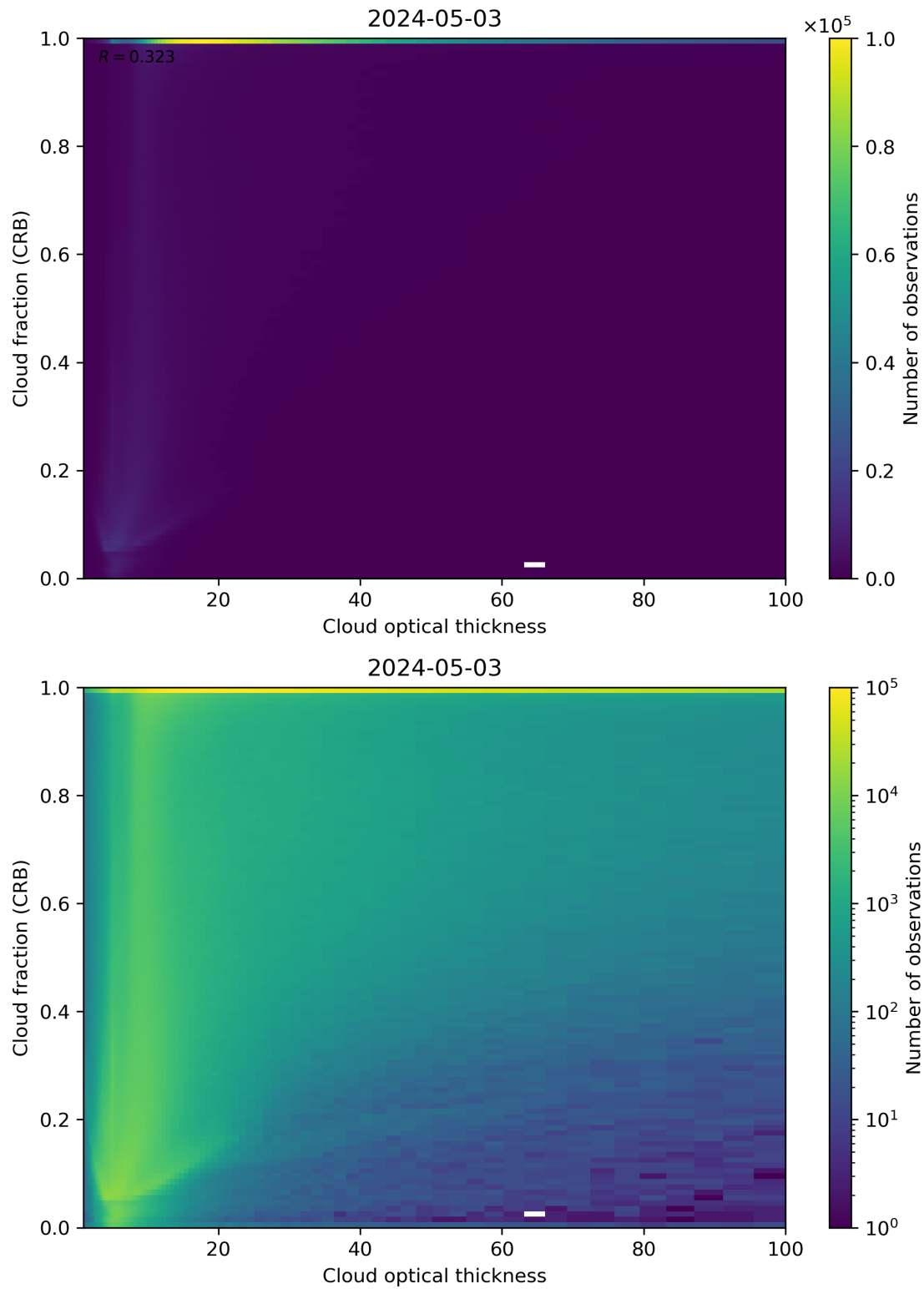
Figure 84: Scatter density plot of “Cloud optical thickness” against “Cloud fraction (CRB)” for 2024-05-02 to 2024-05-04.
