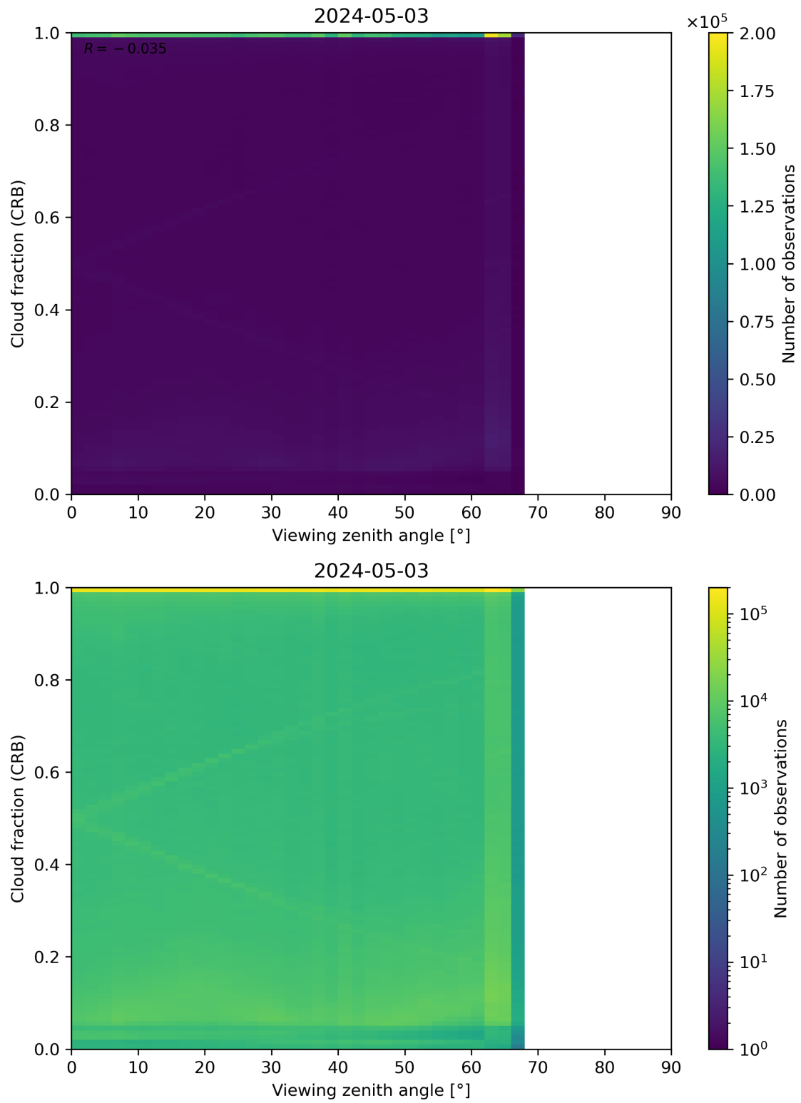
Figure 109: Scatter density plot of “Viewing zenith angle” against “Cloud fraction (CRB)” for 2024-05-02 to 2024-05-04.
