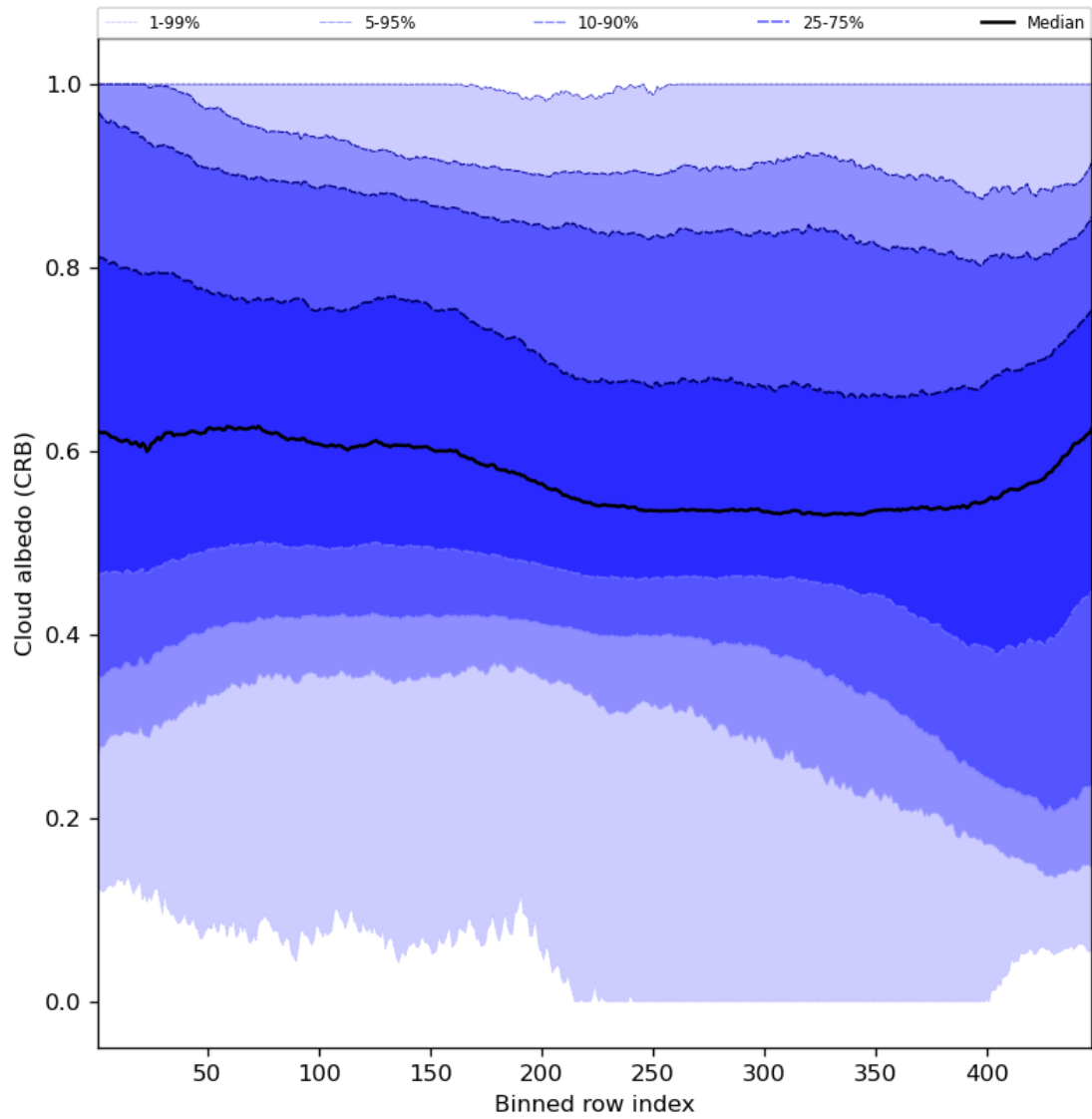
Figure 60: Along track statistics of “Cloud albedo (CRB)” for 2024-05-02 to 2024-05-04
