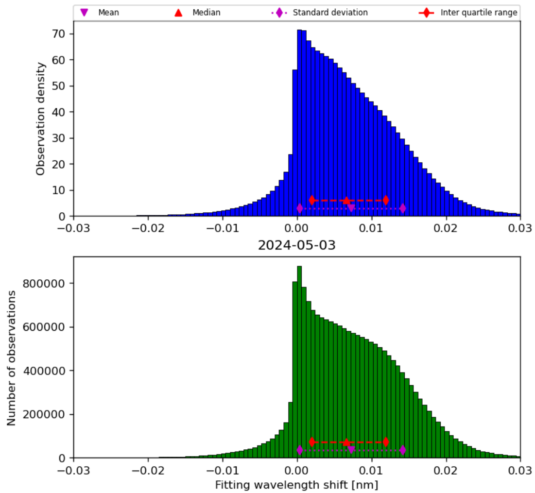
Figure 49: Histogram of “Fitting wavelength shift” for 2024-05-02 to 2024-05-04
