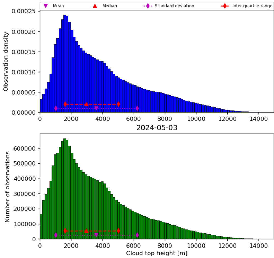
Figure 40: Histogram of “Cloud top height” for 2024-05-02 to 2024-05-04
