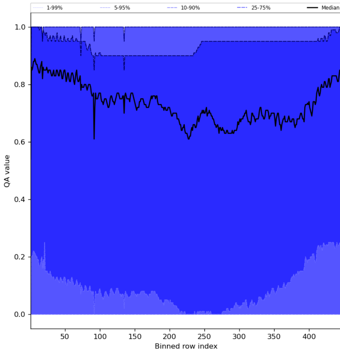
Figure 54: Along track statistics of “QA value” for 2024-05-02 to 2024-05-04
