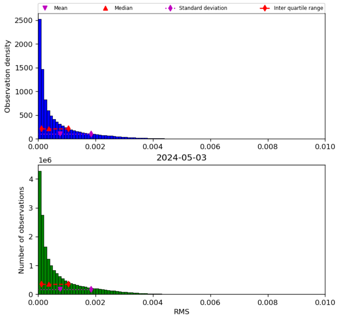
Figure 47: Histogram of “RMS” for 2024-05-02 to 2024-05-04
