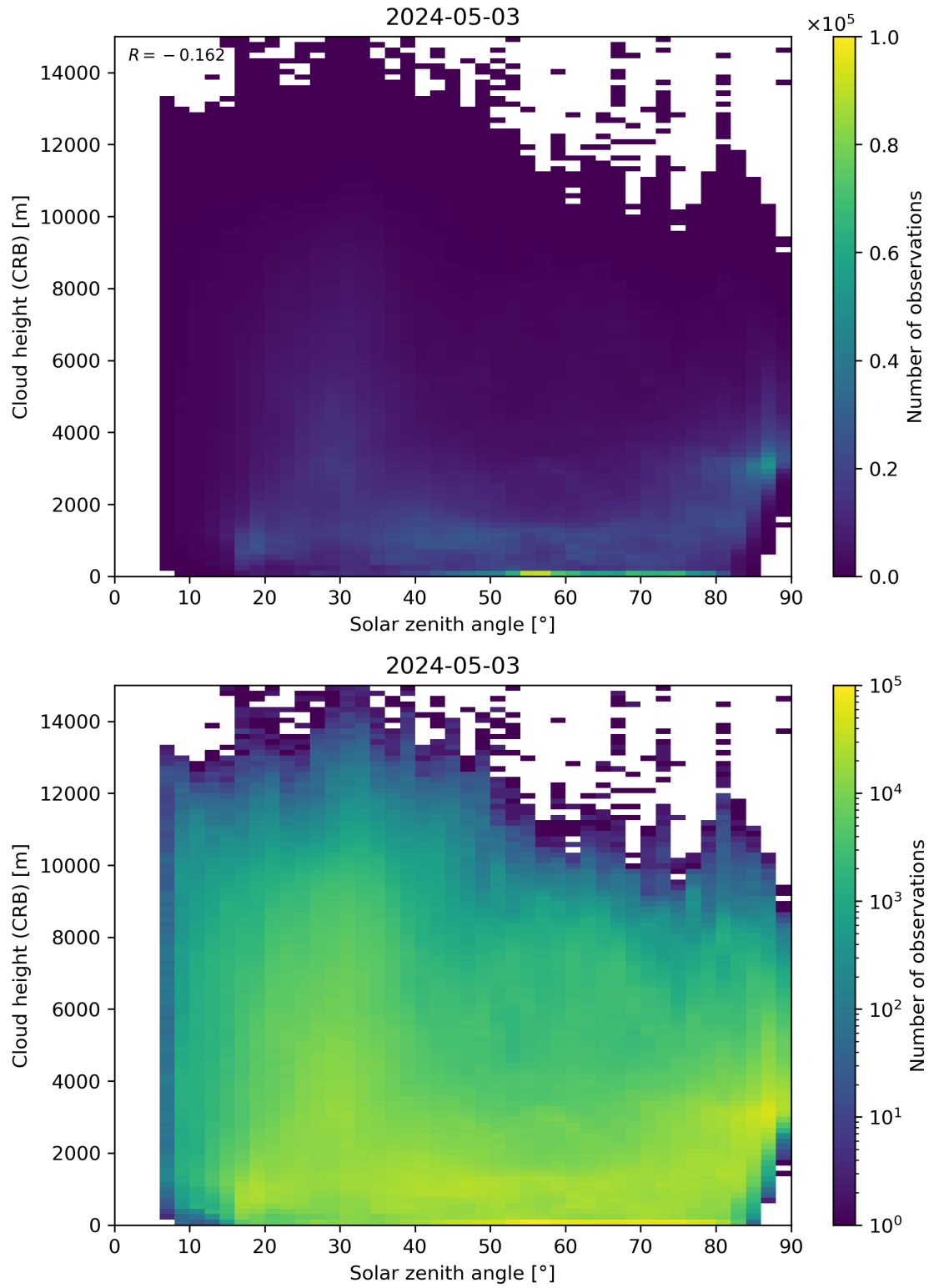
Figure 102: Scatter density plot of “Solar zenith angle” against “Cloud height (CRB)” for 2024-05-02 to 2024-05-04.
