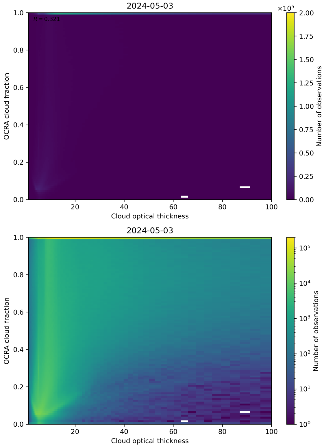
Figure 83: Scatter density plot of “Cloud optical thickness” against “OCRA cloud fraction” for 2024-05-02 to 2024-05-04.
