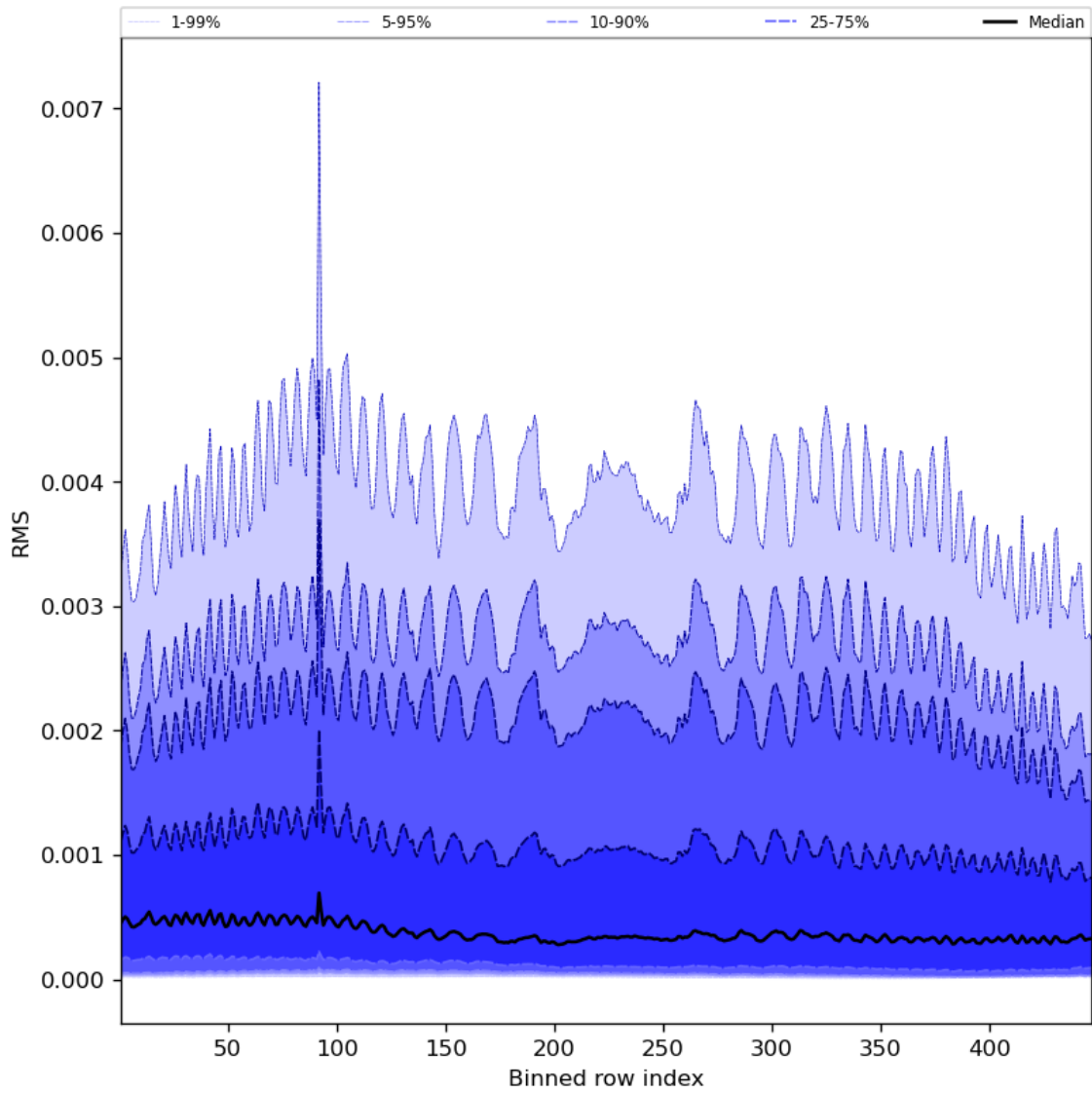
Figure 63: Along track statistics of “RMS” for 2024-05-02 to 2024-05-04
