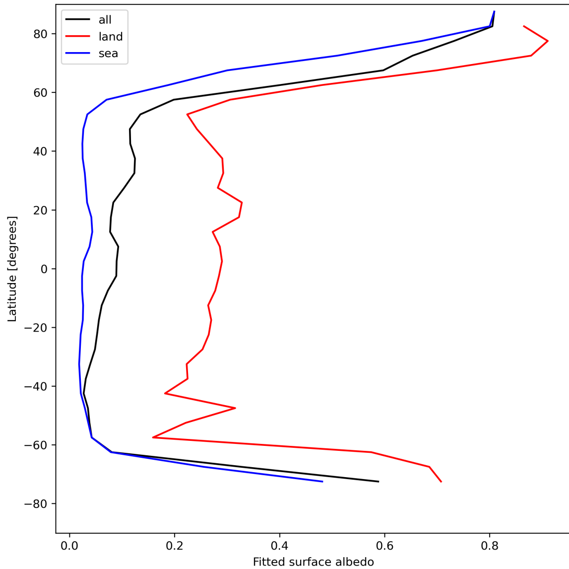
Figure 29: Zonal average of “Fitted surface albedo” for 2024-05-02 to 2024-05-04.
