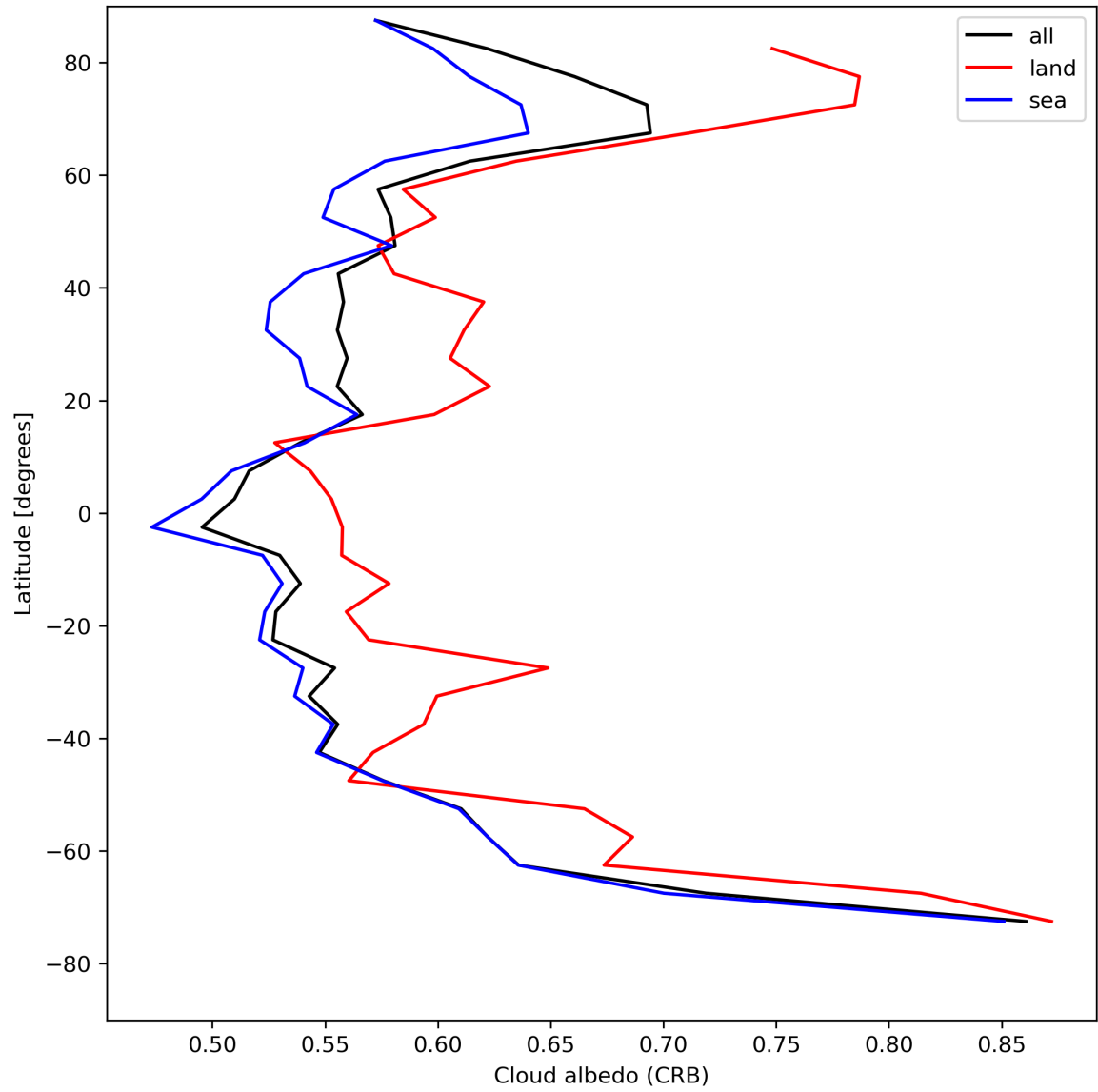
Figure 28: Zonal average of “Cloud albedo (CRB)” for 2024-05-02 to 2024-05-04.
