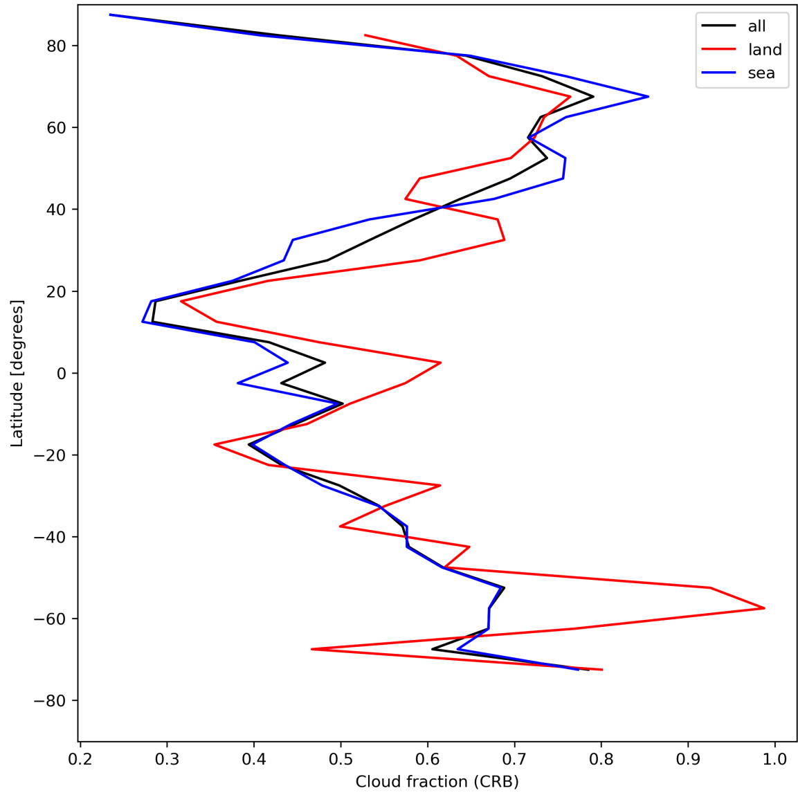
Figure 26: Zonal average of “Cloud fraction (CRB)” for 2024-05-02 to 2024-05-04.
