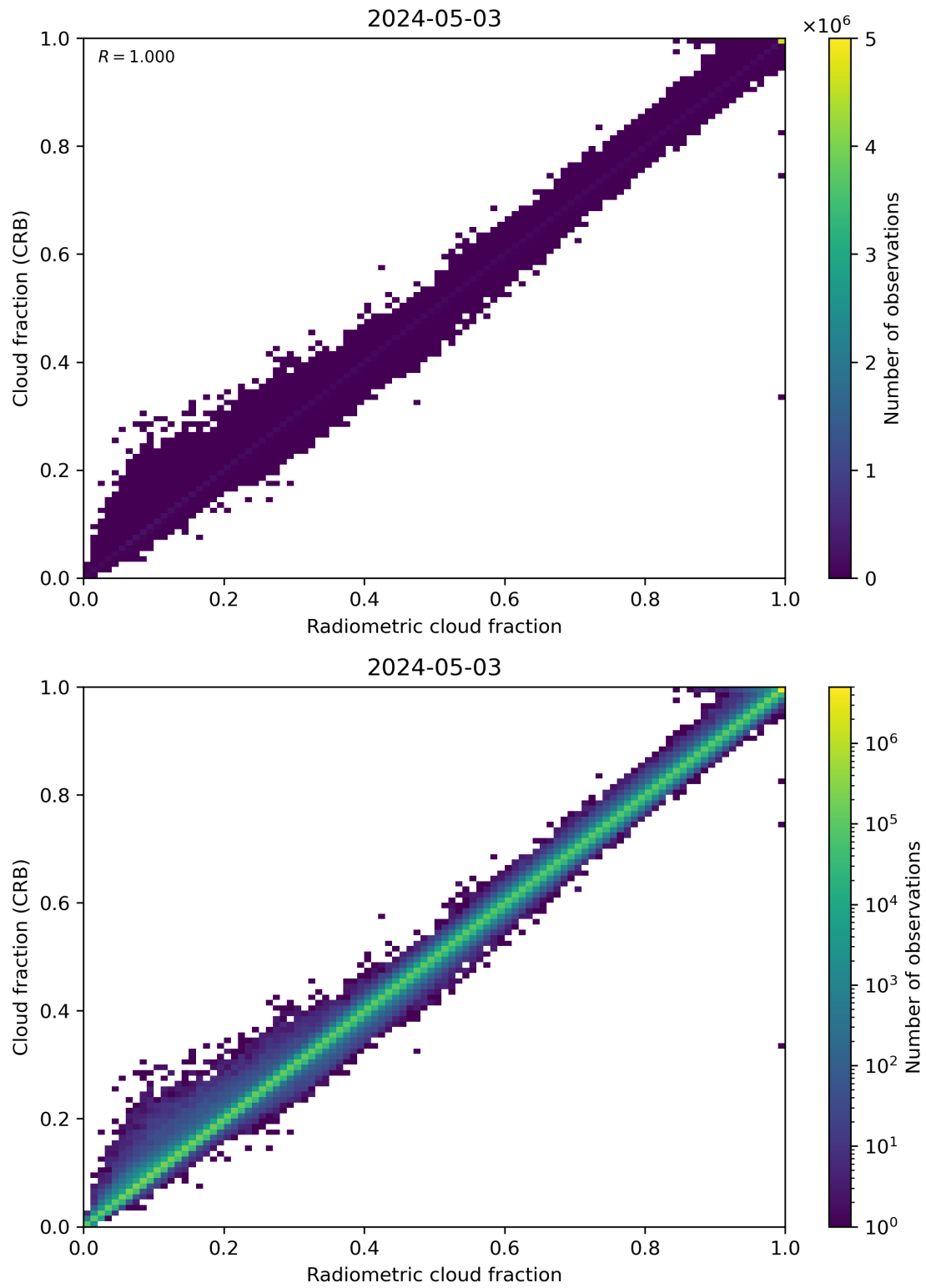
Figure 73: Scatter density plot of “Radiometric cloud fraction” against “Cloud fraction (CRB)” for 2024-05-02 to 2024-05-04.
