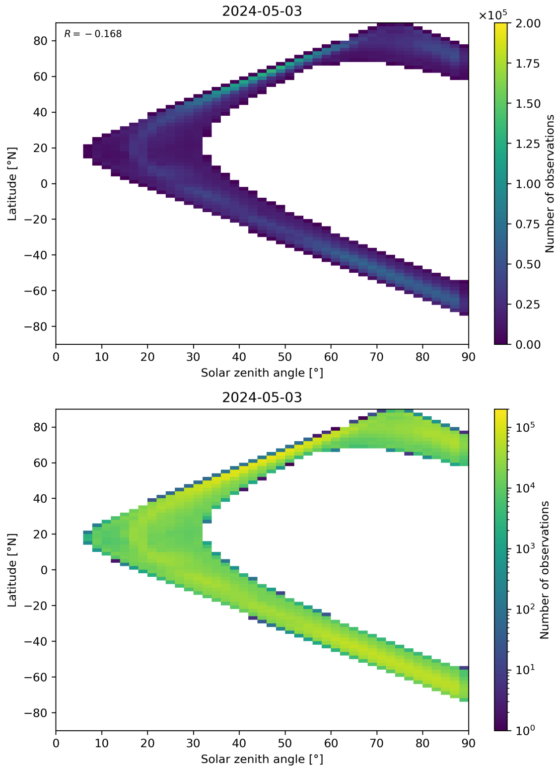
Figure 105: Scatter density plot of “Solar zenith angle” against “Latitude” for 2024-05-02 to 2024-05-04.
