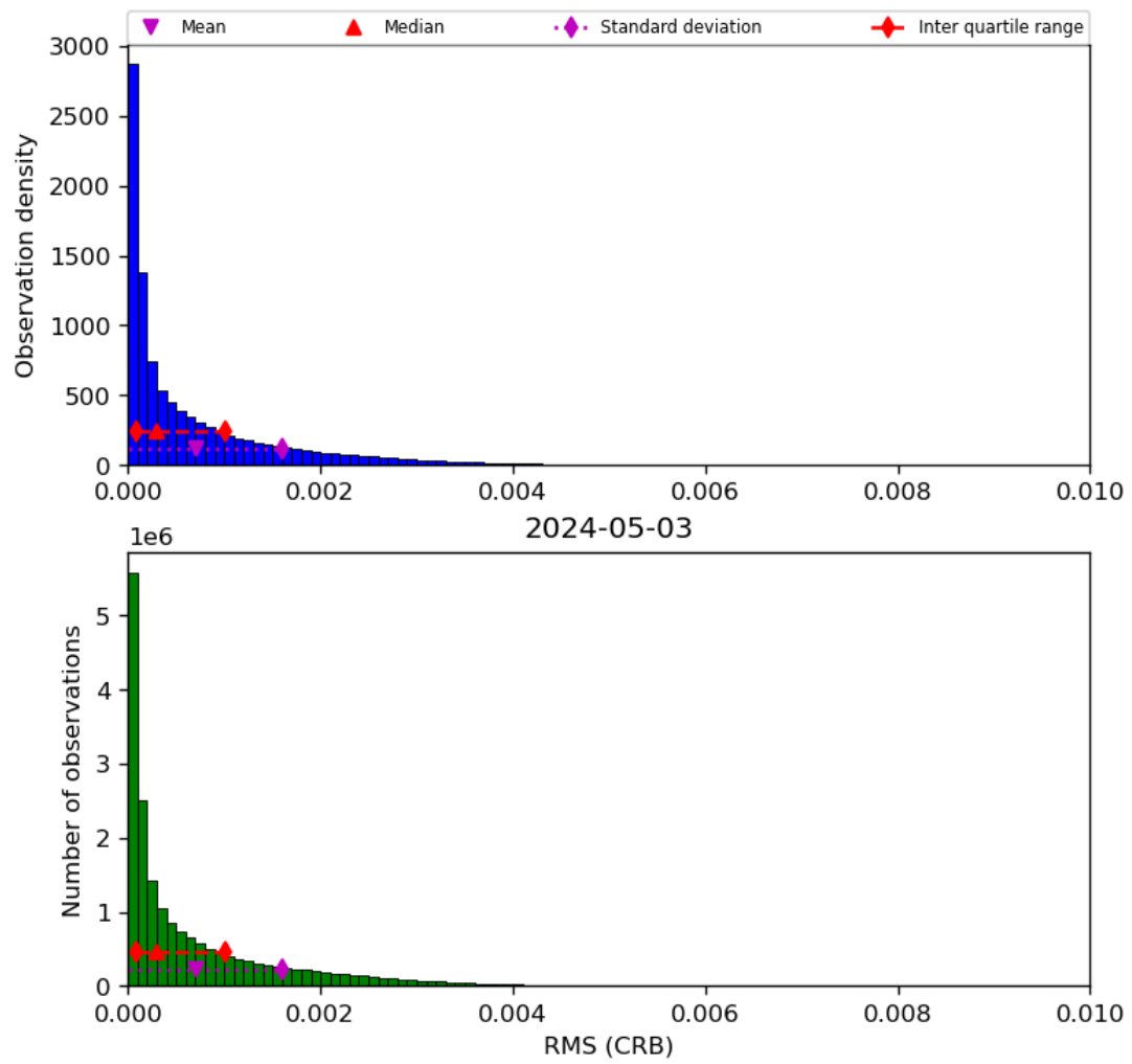
Figure 48: Histogram of “RMS (CRB)” for 2024-05-02 to 2024-05-04
