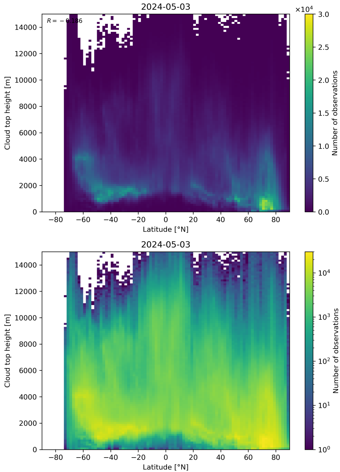
Figure 97: Scatter density plot of “Latitude” against “Cloud top height” for 2024-05-02 to 2024-05-04.
