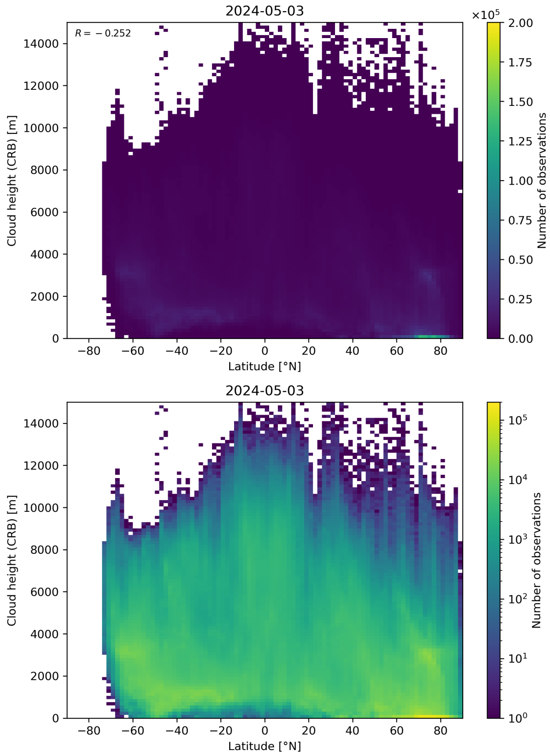
Figure 95: Scatter density plot of “Latitude” against “Cloud height (CRB)” for 2024-05-02 to 2024-05-04.
