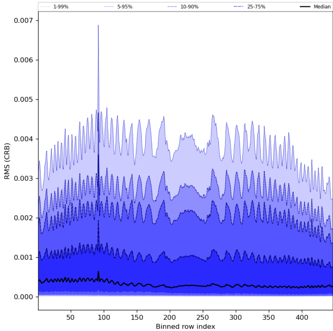
Figure 64: Along track statistics of “RMS (CRB)” for 2024-05-02 to 2024-05-04
