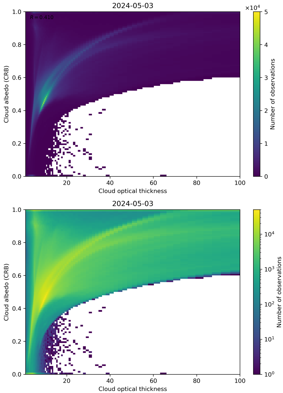
Figure 82: Scatter density plot of “Cloud optical thickness” against “Cloud albedo (CRB)” for 2024-05-02 to 2024-05-04.
