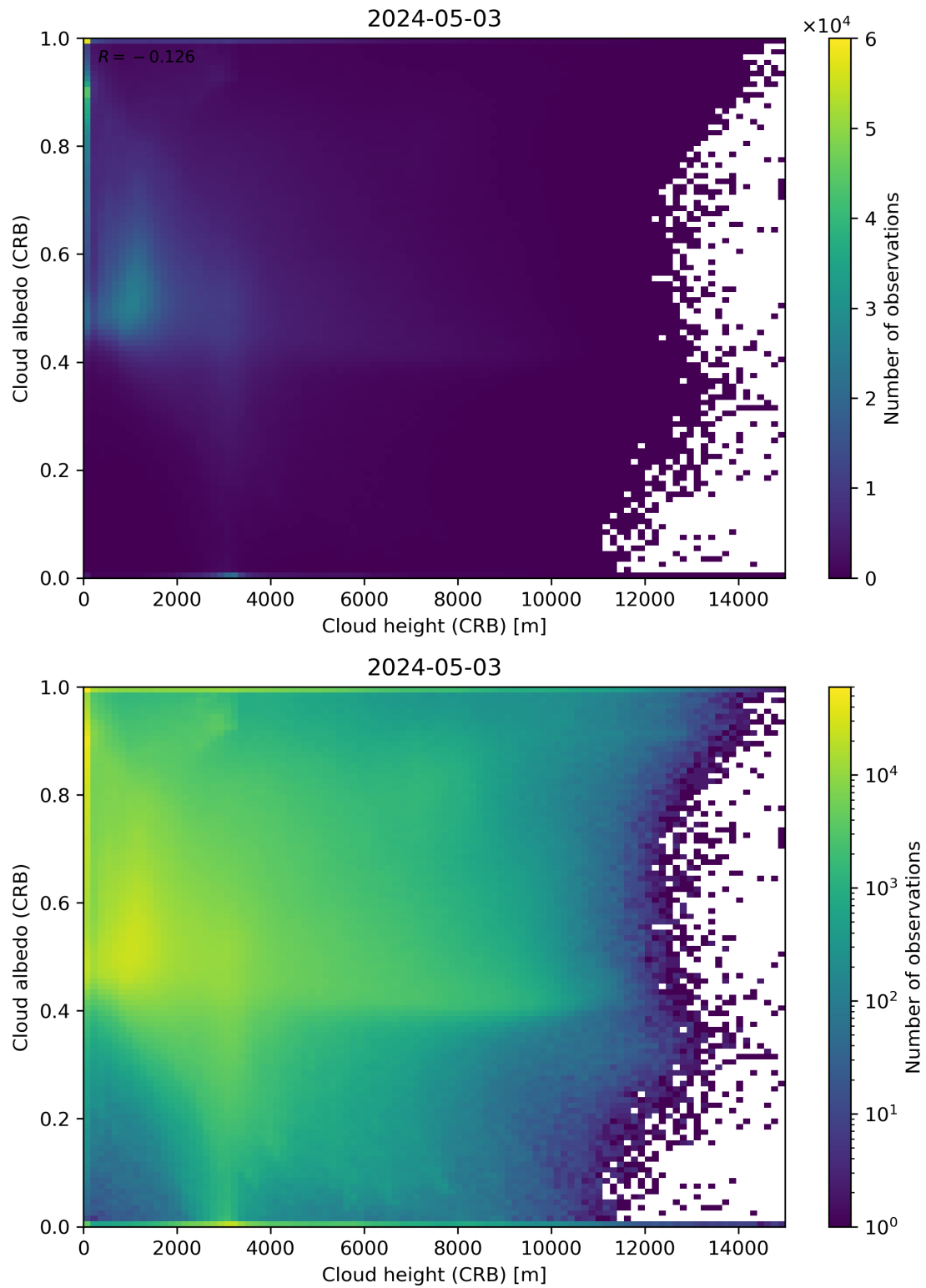
Figure 80: Scatter density plot of “Cloud height (CRB)” against “Cloud albedo (CRB)” for 2024-05-02 to 2024-05-04.
