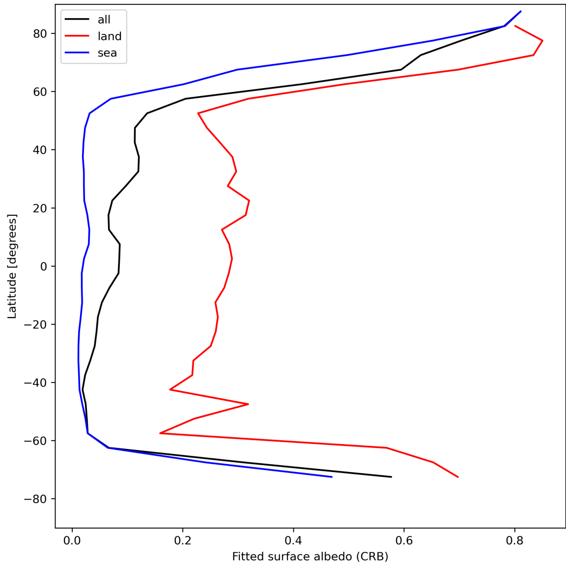
Figure 30: Zonal average of "Fitted surface albedo (CRB)" for 2024-05-02 to 2024-05-04.
