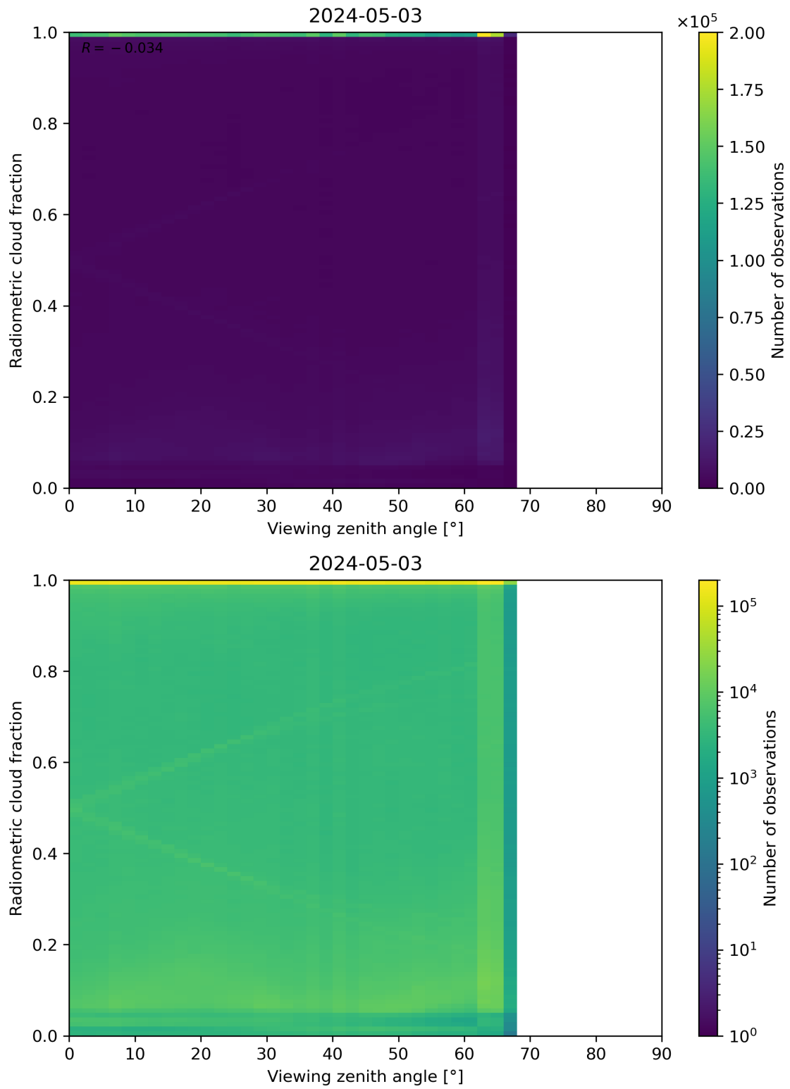
Figure 107: Scatter density plot of “Viewing zenith angle” against “Radiometric cloud fraction” for 2024-05-02 to 2024-05-04.
