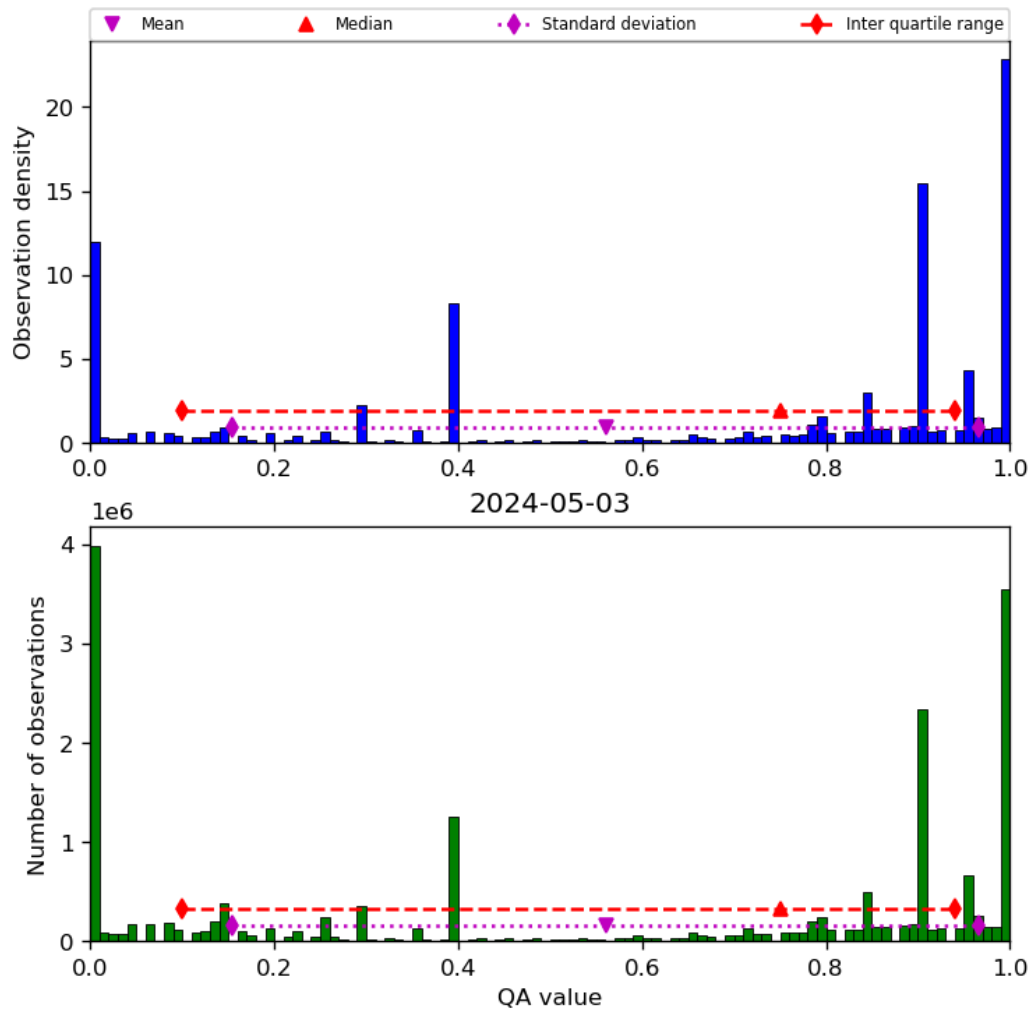
Figure 38: Histogram of “QA value” for 2024-05-02 to 2024-05-04
