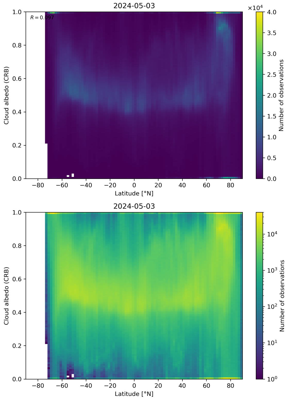
Figure 91: Scatter density plot of “Latitude” against “Cloud albedo (CRB)” for 2024-05-02 to 2024-05-04.
