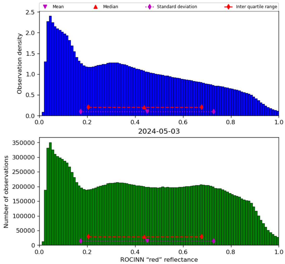
Figure 53: Histogram of “ROCINN “red” reflectance” for 2024-05-02 to 2024-05-04
