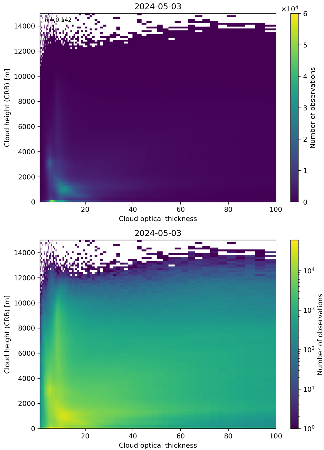
Figure 85: Scatter density plot of “Cloud optical thickness” against “Cloud height (CRB)” for 2024-05-02 to 2024-05-04.
