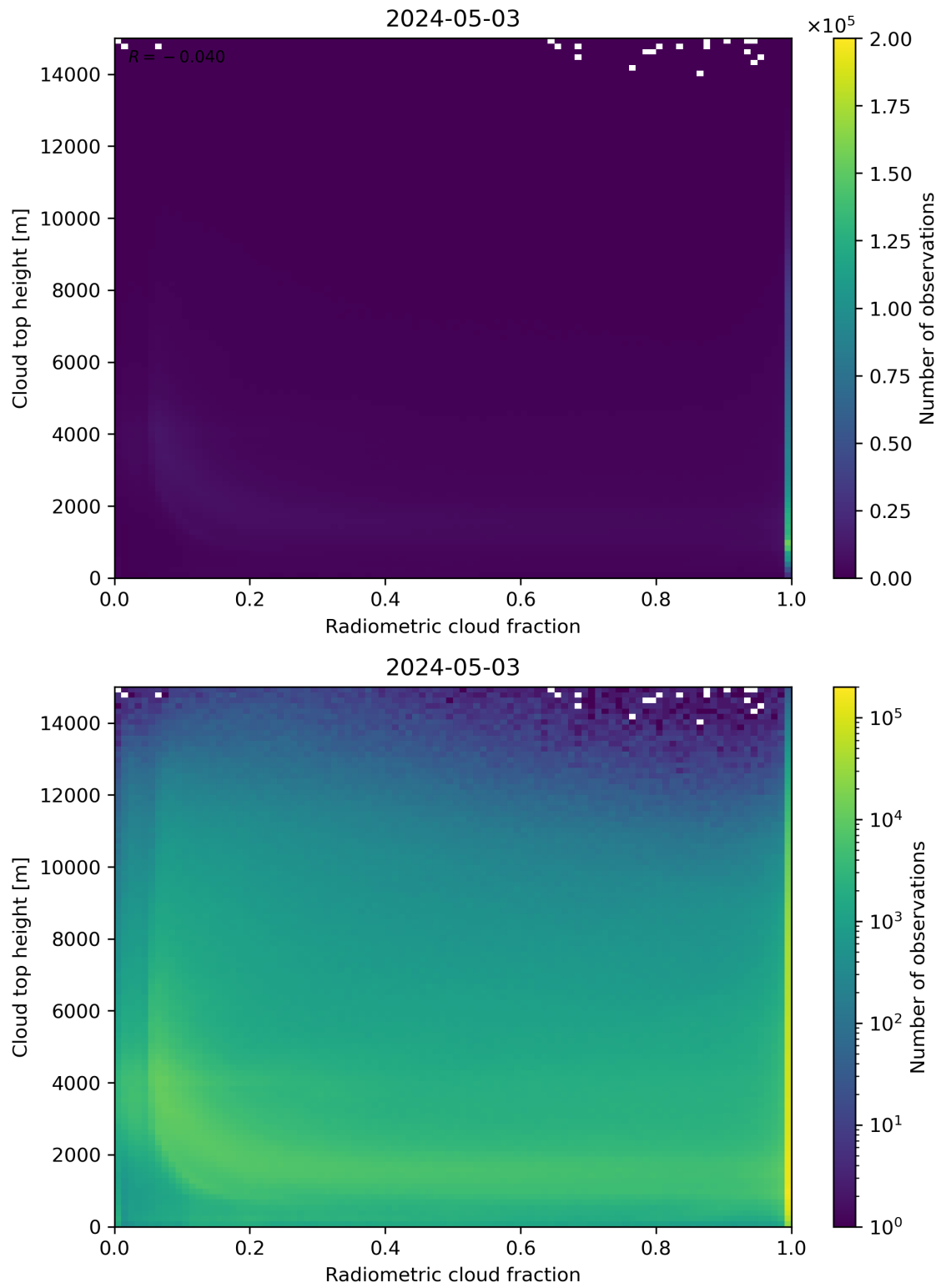
Figure 76: Scatter density plot of “Radiometric cloud fraction” against “Cloud top height” for 2024-05-02 to 2024-05-04.
