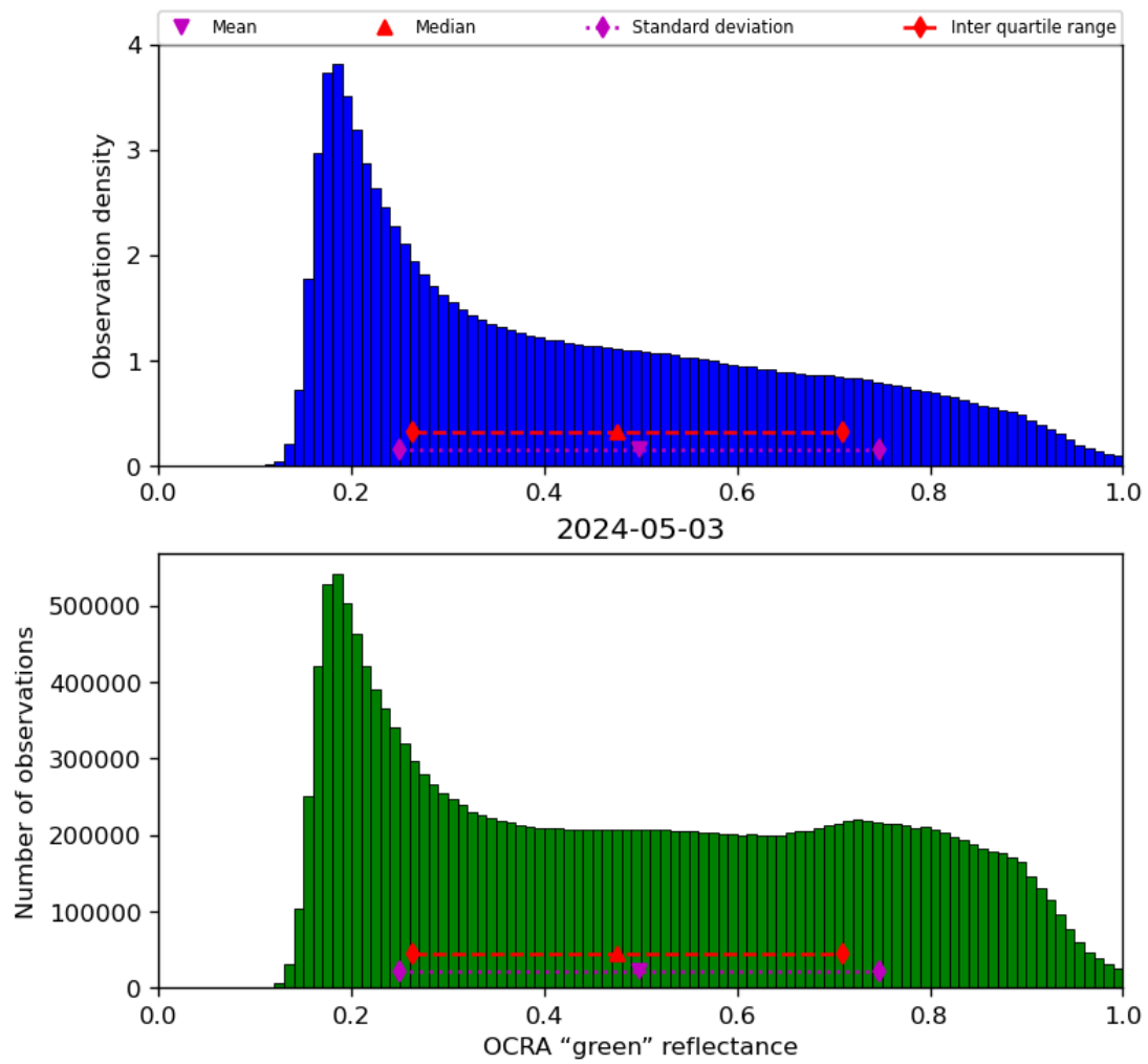
Figure 52: Histogram of “OCRA “green” reflectance” for 2024-05-02 to 2024-05-04
