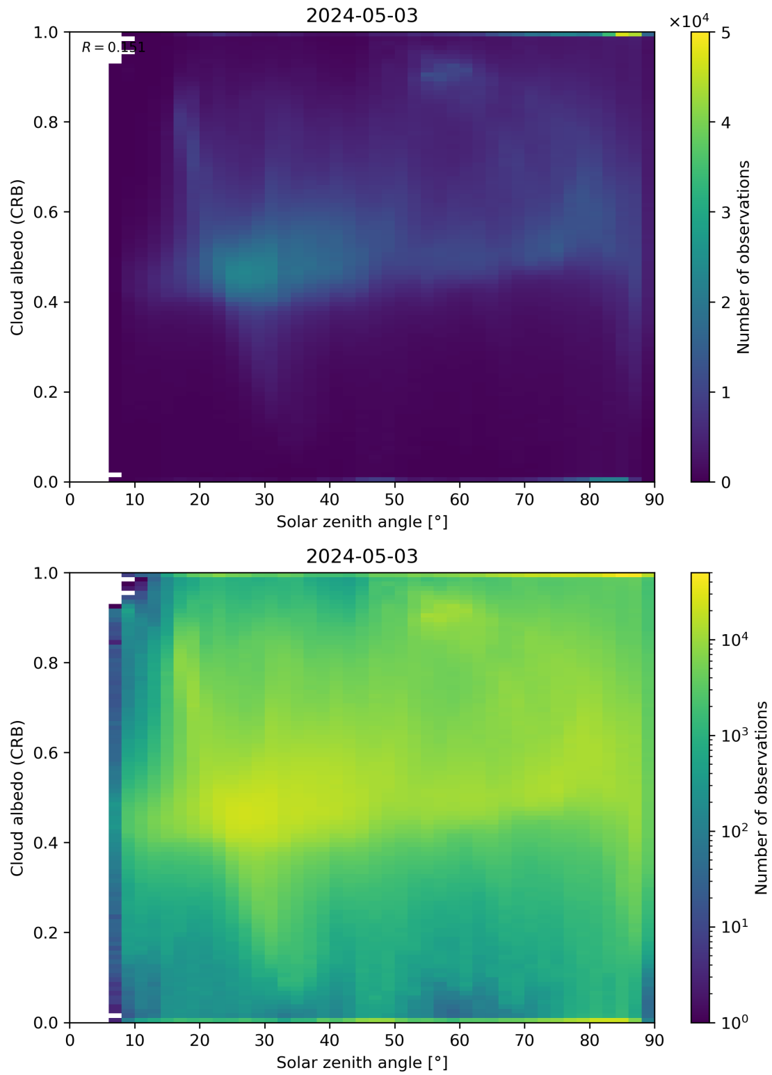
Figure 98: Scatter density plot of “Solar zenith angle” against “Cloud albedo (CRB)” for 2024-05-02 to 2024-05-04.
