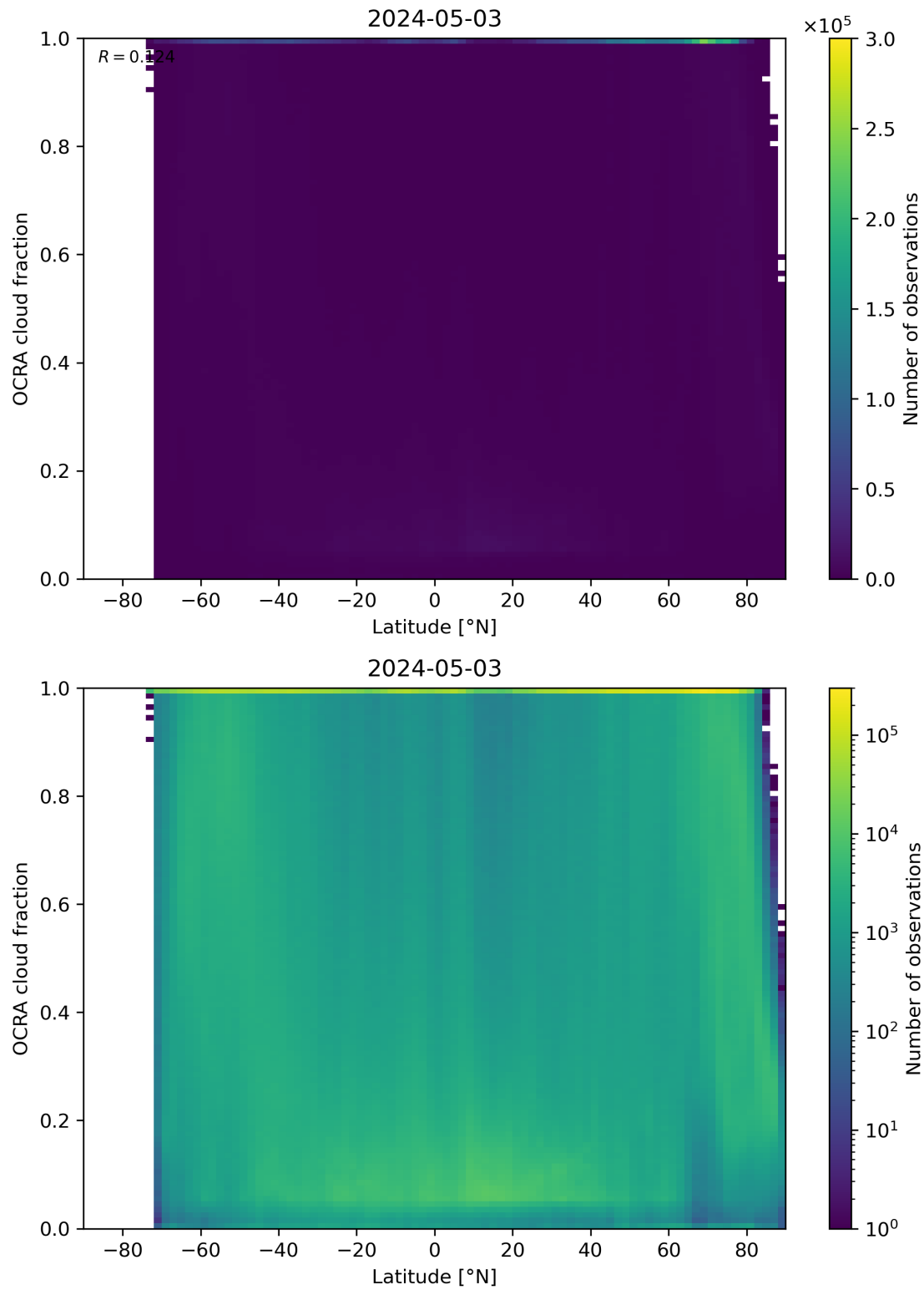
Figure 93: Scatter density plot of “Latitude” against “OCRA cloud fraction” for 2024-05-02 to 2024-05-04.
