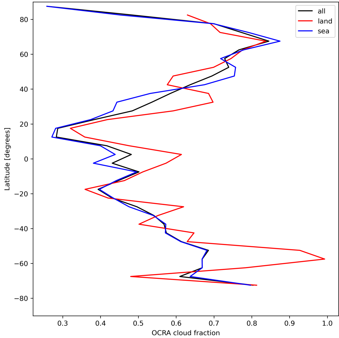
Figure 34: Zonal average of “OCRA cloud fraction” for 2024-05-02 to 2024-05-04.
