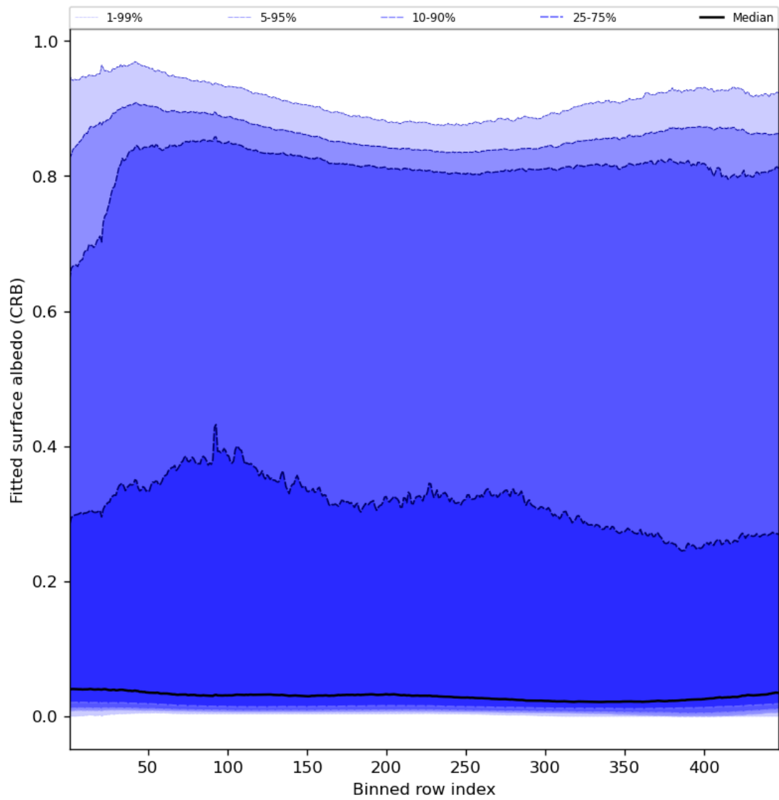
Figure 62: Along track statistics of “Fitted surface albedo (CRB)” for 2024-05-02 to 2024-05-04
