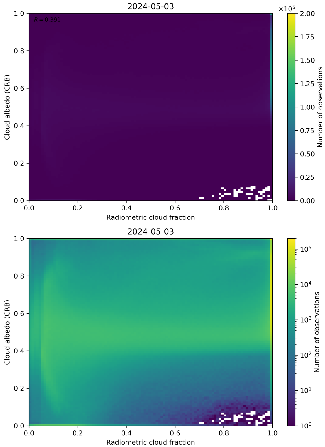
Figure 71: Scatter density plot of “Radiometric cloud fraction” against “Cloud albedo (CRB)” for 2024-05-02 to 2024-05-04.
