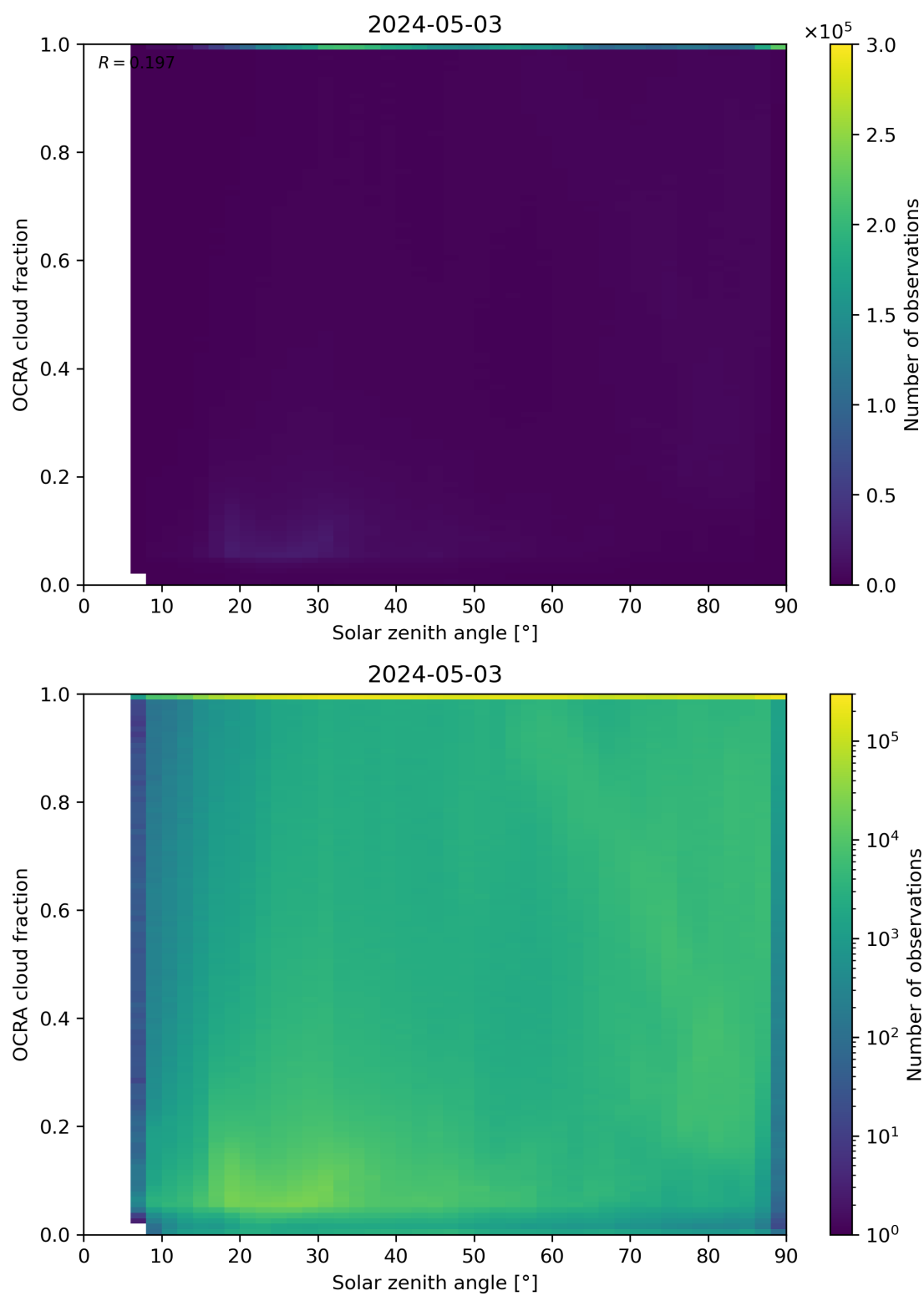
Figure 100: Scatter density plot of “Solar zenith angle” against “OCRA cloud fraction” for 2024-05-02 to 2024-05-04.
