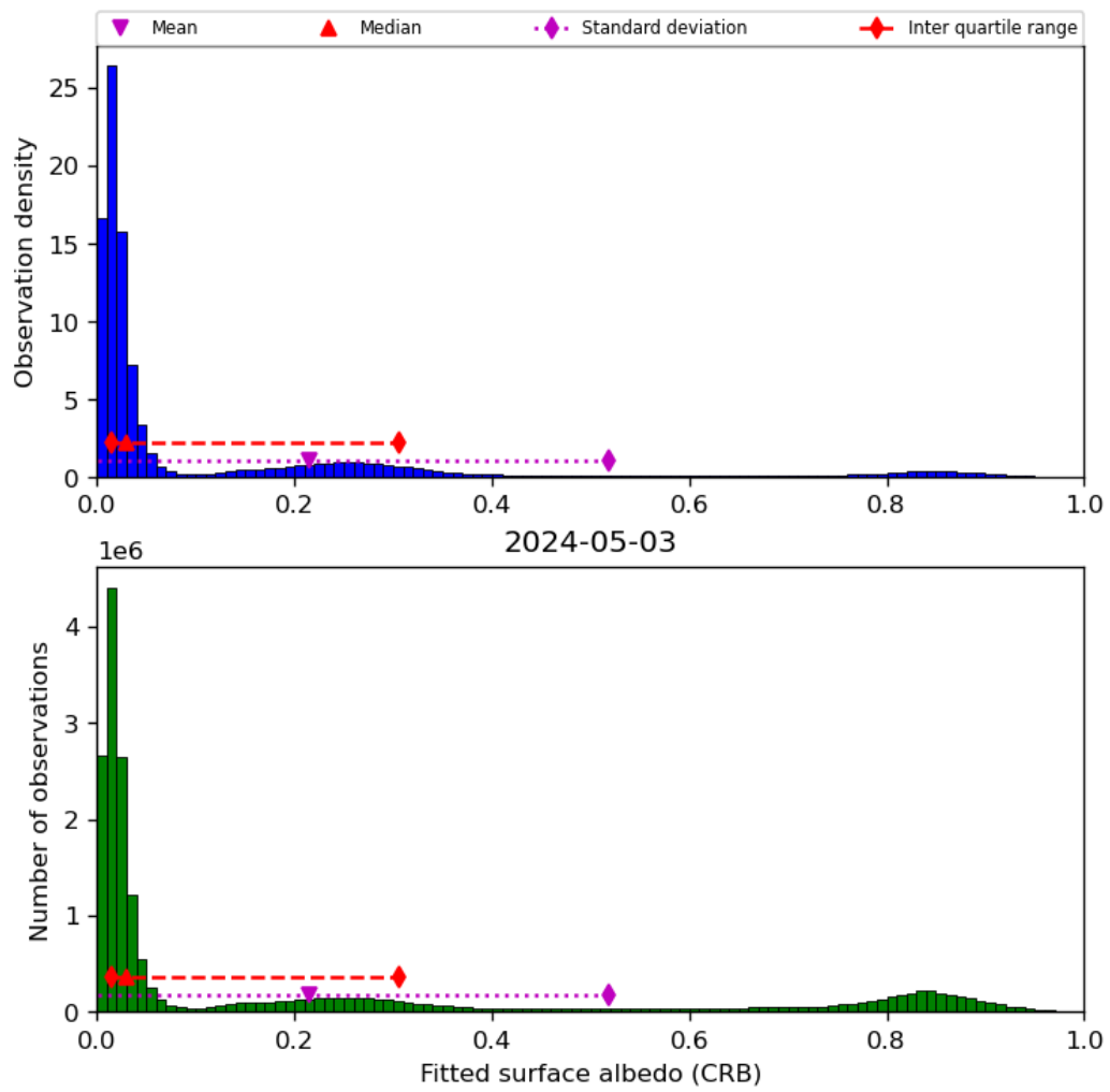
Figure 46: Histogram of “Fitted surface albedo (CRB)” for 2024-05-02 to 2024-05-04
