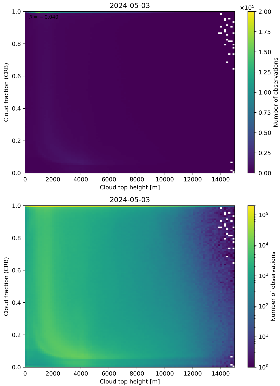
Figure 88: Scatter density plot of “Cloud top height” against “Cloud fraction (CRB)” for 2024-05-02 to 2024-05-04.
