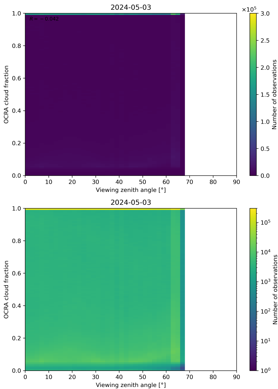
Figure 108: Scatter density plot of “Viewing zenith angle” against “OCRA cloud fraction” for 2024-05-02 to 2024-05-04.
