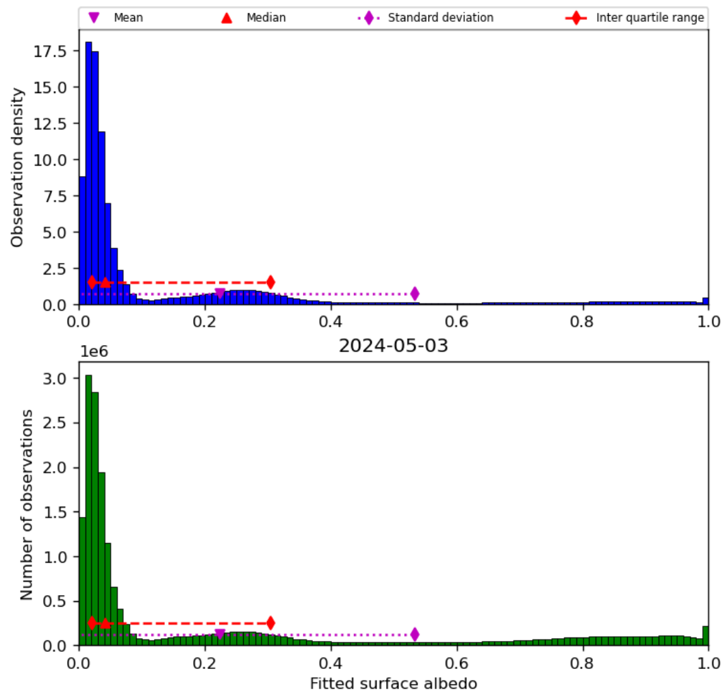
Figure 45: Histogram of “Fitted surface albedo” for 2024-05-02 to 2024-05-04
