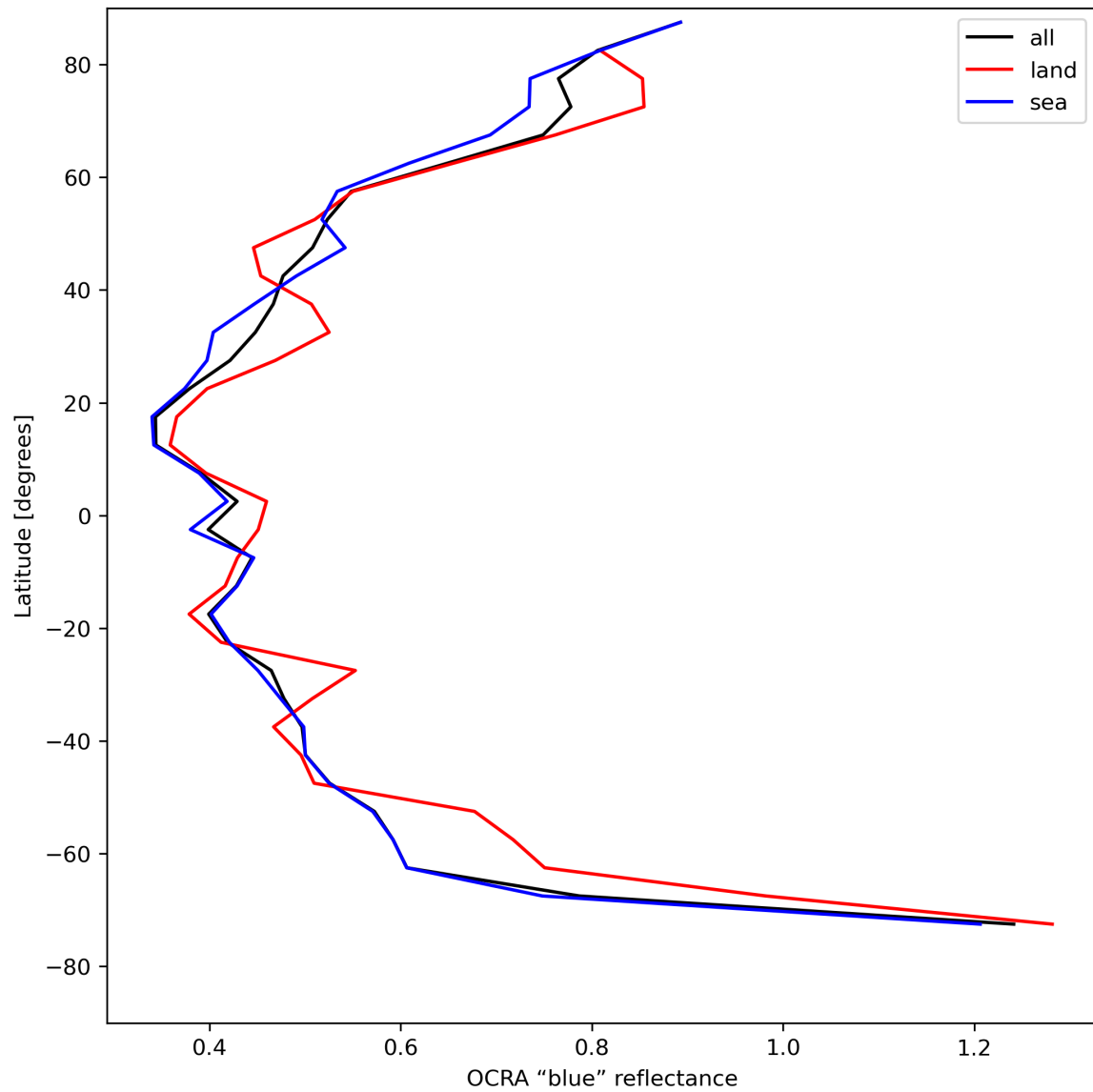
Figure 35: Zonal average of “OCRA “blue” reflectance” for 2024-05-02 to 2024-05-04.
