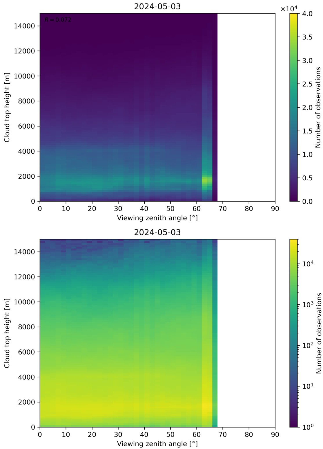
Figure 112: Scatter density plot of “Viewing zenith angle” against “Cloud top height” for 2024-05-02 to 2024-05-04.
