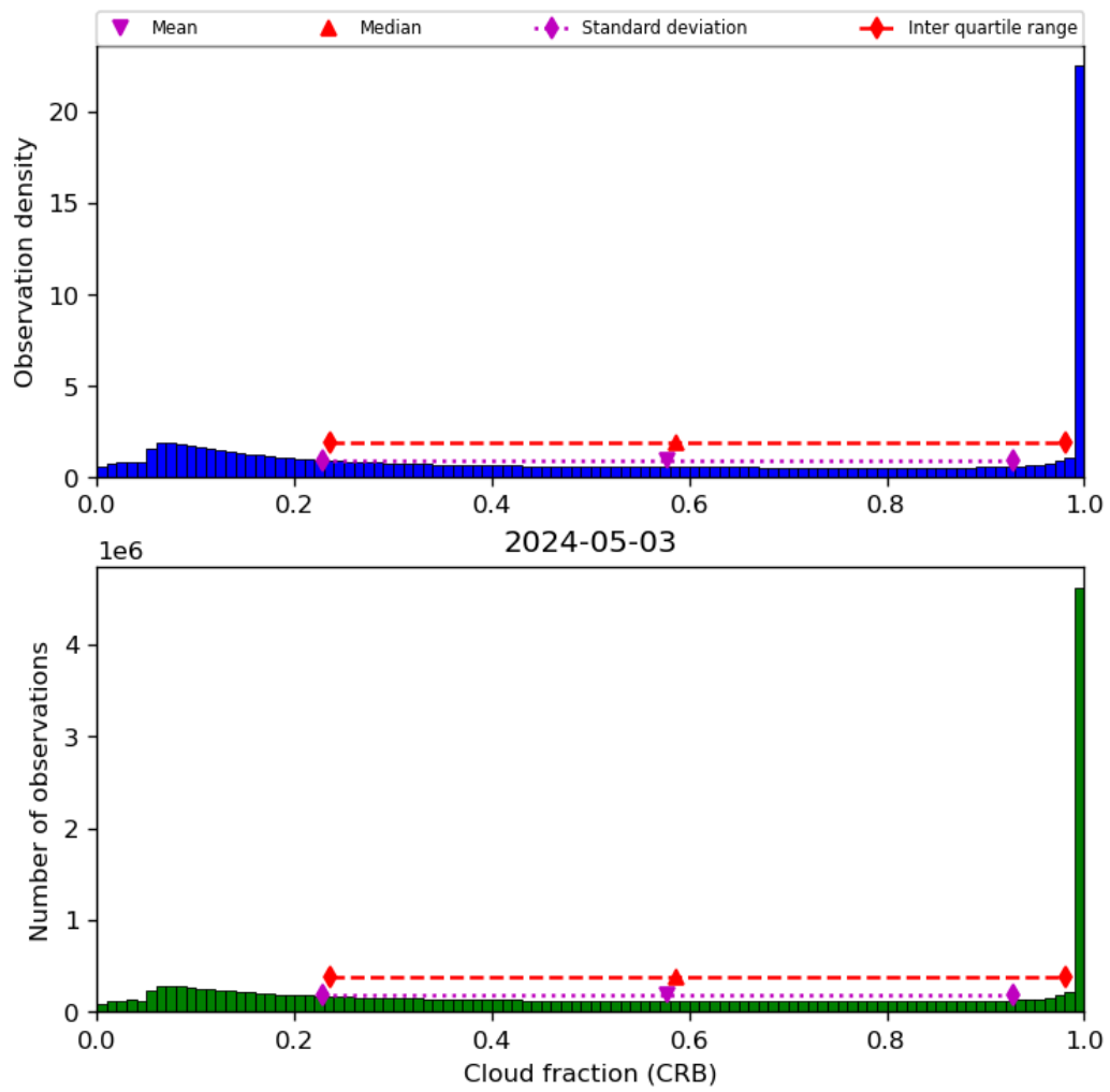
Figure 42: Histogram of “Cloud fraction (CRB)” for 2024-05-02 to 2024-05-04
