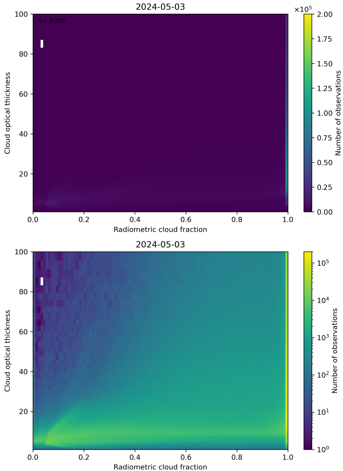
Figure 75: Scatter density plot of “Radiometric cloud fraction” against “Cloud optical thickness” for 2024-05-02 to 2024-05-04.
