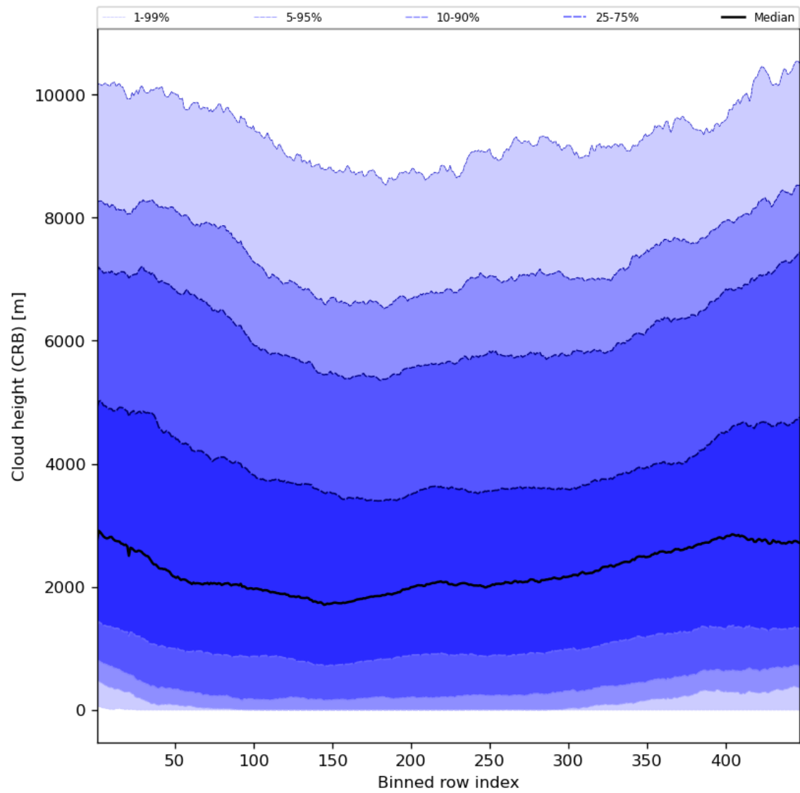
Figure 59: Along track statistics of “Cloud height (CRB)” for 2024-05-02 to 2024-05-04
