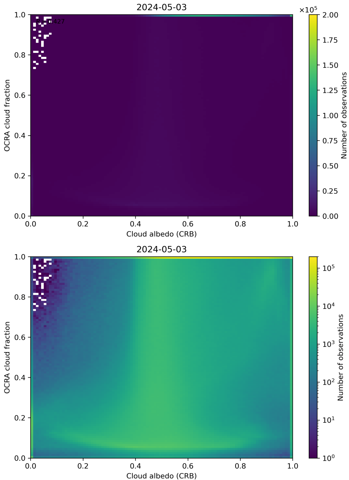
Figure 70: Scatter density plot of “Cloud albedo (CRB)” against “OCRA cloud fraction” for 2024-05-02 to 2024-05-04.
