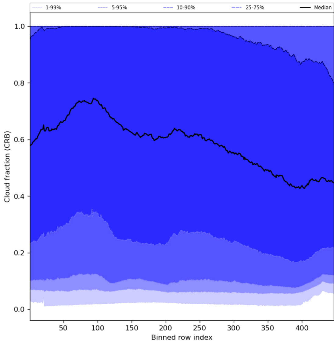
Figure 58: Along track statistics of “Cloud fraction (CRB)” for 2024-05-02 to 2024-05-04
