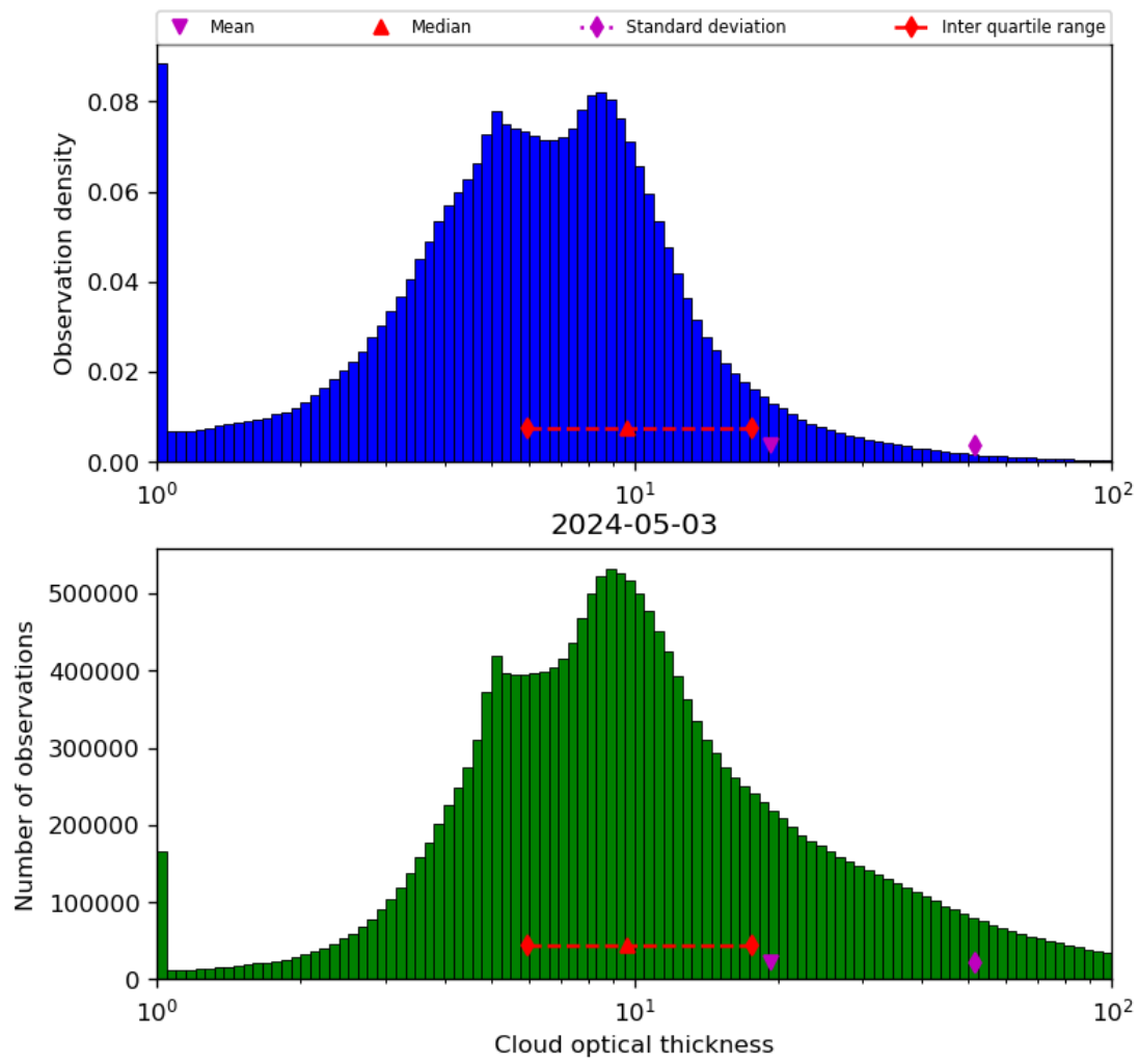
Figure 41: Histogram of “Cloud optical thickness” for 2024-05-02 to 2024-05-04
