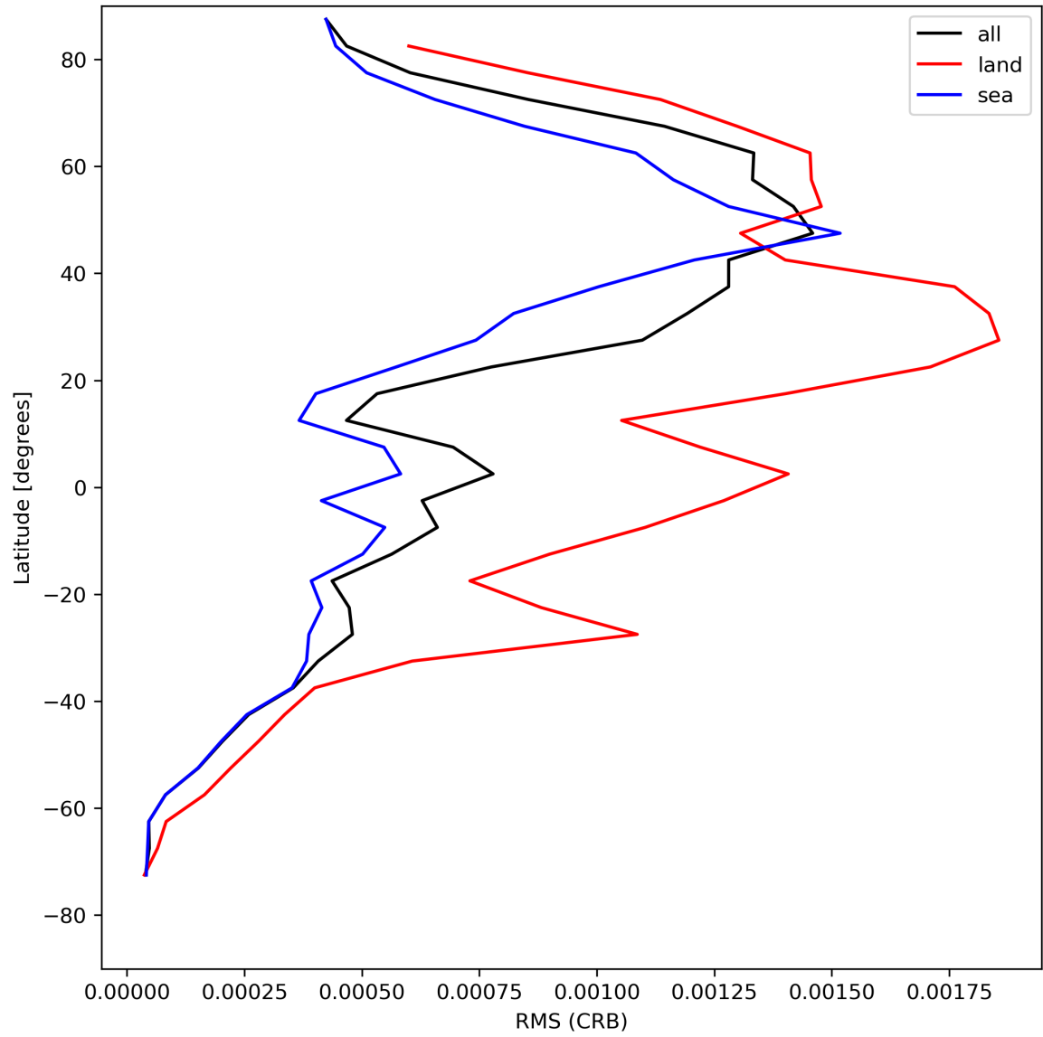
Figure 32: Zonal average of “RMS (CRB)” for 2024-05-02 to 2024-05-04.
