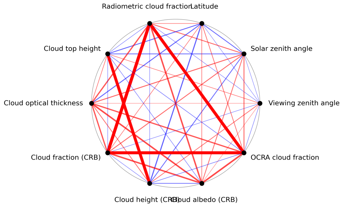
Figure 1: Map of correlation graph for 2024-05-02 to 2024-05-04.
