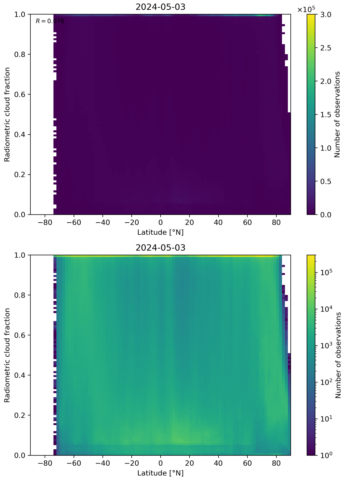
Figure 92: Scatter density plot of “Latitude” against “Radiometric cloud fraction” for 2024-05-02 to 2024-05-04.
