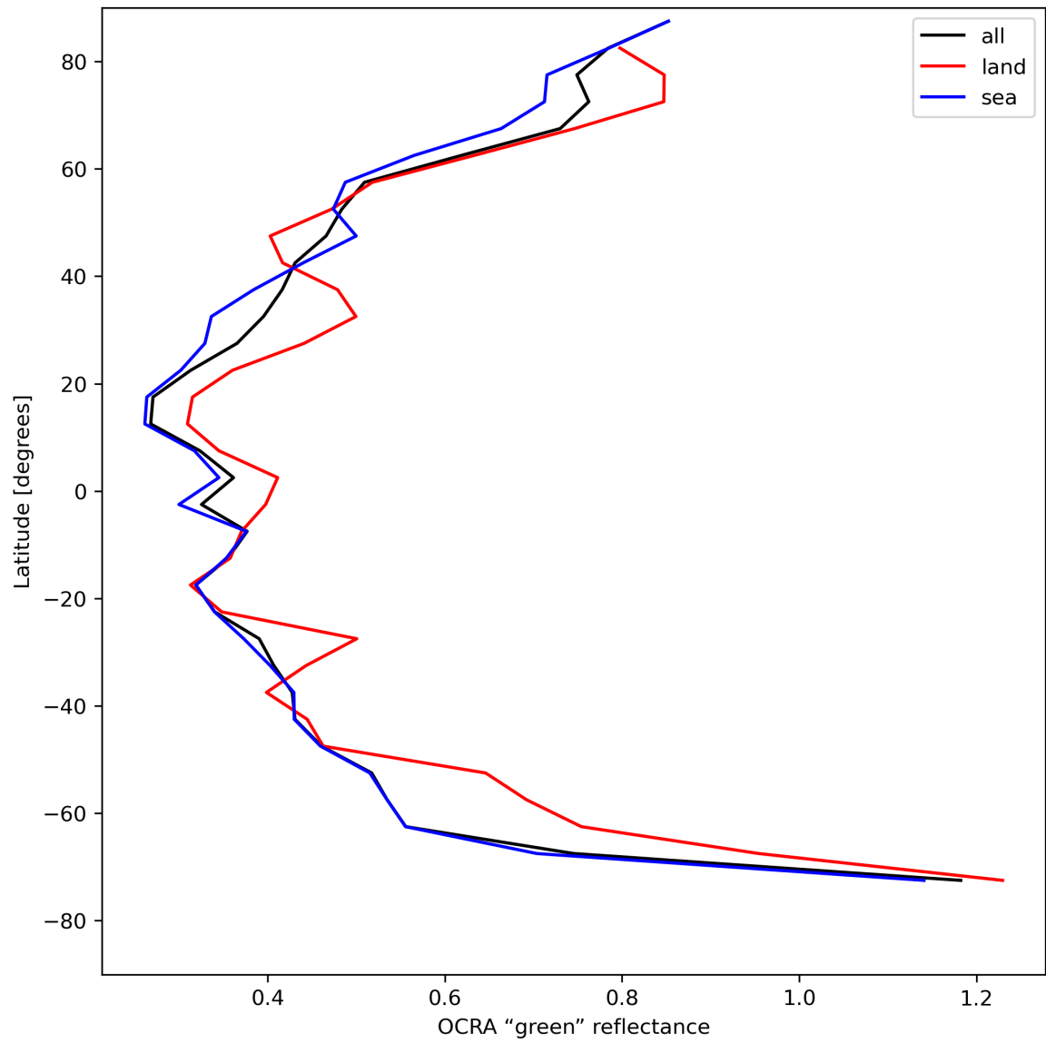
Figure 36: Zonal average of “OCRA “green” reflectance” for 2024-05-02 to 2024-05-04.
