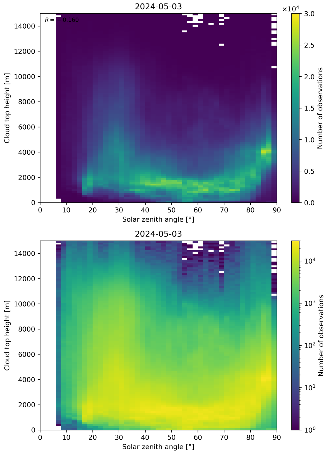
Figure 104: Scatter density plot of “Solar zenith angle” against “Cloud top height” for 2024-05-02 to 2024-05-04.
