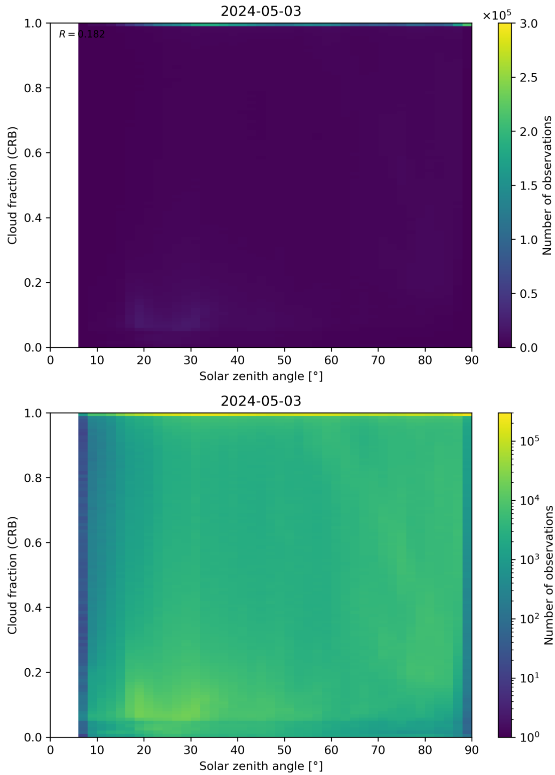
Figure 101: Scatter density plot of “Solar zenith angle” against “Cloud fraction (CRB)” for 2024-05-02 to 2024-05-04.
