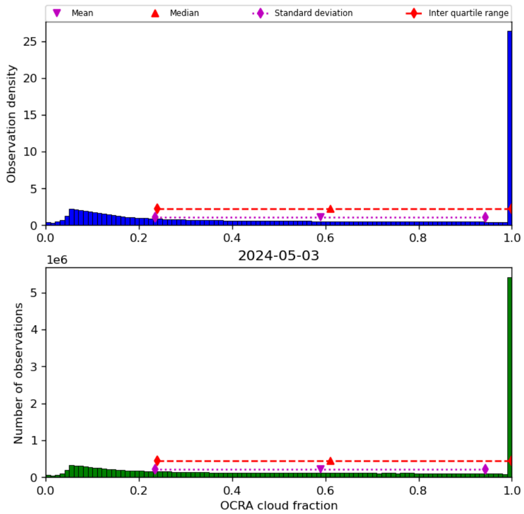
Figure 50: Histogram of “OCRA cloud fraction” for 2024-05-02 to 2024-05-04
