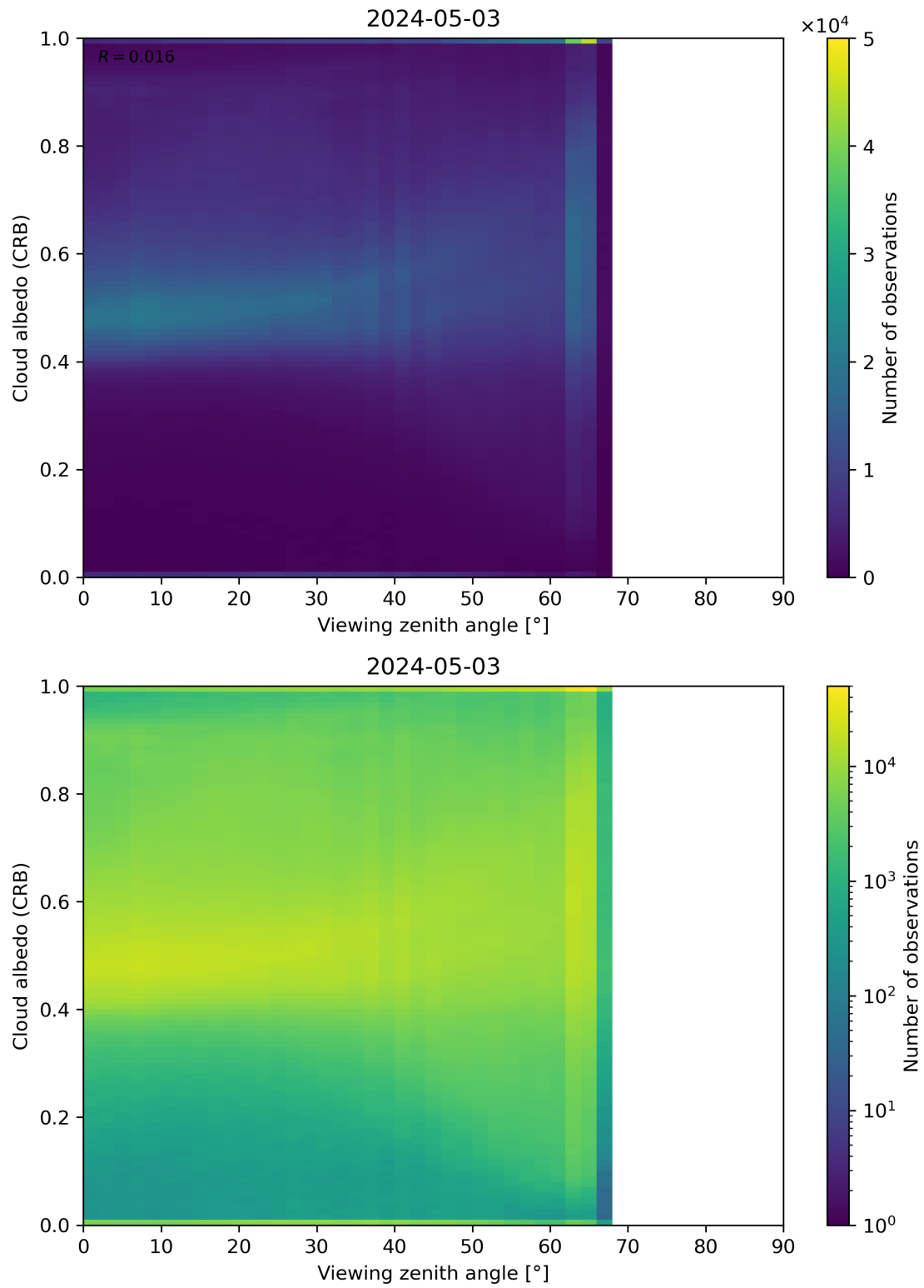
Figure 106: Scatter density plot of “Viewing zenith angle” against “Cloud albedo (CRB)” for 2024-05-02 to 2024-05-04.
