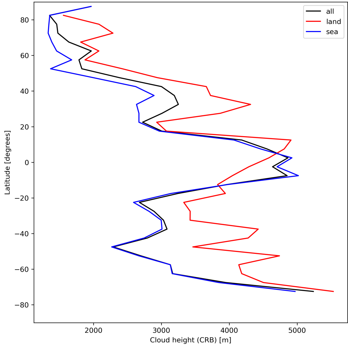
Figure 27: Zonal average of “Cloud height (CRB)” for 2024-05-02 to 2024-05-04.
