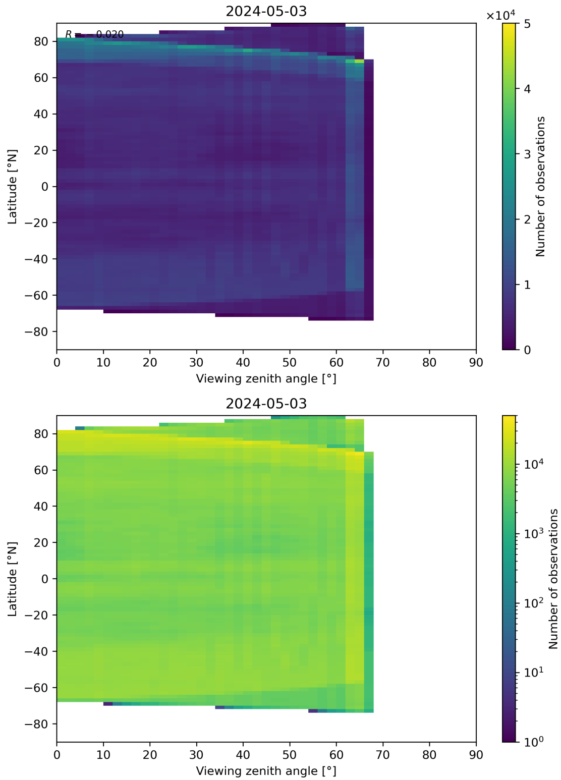
Figure 113: Scatter density plot of “Viewing zenith angle” against “Latitude” for 2024-05-02 to 2024-05-04.
