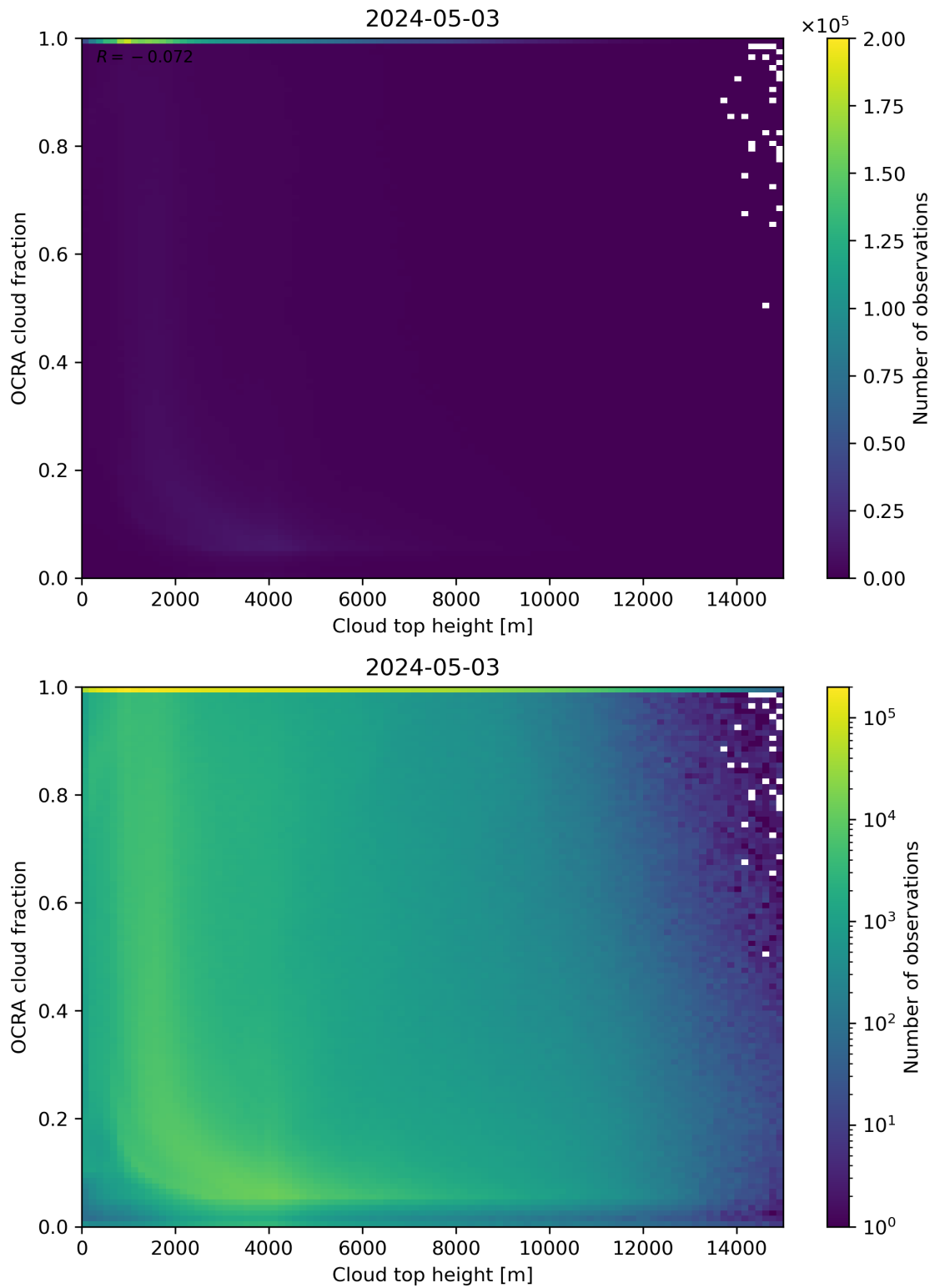
Figure 87: Scatter density plot of “Cloud top height” against “OCRA cloud fraction” for 2024-05-02 to 2024-05-04.
