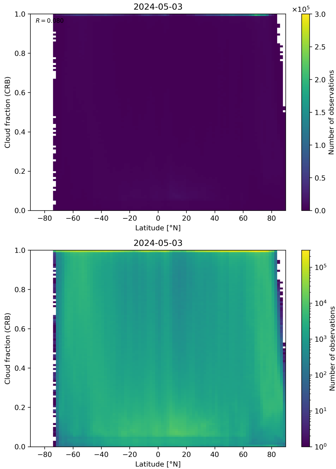
Figure 94: Scatter density plot of “Latitude” against “Cloud fraction (CRB)” for 2024-05-02 to 2024-05-04.
