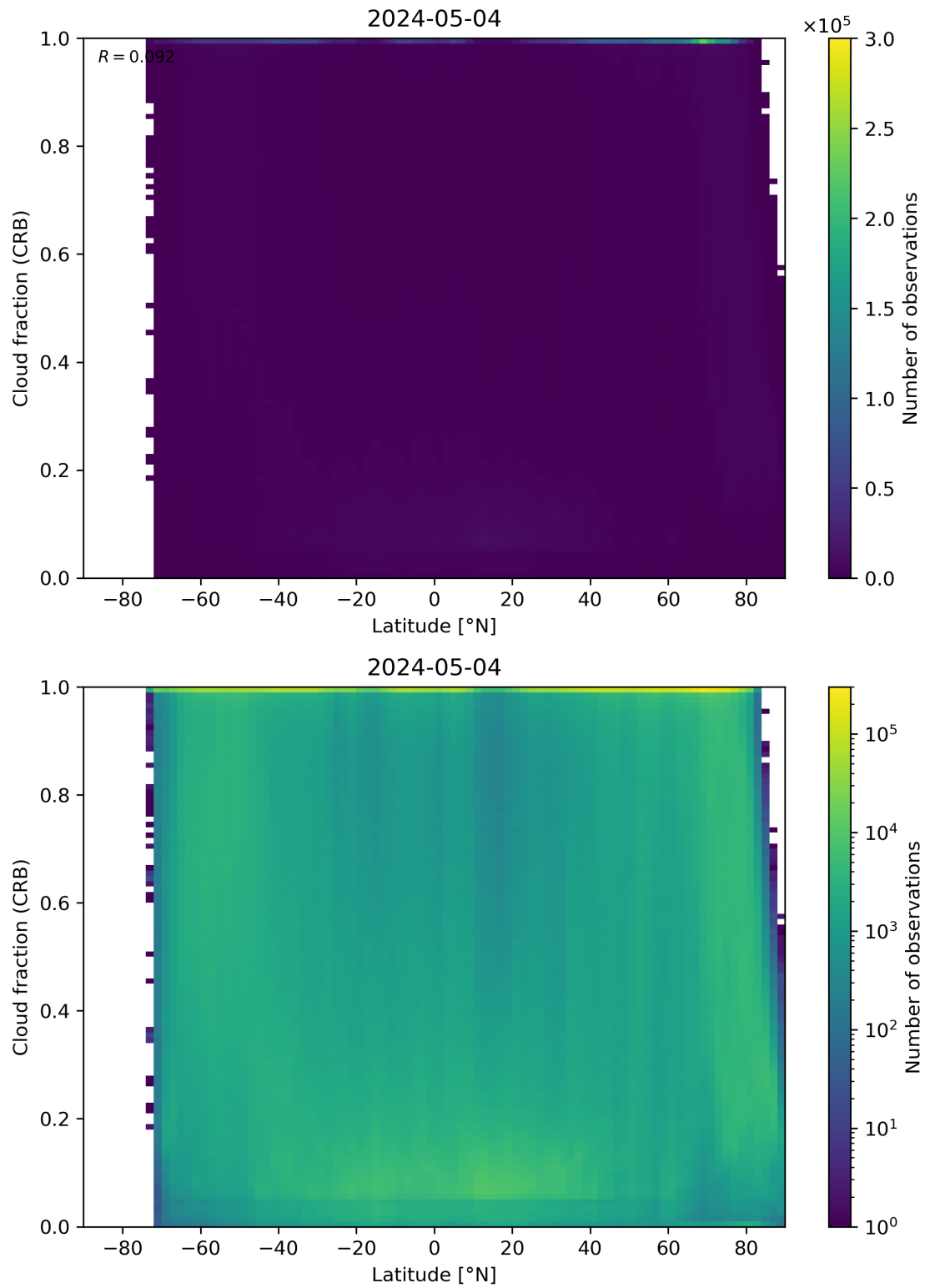
Figure 94: Scatter density plot of “Latitude” against “Cloud fraction (CRB)” for 2024-05-03 to 2024-05-05.
