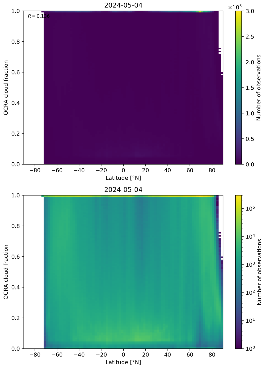
Figure 93: Scatter density plot of “Latitude” against “OCRA cloud fraction” for 2024-05-03 to 2024-05-05.
