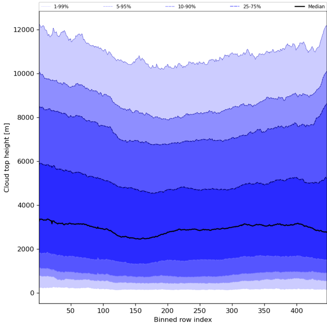
Figure 56: Along track statistics of “Cloud top height” for 2024-05-03 to 2024-05-05
