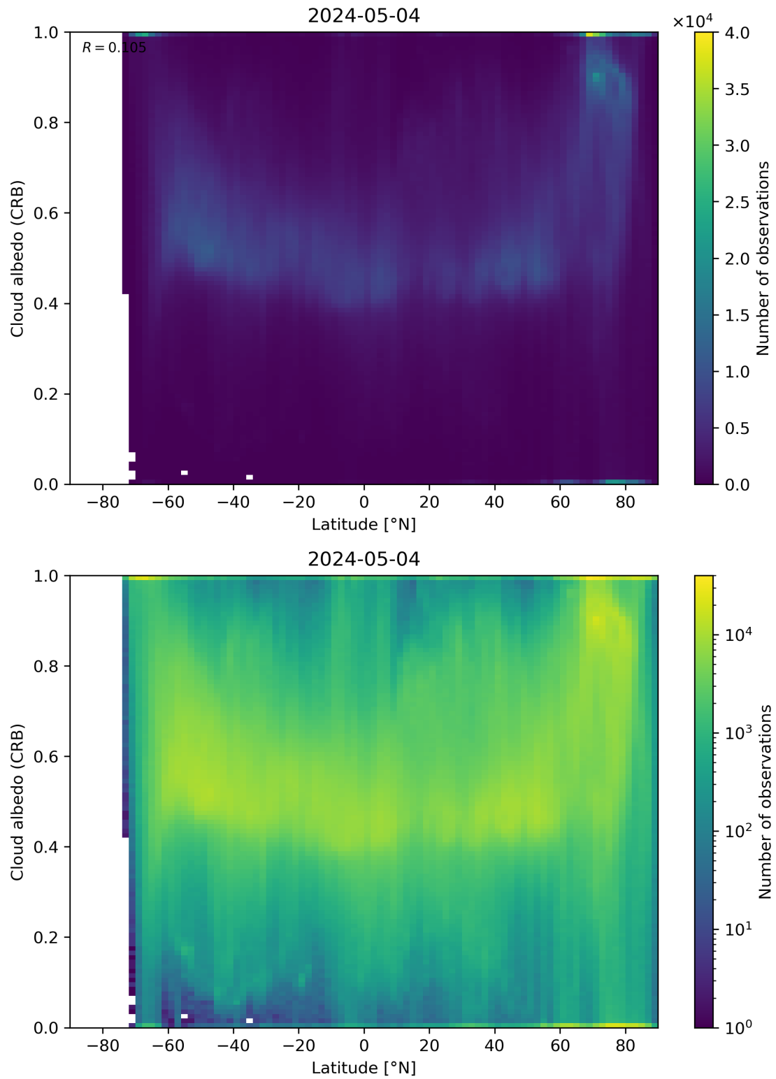
Figure 91: Scatter density plot of “Latitude” against “Cloud albedo (CRB)” for 2024-05-03 to 2024-05-05.
