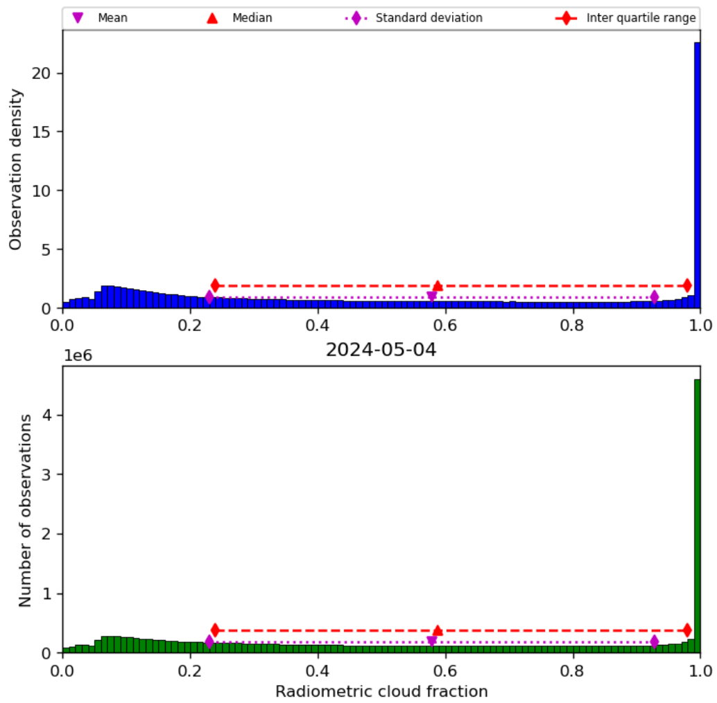
Figure 39: Histogram of “Radiometric cloud fraction” for 2024-05-03 to 2024-05-05
