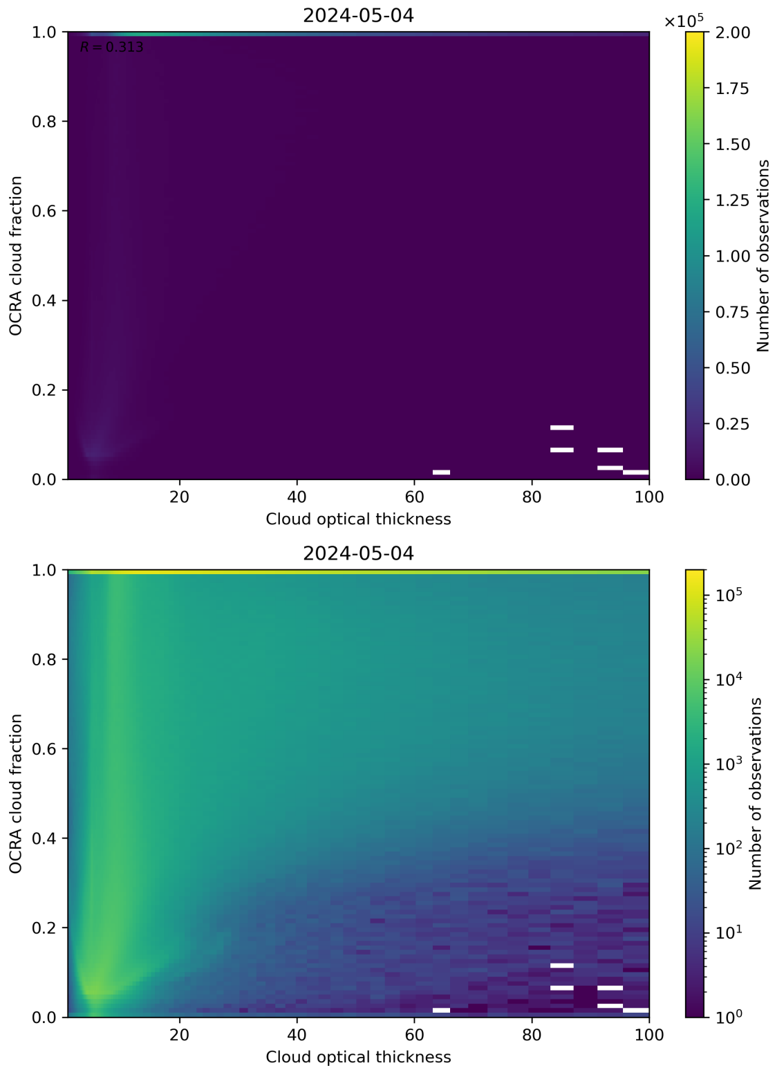
Figure 83: Scatter density plot of “Cloud optical thickness” against “OCRA cloud fraction” for 2024-05-03 to 2024-05-05.
