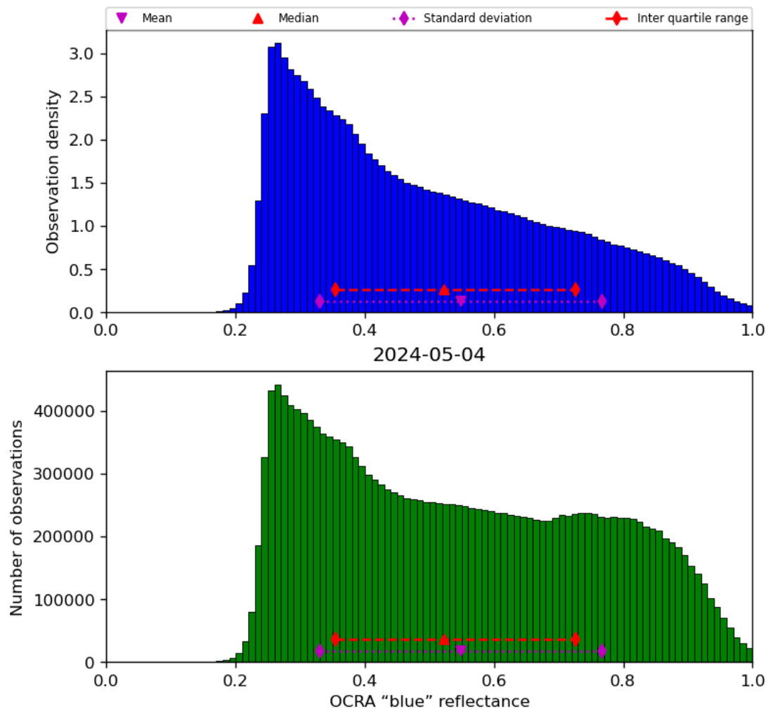
Figure 51: Histogram of “OCRA “blue” reflectance” for 2024-05-03 to 2024-05-05
