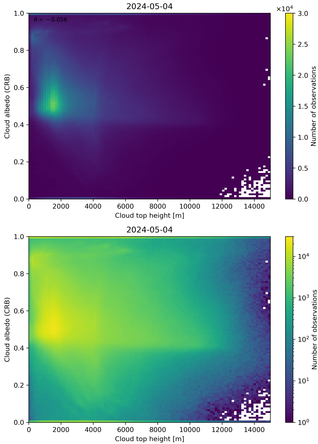
Figure 86: Scatter density plot of “Cloud top height” against “Cloud albedo (CRB)” for 2024-05-03 to 2024-05-05.
