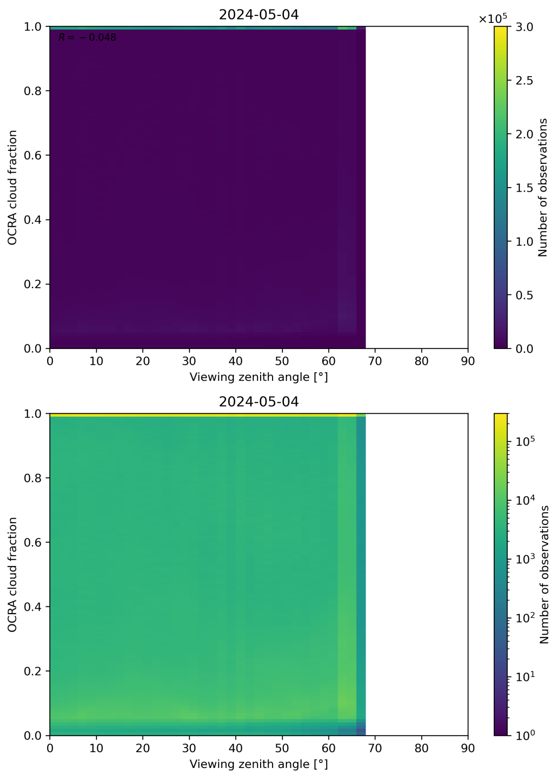
Figure 108: Scatter density plot of “Viewing zenith angle” against “OCRA cloud fraction” for 2024-05-03 to 2024-05-05.
