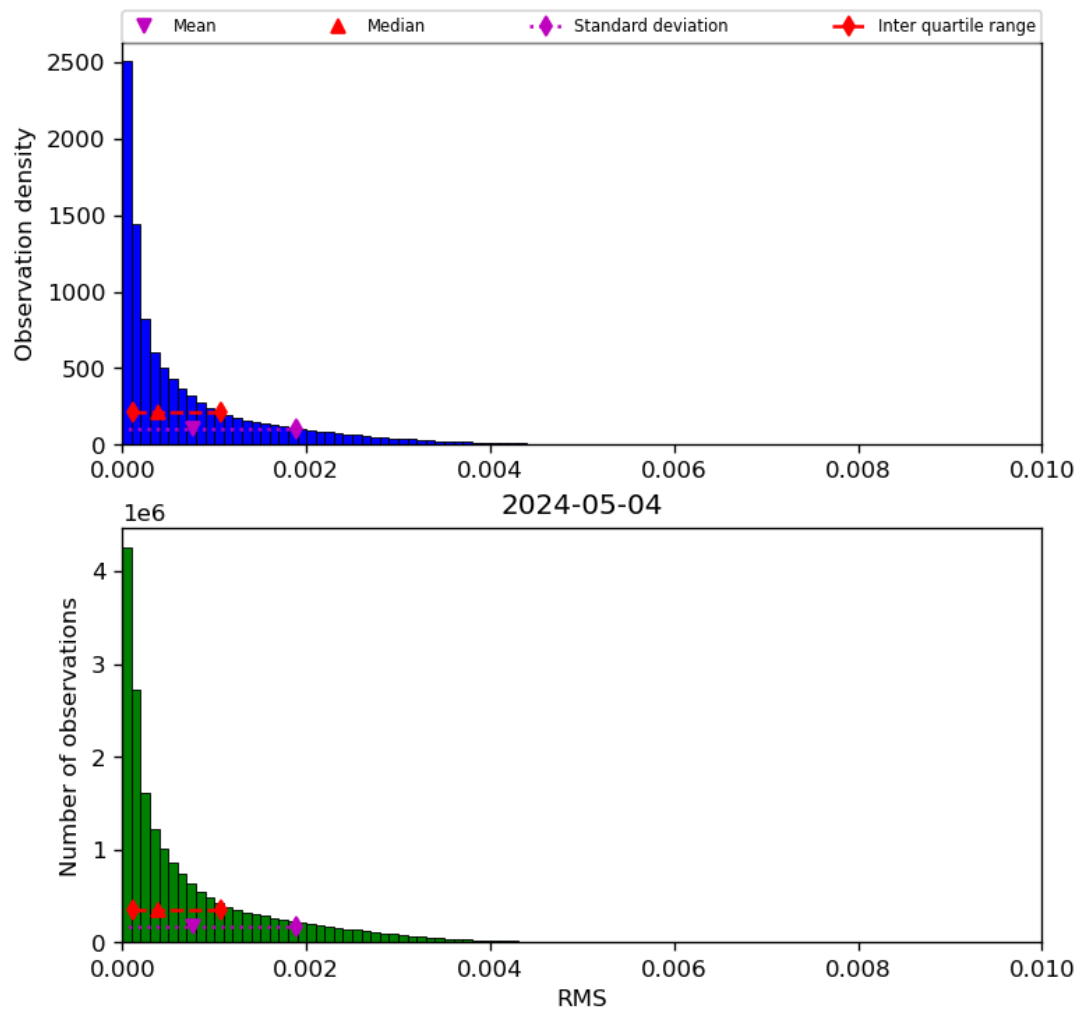
Figure 47: Histogram of “RMS” for 2024-05-03 to 2024-05-05
