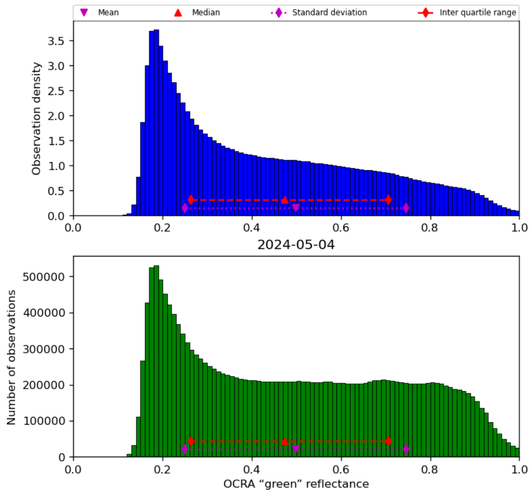
Figure 52: Histogram of “OCRA “green” reflectance” for 2024-05-03 to 2024-05-05
