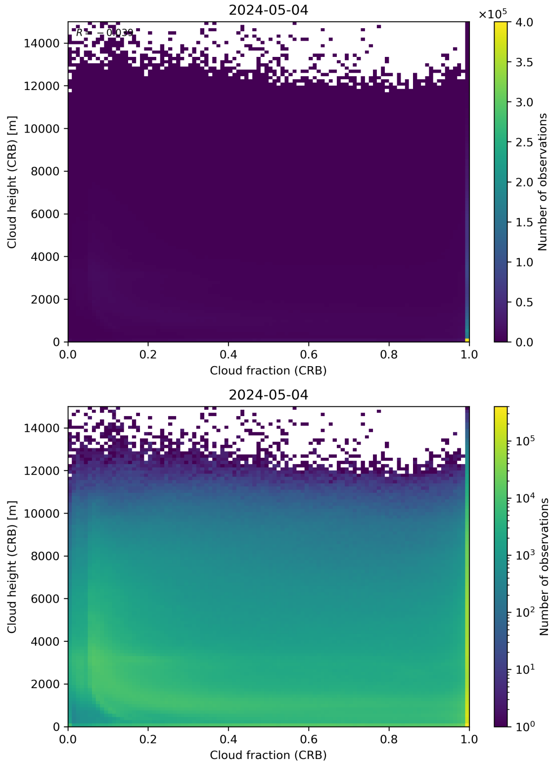
Figure 79: Scatter density plot of “Cloud fraction (CRB)” against “Cloud height (CRB)” for 2024-05-03 to 2024-05-05.
