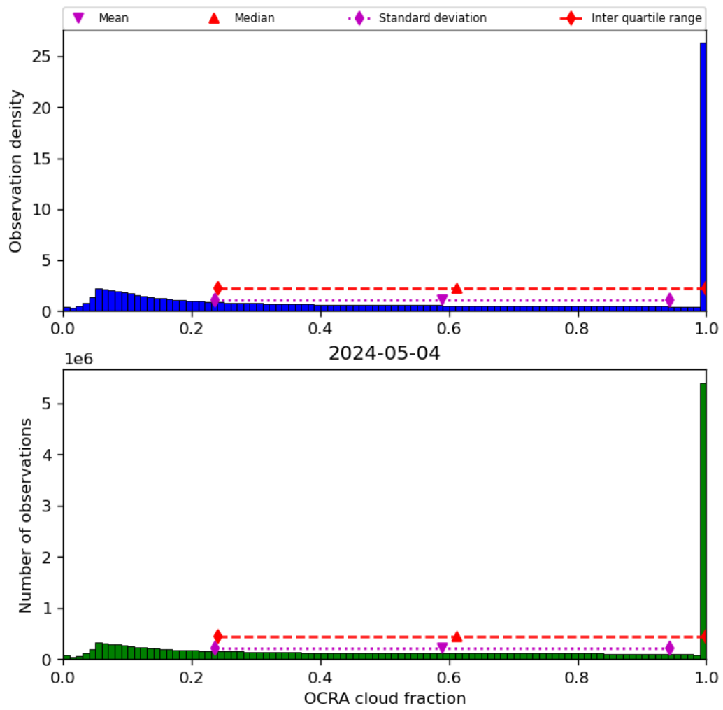
Figure 50: Histogram of “OCRA cloud fraction” for 2024-05-03 to 2024-05-05
