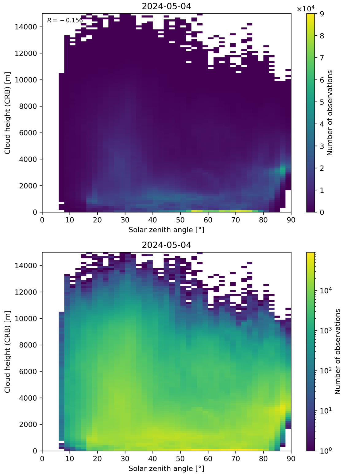
Figure 102: Scatter density plot of “Solar zenith angle” against “Cloud height (CRB)” for 2024-05-03 to 2024-05-05.
