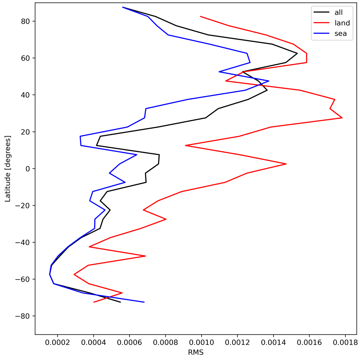
Figure 31: Zonal average of “RMS” for 2024-05-03 to 2024-05-05.
