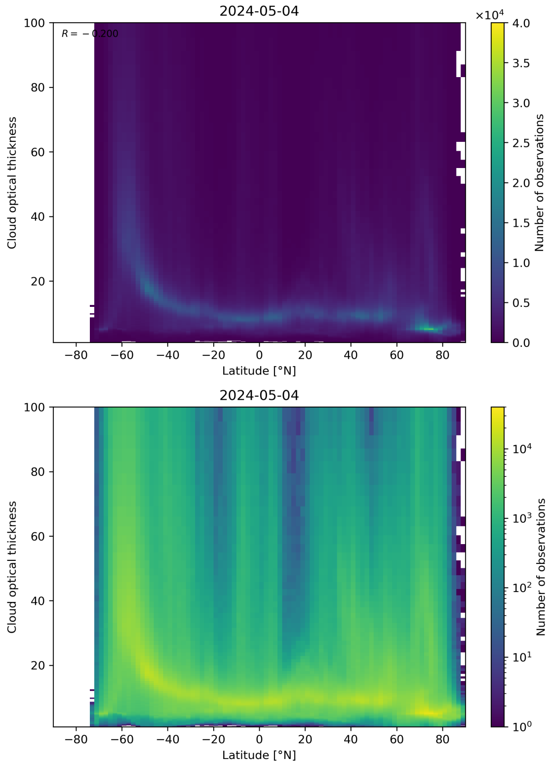
Figure 96: Scatter density plot of “Latitude” against “Cloud optical thickness” for 2024-05-03 to 2024-05-05.
