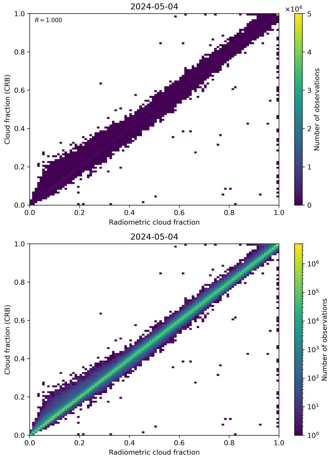
Figure 73: Scatter density plot of “Radiometric cloud fraction” against “Cloud fraction (CRB)” for 2024-05-03 to 2024-05-05.
