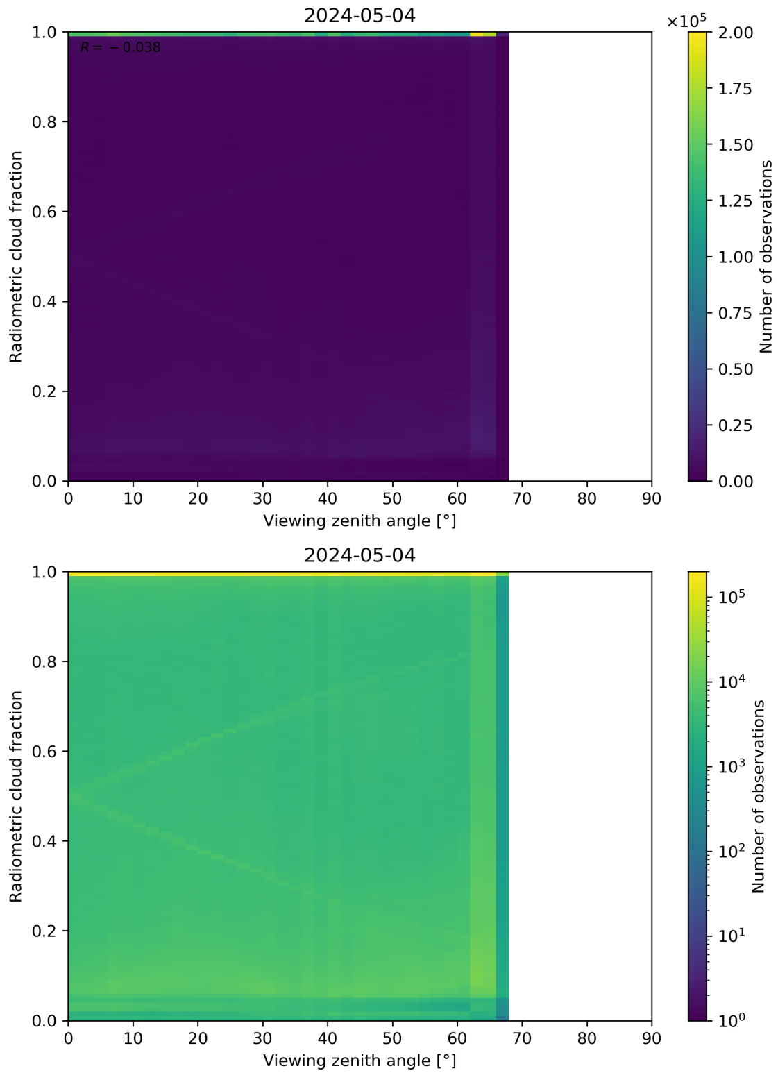
Figure 107: Scatter density plot of “Viewing zenith angle” against “Radiometric cloud fraction” for 2024-05-03 to 2024-05-05.
