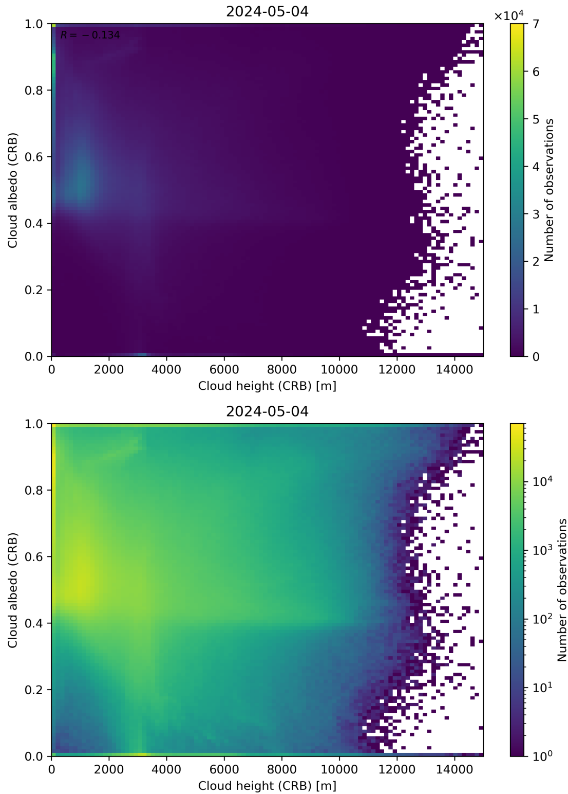
Figure 80: Scatter density plot of “Cloud height (CRB)” against “Cloud albedo (CRB)” for 2024-05-03 to 2024-05-05.
