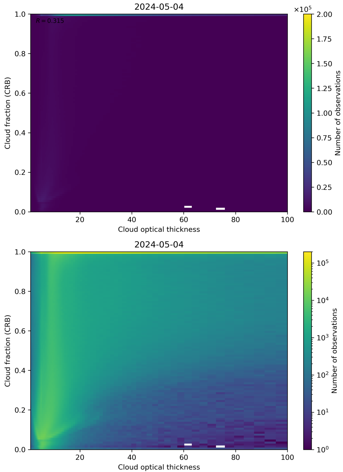
Figure 84: Scatter density plot of “Cloud optical thickness” against “Cloud fraction (CRB)” for 2024-05-03 to 2024-05-05.
