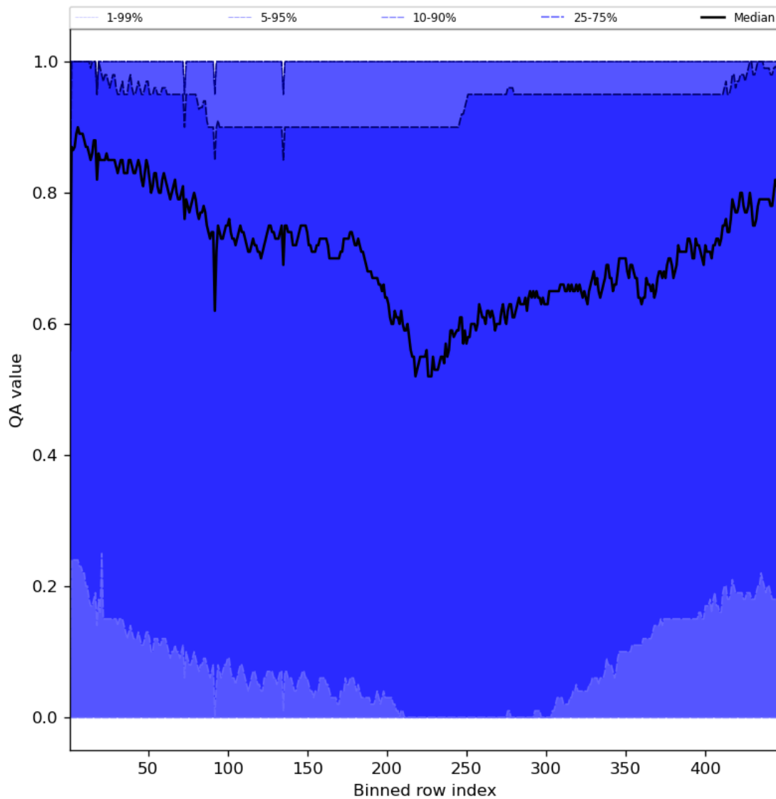
Figure 54: Along track statistics of “QA value” for 2024-05-03 to 2024-05-05
