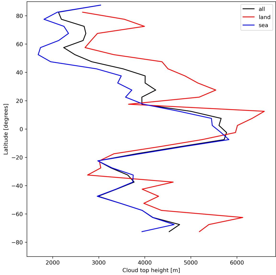
Figure 24: Zonal average of “Cloud top height” for 2024-05-03 to 2024-05-05.
