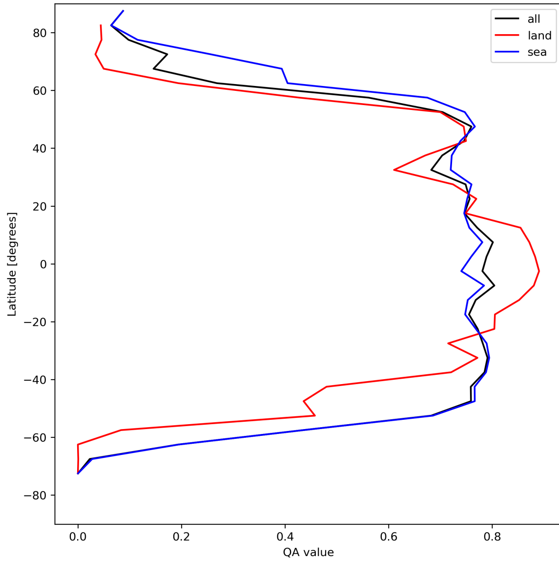
Figure 22: Zonal average of “QA value” for 2024-05-03 to 2024-05-05.
