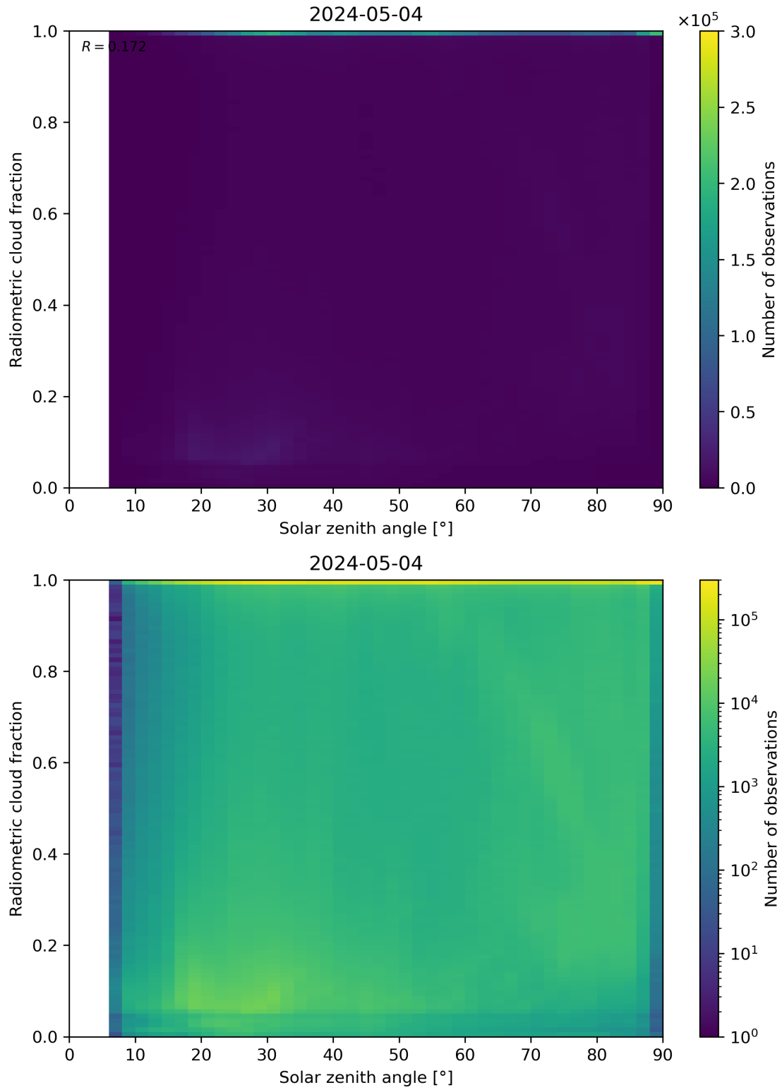
Figure 99: Scatter density plot of “Solar zenith angle” against “Radiometric cloud fraction” for 2024-05-03 to 2024-05-05.
