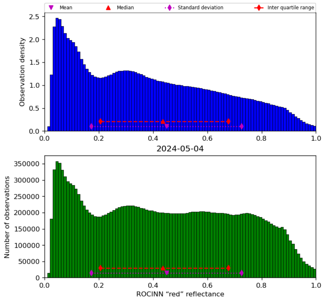
Figure 53: Histogram of “ROCINN “red” reflectance” for 2024-05-03 to 2024-05-05
