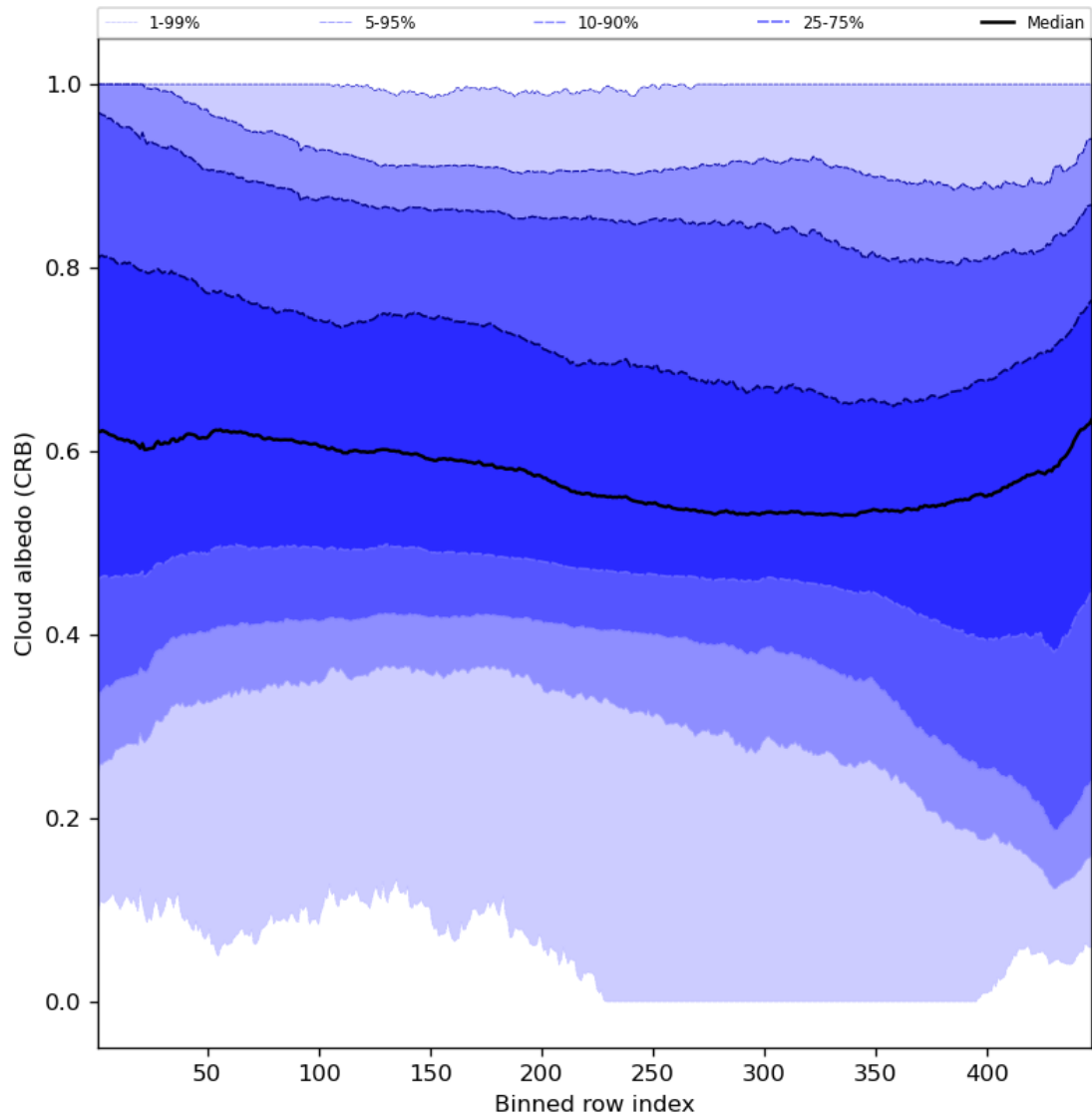
Figure 60: Along track statistics of “Cloud albedo (CRB)” for 2024-05-03 to 2024-05-05
