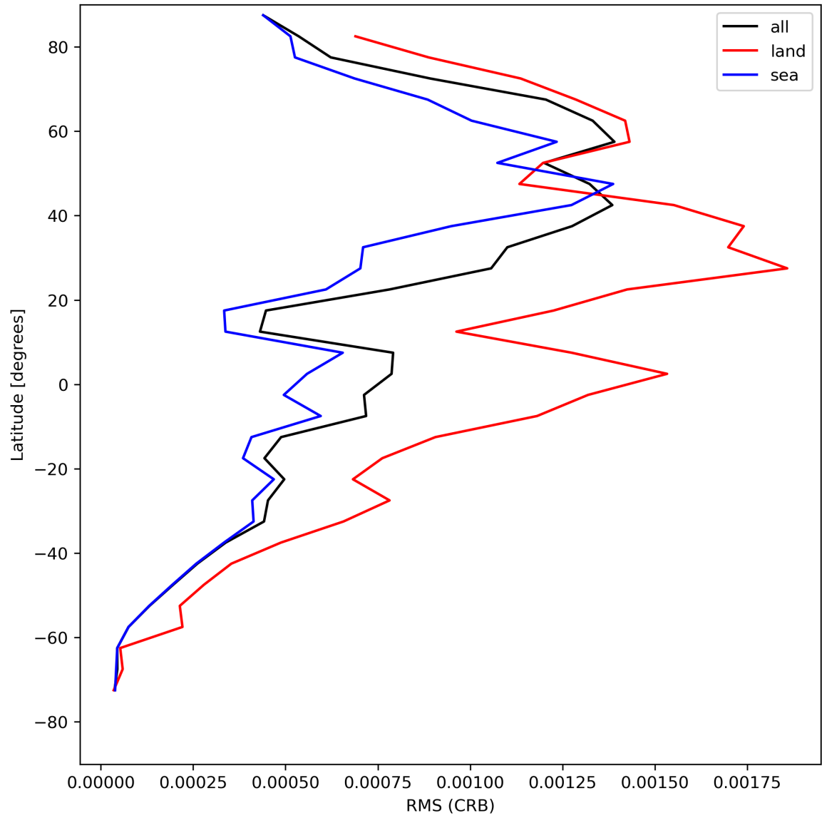
Figure 32: Zonal average of “RMS (CRB)” for 2024-05-03 to 2024-05-05.
