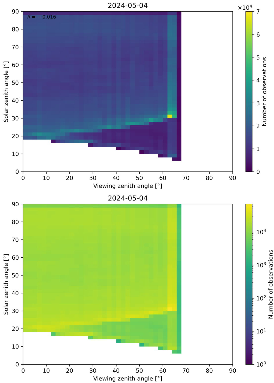
Figure 114: Scatter density plot of “Viewing zenith angle” against “Solar zenith angle” for 2024-05-03 to 2024-05-05.
