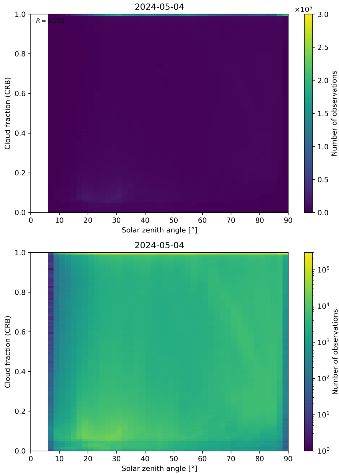
Figure 101: Scatter density plot of “Solar zenith angle” against “Cloud fraction (CRB)” for 2024-05-03 to 2024-05-05.
