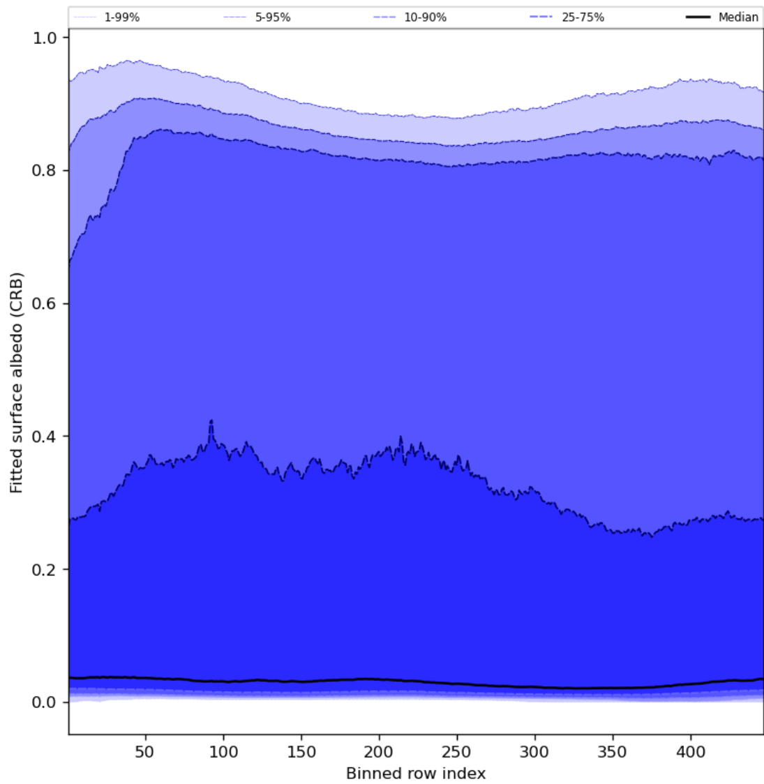
Figure 62: Along track statistics of “Fitted surface albedo (CRB)” for 2024-05-03 to 2024-05-05
