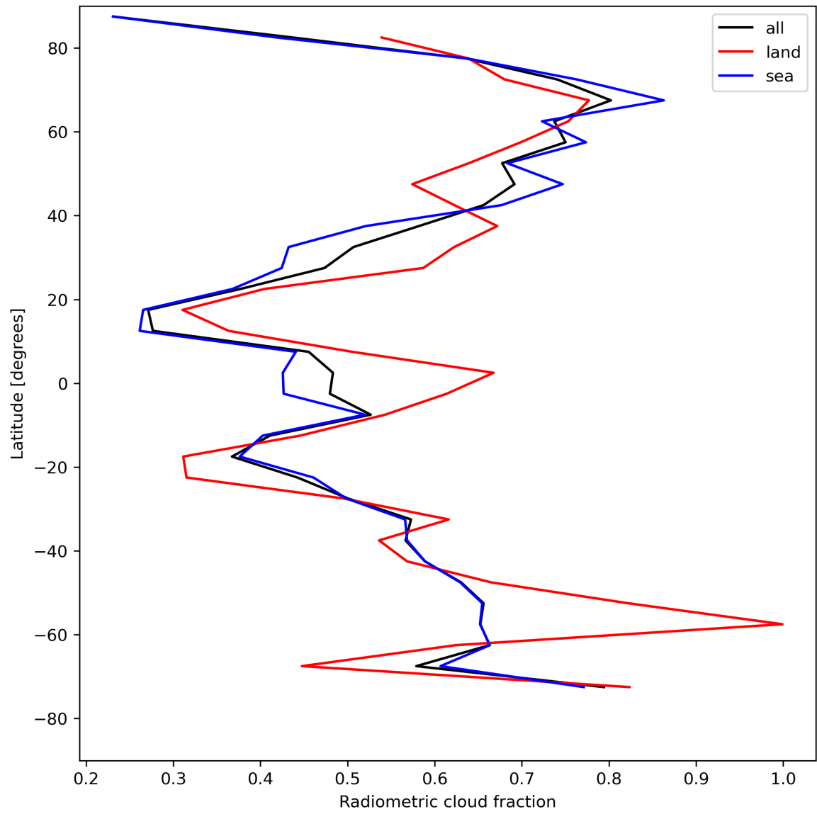
Figure 23: Zonal average of “Radiometric cloud fraction” for 2024-05-03 to 2024-05-05.
