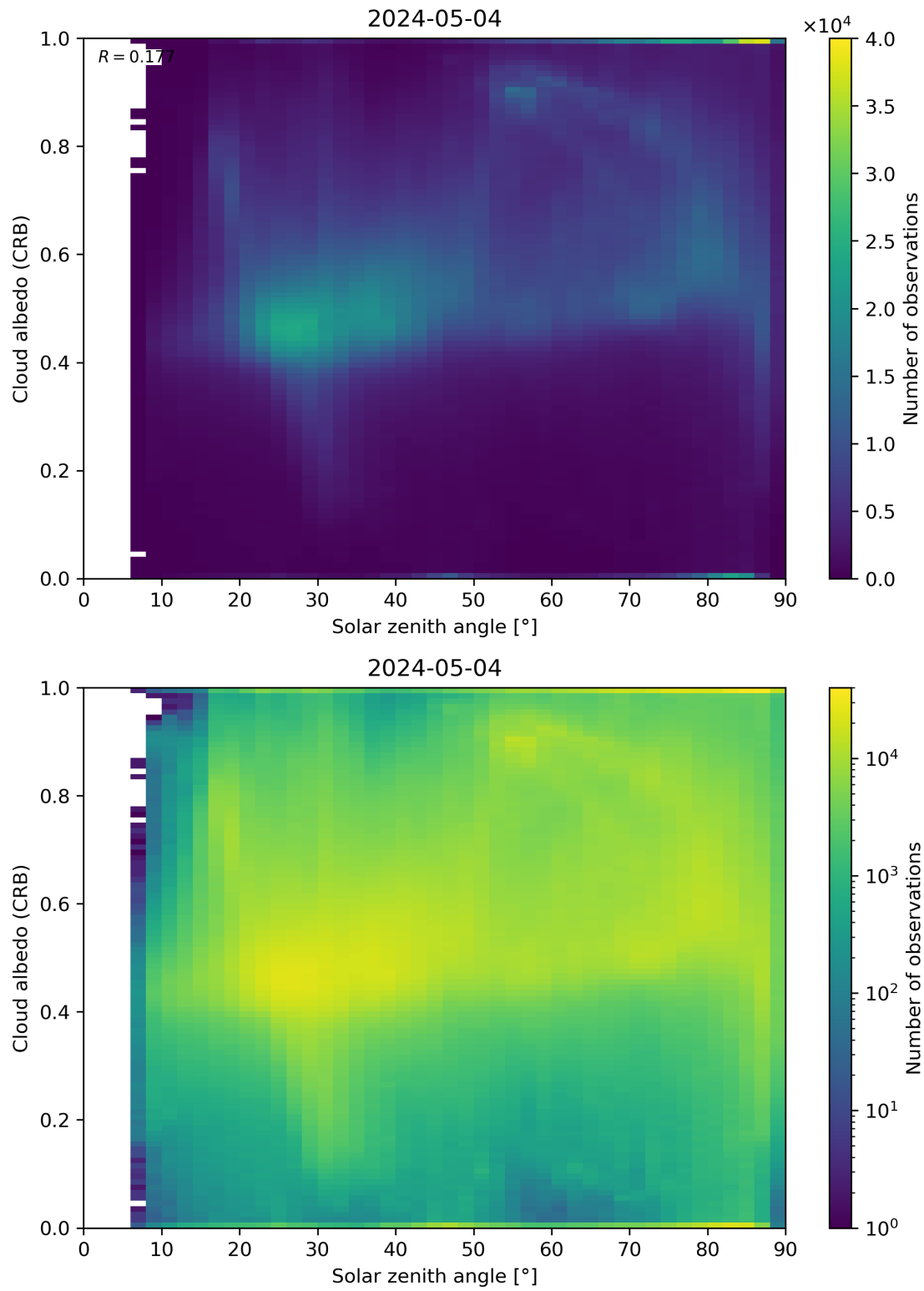
Figure 98: Scatter density plot of “Solar zenith angle” against “Cloud albedo (CRB)” for 2024-05-03 to 2024-05-05.
