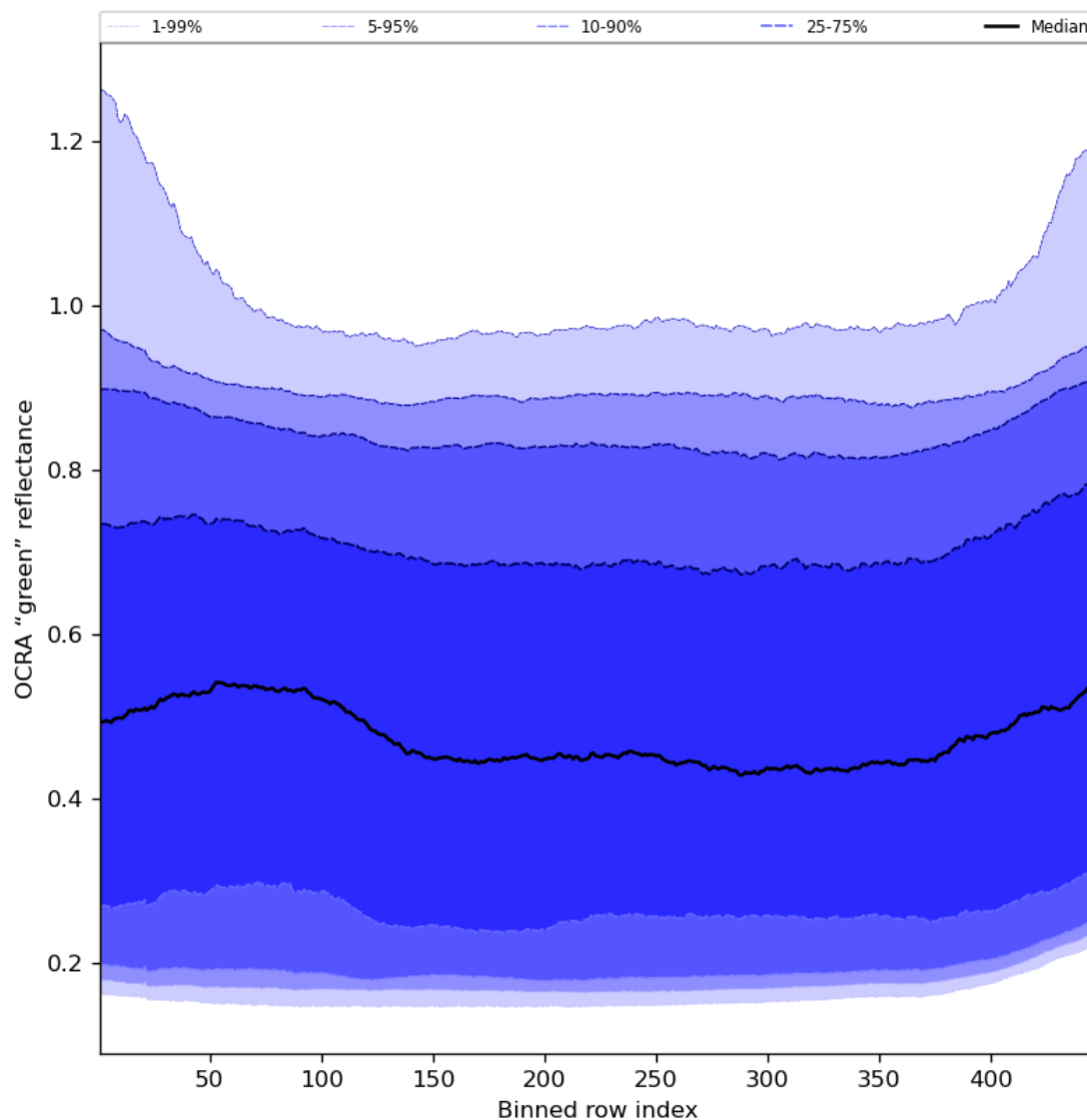
Figure 68: Along track statistics of “OCRA “green” reflectance” for 2024-05-03 to 2024-05-05
