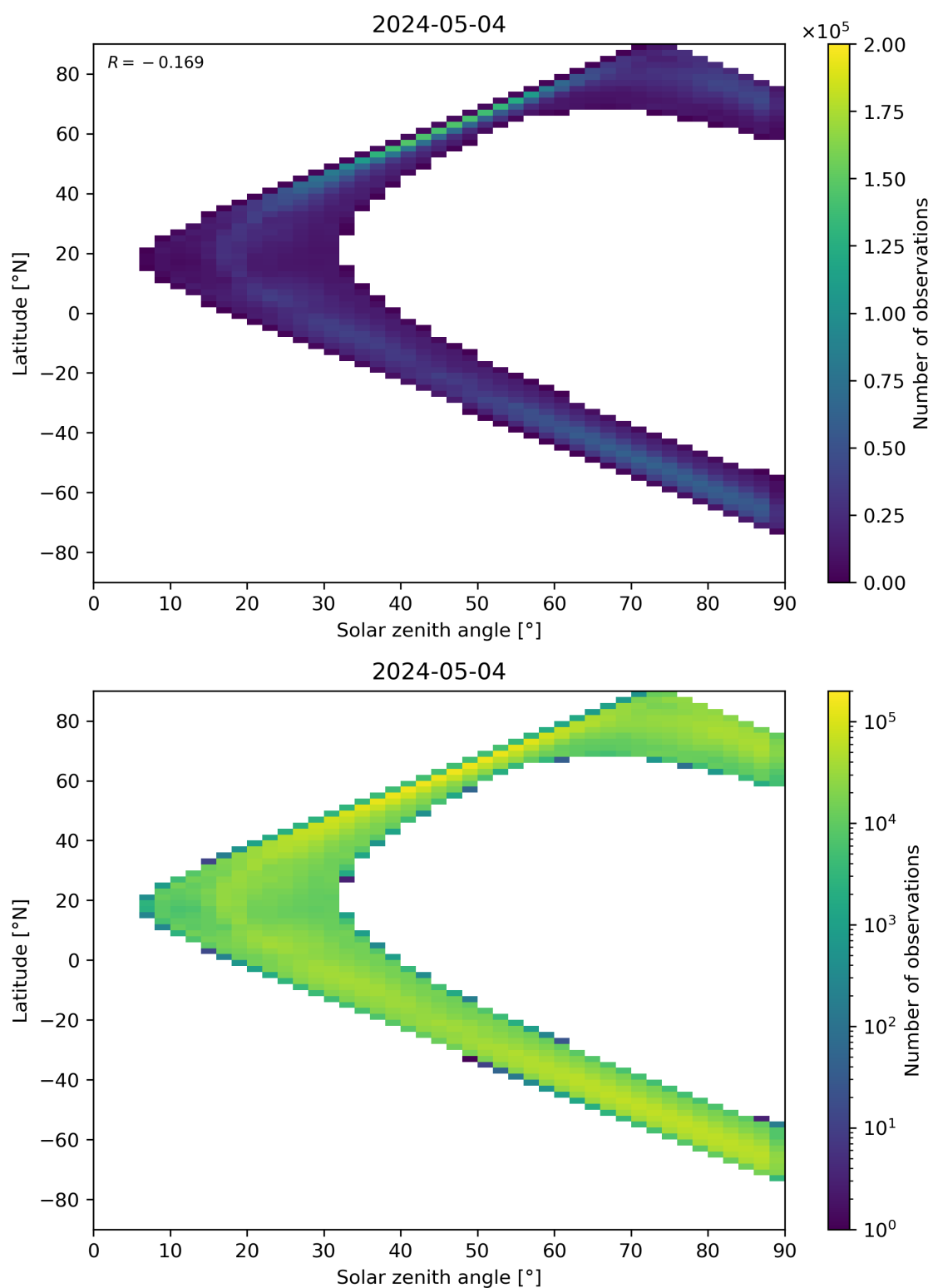
Figure 105: Scatter density plot of “Solar zenith angle” against “Latitude” for 2024-05-03 to 2024-05-05.
