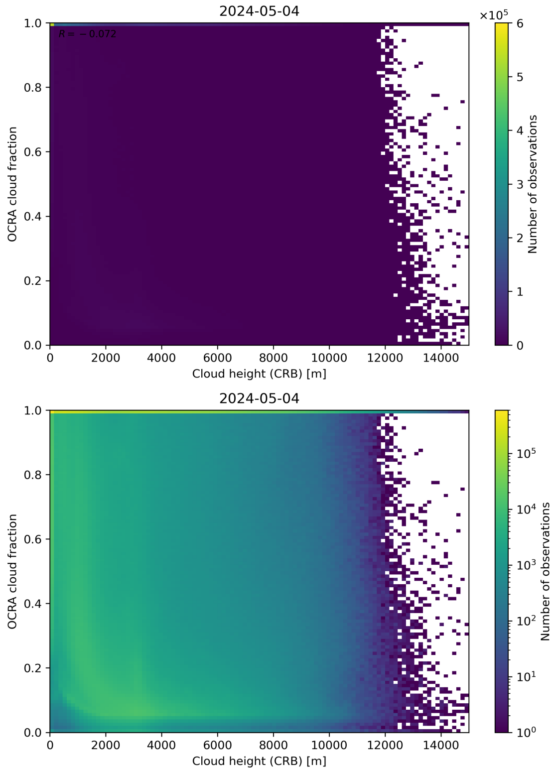
Figure 81: Scatter density plot of “Cloud height (CRB)” against “OCRA cloud fraction” for 2024-05-03 to 2024-05-05.
