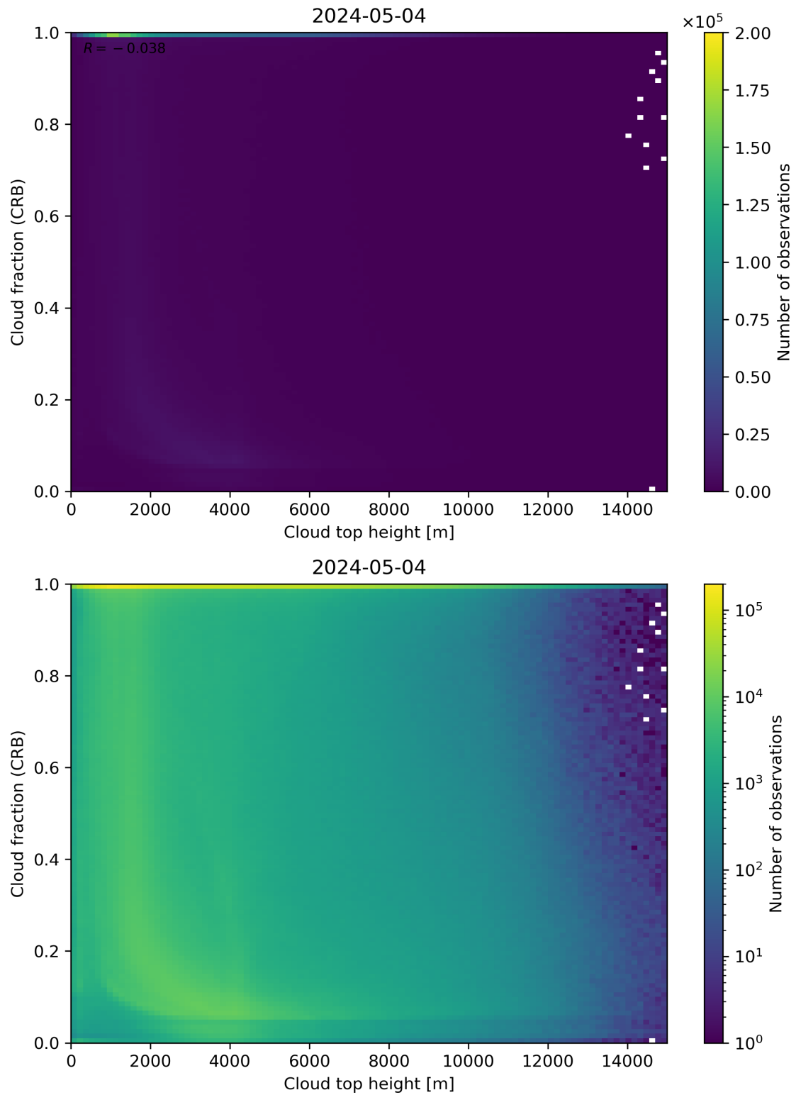
Figure 88: Scatter density plot of “Cloud top height” against “Cloud fraction (CRB)” for 2024-05-03 to 2024-05-05.
