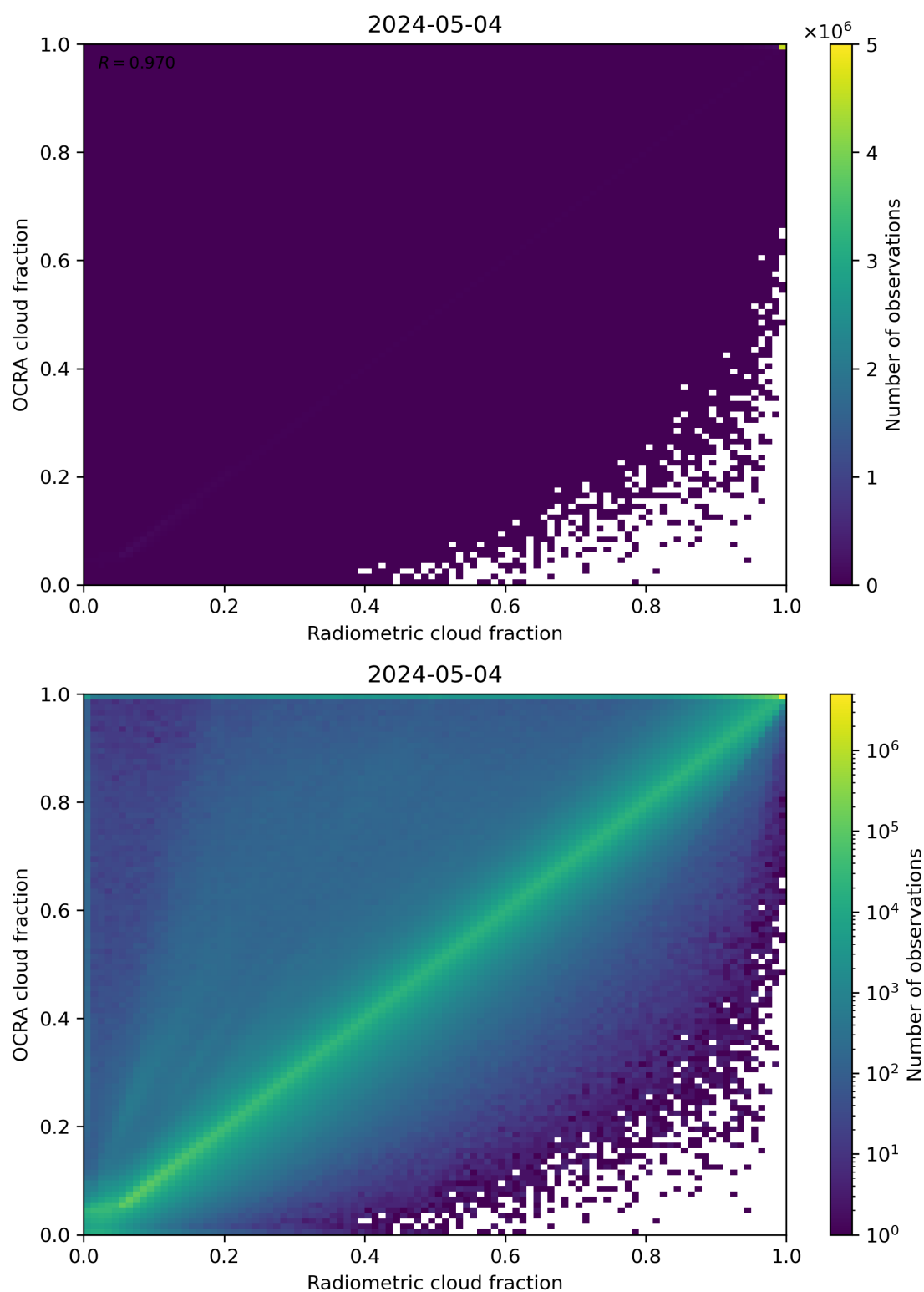
Figure 72: Scatter density plot of “Radiometric cloud fraction” against “OCRA cloud fraction” for 2024-05-03 to 2024-05-05.
