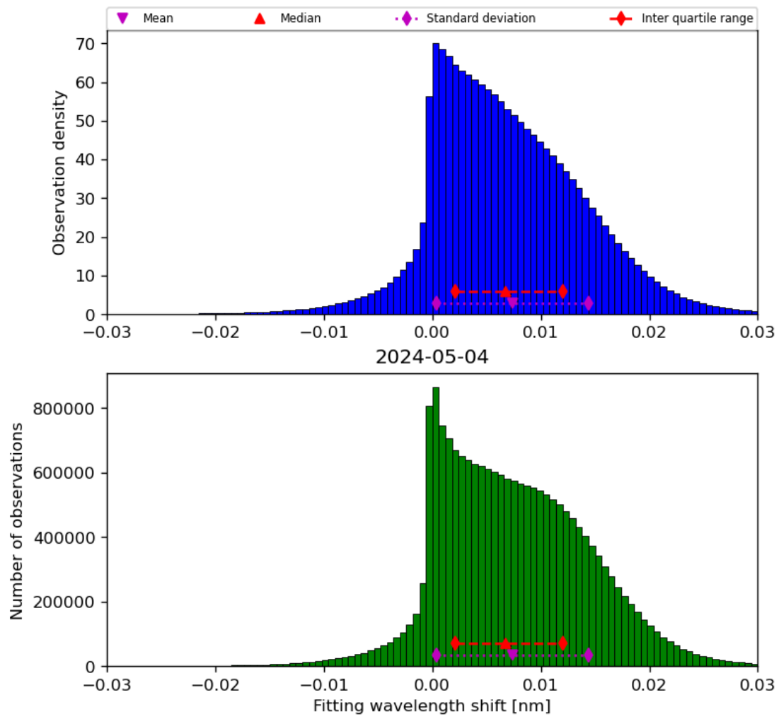
Figure 49: Histogram of “Fitting wavelength shift” for 2024-05-03 to 2024-05-05
