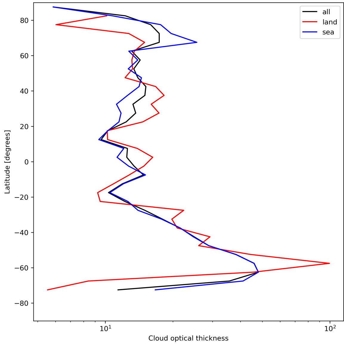
Figure 25: Zonal average of “Cloud optical thickness” for 2024-05-03 to 2024-05-05.
