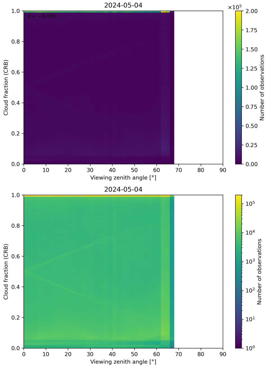
Figure 109: Scatter density plot of “Viewing zenith angle” against “Cloud fraction (CRB)” for 2024-05-03 to 2024-05-05.
