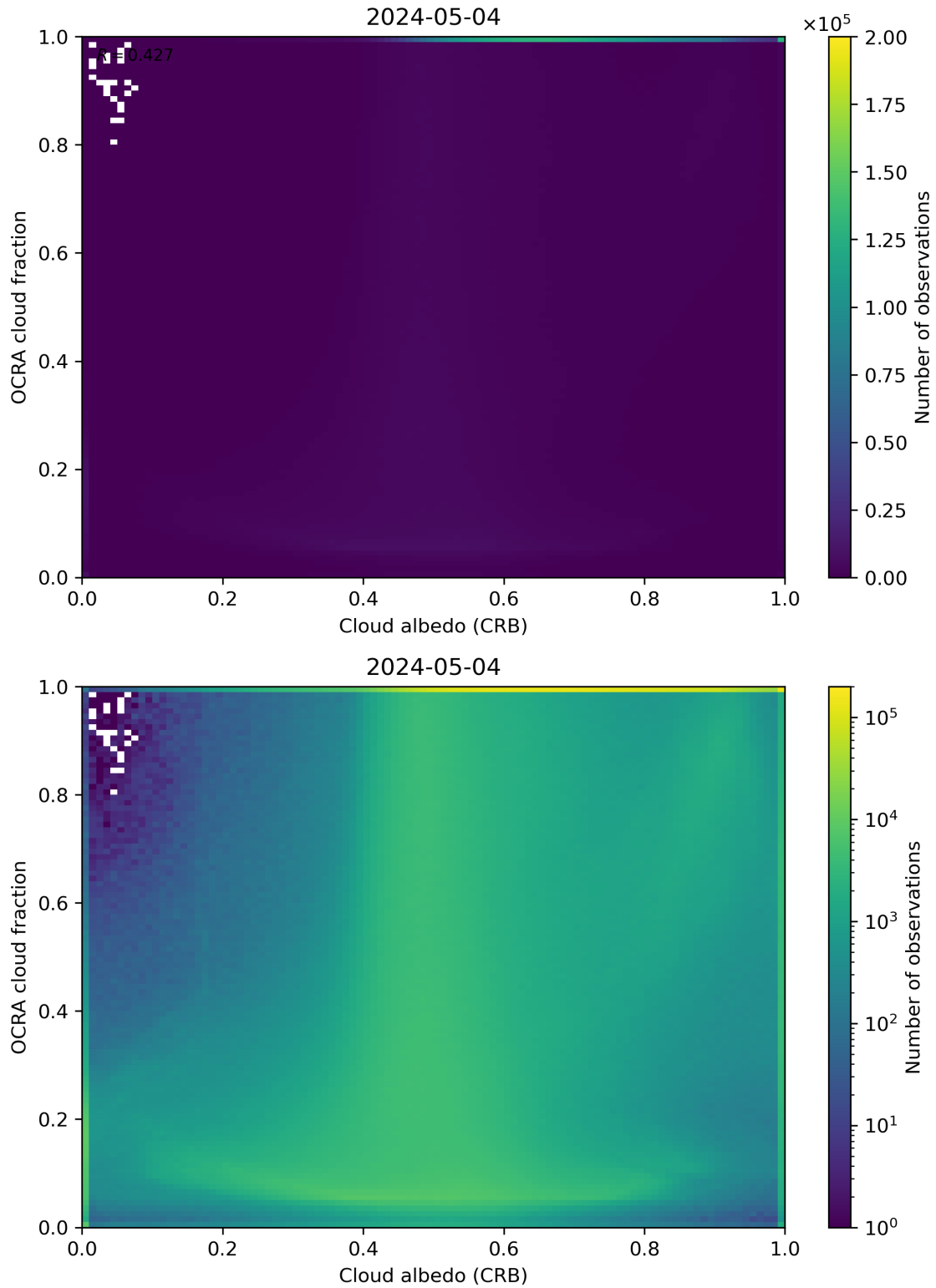
Figure 70: Scatter density plot of “Cloud albedo (CRB)” against “OCRA cloud fraction” for 2024-05-03 to 2024-05-05.
