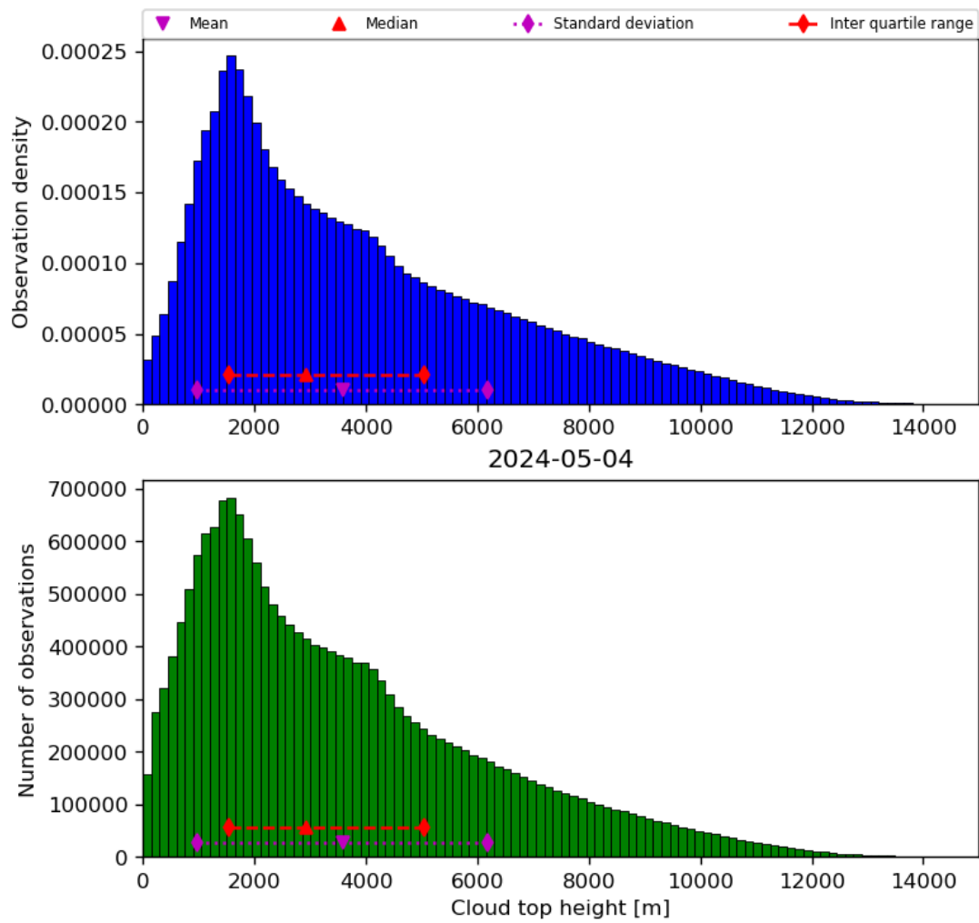
Figure 40: Histogram of “Cloud top height” for 2024-05-03 to 2024-05-05
