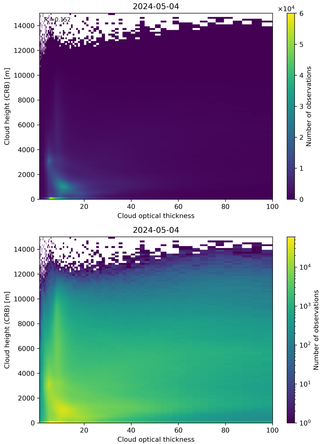
Figure 85: Scatter density plot of “Cloud optical thickness” against “Cloud height (CRB)” for 2024-05-03 to 2024-05-05.
