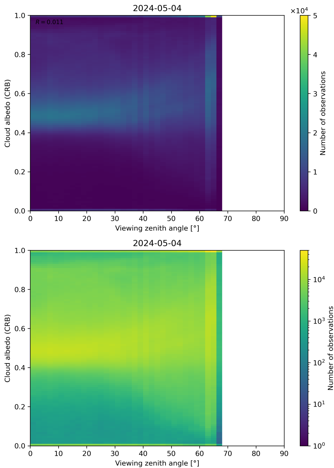
Figure 106: Scatter density plot of “Viewing zenith angle” against “Cloud albedo (CRB)” for 2024-05-03 to 2024-05-05.
