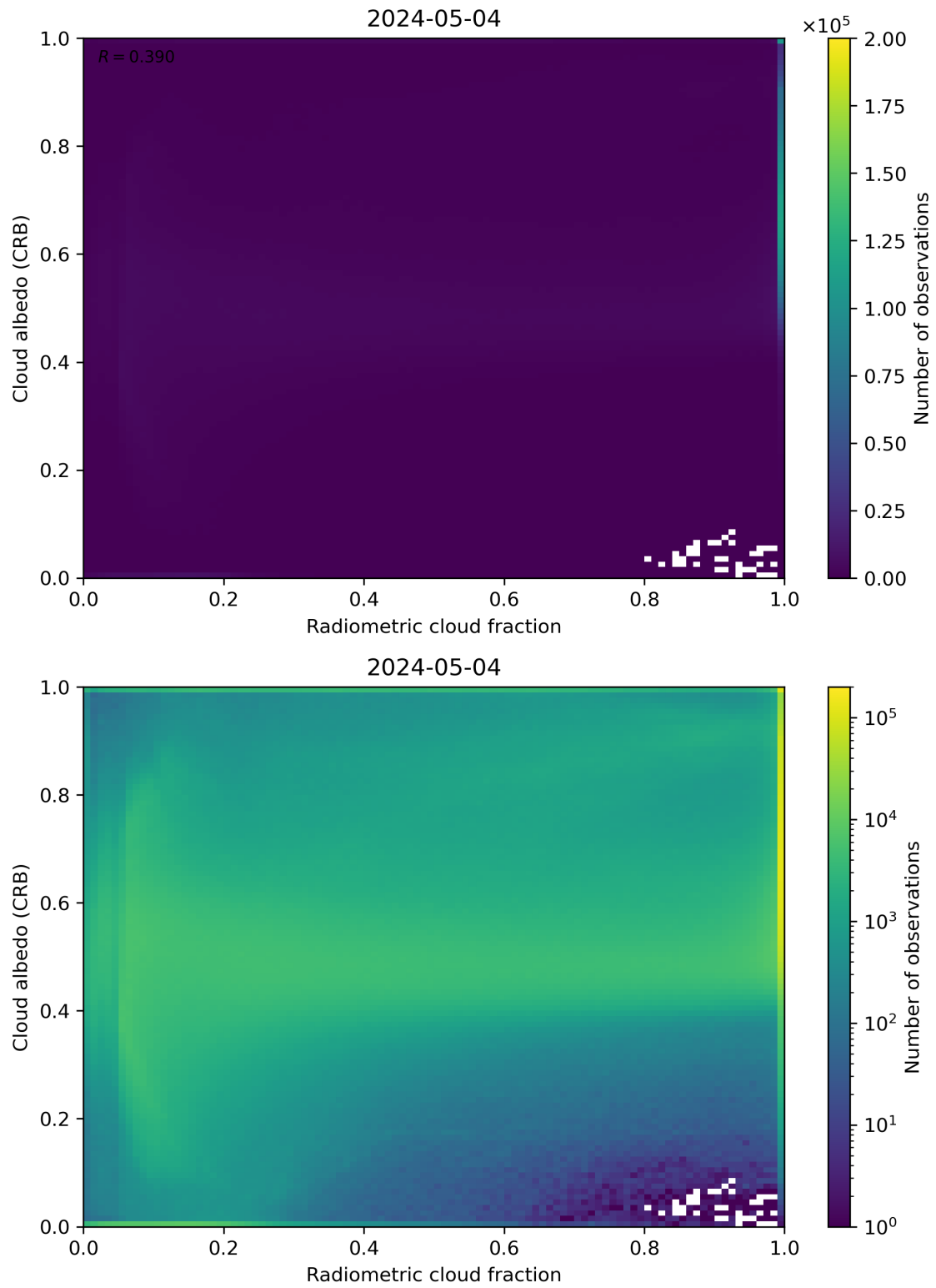
Figure 71: Scatter density plot of “Radiometric cloud fraction” against “Cloud albedo (CRB)” for 2024-05-03 to 2024-05-05.
