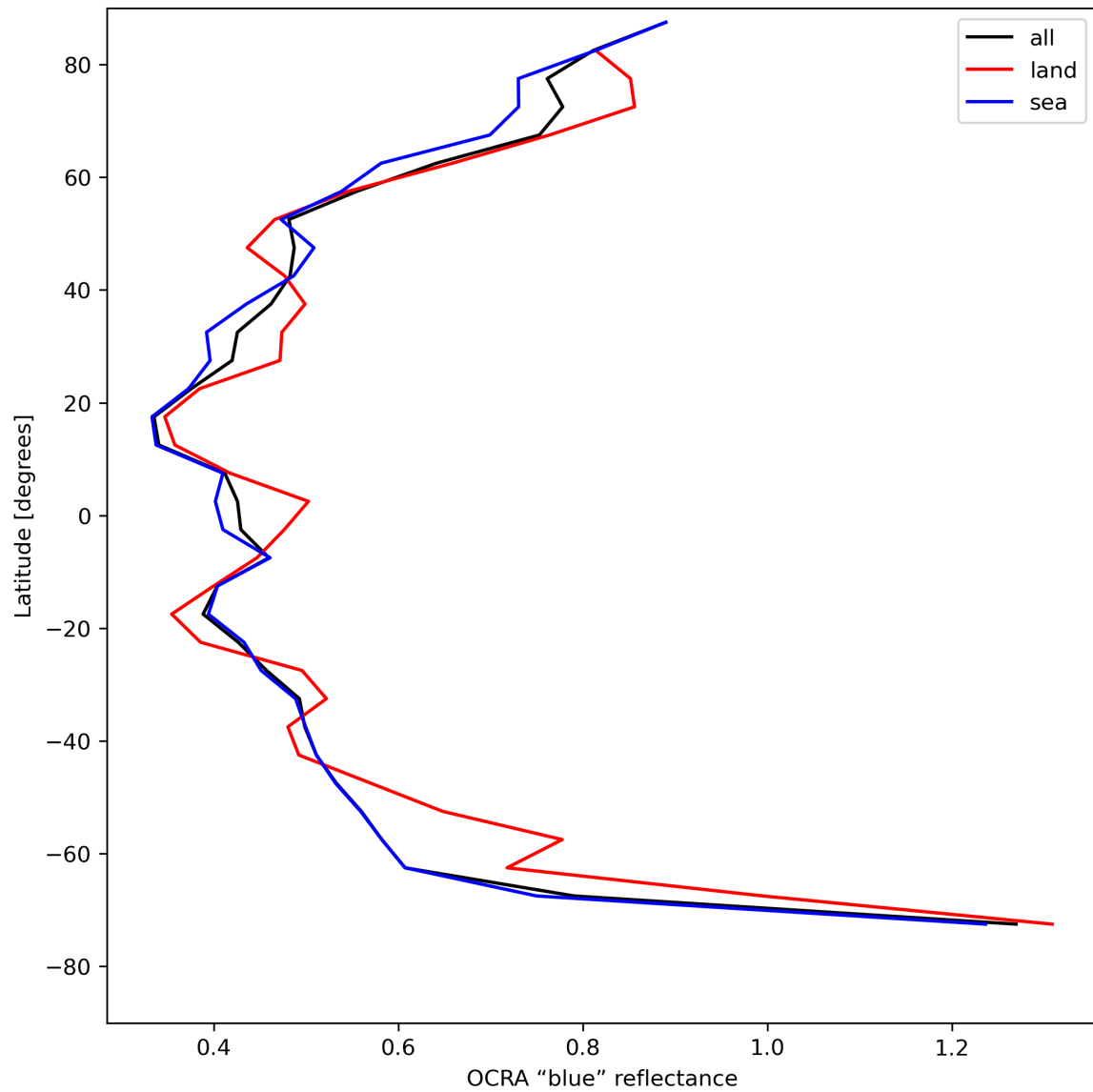
Figure 35: Zonal average of “OCRA “blue” reflectance” for 2024-05-03 to 2024-05-05.
