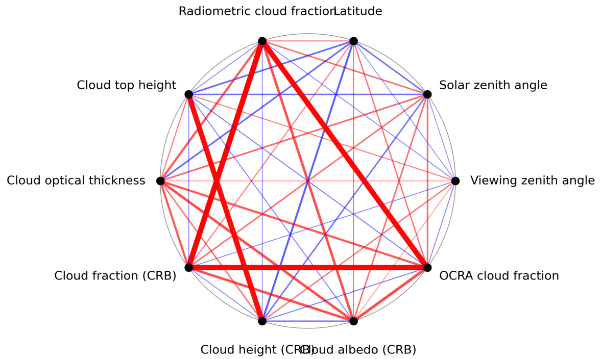
Figure 1: Map of correlation graph for 2024-05-03 to 2024-05-05.
