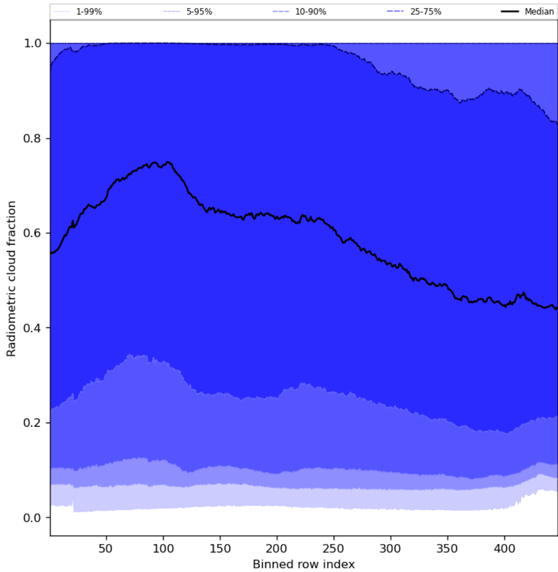
Figure 55: Along track statistics of “Radiometric cloud fraction” for 2024-05-03 to 2024-05-05
