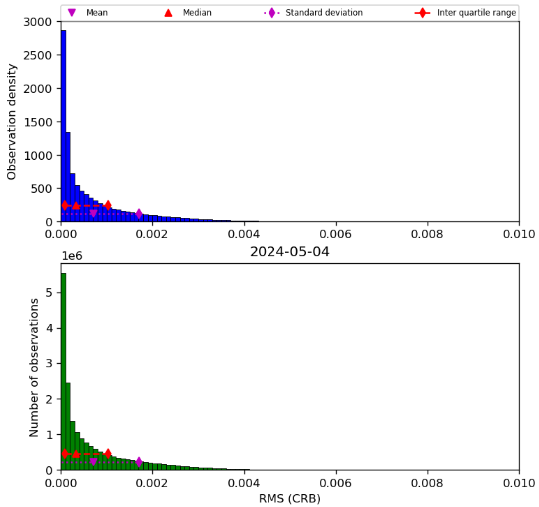
Figure 48: Histogram of “RMS (CRB)” for 2024-05-03 to 2024-05-05
