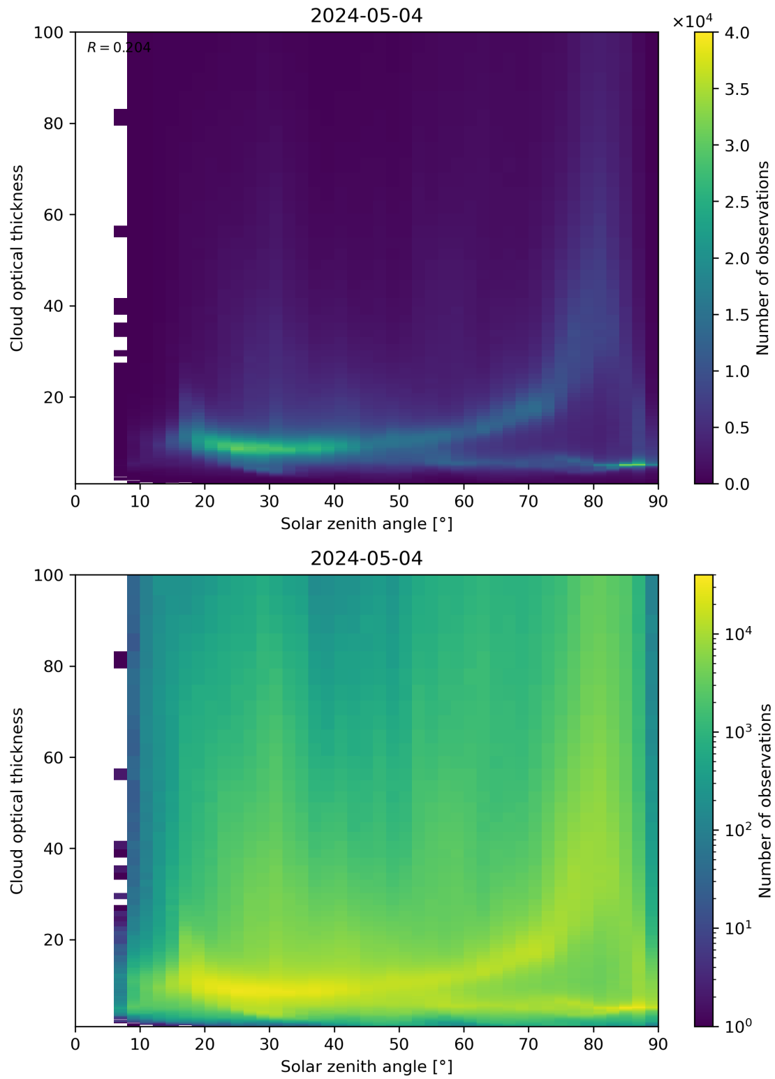
Figure 103: Scatter density plot of “Solar zenith angle” against “Cloud optical thickness” for 2024-05-03 to 2024-05-05.
