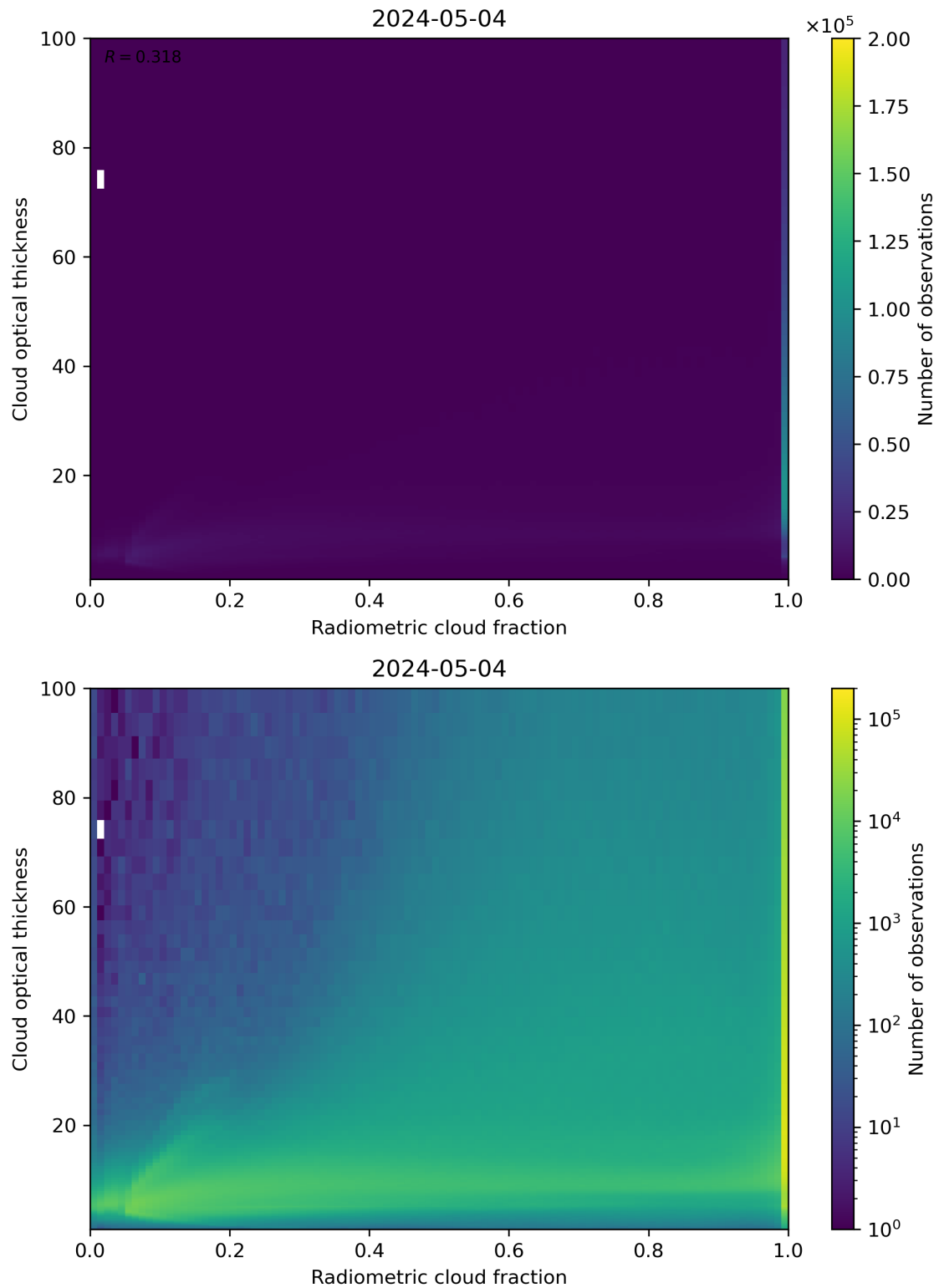
Figure 75: Scatter density plot of “Radiometric cloud fraction” against “Cloud optical thickness” for 2024-05-03 to 2024-05-05.
