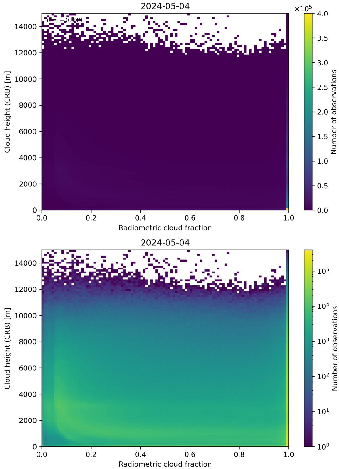
Figure 74: Scatter density plot of “Radiometric cloud fraction” against “Cloud height (CRB)” for 2024-05-03 to 2024-05-05.
