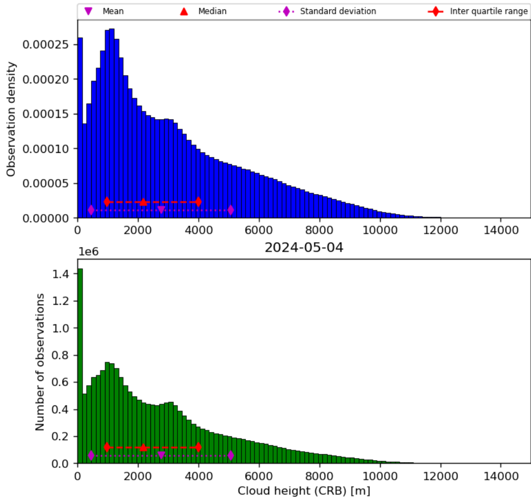
Figure 43: Histogram of “Cloud height (CRB)” for 2024-05-03 to 2024-05-05
