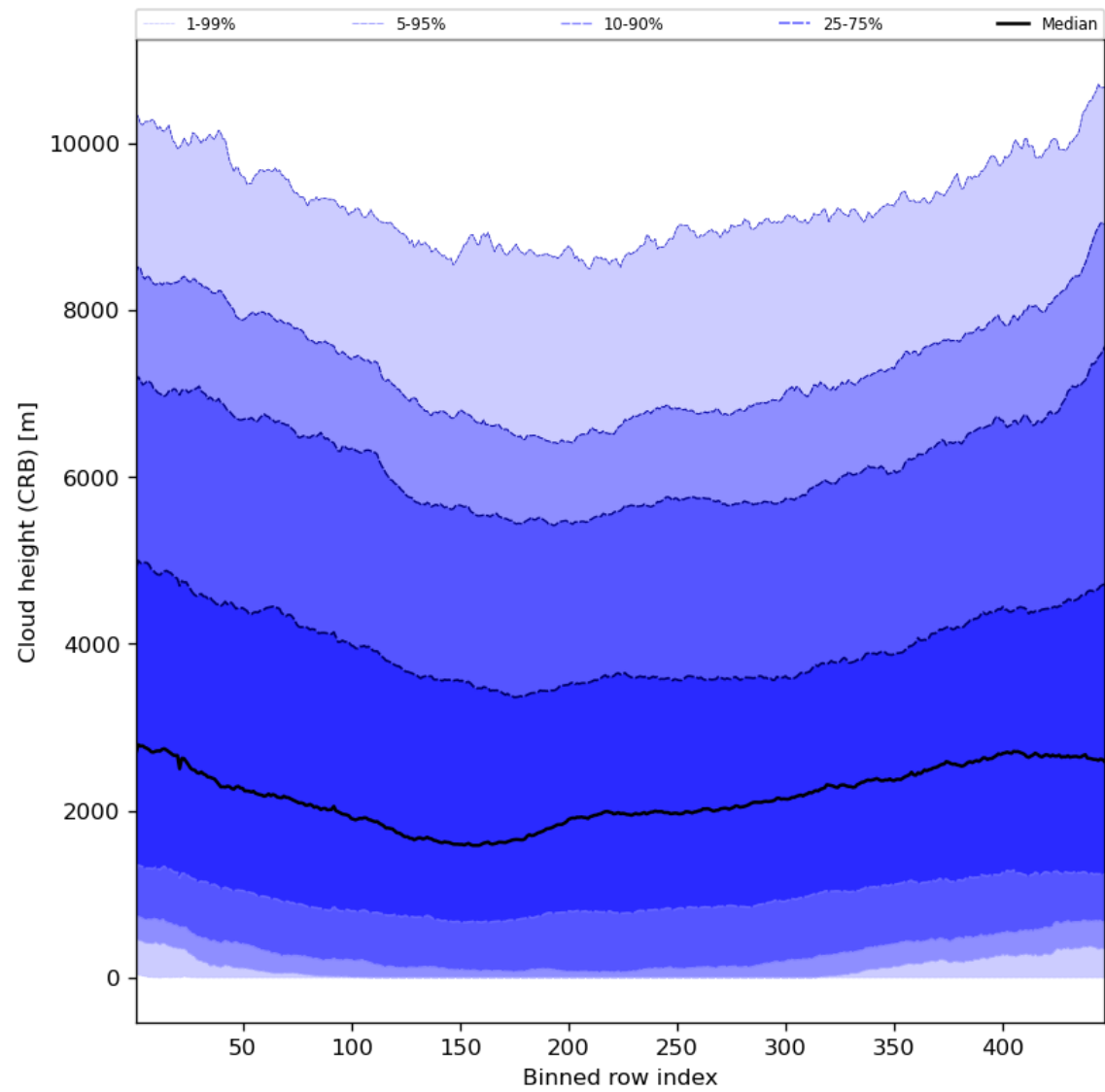
Figure 59: Along track statistics of “Cloud height (CRB)” for 2024-05-03 to 2024-05-05
