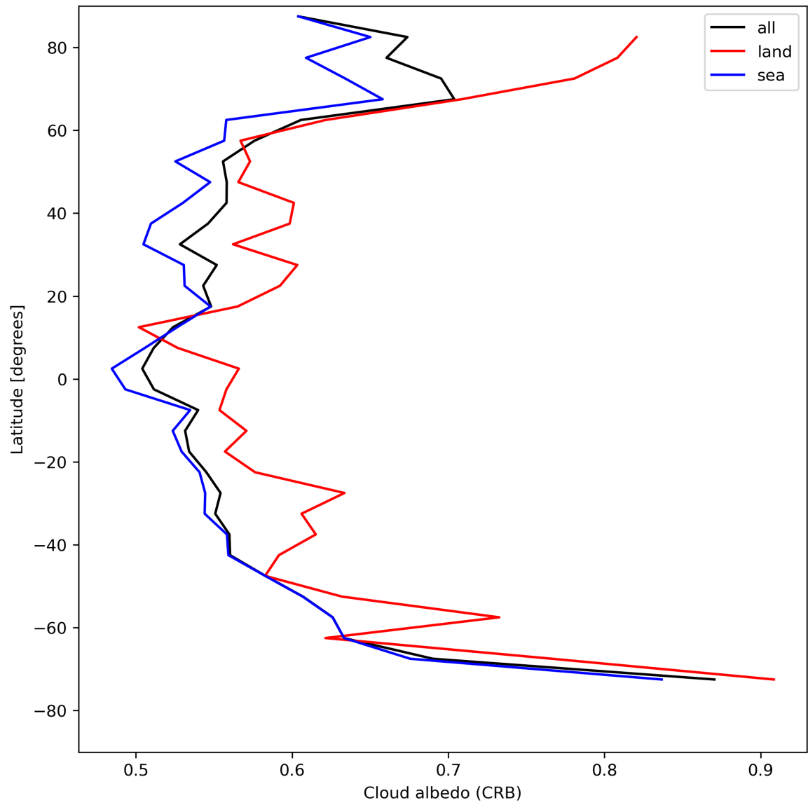
Figure 28: Zonal average of “Cloud albedo (CRB)” for 2024-05-03 to 2024-05-05.
