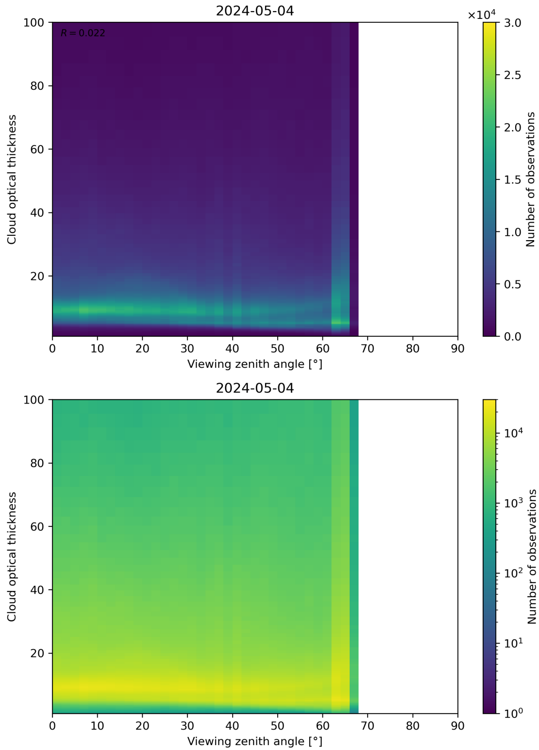
Figure 111: Scatter density plot of “Viewing zenith angle” against “Cloud optical thickness” for 2024-05-03 to 2024-05-05.
