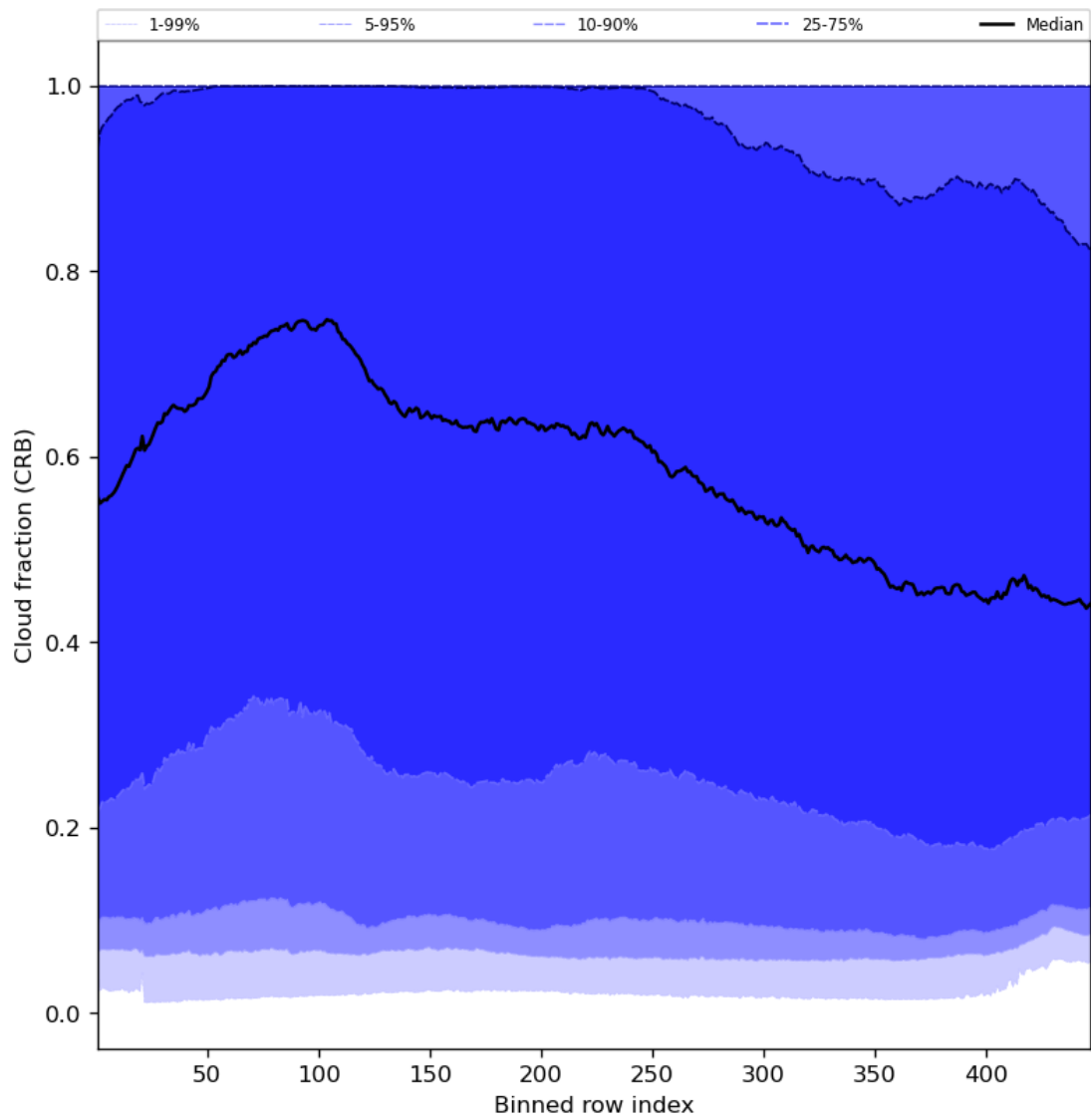
Figure 58: Along track statistics of “Cloud fraction (CRB)” for 2024-05-03 to 2024-05-05
