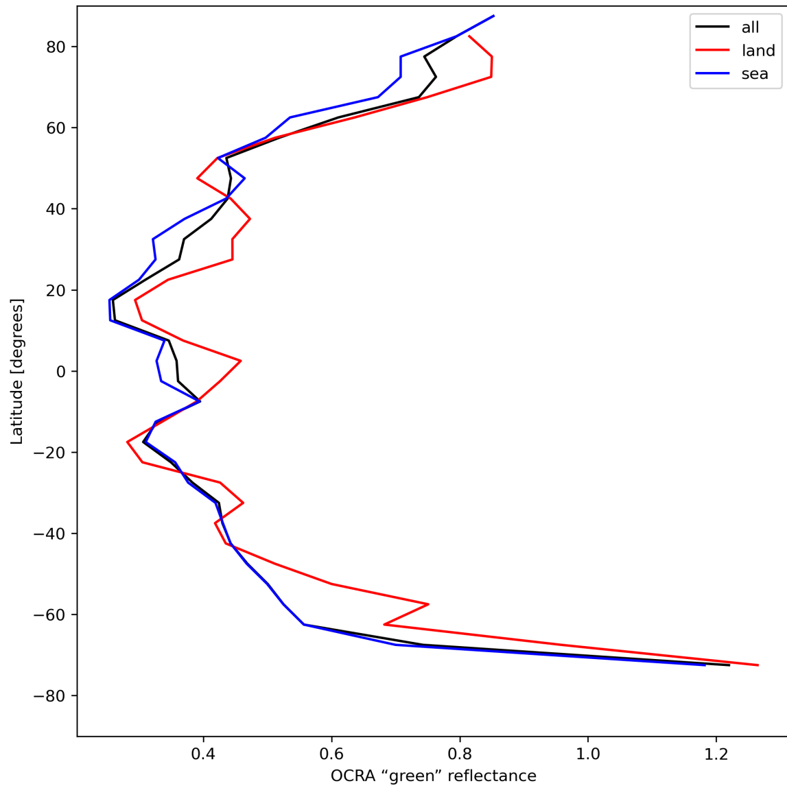
Figure 36: Zonal average of “OCRA “green” reflectance” for 2024-05-03 to 2024-05-05.
