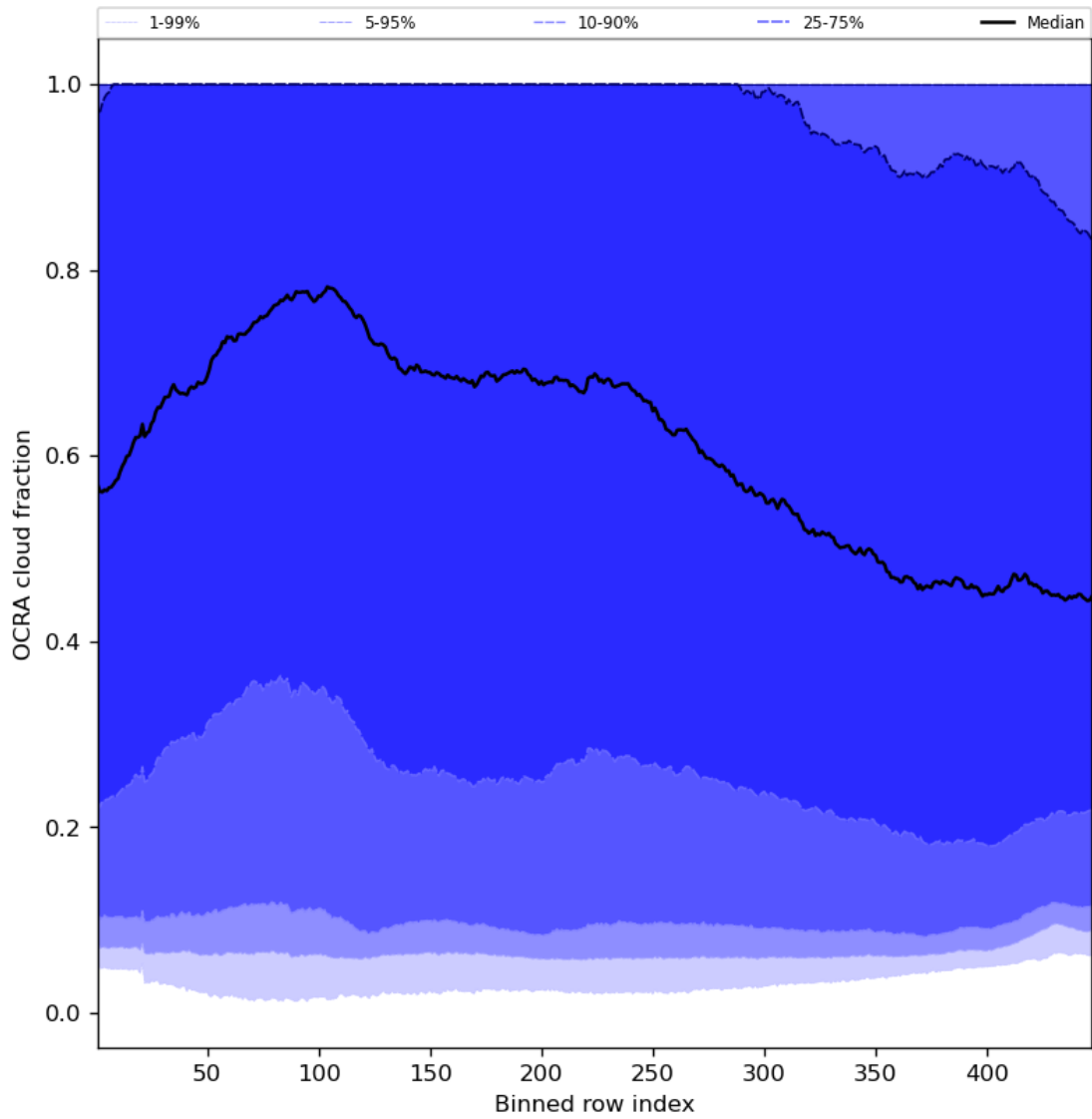
Figure 66: Along track statistics of “OCRA cloud fraction” for 2024-05-03 to 2024-05-05
