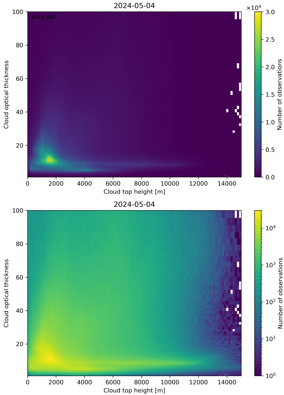
Figure 90: Scatter density plot of “Cloud top height” against “Cloud optical thickness” for 2024-05-03 to 2024-05-05.
