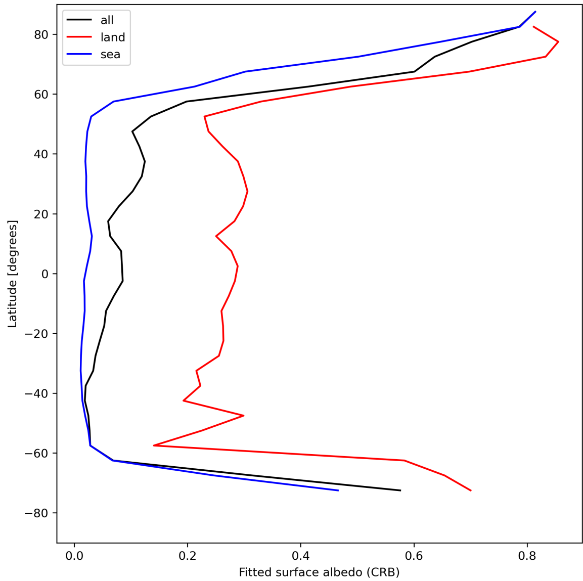
Figure 30: Zonal average of “Fitted surface albedo (CRB)” for 2024-05-03 to 2024-05-05.
