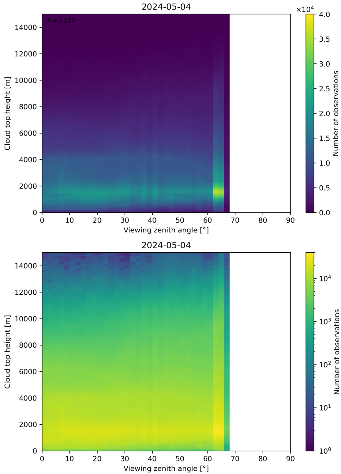
Figure 112: Scatter density plot of “Viewing zenith angle” against “Cloud top height” for 2024-05-03 to 2024-05-05.
