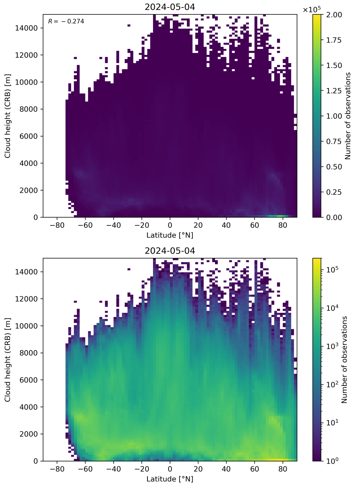
Figure 95: Scatter density plot of “Latitude” against “Cloud height (CRB)” for 2024-05-03 to 2024-05-05.
