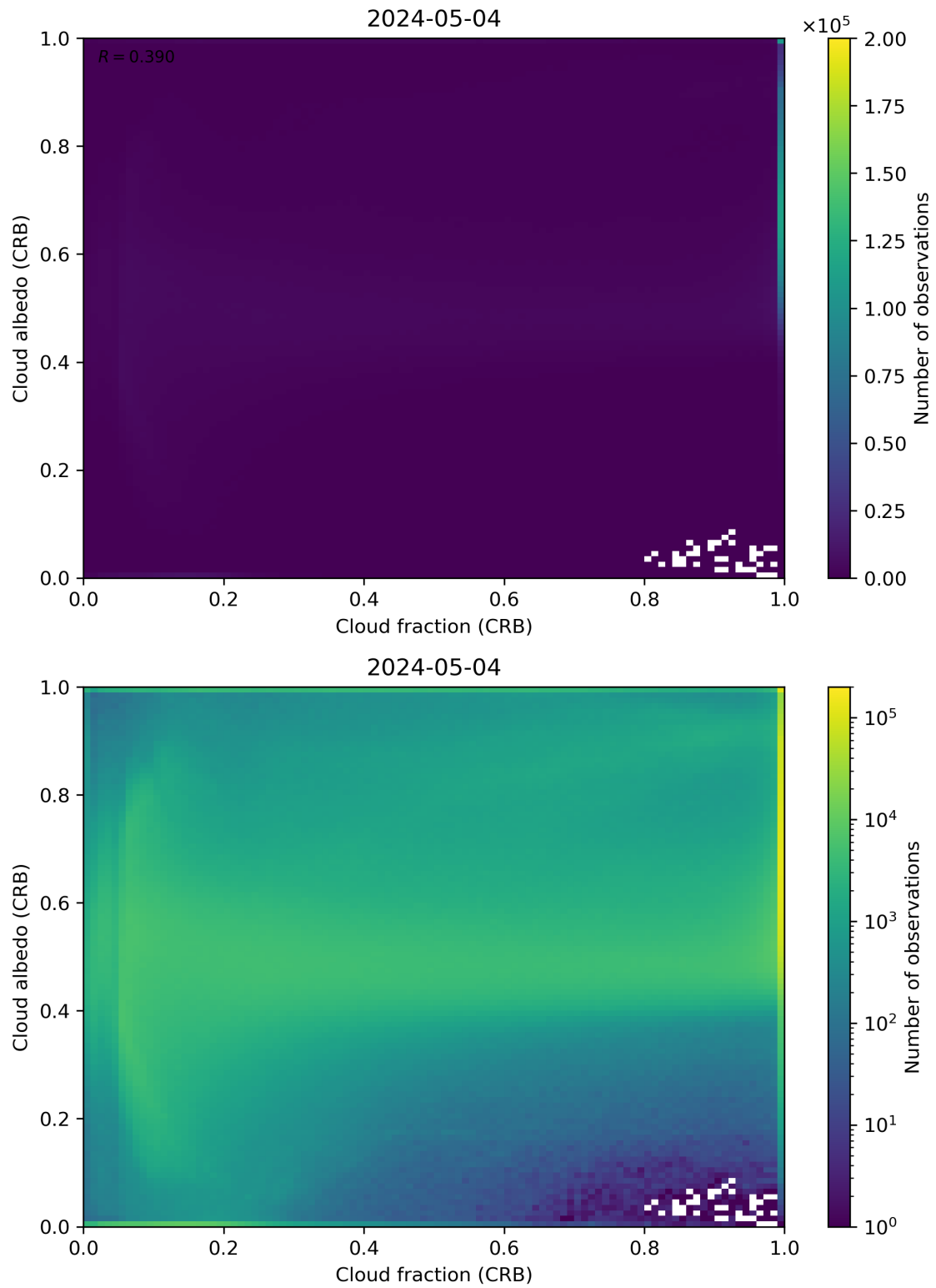
Figure 77: Scatter density plot of “Cloud fraction (CRB)” against “Cloud albedo (CRB)” for 2024-05-03 to 2024-05-05.
