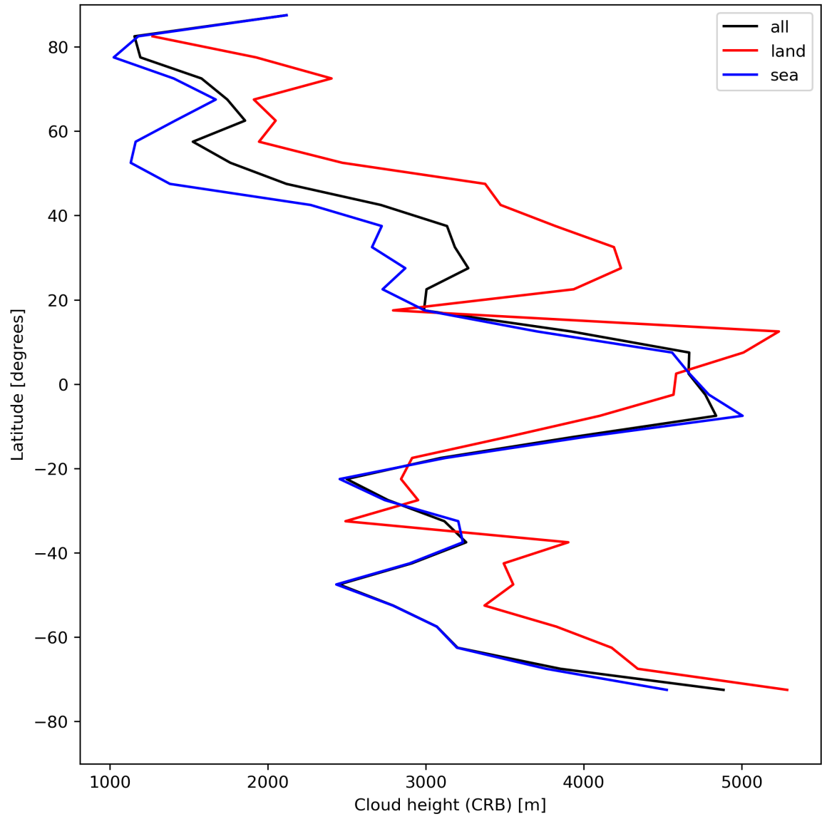
Figure 27: Zonal average of “Cloud height (CRB)” for 2024-05-03 to 2024-05-05.
