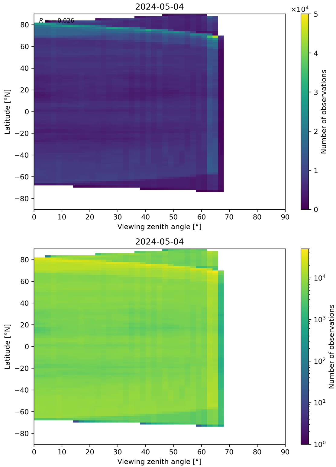
Figure 113: Scatter density plot of “Viewing zenith angle” against “Latitude” for 2024-05-03 to 2024-05-05.
