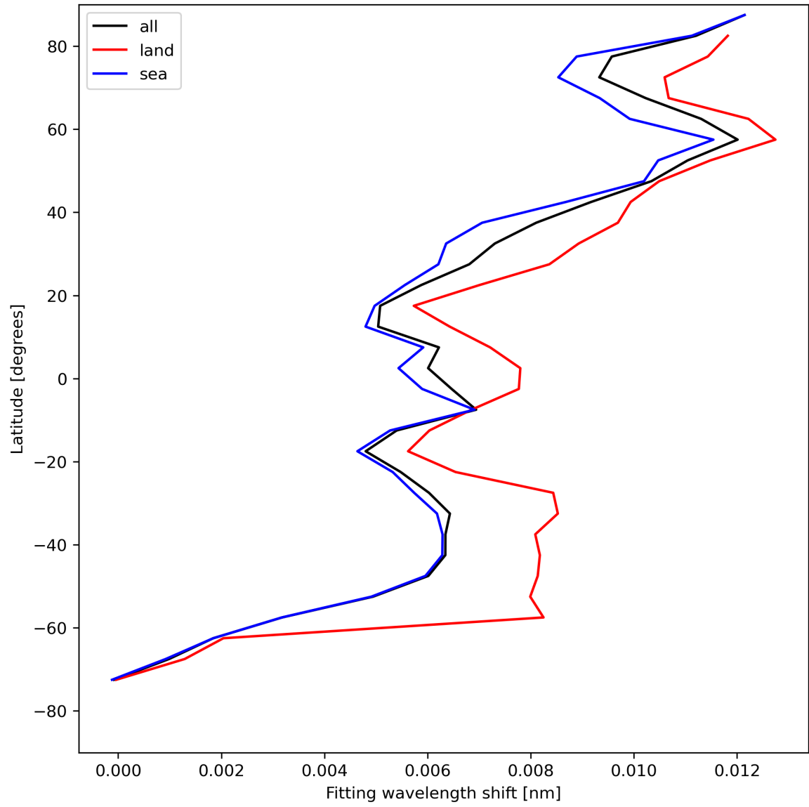
Figure 33: Zonal average of “Fitting wavelength shift” for 2024-05-03 to 2024-05-05.
