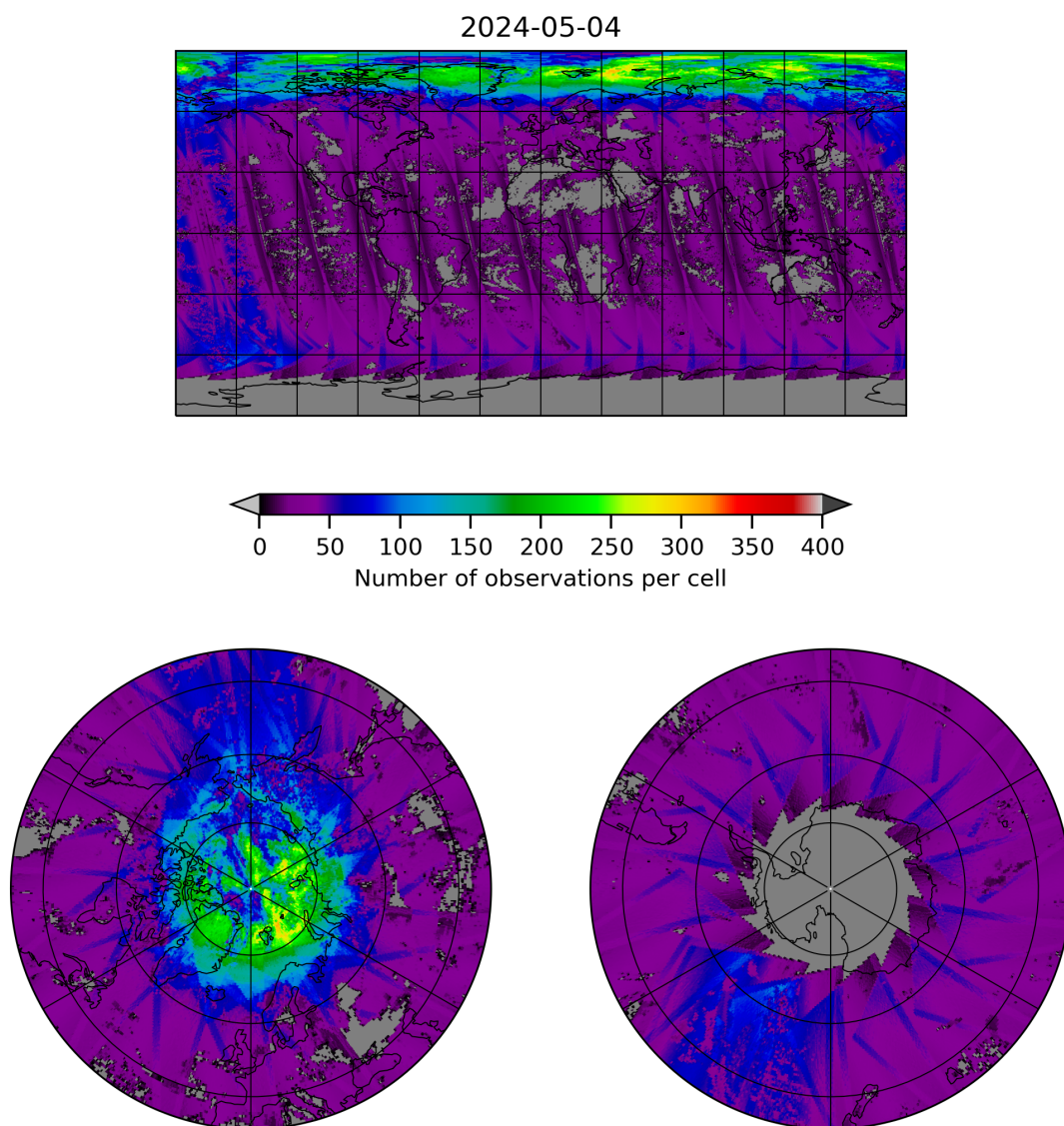
Figure 21: Map of the number of observations for 2024-05-03 to 2024-05-05
