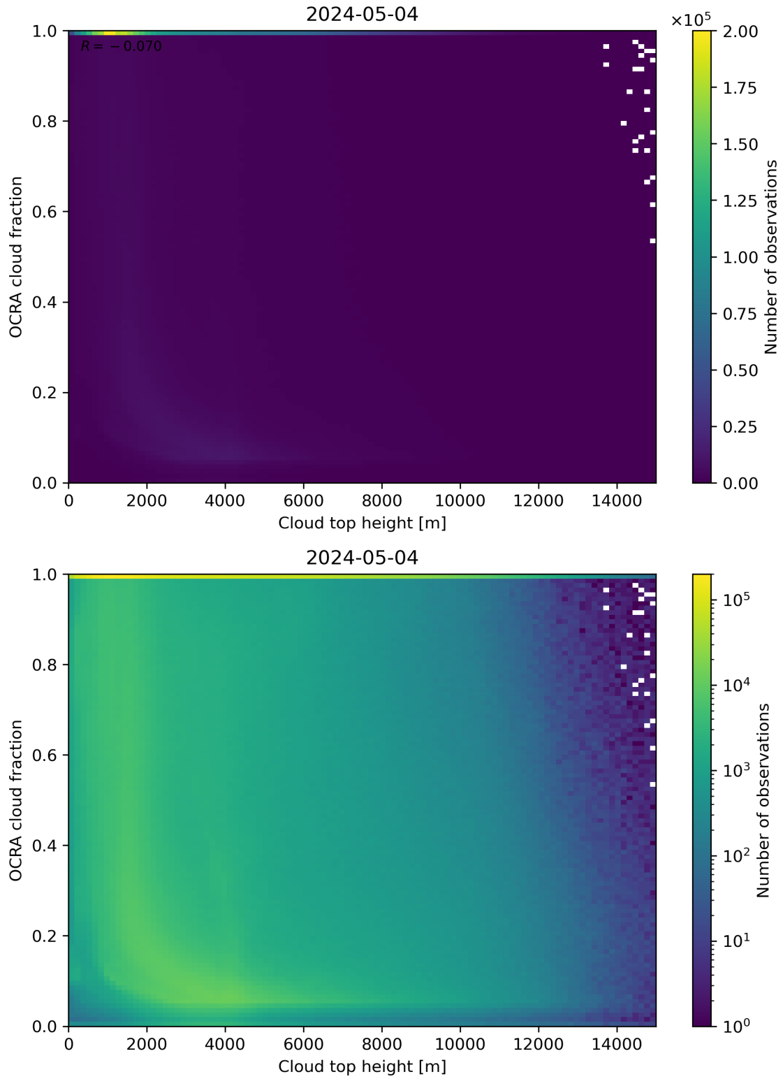
Figure 87: Scatter density plot of “Cloud top height” against “OCRA cloud fraction” for 2024-05-03 to 2024-05-05.
