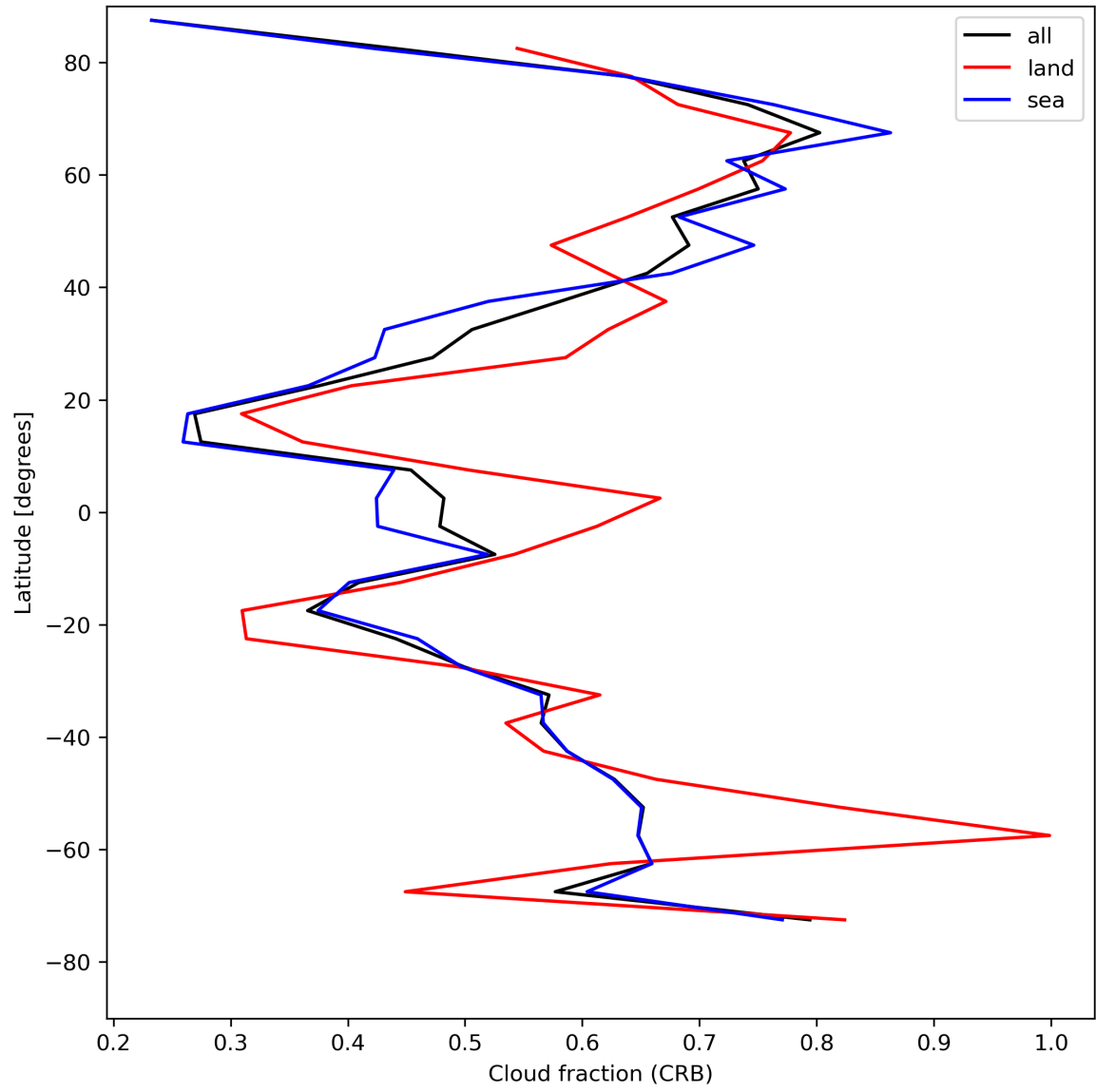
Figure 26: Zonal average of “Cloud fraction (CRB)” for 2024-05-03 to 2024-05-05.
