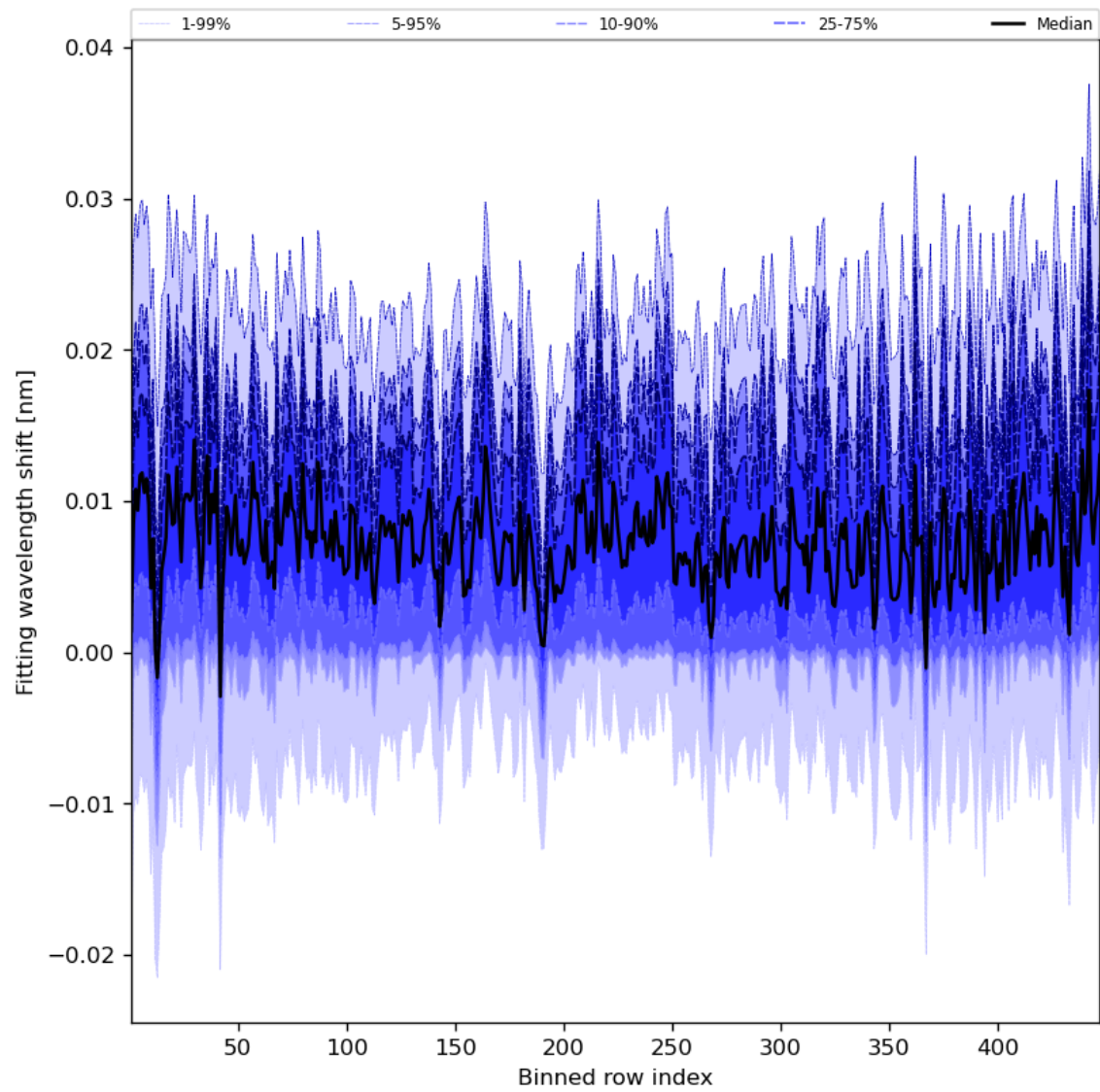
Figure 65: Along track statistics of “Fitting wavelength shift” for 2024-05-03 to 2024-05-05
