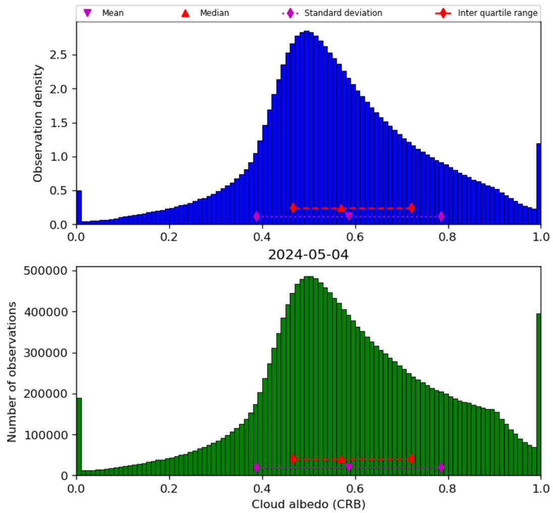
Figure 44: Histogram of “Cloud albedo (CRB)” for 2024-05-03 to 2024-05-05
