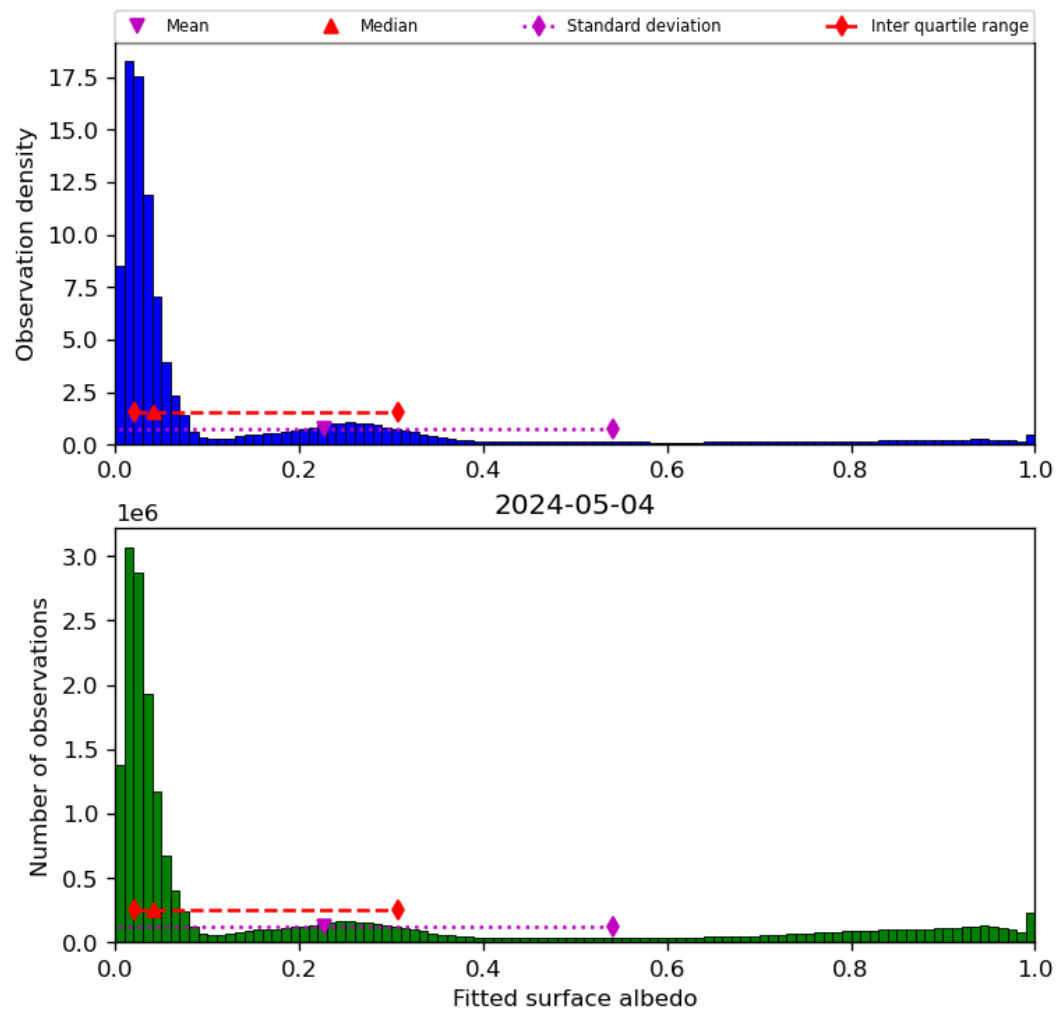
Figure 45: Histogram of “Fitted surface albedo” for 2024-05-03 to 2024-05-05
