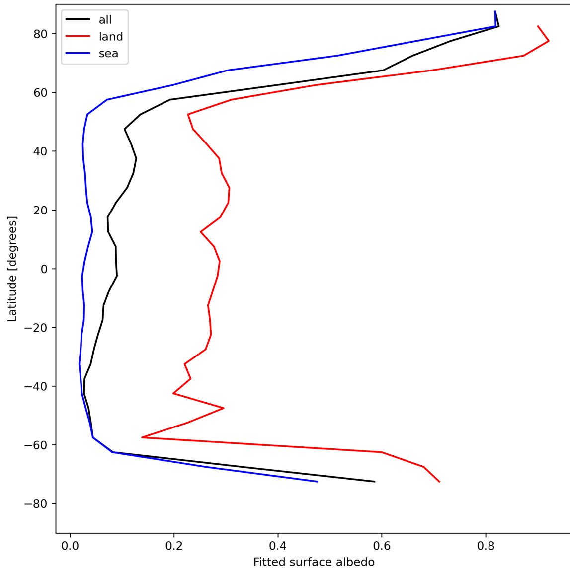
Figure 29: Zonal average of “Fitted surface albedo” for 2024-05-03 to 2024-05-05.
