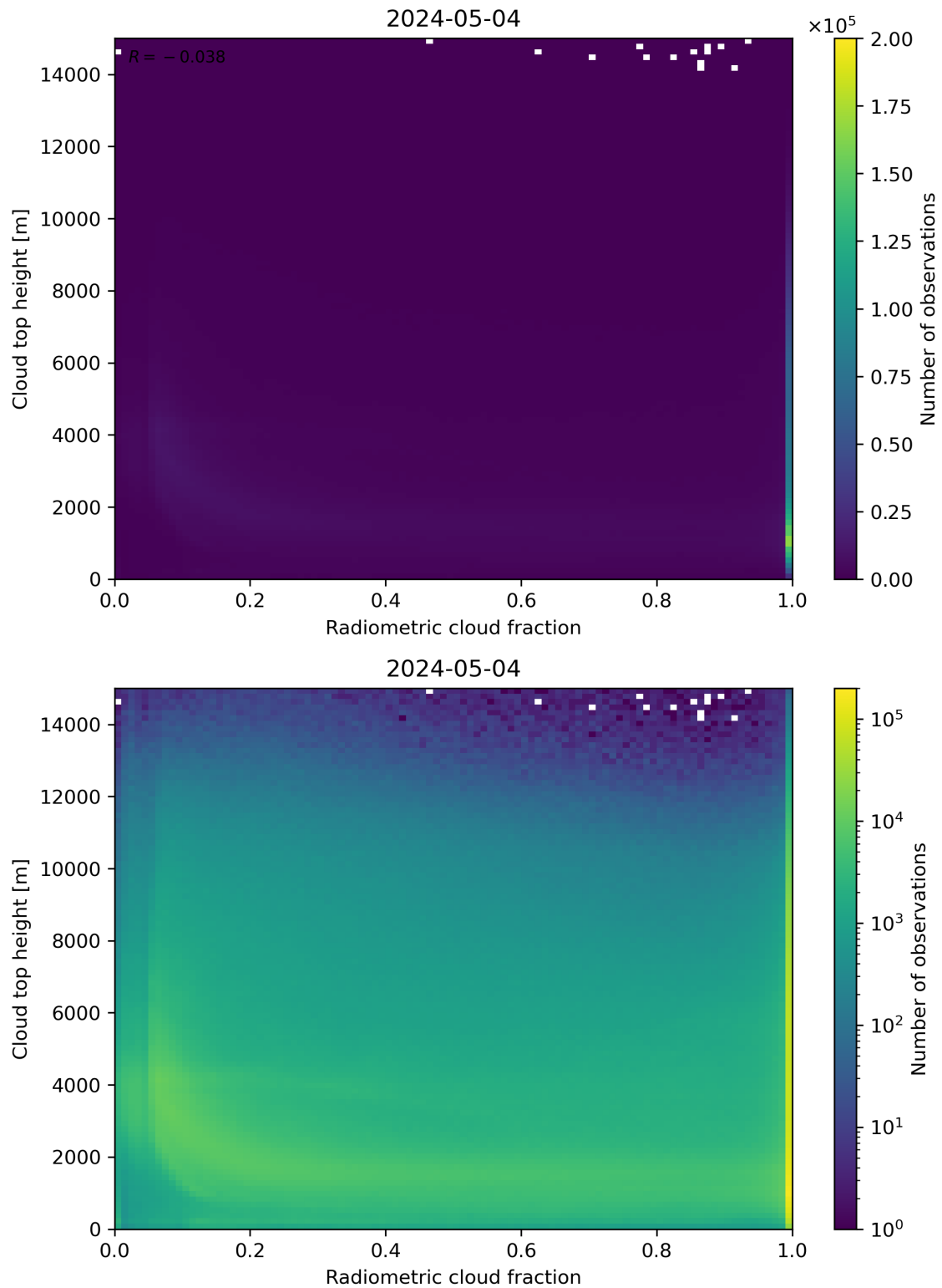
Figure 76: Scatter density plot of “Radiometric cloud fraction” against “Cloud top height” for 2024-05-03 to 2024-05-05.
