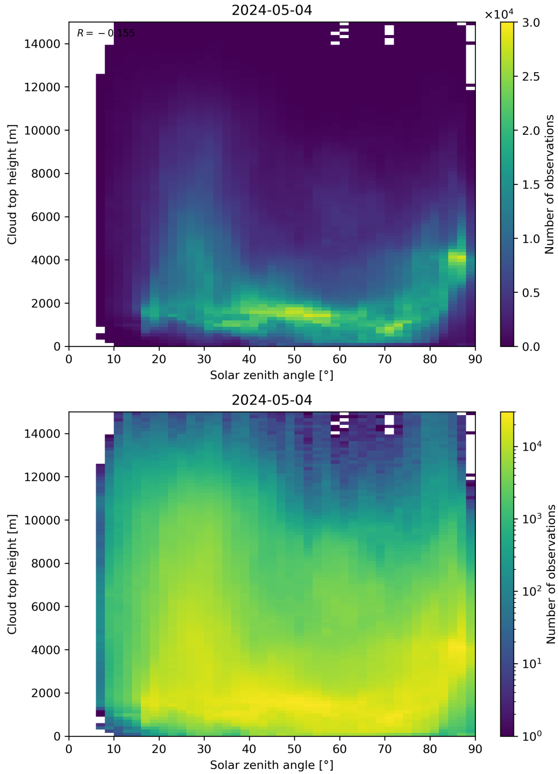
Figure 104: Scatter density plot of “Solar zenith angle” against “Cloud top height” for 2024-05-03 to 2024-05-05.
