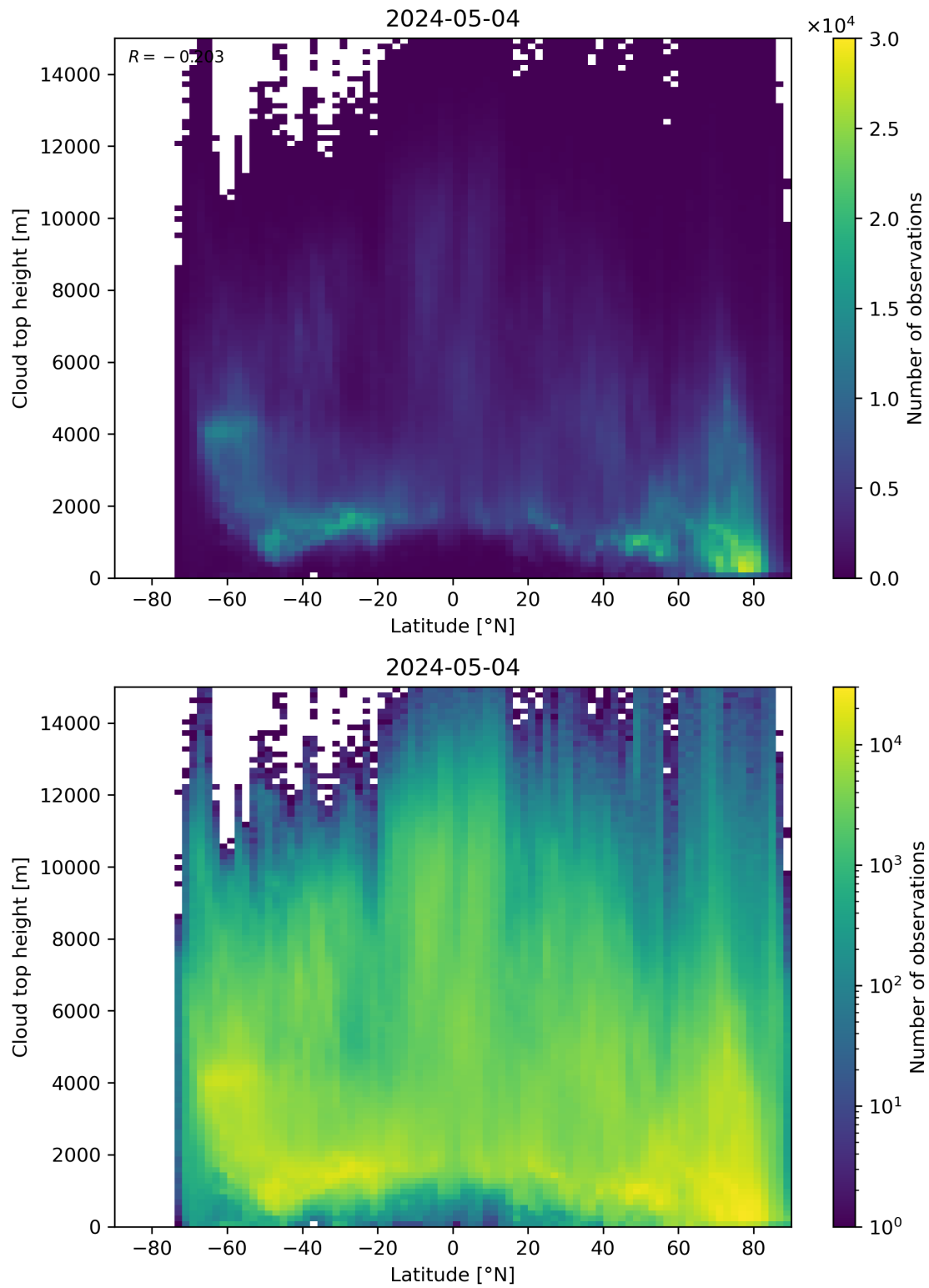
Figure 97: Scatter density plot of “Latitude” against “Cloud top height” for 2024-05-03 to 2024-05-05.
