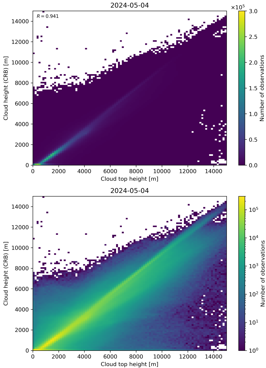
Figure 89: Scatter density plot of “Cloud top height” against “Cloud height (CRB)” for 2024-05-03 to 2024-05-05.
