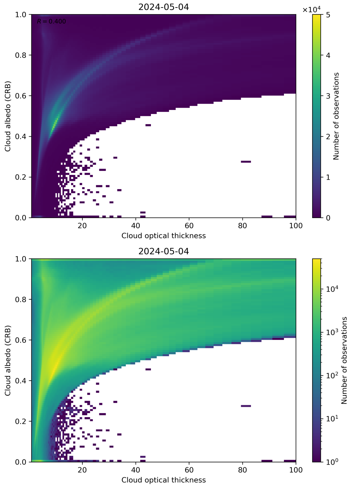
Figure 82: Scatter density plot of “Cloud optical thickness” against “Cloud albedo (CRB)” for 2024-05-03 to 2024-05-05.
