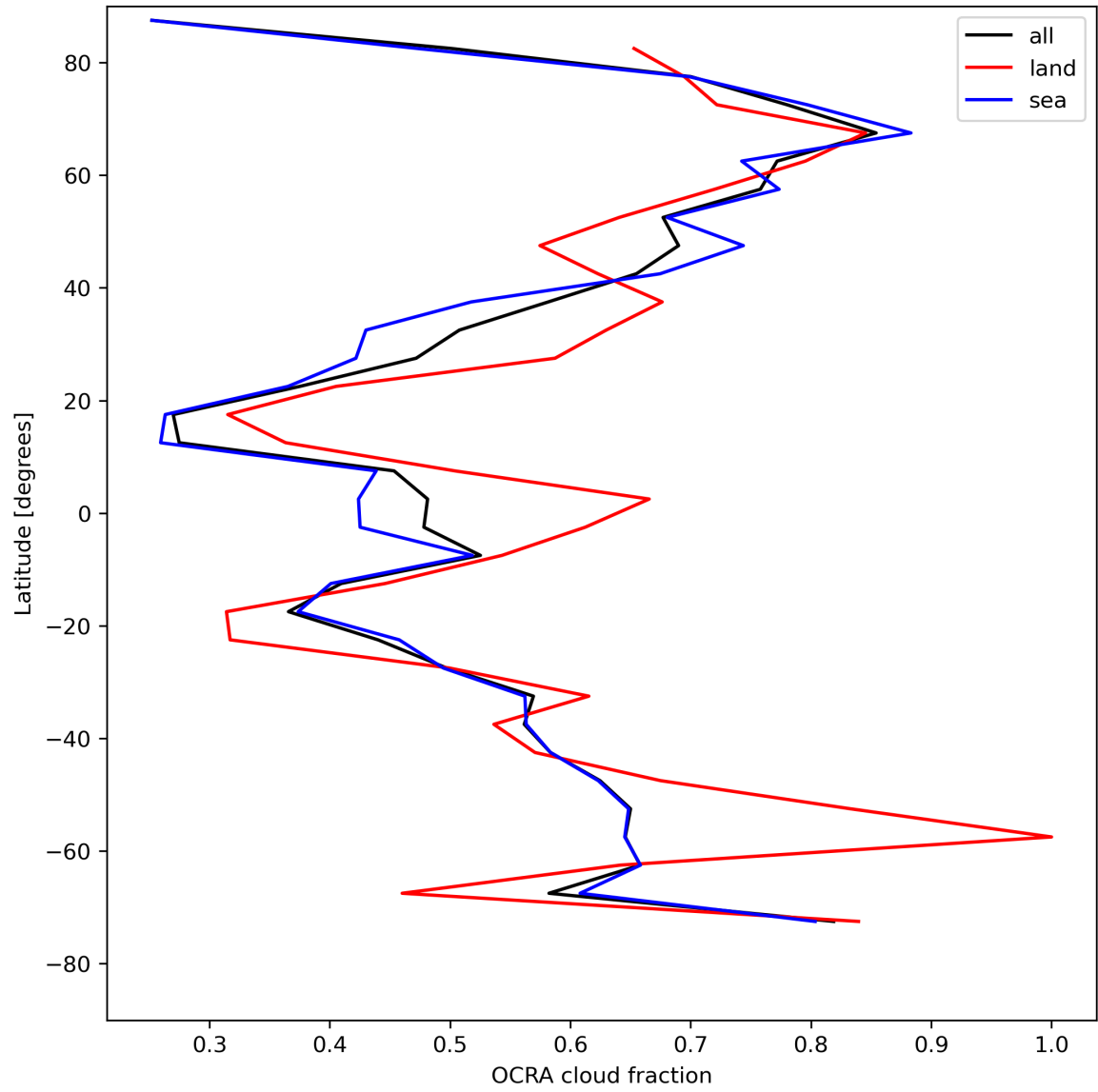
Figure 34: Zonal average of “OCRA cloud fraction” for 2024-05-03 to 2024-05-05.
