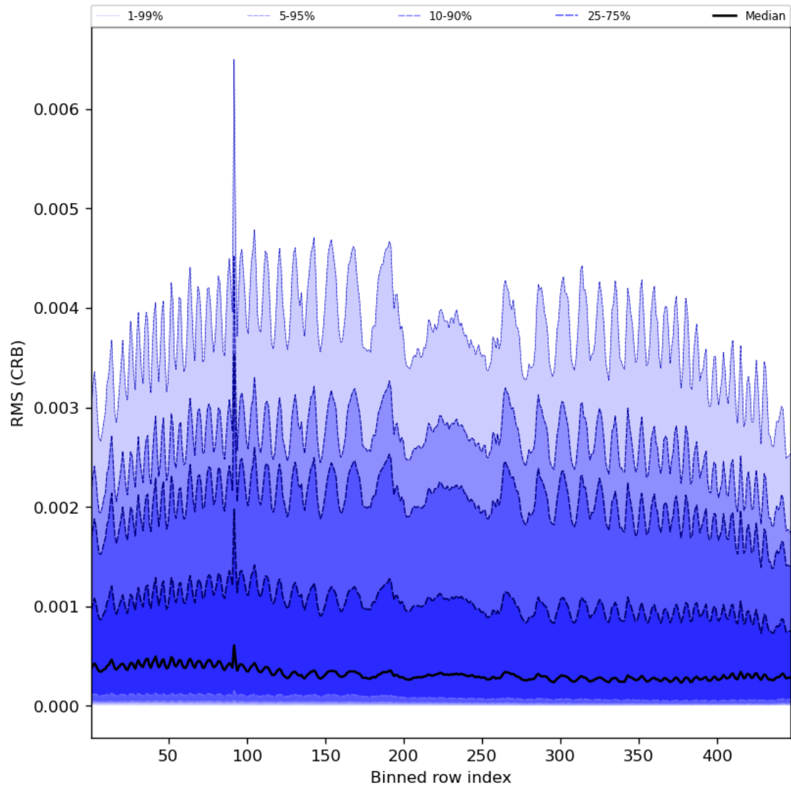
Figure 64: Along track statistics of “RMS (CRB)” for 2024-05-03 to 2024-05-05
