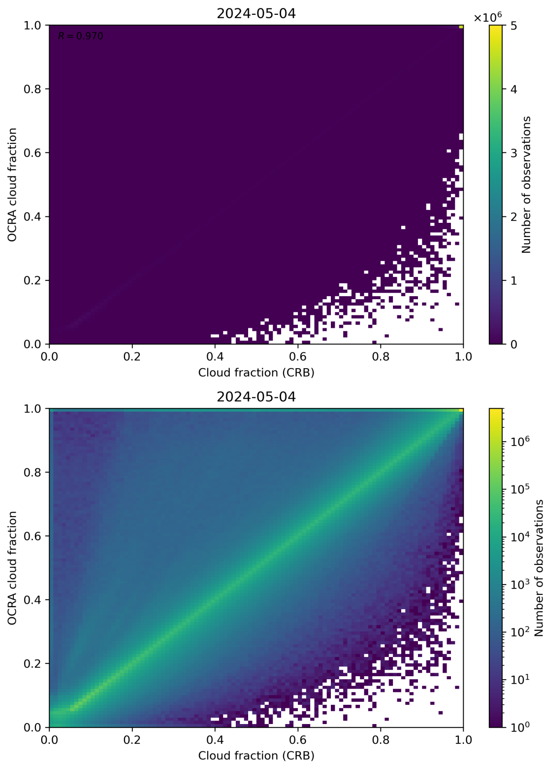
Figure 78: Scatter density plot of “Cloud fraction (CRB)” against “OCRA cloud fraction” for 2024-05-03 to 2024-05-05.
