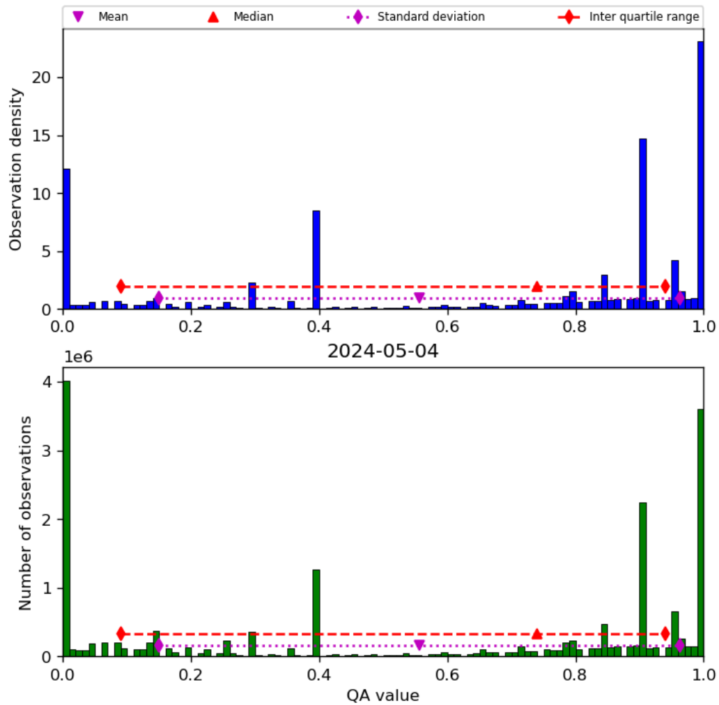
Figure 38: Histogram of “QA value” for 2024-05-03 to 2024-05-05
