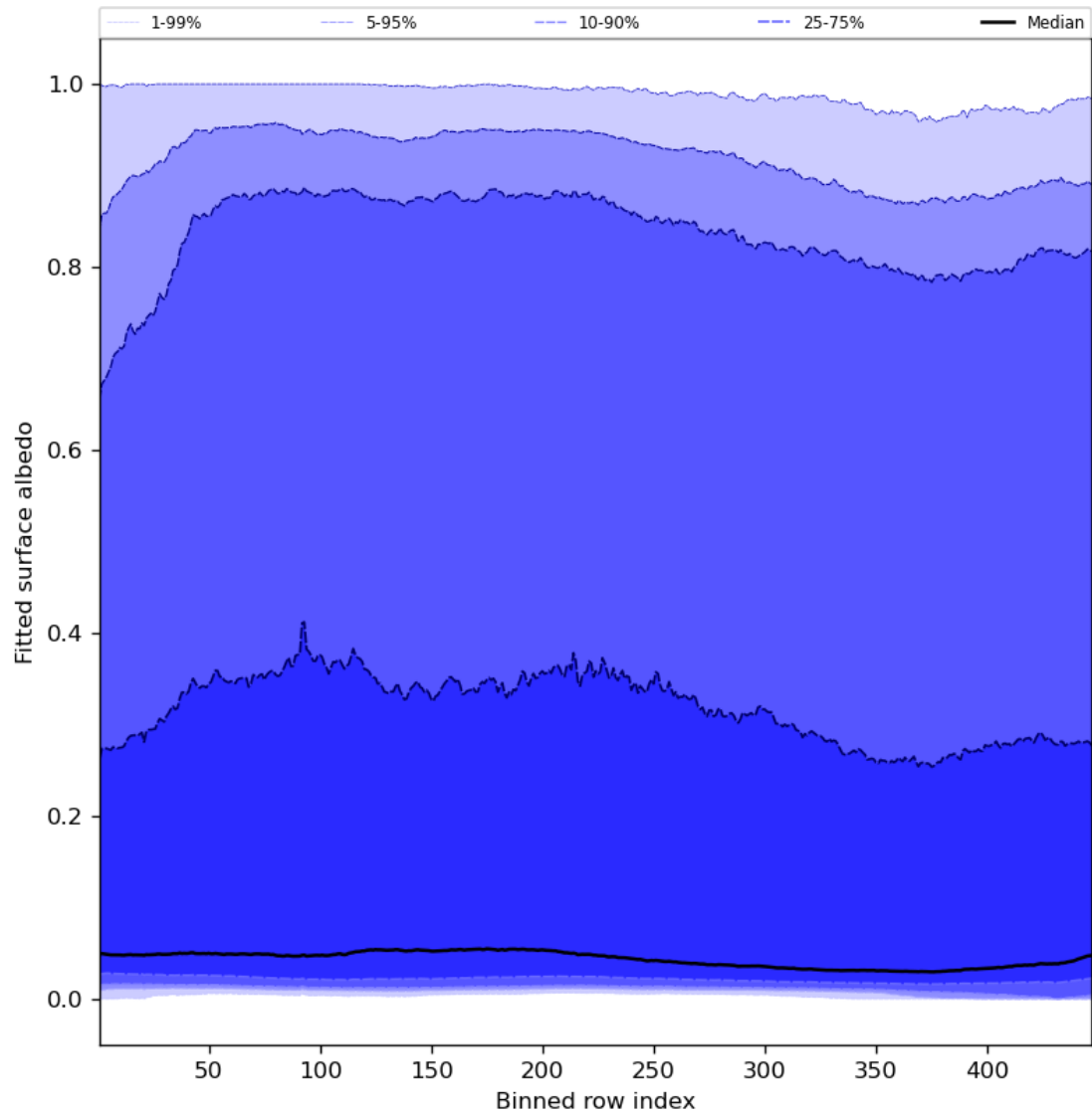
Figure 61: Along track statistics of “Fitted surface albedo” for 2024-05-03 to 2024-05-05
