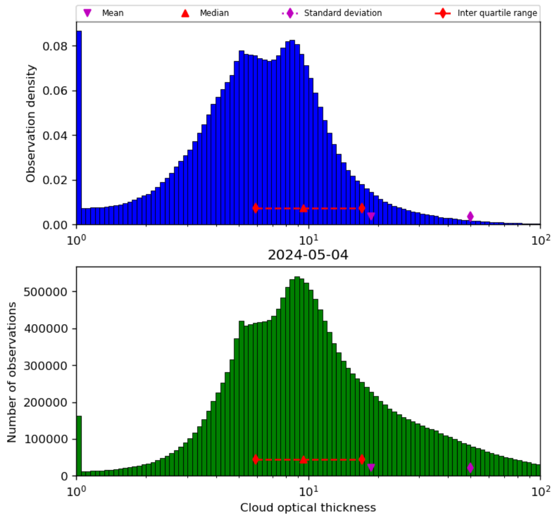
Figure 41: Histogram of “Cloud optical thickness” for 2024-05-03 to 2024-05-05
