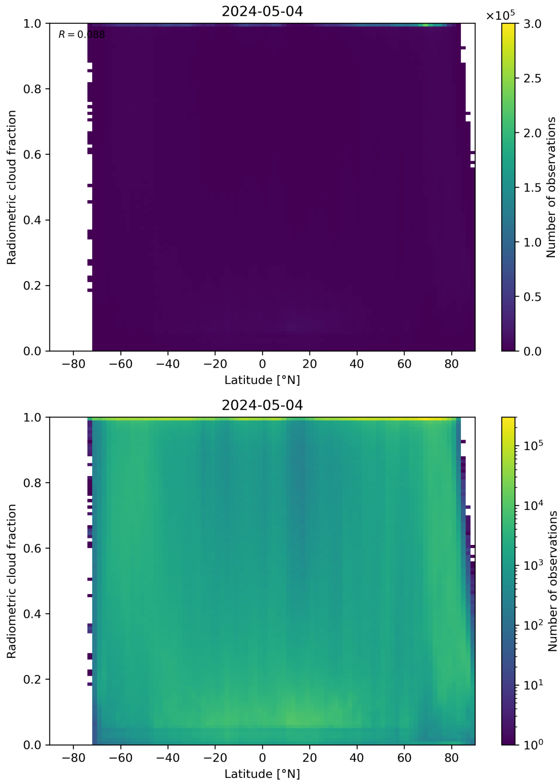
Figure 92: Scatter density plot of “Latitude” against “Radiometric cloud fraction” for 2024-05-03 to 2024-05-05.
