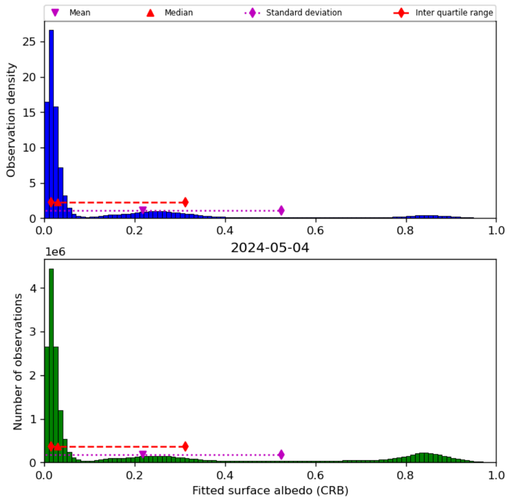
Figure 46: Histogram of “Fitted surface albedo (CRB)” for 2024-05-03 to 2024-05-05
