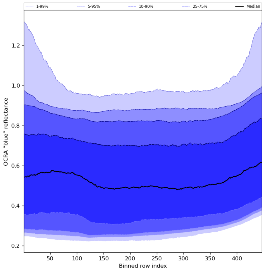
Figure 67: Along track statistics of “OCRA “blue” reflectance” for 2024-05-03 to 2024-05-05
