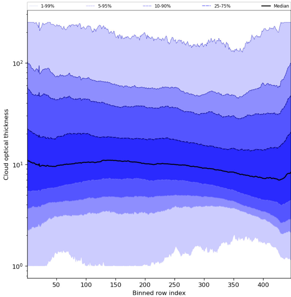
Figure 57: Along track statistics of “Cloud optical thickness” for 2024-05-03 to 2024-05-05
