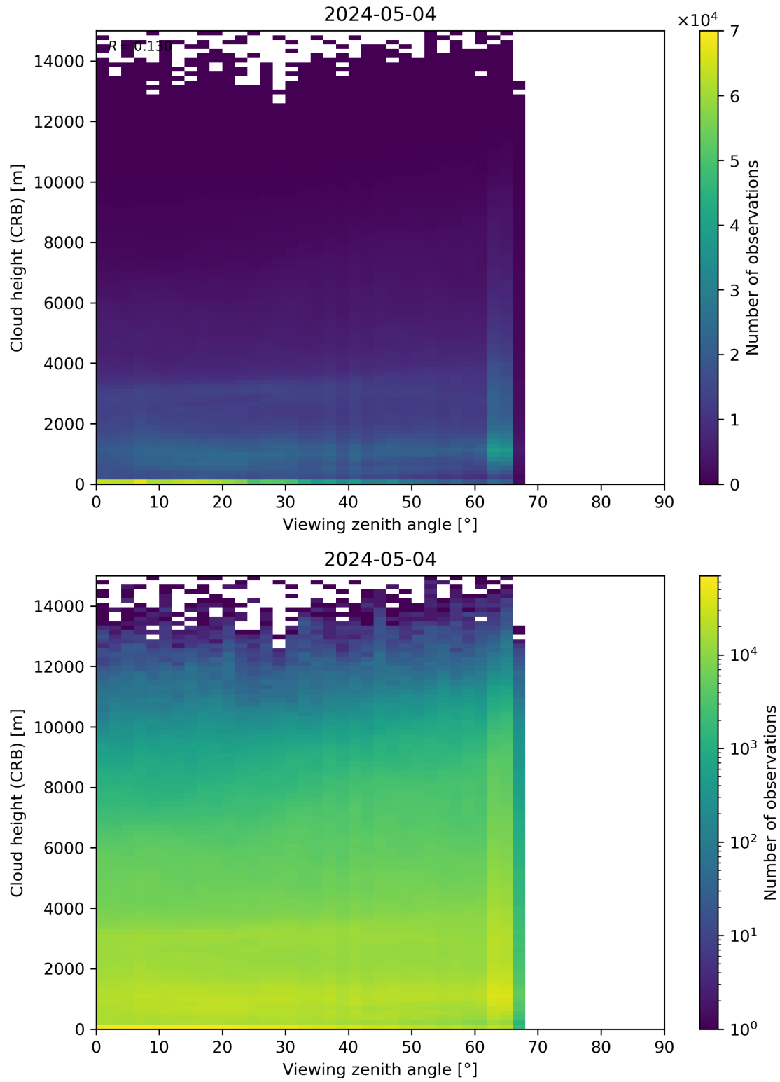
Figure 110: Scatter density plot of “Viewing zenith angle” against “Cloud height (CRB)” for 2024-05-03 to 2024-05-05.
