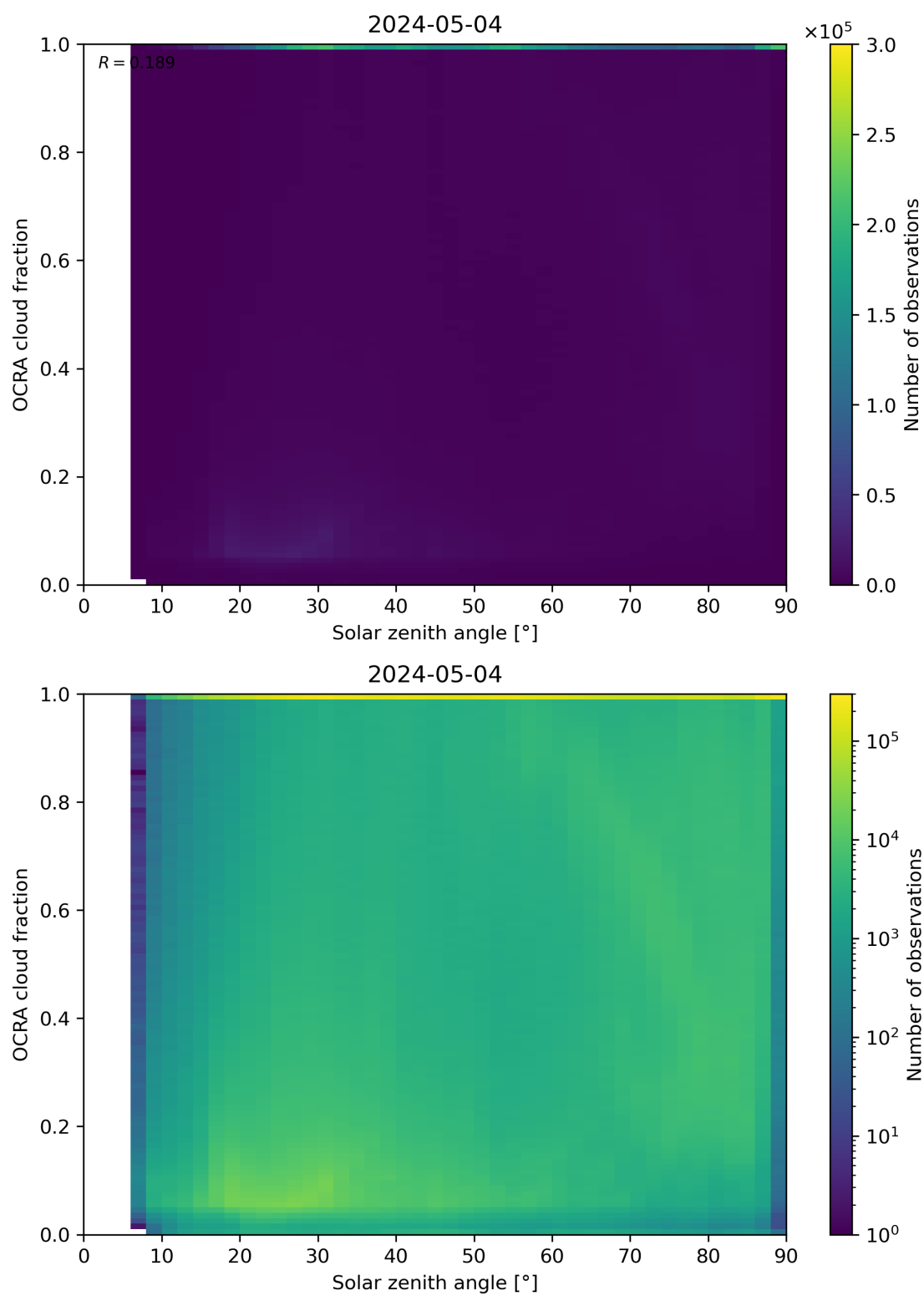
Figure 100: Scatter density plot of “Solar zenith angle” against “OCRA cloud fraction” for 2024-05-03 to 2024-05-05.
