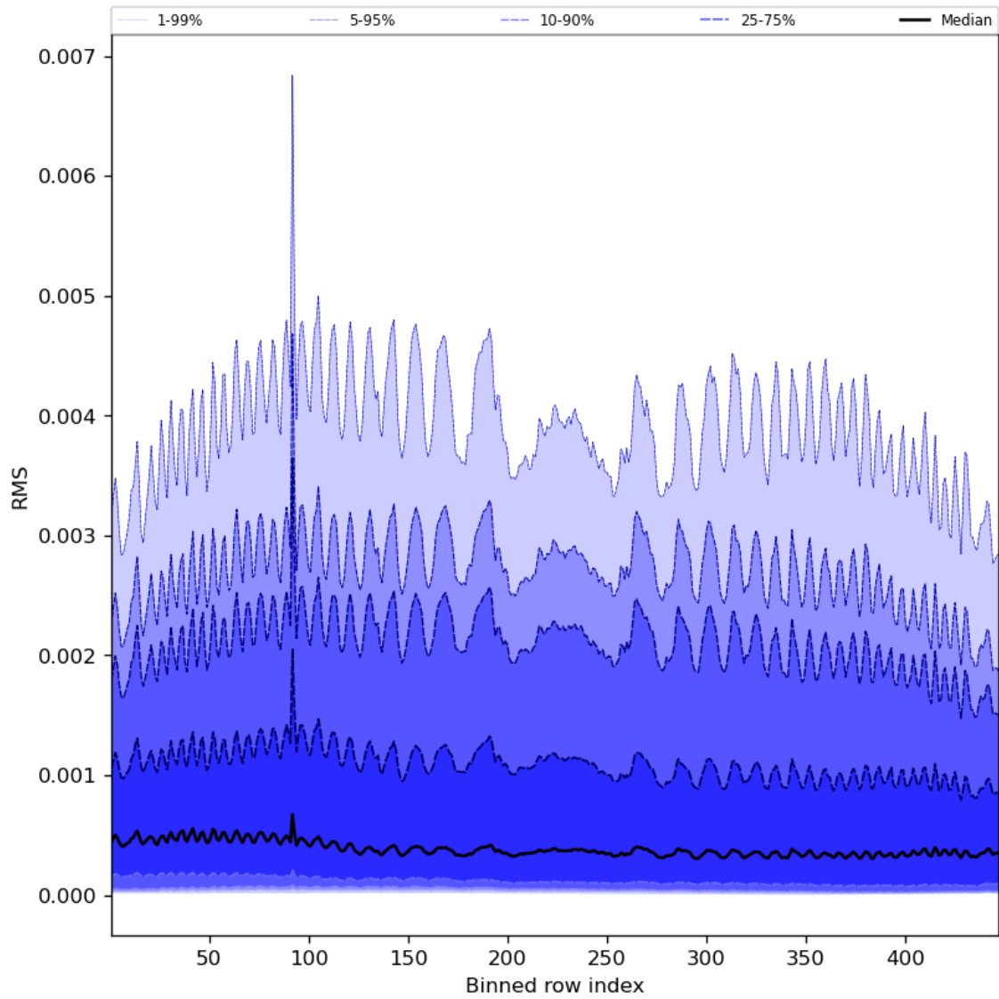
Figure 63: Along track statistics of “RMS” for 2024-05-03 to 2024-05-05
