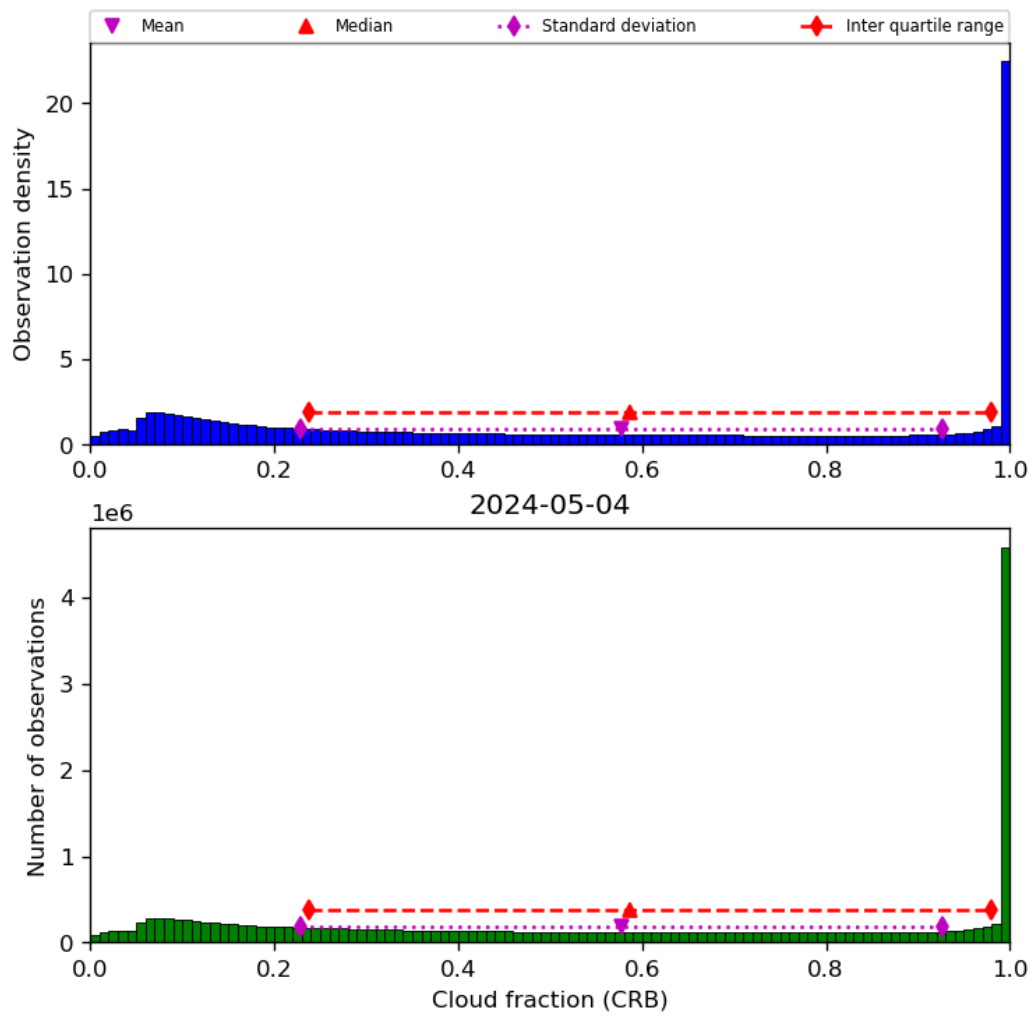
Figure 42: Histogram of “Cloud fraction (CRB)” for 2024-05-03 to 2024-05-05
