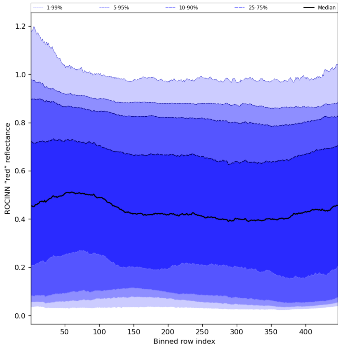
Figure 69: Along track statistics of “ROCINN “red” reflectance” for 2024-05-03 to 2024-05-05
