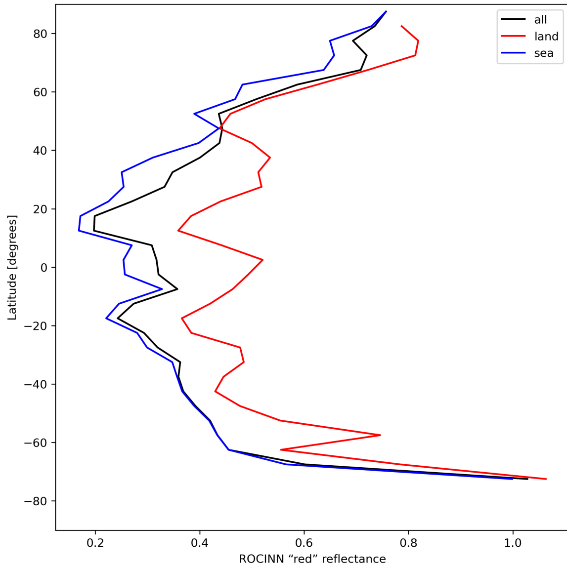
Figure 37: Zonal average of “ROCINN “red” reflectance” for 2024-05-03 to 2024-05-05.
