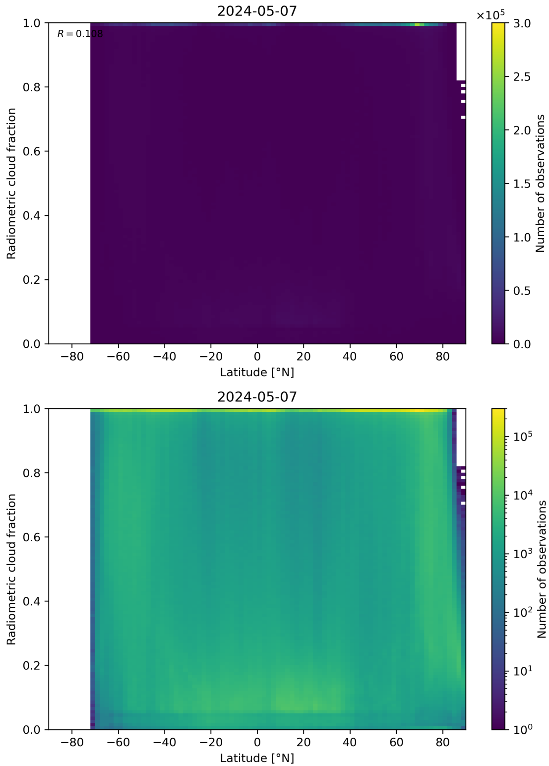
Figure 92: Scatter density plot of “Latitude” against “Radiometric cloud fraction” for 2024-05-07 to 2024-05-08.
