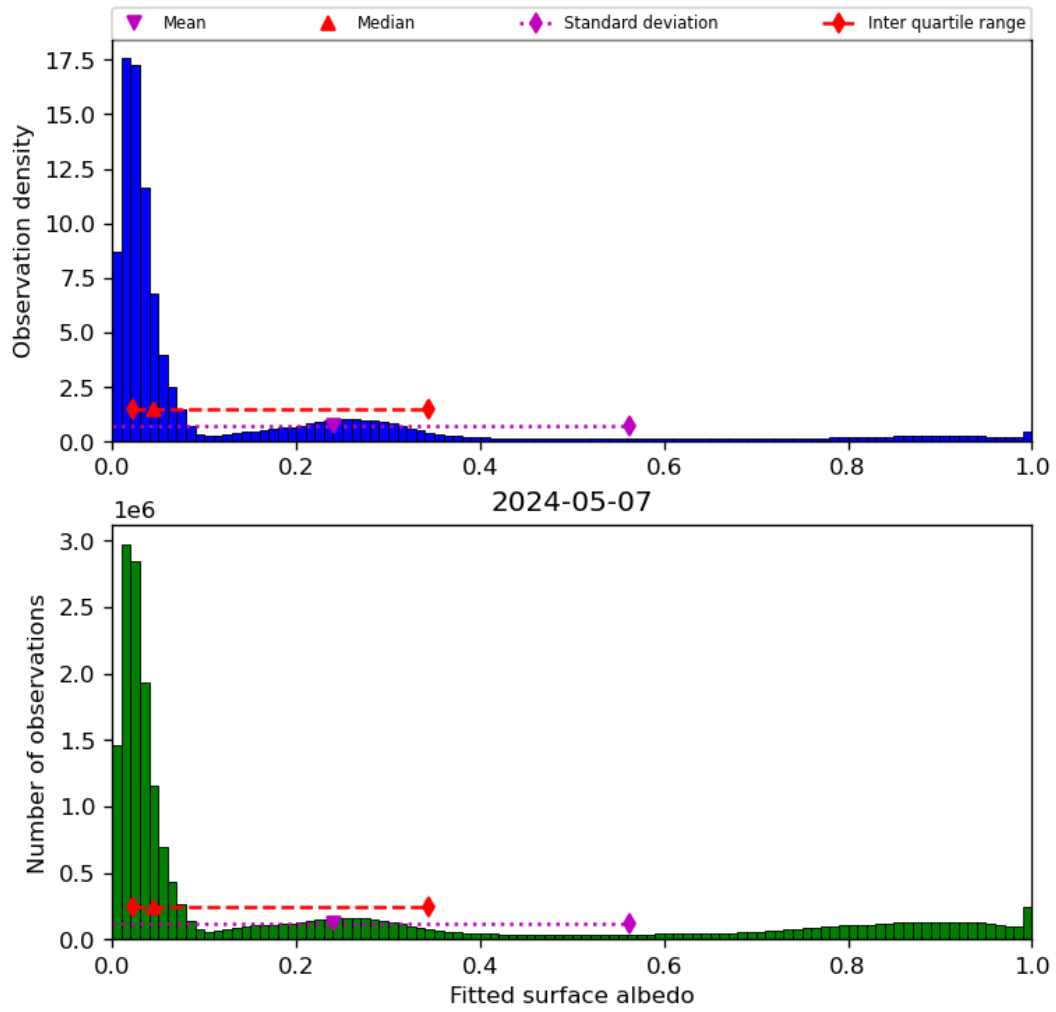
Figure 45: Histogram of “Fitted surface albedo” for 2024-05-07 to 2024-05-08
