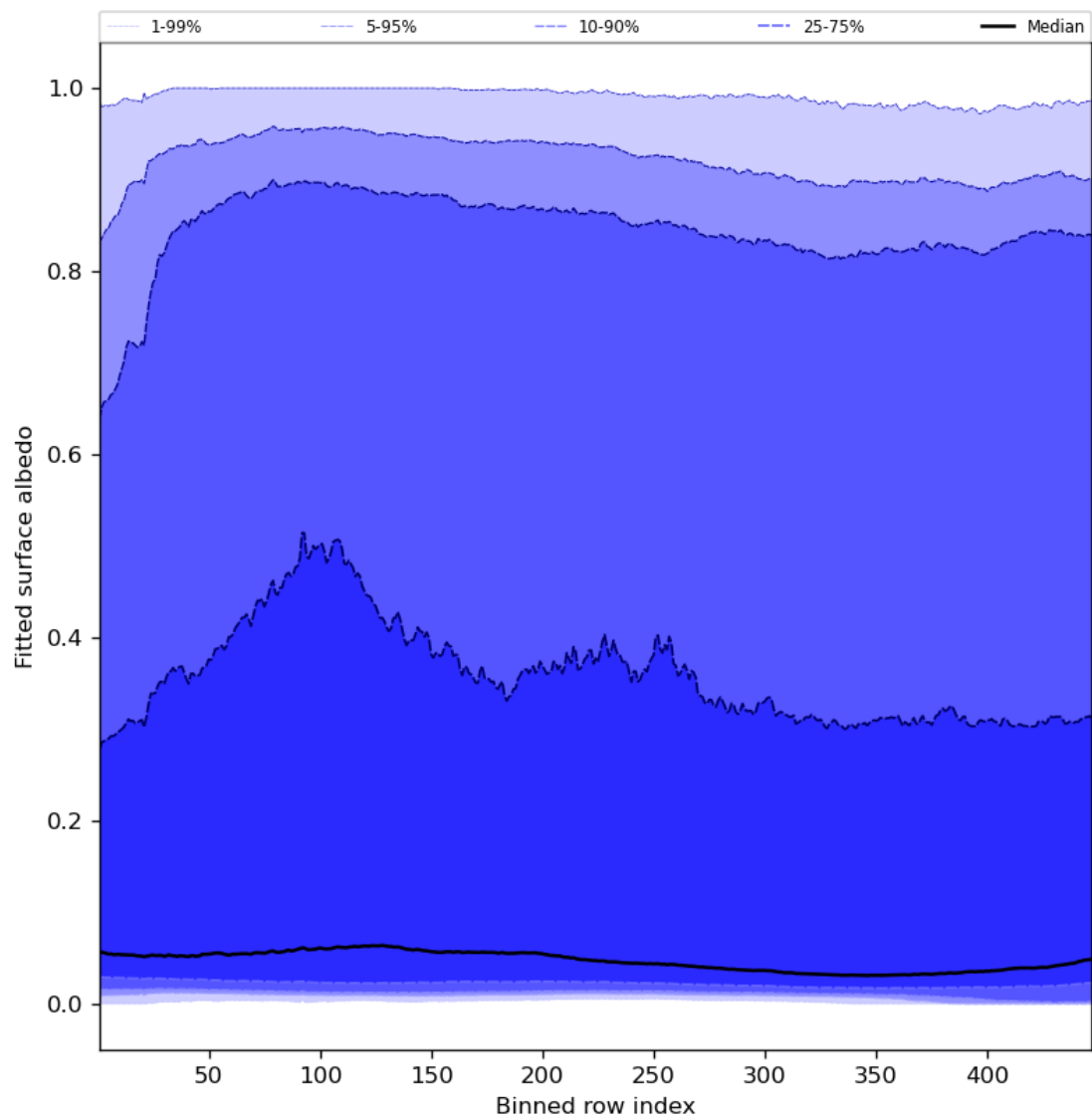
Figure 61: Along track statistics of “Fitted surface albedo” for 2024-05-07 to 2024-05-08
