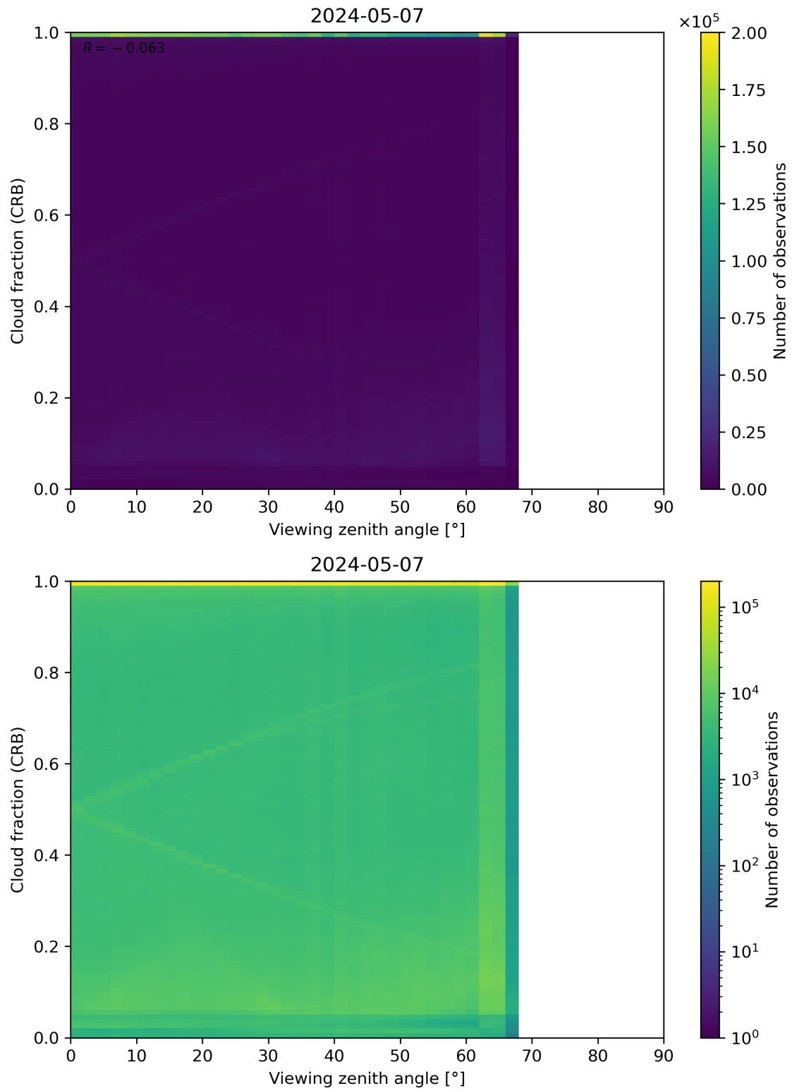
Figure 109: Scatter density plot of “Viewing zenith angle” against “Cloud fraction (CRB)” for 2024-05-07 to 2024-05-08.
