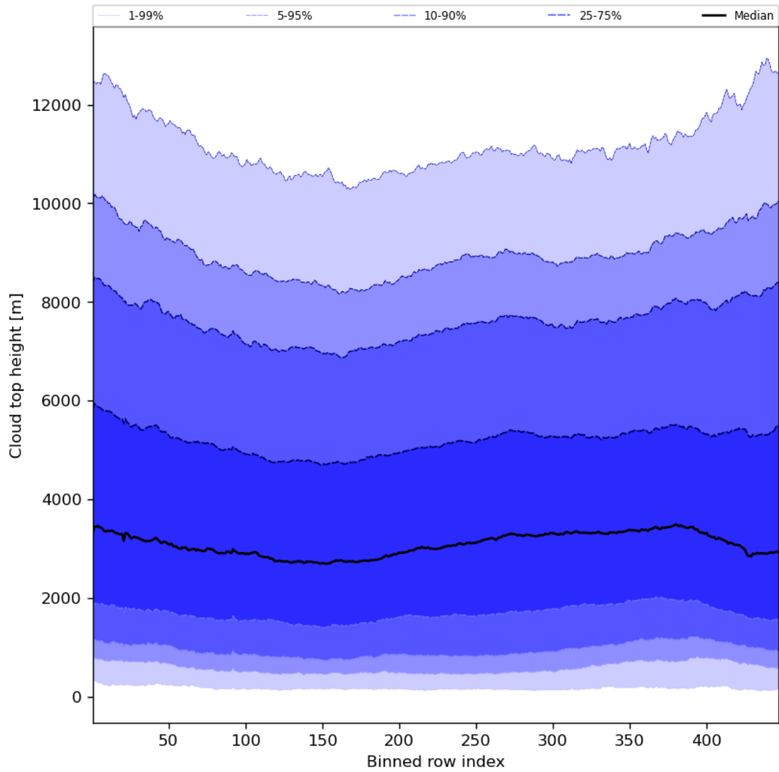
Figure 56: Along track statistics of “Cloud top height” for 2024-05-07 to 2024-05-08
