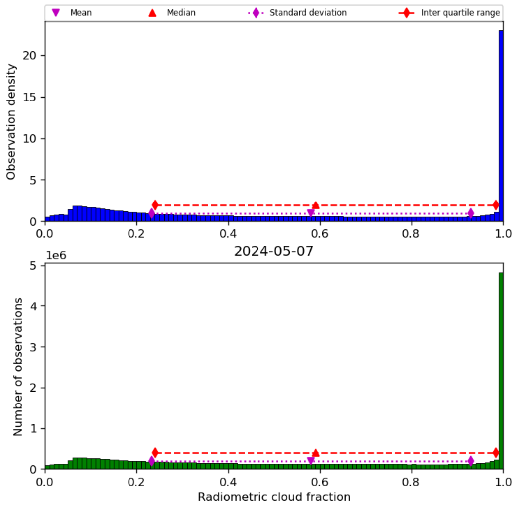
Figure 39: Histogram of “Radiometric cloud fraction” for 2024-05-07 to 2024-05-08
