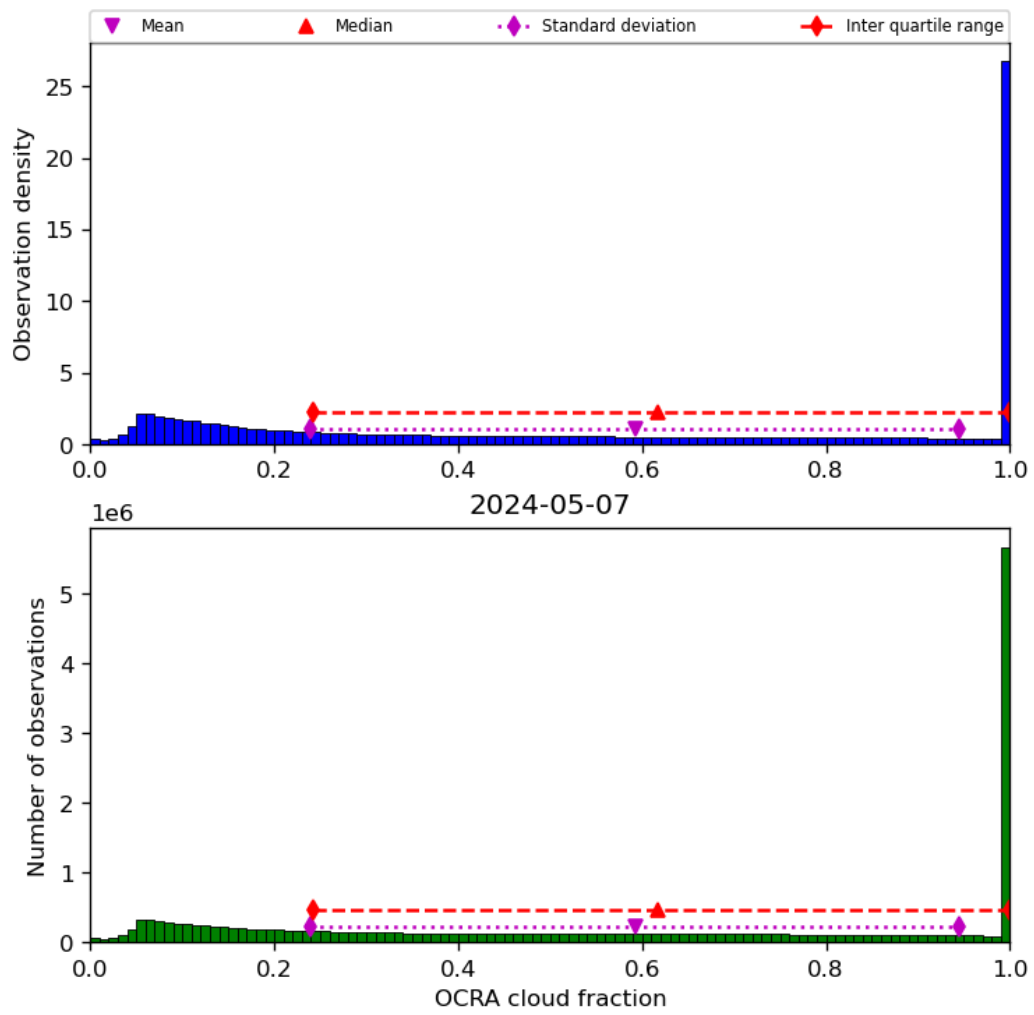
Figure 50: Histogram of “OCRA cloud fraction” for 2024-05-07 to 2024-05-08
