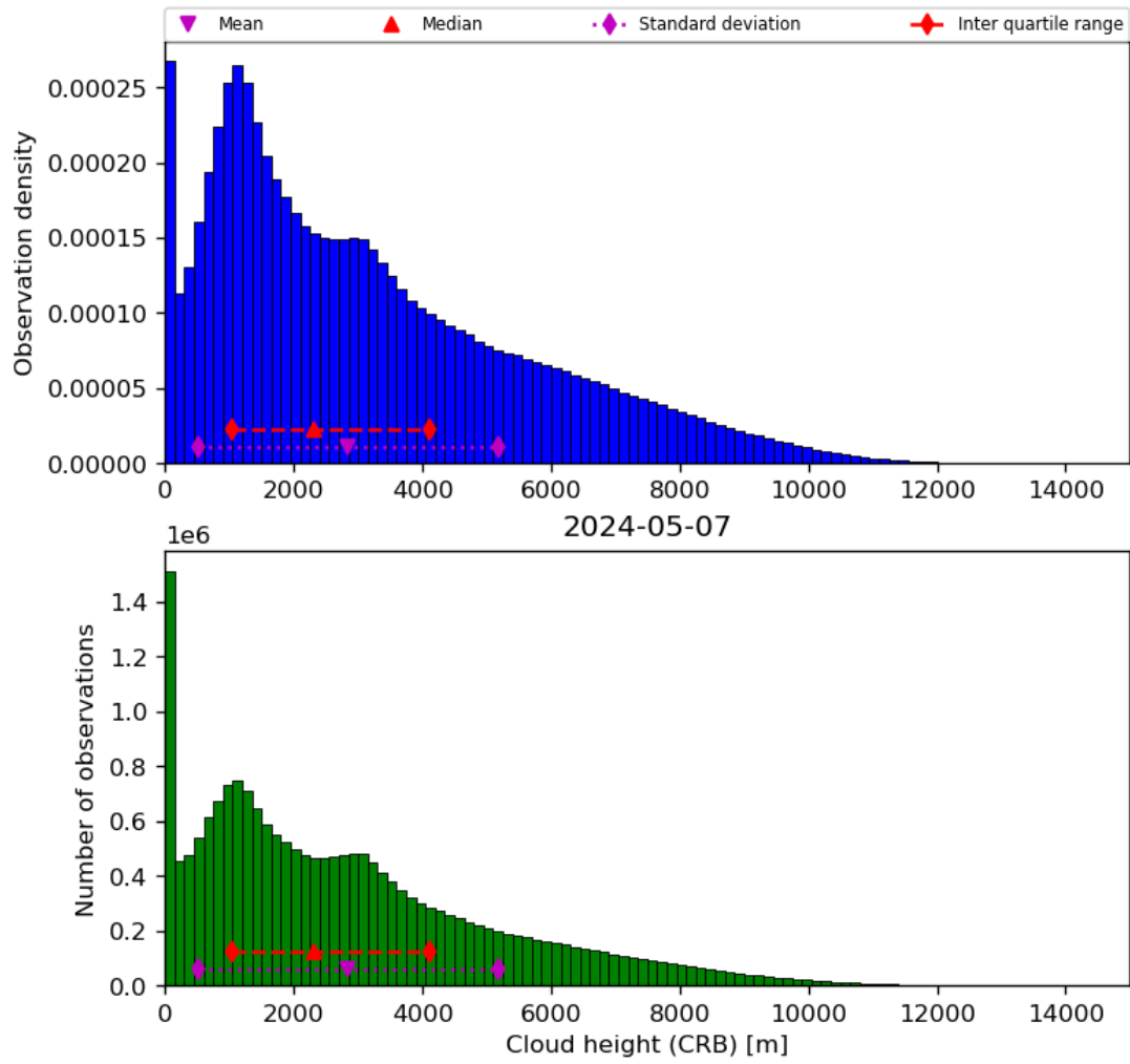
Figure 43: Histogram of “Cloud height (CRB)” for 2024-05-07 to 2024-05-08
