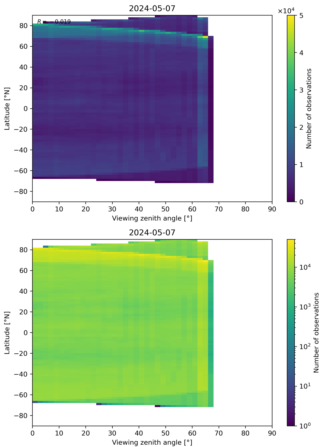
Figure 113: Scatter density plot of “Viewing zenith angle” against “Latitude” for 2024-05-07 to 2024-05-08.
