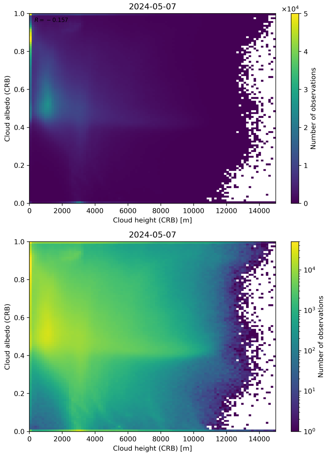
Figure 80: Scatter density plot of “Cloud height (CRB)” against “Cloud albedo (CRB)” for 2024-05-07 to 2024-05-08.
