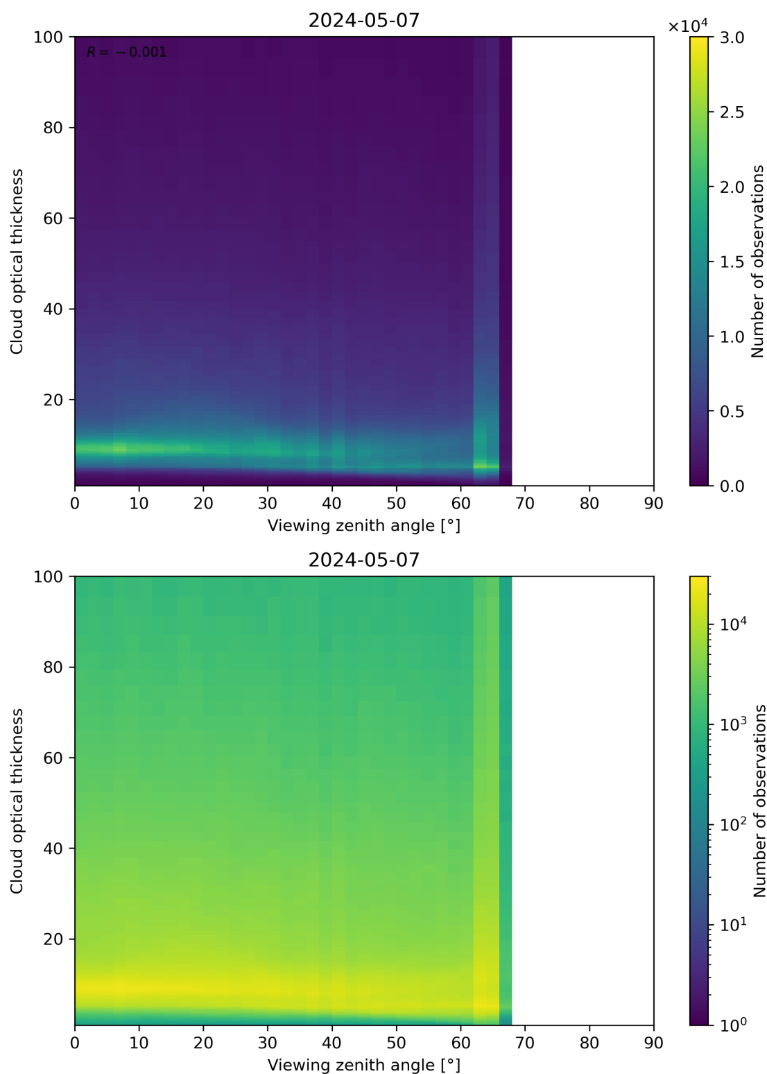
Figure 111: Scatter density plot of “Viewing zenith angle” against “Cloud optical thickness” for 2024-05-07 to 2024-05-08.
