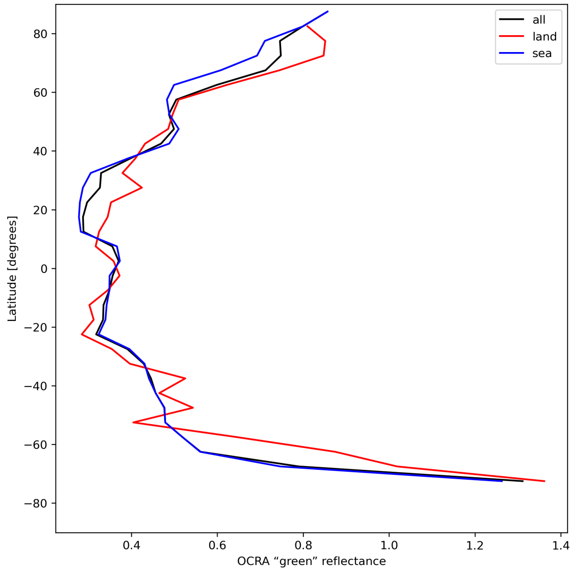
Figure 36: Zonal average of “OCRA “green” reflectance” for 2024-05-07 to 2024-05-08.
