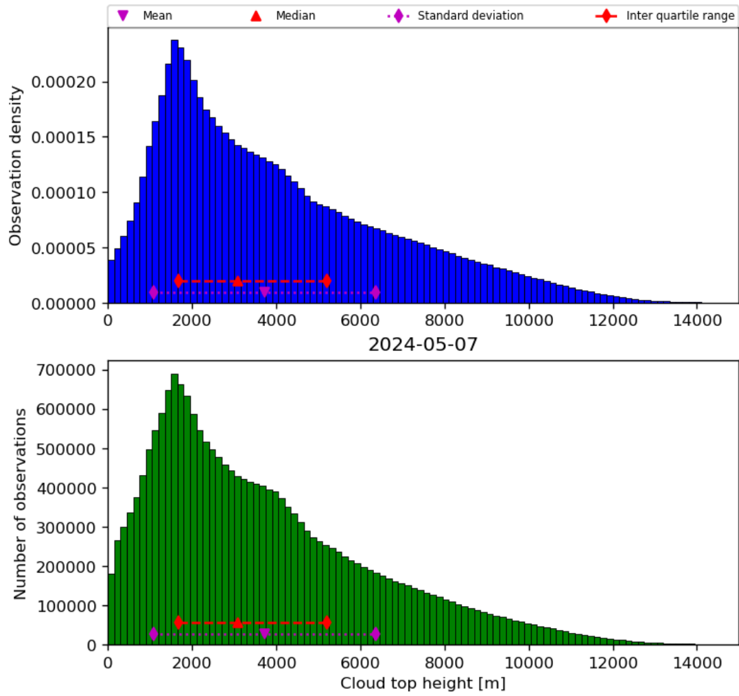
Figure 40: Histogram of “Cloud top height” for 2024-05-07 to 2024-05-08
