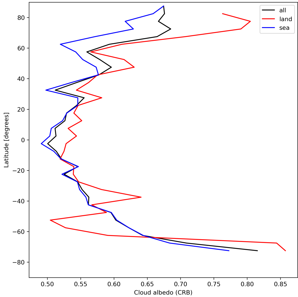
Figure 28: Zonal average of “Cloud albedo (CRB)” for 2024-05-07 to 2024-05-08.
