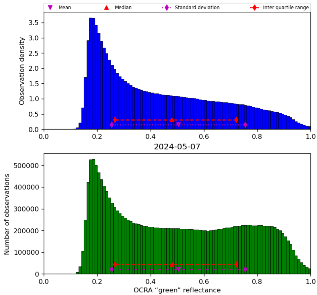
Figure 52: Histogram of “OCRA “green” reflectance” for 2024-05-07 to 2024-05-08
