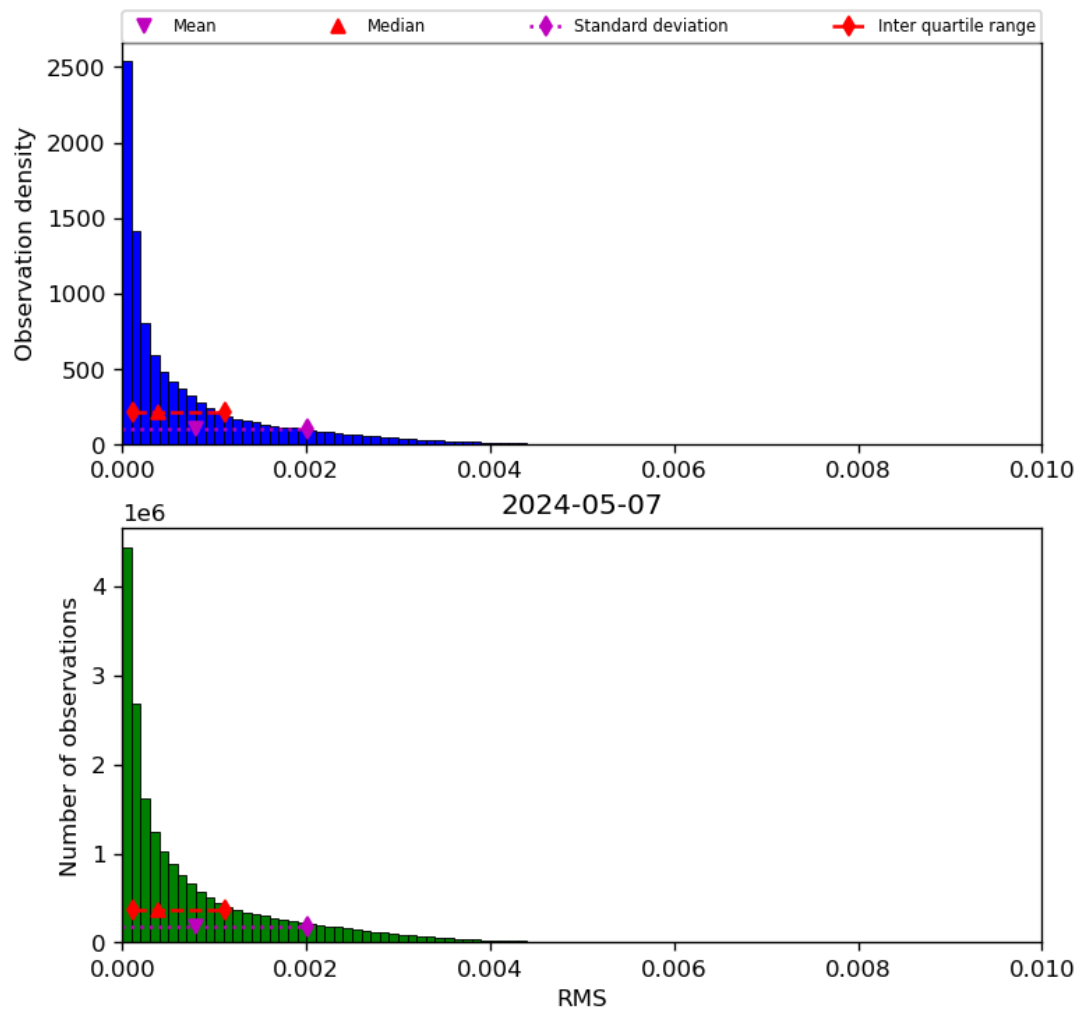
Figure 47: Histogram of “RMS” for 2024-05-07 to 2024-05-08
