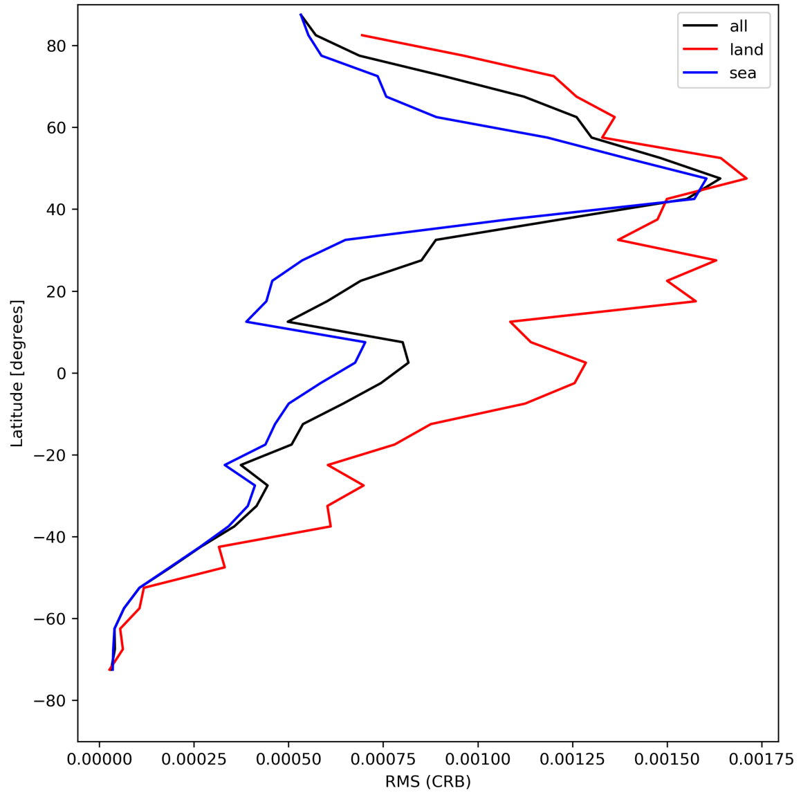
Figure 32: Zonal average of “RMS (CRB)” for 2024-05-07 to 2024-05-08.
