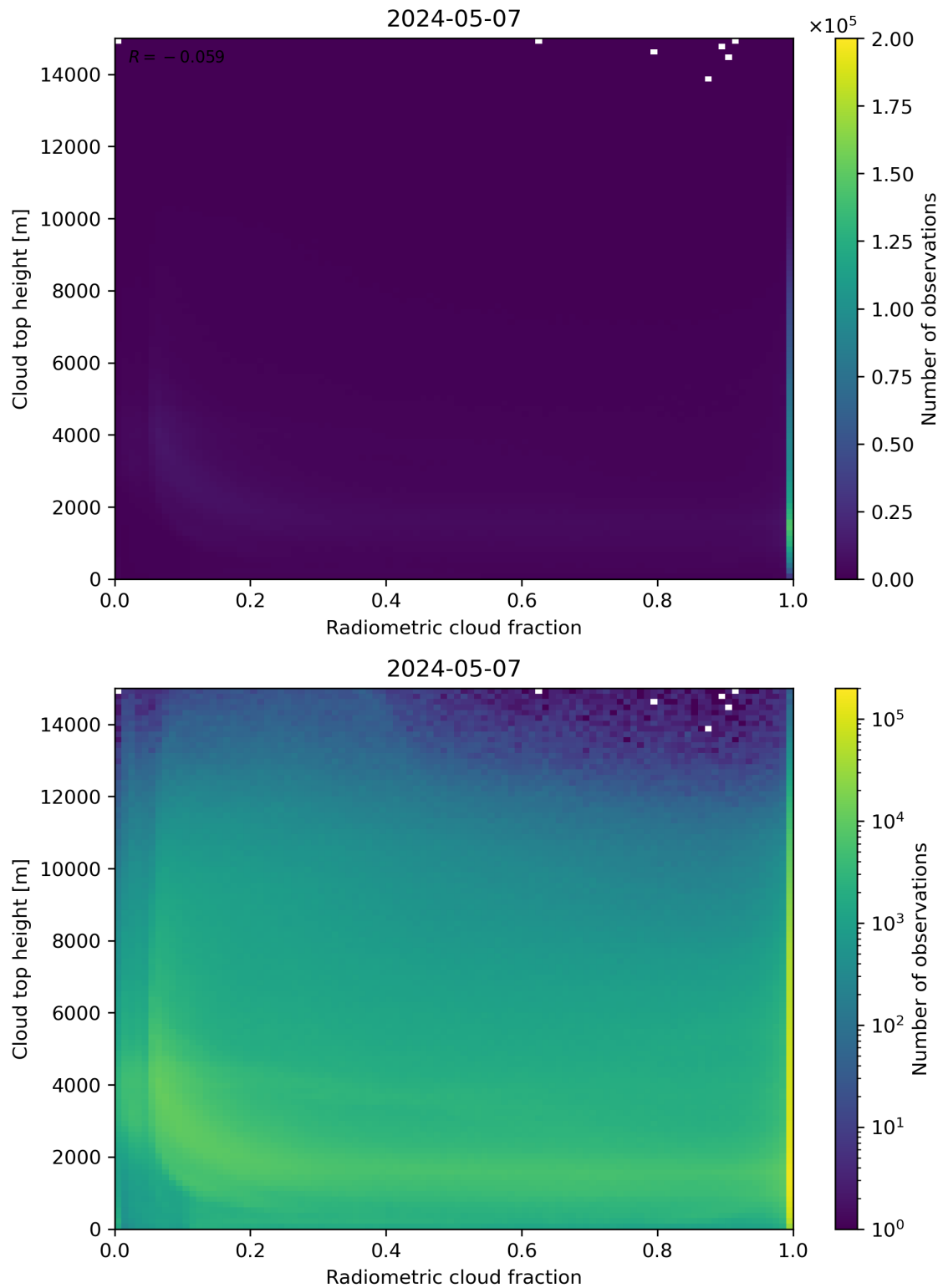
Figure 76: Scatter density plot of “Radiometric cloud fraction” against “Cloud top height” for 2024-05-07 to 2024-05-08.
