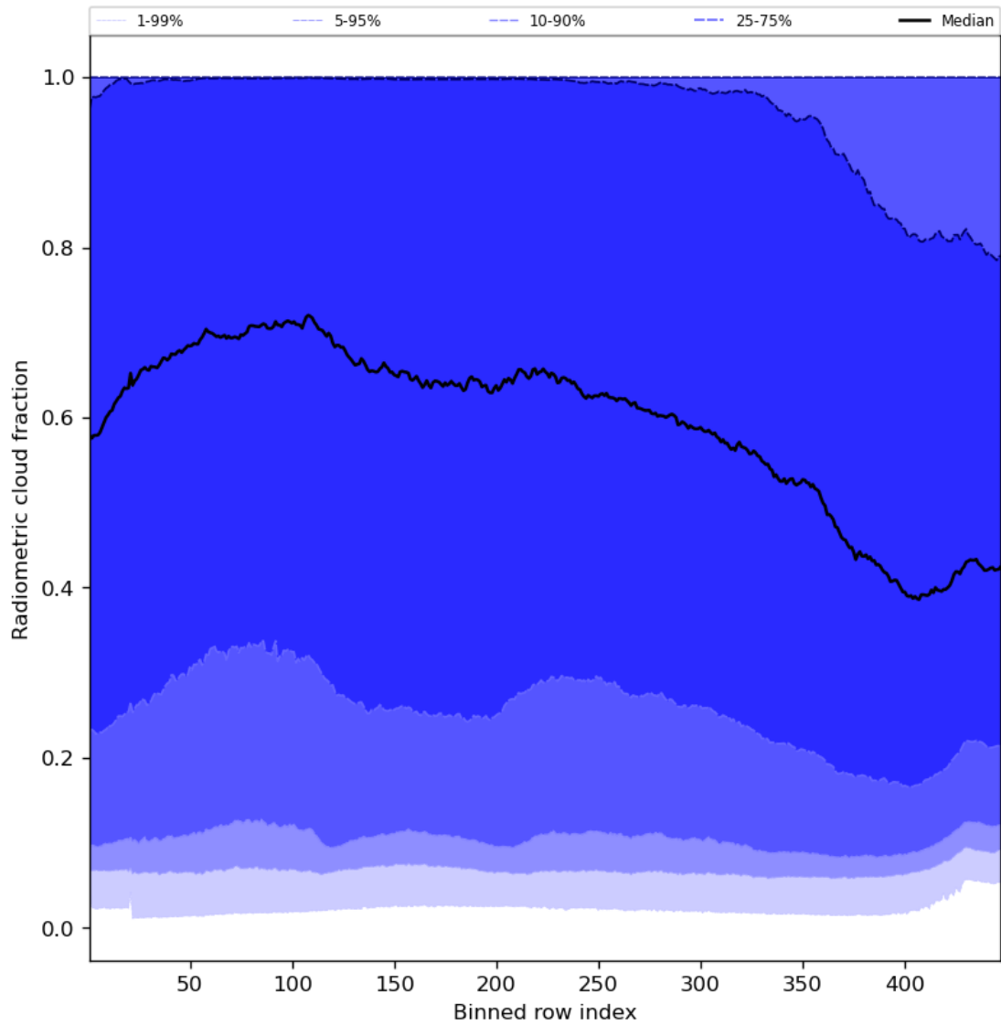
Figure 55: Along track statistics of “Radiometric cloud fraction” for 2024-05-07 to 2024-05-08
