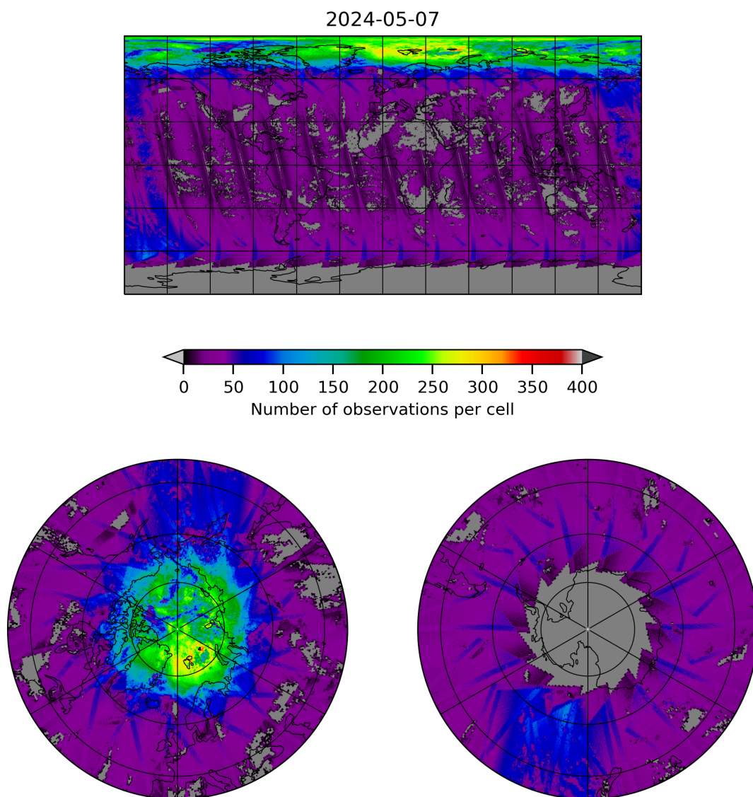
Figure 21: Map of the number of observations for 2024-05-07 to 2024-05-08
