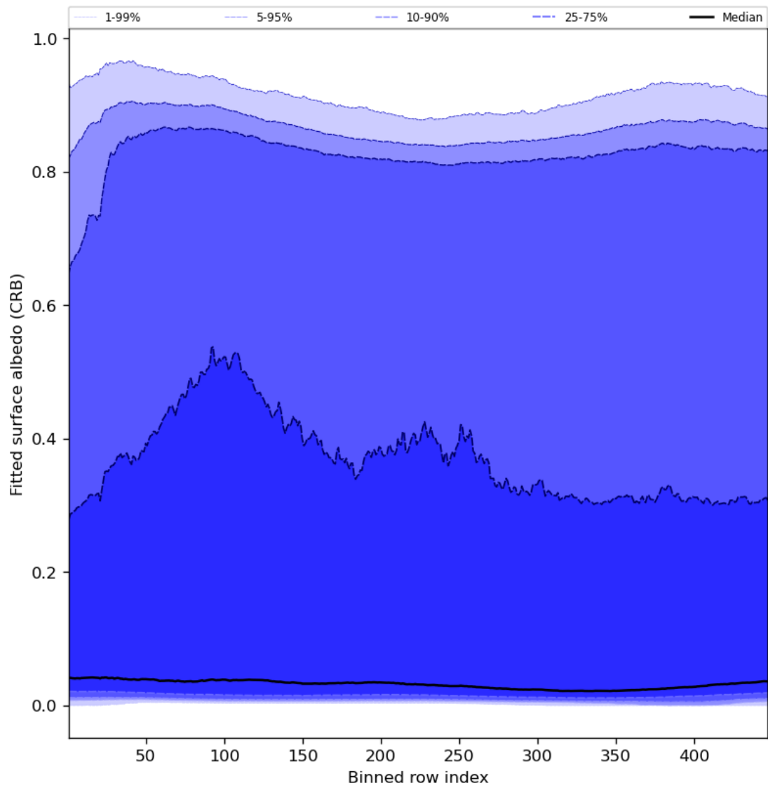
Figure 62: Along track statistics of “Fitted surface albedo (CRB)” for 2024-05-07 to 2024-05-08
