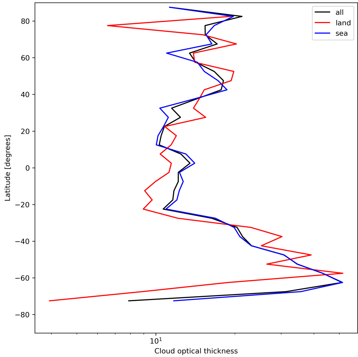
Figure 25: Zonal average of “Cloud optical thickness” for 2024-05-07 to 2024-05-08.
