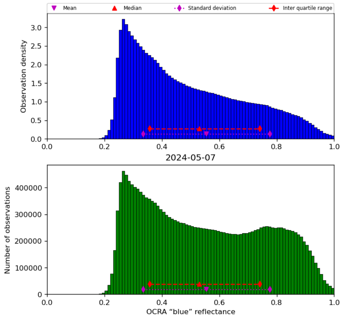
Figure 51: Histogram of “OCRA “blue” reflectance” for 2024-05-07 to 2024-05-08
