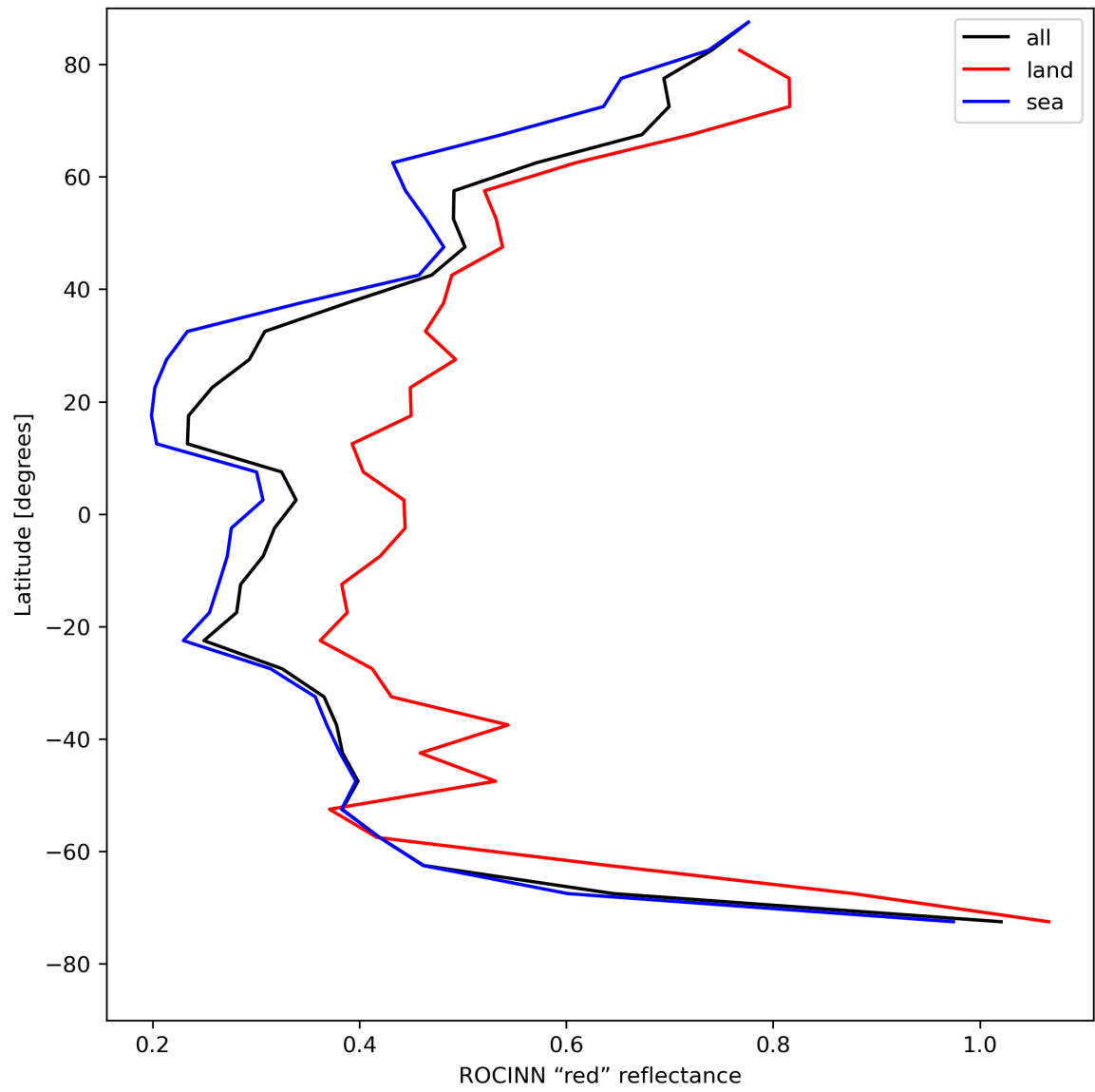
Figure 37: Zonal average of “ROCINN “red” reflectance” for 2024-05-07 to 2024-05-08.
