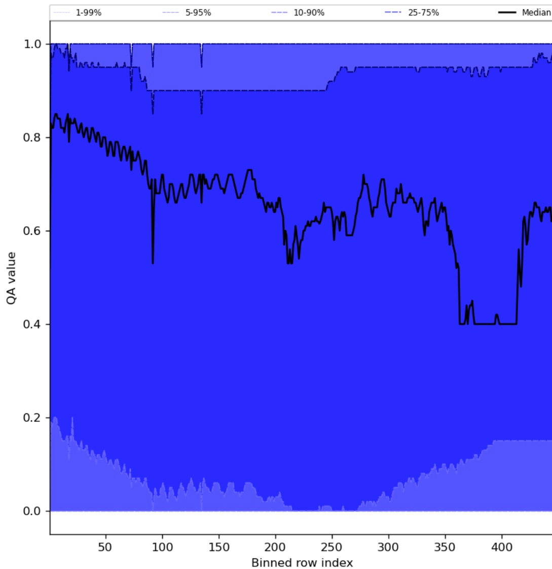
Figure 54: Along track statistics of “QA value” for 2024-05-07 to 2024-05-08
