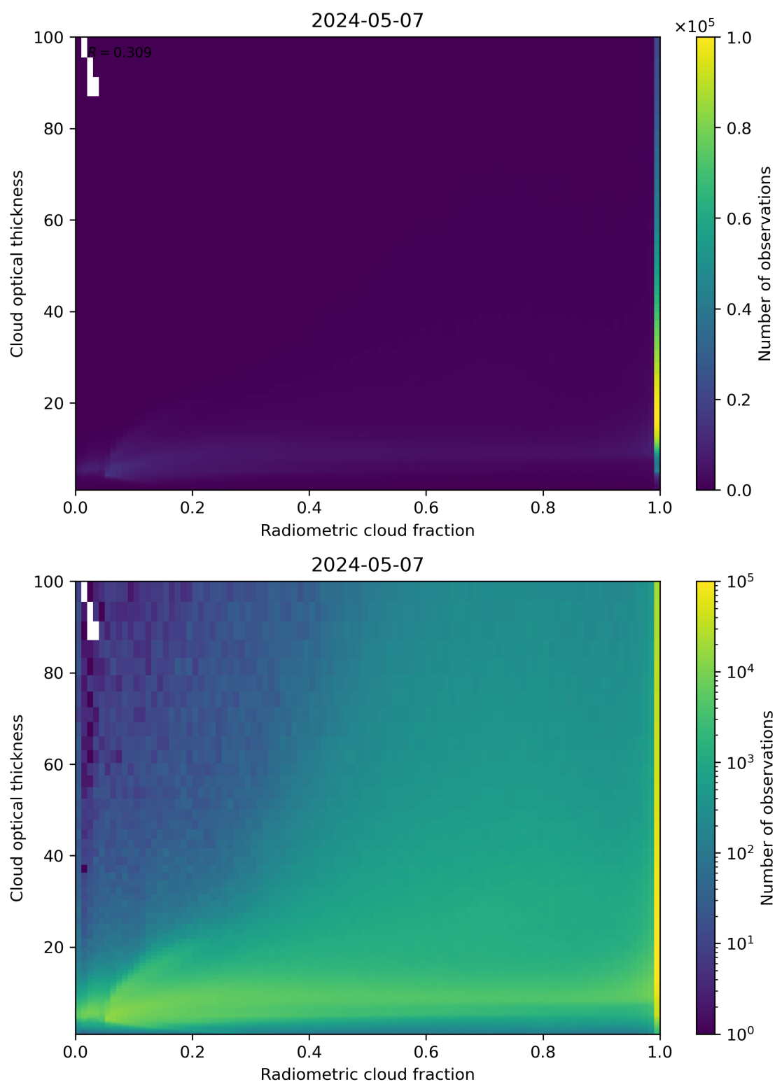
Figure 75: Scatter density plot of “Radiometric cloud fraction” against “Cloud optical thickness” for 2024-05-07 to 2024-05-08.
