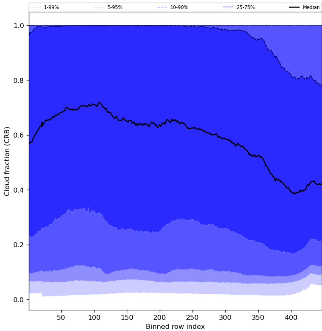
Figure 58: Along track statistics of “Cloud fraction (CRB)” for 2024-05-07 to 2024-05-08
