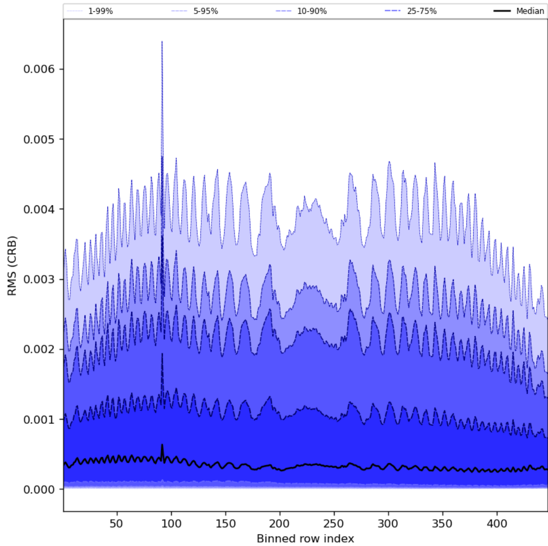
Figure 64: Along track statistics of “RMS (CRB)” for 2024-05-07 to 2024-05-08
