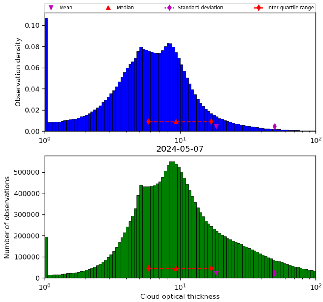
Figure 41: Histogram of “Cloud optical thickness” for 2024-05-07 to 2024-05-08
