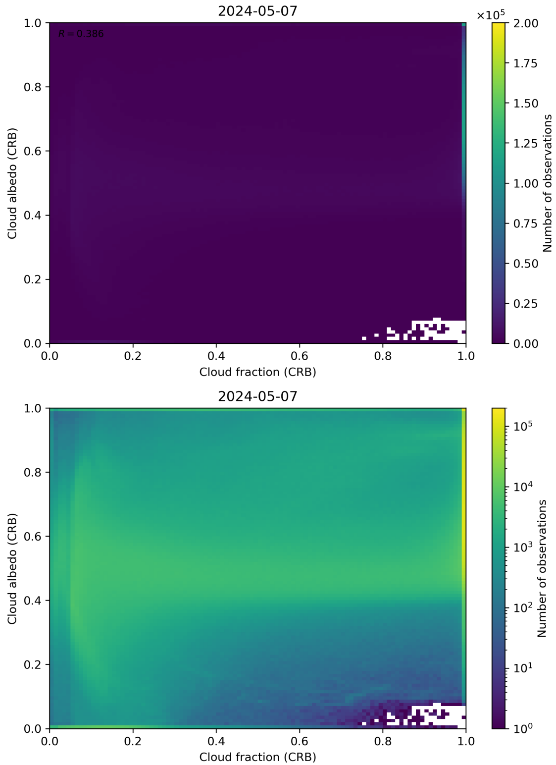
Figure 77: Scatter density plot of “Cloud fraction (CRB)” against “Cloud albedo (CRB)” for 2024-05-07 to 2024-05-08.
