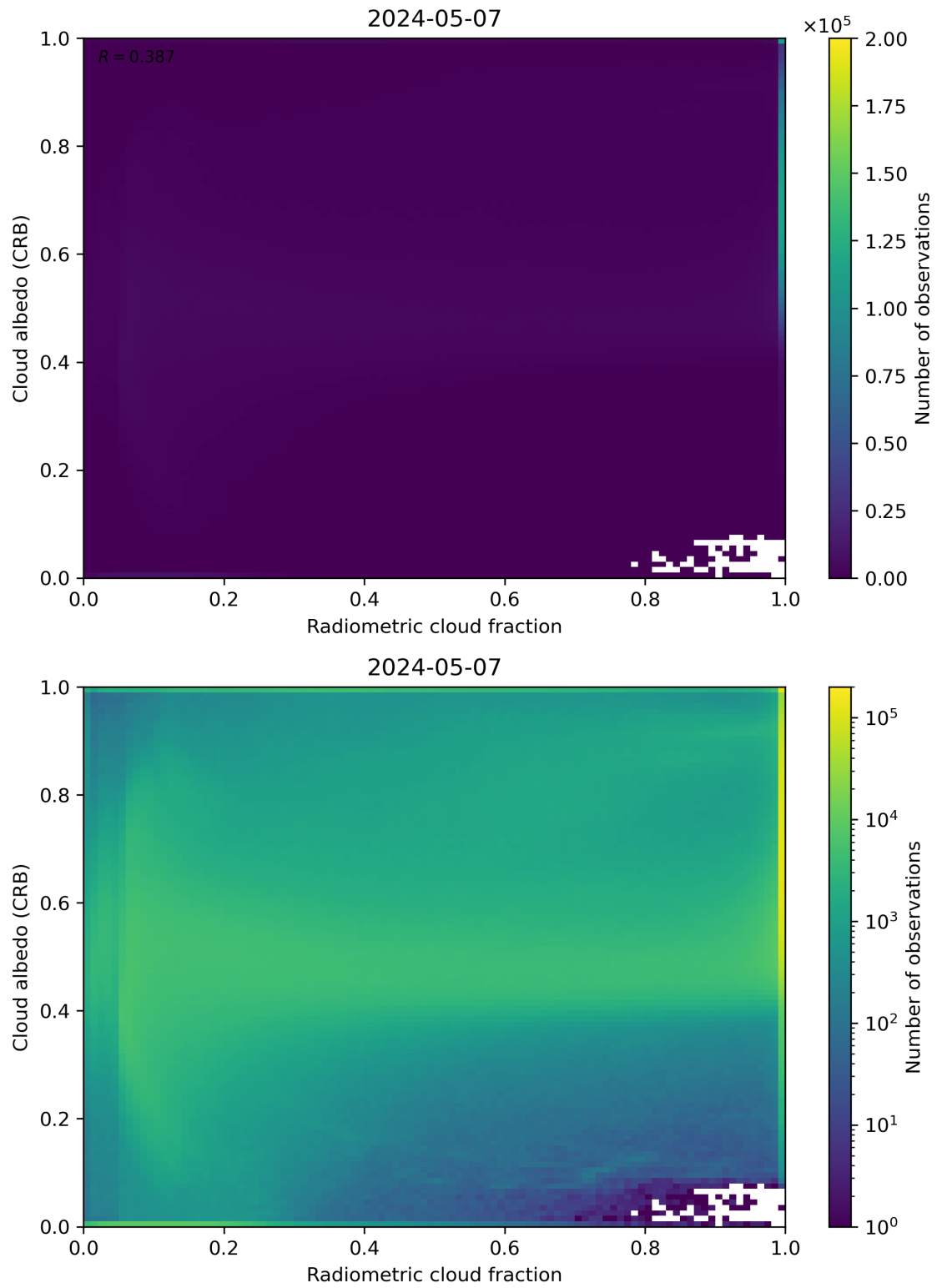
Figure 71: Scatter density plot of “Radiometric cloud fraction” against “Cloud albedo (CRB)” for 2024-05-07 to 2024-05-08.
