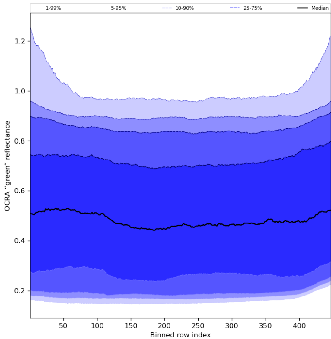
Figure 68: Along track statistics of “OCRA “green” reflectance” for 2024-05-07 to 2024-05-08
