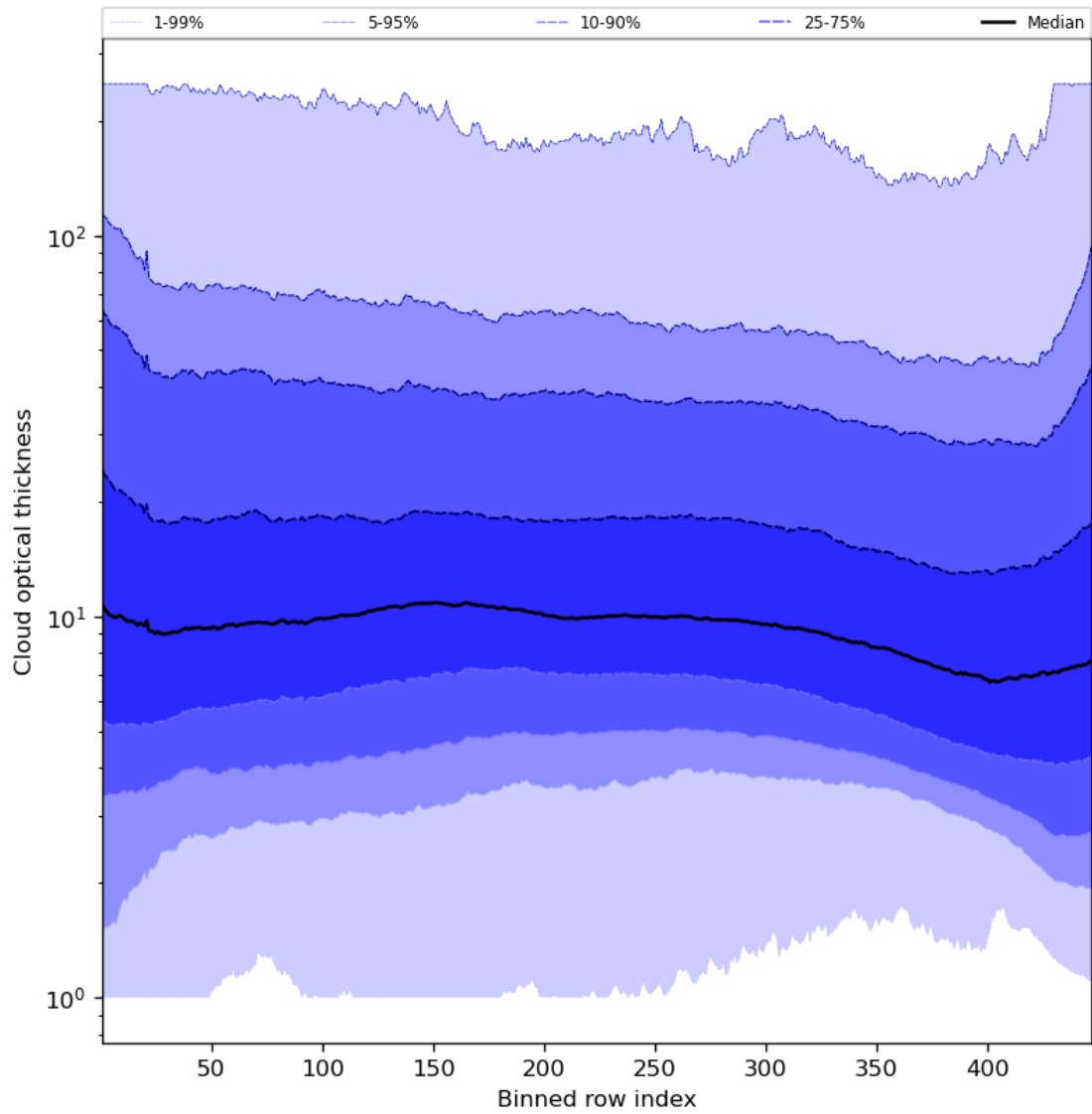
Figure 57: Along track statistics of “Cloud optical thickness” for 2024-05-07 to 2024-05-08
