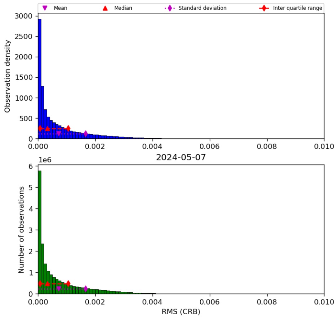
Figure 48: Histogram of “RMS (CRB)” for 2024-05-07 to 2024-05-08
