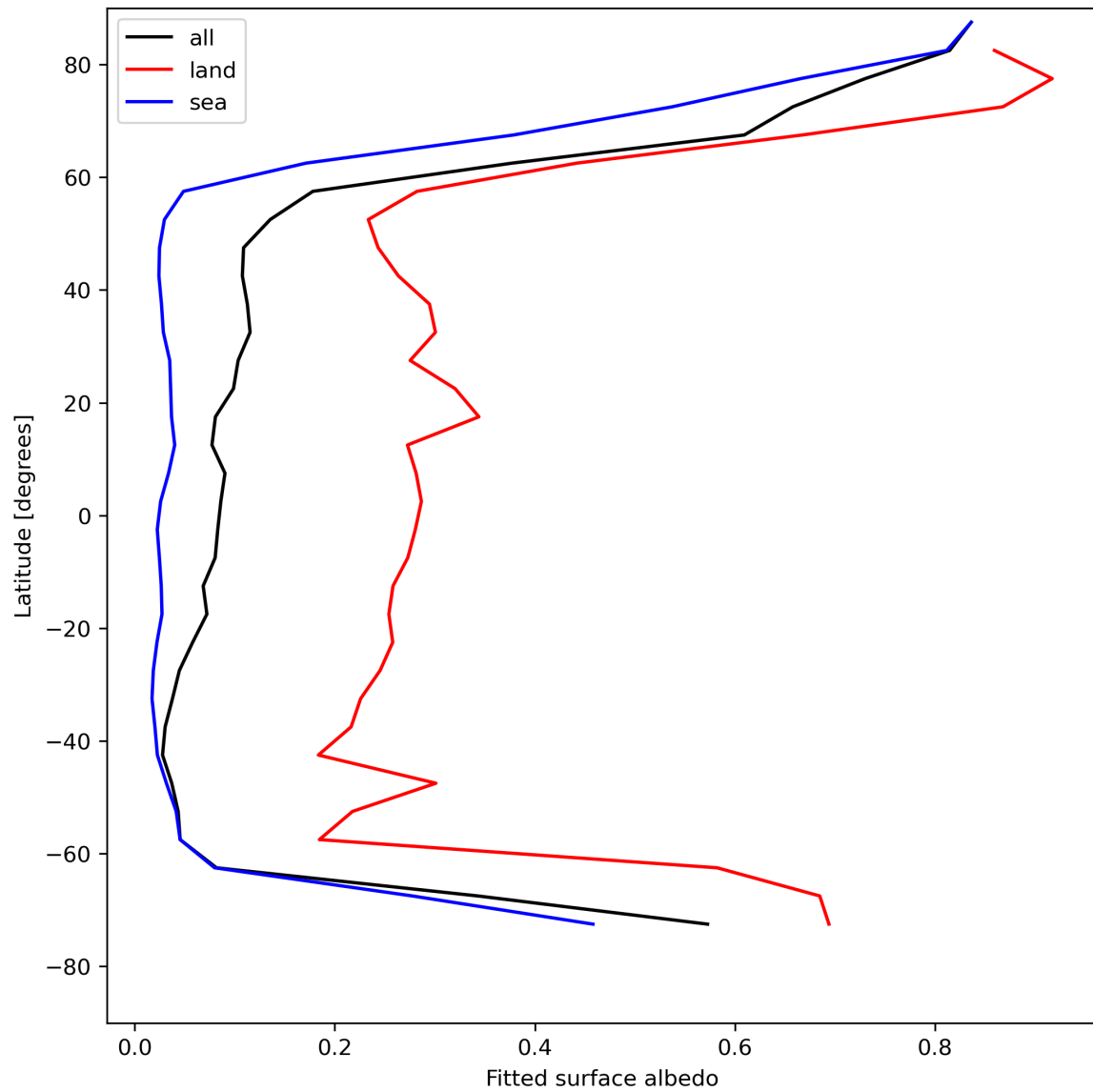
Figure 29: Zonal average of “Fitted surface albedo” for 2024-05-07 to 2024-05-08.
