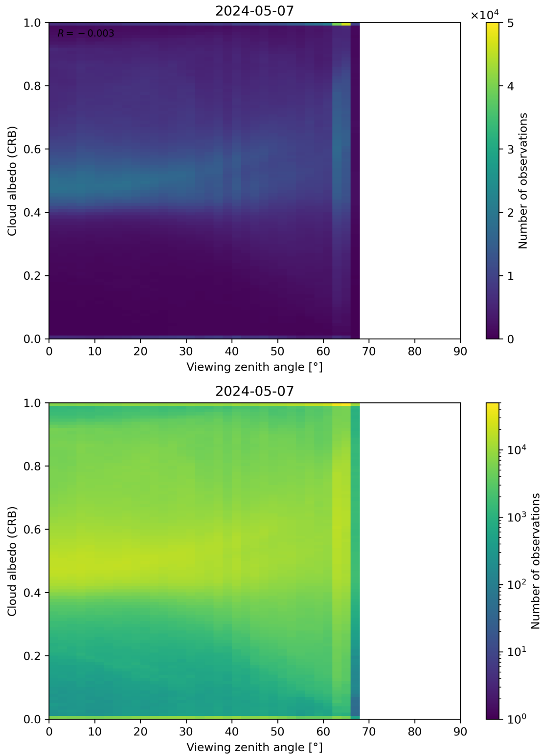
Figure 106: Scatter density plot of “Viewing zenith angle” against “Cloud albedo (CRB)” for 2024-05-07 to 2024-05-08.
