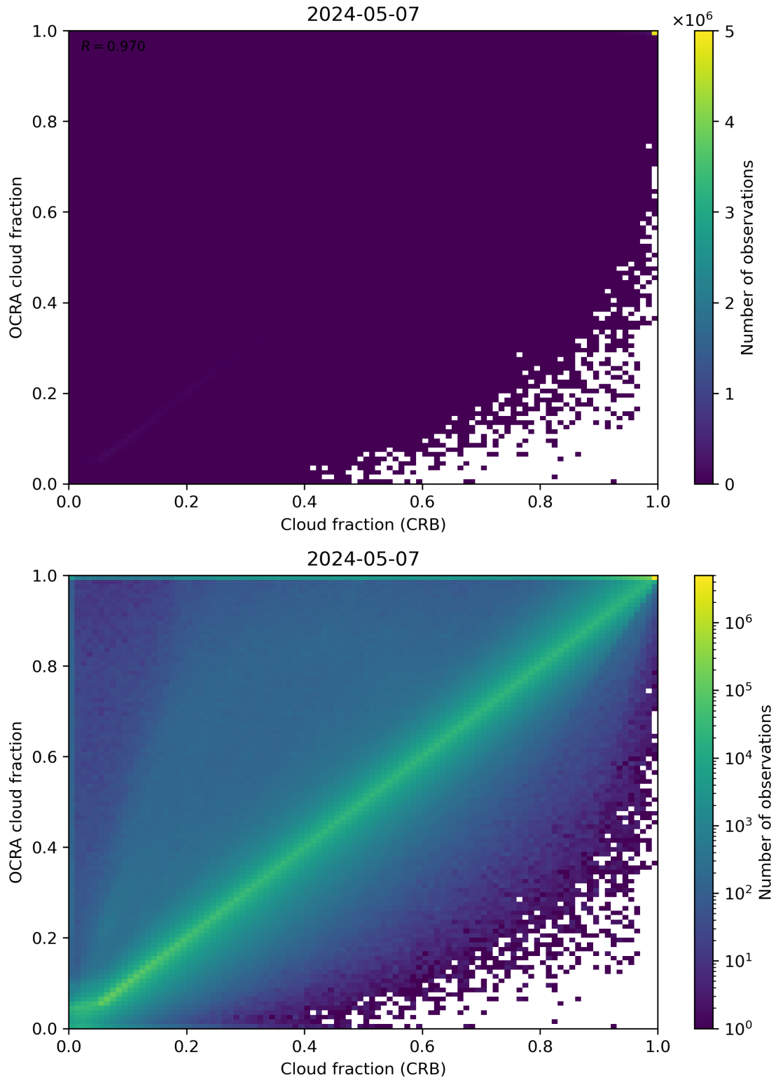
Figure 78: Scatter density plot of “Cloud fraction (CRB)” against “OCRA cloud fraction” for 2024-05-07 to 2024-05-08.
