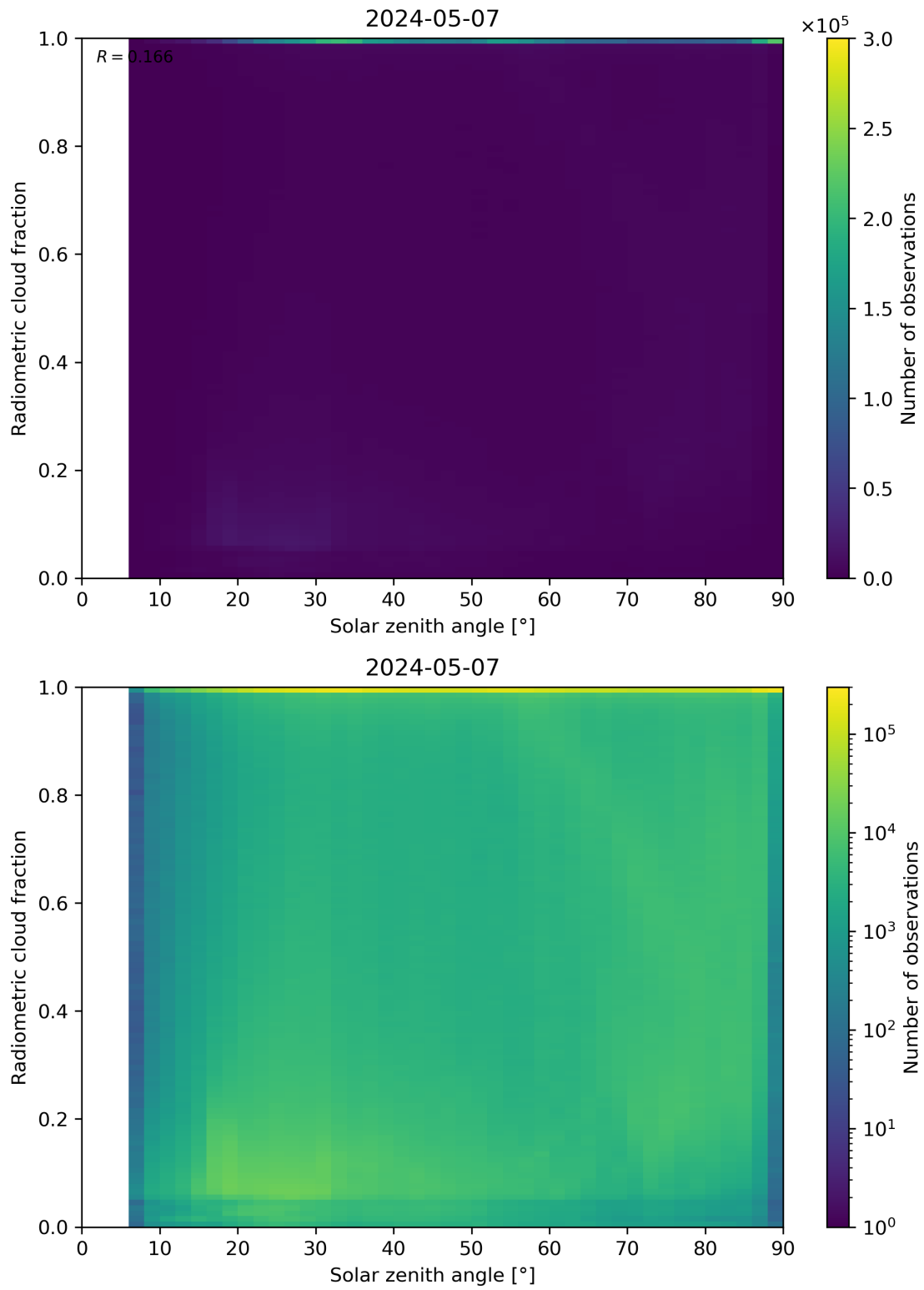
Figure 99: Scatter density plot of “Solar zenith angle” against “Radiometric cloud fraction” for 2024-05-07 to 2024-05-08.
