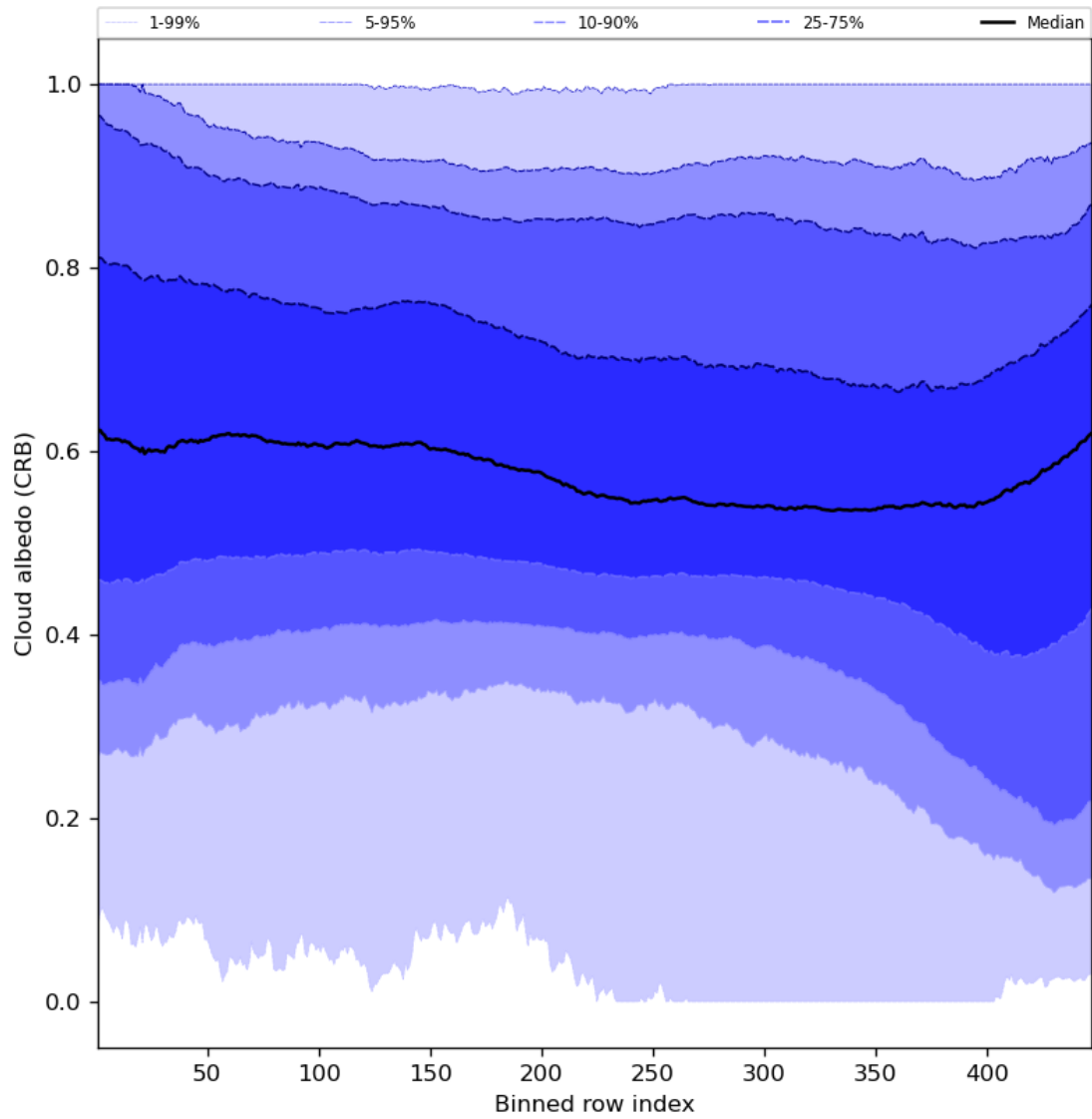
Figure 60: Along track statistics of “Cloud albedo (CRB)” for 2024-05-07 to 2024-05-08
