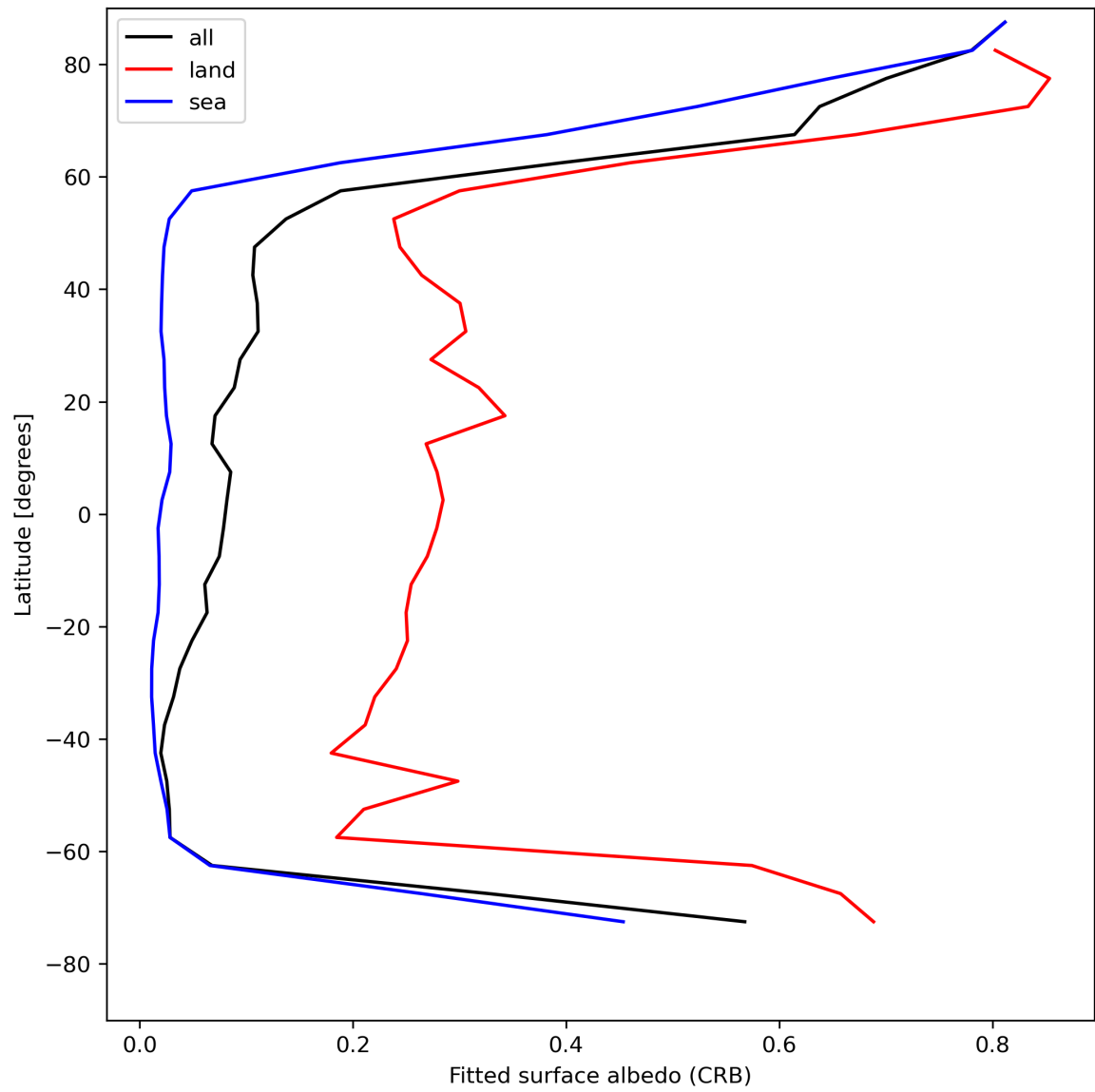
Figure 30: Zonal average of “Fitted surface albedo (CRB)” for 2024-05-07 to 2024-05-08.
