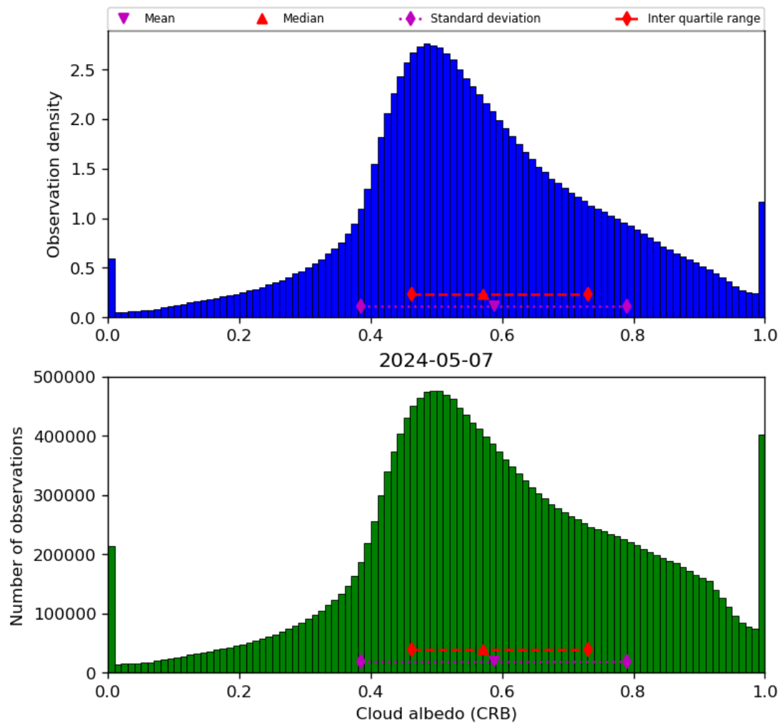
Figure 44: Histogram of “Cloud albedo (CRB)” for 2024-05-07 to 2024-05-08
