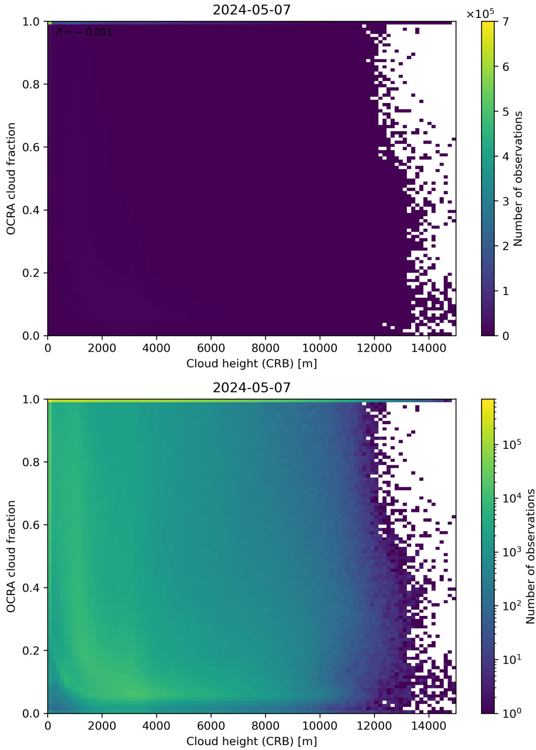
Figure 81: Scatter density plot of “Cloud height (CRB)” against “OCRA cloud fraction” for 2024-05-07 to 2024-05-08.
