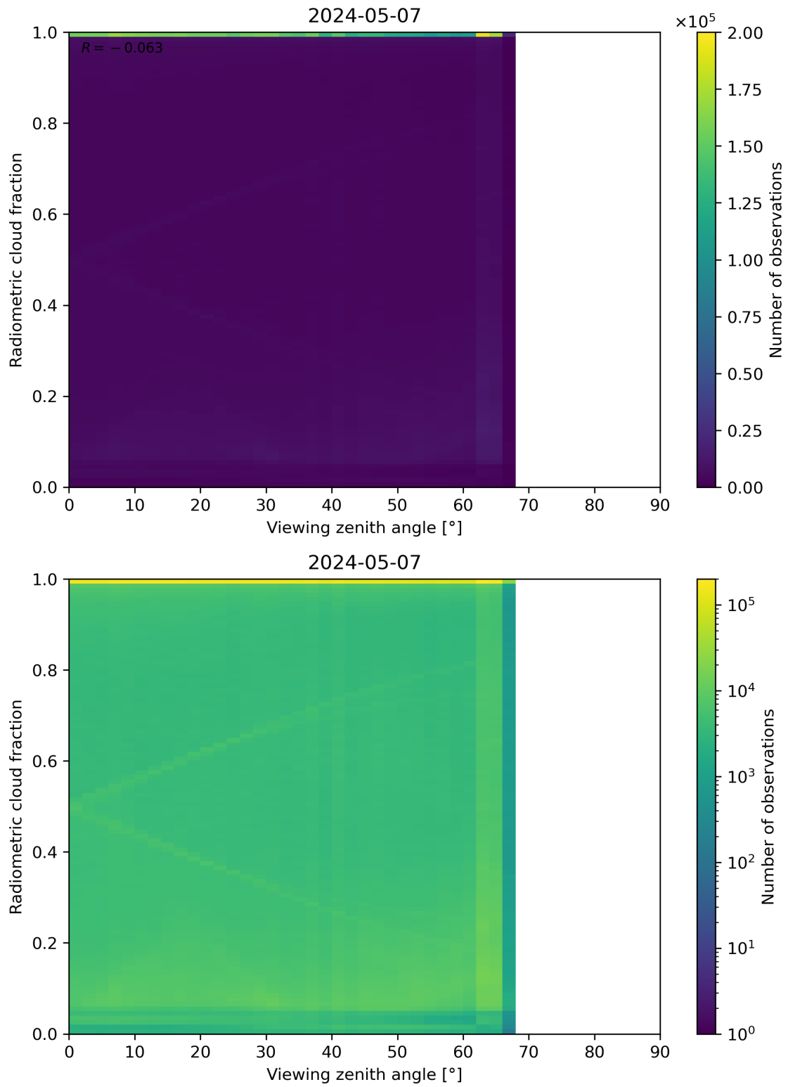
Figure 107: Scatter density plot of “Viewing zenith angle” against “Radiometric cloud fraction” for 2024-05-07 to 2024-05-08.
