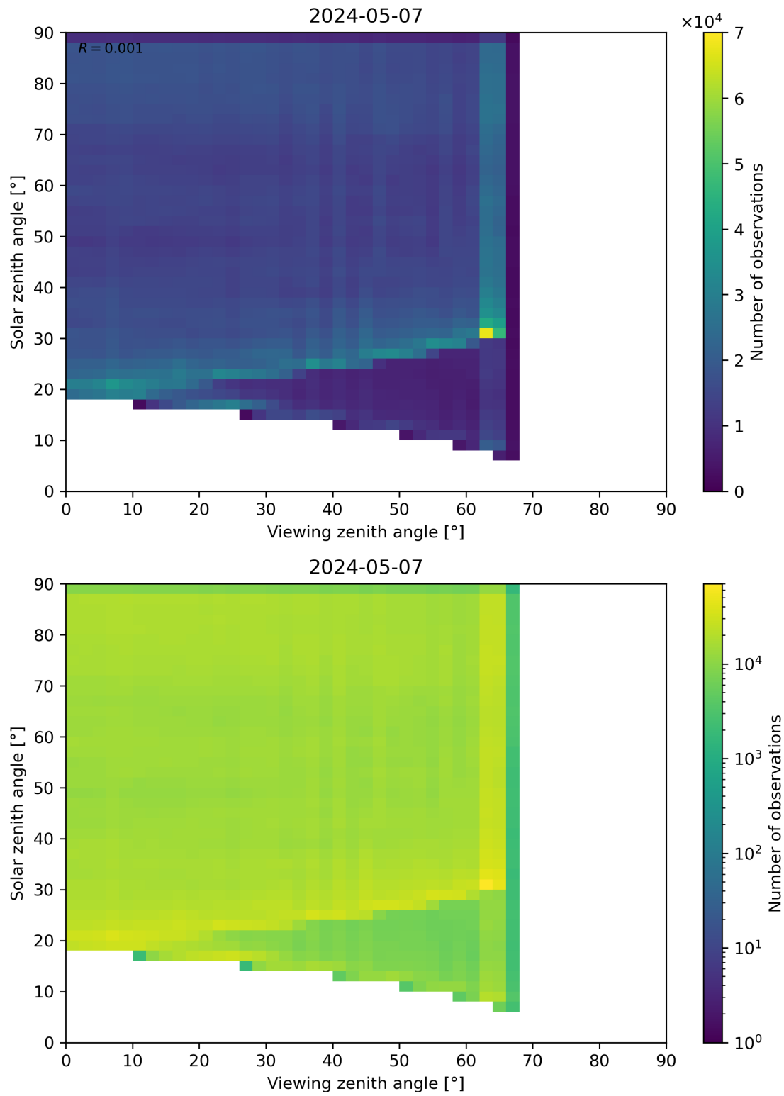
Figure 114: Scatter density plot of “Viewing zenith angle” against “Solar zenith angle” for 2024-05-07 to 2024-05-08.
