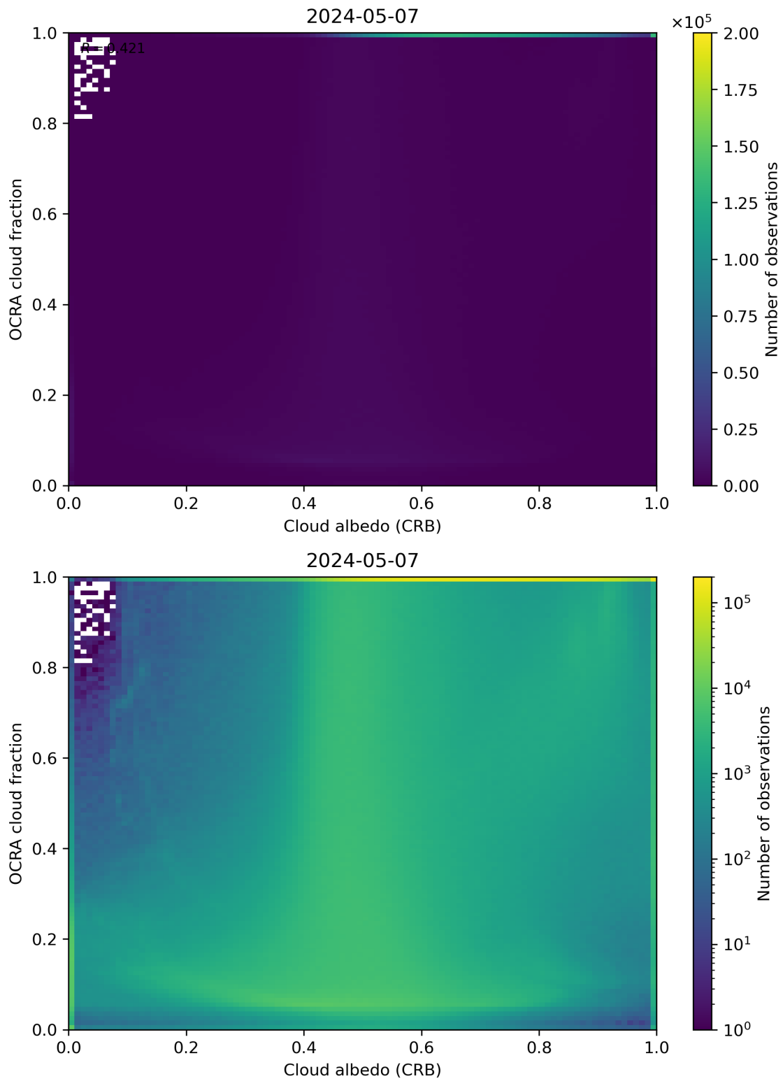
Figure 70: Scatter density plot of “Cloud albedo (CRB)” against “OCRA cloud fraction” for 2024-05-07 to 2024-05-08.
