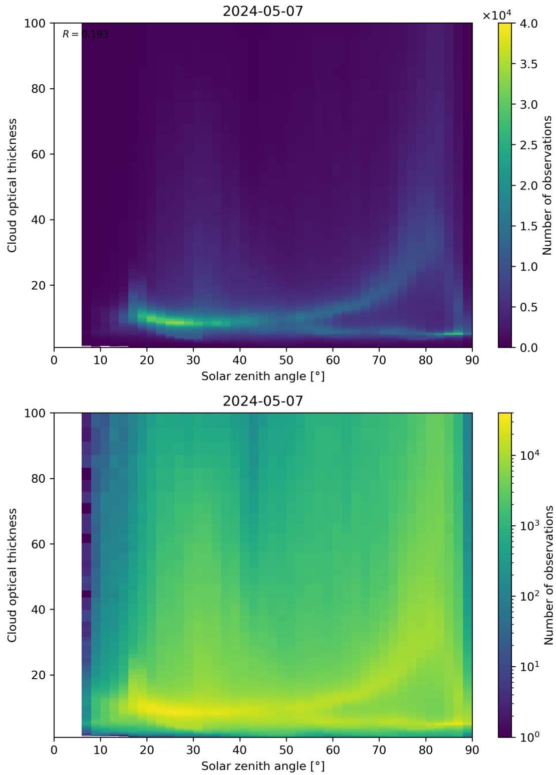
Figure 103: Scatter density plot of “Solar zenith angle” against “Cloud optical thickness” for 2024-05-07 to 2024-05-08.
