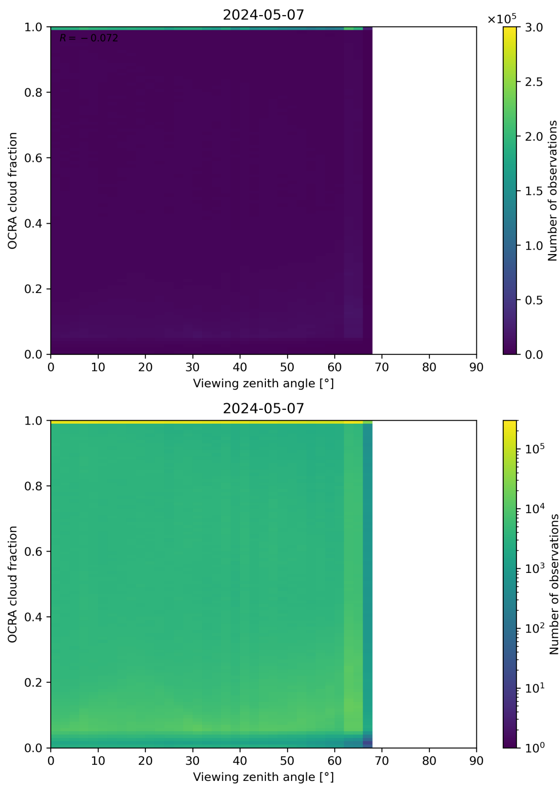
Figure 108: Scatter density plot of “Viewing zenith angle” against “OCRA cloud fraction” for 2024-05-07 to 2024-05-08.
