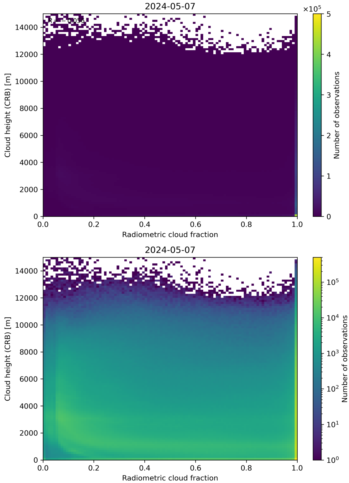
Figure 74: Scatter density plot of “Radiometric cloud fraction” against “Cloud height (CRB)” for 2024-05-07 to 2024-05-08.
