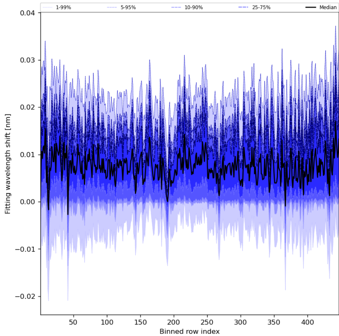
Figure 65: Along track statistics of “Fitting wavelength shift” for 2024-05-07 to 2024-05-08
