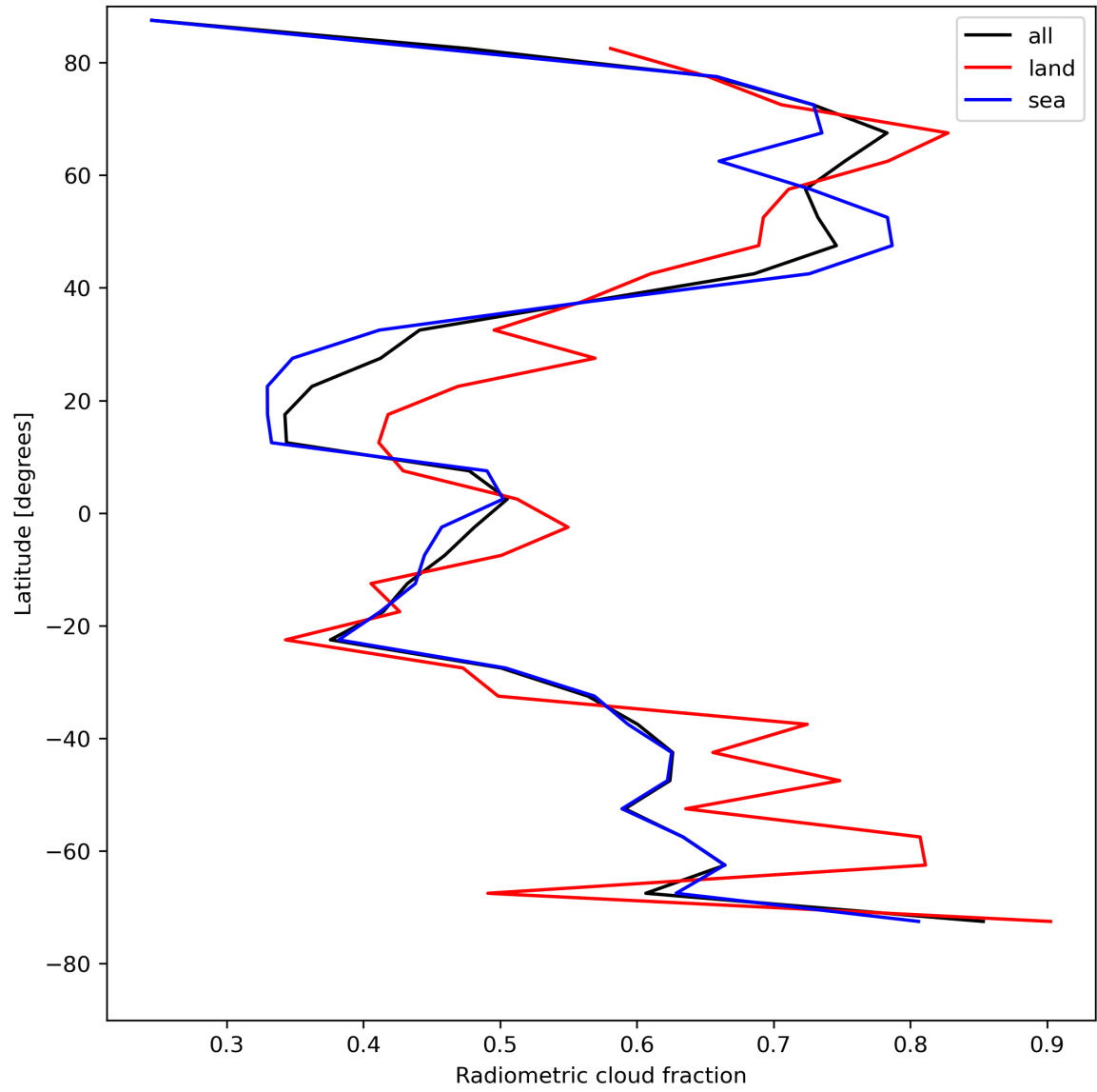
Figure 23: Zonal average of “Radiometric cloud fraction” for 2024-05-07 to 2024-05-08.
