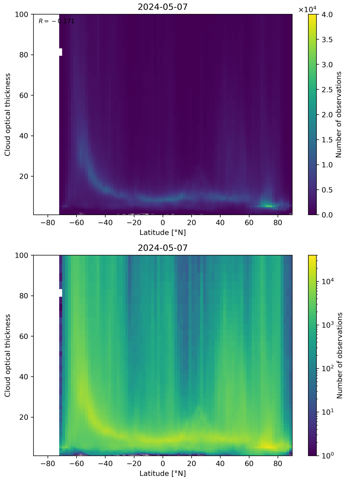
Figure 96: Scatter density plot of “Latitude” against “Cloud optical thickness” for 2024-05-07 to 2024-05-08.
