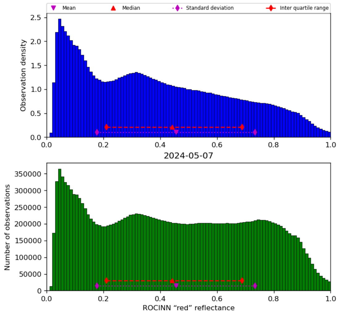
Figure 53: Histogram of “ROCINN “red” reflectance” for 2024-05-07 to 2024-05-08
