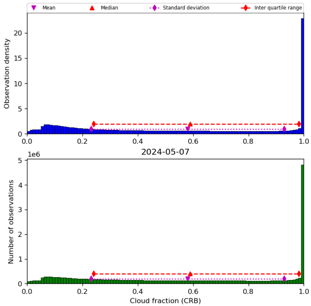
Figure 42: Histogram of “Cloud fraction (CRB)” for 2024-05-07 to 2024-05-08
