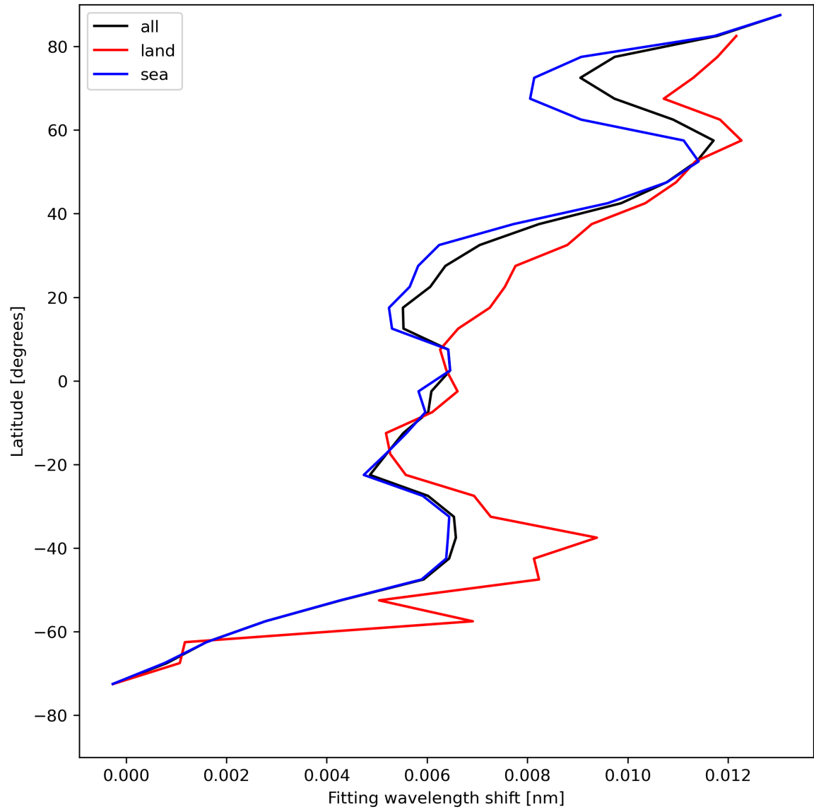
Figure 33: Zonal average of “Fitting wavelength shift” for 2024-05-07 to 2024-05-08.
