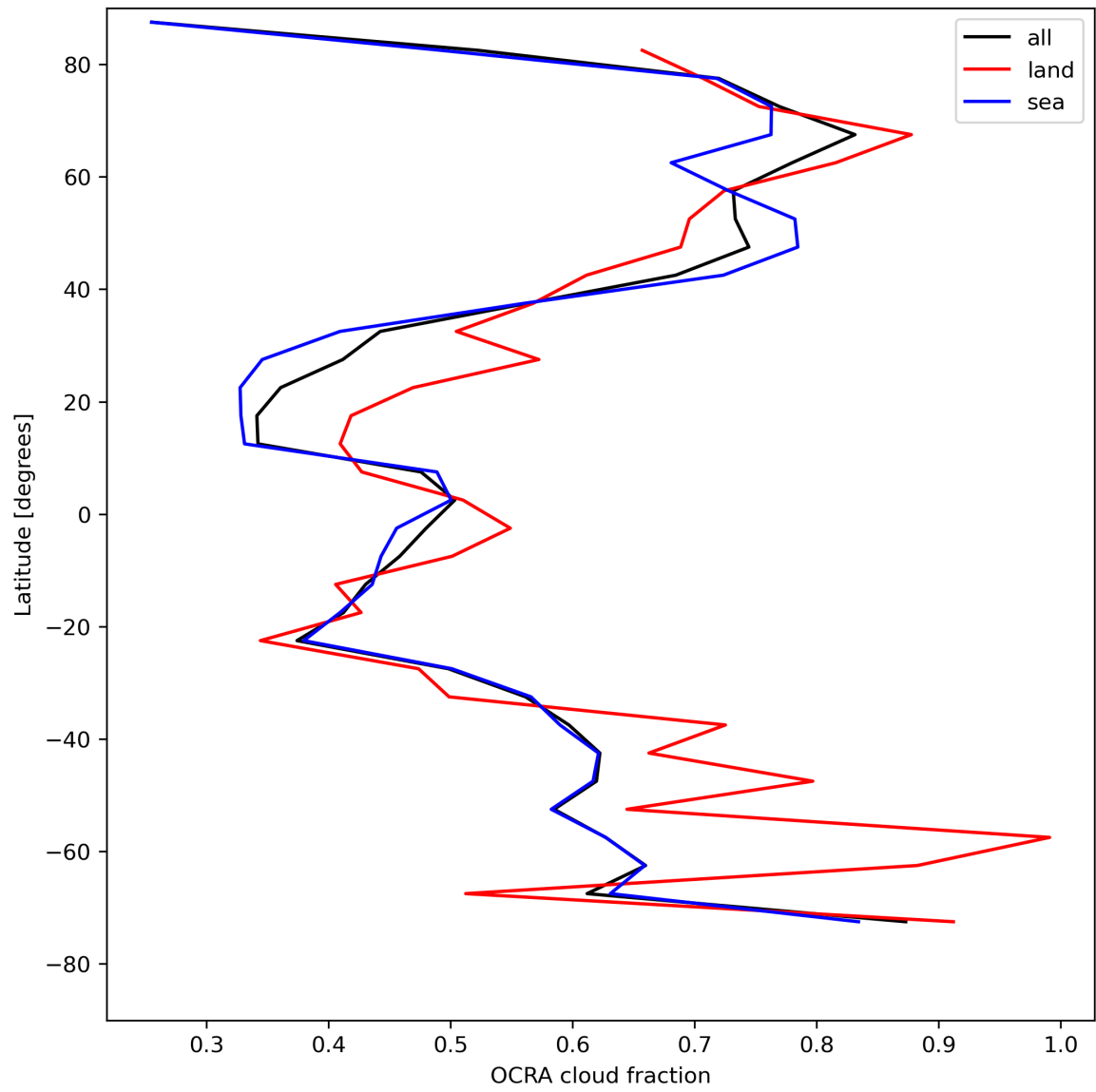
Figure 34: Zonal average of “OCRA cloud fraction” for 2024-05-07 to 2024-05-08.
