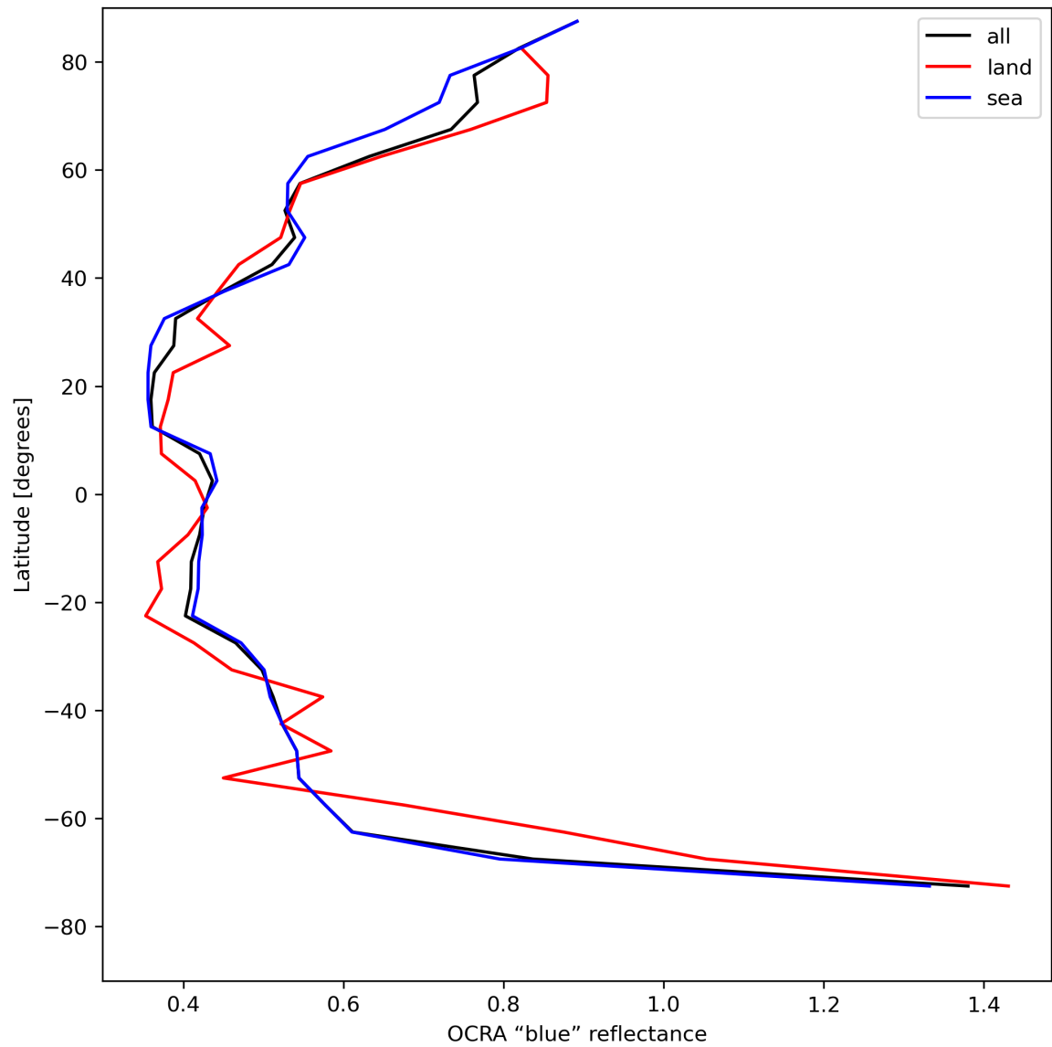
Figure 35: Zonal average of “OCRA “blue” reflectance” for 2024-05-07 to 2024-05-08.
