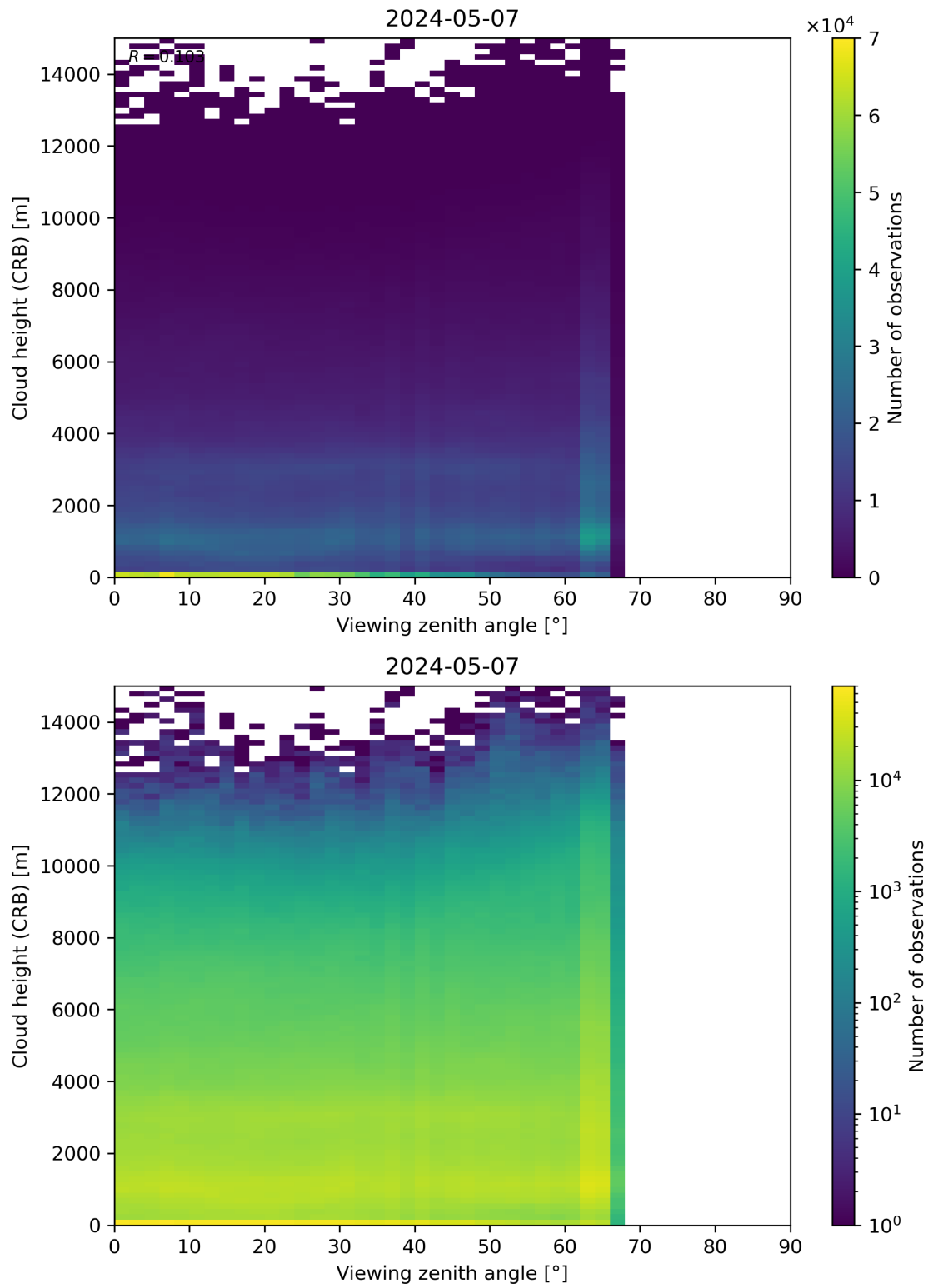
Figure 110: Scatter density plot of “Viewing zenith angle” against “Cloud height (CRB)” for 2024-05-07 to 2024-05-08.
