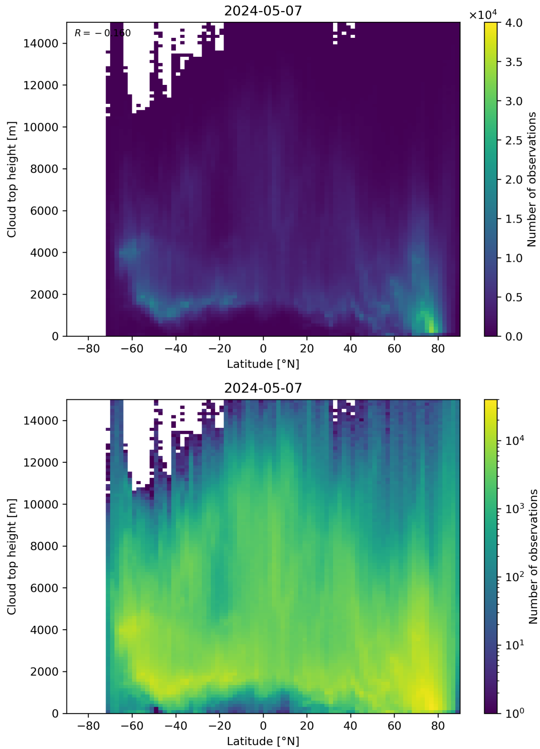
Figure 97: Scatter density plot of “Latitude” against “Cloud top height” for 2024-05-07 to 2024-05-08.
