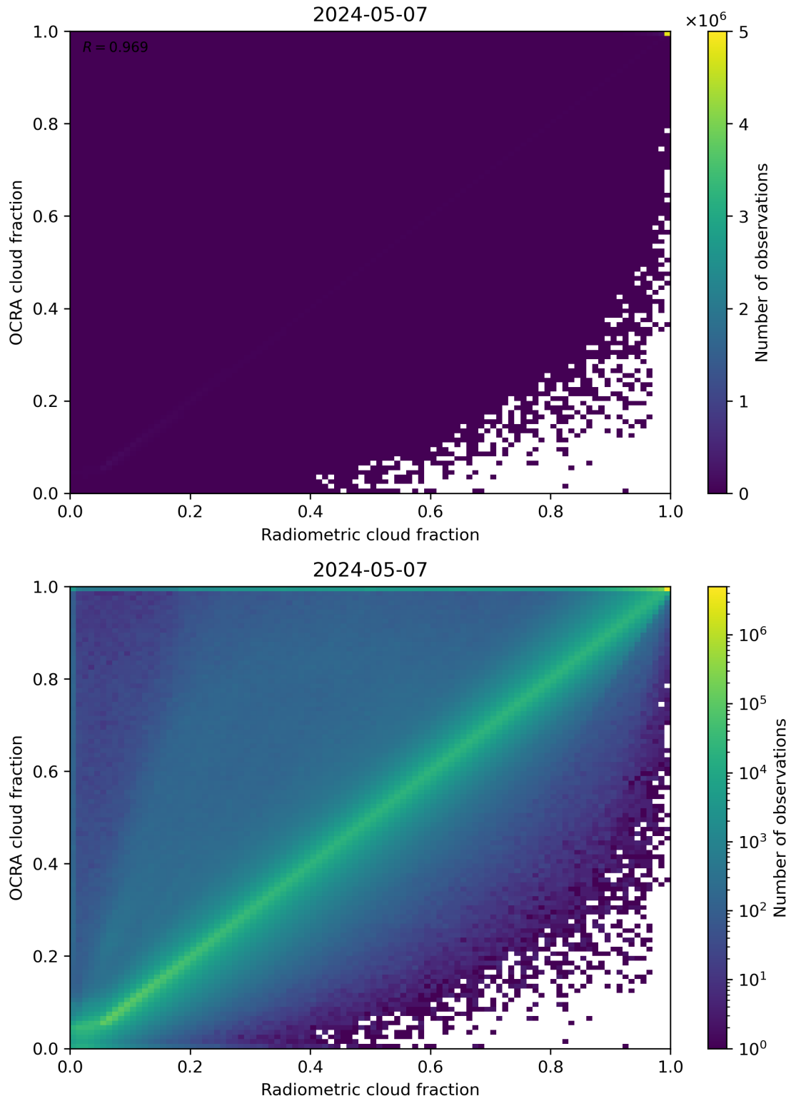
Figure 72: Scatter density plot of “Radiometric cloud fraction” against “OCRA cloud fraction” for 2024-05-07 to 2024-05-08.
