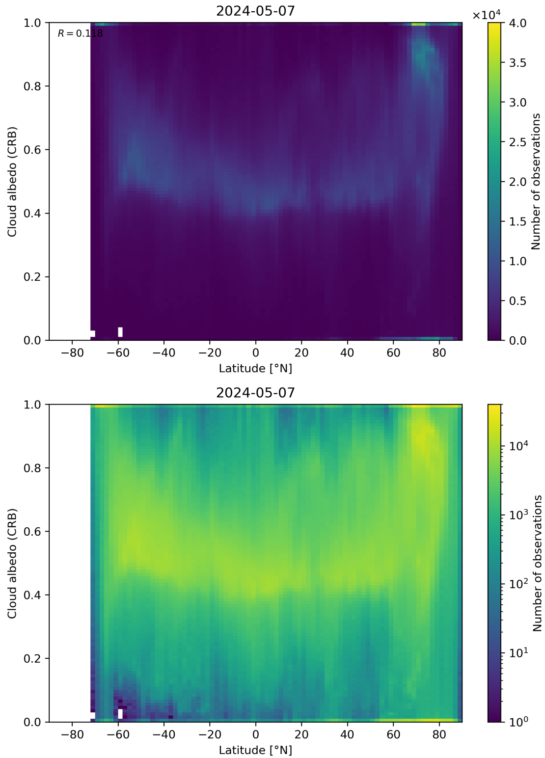
Figure 91: Scatter density plot of “Latitude” against “Cloud albedo (CRB)” for 2024-05-07 to 2024-05-08.
