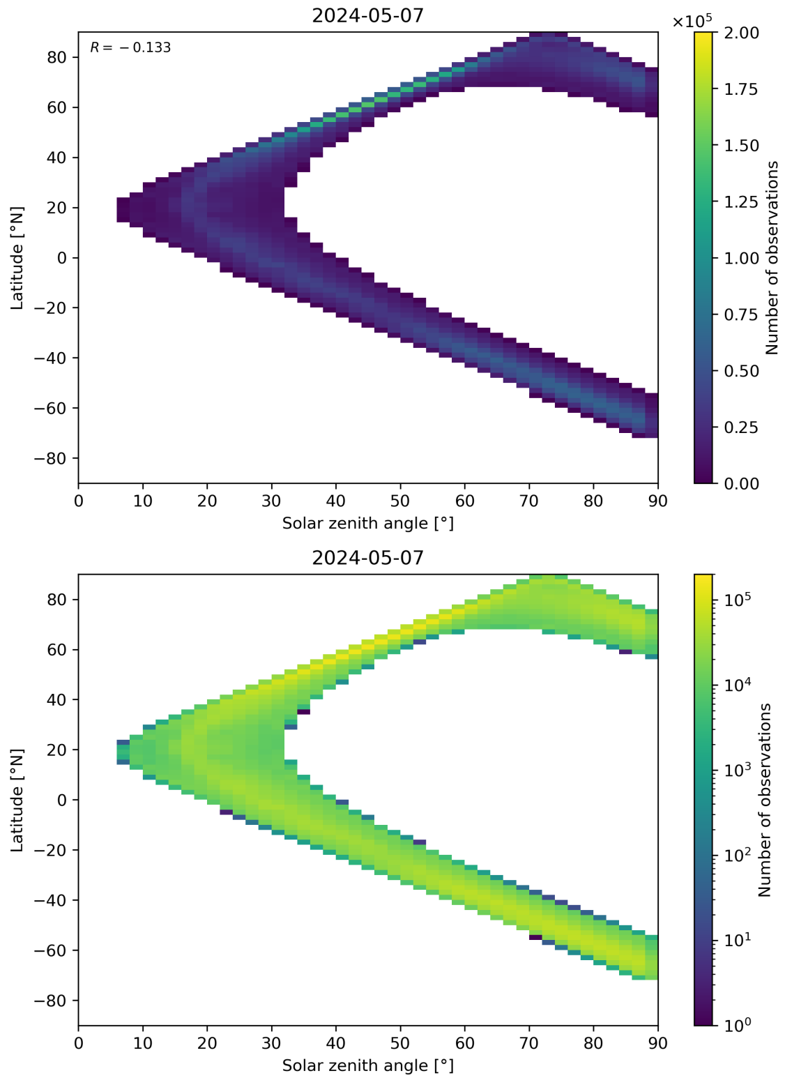
Figure 105: Scatter density plot of “Solar zenith angle” against “Latitude” for 2024-05-07 to 2024-05-08.
