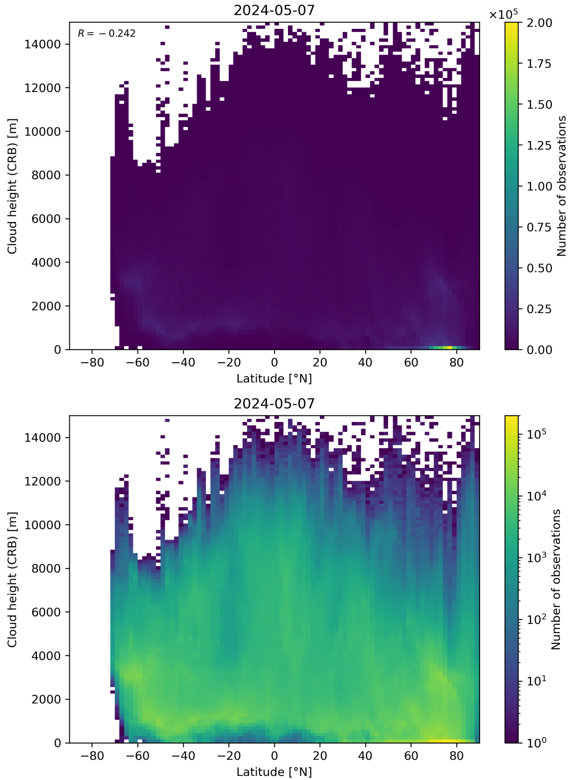
Figure 95: Scatter density plot of “Latitude” against “Cloud height (CRB)” for 2024-05-07 to 2024-05-08.
