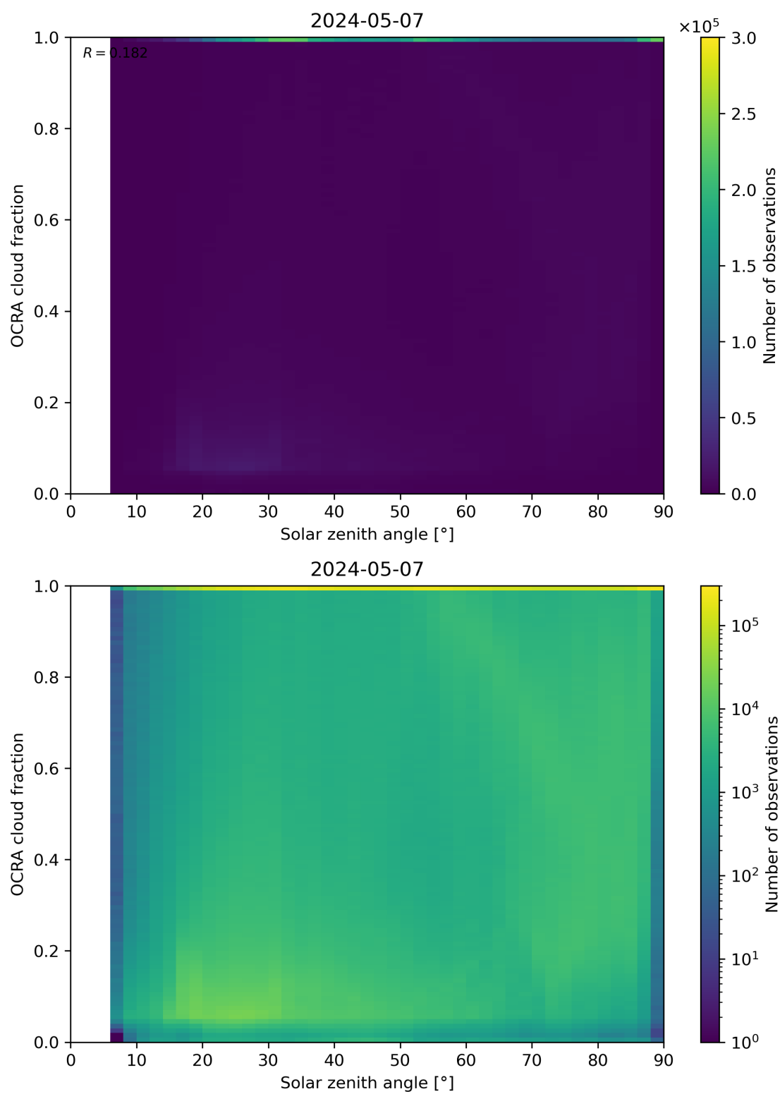
Figure 100: Scatter density plot of “Solar zenith angle” against “OCRA cloud fraction” for 2024-05-07 to 2024-05-08.
