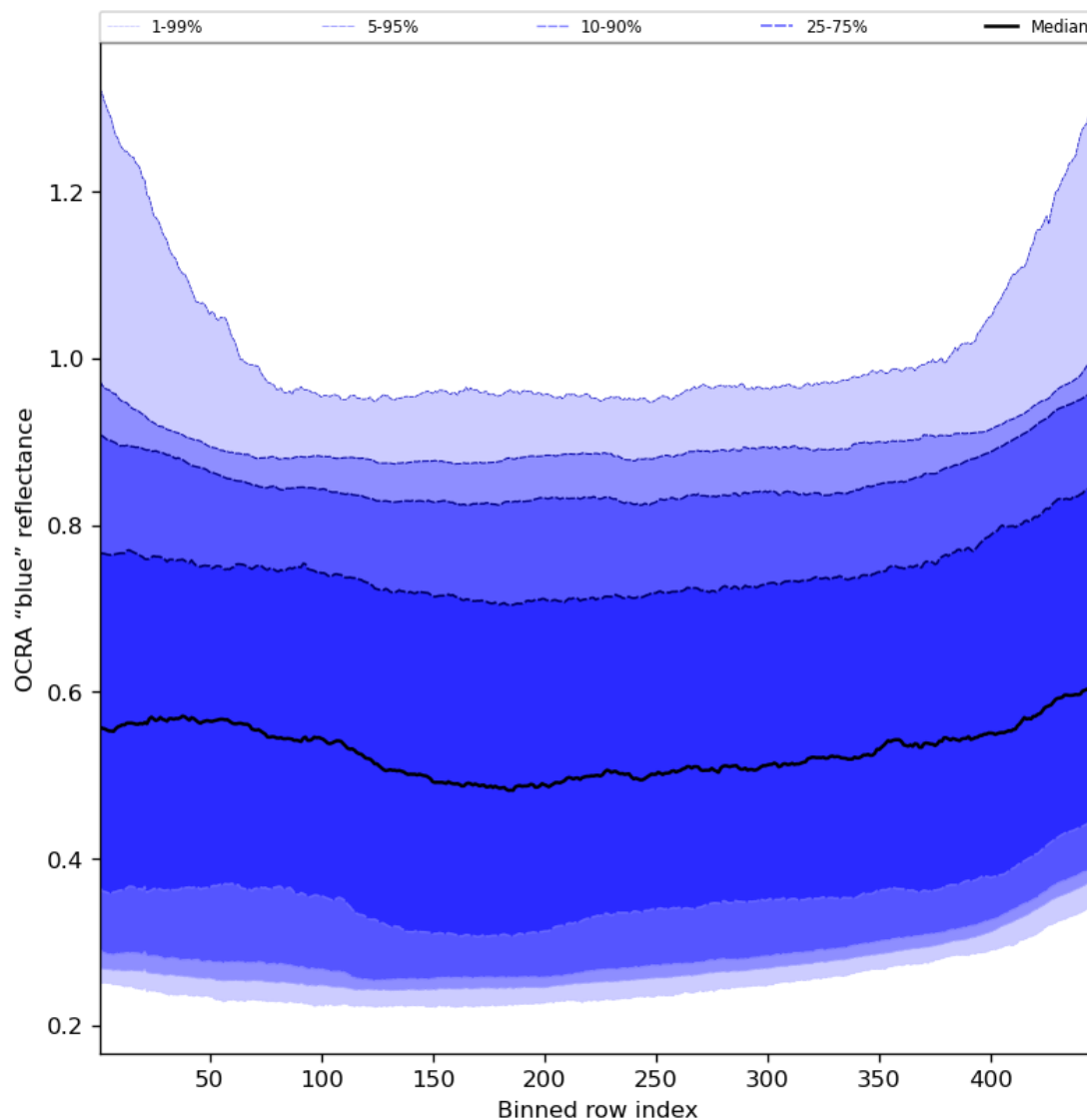
Figure 67: Along track statistics of “OCRA “blue” reflectance” for 2024-05-07 to 2024-05-08
