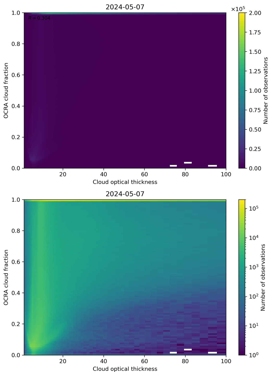
Figure 83: Scatter density plot of “Cloud optical thickness” against “OCRA cloud fraction” for 2024-05-07 to 2024-05-08.
