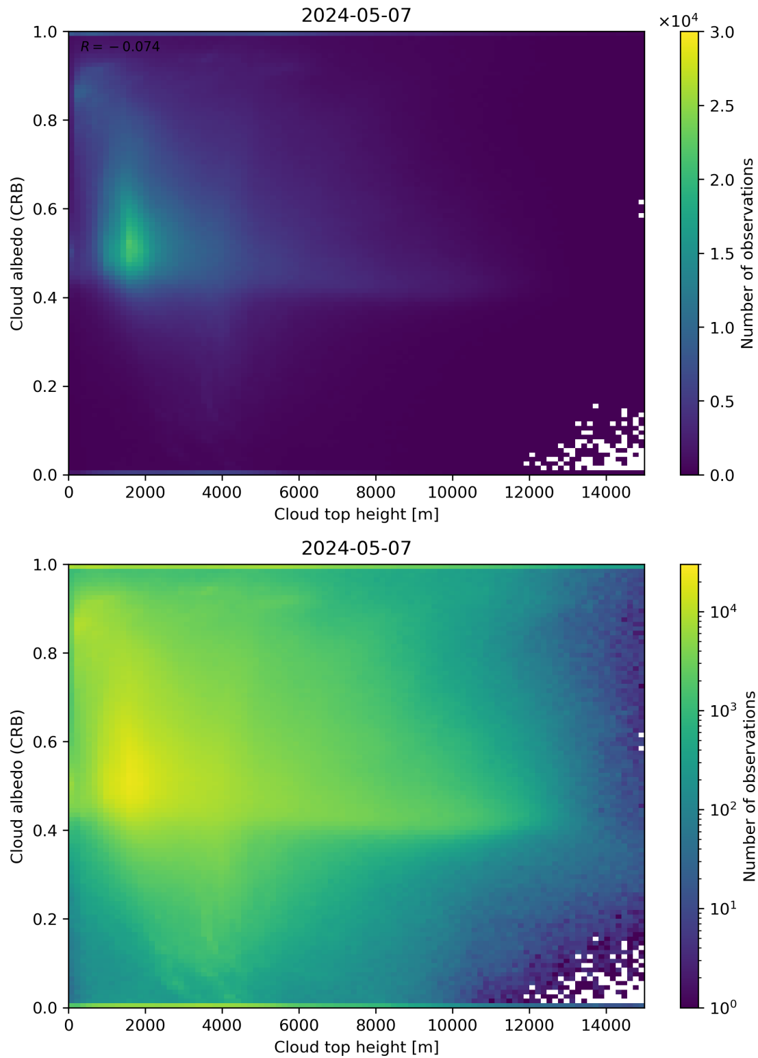
Figure 86: Scatter density plot of “Cloud top height” against “Cloud albedo (CRB)” for 2024-05-07 to 2024-05-08.
