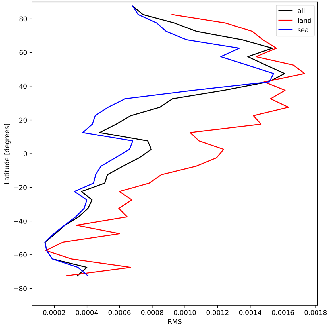
Figure 31: Zonal average of “RMS” for 2024-05-07 to 2024-05-08.
