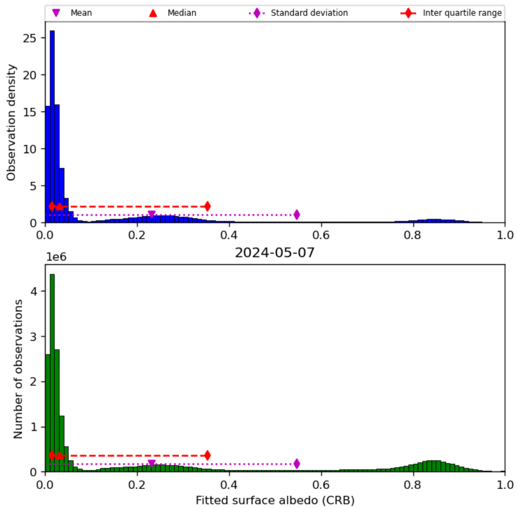
Figure 46: Histogram of “Fitted surface albedo (CRB)” for 2024-05-07 to 2024-05-08
