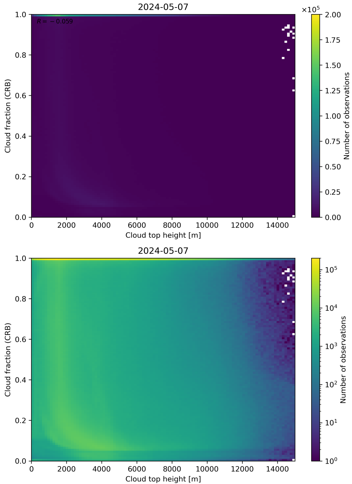
Figure 88: Scatter density plot of “Cloud top height” against “Cloud fraction (CRB)” for 2024-05-07 to 2024-05-08.
