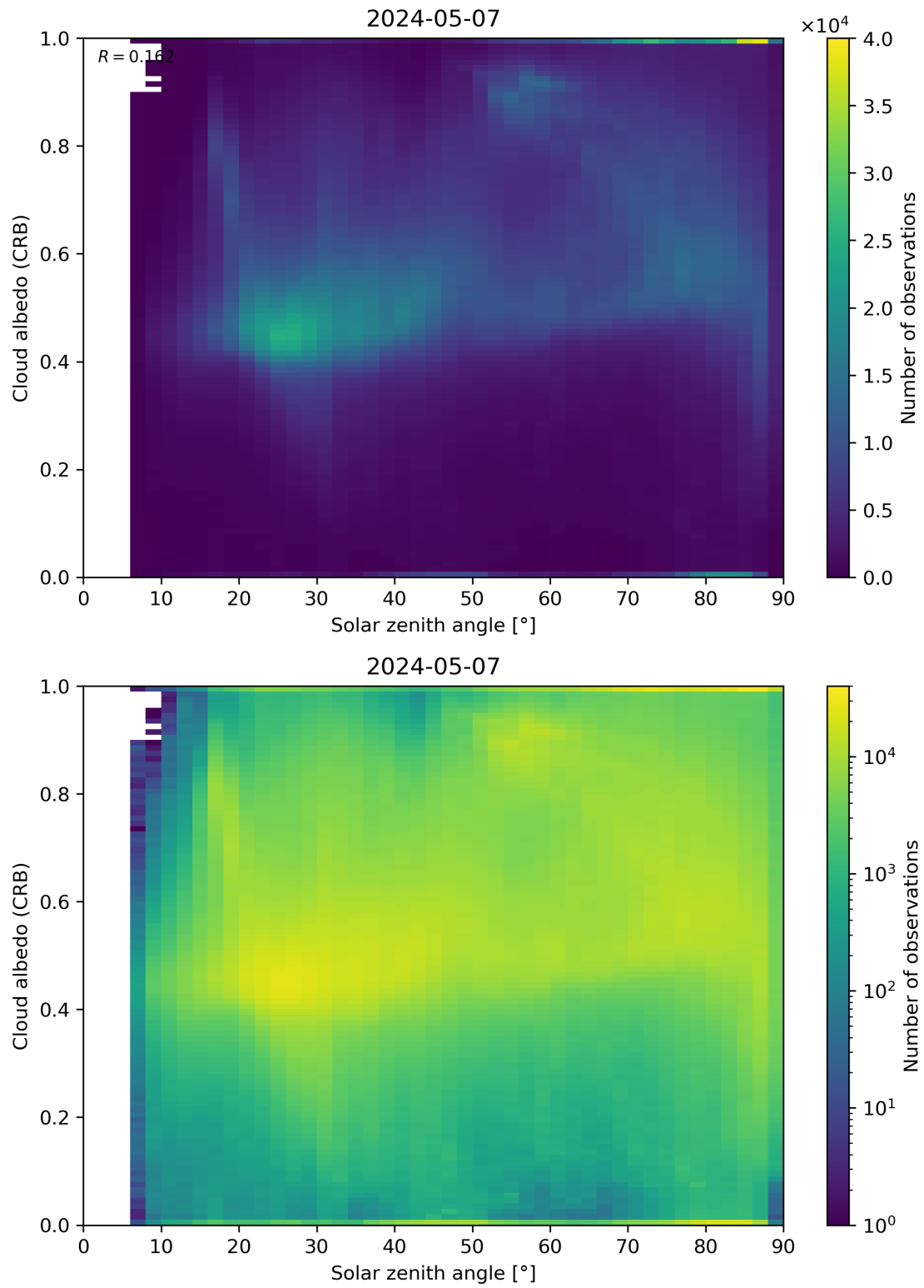
Figure 98: Scatter density plot of “Solar zenith angle” against “Cloud albedo (CRB)” for 2024-05-07 to 2024-05-08.
