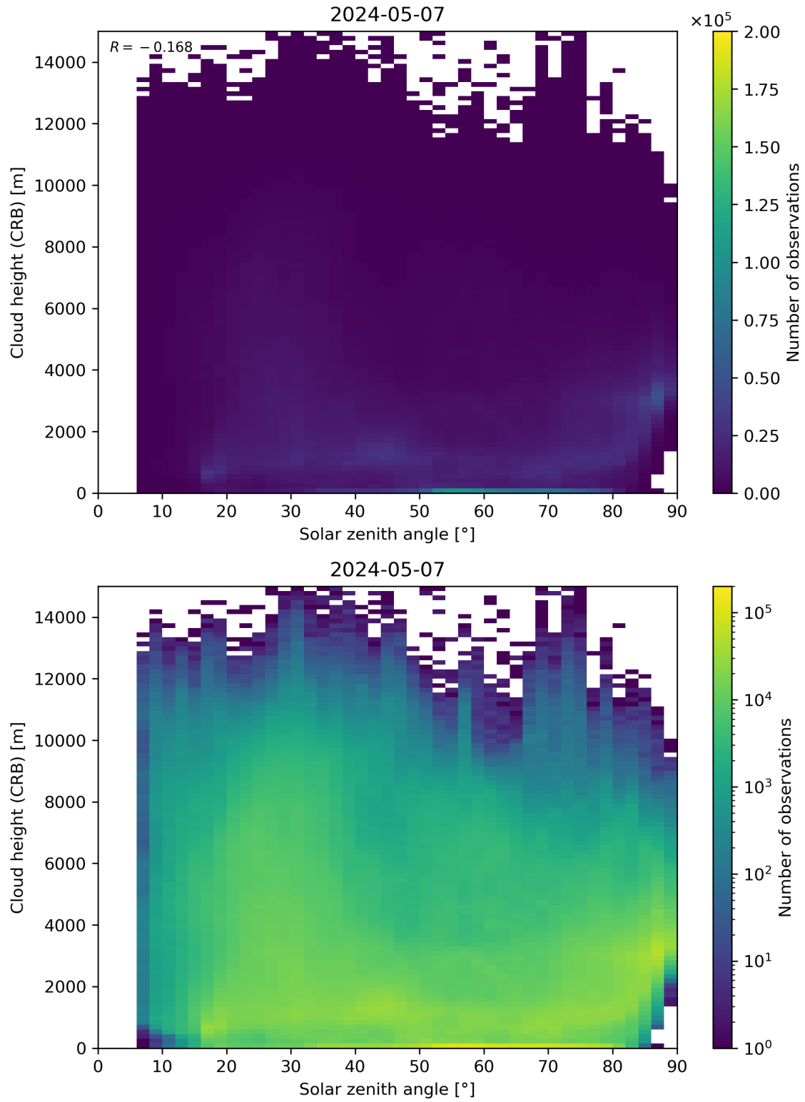
Figure 102: Scatter density plot of “Solar zenith angle” against “Cloud height (CRB)” for 2024-05-07 to 2024-05-08.
