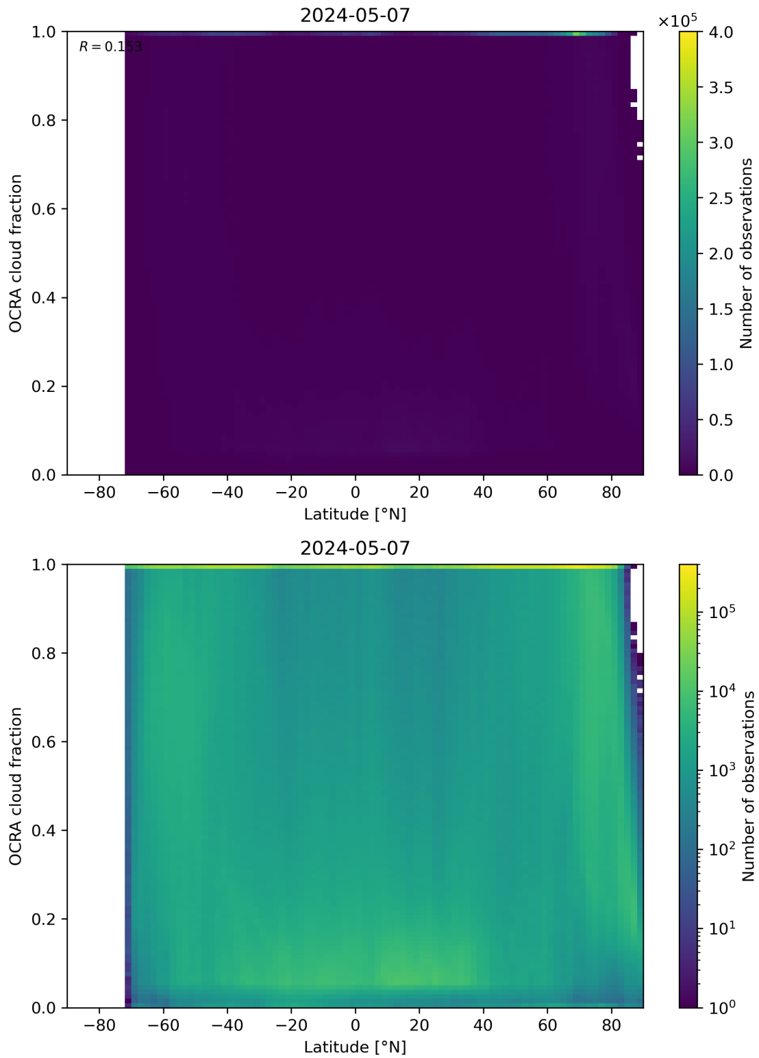
Figure 93: Scatter density plot of “Latitude” against “OCRA cloud fraction” for 2024-05-07 to 2024-05-08.
