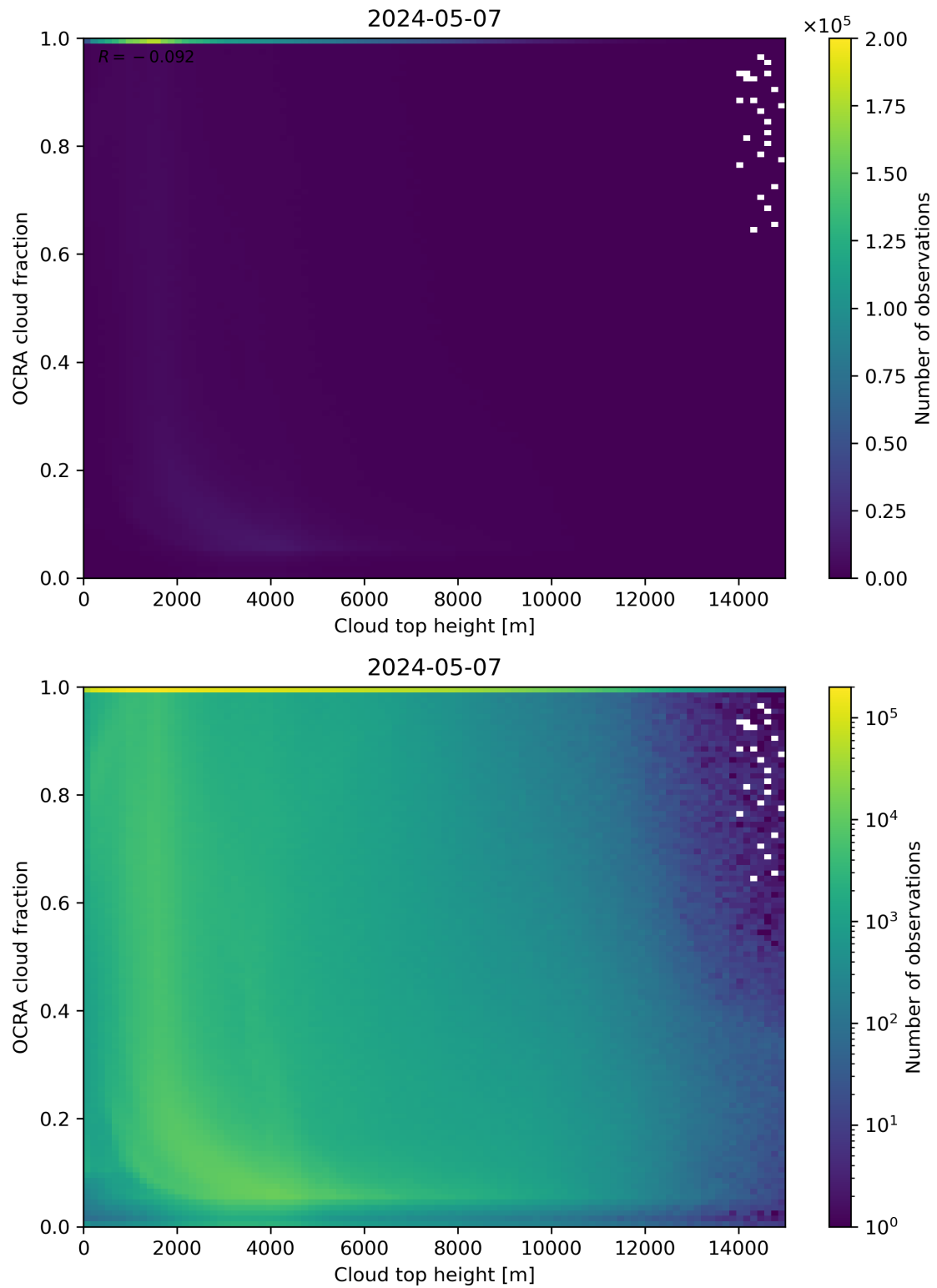
Figure 87: Scatter density plot of “Cloud top height” against “OCRA cloud fraction” for 2024-05-07 to 2024-05-08.
