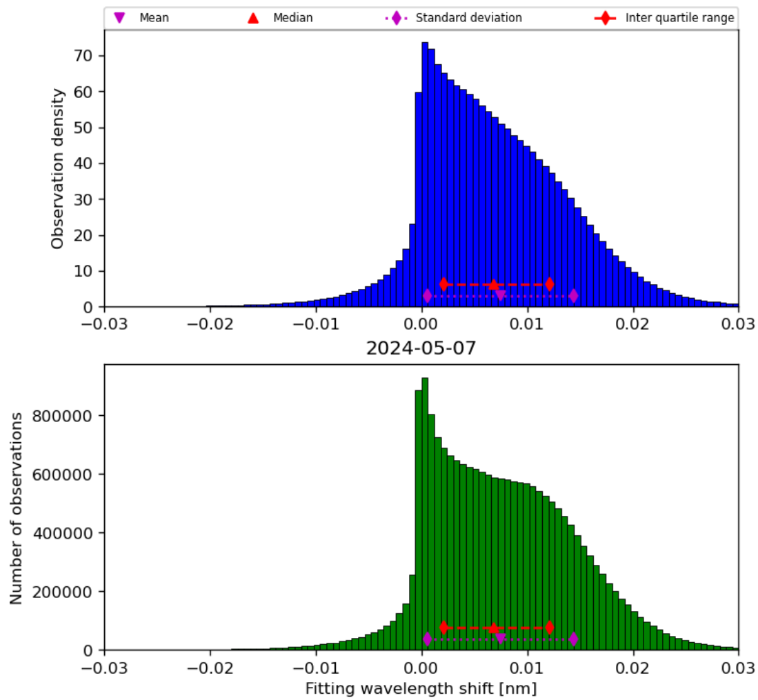
Figure 49: Histogram of “Fitting wavelength shift” for 2024-05-07 to 2024-05-08
