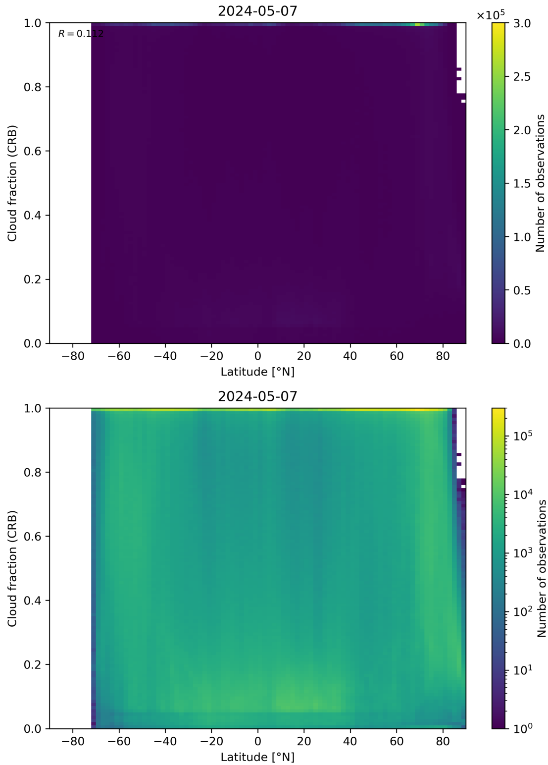
Figure 94: Scatter density plot of “Latitude” against “Cloud fraction (CRB)” for 2024-05-07 to 2024-05-08.
