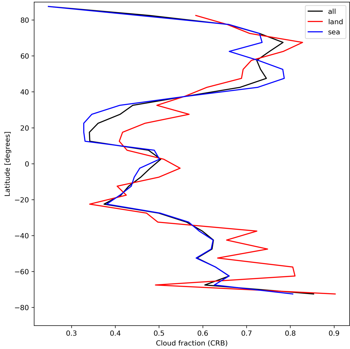
Figure 26: Zonal average of “Cloud fraction (CRB)” for 2024-05-07 to 2024-05-08.
