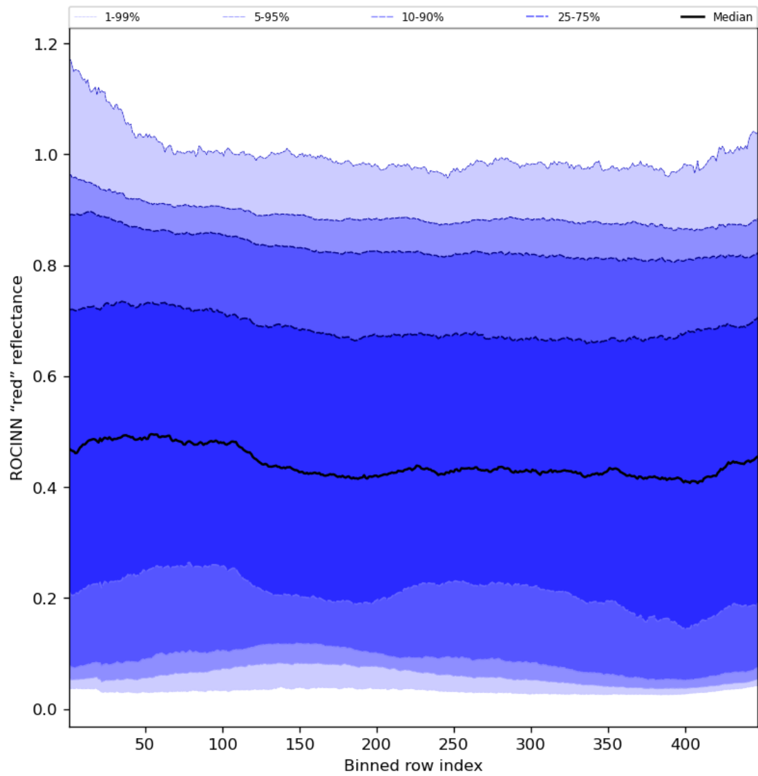
Figure 69: Along track statistics of “ROCINN “red” reflectance” for 2024-05-07 to 2024-05-08
