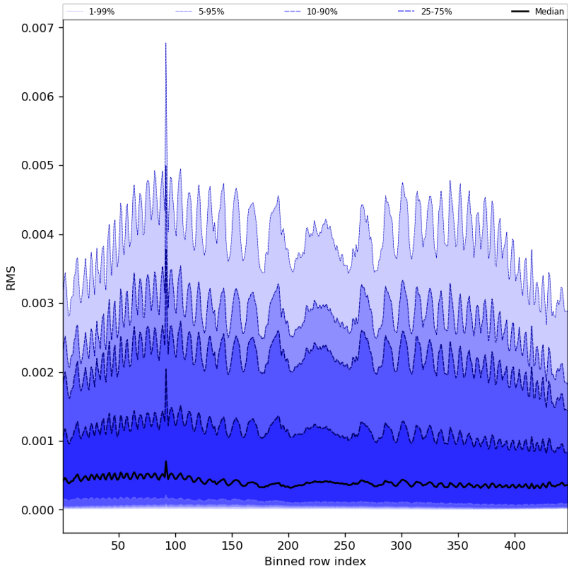
Figure 63: Along track statistics of “RMS” for 2024-05-07 to 2024-05-08
