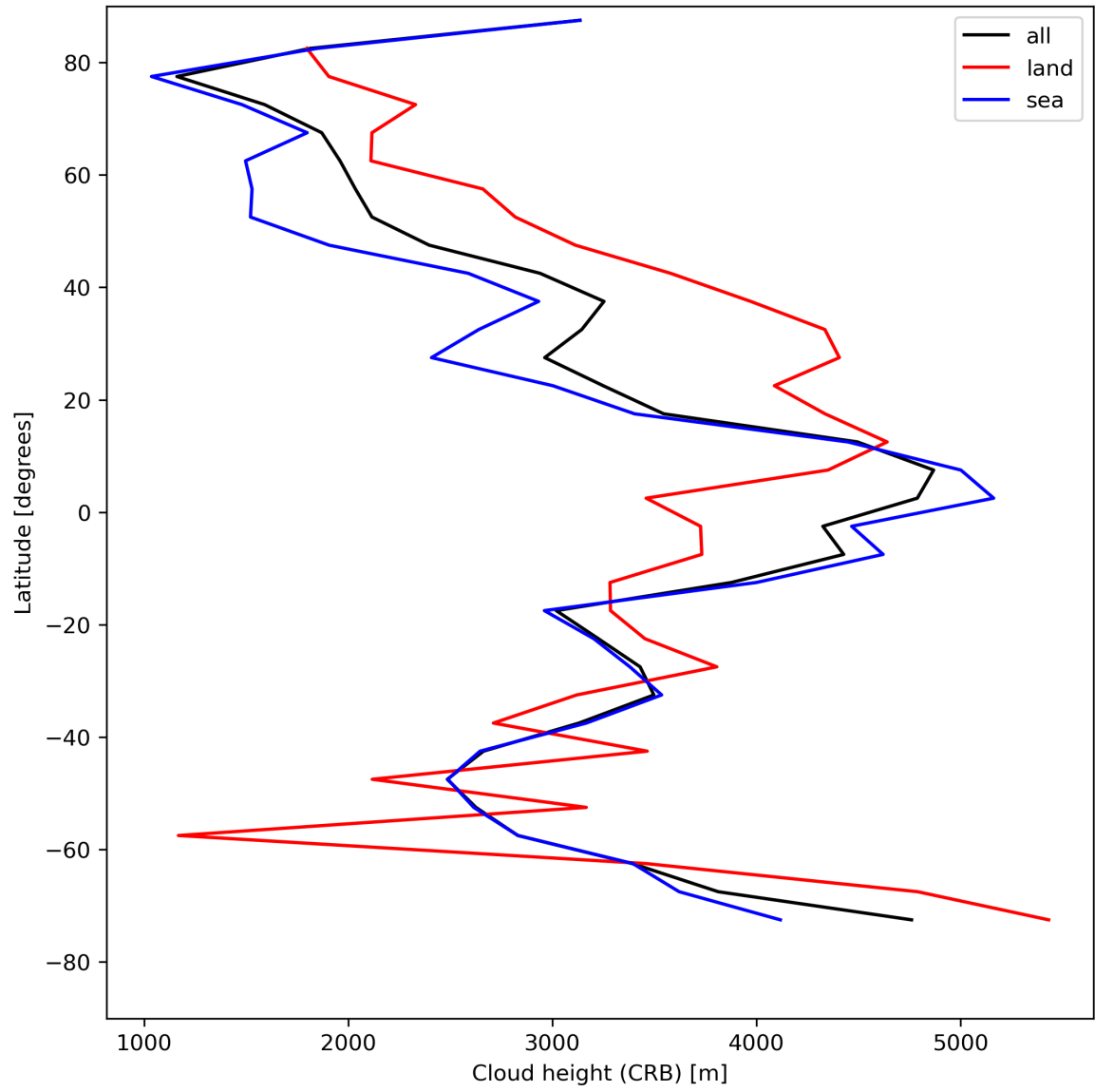
Figure 27: Zonal average of “Cloud height (CRB)” for 2024-05-07 to 2024-05-08.
