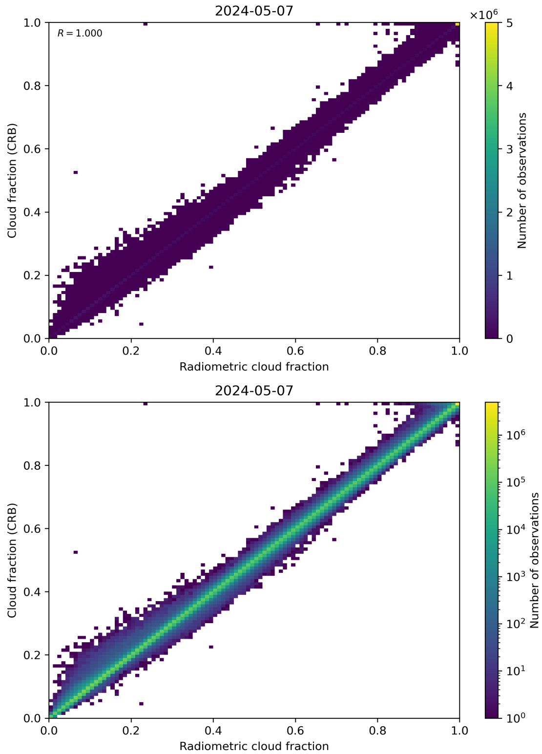
Figure 73: Scatter density plot of “Radiometric cloud fraction” against “Cloud fraction (CRB)” for 2024-05-07 to 2024-05-08.
