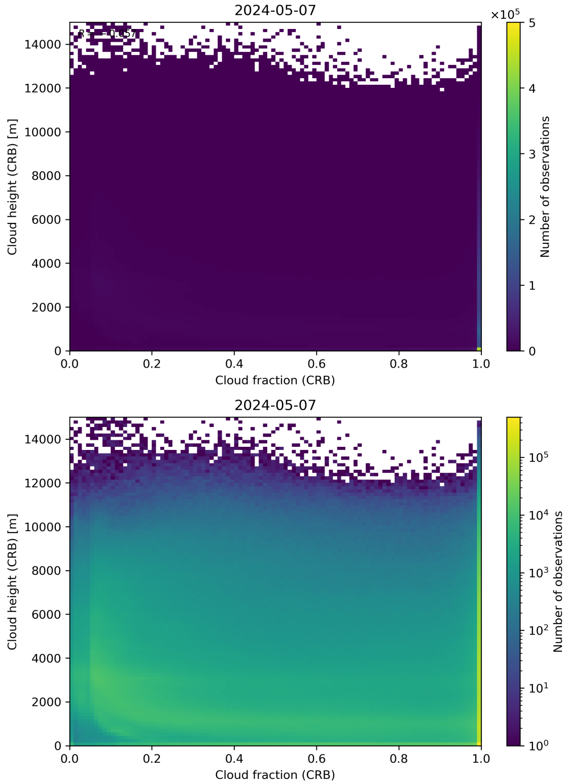
Figure 79: Scatter density plot of “Cloud fraction (CRB)” against “Cloud height (CRB)” for 2024-05-07 to 2024-05-08.
