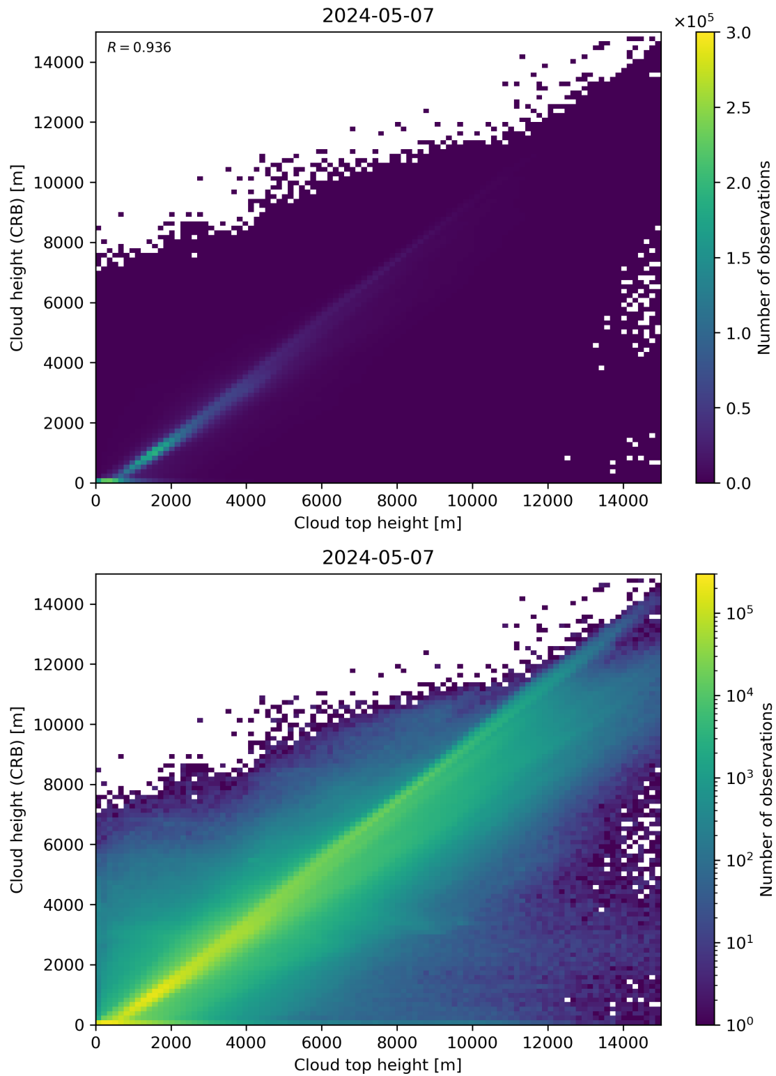
Figure 89: Scatter density plot of “Cloud top height” against “Cloud height (CRB)” for 2024-05-07 to 2024-05-08.
