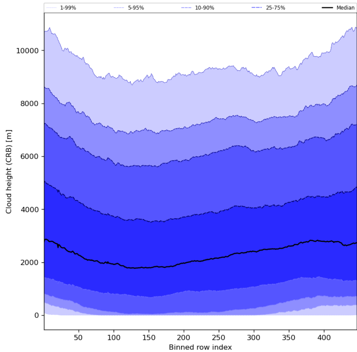
Figure 59: Along track statistics of “Cloud height (CRB)” for 2024-05-07 to 2024-05-08
