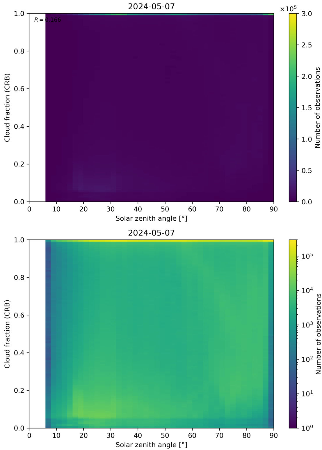
Figure 101: Scatter density plot of “Solar zenith angle” against “Cloud fraction (CRB)” for 2024-05-07 to 2024-05-08.
