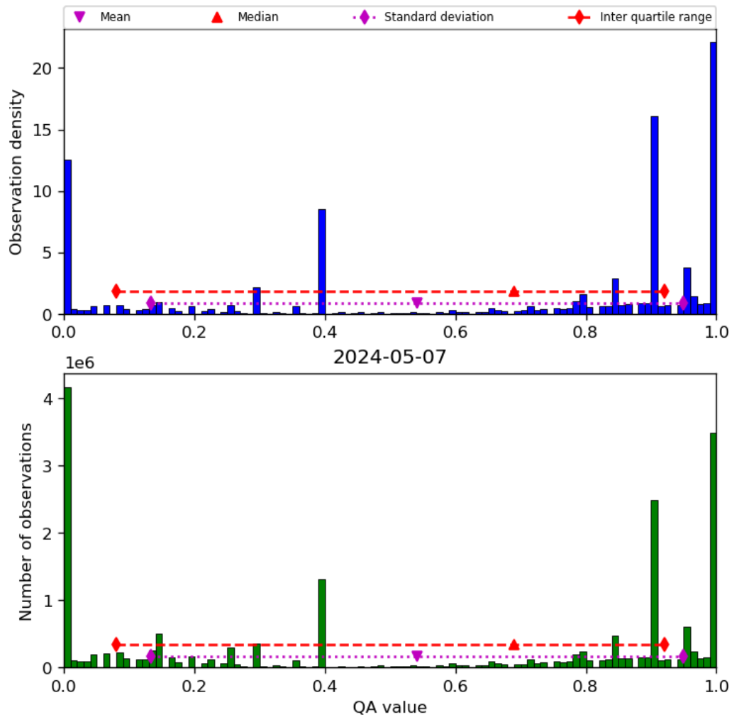
Figure 38: Histogram of “QA value” for 2024-05-07 to 2024-05-08
