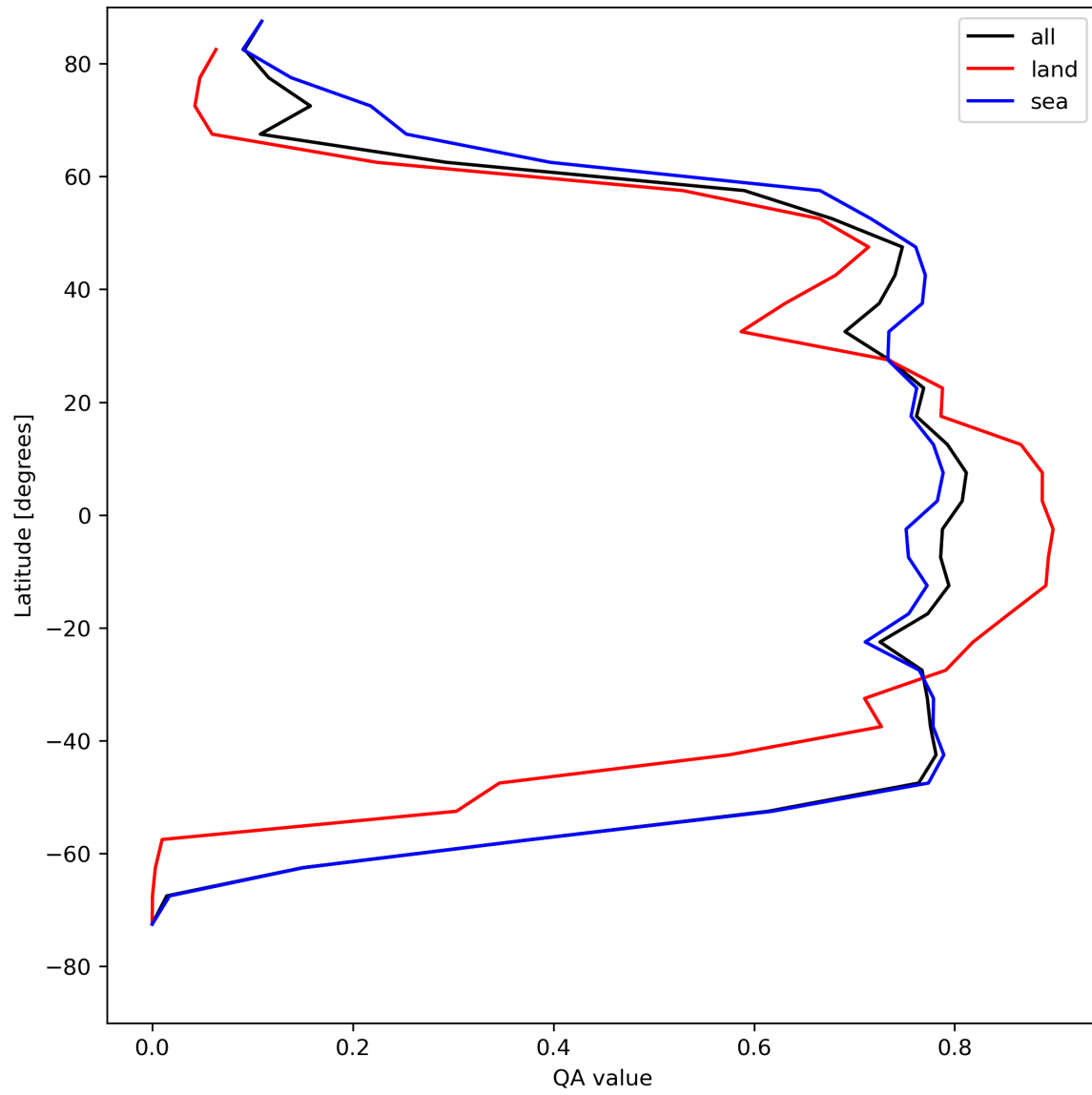
Figure 22: Zonal average of “QA value” for 2024-05-07 to 2024-05-08.
