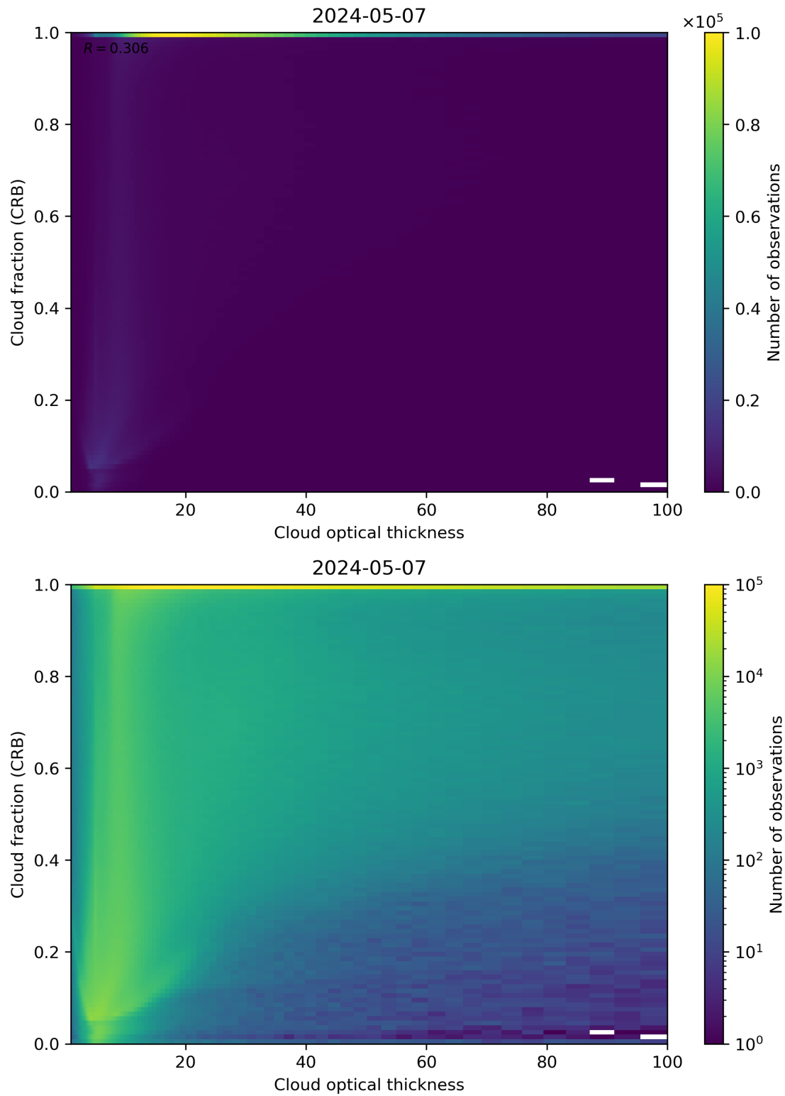
Figure 84: Scatter density plot of “Cloud optical thickness” against “Cloud fraction (CRB)” for 2024-05-07 to 2024-05-08.
