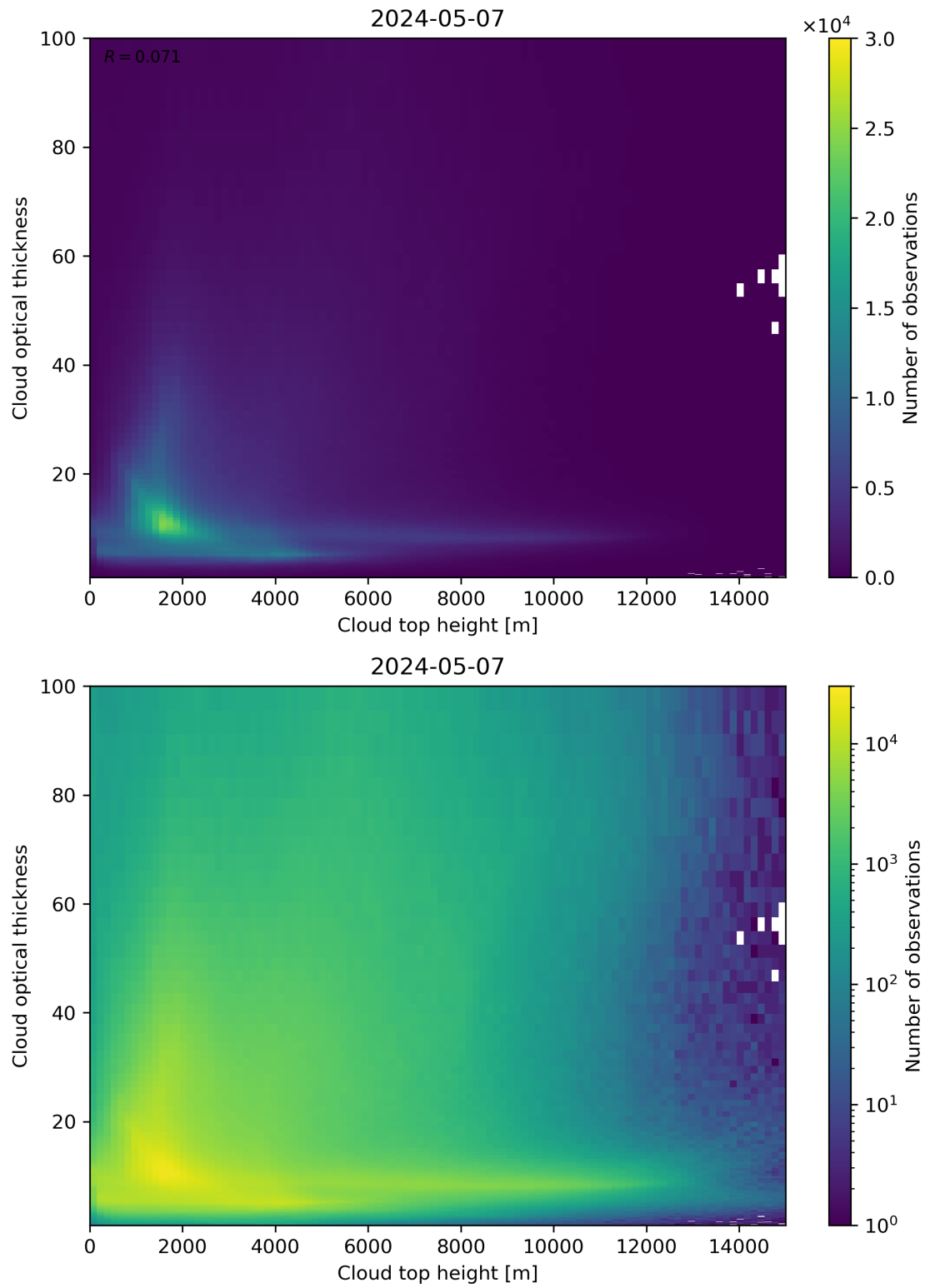
Figure 90: Scatter density plot of “Cloud top height” against “Cloud optical thickness” for 2024-05-07 to 2024-05-08.
