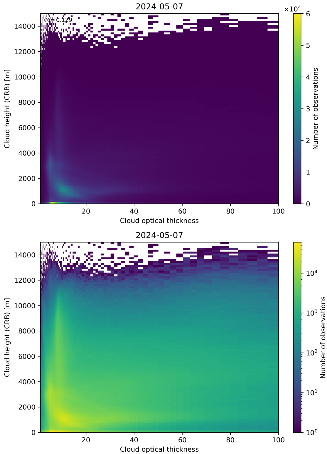
Figure 85: Scatter density plot of “Cloud optical thickness” against “Cloud height (CRB)” for 2024-05-07 to 2024-05-08.
