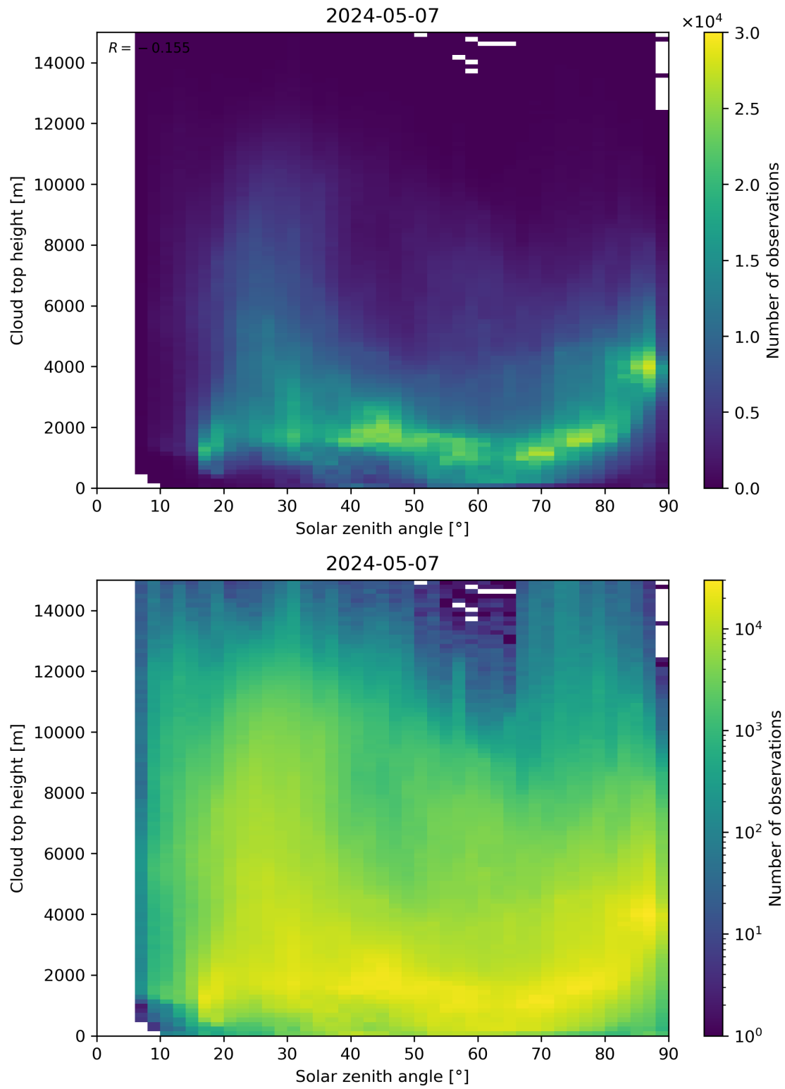
Figure 104: Scatter density plot of “Solar zenith angle” against “Cloud top height” for 2024-05-07 to 2024-05-08.
