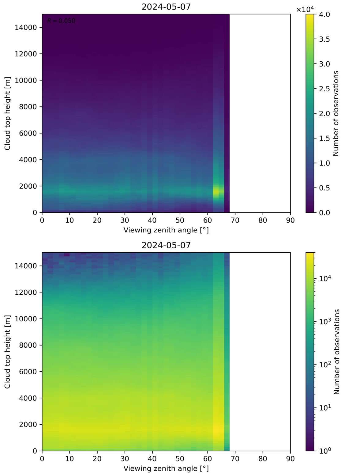
Figure 112: Scatter density plot of “Viewing zenith angle” against “Cloud top height” for 2024-05-07 to 2024-05-08.
