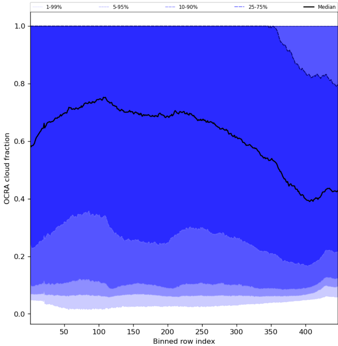
Figure 66: Along track statistics of “OCRA cloud fraction” for 2024-05-07 to 2024-05-08
