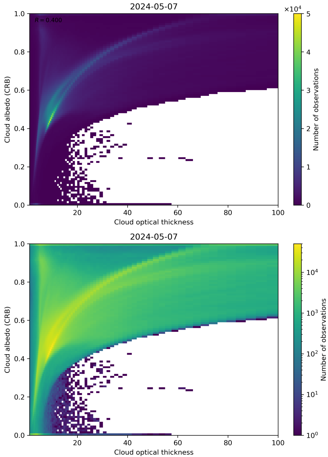
Figure 82: Scatter density plot of “Cloud optical thickness” against “Cloud albedo (CRB)” for 2024-05-07 to 2024-05-08.
