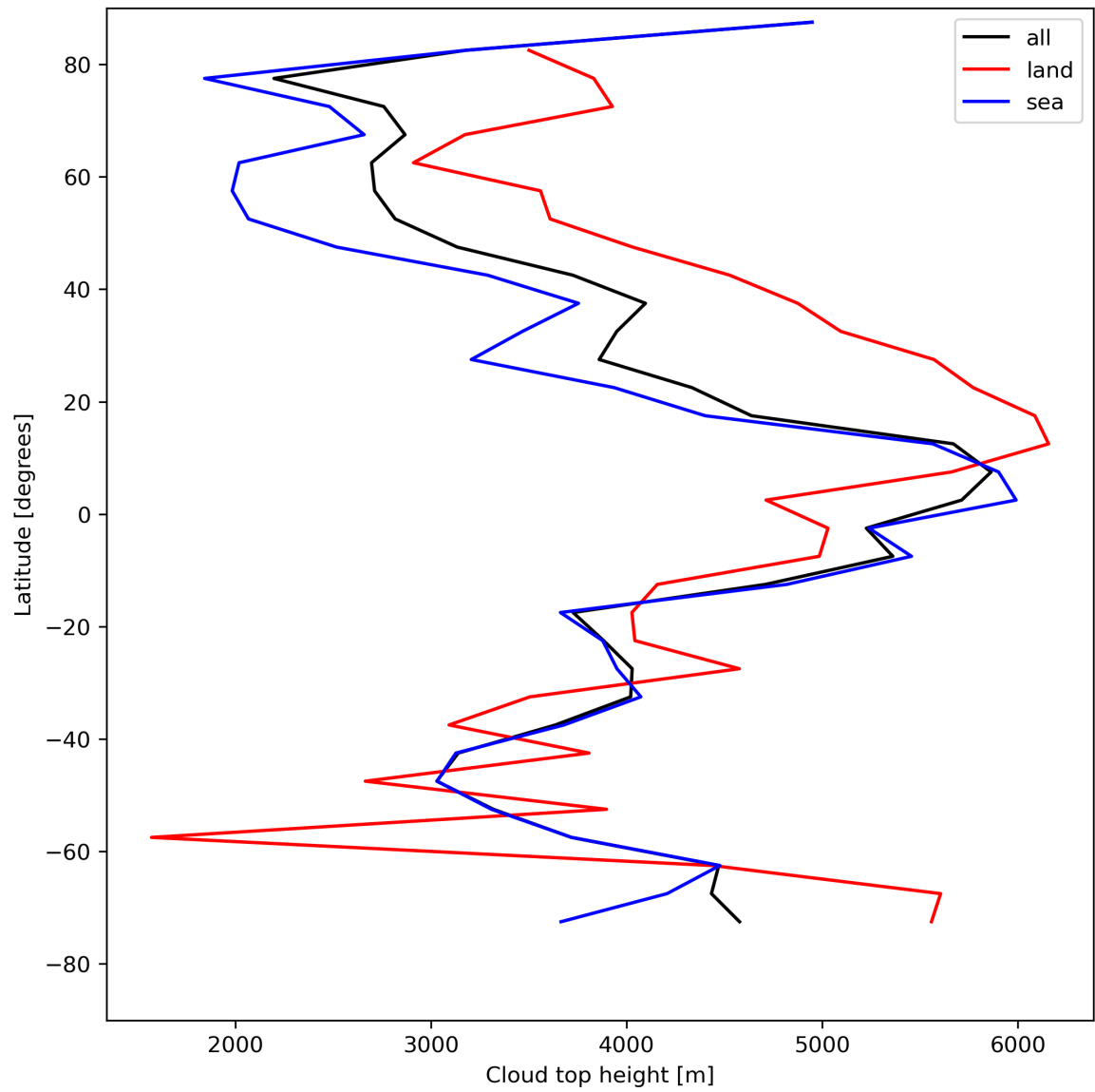
Figure 24: Zonal average of “Cloud top height” for 2024-05-07 to 2024-05-08.
