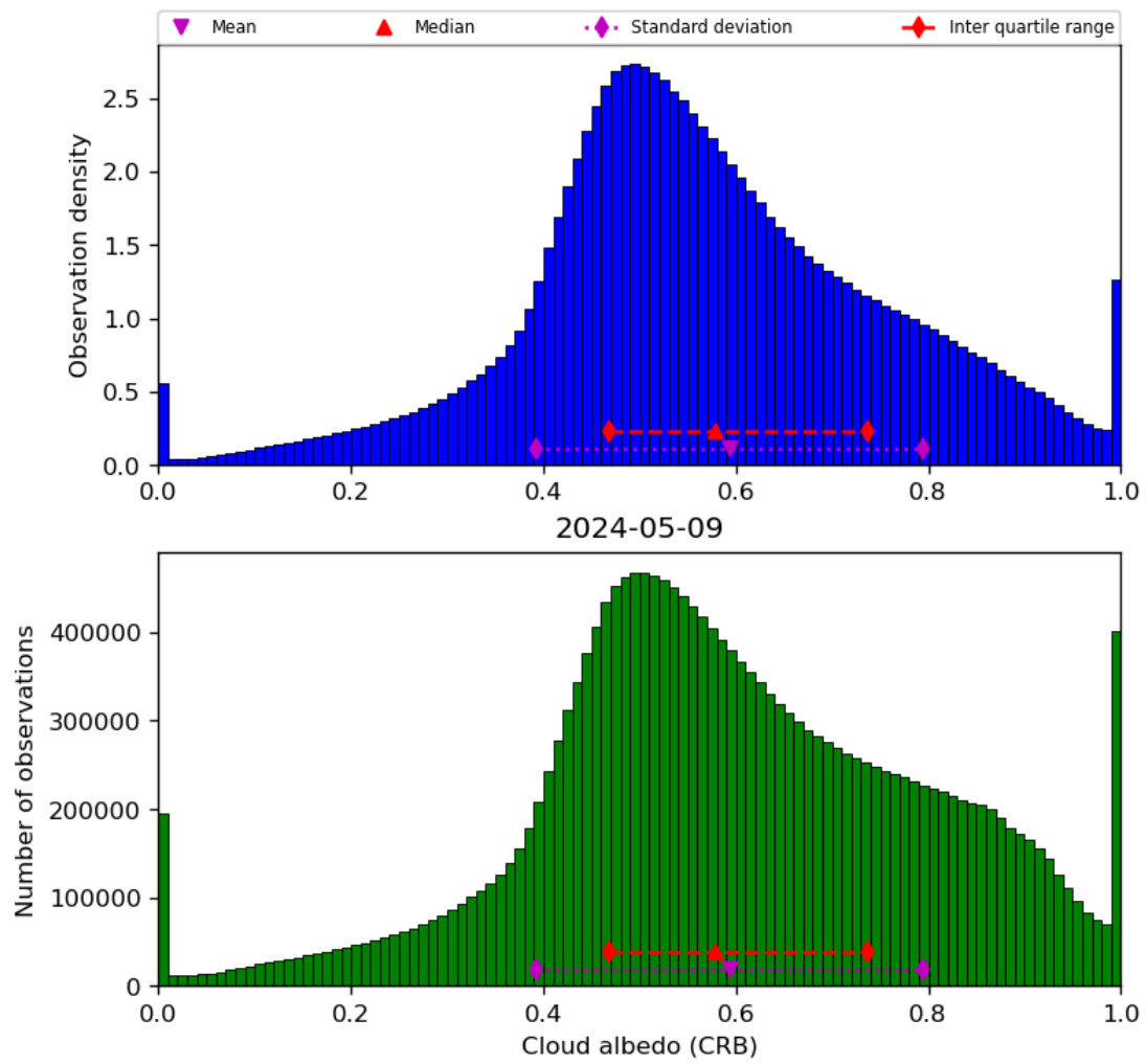
Figure 44: Histogram of “Cloud albedo (CRB)” for 2024-05-08 to 2024-05-10
