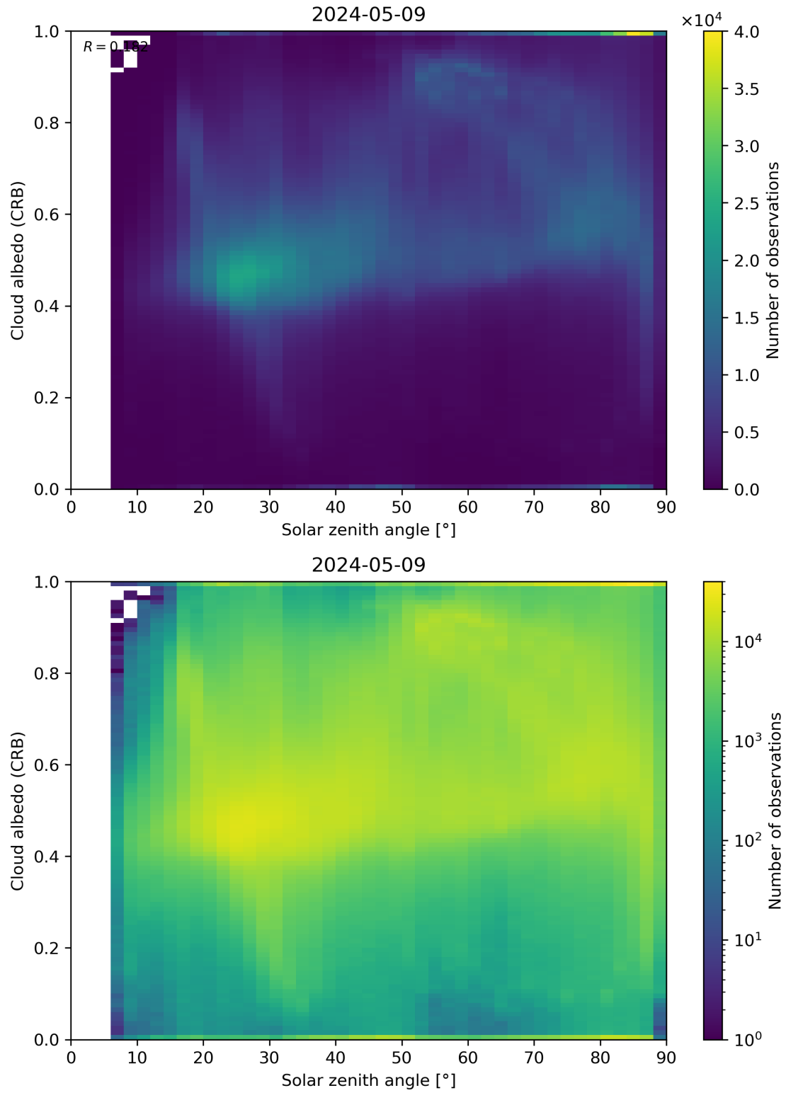
Figure 98: Scatter density plot of “Solar zenith angle” against “Cloud albedo (CRB)” for 2024-05-08 to 2024-05-10.
