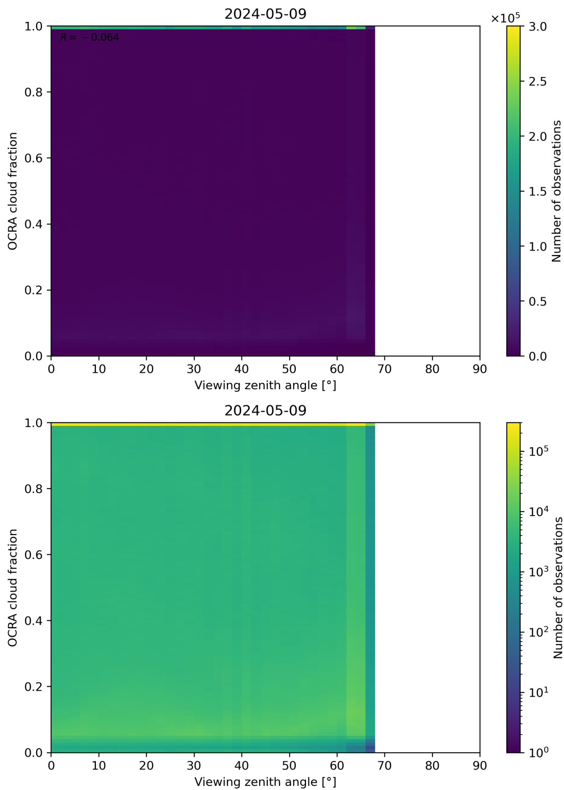
Figure 108: Scatter density plot of “Viewing zenith angle” against “OCRA cloud fraction” for 2024-05-08 to 2024-05-10.
