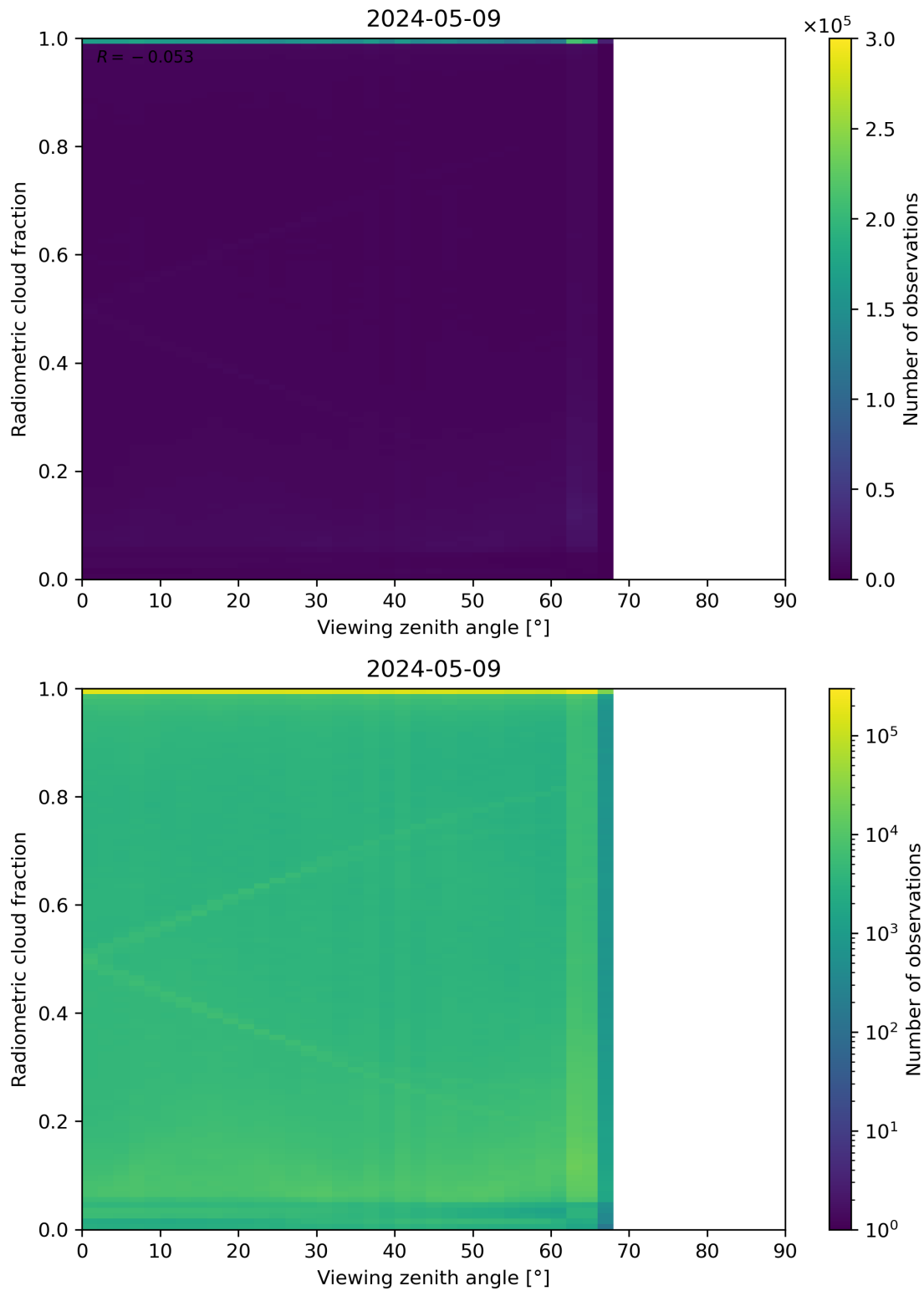
Figure 107: Scatter density plot of “Viewing zenith angle” against “Radiometric cloud fraction” for 2024-05-08 to 2024-05-10.
