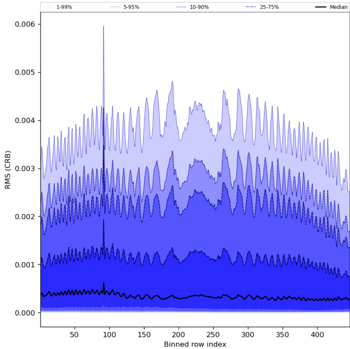
Figure 64: Along track statistics of “RMS (CRB)” for 2024-05-08 to 2024-05-10
