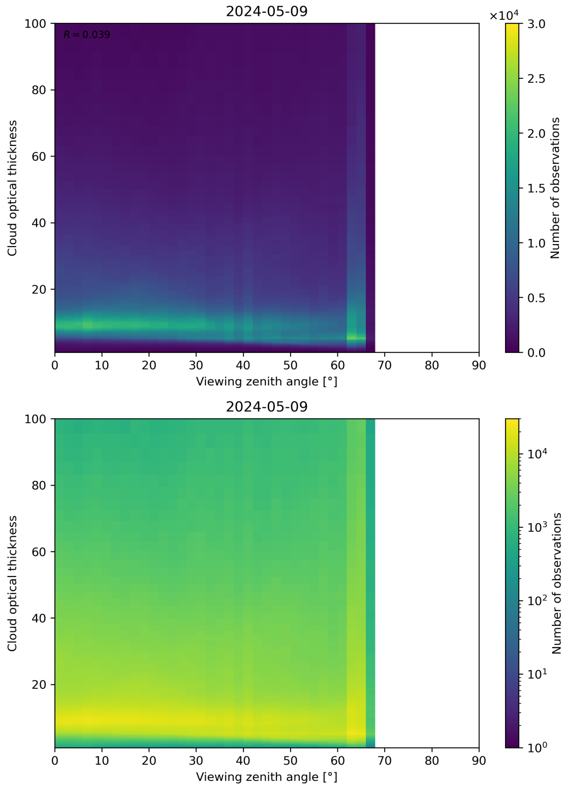
Figure 111: Scatter density plot of “Viewing zenith angle” against “Cloud optical thickness” for 2024-05-08 to 2024-05-10.
