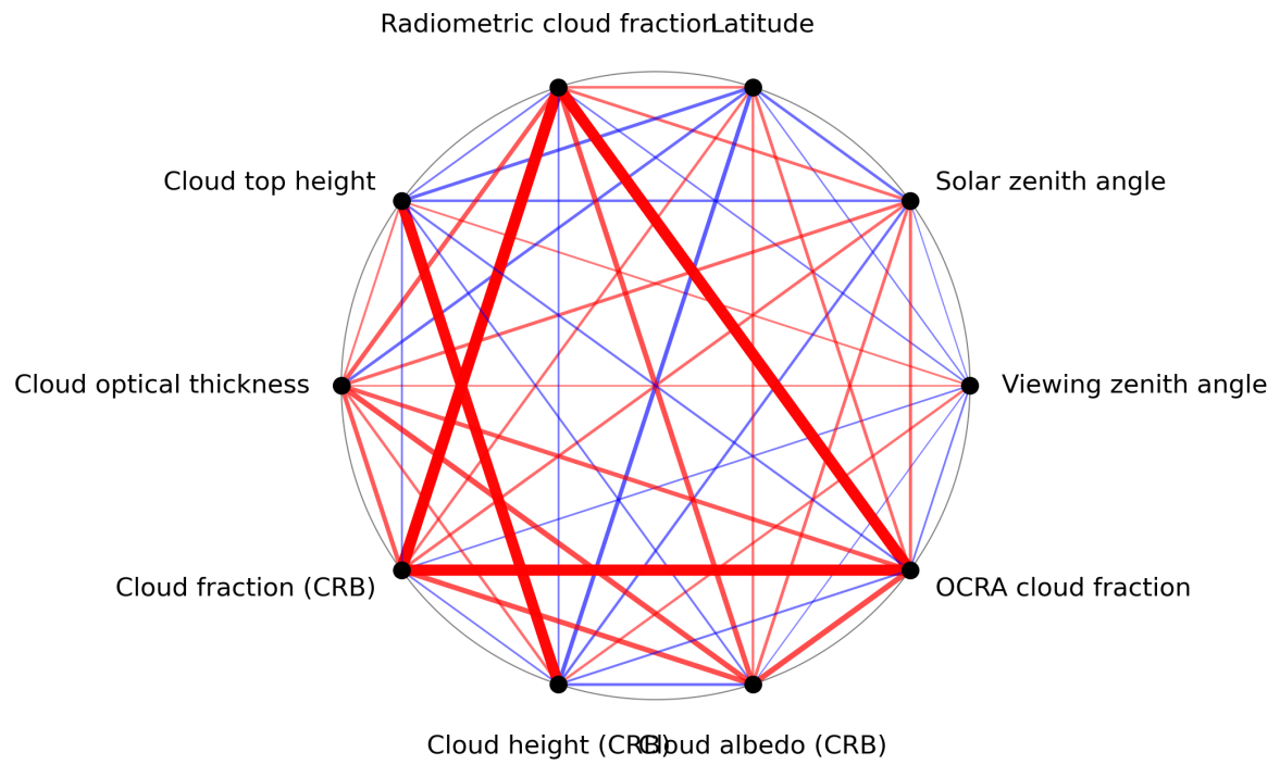
Figure 1: Map of correlation graph for 2024-05-08 to 2024-05-10.
