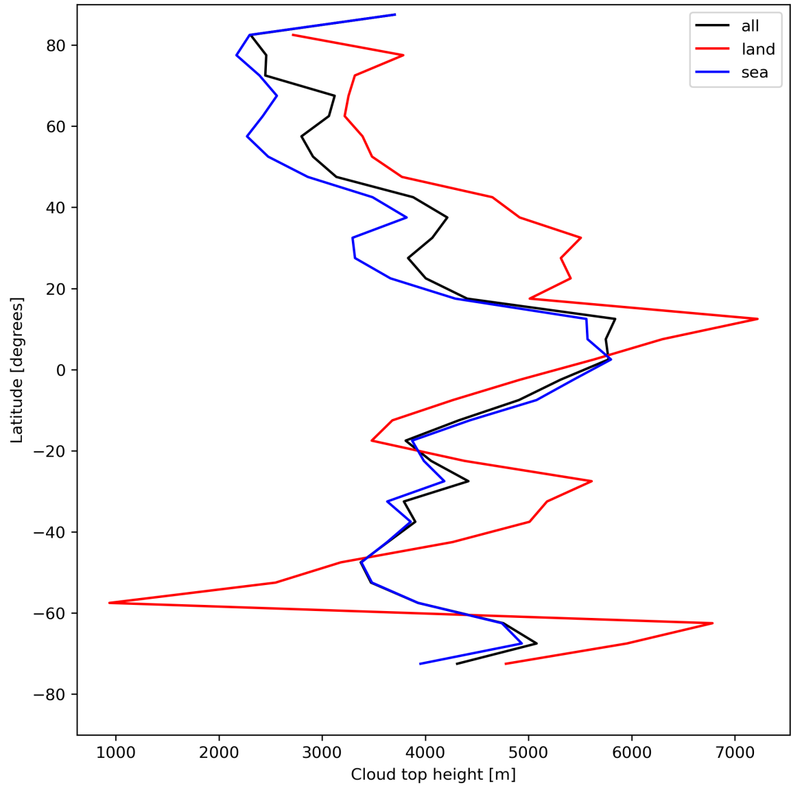
Figure 24: Zonal average of “Cloud top height” for 2024-05-08 to 2024-05-10.
