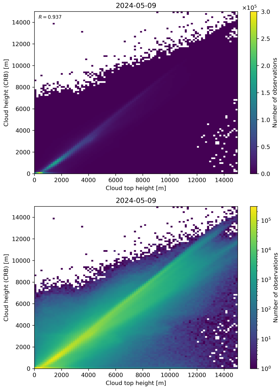
Figure 89: Scatter density plot of “Cloud top height” against “Cloud height (CRB)” for 2024-05-08 to 2024-05-10.
