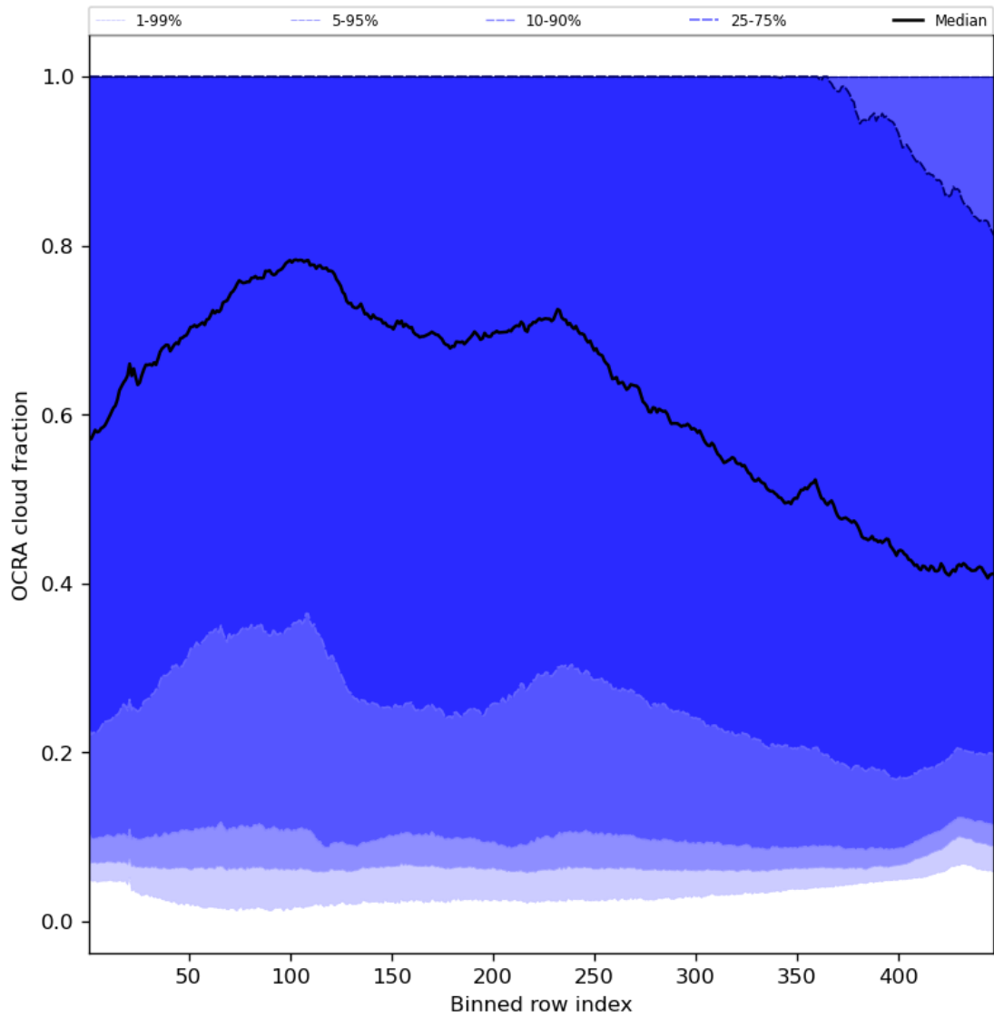
Figure 66: Along track statistics of “OCRA cloud fraction” for 2024-05-08 to 2024-05-10
