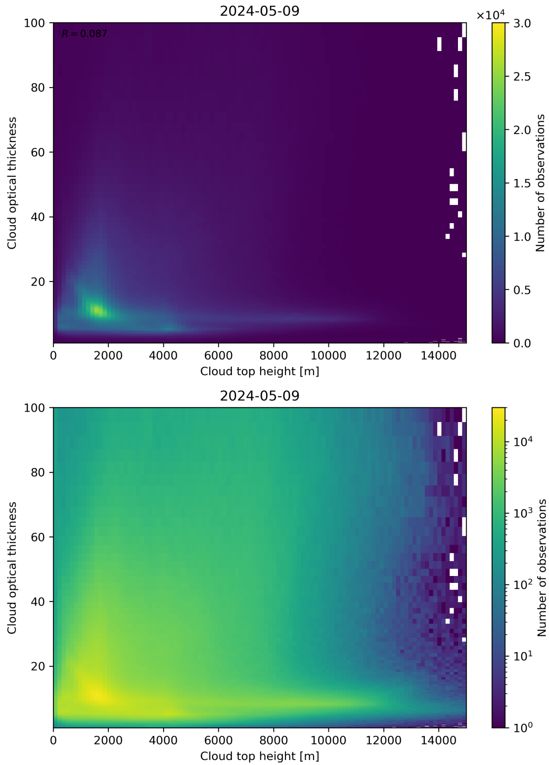
Figure 90: Scatter density plot of “Cloud top height” against “Cloud optical thickness” for 2024-05-08 to 2024-05-10.
