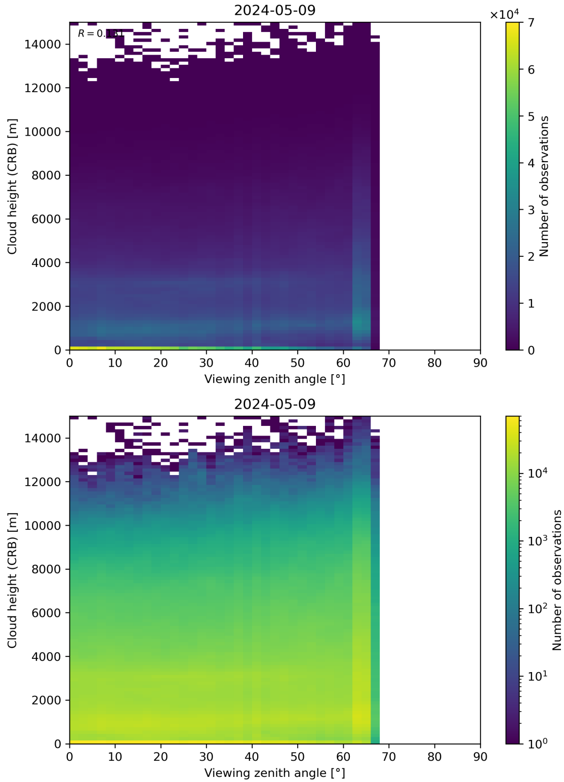
Figure 110: Scatter density plot of “Viewing zenith angle” against “Cloud height (CRB)” for 2024-05-08 to 2024-05-10.
