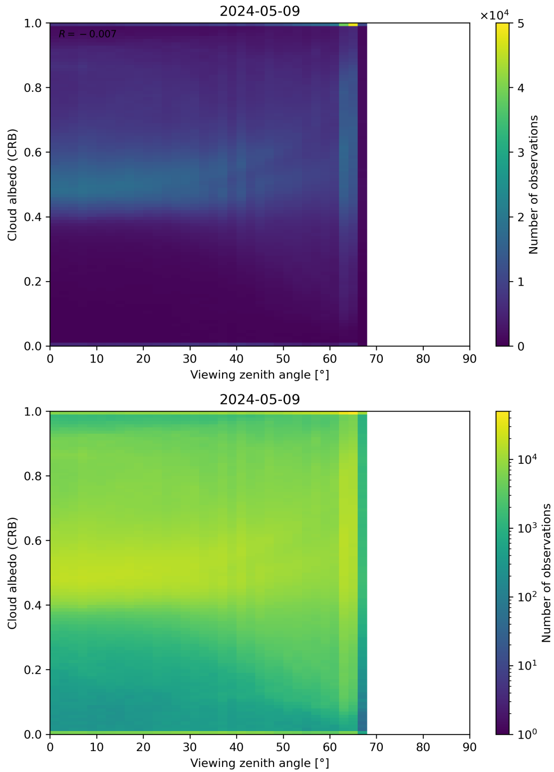
Figure 106: Scatter density plot of “Viewing zenith angle” against “Cloud albedo (CRB)” for 2024-05-08 to 2024-05-10.
