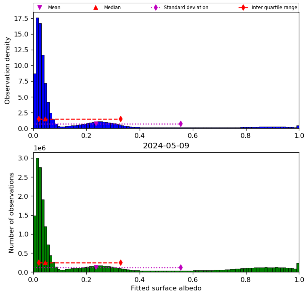
Figure 45: Histogram of “Fitted surface albedo” for 2024-05-08 to 2024-05-10
