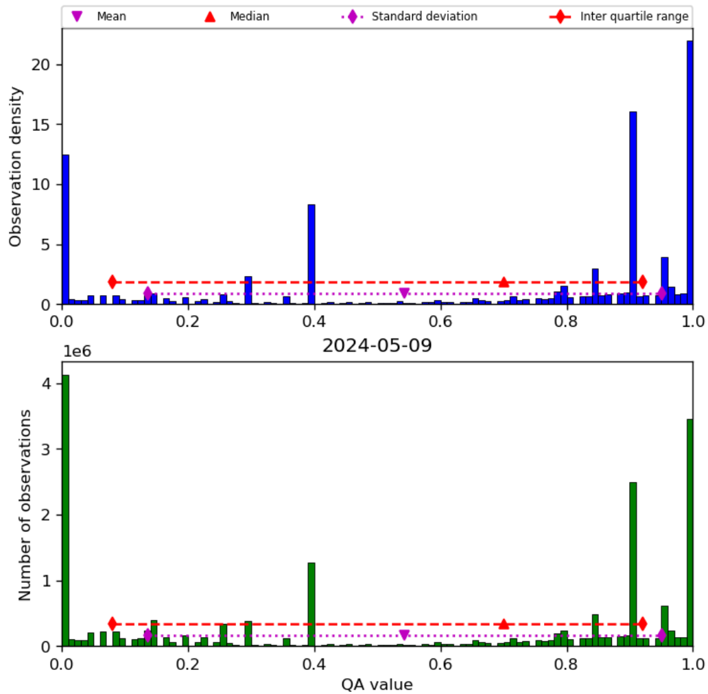
Figure 38: Histogram of “QA value” for 2024-05-08 to 2024-05-10
