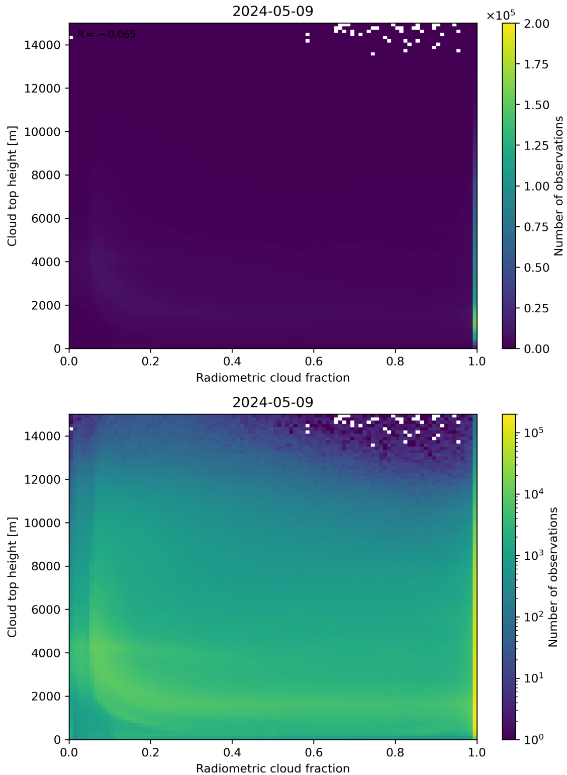
Figure 76: Scatter density plot of “Radiometric cloud fraction” against “Cloud top height” for 2024-05-08 to 2024-05-10.
