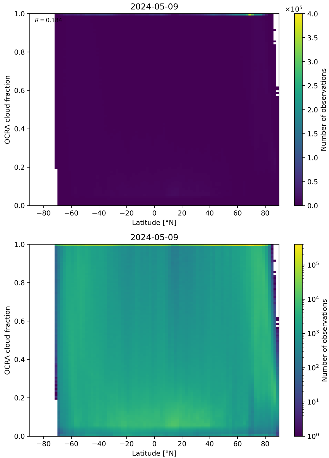
Figure 93: Scatter density plot of “Latitude” against “OCRA cloud fraction” for 2024-05-08 to 2024-05-10.
