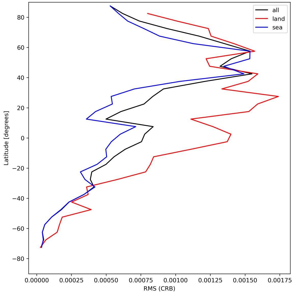
Figure 32: Zonal average of “RMS (CRB)” for 2024-05-08 to 2024-05-10.
