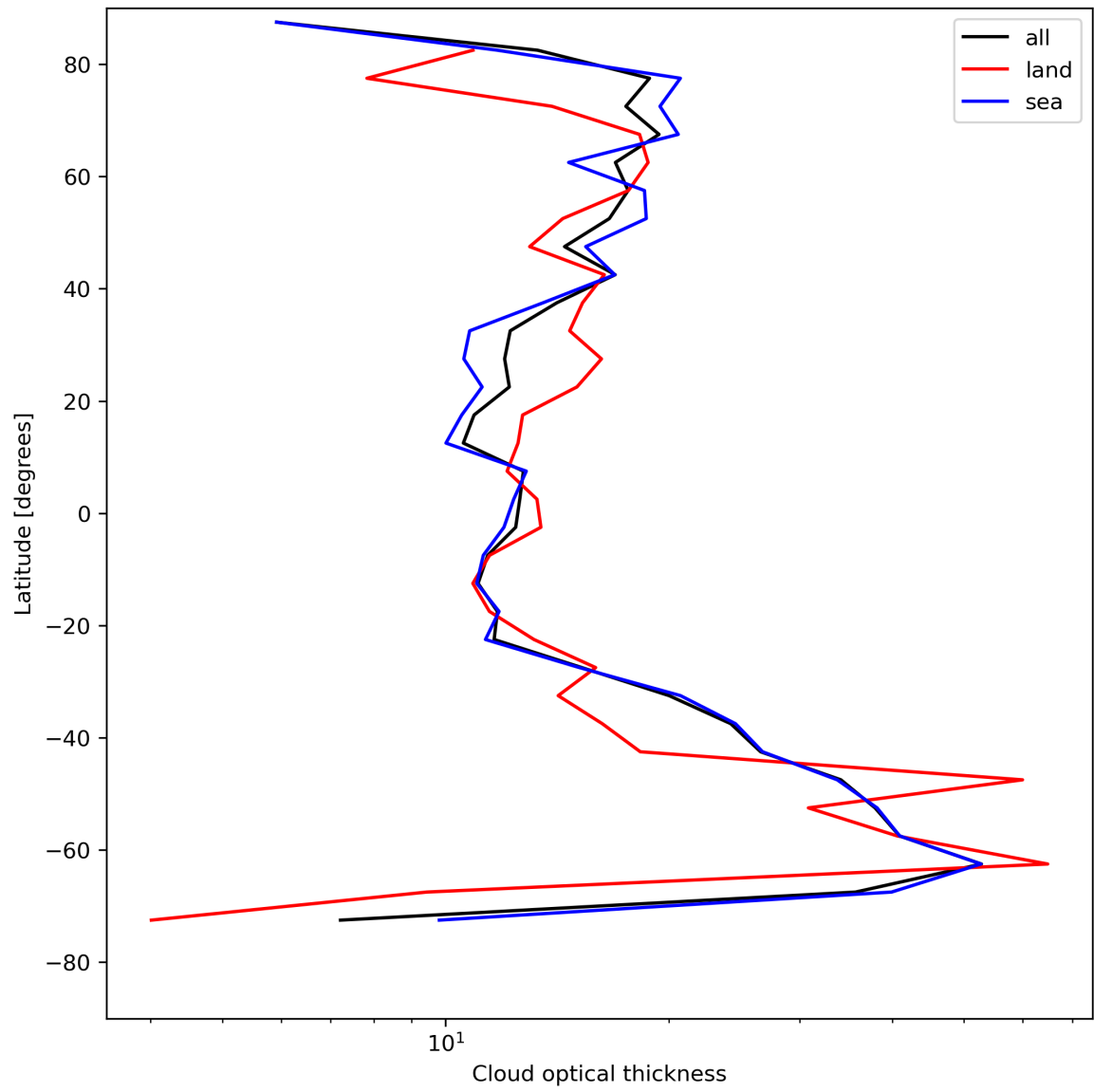
Figure 25: Zonal average of “Cloud optical thickness” for 2024-05-08 to 2024-05-10.
