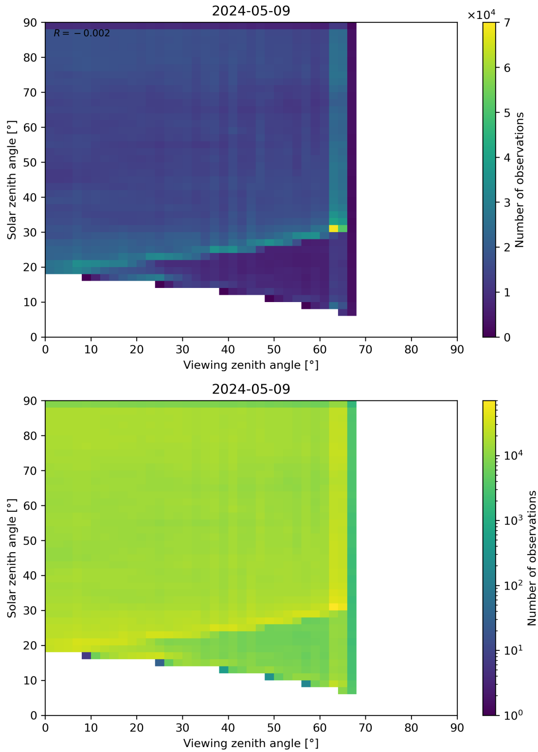
Figure 114: Scatter density plot of “Viewing zenith angle” against “Solar zenith angle” for 2024-05-08 to 2024-05-10.
