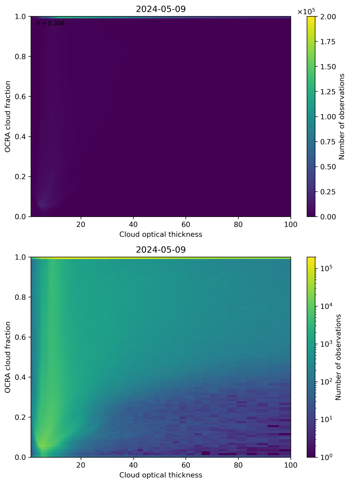
Figure 83: Scatter density plot of “Cloud optical thickness” against “OCRA cloud fraction” for 2024-05-08 to 2024-05-10.
