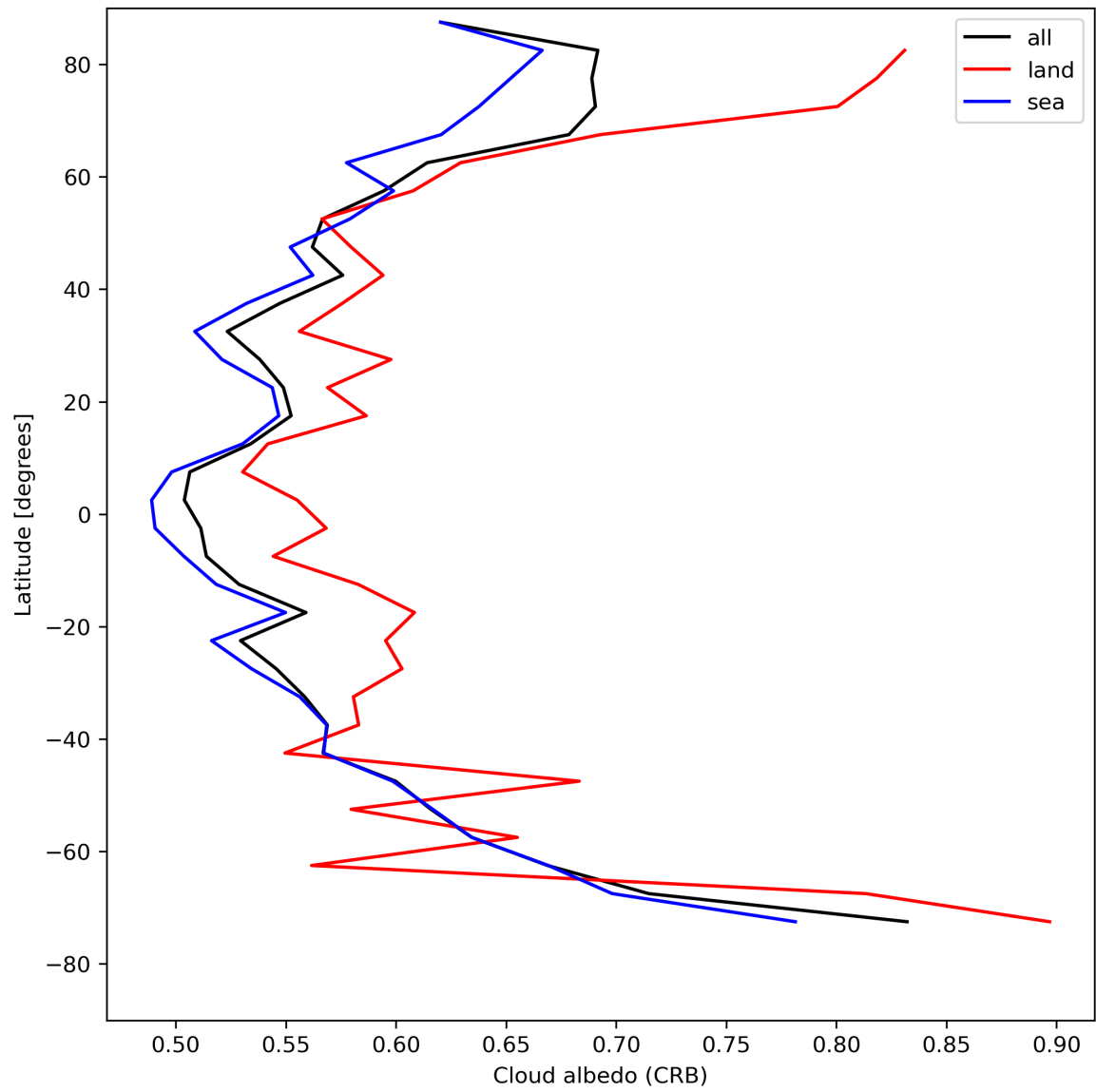
Figure 28: Zonal average of “Cloud albedo (CRB)” for 2024-05-08 to 2024-05-10.
