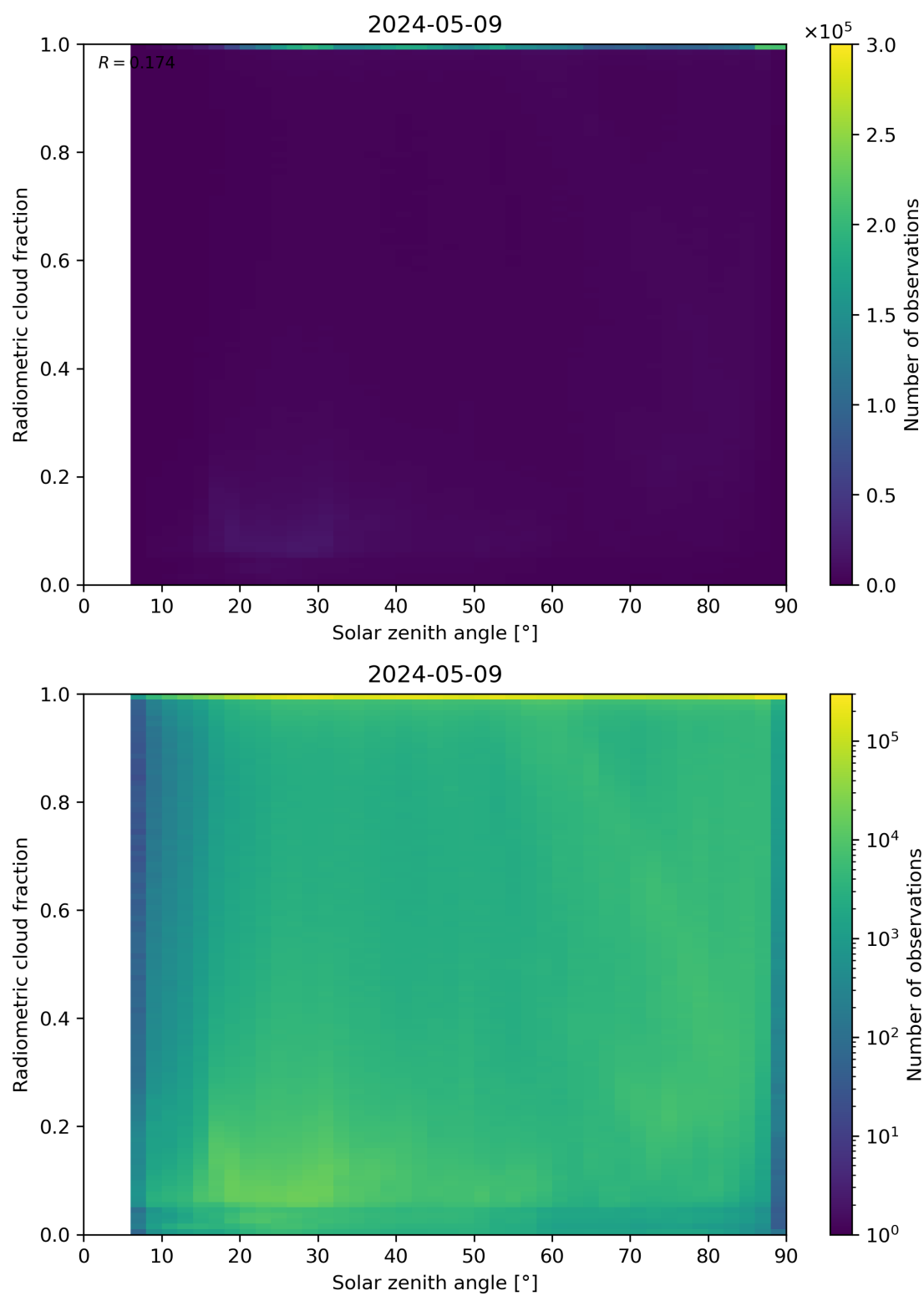
Figure 99: Scatter density plot of “Solar zenith angle” against “Radiometric cloud fraction” for 2024-05-08 to 2024-05-10.
