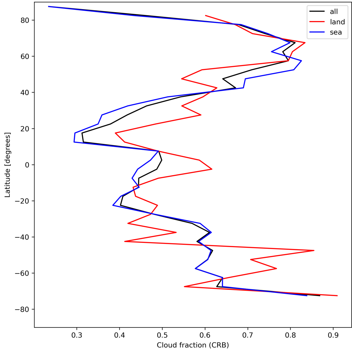
Figure 26: Zonal average of “Cloud fraction (CRB)” for 2024-05-08 to 2024-05-10.
