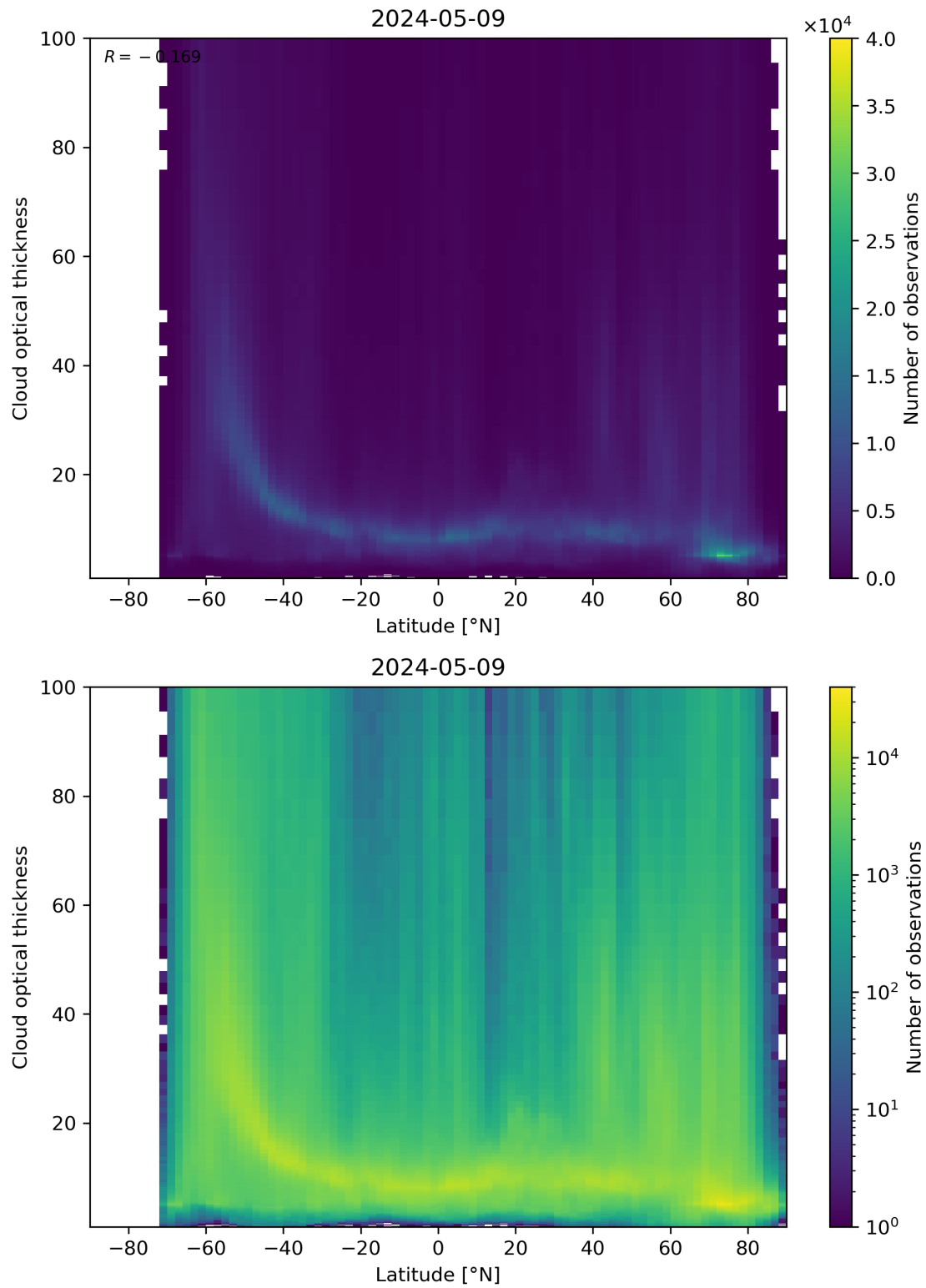
Figure 96: Scatter density plot of “Latitude” against “Cloud optical thickness” for 2024-05-08 to 2024-05-10.
