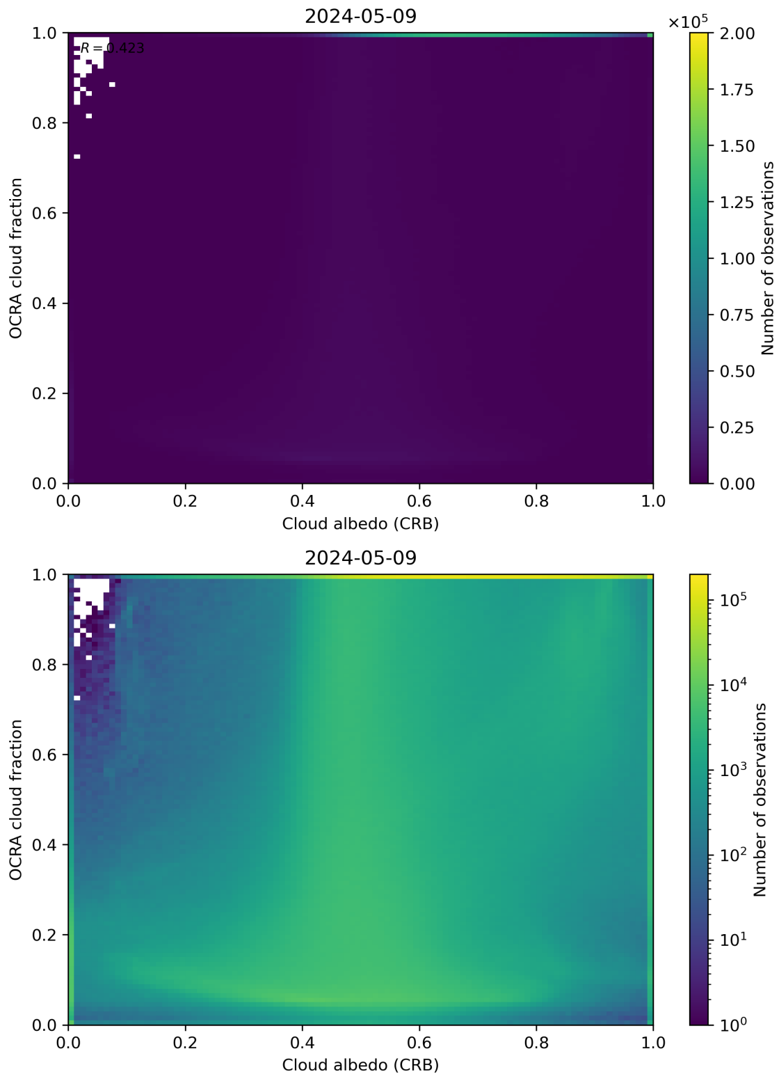
Figure 70: Scatter density plot of “Cloud albedo (CRB)” against “OCRA cloud fraction” for 2024-05-08 to 2024-05-10.
