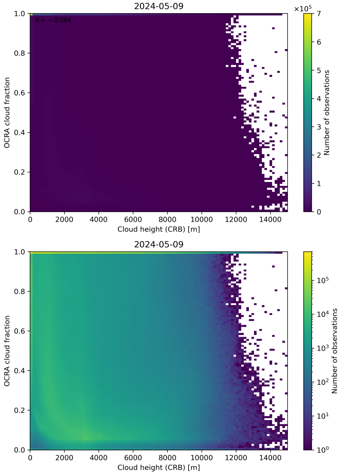
Figure 81: Scatter density plot of “Cloud height (CRB)” against “OCRA cloud fraction” for 2024-05-08 to 2024-05-10.
