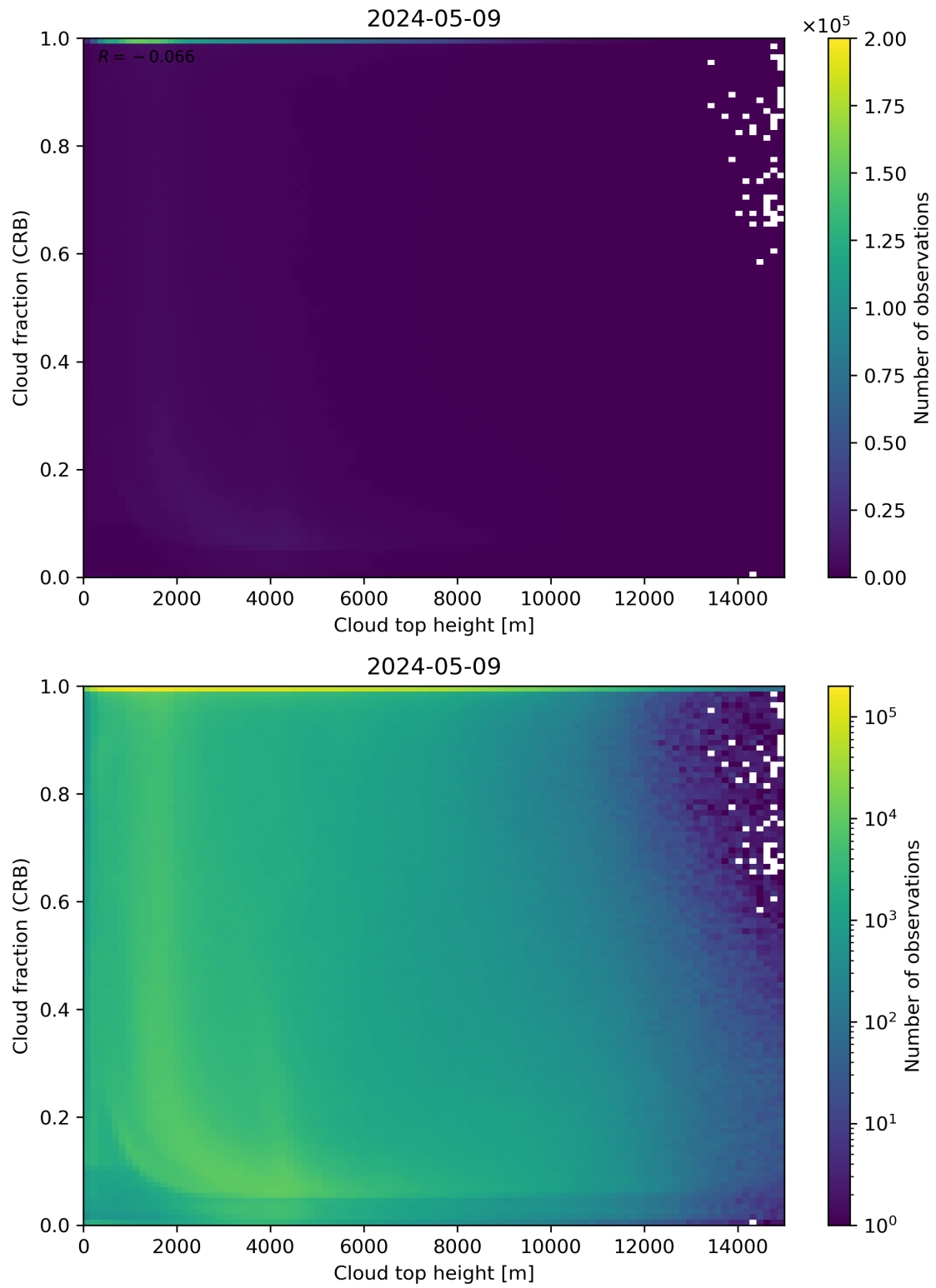
Figure 88: Scatter density plot of “Cloud top height” against “Cloud fraction (CRB)” for 2024-05-08 to 2024-05-10.
