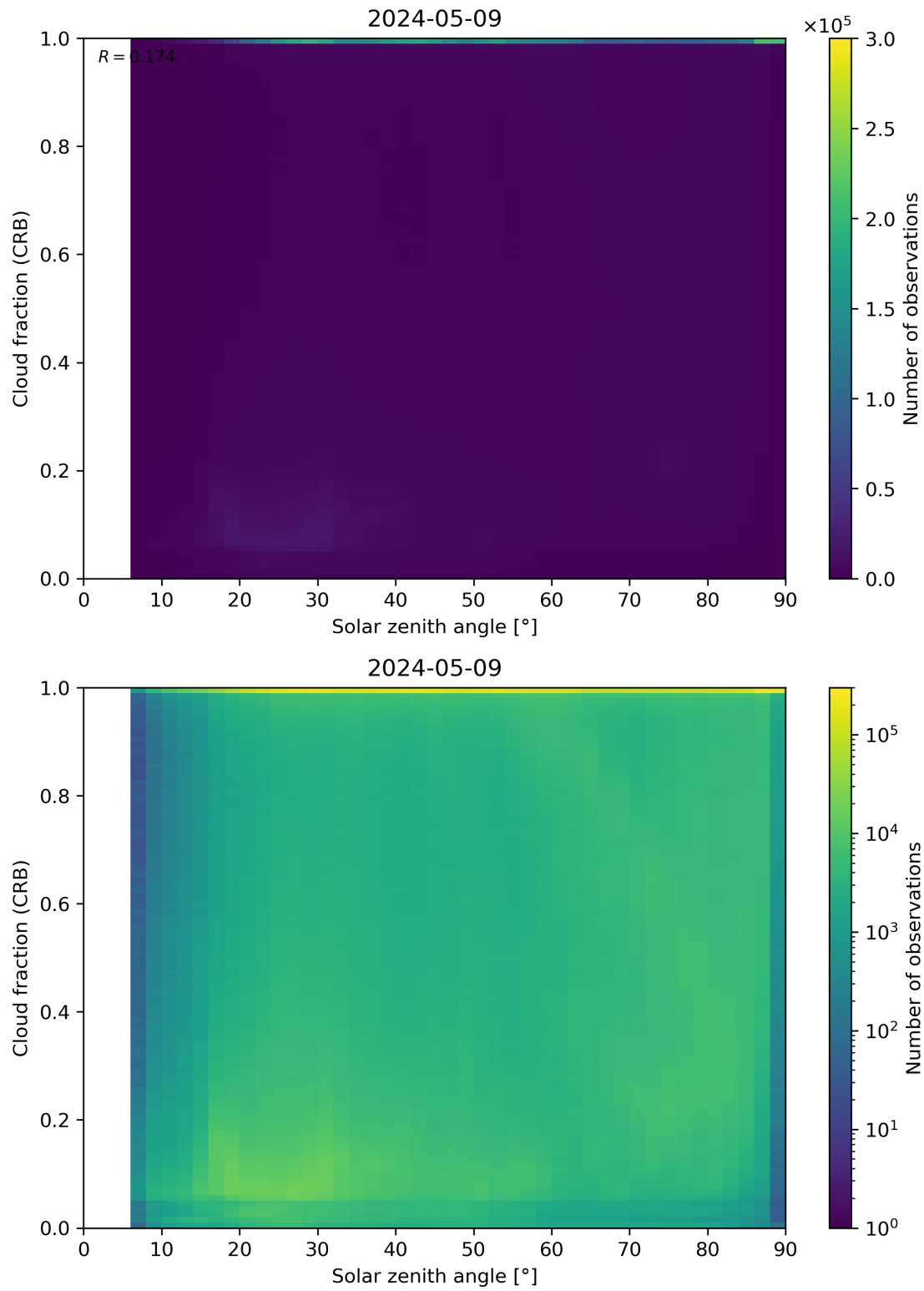
Figure 101: Scatter density plot of “Solar zenith angle” against “Cloud fraction (CRB)” for 2024-05-08 to 2024-05-10.
