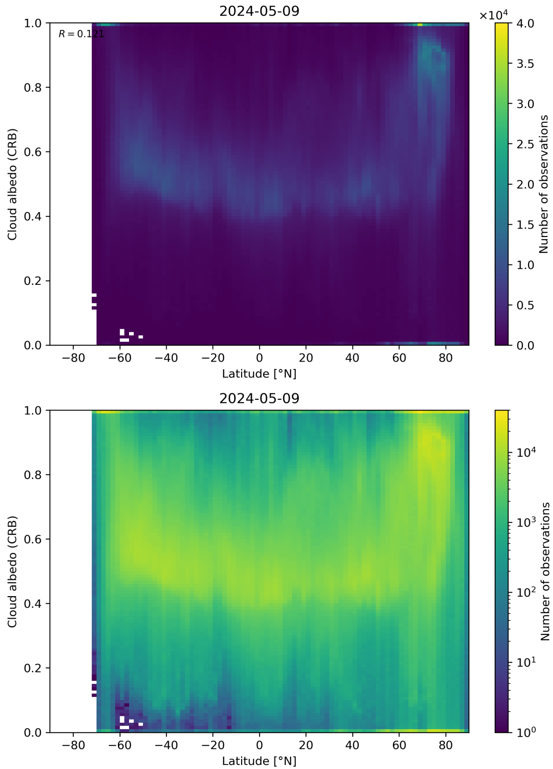
Figure 91: Scatter density plot of “Latitude” against “Cloud albedo (CRB)” for 2024-05-08 to 2024-05-10.
