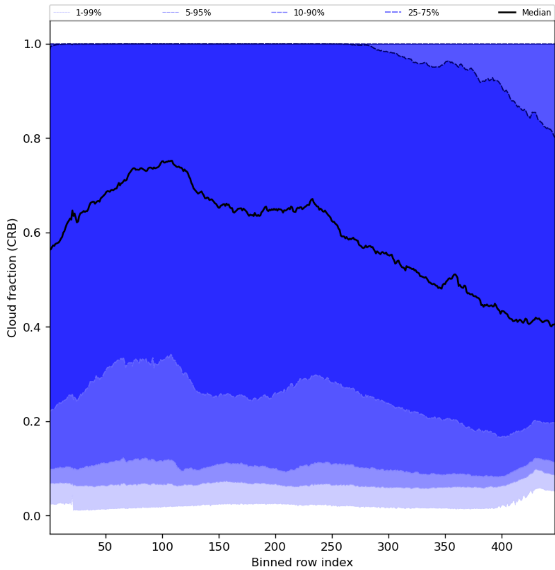
Figure 58: Along track statistics of “Cloud fraction (CRB)” for 2024-05-08 to 2024-05-10
