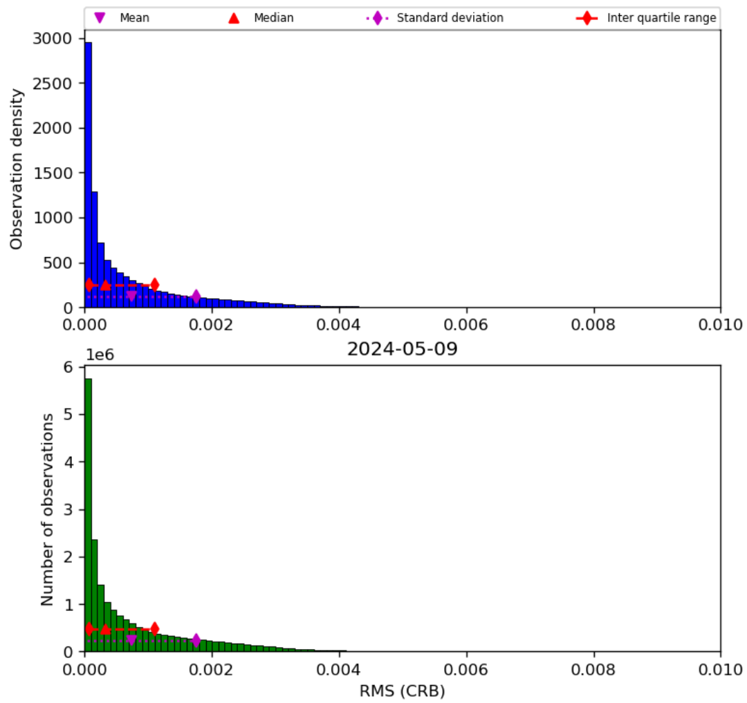
Figure 48: Histogram of “RMS (CRB)” for 2024-05-08 to 2024-05-10
