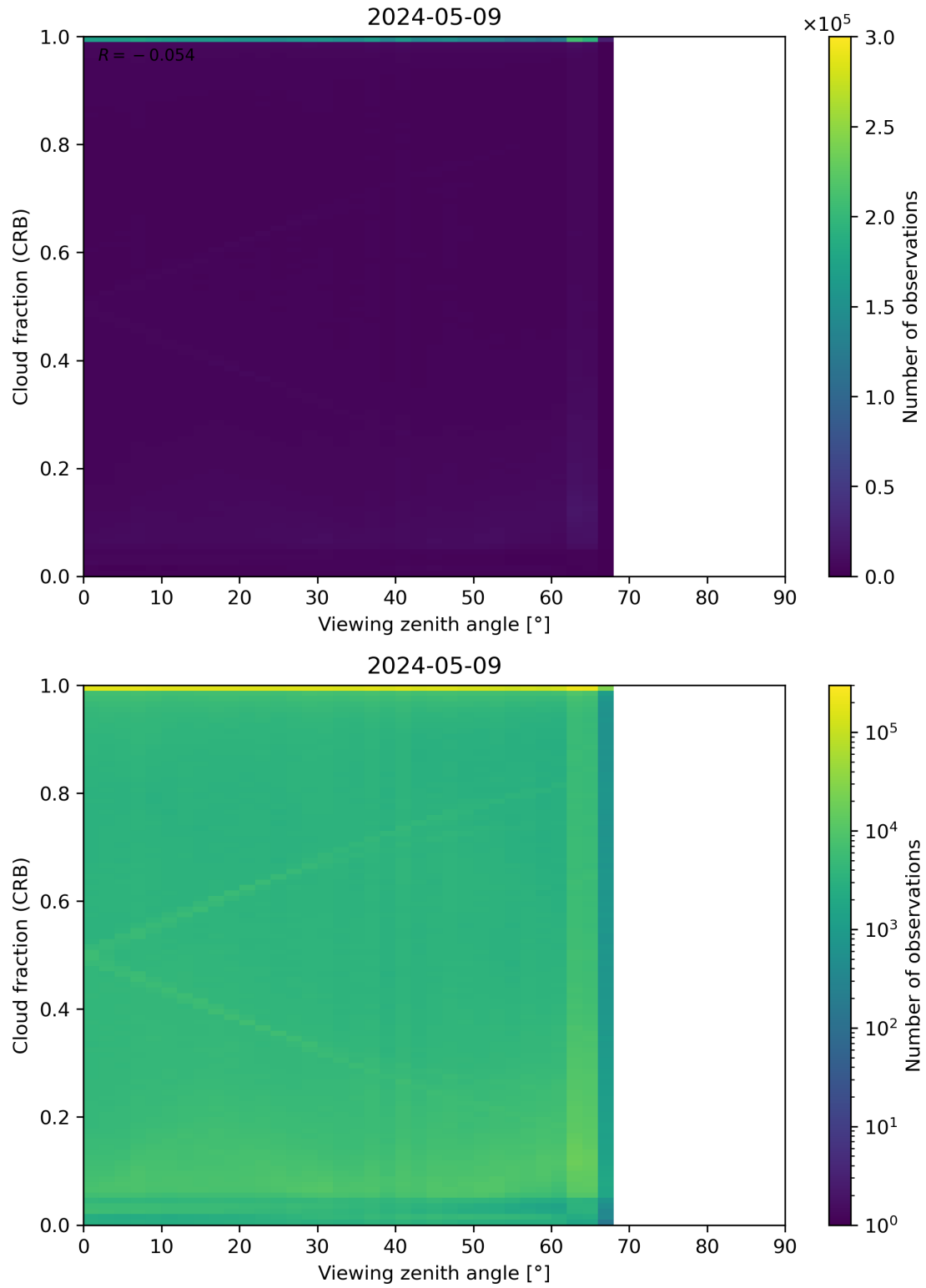
Figure 109: Scatter density plot of “Viewing zenith angle” against “Cloud fraction (CRB)” for 2024-05-08 to 2024-05-10.
