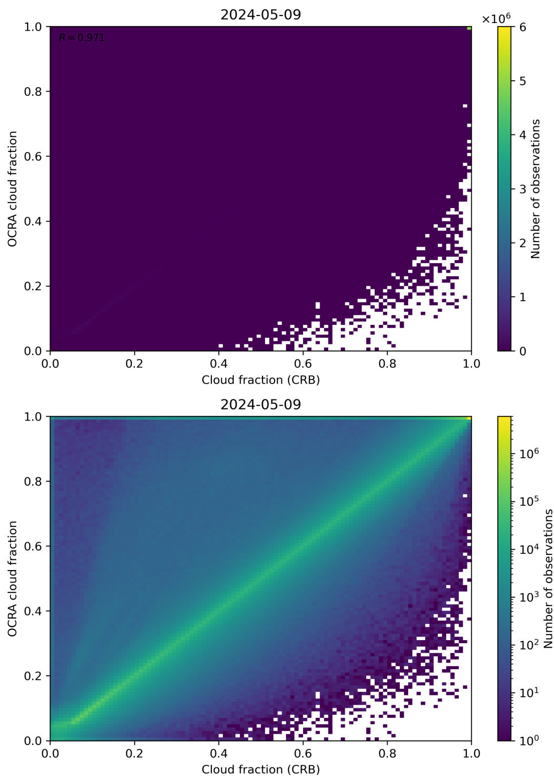
Figure 78: Scatter density plot of “Cloud fraction (CRB)” against “OCRA cloud fraction” for 2024-05-08 to 2024-05-10.
