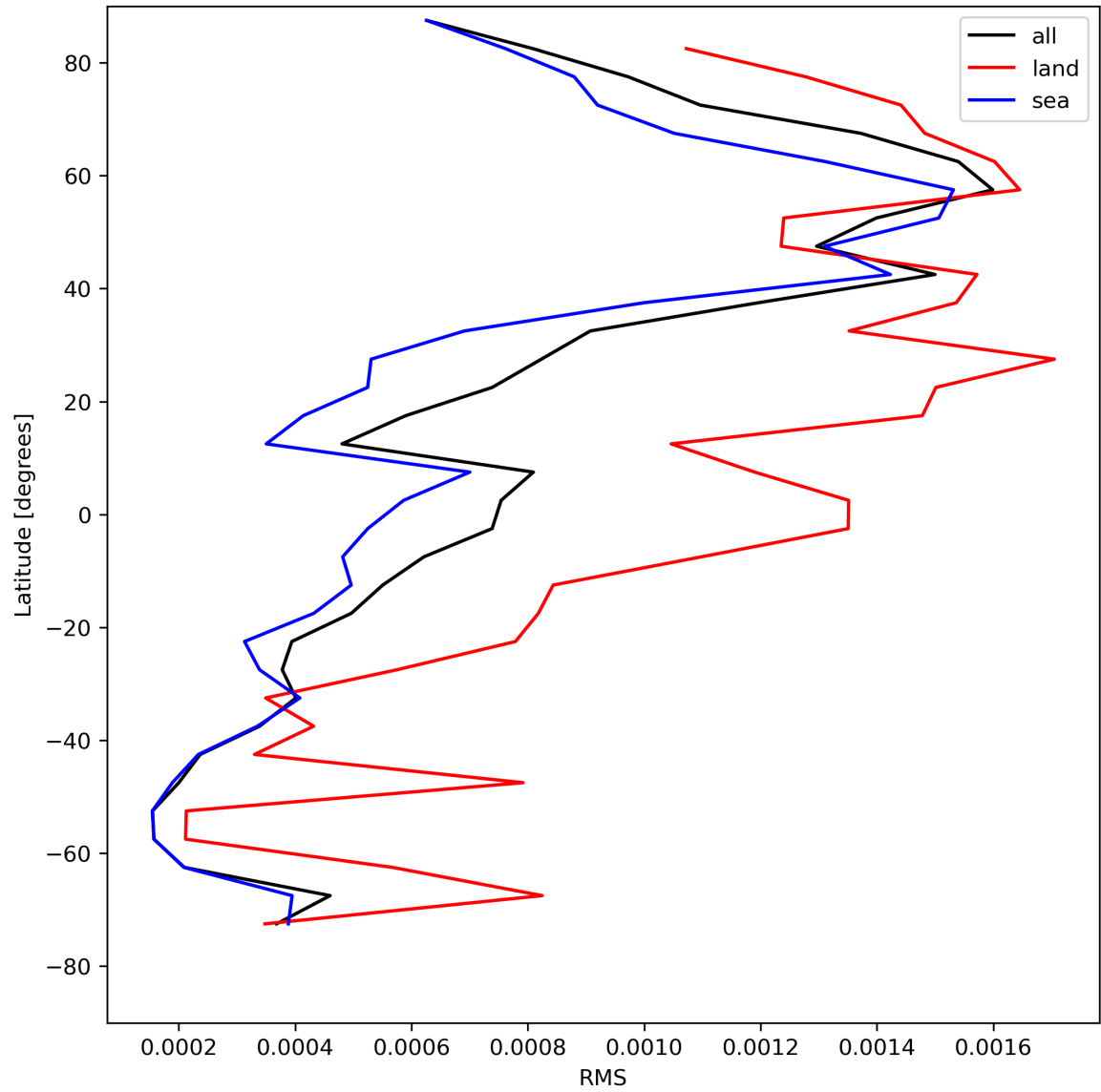
Figure 31: Zonal average of “RMS” for 2024-05-08 to 2024-05-10.
