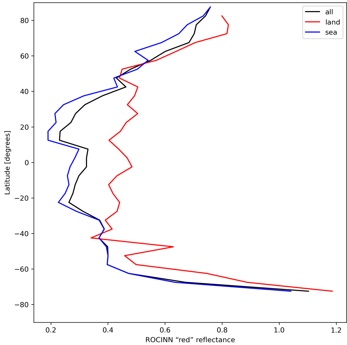
Figure 37: Zonal average of “ROCINN “red” reflectance” for 2024-05-08 to 2024-05-10.
