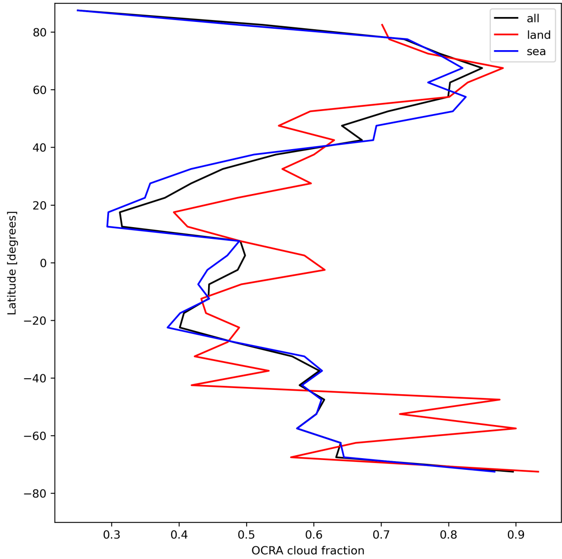
Figure 34: Zonal average of “OCRA cloud fraction” for 2024-05-08 to 2024-05-10.
