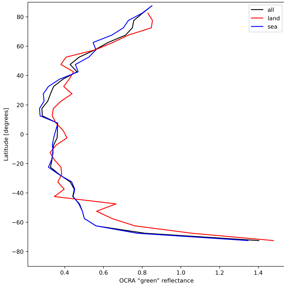
Figure 36: Zonal average of “OCRA “green” reflectance” for 2024-05-08 to 2024-05-10.
