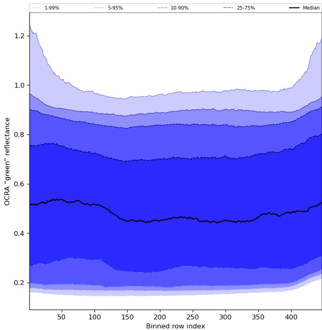
Figure 68: Along track statistics of "OCRA "green" reflectance" for 2024-05-08 to 2024-05-10
