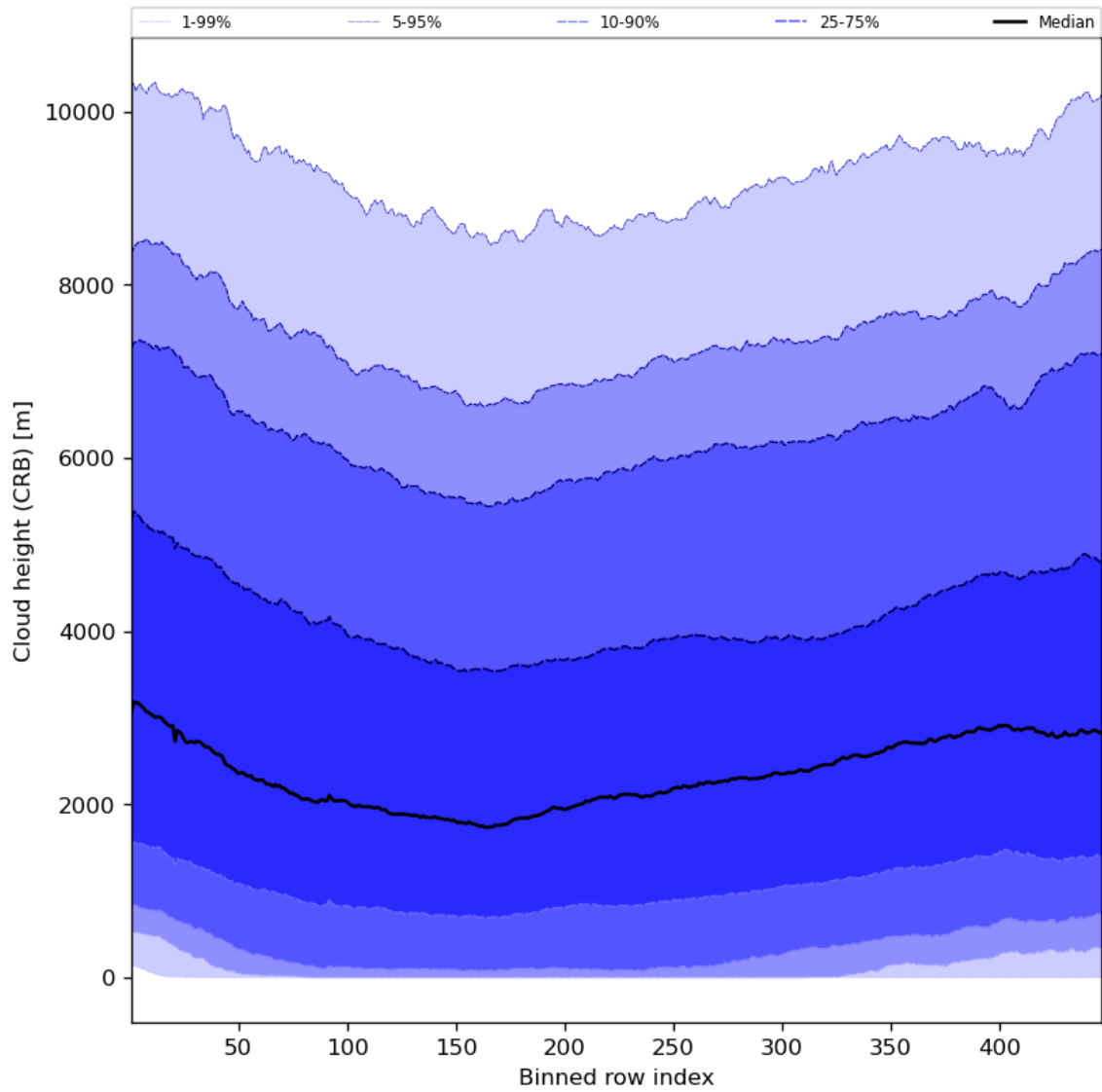
Figure 59: Along track statistics of “Cloud height (CRB)” for 2024-05-08 to 2024-05-10
