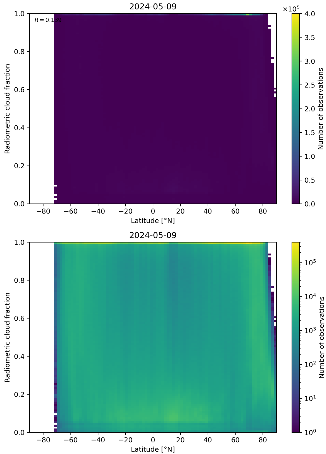
Figure 92: Scatter density plot of “Latitude” against “Radiometric cloud fraction” for 2024-05-08 to 2024-05-10.
