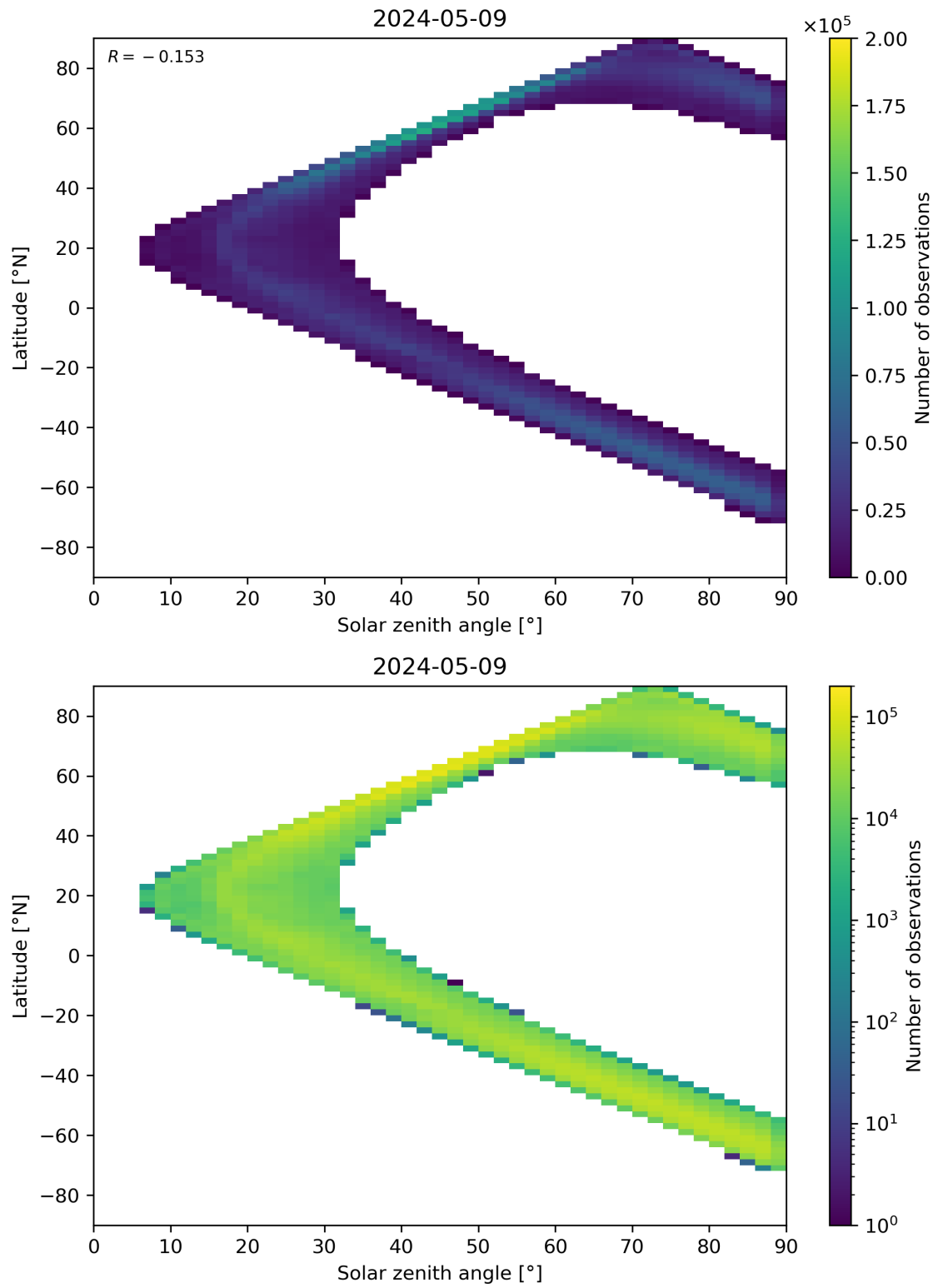
Figure 105: Scatter density plot of “Solar zenith angle” against “Latitude” for 2024-05-08 to 2024-05-10.
