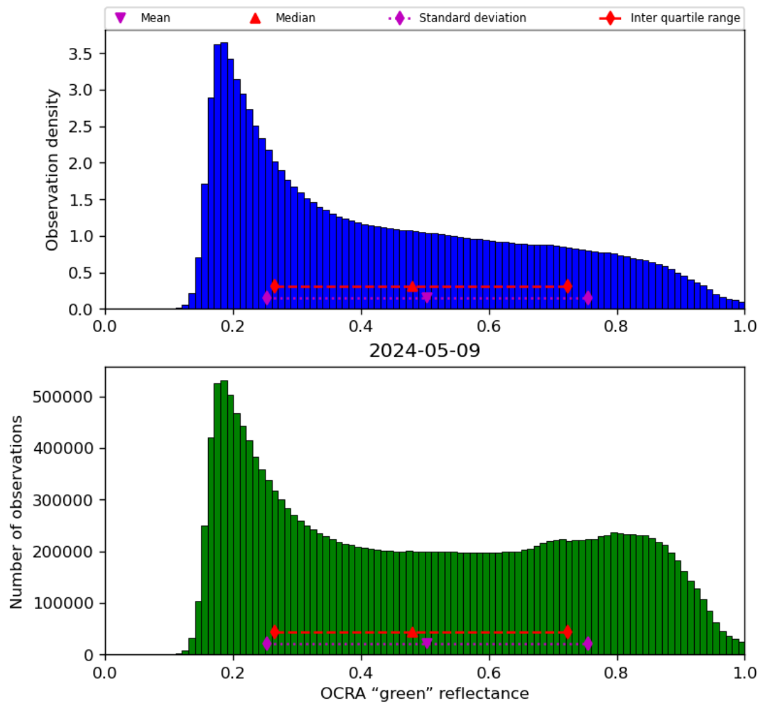
Figure 52: Histogram of “OCRA “green” reflectance” for 2024-05-08 to 2024-05-10
