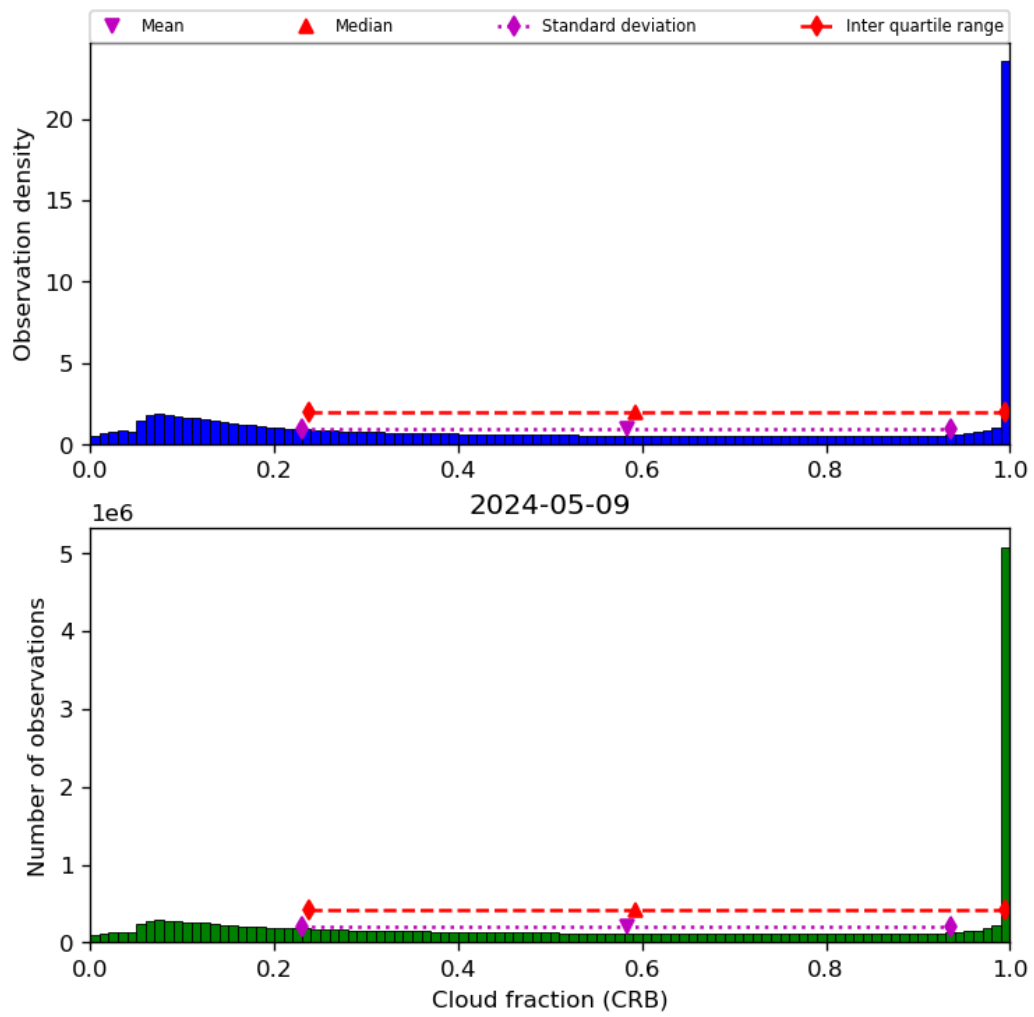
Figure 42: Histogram of “Cloud fraction (CRB)” for 2024-05-08 to 2024-05-10
