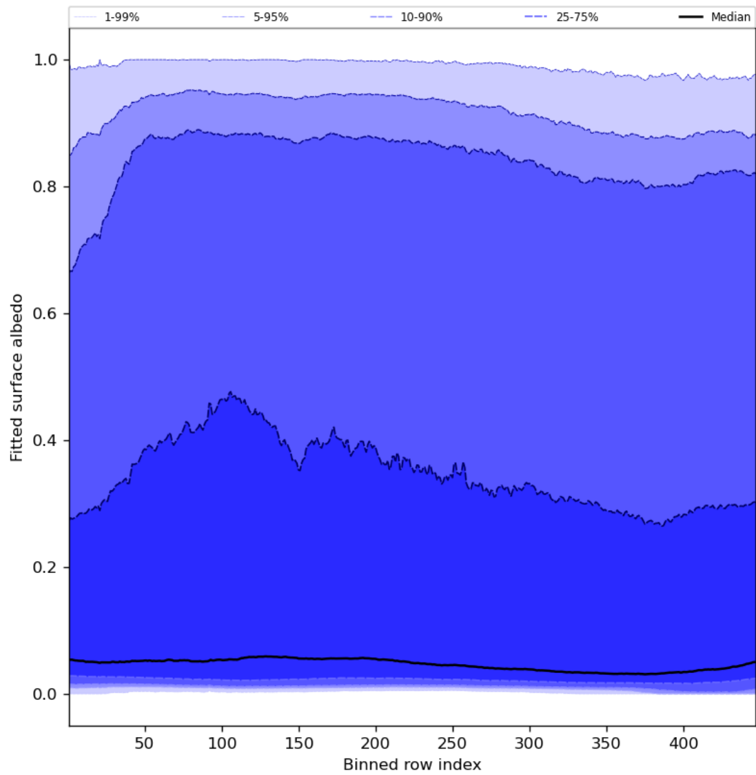
Figure 61: Along track statistics of “Fitted surface albedo” for 2024-05-08 to 2024-05-10
