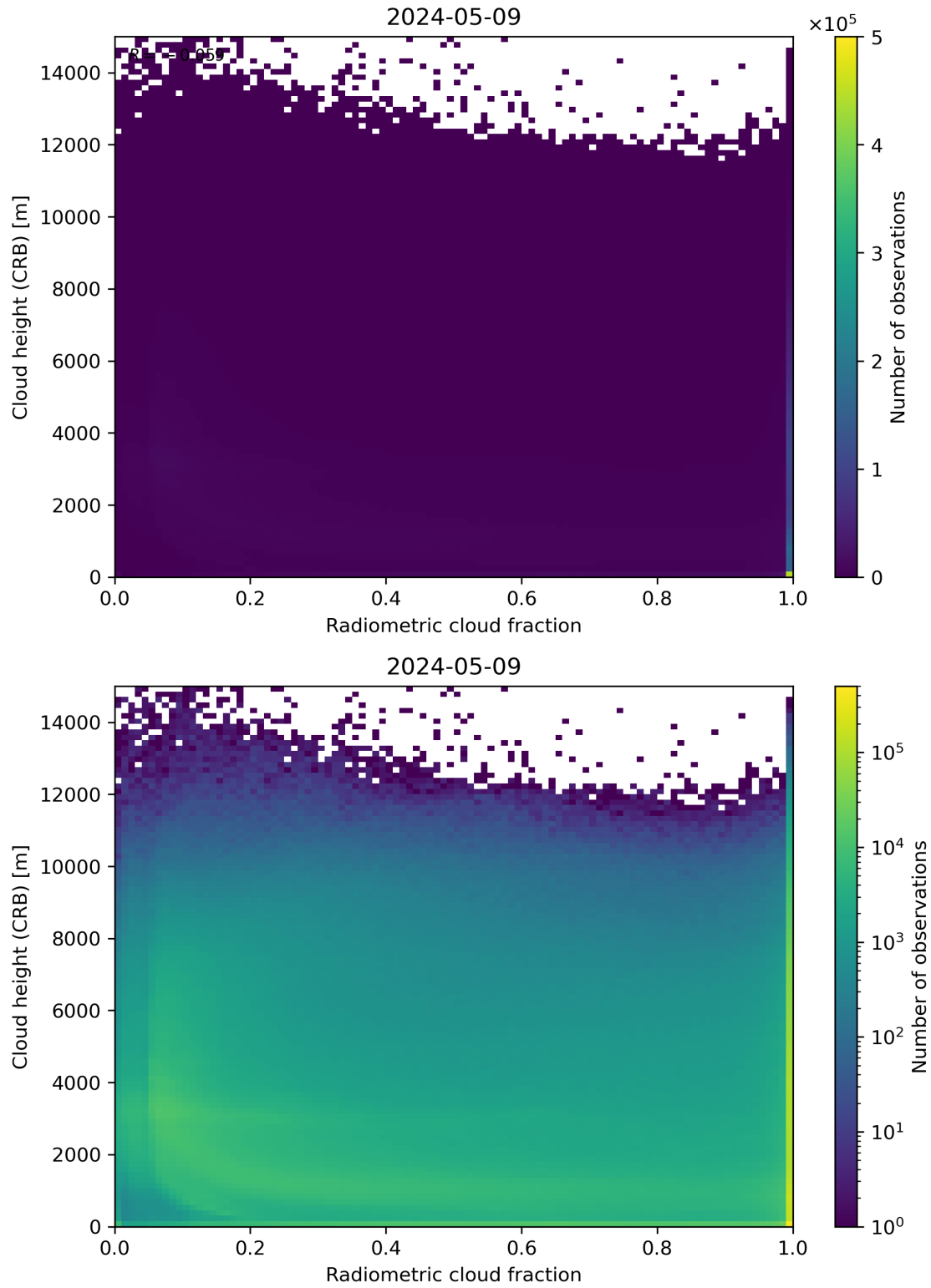
Figure 74: Scatter density plot of “Radiometric cloud fraction” against “Cloud height (CRB)” for 2024-05-08 to 2024-05-10.
