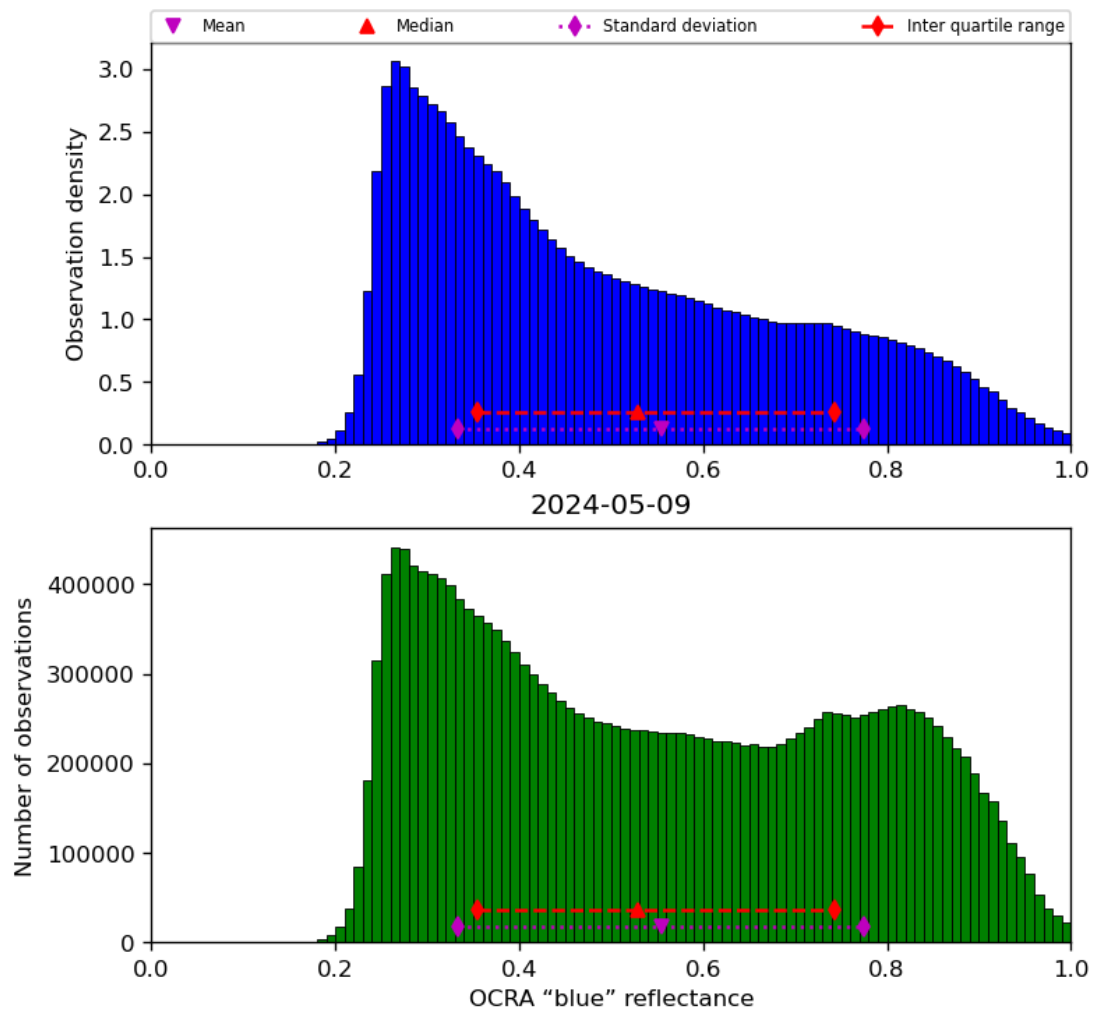
Figure 51: Histogram of “OCRA “blue” reflectance” for 2024-05-08 to 2024-05-10
