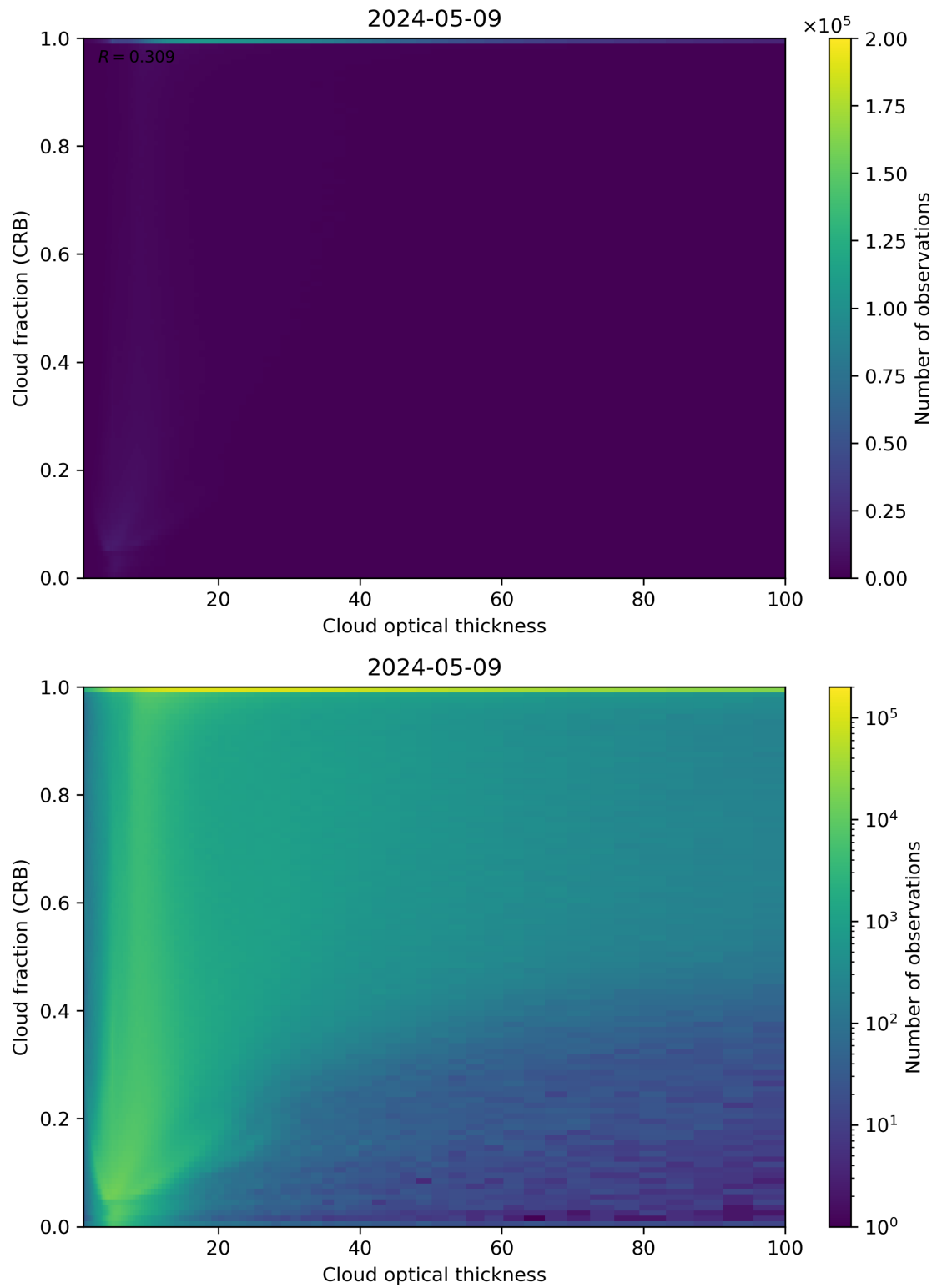
Figure 84: Scatter density plot of “Cloud optical thickness” against “Cloud fraction (CRB)” for 2024-05-08 to 2024-05-10.
