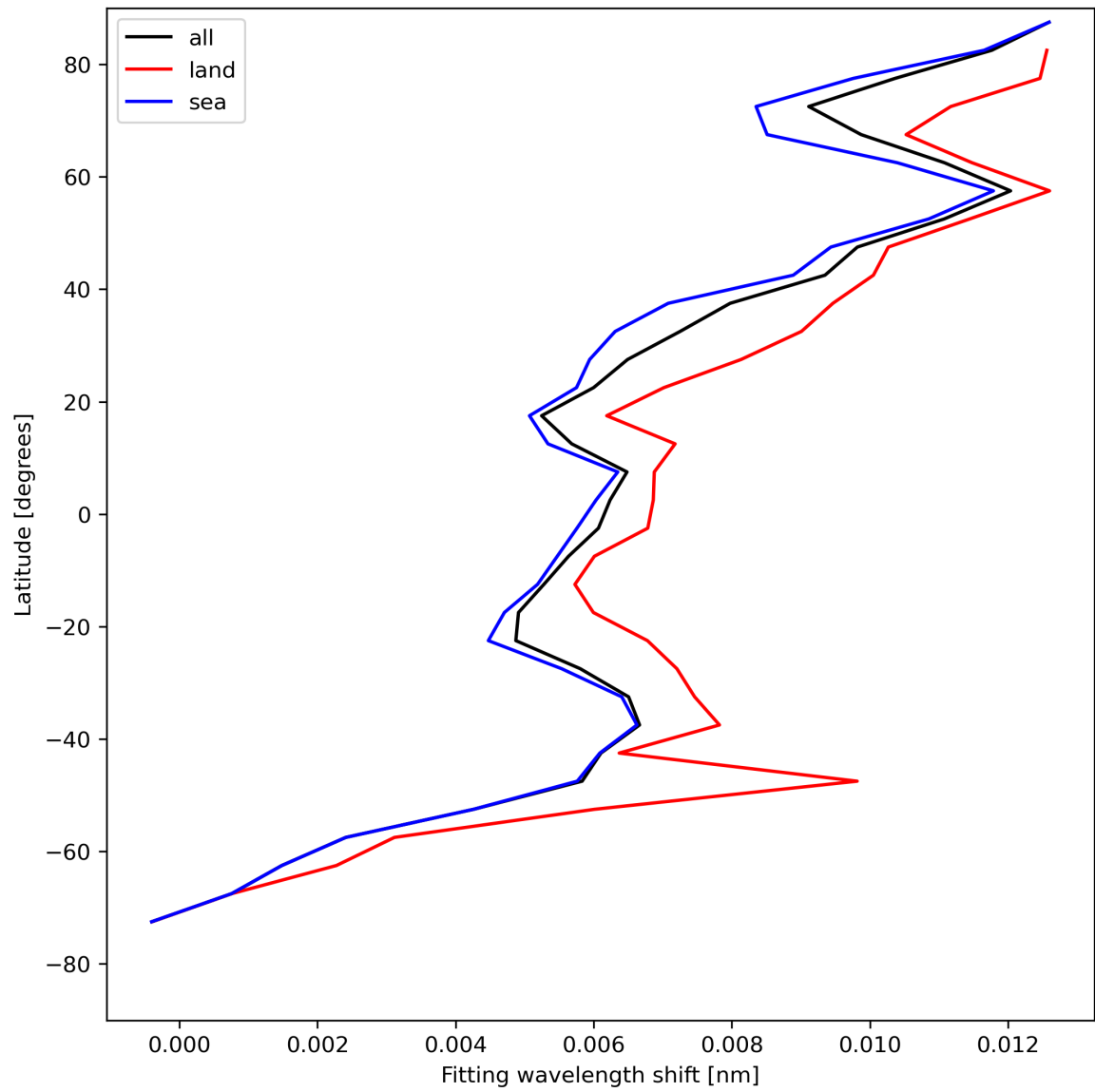
Figure 33: Zonal average of “Fitting wavelength shift” for 2024-05-08 to 2024-05-10.
