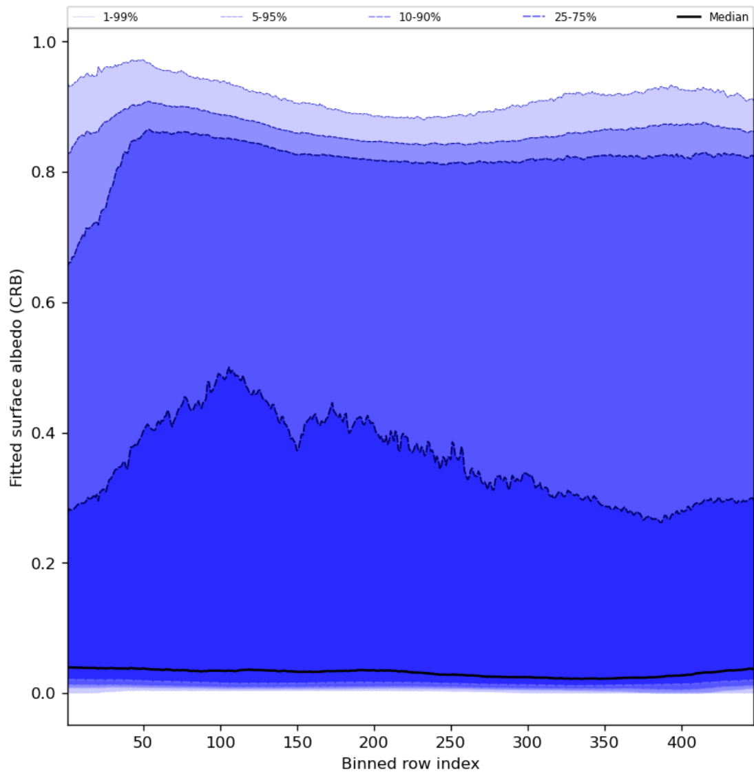
Figure 62: Along track statistics of “Fitted surface albedo (CRB)” for 2024-05-08 to 2024-05-10
