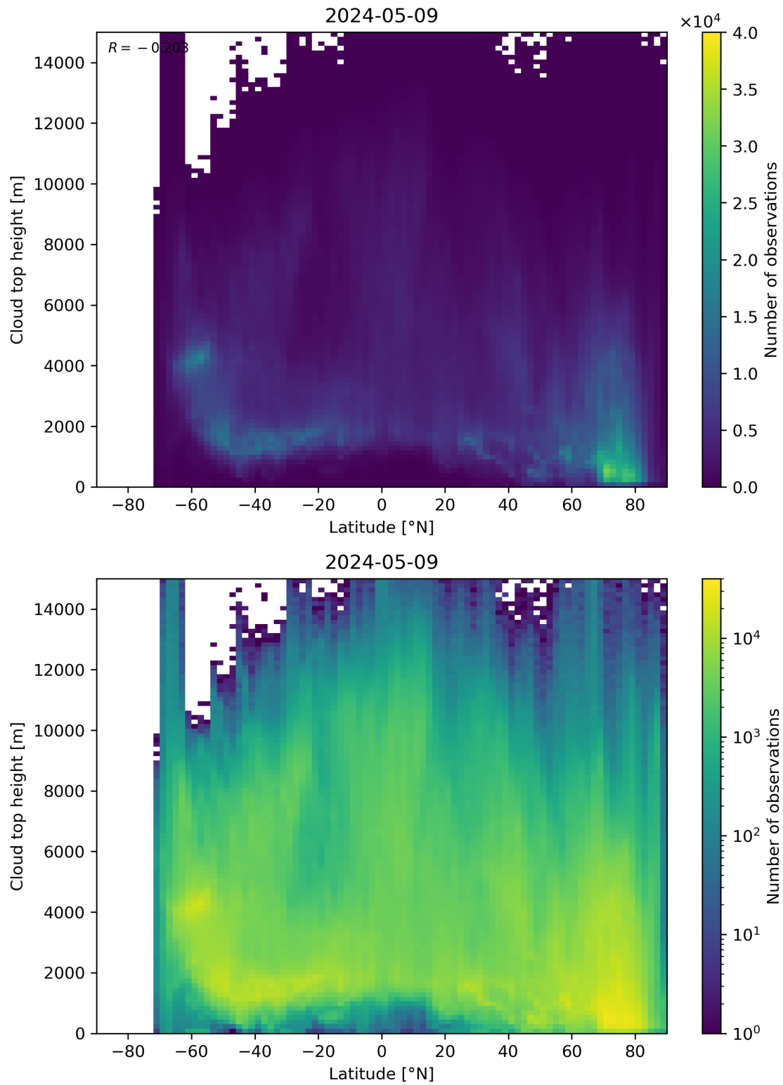
Figure 97: Scatter density plot of “Latitude” against “Cloud top height” for 2024-05-08 to 2024-05-10.
