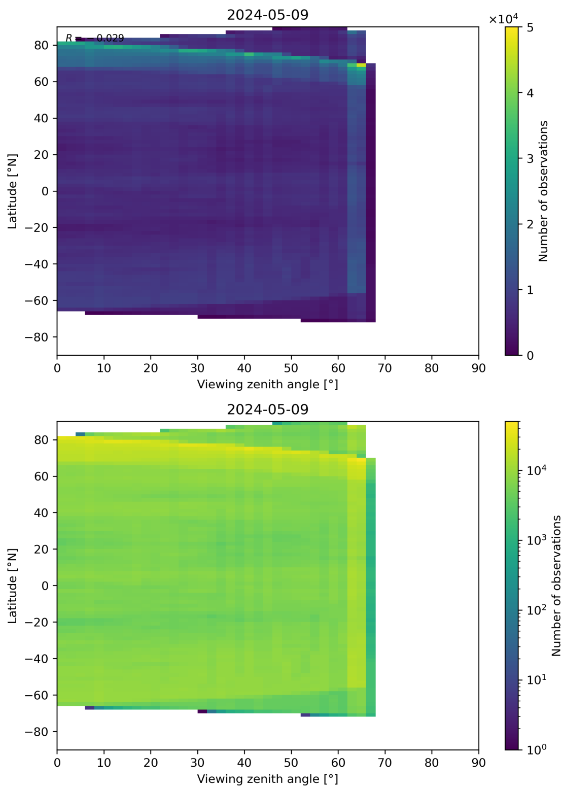
Figure 113: Scatter density plot of “Viewing zenith angle” against “Latitude” for 2024-05-08 to 2024-05-10.
