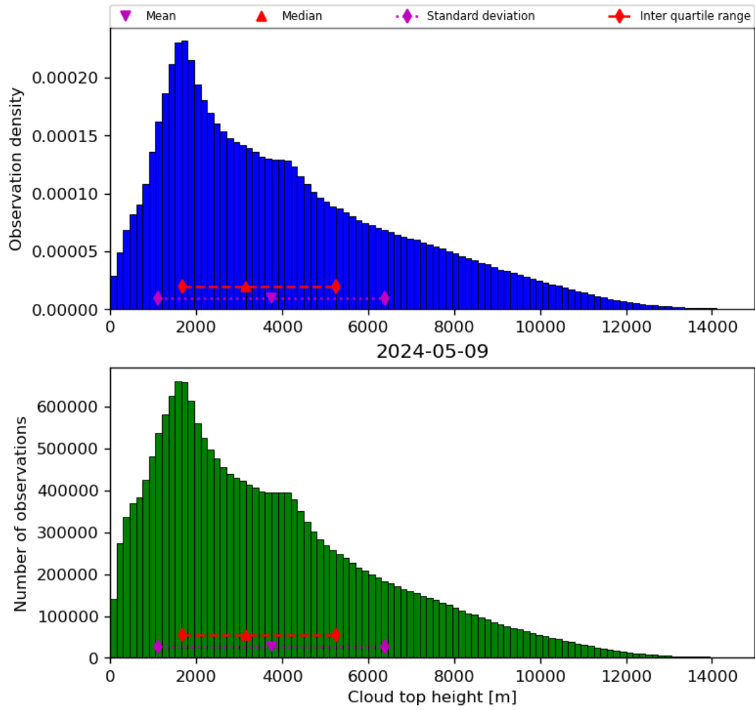
Figure 40: Histogram of “Cloud top height” for 2024-05-08 to 2024-05-10
