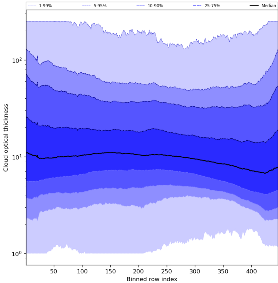
Figure 57: Along track statistics of “Cloud optical thickness” for 2024-05-08 to 2024-05-10
