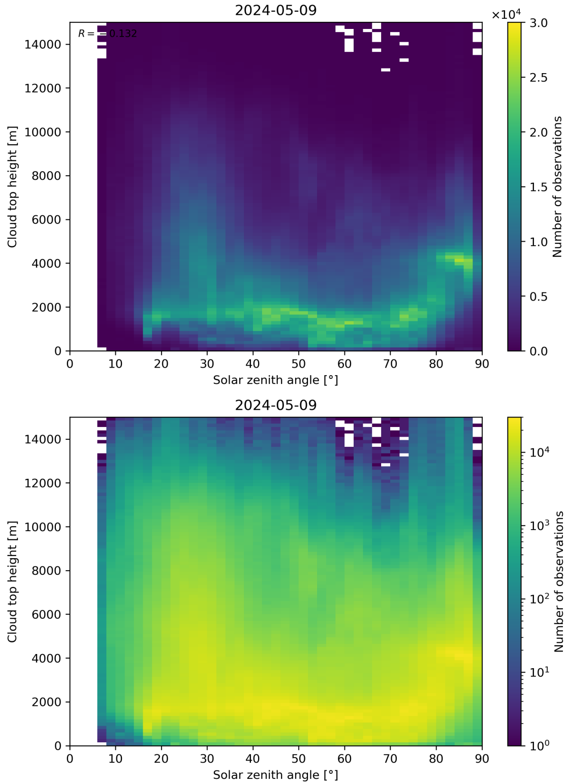
Figure 104: Scatter density plot of “Solar zenith angle” against “Cloud top height” for 2024-05-08 to 2024-05-10.
