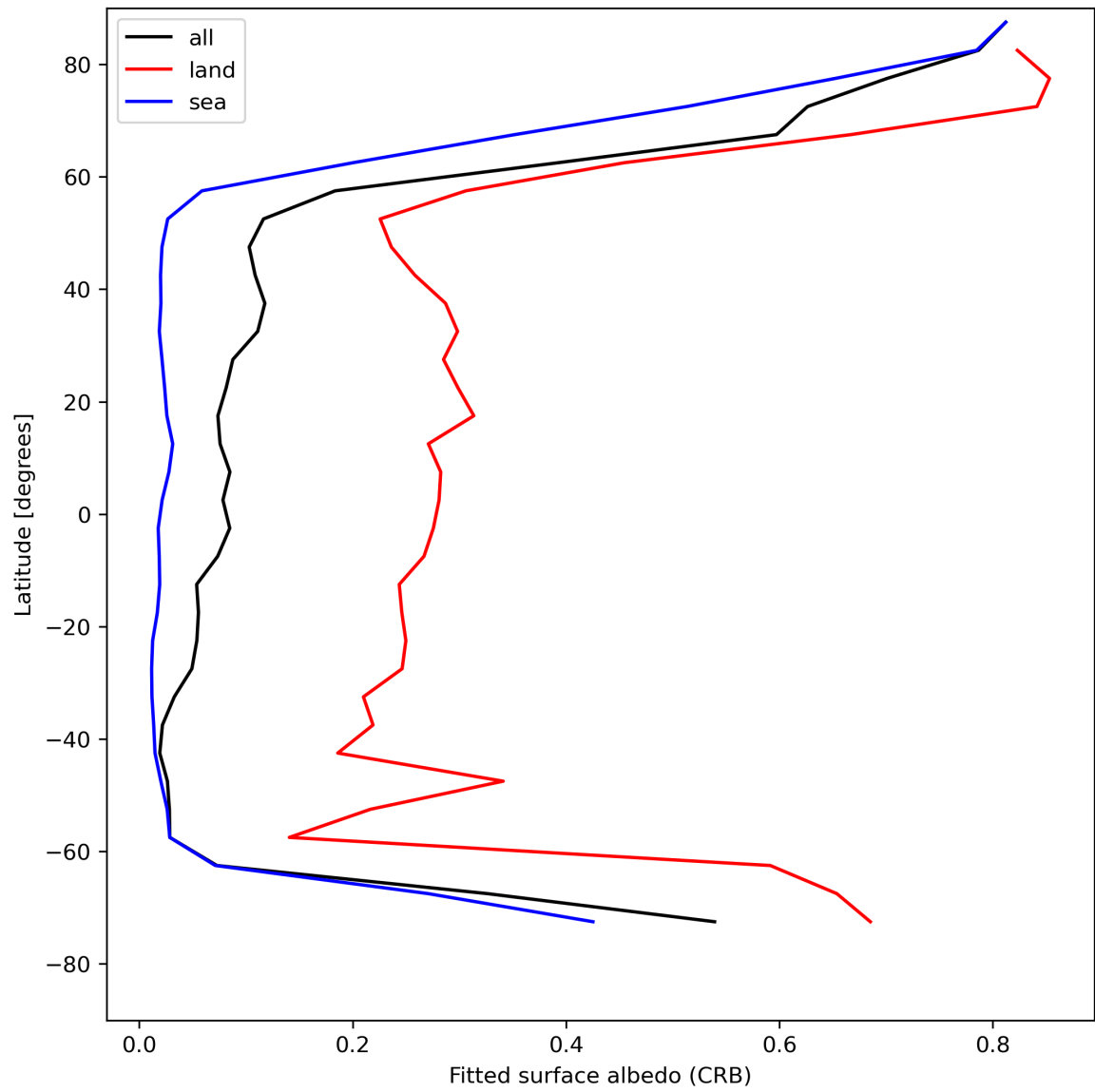
Figure 30: Zonal average of “Fitted surface albedo (CRB)” for 2024-05-08 to 2024-05-10.
