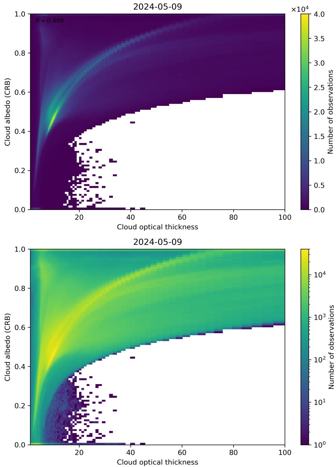
Figure 82: Scatter density plot of “Cloud optical thickness” against “Cloud albedo (CRB)” for 2024-05-08 to 2024-05-10.
