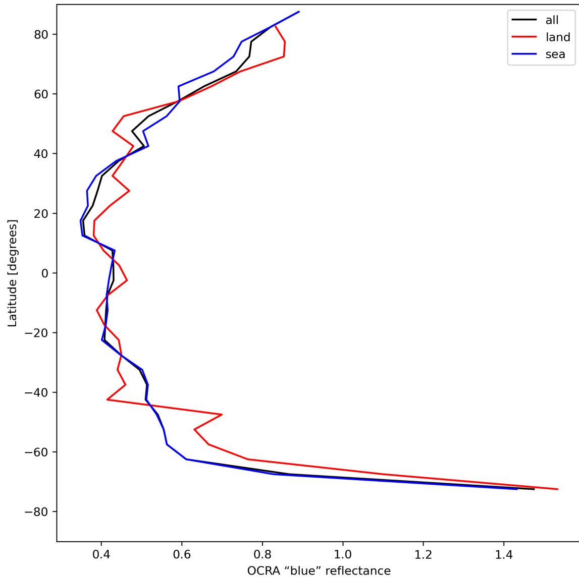
Figure 35: Zonal average of “OCRA “blue” reflectance” for 2024-05-08 to 2024-05-10.
