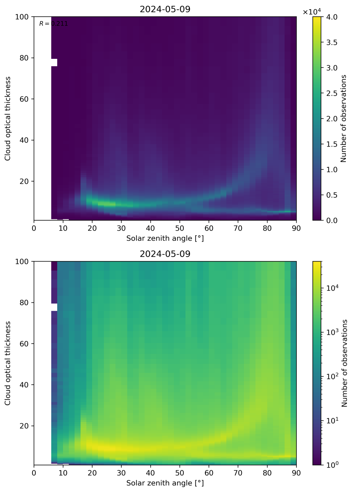
Figure 103: Scatter density plot of “Solar zenith angle” against “Cloud optical thickness” for 2024-05-08 to 2024-05-10.
