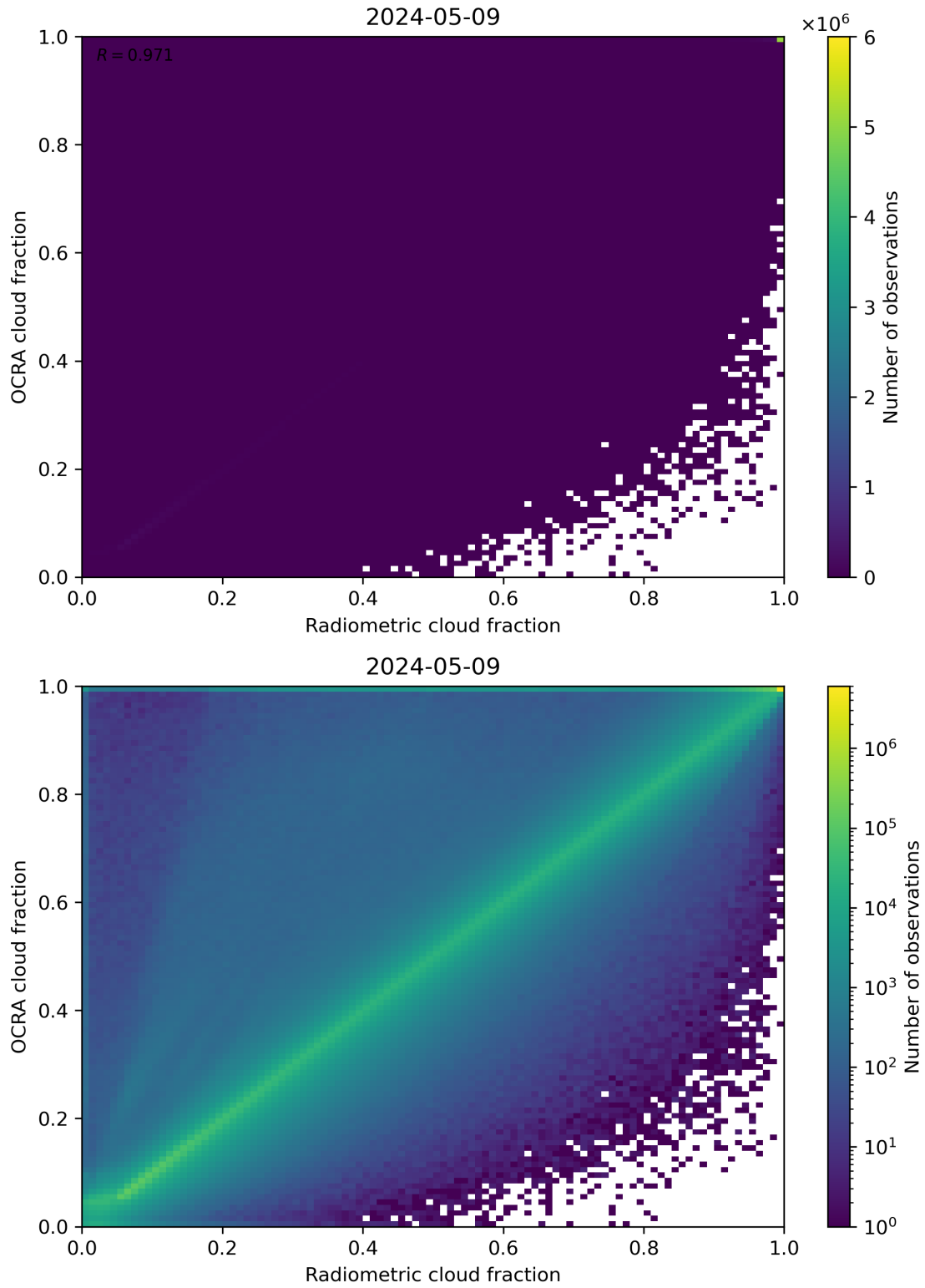
Figure 72: Scatter density plot of “Radiometric cloud fraction” against “OCRA cloud fraction” for 2024-05-08 to 2024-05-10.
