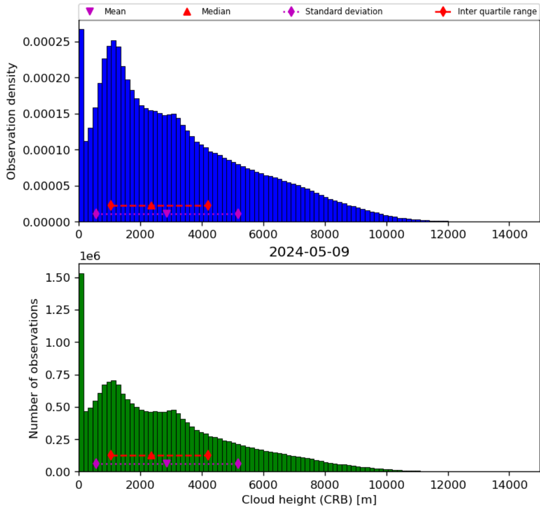
Figure 43: Histogram of “Cloud height (CRB)” for 2024-05-08 to 2024-05-10
