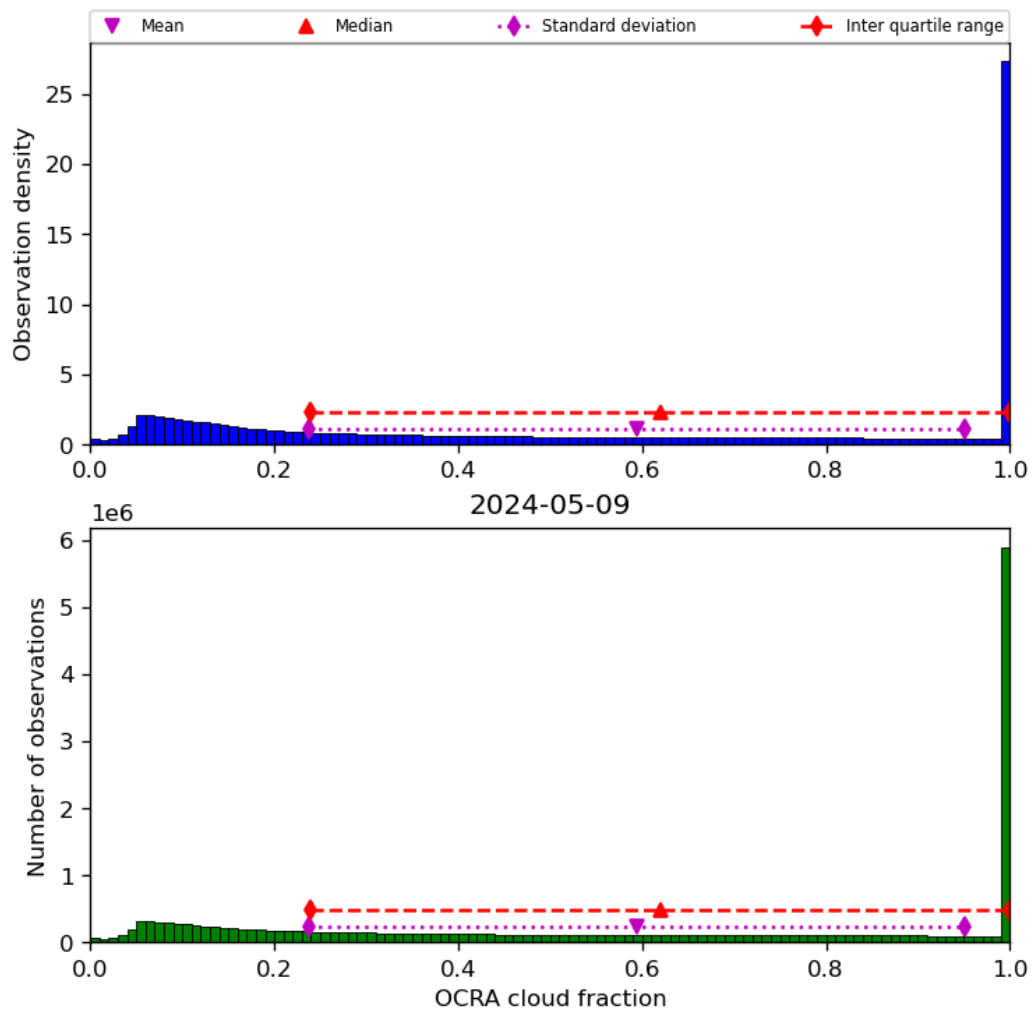
Figure 50: Histogram of “OCRA cloud fraction” for 2024-05-08 to 2024-05-10
