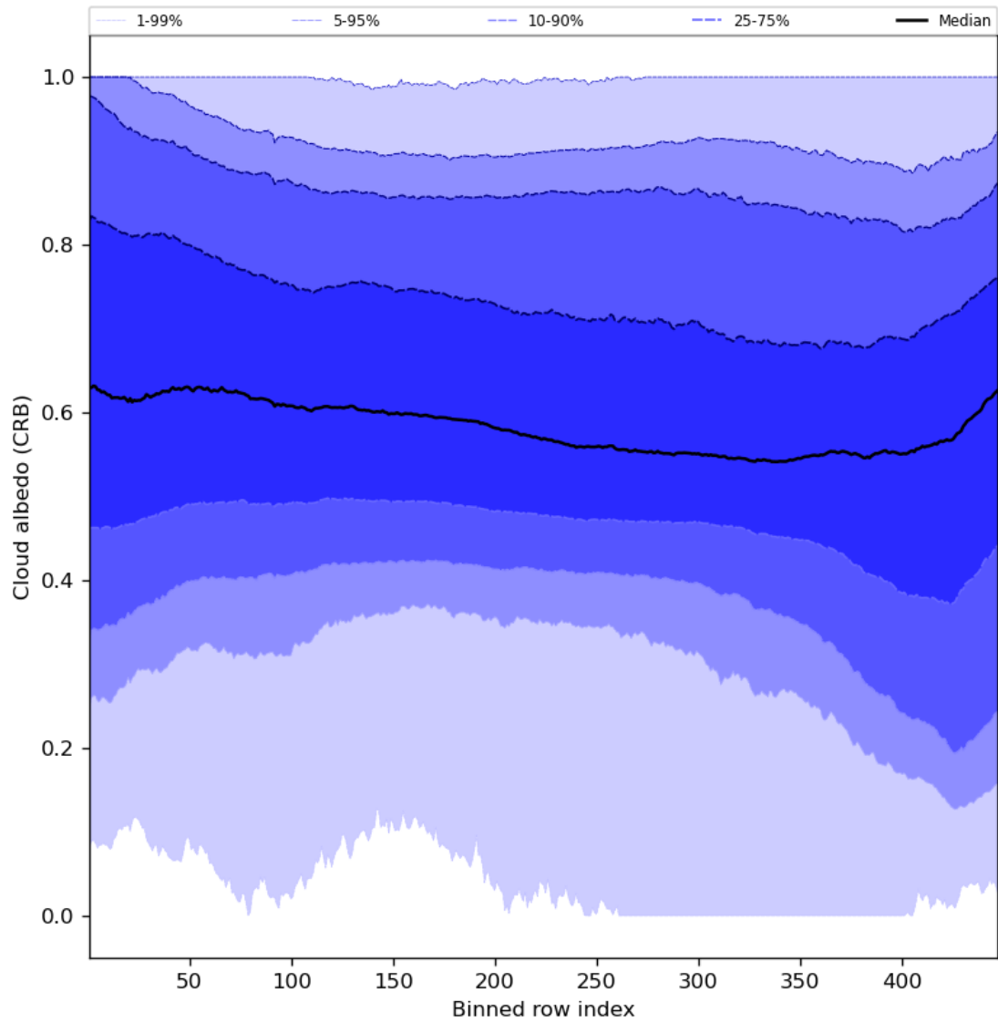
Figure 60: Along track statistics of “Cloud albedo (CRB)” for 2024-05-08 to 2024-05-10
