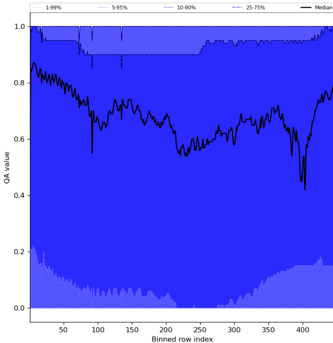
Figure 54: Along track statistics of “QA value” for 2024-05-08 to 2024-05-10
