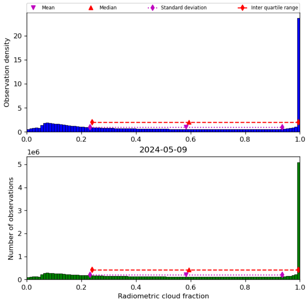
Figure 39: Histogram of “Radiometric cloud fraction” for 2024-05-08 to 2024-05-10
