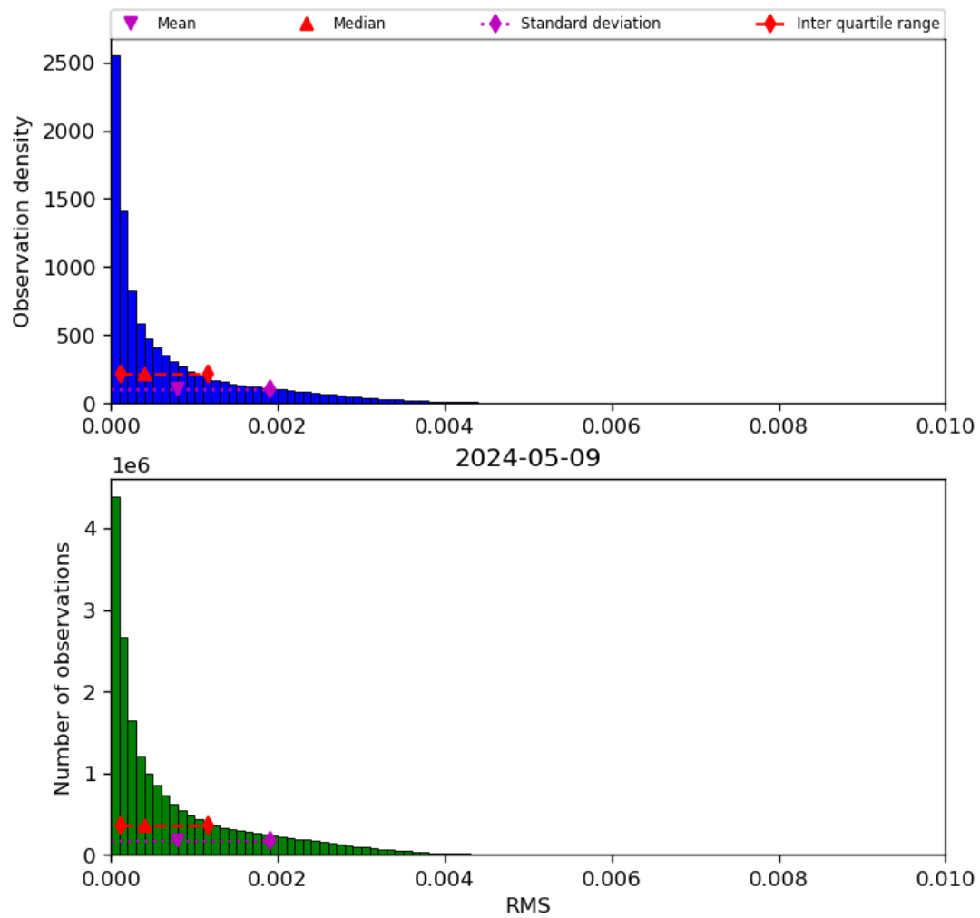
Figure 47: Histogram of “RMS” for 2024-05-08 to 2024-05-10
