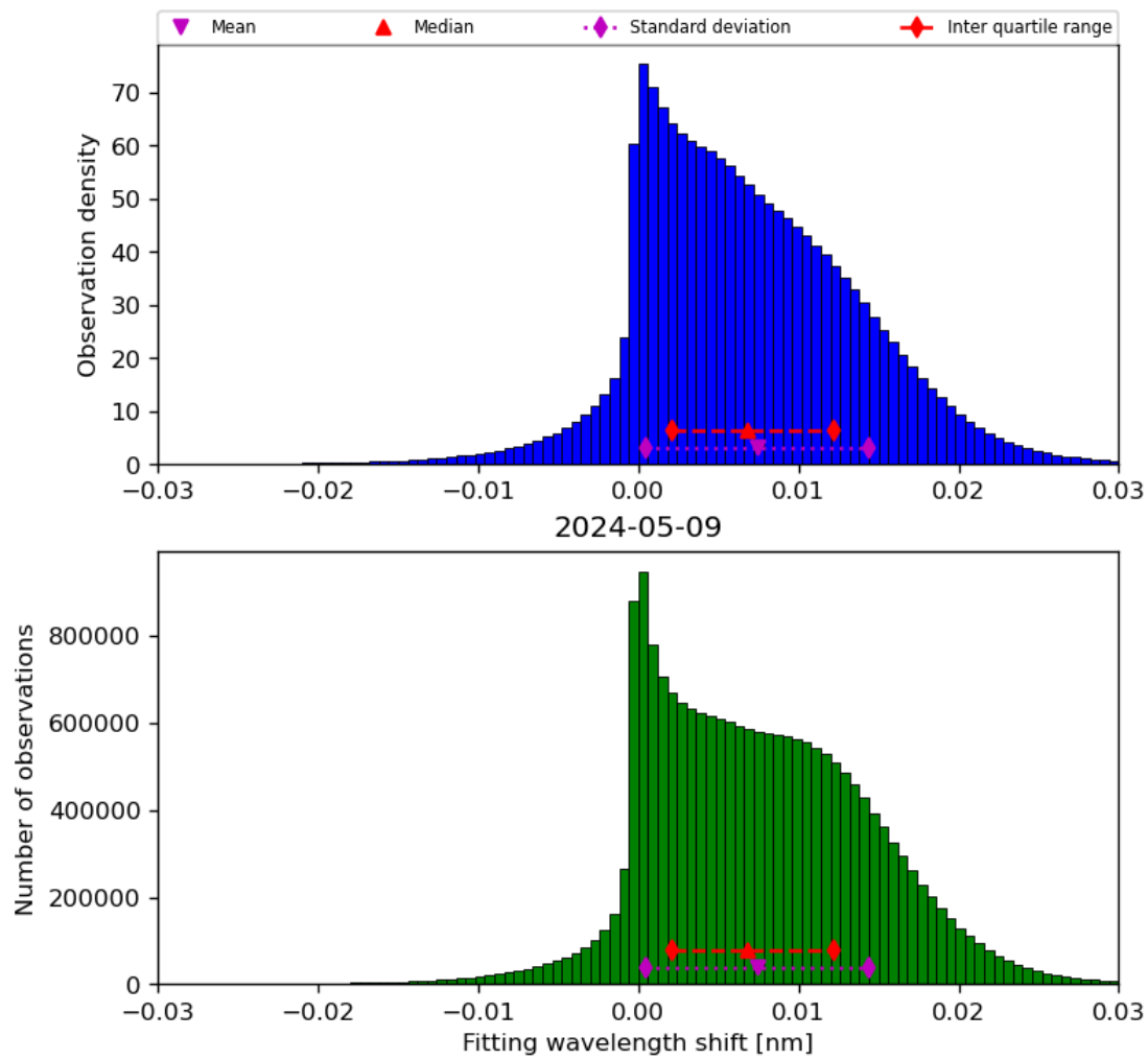
Figure 49: Histogram of “Fitting wavelength shift” for 2024-05-08 to 2024-05-10
