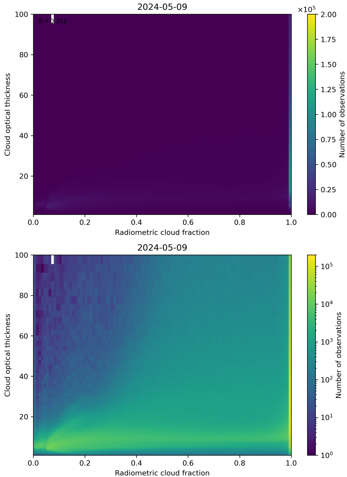
Figure 75: Scatter density plot of “Radiometric cloud fraction” against “Cloud optical thickness” for 2024-05-08 to 2024-05-10.
