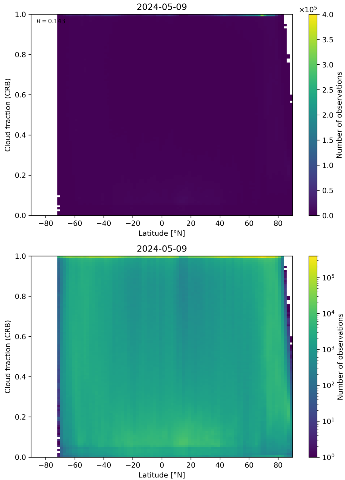
Figure 94: Scatter density plot of “Latitude” against “Cloud fraction (CRB)” for 2024-05-08 to 2024-05-10.
