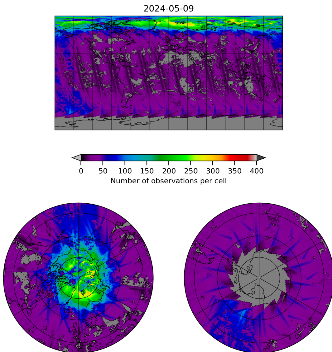
Figure 21: Map of the number of observations for 2024-05-08 to 2024-05-10
