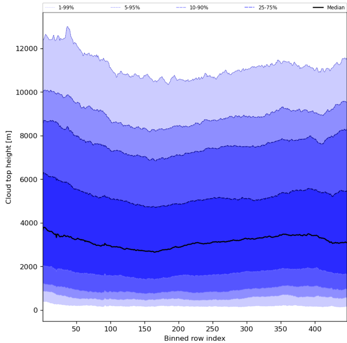
Figure 56: Along track statistics of “Cloud top height” for 2024-05-08 to 2024-05-10
