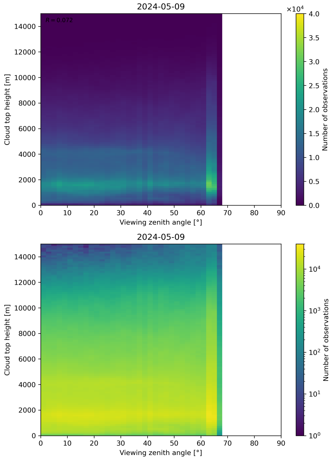
Figure 112: Scatter density plot of “Viewing zenith angle” against “Cloud top height” for 2024-05-08 to 2024-05-10.
