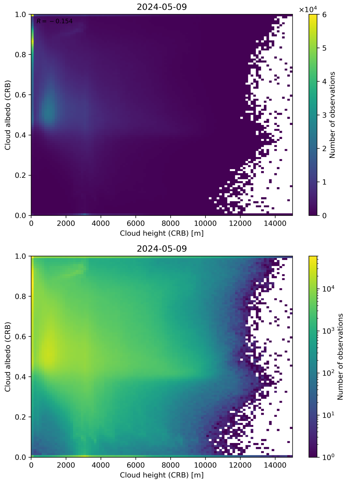
Figure 80: Scatter density plot of “Cloud height (CRB)” against “Cloud albedo (CRB)” for 2024-05-08 to 2024-05-10.
