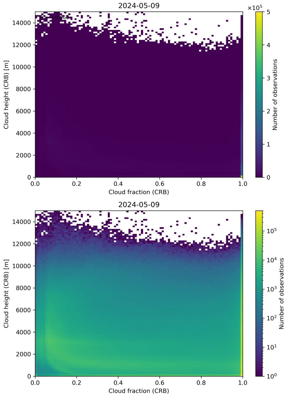
Figure 79: Scatter density plot of “Cloud fraction (CRB)” against “Cloud height (CRB)” for 2024-05-08 to 2024-05-10.
