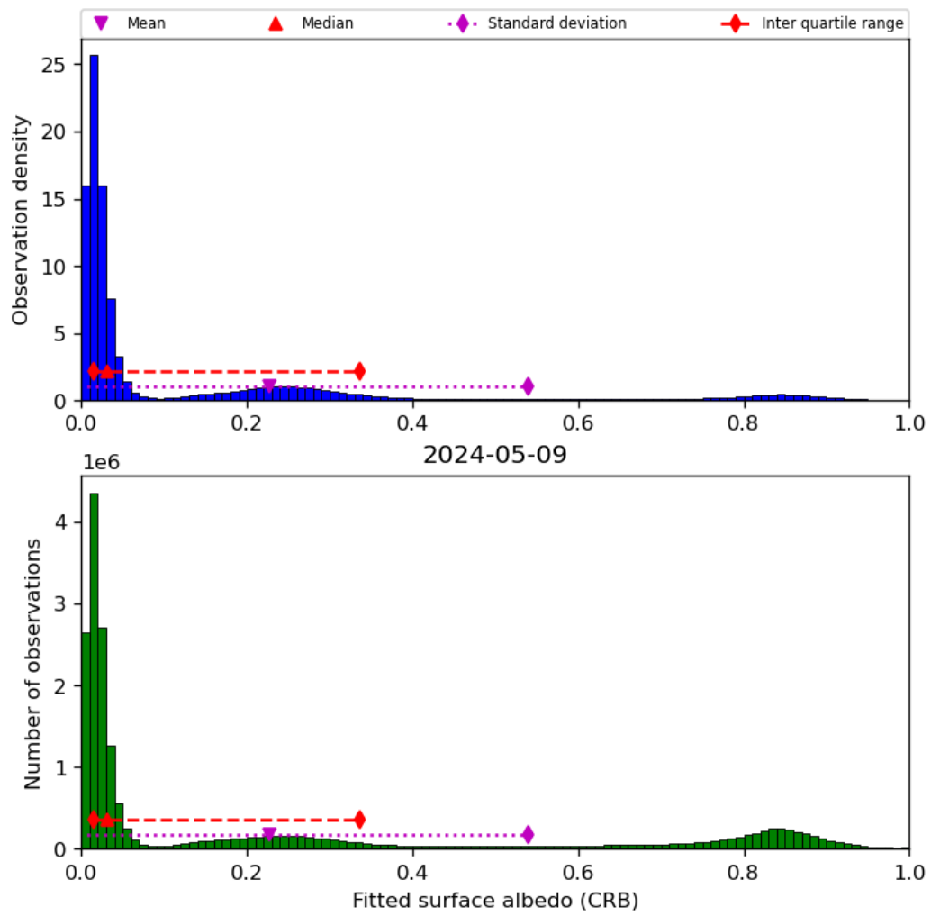
Figure 46: Histogram of “Fitted surface albedo (CRB)” for 2024-05-08 to 2024-05-10
