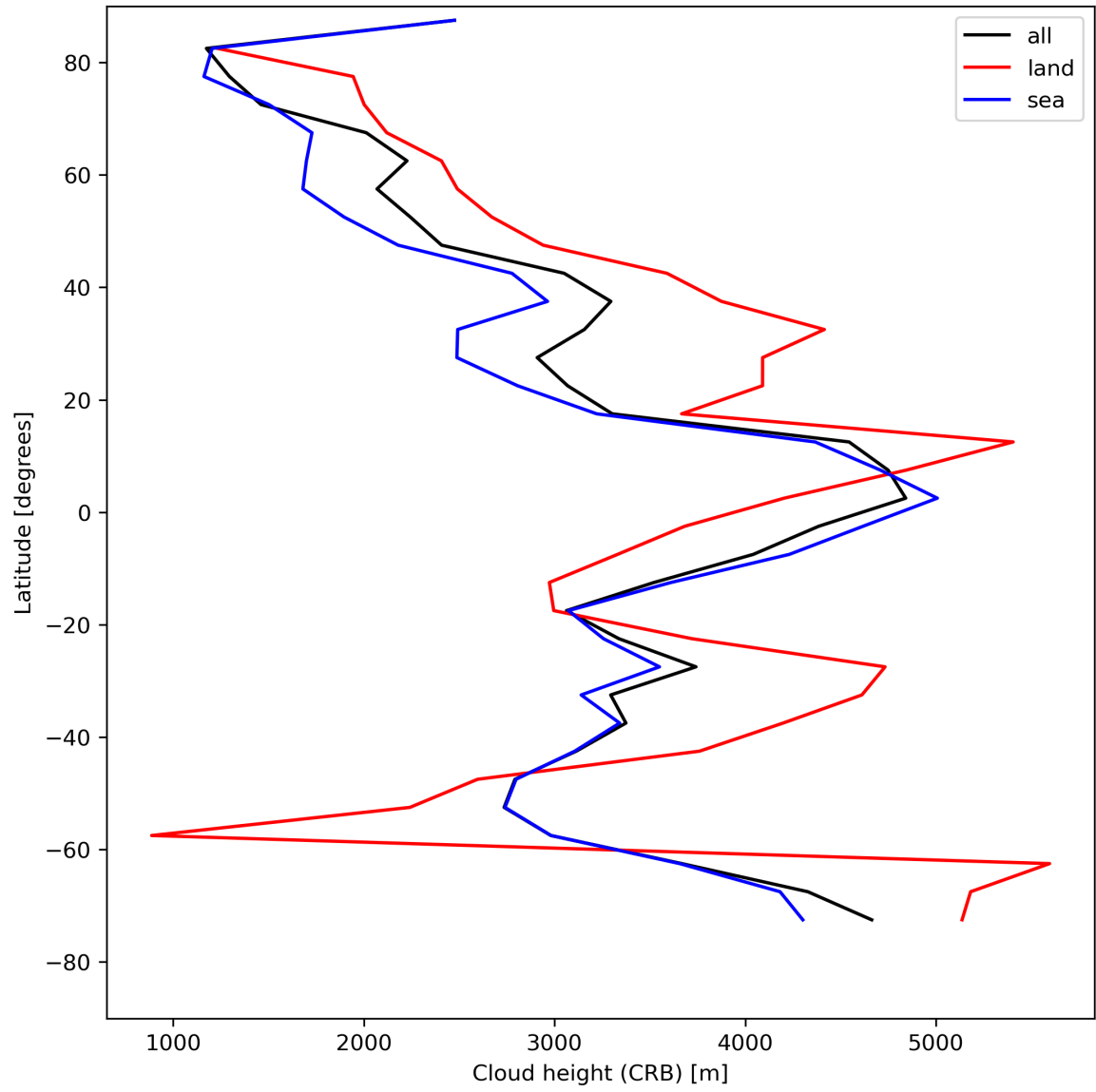
Figure 27: Zonal average of “Cloud height (CRB)” for 2024-05-08 to 2024-05-10.
