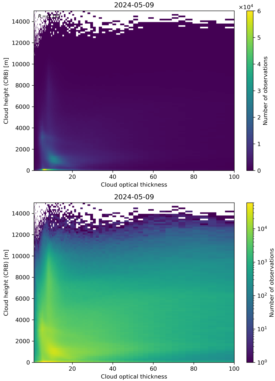
Figure 85: Scatter density plot of “Cloud optical thickness” against “Cloud height (CRB)” for 2024-05-08 to 2024-05-10.
