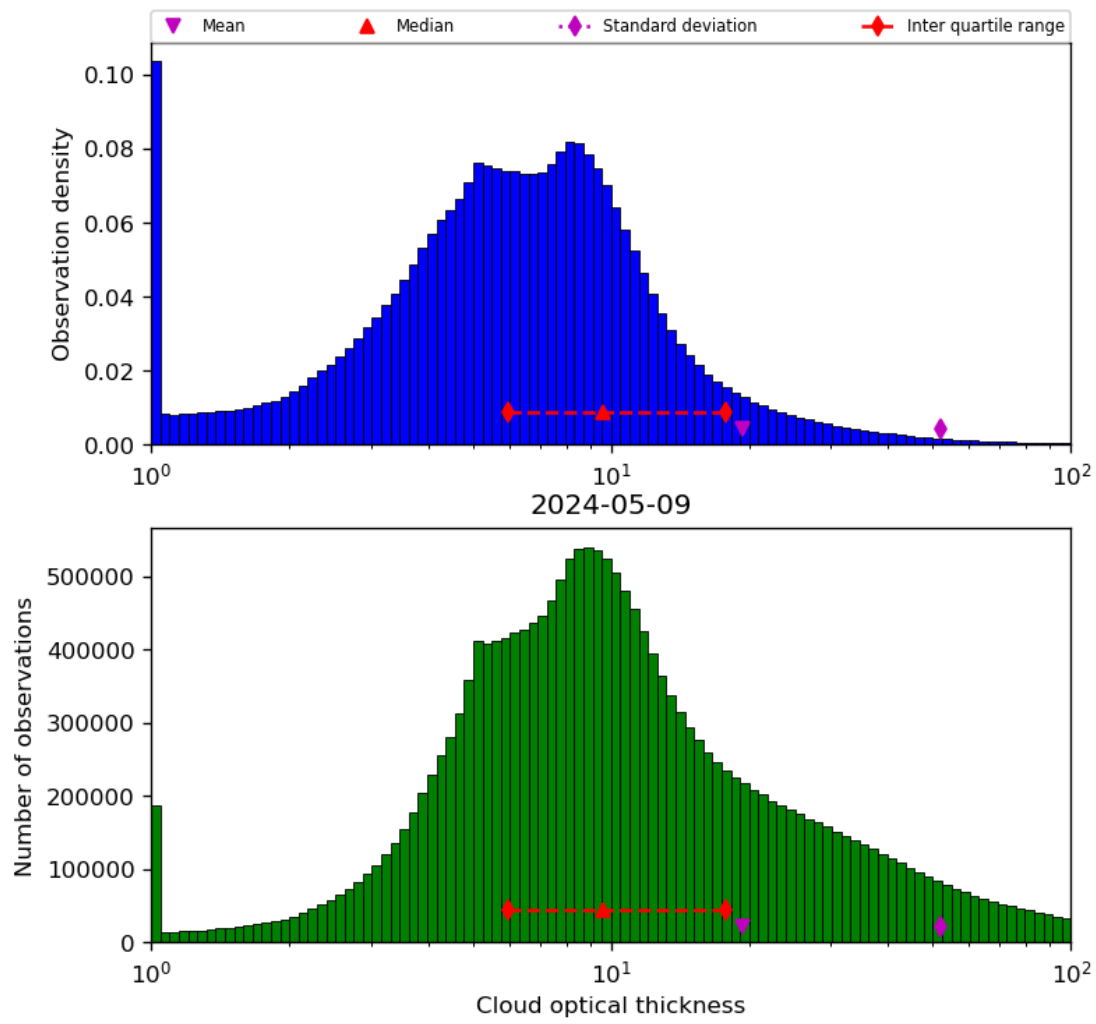
Figure 41: Histogram of “Cloud optical thickness” for 2024-05-08 to 2024-05-10
