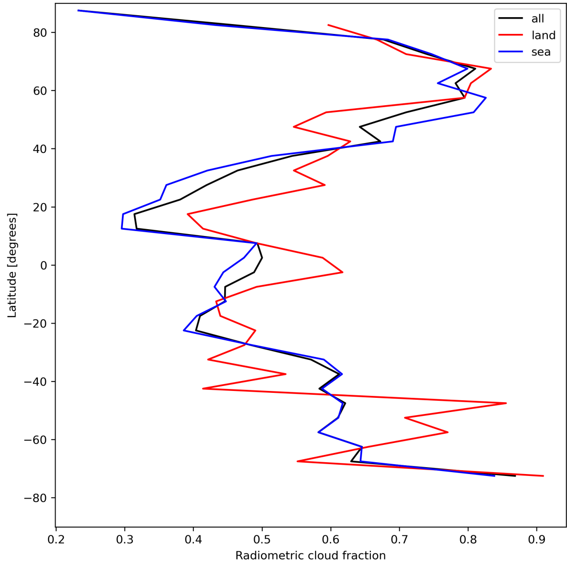
Figure 23: Zonal average of “Radiometric cloud fraction” for 2024-05-08 to 2024-05-10.
