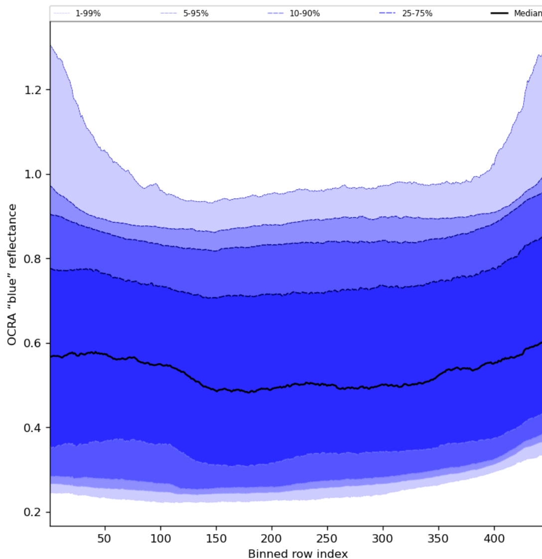
Figure 67: Along track statistics of "OCRA "blue" reflectance" for 2024-05-08 to 2024-05-10
