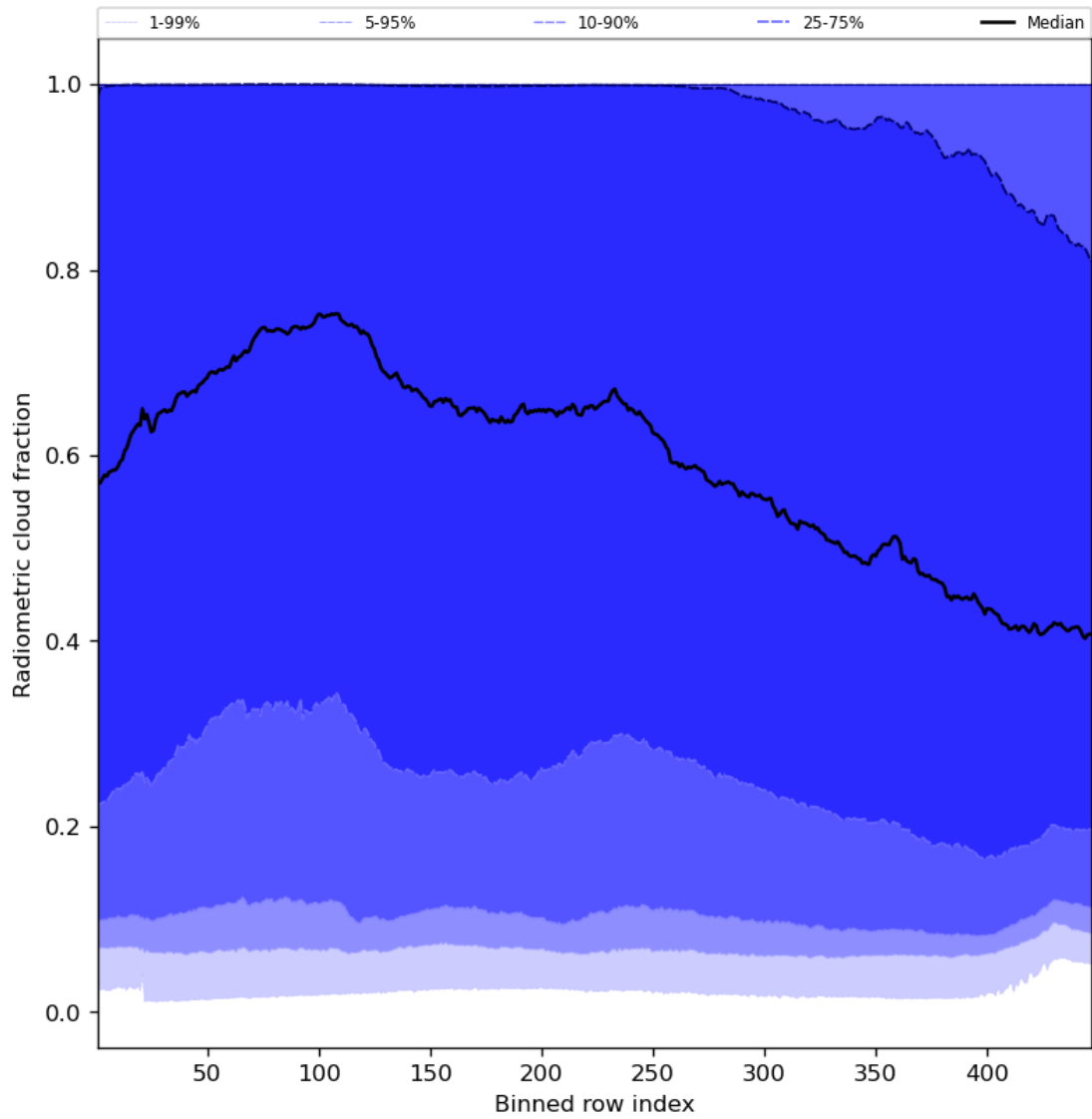
Figure 55: Along track statistics of “Radiometric cloud fraction” for 2024-05-08 to 2024-05-10
