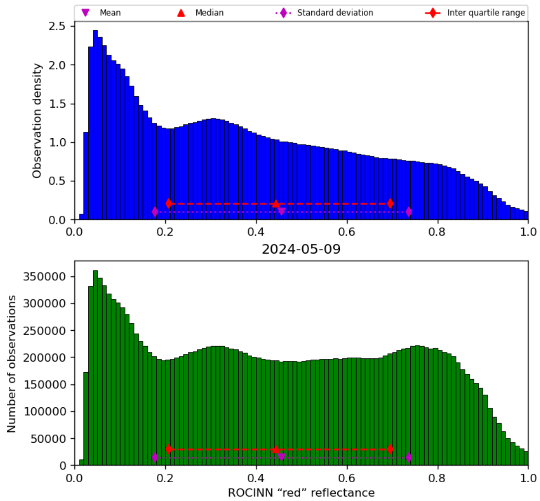
Figure 53: Histogram of “ROCINN “red” reflectance” for 2024-05-08 to 2024-05-10
