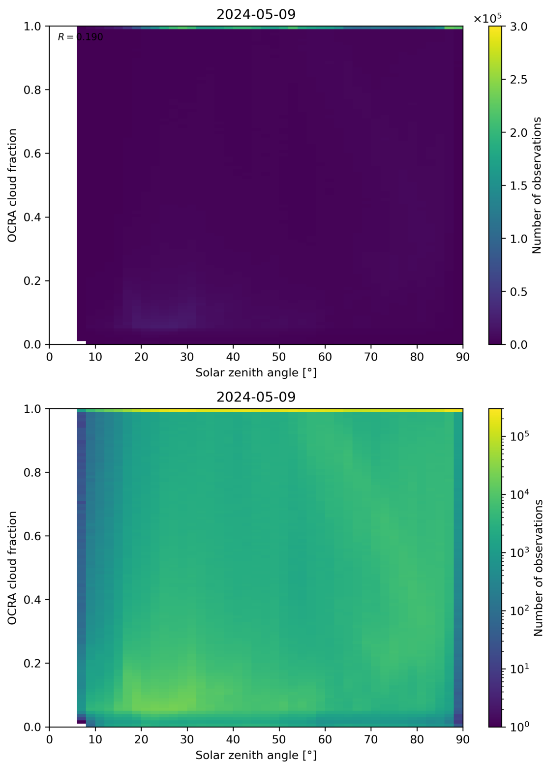
Figure 100: Scatter density plot of “Solar zenith angle” against “OCRA cloud fraction” for 2024-05-08 to 2024-05-10.
