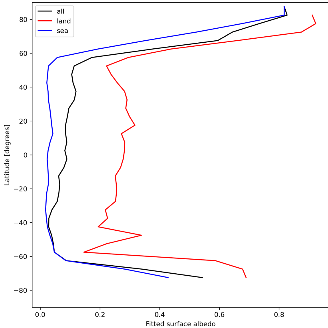
Figure 29: Zonal average of “Fitted surface albedo” for 2024-05-08 to 2024-05-10.
