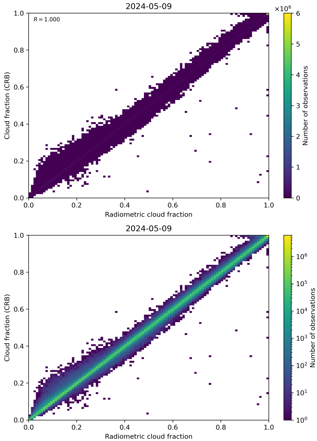
Figure 73: Scatter density plot of “Radiometric cloud fraction” against “Cloud fraction (CRB)” for 2024-05-08 to 2024-05-10.
