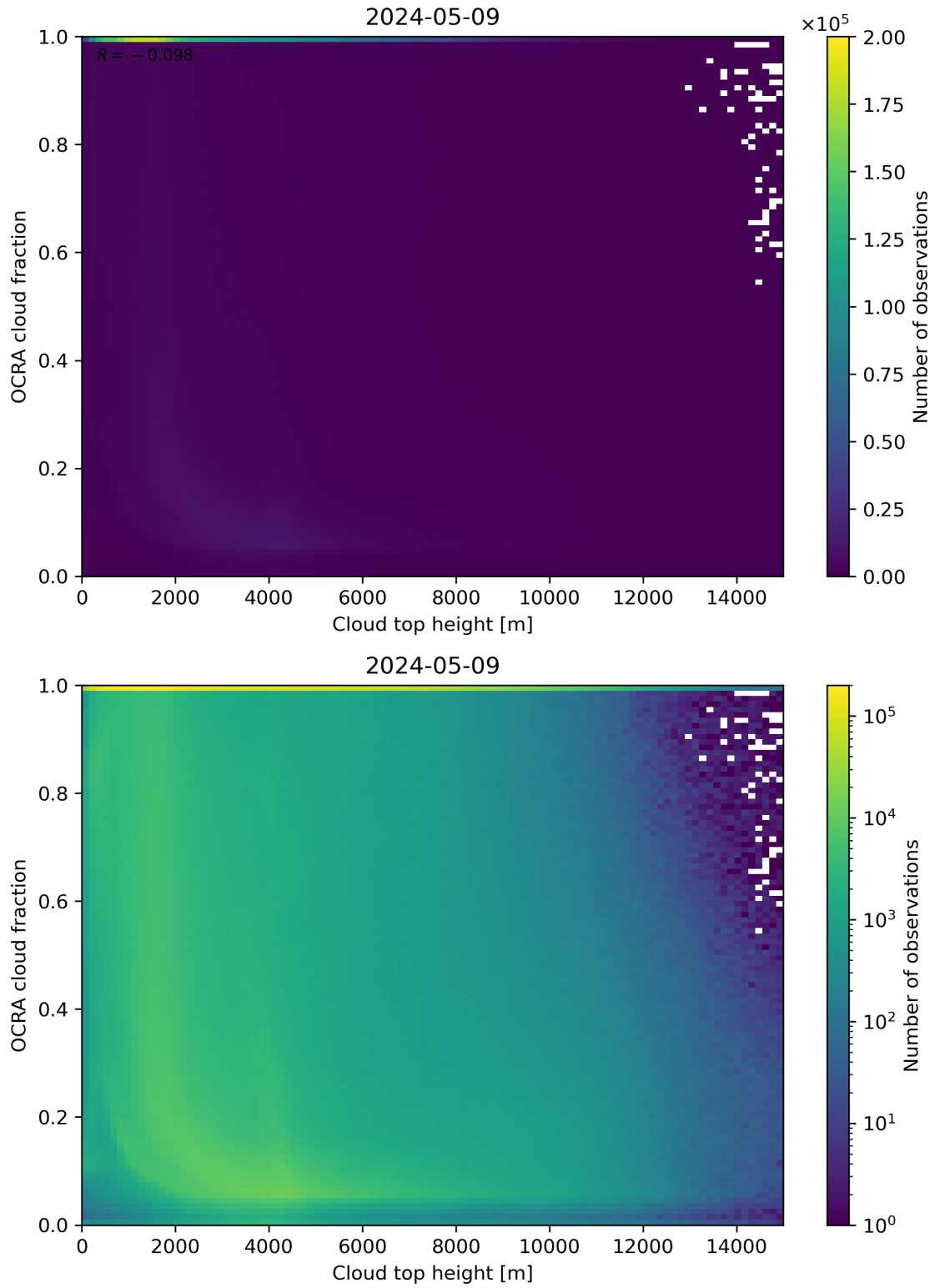
Figure 87: Scatter density plot of “Cloud top height” against “OCRA cloud fraction” for 2024-05-08 to 2024-05-10.
