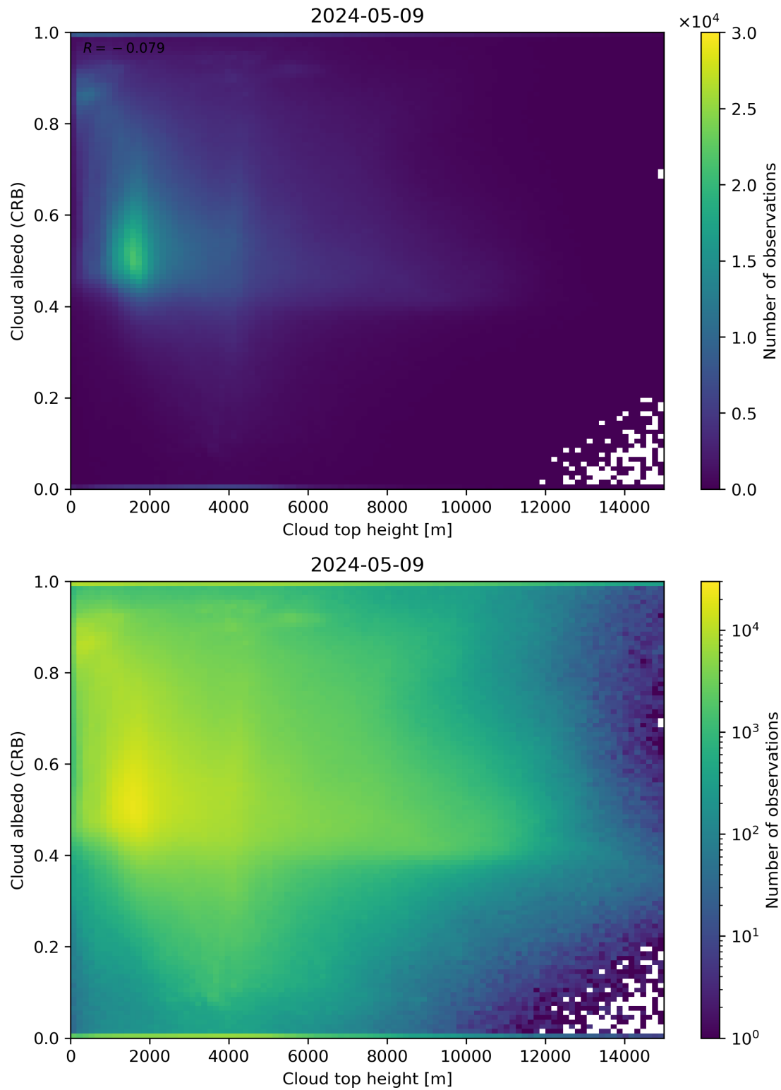
Figure 86: Scatter density plot of “Cloud top height” against “Cloud albedo (CRB)” for 2024-05-08 to 2024-05-10.
