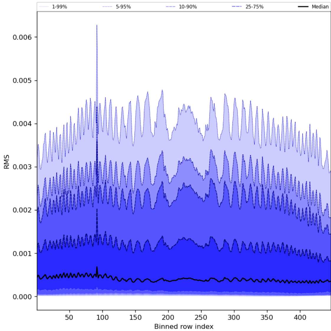
Figure 63: Along track statistics of “RMS” for 2024-05-08 to 2024-05-10
