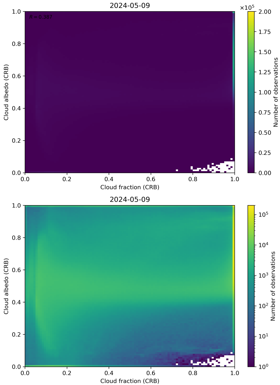
Figure 77: Scatter density plot of “Cloud fraction (CRB)” against “Cloud albedo (CRB)” for 2024-05-08 to 2024-05-10.
