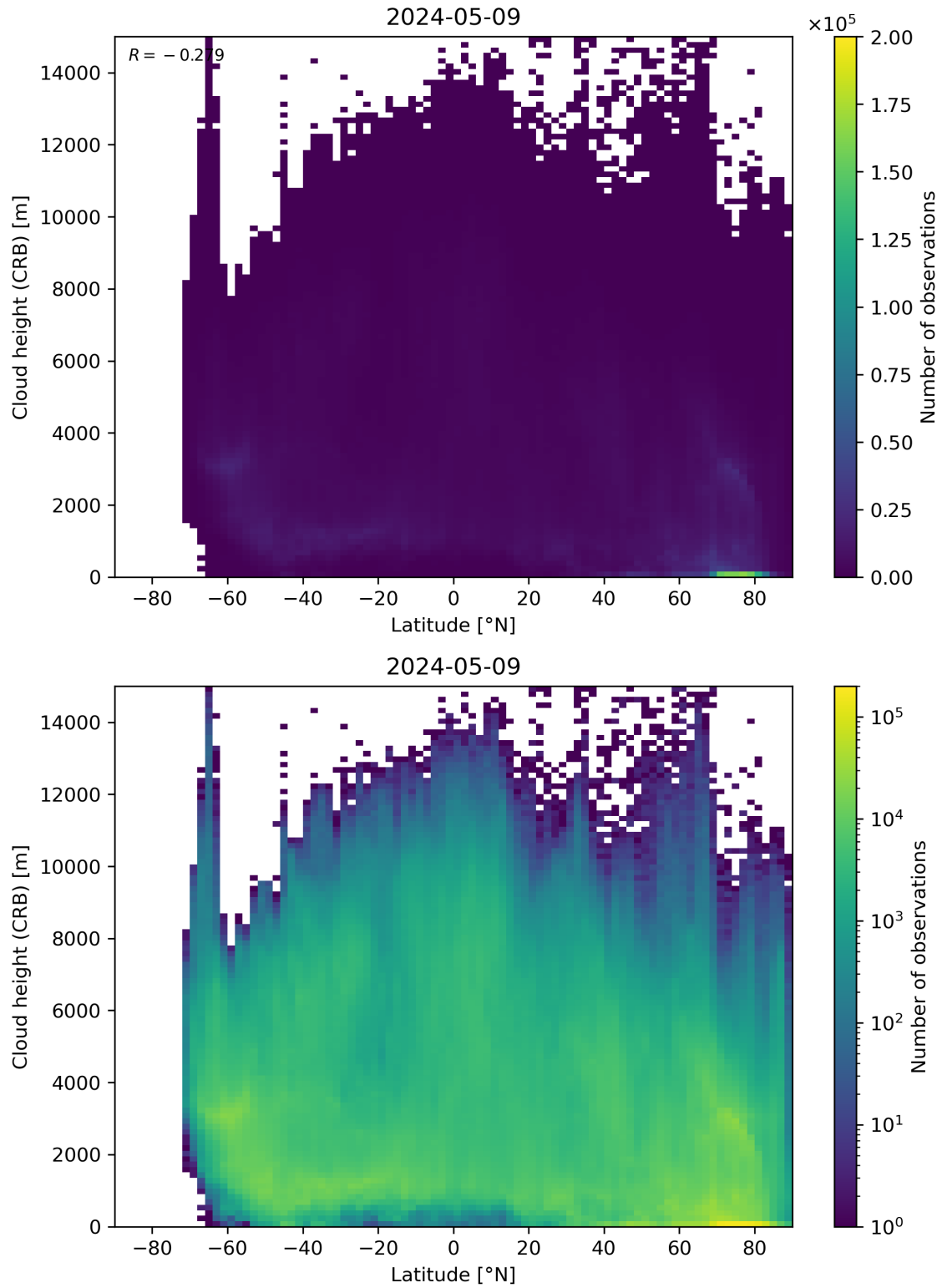
Figure 95: Scatter density plot of “Latitude” against “Cloud height (CRB)” for 2024-05-08 to 2024-05-10.
