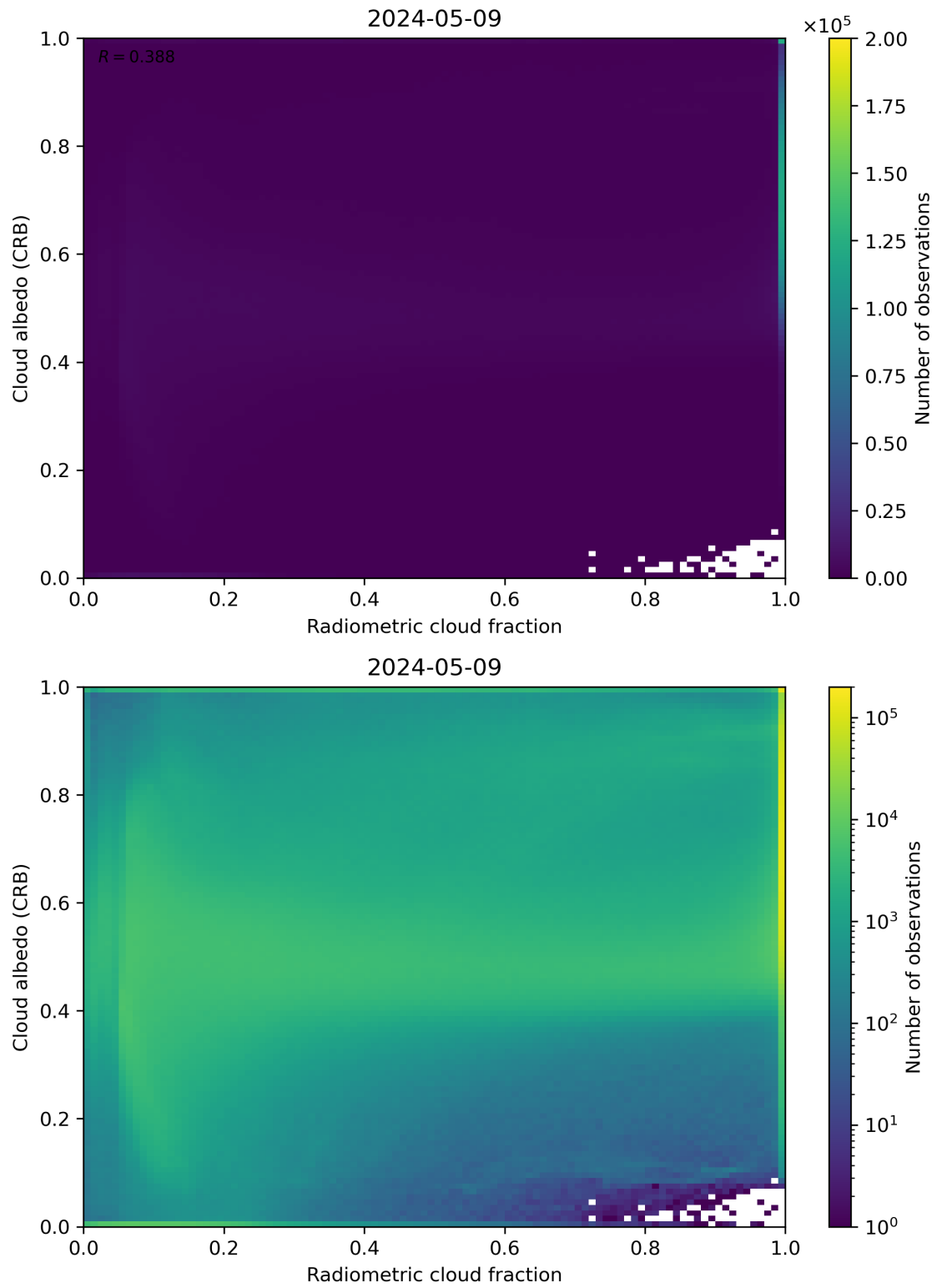
Figure 71: Scatter density plot of “Radiometric cloud fraction” against “Cloud albedo (CRB)” for 2024-05-08 to 2024-05-10.
