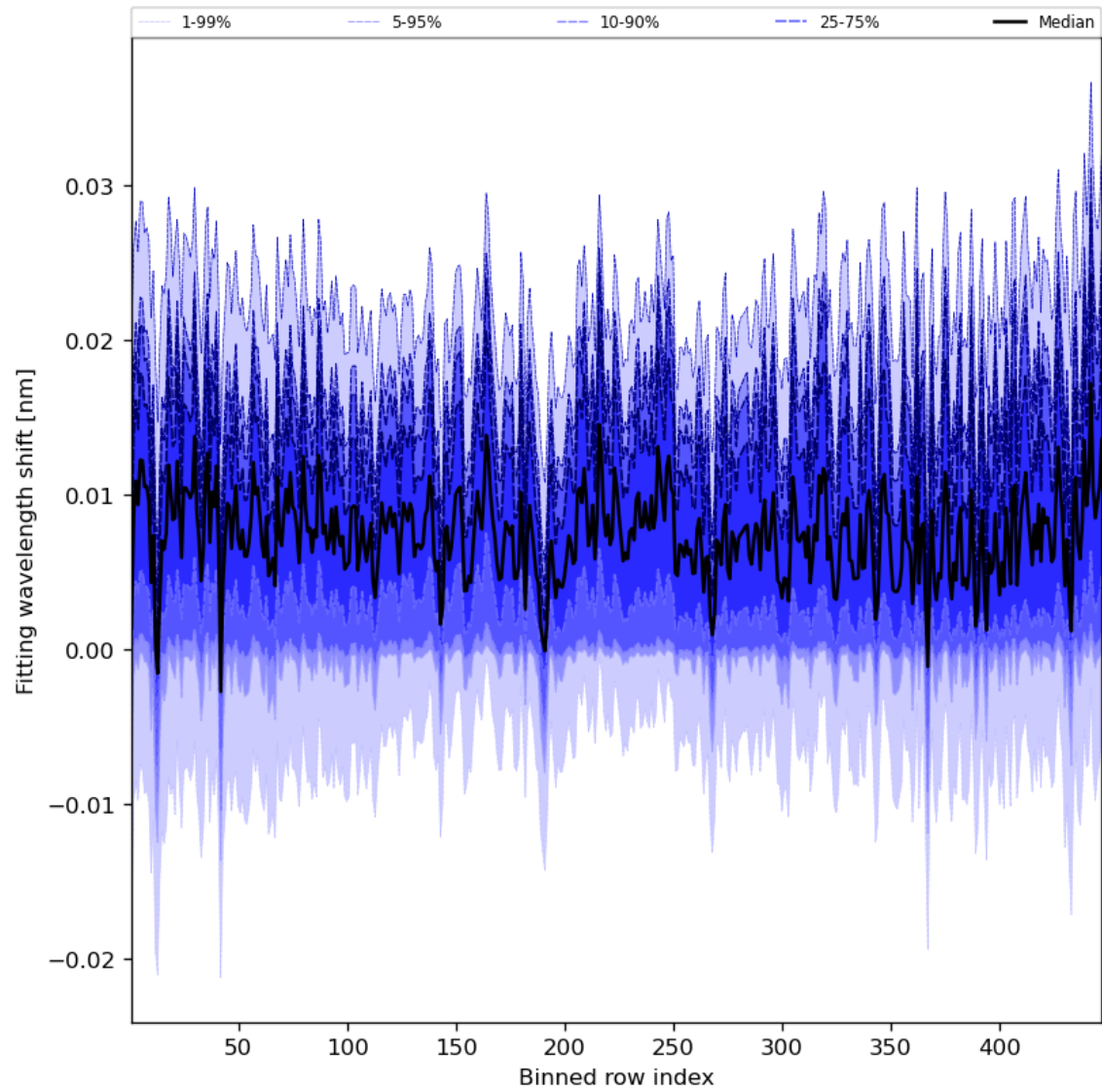
Figure 65: Along track statistics of “Fitting wavelength shift” for 2024-05-08 to 2024-05-10
