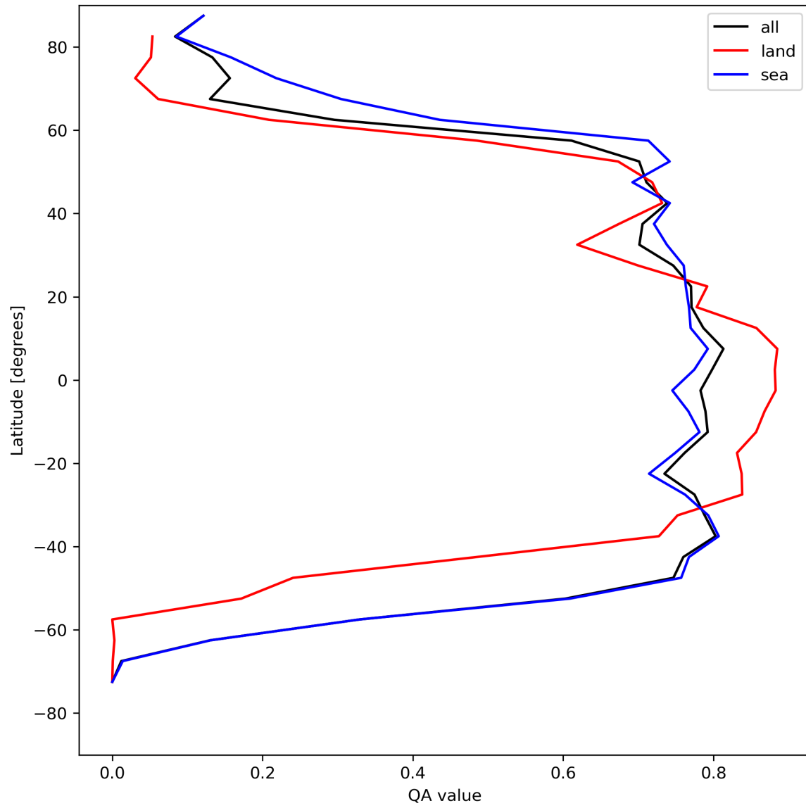
Figure 22: Zonal average of “QA value” for 2024-05-08 to 2024-05-10.
