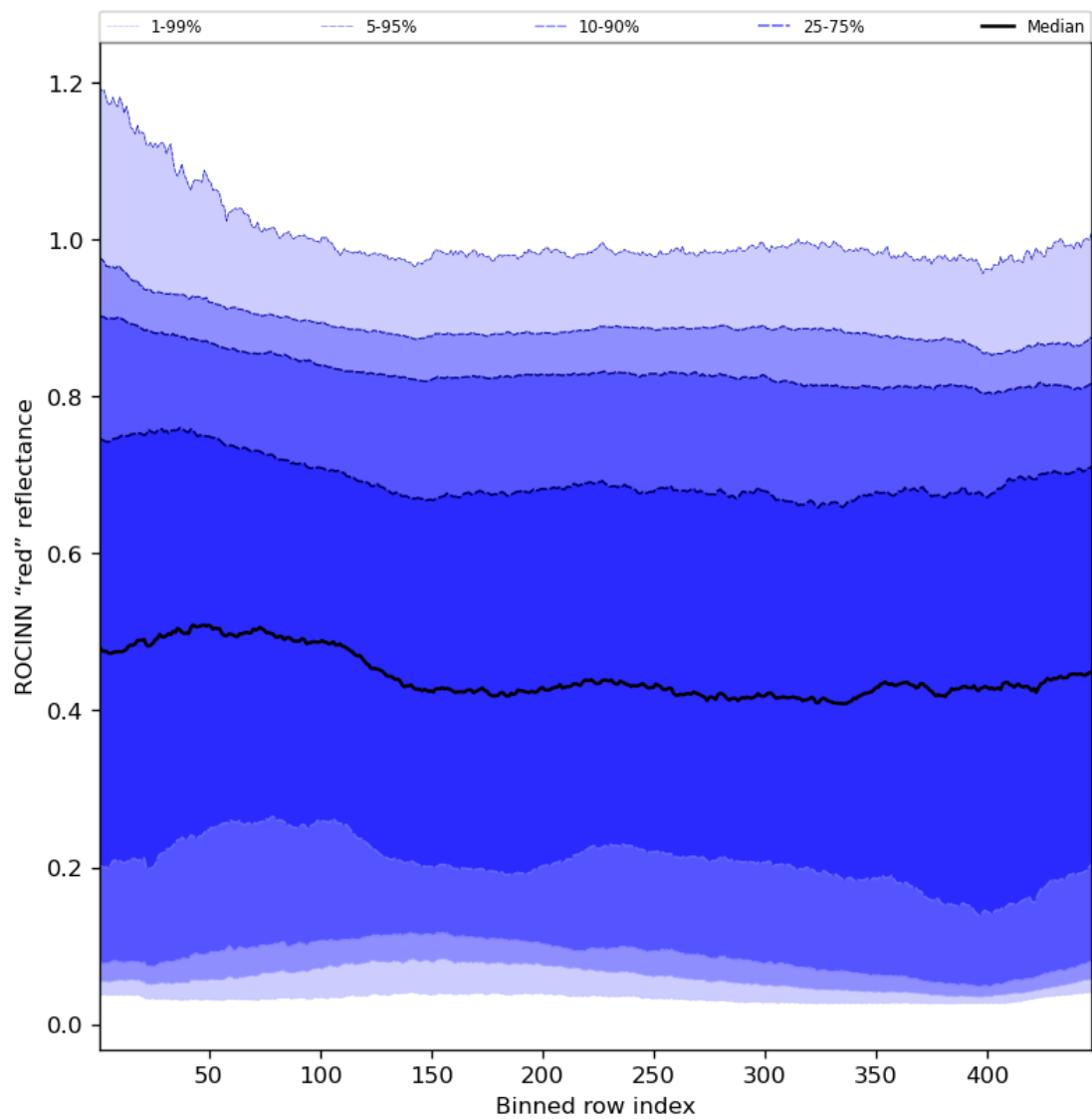
Figure 69: Along track statistics of “ROCINN “red” reflectance” for 2024-05-08 to 2024-05-10
