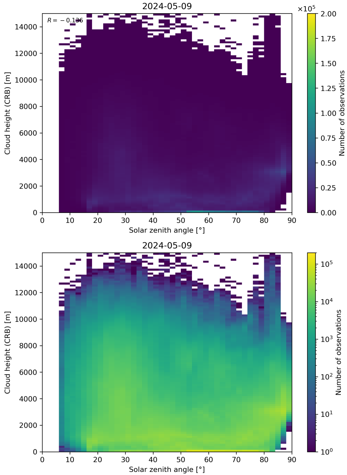
Figure 102: Scatter density plot of “Solar zenith angle” against “Cloud height (CRB)” for 2024-05-08 to 2024-05-10.
