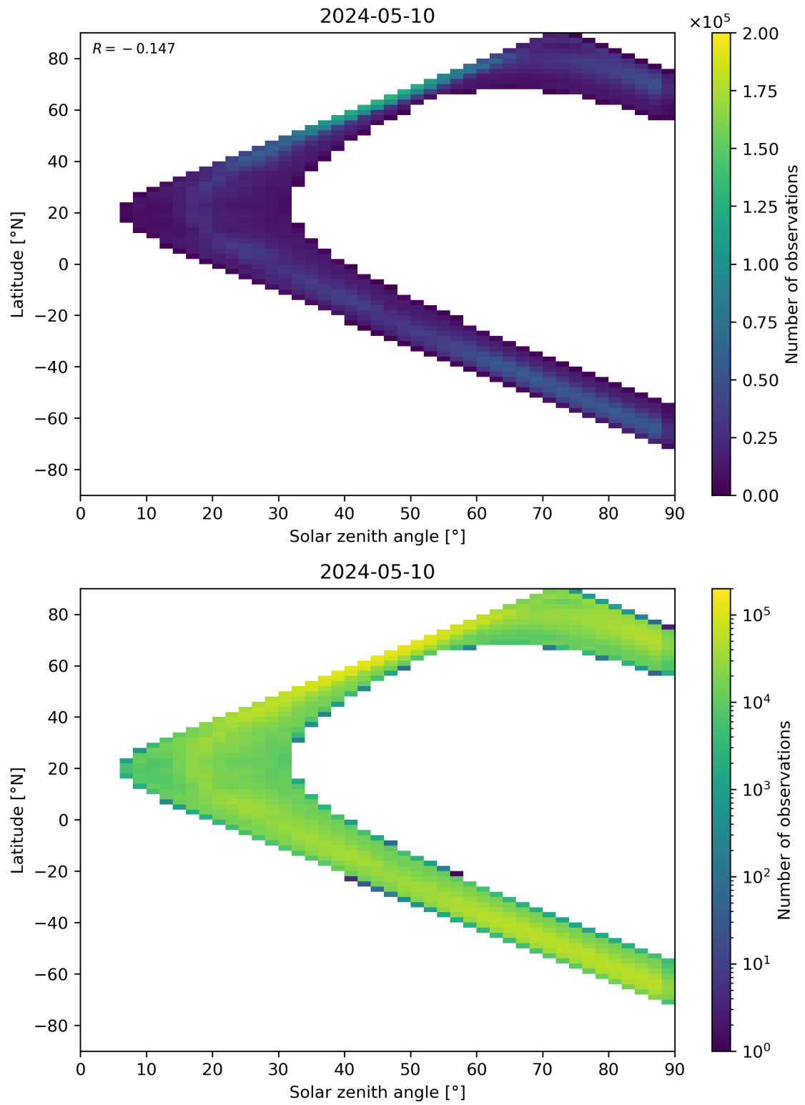
Figure 105: Scatter density plot of “Solar zenith angle” against “Latitude” for 2024-05-09 to 2024-05-11.
