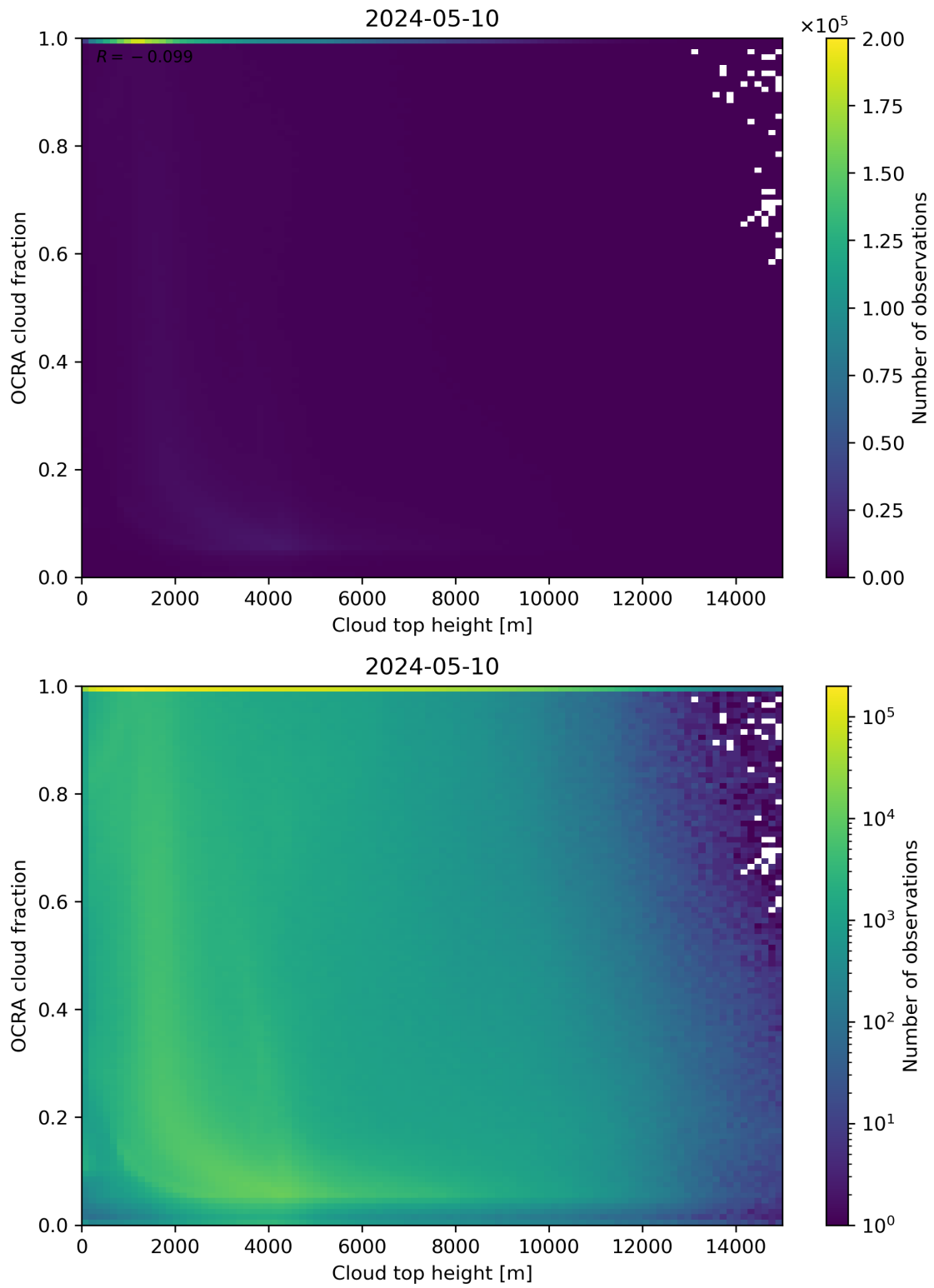
Figure 87: Scatter density plot of “Cloud top height” against “OCRA cloud fraction” for 2024-05-09 to 2024-05-11.
