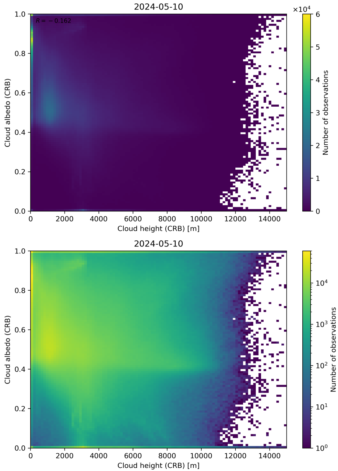
Figure 80: Scatter density plot of “Cloud height (CRB)” against “Cloud albedo (CRB)” for 2024-05-09 to 2024-05-11.
