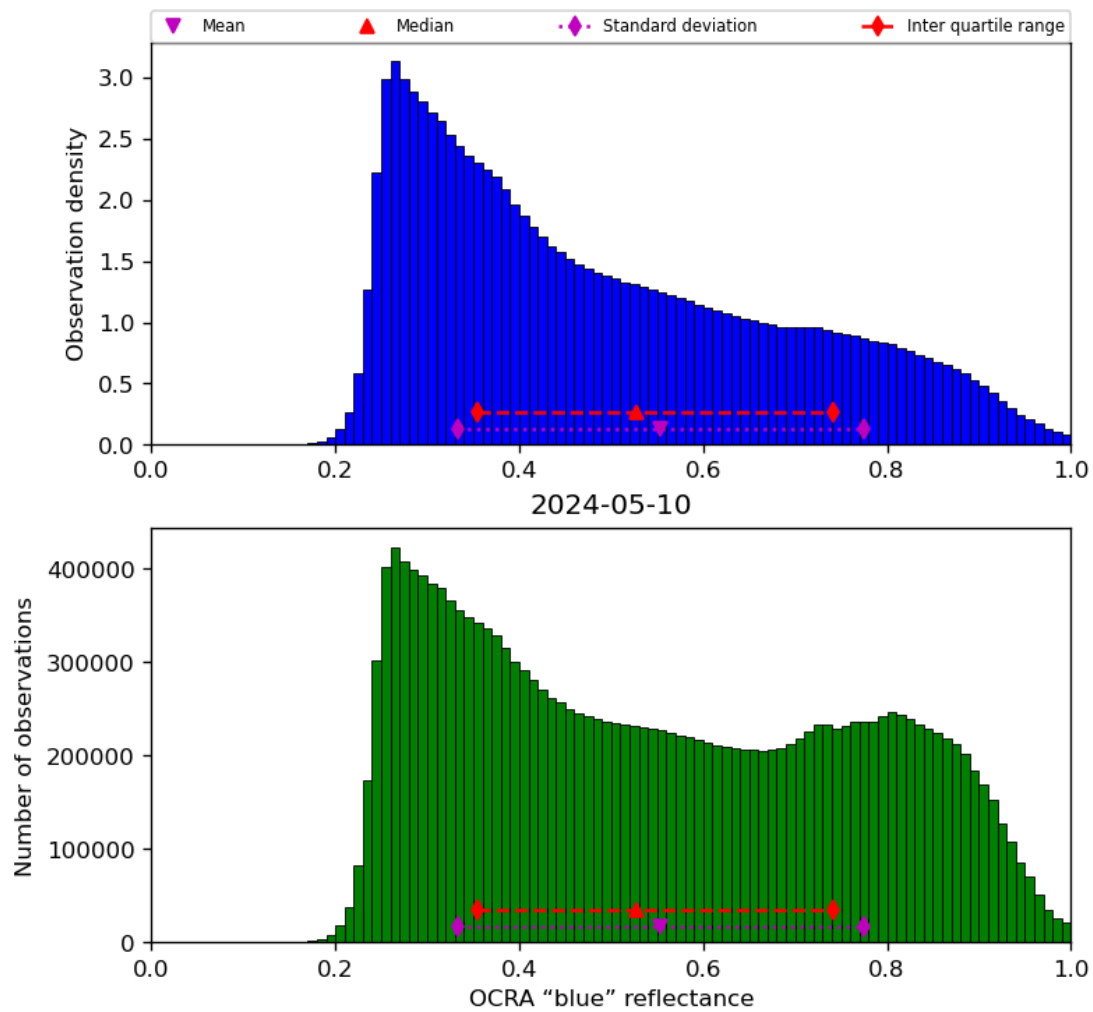
Figure 51: Histogram of “OCRA “blue” reflectance” for 2024-05-09 to 2024-05-11
