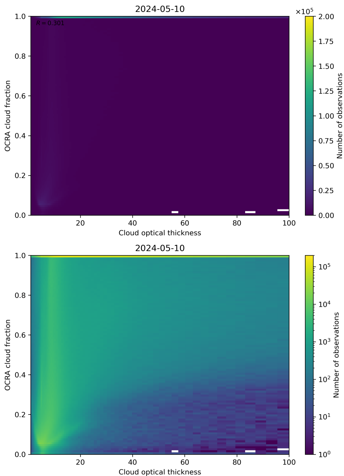
Figure 83: Scatter density plot of “Cloud optical thickness” against “OCRA cloud fraction” for 2024-05-09 to 2024-05-11.
