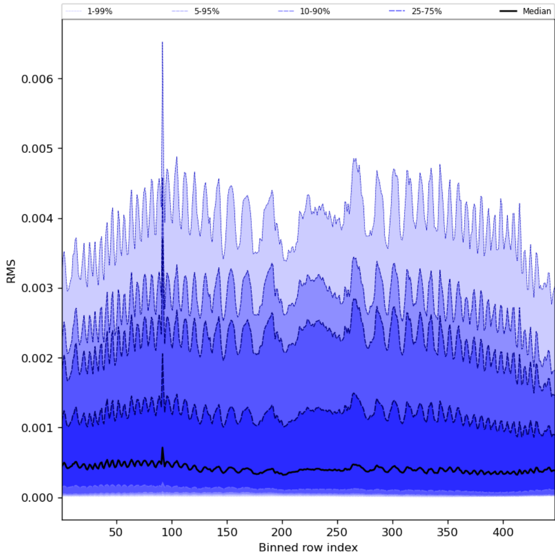
Figure 63: Along track statistics of “RMS” for 2024-05-09 to 2024-05-11
