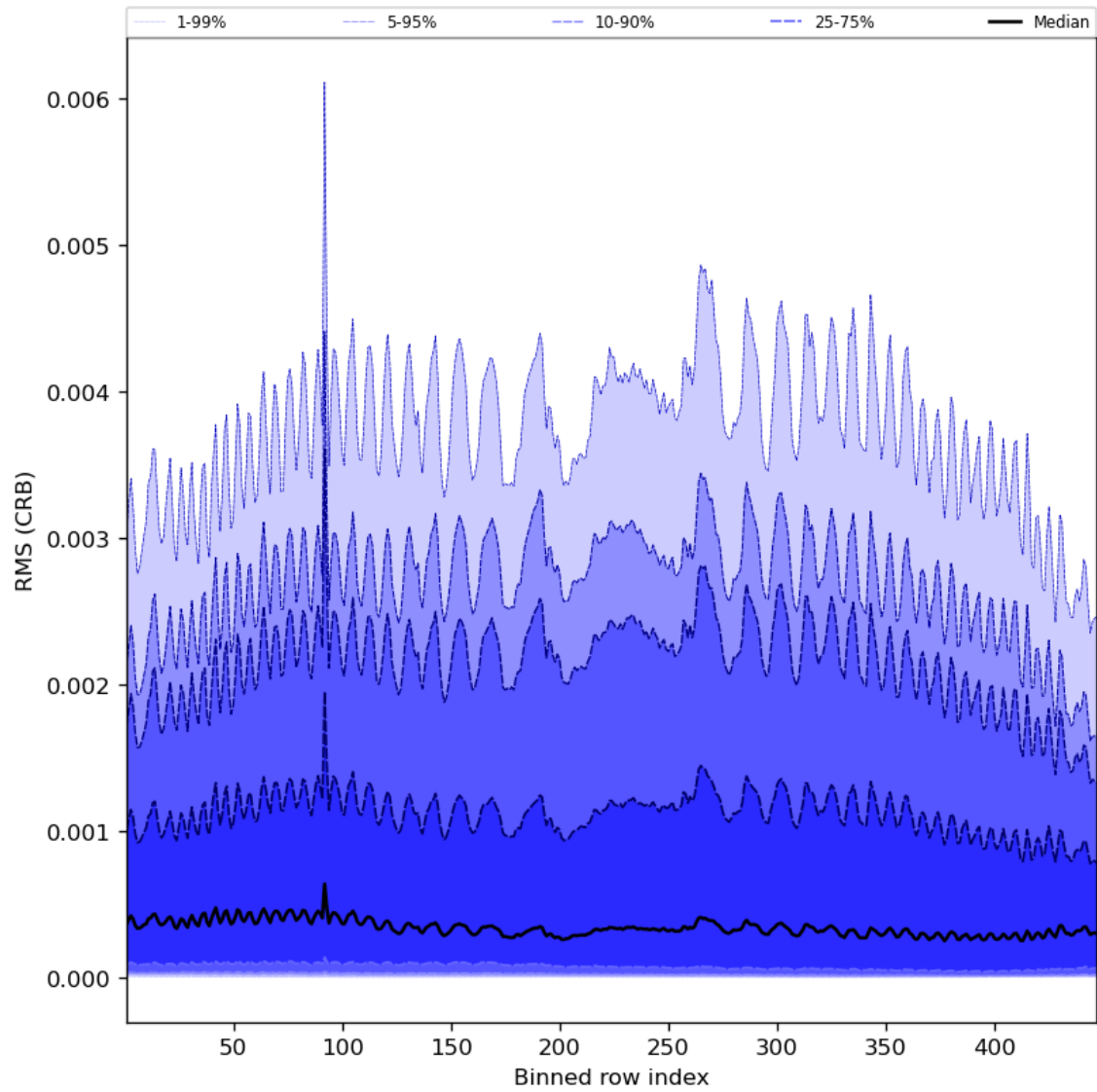
Figure 64: Along track statistics of “RMS (CRB)” for 2024-05-09 to 2024-05-11
