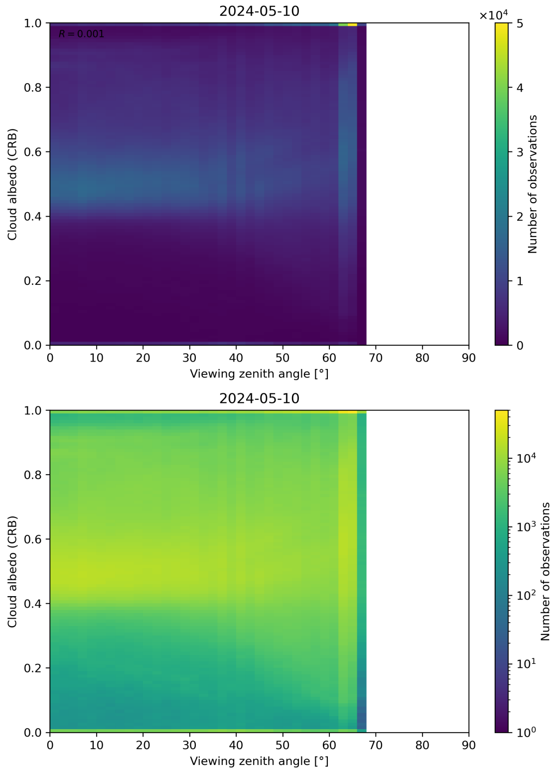
Figure 106: Scatter density plot of “Viewing zenith angle” against “Cloud albedo (CRB)” for 2024-05-09 to 2024-05-11.
