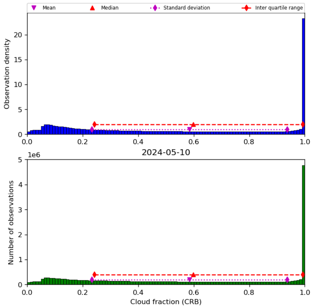
Figure 42: Histogram of “Cloud fraction (CRB)” for 2024-05-09 to 2024-05-11
