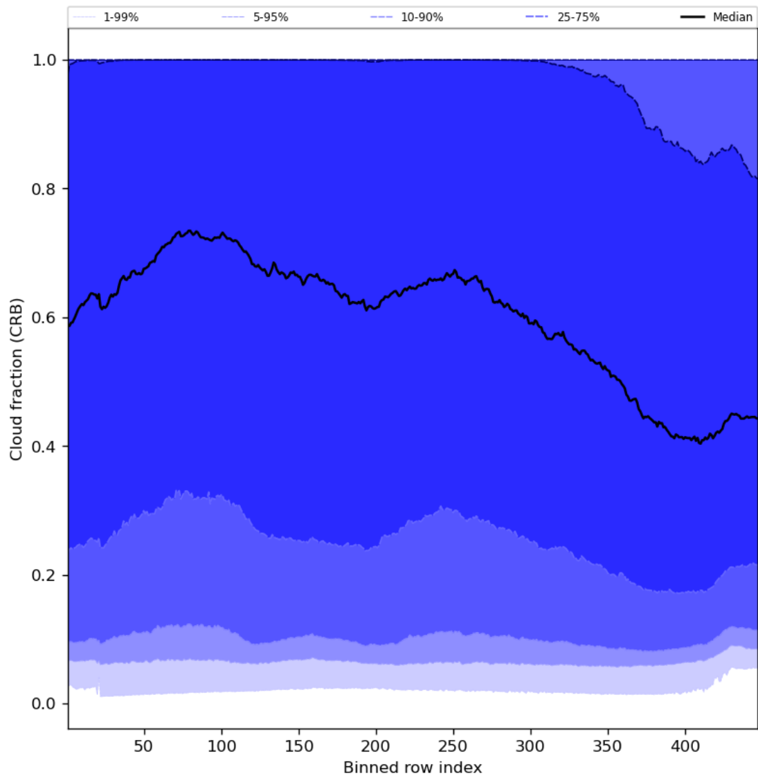
Figure 58: Along track statistics of “Cloud fraction (CRB)” for 2024-05-09 to 2024-05-11
