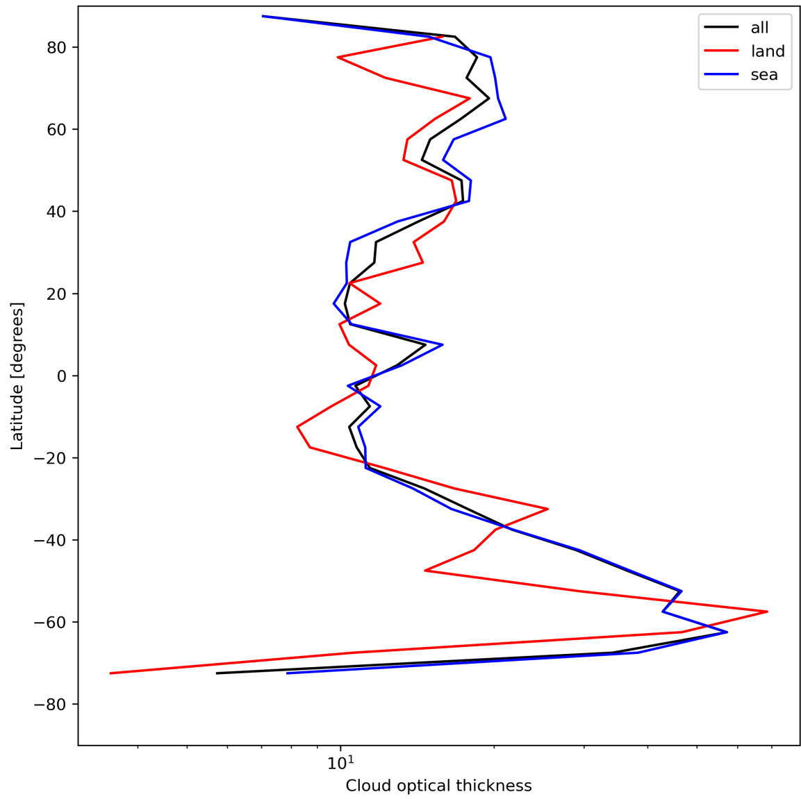
Figure 25: Zonal average of “Cloud optical thickness” for 2024-05-09 to 2024-05-11.
