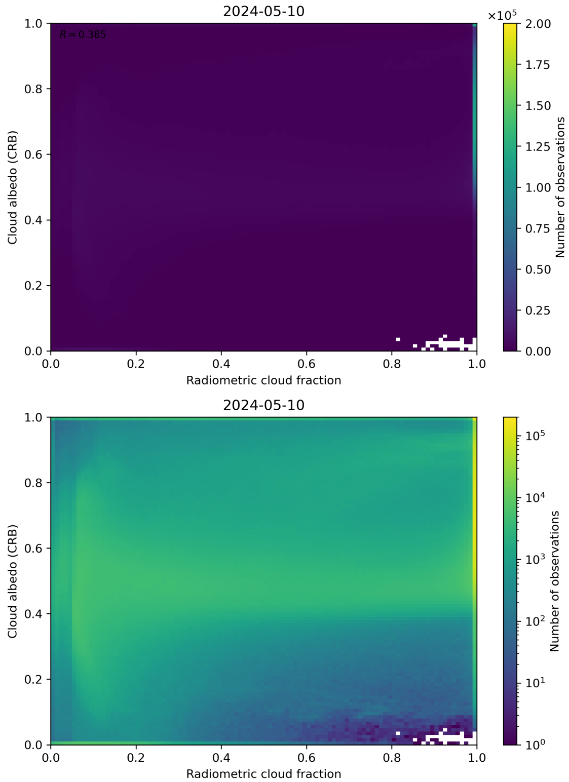
Figure 71: Scatter density plot of “Radiometric cloud fraction” against “Cloud albedo (CRB)” for 2024-05-09 to 2024-05-11.
