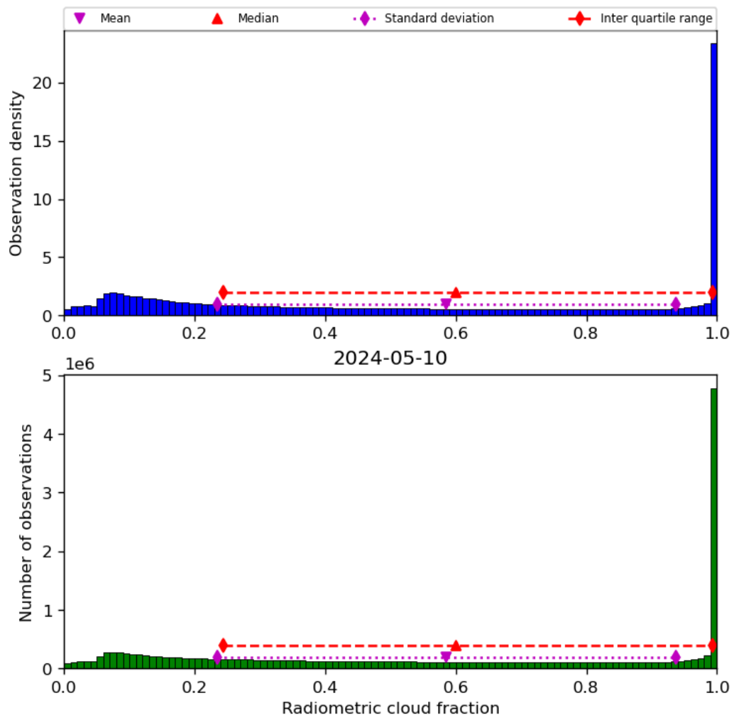
Figure 39: Histogram of “Radiometric cloud fraction” for 2024-05-09 to 2024-05-11
