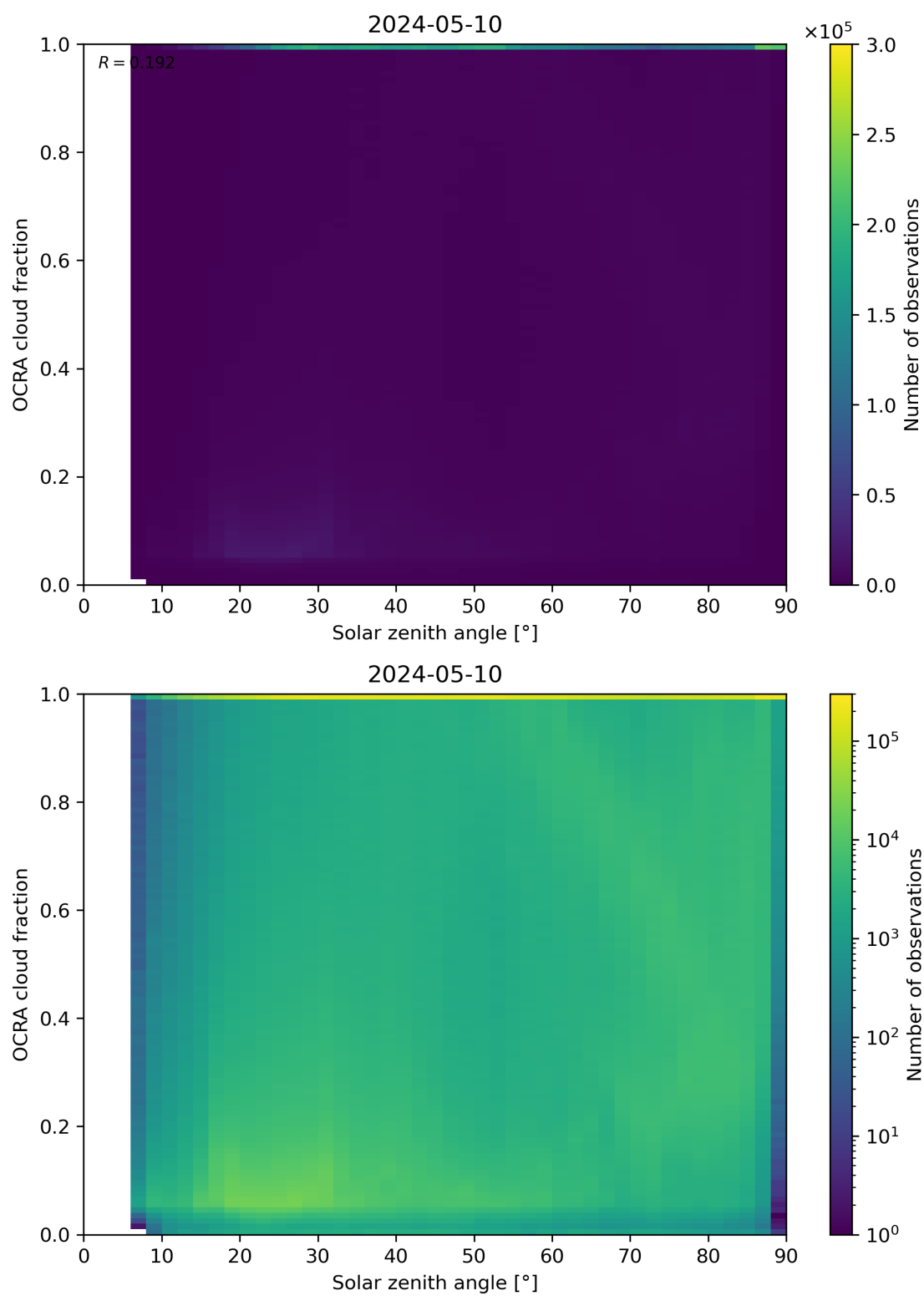
Figure 100: Scatter density plot of “Solar zenith angle” against “OCRA cloud fraction” for 2024-05-09 to 2024-05-11.
