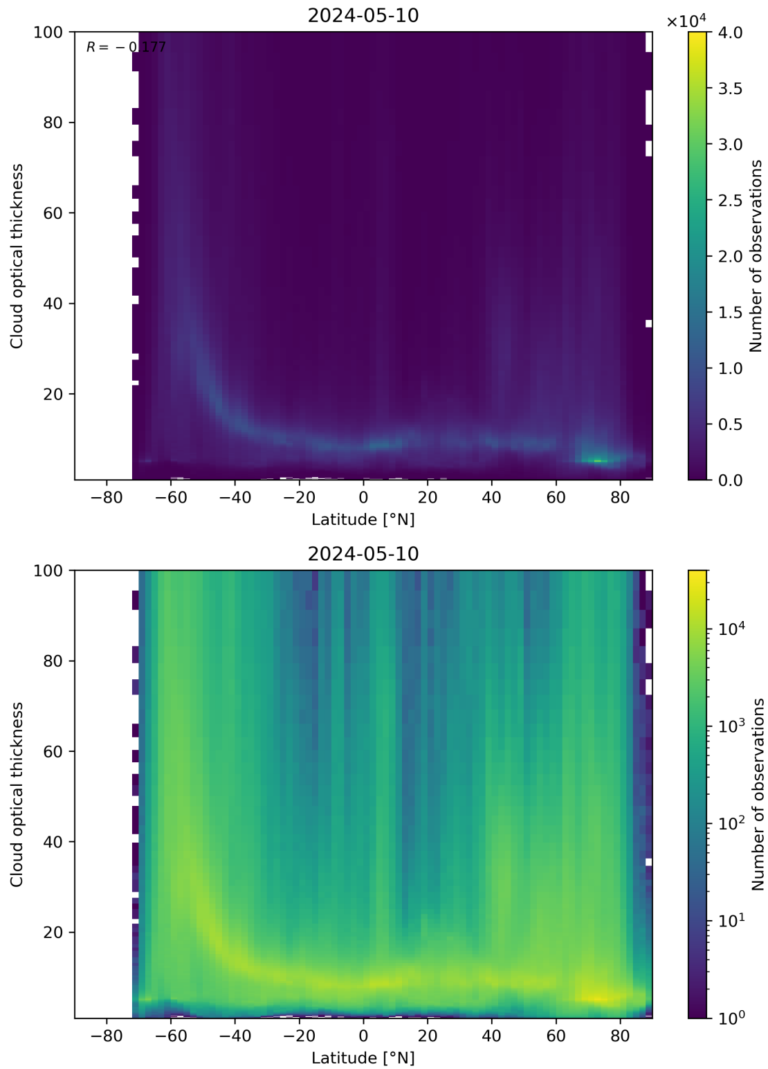
Figure 96: Scatter density plot of “Latitude” against “Cloud optical thickness” for 2024-05-09 to 2024-05-11.
