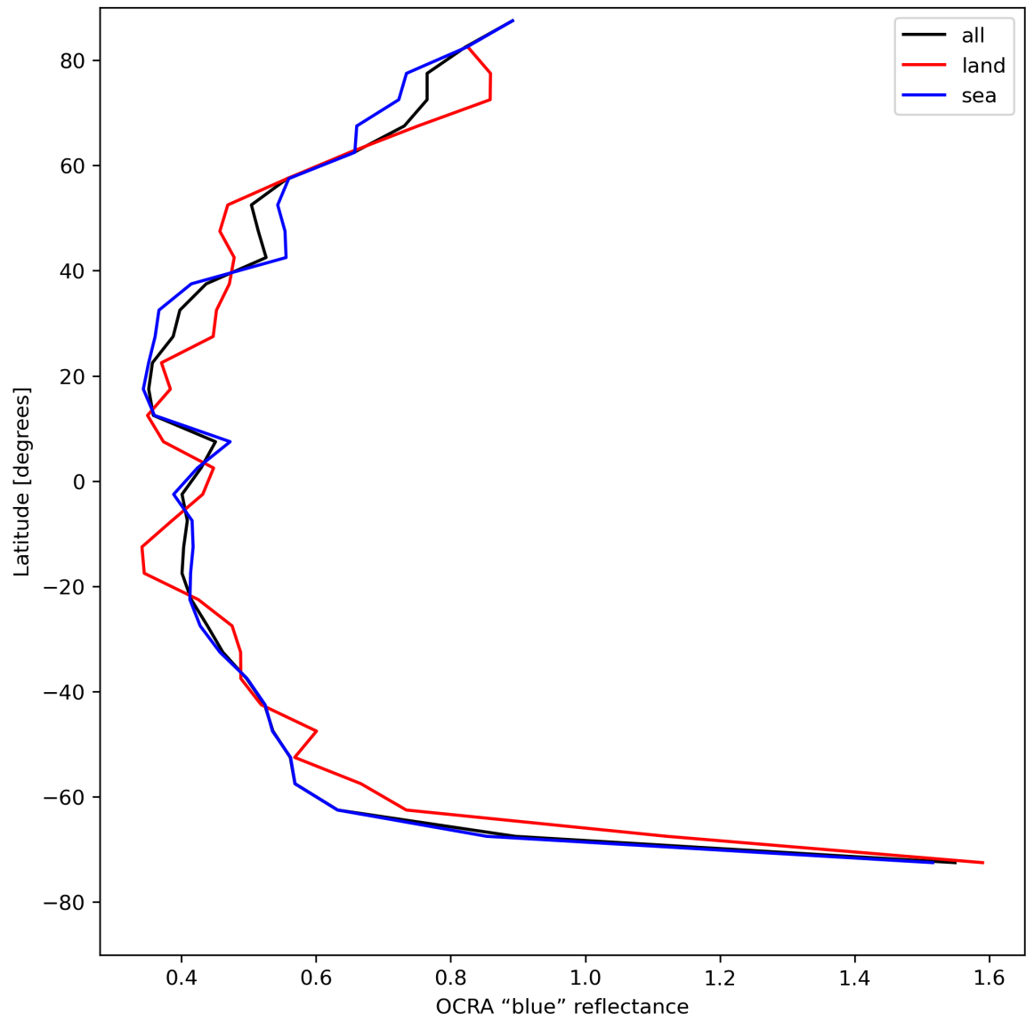
Figure 35: Zonal average of “OCRA “blue” reflectance” for 2024-05-09 to 2024-05-11.
