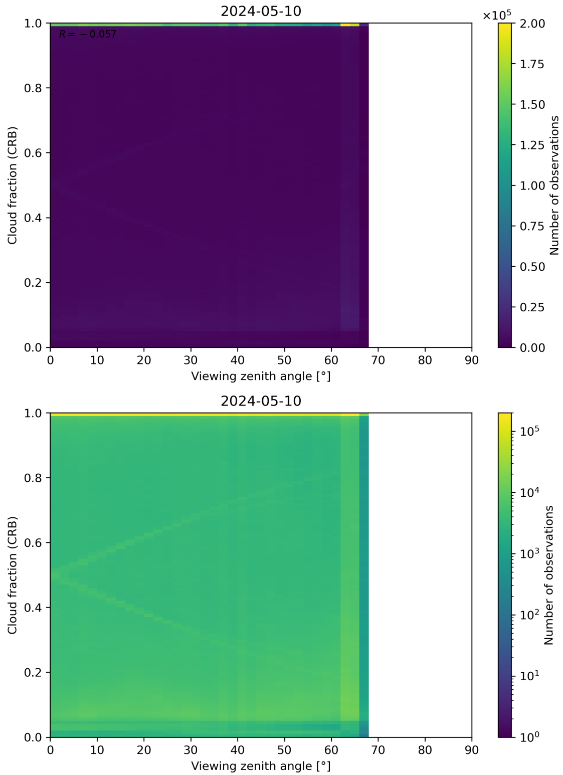
Figure 109: Scatter density plot of “Viewing zenith angle” against “Cloud fraction (CRB)” for 2024-05-09 to 2024-05-11.
