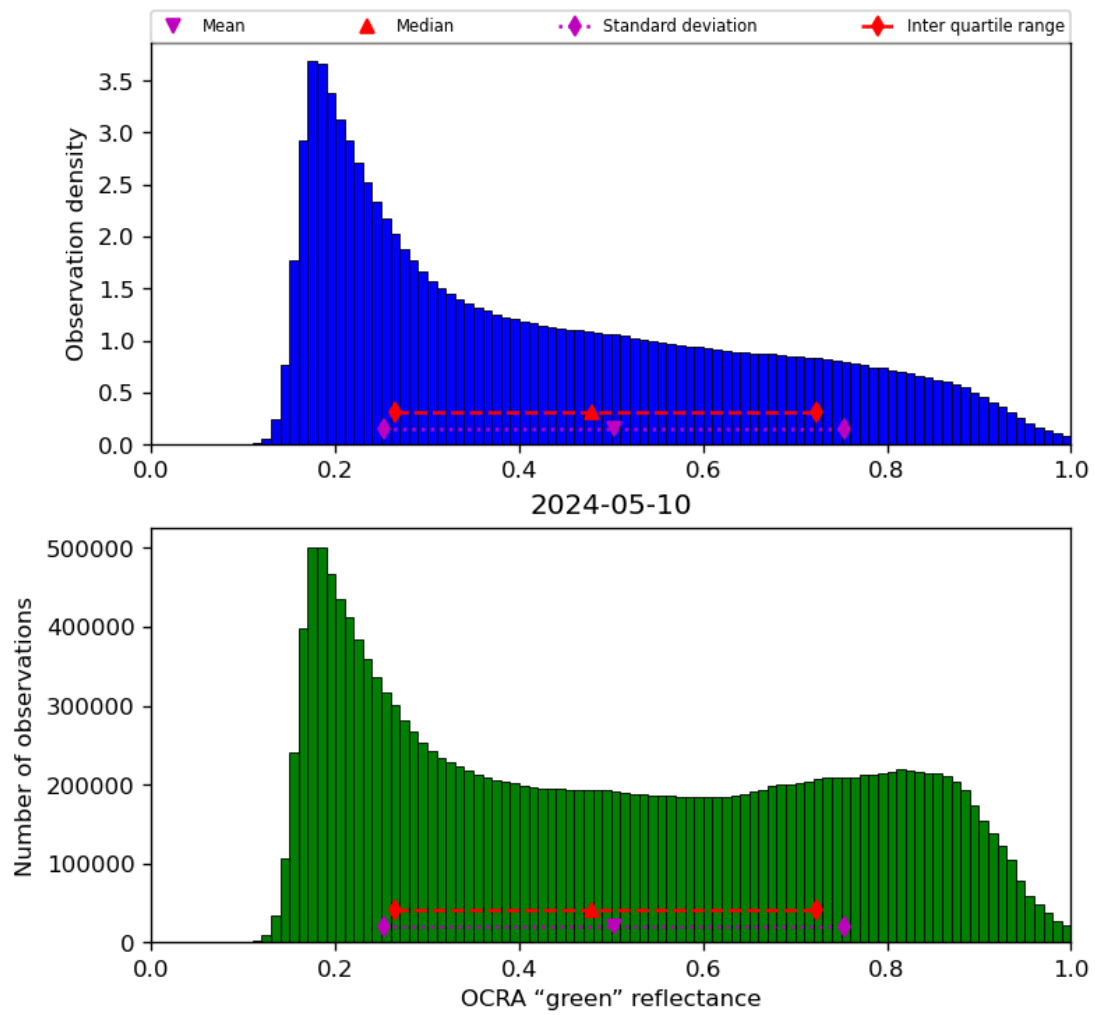
Figure 52: Histogram of “OCRA “green” reflectance” for 2024-05-09 to 2024-05-11
