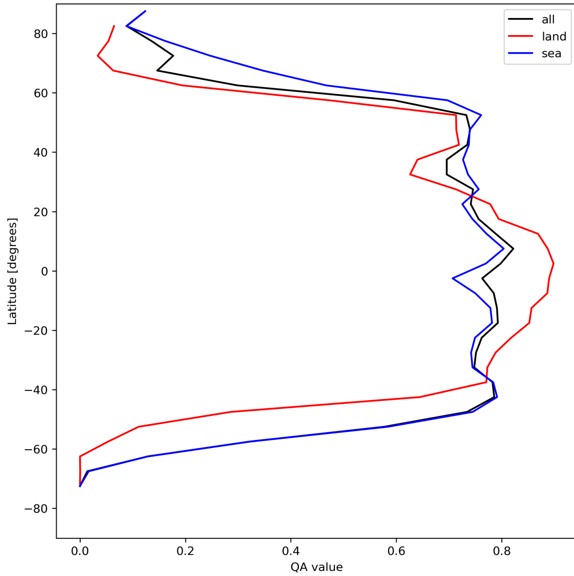
Figure 22: Zonal average of “QA value” for 2024-05-09 to 2024-05-11.
