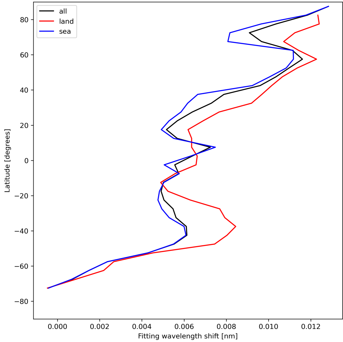
Figure 33: Zonal average of “Fitting wavelength shift” for 2024-05-09 to 2024-05-11.
