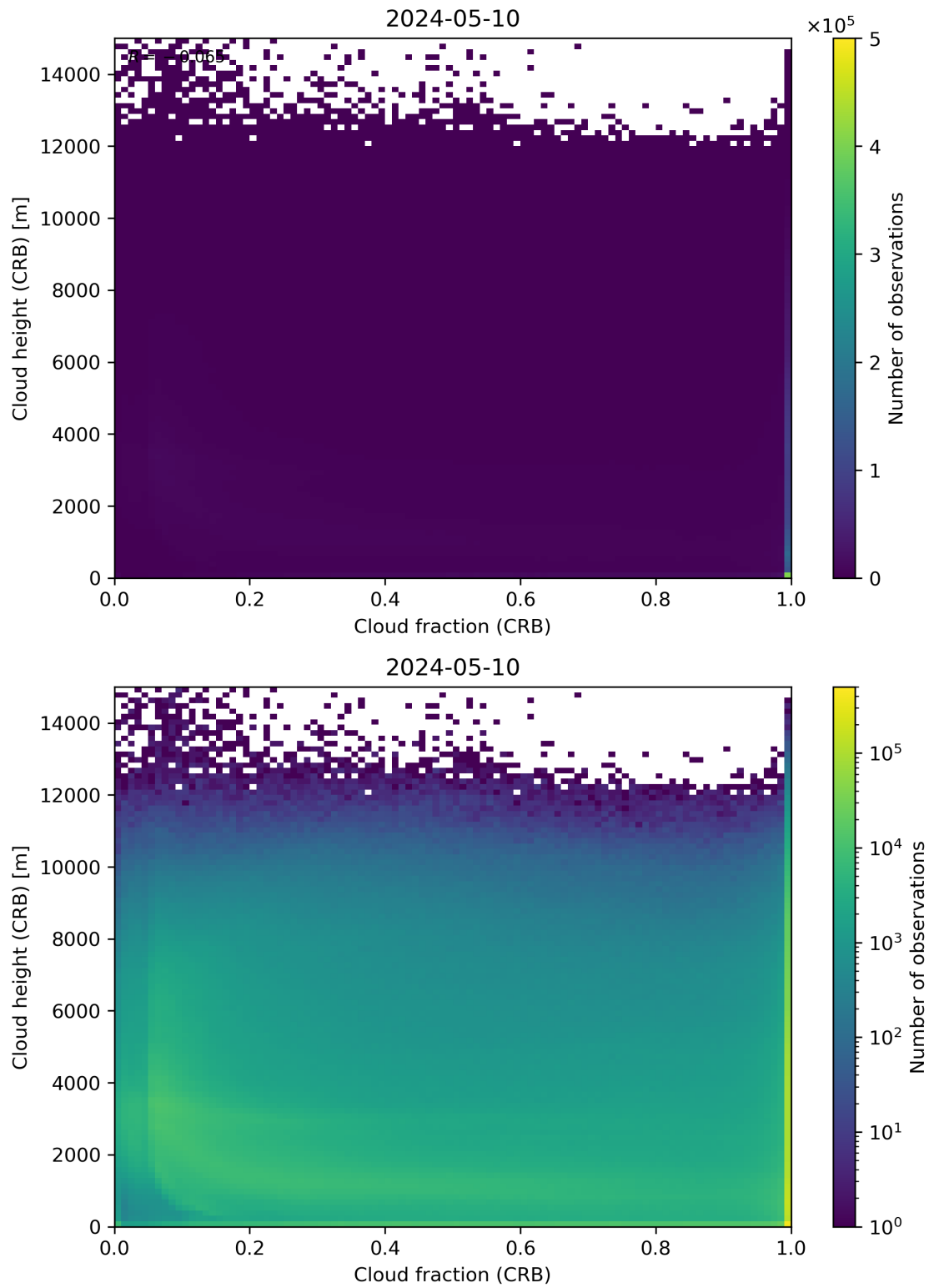
Figure 79: Scatter density plot of “Cloud fraction (CRB)” against “Cloud height (CRB)” for 2024-05-09 to 2024-05-11.
