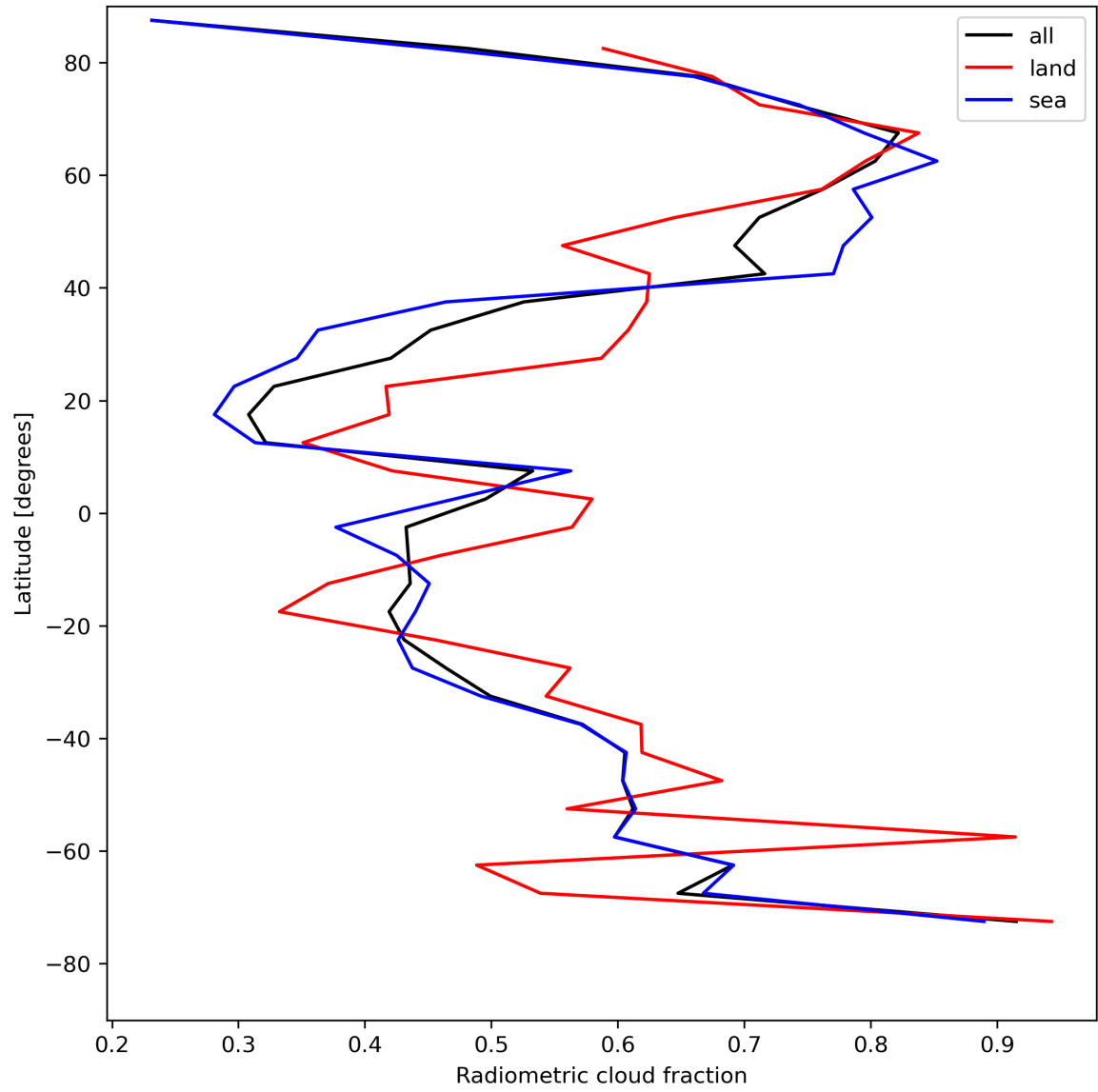
Figure 23: Zonal average of “Radiometric cloud fraction” for 2024-05-09 to 2024-05-11.
