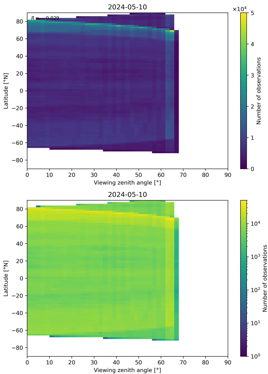
Figure 113: Scatter density plot of “Viewing zenith angle” against “Latitude” for 2024-05-09 to 2024-05-11.
