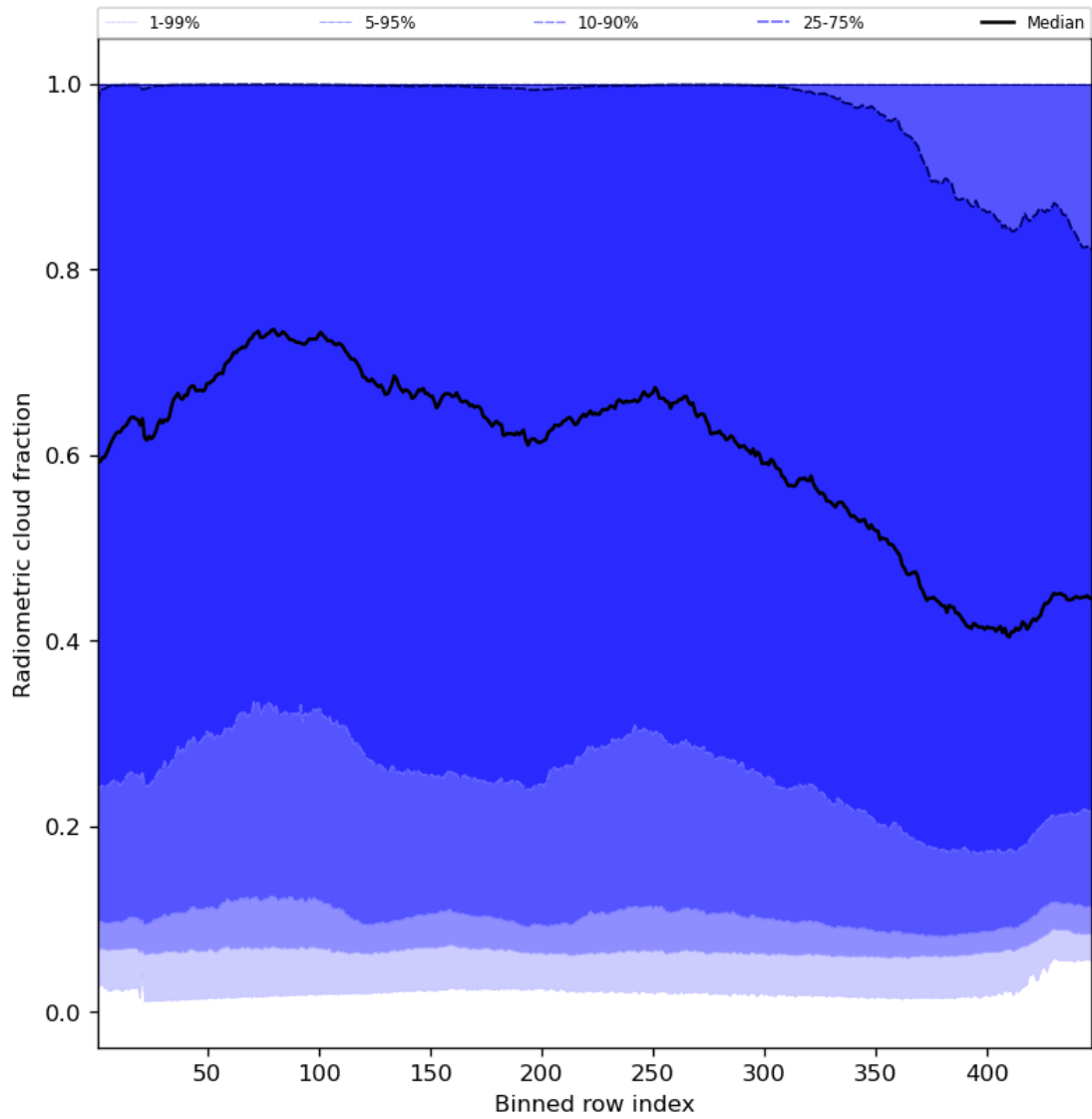
Figure 55: Along track statistics of “Radiometric cloud fraction” for 2024-05-09 to 2024-05-11
