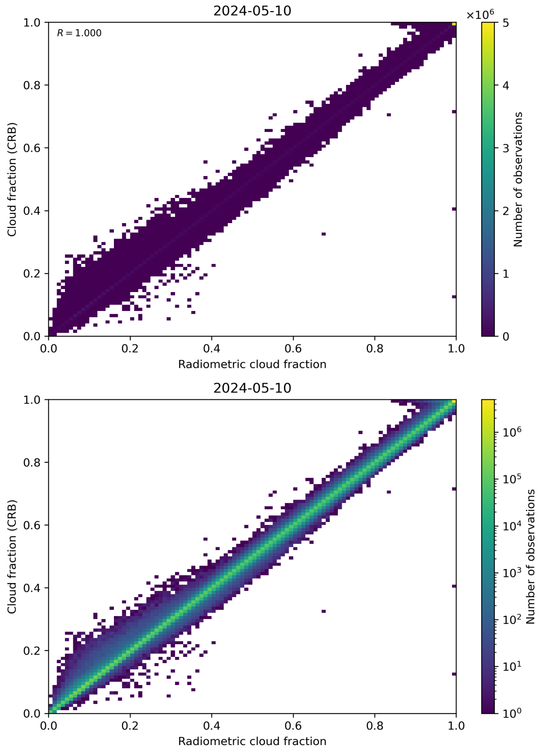
Figure 73: Scatter density plot of “Radiometric cloud fraction” against “Cloud fraction (CRB)” for 2024-05-09 to 2024-05-11.
