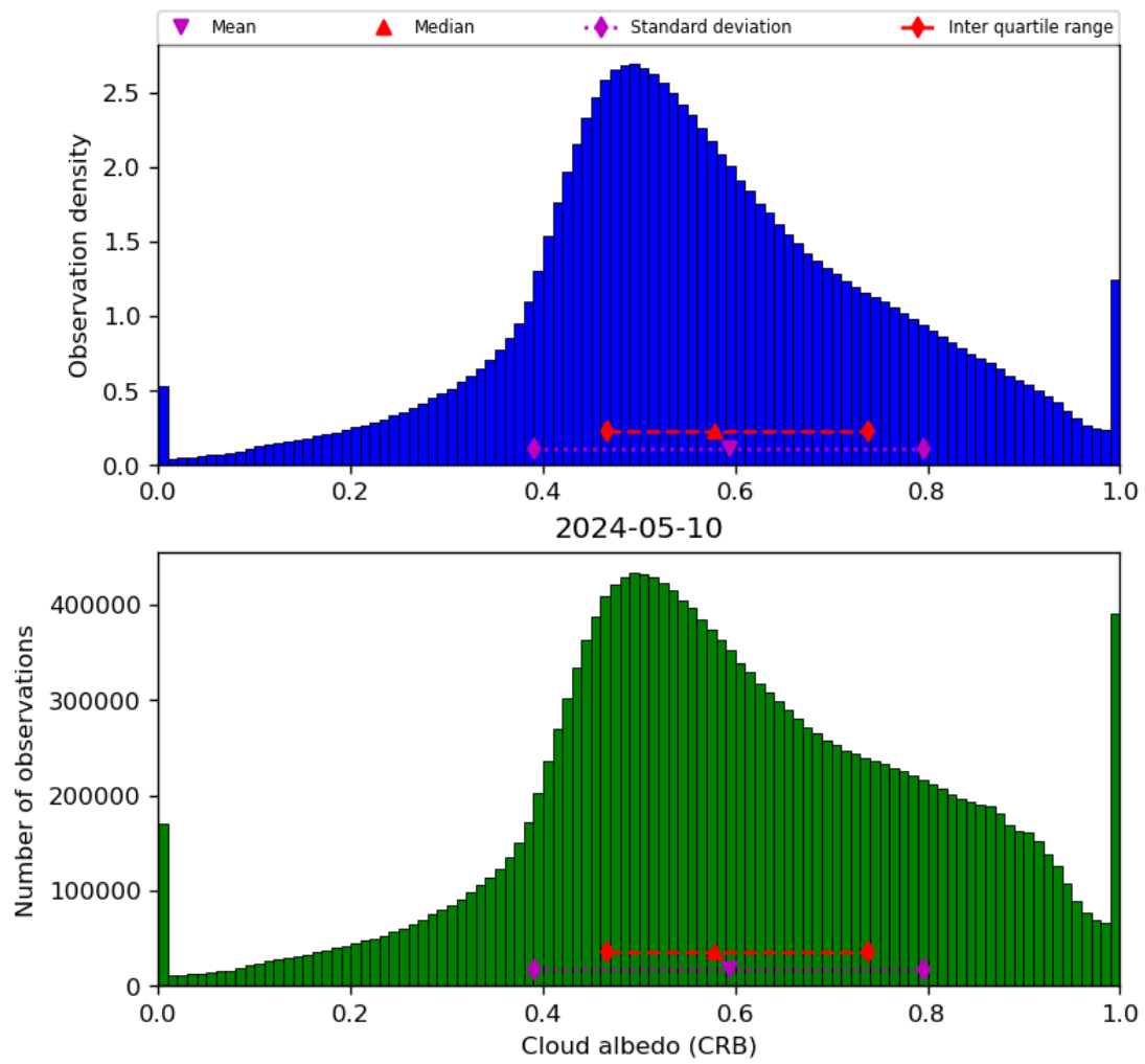
Figure 44: Histogram of “Cloud albedo (CRB)” for 2024-05-09 to 2024-05-11
