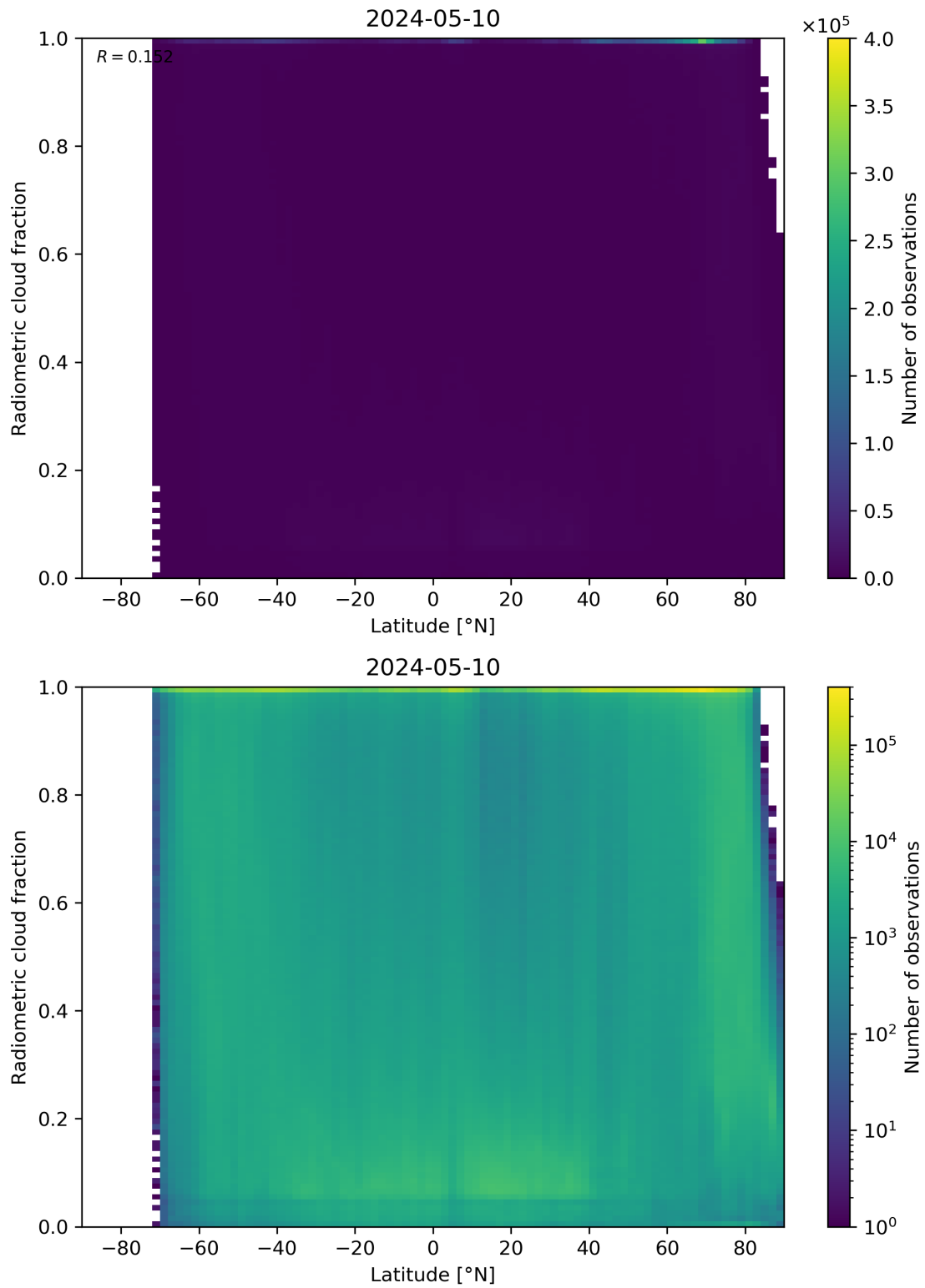
Figure 92: Scatter density plot of “Latitude” against “Radiometric cloud fraction” for 2024-05-09 to 2024-05-11.
