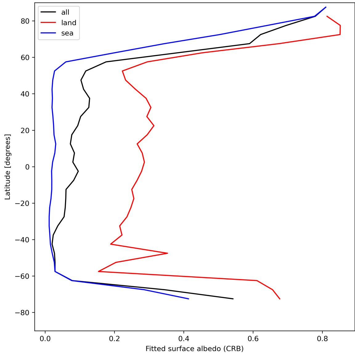
Figure 30: Zonal average of “Fitted surface albedo (CRB)” for 2024-05-09 to 2024-05-11.
