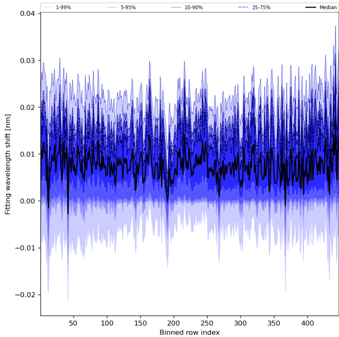
Figure 65: Along track statistics of “Fitting wavelength shift” for 2024-05-09 to 2024-05-11
