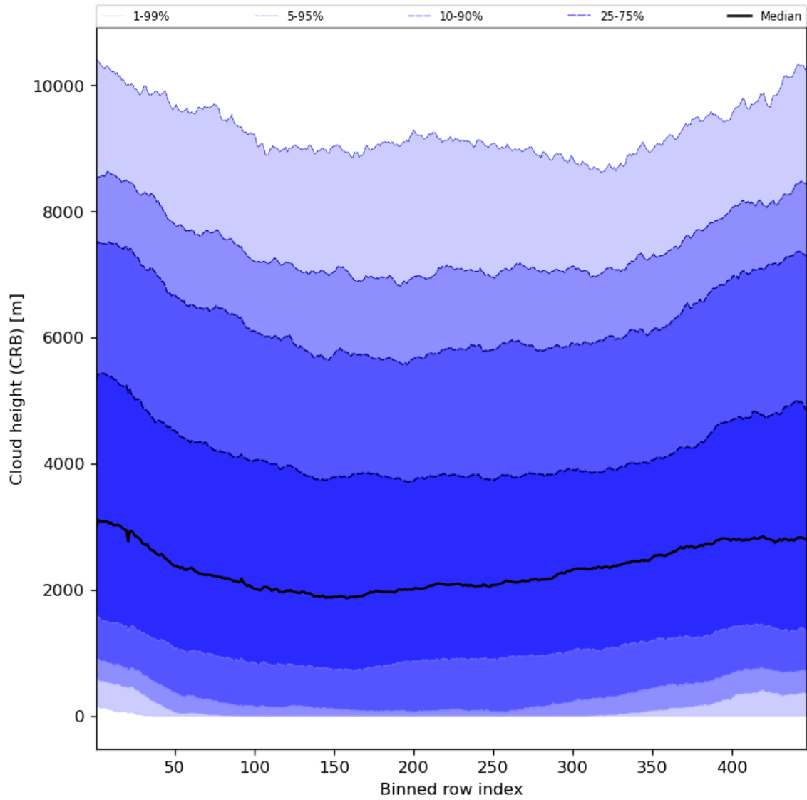
Figure 59: Along track statistics of “Cloud height (CRB)” for 2024-05-09 to 2024-05-11
