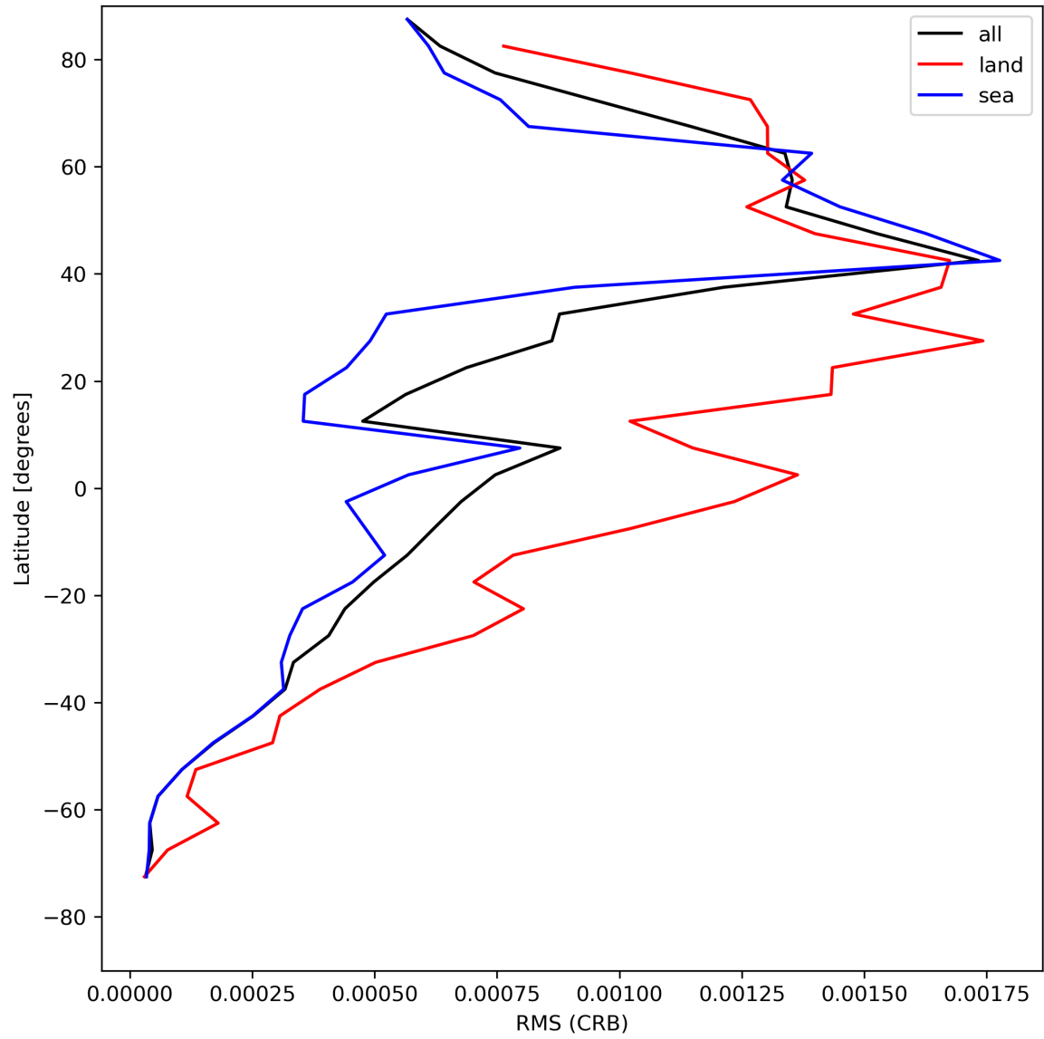
Figure 32: Zonal average of “RMS (CRB)” for 2024-05-09 to 2024-05-11.
