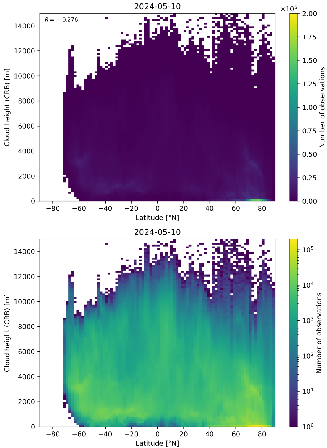
Figure 95: Scatter density plot of “Latitude” against “Cloud height (CRB)” for 2024-05-09 to 2024-05-11.
