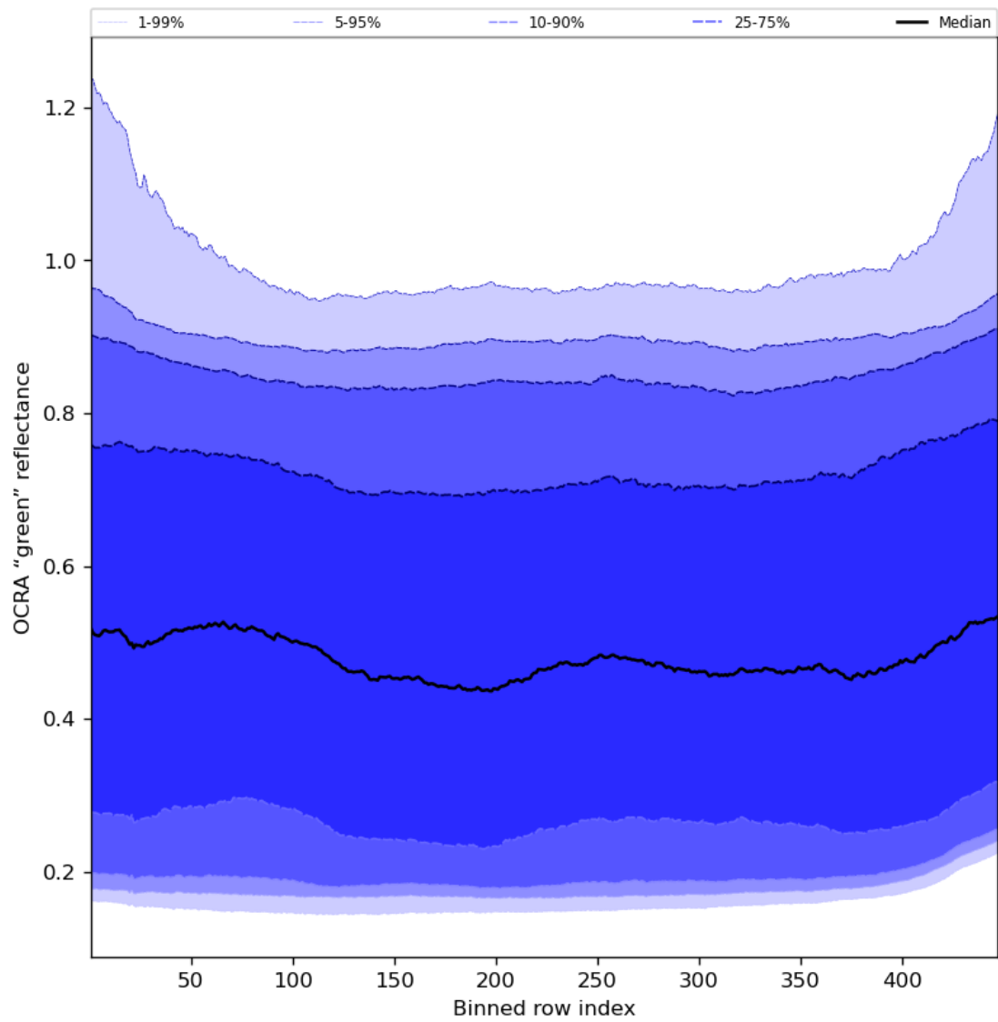
Figure 68: Along track statistics of “OCRA “green” reflectance” for 2024-05-09 to 2024-05-11
