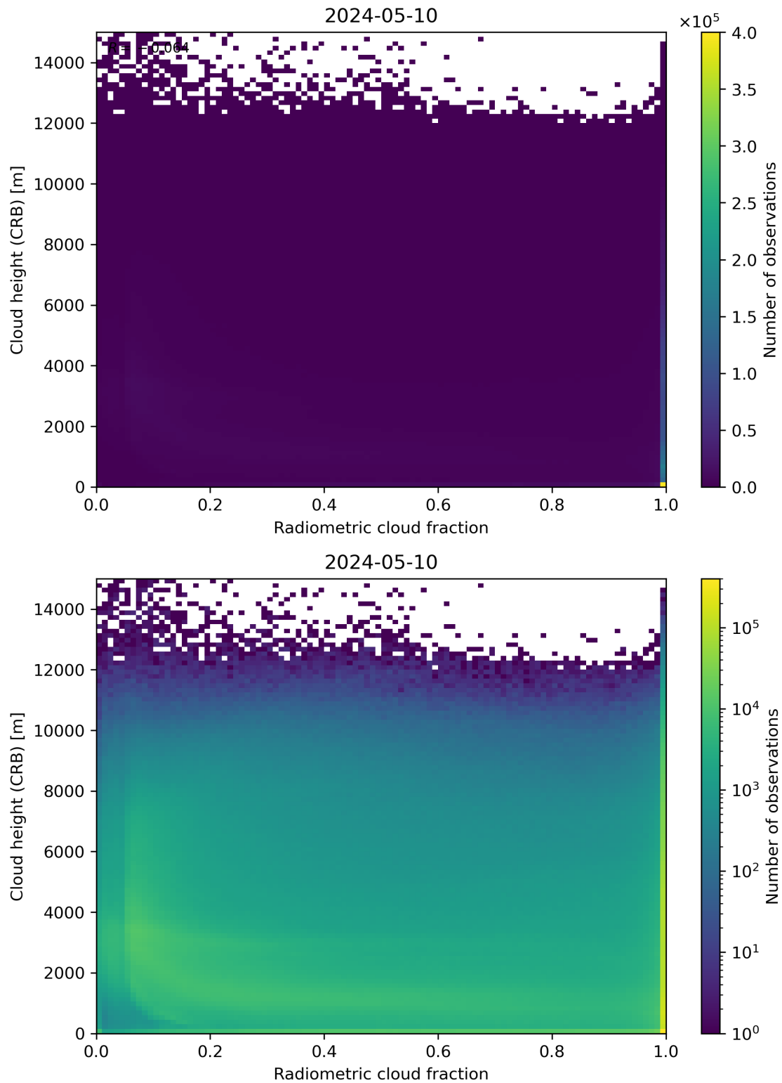
Figure 74: Scatter density plot of “Radiometric cloud fraction” against “Cloud height (CRB)” for 2024-05-09 to 2024-05-11.
