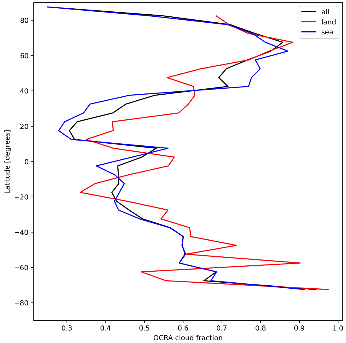
Figure 34: Zonal average of “OCRA cloud fraction” for 2024-05-09 to 2024-05-11.
