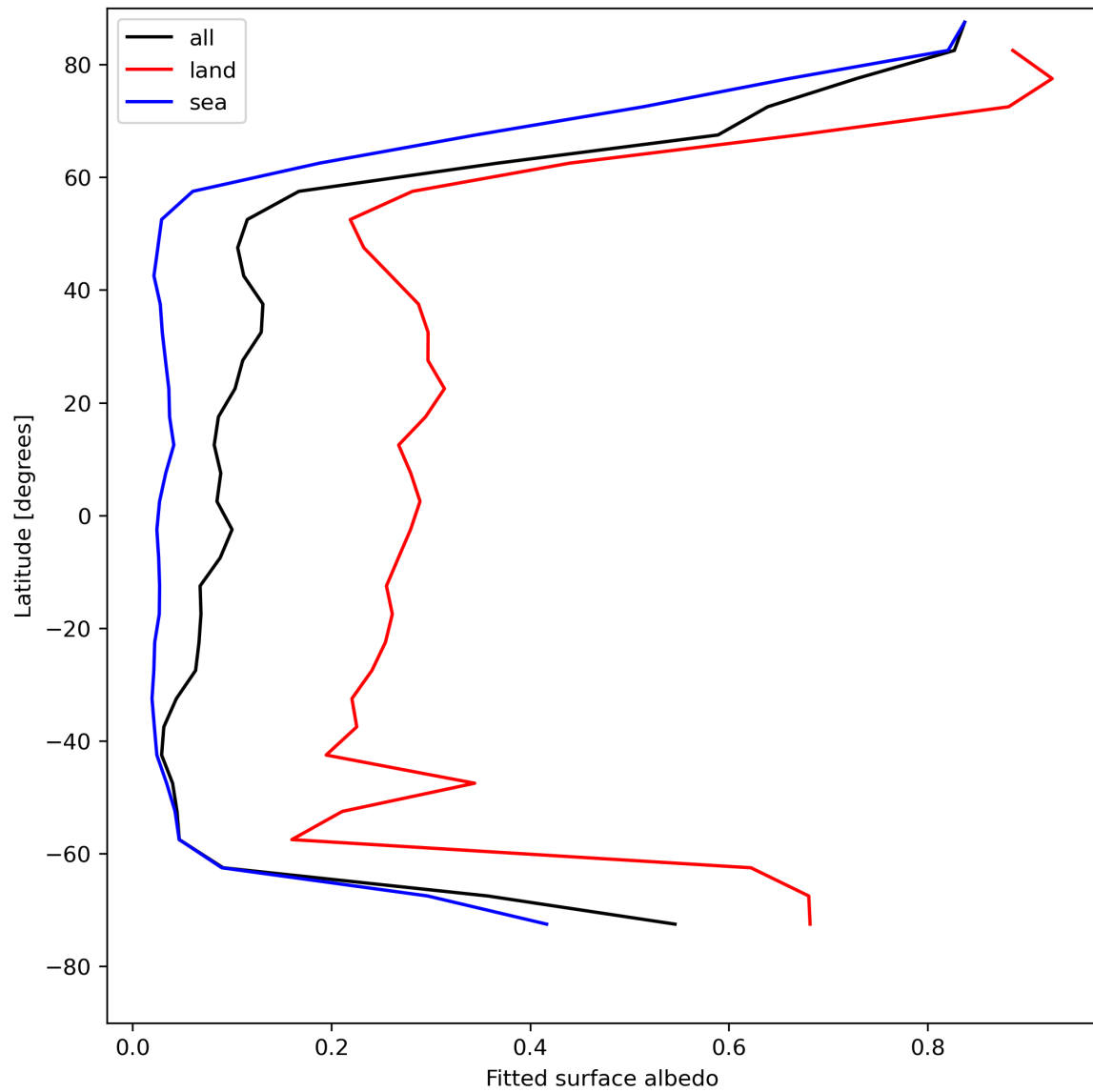
Figure 29: Zonal average of “Fitted surface albedo” for 2024-05-09 to 2024-05-11.
