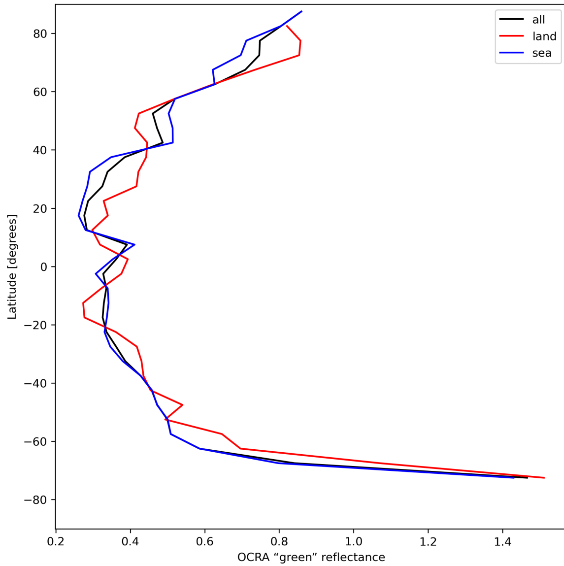
Figure 36: Zonal average of “OCRA “green” reflectance” for 2024-05-09 to 2024-05-11.
