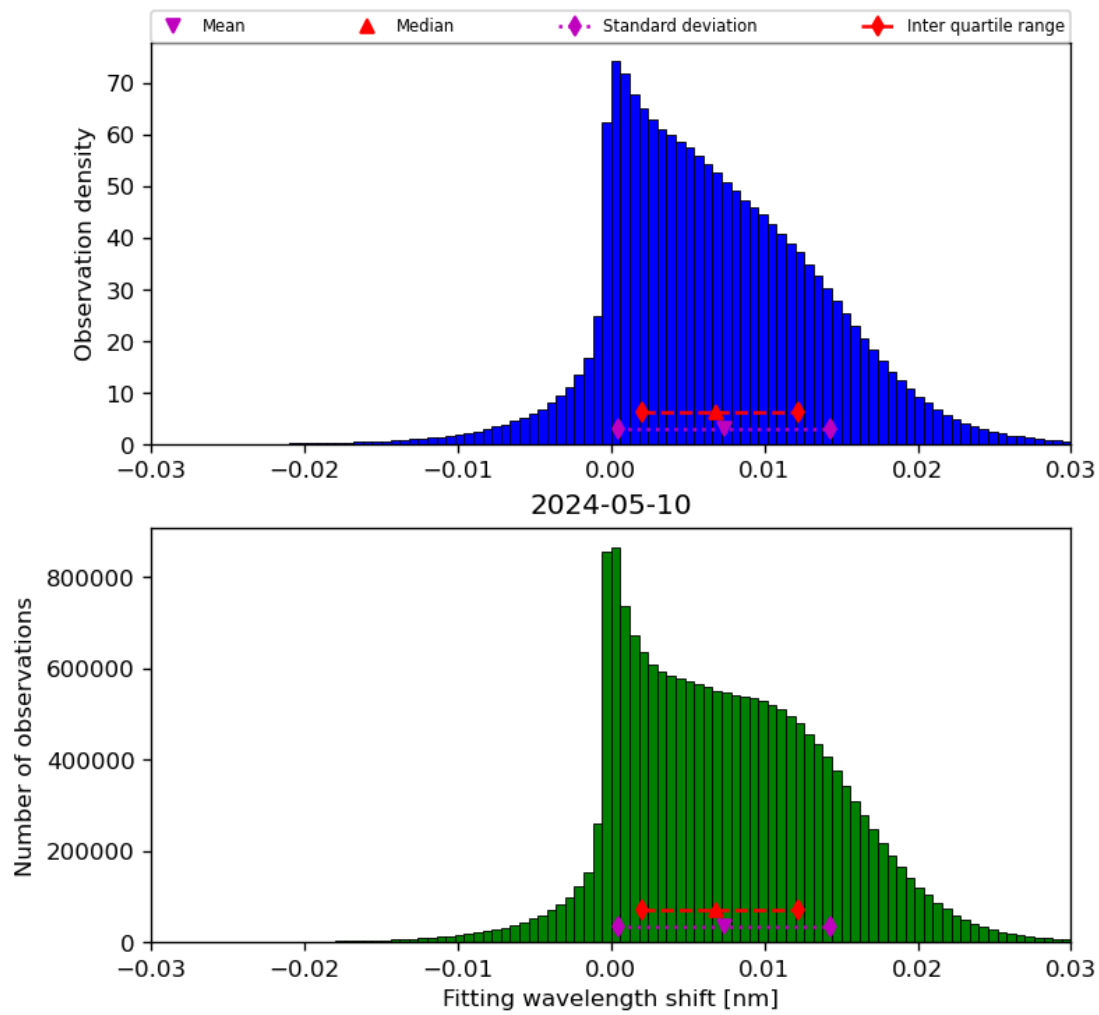
Figure 49: Histogram of “Fitting wavelength shift” for 2024-05-09 to 2024-05-11
