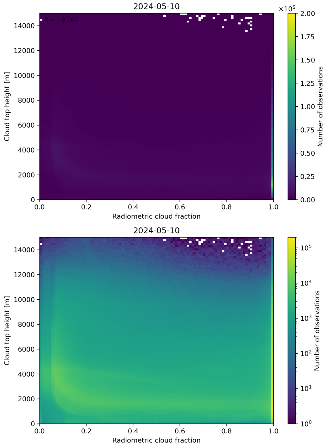
Figure 76: Scatter density plot of “Radiometric cloud fraction” against “Cloud top height” for 2024-05-09 to 2024-05-11.
