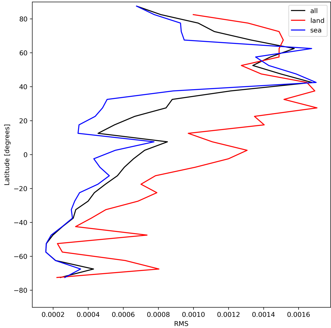
Figure 31: Zonal average of “RMS” for 2024-05-09 to 2024-05-11.
