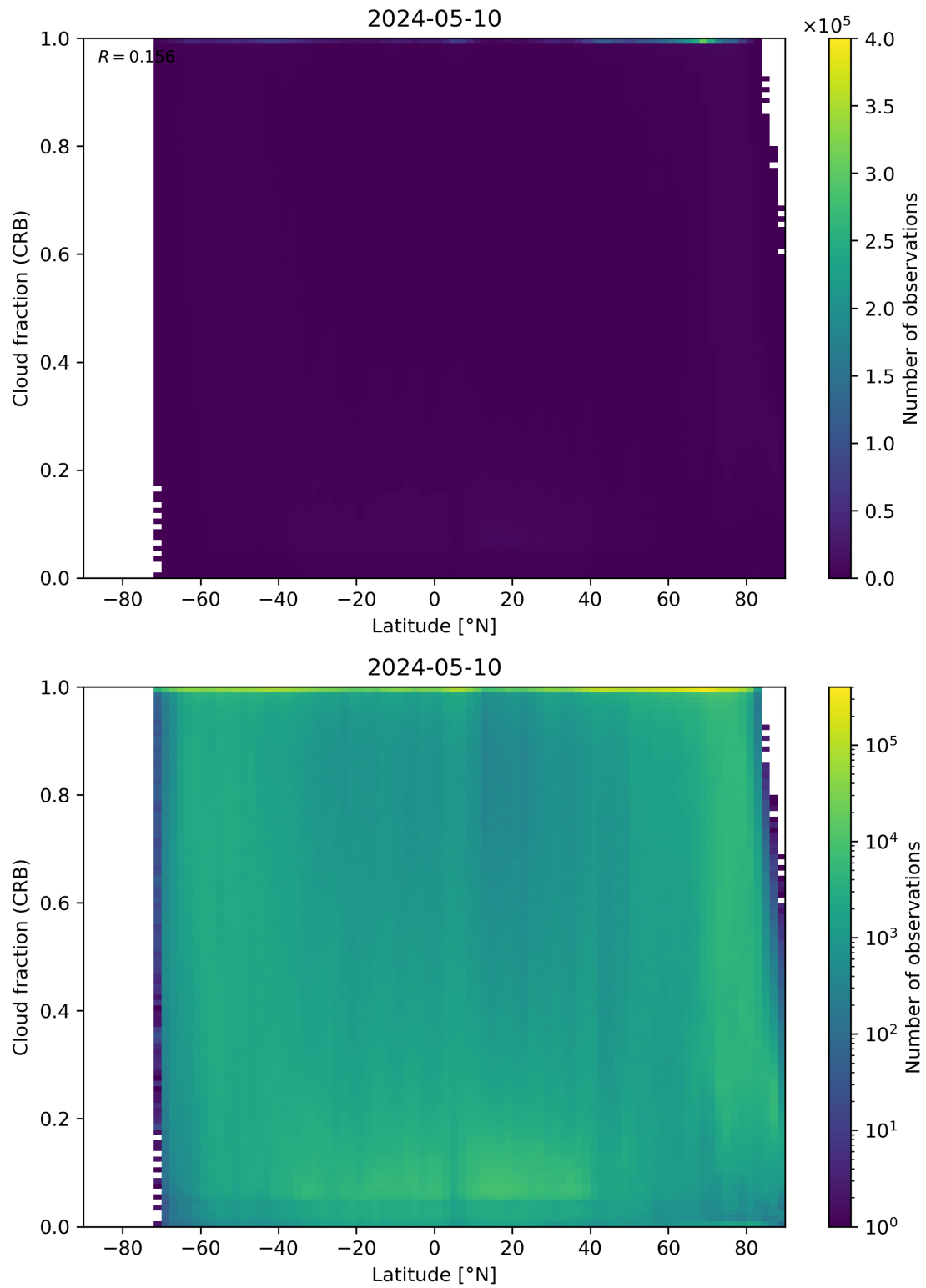
Figure 94: Scatter density plot of “Latitude” against “Cloud fraction (CRB)” for 2024-05-09 to 2024-05-11.
