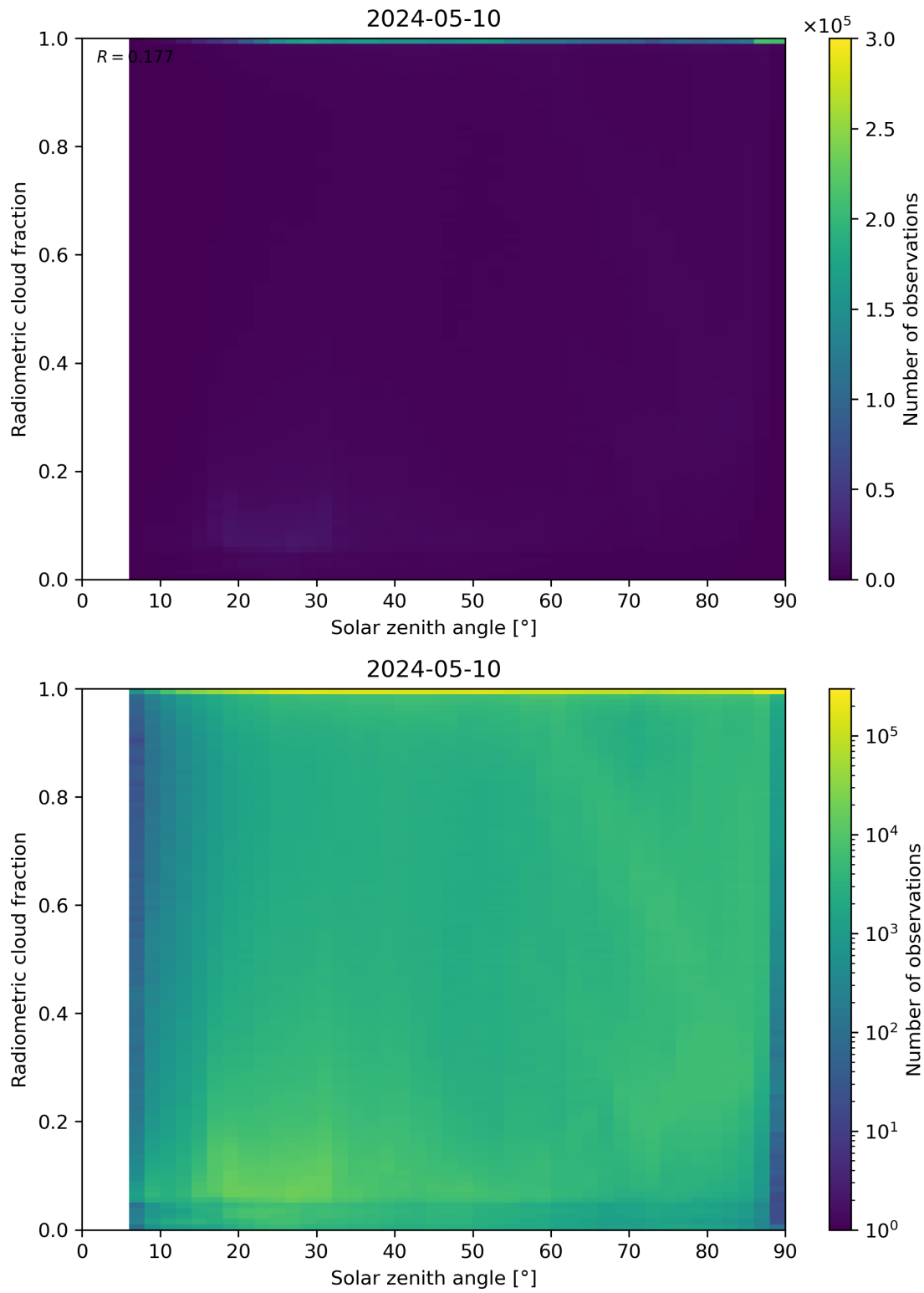
Figure 99: Scatter density plot of “Solar zenith angle” against “Radiometric cloud fraction” for 2024-05-09 to 2024-05-11.
