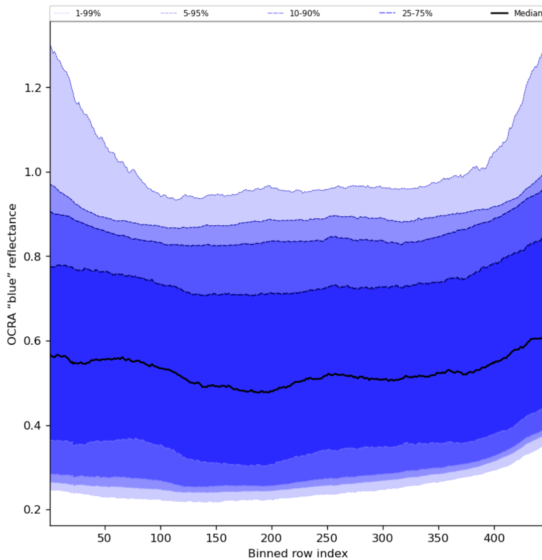
Figure 67: Along track statistics of “OCRA “blue” reflectance” for 2024-05-09 to 2024-05-11
