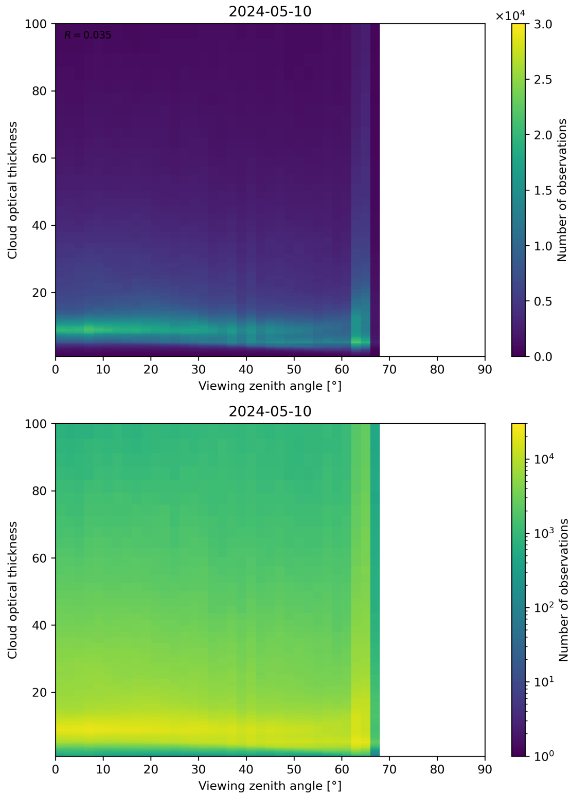
Figure 111: Scatter density plot of “Viewing zenith angle” against “Cloud optical thickness” for 2024-05-09 to 2024-05-11.
