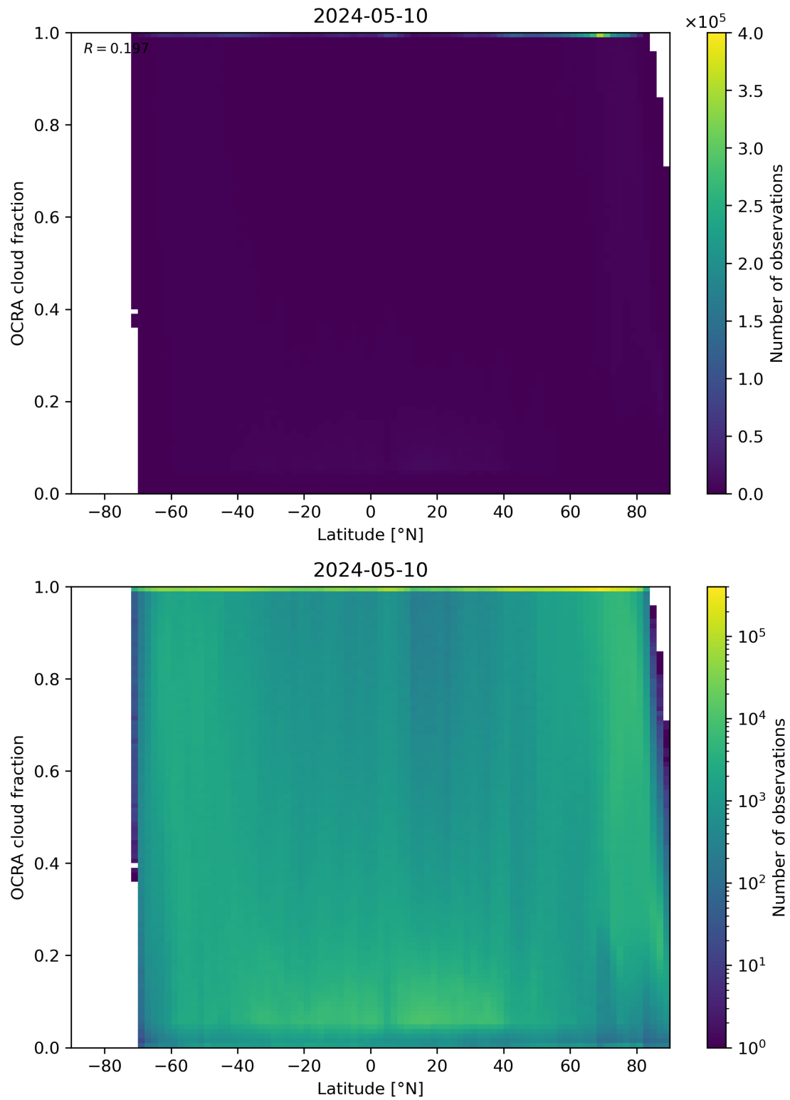
Figure 93: Scatter density plot of “Latitude” against “OCRA cloud fraction” for 2024-05-09 to 2024-05-11.
