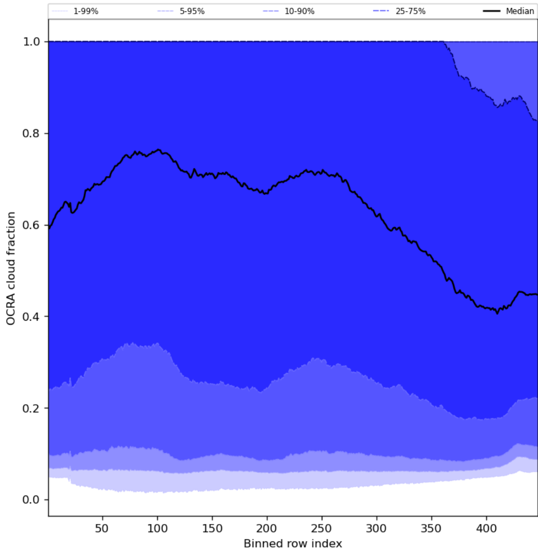
Figure 66: Along track statistics of “OCRA cloud fraction” for 2024-05-09 to 2024-05-11
