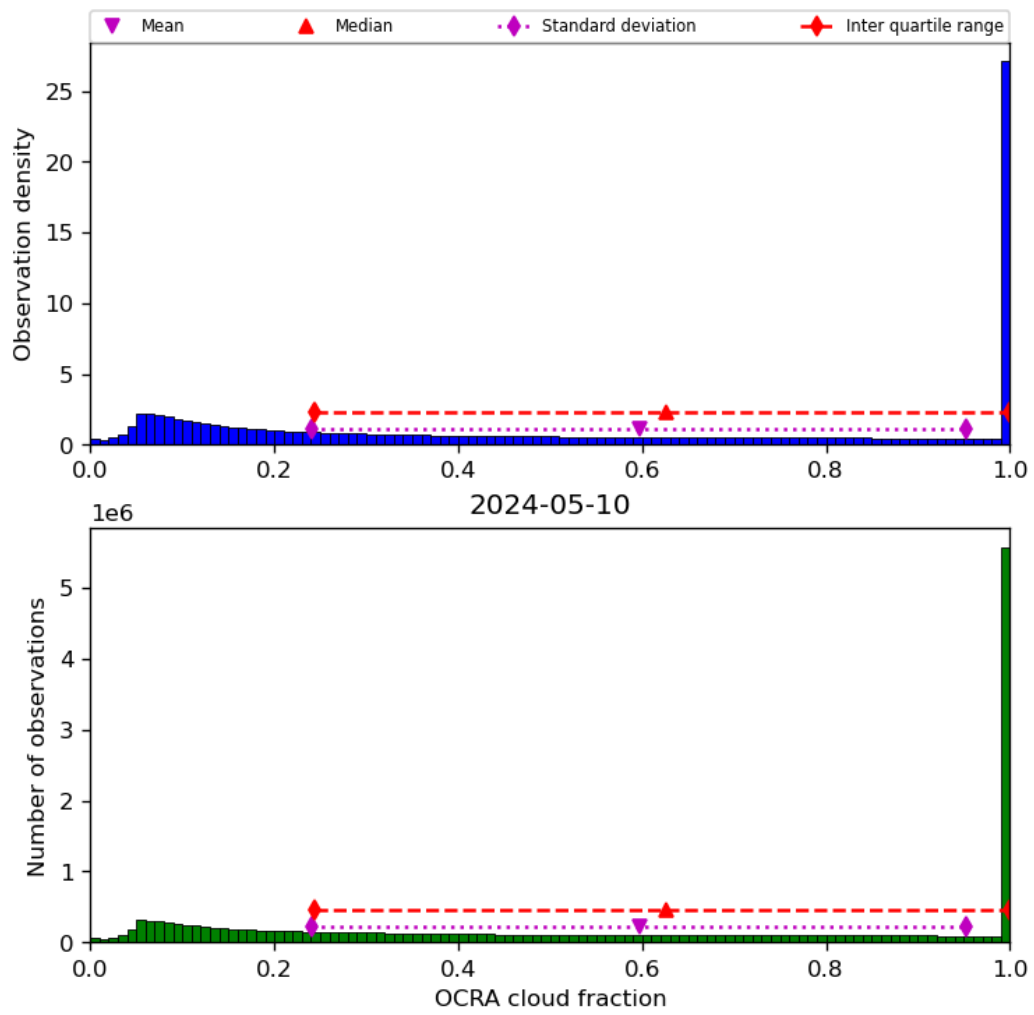
Figure 50: Histogram of “OCRA cloud fraction” for 2024-05-09 to 2024-05-11
