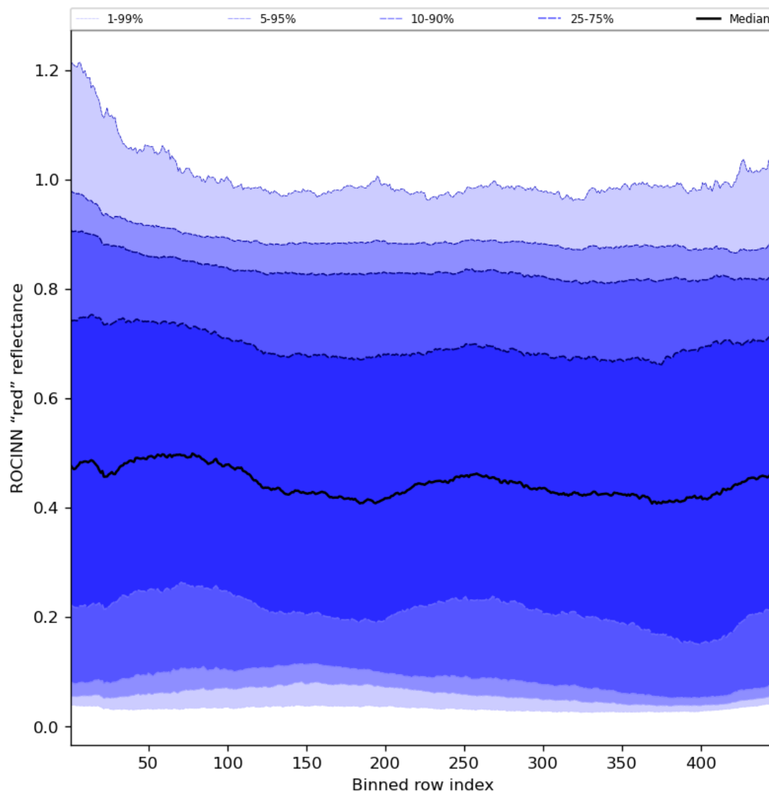
Figure 69: Along track statistics of "ROCINN "red" reflectance" for 2024-05-09 to 2024-05-11
