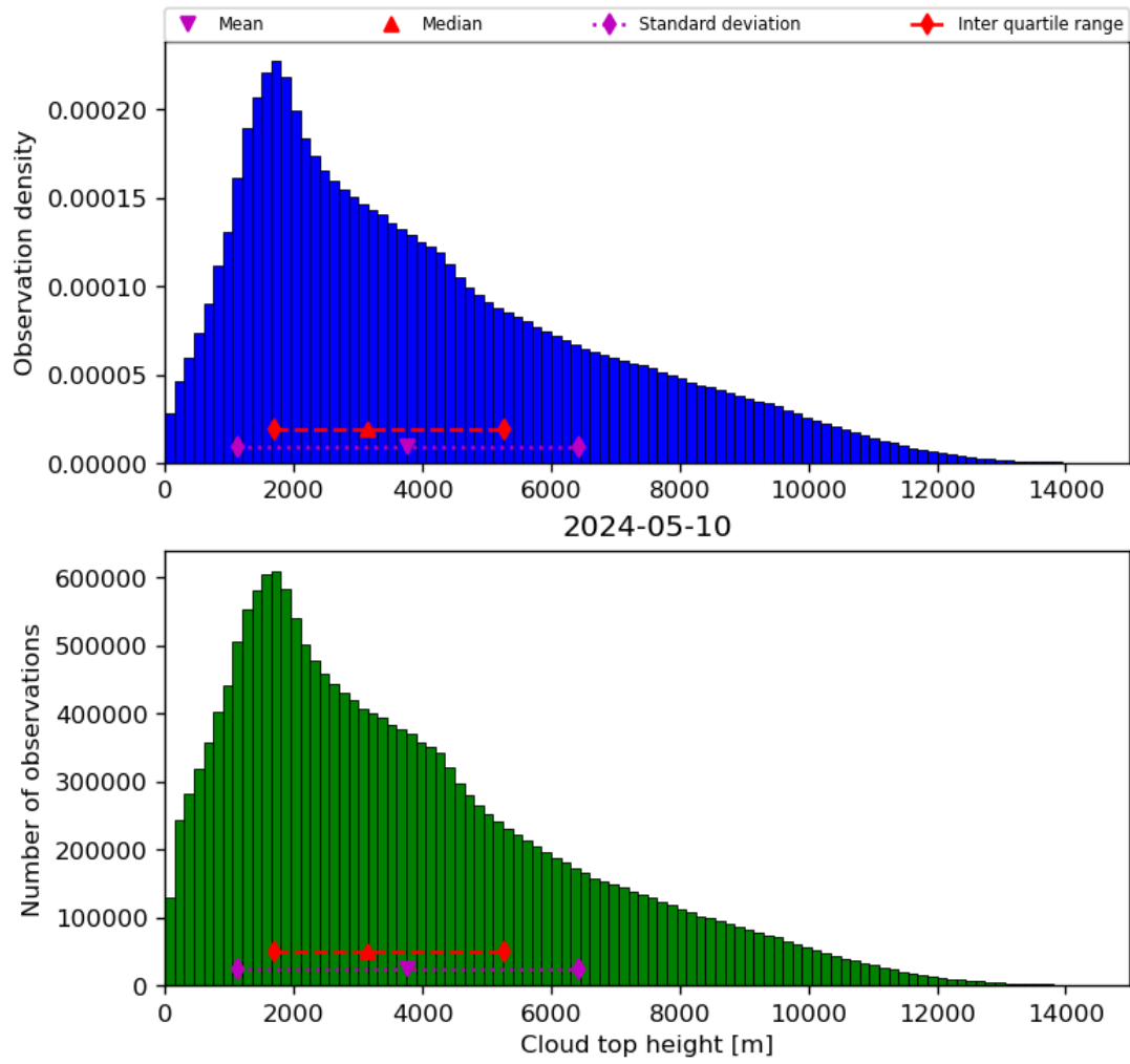
Figure 40: Histogram of “Cloud top height” for 2024-05-09 to 2024-05-11
