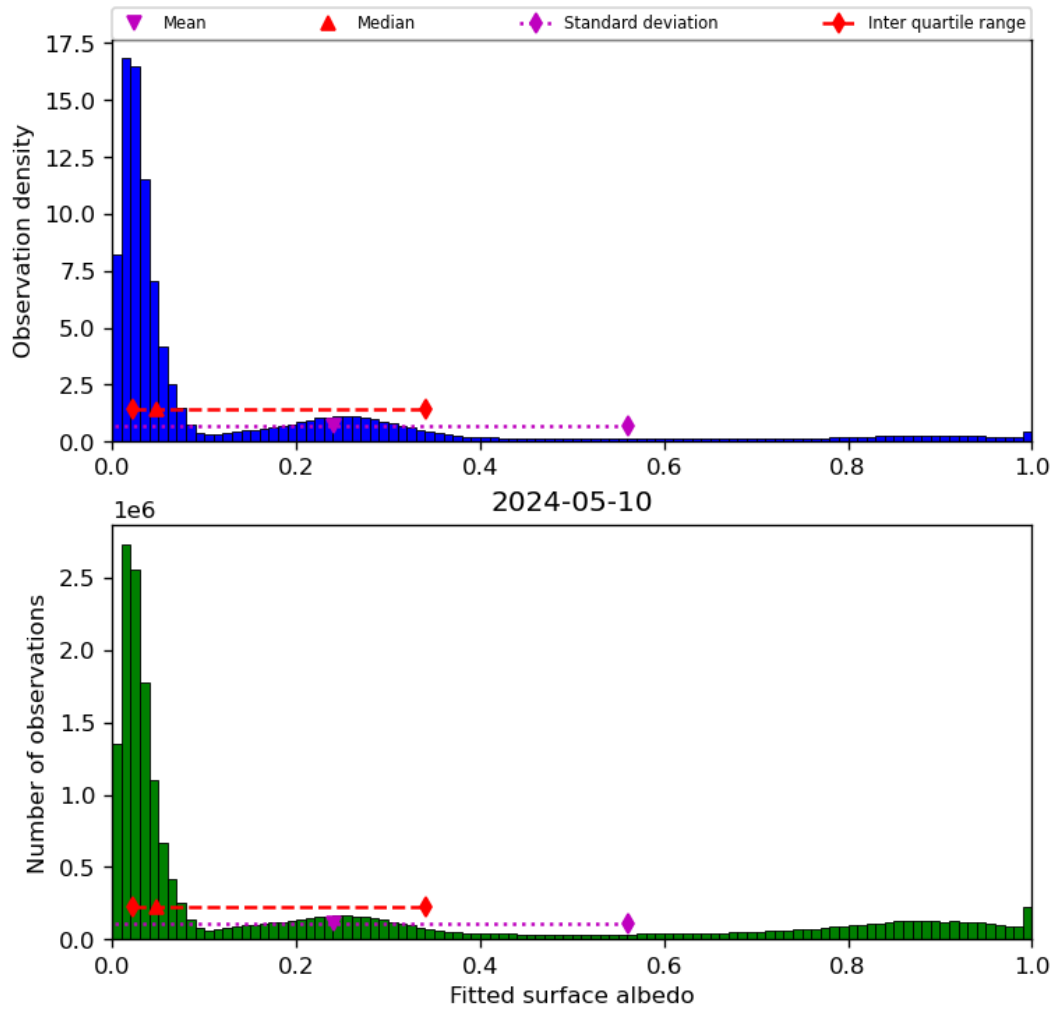
Figure 45: Histogram of “Fitted surface albedo” for 2024-05-09 to 2024-05-11
