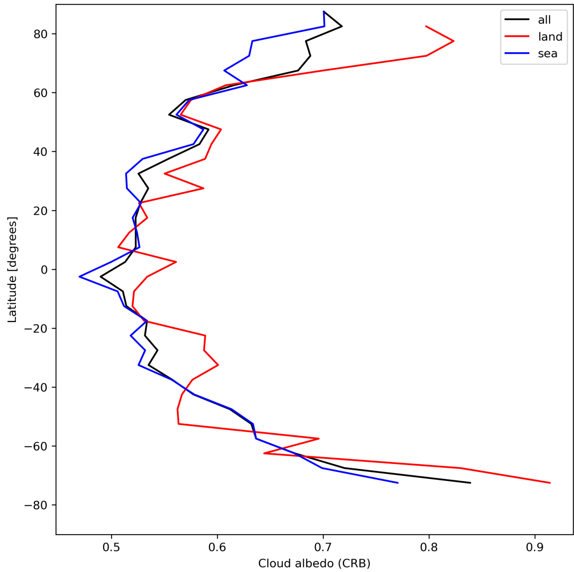
Figure 28: Zonal average of “Cloud albedo (CRB)” for 2024-05-09 to 2024-05-11.
