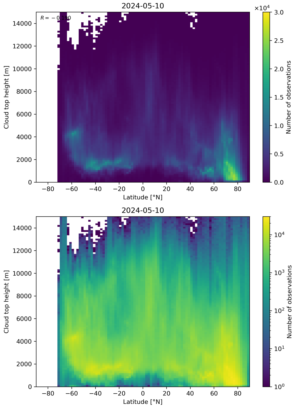
Figure 97: Scatter density plot of “Latitude” against “Cloud top height” for 2024-05-09 to 2024-05-11.
