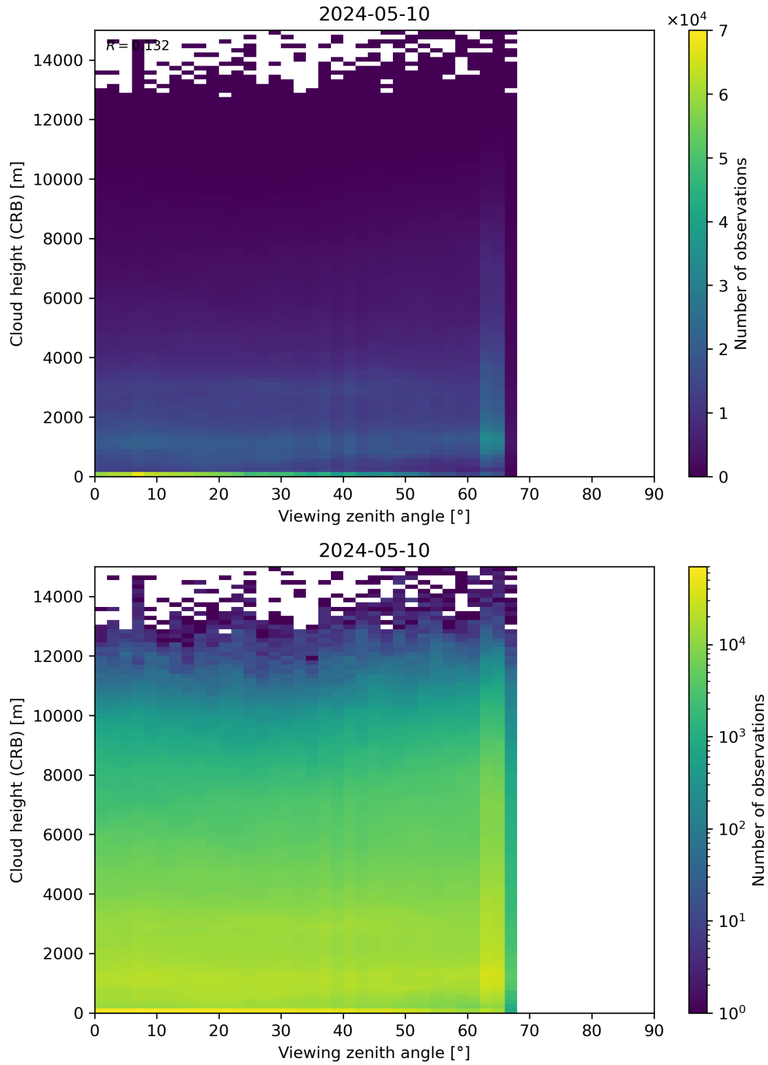
Figure 110: Scatter density plot of “Viewing zenith angle” against “Cloud height (CRB)” for 2024-05-09 to 2024-05-11.
