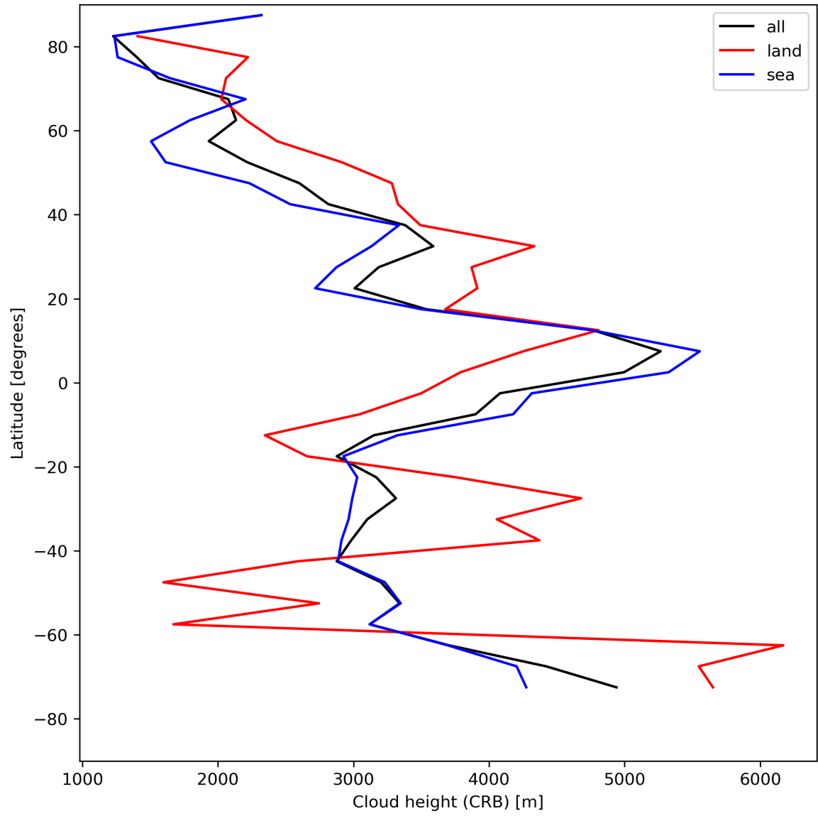
Figure 27: Zonal average of “Cloud height (CRB)” for 2024-05-09 to 2024-05-11.
