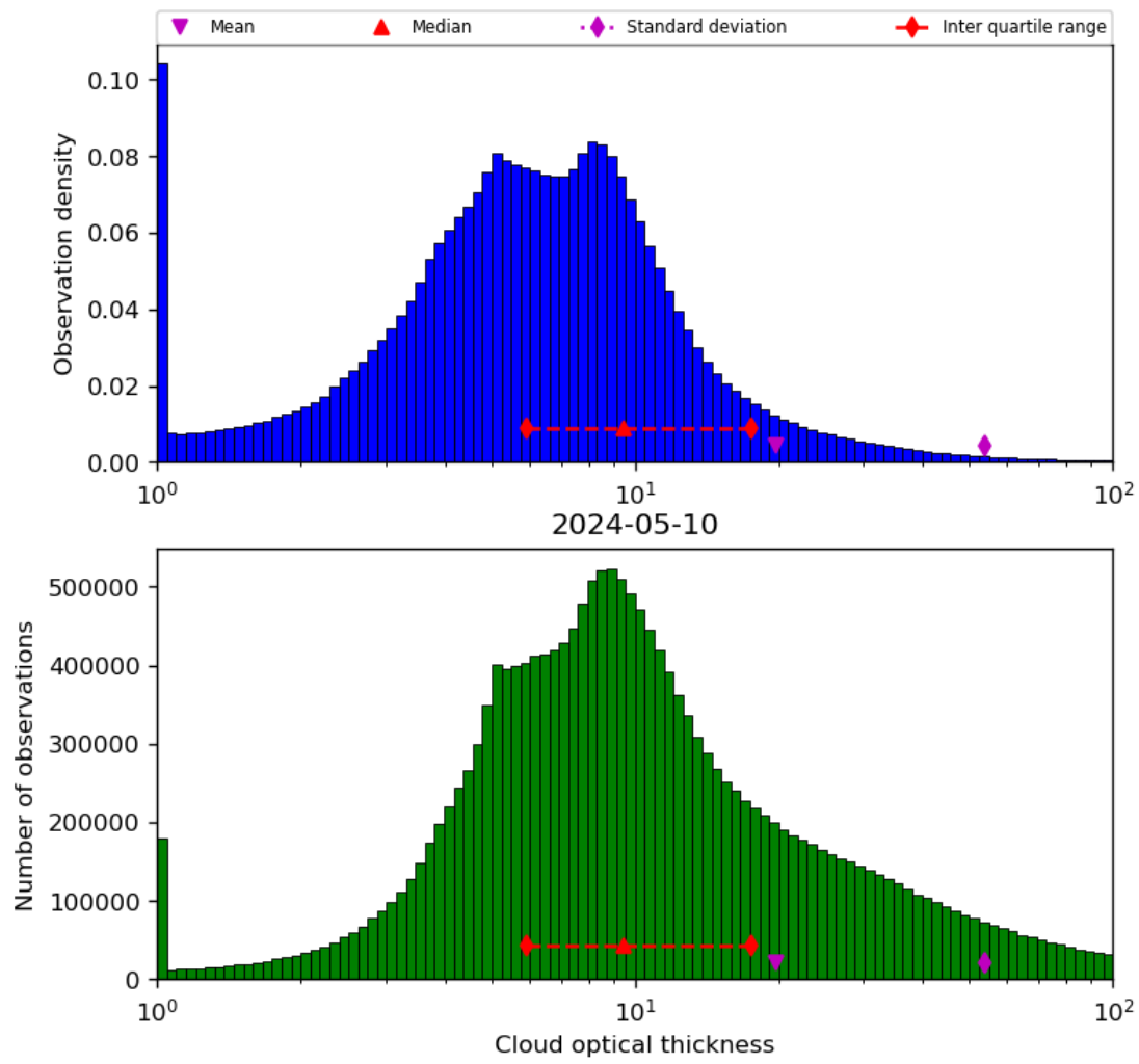
Figure 41: Histogram of “Cloud optical thickness” for 2024-05-09 to 2024-05-11
