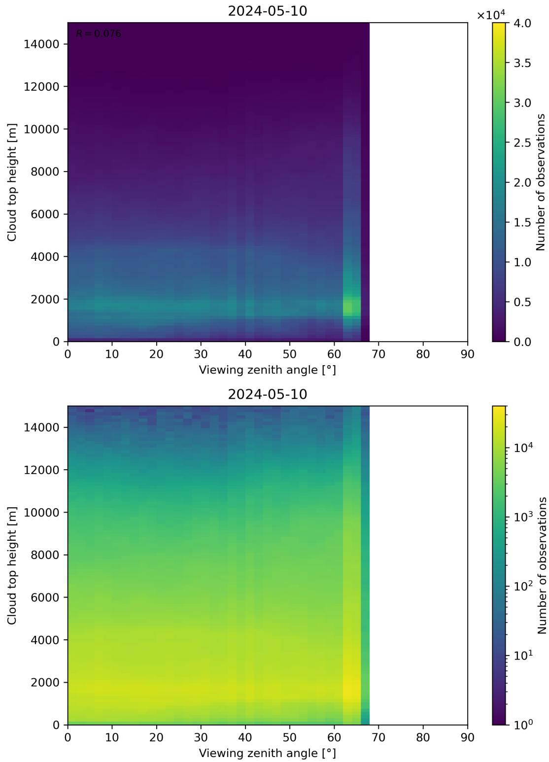
Figure 112: Scatter density plot of “Viewing zenith angle” against “Cloud top height” for 2024-05-09 to 2024-05-11.
