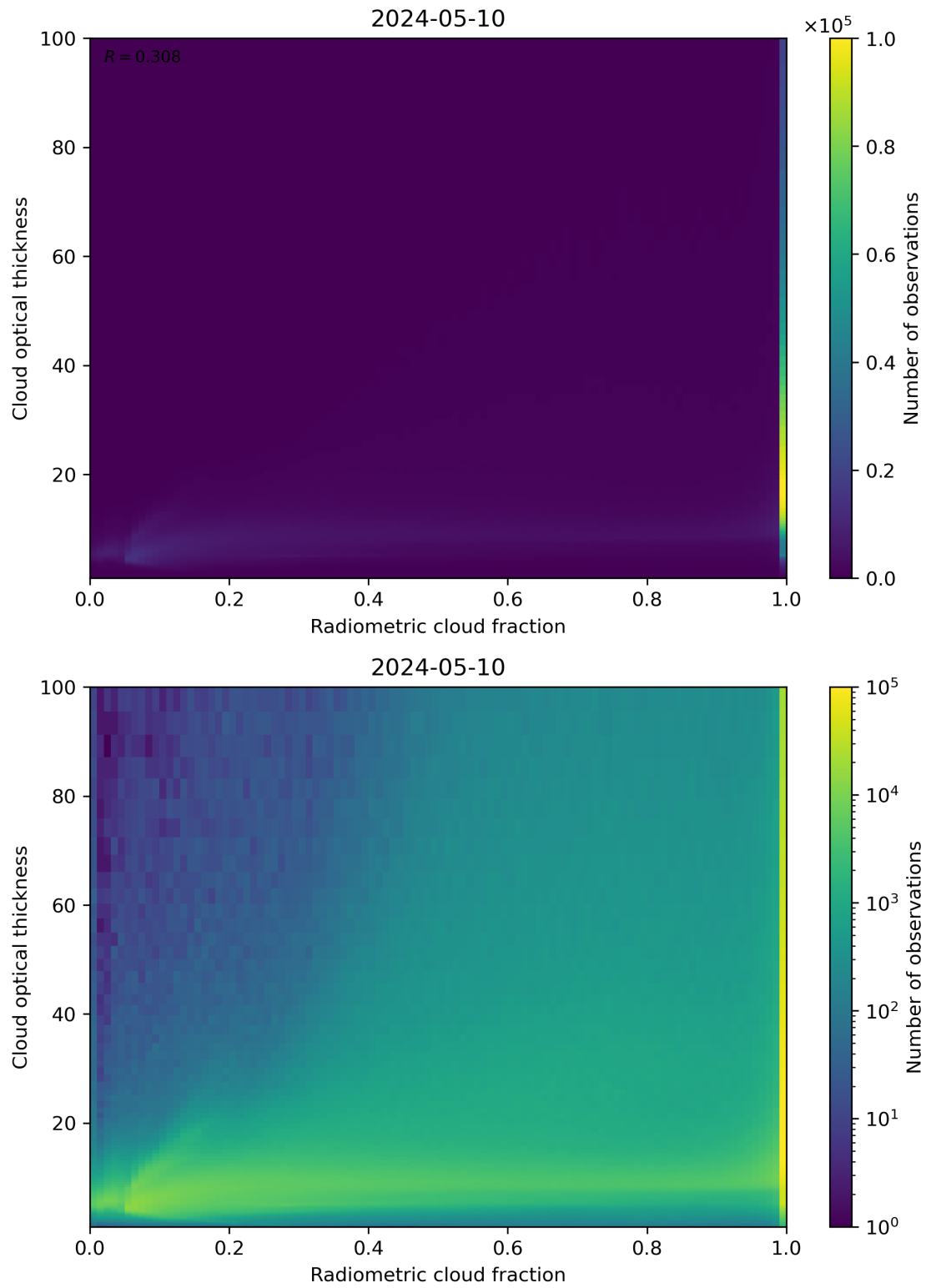
Figure 75: Scatter density plot of “Radiometric cloud fraction” against “Cloud optical thickness” for 2024-05-09 to 2024-05-11.
