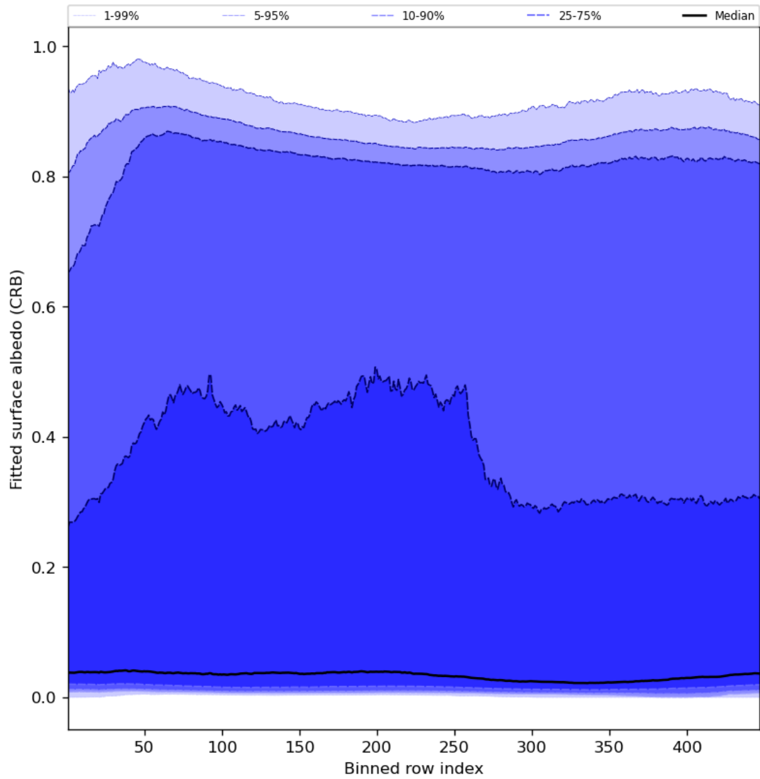
Figure 62: Along track statistics of “Fitted surface albedo (CRB)” for 2024-05-09 to 2024-05-11
