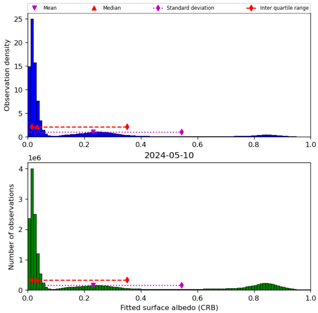
Figure 46: Histogram of “Fitted surface albedo (CRB)” for 2024-05-09 to 2024-05-11
