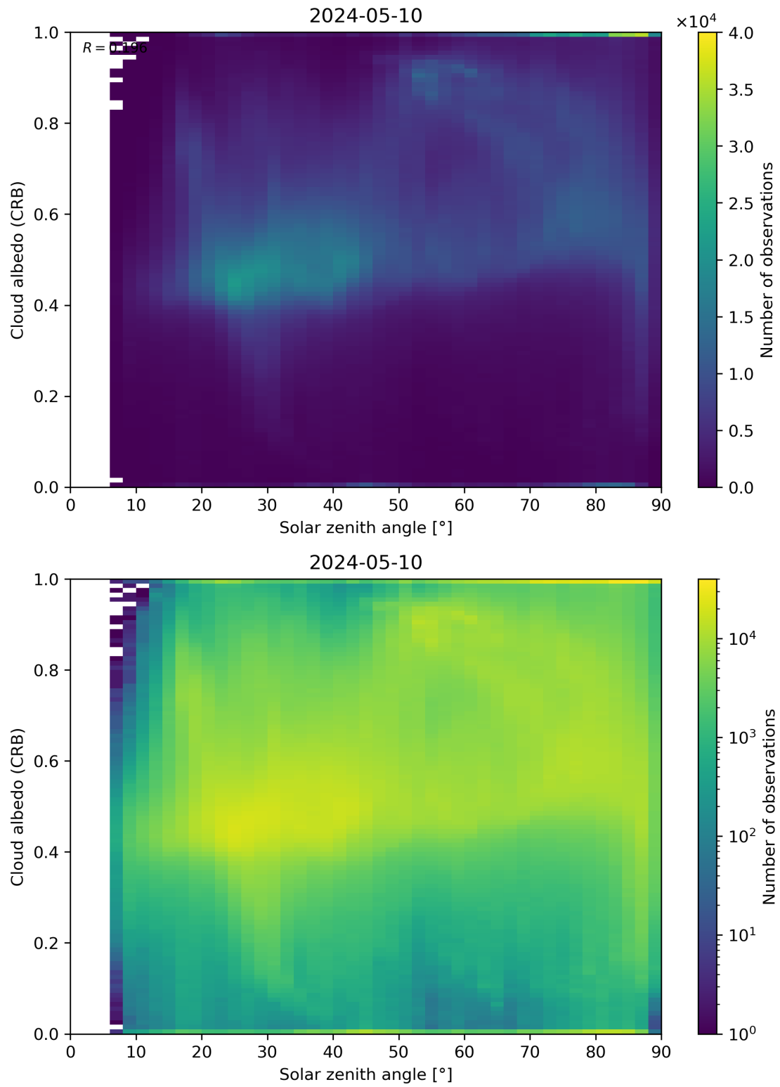
Figure 98: Scatter density plot of “Solar zenith angle” against “Cloud albedo (CRB)” for 2024-05-09 to 2024-05-11.
