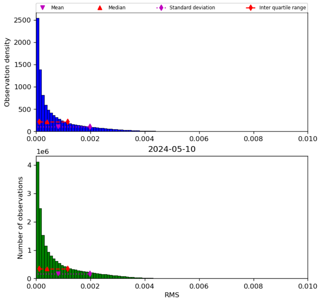
Figure 47: Histogram of “RMS” for 2024-05-09 to 2024-05-11
