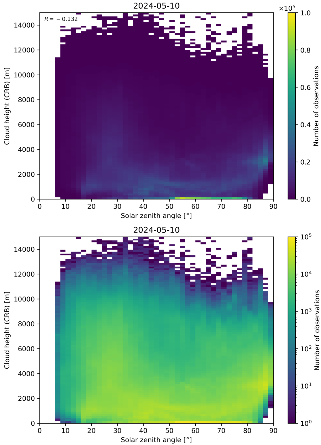
Figure 102: Scatter density plot of “Solar zenith angle” against “Cloud height (CRB)” for 2024-05-09 to 2024-05-11.
