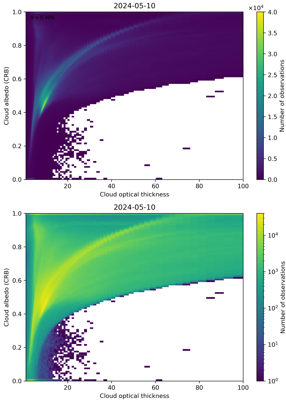
Figure 82: Scatter density plot of “Cloud optical thickness” against “Cloud albedo (CRB)” for 2024-05-09 to 2024-05-11.
