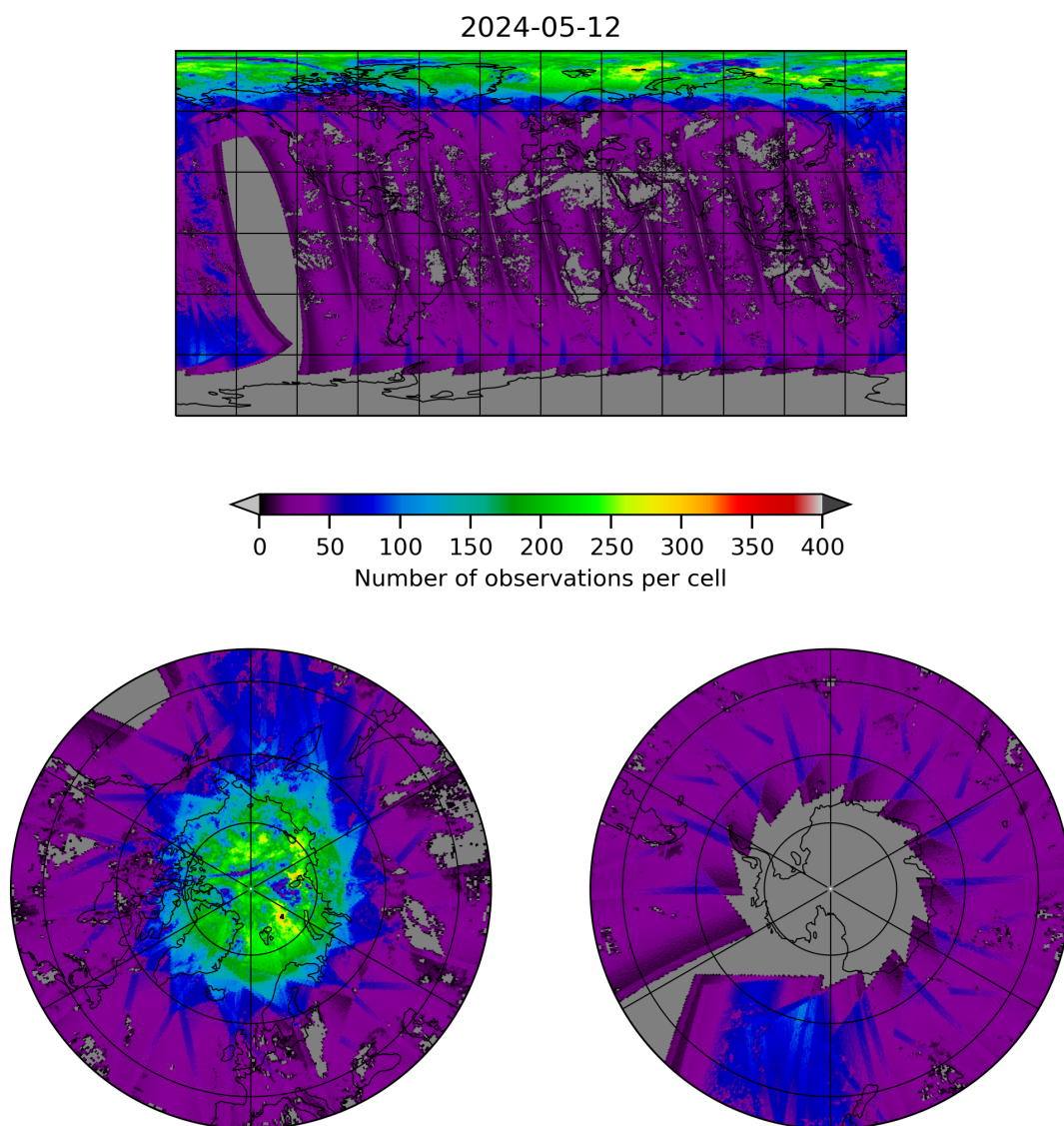
Figure 21: Map of the number of observations for 2024-05-12 to 2024-05-13
