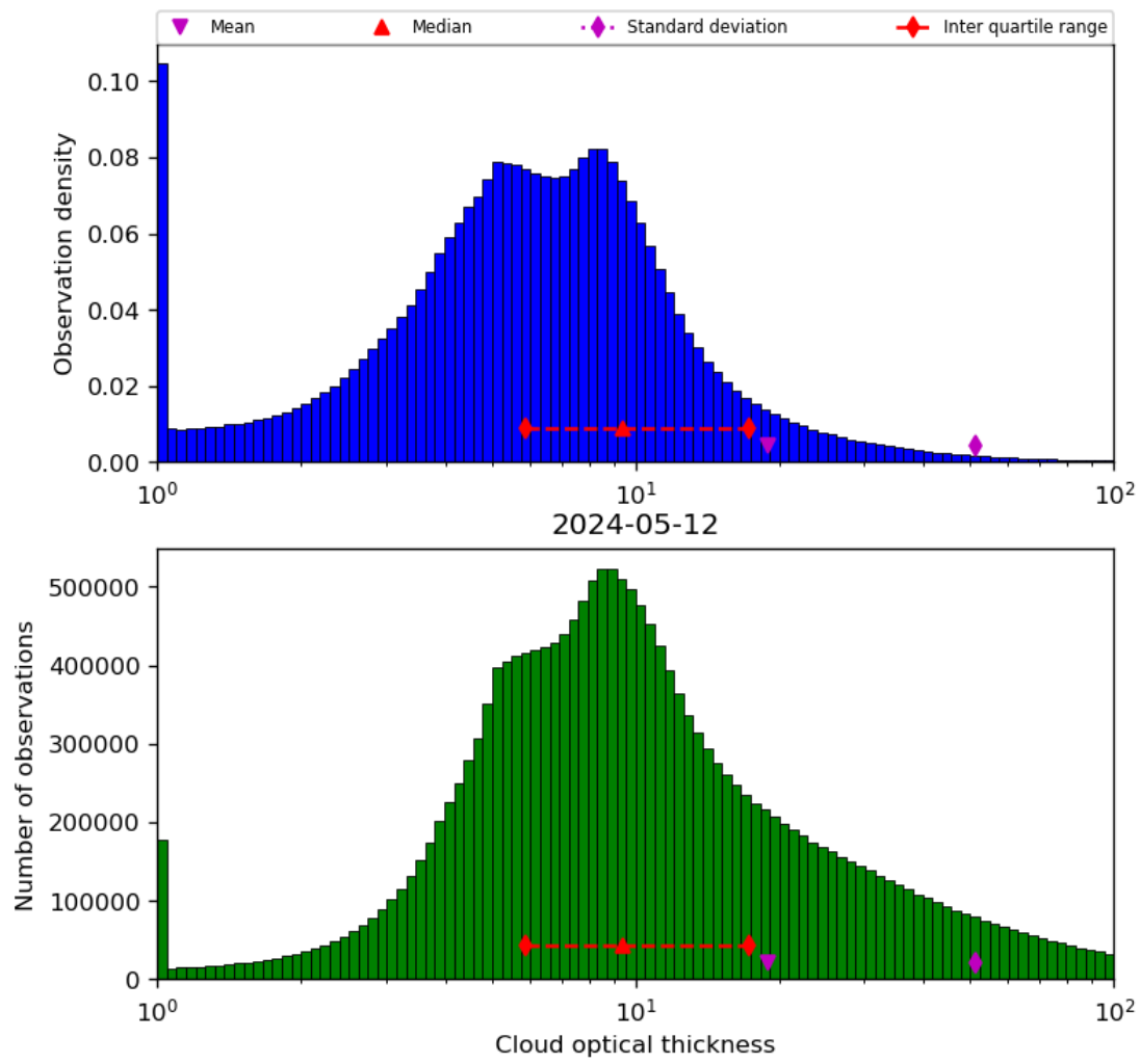
Figure 41: Histogram of “Cloud optical thickness” for 2024-05-12 to 2024-05-13
