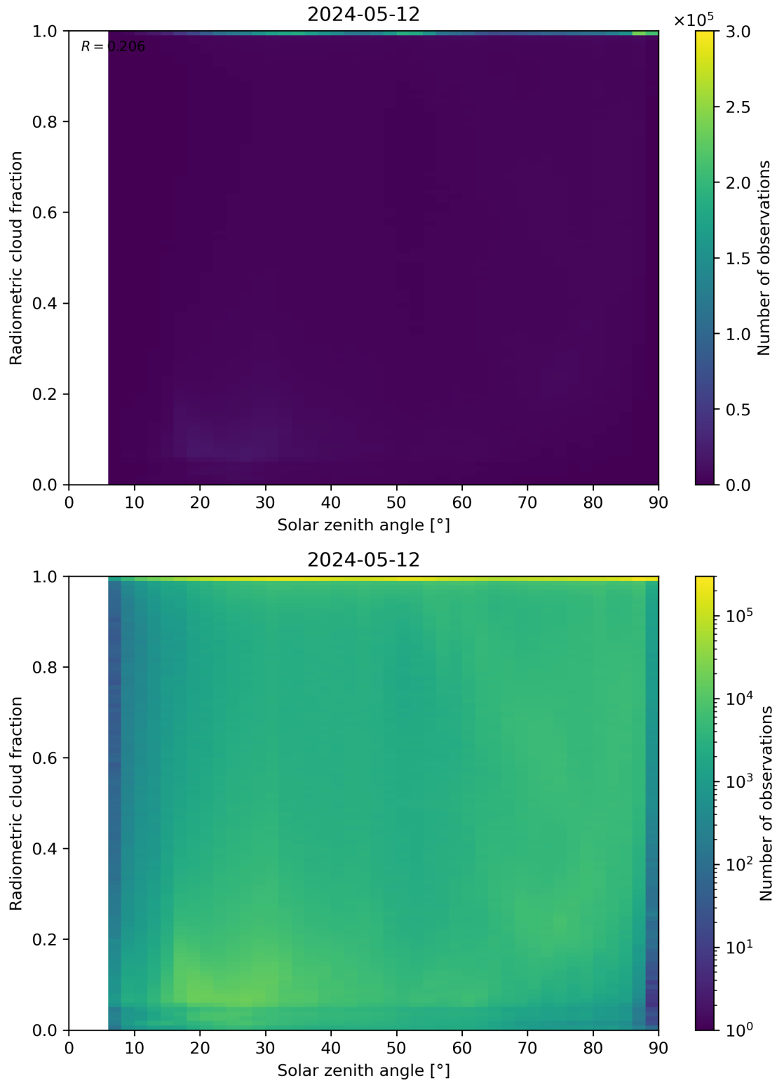
Figure 99: Scatter density plot of “Solar zenith angle” against “Radiometric cloud fraction” for 2024-05-12 to 2024-05-13.
