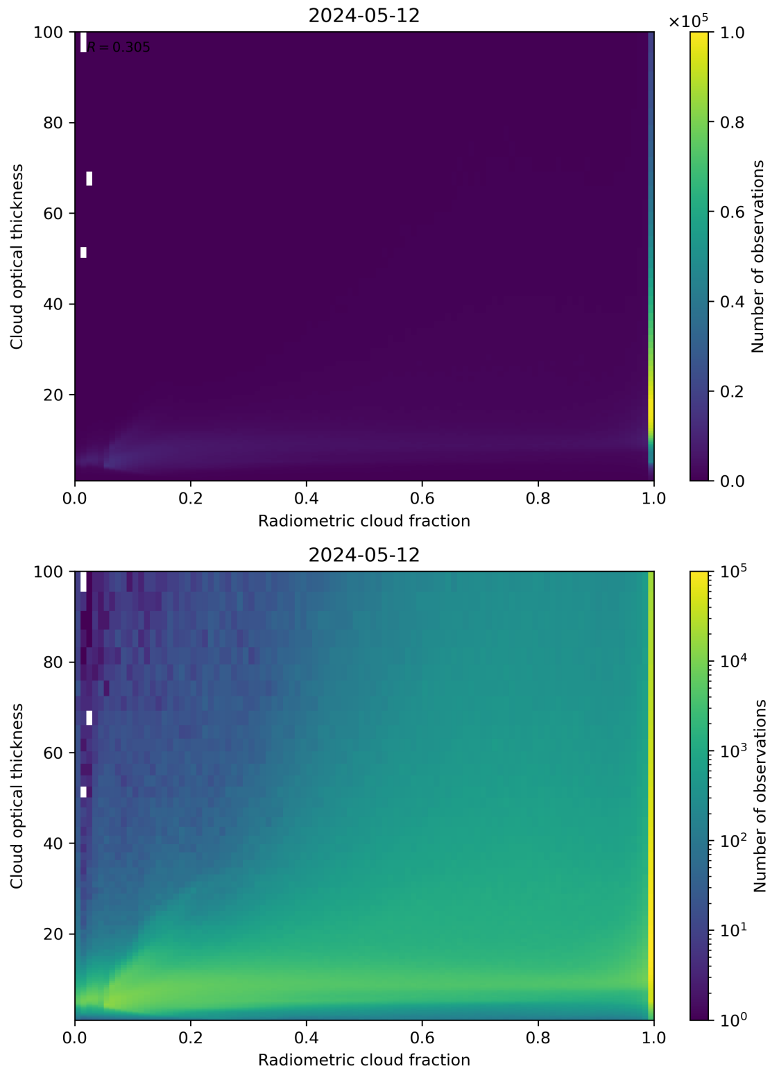
Figure 75: Scatter density plot of “Radiometric cloud fraction” against “Cloud optical thickness” for 2024-05-12 to 2024-05-13.
