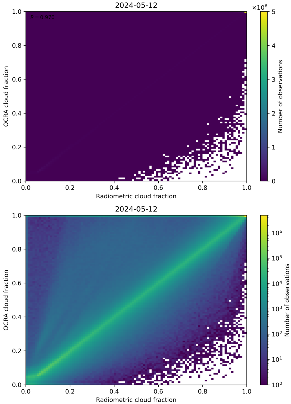
Figure 72: Scatter density plot of “Radiometric cloud fraction” against “OCRA cloud fraction” for 2024-05-12 to 2024-05-13.
