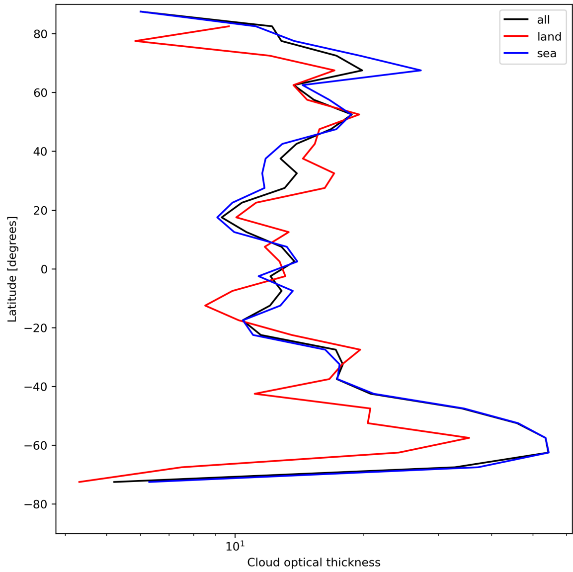
Figure 25: Zonal average of “Cloud optical thickness” for 2024-05-12 to 2024-05-13.
