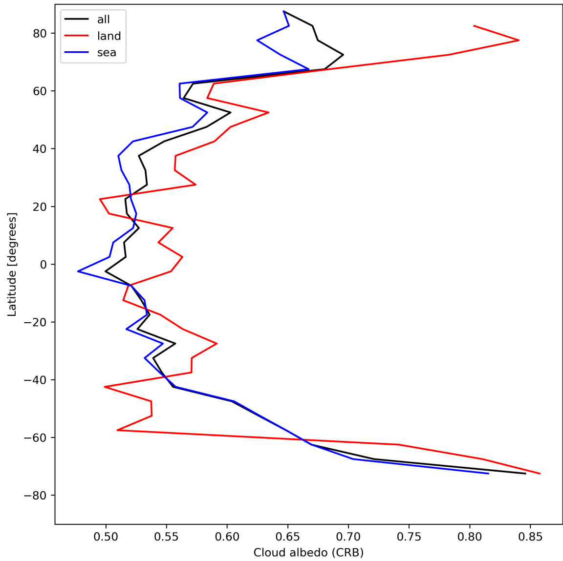
Figure 28: Zonal average of “Cloud albedo (CRB)” for 2024-05-12 to 2024-05-13.
