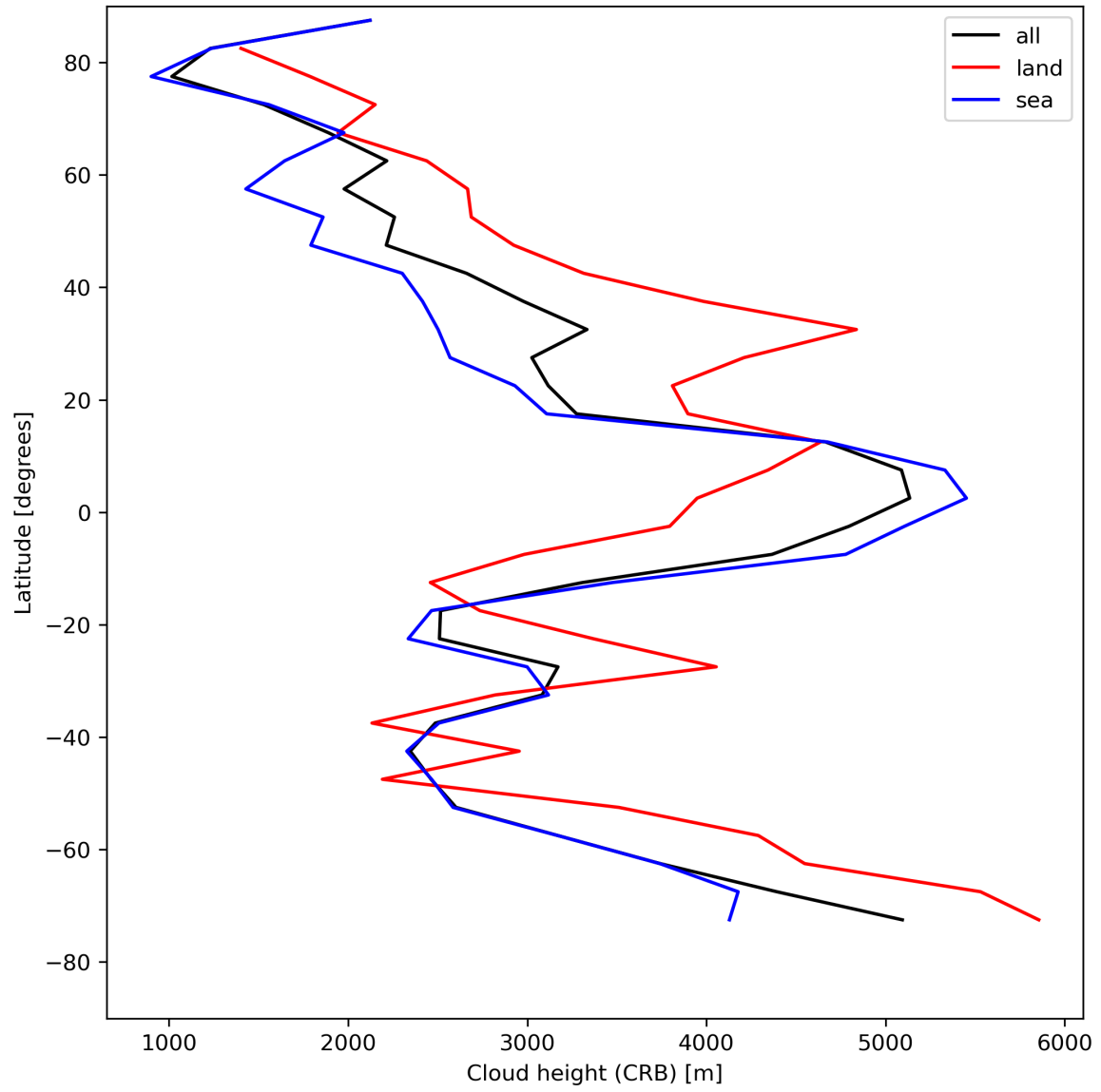
Figure 27: Zonal average of “Cloud height (CRB)” for 2024-05-12 to 2024-05-13.
