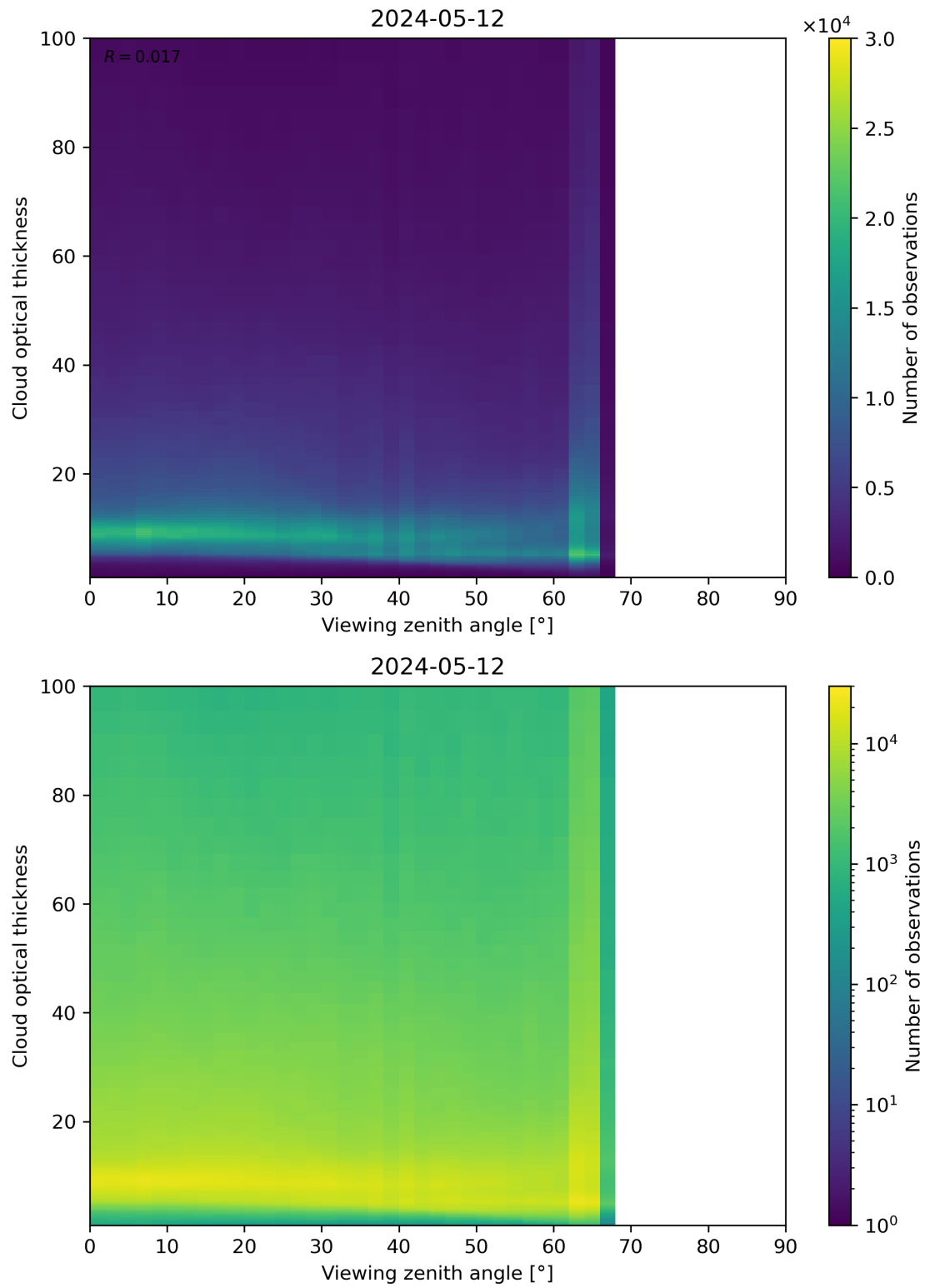
Figure 111: Scatter density plot of “Viewing zenith angle” against “Cloud optical thickness” for 2024-05-12 to 2024-05-13.
