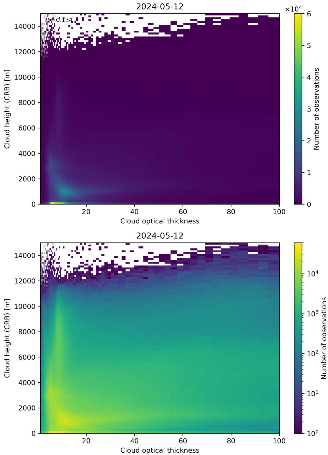
Figure 85: Scatter density plot of “Cloud optical thickness” against “Cloud height (CRB)” for 2024-05-12 to 2024-05-13.
