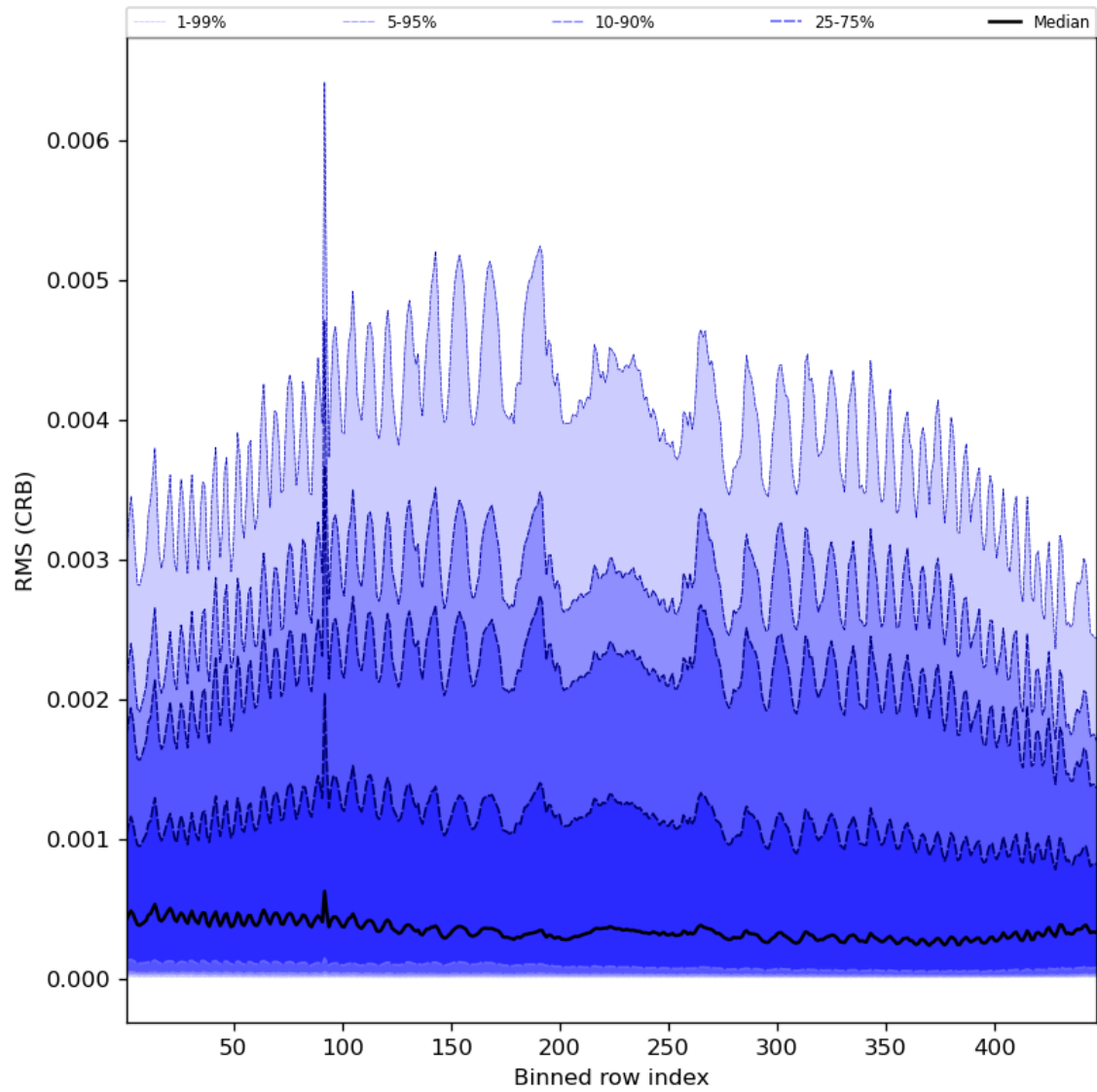
Figure 64: Along track statistics of “RMS (CRB)” for 2024-05-12 to 2024-05-13
