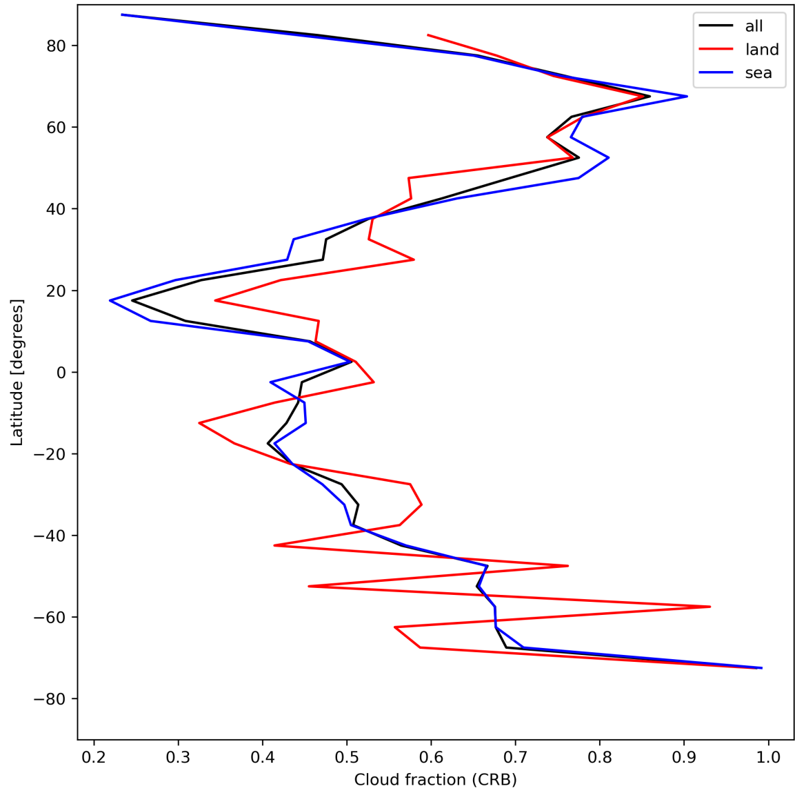
Figure 26: Zonal average of “Cloud fraction (CRB)” for 2024-05-12 to 2024-05-13.
