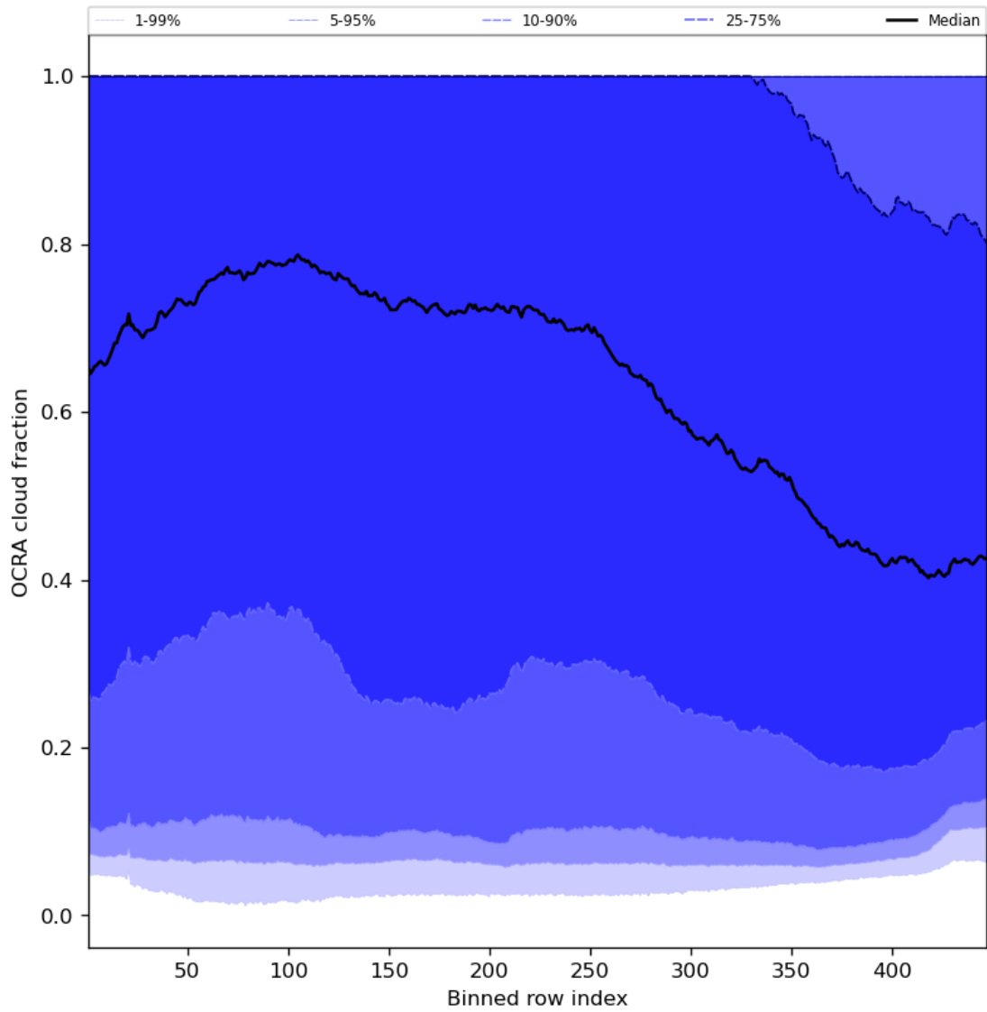
Figure 66: Along track statistics of “OCRA cloud fraction” for 2024-05-12 to 2024-05-13
