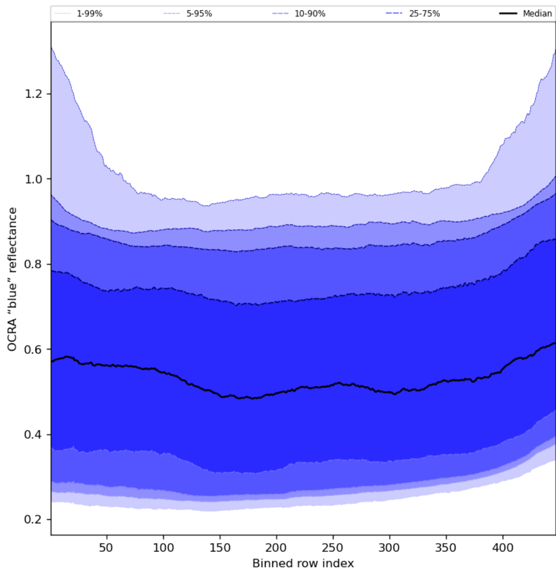
Figure 67: Along track statistics of “OCRA “blue” reflectance” for 2024-05-12 to 2024-05-13
