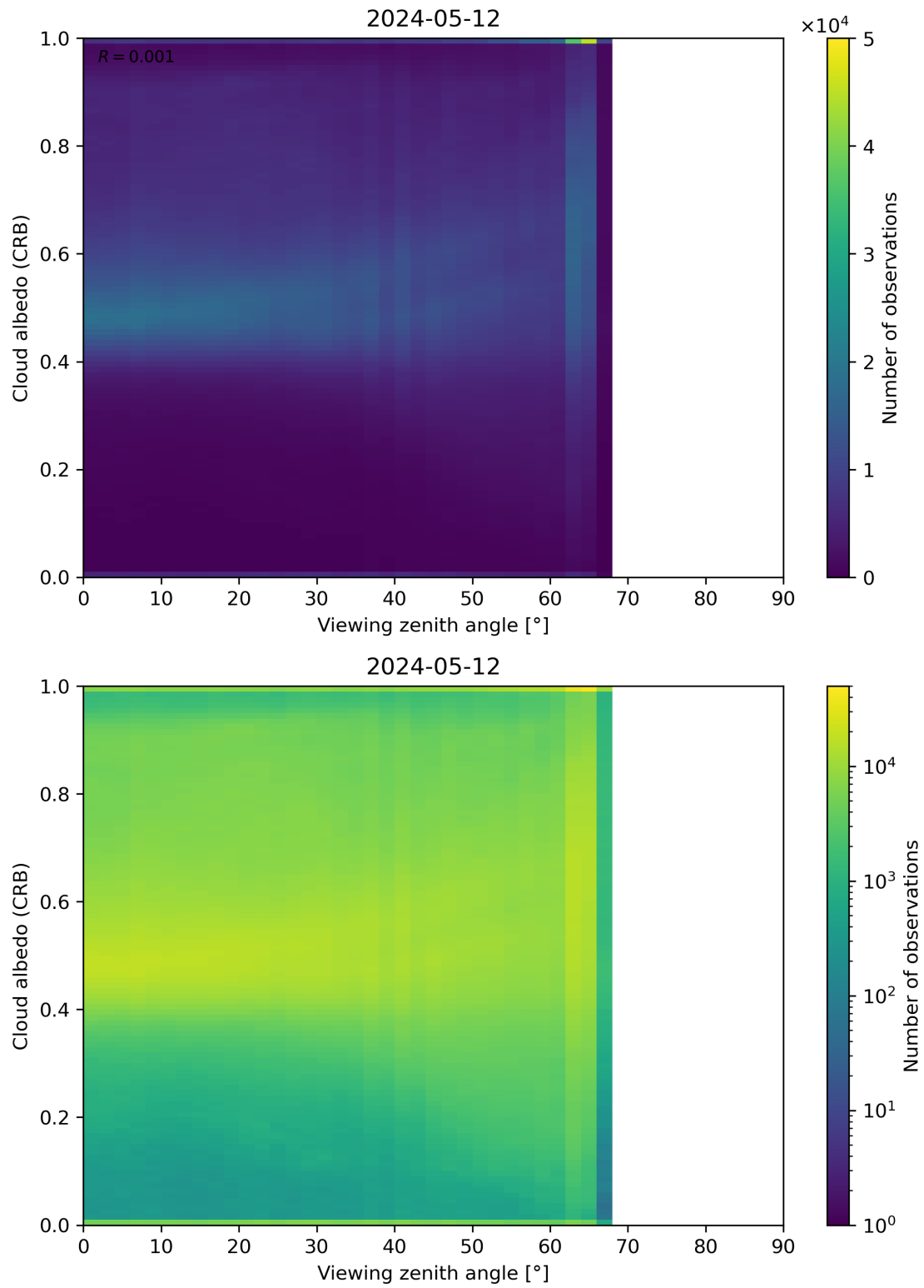
Figure 106: Scatter density plot of “Viewing zenith angle” against “Cloud albedo (CRB)” for 2024-05-12 to 2024-05-13.
