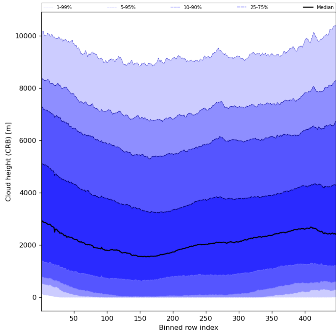
Figure 59: Along track statistics of “Cloud height (CRB)” for 2024-05-12 to 2024-05-13
