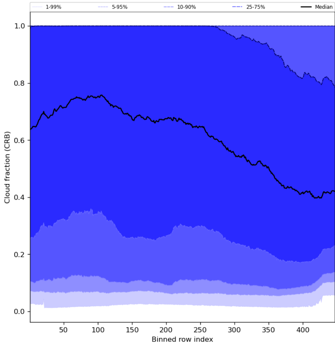
Figure 58: Along track statistics of “Cloud fraction (CRB)” for 2024-05-12 to 2024-05-13
