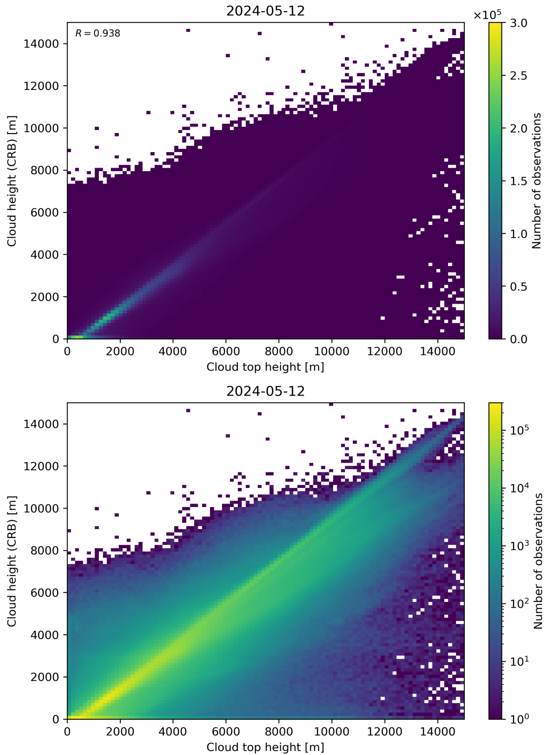
Figure 89: Scatter density plot of “Cloud top height” against “Cloud height (CRB)” for 2024-05-12 to 2024-05-13.
