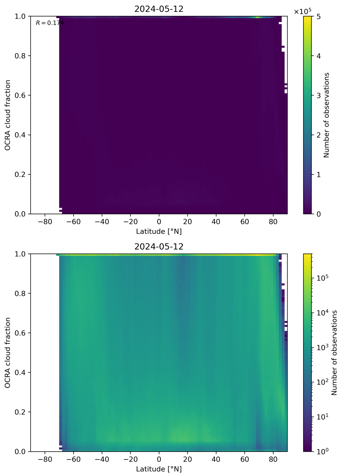
Figure 93: Scatter density plot of “Latitude” against “OCRA cloud fraction” for 2024-05-12 to 2024-05-13.
