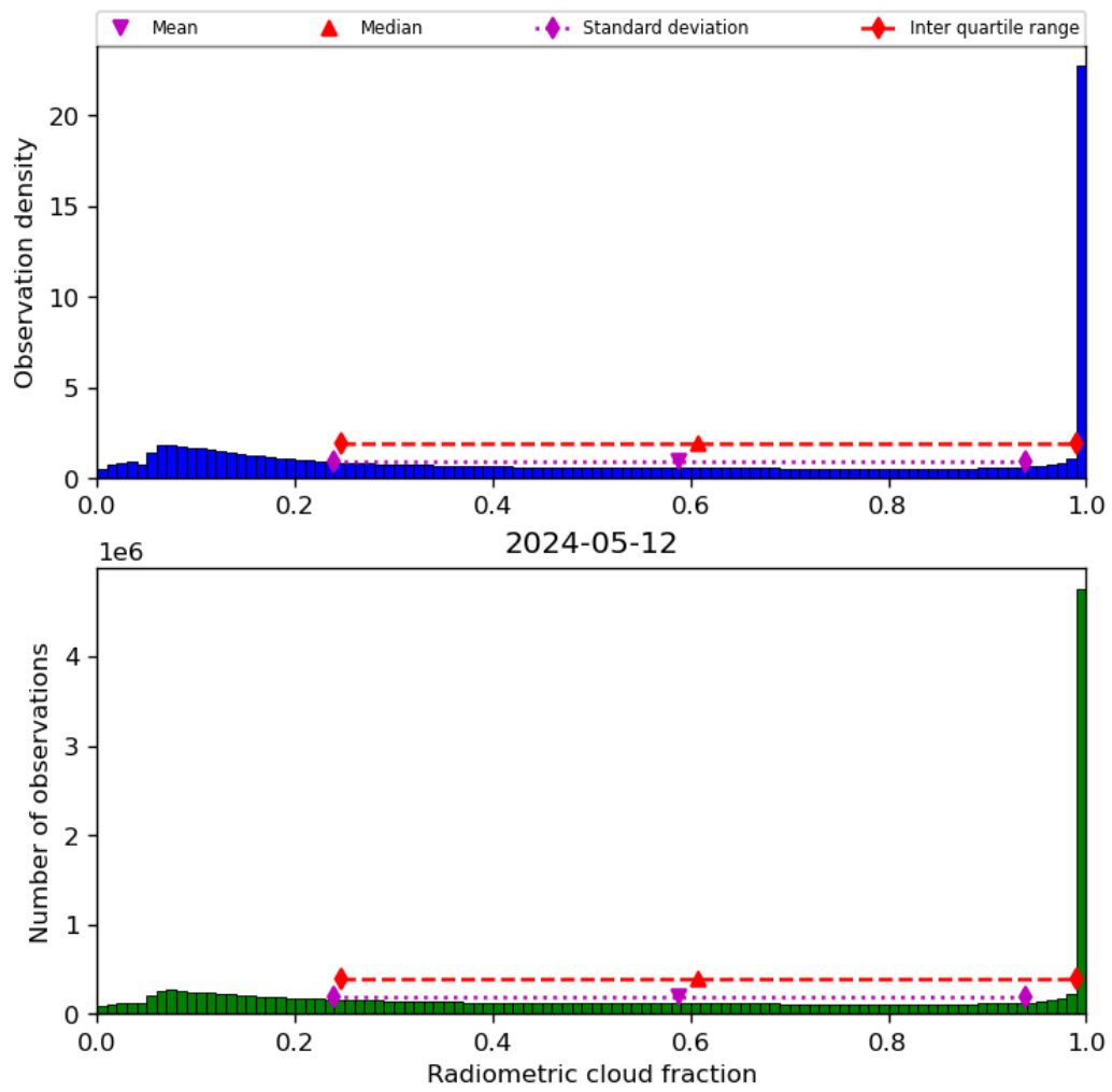
Figure 39: Histogram of “Radiometric cloud fraction” for 2024-05-12 to 2024-05-13
