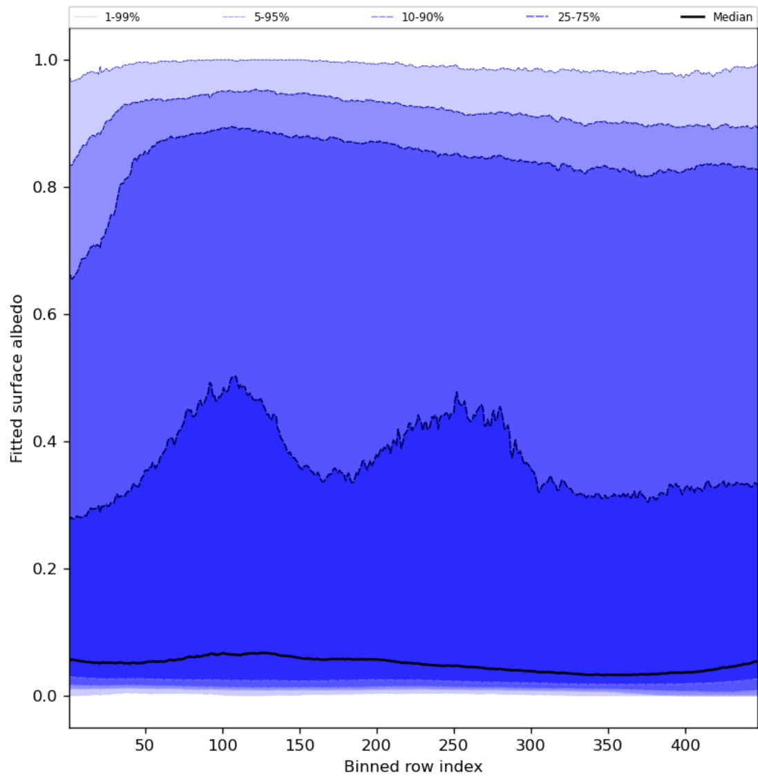
Figure 61: Along track statistics of “Fitted surface albedo” for 2024-05-12 to 2024-05-13
