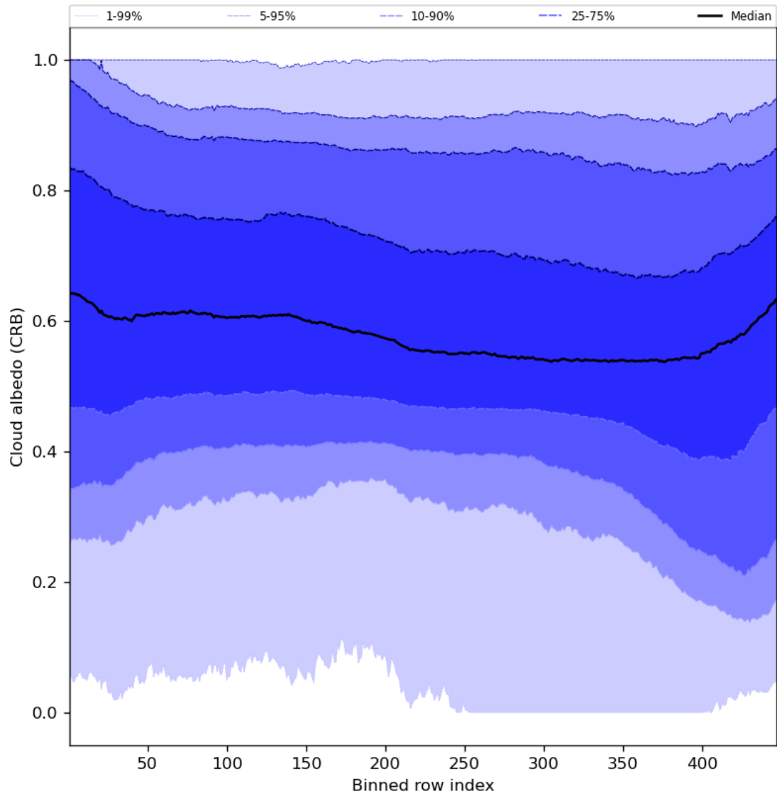
Figure 60: Along track statistics of “Cloud albedo (CRB)” for 2024-05-12 to 2024-05-13
