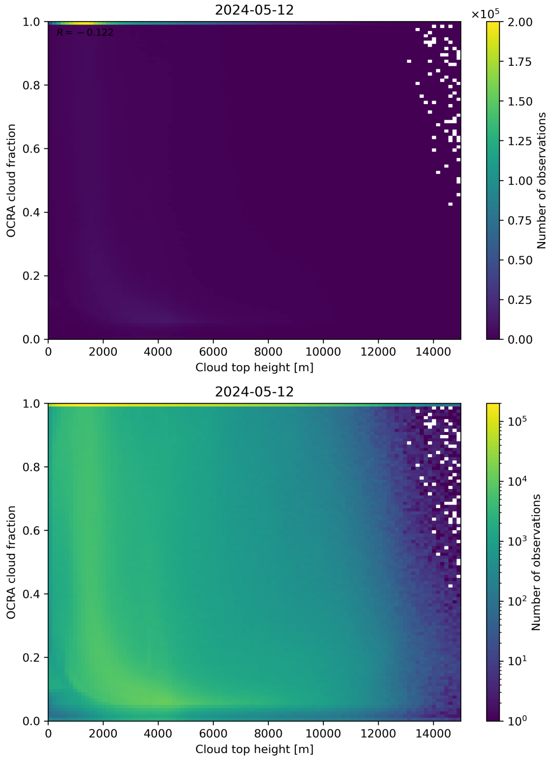
Figure 87: Scatter density plot of “Cloud top height” against “OCRA cloud fraction” for 2024-05-12 to 2024-05-13.
