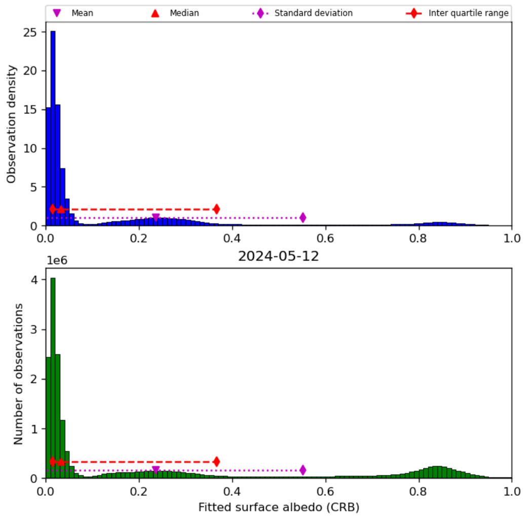
Figure 46: Histogram of “Fitted surface albedo (CRB)” for 2024-05-12 to 2024-05-13
