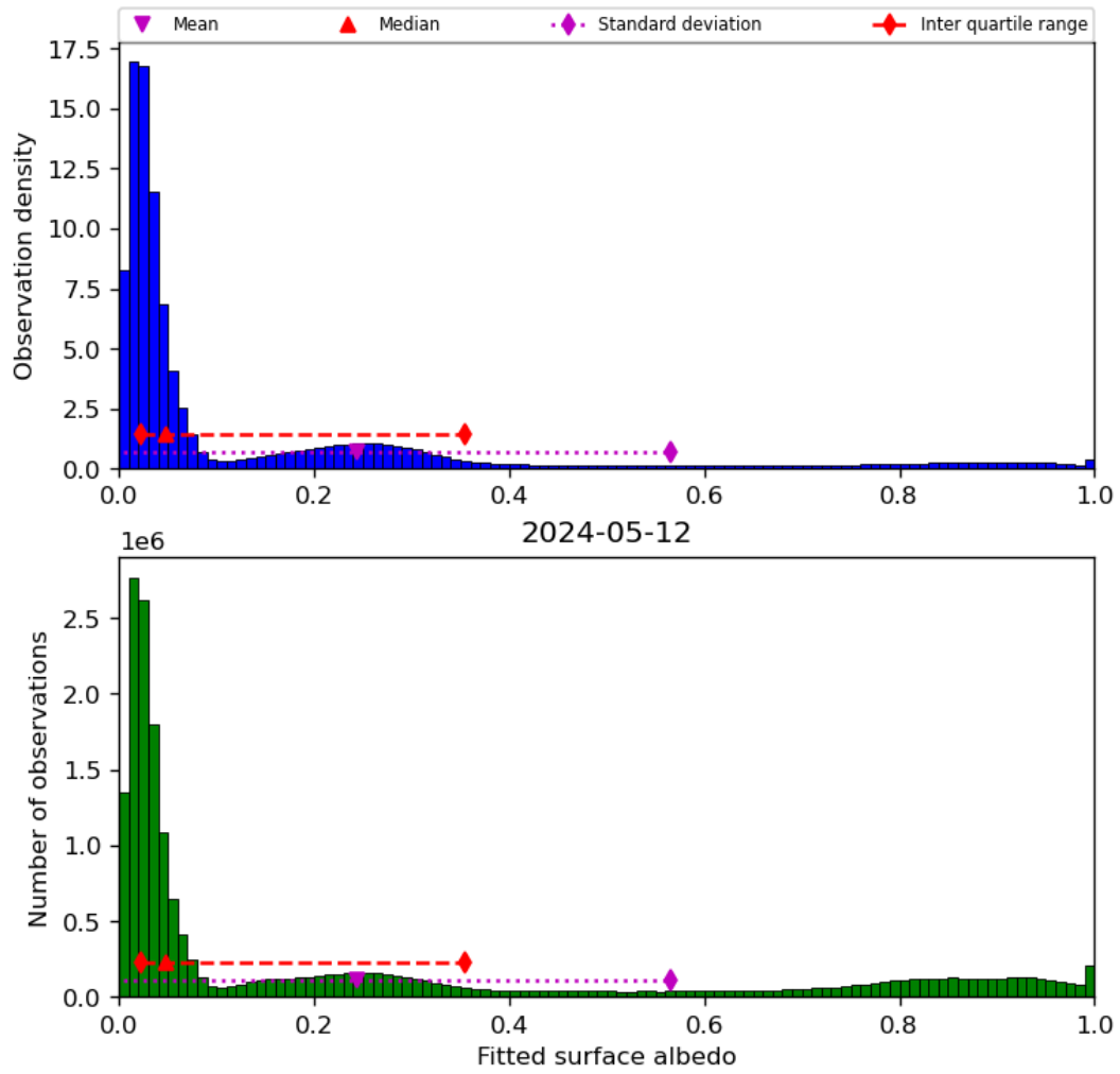
Figure 45: Histogram of “Fitted surface albedo” for 2024-05-12 to 2024-05-13
