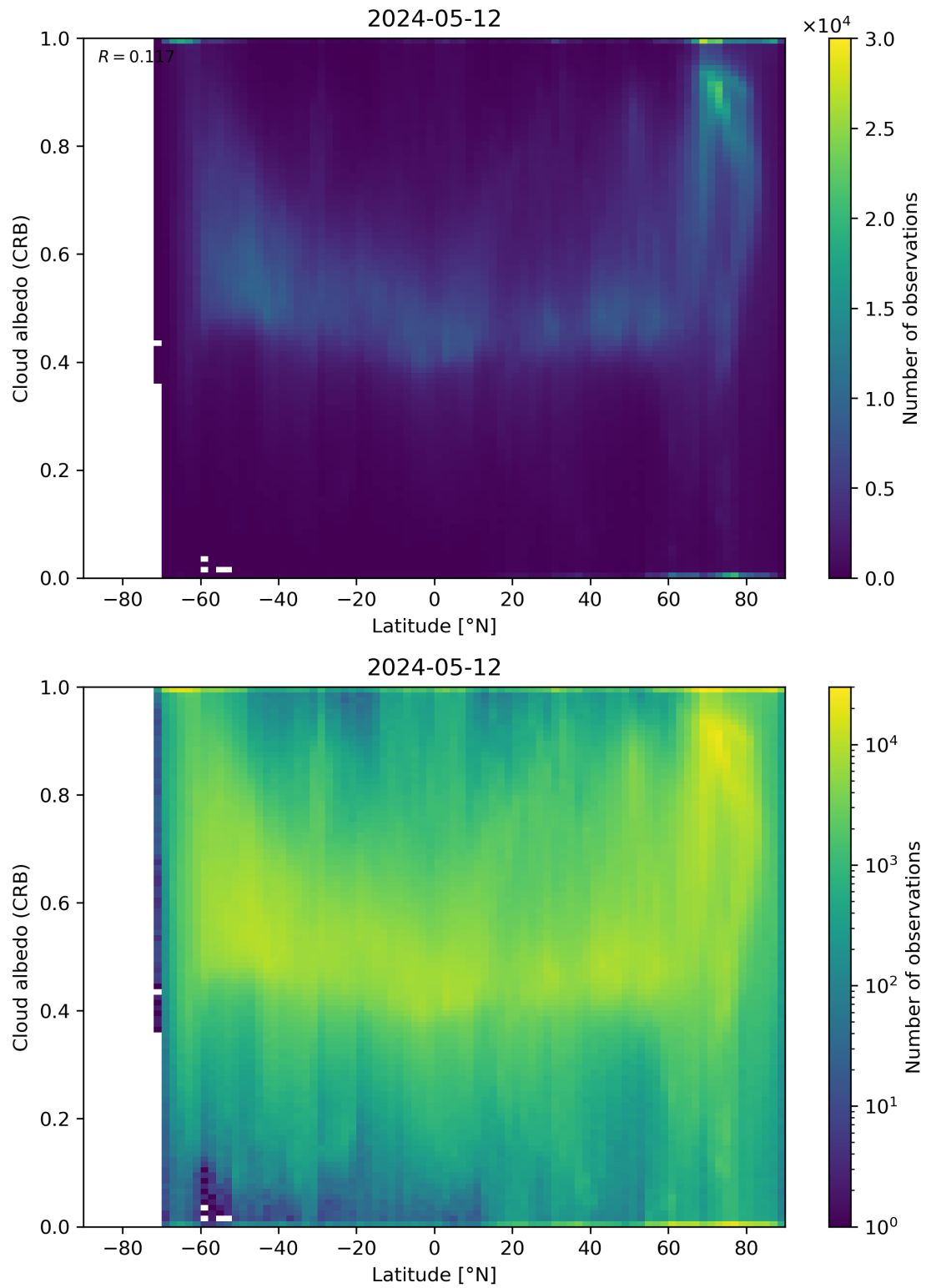
Figure 91: Scatter density plot of “Latitude” against “Cloud albedo (CRB)” for 2024-05-12 to 2024-05-13.
