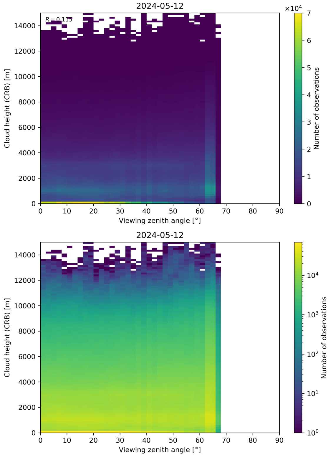
Figure 110: Scatter density plot of “Viewing zenith angle” against “Cloud height (CRB)” for 2024-05-12 to 2024-05-13.
