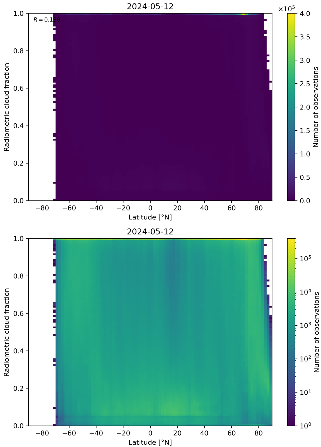
Figure 92: Scatter density plot of “Latitude” against “Radiometric cloud fraction” for 2024-05-12 to 2024-05-13.
