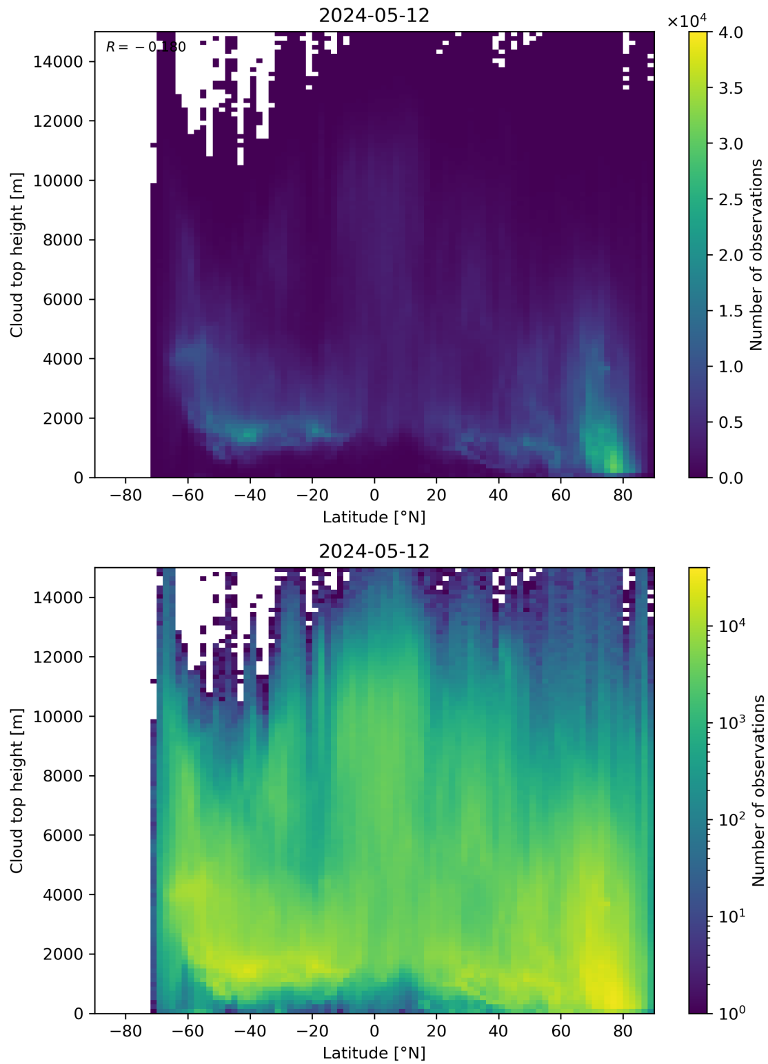
Figure 97: Scatter density plot of “Latitude” against “Cloud top height” for 2024-05-12 to 2024-05-13.
