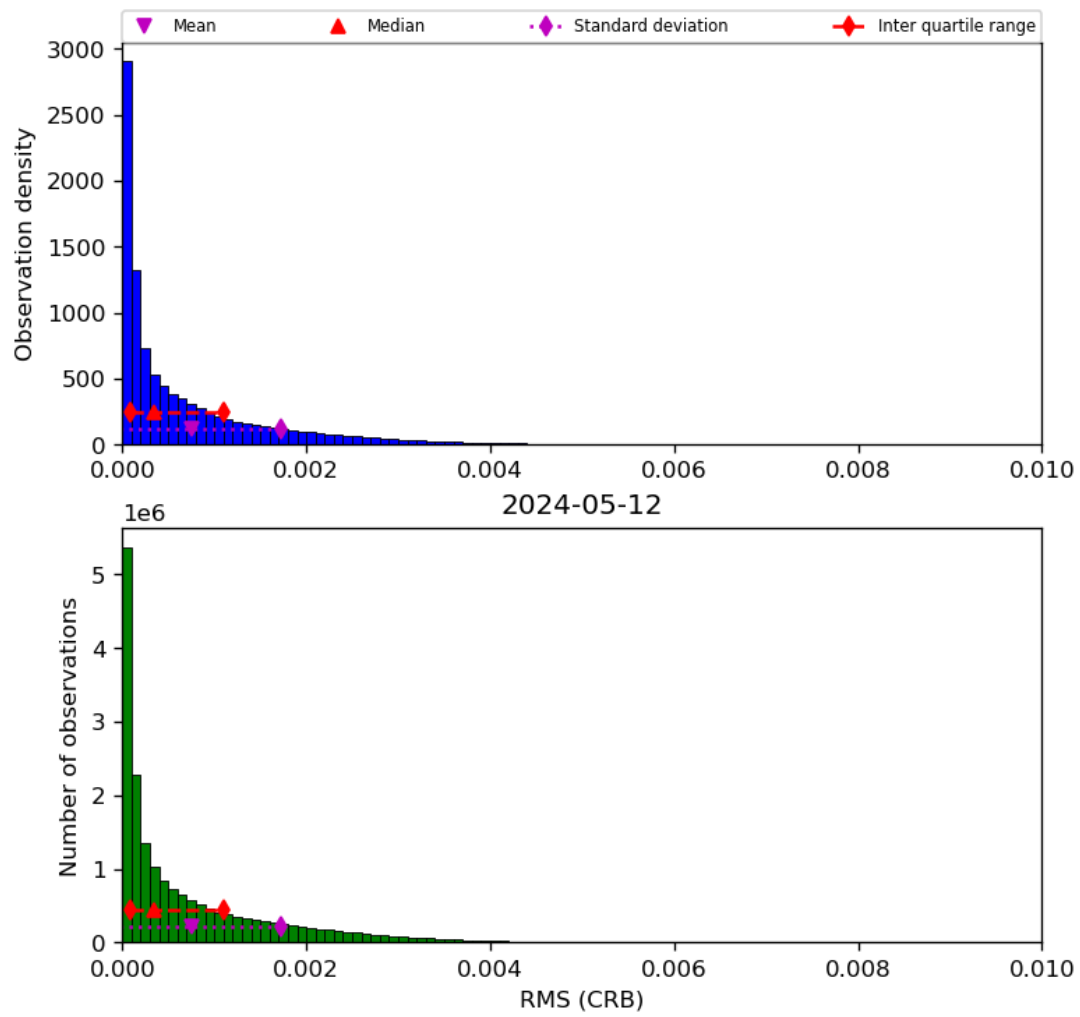
Figure 48: Histogram of “RMS (CRB)” for 2024-05-12 to 2024-05-13
