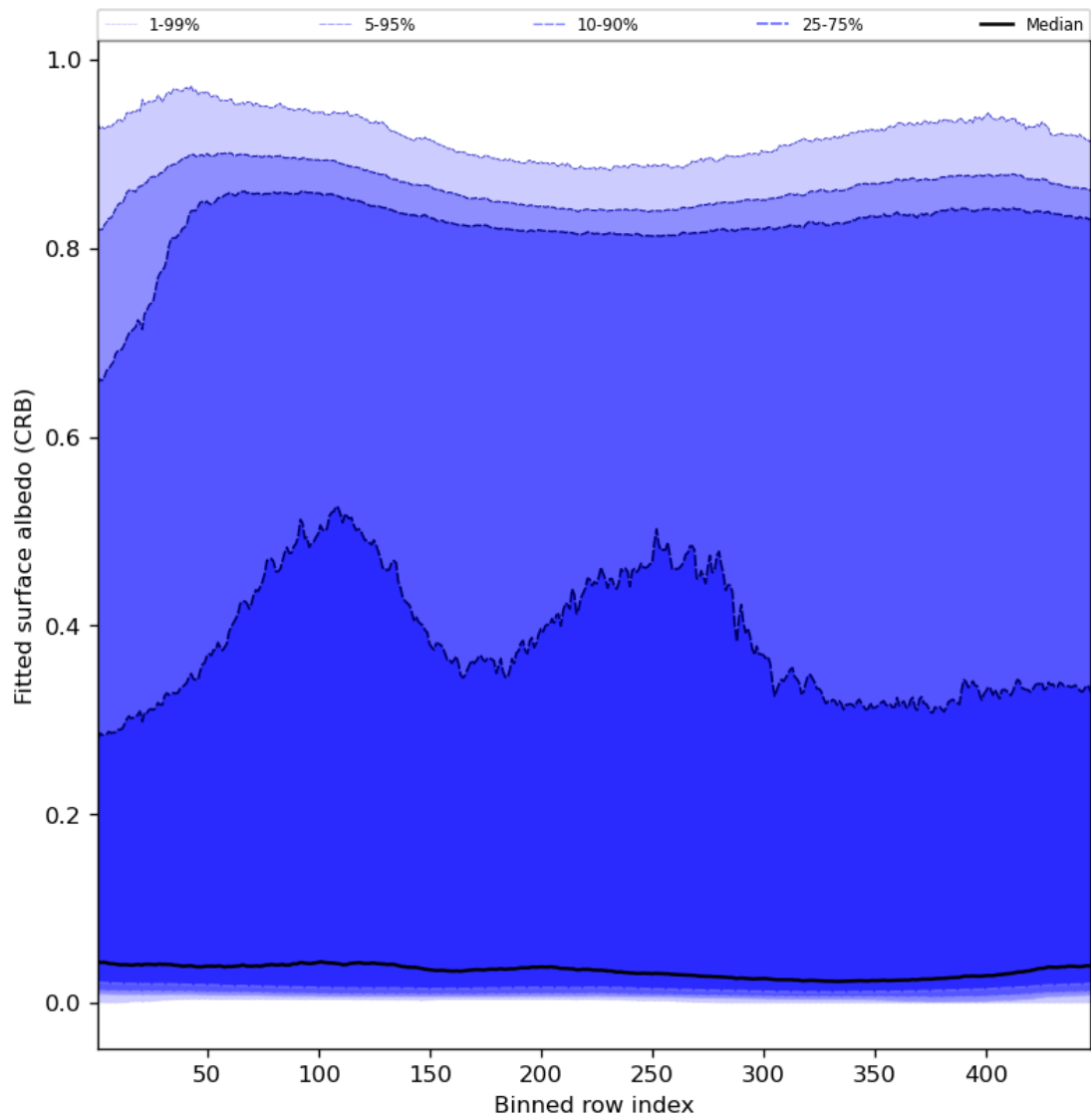
Figure 62: Along track statistics of “Fitted surface albedo (CRB)” for 2024-05-12 to 2024-05-13
