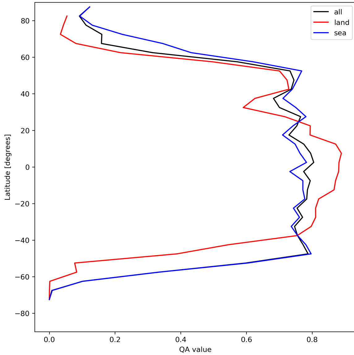
Figure 22: Zonal average of “QA value” for 2024-05-12 to 2024-05-13.
