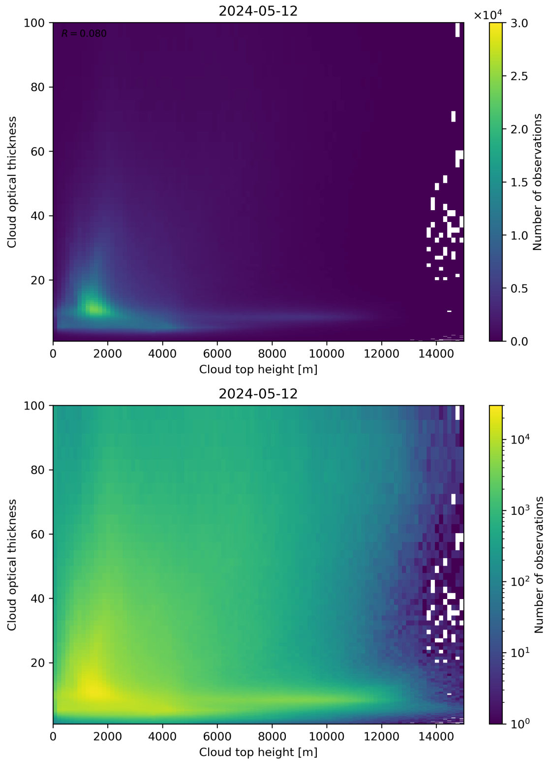
Figure 90: Scatter density plot of “Cloud top height” against “Cloud optical thickness” for 2024-05-12 to 2024-05-13.
