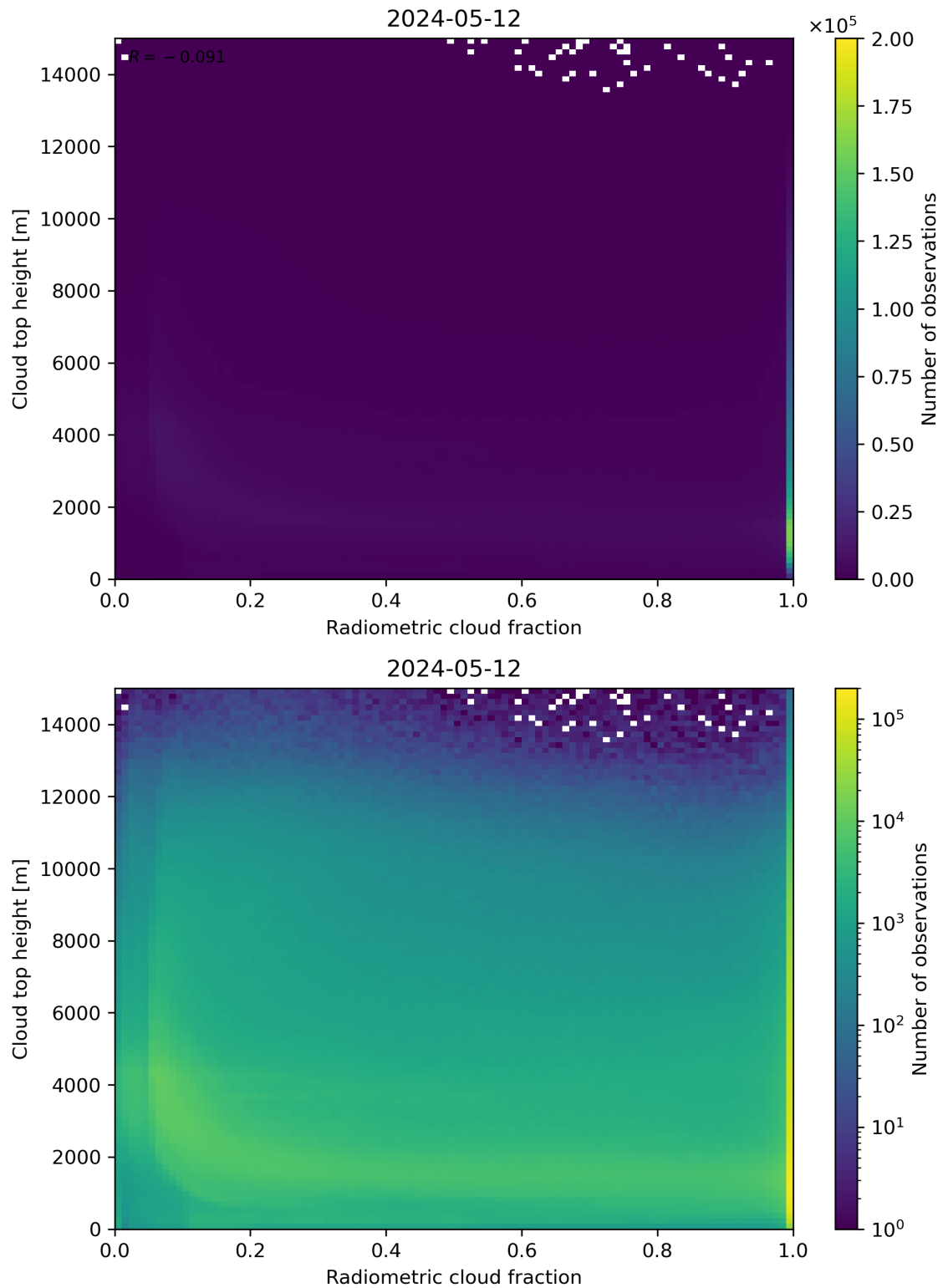
Figure 76: Scatter density plot of “Radiometric cloud fraction” against “Cloud top height” for 2024-05-12 to 2024-05-13.
