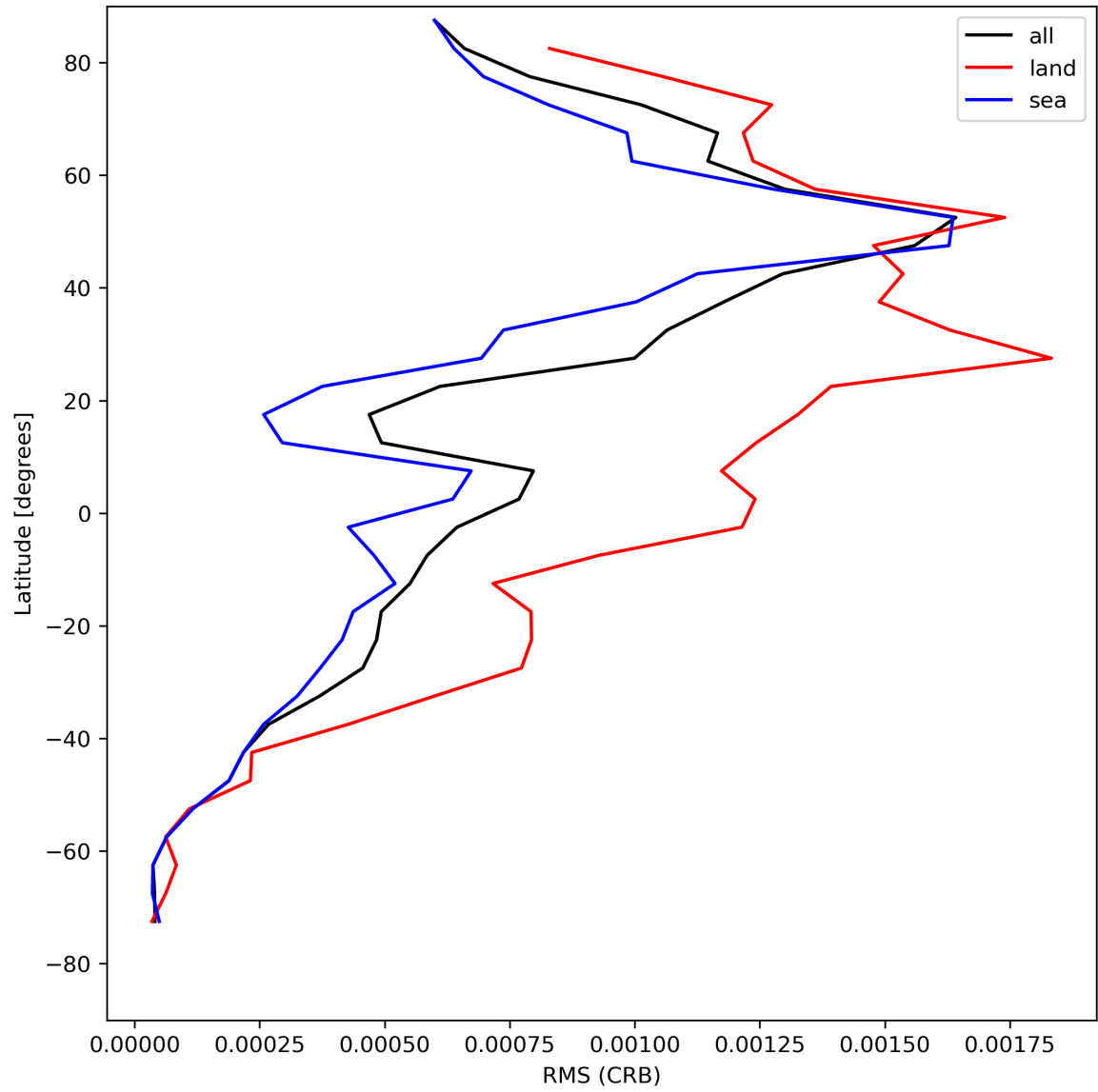
Figure 32: Zonal average of “RMS (CRB)” for 2024-05-12 to 2024-05-13.
