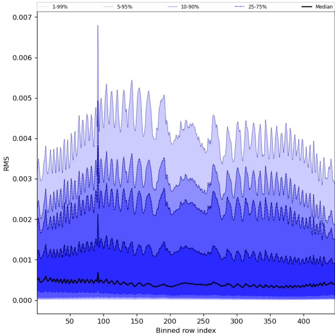
Figure 63: Along track statistics of “RMS” for 2024-05-12 to 2024-05-13
