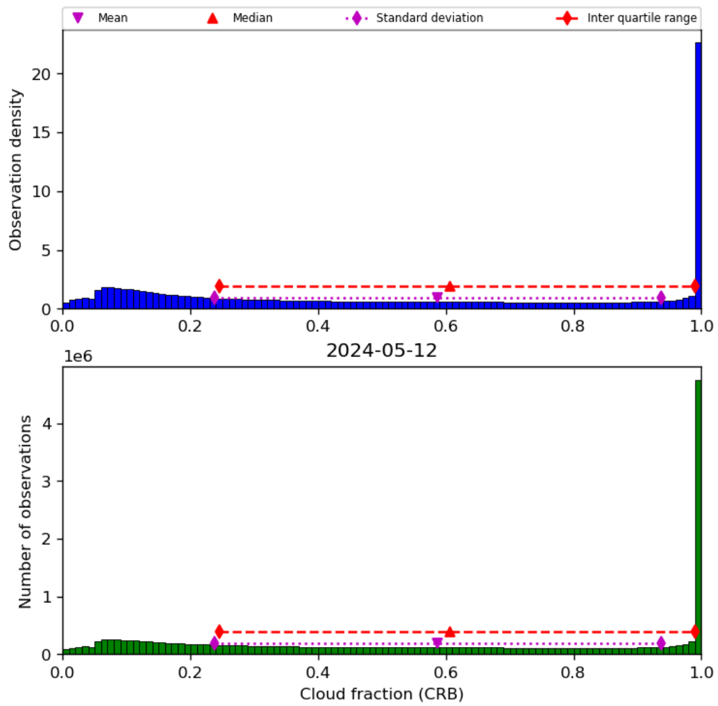
Figure 42: Histogram of “Cloud fraction (CRB)” for 2024-05-12 to 2024-05-13
