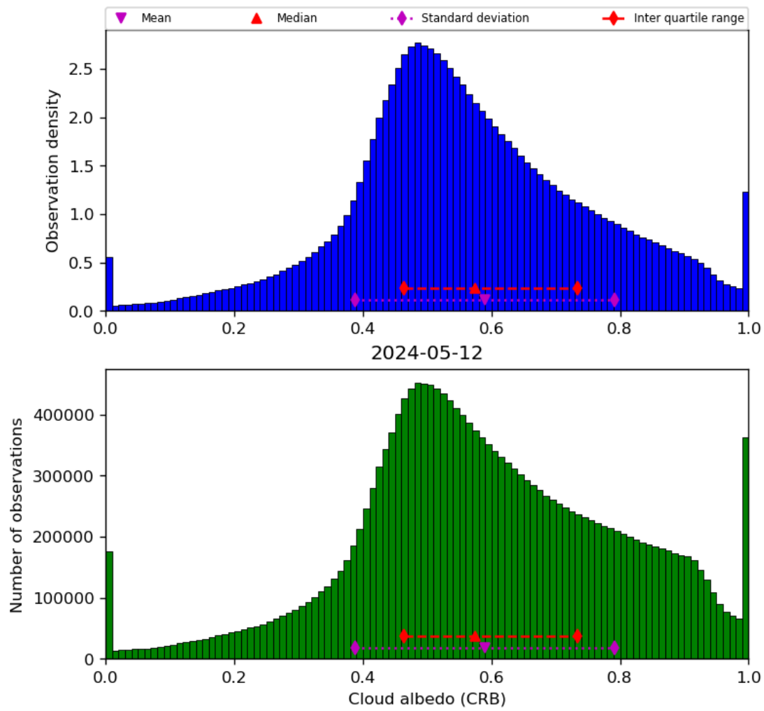
Figure 44: Histogram of “Cloud albedo (CRB)” for 2024-05-12 to 2024-05-13
