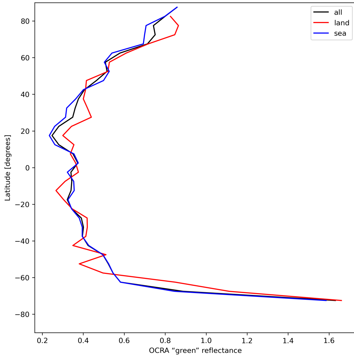
Figure 36: Zonal average of “OCRA “green” reflectance” for 2024-05-12 to 2024-05-13.
