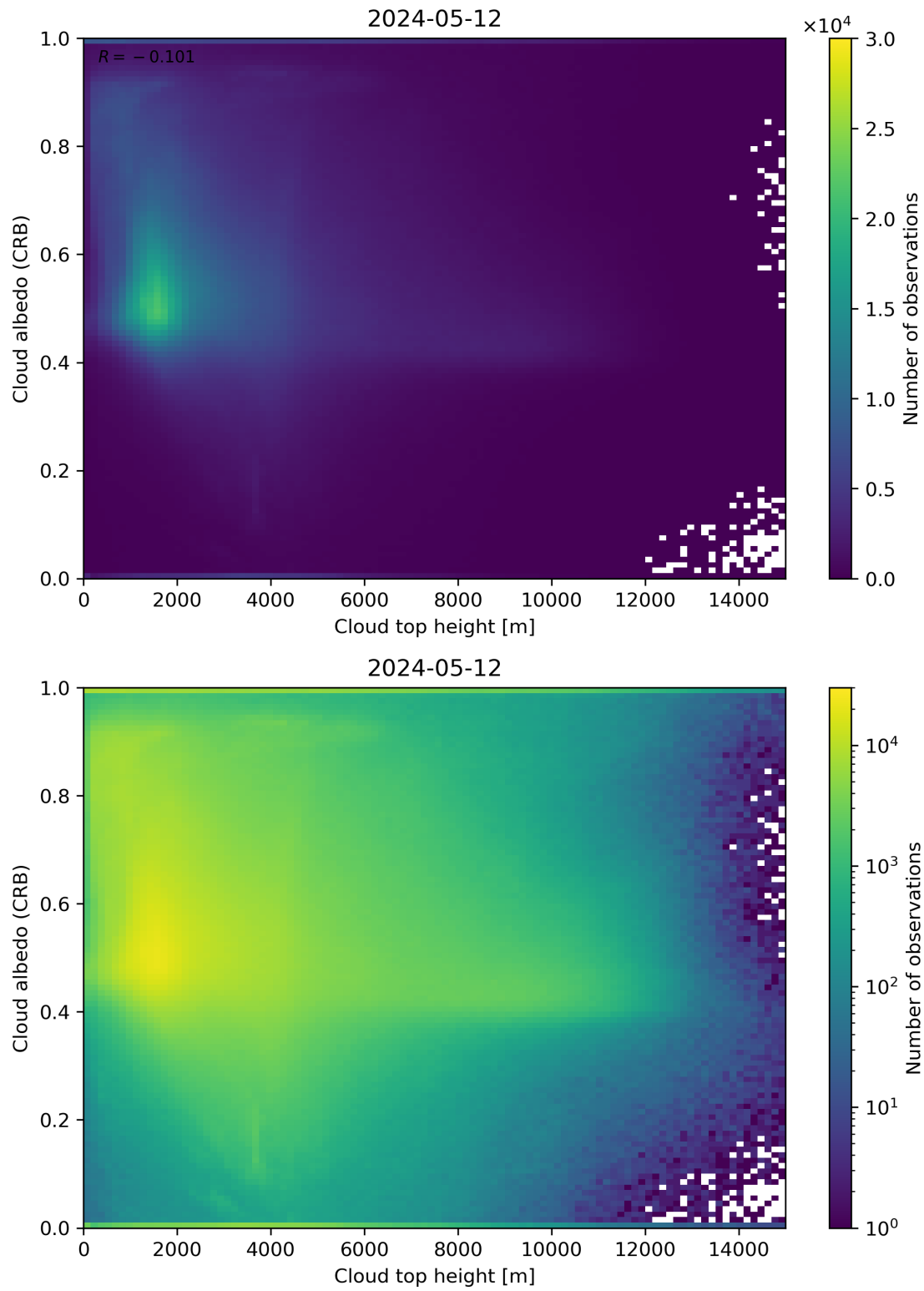
Figure 86: Scatter density plot of “Cloud top height” against “Cloud albedo (CRB)” for 2024-05-12 to 2024-05-13.
