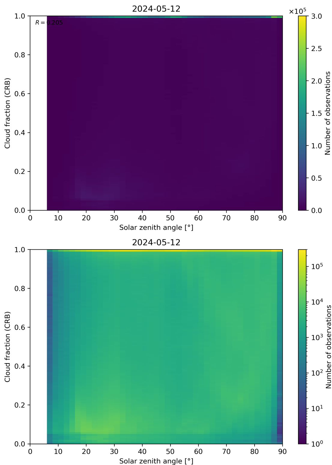
Figure 101: Scatter density plot of “Solar zenith angle” against “Cloud fraction (CRB)” for 2024-05-12 to 2024-05-13.
