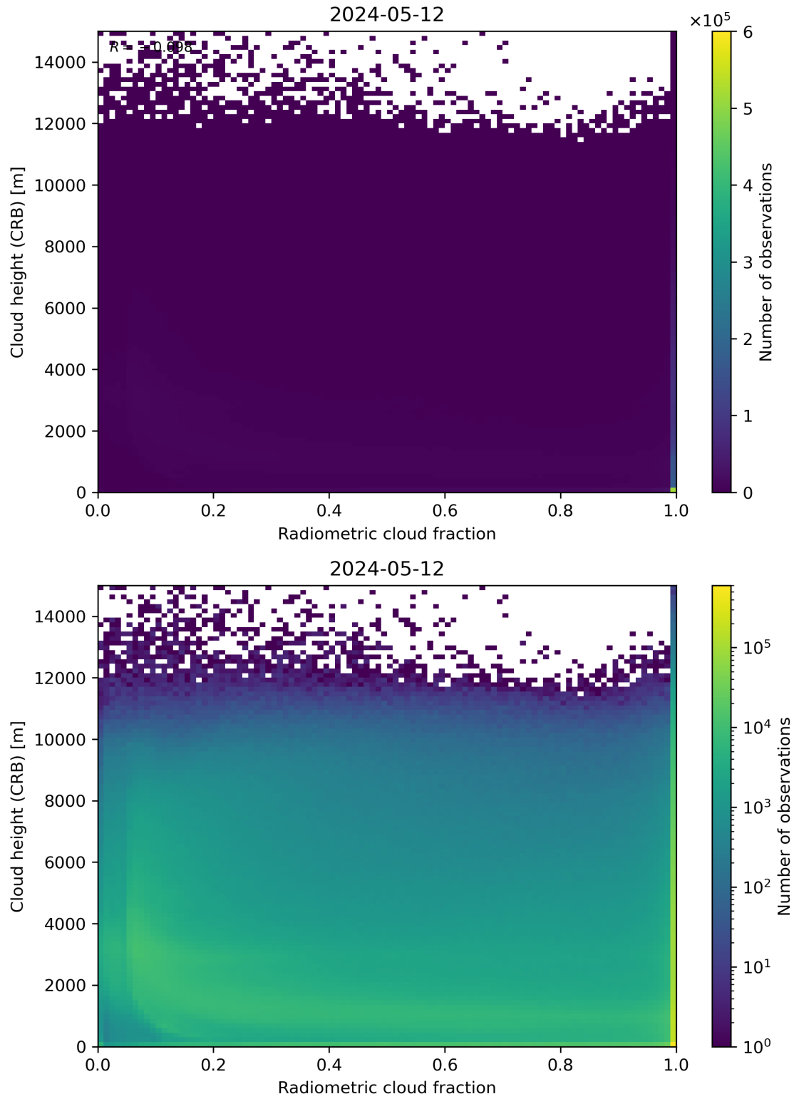
Figure 74: Scatter density plot of “Radiometric cloud fraction” against “Cloud height (CRB)” for 2024-05-12 to 2024-05-13.
