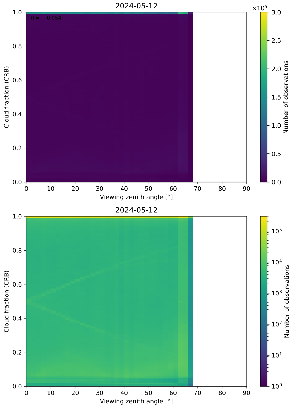
Figure 109: Scatter density plot of “Viewing zenith angle” against “Cloud fraction (CRB)” for 2024-05-12 to 2024-05-13.
