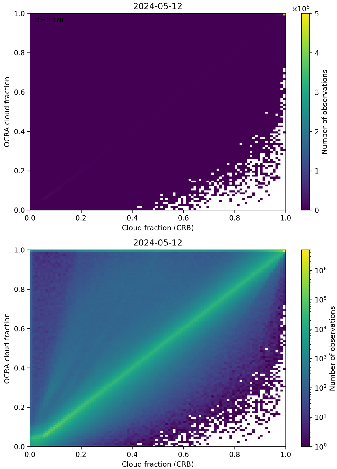
Figure 78: Scatter density plot of “Cloud fraction (CRB)” against “OCRA cloud fraction” for 2024-05-12 to 2024-05-13.
