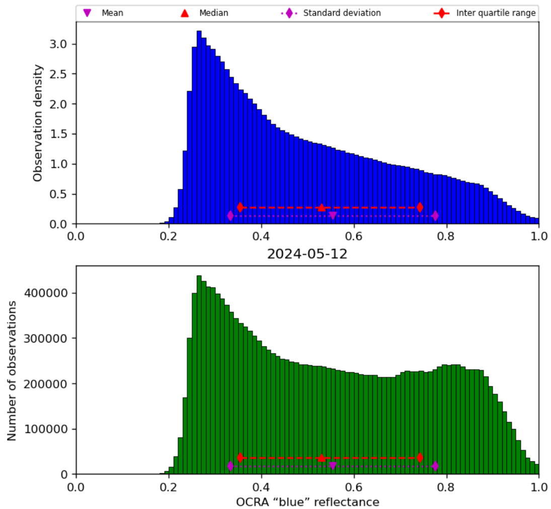
Figure 51: Histogram of “OCRA “blue” reflectance” for 2024-05-12 to 2024-05-13
