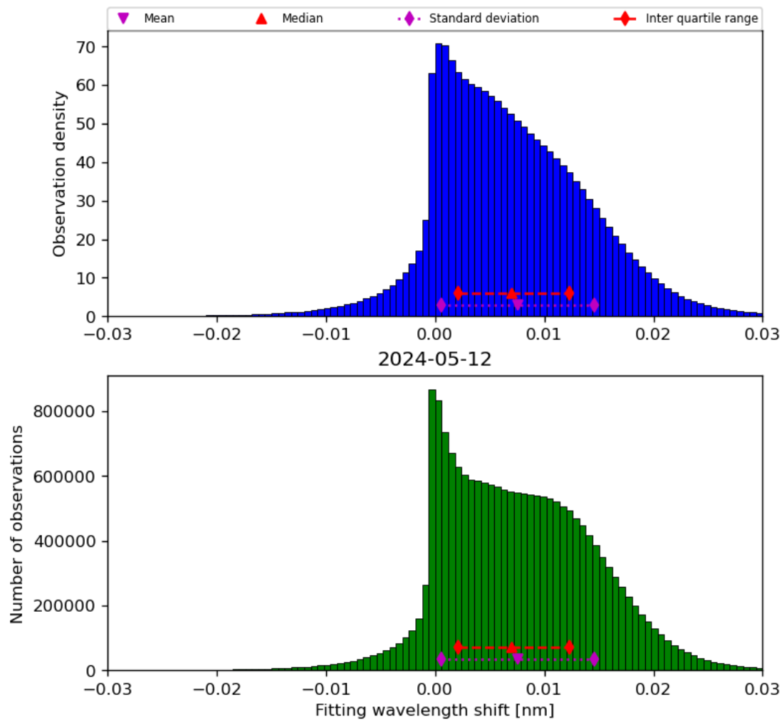
Figure 49: Histogram of “Fitting wavelength shift” for 2024-05-12 to 2024-05-13
