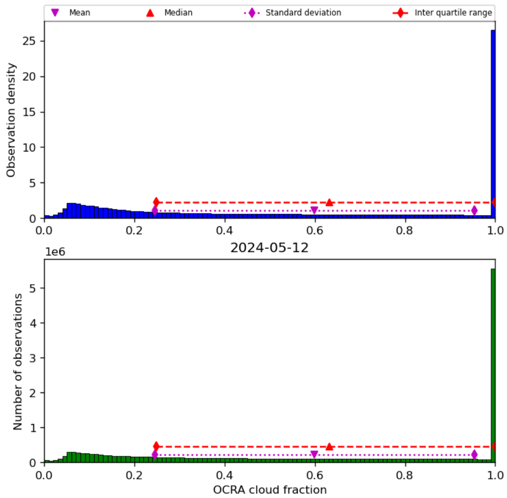
Figure 50: Histogram of “OCRA cloud fraction” for 2024-05-12 to 2024-05-13
