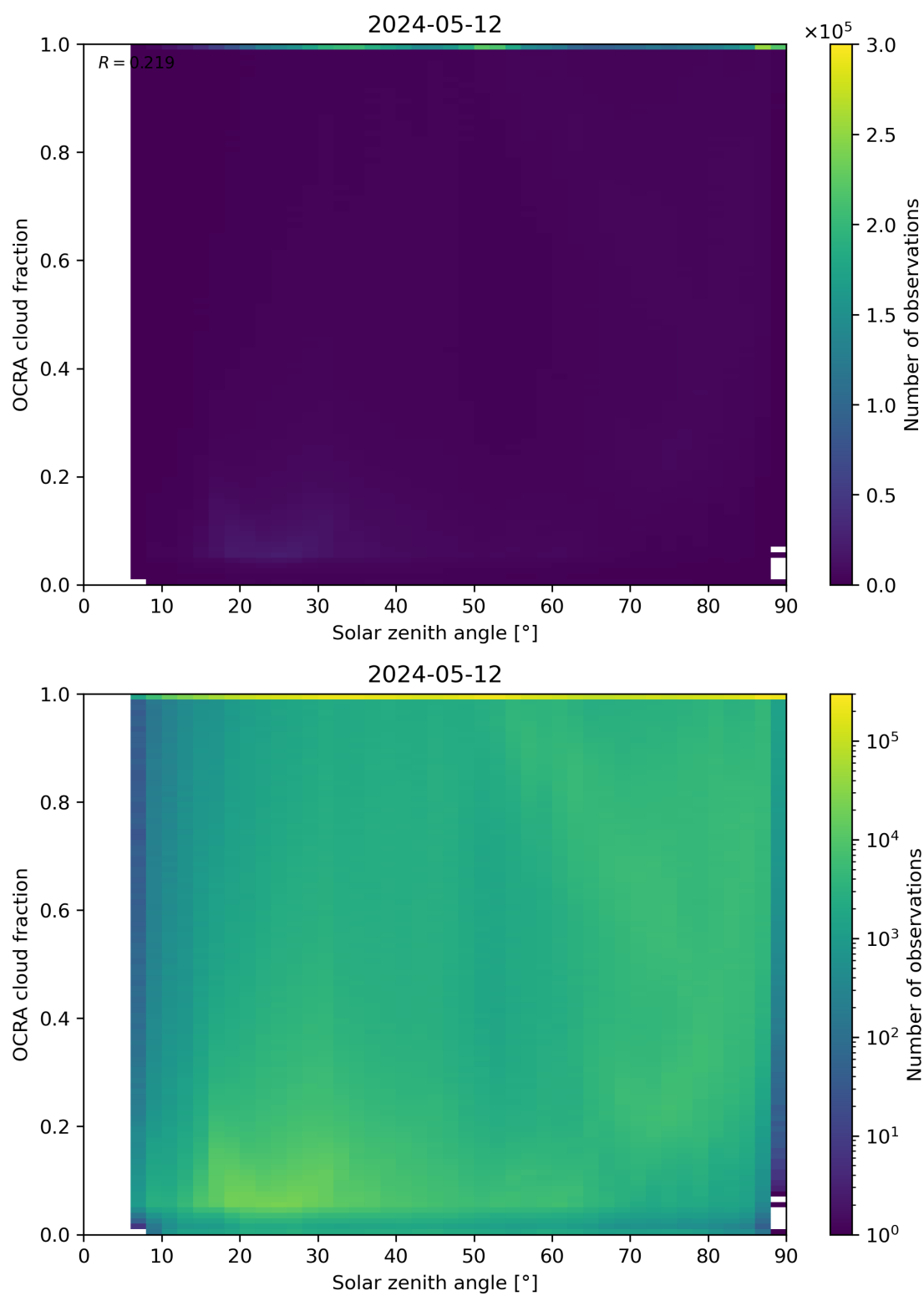
Figure 100: Scatter density plot of “Solar zenith angle” against “OCRA cloud fraction” for 2024-05-12 to 2024-05-13.
