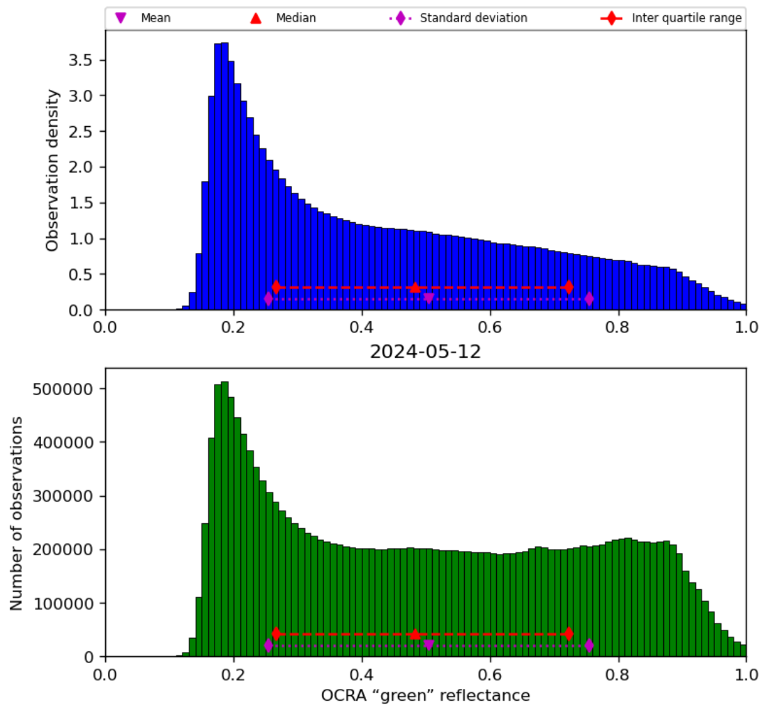
Figure 52: Histogram of “OCRA “green” reflectance” for 2024-05-12 to 2024-05-13
