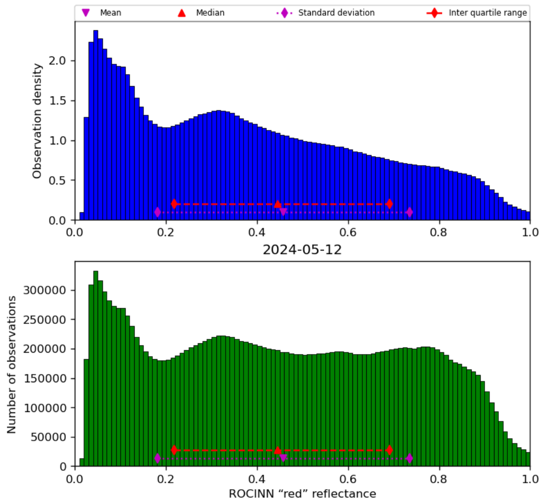
Figure 53: Histogram of “ROCINN “red” reflectance” for 2024-05-12 to 2024-05-13
