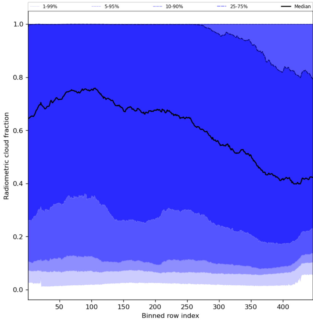
Figure 55: Along track statistics of “Radiometric cloud fraction” for 2024-05-12 to 2024-05-13
