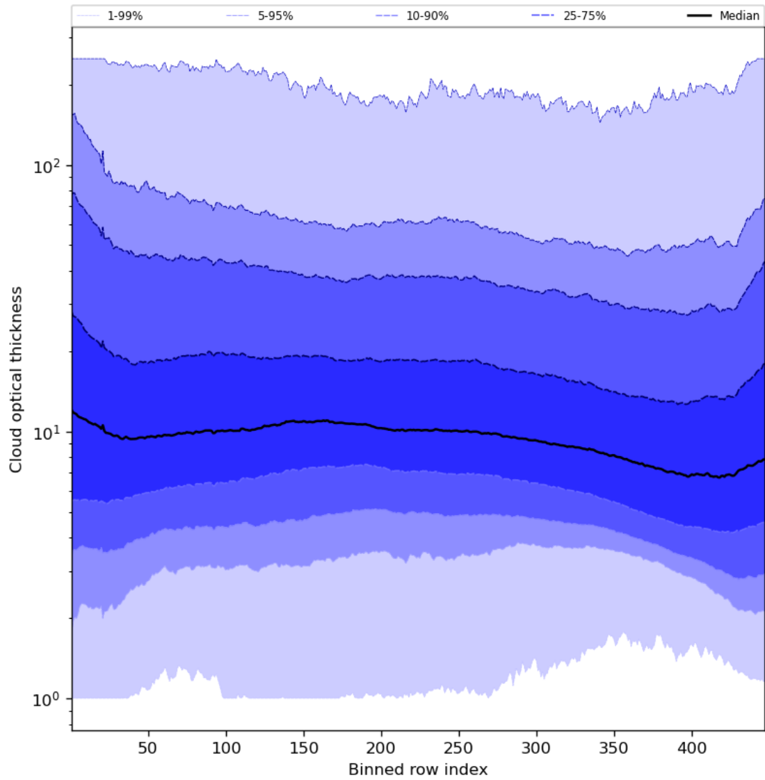
Figure 57: Along track statistics of “Cloud optical thickness” for 2024-05-12 to 2024-05-13
