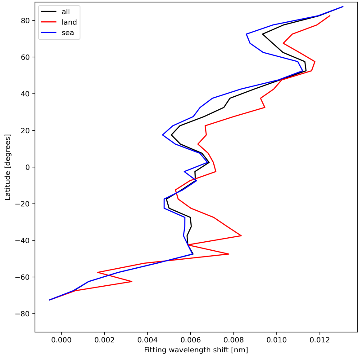
Figure 33: Zonal average of “Fitting wavelength shift” for 2024-05-12 to 2024-05-13.
