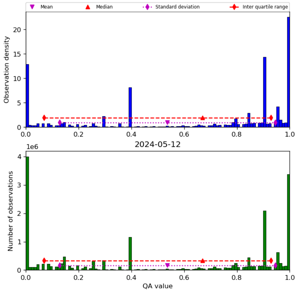
Figure 38: Histogram of “QA value” for 2024-05-12 to 2024-05-13
