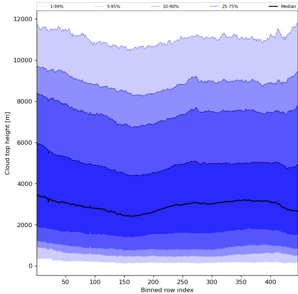
Figure 56: Along track statistics of “Cloud top height” for 2024-05-12 to 2024-05-13
