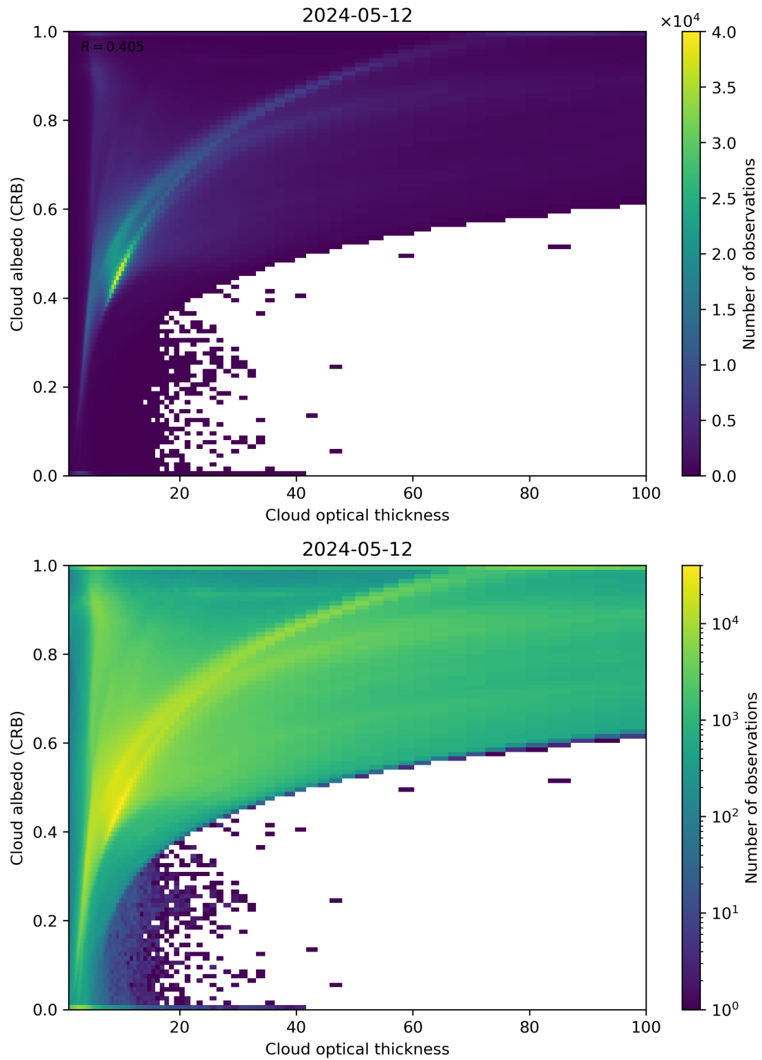
Figure 82: Scatter density plot of “Cloud optical thickness” against “Cloud albedo (CRB)” for 2024-05-12 to 2024-05-13.
