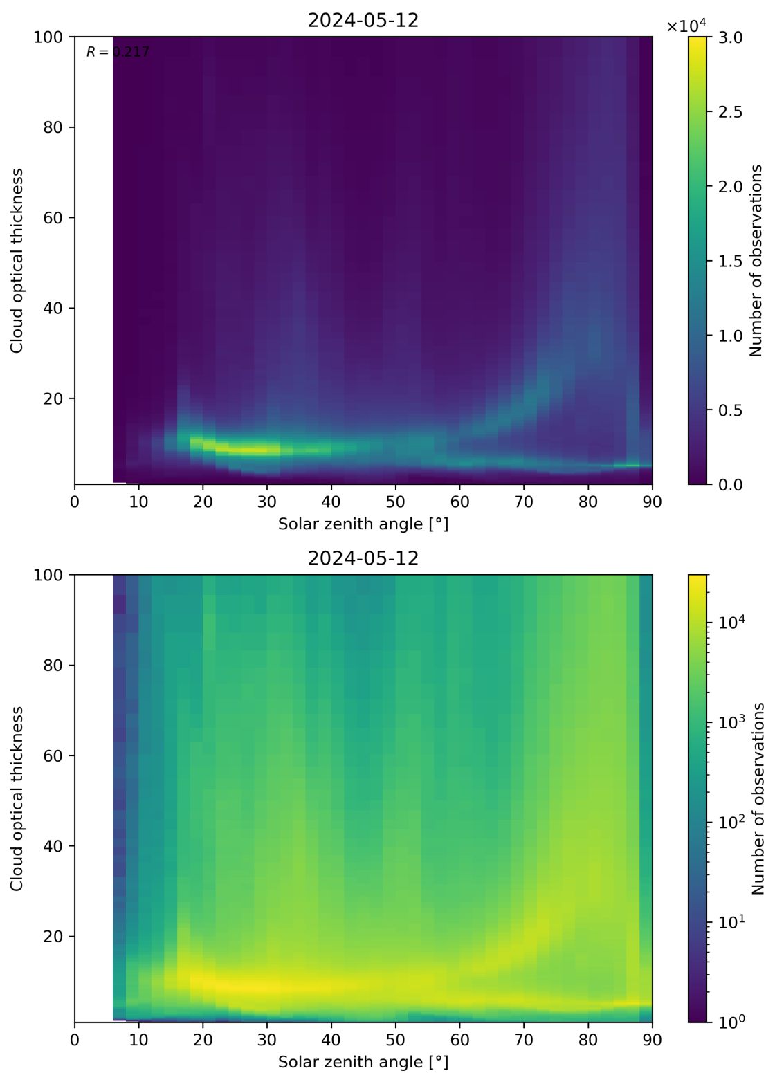
Figure 103: Scatter density plot of “Solar zenith angle” against “Cloud optical thickness” for 2024-05-12 to 2024-05-13.
