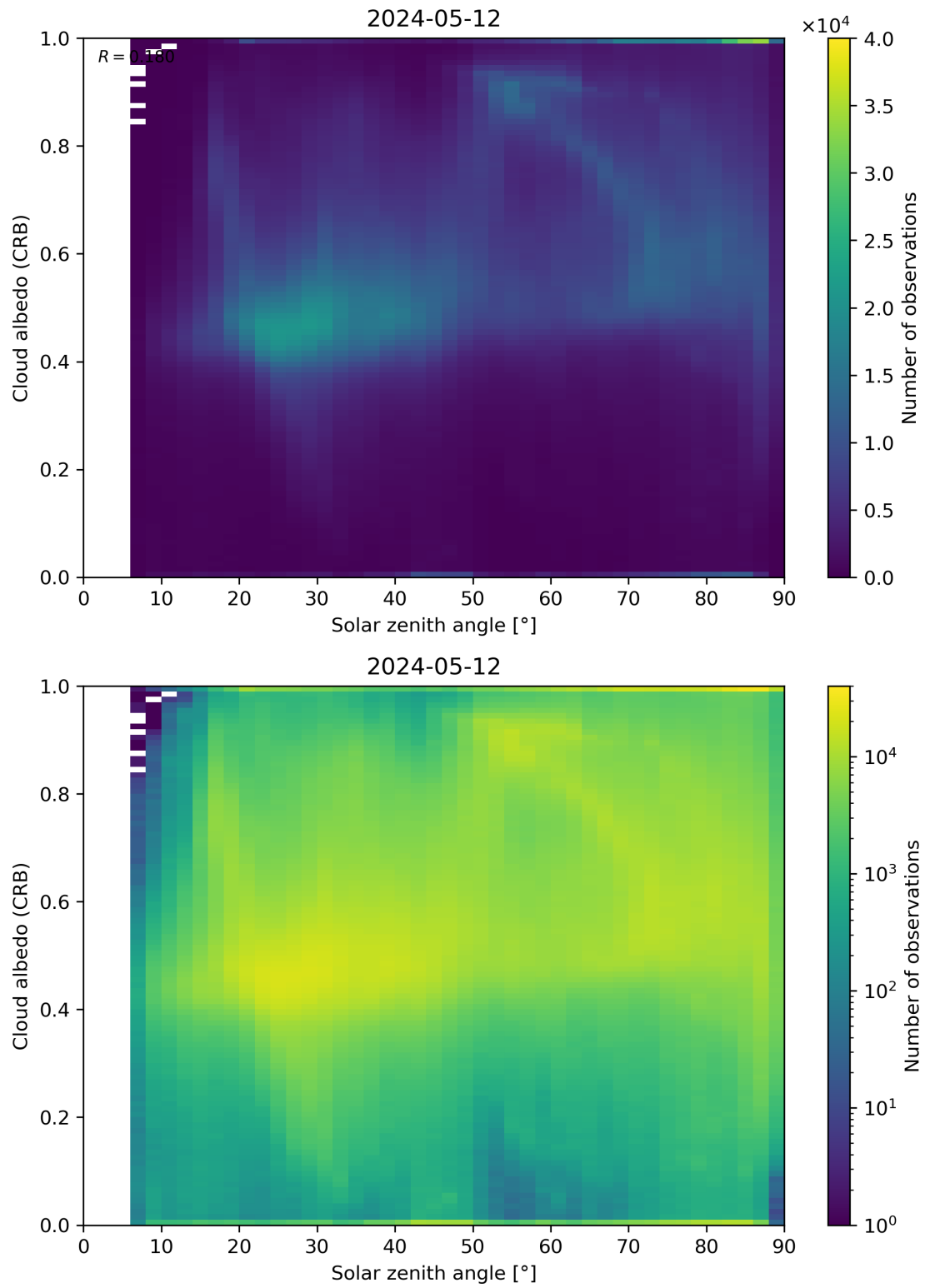
Figure 98: Scatter density plot of “Solar zenith angle” against “Cloud albedo (CRB)” for 2024-05-12 to 2024-05-13.
