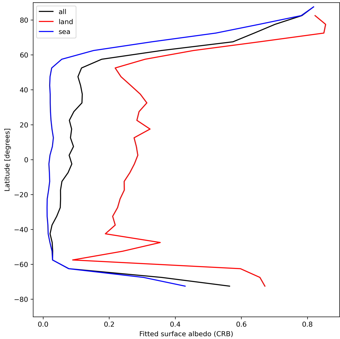
Figure 30: Zonal average of “Fitted surface albedo (CRB)” for 2024-05-12 to 2024-05-13.
