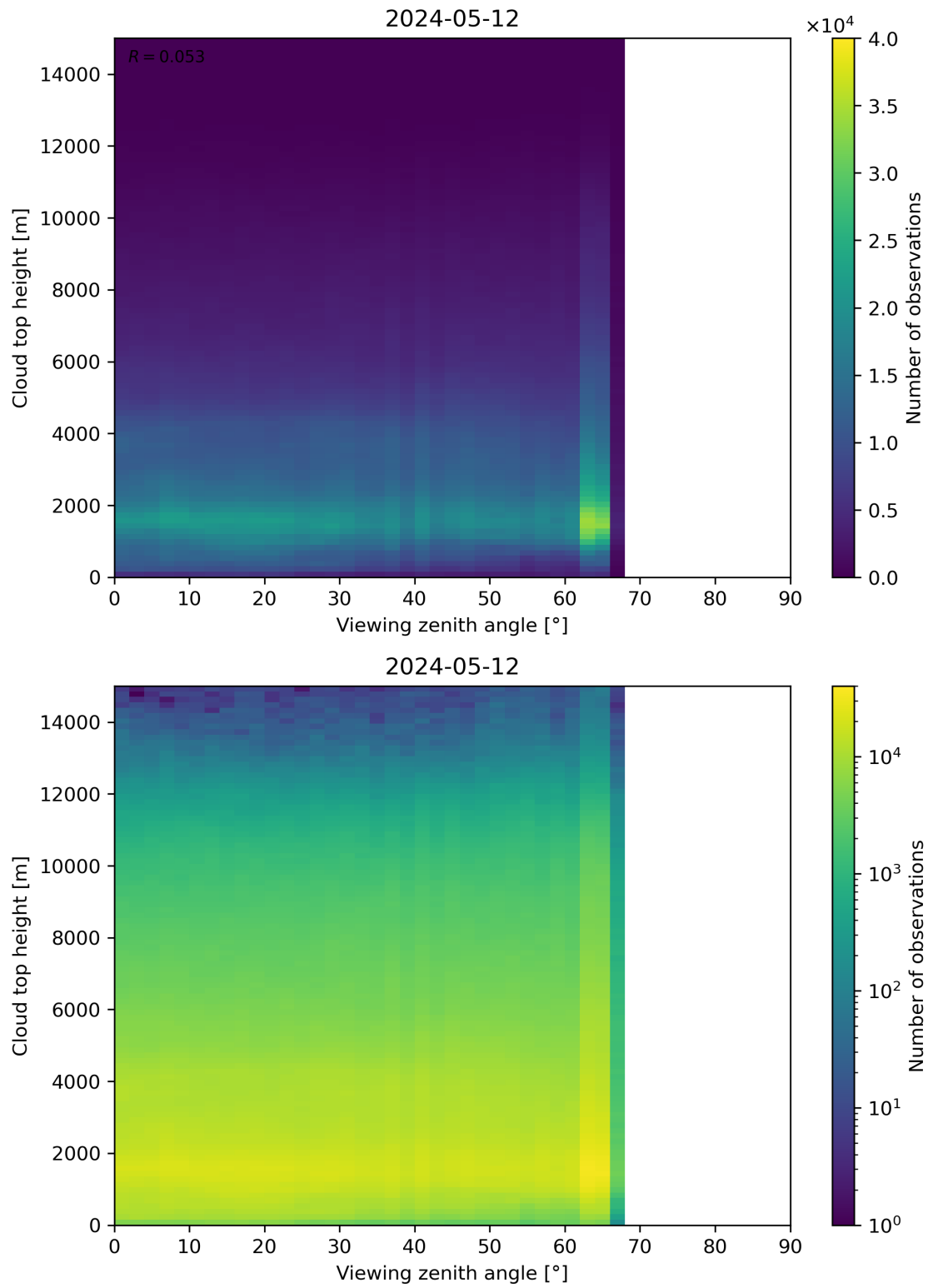
Figure 112: Scatter density plot of “Viewing zenith angle” against “Cloud top height” for 2024-05-12 to 2024-05-13.
