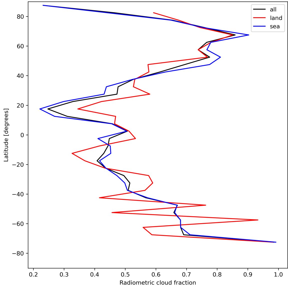
Figure 23: Zonal average of “Radiometric cloud fraction” for 2024-05-12 to 2024-05-13.
