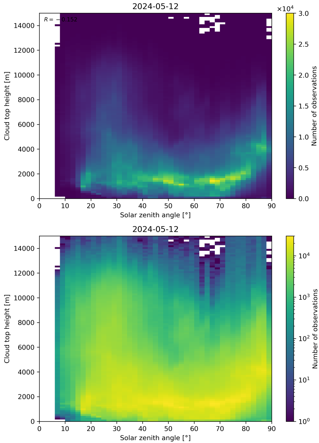
Figure 104: Scatter density plot of “Solar zenith angle” against “Cloud top height” for 2024-05-12 to 2024-05-13.
