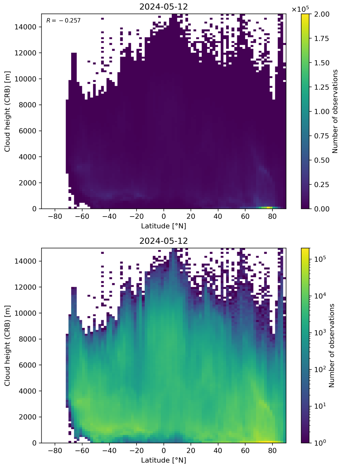
Figure 95: Scatter density plot of “Latitude” against “Cloud height (CRB)” for 2024-05-12 to 2024-05-13.
