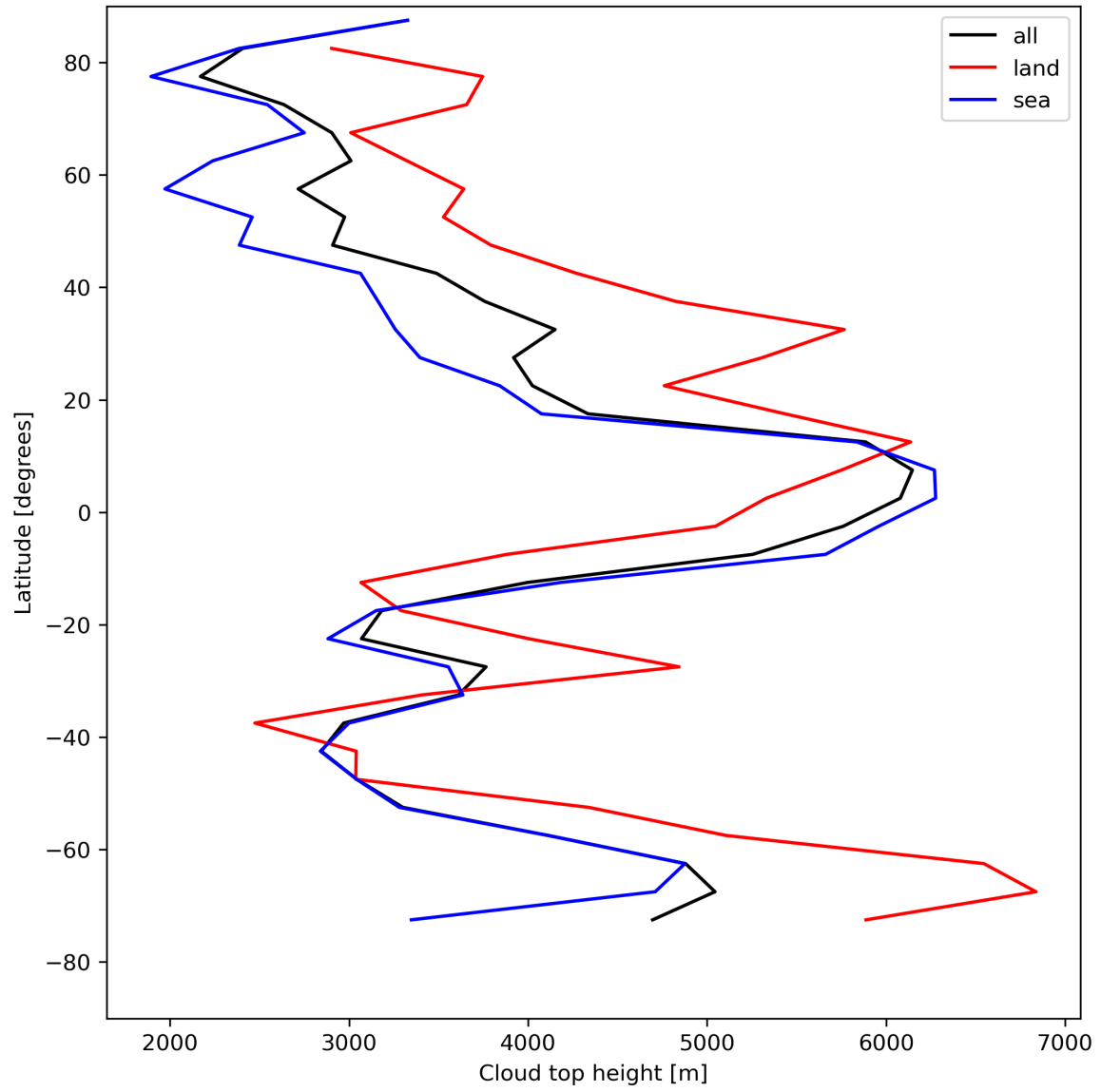
Figure 24: Zonal average of “Cloud top height” for 2024-05-12 to 2024-05-13.
