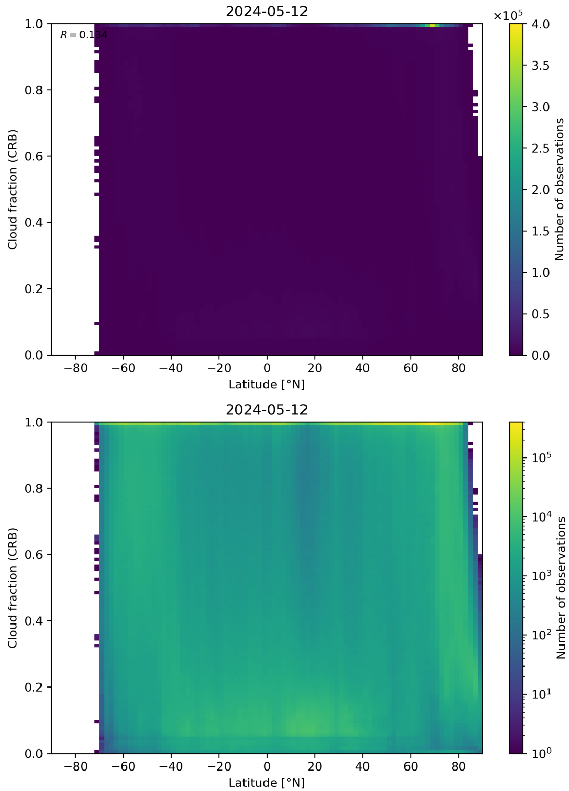
Figure 94: Scatter density plot of “Latitude” against “Cloud fraction (CRB)” for 2024-05-12 to 2024-05-13.
