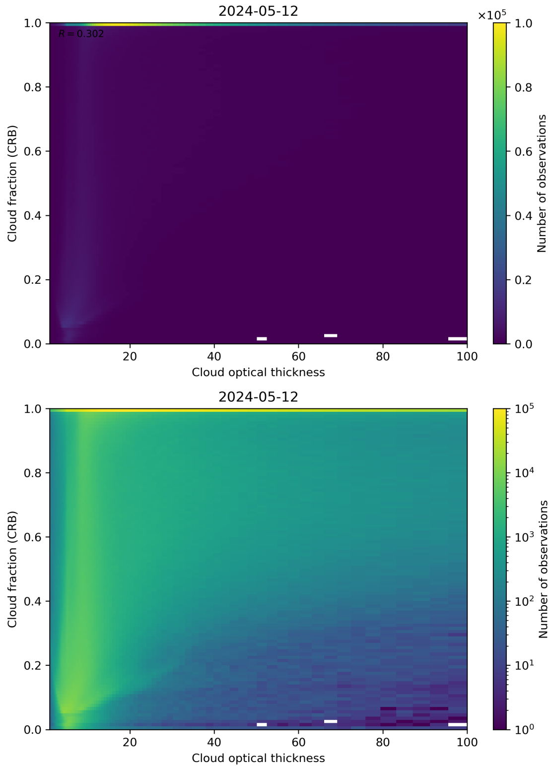
Figure 84: Scatter density plot of “Cloud optical thickness” against “Cloud fraction (CRB)” for 2024-05-12 to 2024-05-13.
