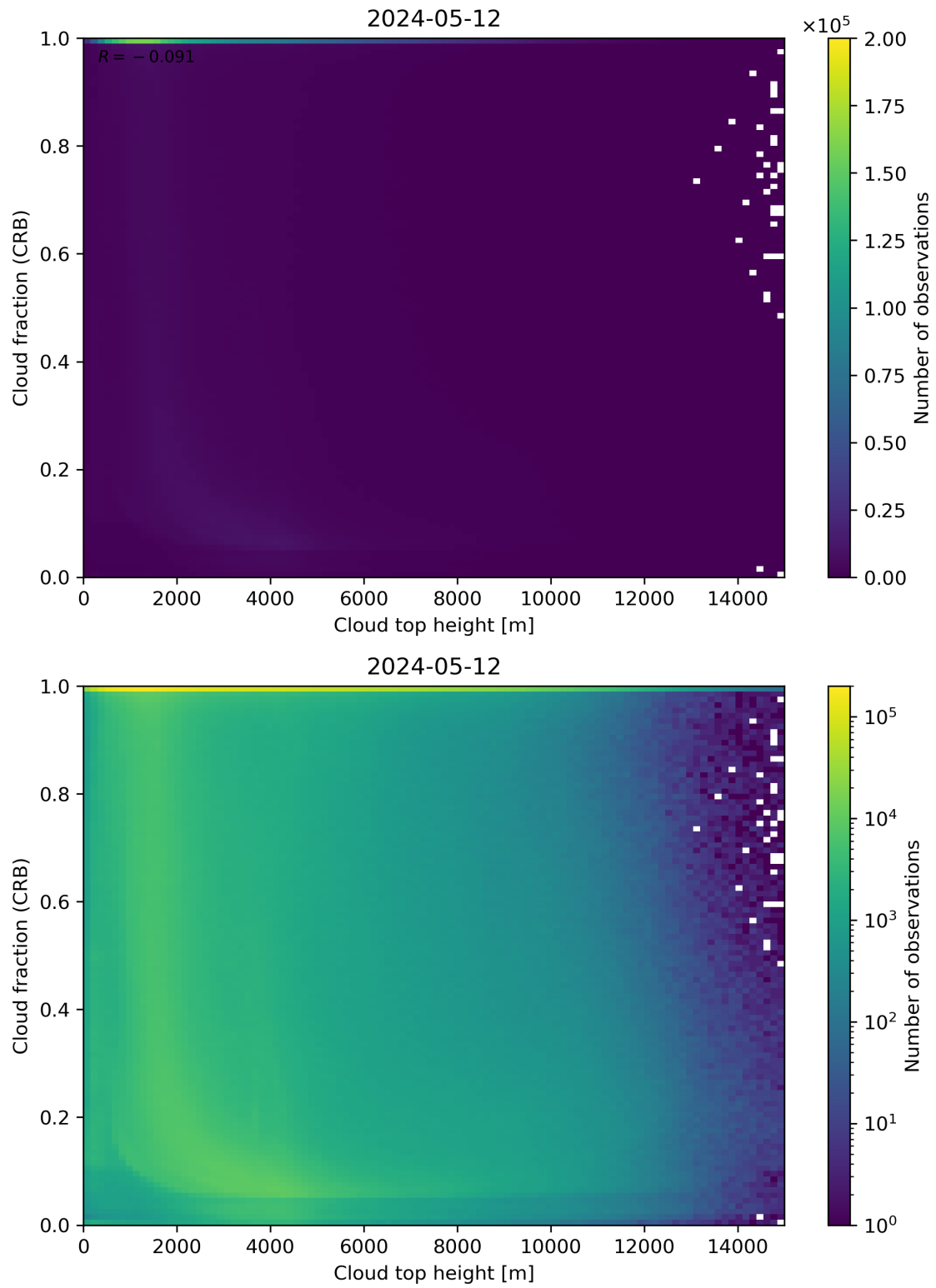
Figure 88: Scatter density plot of “Cloud top height” against “Cloud fraction (CRB)” for 2024-05-12 to 2024-05-13.
