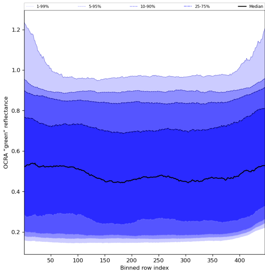
Figure 68: Along track statistics of “OCRA “green” reflectance” for 2024-05-12 to 2024-05-13
