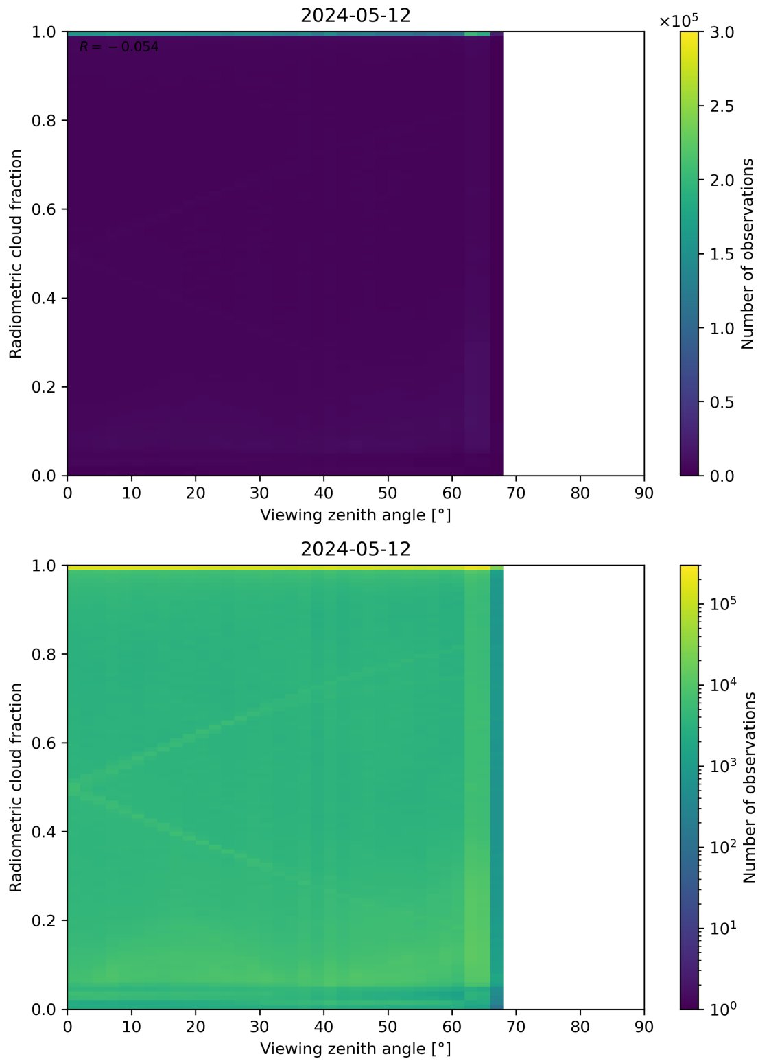
Figure 107: Scatter density plot of “Viewing zenith angle” against “Radiometric cloud fraction” for 2024-05-12 to 2024-05-13.
