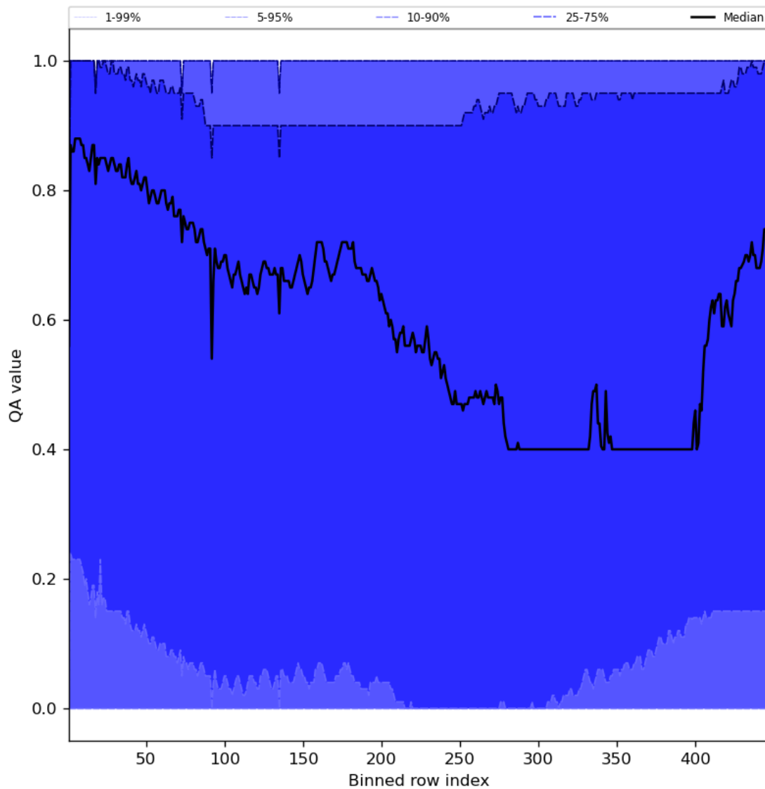
Figure 54: Along track statistics of “QA value” for 2024-05-12 to 2024-05-13
