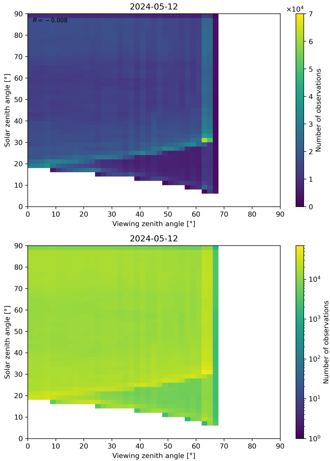
Figure 114: Scatter density plot of “Viewing zenith angle” against “Solar zenith angle” for 2024-05-12 to 2024-05-13.
