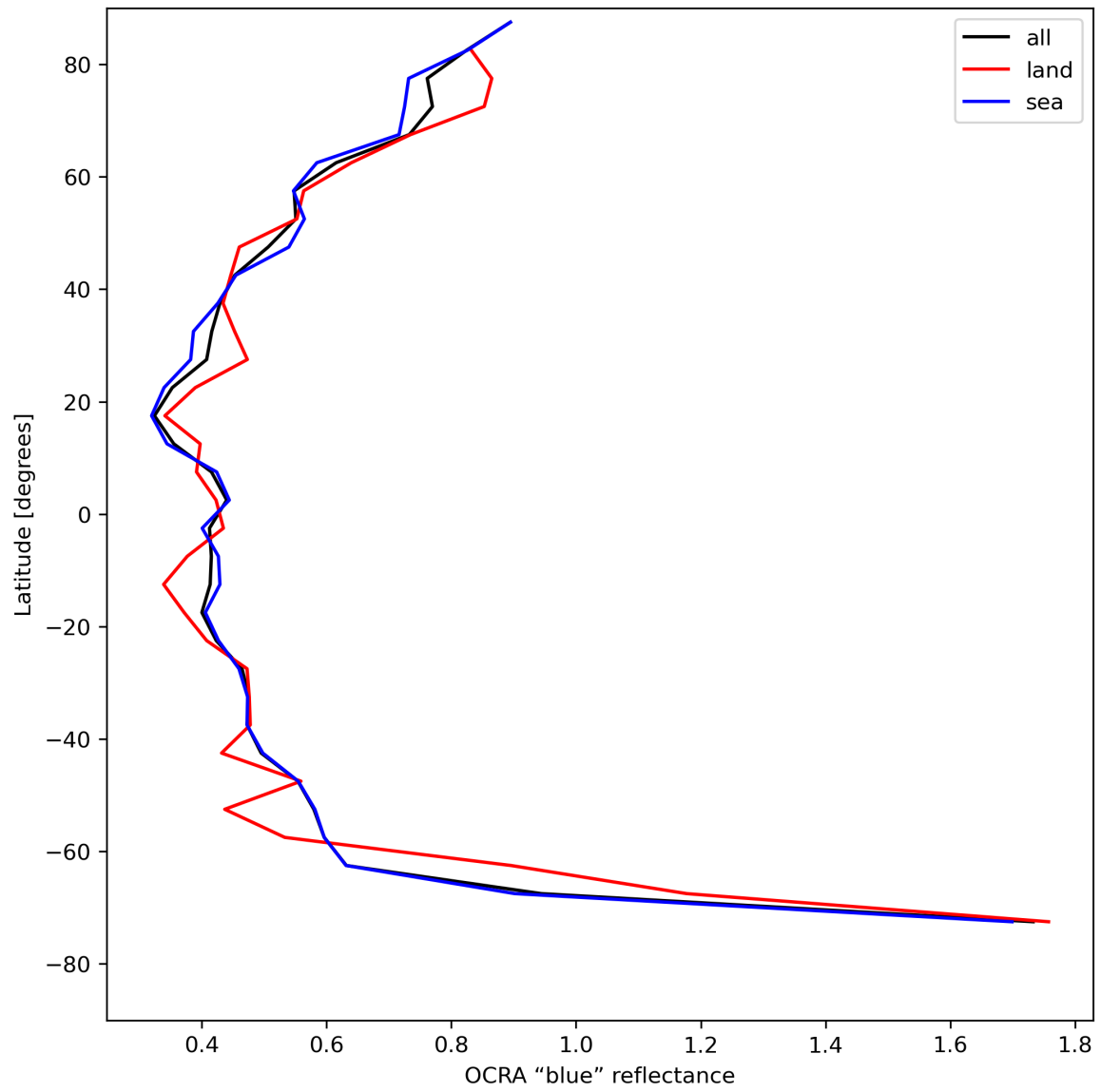
Figure 35: Zonal average of "OCRA "blue" reflectance" for 2024-05-12 to 2024-05-13.
