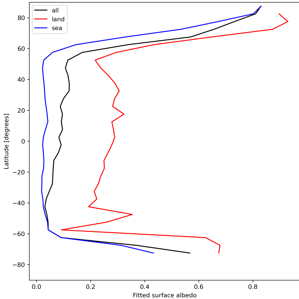
Figure 29: Zonal average of “Fitted surface albedo” for 2024-05-12 to 2024-05-13.
