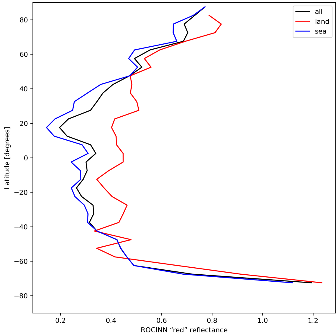
Figure 37: Zonal average of “ROCINN “red” reflectance” for 2024-05-12 to 2024-05-13.
