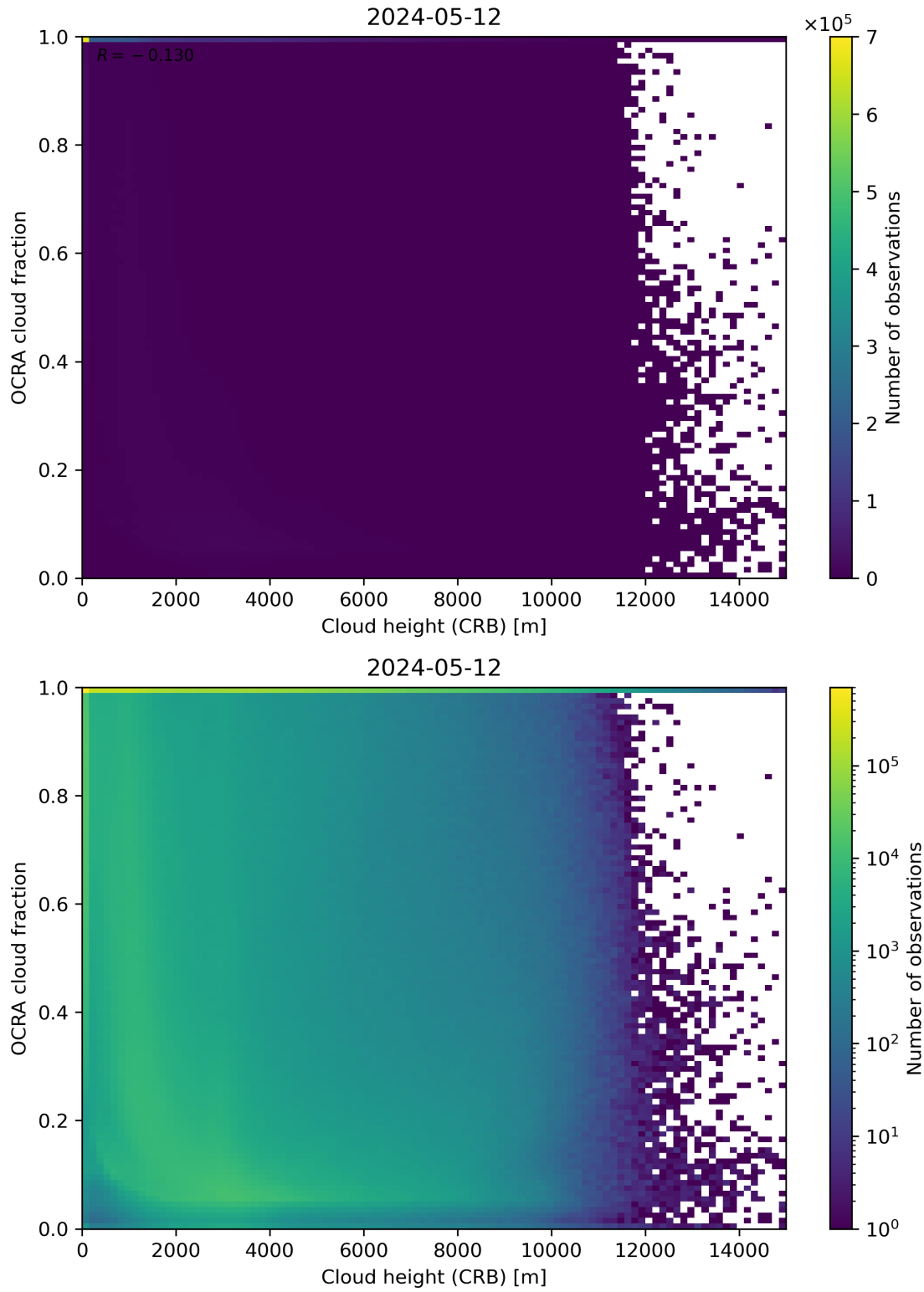
Figure 81: Scatter density plot of “Cloud height (CRB)” against “OCRA cloud fraction” for 2024-05-12 to 2024-05-13.
