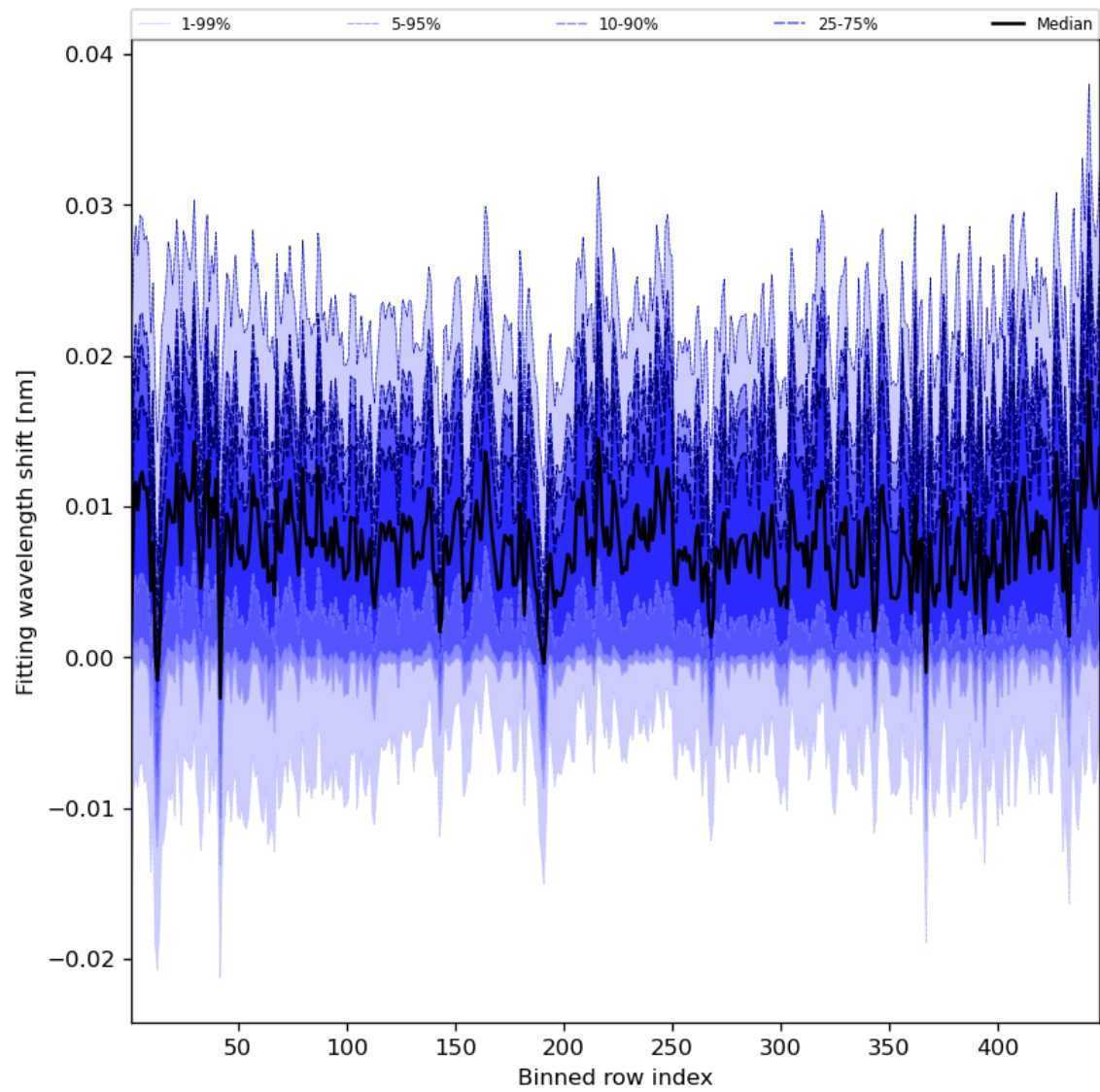
Figure 65: Along track statistics of “Fitting wavelength shift” for 2024-05-12 to 2024-05-13
