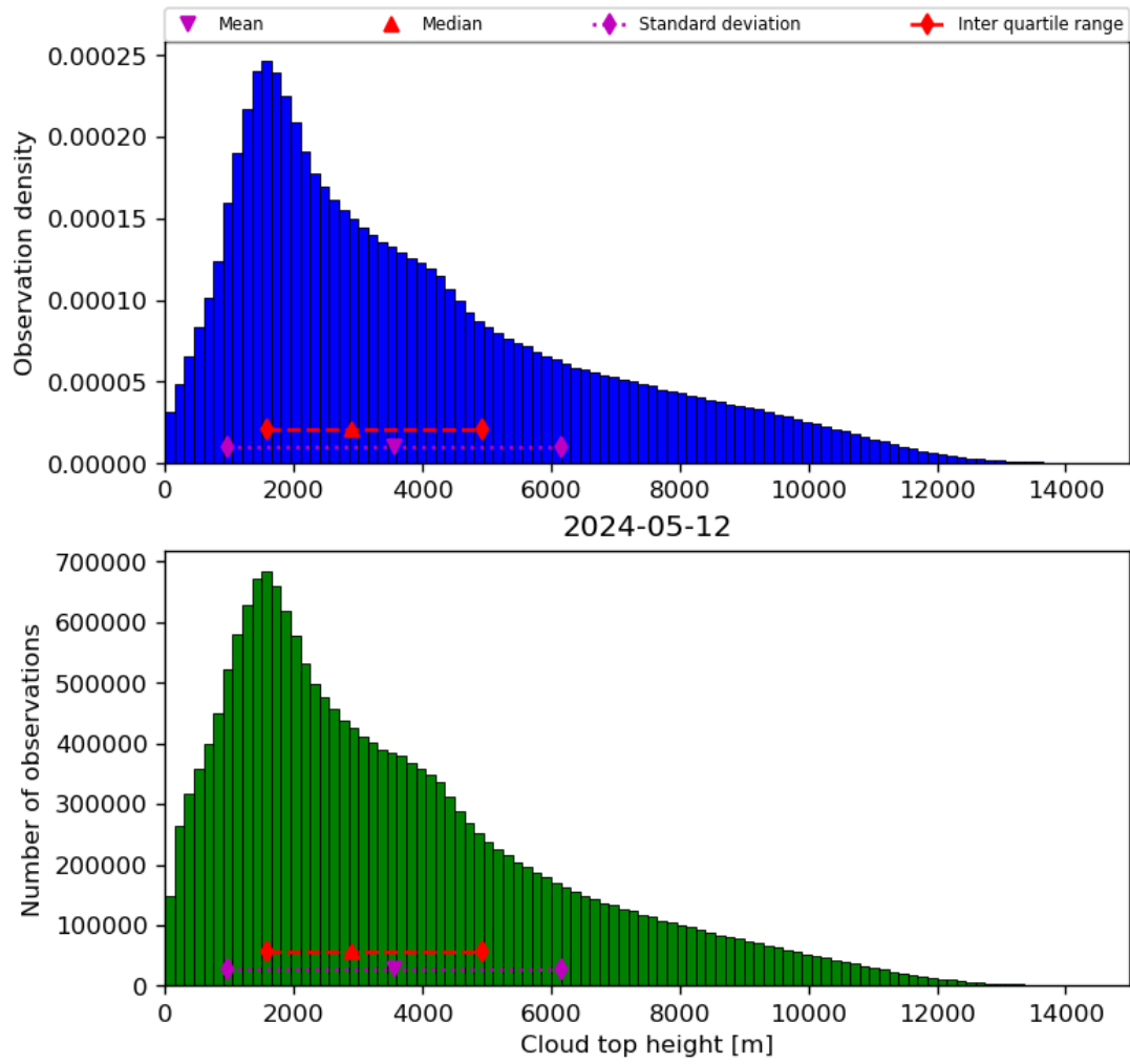
Figure 40: Histogram of “Cloud top height” for 2024-05-12 to 2024-05-13
