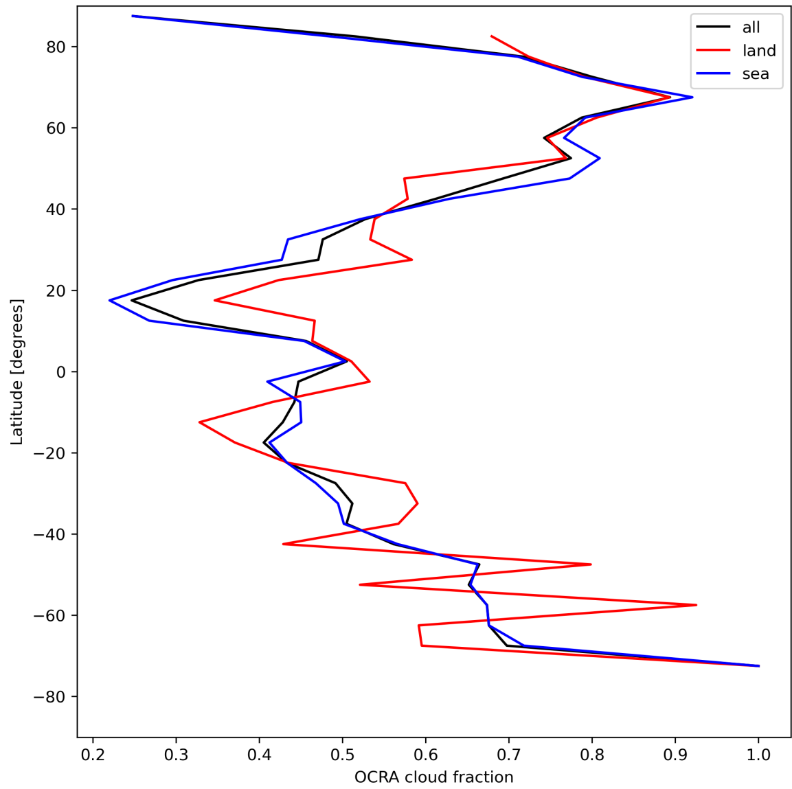
Figure 34: Zonal average of “OCRA cloud fraction” for 2024-05-12 to 2024-05-13.
