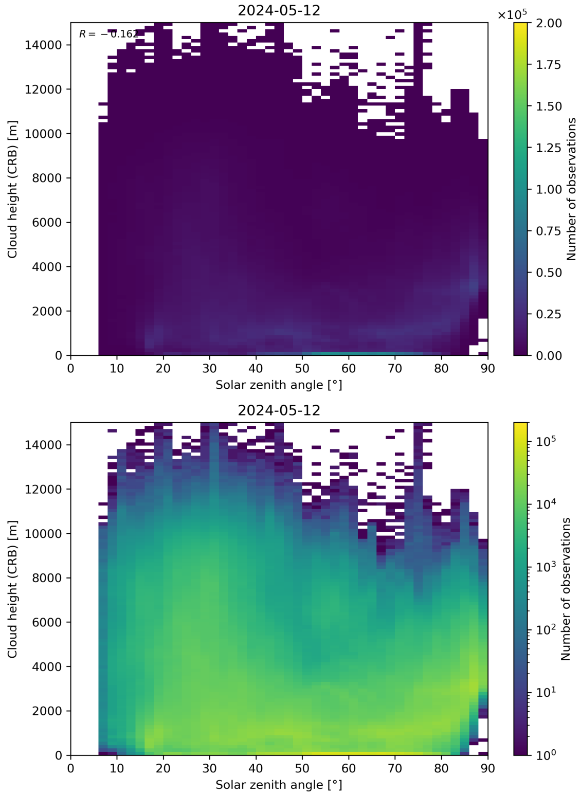
Figure 102: Scatter density plot of “Solar zenith angle” against “Cloud height (CRB)” for 2024-05-12 to 2024-05-13.
