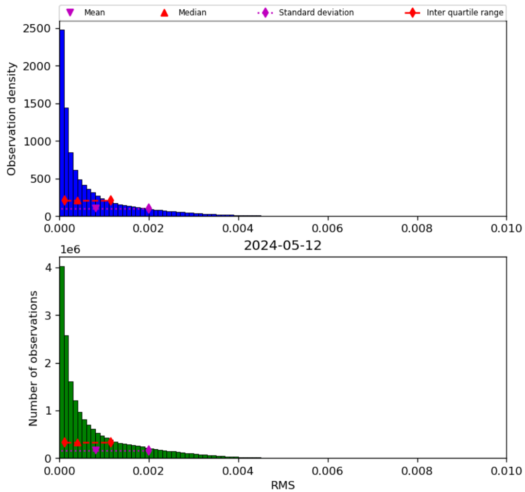
Figure 47: Histogram of “RMS” for 2024-05-12 to 2024-05-13
