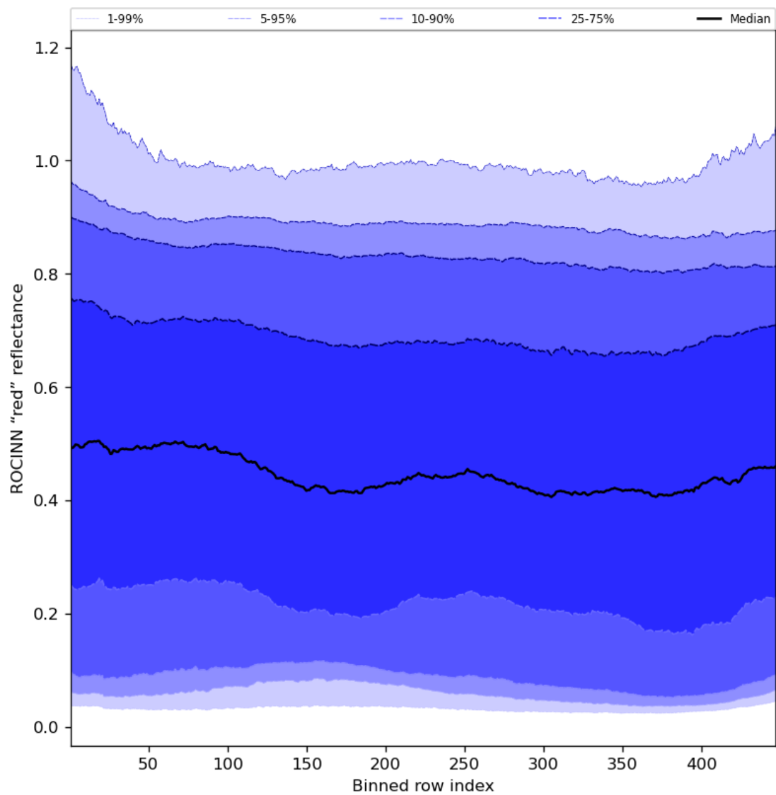
Figure 69: Along track statistics of “ROCINN “red” reflectance” for 2024-05-12 to 2024-05-13
