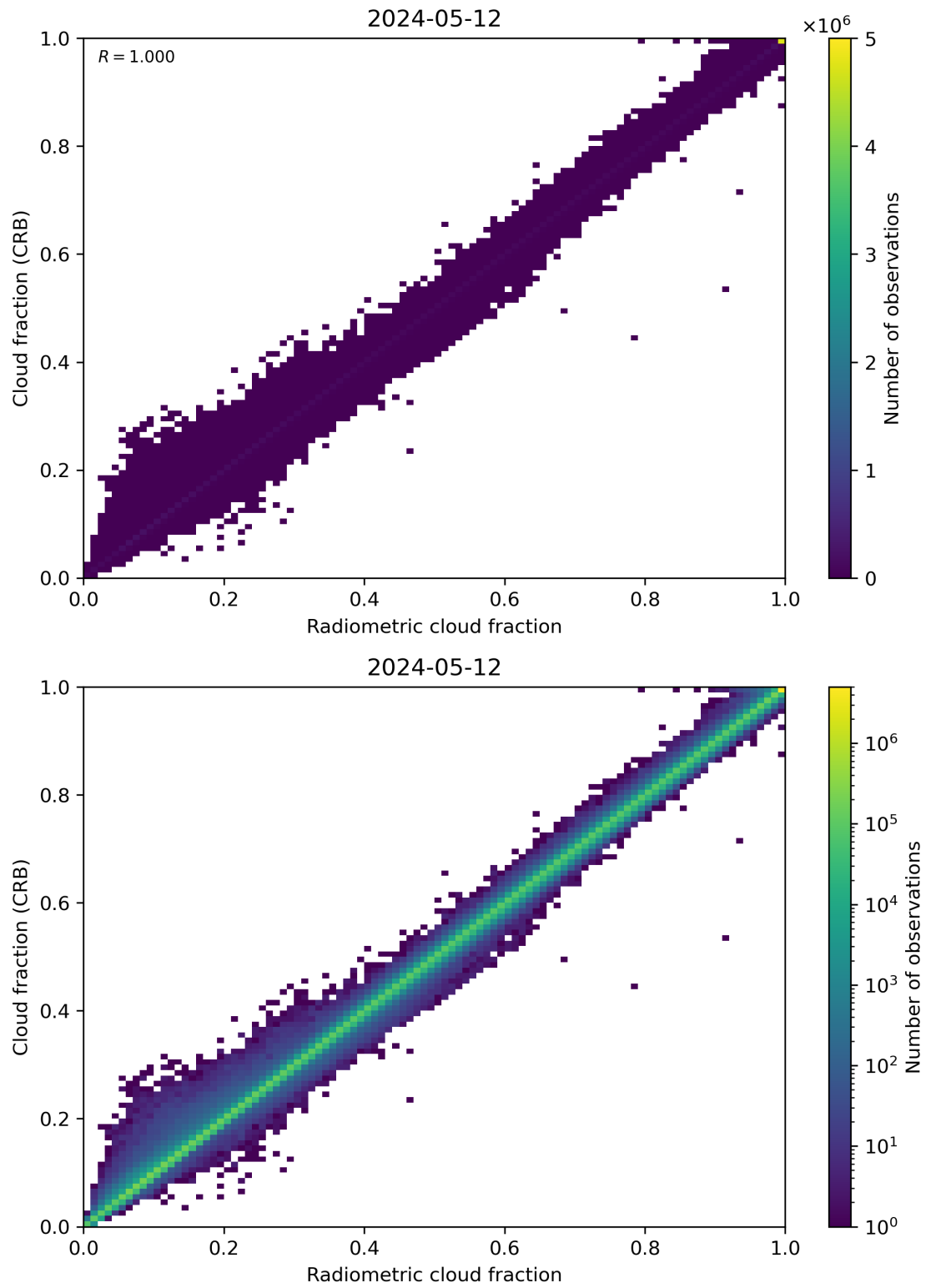
Figure 73: Scatter density plot of “Radiometric cloud fraction” against “Cloud fraction (CRB)” for 2024-05-12 to 2024-05-13.
