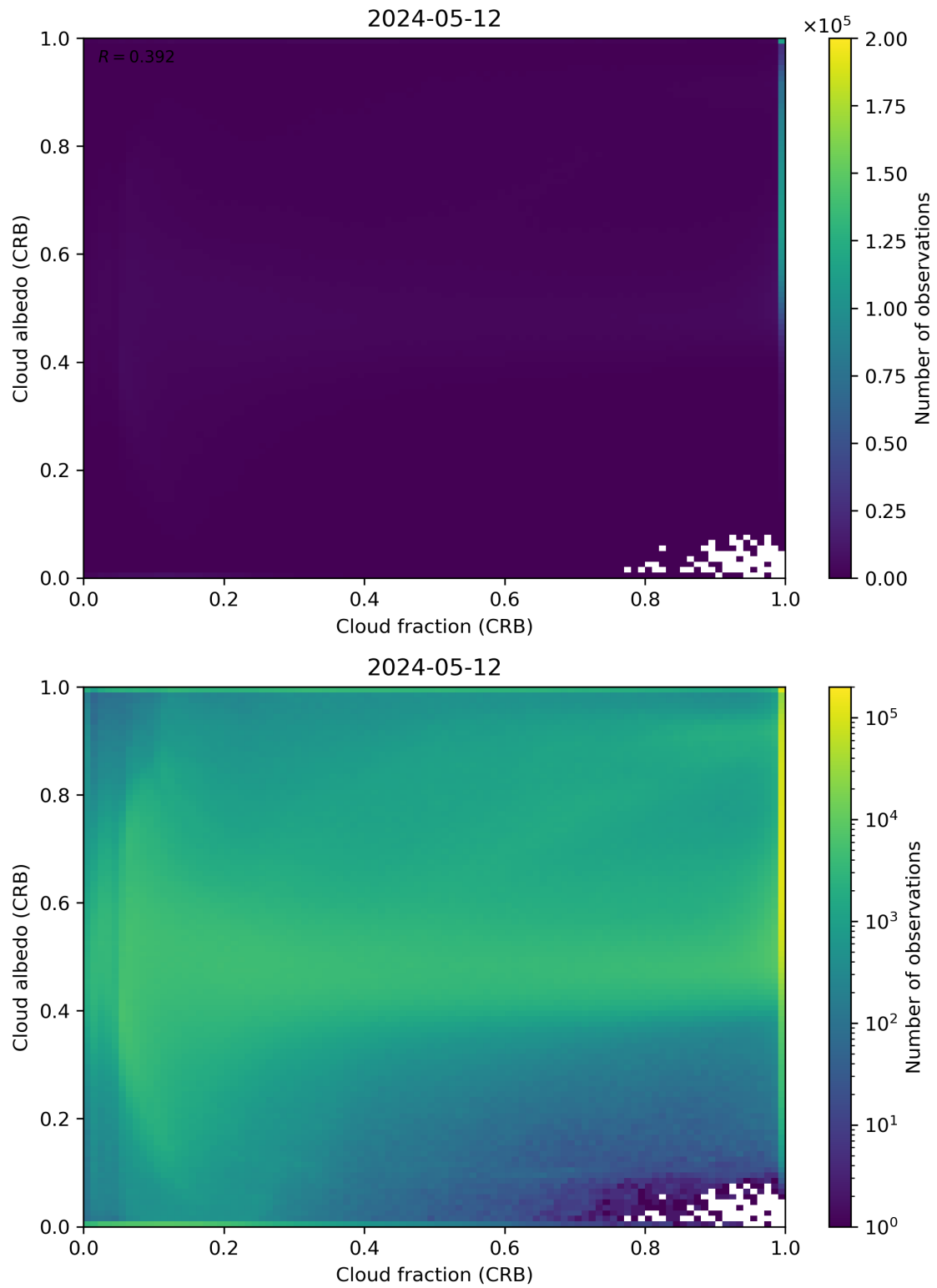
Figure 77: Scatter density plot of “Cloud fraction (CRB)” against “Cloud albedo (CRB)” for 2024-05-12 to 2024-05-13.
