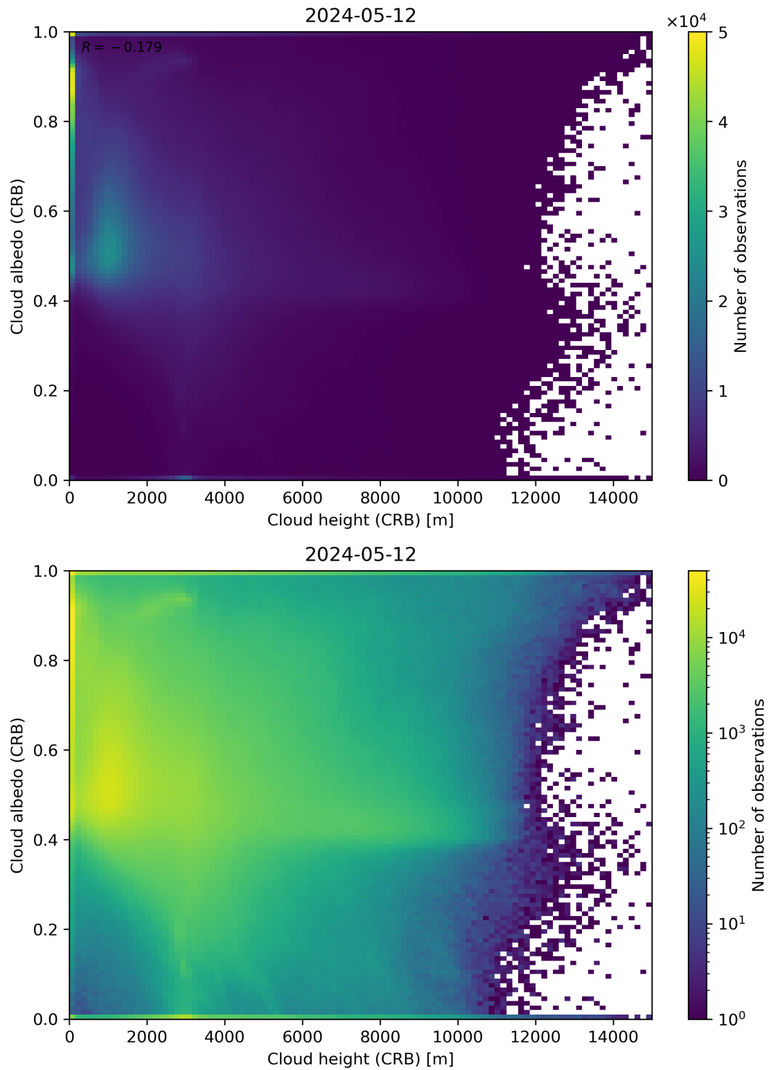
Figure 80: Scatter density plot of “Cloud height (CRB)” against “Cloud albedo (CRB)” for 2024-05-12 to 2024-05-13.
