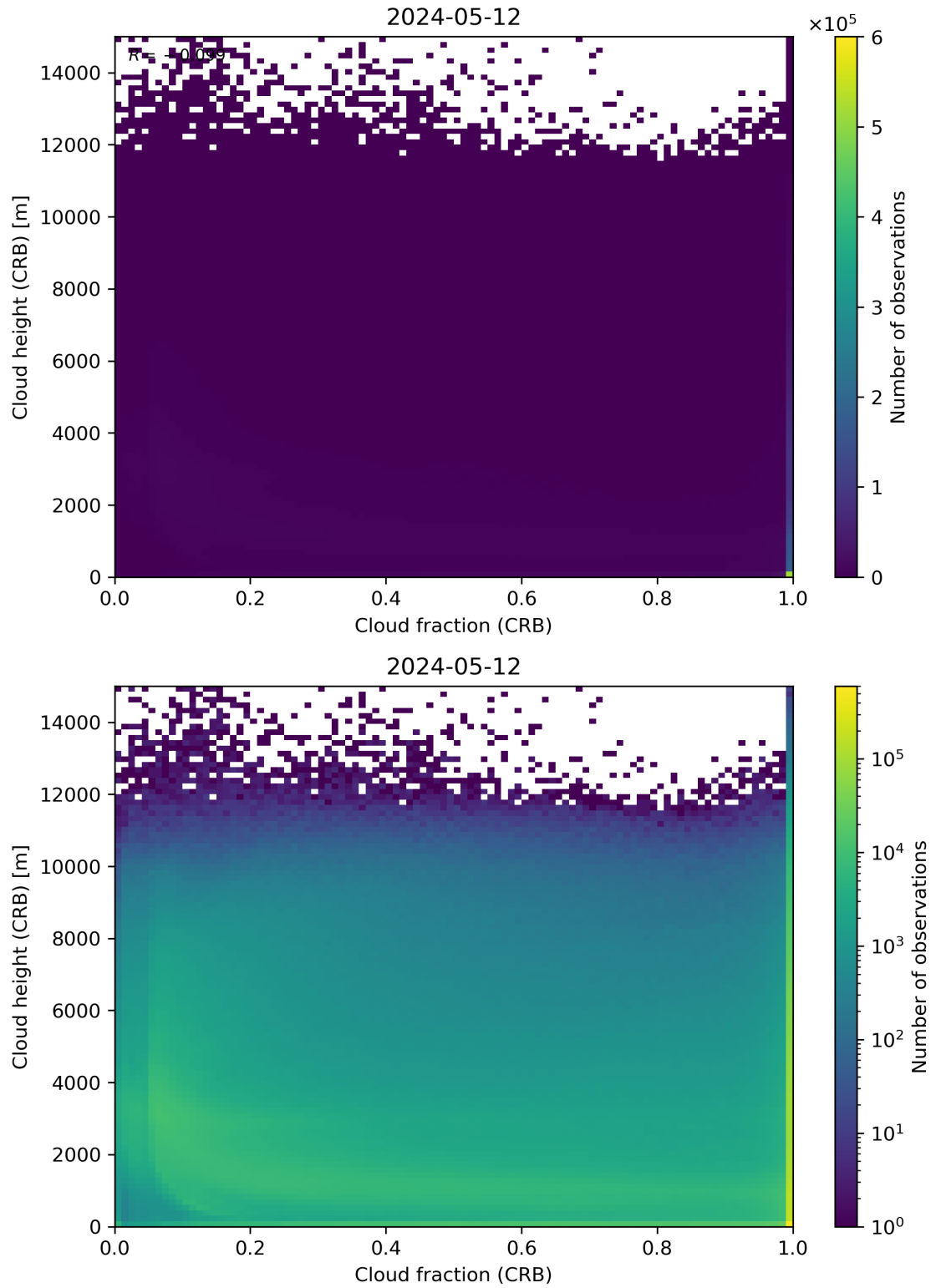
Figure 79: Scatter density plot of “Cloud fraction (CRB)” against “Cloud height (CRB)” for 2024-05-12 to 2024-05-13.
