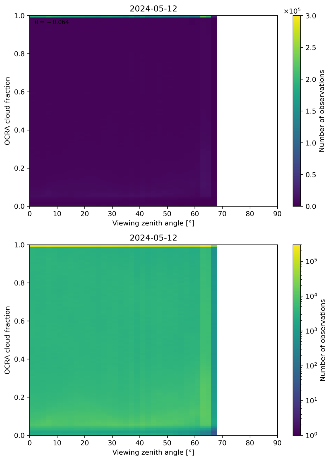
Figure 108: Scatter density plot of “Viewing zenith angle” against “OCRA cloud fraction” for 2024-05-12 to 2024-05-13.
