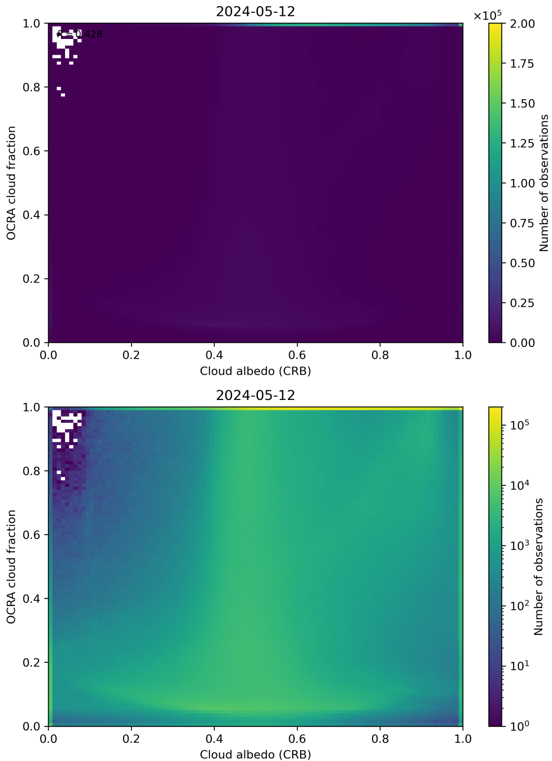
Figure 70: Scatter density plot of “Cloud albedo (CRB)” against “OCRA cloud fraction” for 2024-05-12 to 2024-05-13.
