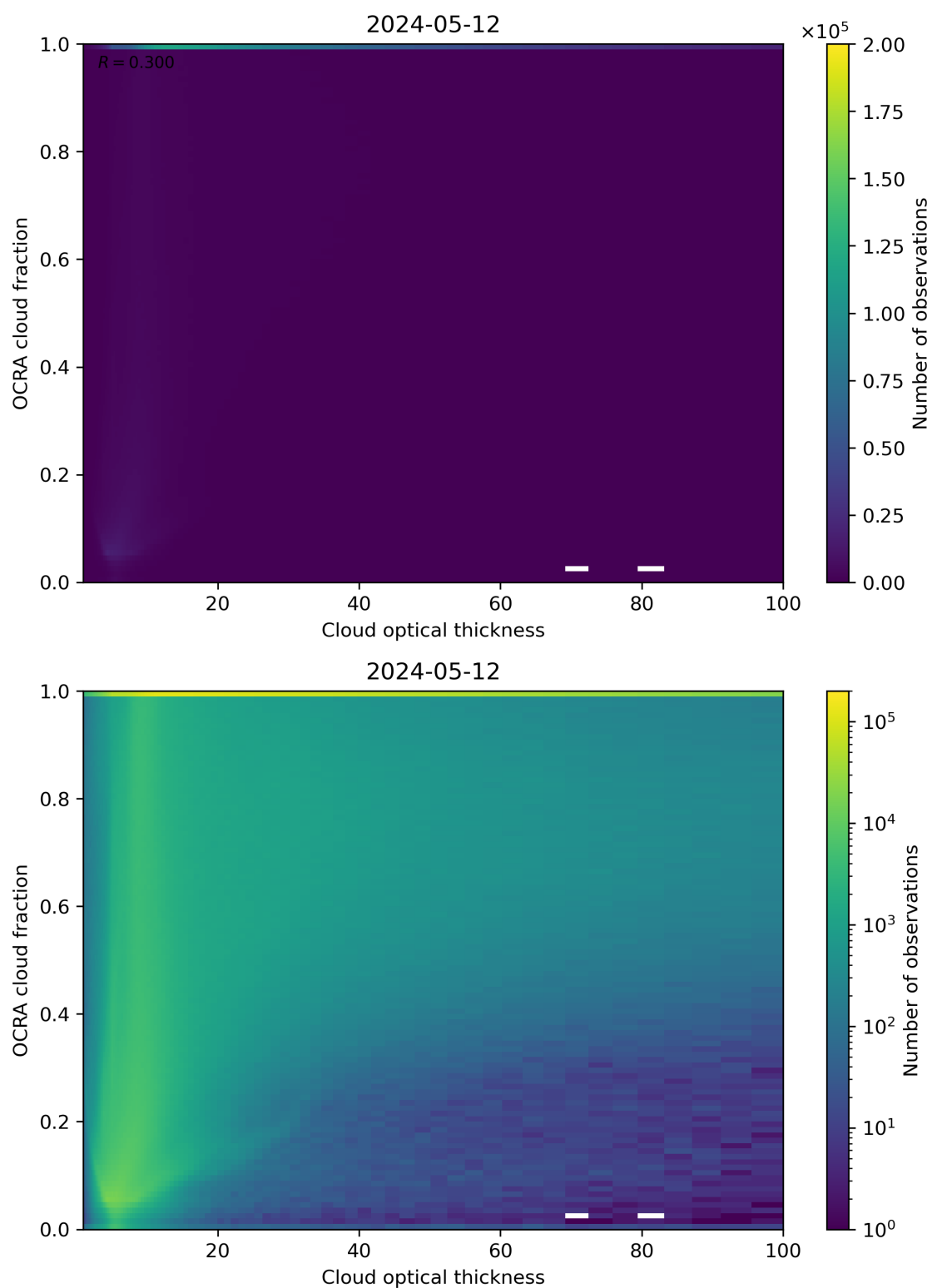
Figure 83: Scatter density plot of “Cloud optical thickness” against “OCRA cloud fraction” for 2024-05-12 to 2024-05-13.
