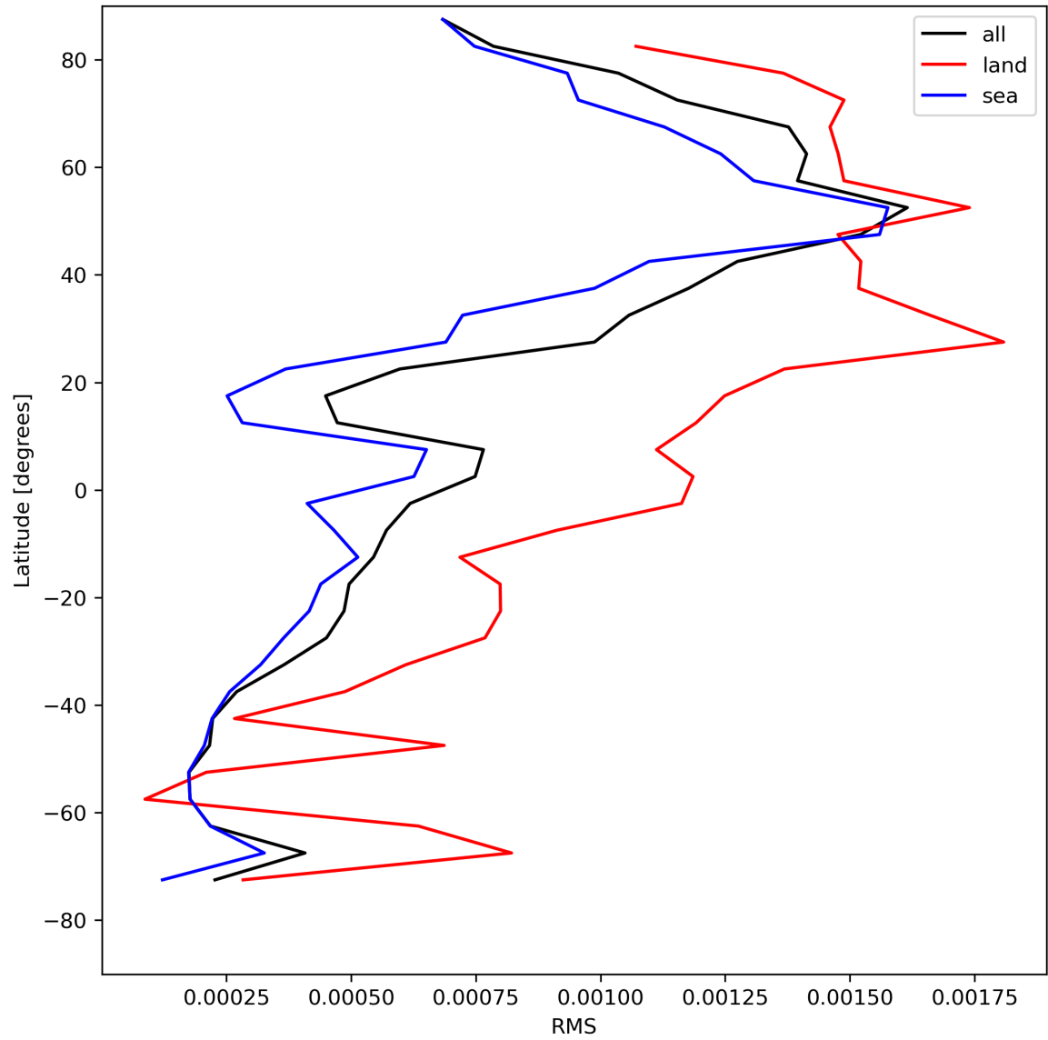
Figure 31: Zonal average of “RMS” for 2024-05-12 to 2024-05-13.
