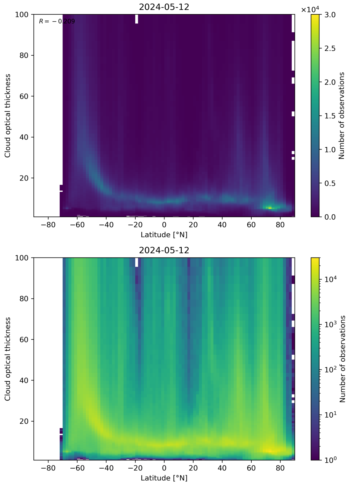
Figure 96: Scatter density plot of “Latitude” against “Cloud optical thickness” for 2024-05-12 to 2024-05-13.
