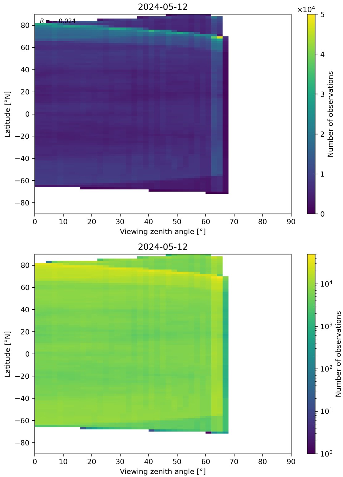
Figure 113: Scatter density plot of “Viewing zenith angle” against “Latitude” for 2024-05-12 to 2024-05-13.
