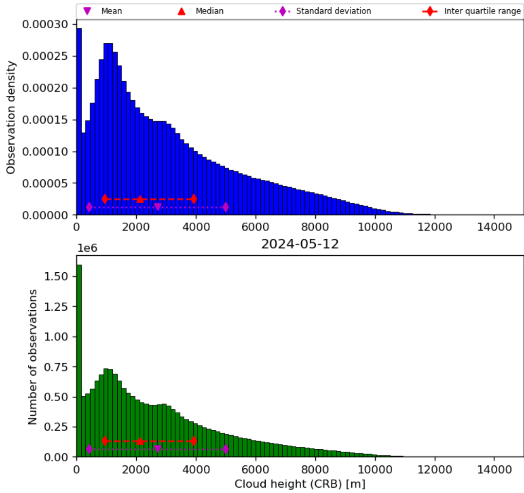
Figure 43: Histogram of “Cloud height (CRB)” for 2024-05-12 to 2024-05-13
