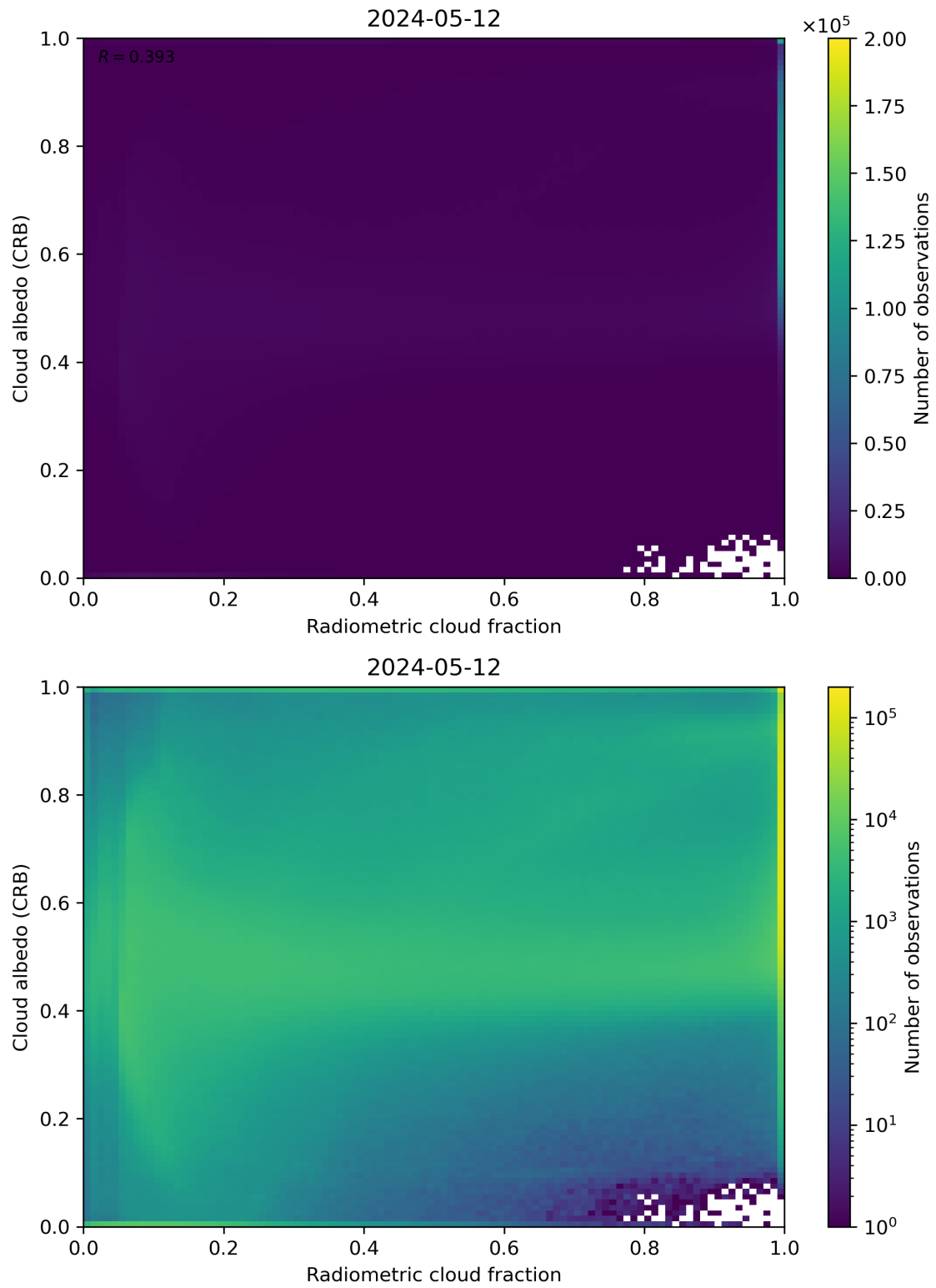
Figure 71: Scatter density plot of “Radiometric cloud fraction” against “Cloud albedo (CRB)” for 2024-05-12 to 2024-05-13.
