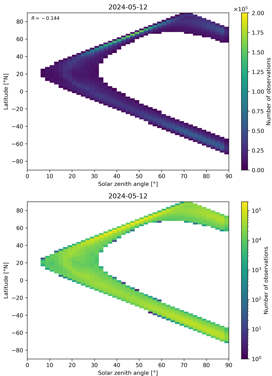
Figure 105: Scatter density plot of “Solar zenith angle” against “Latitude” for 2024-05-12 to 2024-05-13.
