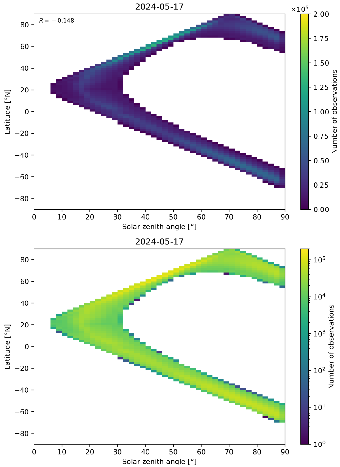
Figure 105: Scatter density plot of “Solar zenith angle” against “Latitude” for 2024-05-16 to 2024-05-18.
