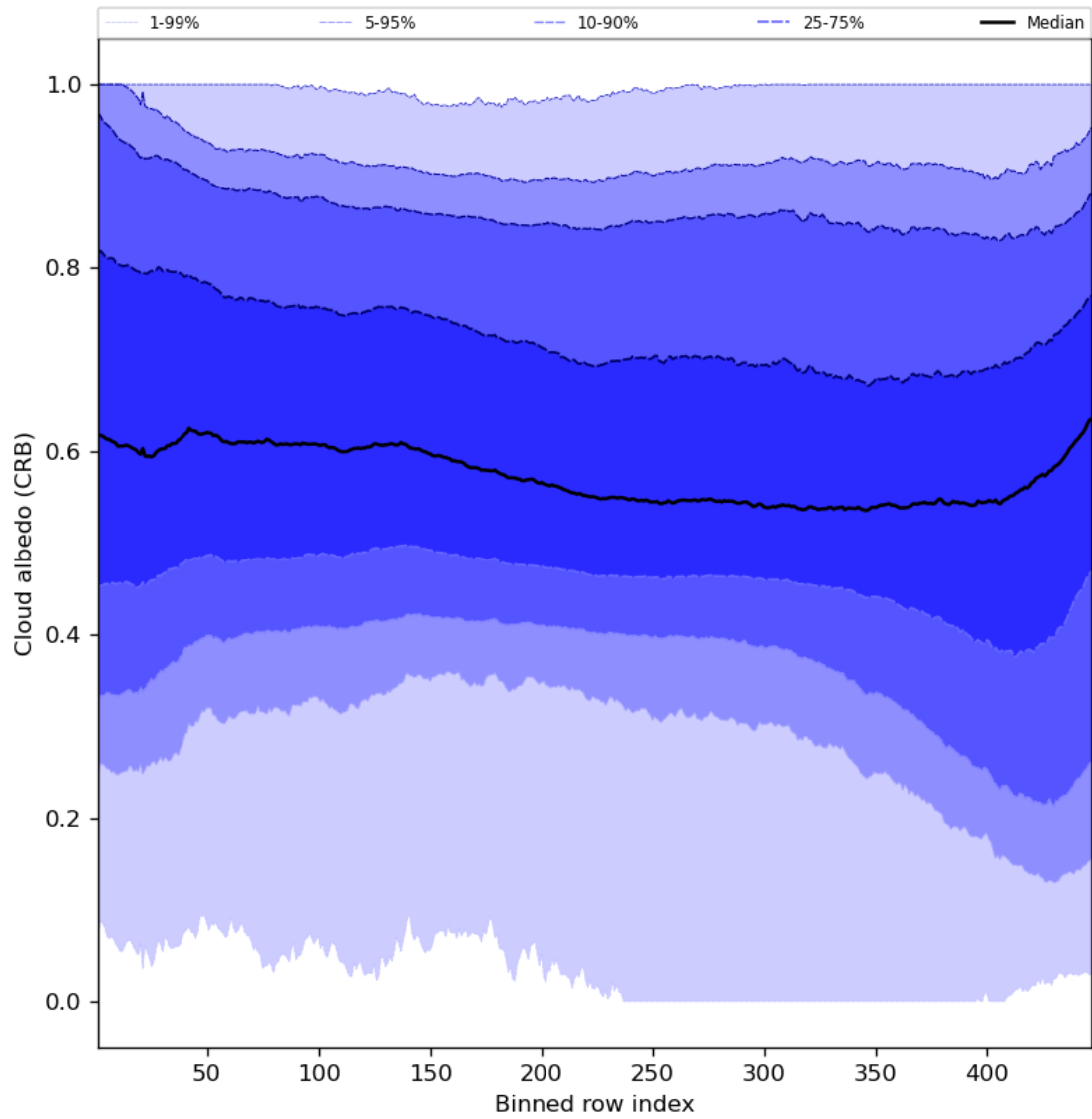
Figure 60: Along track statistics of “Cloud albedo (CRB)” for 2024-05-16 to 2024-05-18
