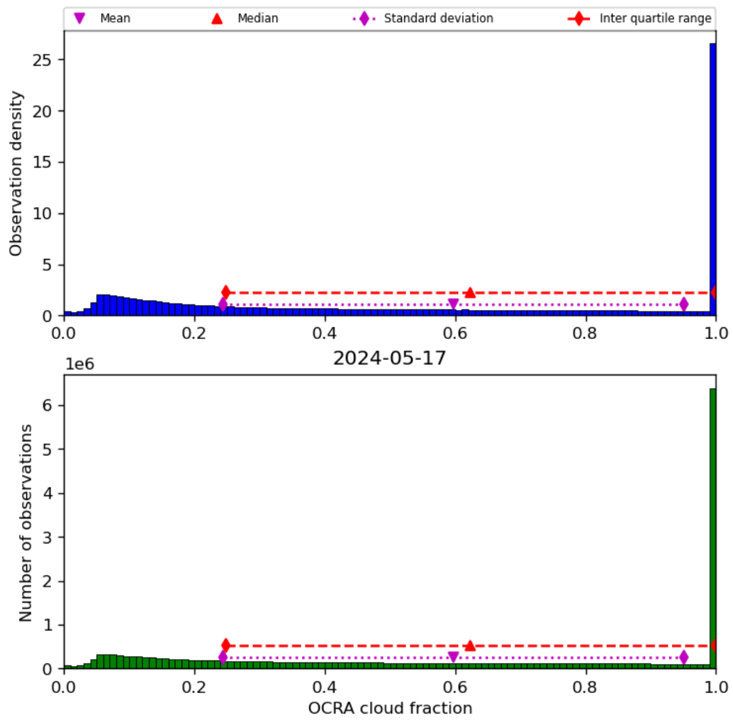
Figure 50: Histogram of “OCRA cloud fraction” for 2024-05-16 to 2024-05-18
