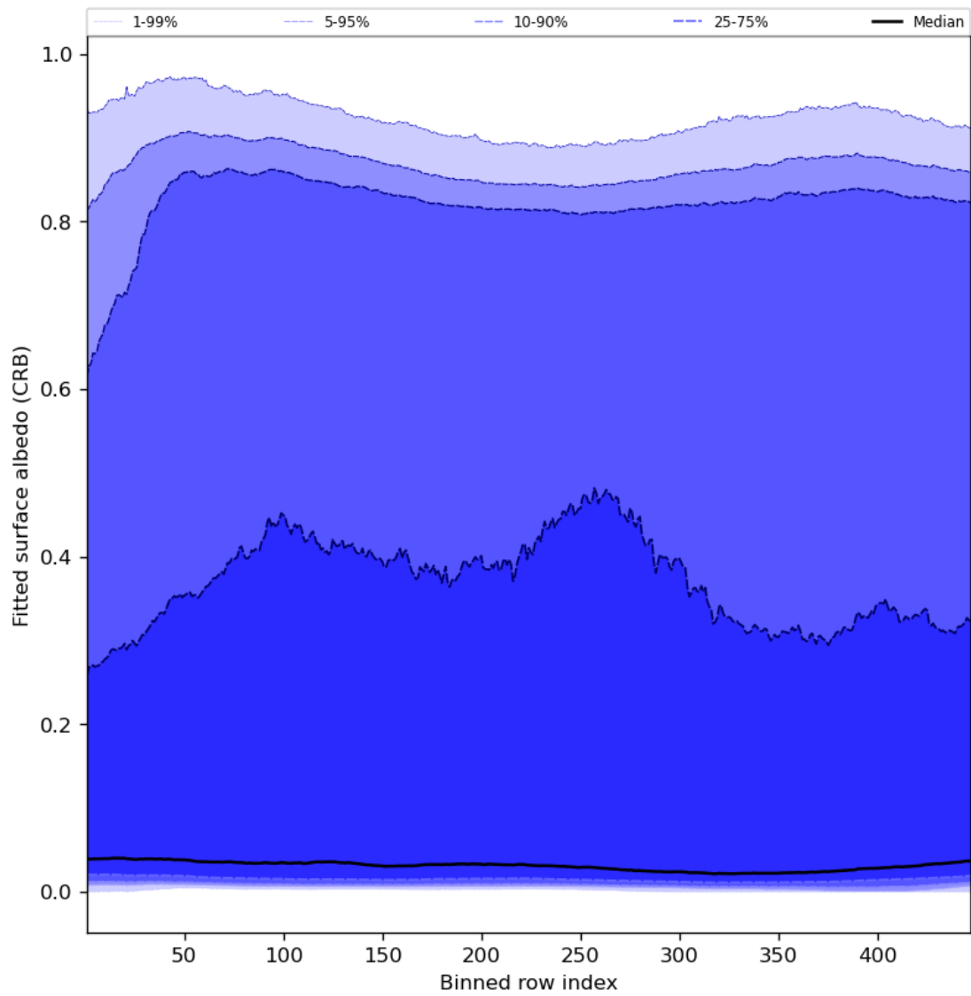
Figure 62: Along track statistics of “Fitted surface albedo (CRB)” for 2024-05-16 to 2024-05-18
