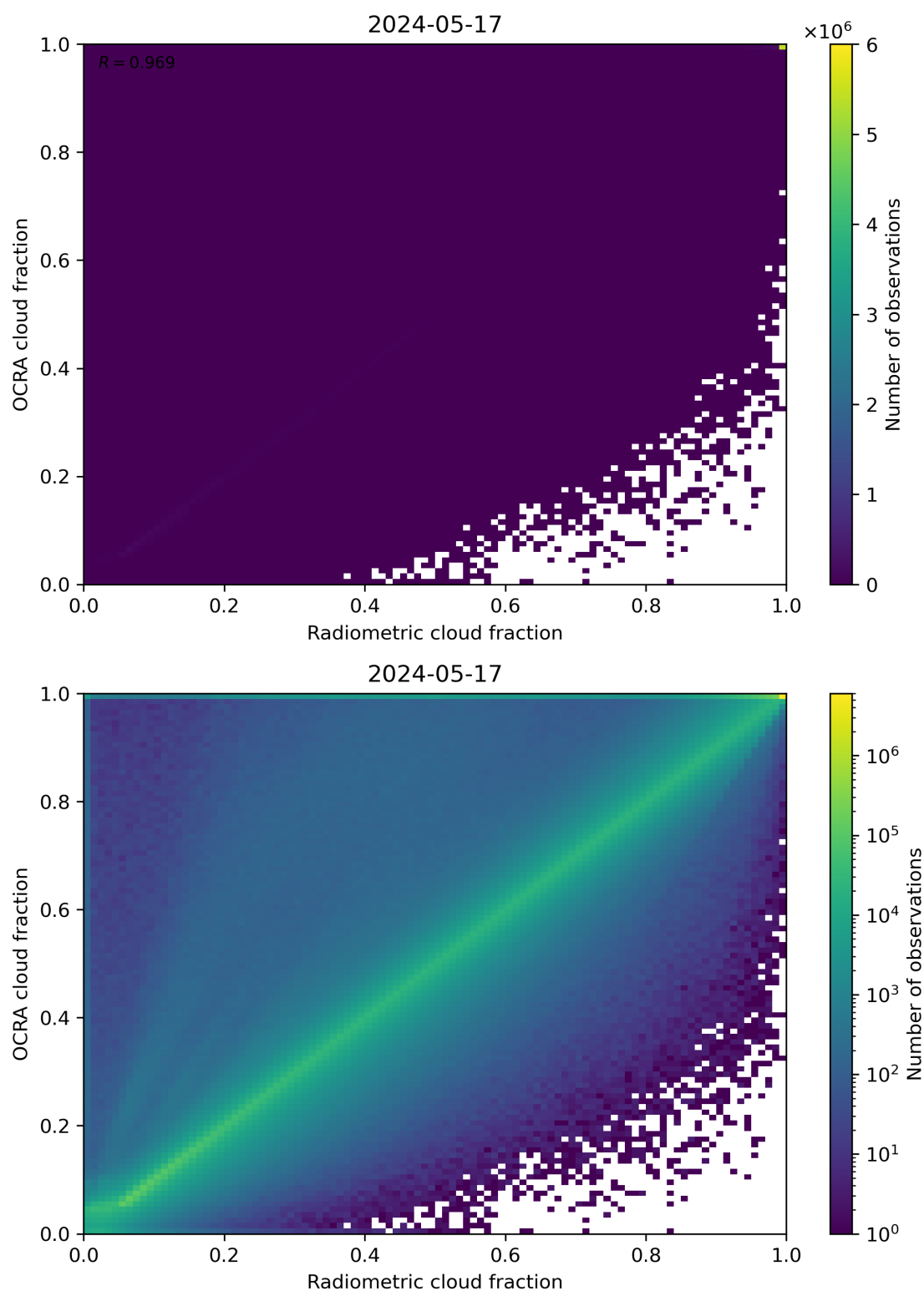
Figure 72: Scatter density plot of “Radiometric cloud fraction” against “OCRA cloud fraction” for 2024-05-16 to 2024-05-18.
