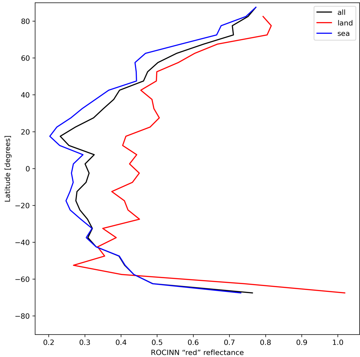
Figure 37: Zonal average of “ROCINN “red” reflectance” for 2024-05-16 to 2024-05-18.
