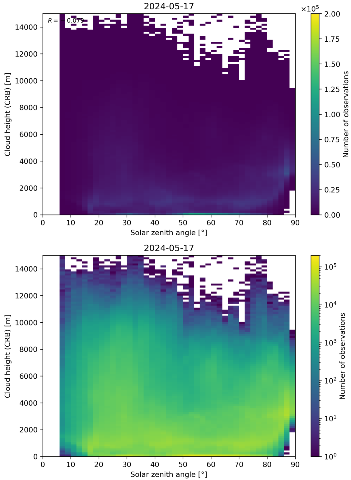
Figure 102: Scatter density plot of “Solar zenith angle” against “Cloud height (CRB)” for 2024-05-16 to 2024-05-18.
