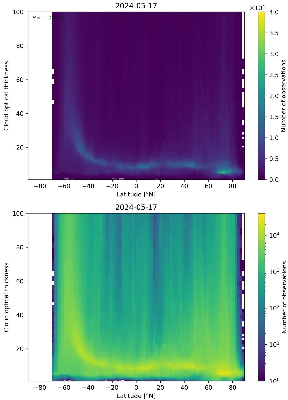
Figure 96: Scatter density plot of “Latitude” against “Cloud optical thickness” for 2024-05-16 to 2024-05-18.
