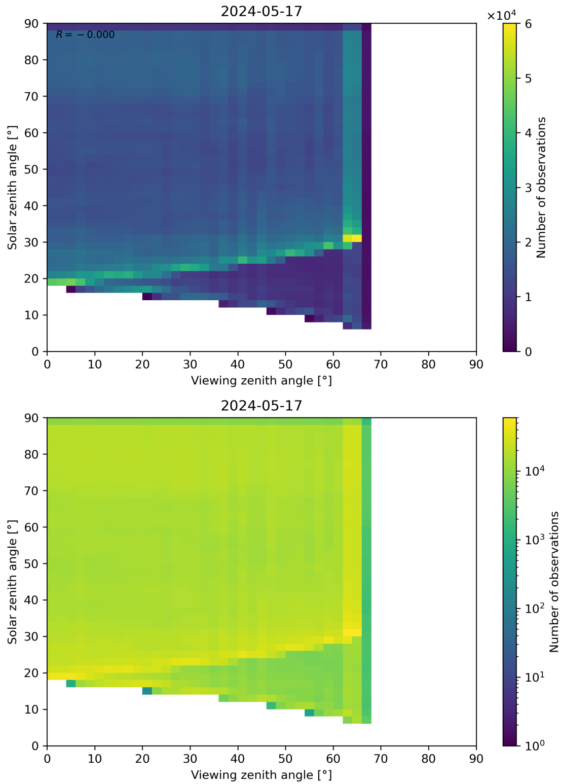
Figure 114: Scatter density plot of “Viewing zenith angle” against “Solar zenith angle” for 2024-05-16 to 2024-05-18.
