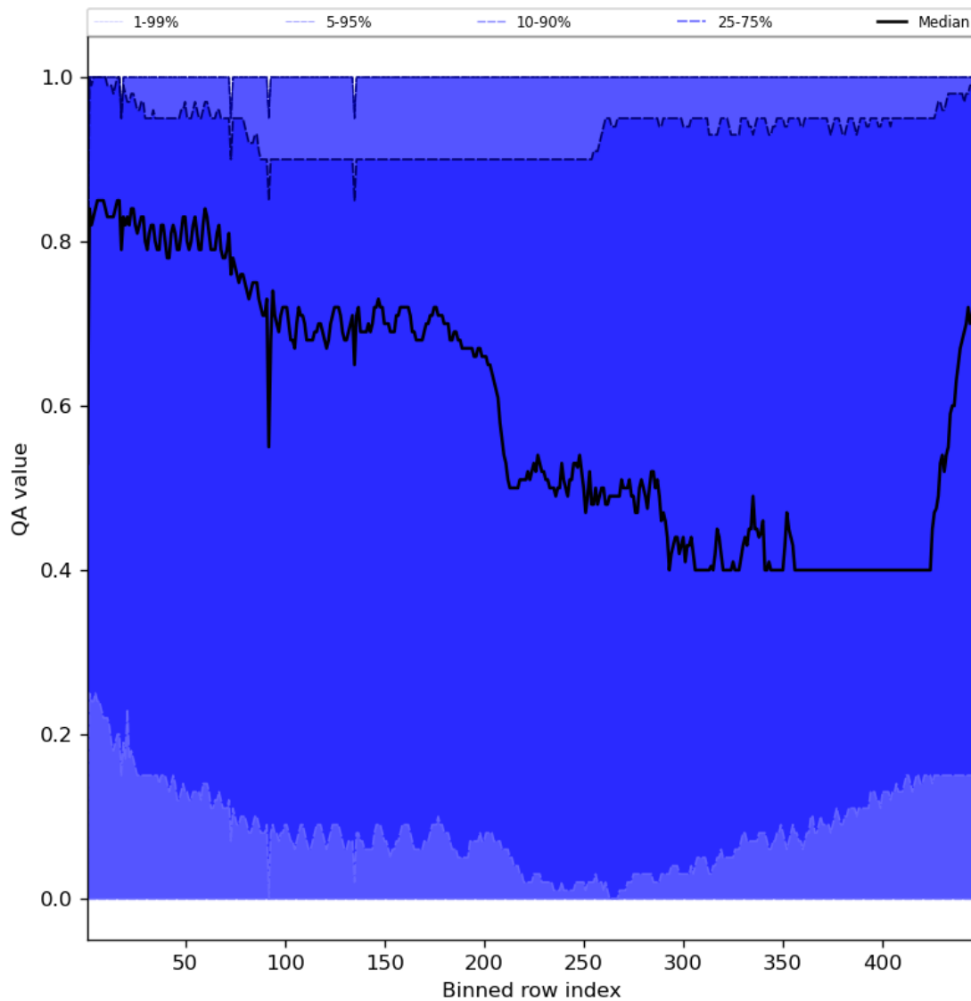
Figure 54: Along track statistics of “QA value” for 2024-05-16 to 2024-05-18
