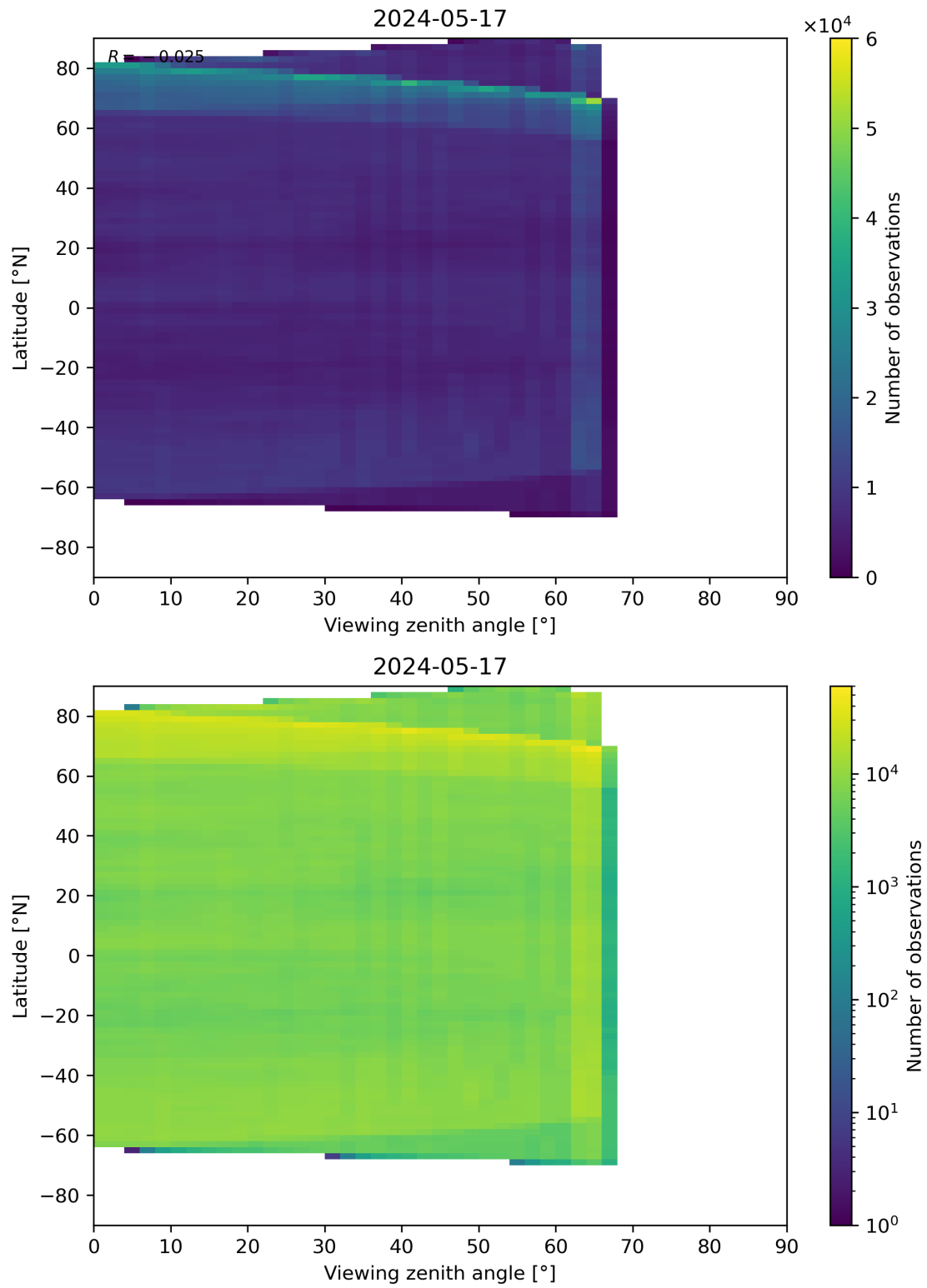
Figure 113: Scatter density plot of “Viewing zenith angle” against “Latitude” for 2024-05-16 to 2024-05-18.
