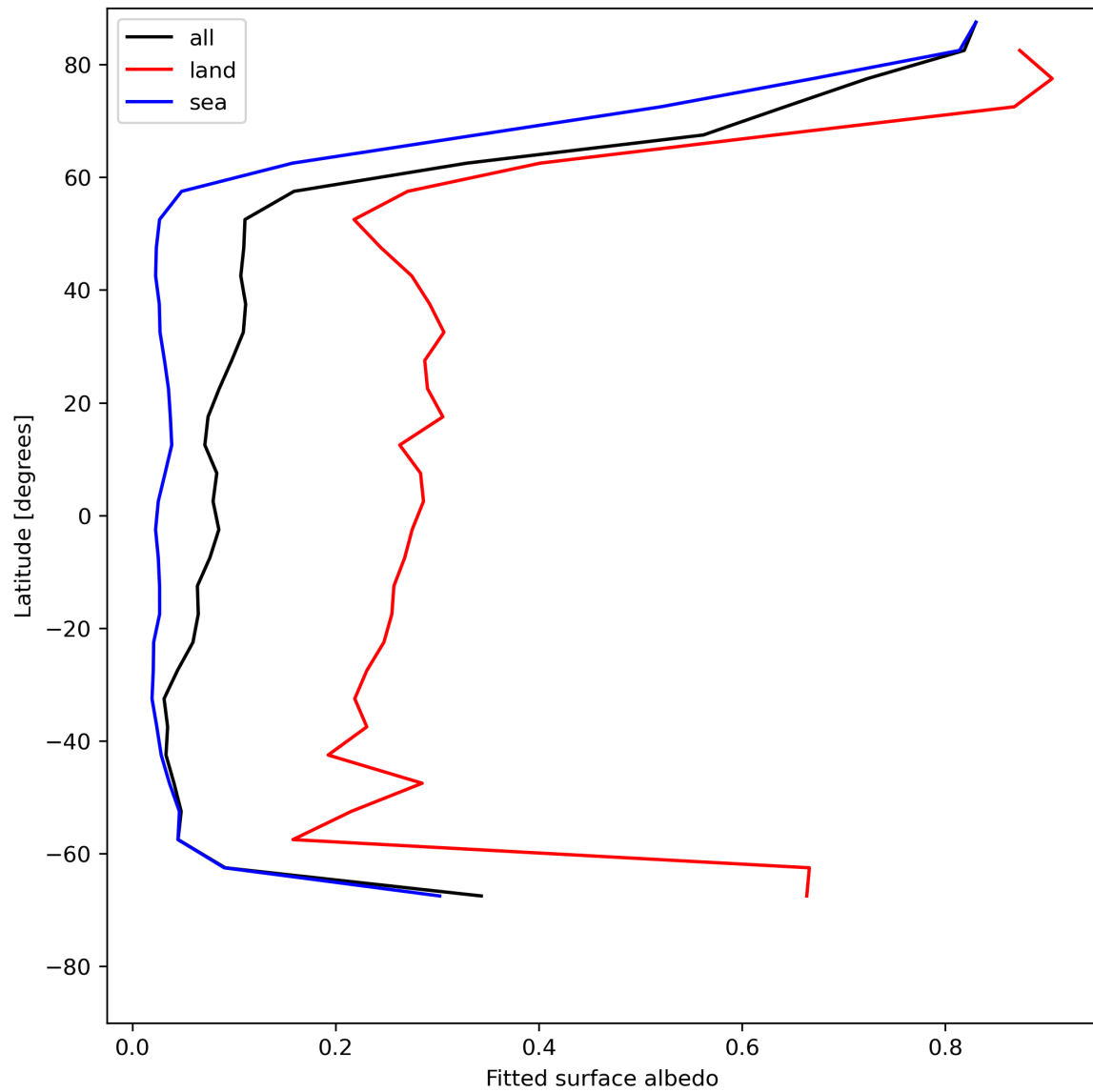
Figure 29: Zonal average of “Fitted surface albedo” for 2024-05-16 to 2024-05-18.
