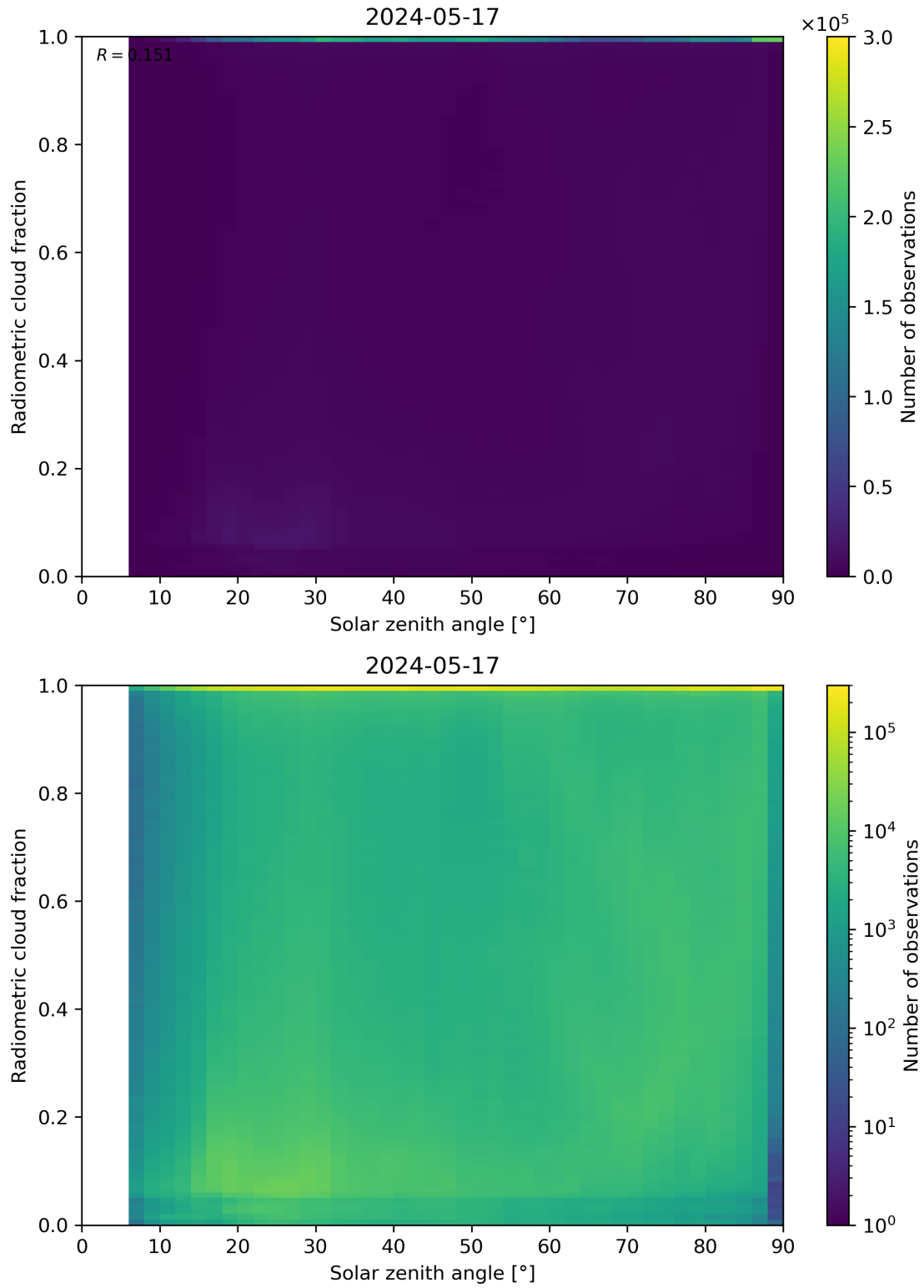
Figure 99: Scatter density plot of “Solar zenith angle” against “Radiometric cloud fraction” for 2024-05-16 to 2024-05-18.
