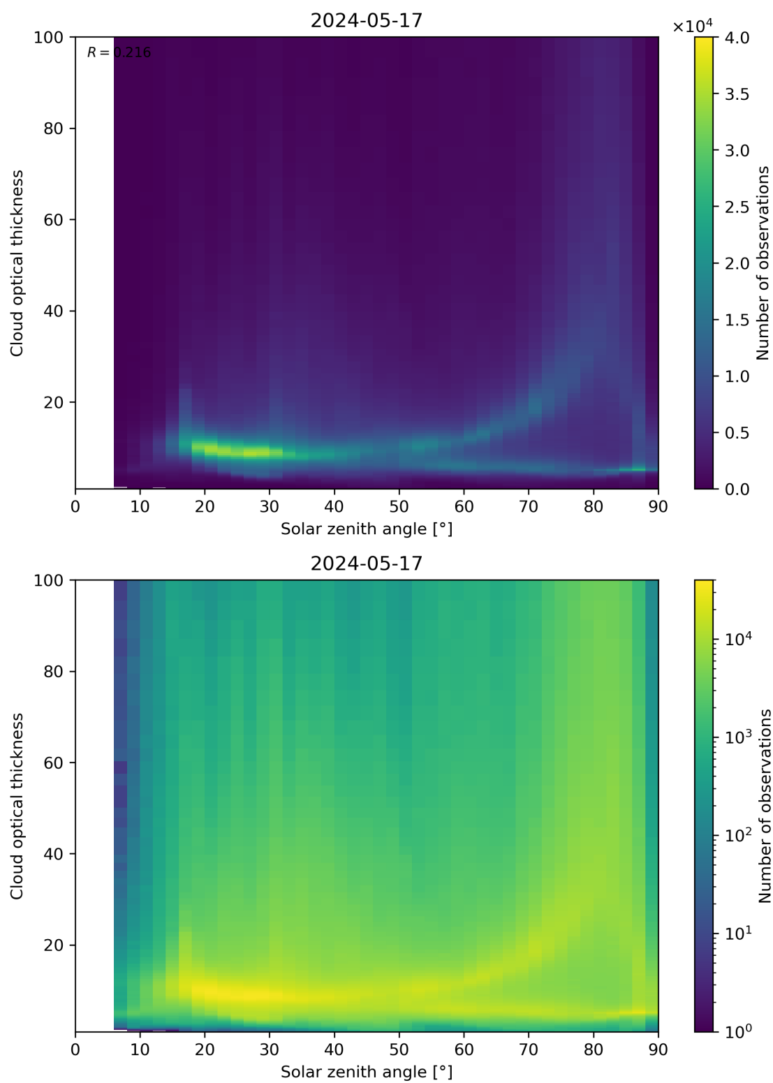
Figure 103: Scatter density plot of “Solar zenith angle” against “Cloud optical thickness” for 2024-05-16 to 2024-05-18.
