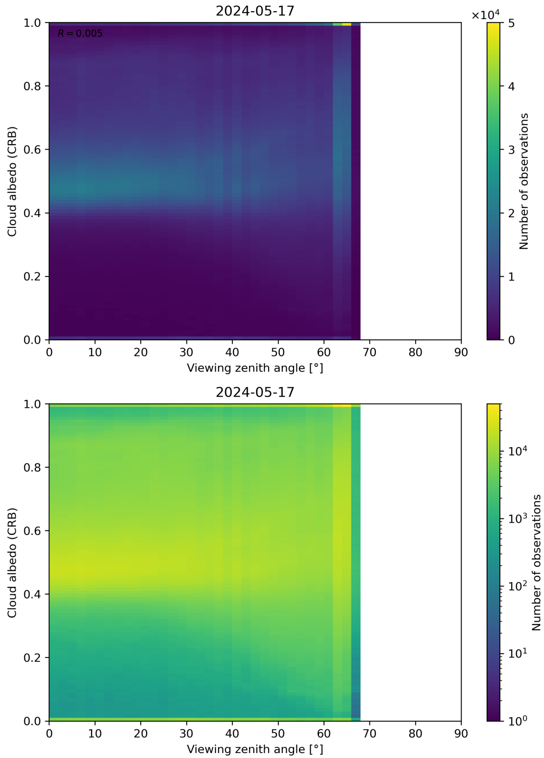
Figure 106: Scatter density plot of “Viewing zenith angle” against “Cloud albedo (CRB)” for 2024-05-16 to 2024-05-18.
