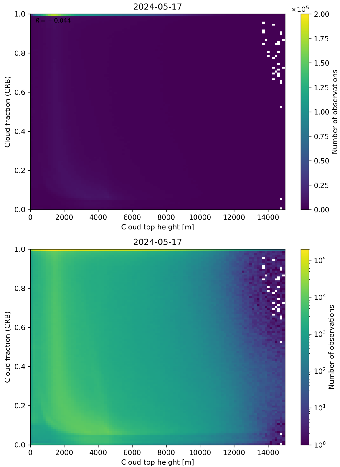
Figure 88: Scatter density plot of “Cloud top height” against “Cloud fraction (CRB)” for 2024-05-16 to 2024-05-18.
