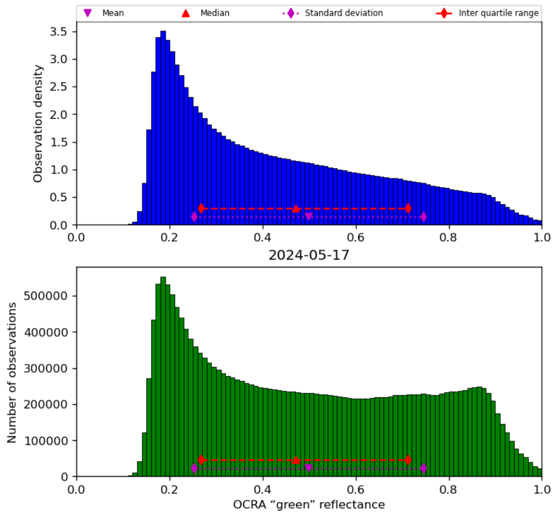
Figure 52: Histogram of “OCRA “green” reflectance” for 2024-05-16 to 2024-05-18
