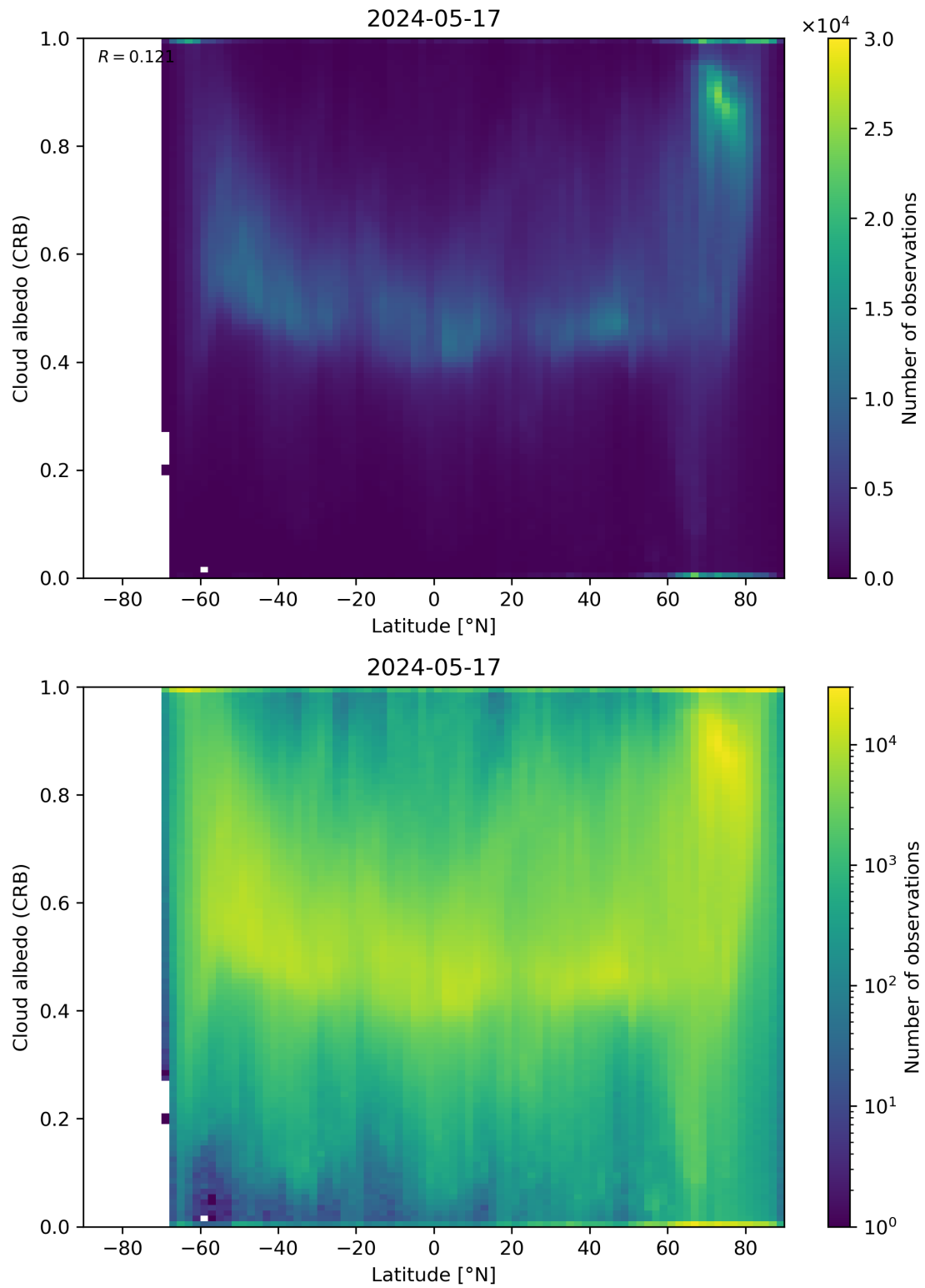
Figure 91: Scatter density plot of “Latitude” against “Cloud albedo (CRB)” for 2024-05-16 to 2024-05-18.
