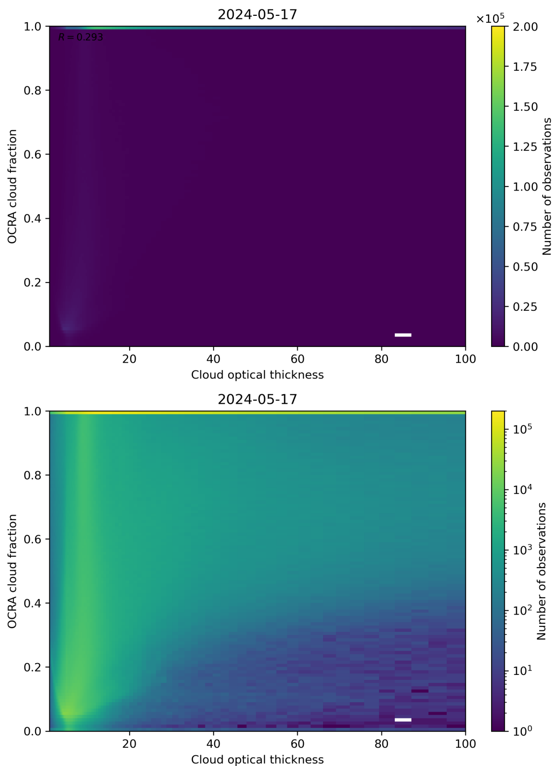
Figure 83: Scatter density plot of “Cloud optical thickness” against “OCRA cloud fraction” for 2024-05-16 to 2024-05-18.
