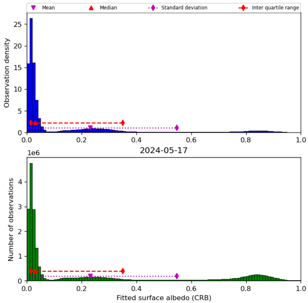
Figure 46: Histogram of “Fitted surface albedo (CRB)” for 2024-05-16 to 2024-05-18
