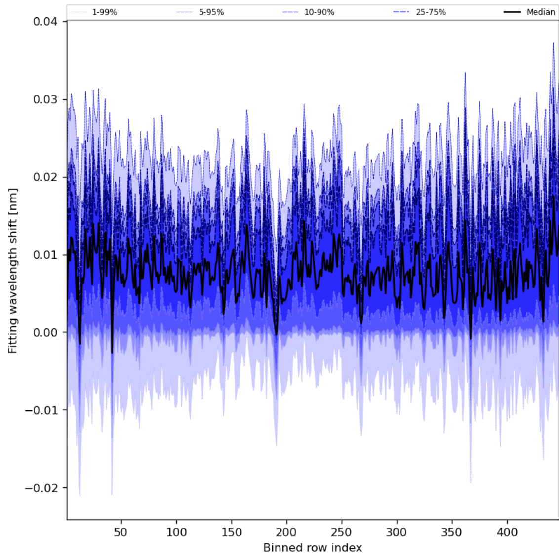
Figure 65: Along track statistics of “Fitting wavelength shift” for 2024-05-16 to 2024-05-18
