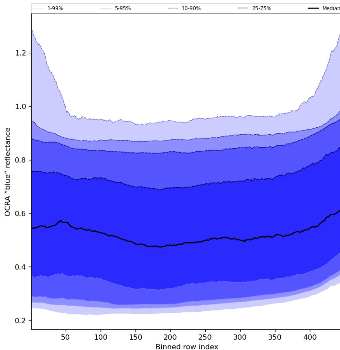
Figure 67: Along track statistics of “OCRA “blue” reflectance” for 2024-05-16 to 2024-05-18
