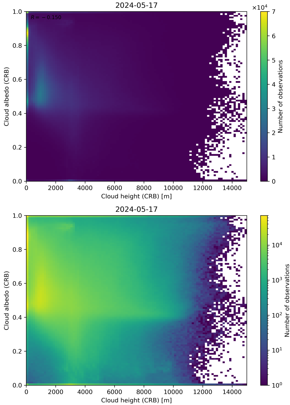
Figure 80: Scatter density plot of “Cloud height (CRB)” against “Cloud albedo (CRB)” for 2024-05-16 to 2024-05-18.
