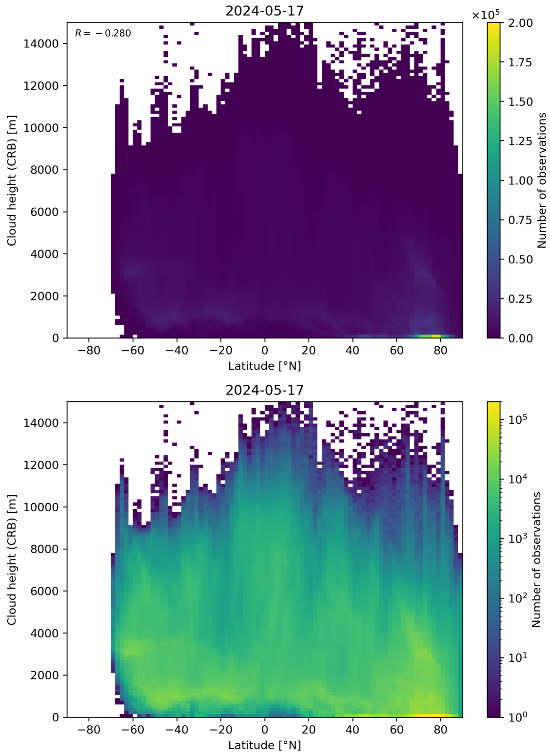
Figure 95: Scatter density plot of “Latitude” against “Cloud height (CRB)” for 2024-05-16 to 2024-05-18.
