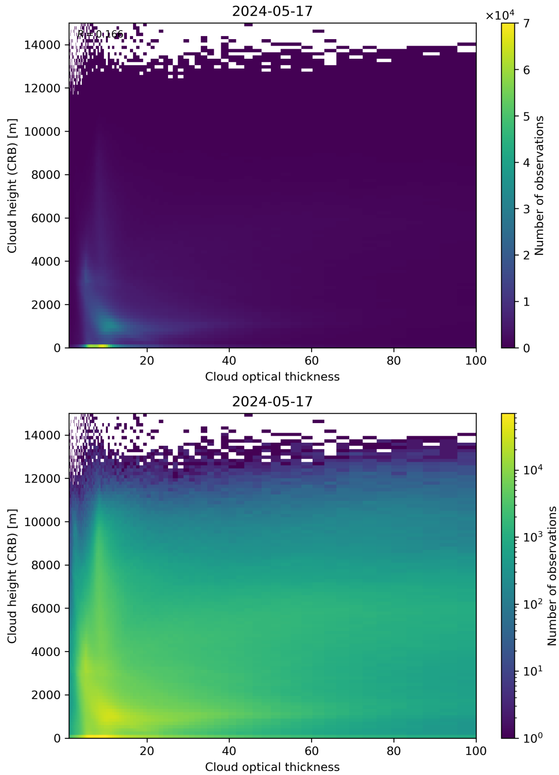
Figure 85: Scatter density plot of “Cloud optical thickness” against “Cloud height (CRB)” for 2024-05-16 to 2024-05-18.
