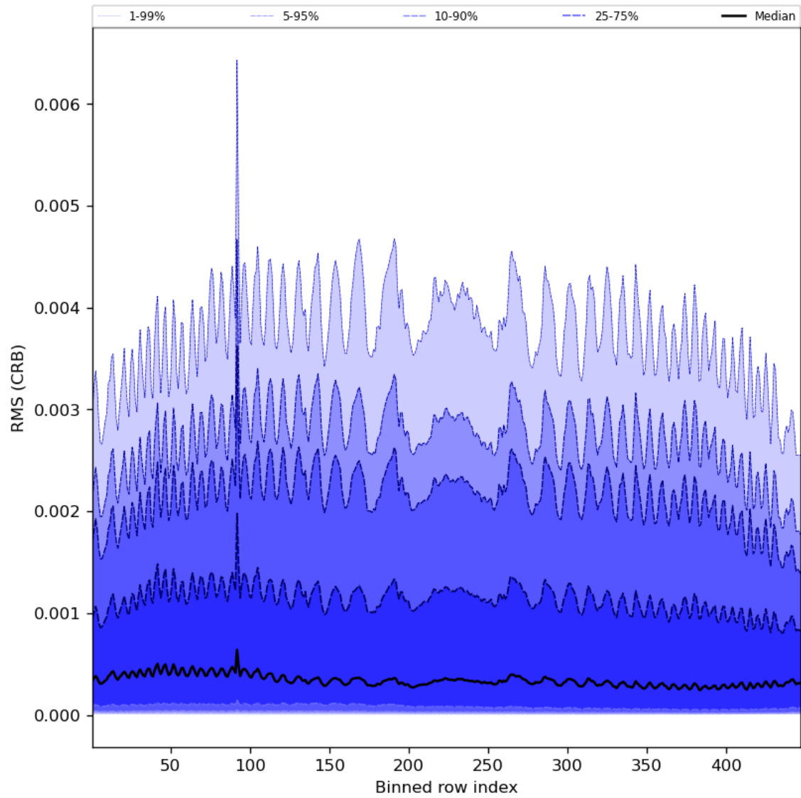
Figure 64: Along track statistics of “RMS (CRB)” for 2024-05-16 to 2024-05-18
