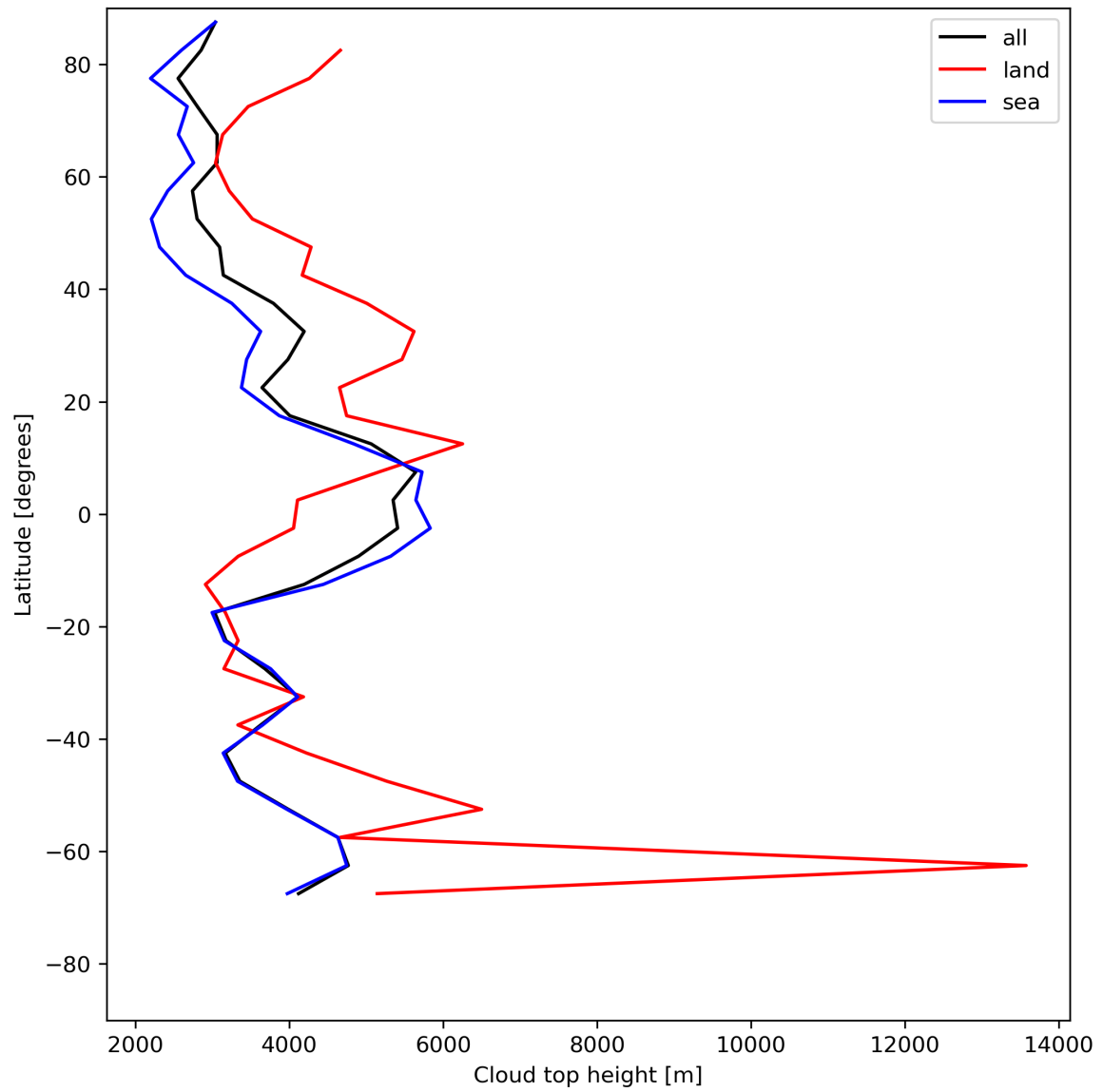
Figure 24: Zonal average of “Cloud top height” for 2024-05-16 to 2024-05-18.
