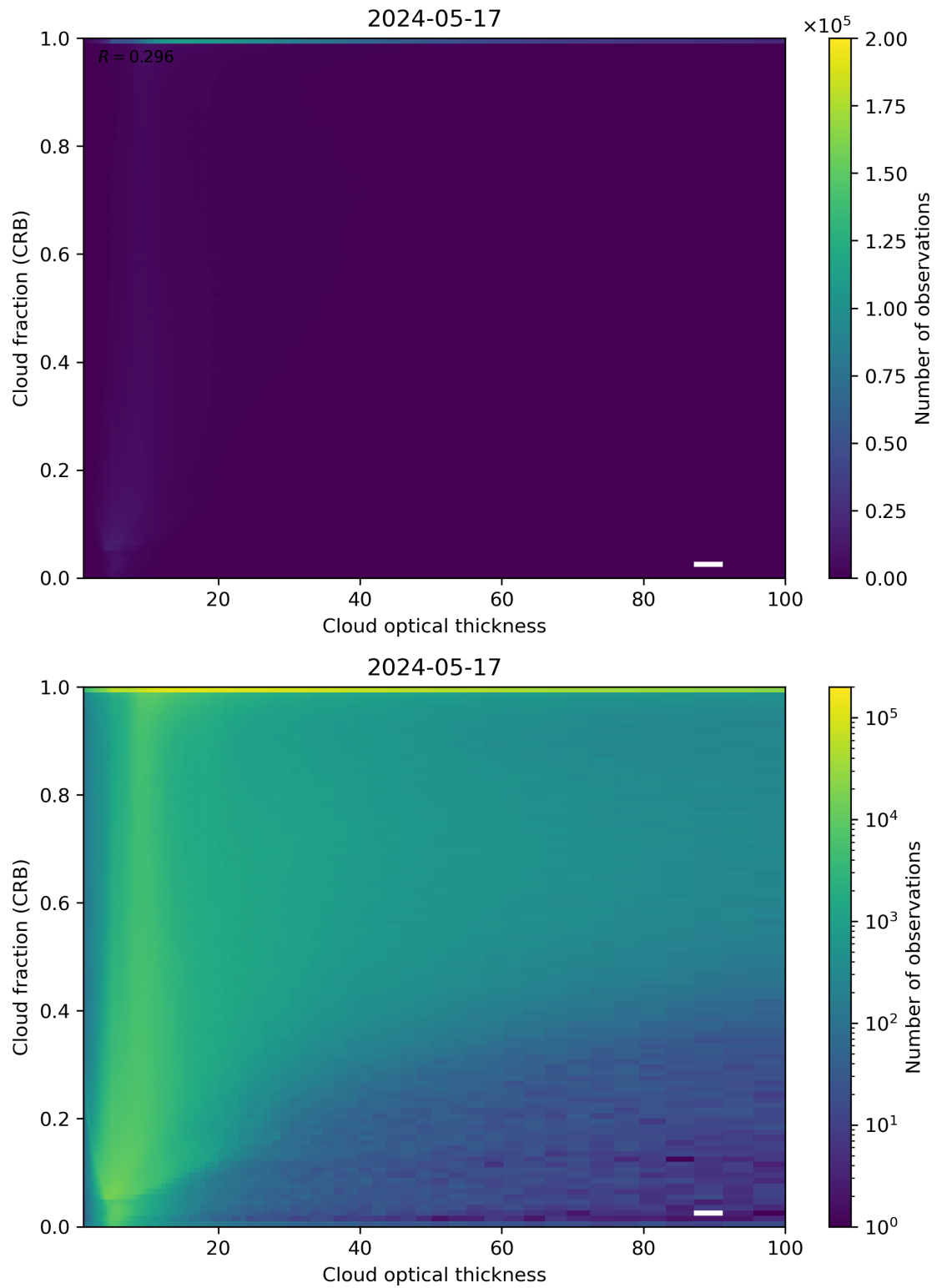
Figure 84: Scatter density plot of “Cloud optical thickness” against “Cloud fraction (CRB)” for 2024-05-16 to 2024-05-18.
