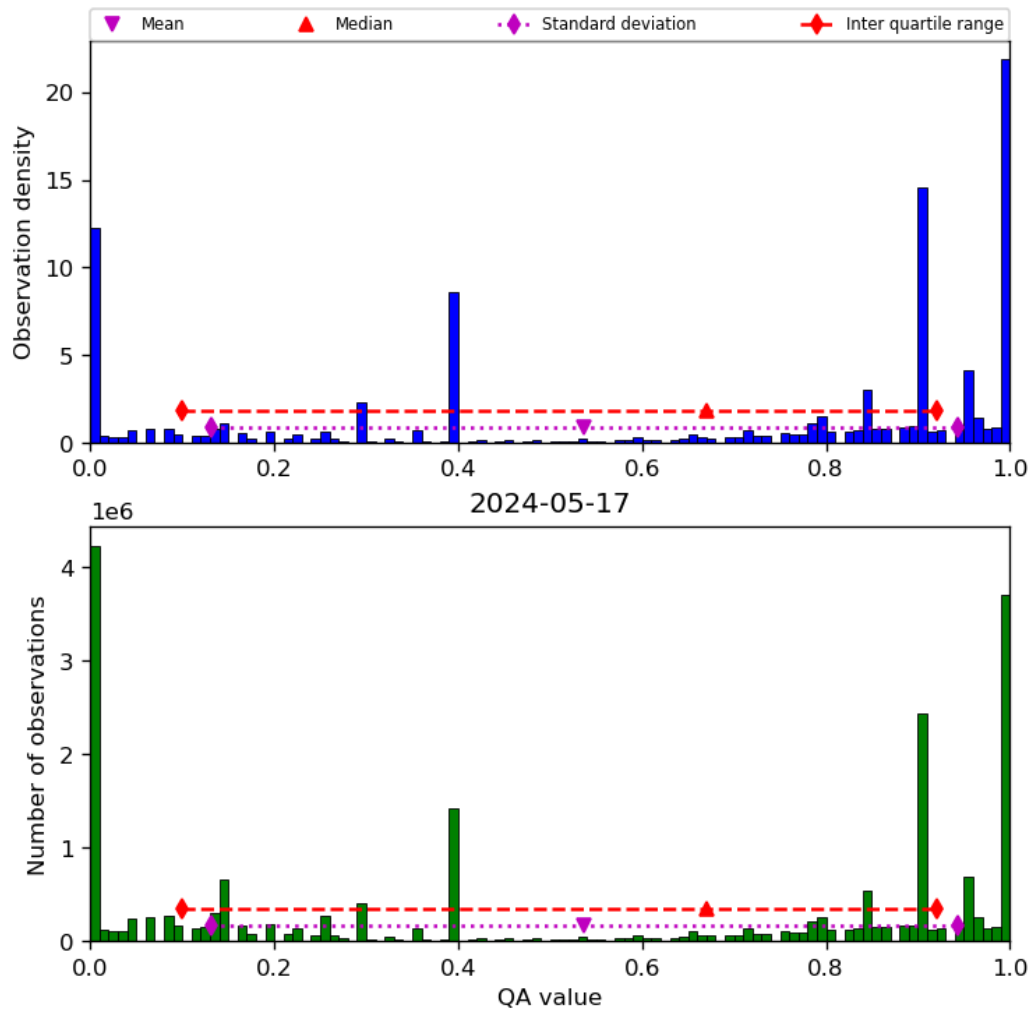
Figure 38: Histogram of “QA value” for 2024-05-16 to 2024-05-18
