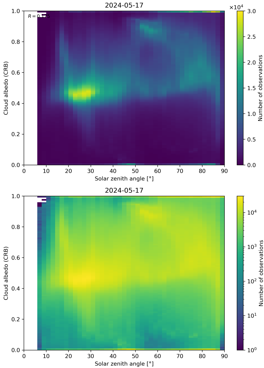
Figure 98: Scatter density plot of “Solar zenith angle” against “Cloud albedo (CRB)” for 2024-05-16 to 2024-05-18.
