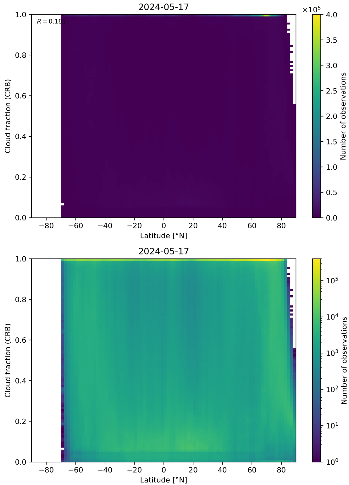
Figure 94: Scatter density plot of “Latitude” against “Cloud fraction (CRB)” for 2024-05-16 to 2024-05-18.
