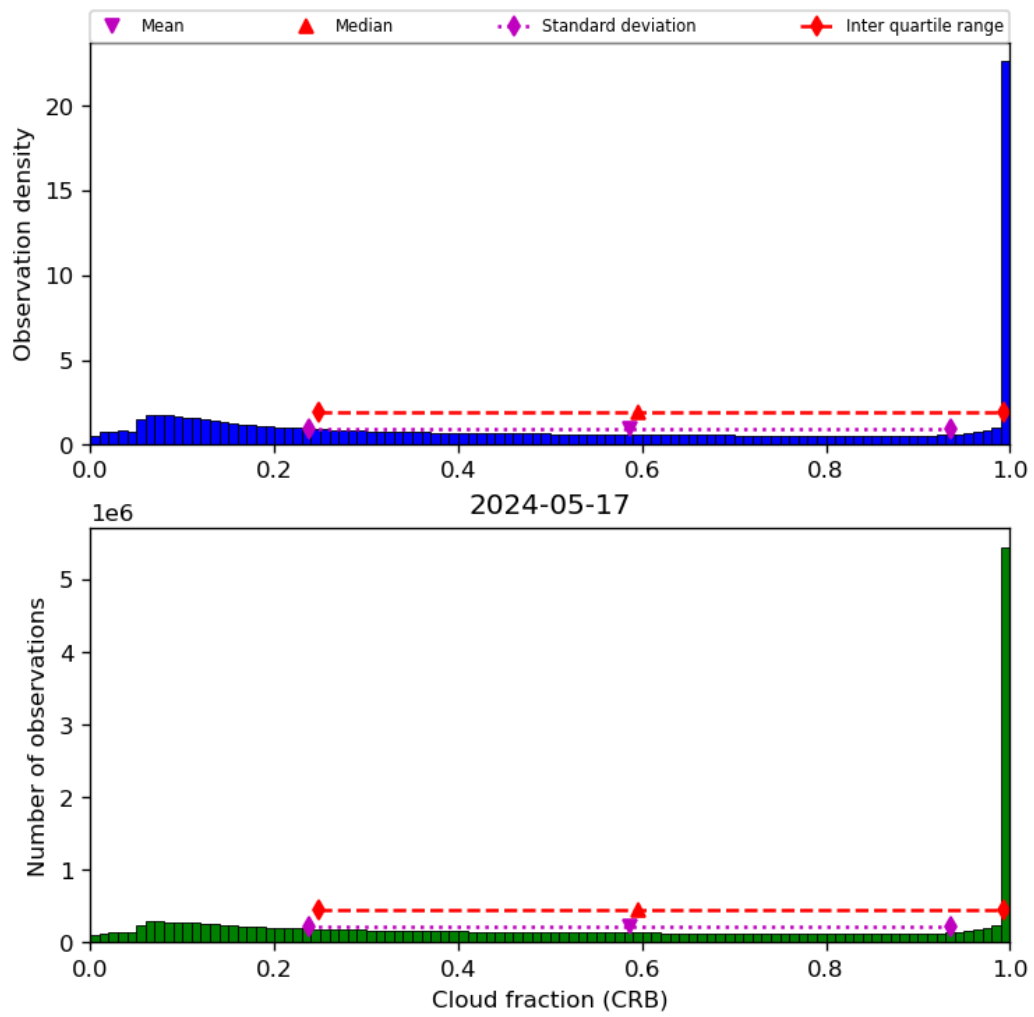
Figure 42: Histogram of “Cloud fraction (CRB)” for 2024-05-16 to 2024-05-18
