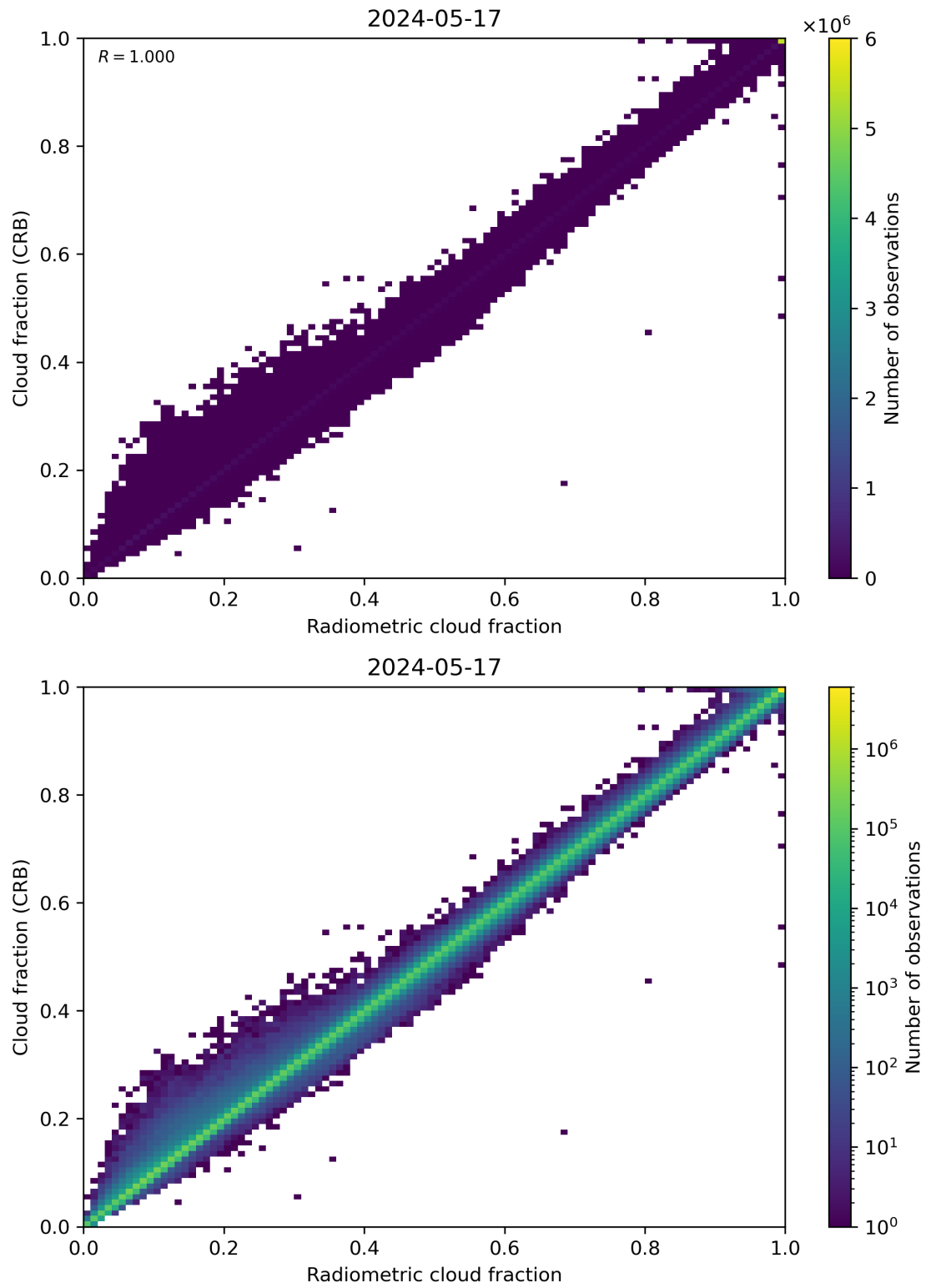
Figure 73: Scatter density plot of “Radiometric cloud fraction” against “Cloud fraction (CRB)” for 2024-05-16 to 2024-05-18.
