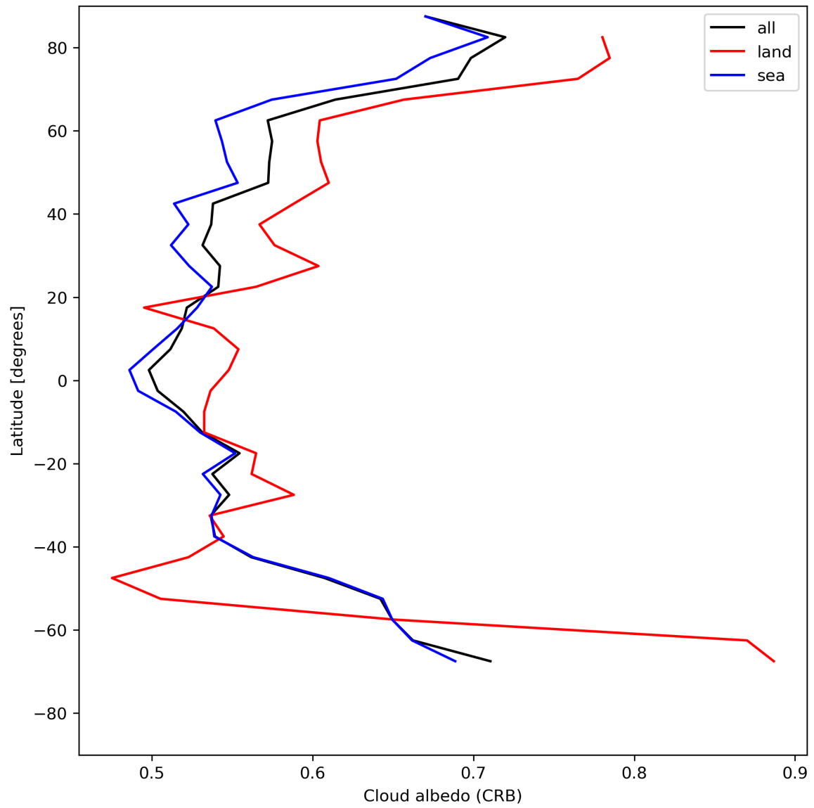
Figure 28: Zonal average of “Cloud albedo (CRB)” for 2024-05-16 to 2024-05-18.
