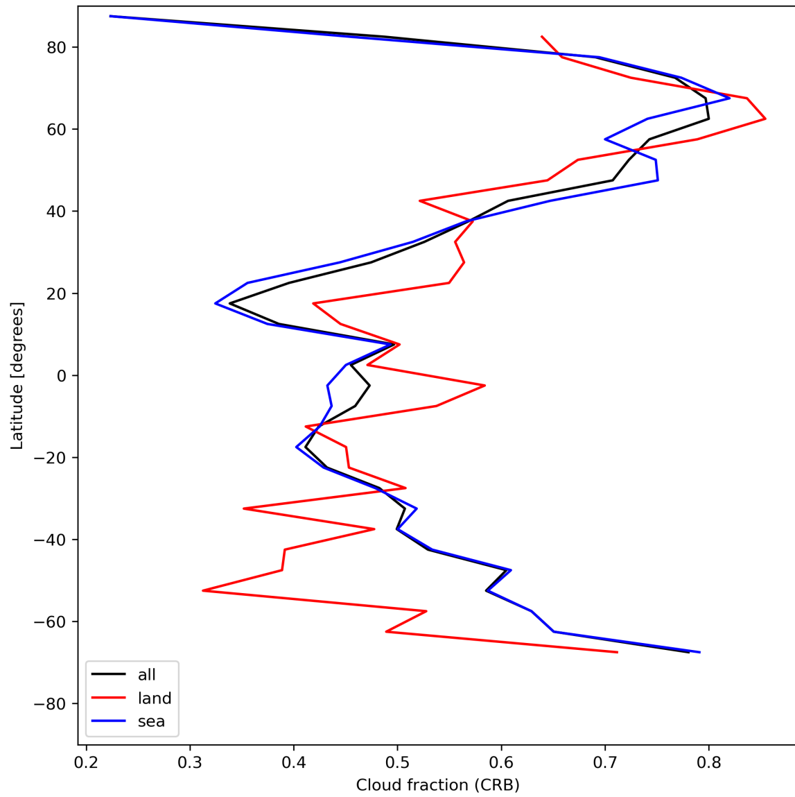
Figure 26: Zonal average of “Cloud fraction (CRB)” for 2024-05-16 to 2024-05-18.
