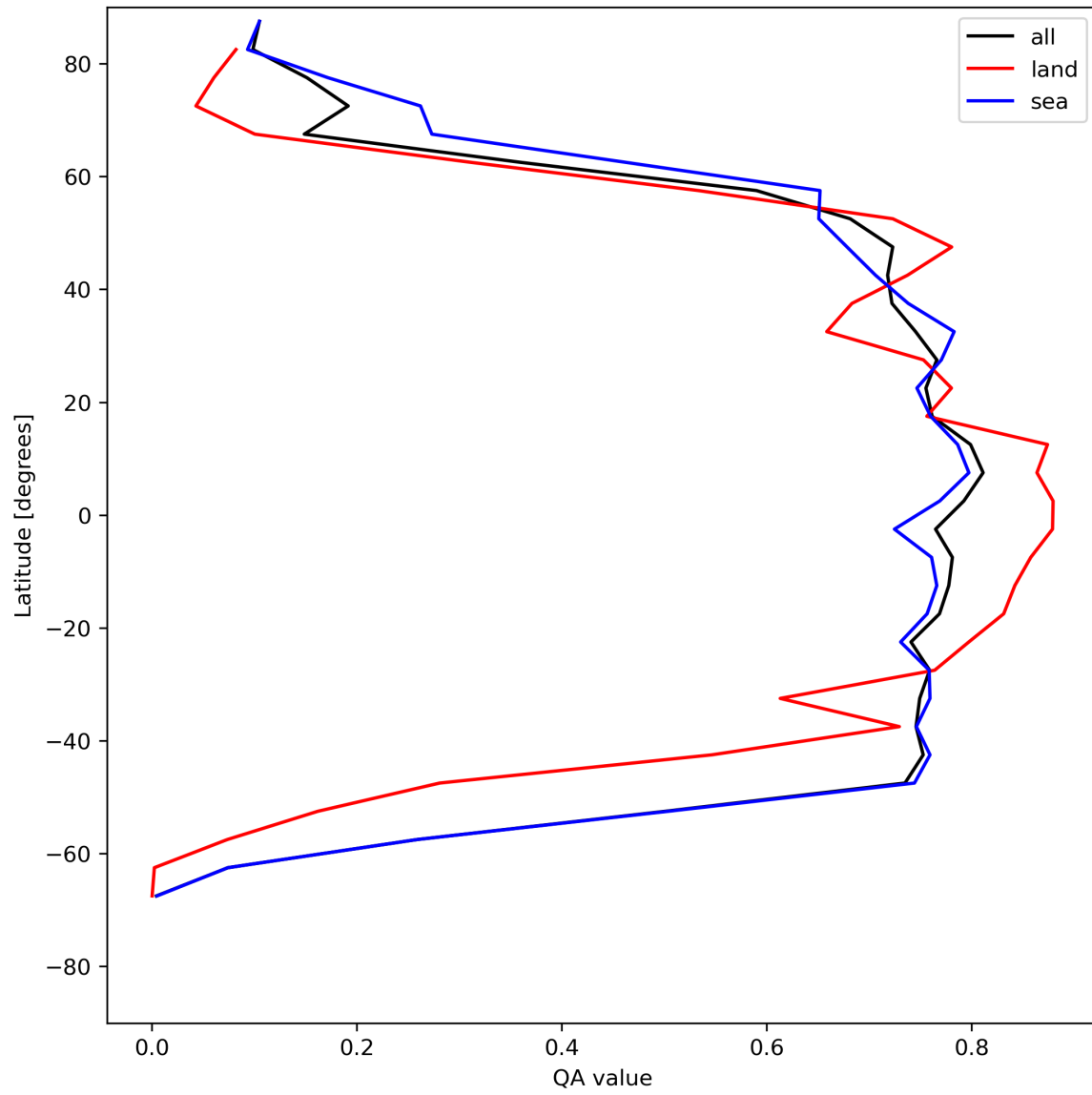
Figure 22: Zonal average of “QA value” for 2024-05-16 to 2024-05-18.
