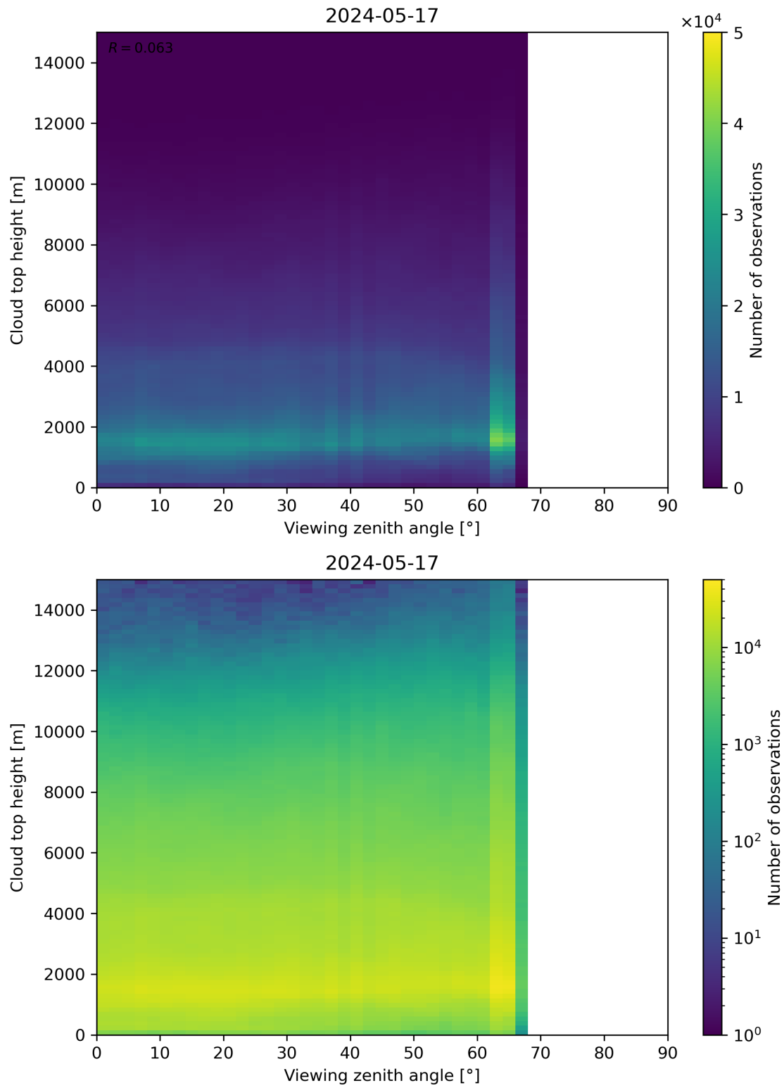
Figure 112: Scatter density plot of “Viewing zenith angle” against “Cloud top height” for 2024-05-16 to 2024-05-18.
