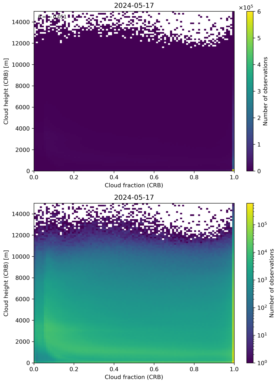
Figure 79: Scatter density plot of “Cloud fraction (CRB)” against “Cloud height (CRB)” for 2024-05-16 to 2024-05-18.
