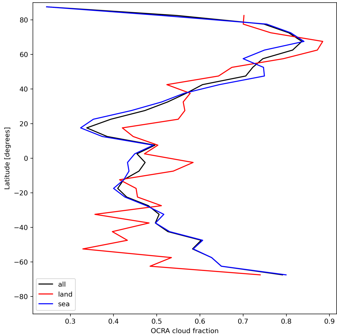
Figure 34: Zonal average of “OCRA cloud fraction” for 2024-05-16 to 2024-05-18.
