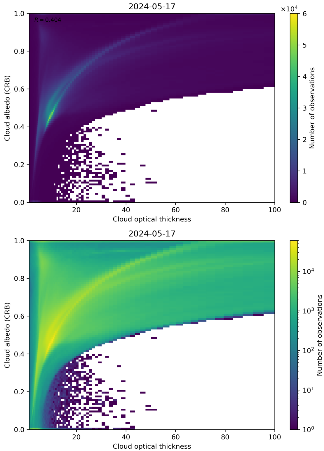
Figure 82: Scatter density plot of “Cloud optical thickness” against “Cloud albedo (CRB)” for 2024-05-16 to 2024-05-18.
