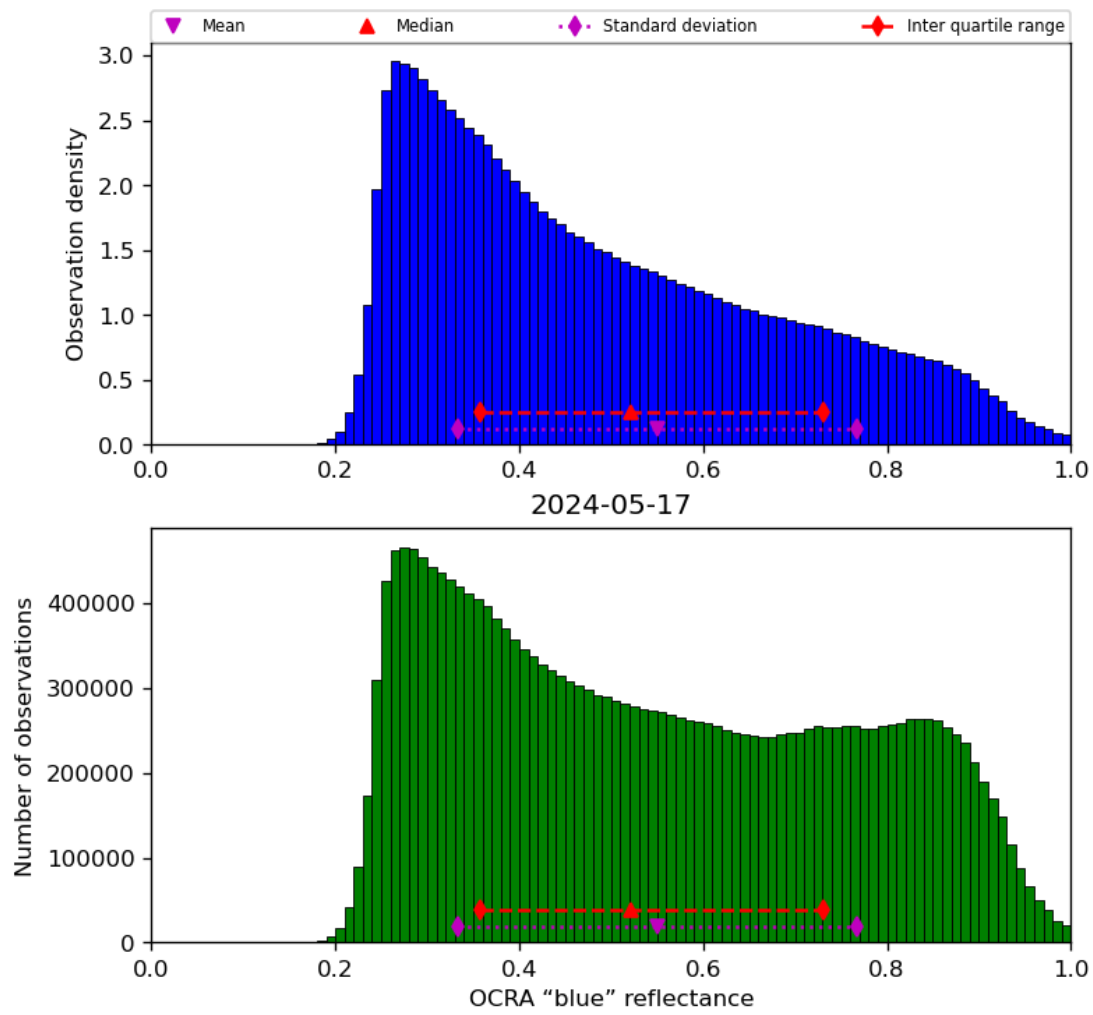
Figure 51: Histogram of “OCRA “blue” reflectance” for 2024-05-16 to 2024-05-18
