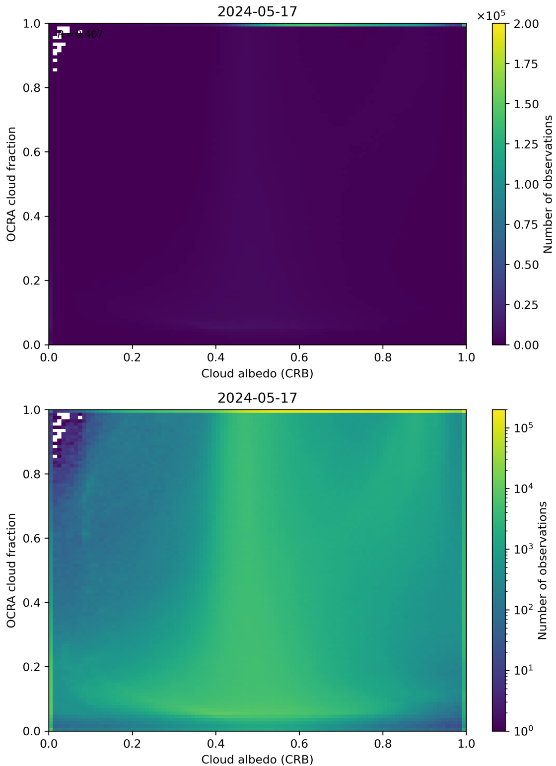
Figure 70: Scatter density plot of “Cloud albedo (CRB)” against “OCRA cloud fraction” for 2024-05-16 to 2024-05-18.
