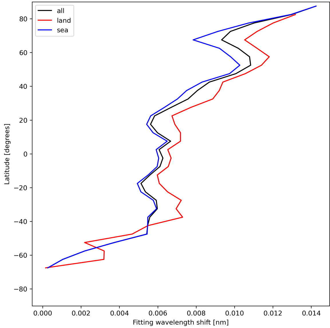
Figure 33: Zonal average of “Fitting wavelength shift” for 2024-05-16 to 2024-05-18.
