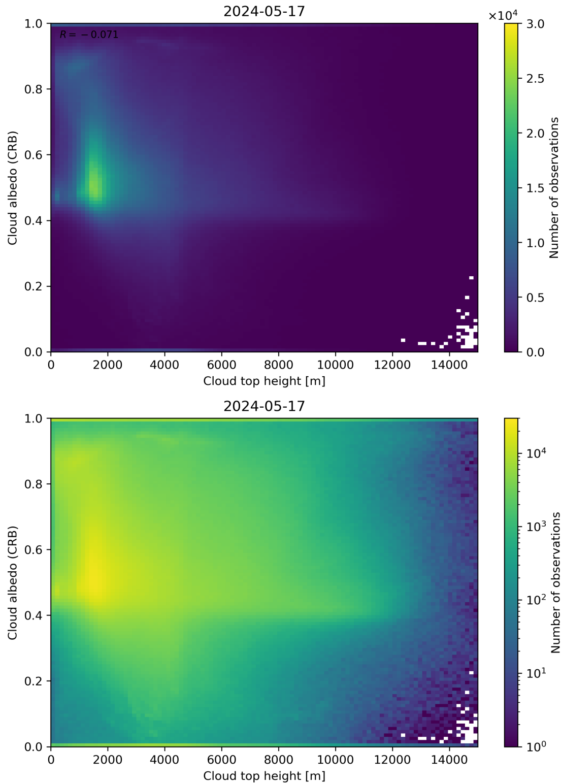
Figure 86: Scatter density plot of “Cloud top height” against “Cloud albedo (CRB)” for 2024-05-16 to 2024-05-18.
