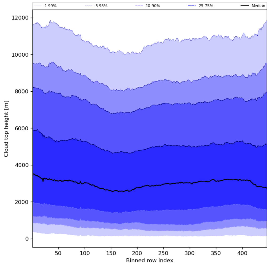
Figure 56: Along track statistics of “Cloud top height” for 2024-05-16 to 2024-05-18
