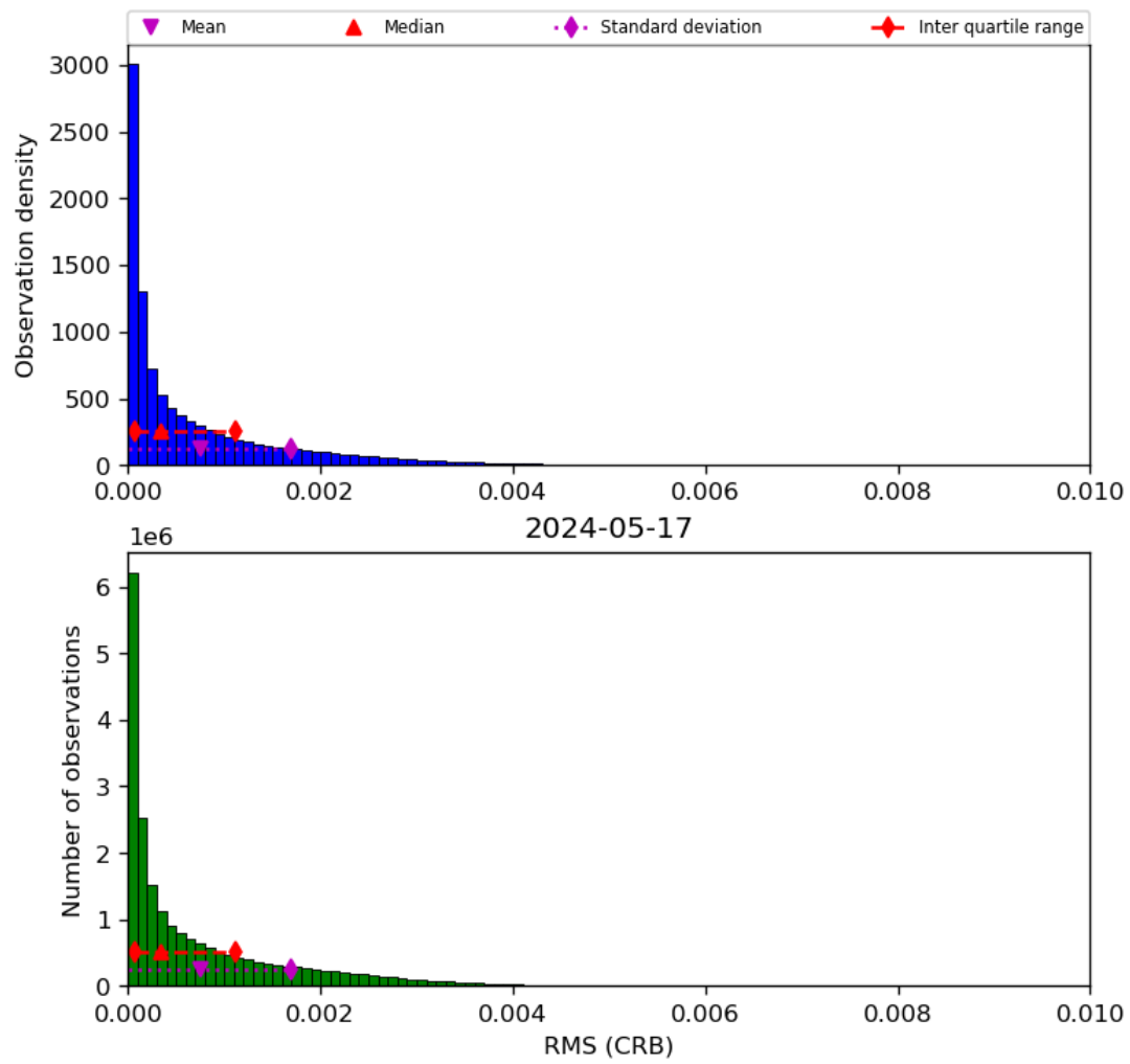
Figure 48: Histogram of “RMS (CRB)” for 2024-05-16 to 2024-05-18
