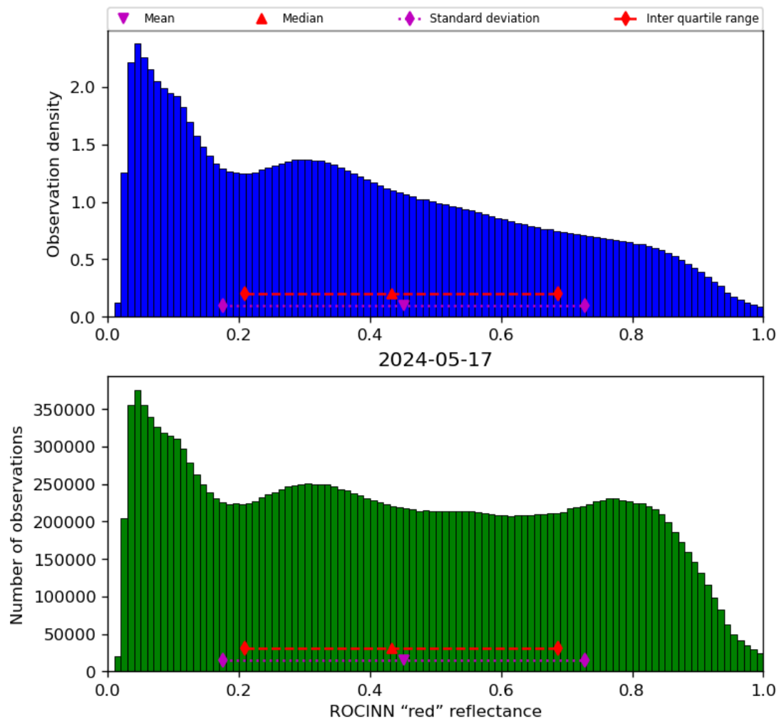
Figure 53: Histogram of “ROCINN “red” reflectance” for 2024-05-16 to 2024-05-18
