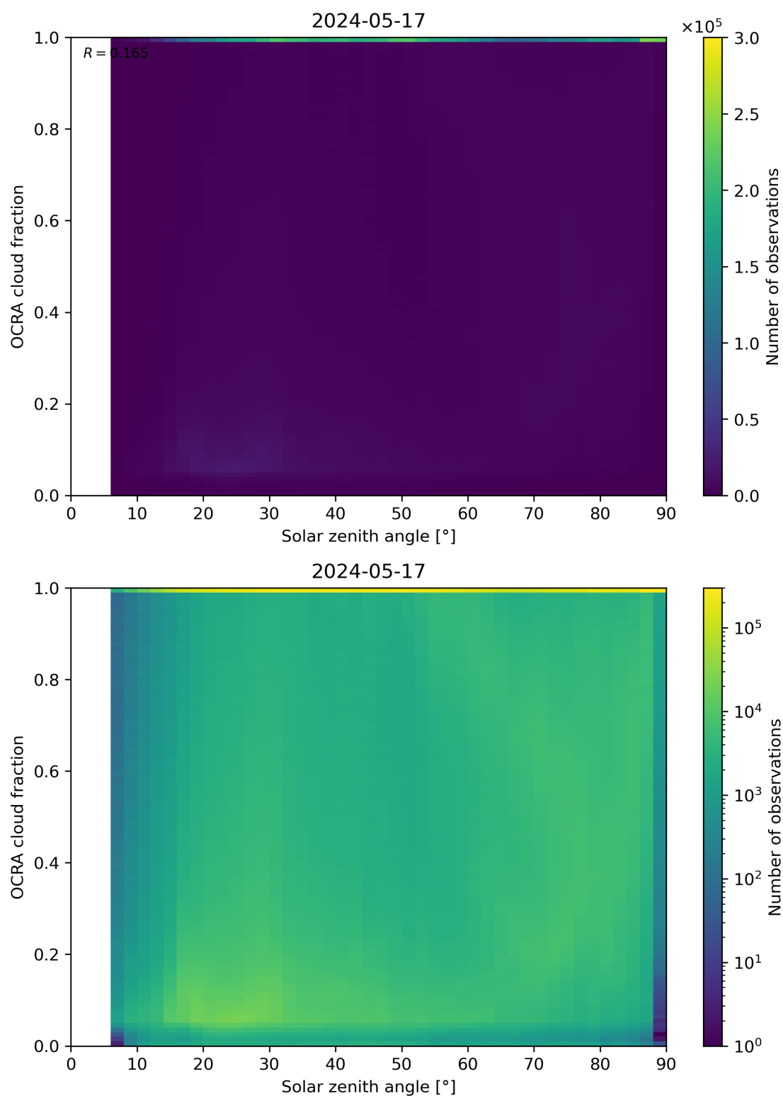
Figure 100: Scatter density plot of “Solar zenith angle” against “OCRA cloud fraction” for 2024-05-16 to 2024-05-18.
