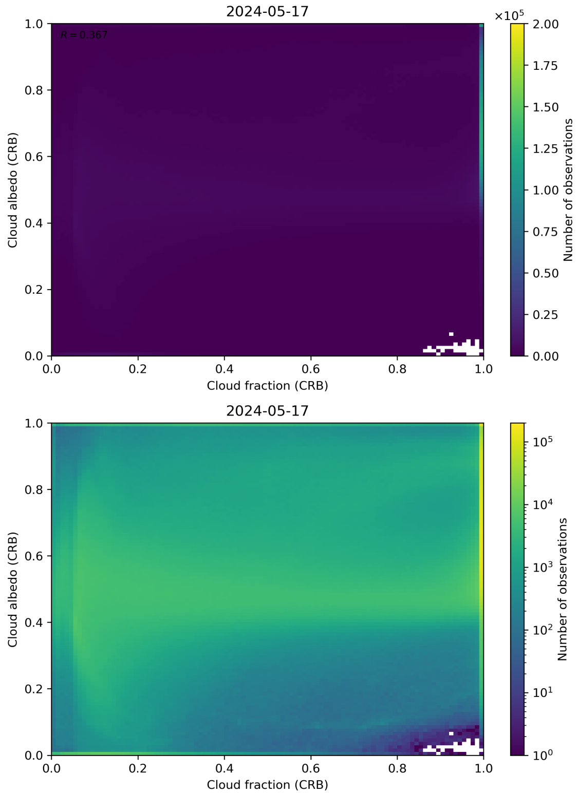
Figure 77: Scatter density plot of “Cloud fraction (CRB)” against “Cloud albedo (CRB)” for 2024-05-16 to 2024-05-18.
