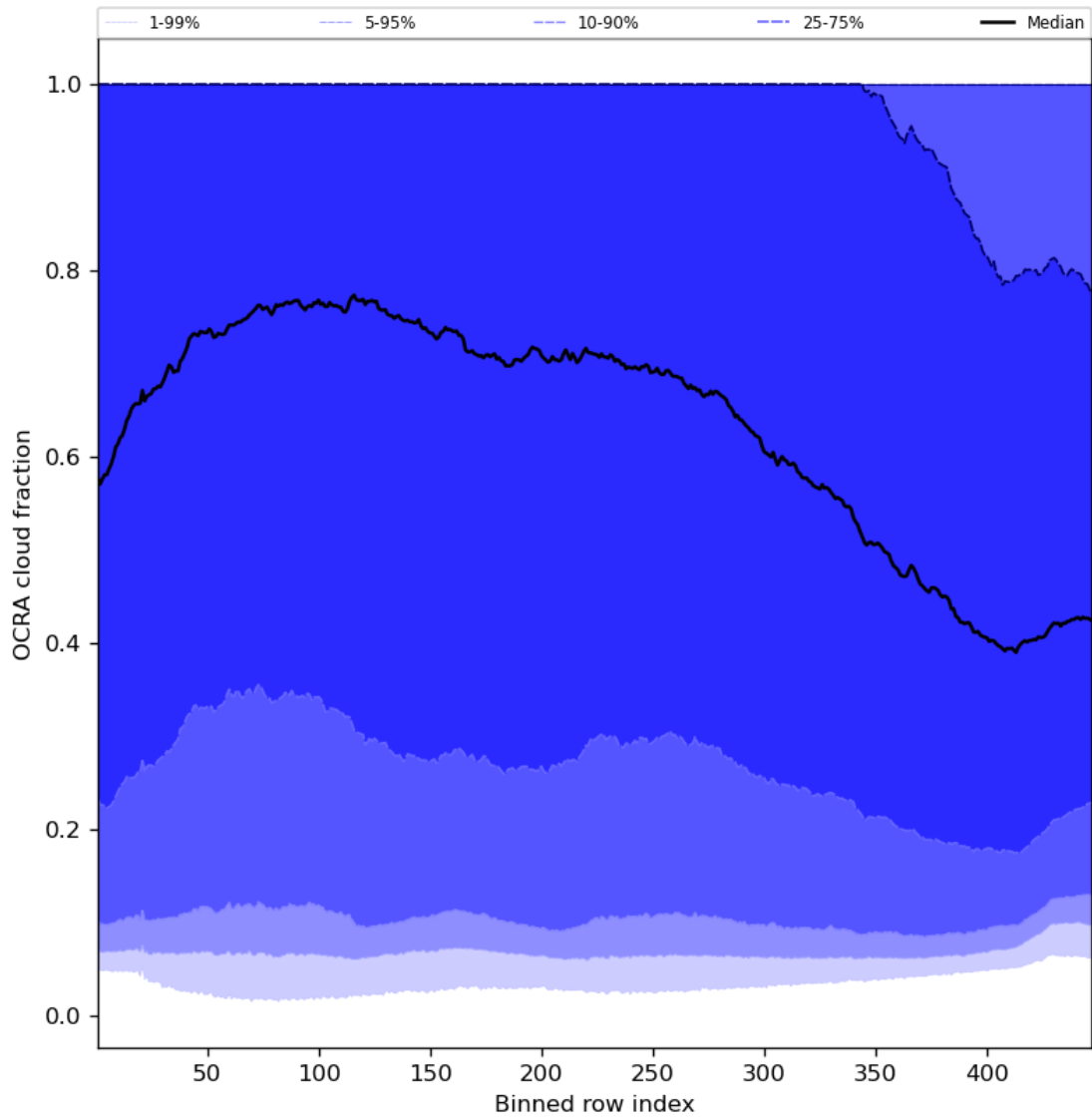
Figure 66: Along track statistics of “OCRA cloud fraction” for 2024-05-16 to 2024-05-18
