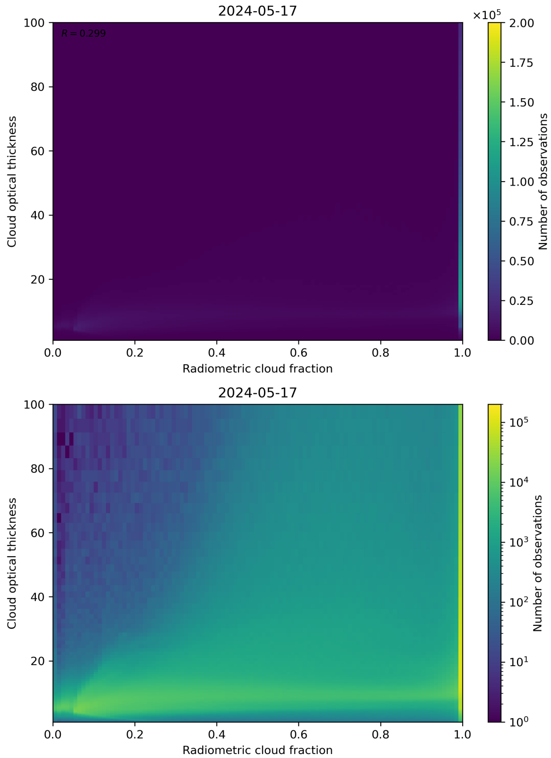
Figure 75: Scatter density plot of “Radiometric cloud fraction” against “Cloud optical thickness” for 2024-05-16 to 2024-05-18.
