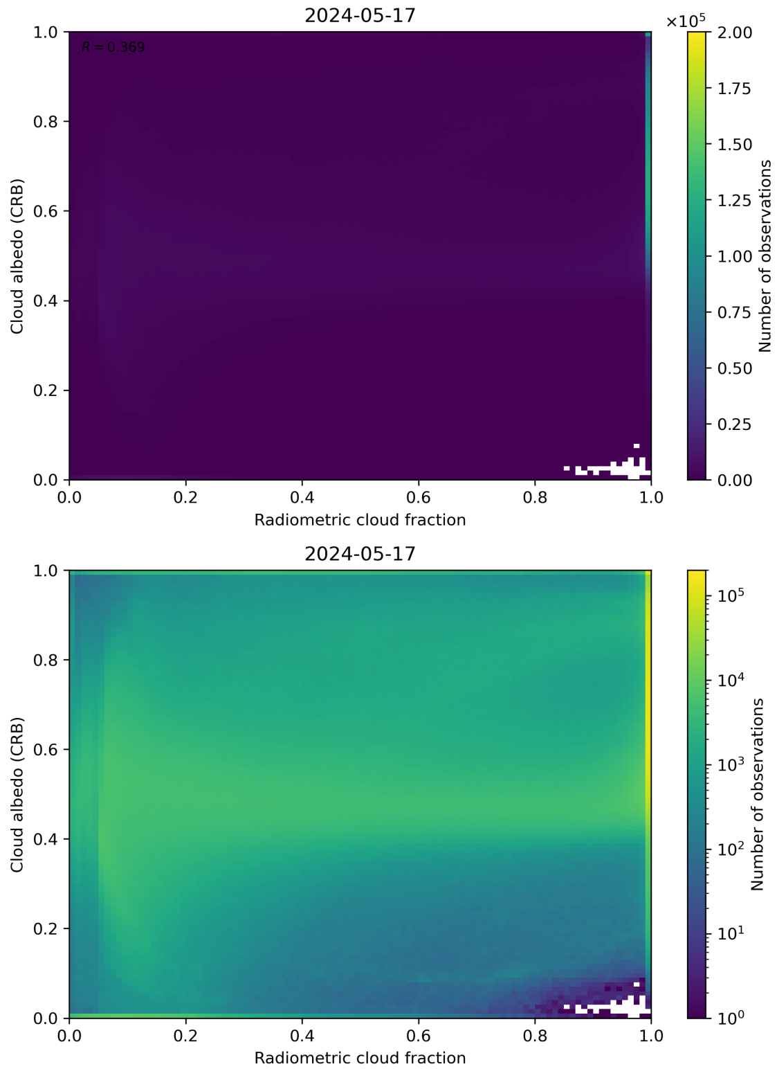
Figure 71: Scatter density plot of “Radiometric cloud fraction” against “Cloud albedo (CRB)” for 2024-05-16 to 2024-05-18.
