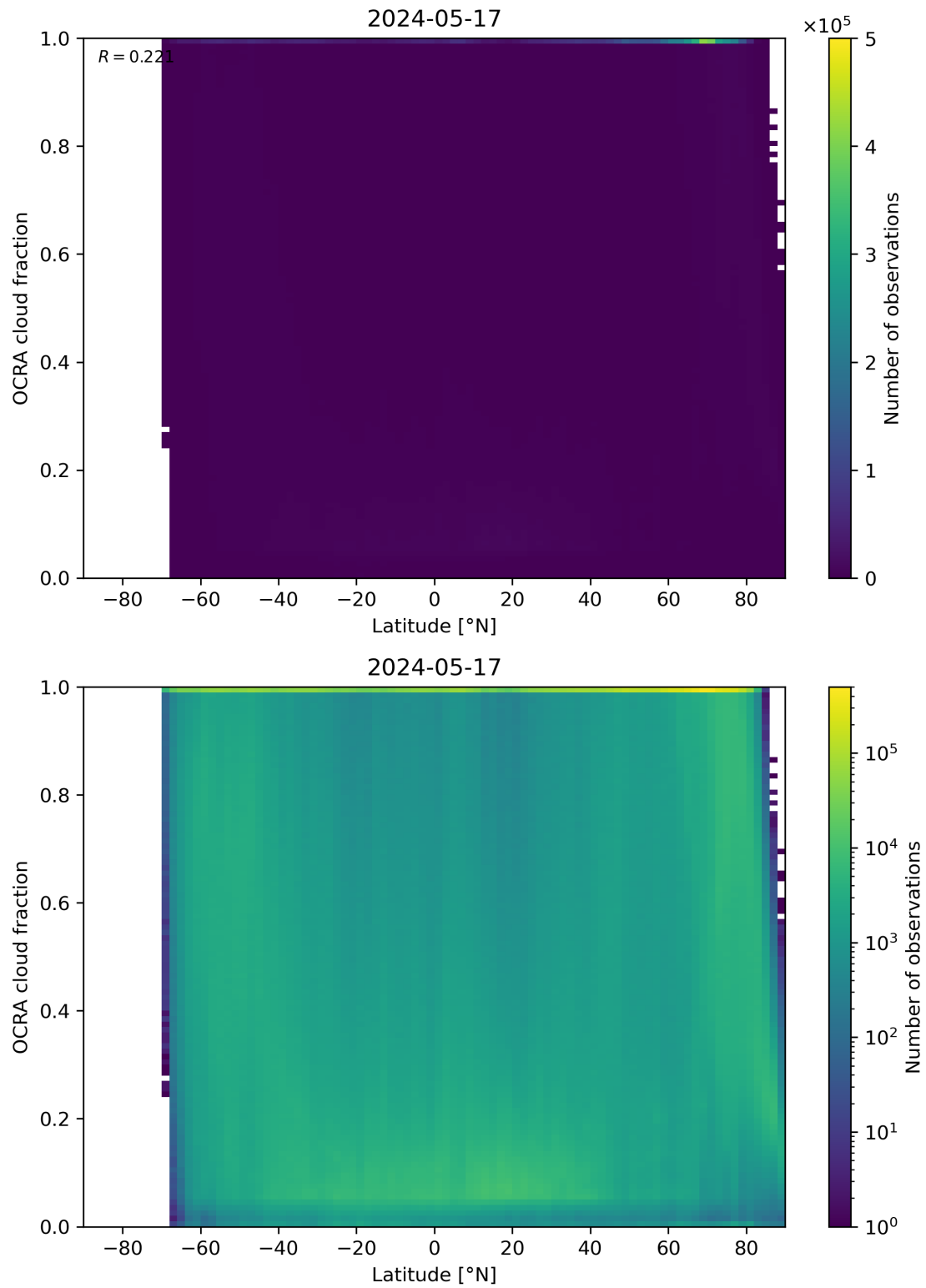
Figure 93: Scatter density plot of “Latitude” against “OCRA cloud fraction” for 2024-05-16 to 2024-05-18.
