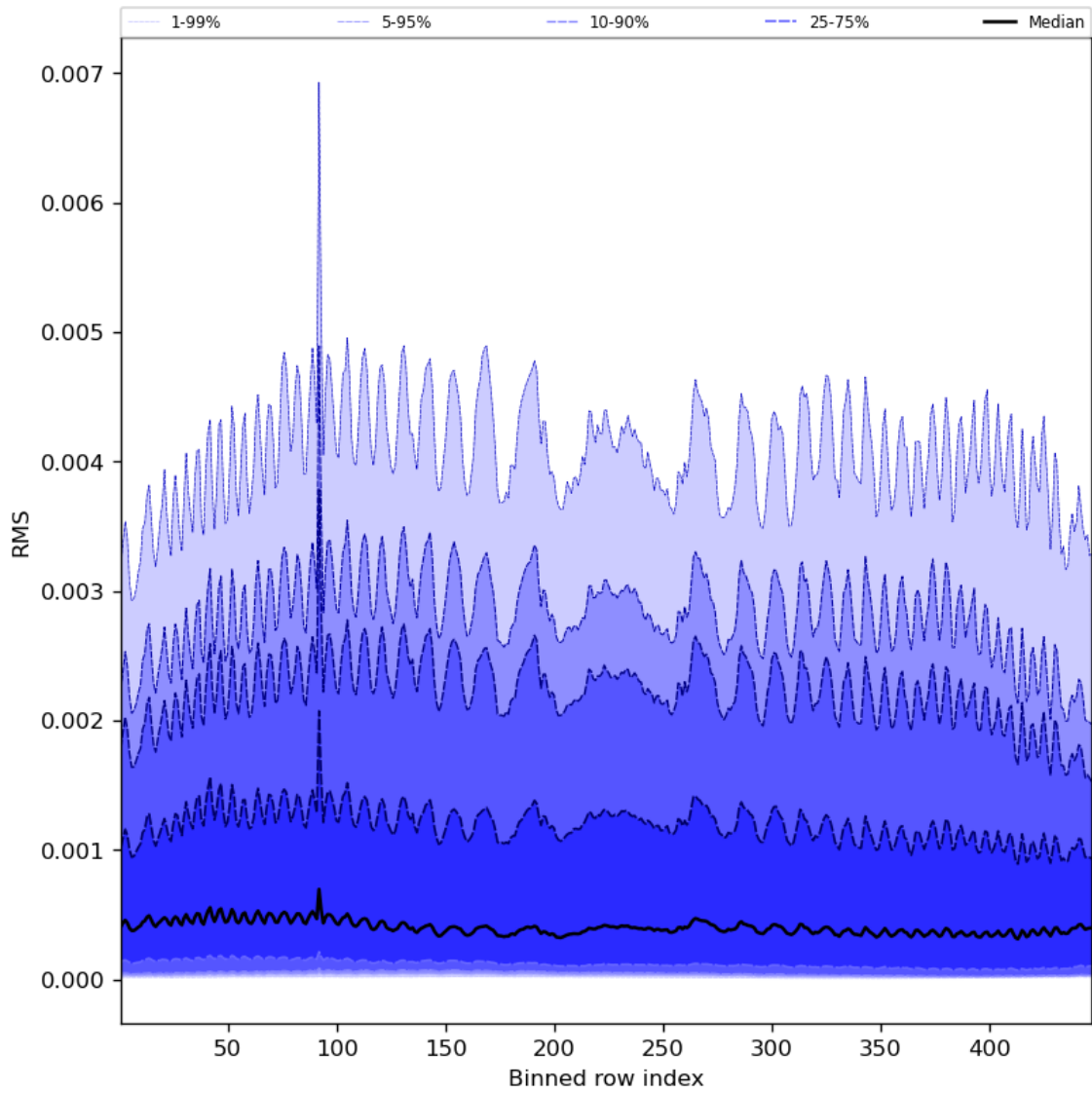
Figure 63: Along track statistics of “RMS” for 2024-05-16 to 2024-05-18
