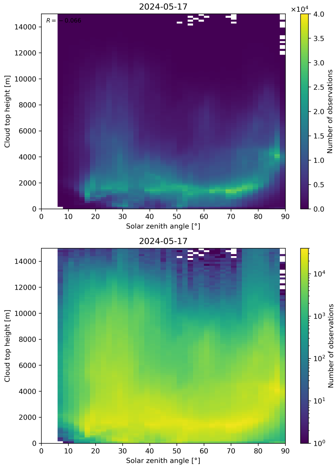
Figure 104: Scatter density plot of “Solar zenith angle” against “Cloud top height” for 2024-05-16 to 2024-05-18.
