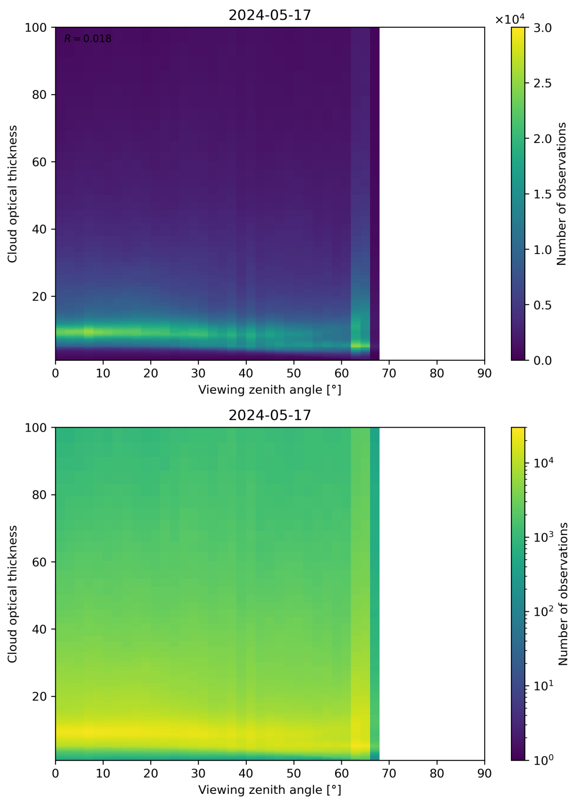
Figure 111: Scatter density plot of “Viewing zenith angle” against “Cloud optical thickness” for 2024-05-16 to 2024-05-18.
