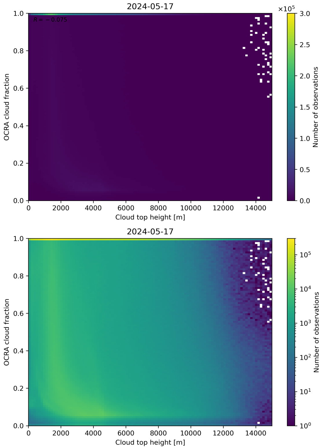
Figure 87: Scatter density plot of “Cloud top height” against “OCRA cloud fraction” for 2024-05-16 to 2024-05-18.
