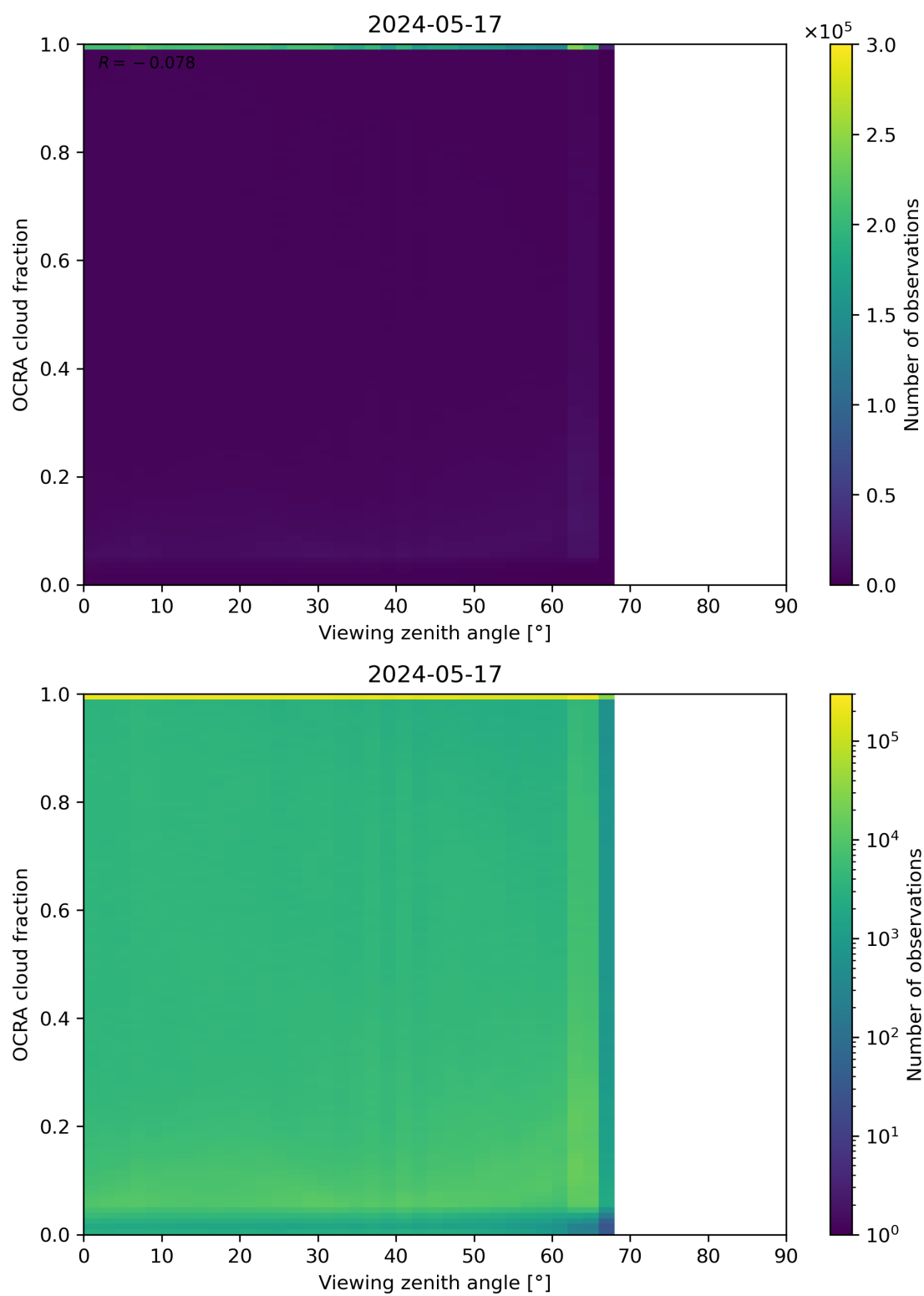
Figure 108: Scatter density plot of “Viewing zenith angle” against “OCRA cloud fraction” for 2024-05-16 to 2024-05-18.
