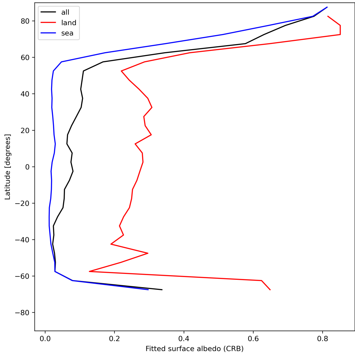
Figure 30: Zonal average of “Fitted surface albedo (CRB)” for 2024-05-16 to 2024-05-18.
