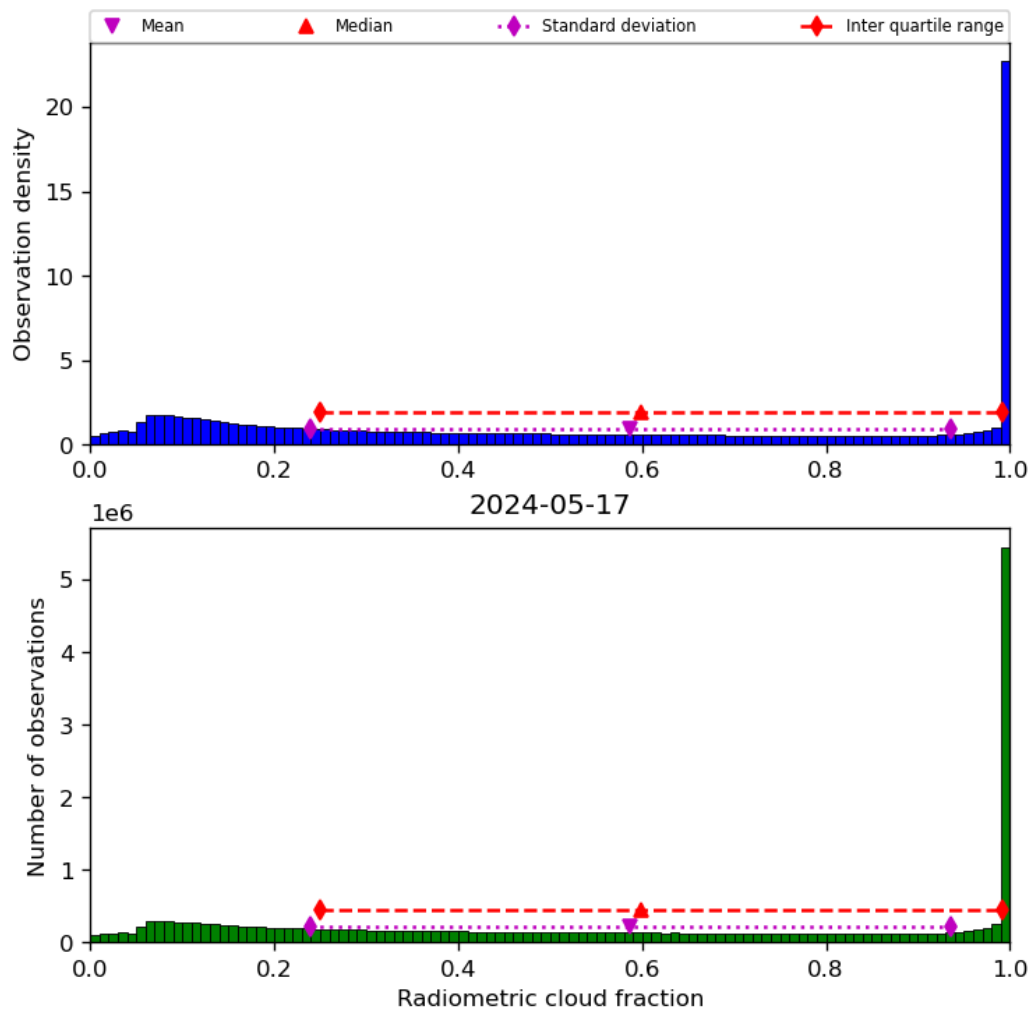
Figure 39: Histogram of “Radiometric cloud fraction” for 2024-05-16 to 2024-05-18
