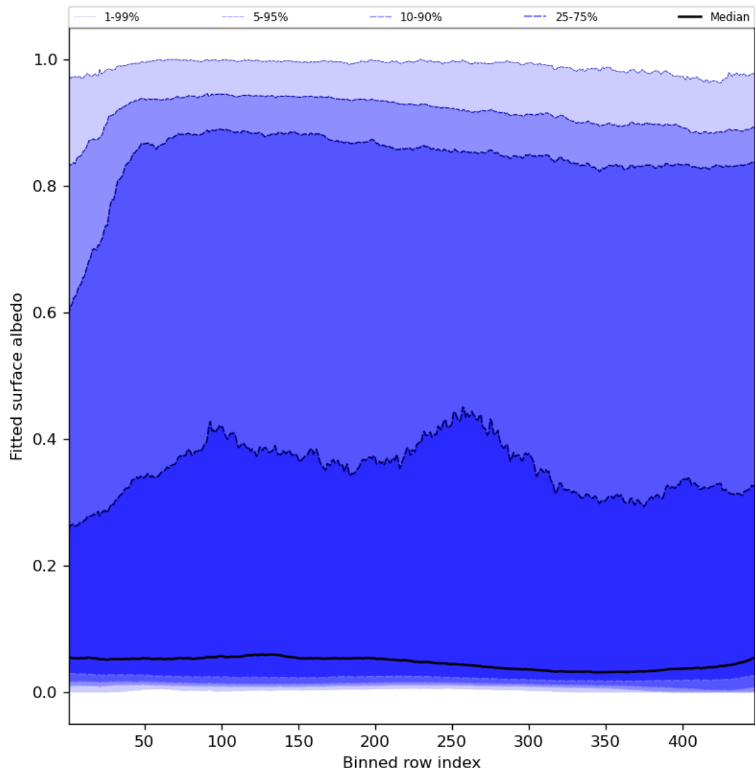
Figure 61: Along track statistics of “Fitted surface albedo” for 2024-05-16 to 2024-05-18
