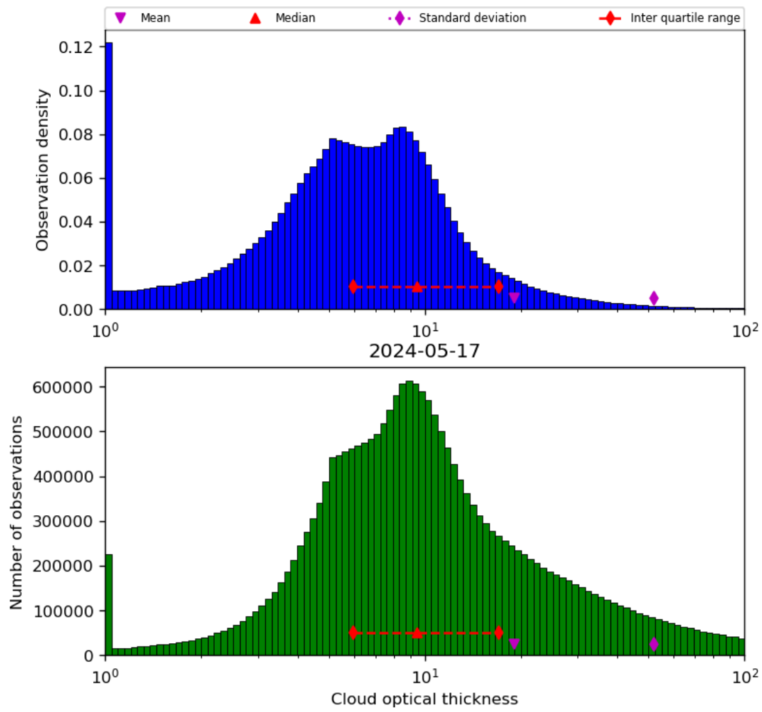
Figure 41: Histogram of “Cloud optical thickness” for 2024-05-16 to 2024-05-18
