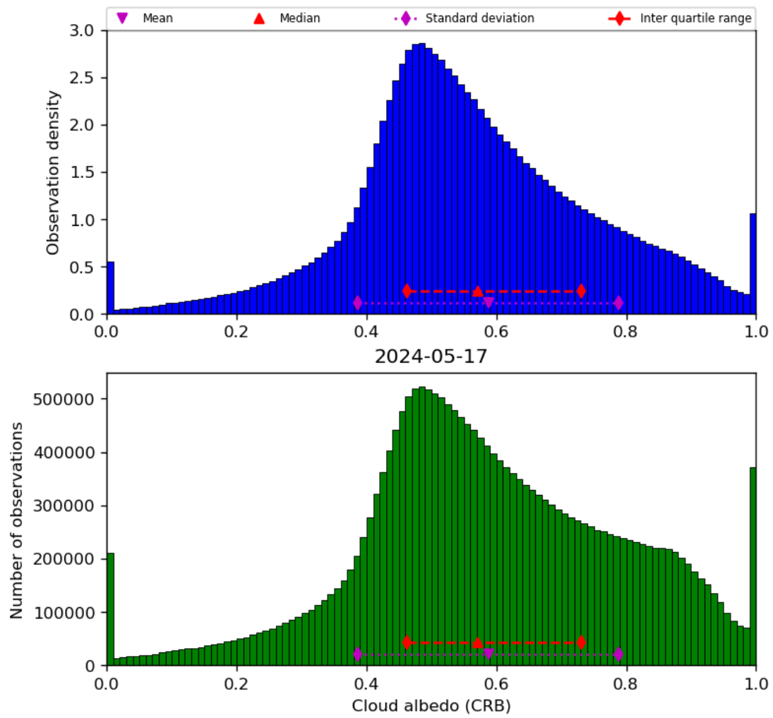
Figure 44: Histogram of “Cloud albedo (CRB)” for 2024-05-16 to 2024-05-18
