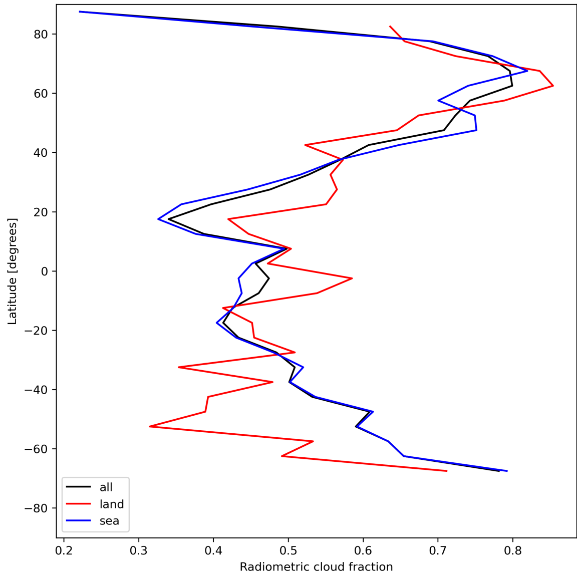
Figure 23: Zonal average of “Radiometric cloud fraction” for 2024-05-16 to 2024-05-18.
