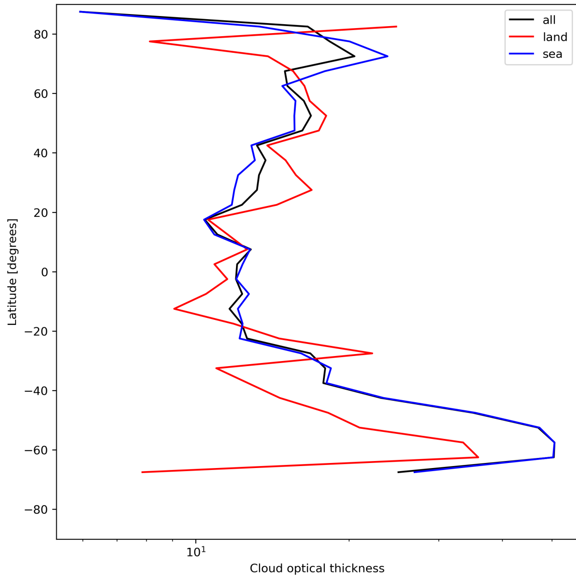
Figure 25: Zonal average of “Cloud optical thickness” for 2024-05-16 to 2024-05-18.
