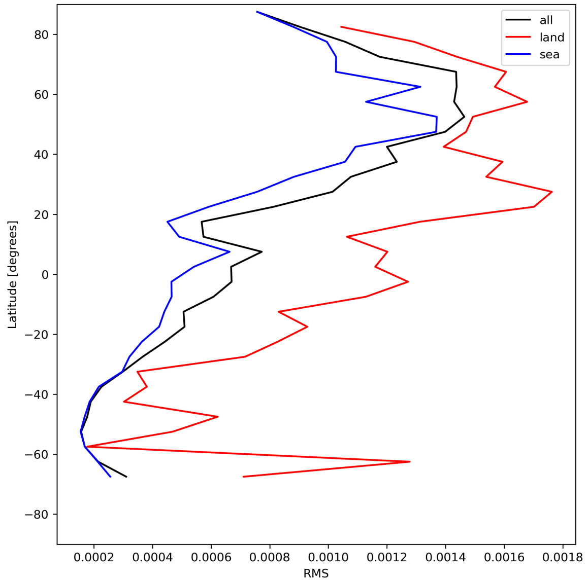
Figure 31: Zonal average of “RMS” for 2024-05-16 to 2024-05-18.
