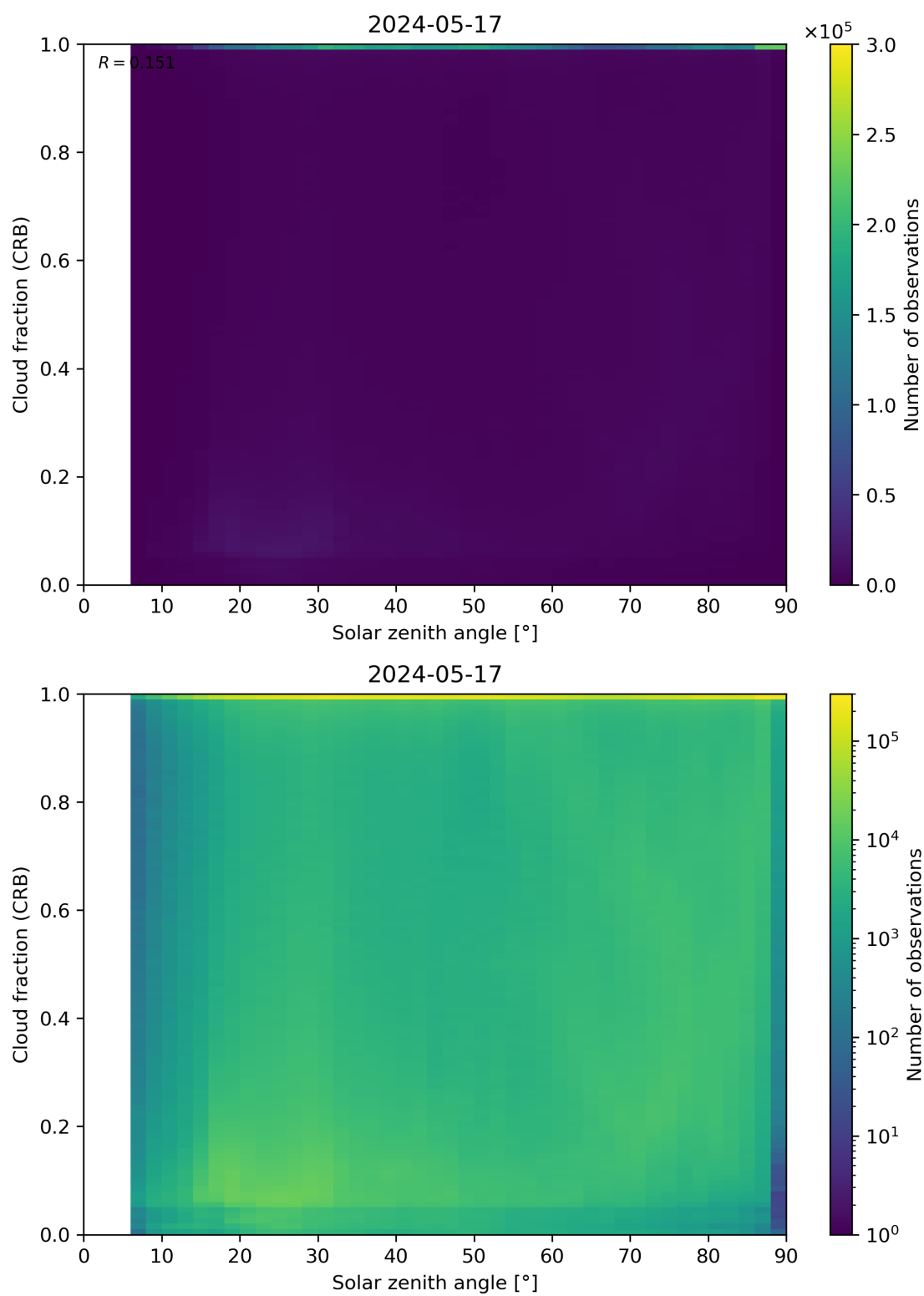
Figure 101: Scatter density plot of “Solar zenith angle” against “Cloud fraction (CRB)” for 2024-05-16 to 2024-05-18.
