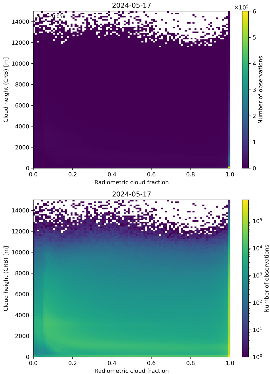
Figure 74: Scatter density plot of “Radiometric cloud fraction” against “Cloud height (CRB)” for 2024-05-16 to 2024-05-18.
