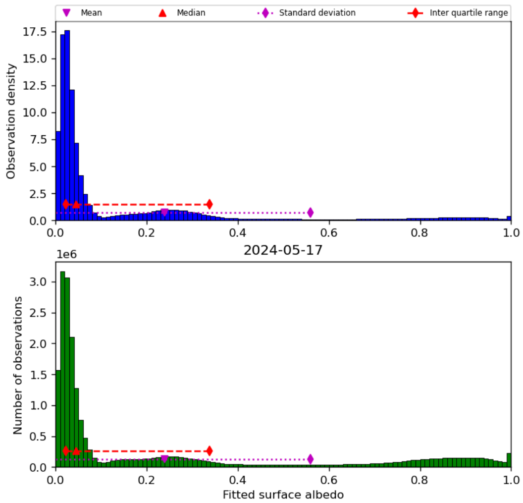
Figure 45: Histogram of “Fitted surface albedo” for 2024-05-16 to 2024-05-18
