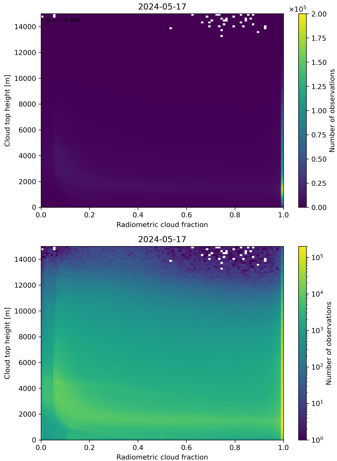
Figure 76: Scatter density plot of “Radiometric cloud fraction” against “Cloud top height” for 2024-05-16 to 2024-05-18.
