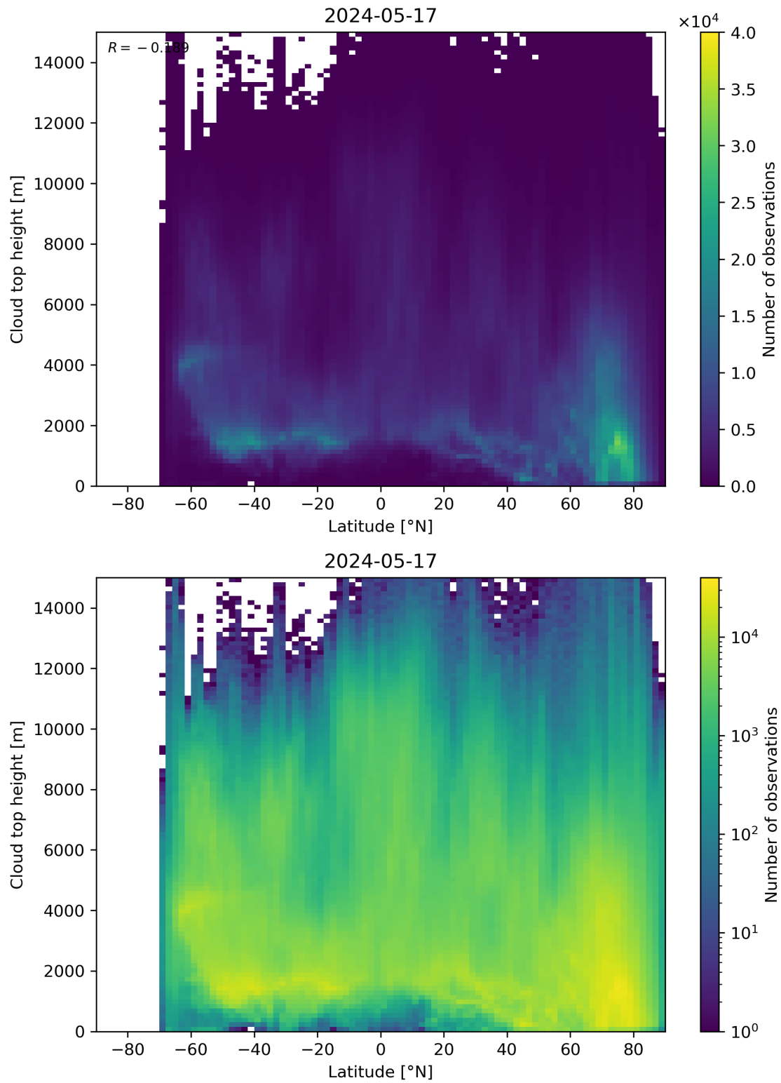
Figure 97: Scatter density plot of “Latitude” against “Cloud top height” for 2024-05-16 to 2024-05-18.
