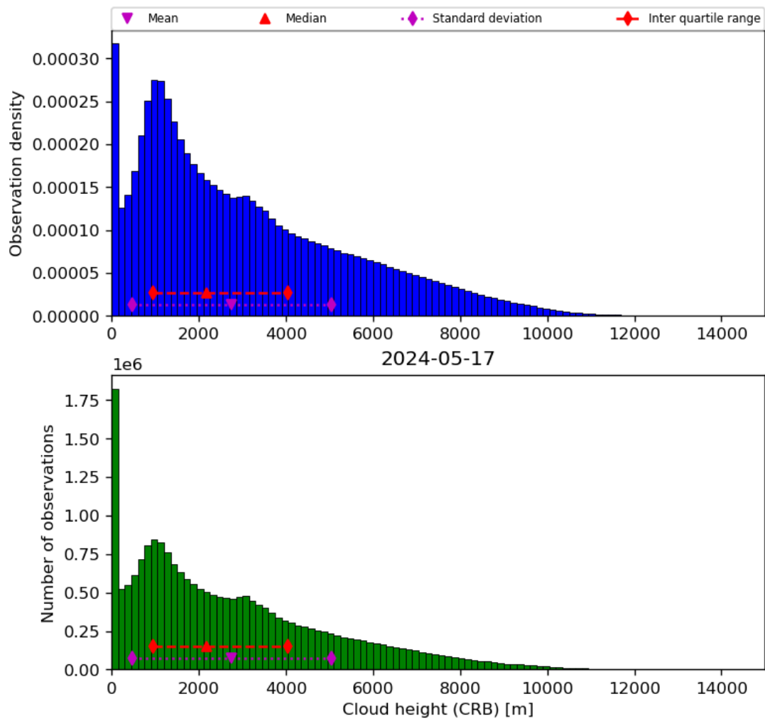
Figure 43: Histogram of “Cloud height (CRB)” for 2024-05-16 to 2024-05-18
