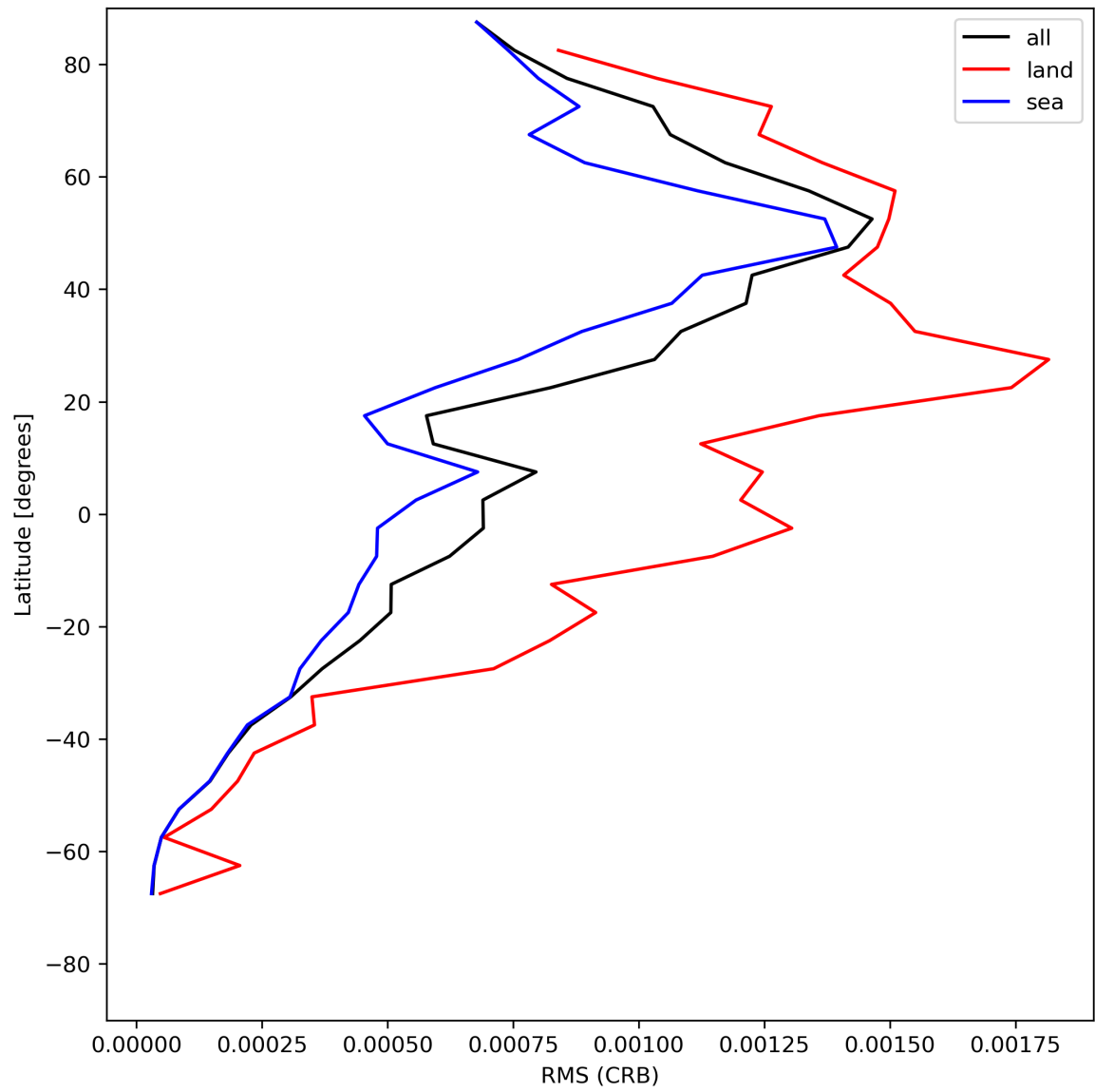
Figure 32: Zonal average of “RMS (CRB)” for 2024-05-16 to 2024-05-18.
