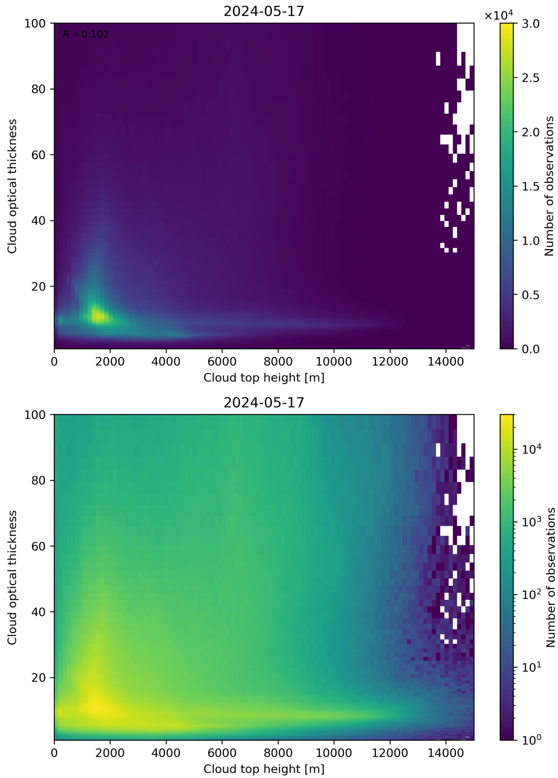
Figure 90: Scatter density plot of “Cloud top height” against “Cloud optical thickness” for 2024-05-16 to 2024-05-18.
