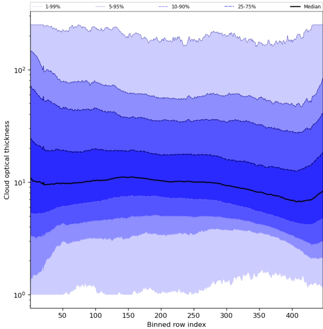
Figure 57: Along track statistics of “Cloud optical thickness” for 2024-05-16 to 2024-05-18
