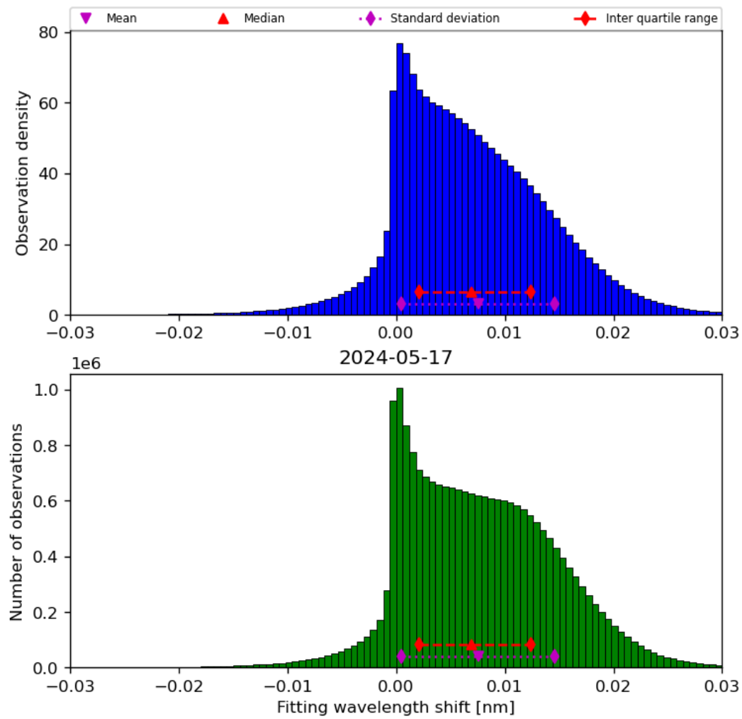
Figure 49: Histogram of “Fitting wavelength shift” for 2024-05-16 to 2024-05-18
