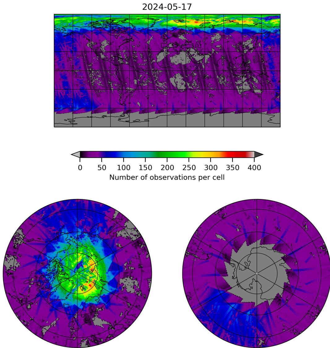
Figure 21: Map of the number of observations for 2024-05-16 to 2024-05-18
