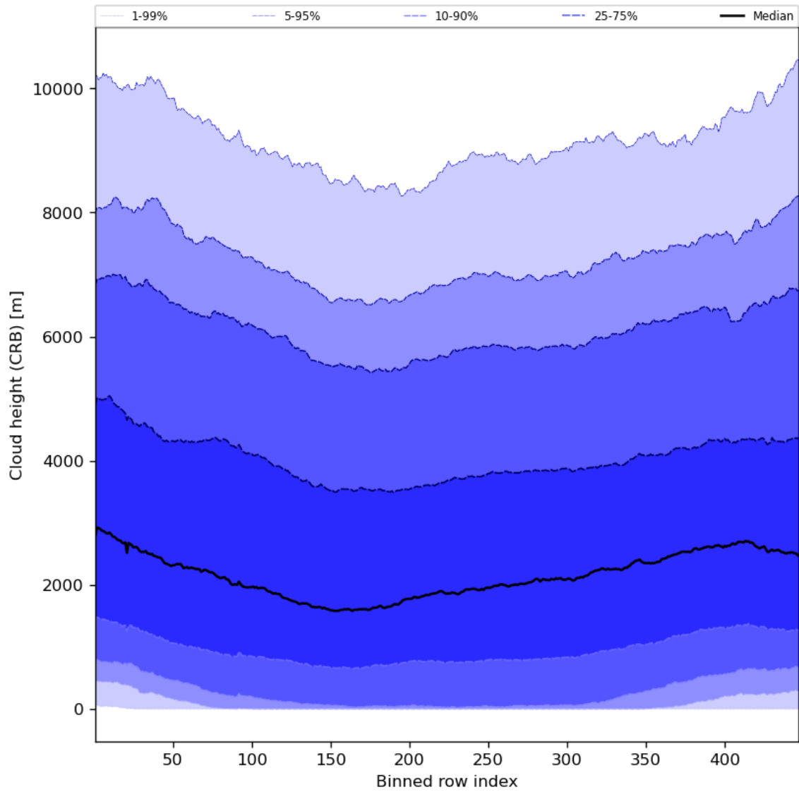
Figure 59: Along track statistics of “Cloud height (CRB)” for 2024-05-16 to 2024-05-18
