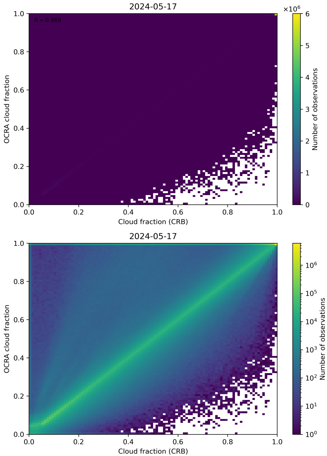
Figure 78: Scatter density plot of “Cloud fraction (CRB)” against “OCRA cloud fraction” for 2024-05-16 to 2024-05-18.
