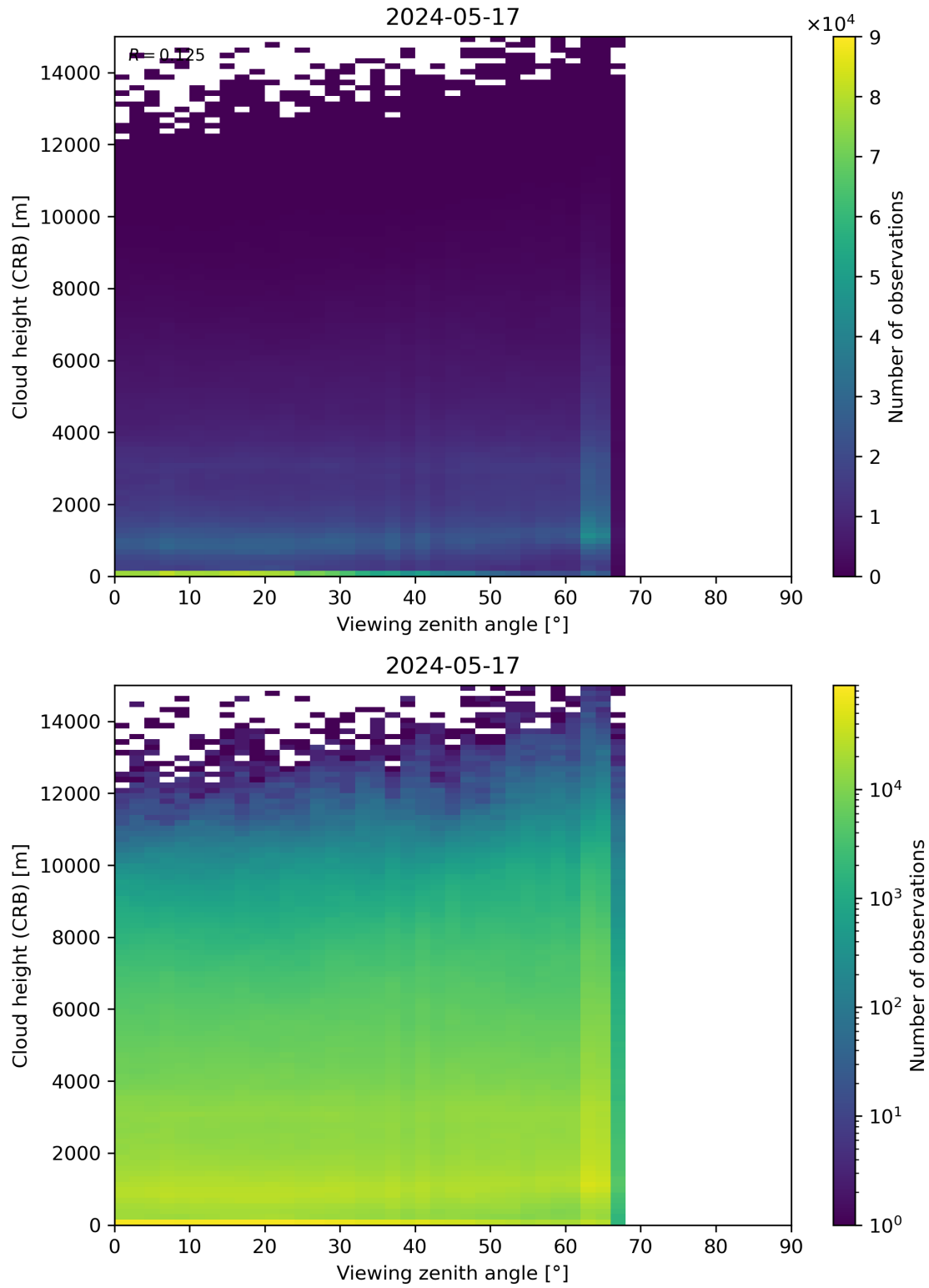
Figure 110: Scatter density plot of “Viewing zenith angle” against “Cloud height (CRB)” for 2024-05-16 to 2024-05-18.
