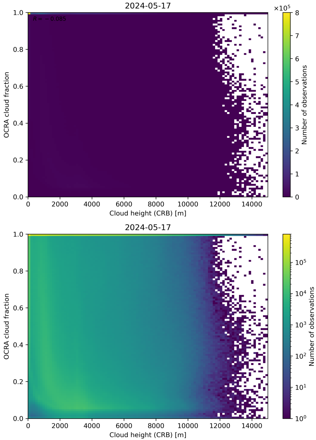
Figure 81: Scatter density plot of “Cloud height (CRB)” against “OCRA cloud fraction” for 2024-05-16 to 2024-05-18.
