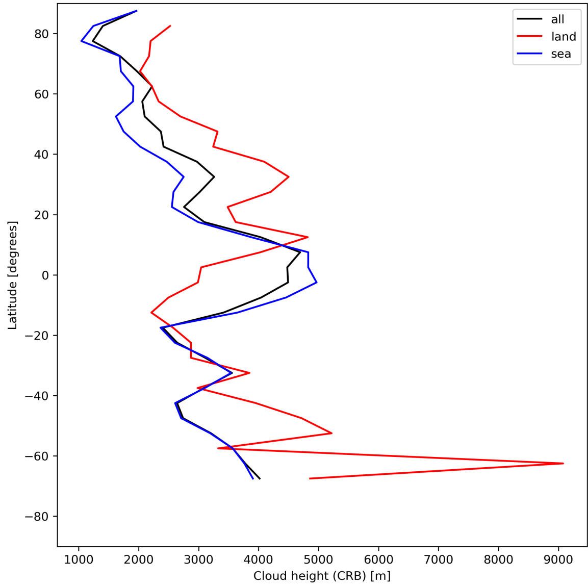
Figure 27: Zonal average of “Cloud height (CRB)” for 2024-05-16 to 2024-05-18.
