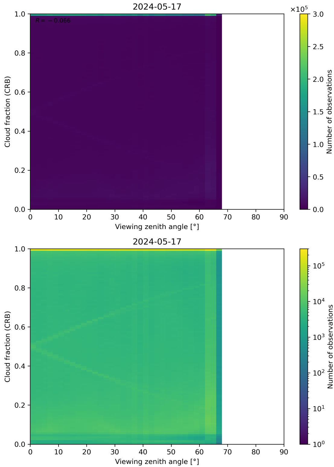
Figure 109: Scatter density plot of “Viewing zenith angle” against “Cloud fraction (CRB)” for 2024-05-16 to 2024-05-18.
