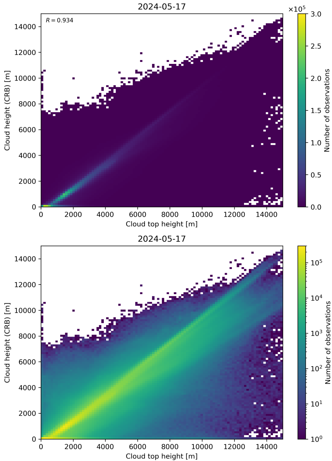
Figure 89: Scatter density plot of “Cloud top height” against “Cloud height (CRB)” for 2024-05-16 to 2024-05-18.
