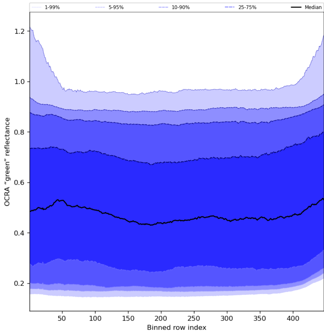
Figure 68: Along track statistics of “OCRA “green” reflectance” for 2024-05-16 to 2024-05-18
