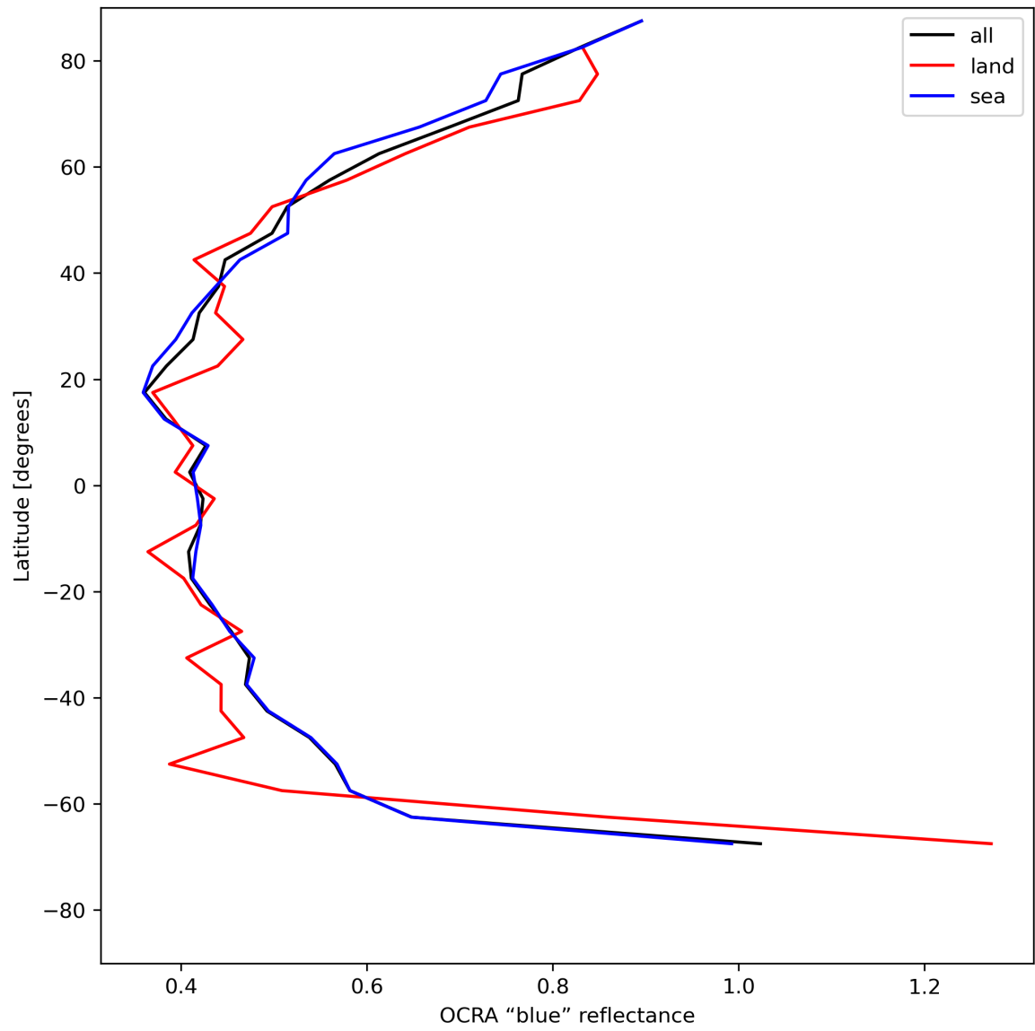
Figure 35: Zonal average of “OCRA “blue” reflectance” for 2024-05-16 to 2024-05-18.
