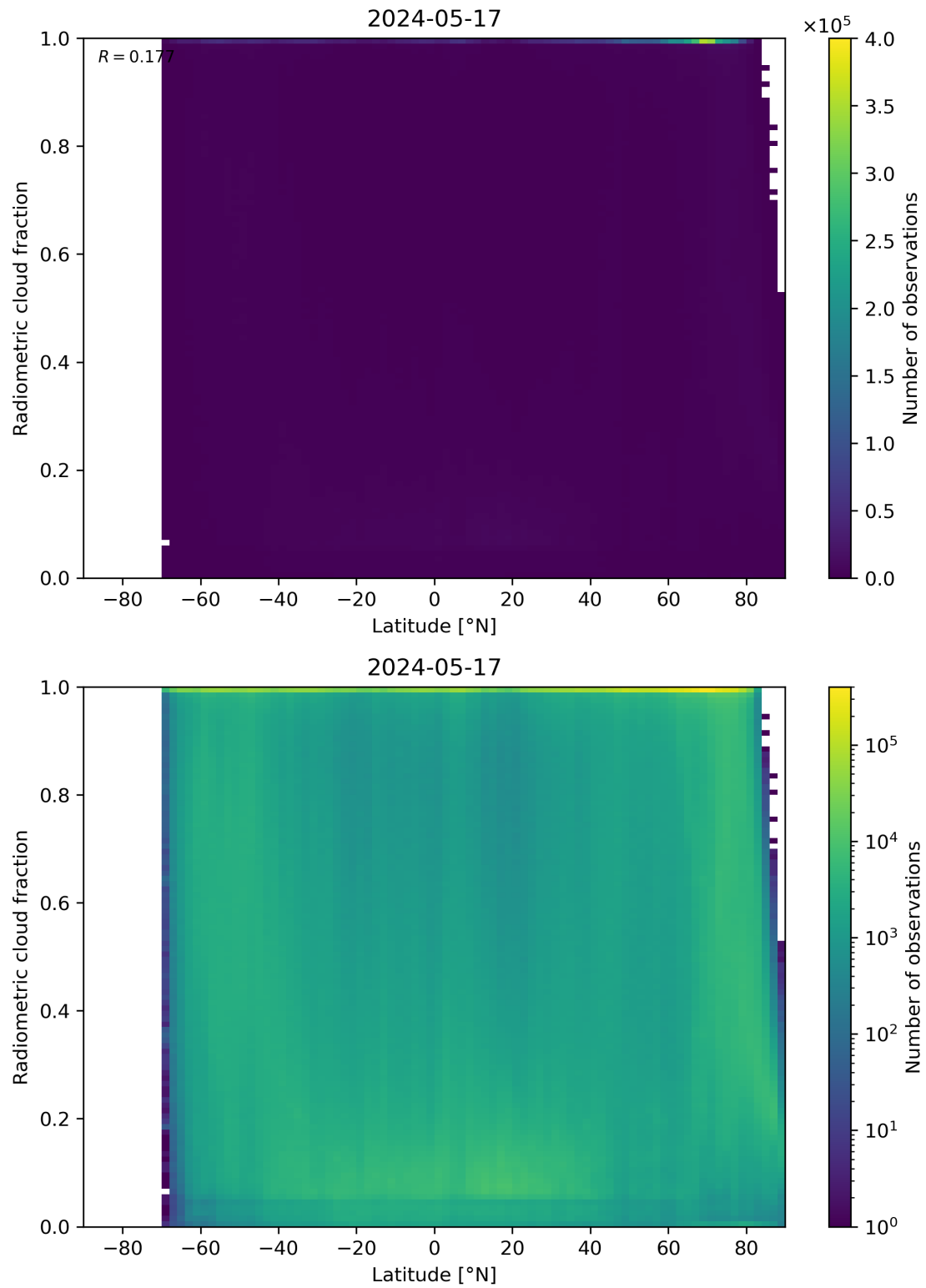
Figure 92: Scatter density plot of “Latitude” against “Radiometric cloud fraction” for 2024-05-16 to 2024-05-18.
