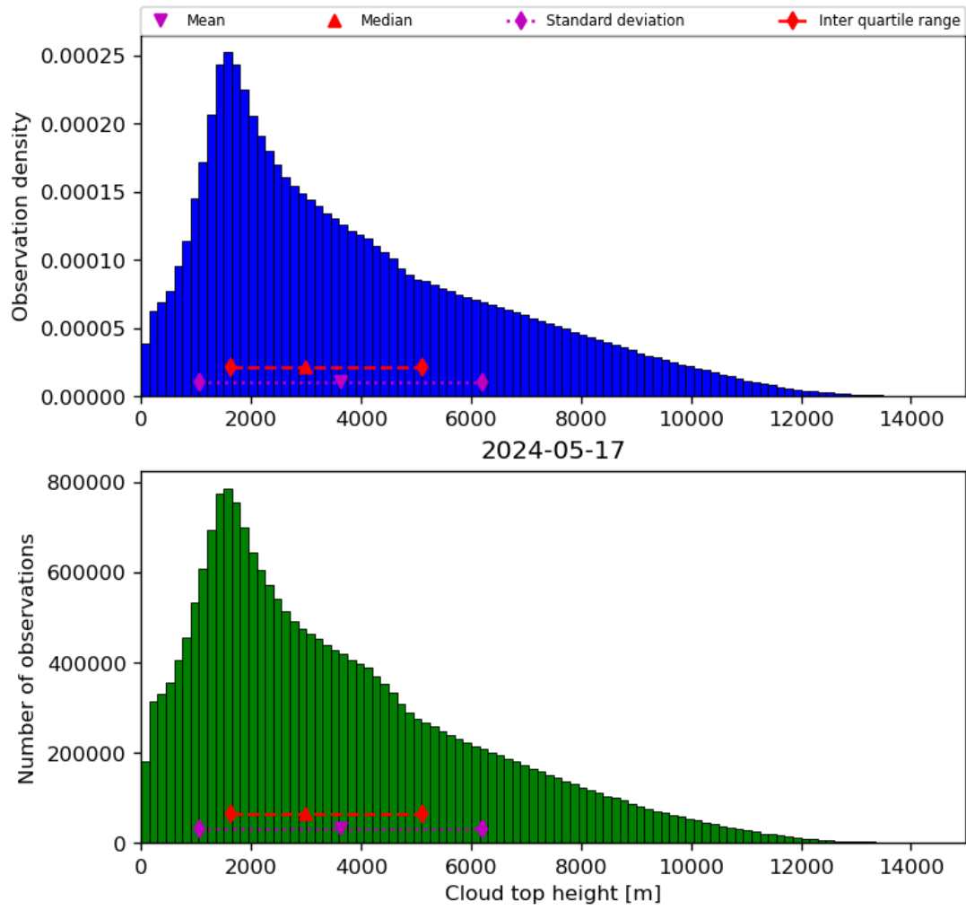
Figure 40: Histogram of “Cloud top height” for 2024-05-16 to 2024-05-18
