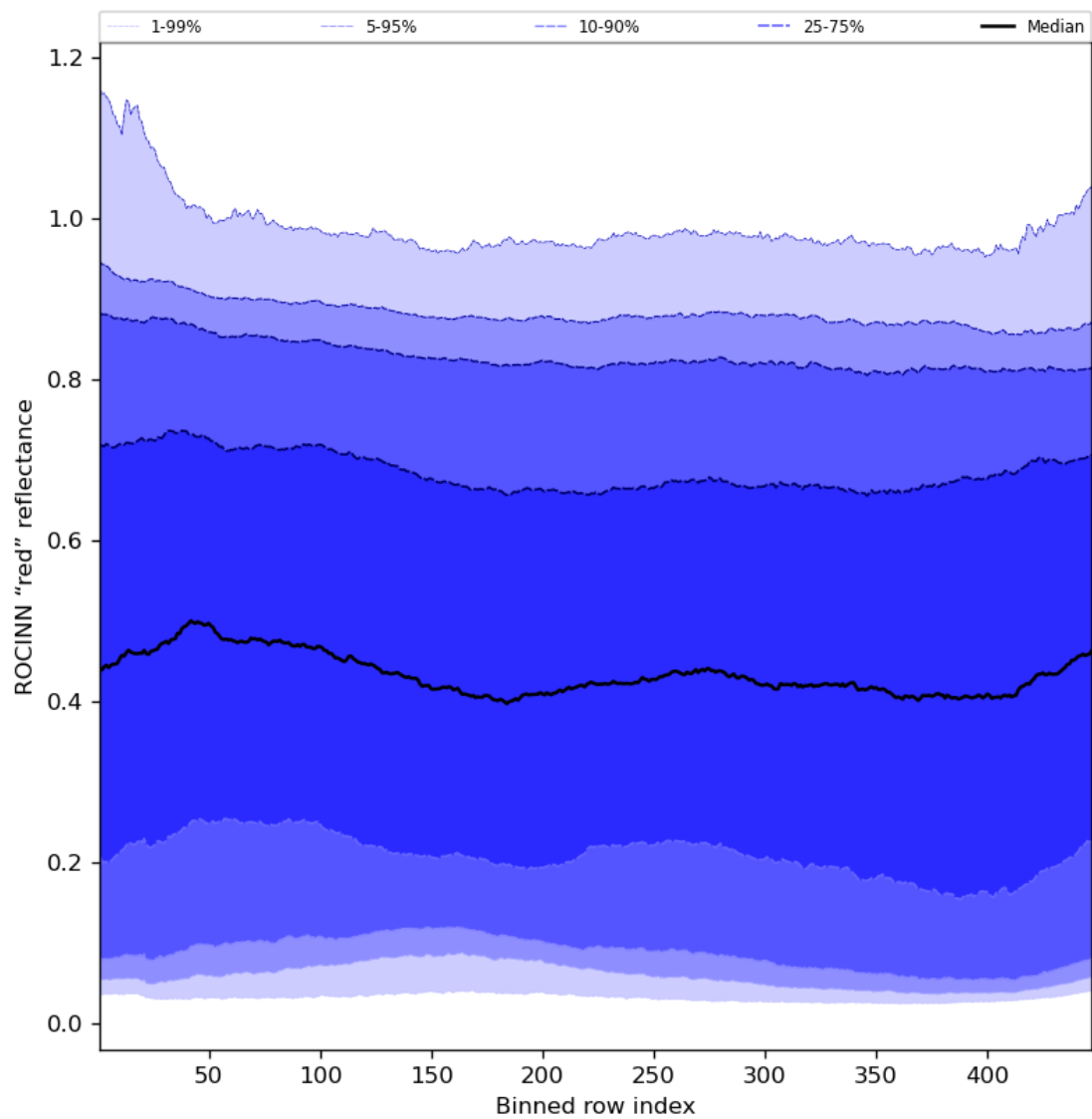
Figure 69: Along track statistics of “ROCINN “red” reflectance” for 2024-05-16 to 2024-05-18
