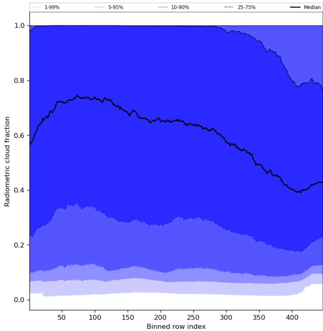
Figure 55: Along track statistics of “Radiometric cloud fraction” for 2024-05-16 to 2024-05-18
