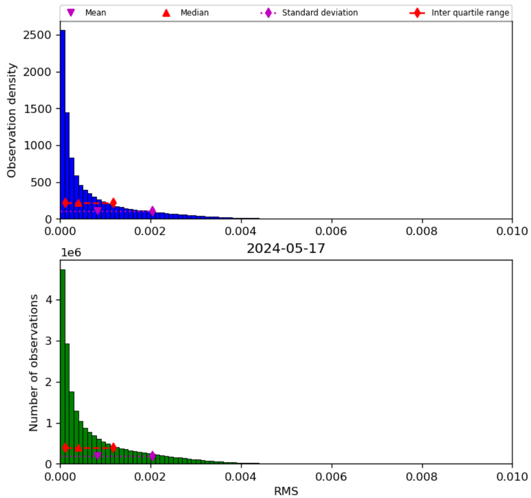
Figure 47: Histogram of “RMS” for 2024-05-16 to 2024-05-18
