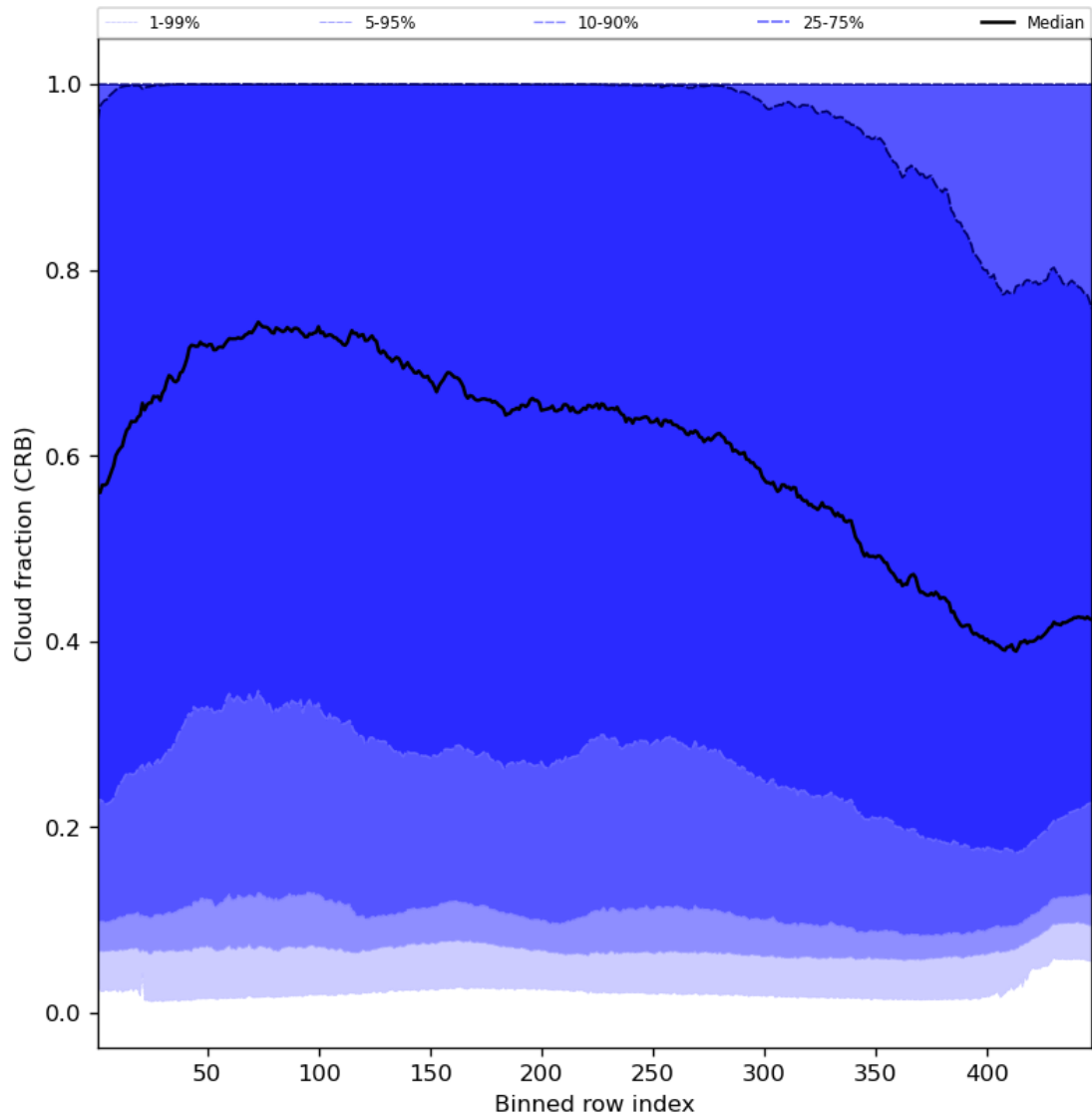
Figure 58: Along track statistics of “Cloud fraction (CRB)” for 2024-05-16 to 2024-05-18
