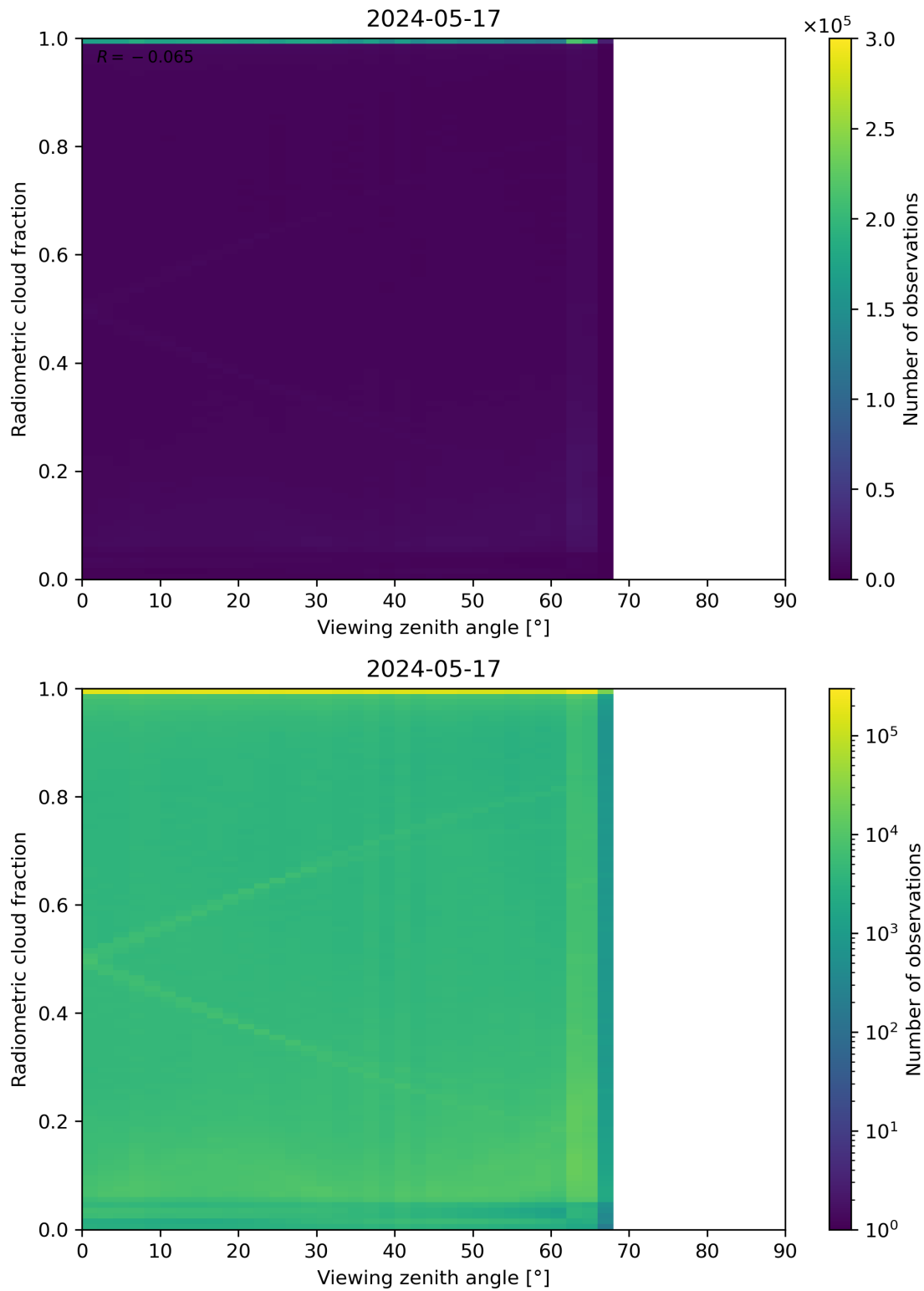
Figure 107: Scatter density plot of “Viewing zenith angle” against “Radiometric cloud fraction” for 2024-05-16 to 2024-05-18.
