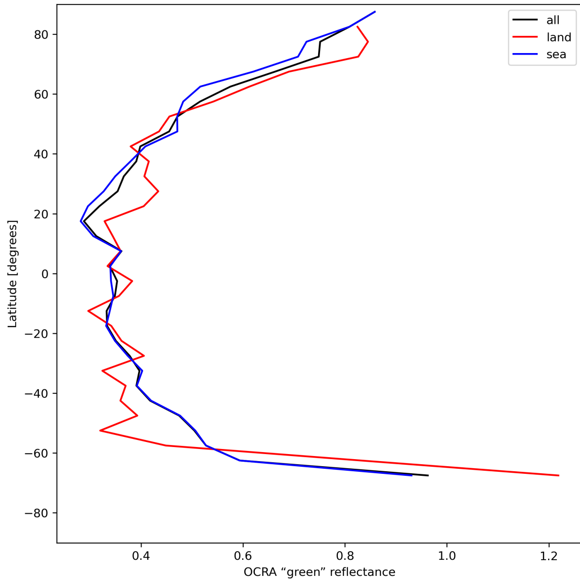
Figure 36: Zonal average of “OCRA “green” reflectance” for 2024-05-16 to 2024-05-18.
