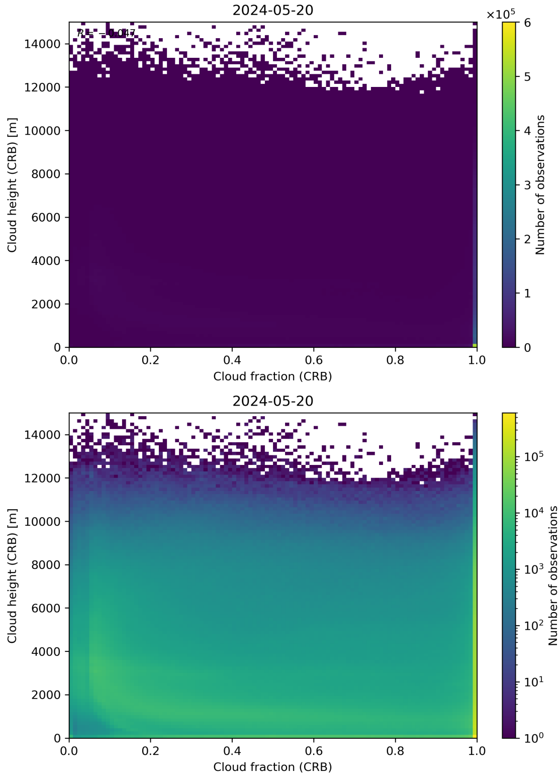
Figure 79: Scatter density plot of “Cloud fraction (CRB)” against “Cloud height (CRB)” for 2024-05-19 to 2024-05-21.
