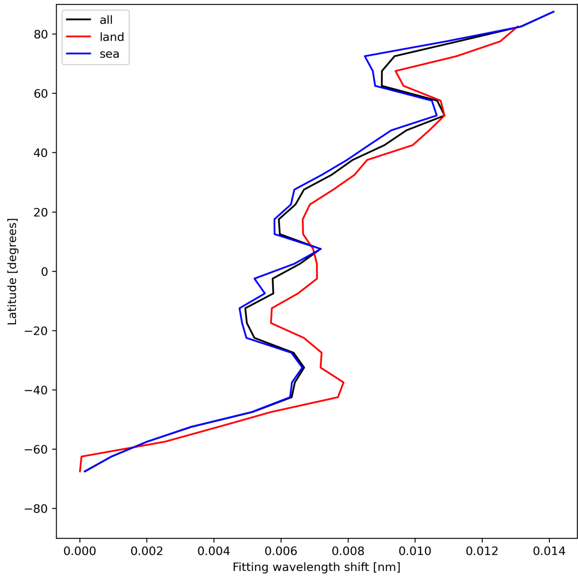
Figure 33: Zonal average of “Fitting wavelength shift” for 2024-05-19 to 2024-05-21.
