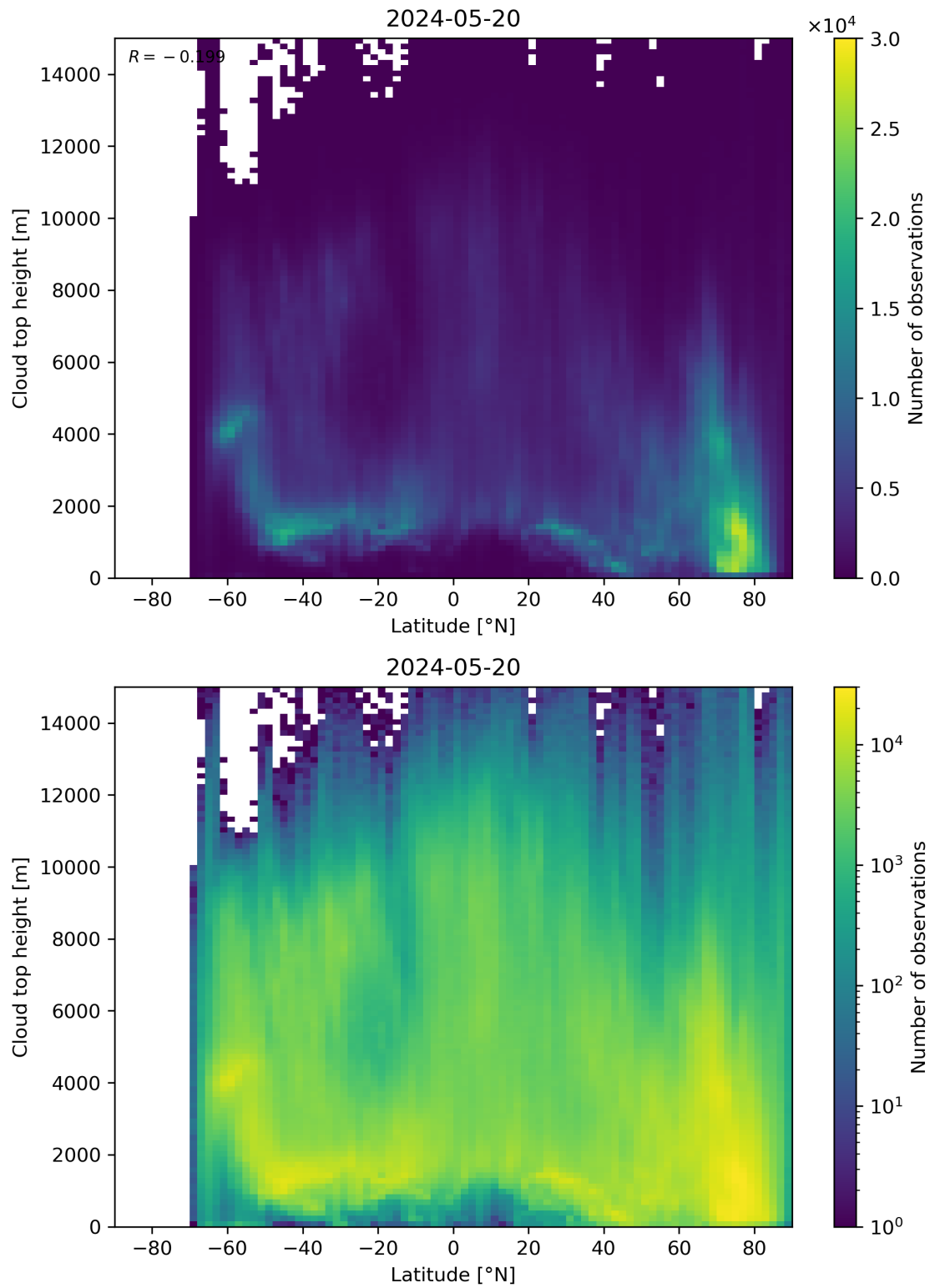
Figure 97: Scatter density plot of “Latitude” against “Cloud top height” for 2024-05-19 to 2024-05-21.
