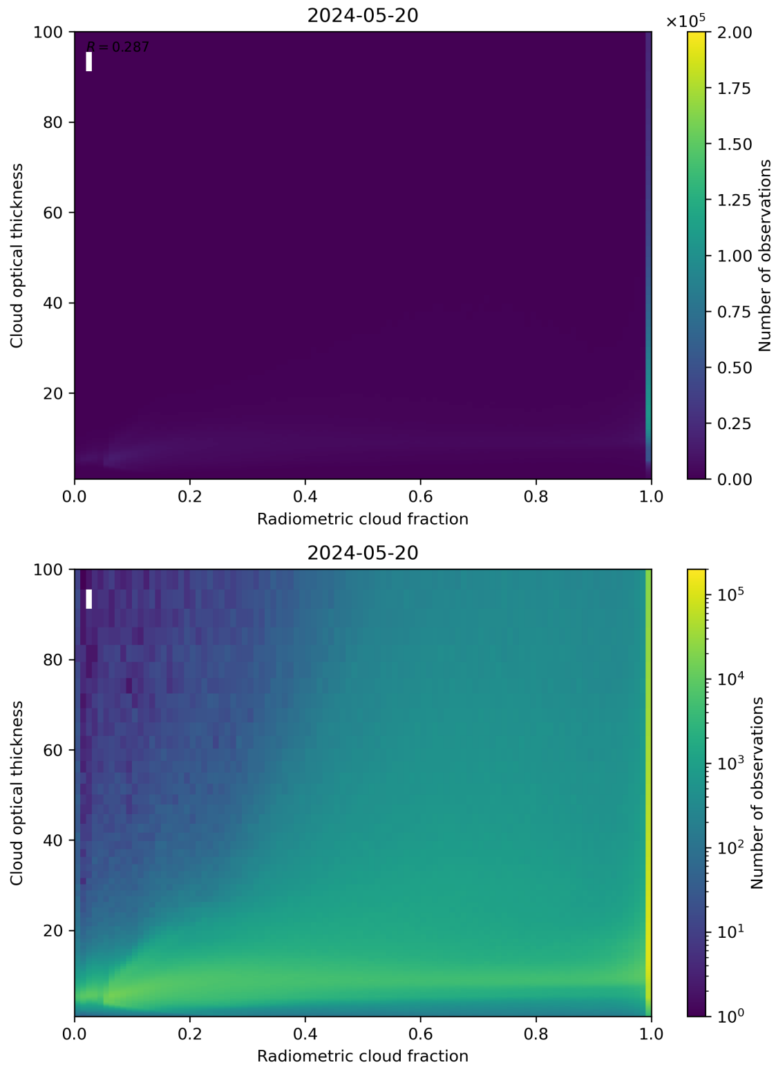
Figure 75: Scatter density plot of “Radiometric cloud fraction” against “Cloud optical thickness” for 2024-05-19 to 2024-05-21.
