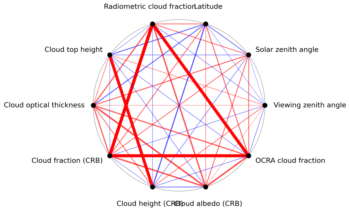
Figure 1: Map of correlation graph for 2024-05-19 to 2024-05-21.
