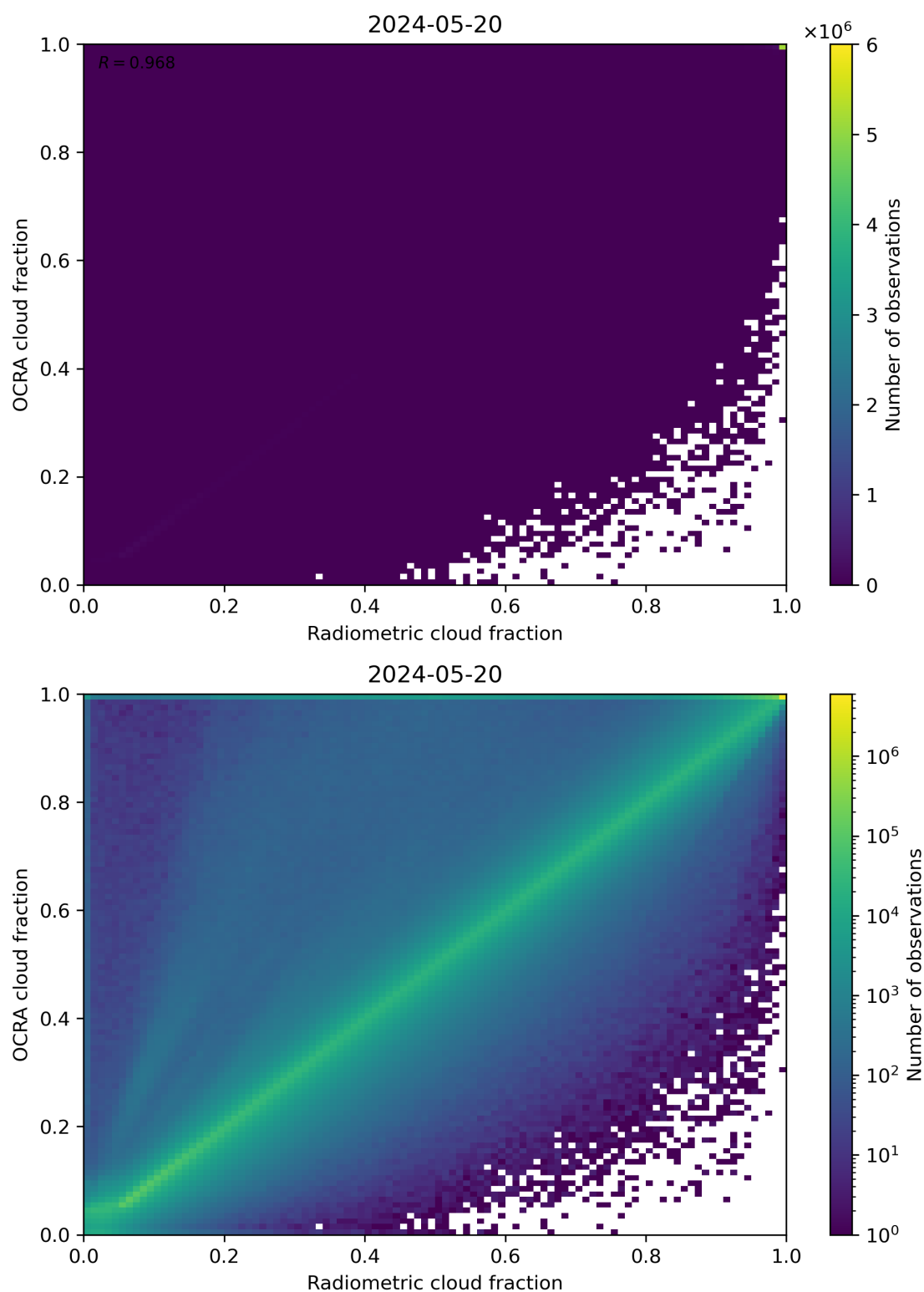
Figure 72: Scatter density plot of “Radiometric cloud fraction” against “OCRA cloud fraction” for 2024-05-19 to 2024-05-21.
