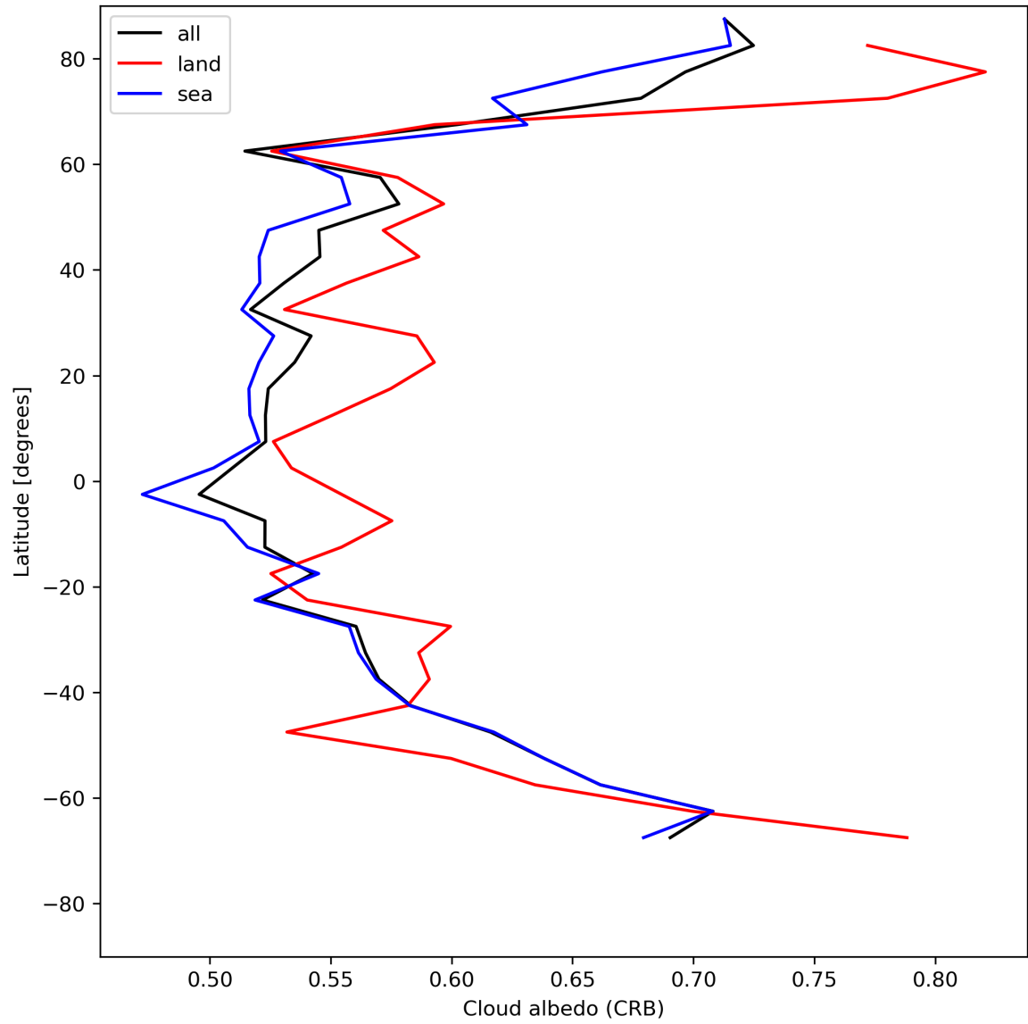
Figure 28: Zonal average of “Cloud albedo (CRB)” for 2024-05-19 to 2024-05-21.
