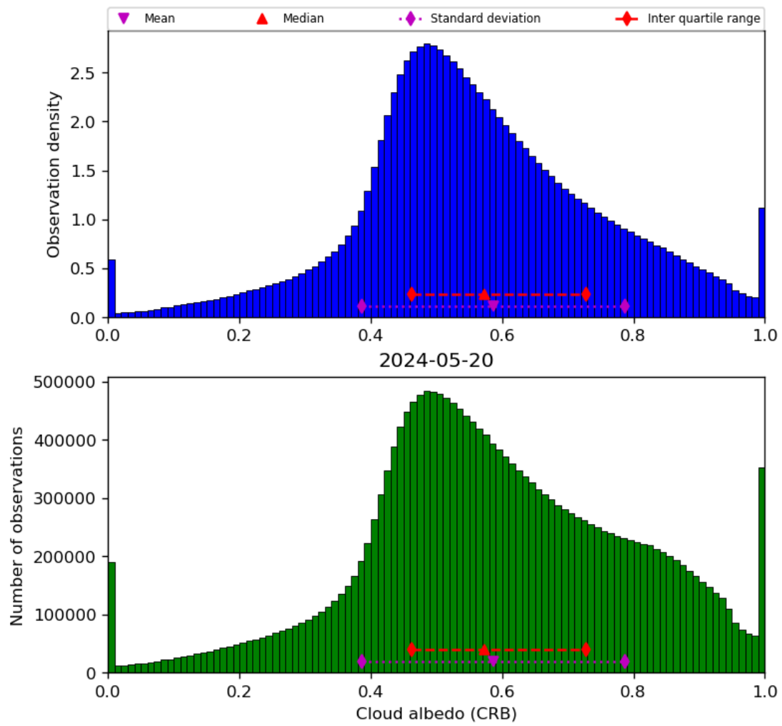
Figure 44: Histogram of “Cloud albedo (CRB)” for 2024-05-19 to 2024-05-21
