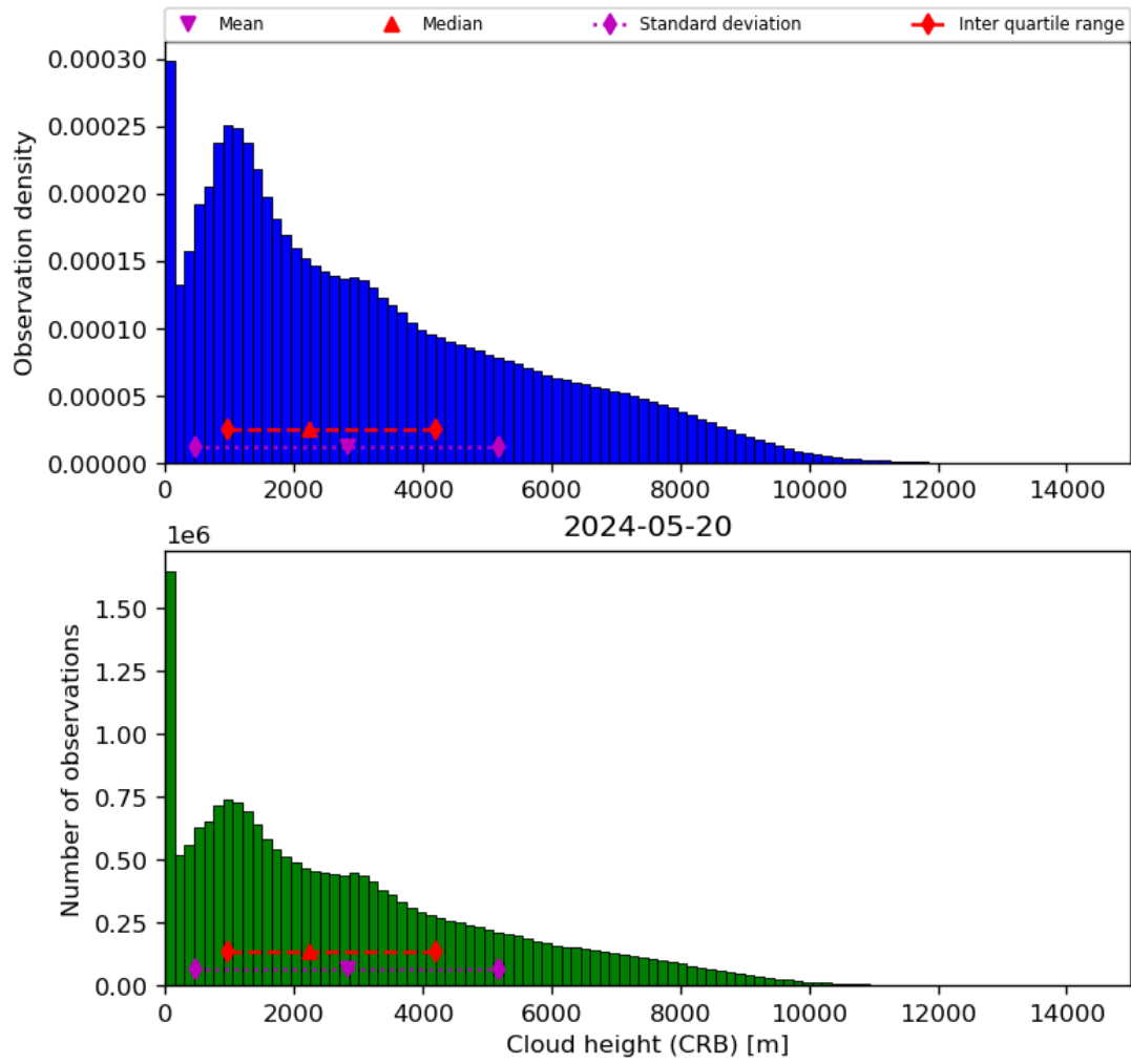
Figure 43: Histogram of “Cloud height (CRB)” for 2024-05-19 to 2024-05-21
