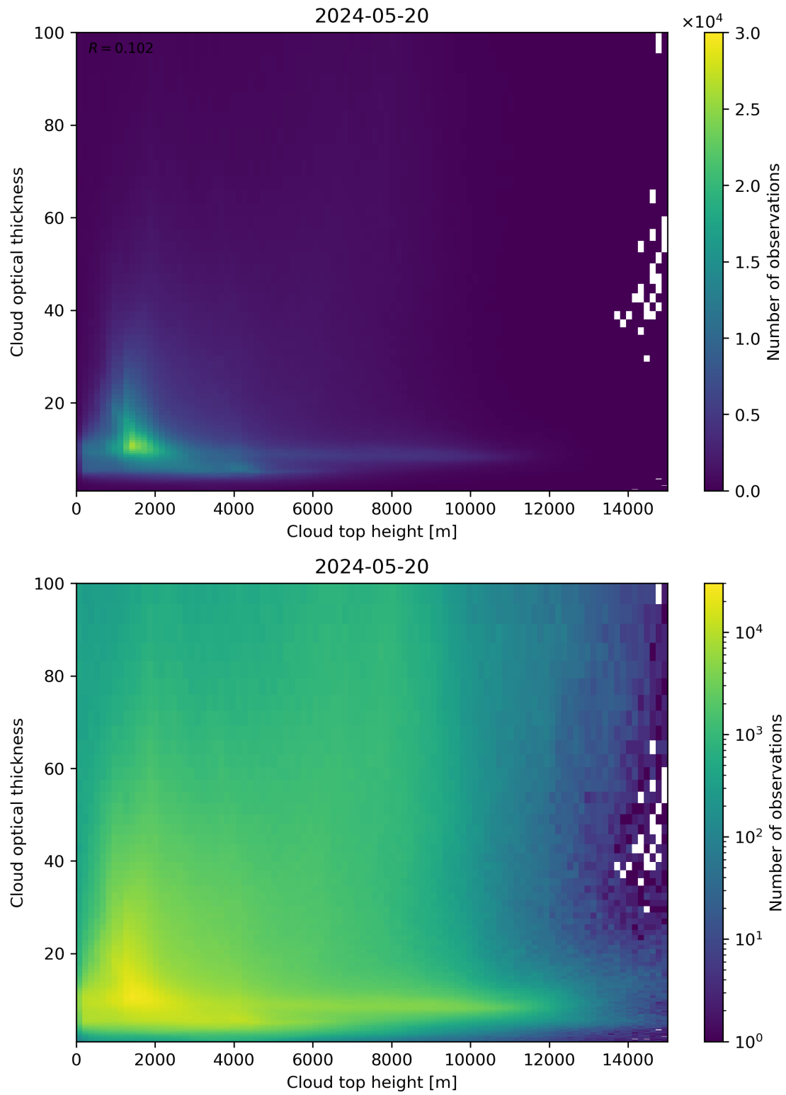
Figure 90: Scatter density plot of “Cloud top height” against “Cloud optical thickness” for 2024-05-19 to 2024-05-21.
