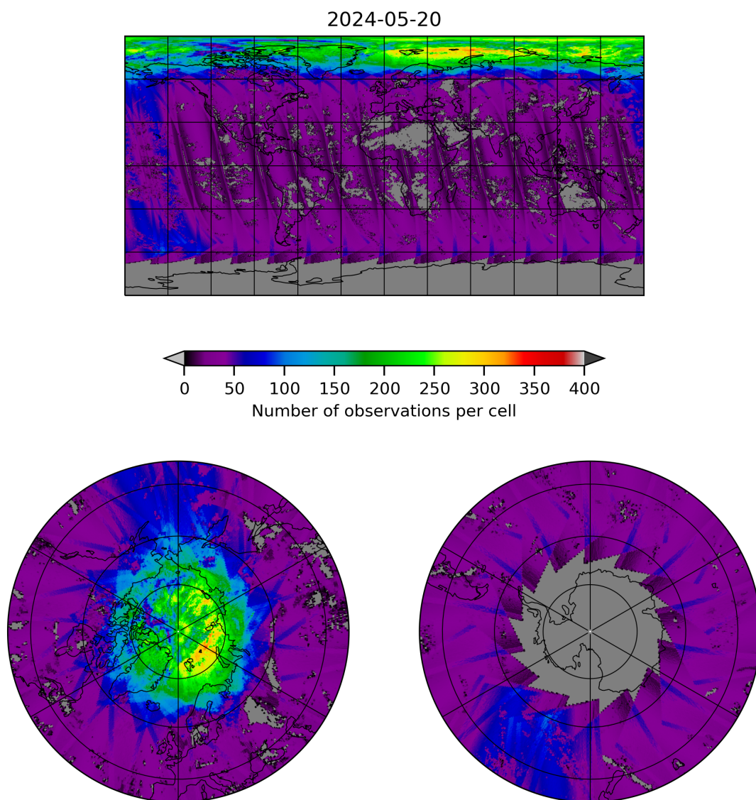
Figure 21: Map of the number of observations for 2024-05-19 to 2024-05-21
