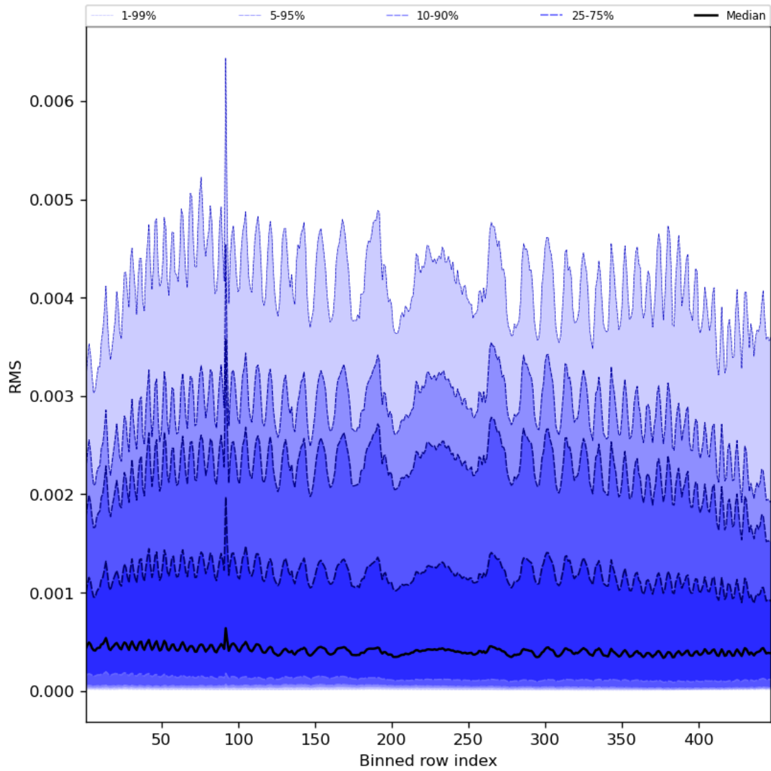
Figure 63: Along track statistics of “RMS” for 2024-05-19 to 2024-05-21
