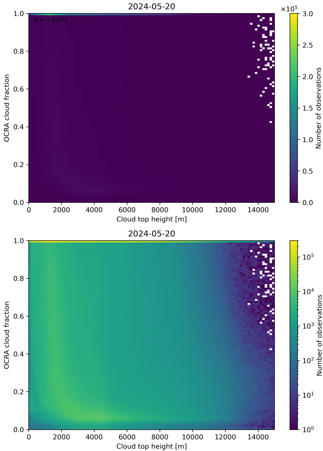
Figure 87: Scatter density plot of “Cloud top height” against “OCRA cloud fraction” for 2024-05-19 to 2024-05-21.
