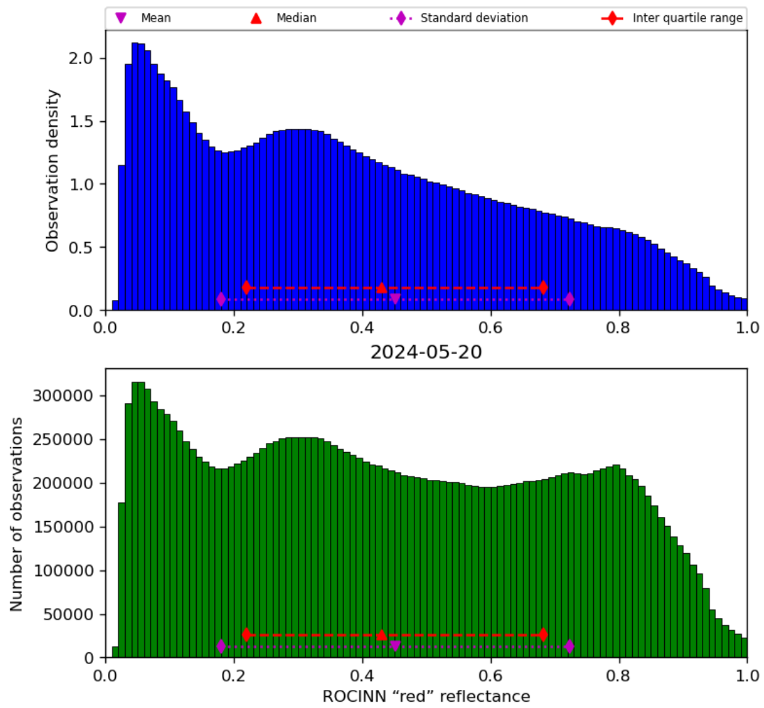
Figure 53: Histogram of “ROCINN “red” reflectance” for 2024-05-19 to 2024-05-21
