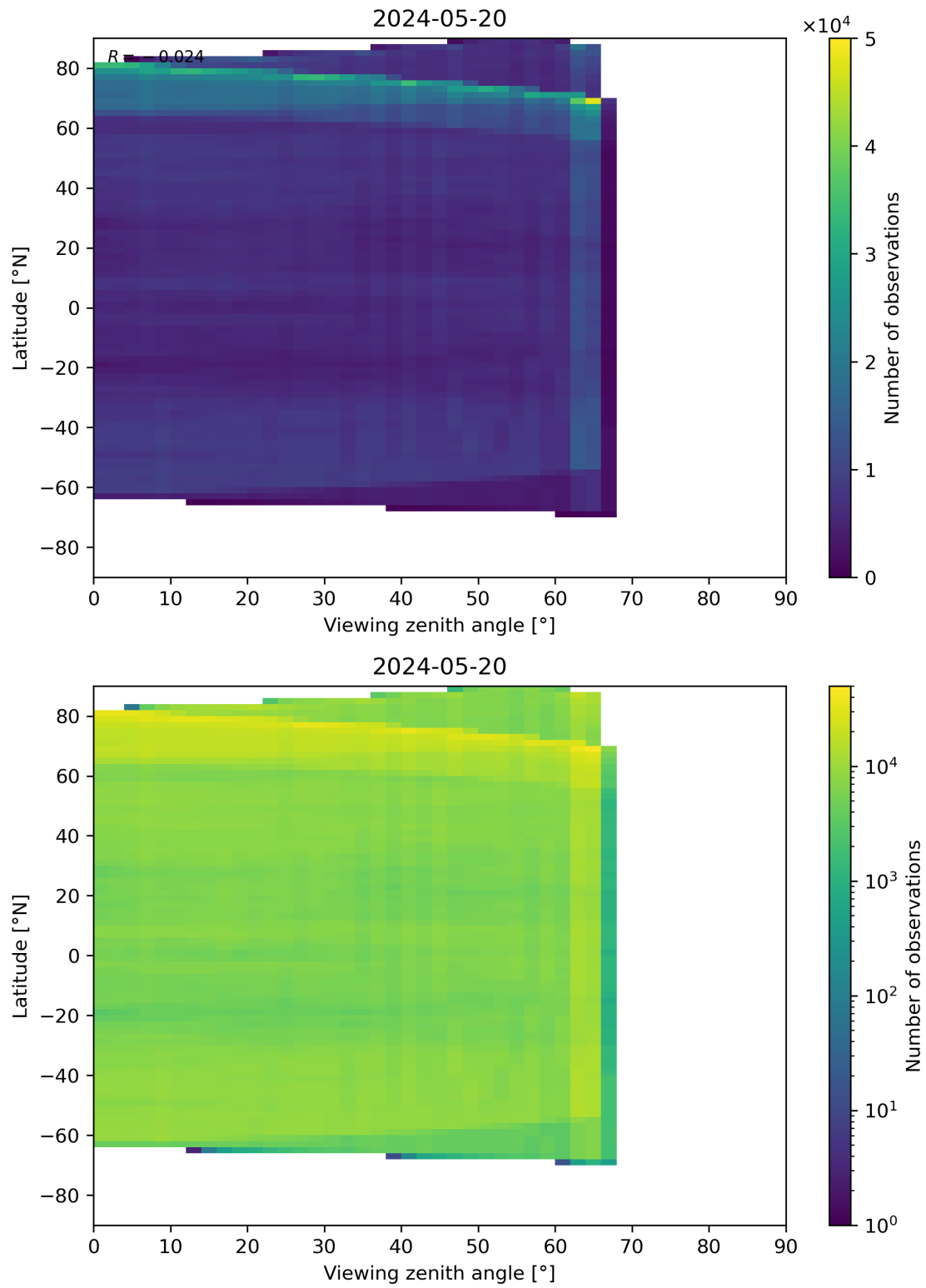
Figure 113: Scatter density plot of “Viewing zenith angle” against “Latitude” for 2024-05-19 to 2024-05-21.
