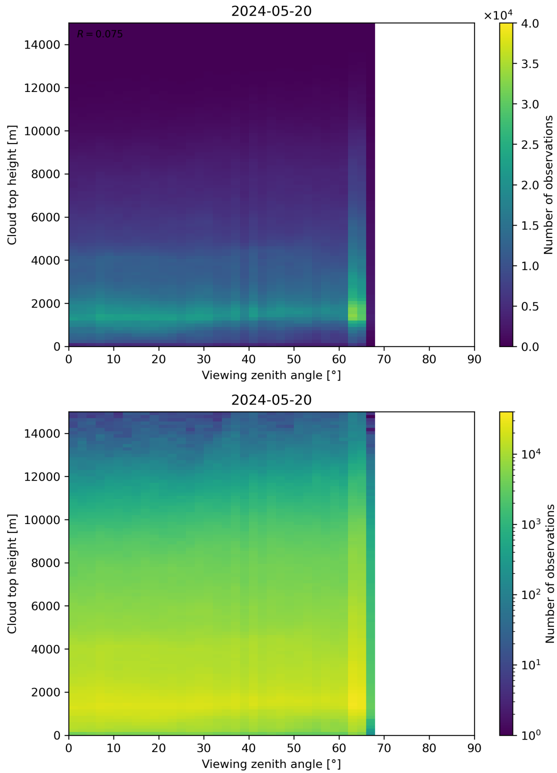
Figure 112: Scatter density plot of “Viewing zenith angle” against “Cloud top height” for 2024-05-19 to 2024-05-21.
