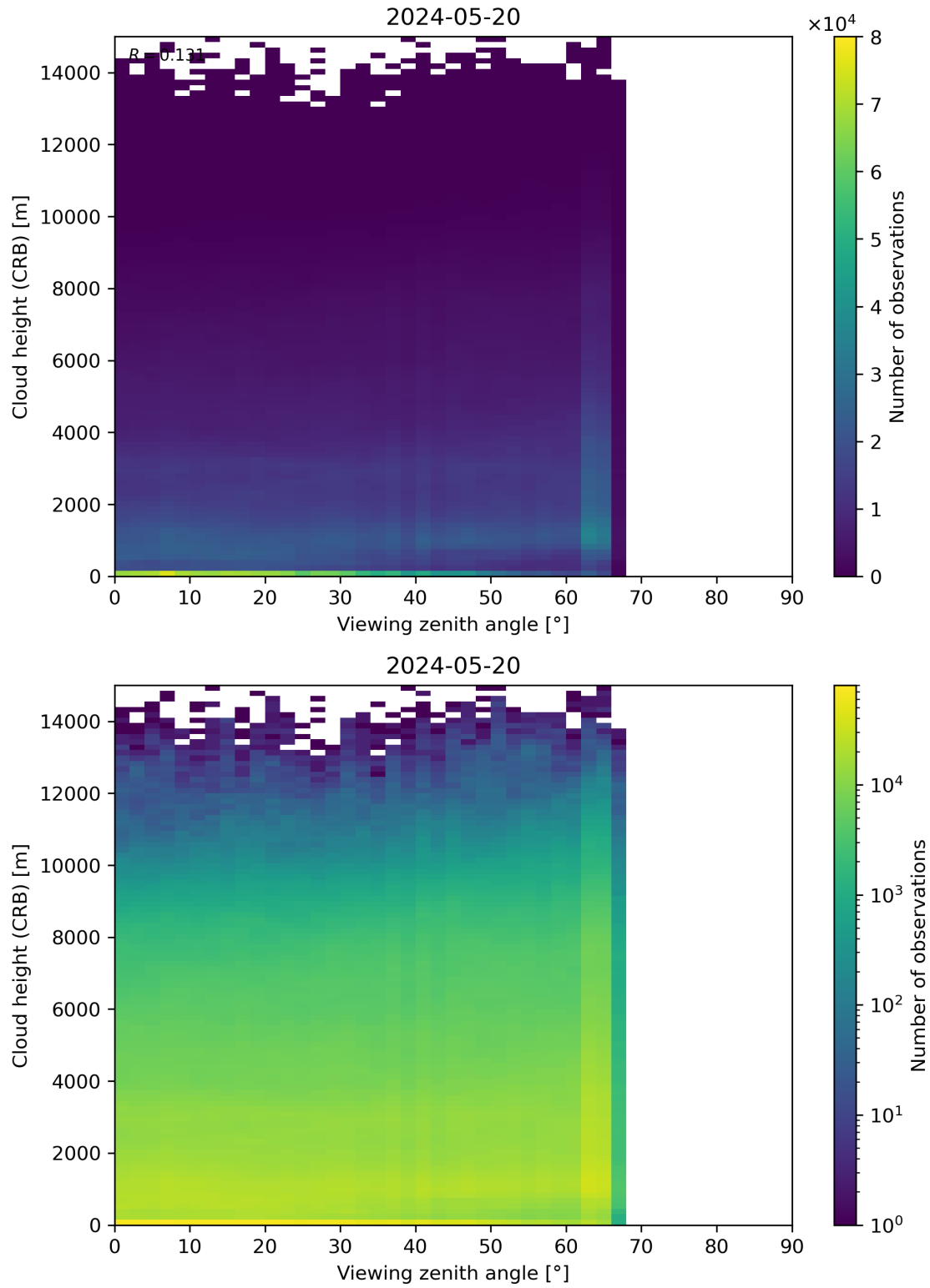
Figure 110: Scatter density plot of “Viewing zenith angle” against “Cloud height (CRB)” for 2024-05-19 to 2024-05-21.
