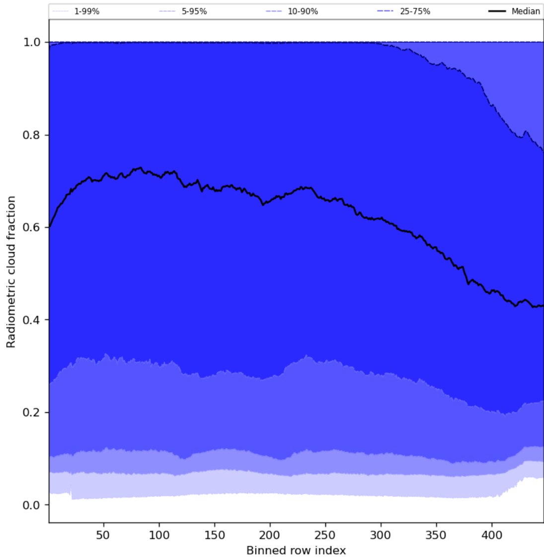
Figure 55: Along track statistics of “Radiometric cloud fraction” for 2024-05-19 to 2024-05-21
