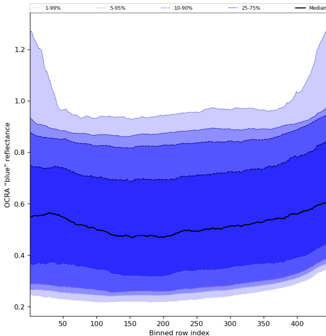
Figure 67: Along track statistics of “OCRA “blue” reflectance” for 2024-05-19 to 2024-05-21
