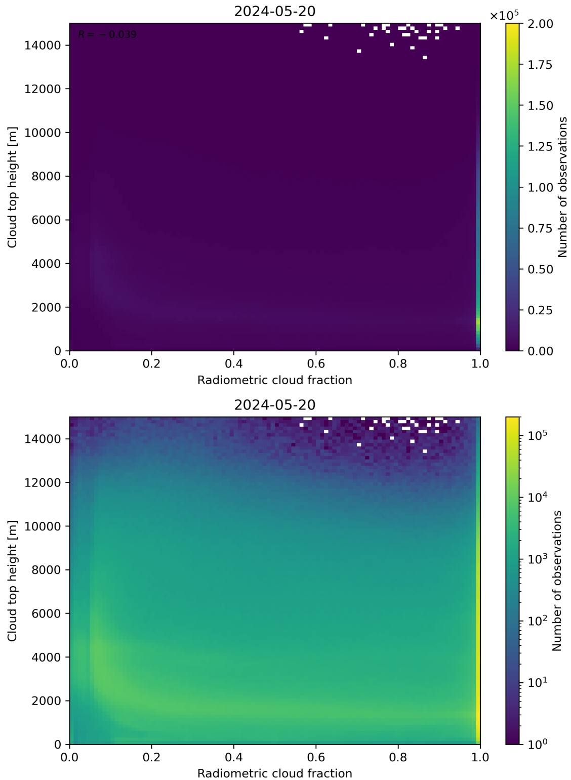
Figure 76: Scatter density plot of “Radiometric cloud fraction” against “Cloud top height” for 2024-05-19 to 2024-05-21.
