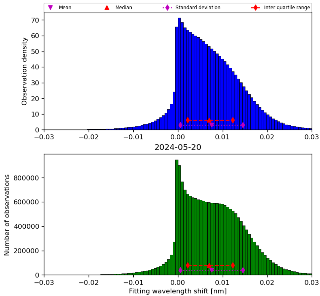
Figure 49: Histogram of “Fitting wavelength shift” for 2024-05-19 to 2024-05-21
