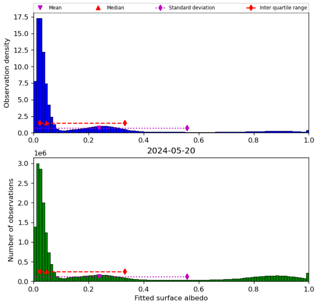
Figure 45: Histogram of “Fitted surface albedo” for 2024-05-19 to 2024-05-21
