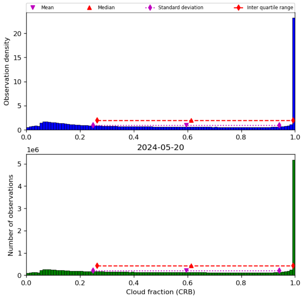
Figure 42: Histogram of “Cloud fraction (CRB)” for 2024-05-19 to 2024-05-21
