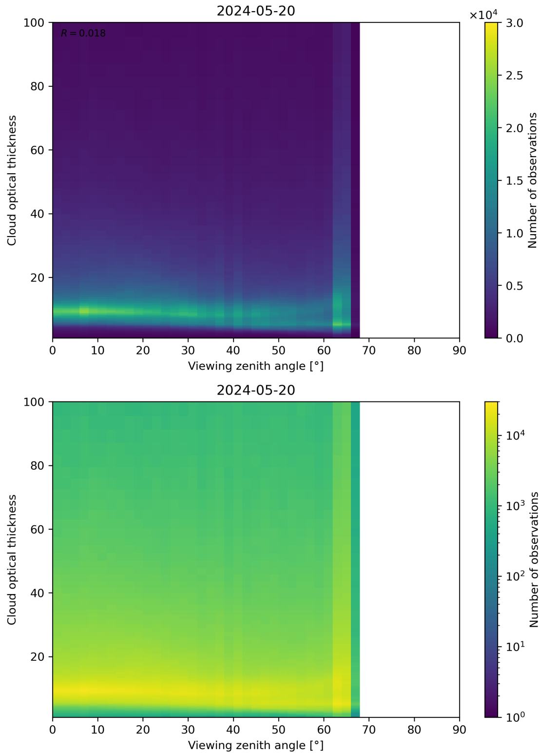
Figure 111: Scatter density plot of “Viewing zenith angle” against “Cloud optical thickness” for 2024-05-19 to 2024-05-21.
