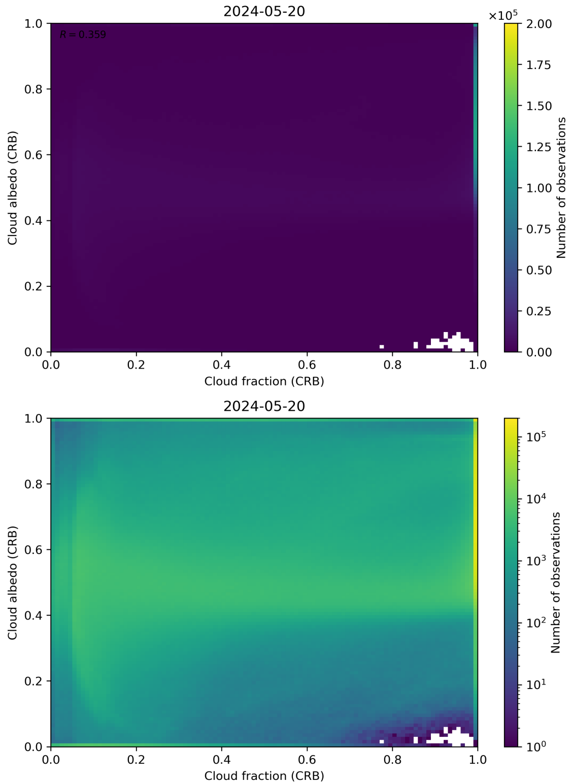
Figure 77: Scatter density plot of “Cloud fraction (CRB)” against “Cloud albedo (CRB)” for 2024-05-19 to 2024-05-21.
