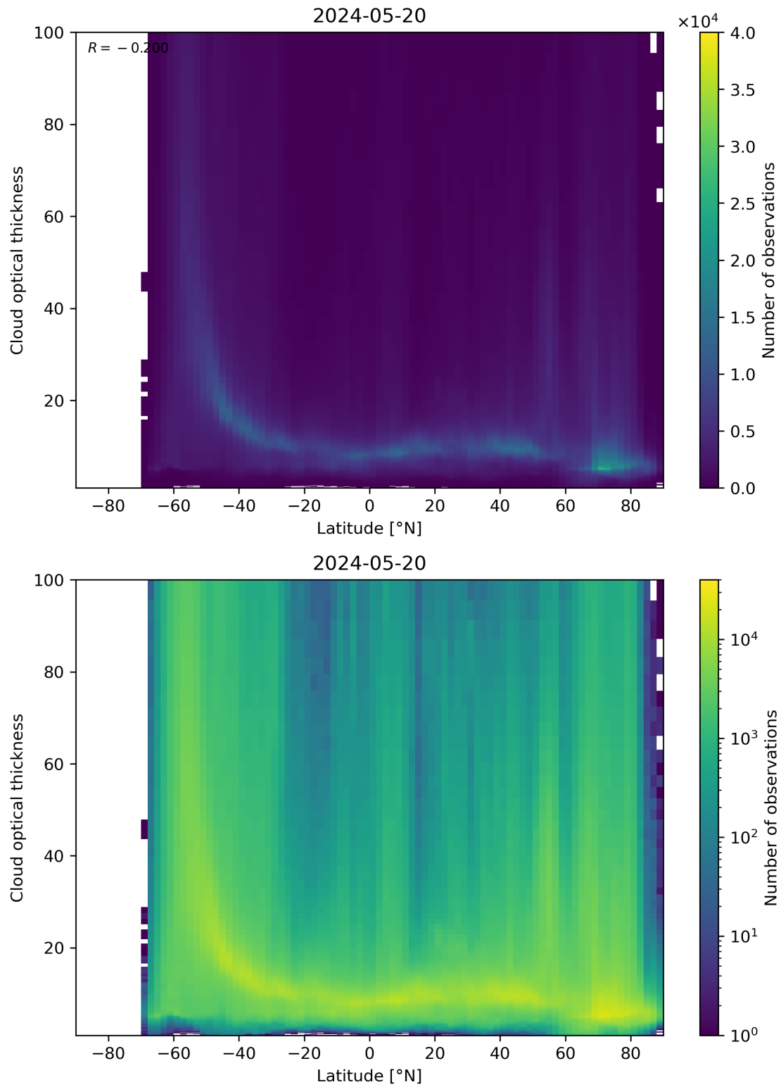
Figure 96: Scatter density plot of “Latitude” against “Cloud optical thickness” for 2024-05-19 to 2024-05-21.
