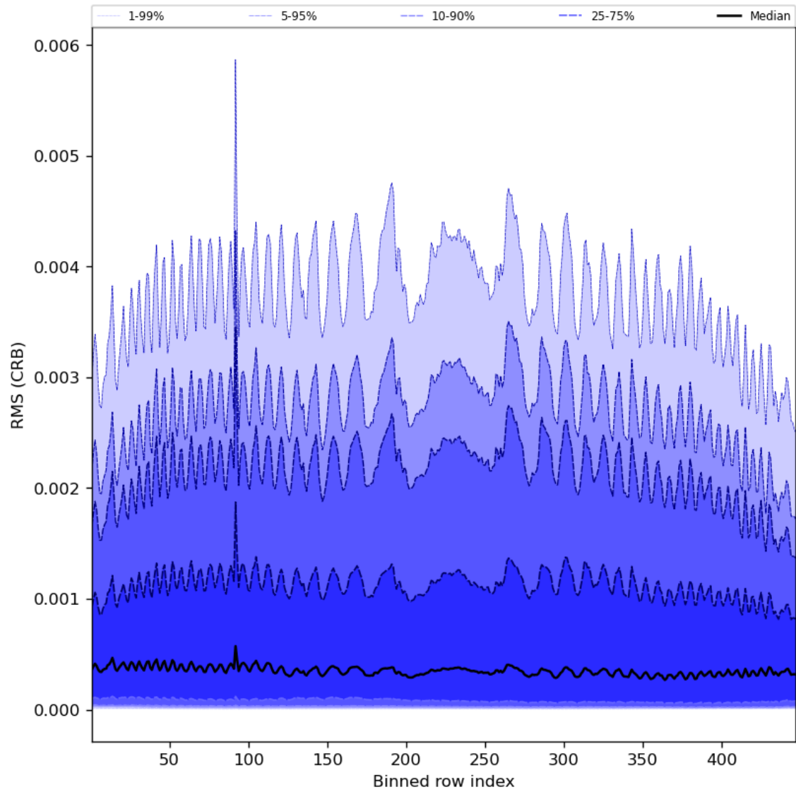
Figure 64: Along track statistics of “RMS (CRB)” for 2024-05-19 to 2024-05-21
