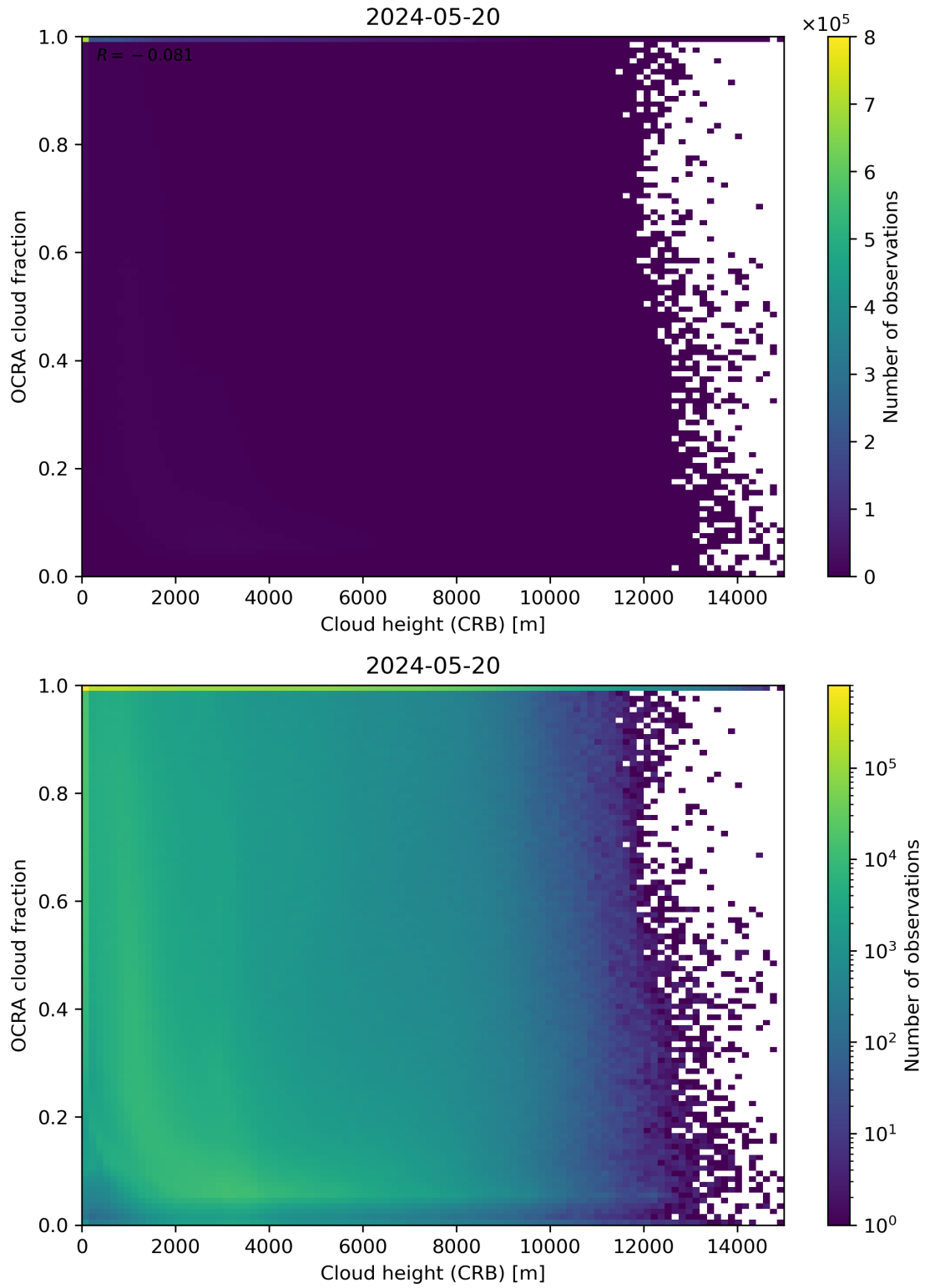
Figure 81: Scatter density plot of “Cloud height (CRB)” against “OCRA cloud fraction” for 2024-05-19 to 2024-05-21.
