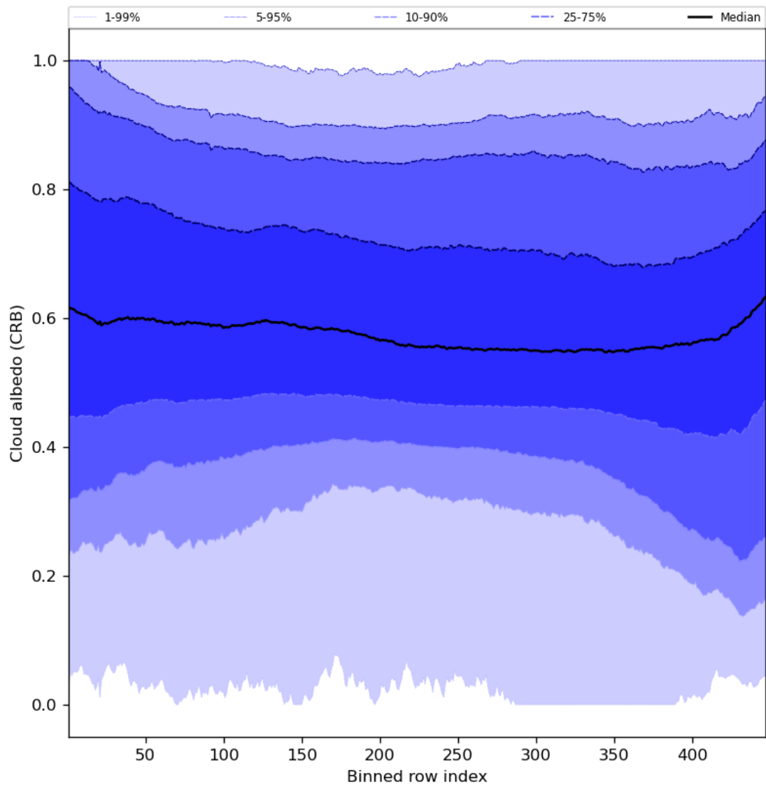
Figure 60: Along track statistics of “Cloud albedo (CRB)” for 2024-05-19 to 2024-05-21
