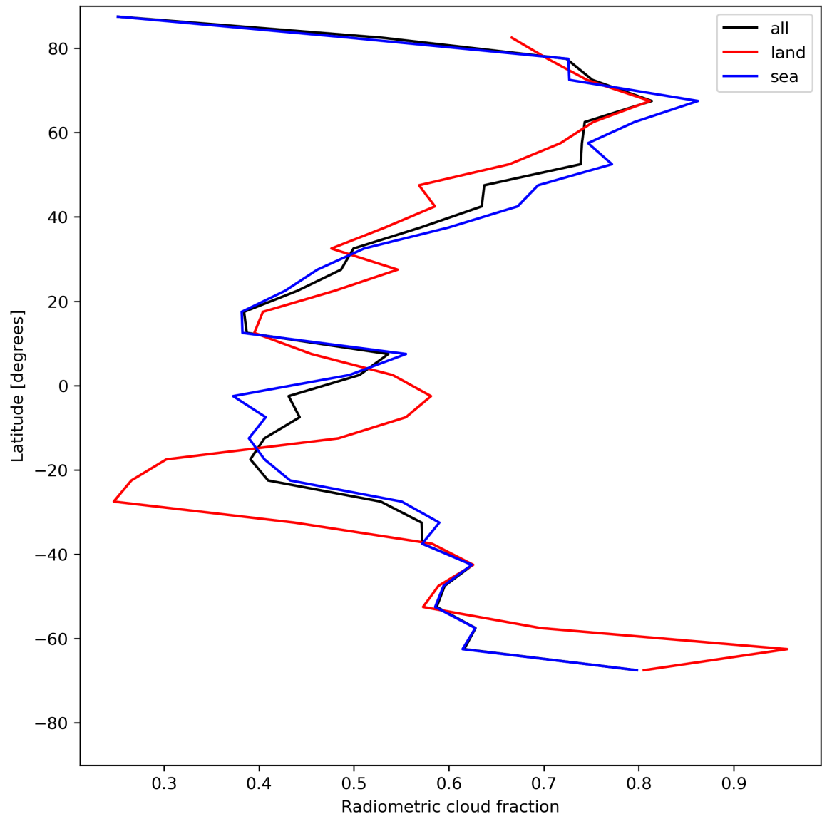
Figure 23: Zonal average of “Radiometric cloud fraction” for 2024-05-19 to 2024-05-21.
