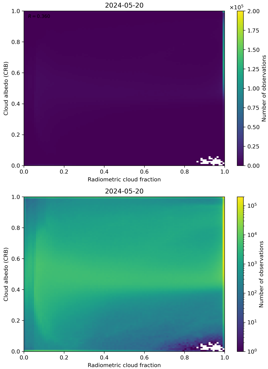
Figure 71: Scatter density plot of “Radiometric cloud fraction” against “Cloud albedo (CRB)” for 2024-05-19 to 2024-05-21.
