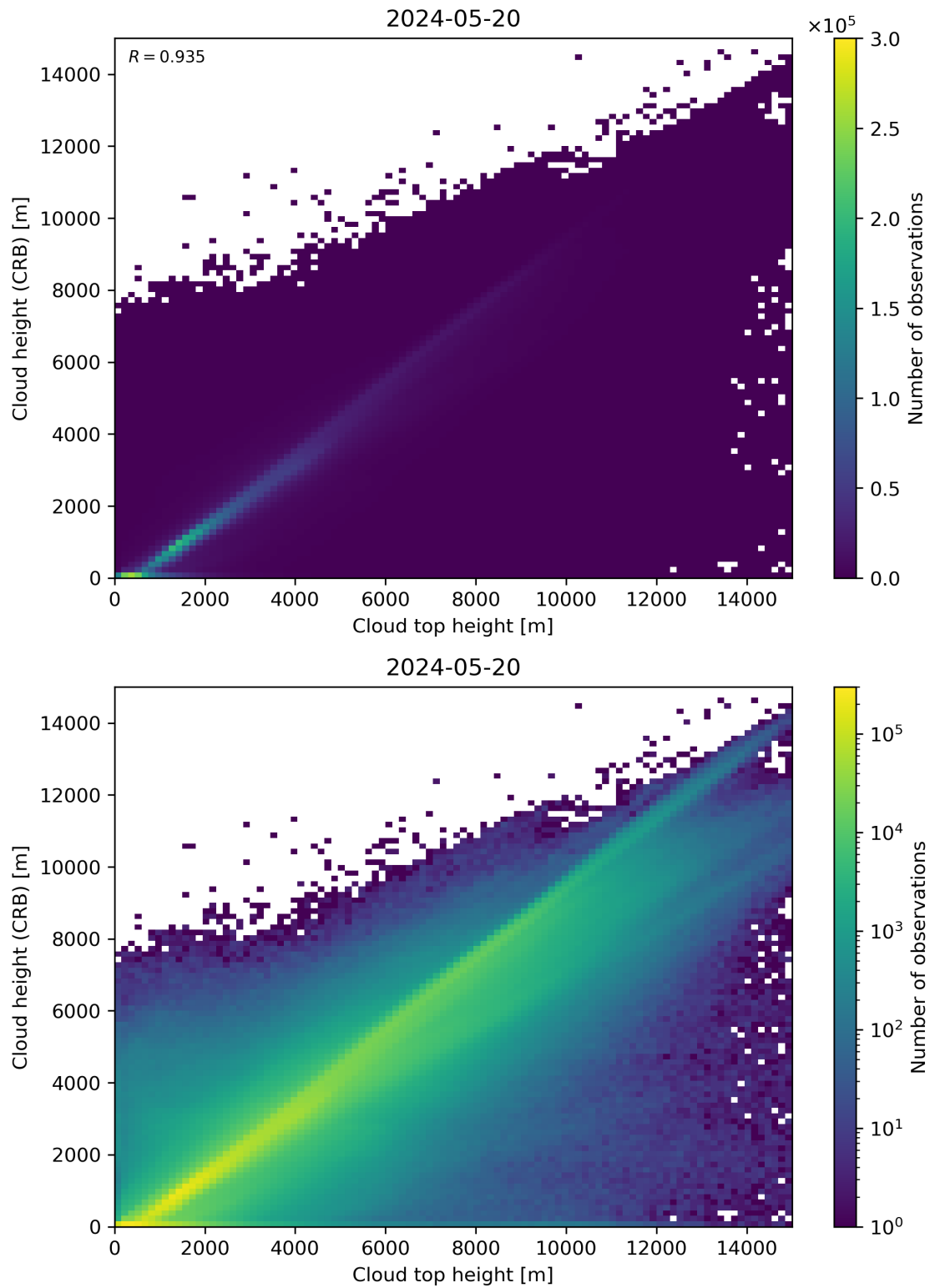
Figure 89: Scatter density plot of “Cloud top height” against “Cloud height (CRB)” for 2024-05-19 to 2024-05-21.
