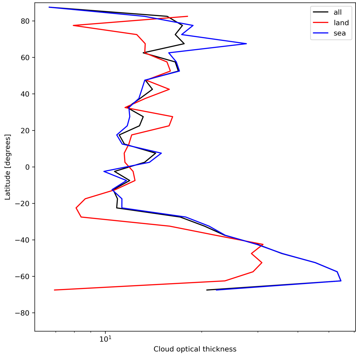
Figure 25: Zonal average of “Cloud optical thickness” for 2024-05-19 to 2024-05-21.
