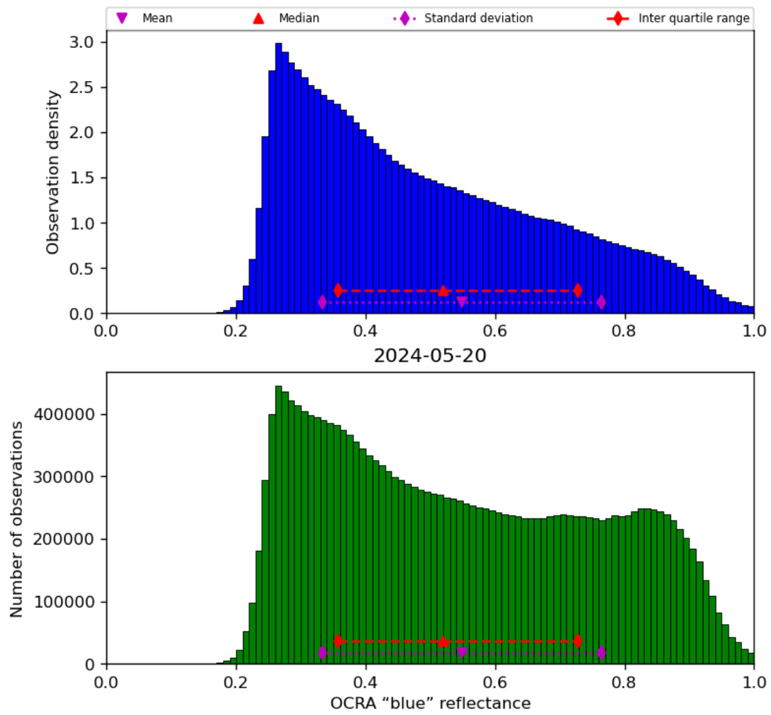
Figure 51: Histogram of “OCRA “blue” reflectance” for 2024-05-19 to 2024-05-21
