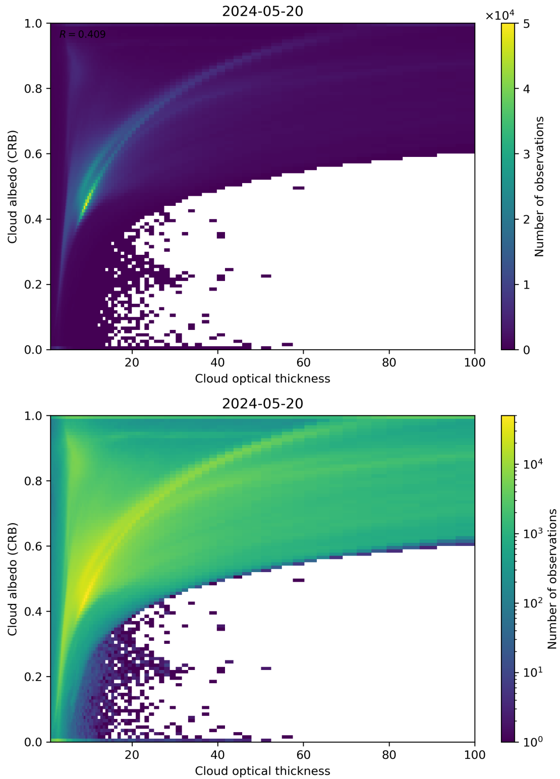
Figure 82: Scatter density plot of “Cloud optical thickness” against “Cloud albedo (CRB)” for 2024-05-19 to 2024-05-21.
