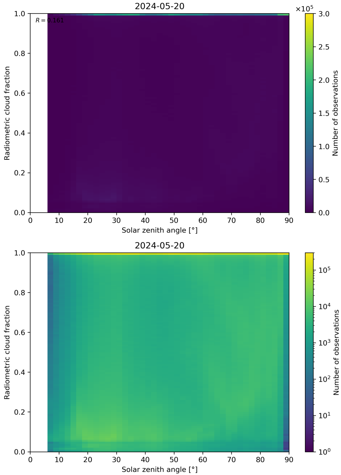
Figure 99: Scatter density plot of “Solar zenith angle” against “Radiometric cloud fraction” for 2024-05-19 to 2024-05-21.
