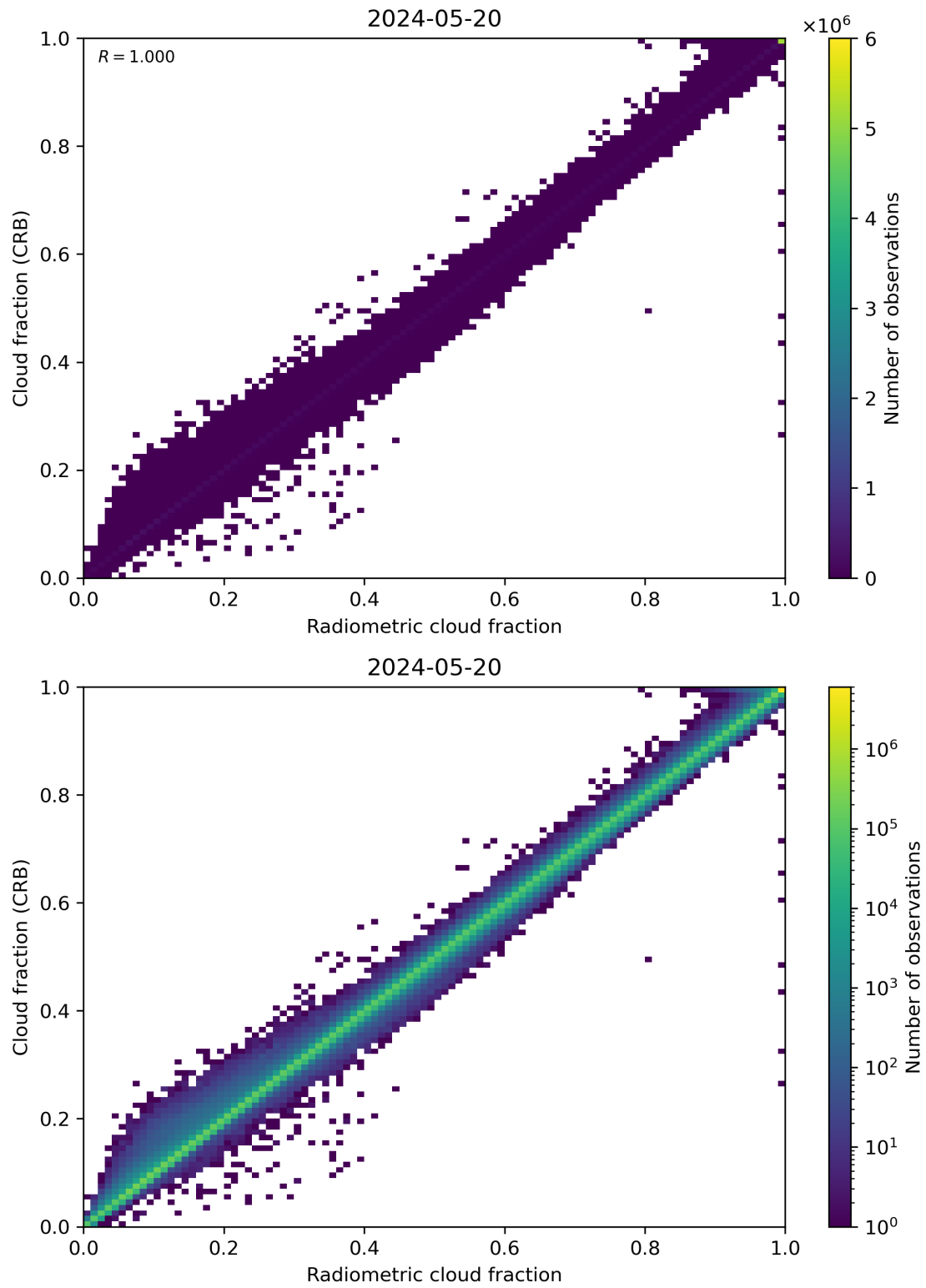
Figure 73: Scatter density plot of “Radiometric cloud fraction” against “Cloud fraction (CRB)” for 2024-05-19 to 2024-05-21.
