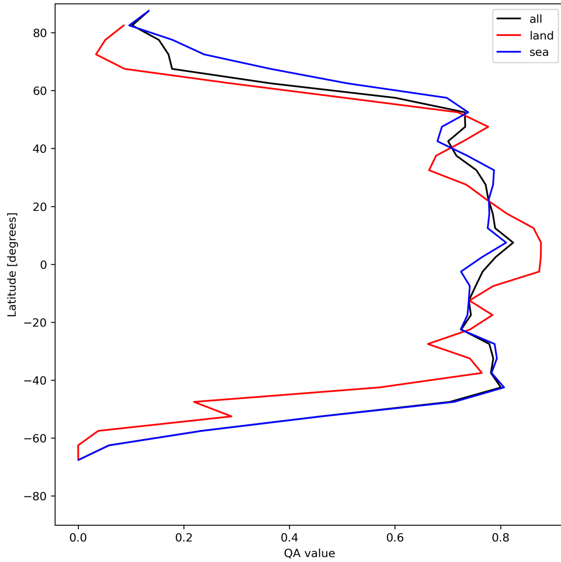
Figure 22: Zonal average of “QA value” for 2024-05-19 to 2024-05-21.
