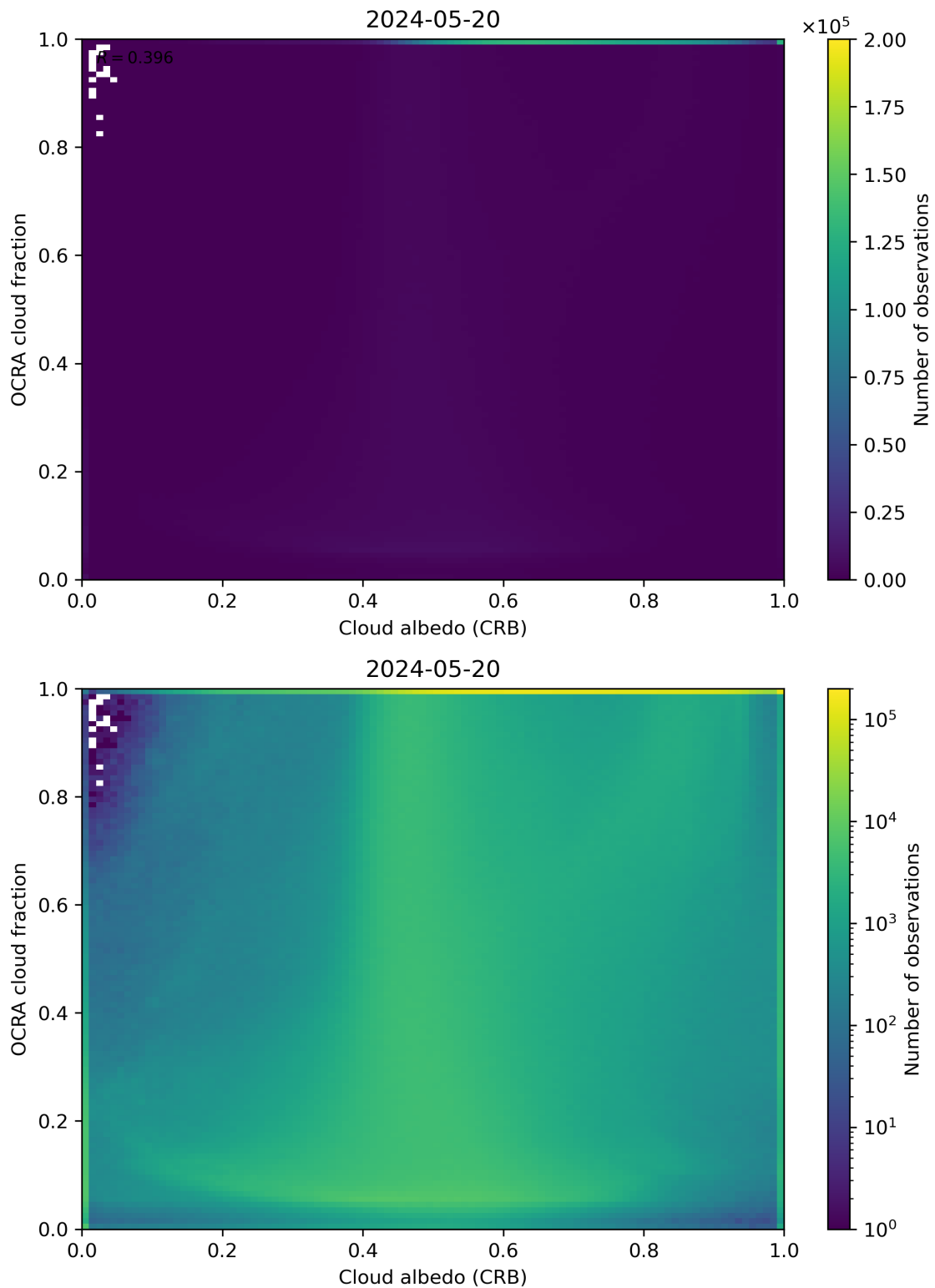
Figure 70: Scatter density plot of “Cloud albedo (CRB)” against “OCRA cloud fraction” for 2024-05-19 to 2024-05-21.
