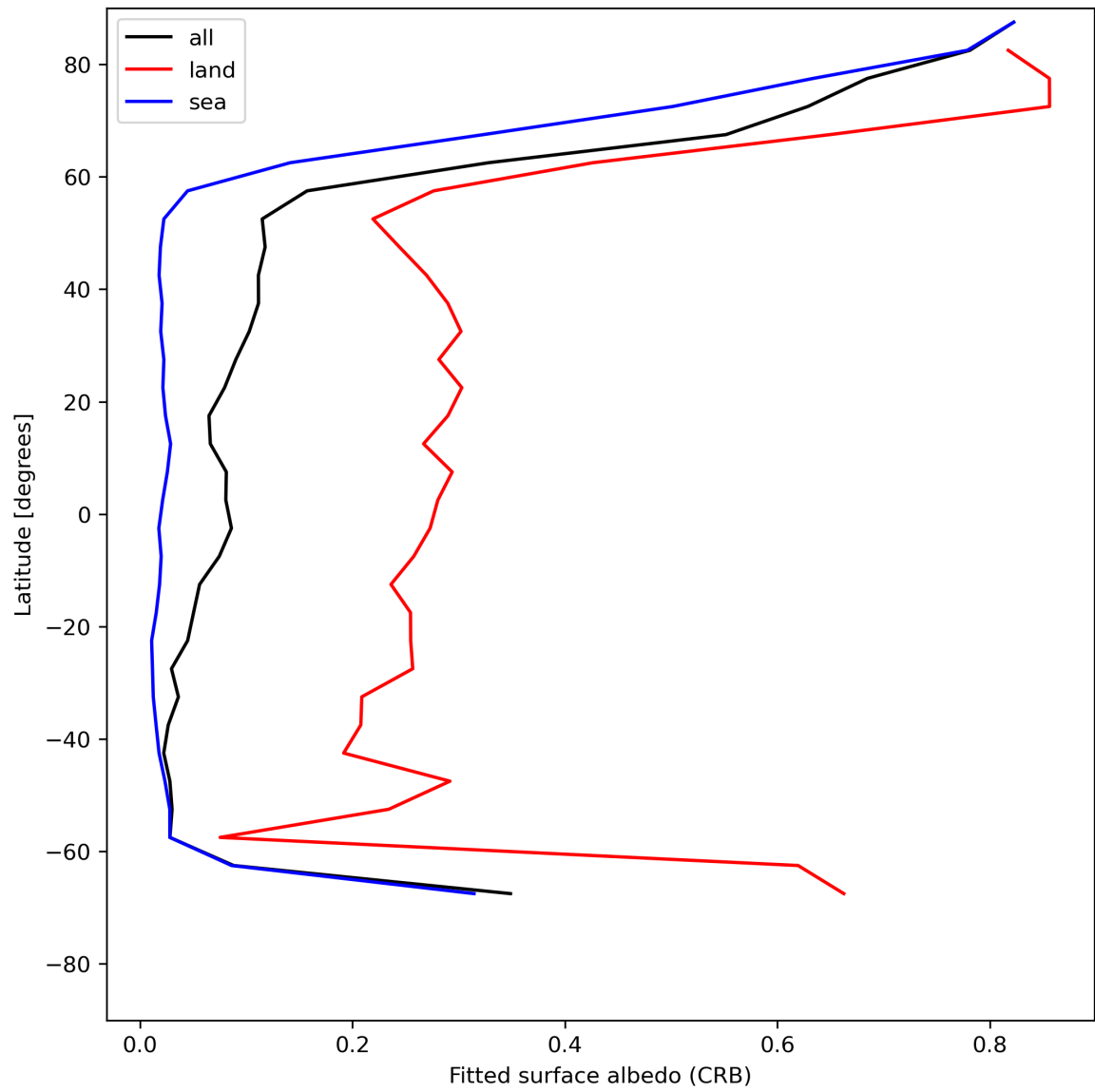
Figure 30: Zonal average of “Fitted surface albedo (CRB)” for 2024-05-19 to 2024-05-21.
