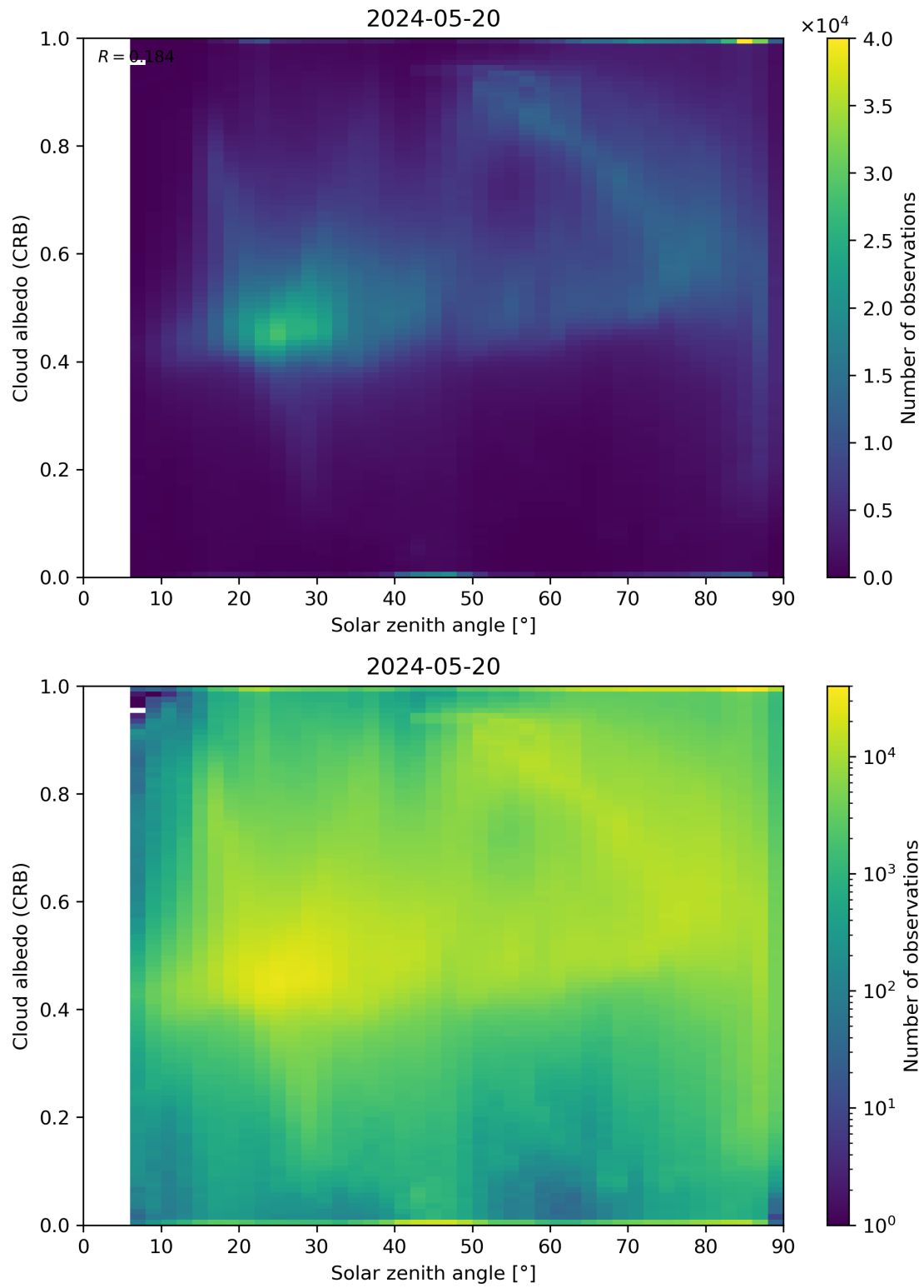
Figure 98: Scatter density plot of “Solar zenith angle” against “Cloud albedo (CRB)” for 2024-05-19 to 2024-05-21.
