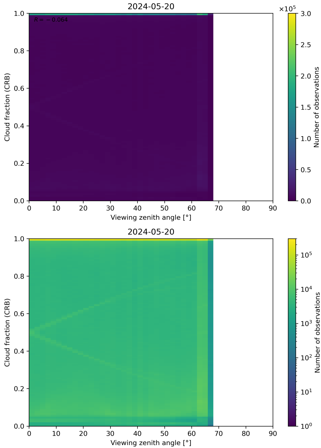
Figure 109: Scatter density plot of “Viewing zenith angle” against “Cloud fraction (CRB)” for 2024-05-19 to 2024-05-21.
