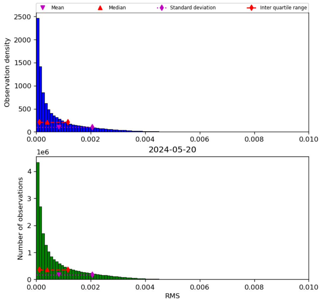
Figure 47: Histogram of “RMS” for 2024-05-19 to 2024-05-21
