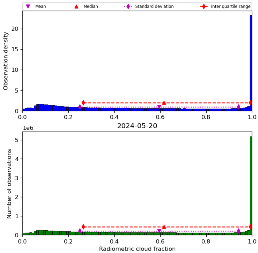
Figure 39: Histogram of “Radiometric cloud fraction” for 2024-05-19 to 2024-05-21
