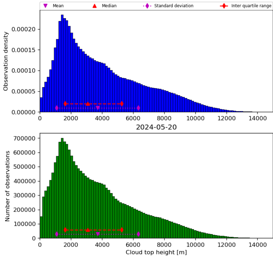
Figure 40: Histogram of “Cloud top height” for 2024-05-19 to 2024-05-21
