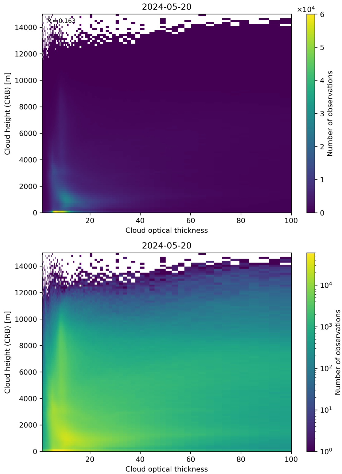
Figure 85: Scatter density plot of “Cloud optical thickness” against “Cloud height (CRB)” for 2024-05-19 to 2024-05-21.
