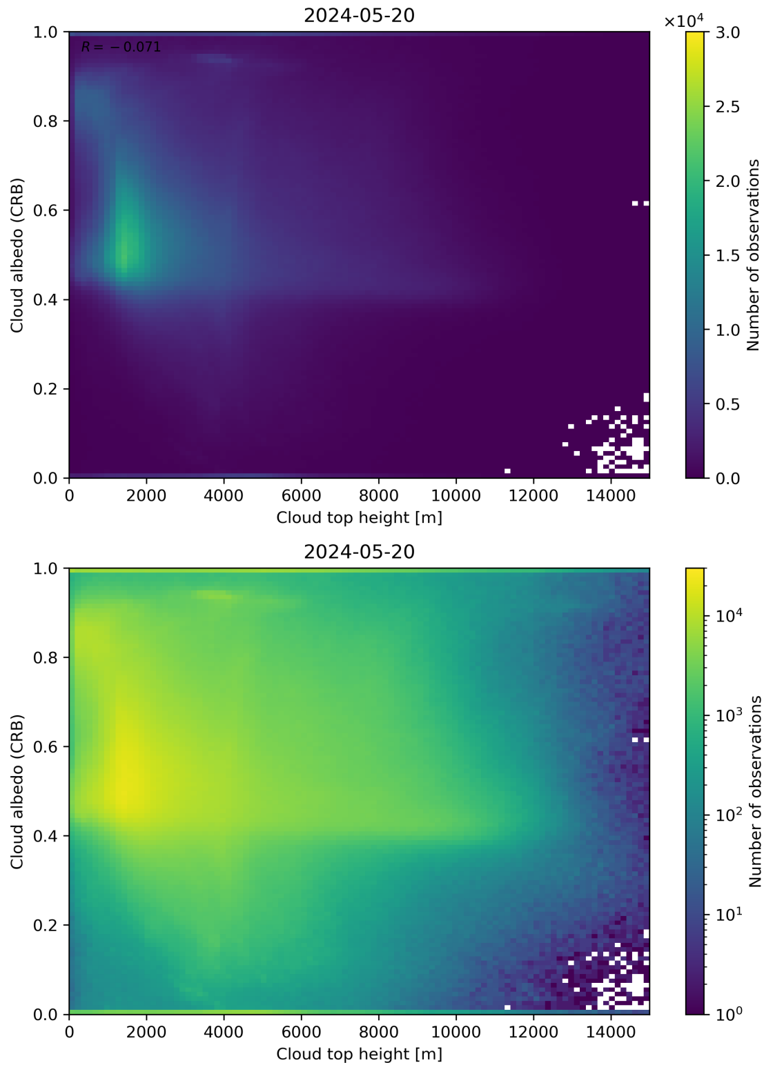
Figure 86: Scatter density plot of “Cloud top height” against “Cloud albedo (CRB)” for 2024-05-19 to 2024-05-21.
