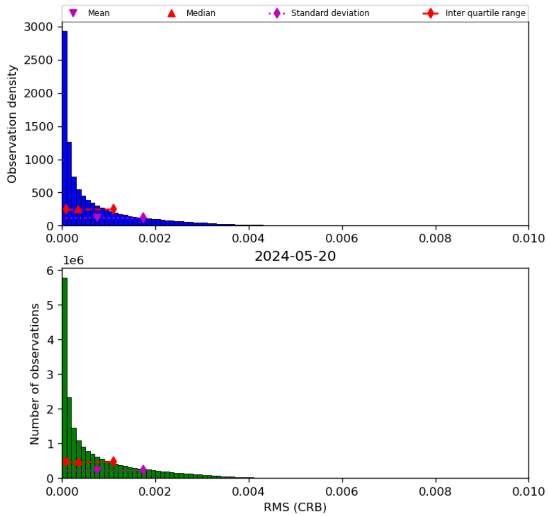
Figure 48: Histogram of “RMS (CRB)” for 2024-05-19 to 2024-05-21
