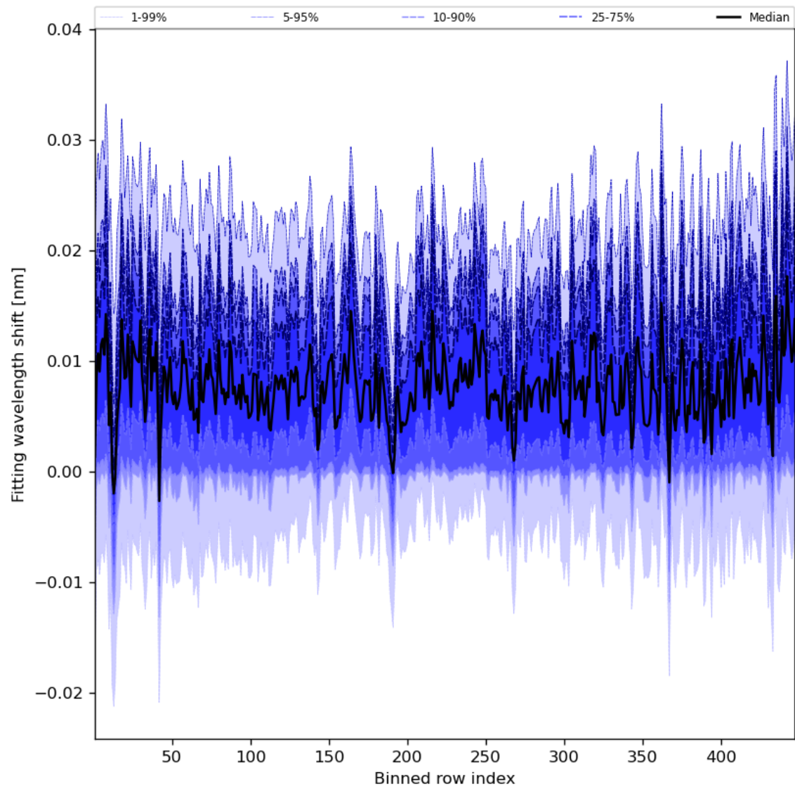
Figure 65: Along track statistics of “Fitting wavelength shift” for 2024-05-19 to 2024-05-21
