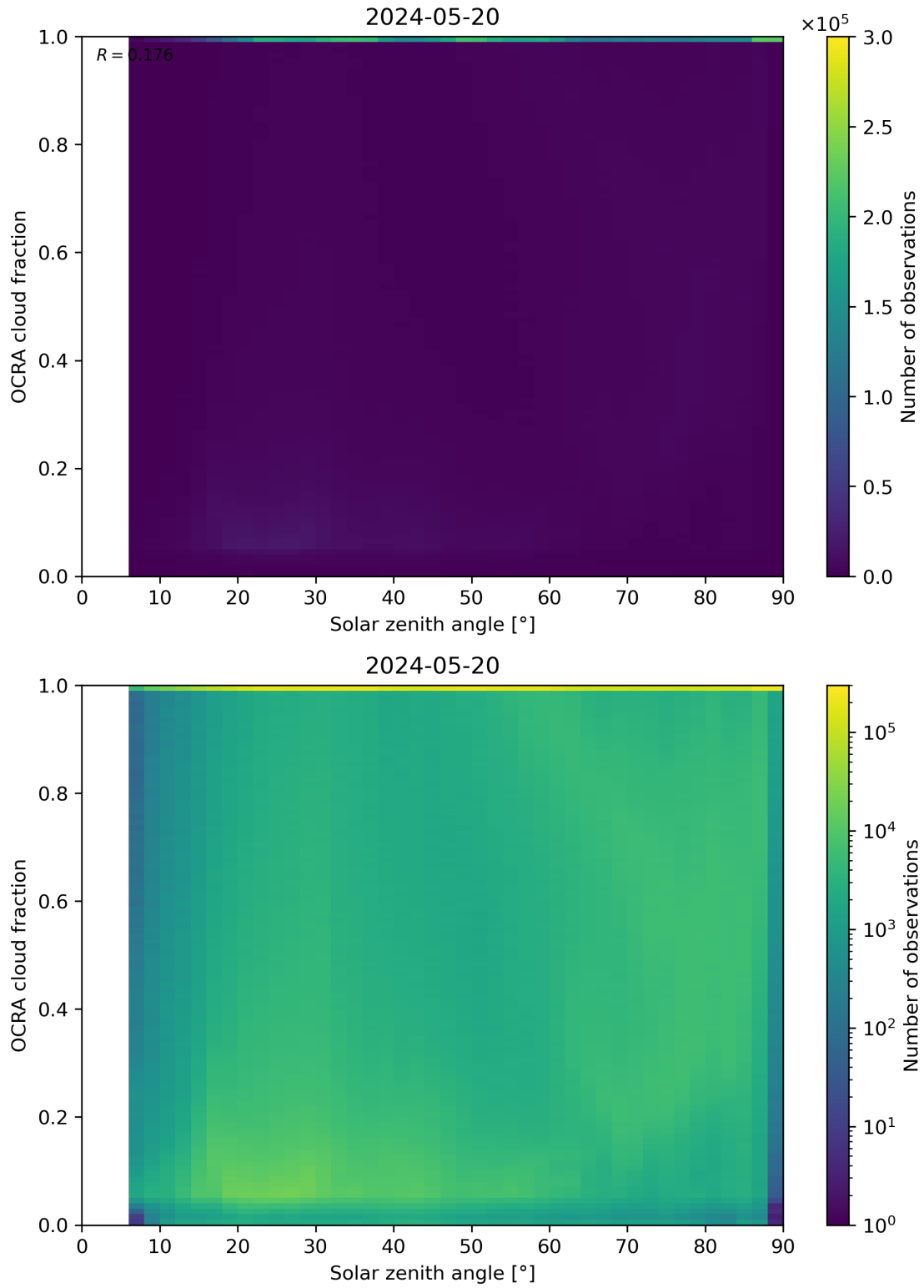
Figure 100: Scatter density plot of “Solar zenith angle” against “OCRA cloud fraction” for 2024-05-19 to 2024-05-21.
