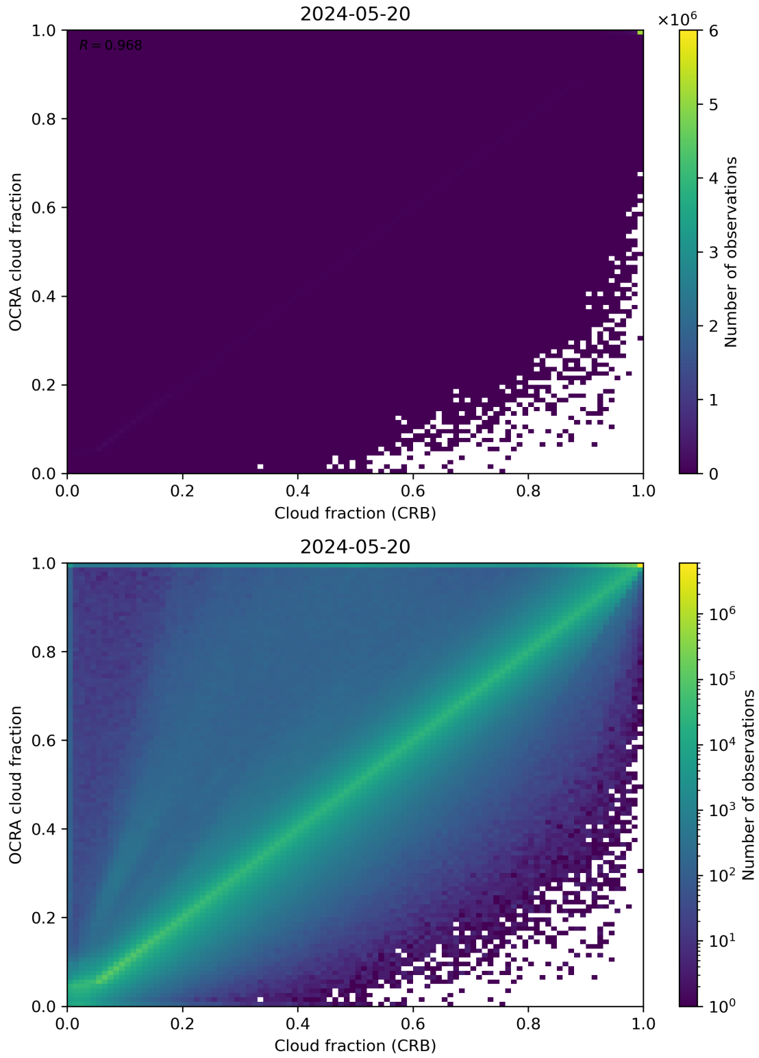
Figure 78: Scatter density plot of “Cloud fraction (CRB)” against “OCRA cloud fraction” for 2024-05-19 to 2024-05-21.
