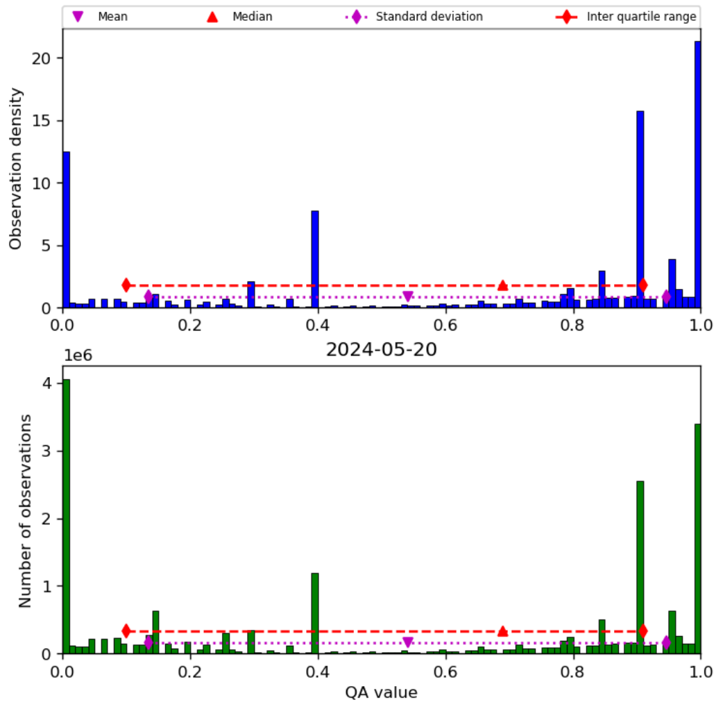
Figure 38: Histogram of “QA value” for 2024-05-19 to 2024-05-21
