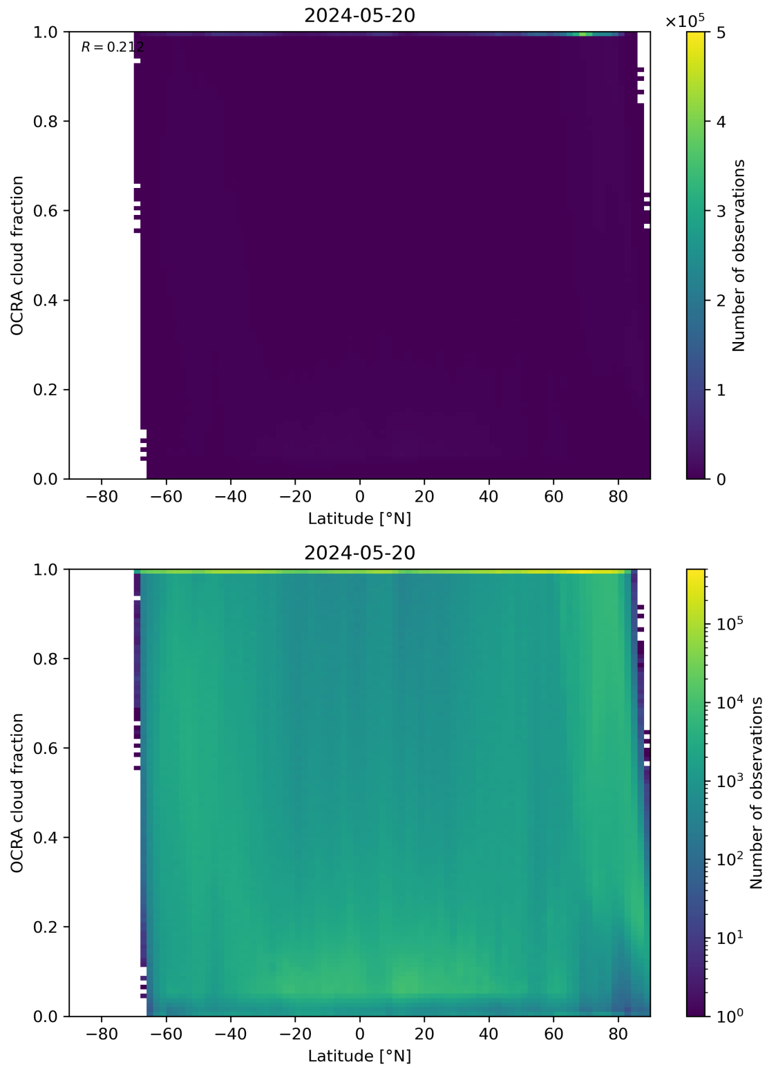
Figure 93: Scatter density plot of “Latitude” against “OCRA cloud fraction” for 2024-05-19 to 2024-05-21.
