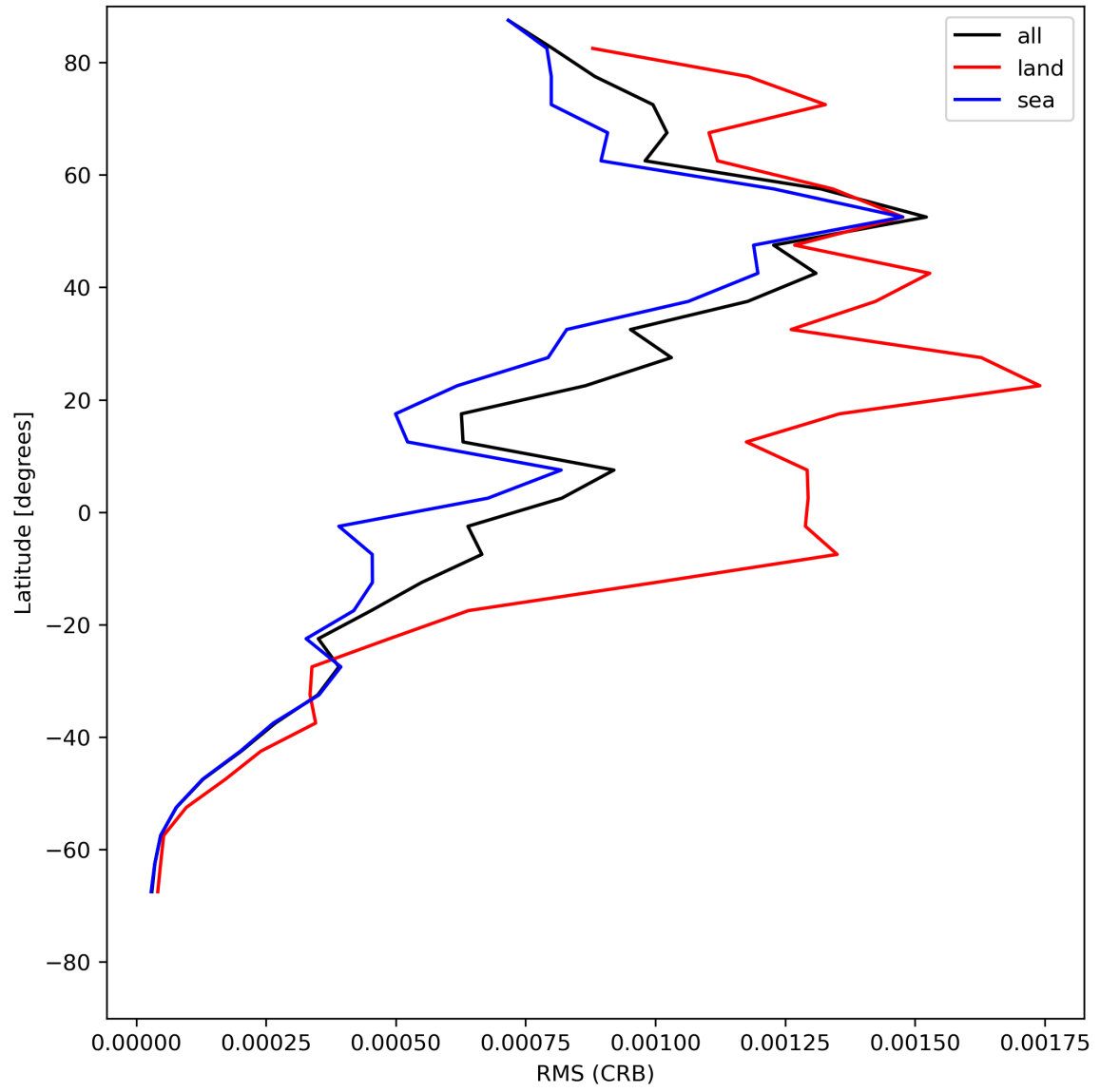
Figure 32: Zonal average of “RMS (CRB)” for 2024-05-19 to 2024-05-21.
