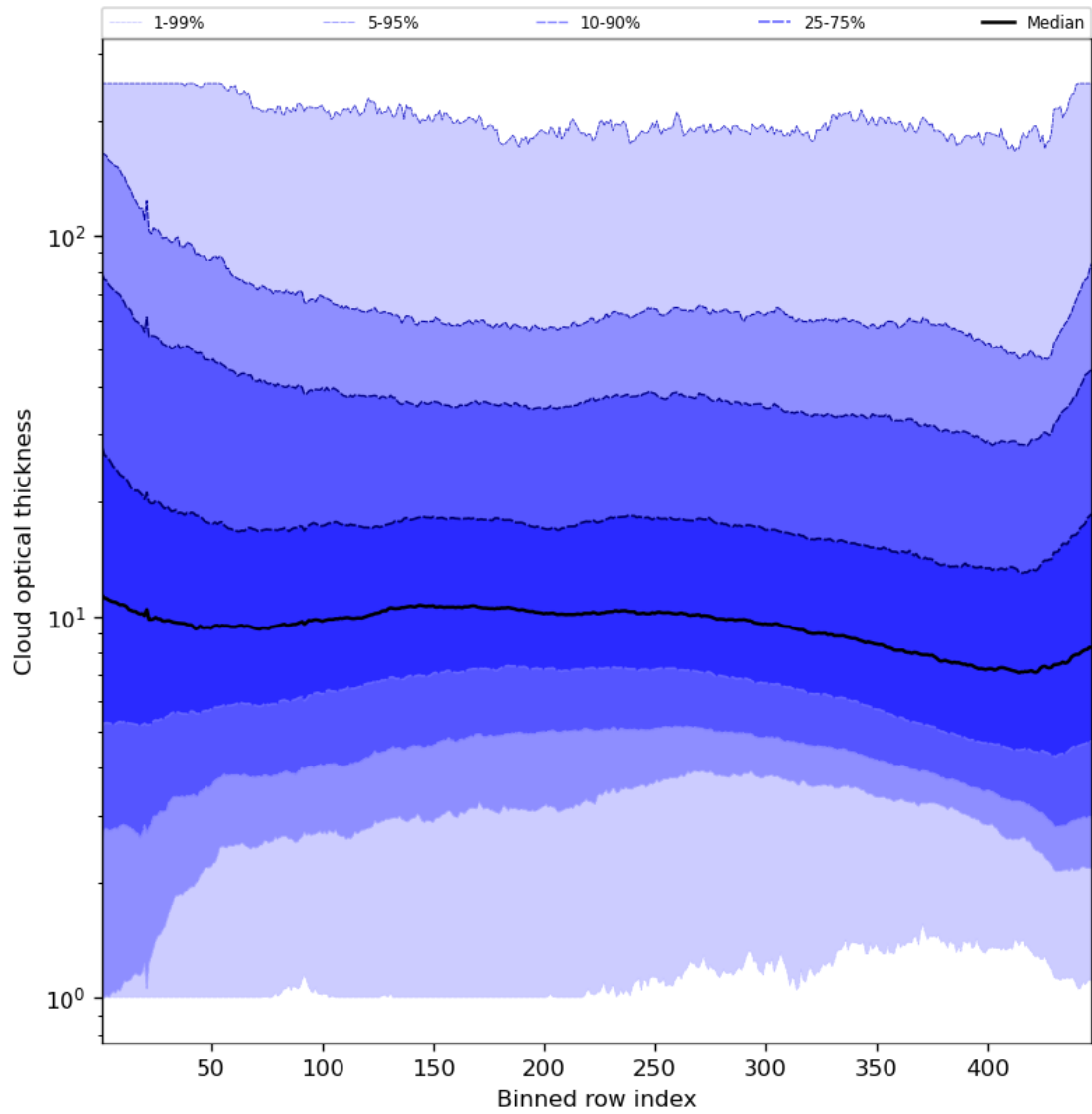
Figure 57: Along track statistics of “Cloud optical thickness” for 2024-05-19 to 2024-05-21
