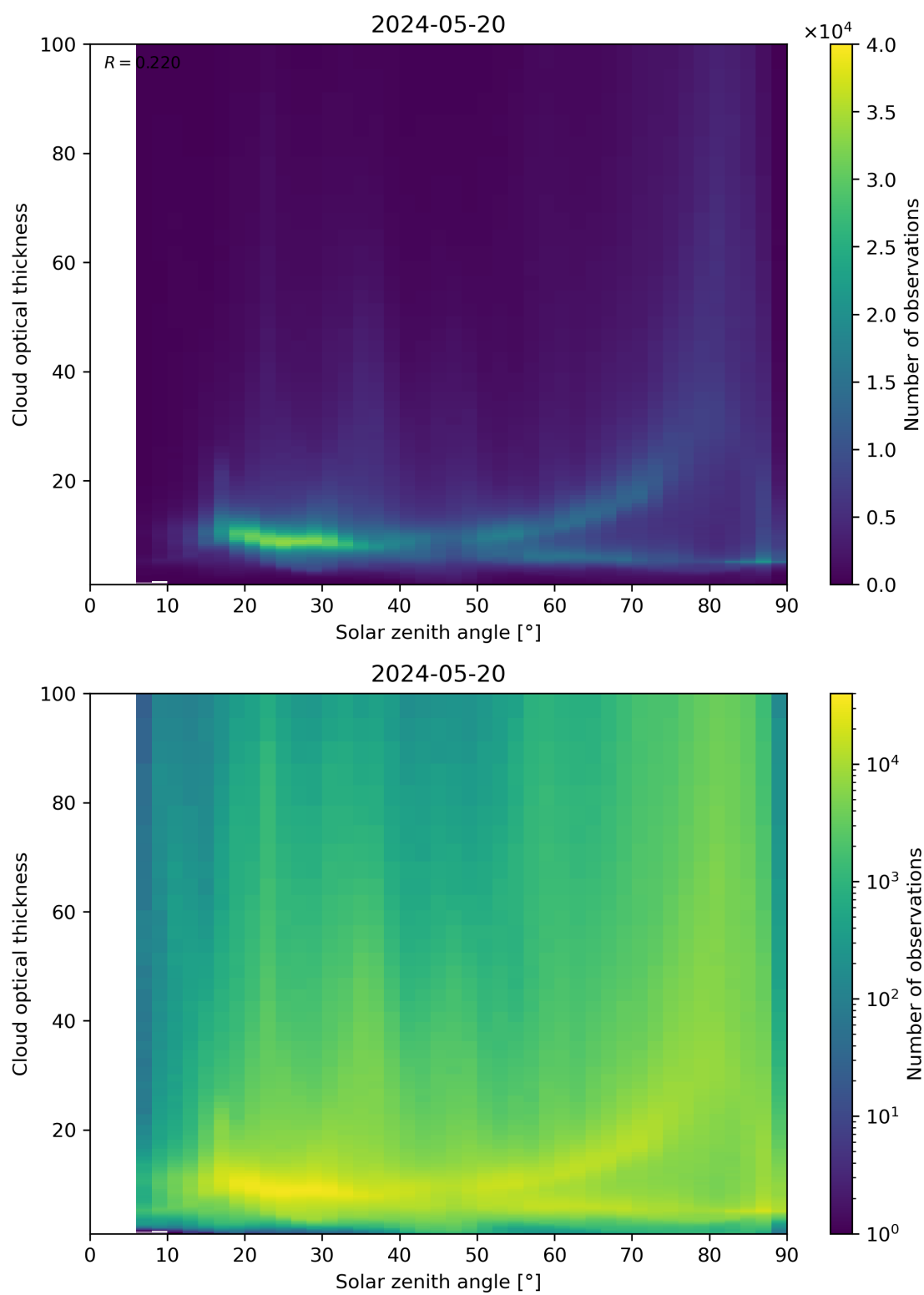
Figure 103: Scatter density plot of “Solar zenith angle” against “Cloud optical thickness” for 2024-05-19 to 2024-05-21.
