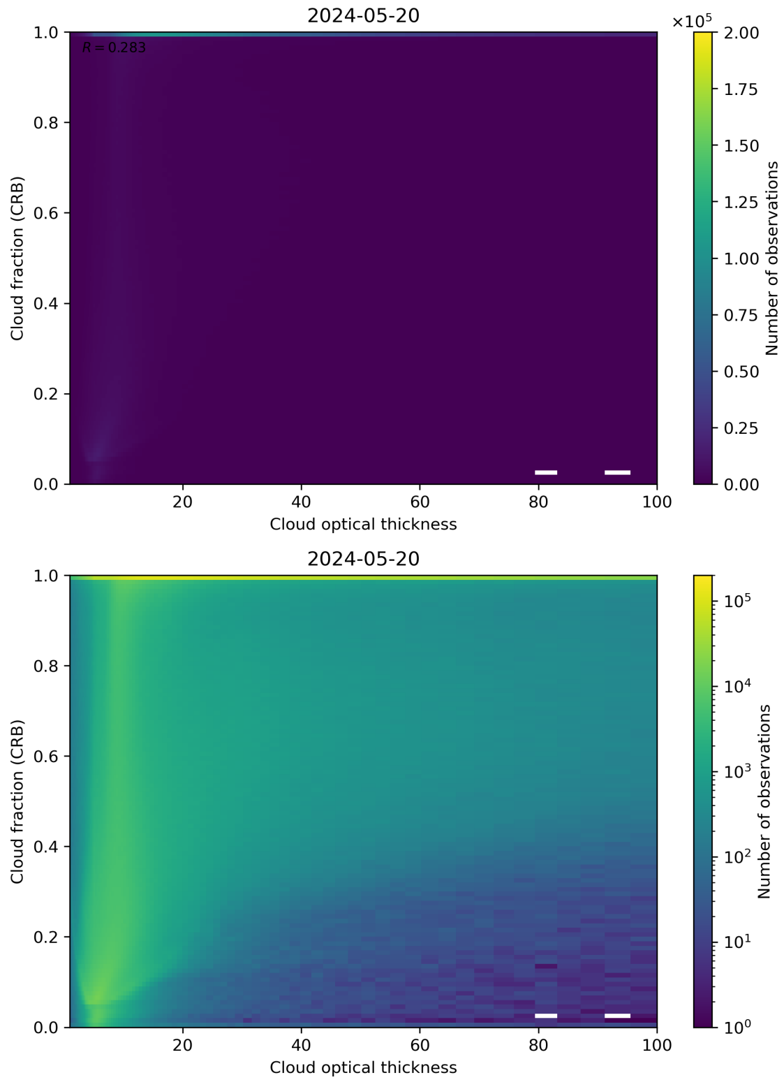
Figure 84: Scatter density plot of “Cloud optical thickness” against “Cloud fraction (CRB)” for 2024-05-19 to 2024-05-21.
