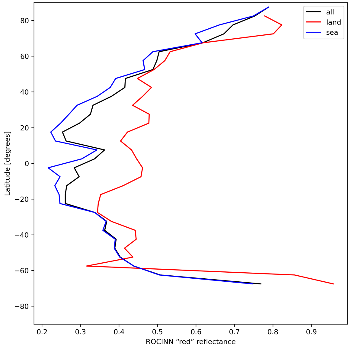
Figure 37: Zonal average of “ROCINN “red” reflectance” for 2024-05-19 to 2024-05-21.
