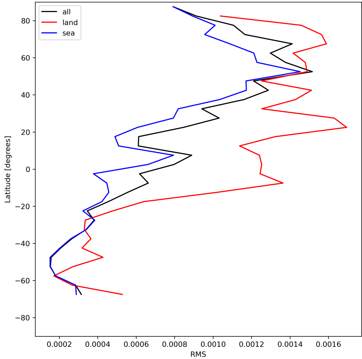
Figure 31: Zonal average of “RMS” for 2024-05-19 to 2024-05-21.
