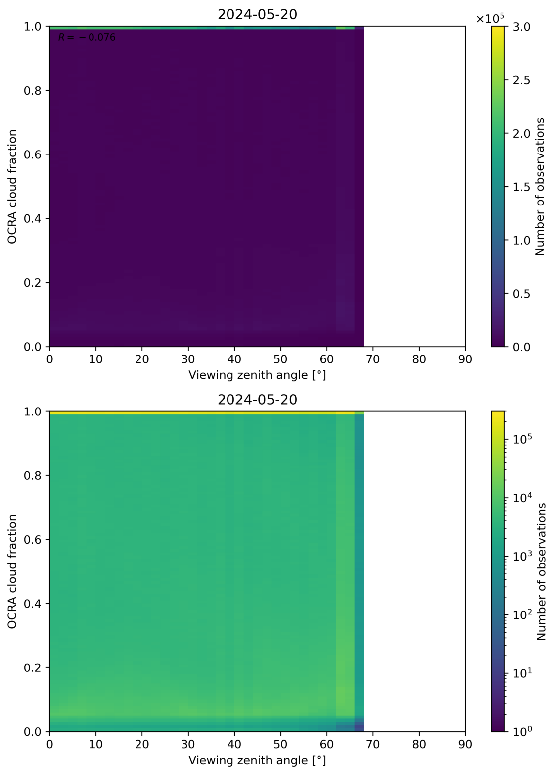
Figure 108: Scatter density plot of “Viewing zenith angle” against “OCRA cloud fraction” for 2024-05-19 to 2024-05-21.
