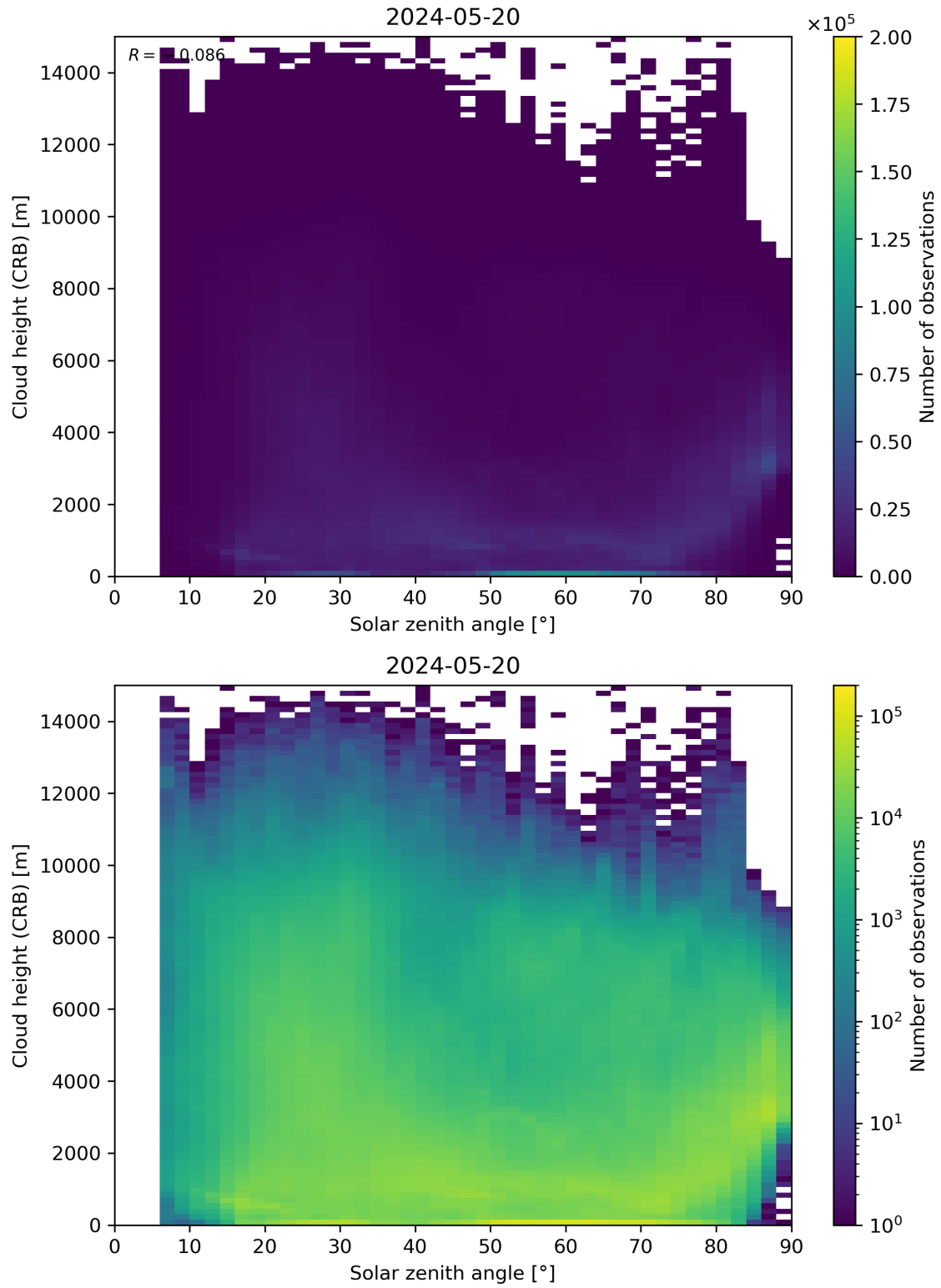
Figure 102: Scatter density plot of “Solar zenith angle” against “Cloud height (CRB)” for 2024-05-19 to 2024-05-21.
