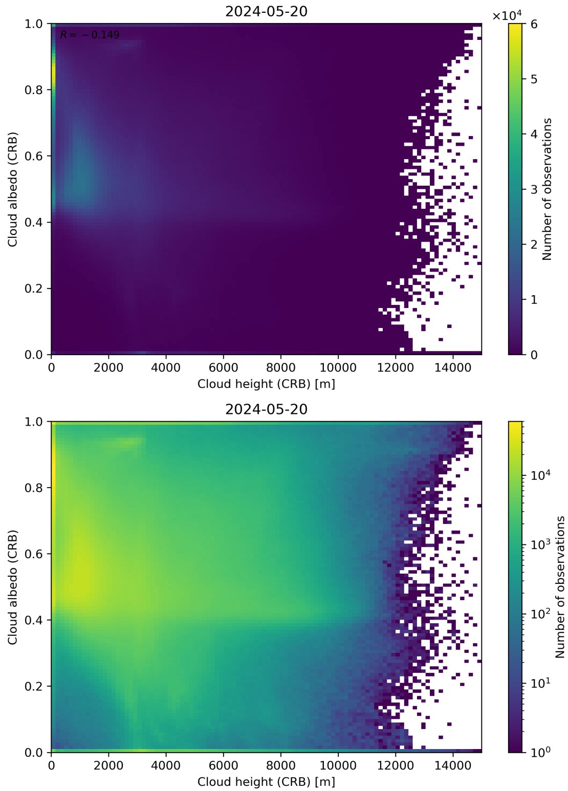
Figure 80: Scatter density plot of “Cloud height (CRB)” against “Cloud albedo (CRB)” for 2024-05-19 to 2024-05-21.
