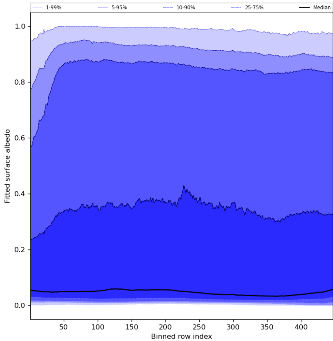
Figure 61: Along track statistics of “Fitted surface albedo” for 2024-05-19 to 2024-05-21
