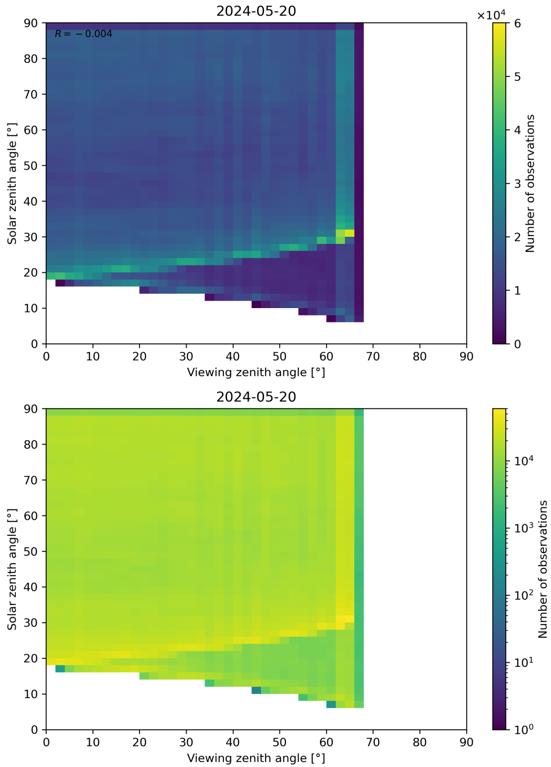
Figure 114: Scatter density plot of “Viewing zenith angle” against “Solar zenith angle” for 2024-05-19 to 2024-05-21.
