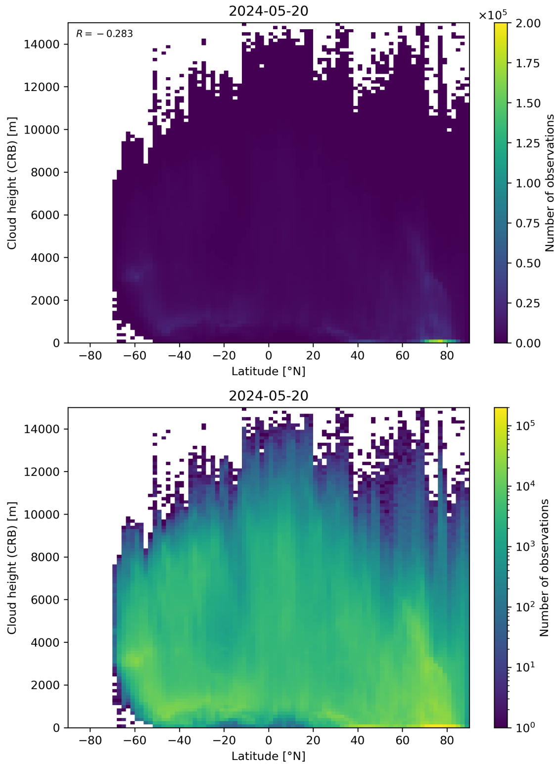
Figure 95: Scatter density plot of “Latitude” against “Cloud height (CRB)” for 2024-05-19 to 2024-05-21.
