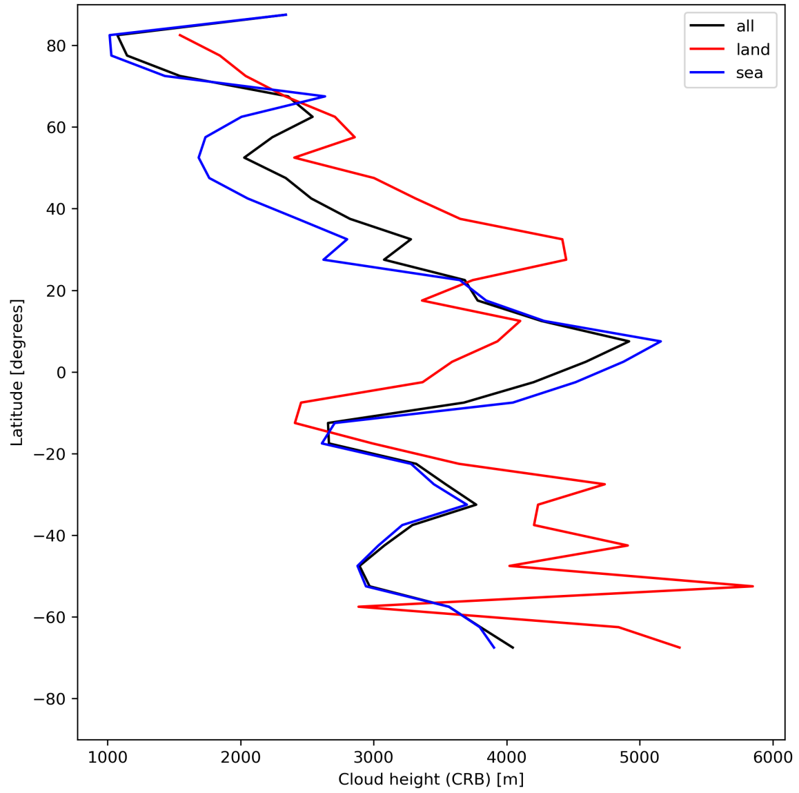
Figure 27: Zonal average of “Cloud height (CRB)” for 2024-05-19 to 2024-05-21.
