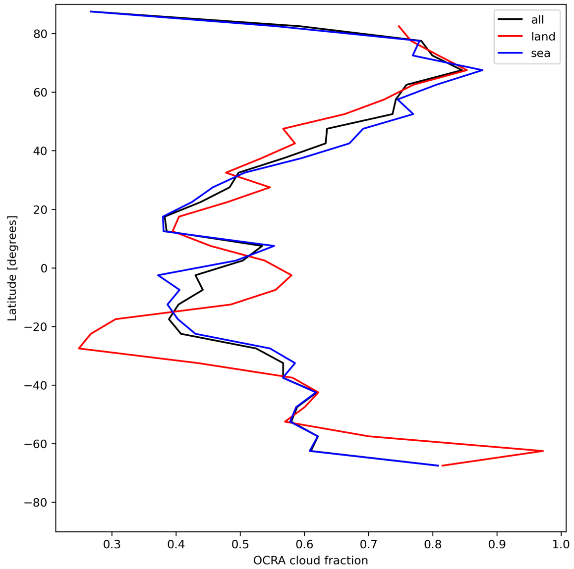
Figure 34: Zonal average of “OCRA cloud fraction” for 2024-05-19 to 2024-05-21.
