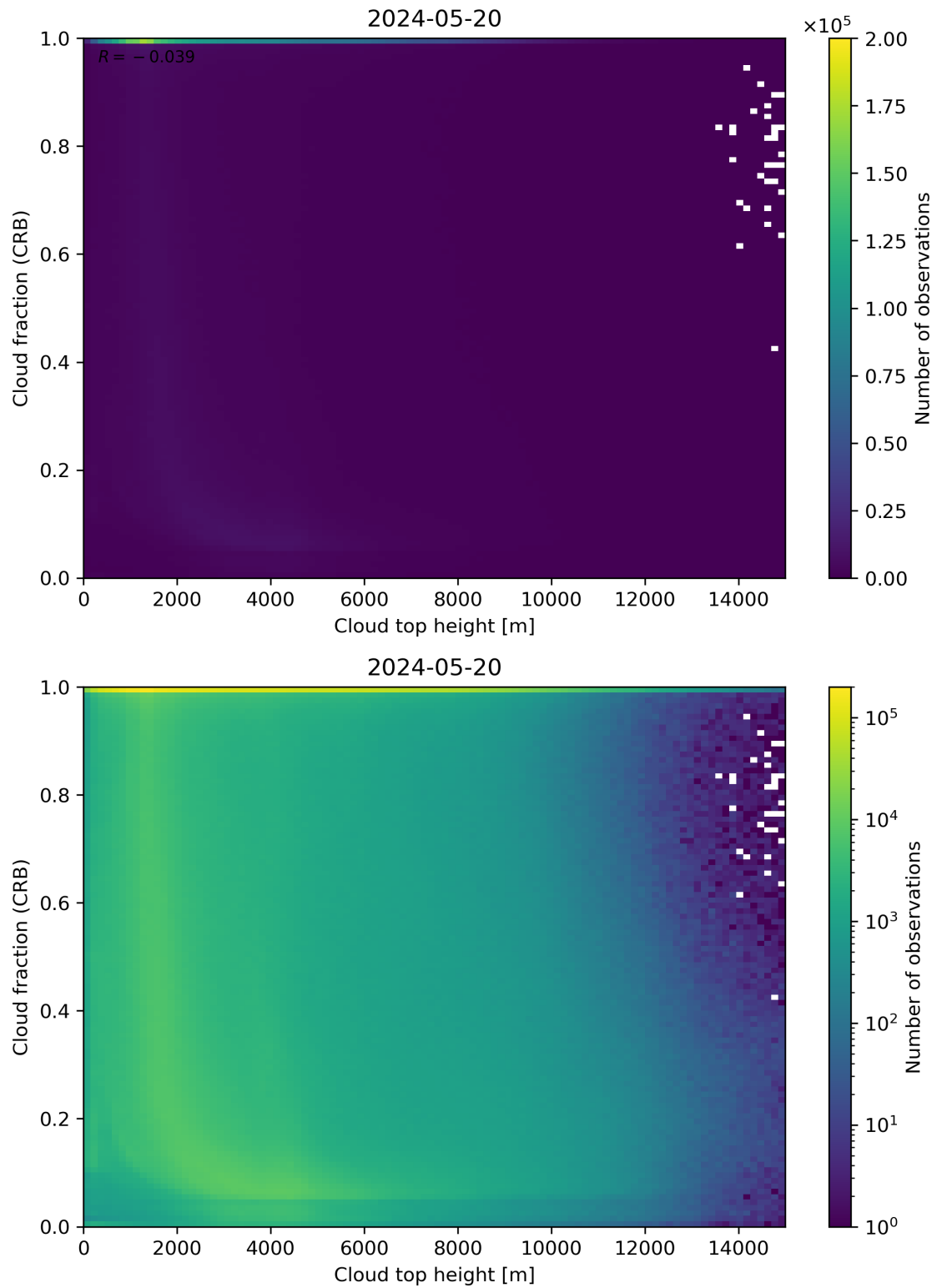
Figure 88: Scatter density plot of “Cloud top height” against “Cloud fraction (CRB)” for 2024-05-19 to 2024-05-21.
