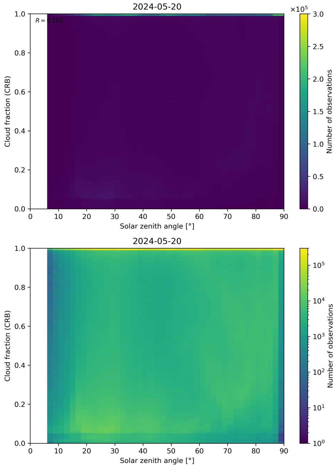
Figure 101: Scatter density plot of “Solar zenith angle” against “Cloud fraction (CRB)” for 2024-05-19 to 2024-05-21.
