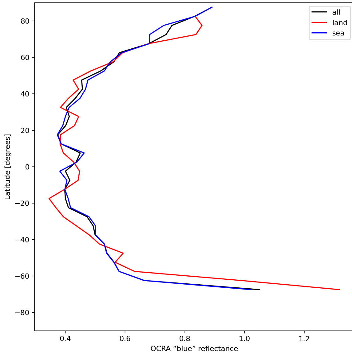
Figure 35: Zonal average of “OCRA “blue” reflectance” for 2024-05-19 to 2024-05-21.
