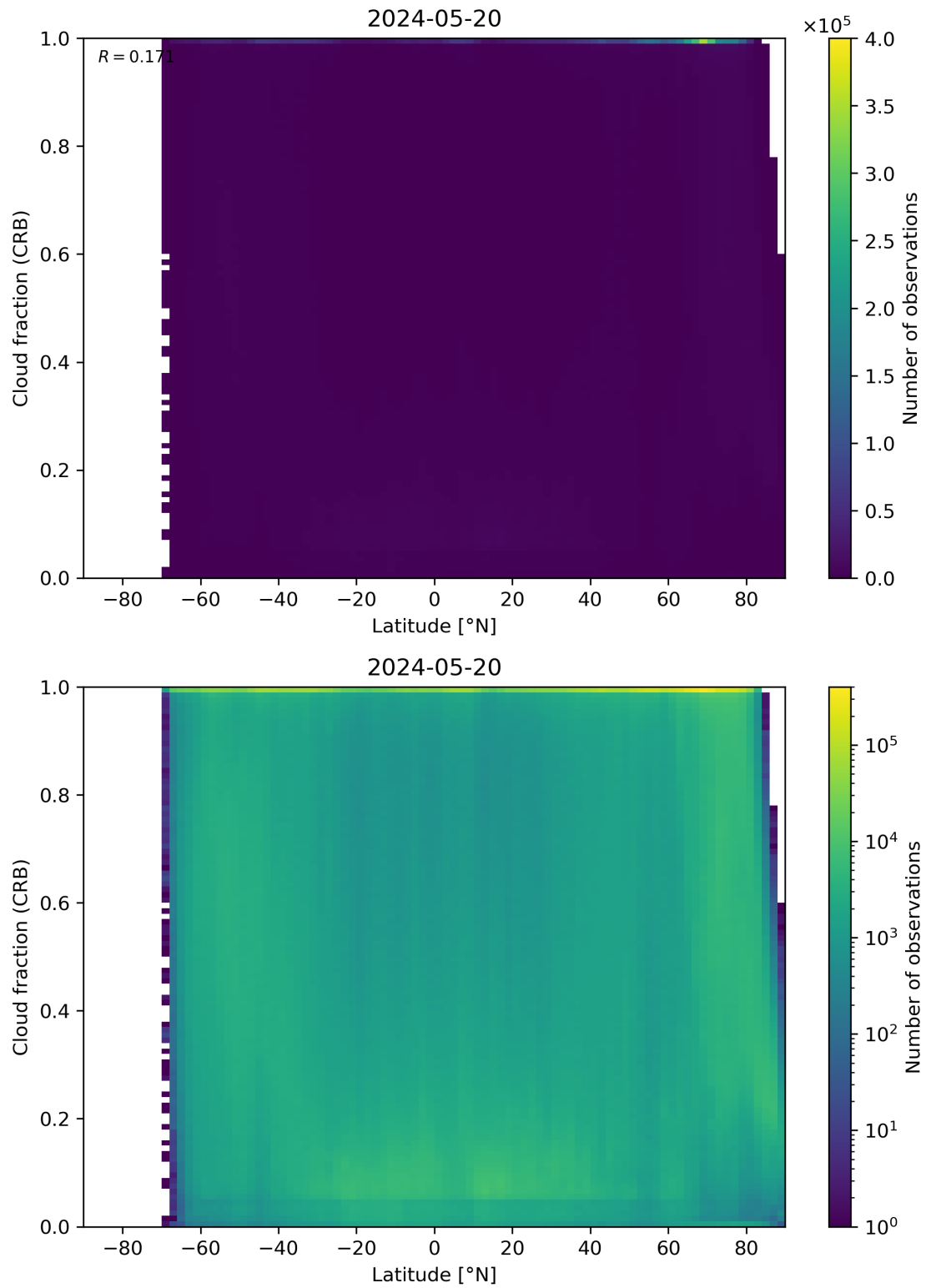
Figure 94: Scatter density plot of “Latitude” against “Cloud fraction (CRB)” for 2024-05-19 to 2024-05-21.
