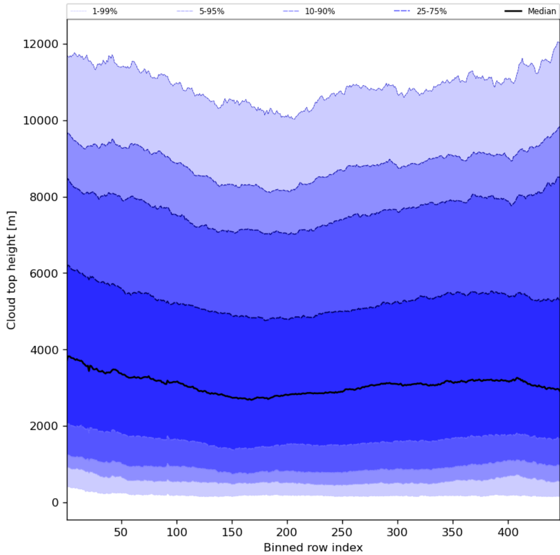
Figure 56: Along track statistics of “Cloud top height” for 2024-05-19 to 2024-05-21
