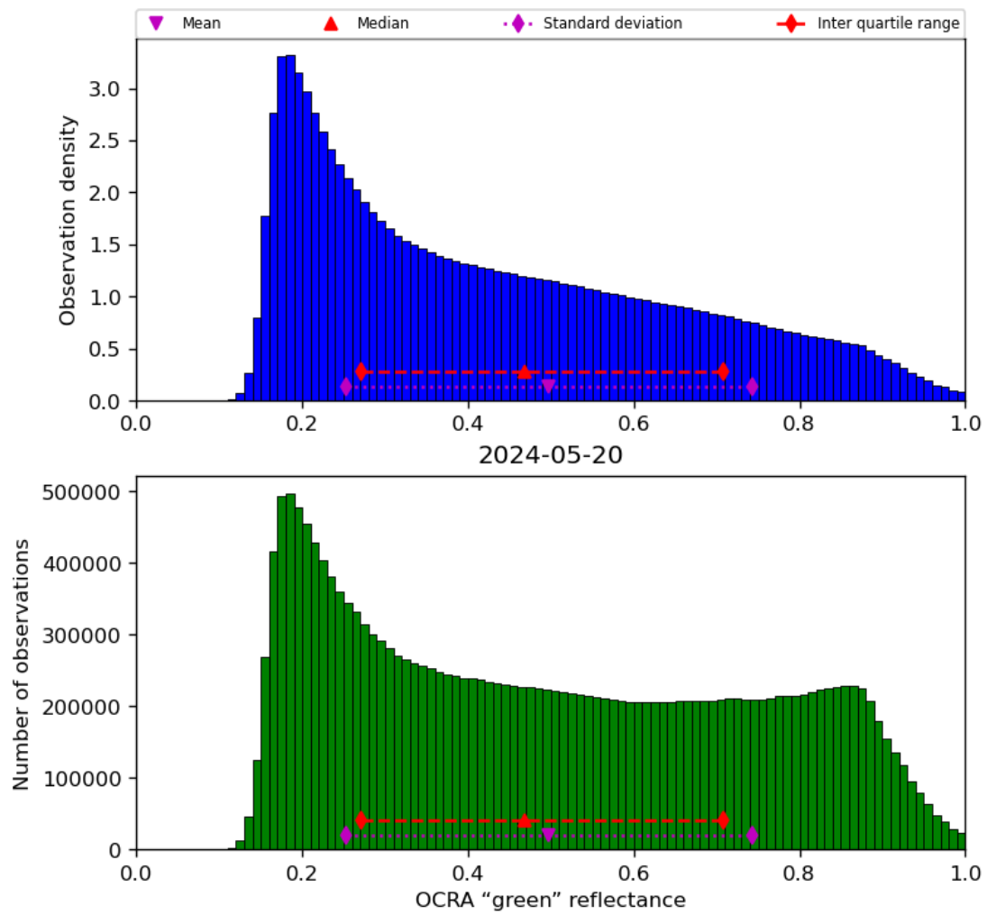
Figure 52: Histogram of “OCRA “green” reflectance” for 2024-05-19 to 2024-05-21
