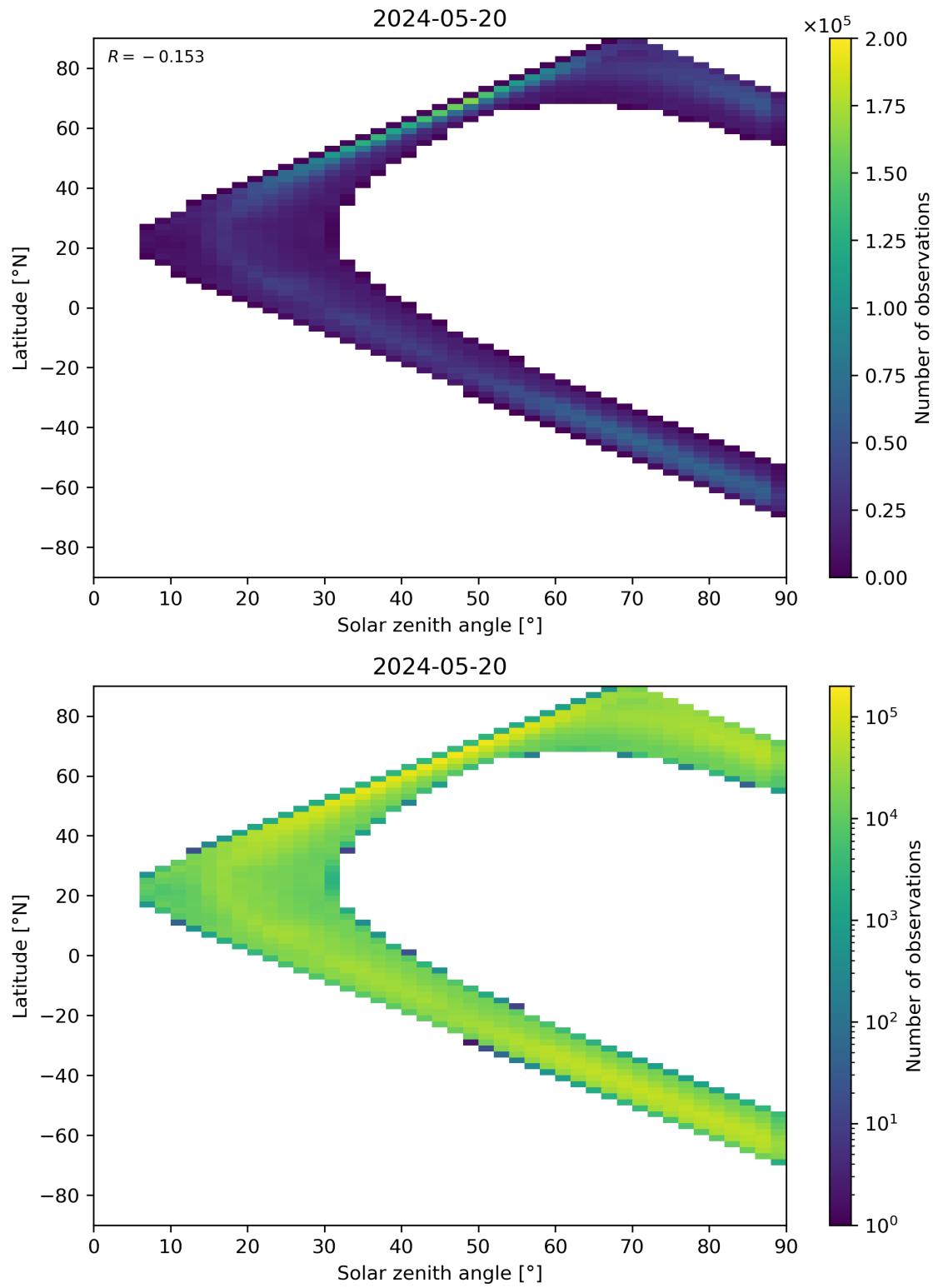
Figure 105: Scatter density plot of “Solar zenith angle” against “Latitude” for 2024-05-19 to 2024-05-21.
