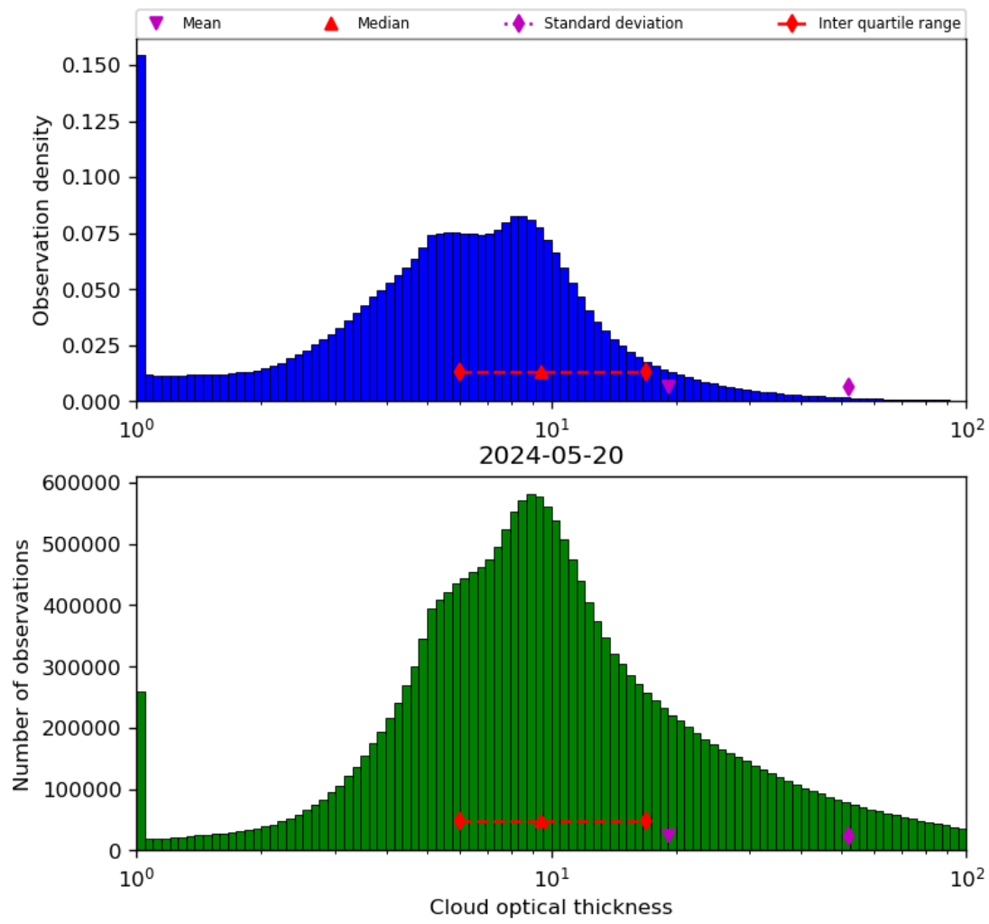
Figure 41: Histogram of “Cloud optical thickness” for 2024-05-19 to 2024-05-21
