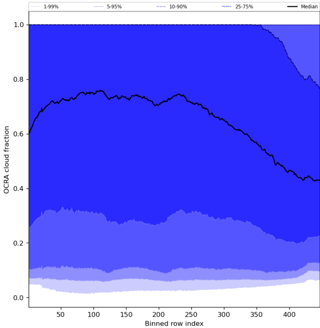
Figure 66: Along track statistics of “OCRA cloud fraction” for 2024-05-19 to 2024-05-21
