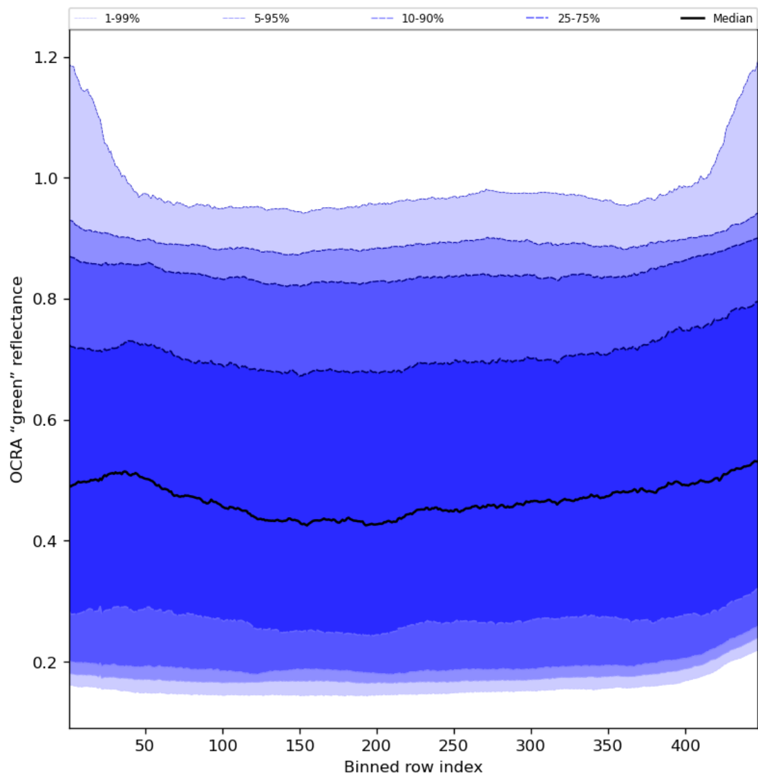
Figure 68: Along track statistics of “OCRA “green” reflectance” for 2024-05-19 to 2024-05-21
