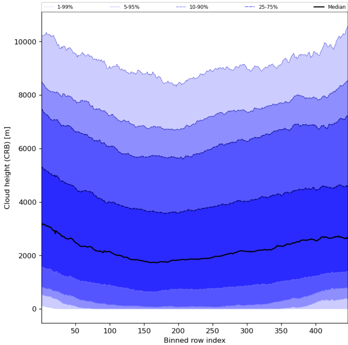
Figure 59: Along track statistics of “Cloud height (CRB)” for 2024-05-19 to 2024-05-21
