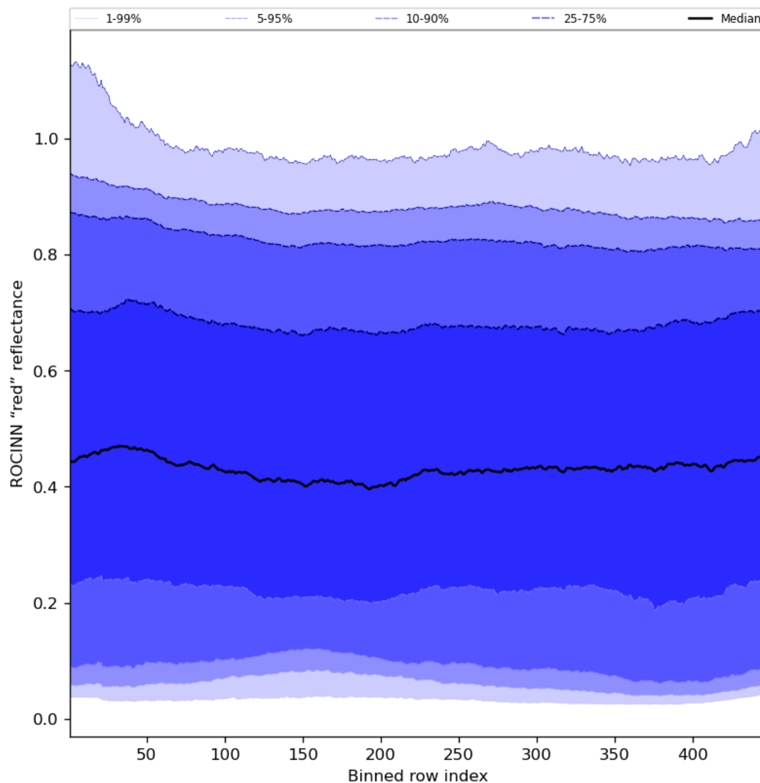
Figure 69: Along track statistics of "ROCINN "red" reflectance" for 2024-05-19 to 2024-05-21
