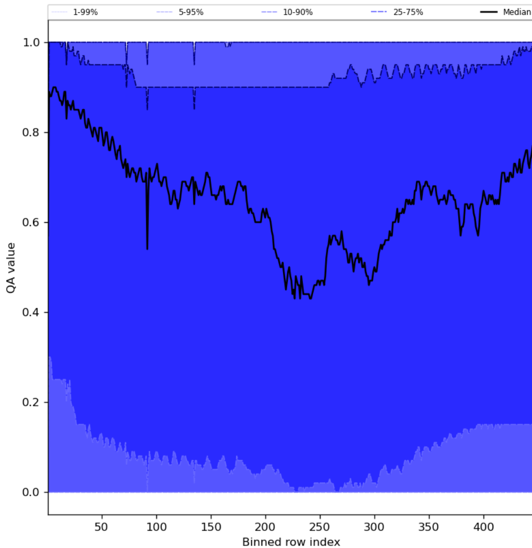
Figure 54: Along track statistics of “QA value” for 2024-05-19 to 2024-05-21
