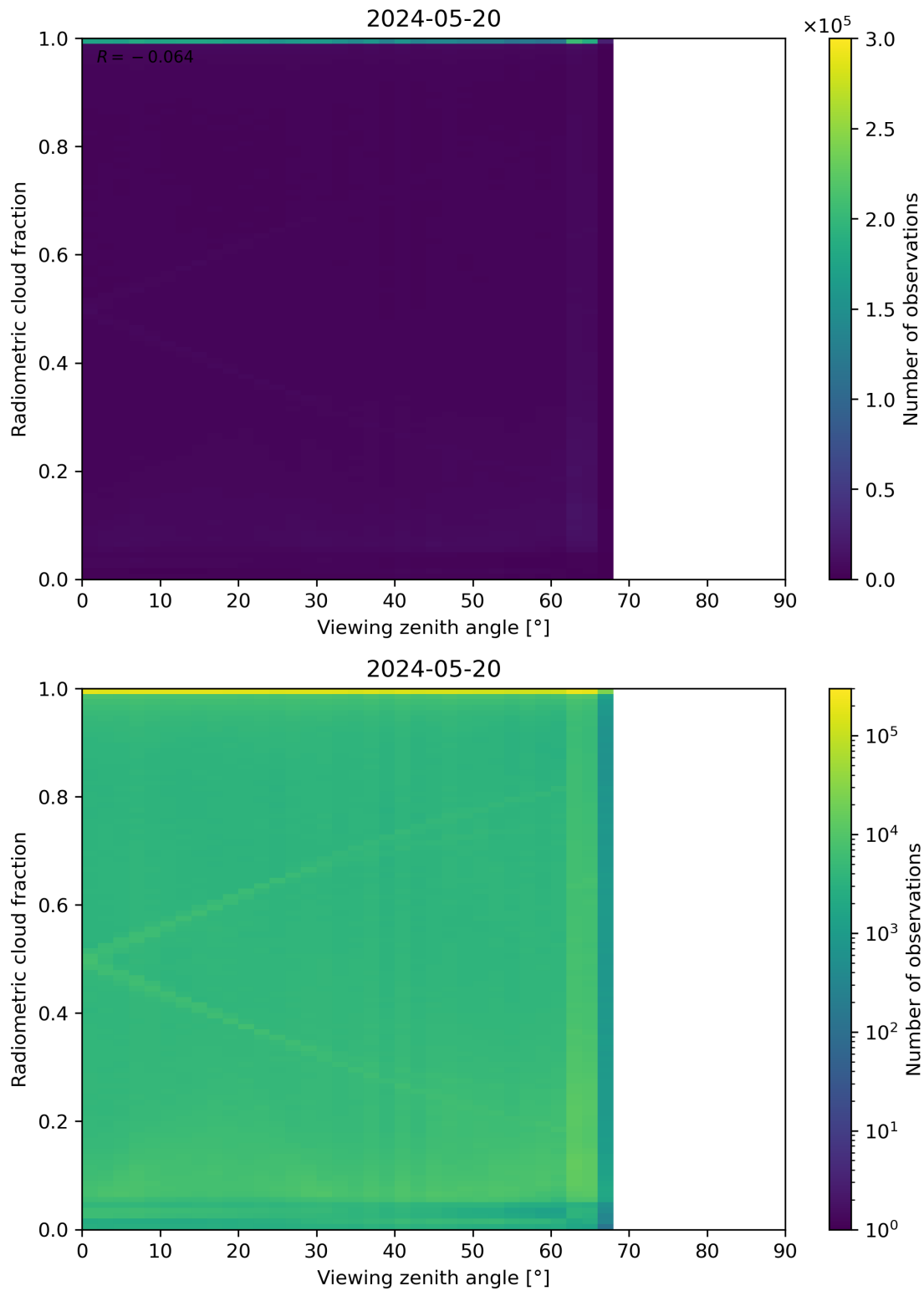
Figure 107: Scatter density plot of “Viewing zenith angle” against “Radiometric cloud fraction” for 2024-05-19 to 2024-05-21.
