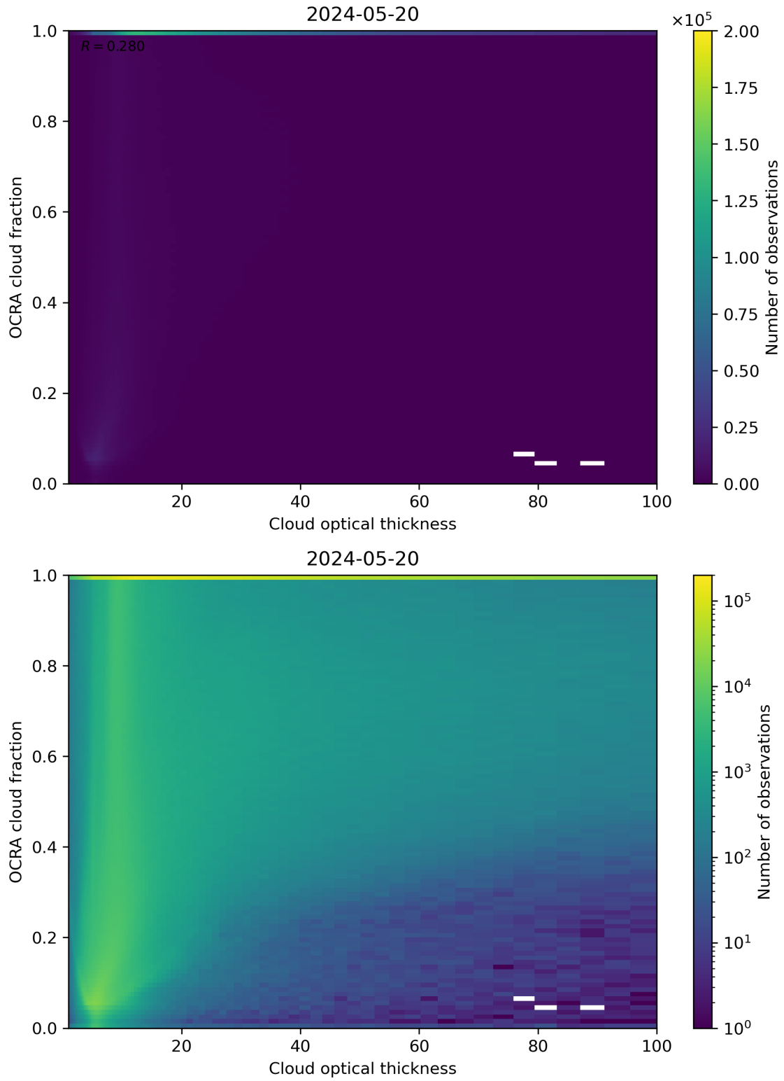
Figure 83: Scatter density plot of “Cloud optical thickness” against “OCRA cloud fraction” for 2024-05-19 to 2024-05-21.
