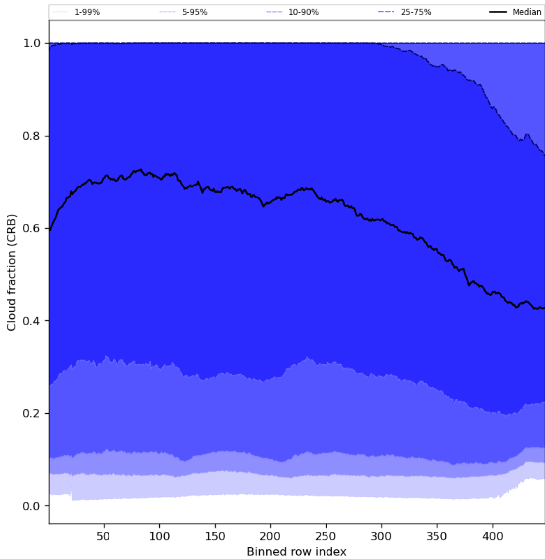
Figure 58: Along track statistics of “Cloud fraction (CRB)” for 2024-05-19 to 2024-05-21
