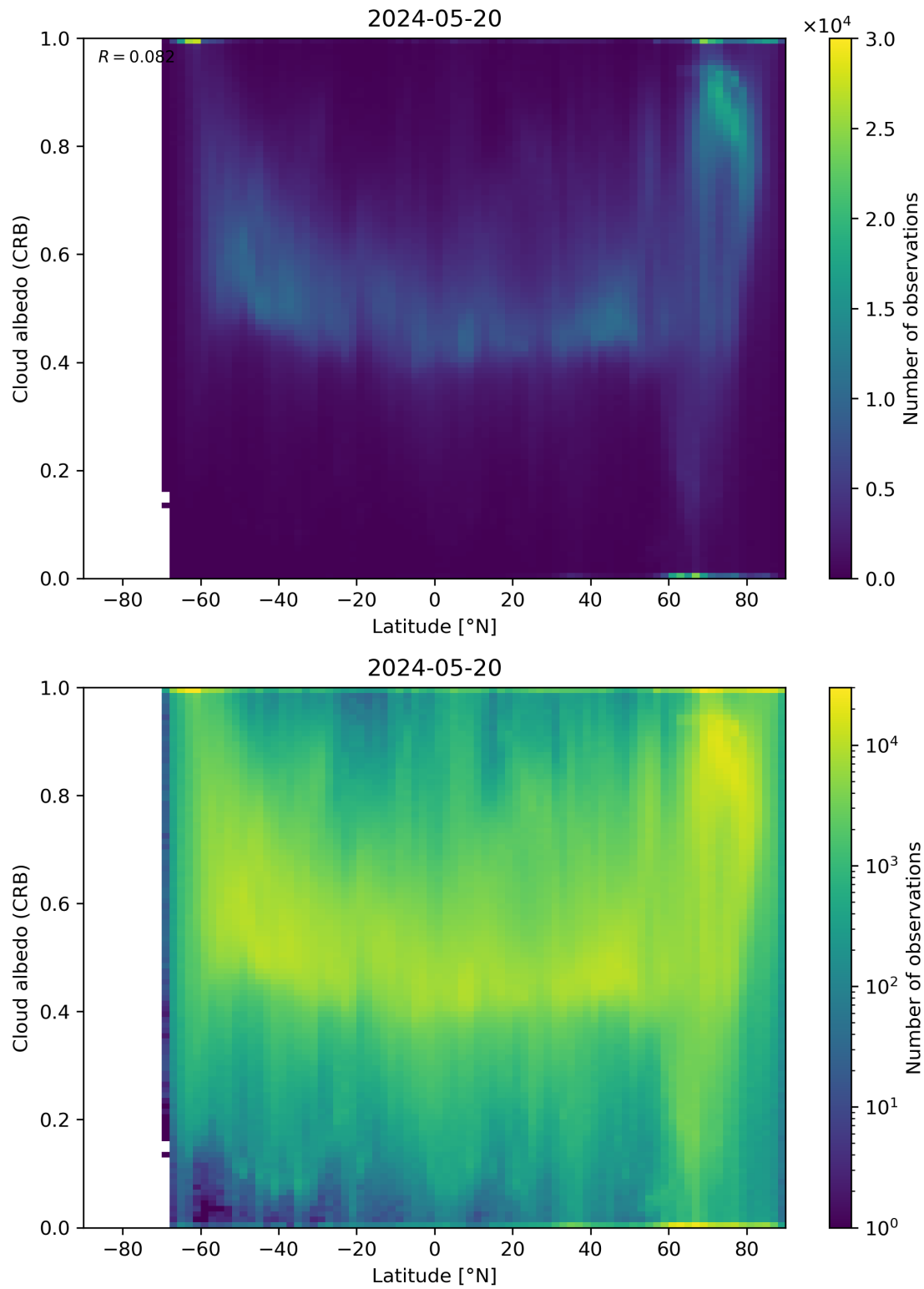
Figure 91: Scatter density plot of “Latitude” against “Cloud albedo (CRB)” for 2024-05-19 to 2024-05-21.
