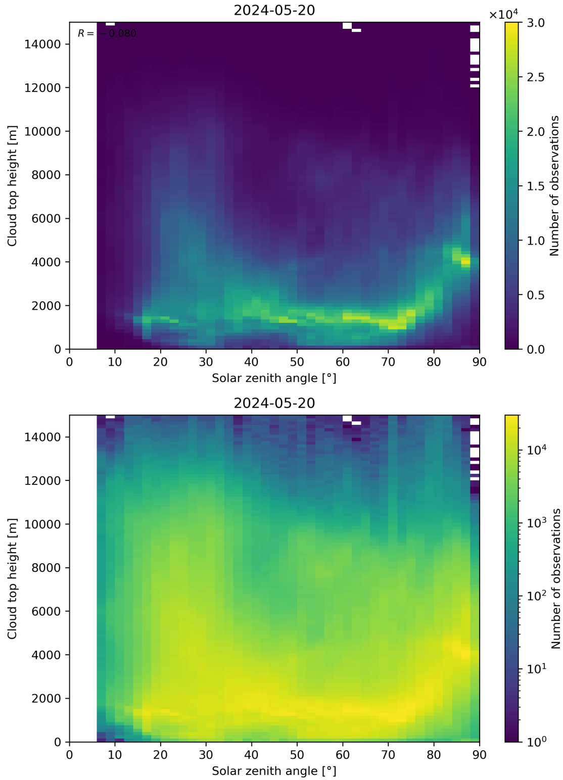
Figure 104: Scatter density plot of “Solar zenith angle” against “Cloud top height” for 2024-05-19 to 2024-05-21.
