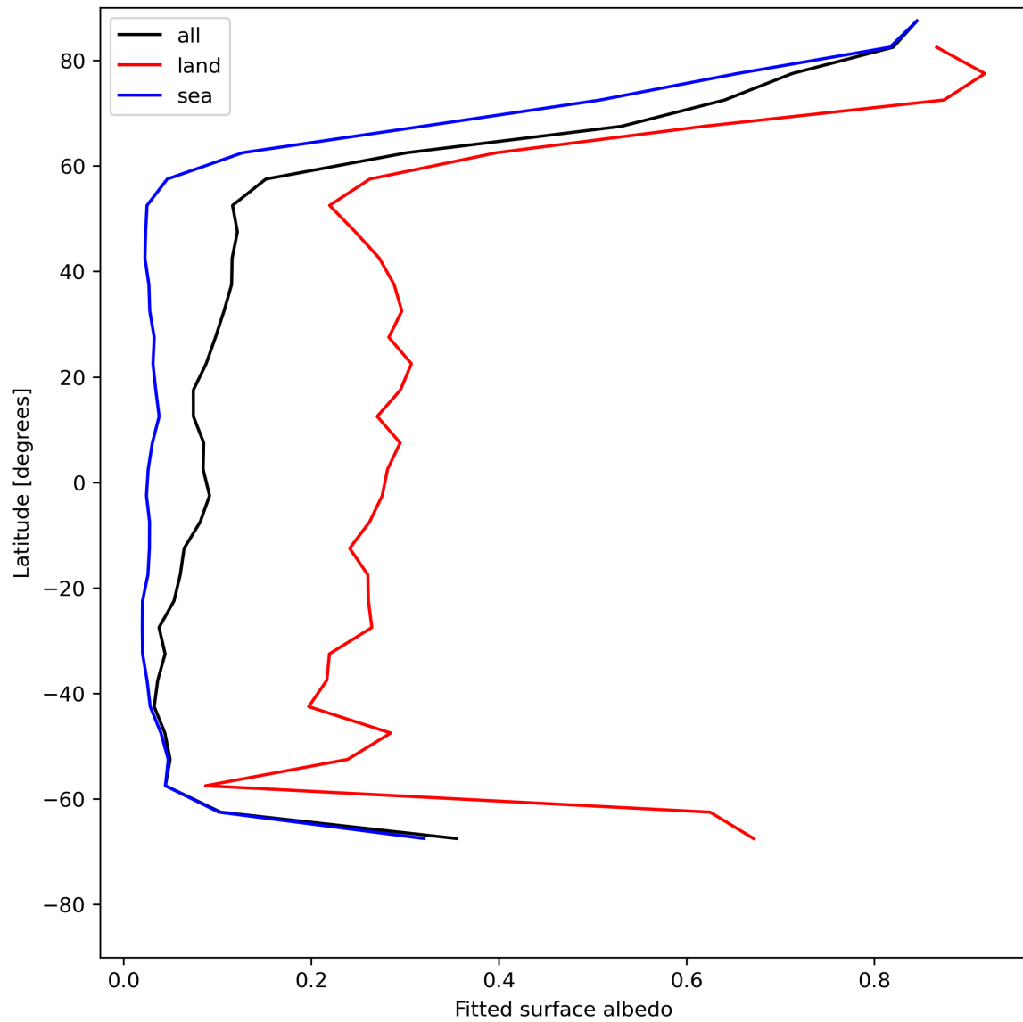
Figure 29: Zonal average of “Fitted surface albedo” for 2024-05-19 to 2024-05-21.
