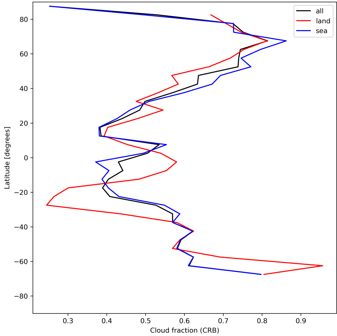
Figure 26: Zonal average of “Cloud fraction (CRB)” for 2024-05-19 to 2024-05-21.
