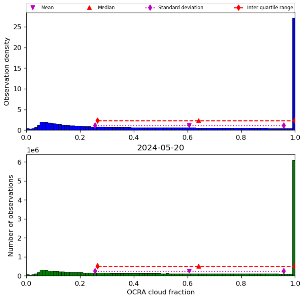
Figure 50: Histogram of “OCRA cloud fraction” for 2024-05-19 to 2024-05-21
