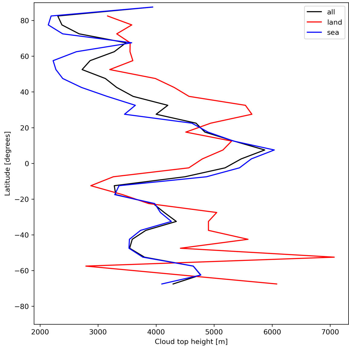
Figure 24: Zonal average of “Cloud top height” for 2024-05-19 to 2024-05-21.
