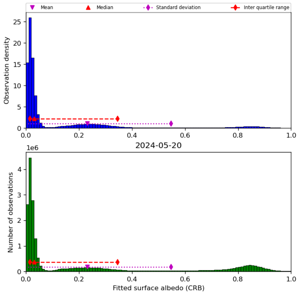
Figure 46: Histogram of “Fitted surface albedo (CRB)” for 2024-05-19 to 2024-05-21
