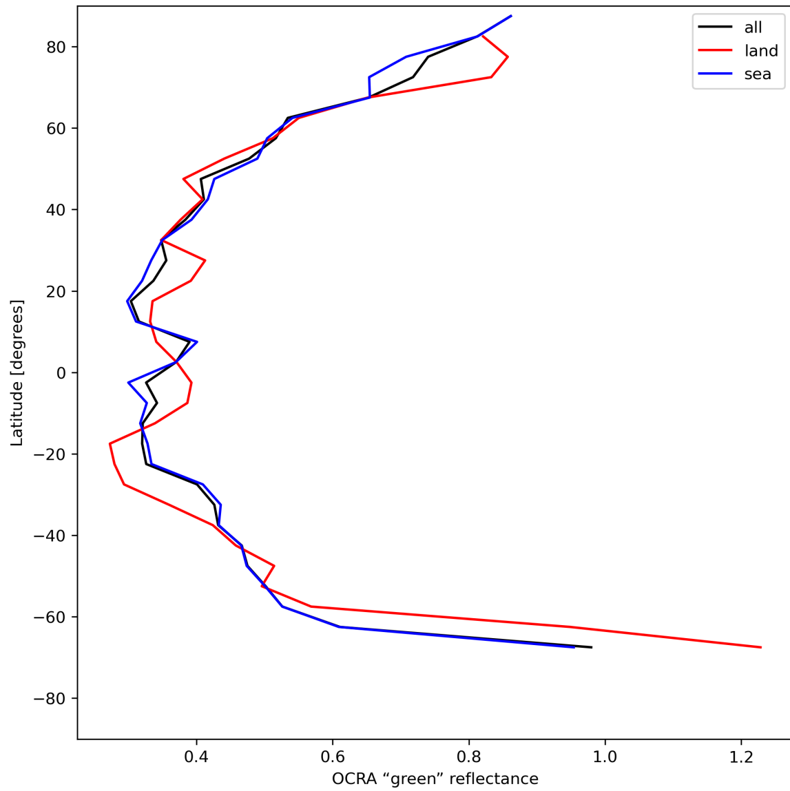
Figure 36: Zonal average of “OCRA “green” reflectance” for 2024-05-19 to 2024-05-21.
