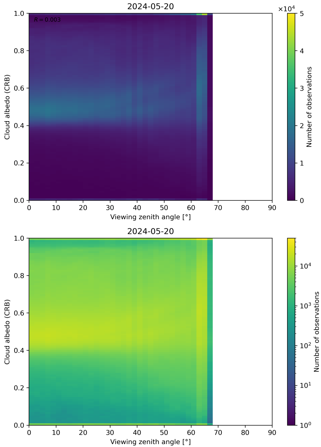
Figure 106: Scatter density plot of “Viewing zenith angle” against “Cloud albedo (CRB)” for 2024-05-19 to 2024-05-21.
