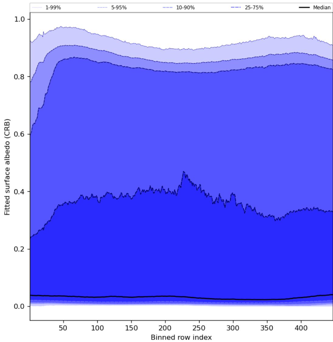
Figure 62: Along track statistics of “Fitted surface albedo (CRB)” for 2024-05-19 to 2024-05-21
