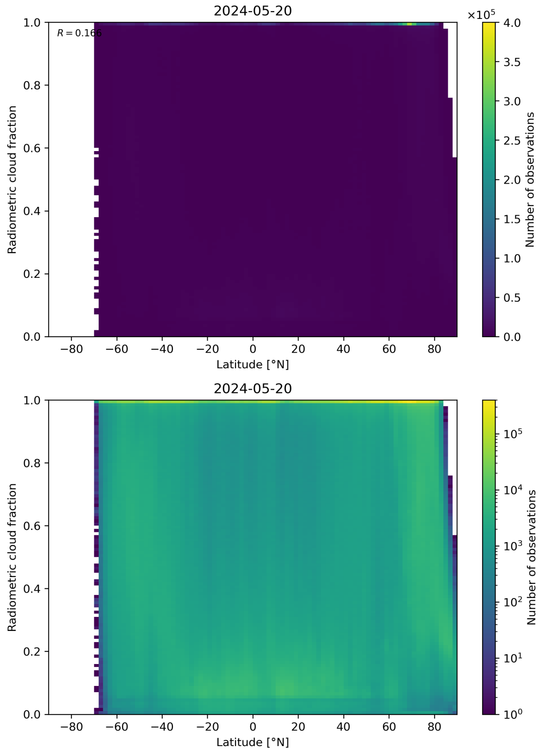
Figure 92: Scatter density plot of “Latitude” against “Radiometric cloud fraction” for 2024-05-19 to 2024-05-21.
