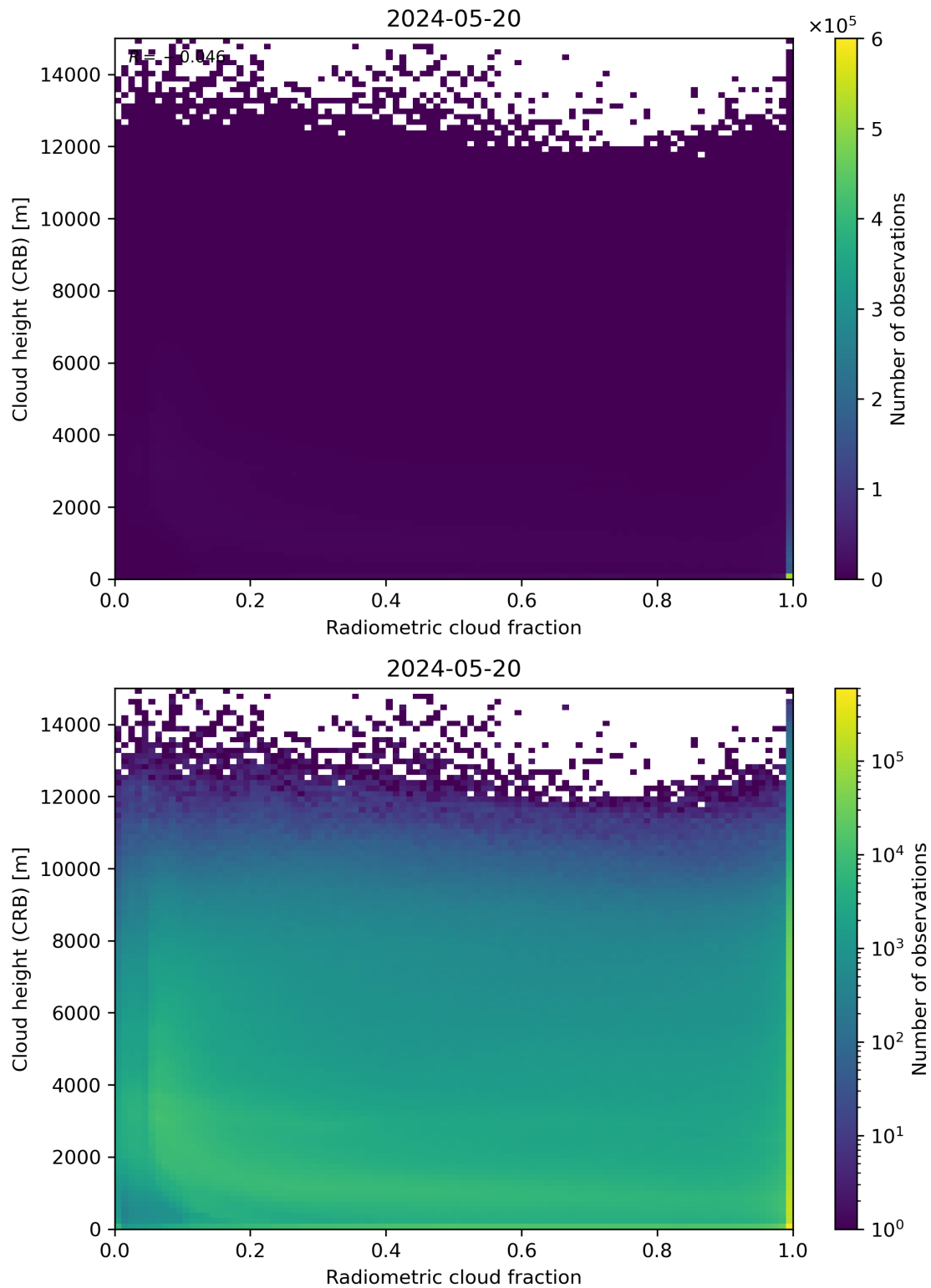
Figure 74: Scatter density plot of “Radiometric cloud fraction” against “Cloud height (CRB)” for 2024-05-19 to 2024-05-21.
