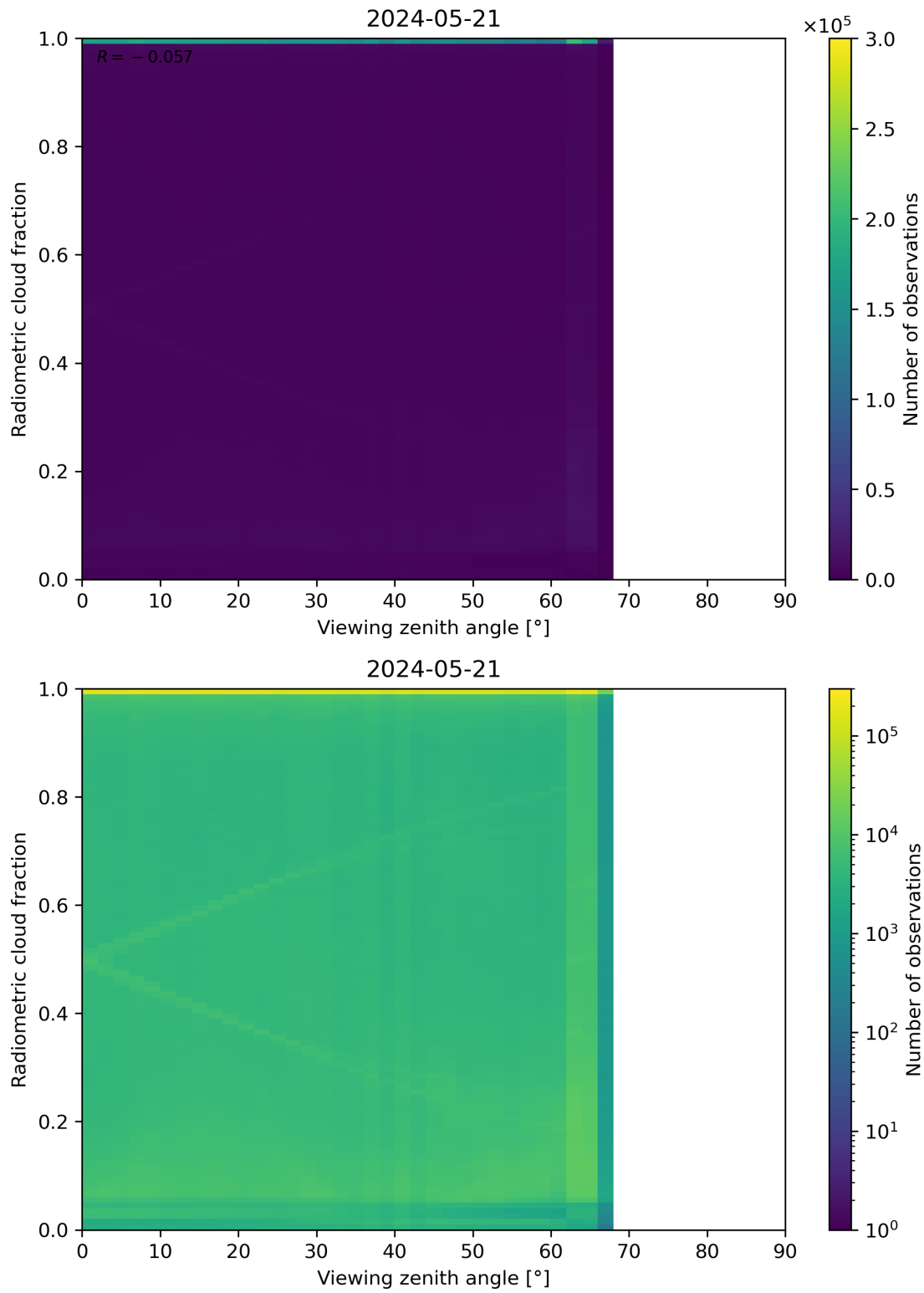
Figure 107: Scatter density plot of “Viewing zenith angle” against “Radiometric cloud fraction” for 2024-05-20 to 2024-05-22.
