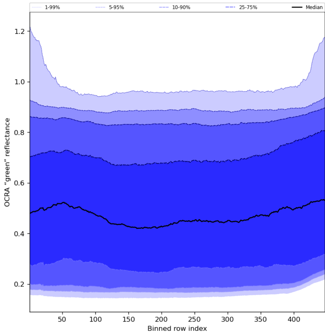
Figure 68: Along track statistics of “OCRA “green” reflectance” for 2024-05-20 to 2024-05-22
