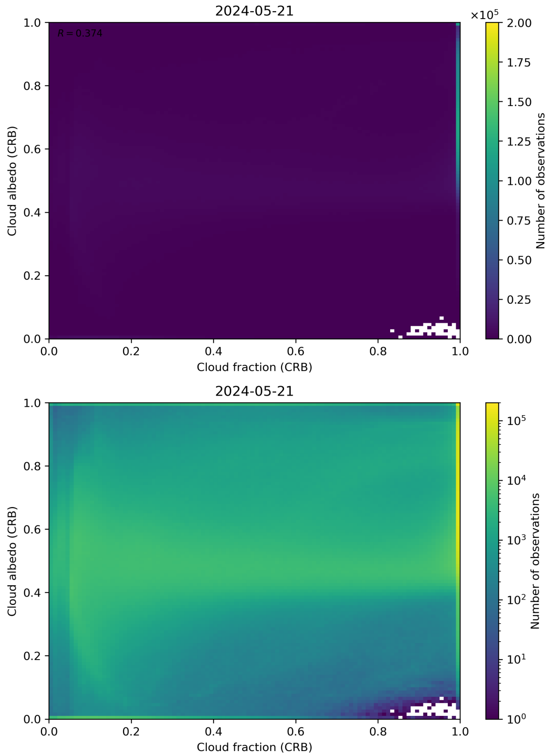
Figure 77: Scatter density plot of “Cloud fraction (CRB)” against “Cloud albedo (CRB)” for 2024-05-20 to 2024-05-22.
