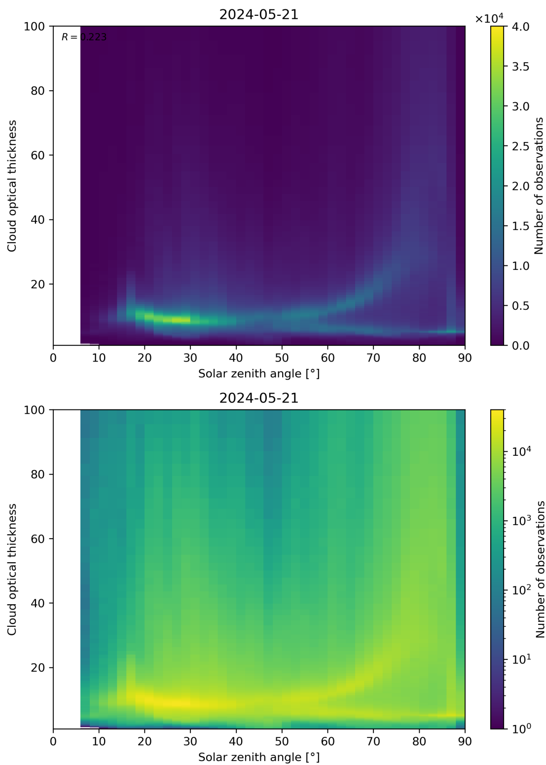
Figure 103: Scatter density plot of “Solar zenith angle” against “Cloud optical thickness” for 2024-05-20 to 2024-05-22.
