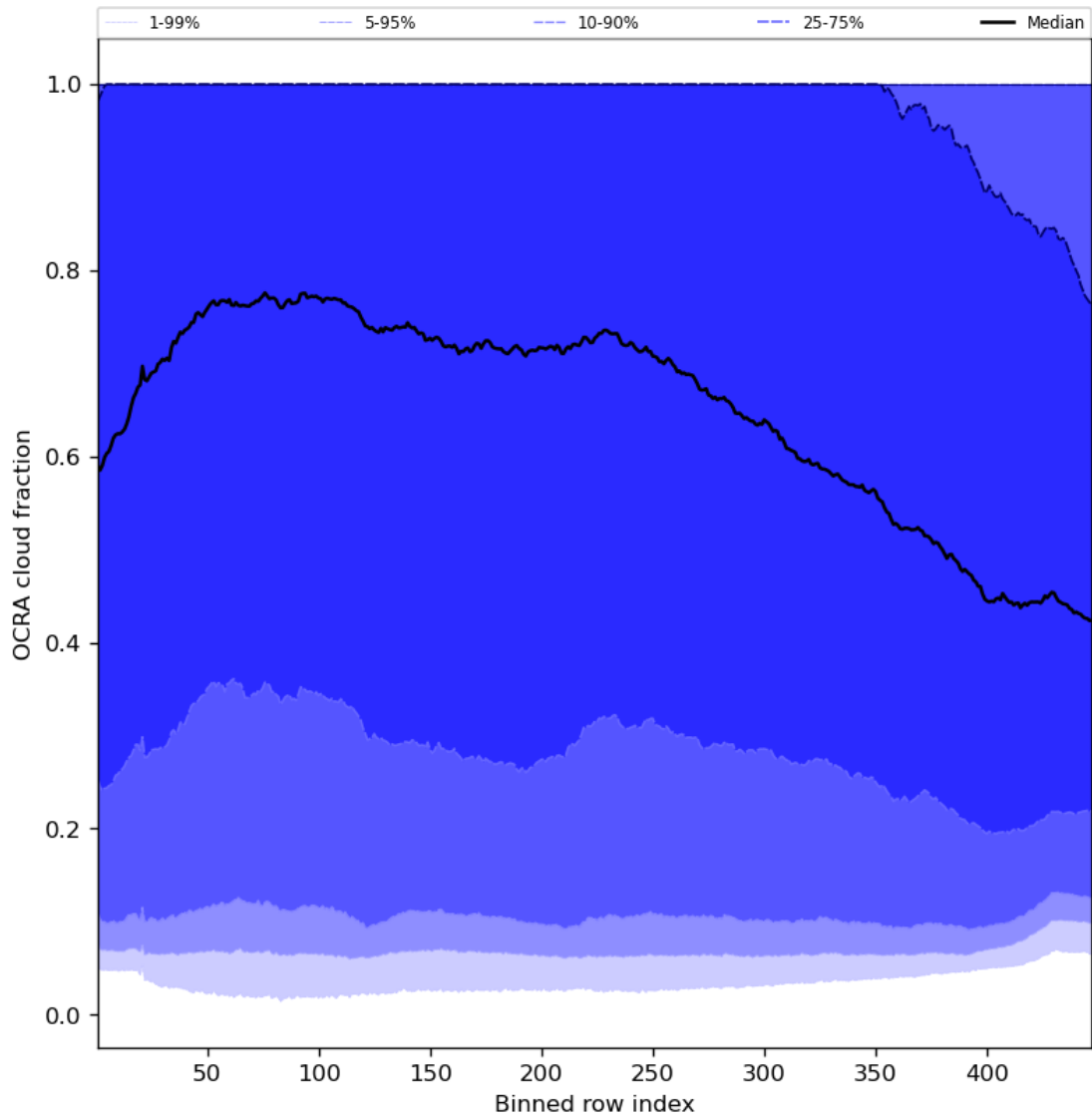
Figure 66: Along track statistics of “OCRA cloud fraction” for 2024-05-20 to 2024-05-22
