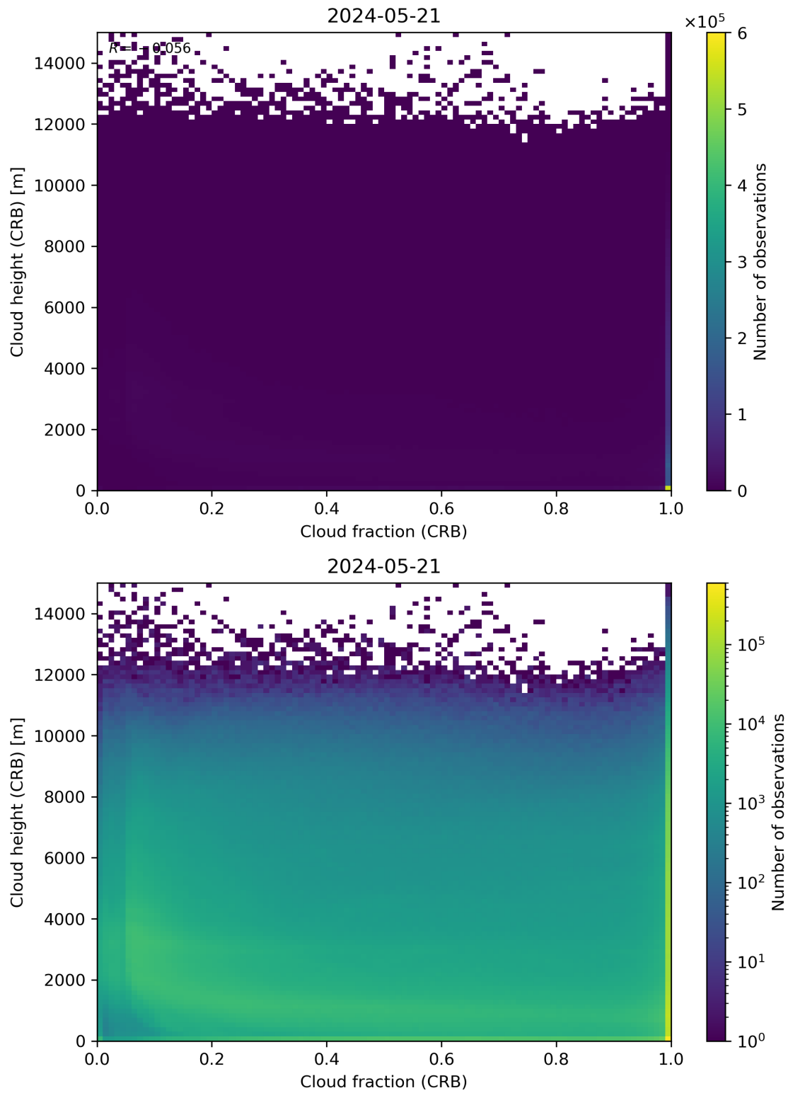
Figure 79: Scatter density plot of “Cloud fraction (CRB)” against “Cloud height (CRB)” for 2024-05-20 to 2024-05-22.
