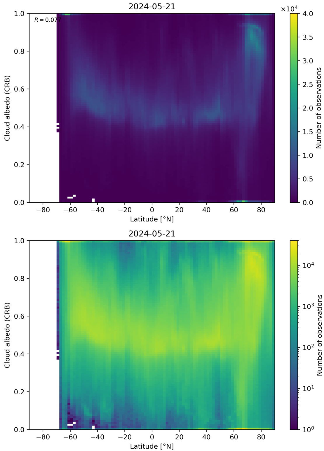
Figure 91: Scatter density plot of “Latitude” against “Cloud albedo (CRB)” for 2024-05-20 to 2024-05-22.
