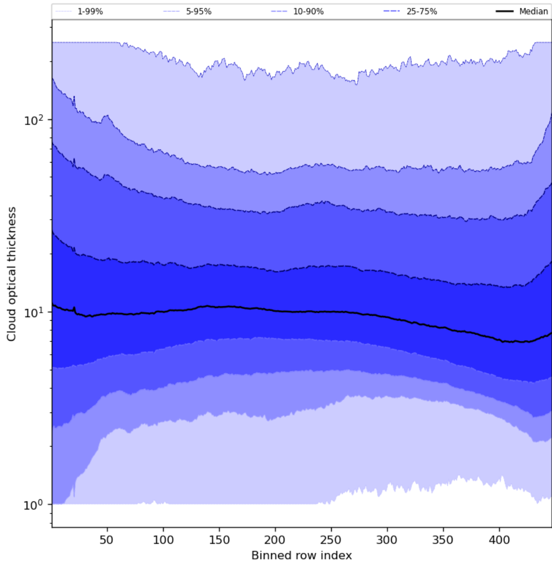
Figure 57: Along track statistics of “Cloud optical thickness” for 2024-05-20 to 2024-05-22
