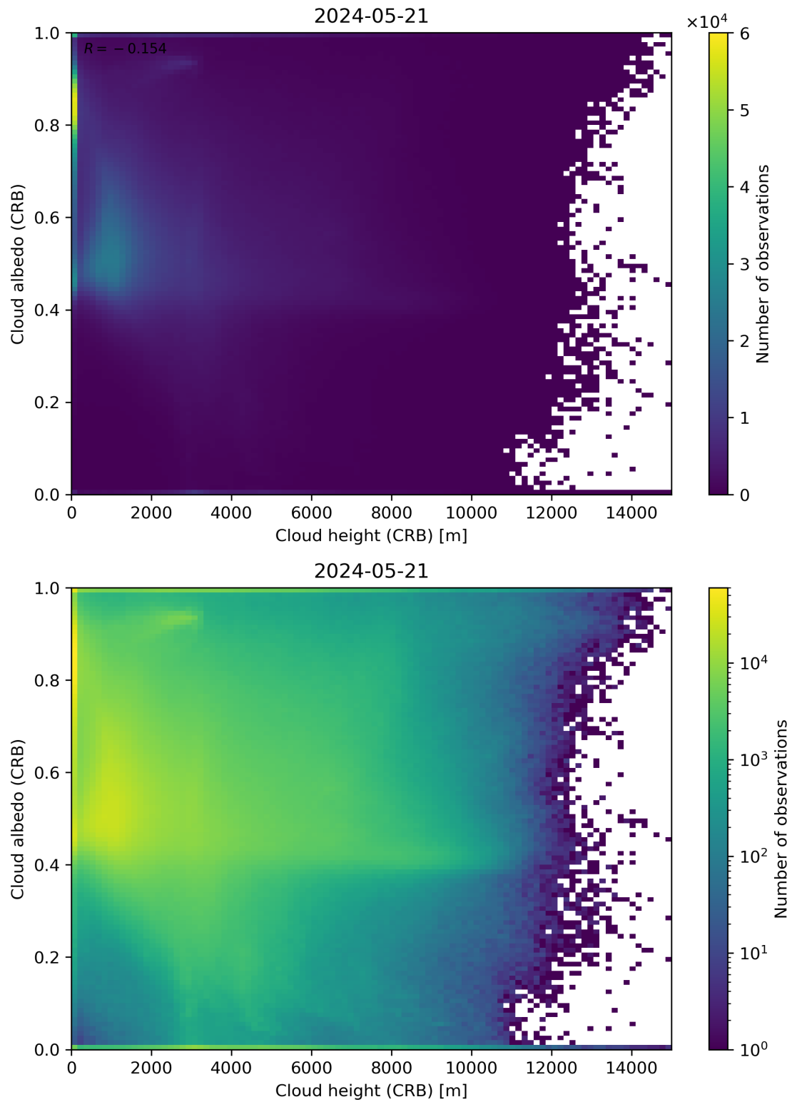
Figure 80: Scatter density plot of “Cloud height (CRB)” against “Cloud albedo (CRB)” for 2024-05-20 to 2024-05-22.
