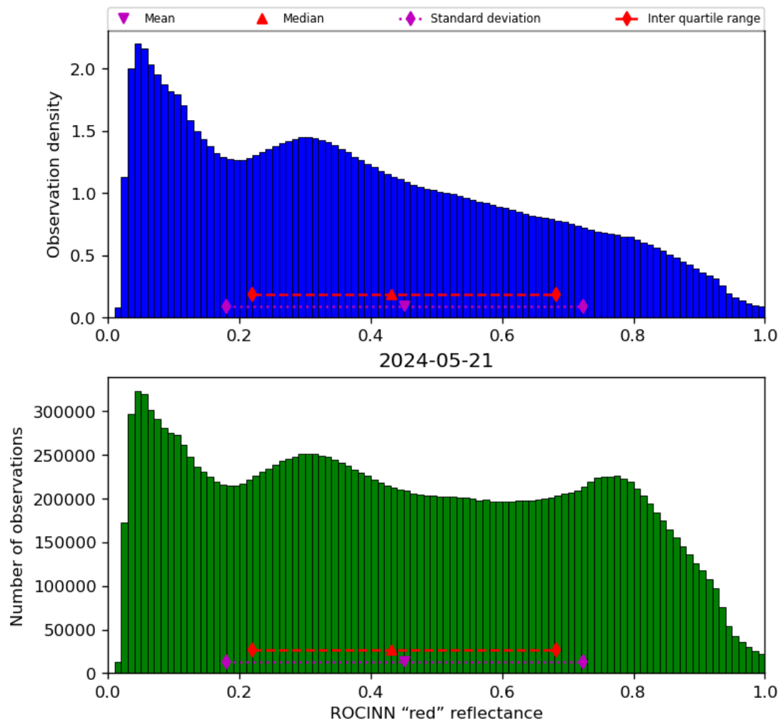
Figure 53: Histogram of “ROCINN “red” reflectance” for 2024-05-20 to 2024-05-22
