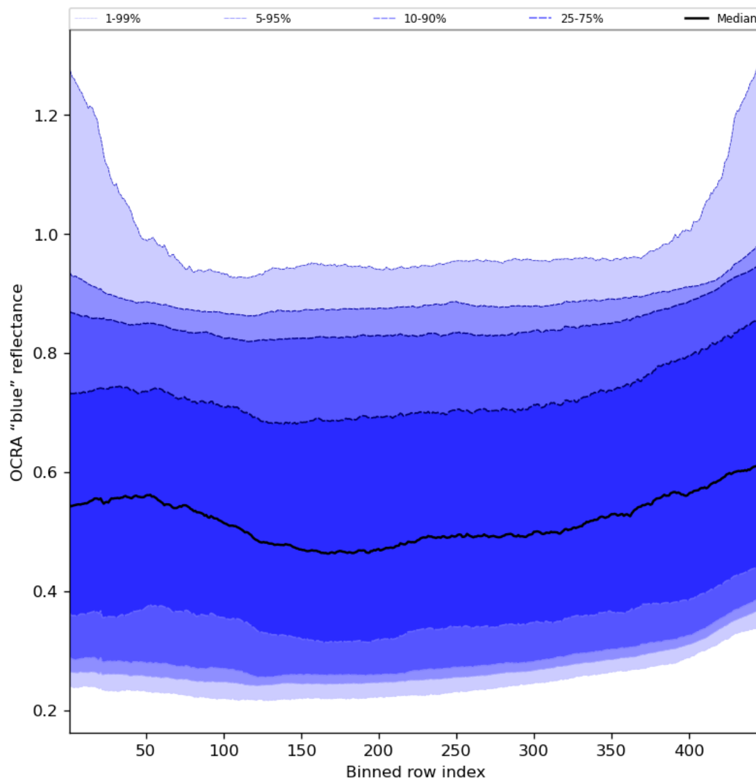
Figure 67: Along track statistics of “OCRA “blue” reflectance” for 2024-05-20 to 2024-05-22
