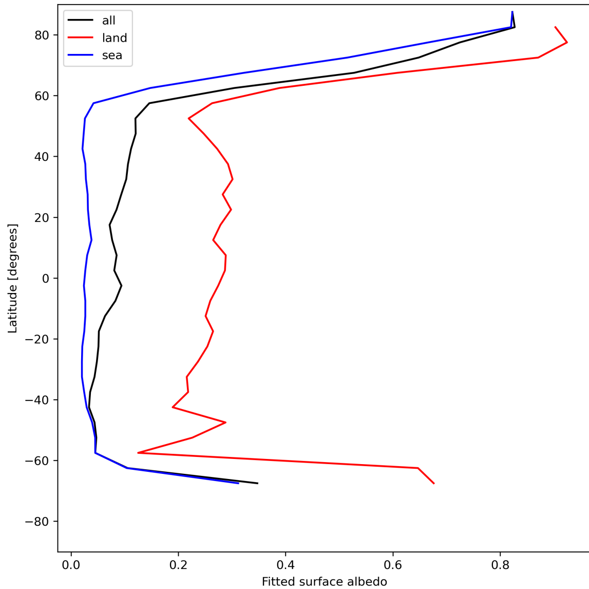
Figure 29: Zonal average of “Fitted surface albedo” for 2024-05-20 to 2024-05-22.
