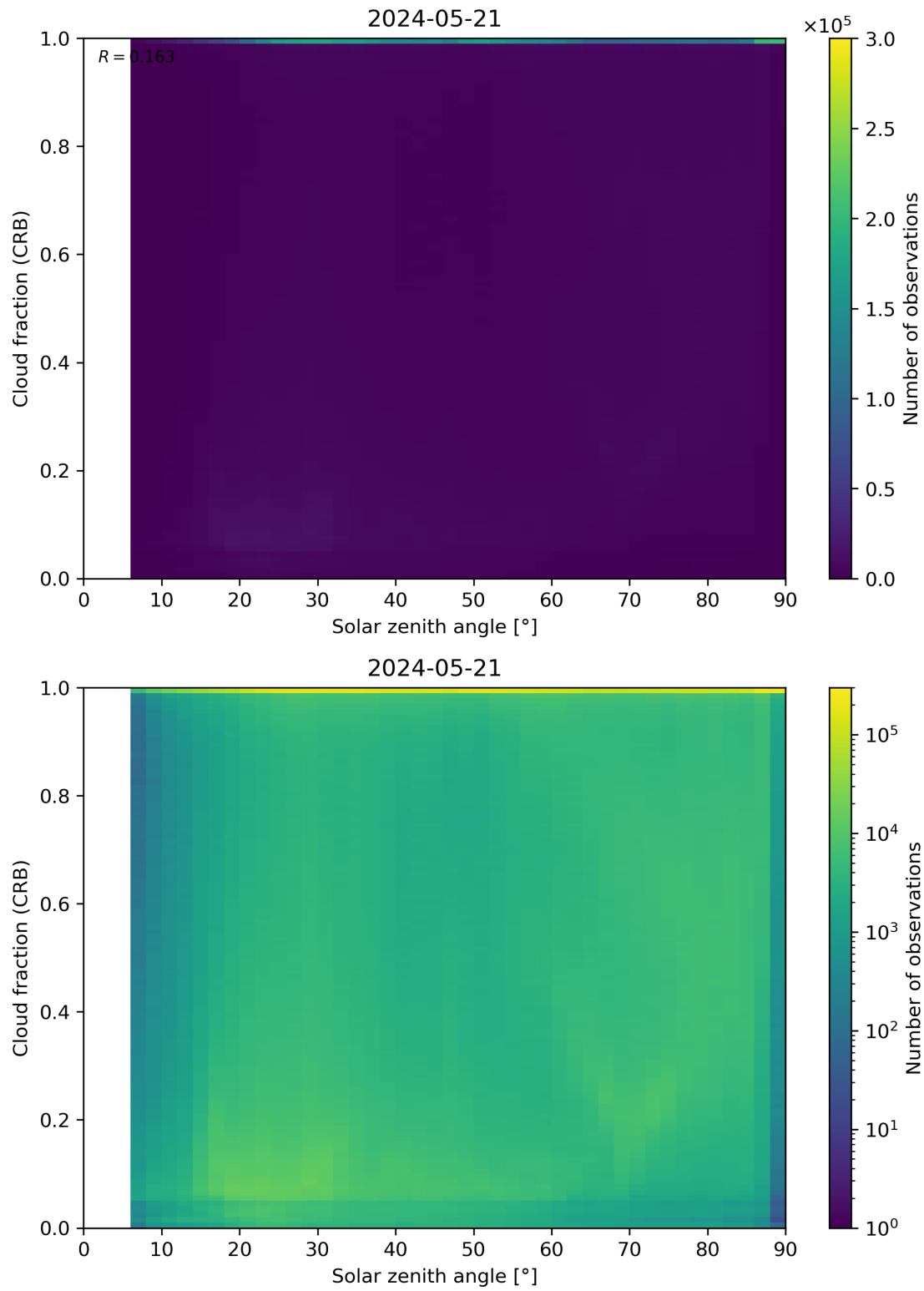
Figure 101: Scatter density plot of “Solar zenith angle” against “Cloud fraction (CRB)” for 2024-05-20 to 2024-05-22.
