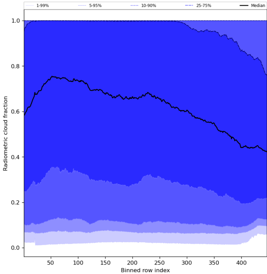
Figure 55: Along track statistics of “Radiometric cloud fraction” for 2024-05-20 to 2024-05-22
