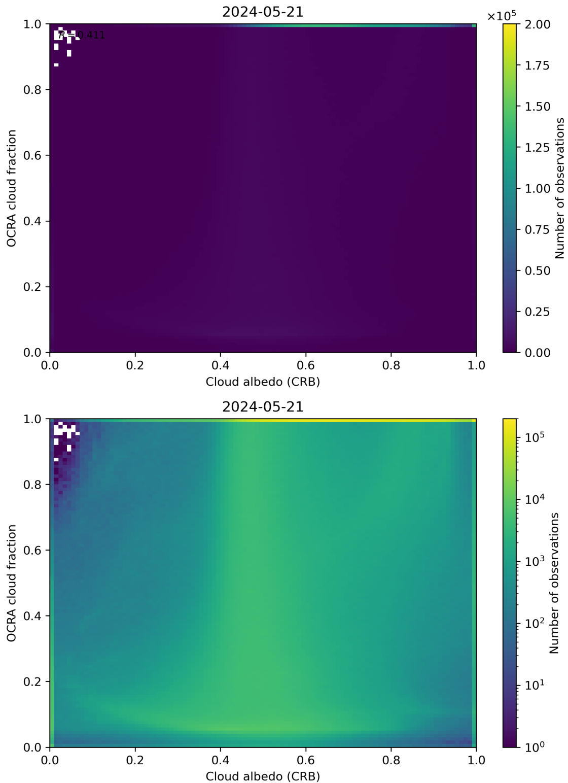
Figure 70: Scatter density plot of “Cloud albedo (CRB)” against “OCRA cloud fraction” for 2024-05-20 to 2024-05-22.
