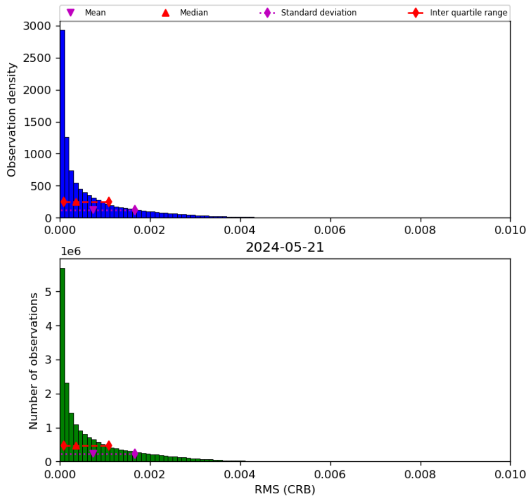
Figure 48: Histogram of “RMS (CRB)” for 2024-05-20 to 2024-05-22
