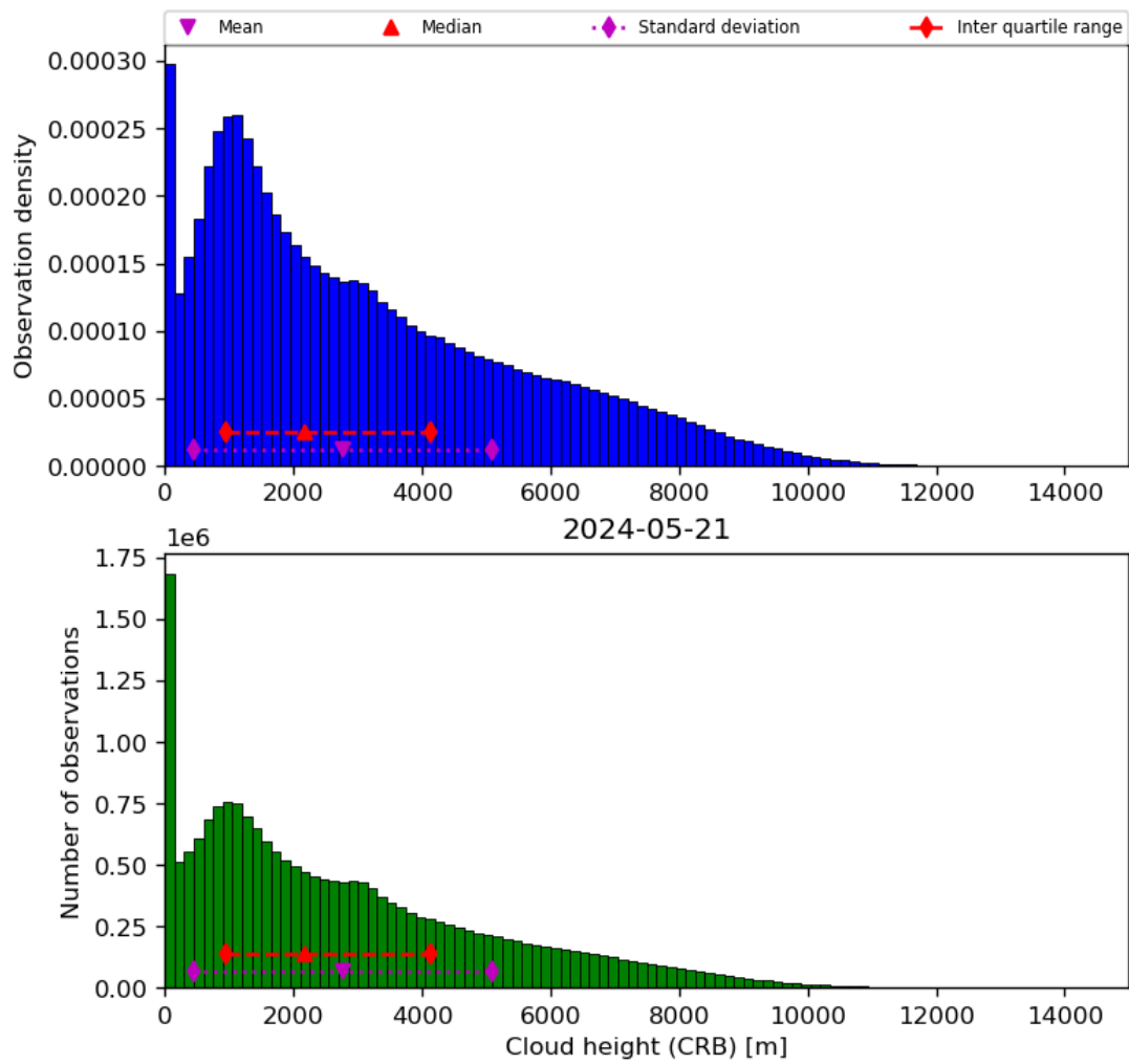
Figure 43: Histogram of “Cloud height (CRB)” for 2024-05-20 to 2024-05-22
