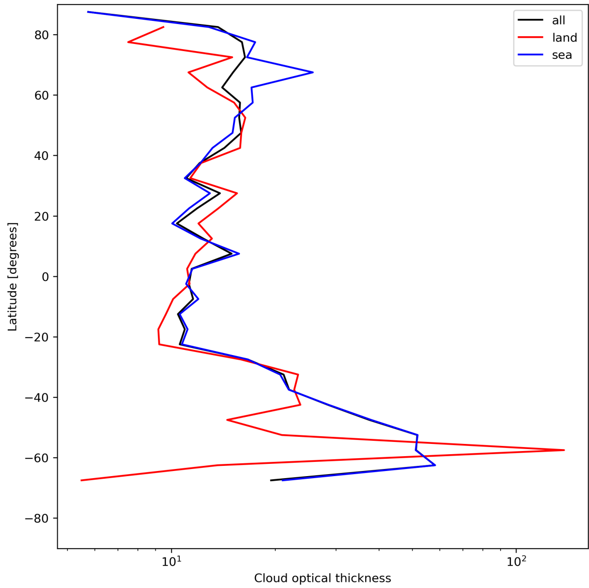
Figure 25: Zonal average of “Cloud optical thickness” for 2024-05-20 to 2024-05-22.
