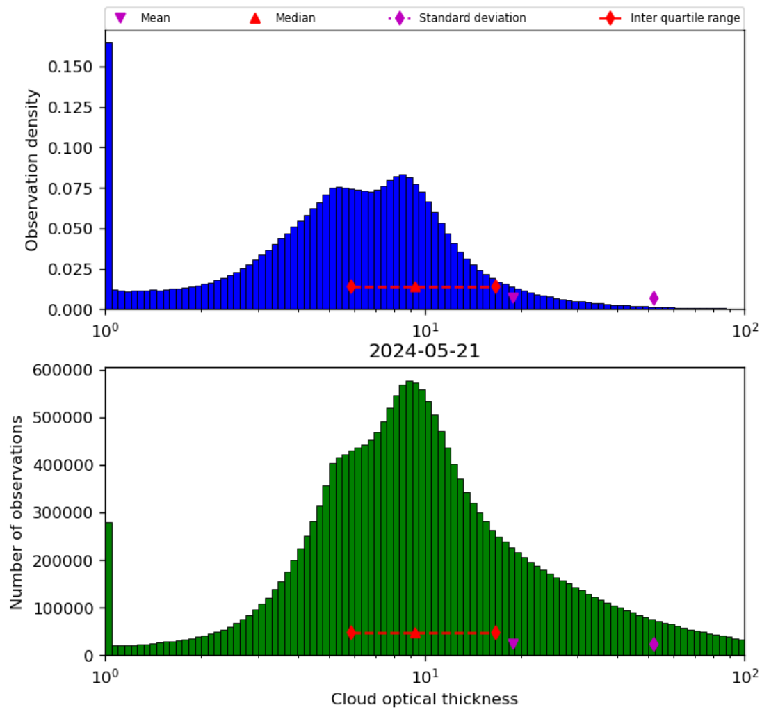
Figure 41: Histogram of “Cloud optical thickness” for 2024-05-20 to 2024-05-22
