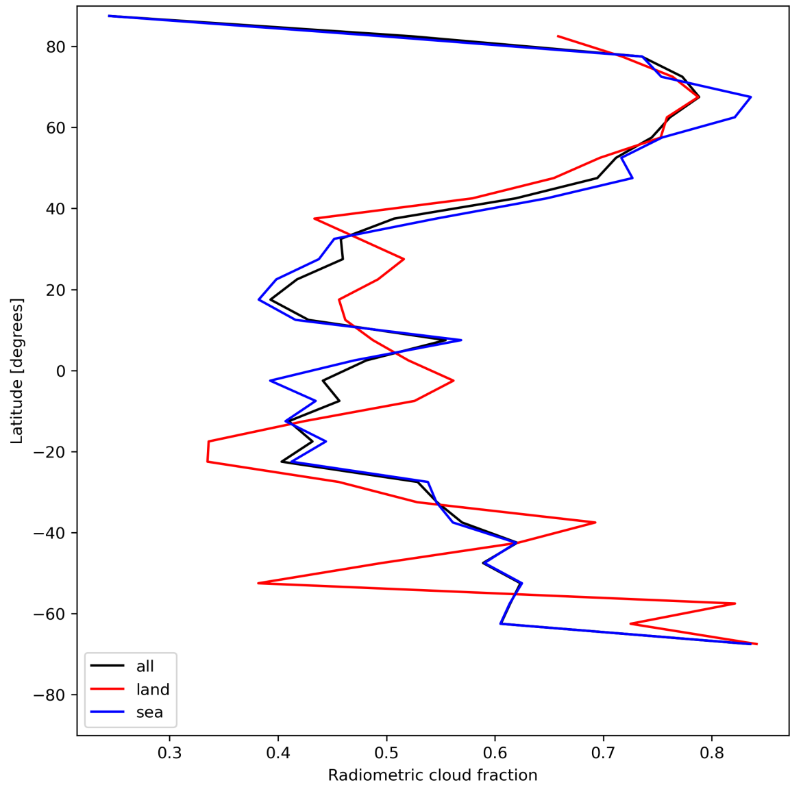
Figure 23: Zonal average of “Radiometric cloud fraction” for 2024-05-20 to 2024-05-22.
