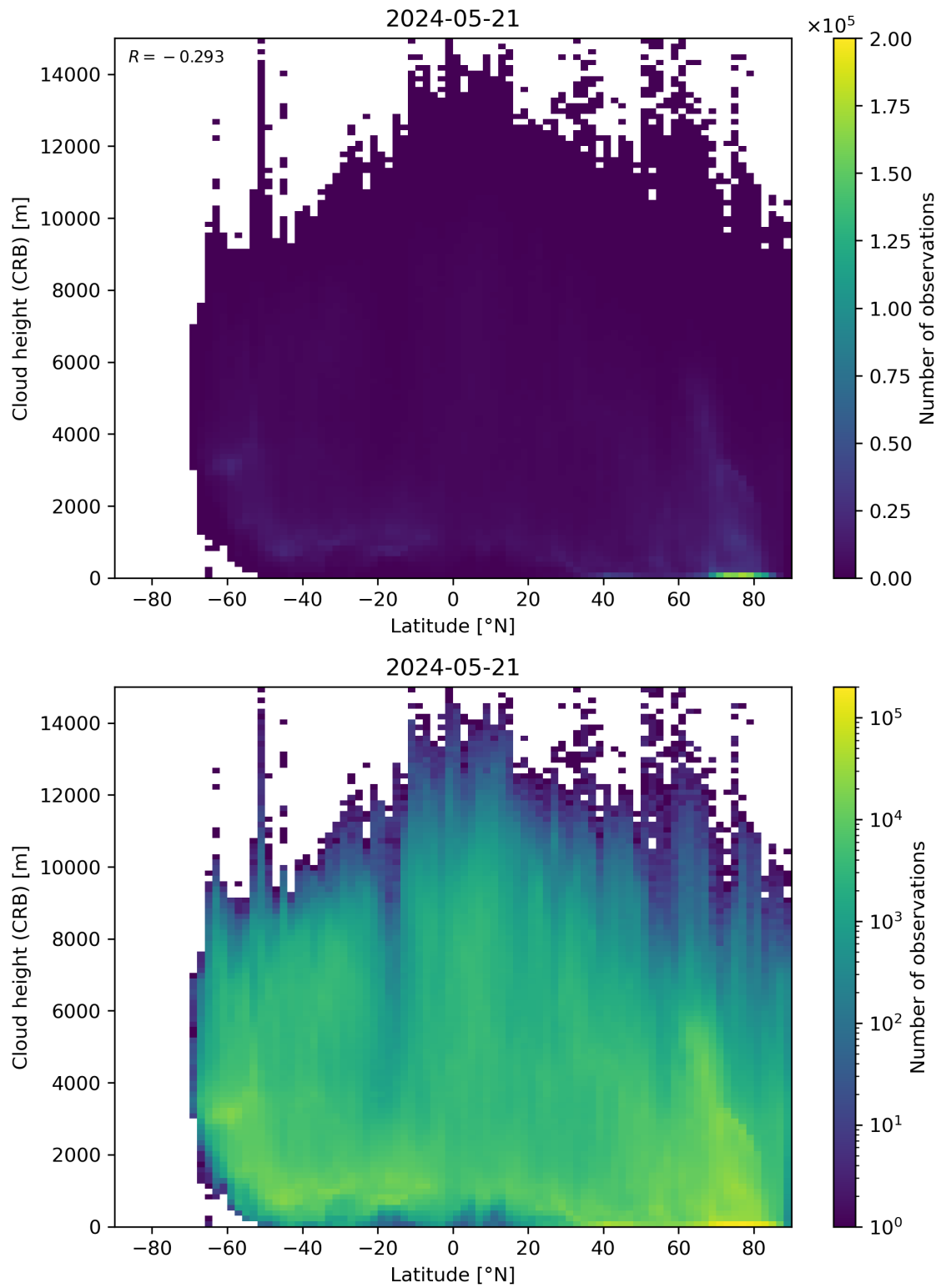
Figure 95: Scatter density plot of “Latitude” against “Cloud height (CRB)” for 2024-05-20 to 2024-05-22.
