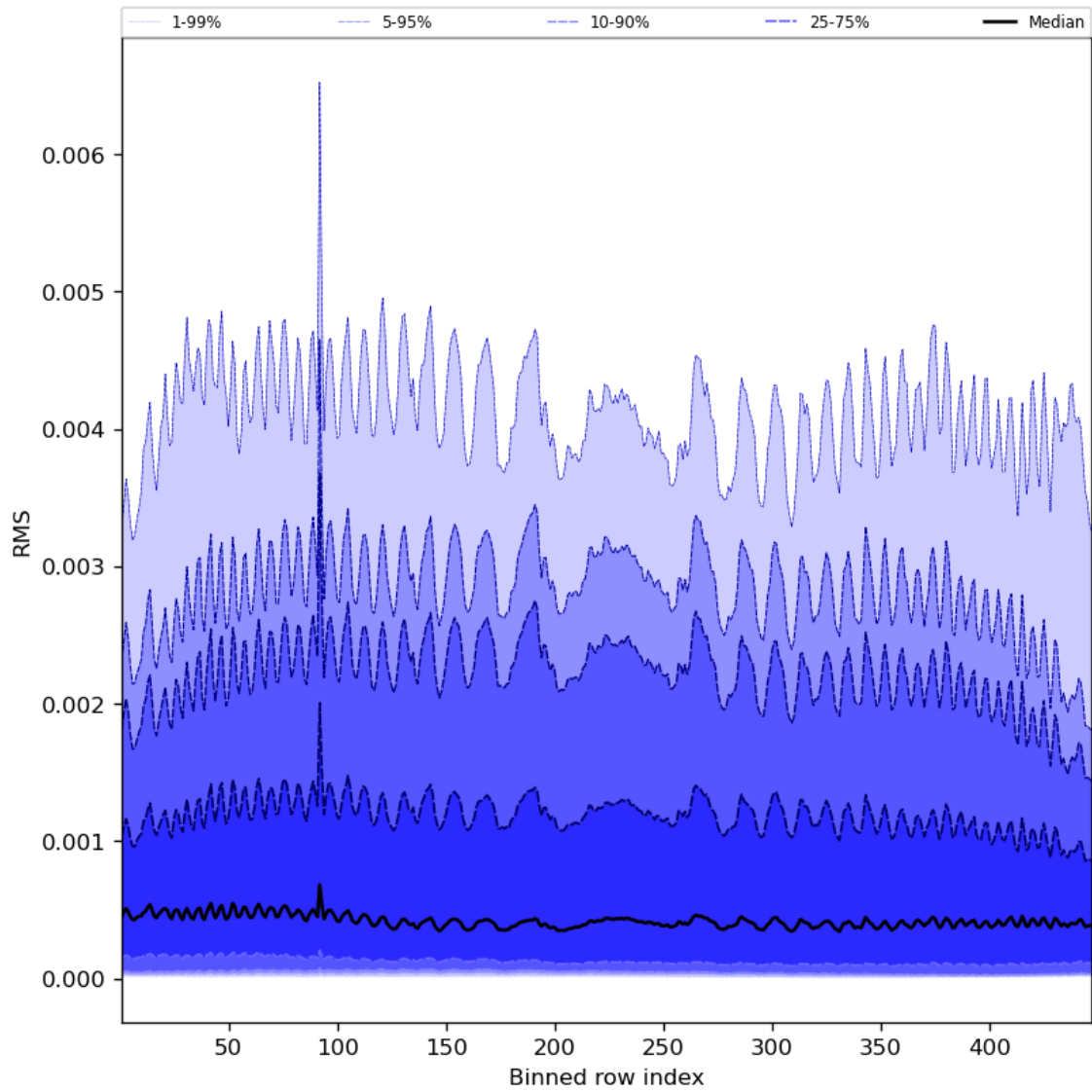
Figure 63: Along track statistics of “RMS” for 2024-05-20 to 2024-05-22
