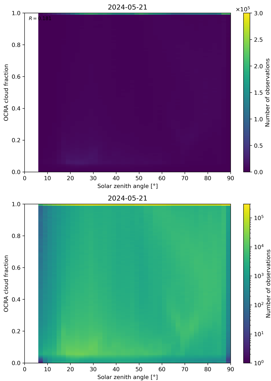
Figure 100: Scatter density plot of “Solar zenith angle” against “OCRA cloud fraction” for 2024-05-20 to 2024-05-22.
