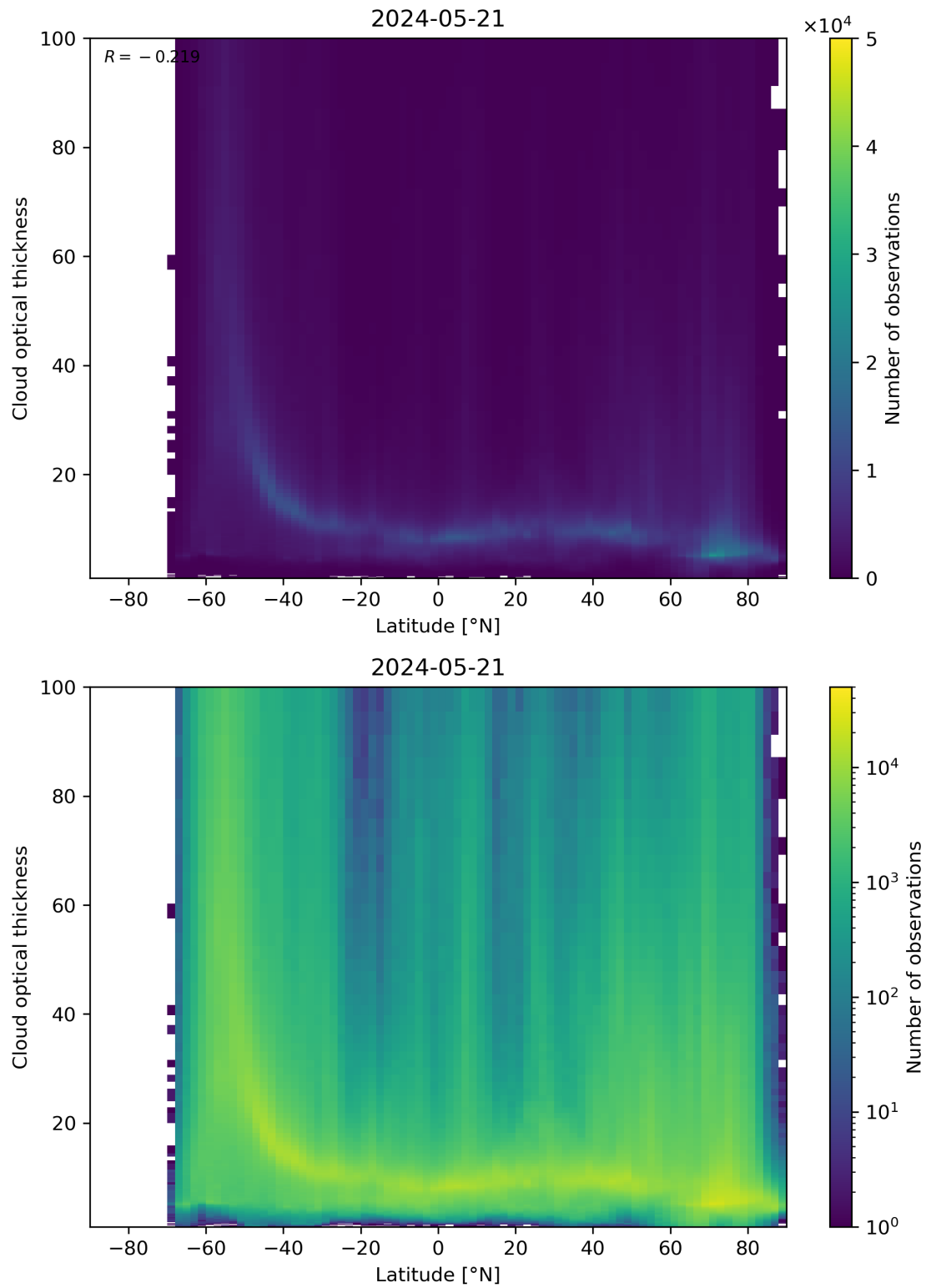
Figure 96: Scatter density plot of “Latitude” against “Cloud optical thickness” for 2024-05-20 to 2024-05-22.
