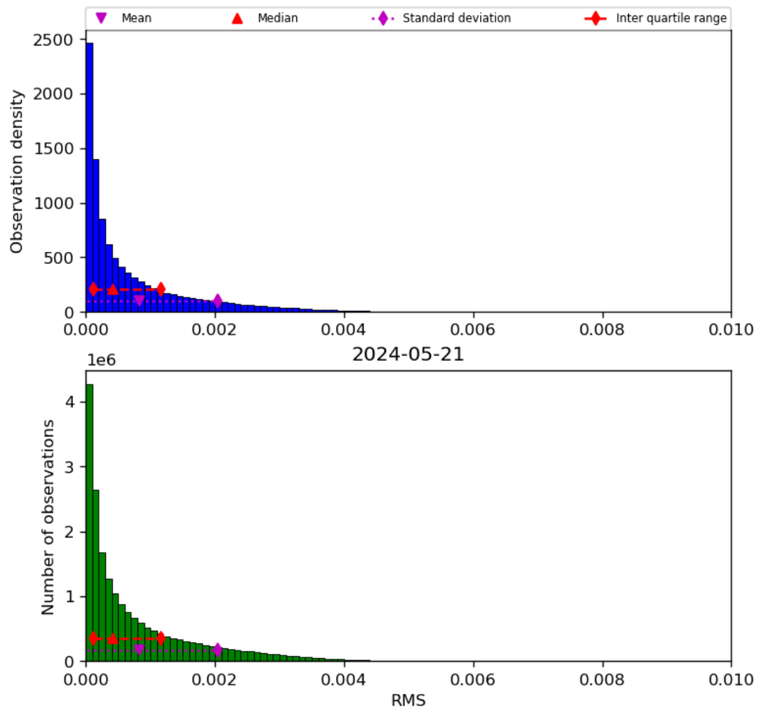
Figure 47: Histogram of “RMS” for 2024-05-20 to 2024-05-22
