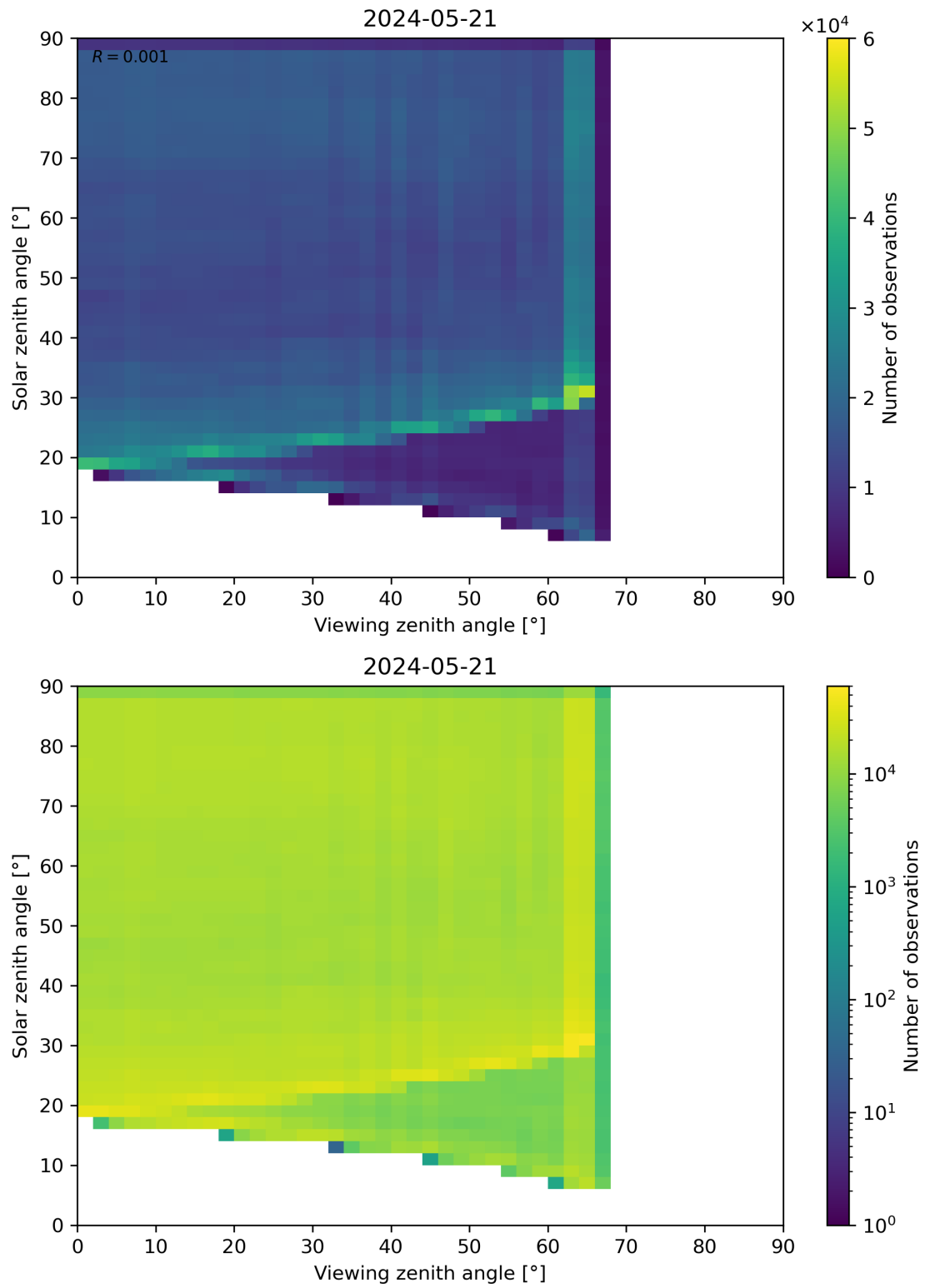
Figure 114: Scatter density plot of “Viewing zenith angle” against “Solar zenith angle” for 2024-05-20 to 2024-05-22.
