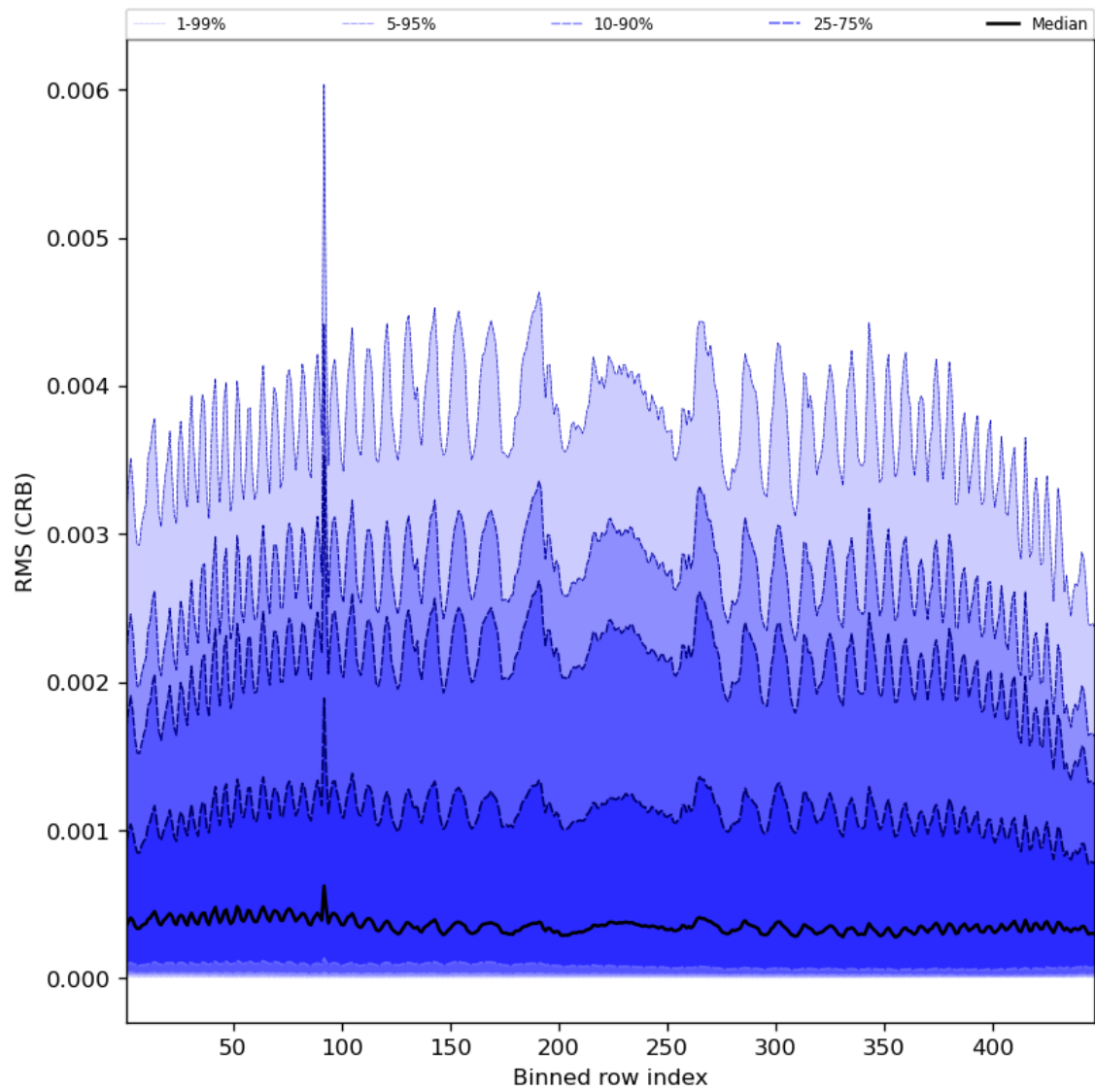
Figure 64: Along track statistics of “RMS (CRB)” for 2024-05-20 to 2024-05-22
