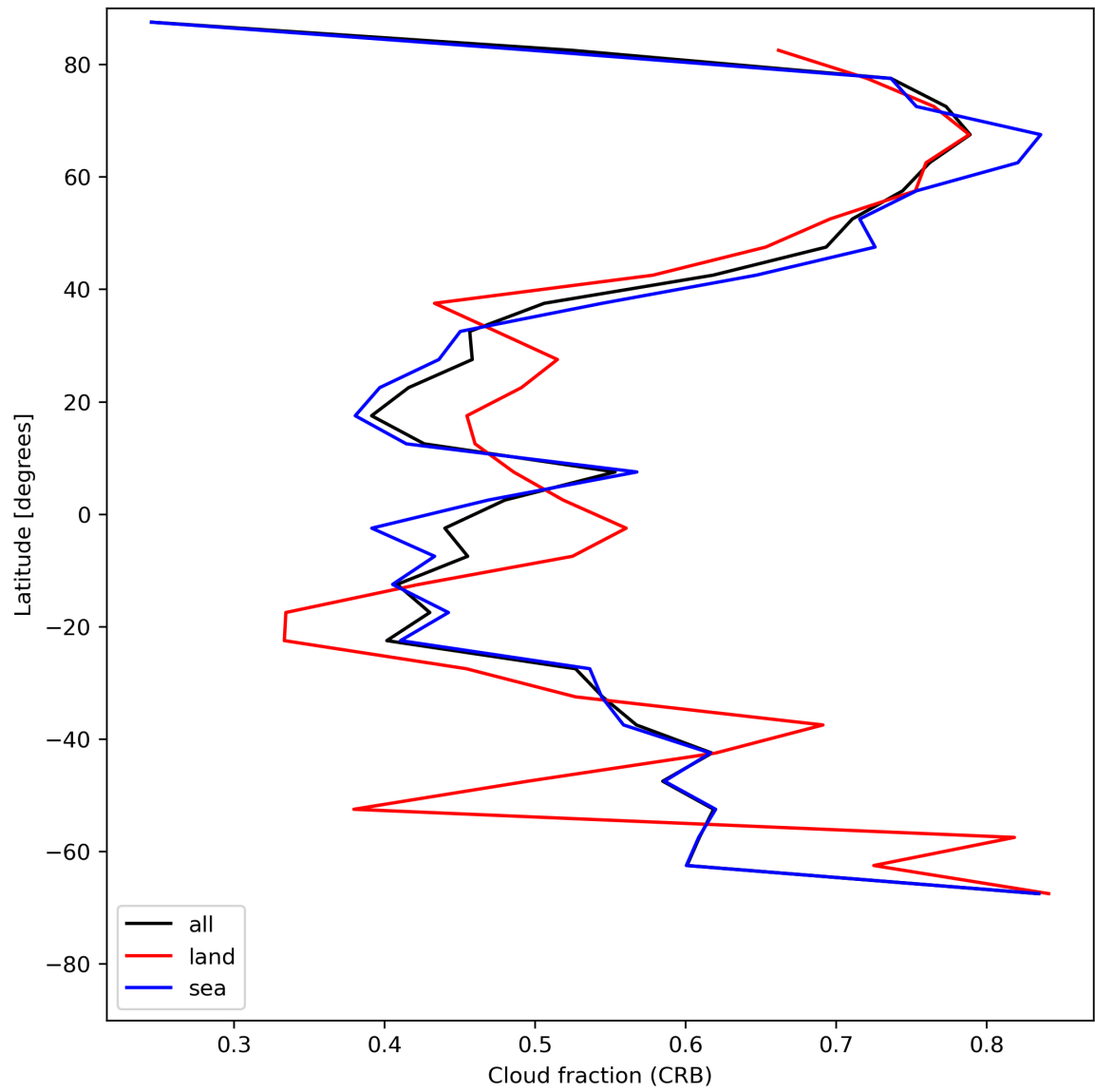
Figure 26: Zonal average of “Cloud fraction (CRB)” for 2024-05-20 to 2024-05-22.
