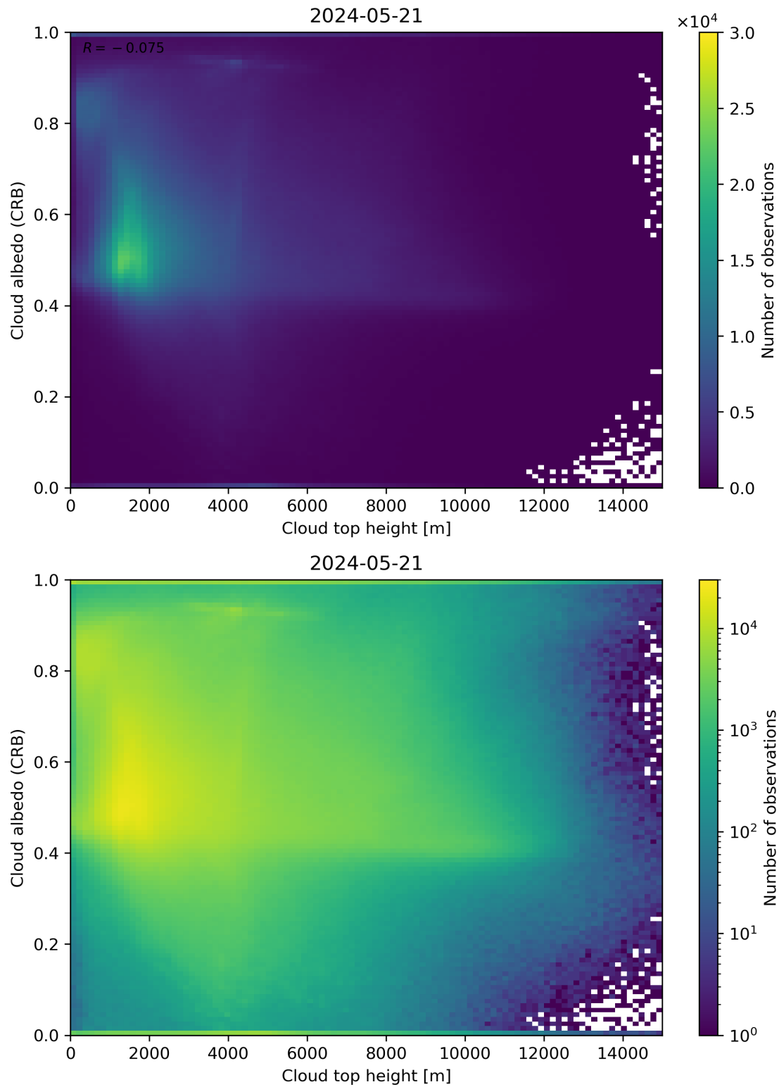
Figure 86: Scatter density plot of “Cloud top height” against “Cloud albedo (CRB)” for 2024-05-20 to 2024-05-22.
