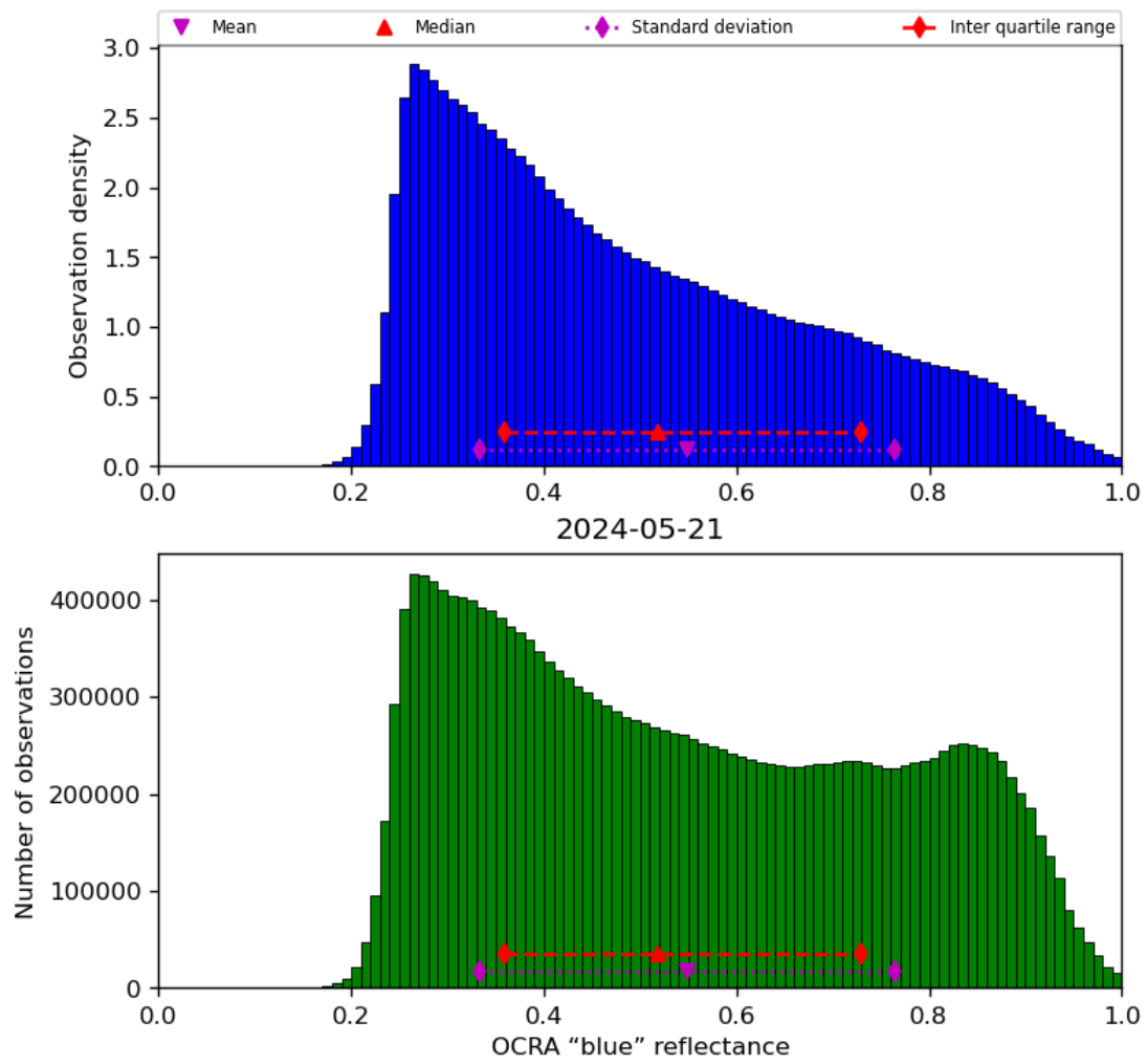
Figure 51: Histogram of “OCRA “blue” reflectance” for 2024-05-20 to 2024-05-22
