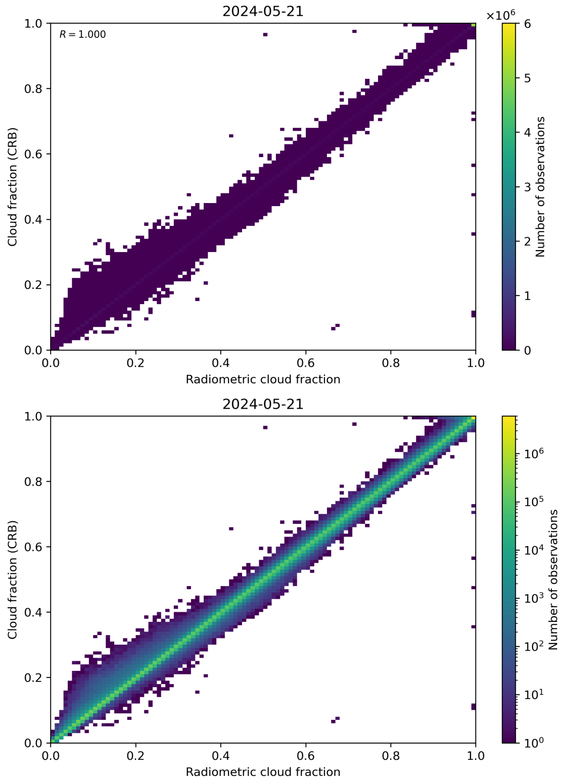
Figure 73: Scatter density plot of “Radiometric cloud fraction” against “Cloud fraction (CRB)” for 2024-05-20 to 2024-05-22.
