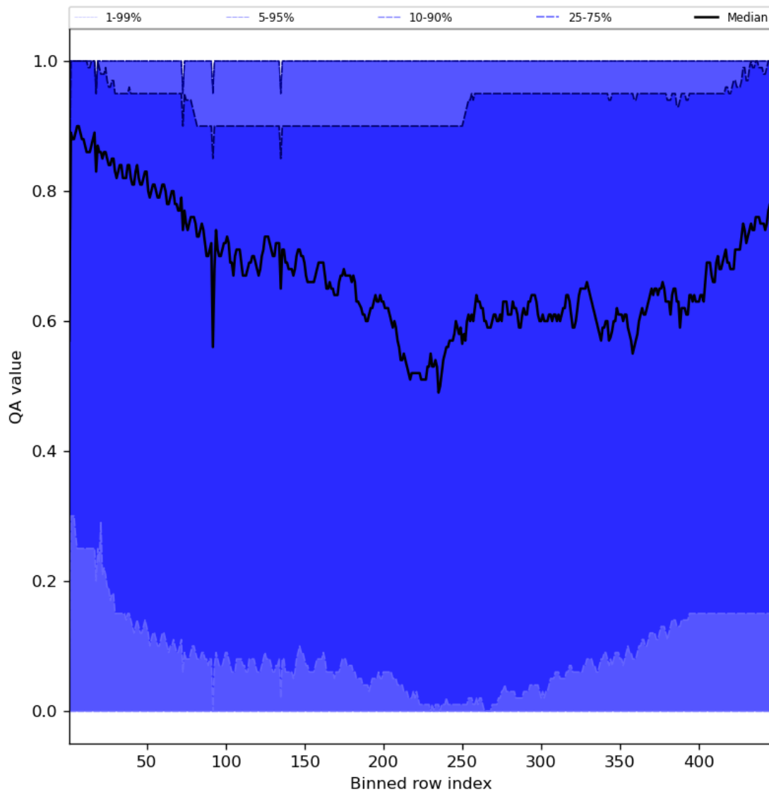
Figure 54: Along track statistics of “QA value” for 2024-05-20 to 2024-05-22
