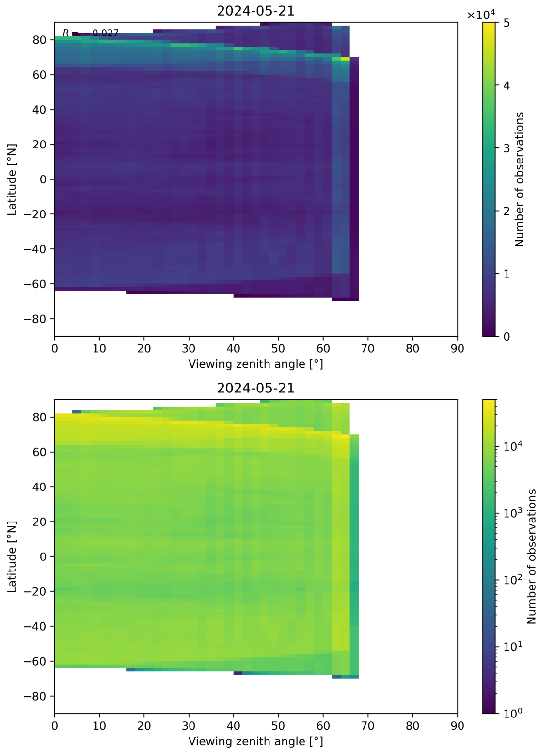
Figure 113: Scatter density plot of “Viewing zenith angle” against “Latitude” for 2024-05-20 to 2024-05-22.
