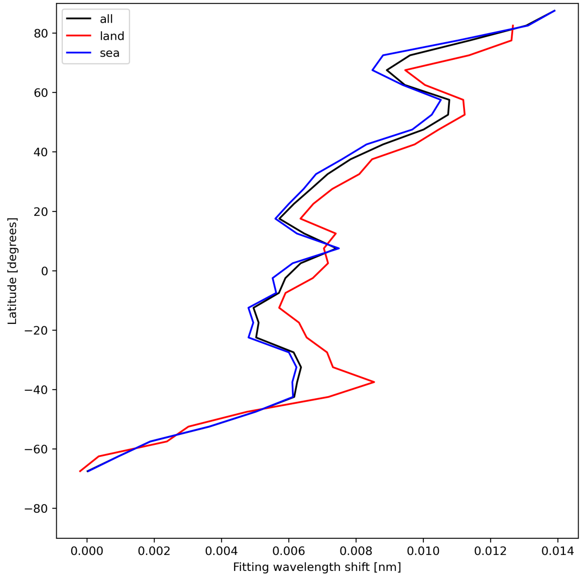
Figure 33: Zonal average of “Fitting wavelength shift” for 2024-05-20 to 2024-05-22.
