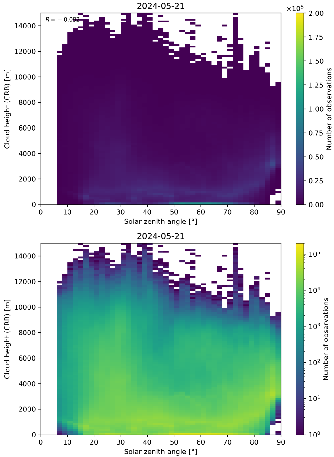
Figure 102: Scatter density plot of “Solar zenith angle” against “Cloud height (CRB)” for 2024-05-20 to 2024-05-22.
