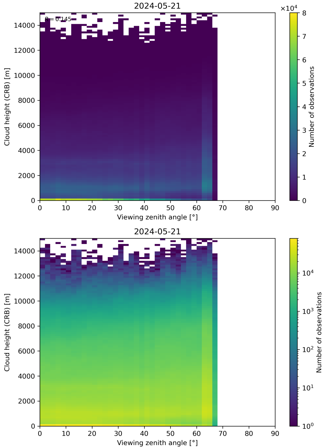
Figure 110: Scatter density plot of “Viewing zenith angle” against “Cloud height (CRB)” for 2024-05-20 to 2024-05-22.
