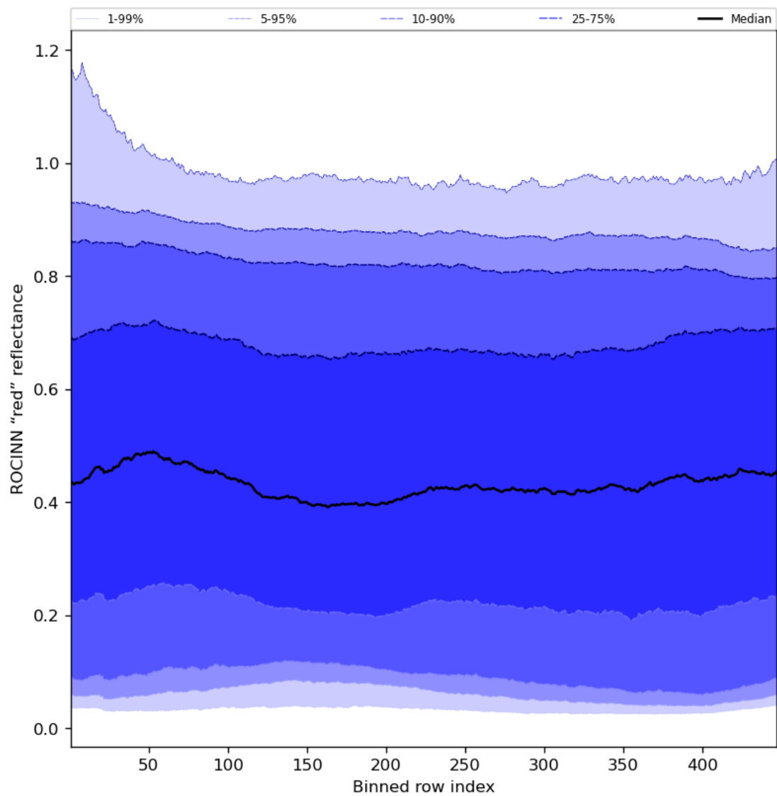
Figure 69: Along track statistics of “ROCINN “red” reflectance” for 2024-05-20 to 2024-05-22
