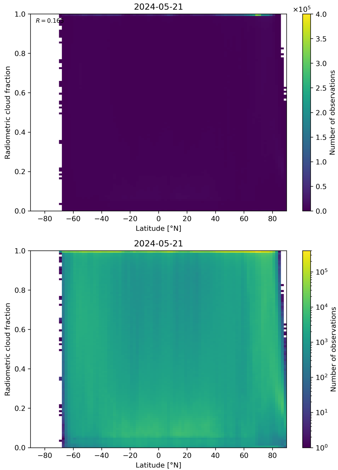
Figure 92: Scatter density plot of “Latitude” against “Radiometric cloud fraction” for 2024-05-20 to 2024-05-22.
