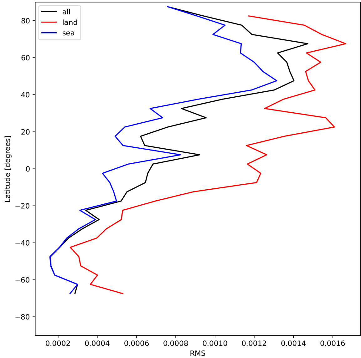
Figure 31: Zonal average of “RMS” for 2024-05-20 to 2024-05-22.
