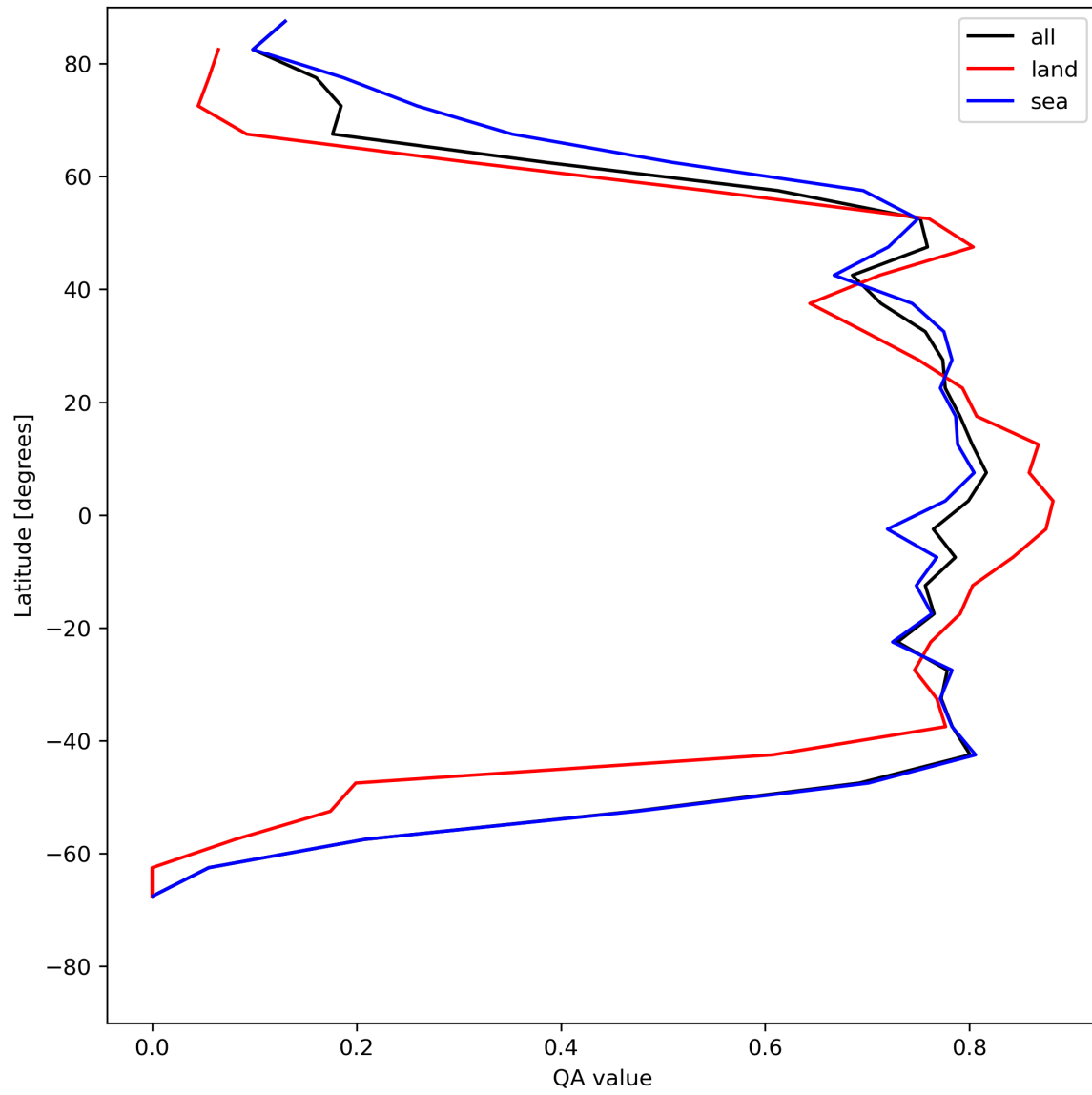
Figure 22: Zonal average of “QA value” for 2024-05-20 to 2024-05-22.
