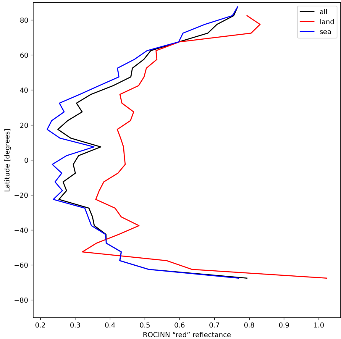
Figure 37: Zonal average of “ROCINN “red” reflectance” for 2024-05-20 to 2024-05-22.
