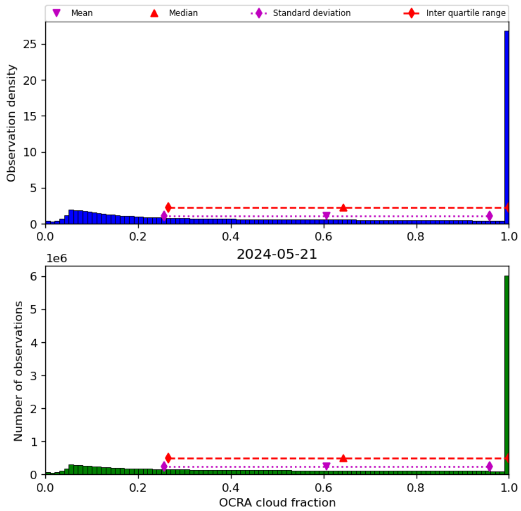
Figure 50: Histogram of “OCRA cloud fraction” for 2024-05-20 to 2024-05-22
