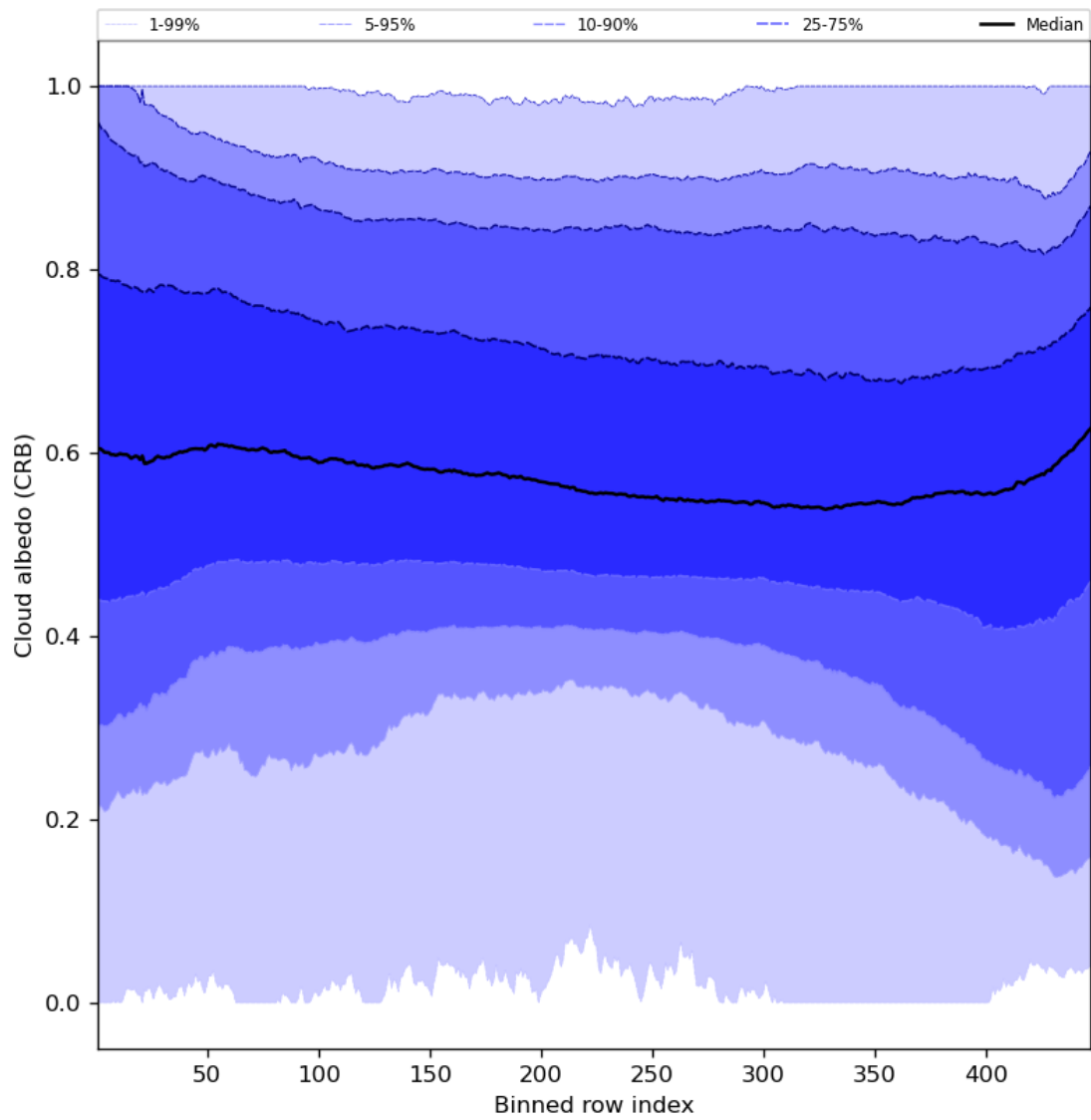
Figure 60: Along track statistics of “Cloud albedo (CRB)” for 2024-05-20 to 2024-05-22
