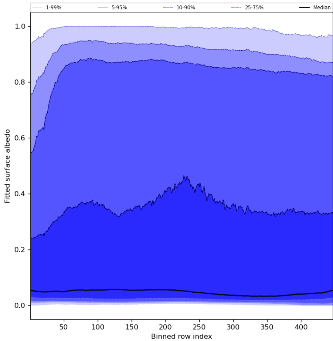
Figure 61: Along track statistics of “Fitted surface albedo” for 2024-05-20 to 2024-05-22
