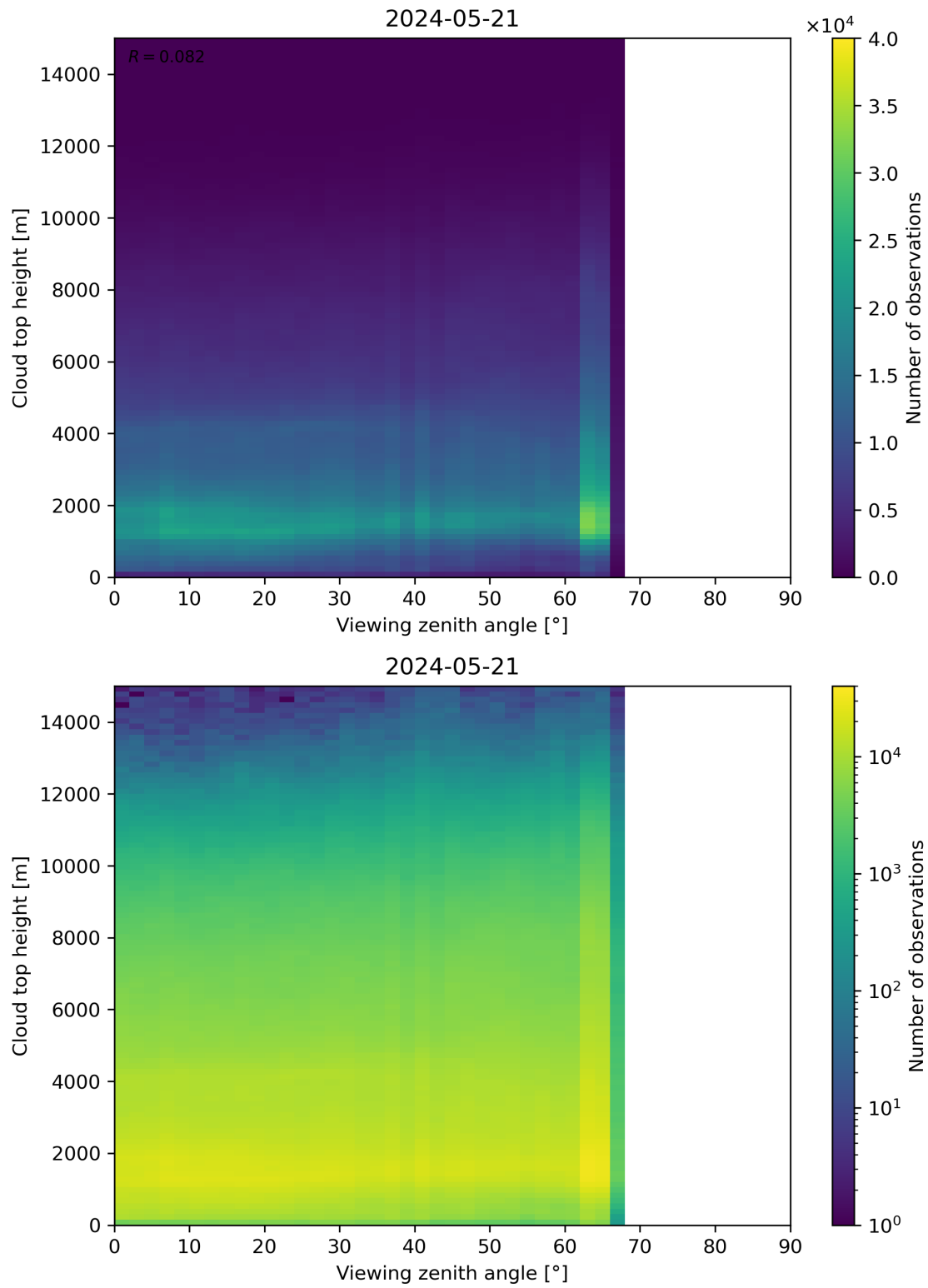
Figure 112: Scatter density plot of “Viewing zenith angle” against “Cloud top height” for 2024-05-20 to 2024-05-22.
