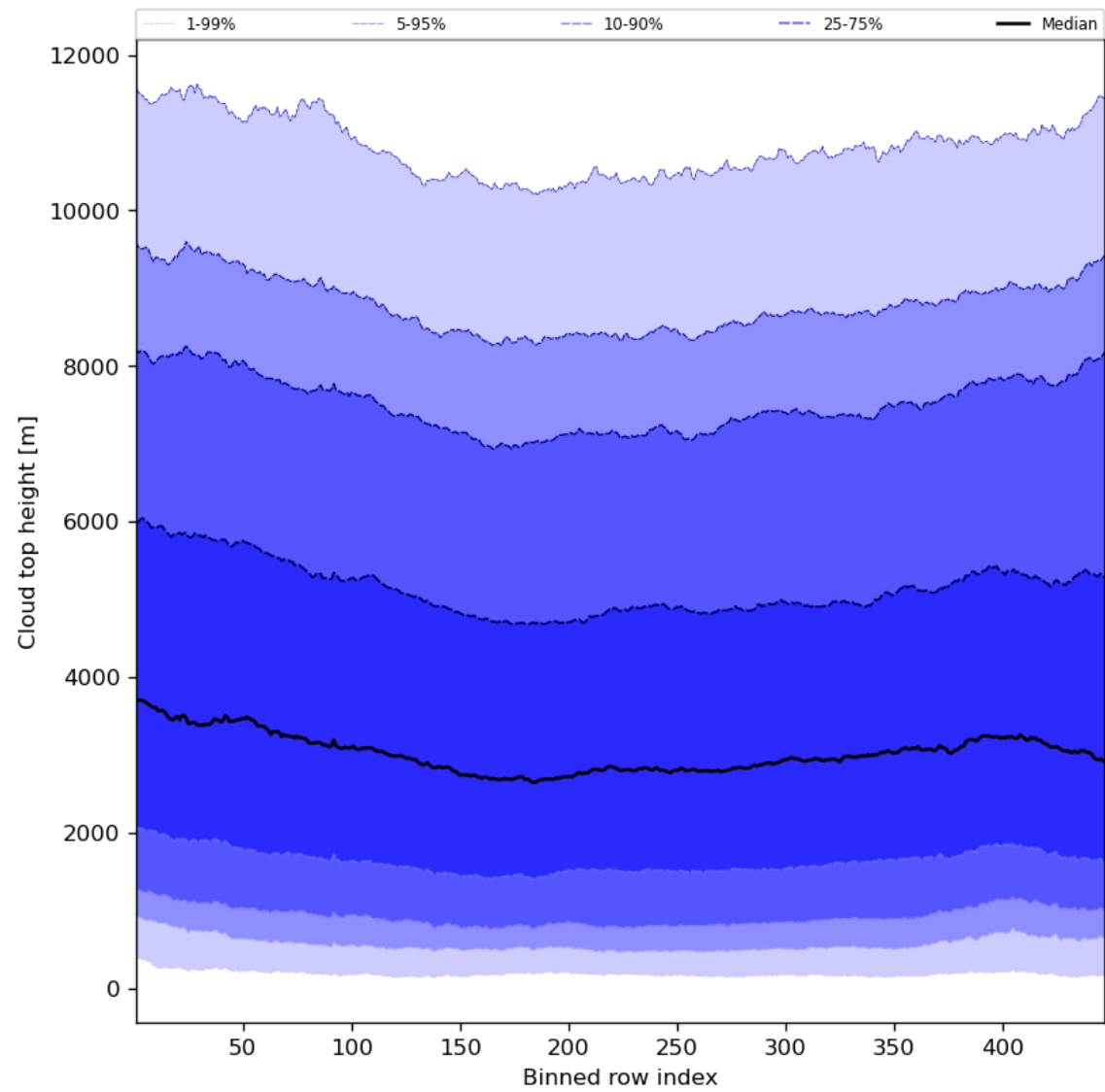
Figure 56: Along track statistics of “Cloud top height” for 2024-05-20 to 2024-05-22
