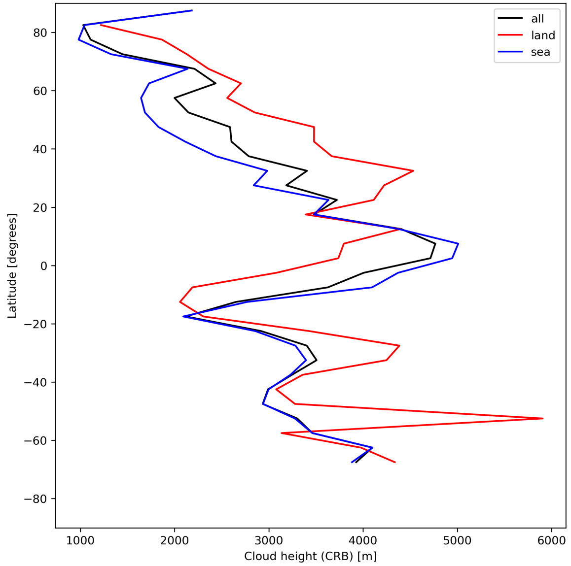
Figure 27: Zonal average of “Cloud height (CRB)” for 2024-05-20 to 2024-05-22.
