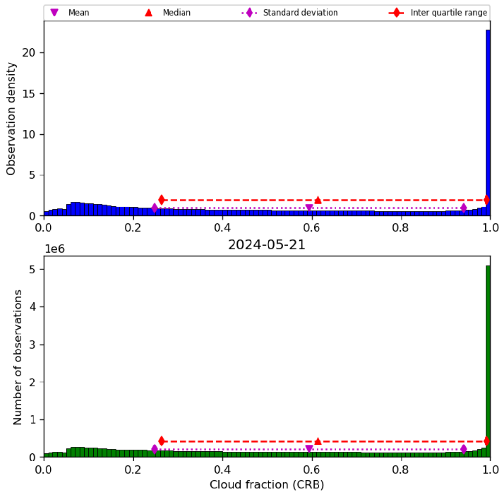
Figure 42: Histogram of “Cloud fraction (CRB)” for 2024-05-20 to 2024-05-22
