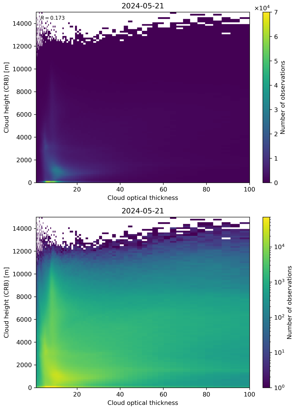
Figure 85: Scatter density plot of “Cloud optical thickness” against “Cloud height (CRB)” for 2024-05-20 to 2024-05-22.
