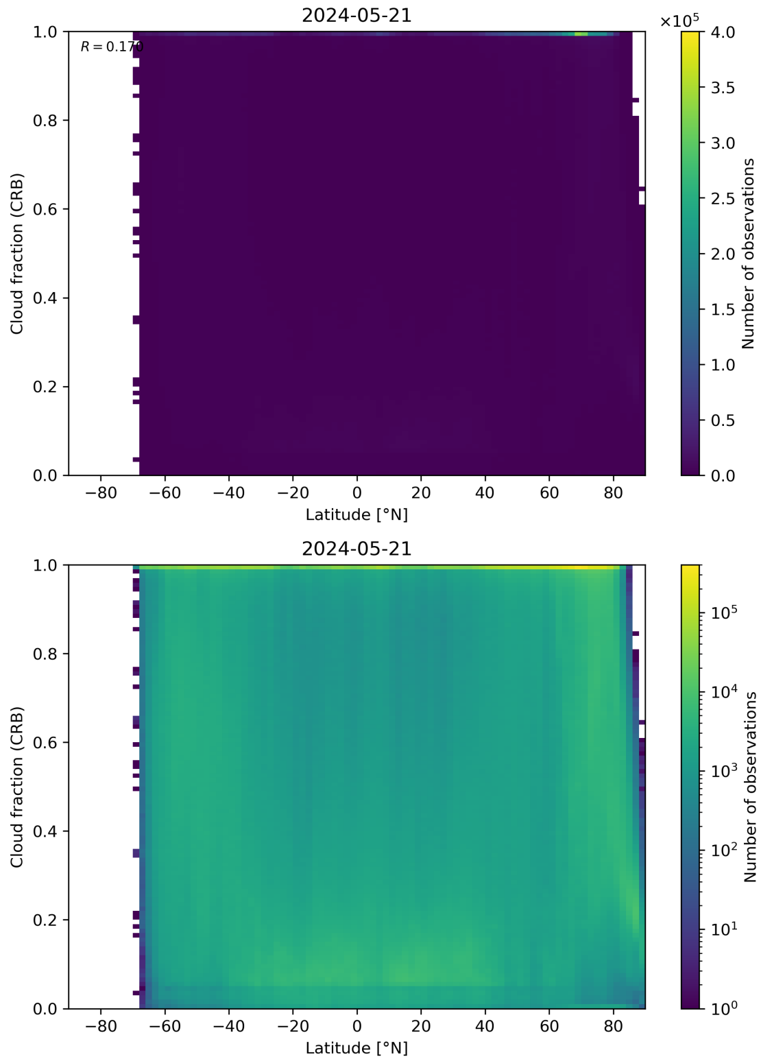
Figure 94: Scatter density plot of “Latitude” against “Cloud fraction (CRB)” for 2024-05-20 to 2024-05-22.
