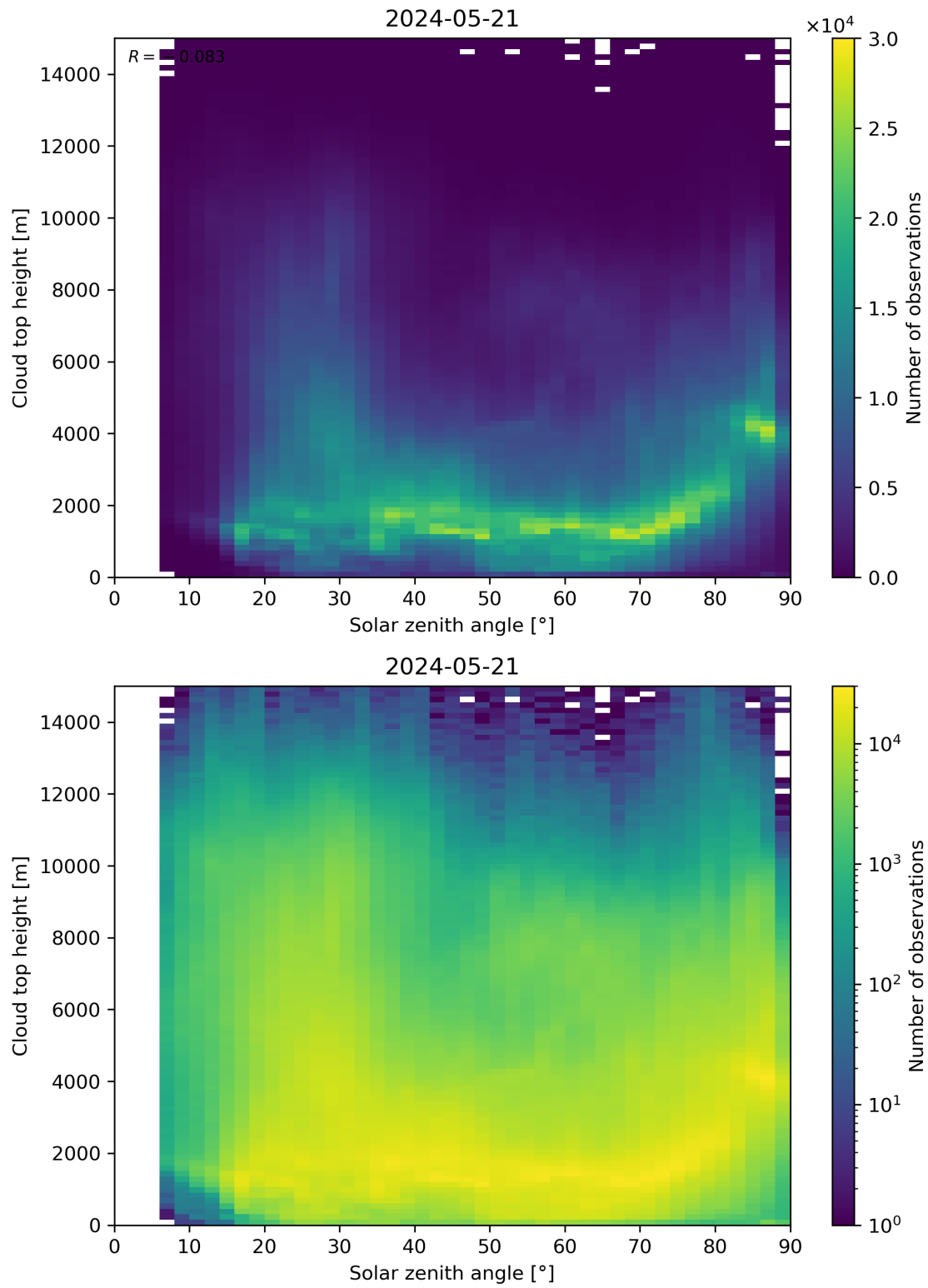
Figure 104: Scatter density plot of “Solar zenith angle” against “Cloud top height” for 2024-05-20 to 2024-05-22.
