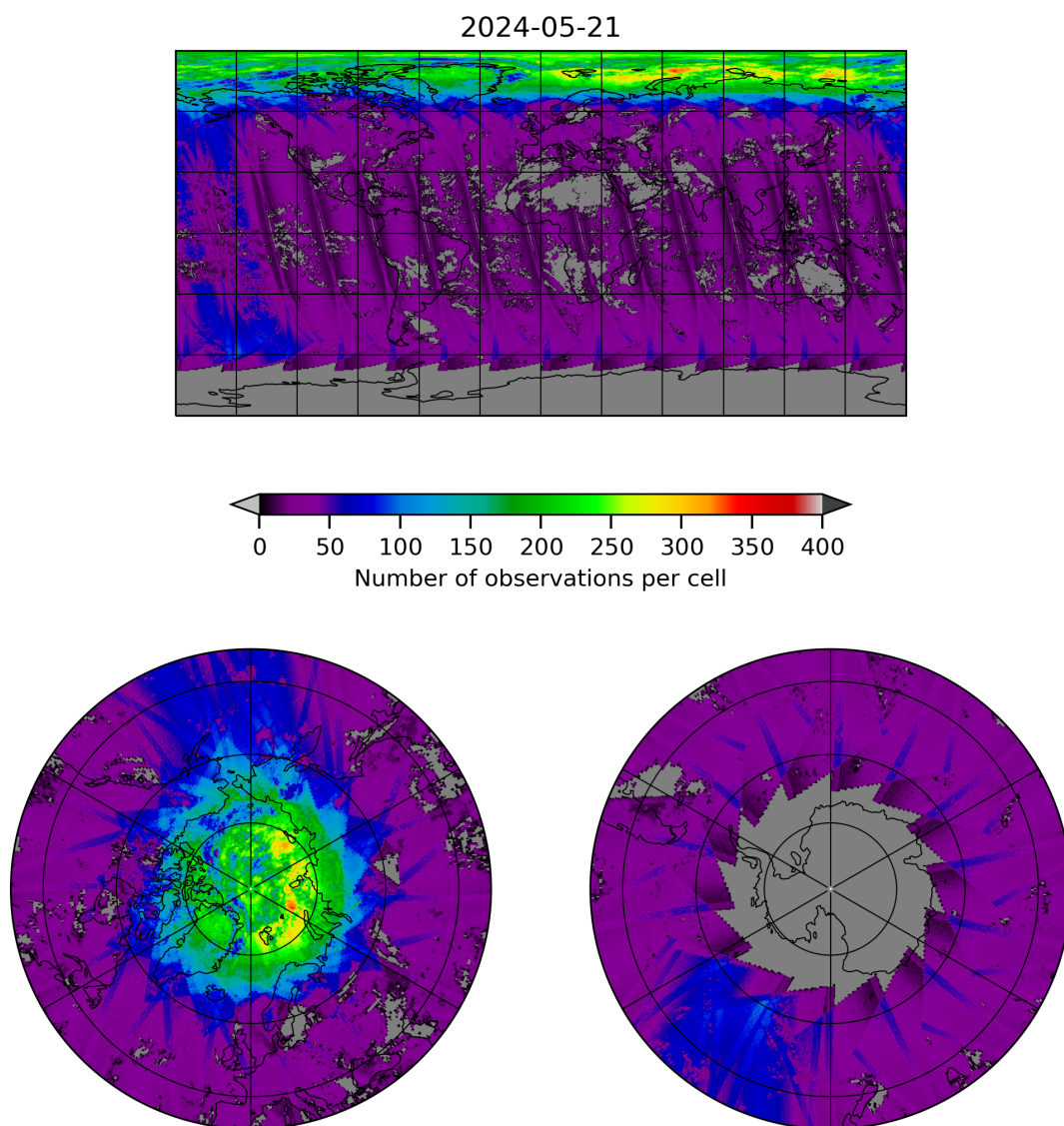
Figure 21: Map of the number of observations for 2024-05-20 to 2024-05-22
