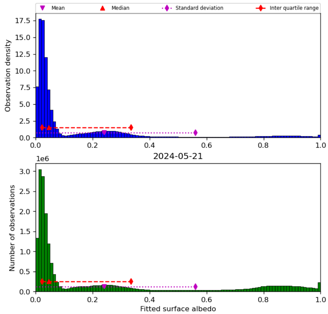
Figure 45: Histogram of “Fitted surface albedo” for 2024-05-20 to 2024-05-22
