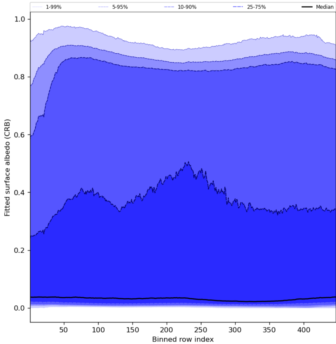
Figure 62: Along track statistics of “Fitted surface albedo (CRB)” for 2024-05-20 to 2024-05-22
