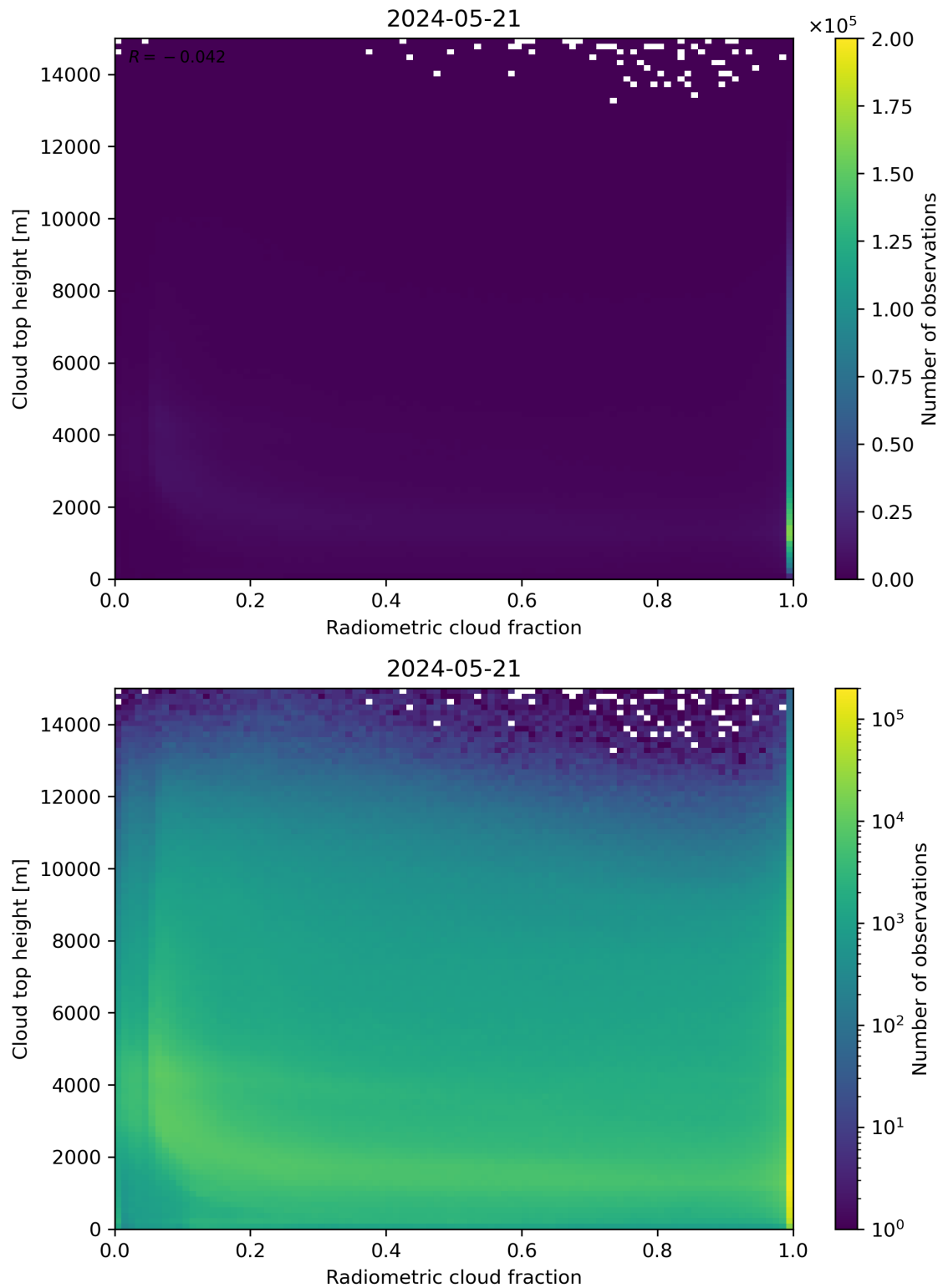
Figure 76: Scatter density plot of “Radiometric cloud fraction” against “Cloud top height” for 2024-05-20 to 2024-05-22.
