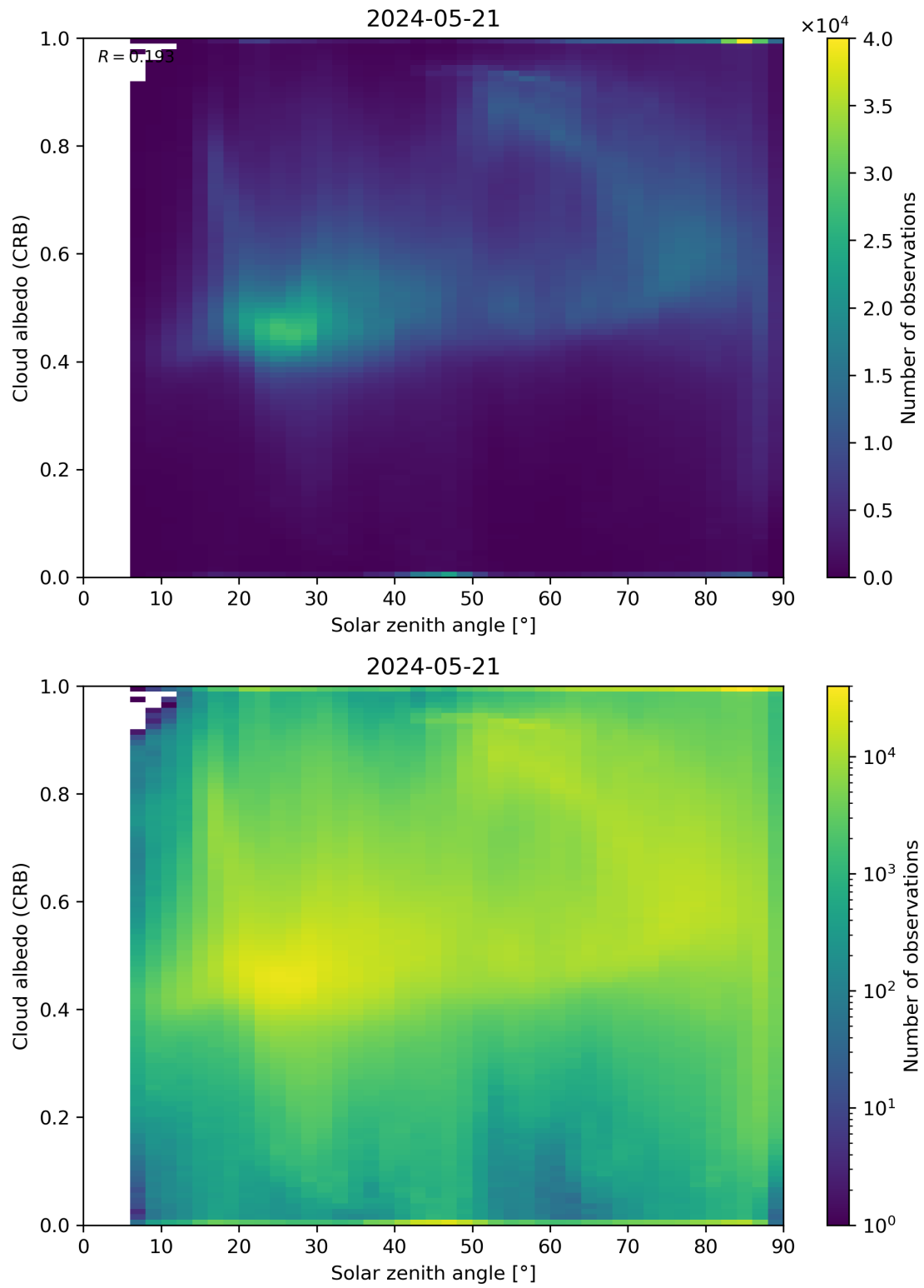
Figure 98: Scatter density plot of “Solar zenith angle” against “Cloud albedo (CRB)” for 2024-05-20 to 2024-05-22.
