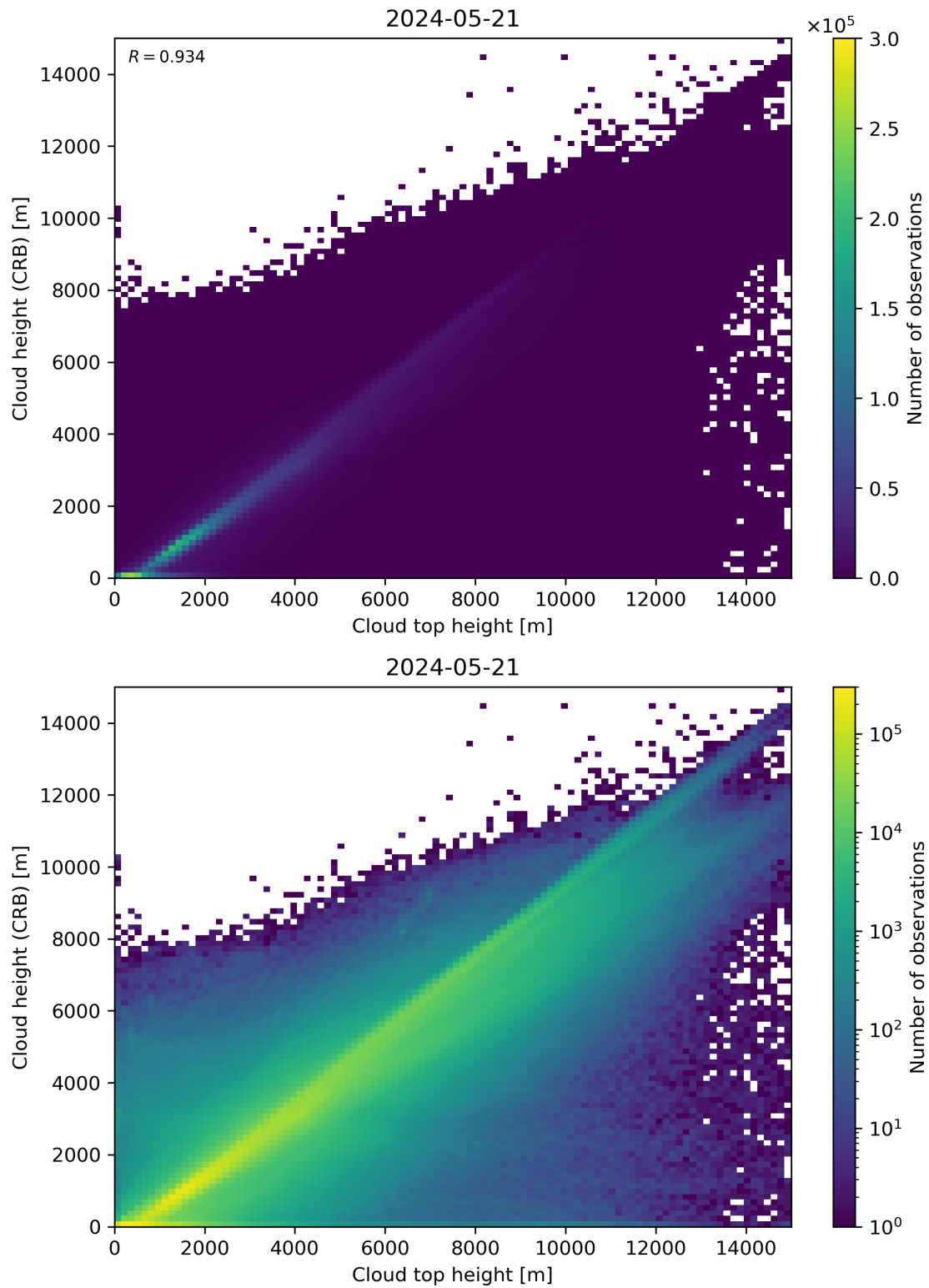
Figure 89: Scatter density plot of “Cloud top height” against “Cloud height (CRB)” for 2024-05-20 to 2024-05-22.
