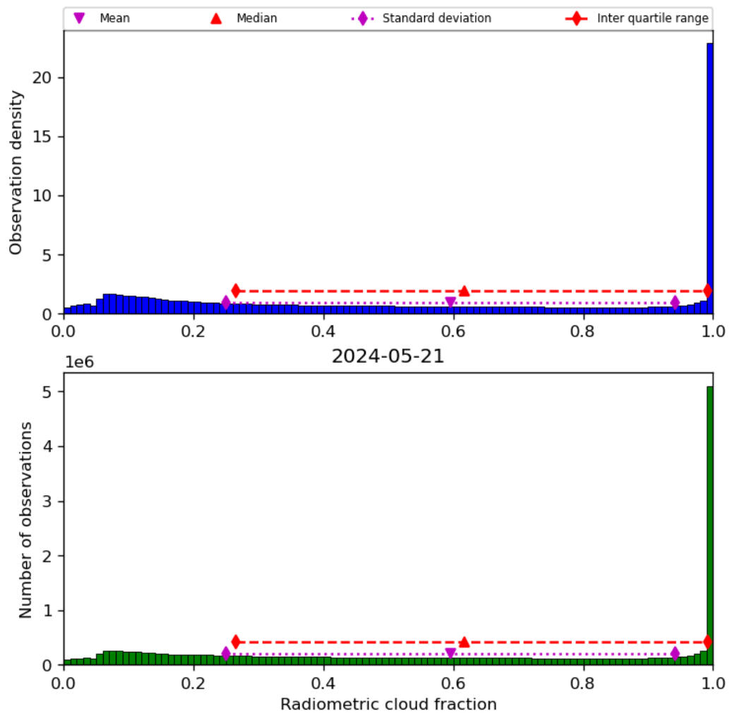
Figure 39: Histogram of “Radiometric cloud fraction” for 2024-05-20 to 2024-05-22
