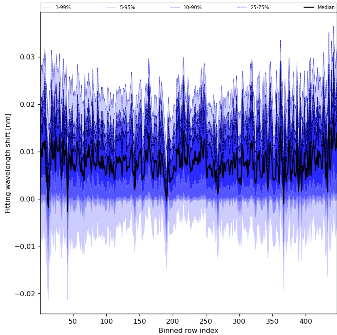
Figure 65: Along track statistics of “Fitting wavelength shift” for 2024-05-20 to 2024-05-22
