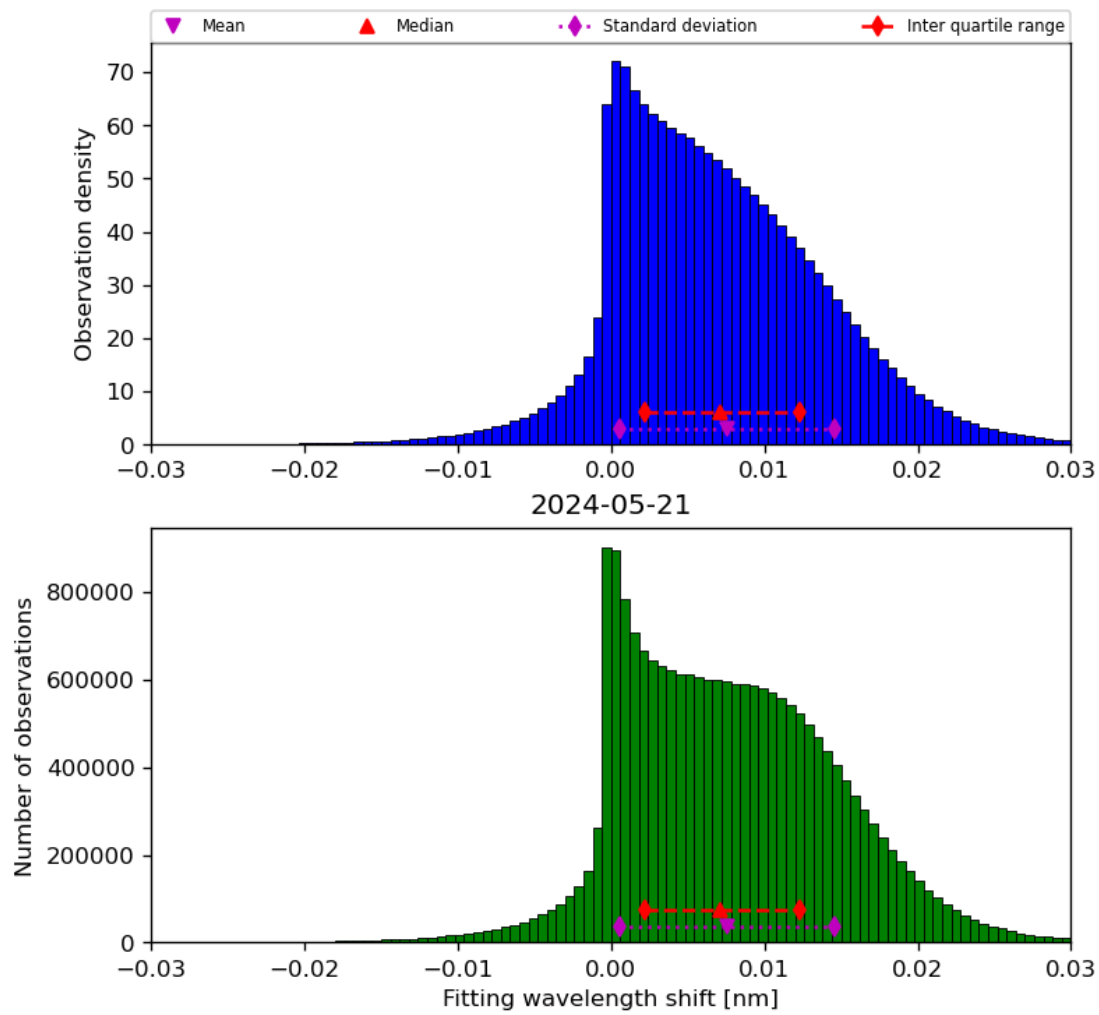
Figure 49: Histogram of “Fitting wavelength shift” for 2024-05-20 to 2024-05-22
