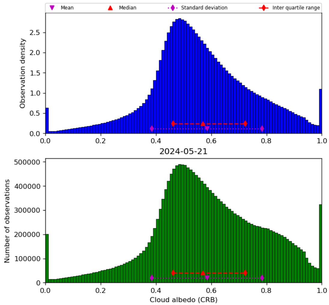
Figure 44: Histogram of “Cloud albedo (CRB)” for 2024-05-20 to 2024-05-22
