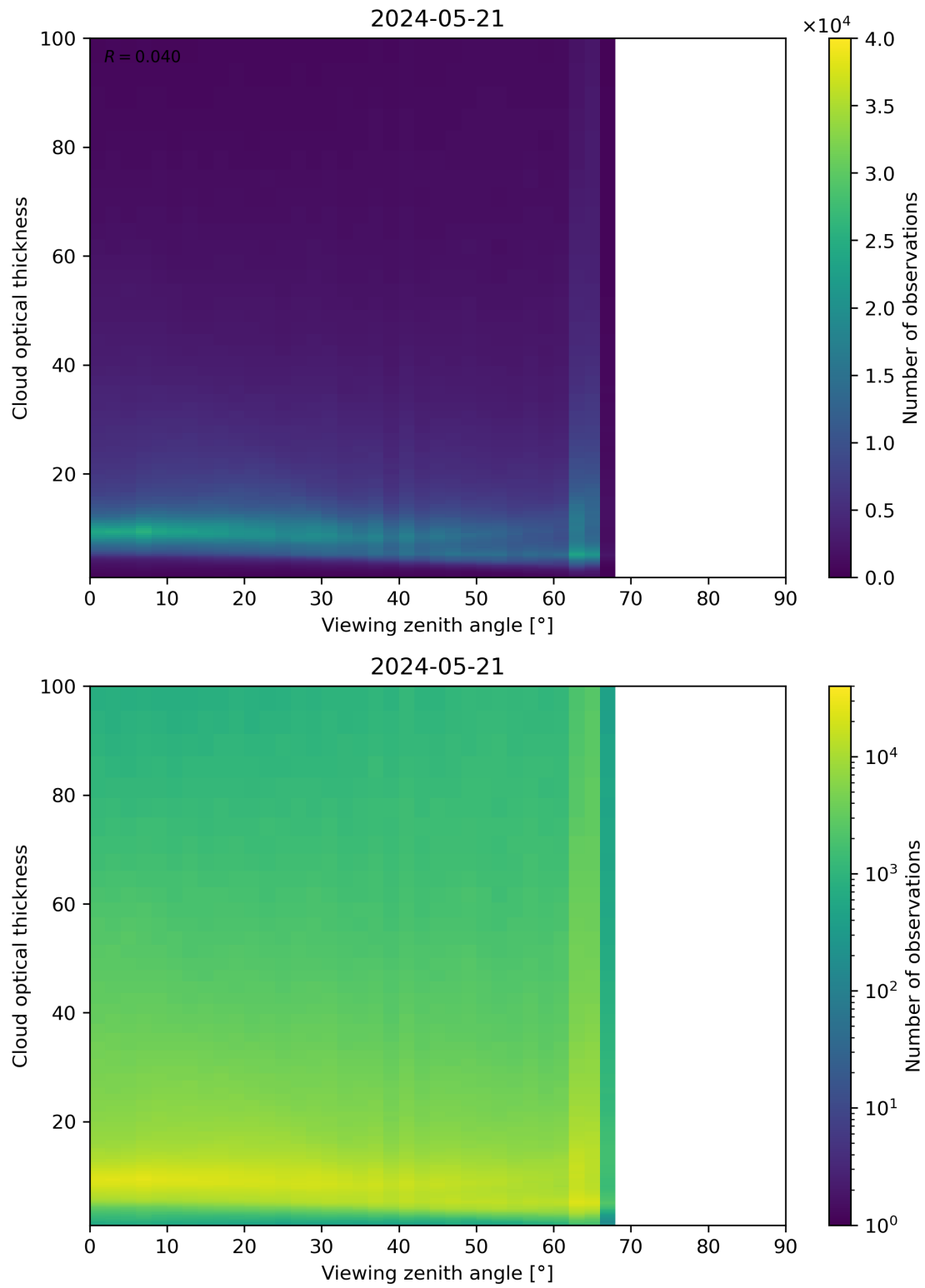
Figure 111: Scatter density plot of “Viewing zenith angle” against “Cloud optical thickness” for 2024-05-20 to 2024-05-22.
