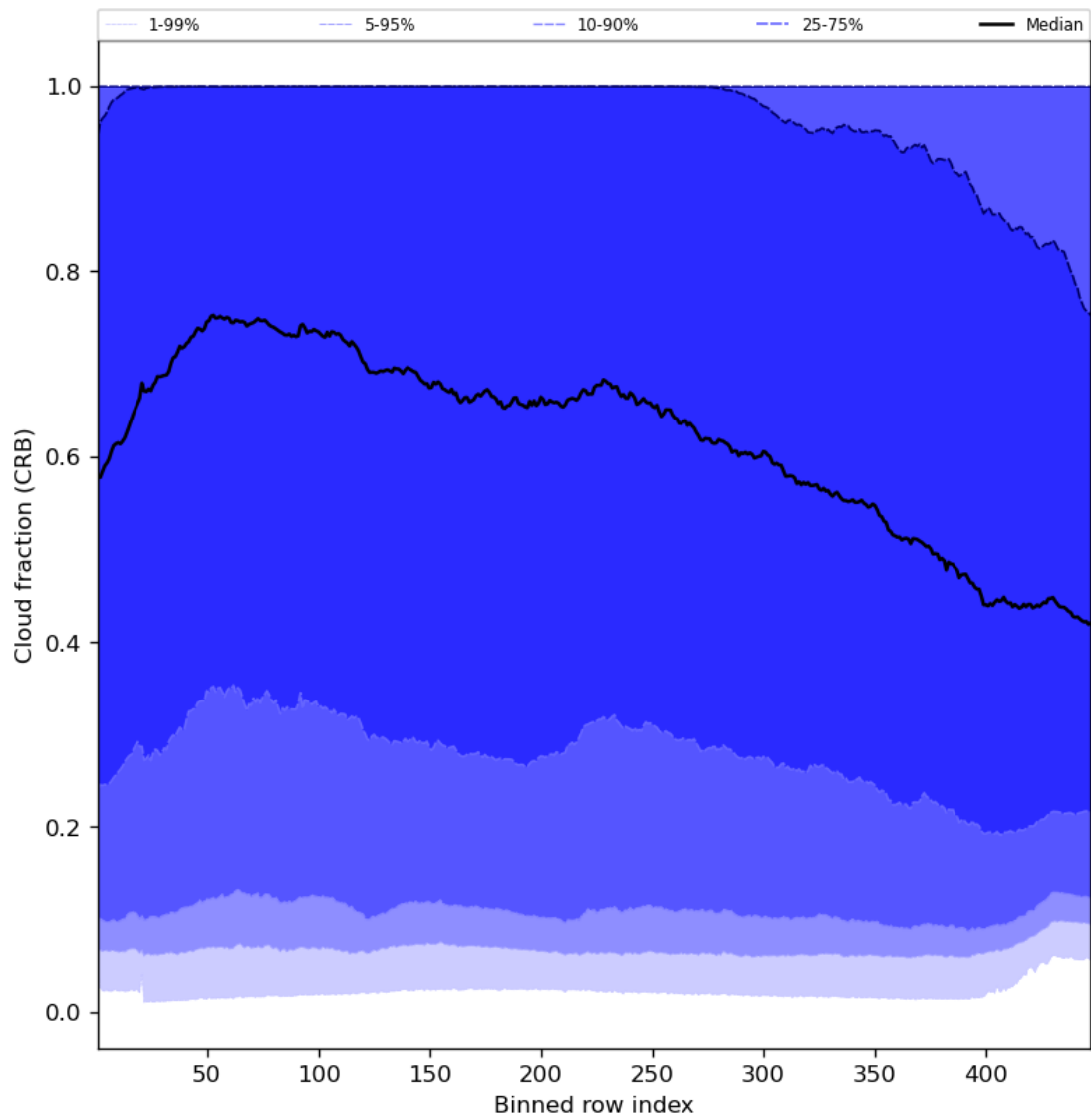
Figure 58: Along track statistics of “Cloud fraction (CRB)” for 2024-05-20 to 2024-05-22
