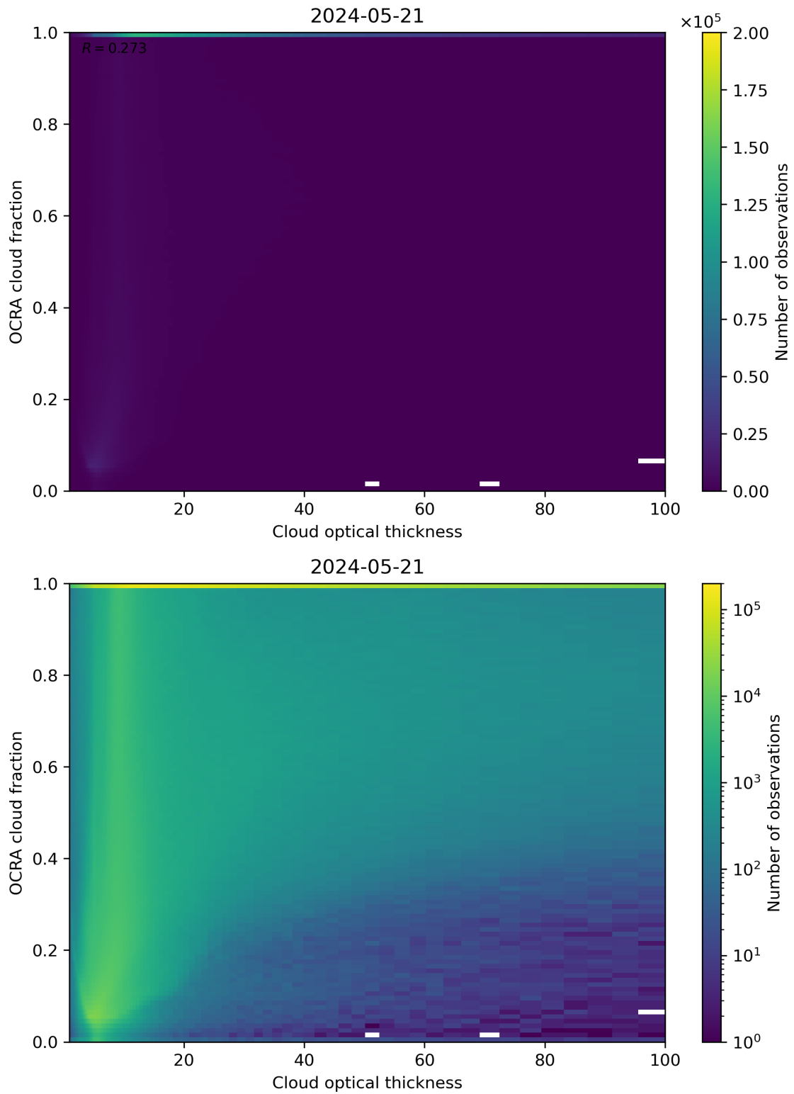
Figure 83: Scatter density plot of “Cloud optical thickness” against “OCRA cloud fraction” for 2024-05-20 to 2024-05-22.
