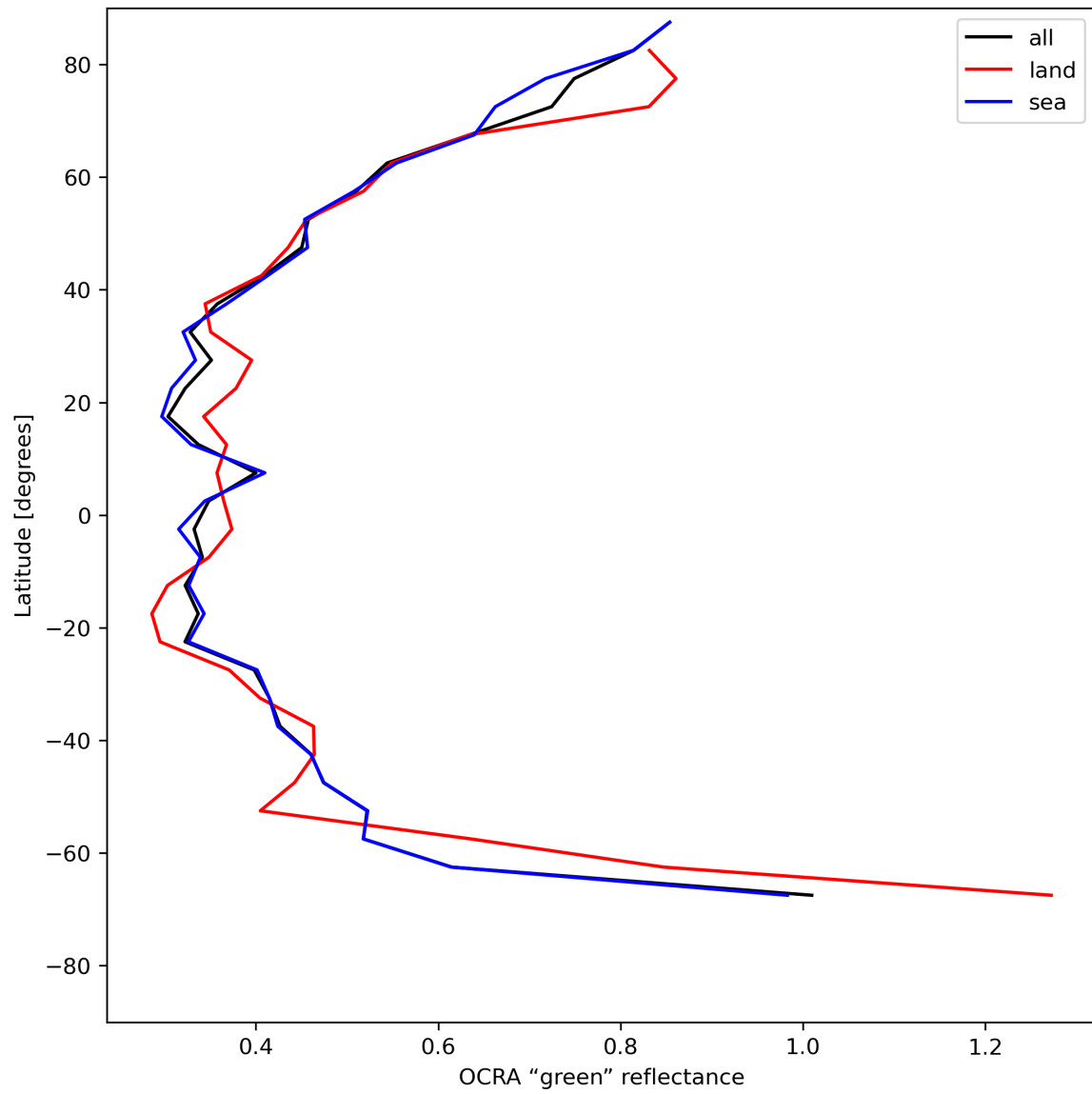
Figure 36: Zonal average of “OCRA “green” reflectance” for 2024-05-20 to 2024-05-22.
