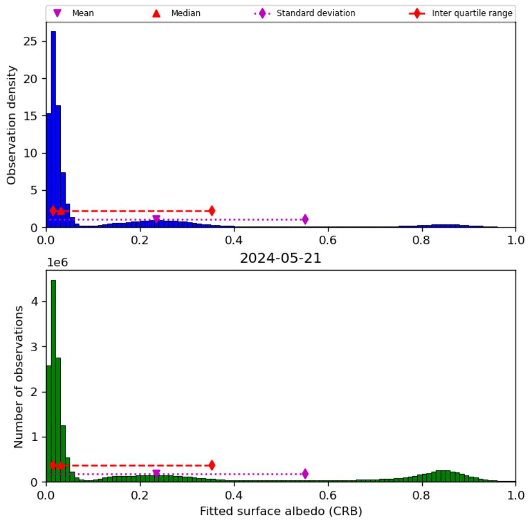
Figure 46: Histogram of “Fitted surface albedo (CRB)” for 2024-05-20 to 2024-05-22
