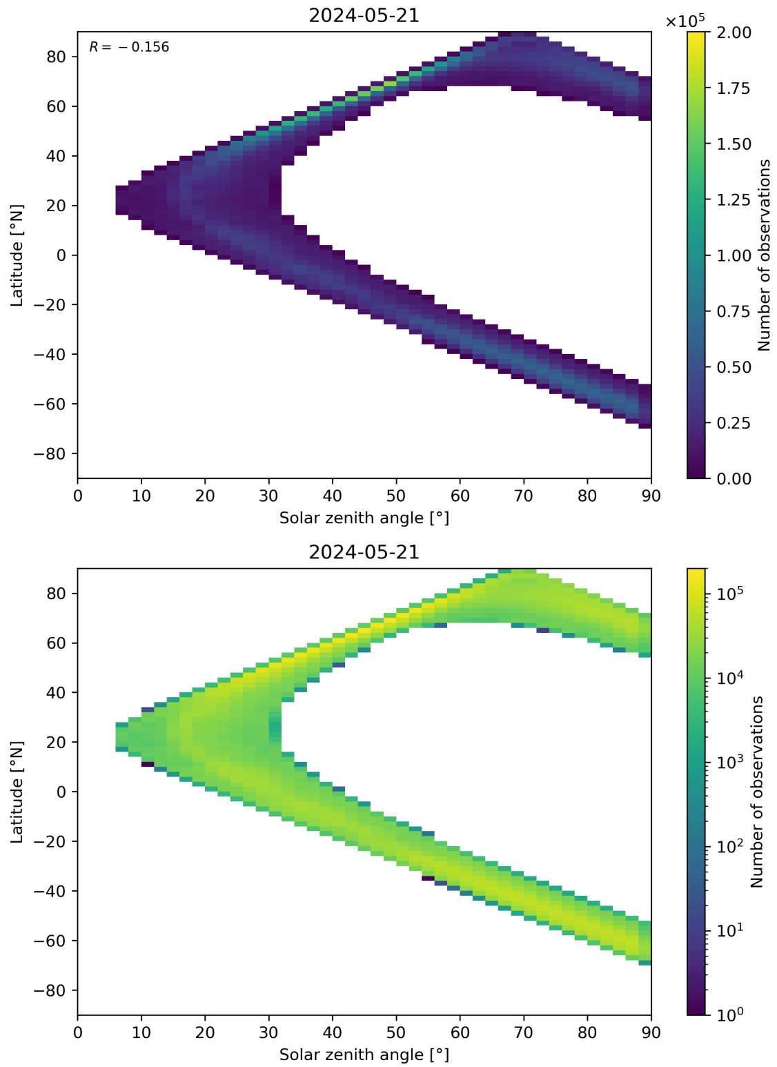
Figure 105: Scatter density plot of “Solar zenith angle” against “Latitude” for 2024-05-20 to 2024-05-22.
