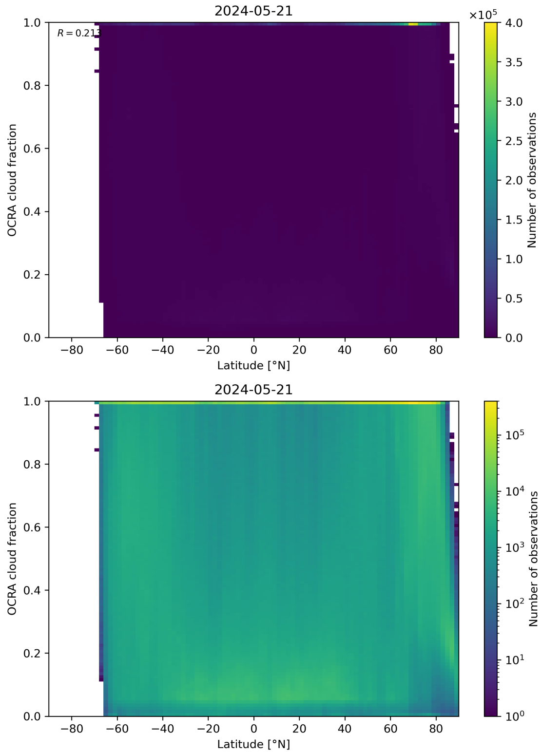
Figure 93: Scatter density plot of “Latitude” against “OCRA cloud fraction” for 2024-05-20 to 2024-05-22.
