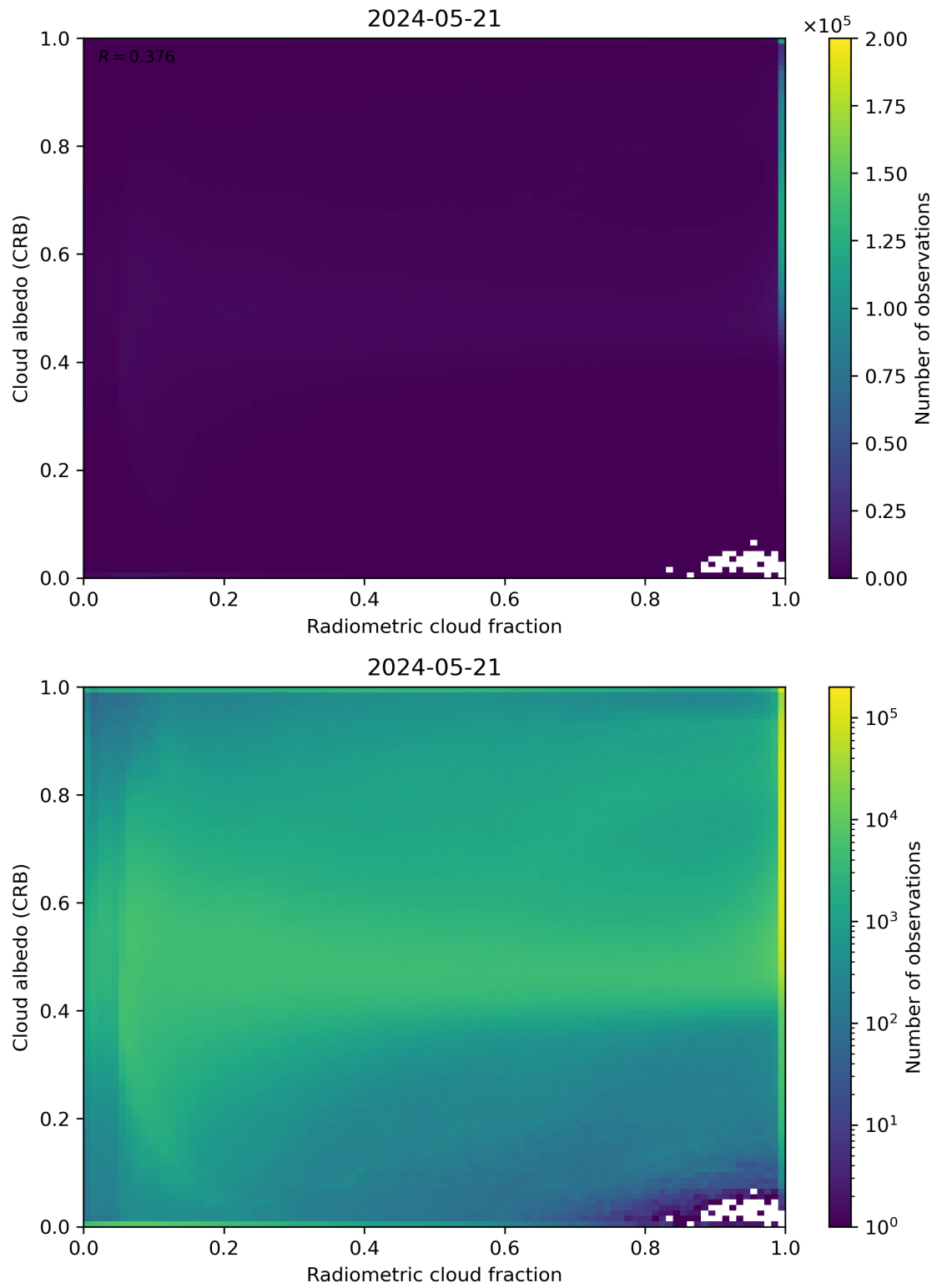
Figure 71: Scatter density plot of “Radiometric cloud fraction” against “Cloud albedo (CRB)” for 2024-05-20 to 2024-05-22.
