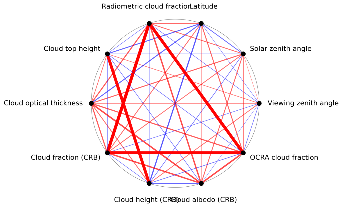
Figure 1: Map of correlation graph for 2024-05-20 to 2024-05-22.
