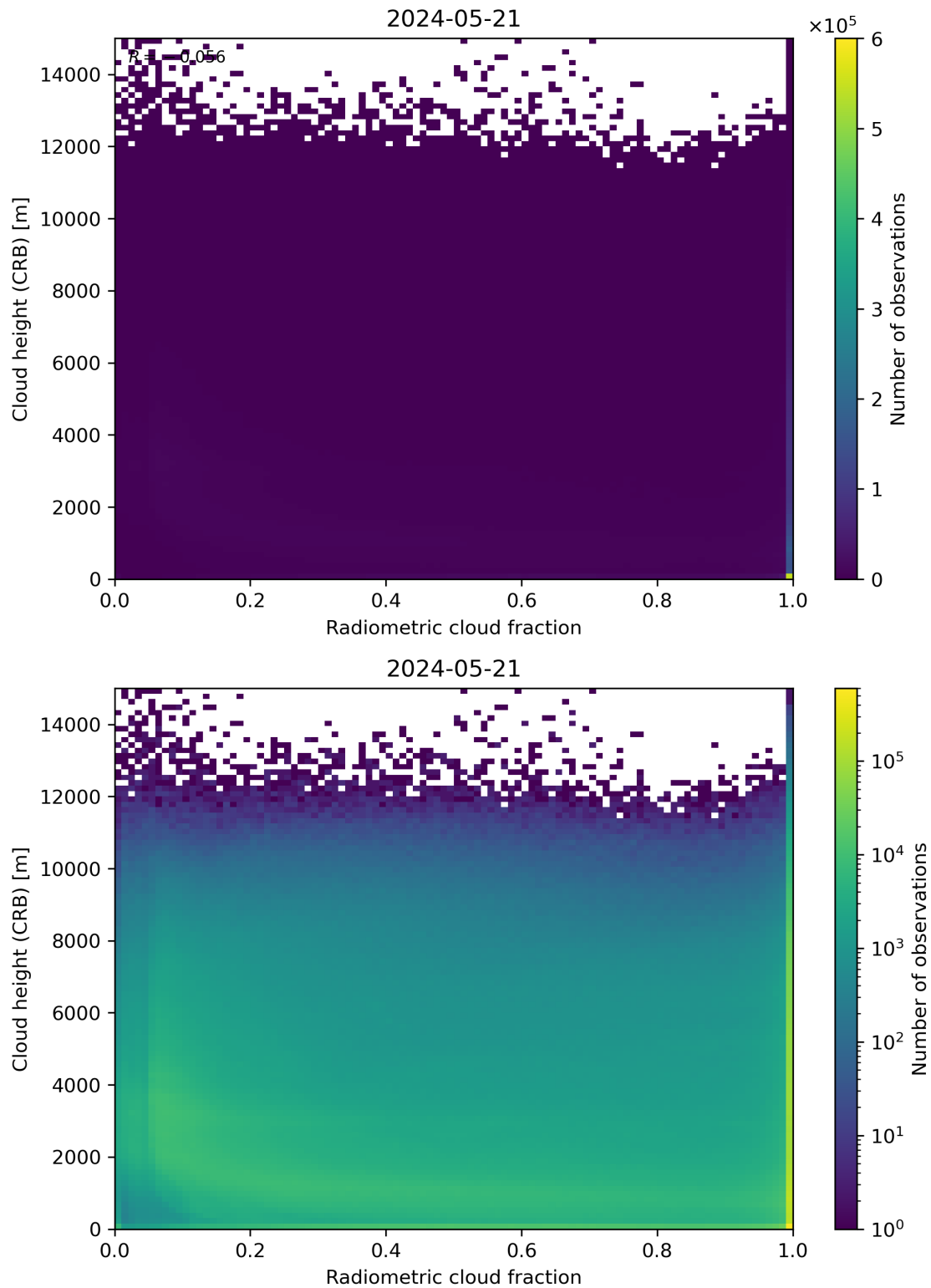
Figure 74: Scatter density plot of “Radiometric cloud fraction” against “Cloud height (CRB)” for 2024-05-20 to 2024-05-22.
