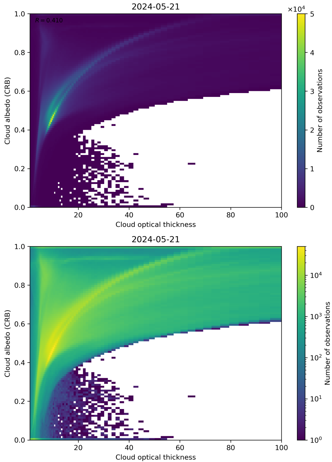
Figure 82: Scatter density plot of “Cloud optical thickness” against “Cloud albedo (CRB)” for 2024-05-20 to 2024-05-22.
