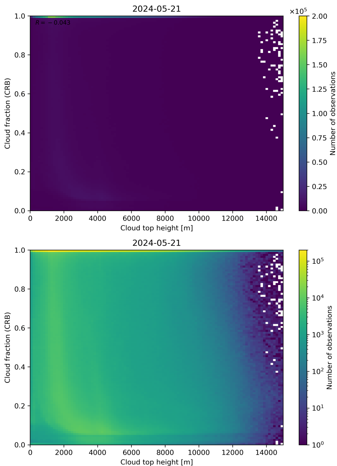
Figure 88: Scatter density plot of “Cloud top height” against “Cloud fraction (CRB)” for 2024-05-20 to 2024-05-22.
