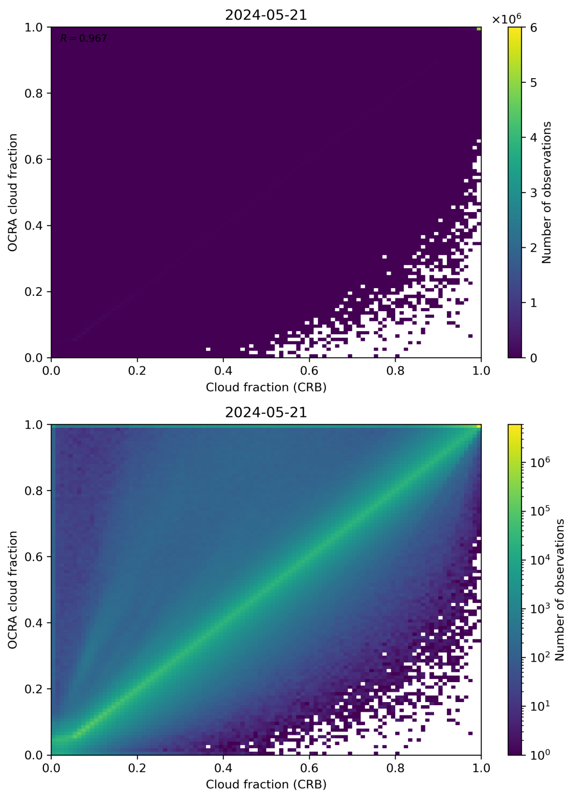
Figure 78: Scatter density plot of “Cloud fraction (CRB)” against “OCRA cloud fraction” for 2024-05-20 to 2024-05-22.
