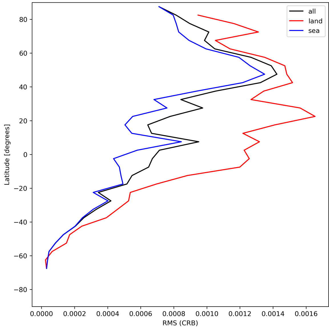
Figure 32: Zonal average of “RMS (CRB)” for 2024-05-20 to 2024-05-22.
