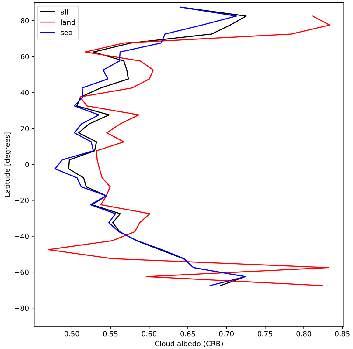
Figure 28: Zonal average of “Cloud albedo (CRB)” for 2024-05-20 to 2024-05-22.
