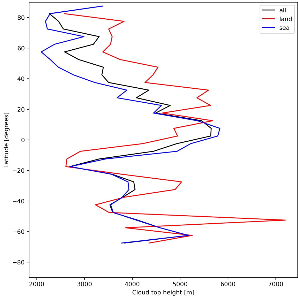
Figure 24: Zonal average of “Cloud top height” for 2024-05-20 to 2024-05-22.
