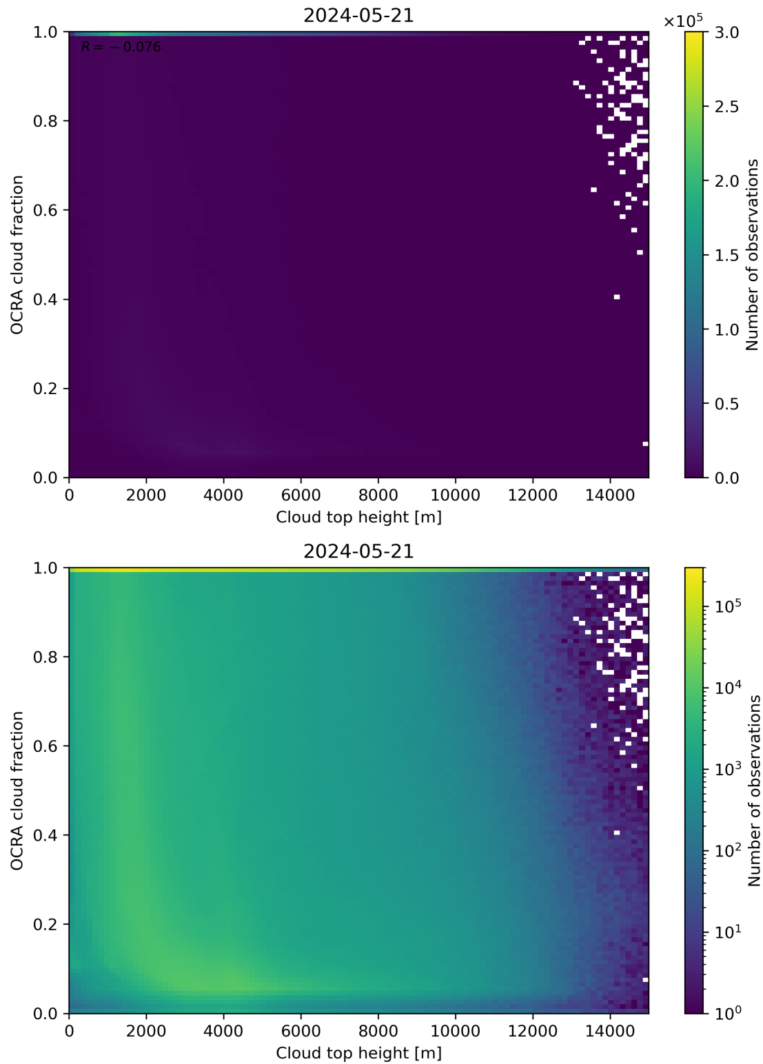
Figure 87: Scatter density plot of “Cloud top height” against “OCRA cloud fraction” for 2024-05-20 to 2024-05-22.
