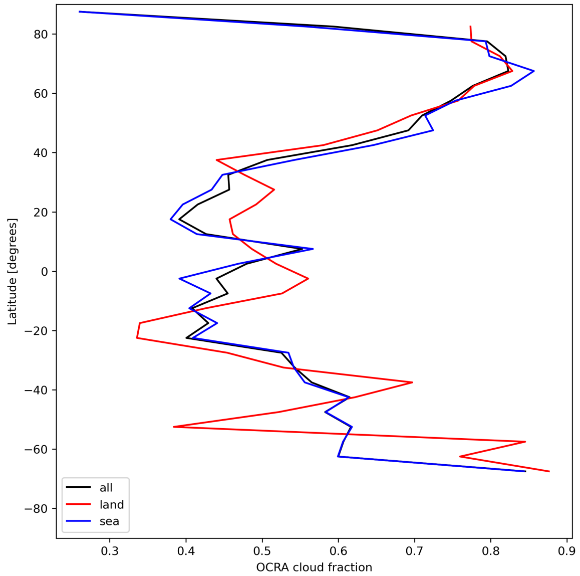
Figure 34: Zonal average of “OCRA cloud fraction” for 2024-05-20 to 2024-05-22.
