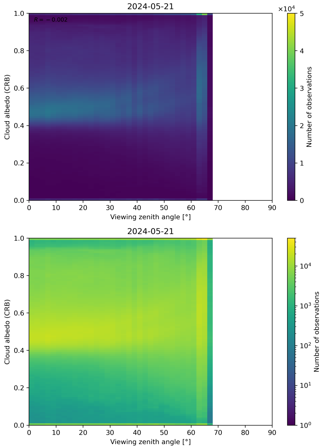
Figure 106: Scatter density plot of “Viewing zenith angle” against “Cloud albedo (CRB)” for 2024-05-20 to 2024-05-22.
