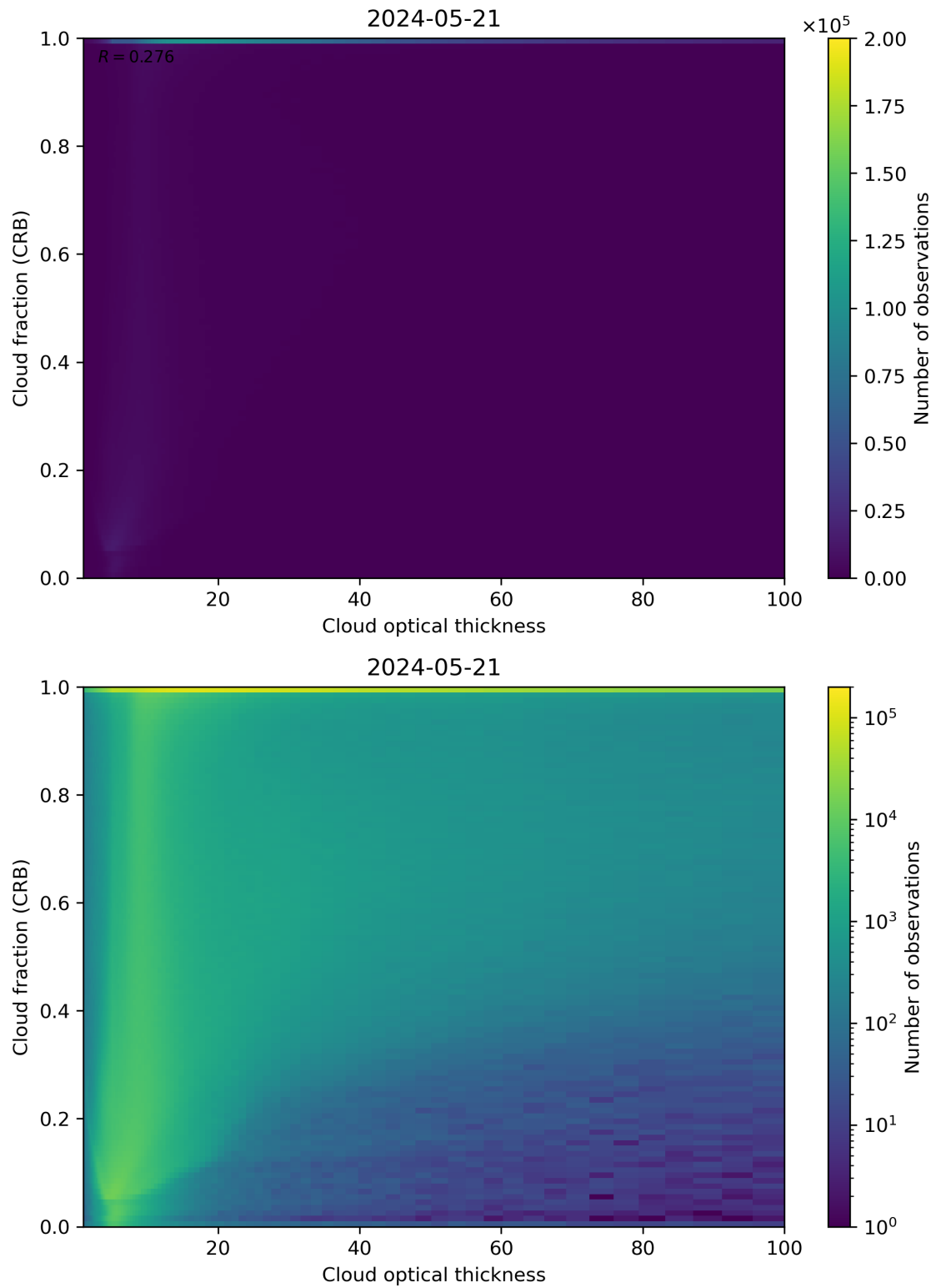
Figure 84: Scatter density plot of “Cloud optical thickness” against “Cloud fraction (CRB)” for 2024-05-20 to 2024-05-22.
