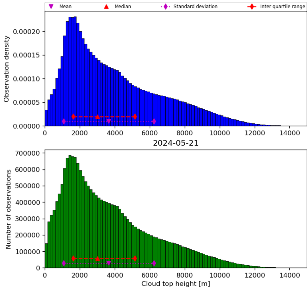
Figure 40: Histogram of “Cloud top height” for 2024-05-20 to 2024-05-22
