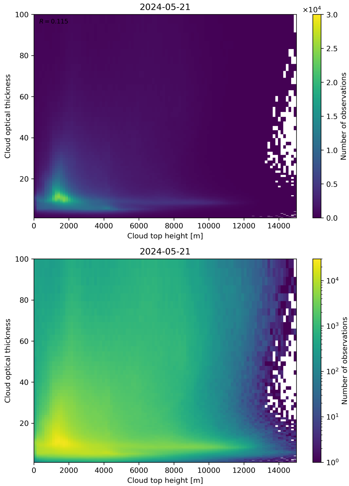
Figure 90: Scatter density plot of “Cloud top height” against “Cloud optical thickness” for 2024-05-20 to 2024-05-22.
