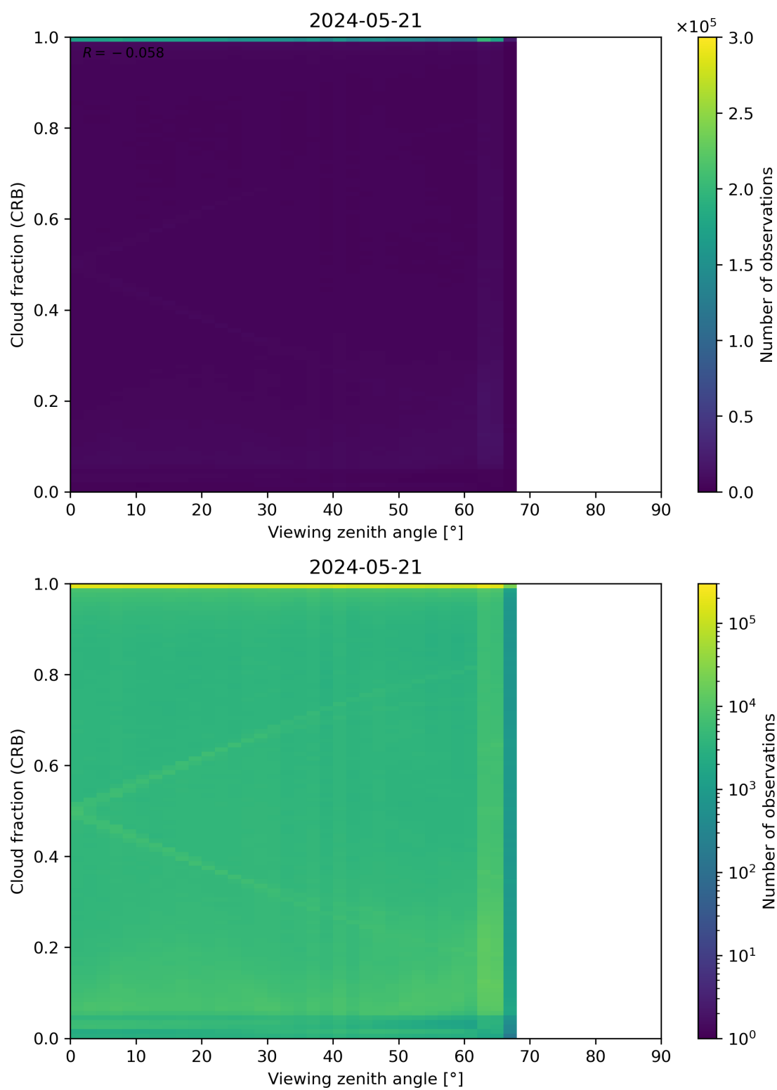
Figure 109: Scatter density plot of “Viewing zenith angle” against “Cloud fraction (CRB)” for 2024-05-20 to 2024-05-22.
