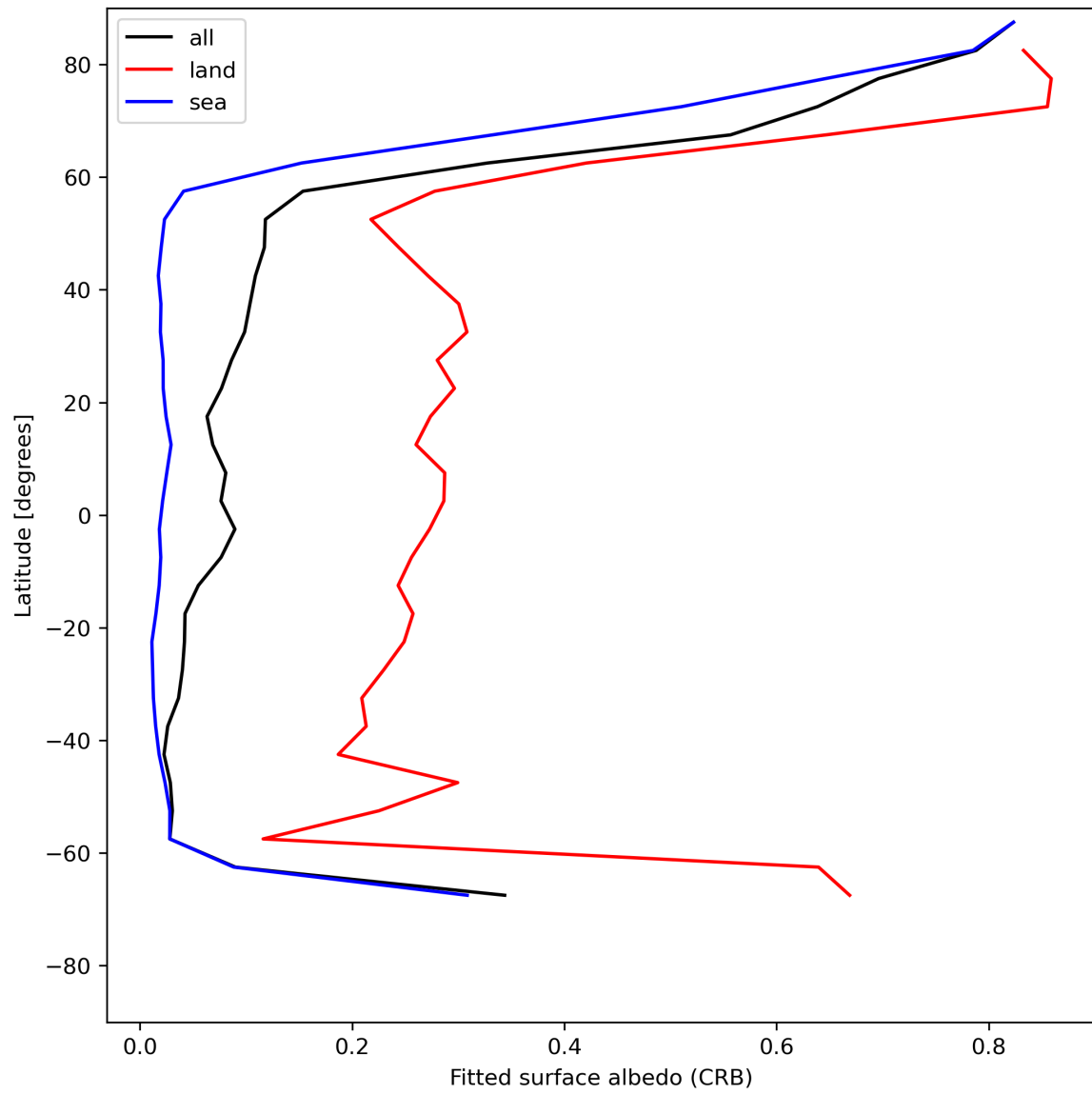
Figure 30: Zonal average of “Fitted surface albedo (CRB)” for 2024-05-20 to 2024-05-22.
