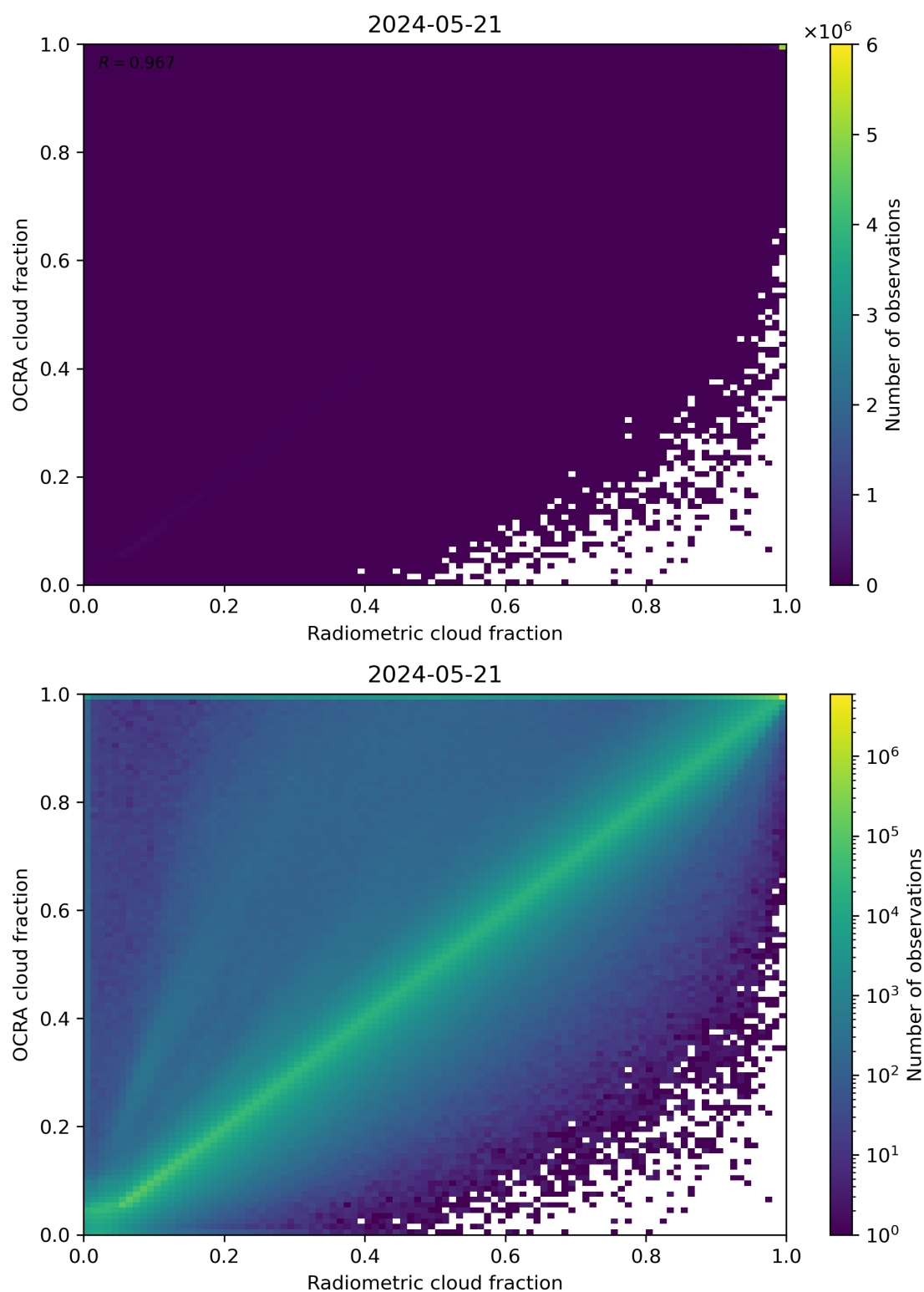
Figure 72: Scatter density plot of “Radiometric cloud fraction” against “OCRA cloud fraction” for 2024-05-20 to 2024-05-22.
