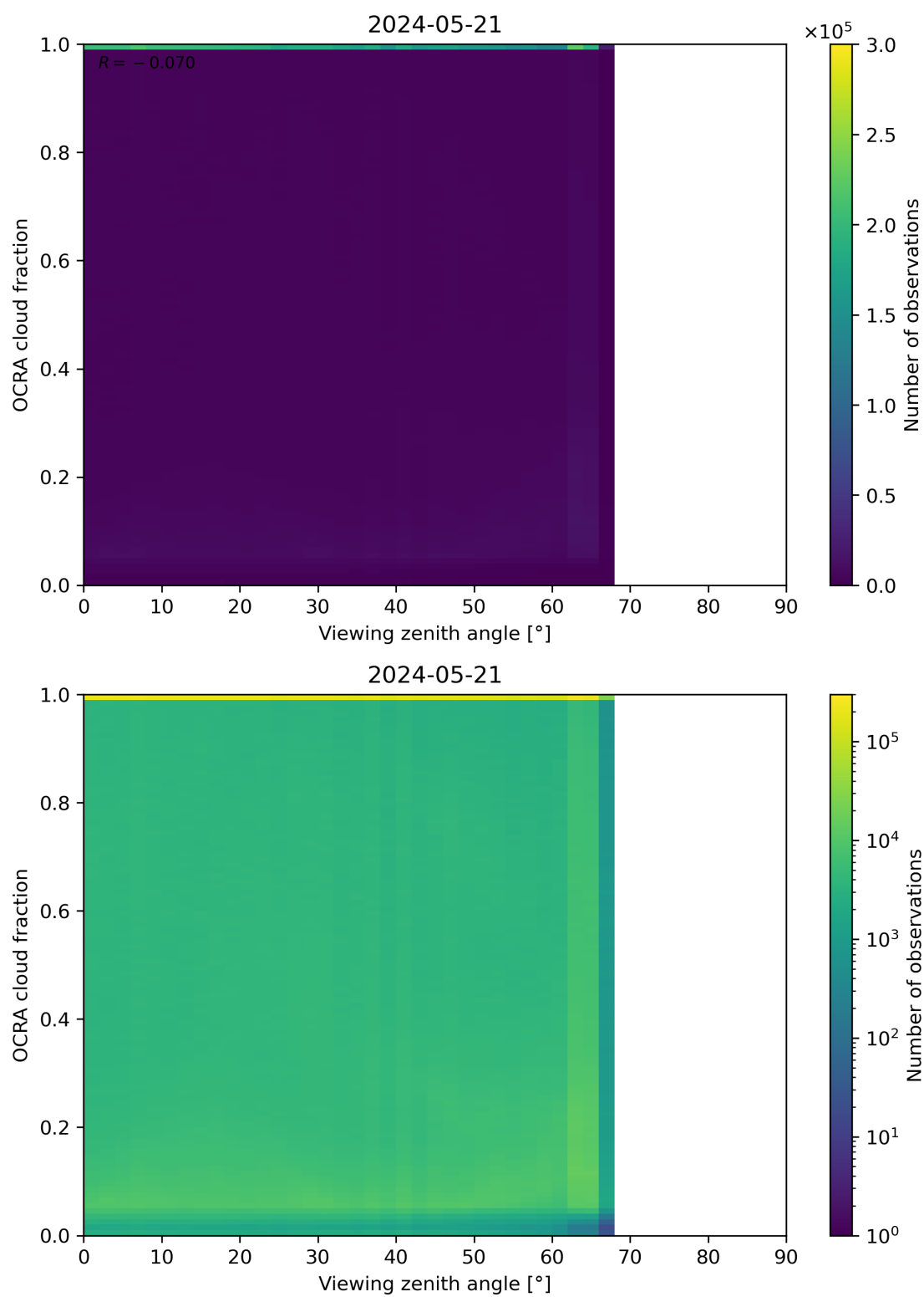
Figure 108: Scatter density plot of “Viewing zenith angle” against “OCRA cloud fraction” for 2024-05-20 to 2024-05-22.
