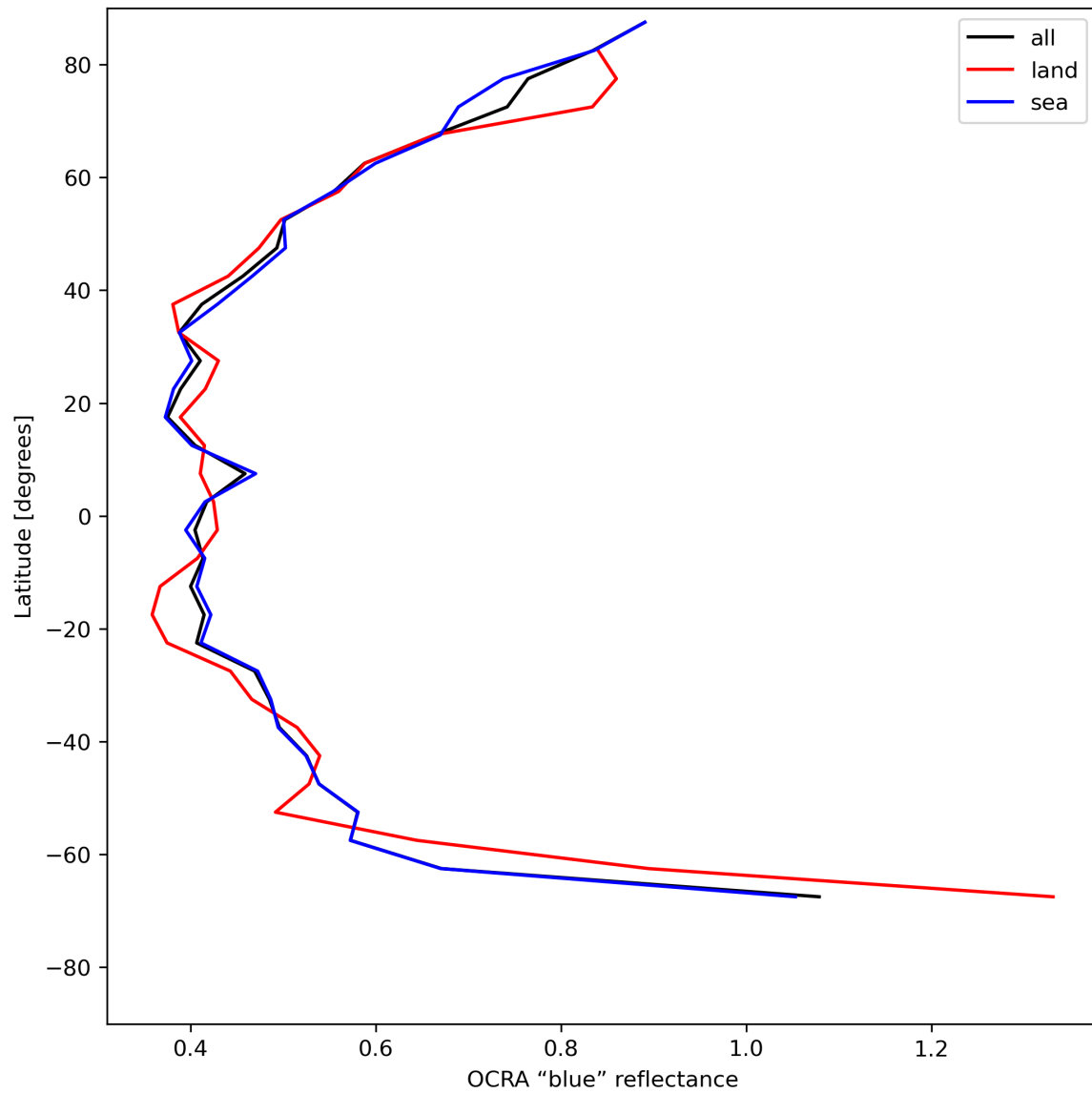
Figure 35: Zonal average of “OCRA “blue” reflectance” for 2024-05-20 to 2024-05-22.
