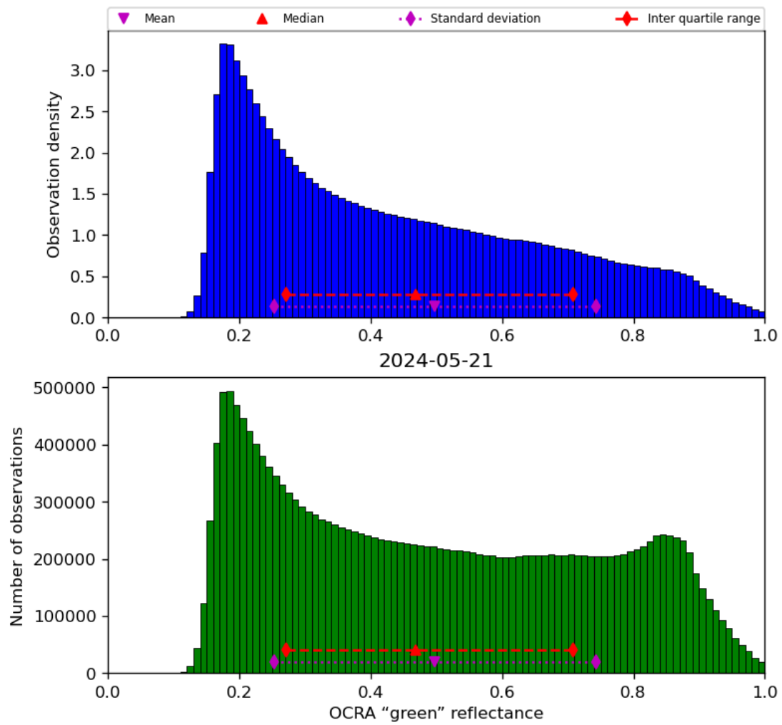
Figure 52: Histogram of “OCRA “green” reflectance” for 2024-05-20 to 2024-05-22
