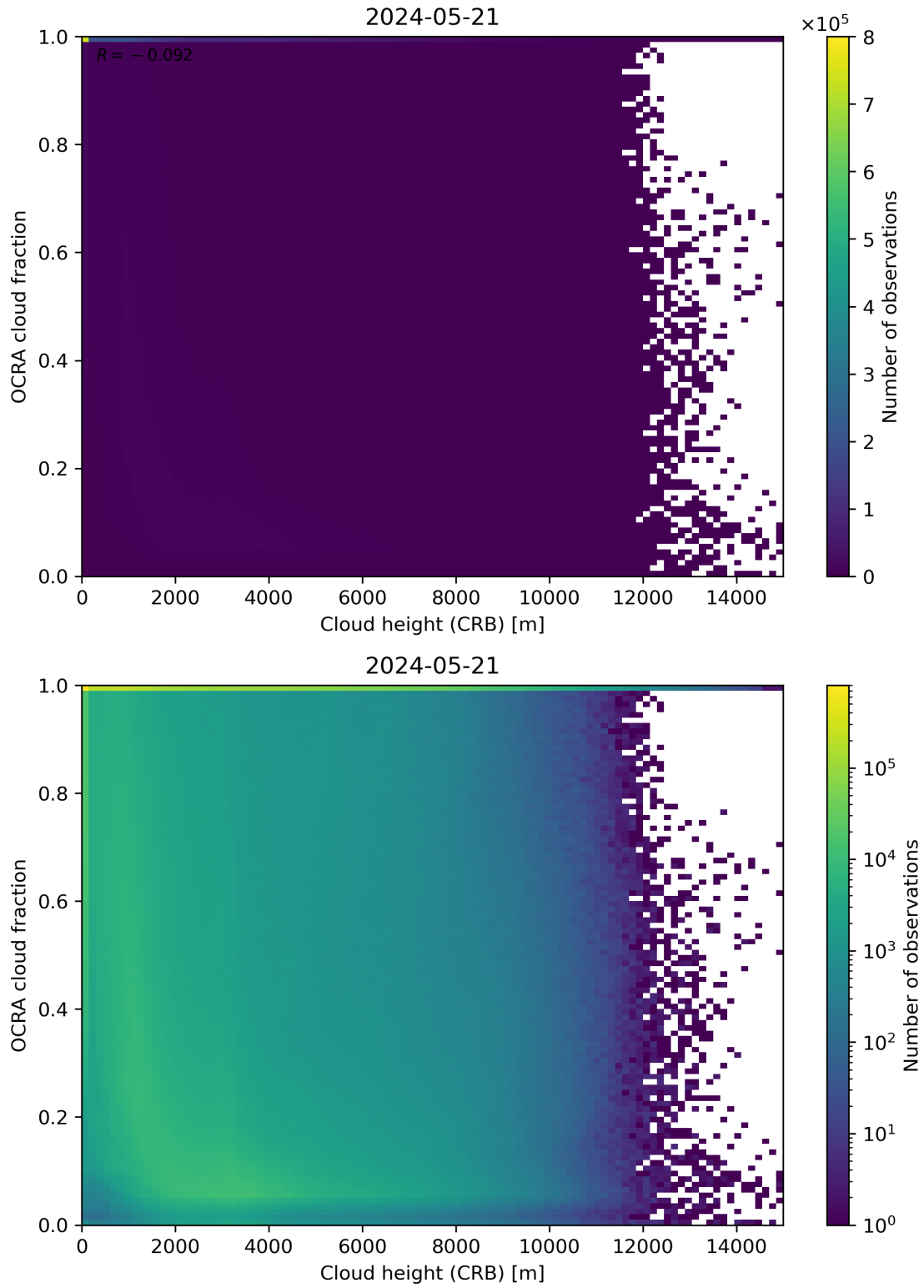
Figure 81: Scatter density plot of “Cloud height (CRB)” against “OCRA cloud fraction” for 2024-05-20 to 2024-05-22.
