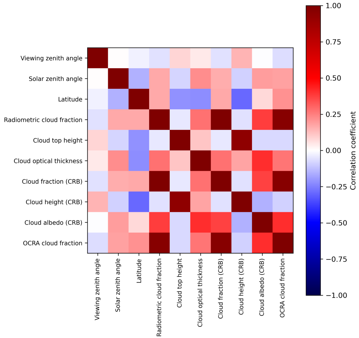
Figure 2: Map of correlation matrix for 2024-05-20 to 2024-05-22.
