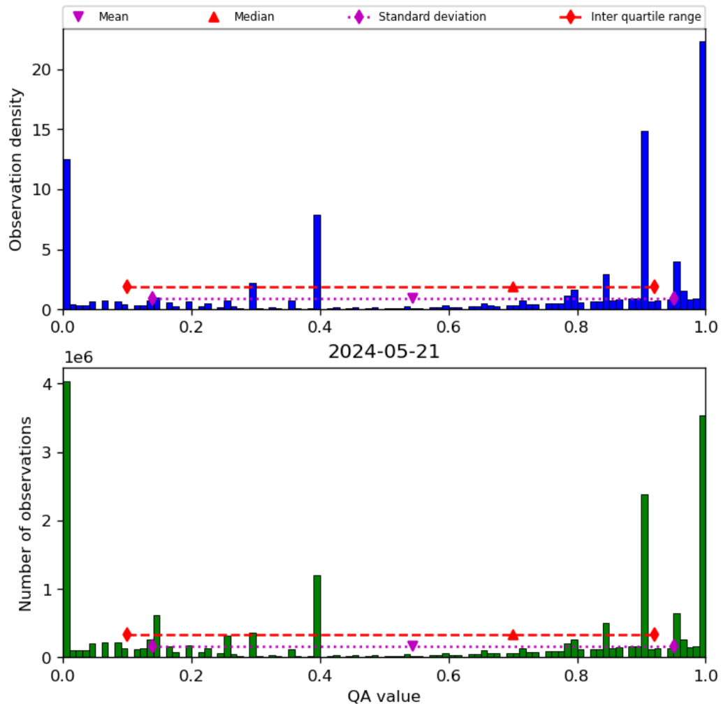
Figure 38: Histogram of “QA value” for 2024-05-20 to 2024-05-22
