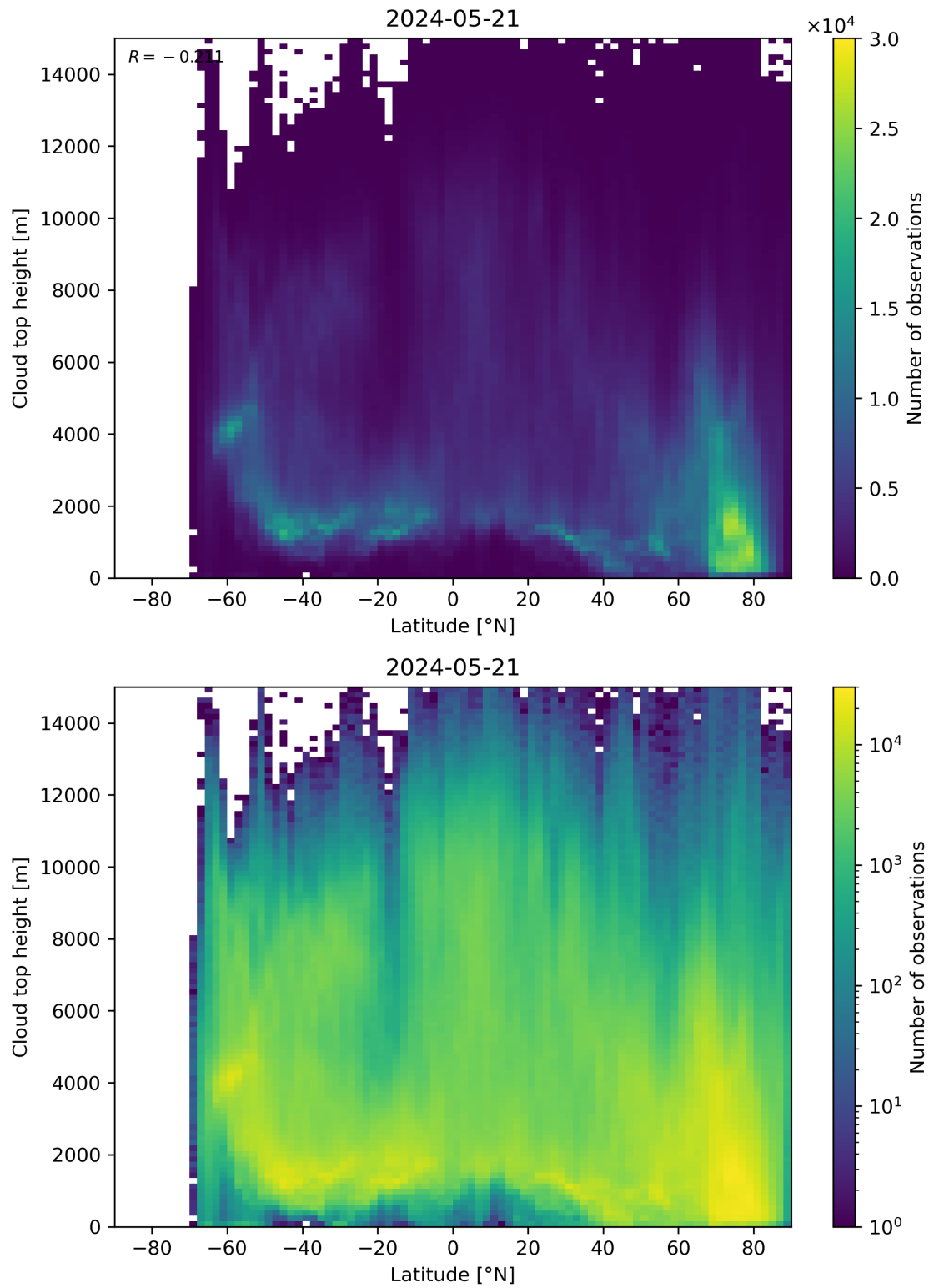
Figure 97: Scatter density plot of “Latitude” against “Cloud top height” for 2024-05-20 to 2024-05-22.
