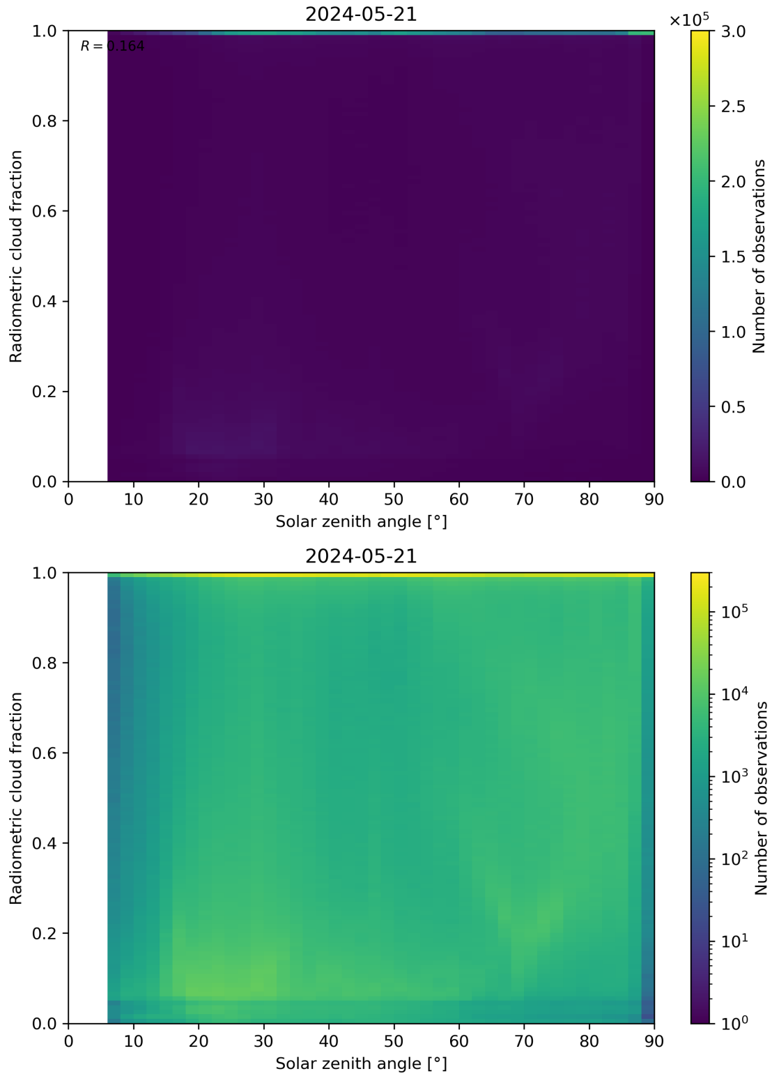
Figure 99: Scatter density plot of “Solar zenith angle” against “Radiometric cloud fraction” for 2024-05-20 to 2024-05-22.
