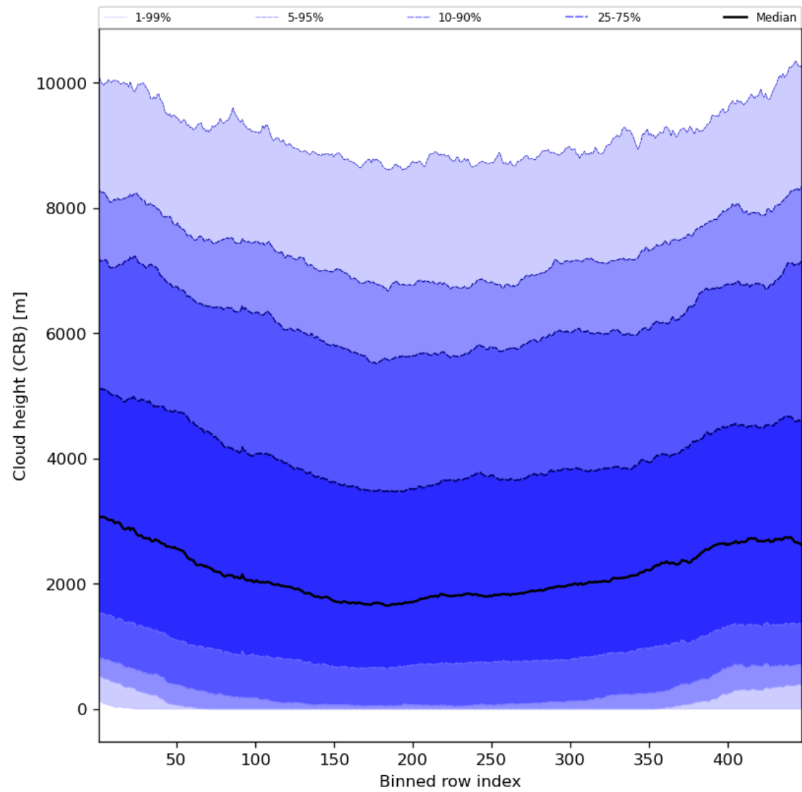
Figure 59: Along track statistics of “Cloud height (CRB)” for 2024-05-20 to 2024-05-22
