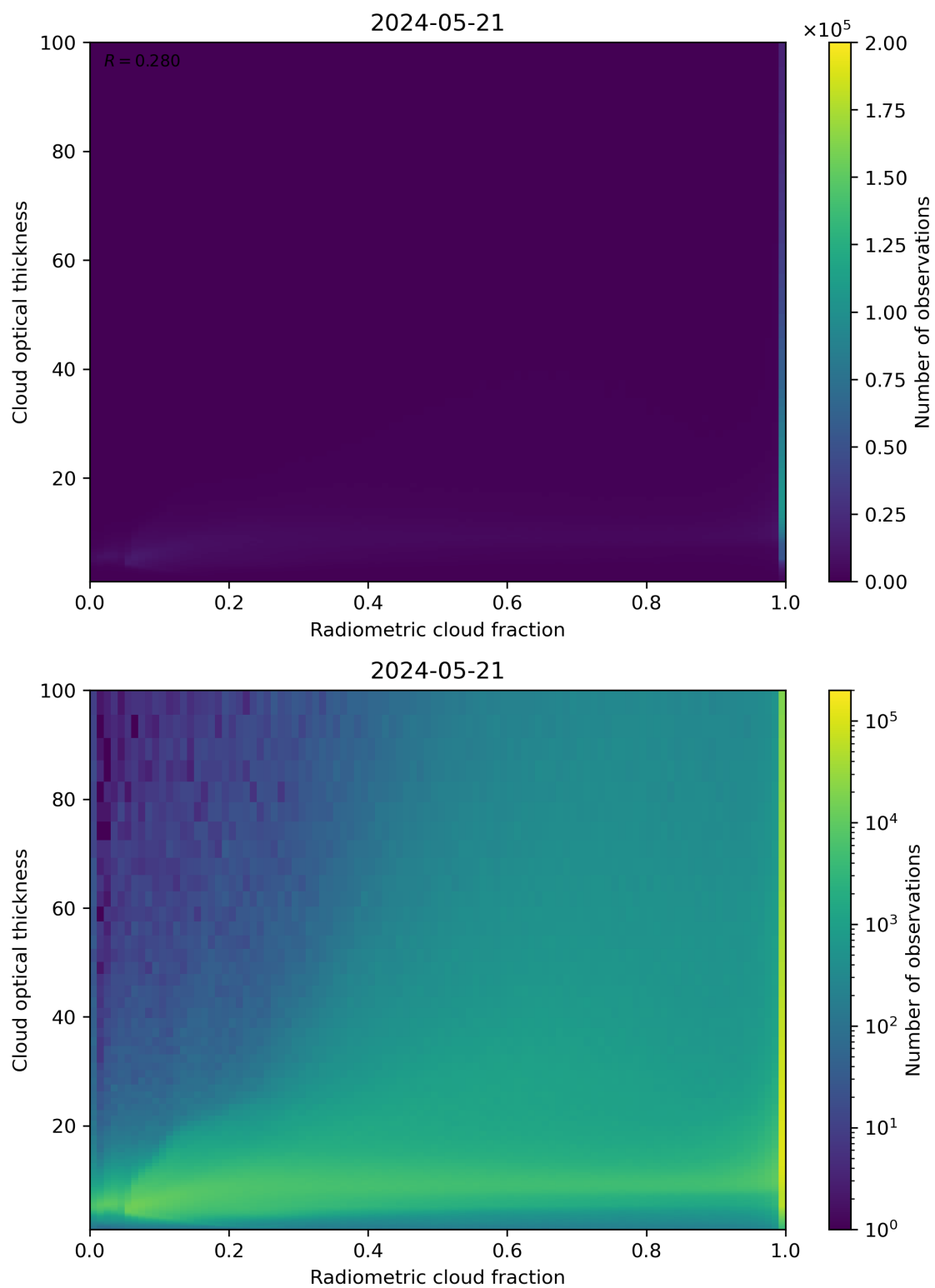
Figure 75: Scatter density plot of “Radiometric cloud fraction” against “Cloud optical thickness” for 2024-05-20 to 2024-05-22.
