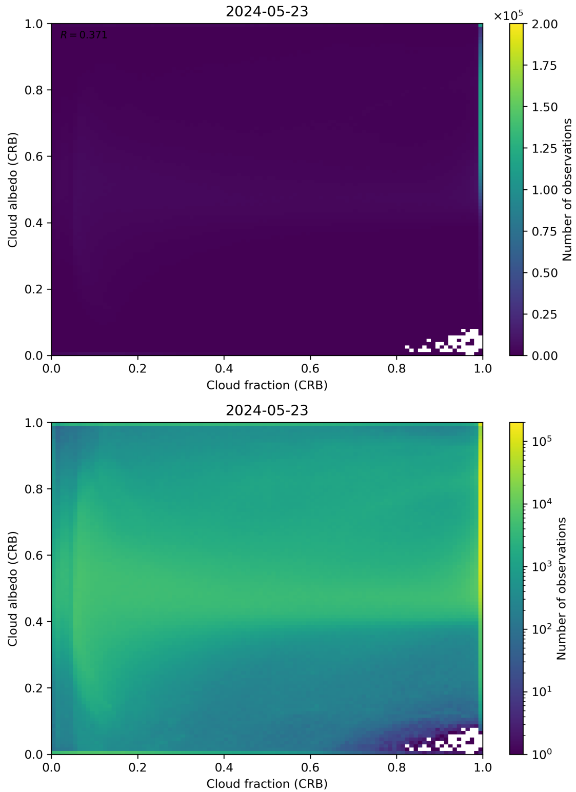
Figure 77: Scatter density plot of “Cloud fraction (CRB)” against “Cloud albedo (CRB)” for 2024-05-23 to 2024-05-24.
