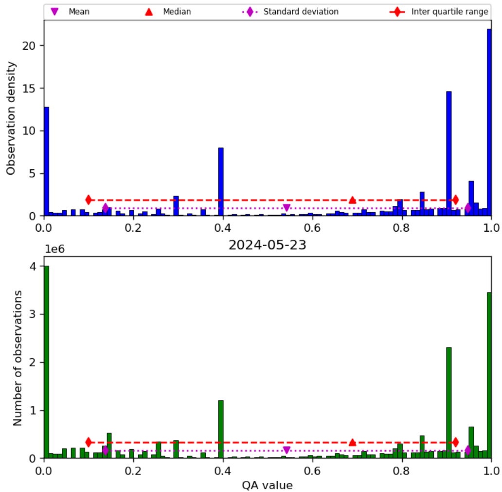
Figure 38: Histogram of “QA value” for 2024-05-23 to 2024-05-24
