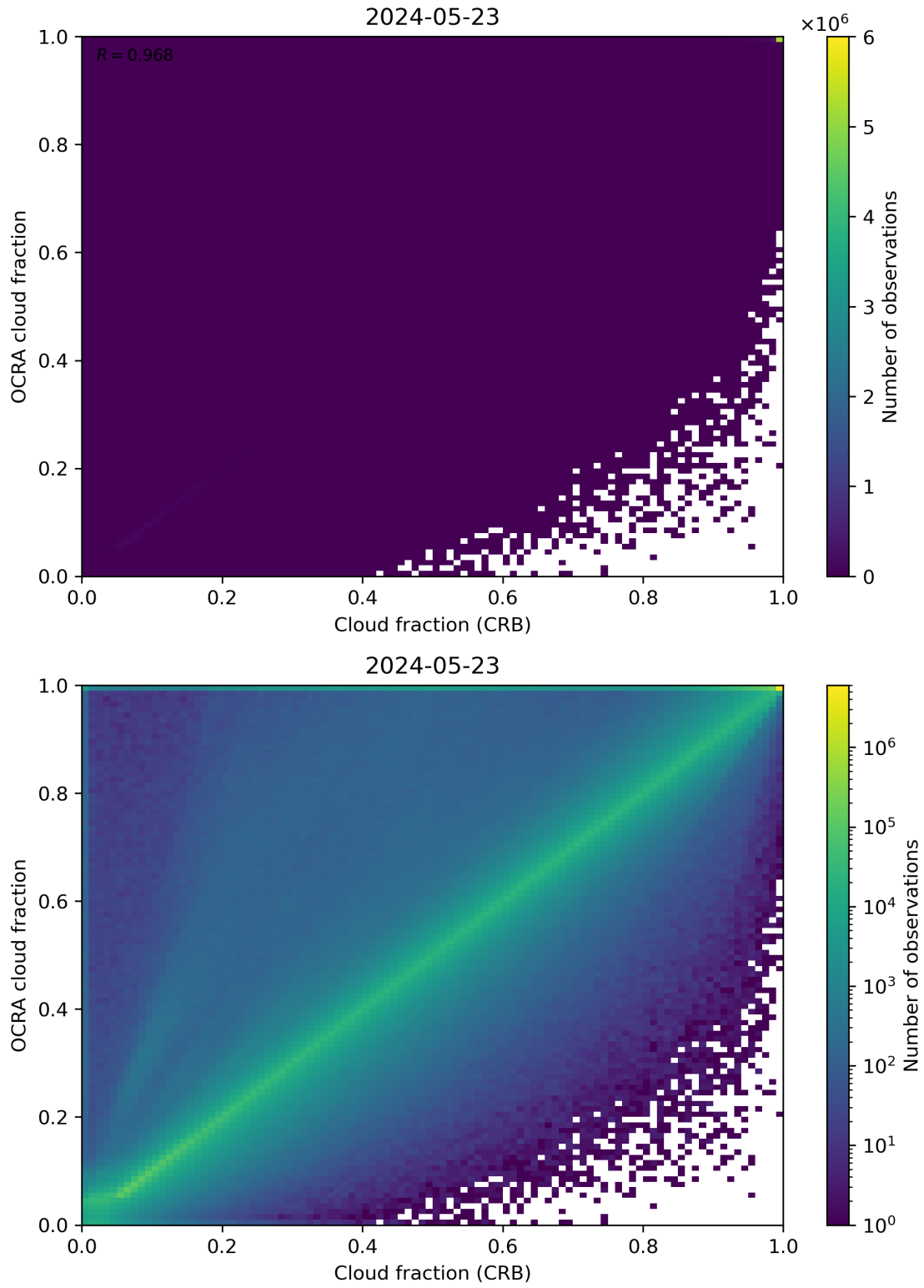
Figure 78: Scatter density plot of “Cloud fraction (CRB)” against “OCRA cloud fraction” for 2024-05-23 to 2024-05-24.
