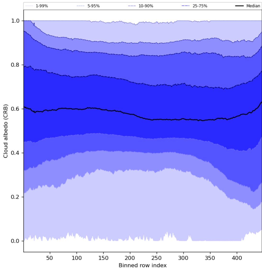
Figure 60: Along track statistics of “Cloud albedo (CRB)” for 2024-05-23 to 2024-05-24
