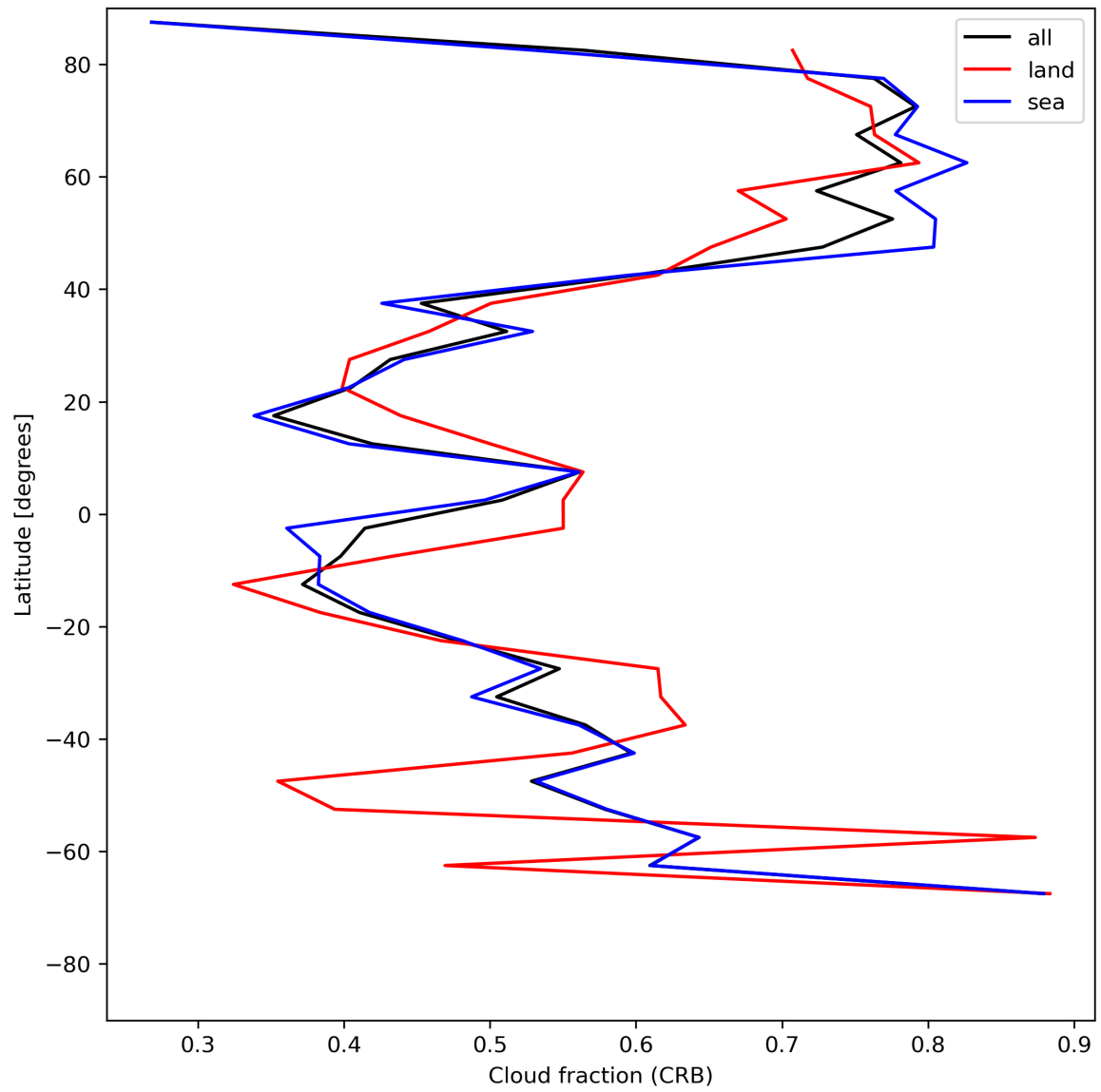
Figure 26: Zonal average of “Cloud fraction (CRB)” for 2024-05-23 to 2024-05-24.
