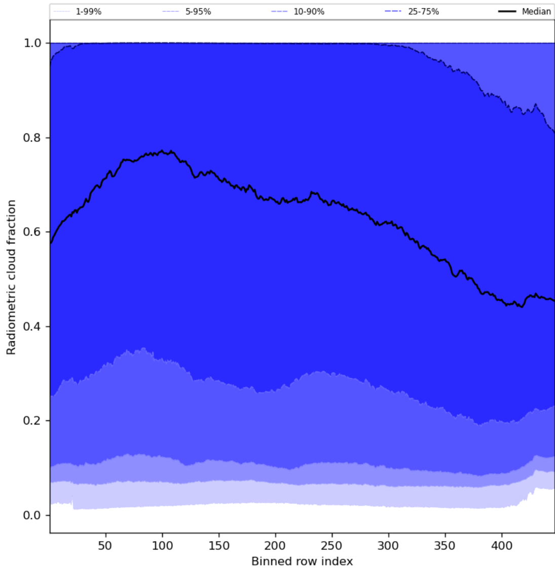
Figure 55: Along track statistics of “Radiometric cloud fraction” for 2024-05-23 to 2024-05-24
