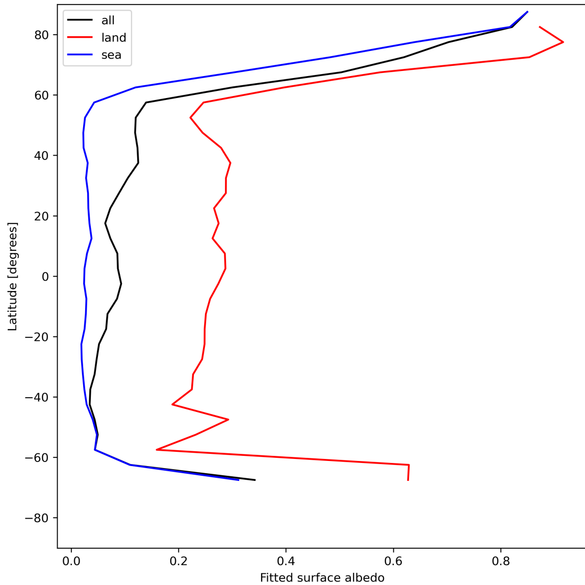
Figure 29: Zonal average of “Fitted surface albedo” for 2024-05-23 to 2024-05-24.
