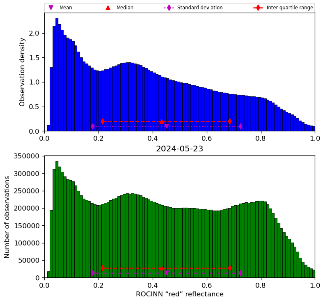
Figure 53: Histogram of “ROCINN “red” reflectance” for 2024-05-23 to 2024-05-24
