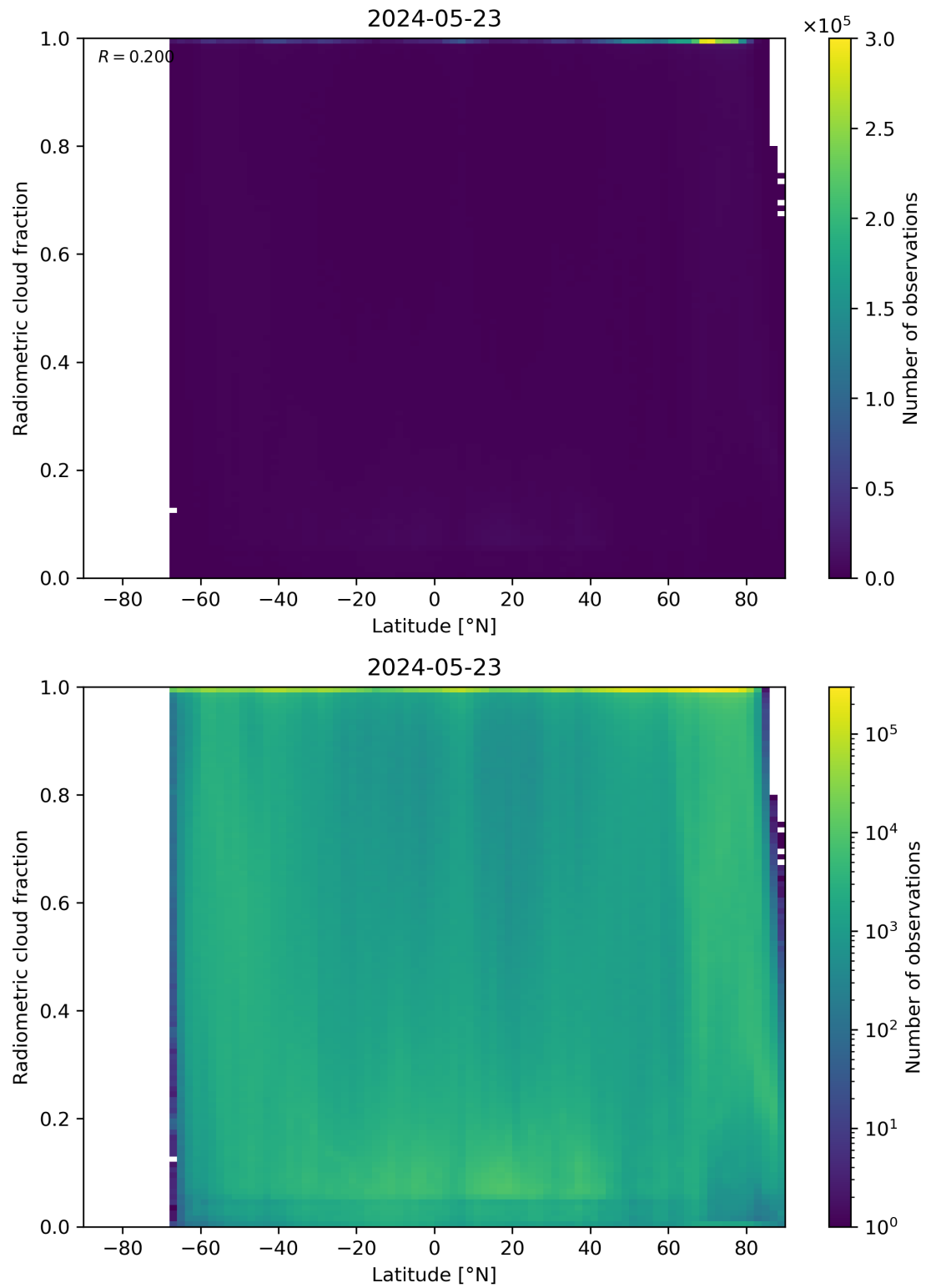
Figure 92: Scatter density plot of “Latitude” against “Radiometric cloud fraction” for 2024-05-23 to 2024-05-24.
