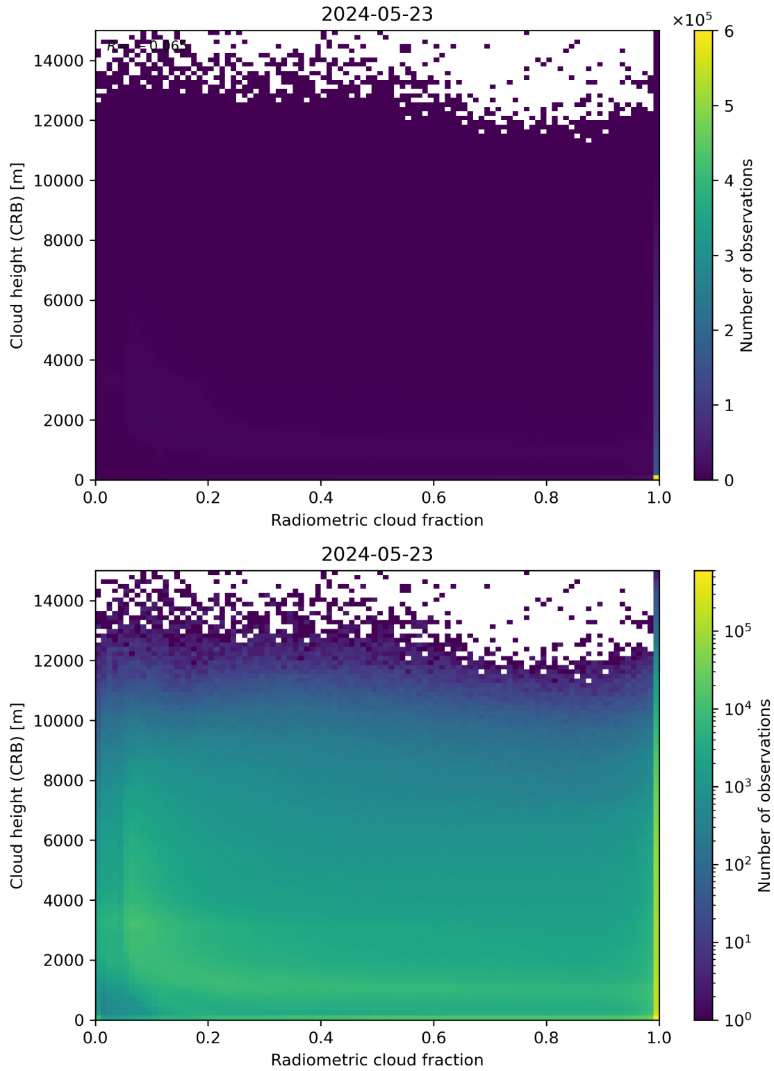
Figure 74: Scatter density plot of “Radiometric cloud fraction” against “Cloud height (CRB)” for 2024-05-23 to 2024-05-24.
