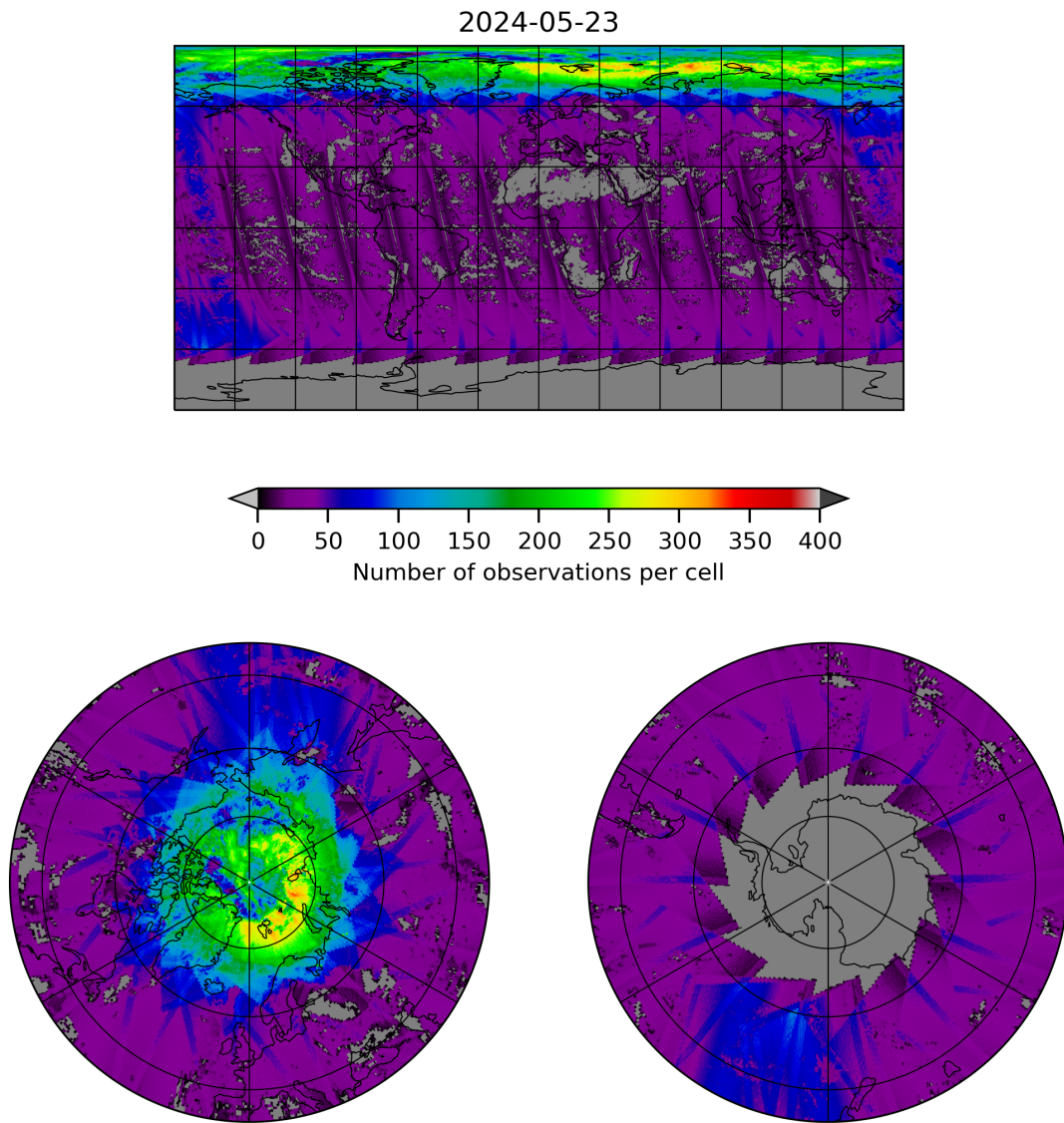
Figure 21: Map of the number of observations for 2024-05-23 to 2024-05-24
