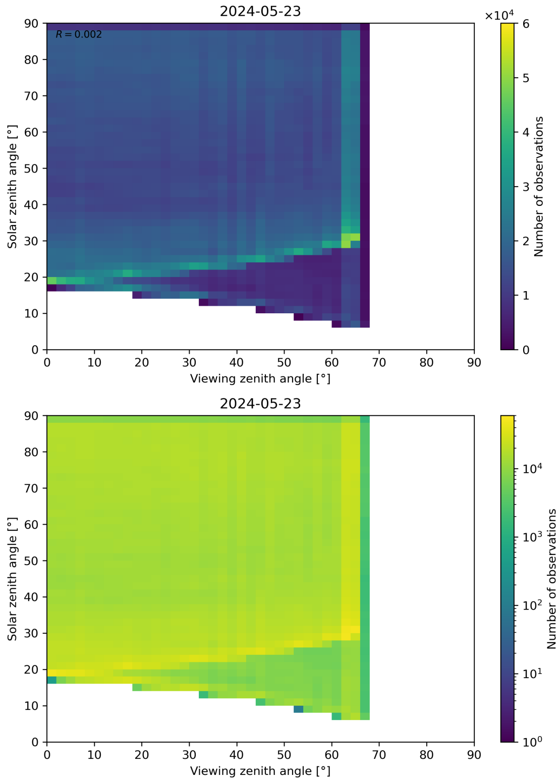
Figure 114: Scatter density plot of “Viewing zenith angle” against “Solar zenith angle” for 2024-05-23 to 2024-05-24.
