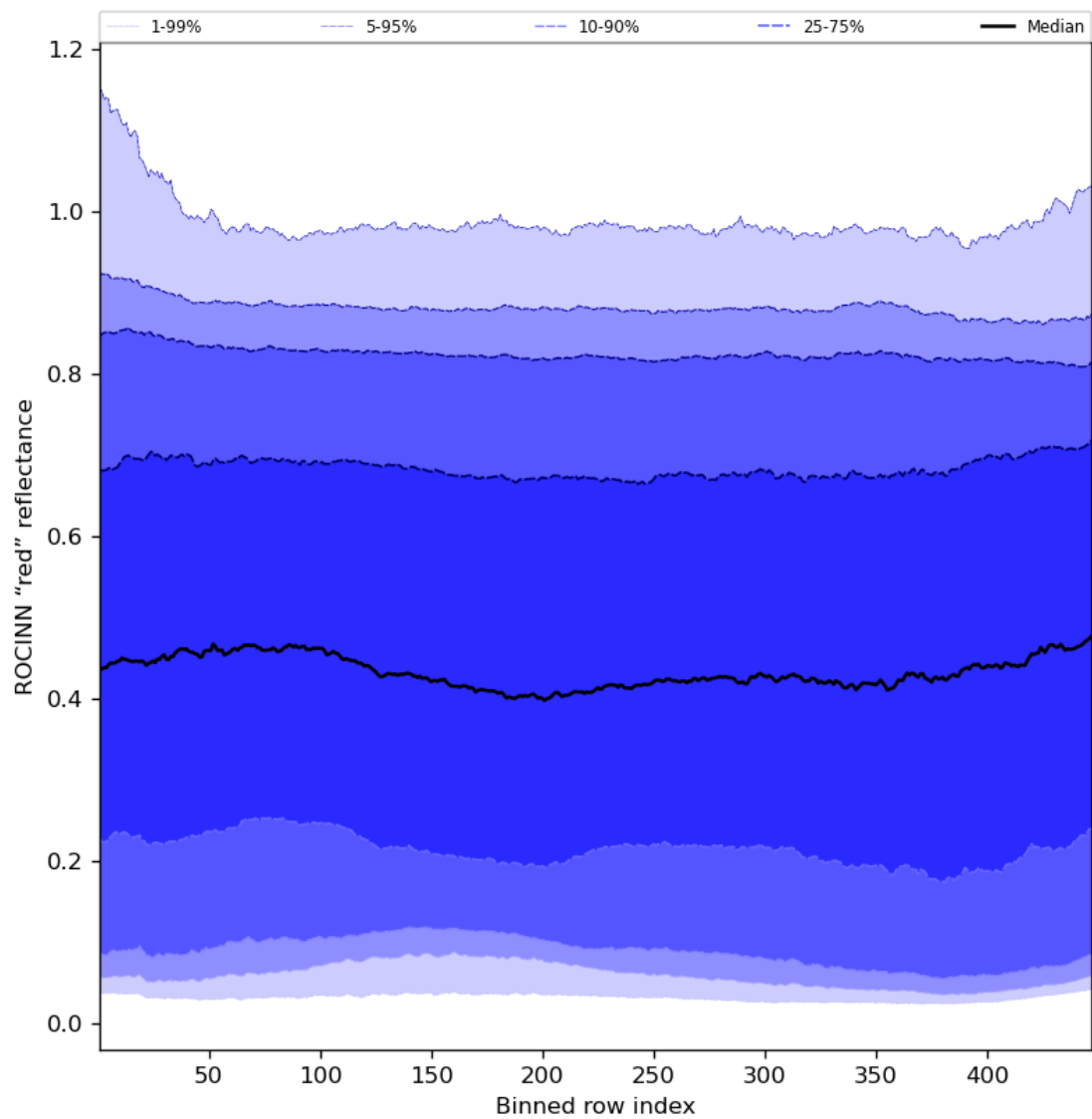
Figure 69: Along track statistics of “ROCINN “red” reflectance” for 2024-05-23 to 2024-05-24
