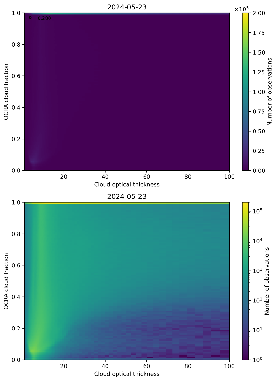
Figure 83: Scatter density plot of “Cloud optical thickness” against “OCRA cloud fraction” for 2024-05-23 to 2024-05-24.
