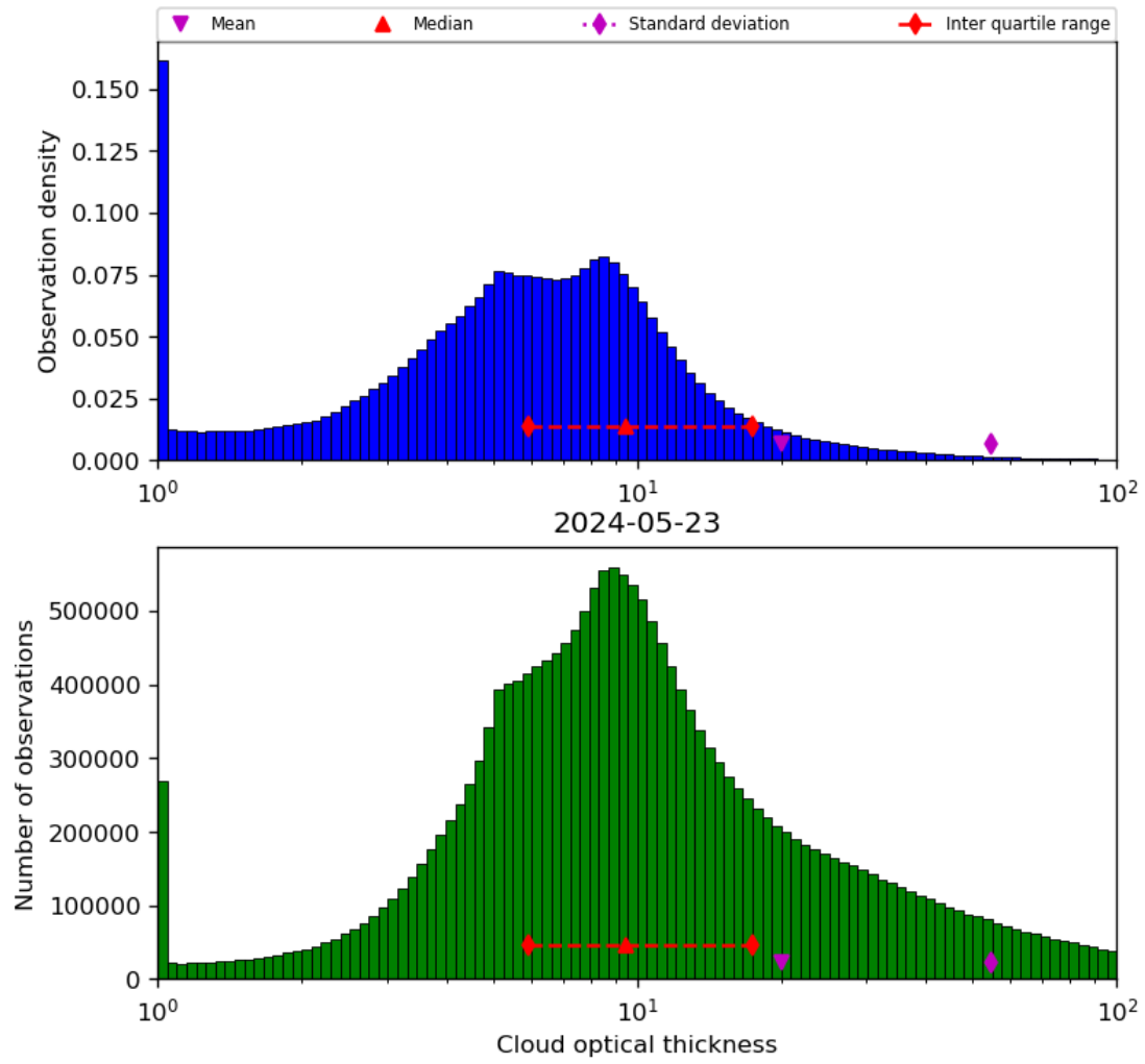
Figure 41: Histogram of “Cloud optical thickness” for 2024-05-23 to 2024-05-24
