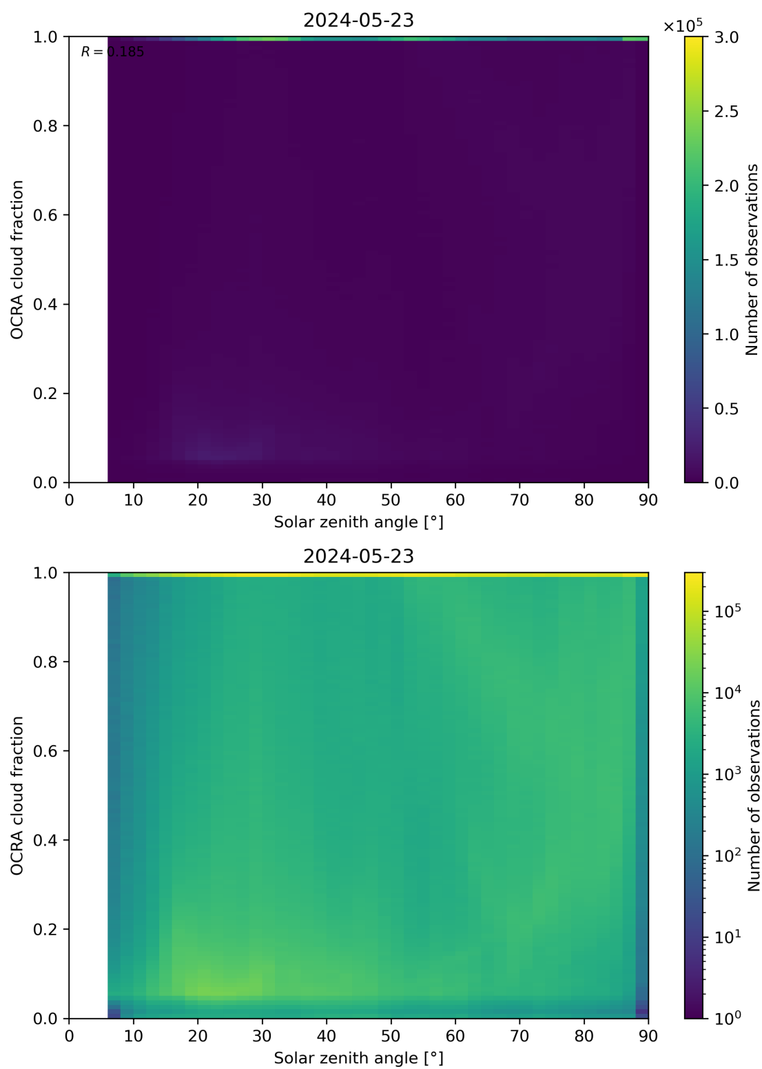
Figure 100: Scatter density plot of “Solar zenith angle” against “OCRA cloud fraction” for 2024-05-23 to 2024-05-24.
