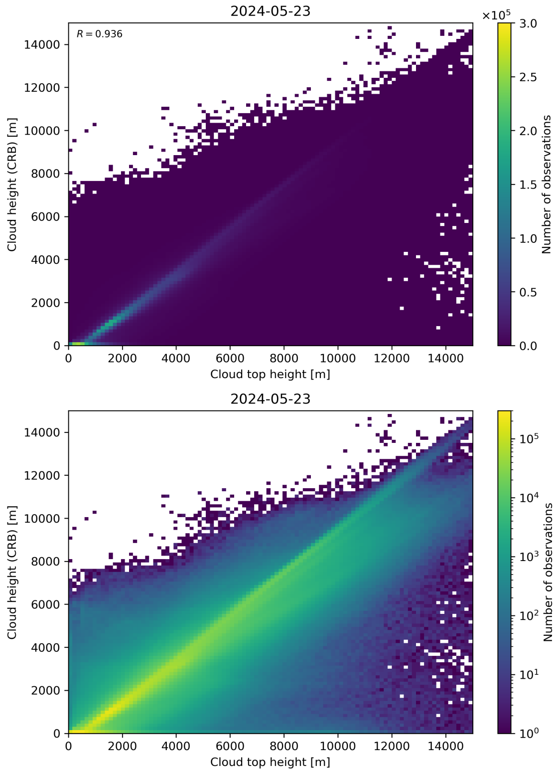
Figure 89: Scatter density plot of “Cloud top height” against “Cloud height (CRB)” for 2024-05-23 to 2024-05-24.
