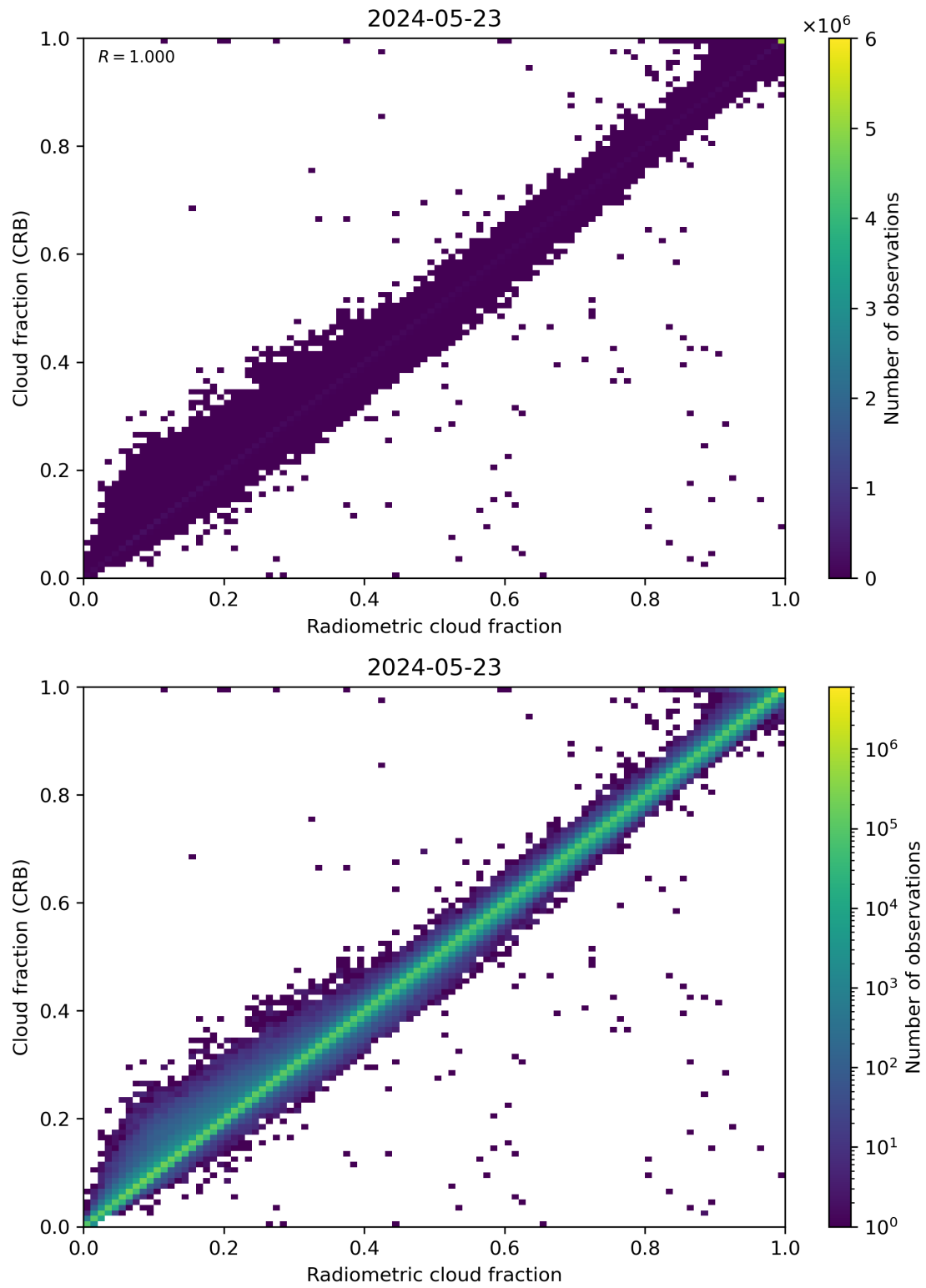
Figure 73: Scatter density plot of “Radiometric cloud fraction” against “Cloud fraction (CRB)” for 2024-05-23 to 2024-05-24.
