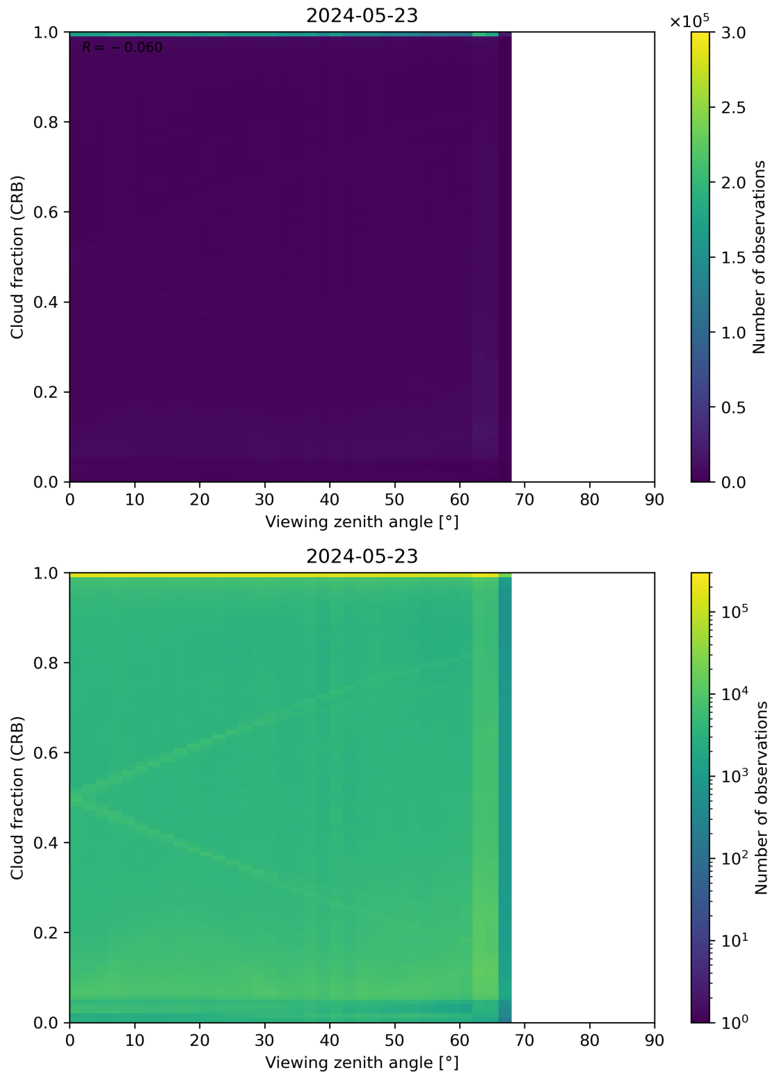
Figure 109: Scatter density plot of “Viewing zenith angle” against “Cloud fraction (CRB)” for 2024-05-23 to 2024-05-24.
