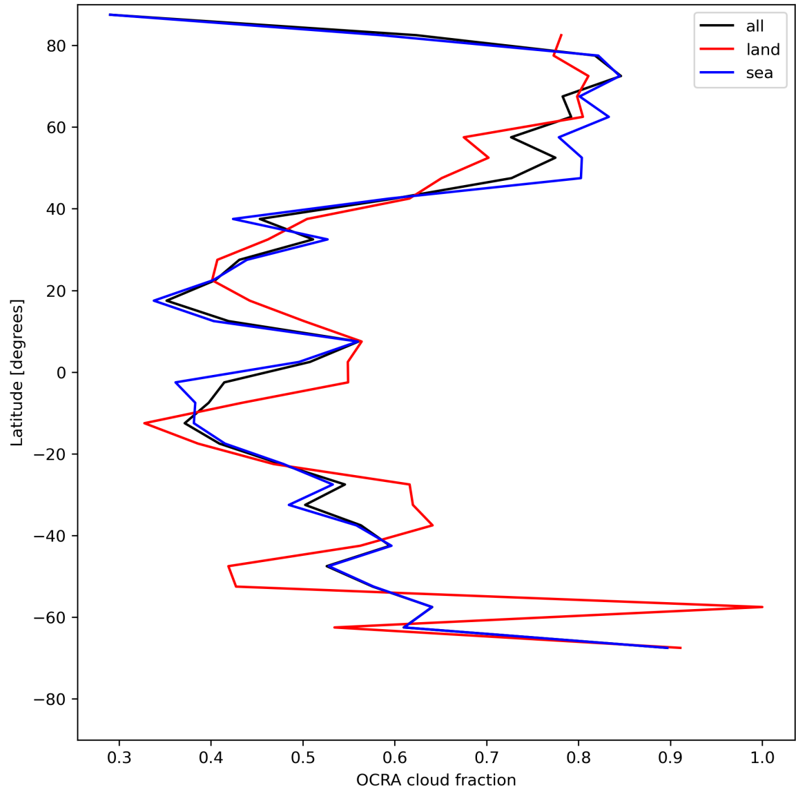
Figure 34: Zonal average of “OCRA cloud fraction” for 2024-05-23 to 2024-05-24.
