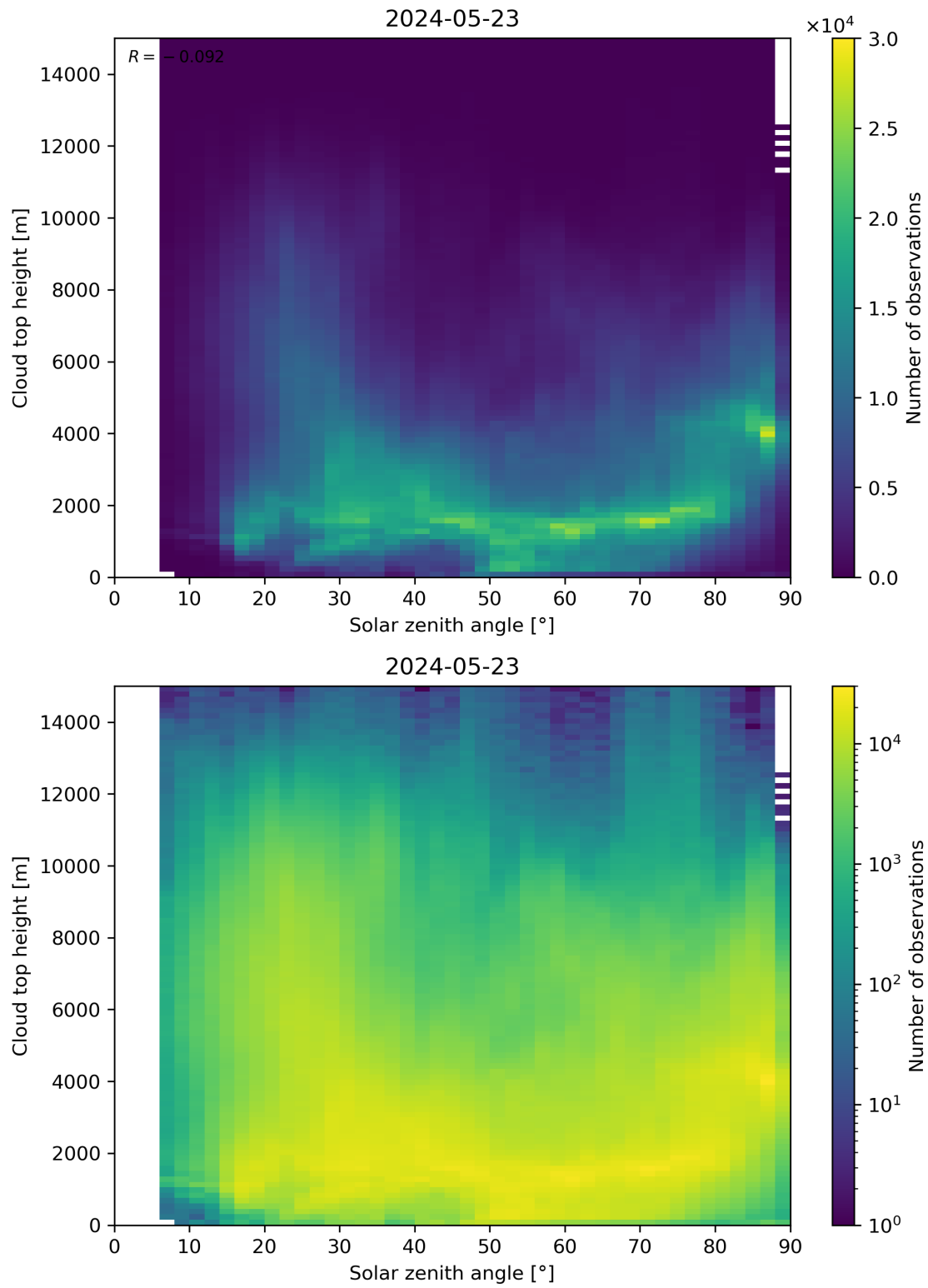
Figure 104: Scatter density plot of “Solar zenith angle” against “Cloud top height” for 2024-05-23 to 2024-05-24.
