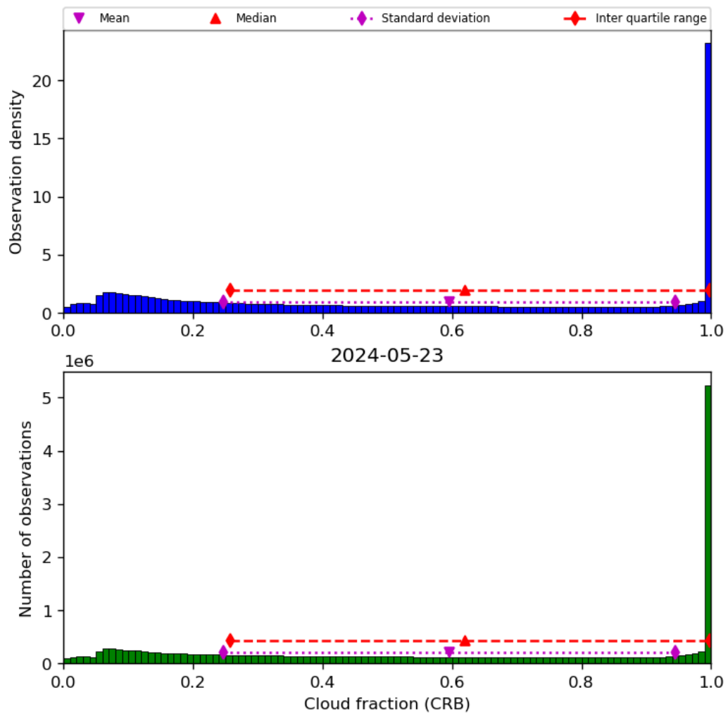
Figure 42: Histogram of “Cloud fraction (CRB)” for 2024-05-23 to 2024-05-24
