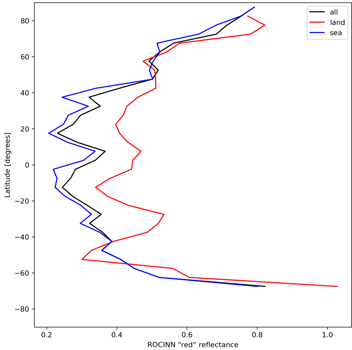
Figure 37: Zonal average of “ROCINN “red” reflectance” for 2024-05-23 to 2024-05-24.
