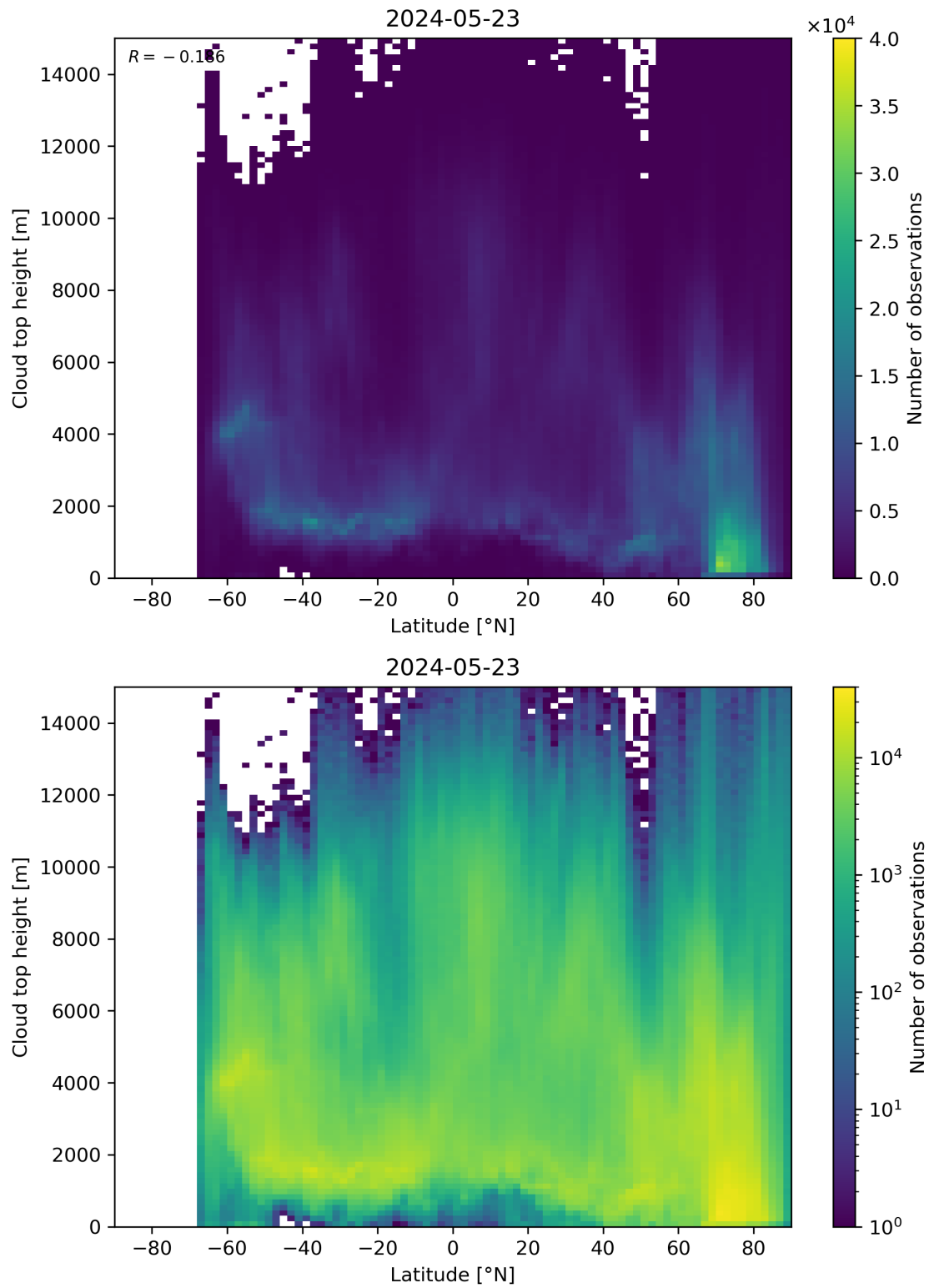
Figure 97: Scatter density plot of “Latitude” against “Cloud top height” for 2024-05-23 to 2024-05-24.
