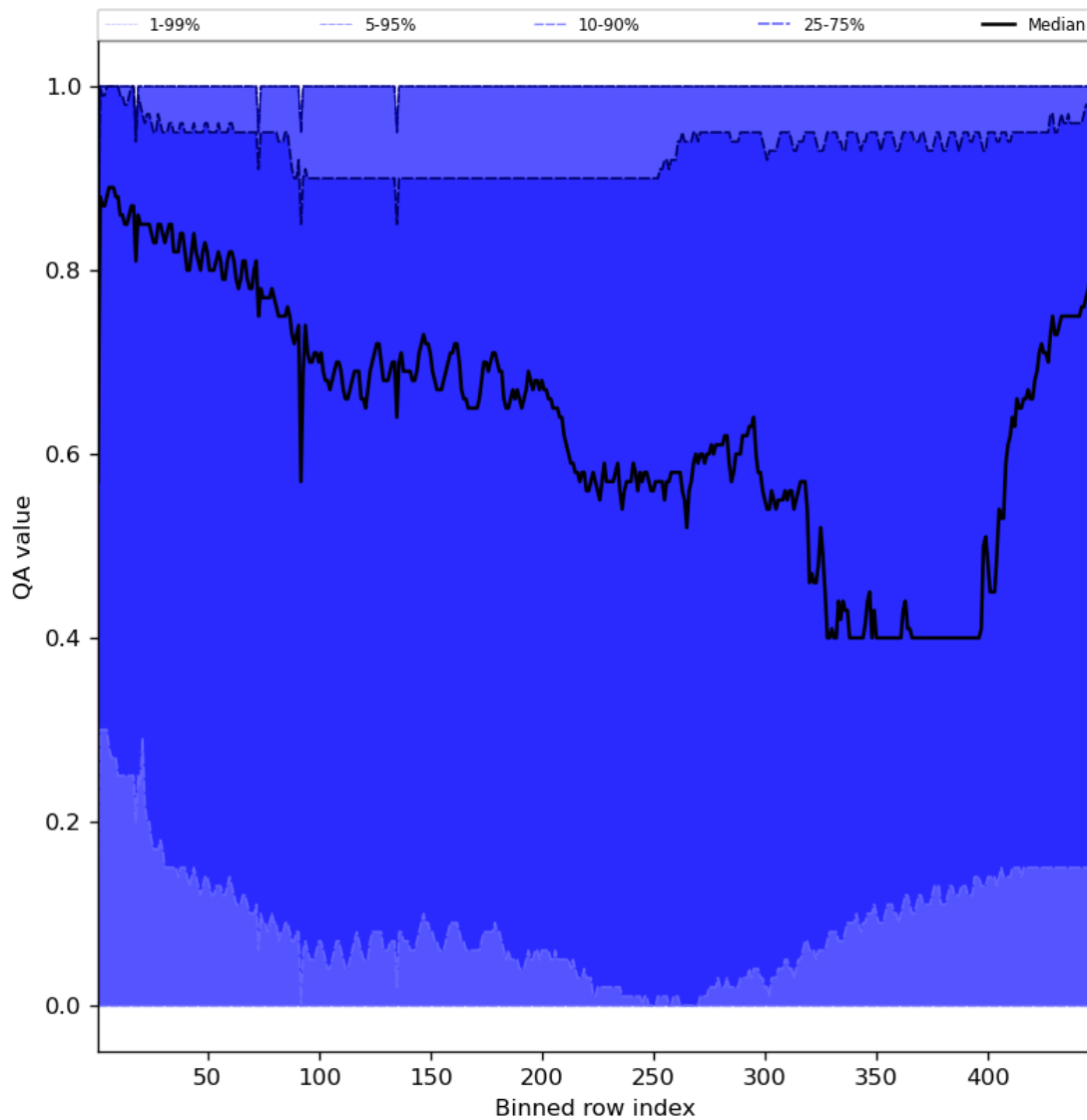
Figure 54: Along track statistics of “QA value” for 2024-05-23 to 2024-05-24
