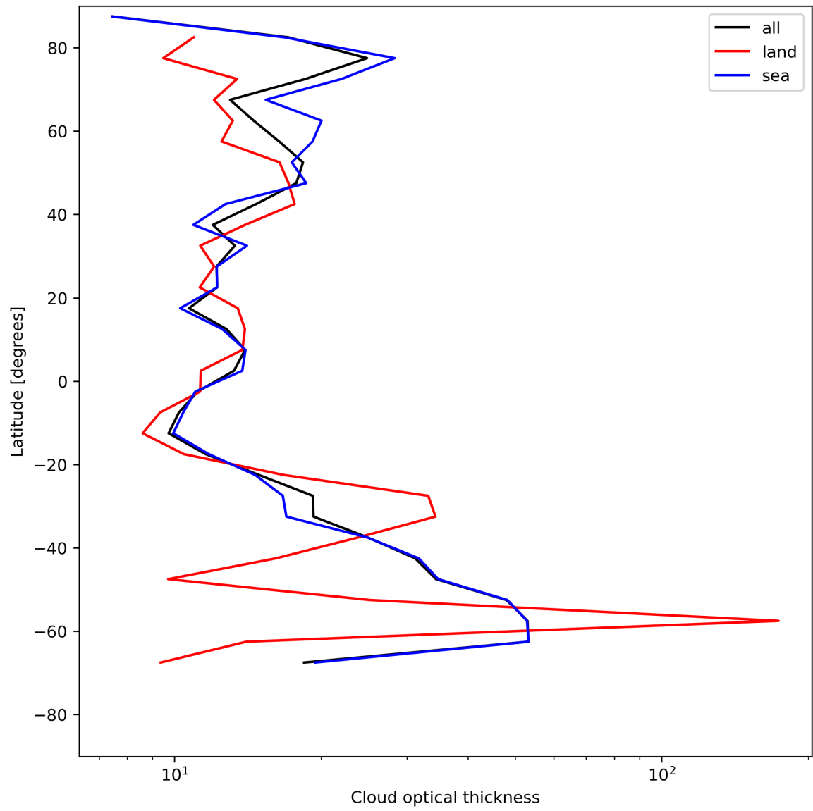
Figure 25: Zonal average of “Cloud optical thickness” for 2024-05-23 to 2024-05-24.
