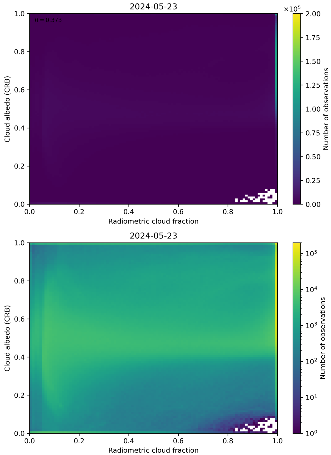
Figure 71: Scatter density plot of “Radiometric cloud fraction” against “Cloud albedo (CRB)” for 2024-05-23 to 2024-05-24.
