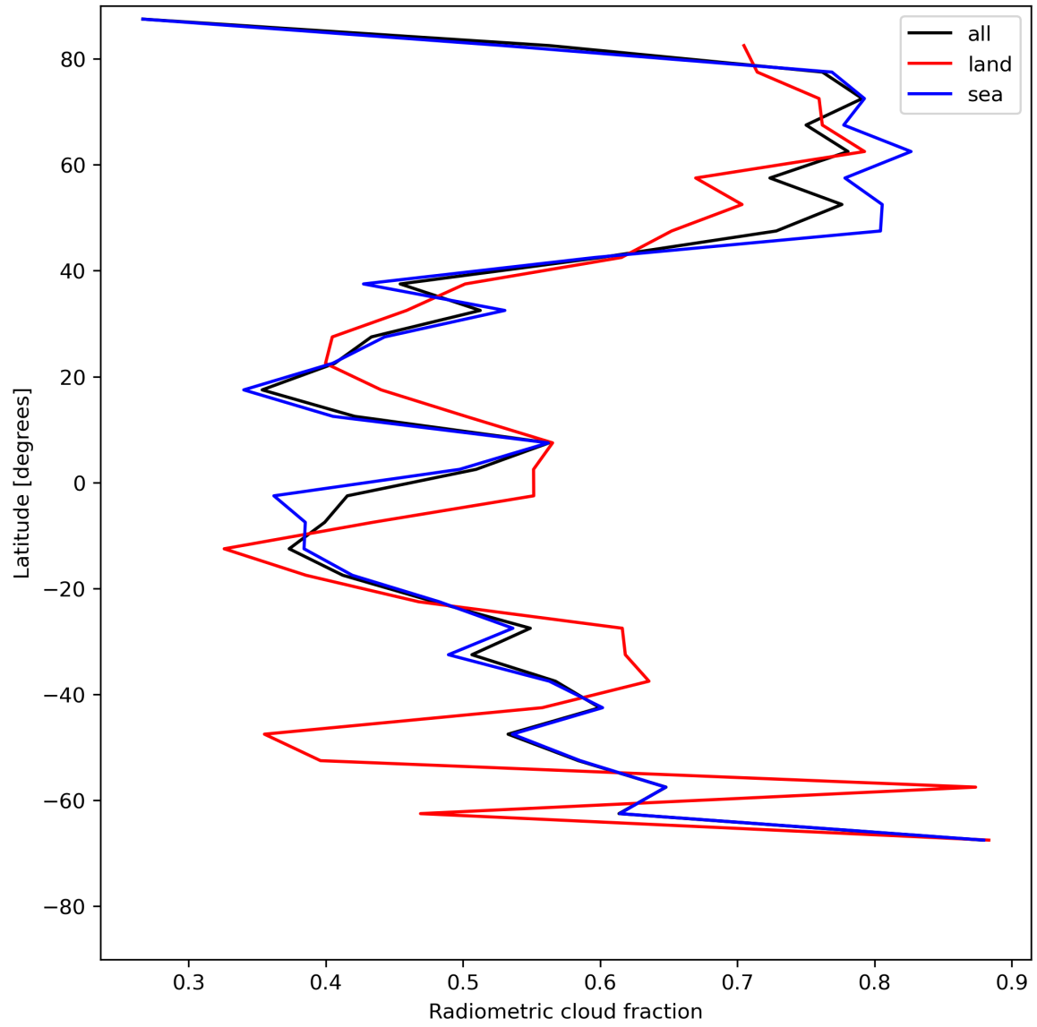
Figure 23: Zonal average of “Radiometric cloud fraction” for 2024-05-23 to 2024-05-24.
