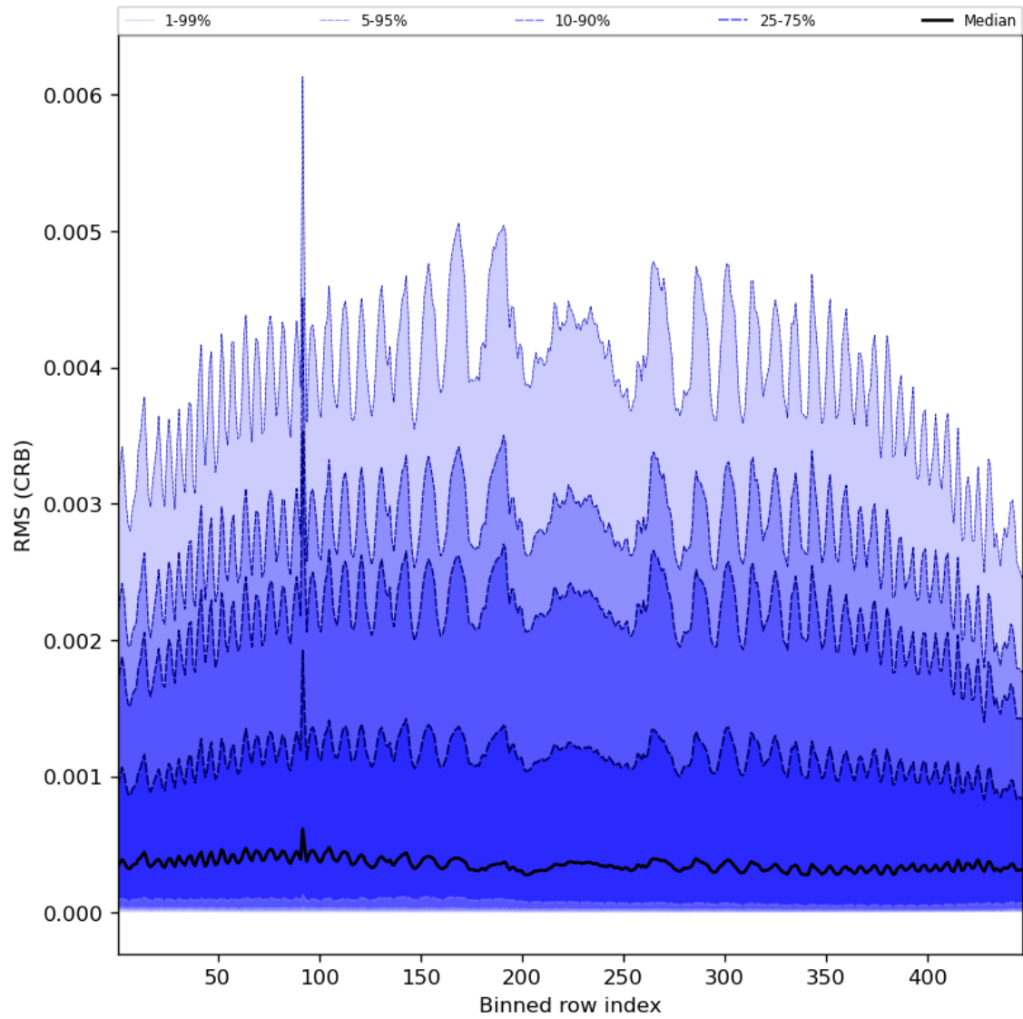
Figure 64: Along track statistics of “RMS (CRB)” for 2024-05-23 to 2024-05-24
