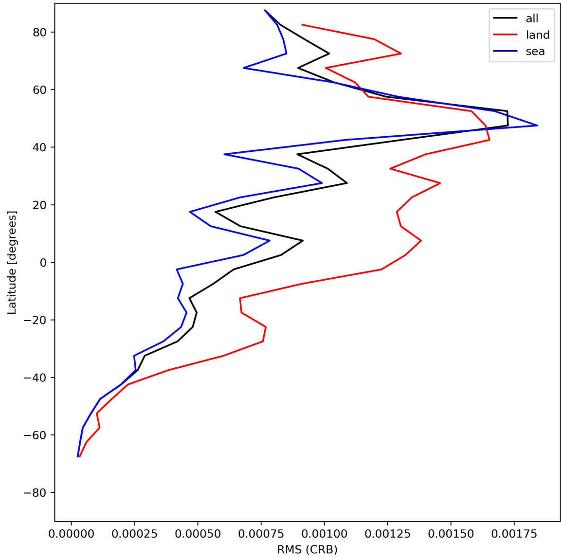
Figure 32: Zonal average of “RMS (CRB)” for 2024-05-23 to 2024-05-24.
