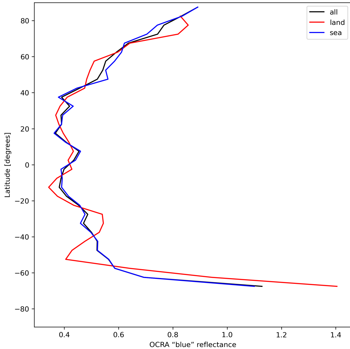
Figure 35: Zonal average of “OCRA “blue” reflectance” for 2024-05-23 to 2024-05-24.
