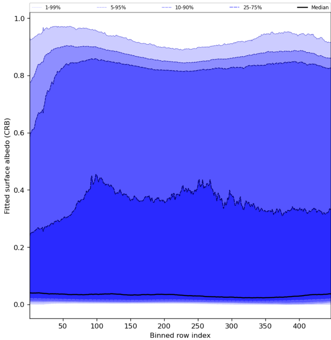
Figure 62: Along track statistics of “Fitted surface albedo (CRB)” for 2024-05-23 to 2024-05-24
