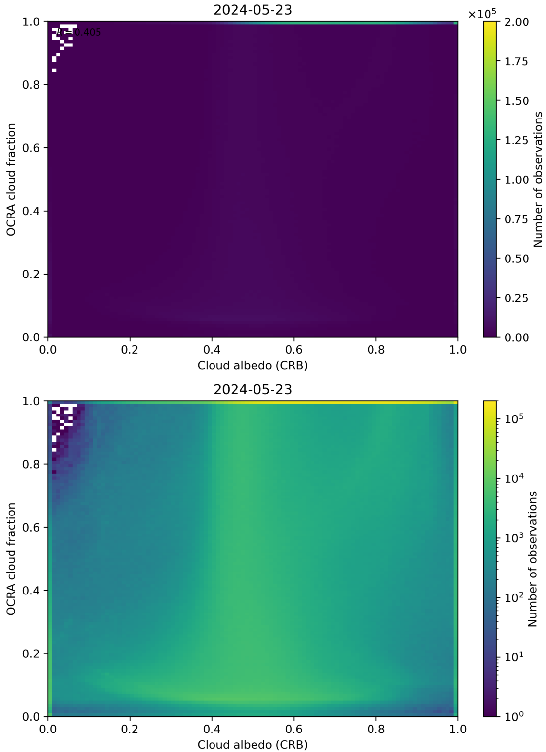
Figure 70: Scatter density plot of “Cloud albedo (CRB)” against “OCRA cloud fraction” for 2024-05-23 to 2024-05-24.
