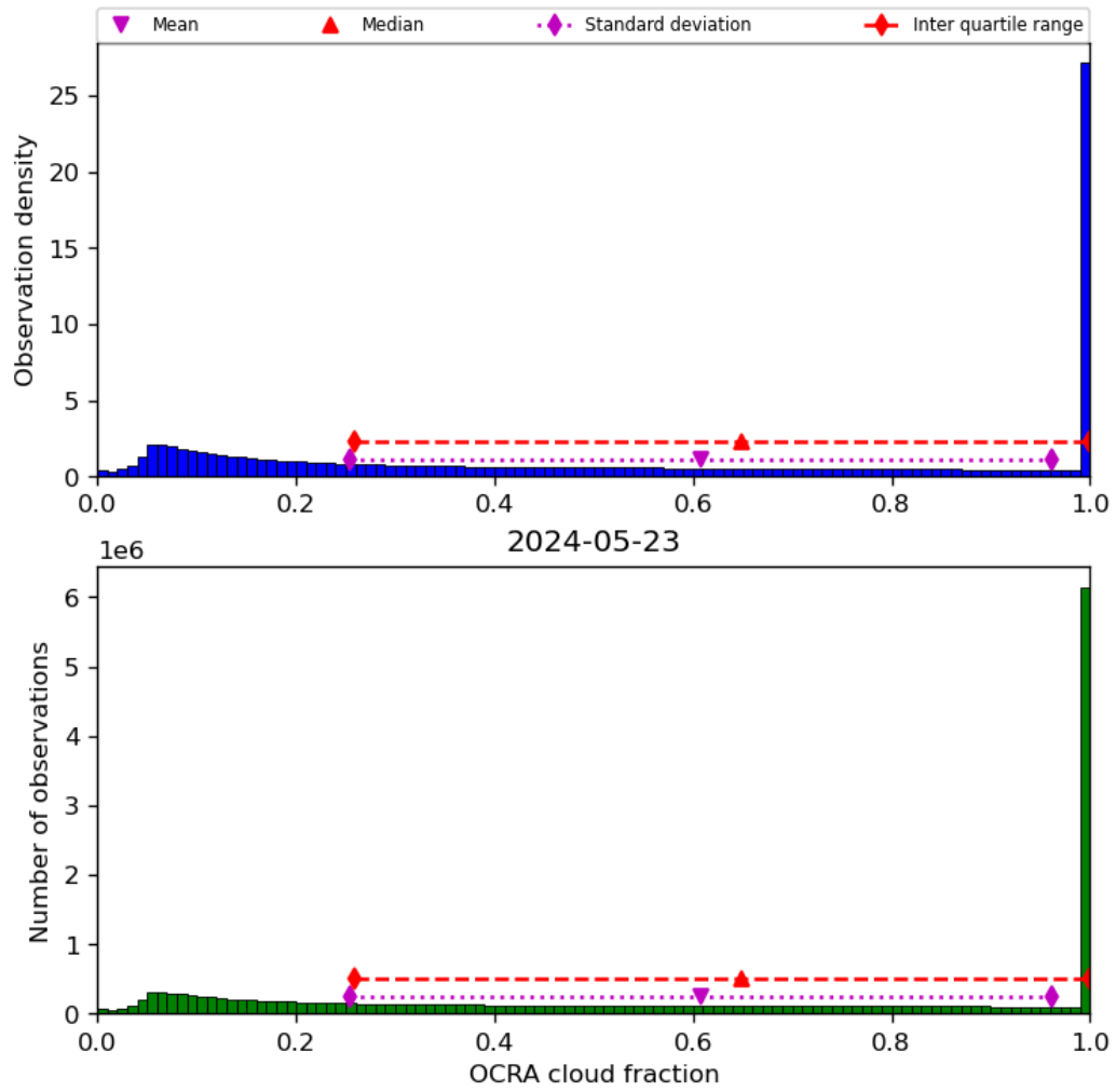
Figure 50: Histogram of “OCRA cloud fraction” for 2024-05-23 to 2024-05-24
