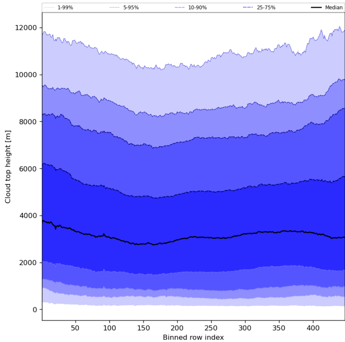
Figure 56: Along track statistics of “Cloud top height” for 2024-05-23 to 2024-05-24
