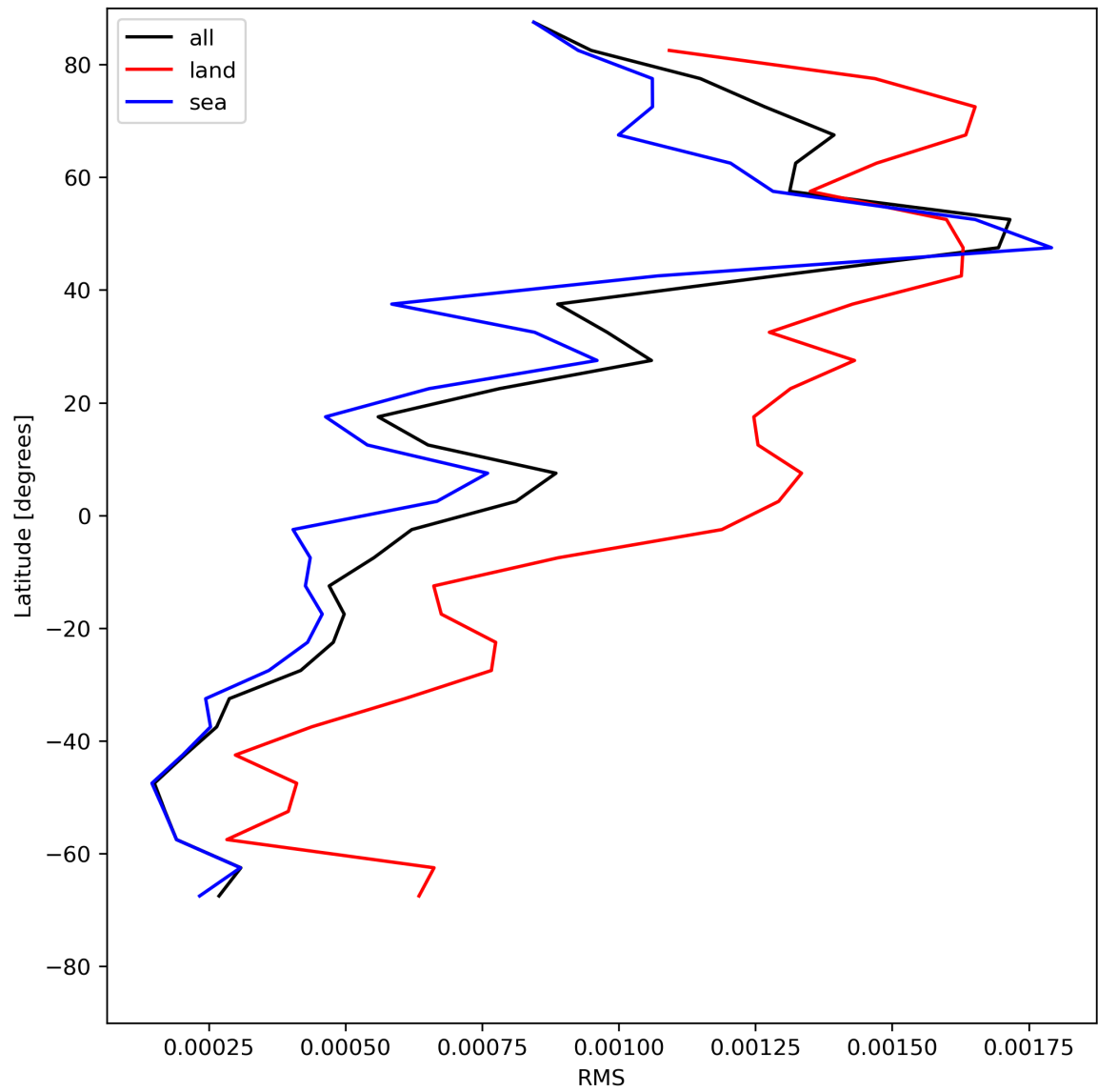
Figure 31: Zonal average of “RMS” for 2024-05-23 to 2024-05-24.
