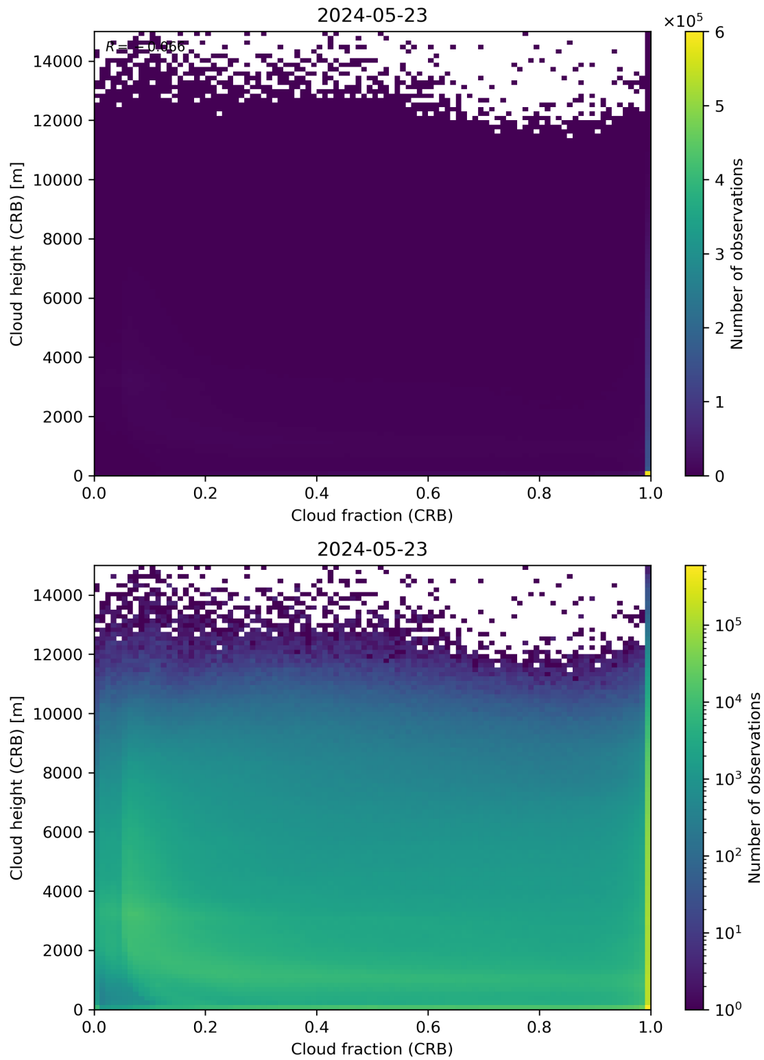
Figure 79: Scatter density plot of “Cloud fraction (CRB)” against “Cloud height (CRB)” for 2024-05-23 to 2024-05-24.
