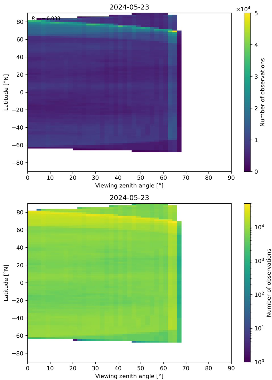
Figure 113: Scatter density plot of “Viewing zenith angle” against “Latitude” for 2024-05-23 to 2024-05-24.
