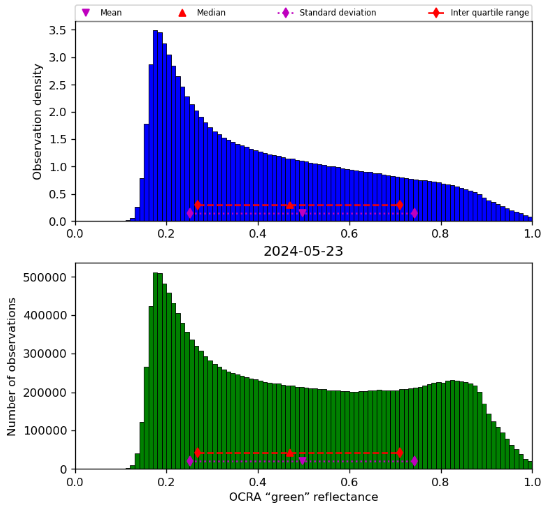
Figure 52: Histogram of “OCRA “green” reflectance” for 2024-05-23 to 2024-05-24
