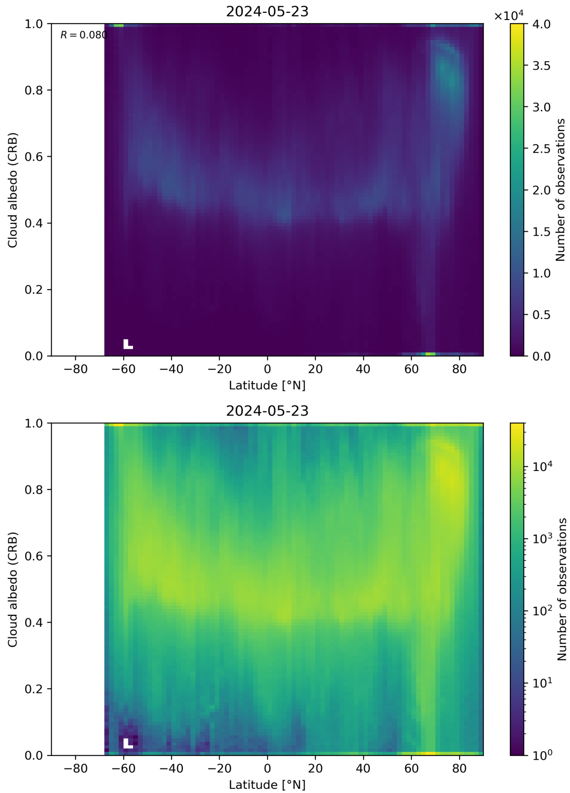
Figure 91: Scatter density plot of “Latitude” against “Cloud albedo (CRB)” for 2024-05-23 to 2024-05-24.
