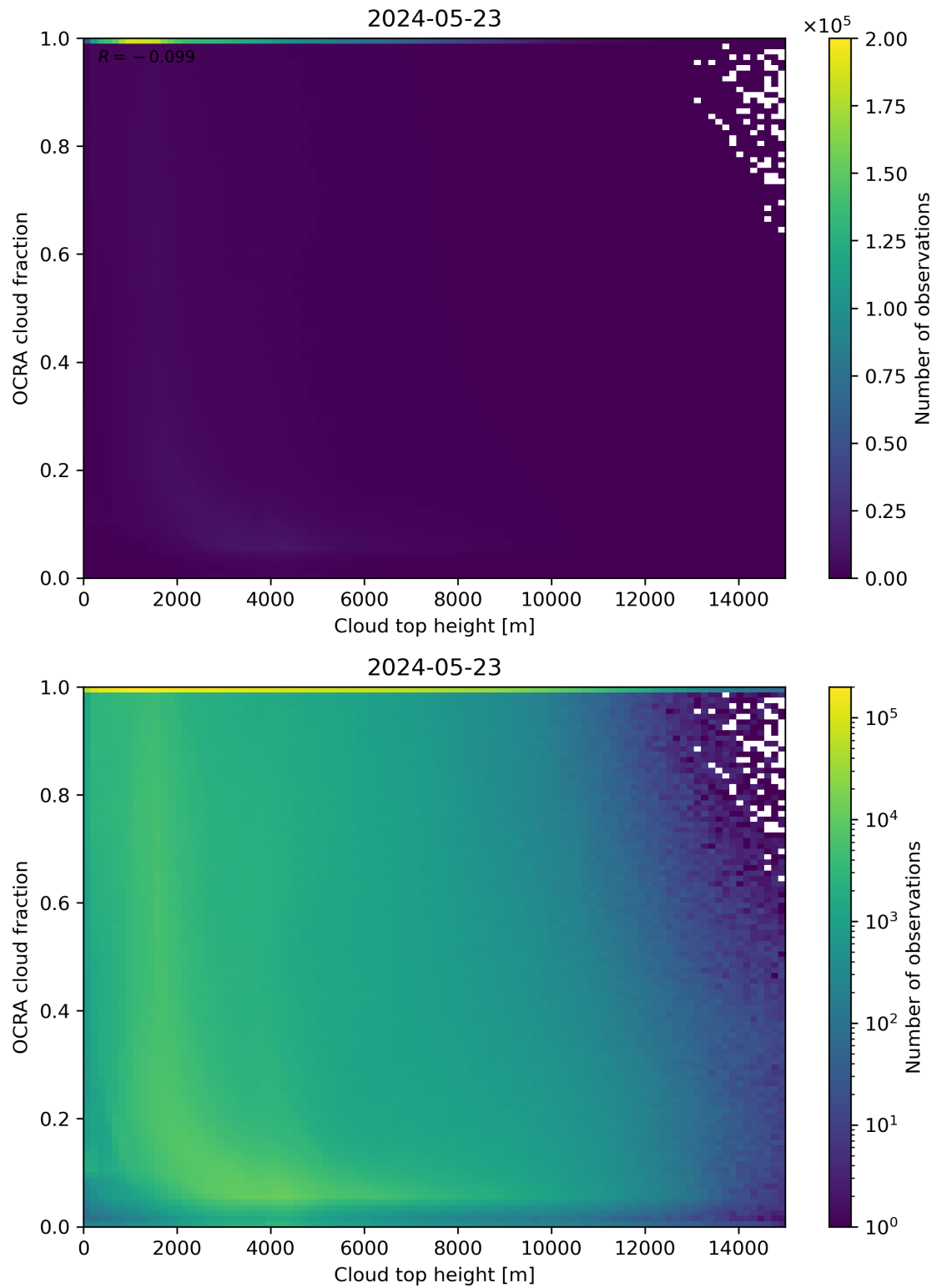
Figure 87: Scatter density plot of “Cloud top height” against “OCRA cloud fraction” for 2024-05-23 to 2024-05-24.
