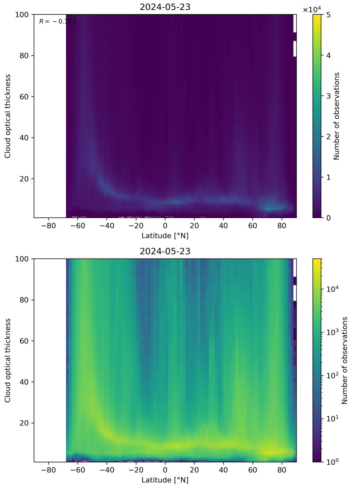
Figure 96: Scatter density plot of “Latitude” against “Cloud optical thickness” for 2024-05-23 to 2024-05-24.
