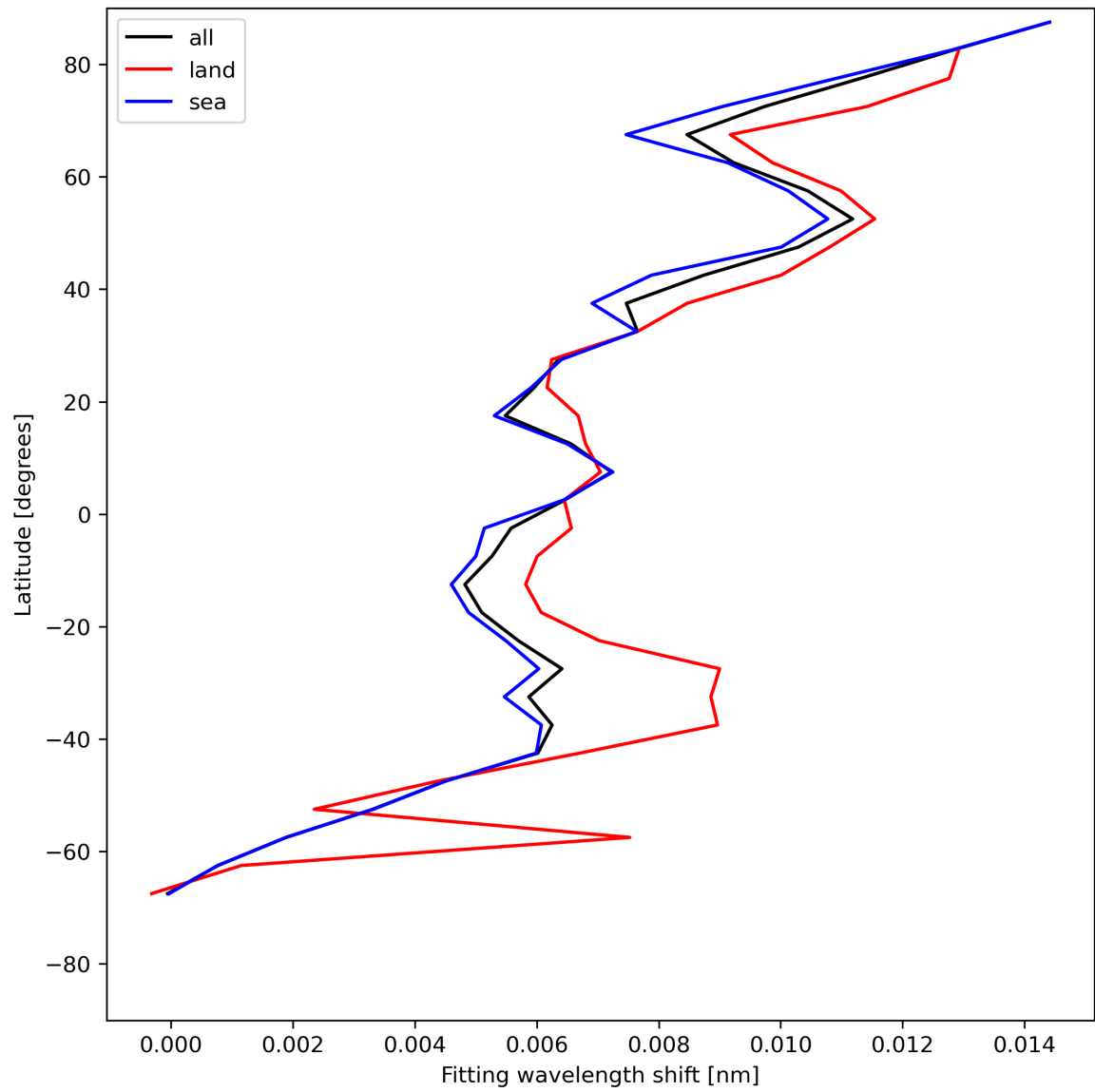
Figure 33: Zonal average of “Fitting wavelength shift” for 2024-05-23 to 2024-05-24.
