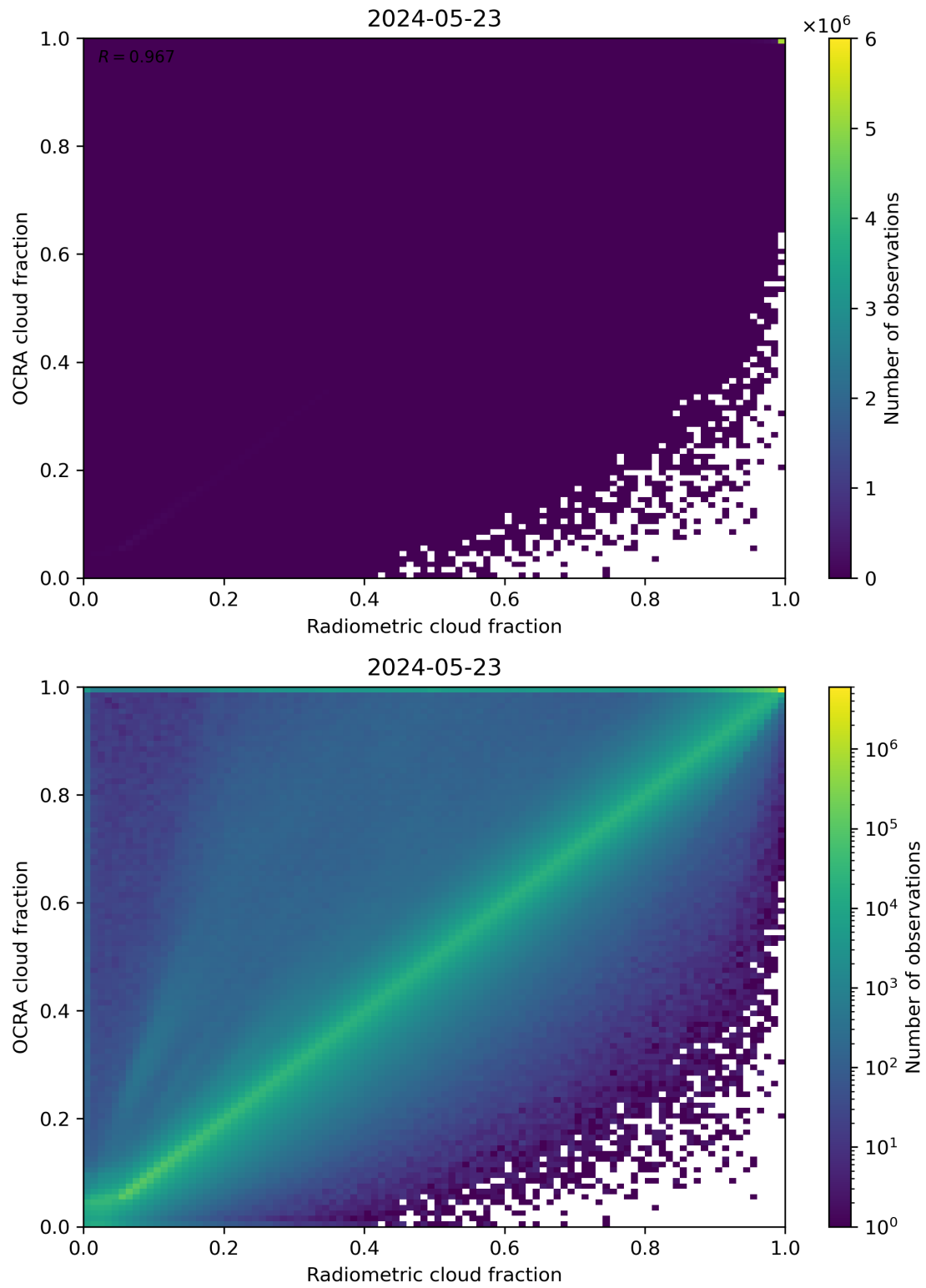
Figure 72: Scatter density plot of “Radiometric cloud fraction” against “OCRA cloud fraction” for 2024-05-23 to 2024-05-24.
