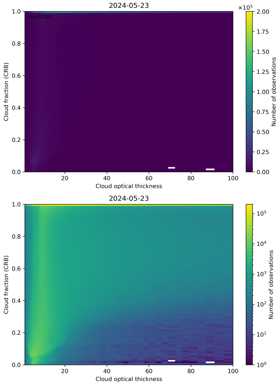
Figure 84: Scatter density plot of “Cloud optical thickness” against “Cloud fraction (CRB)” for 2024-05-23 to 2024-05-24.
