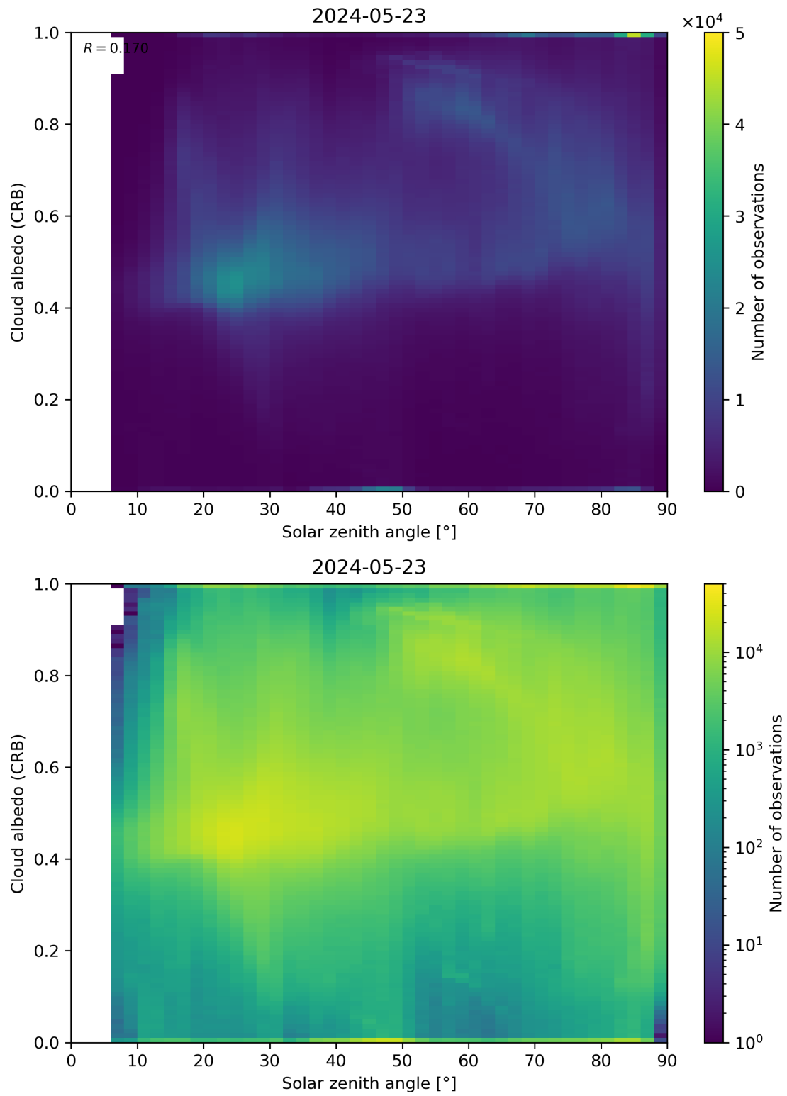
Figure 98: Scatter density plot of “Solar zenith angle” against “Cloud albedo (CRB)” for 2024-05-23 to 2024-05-24.
