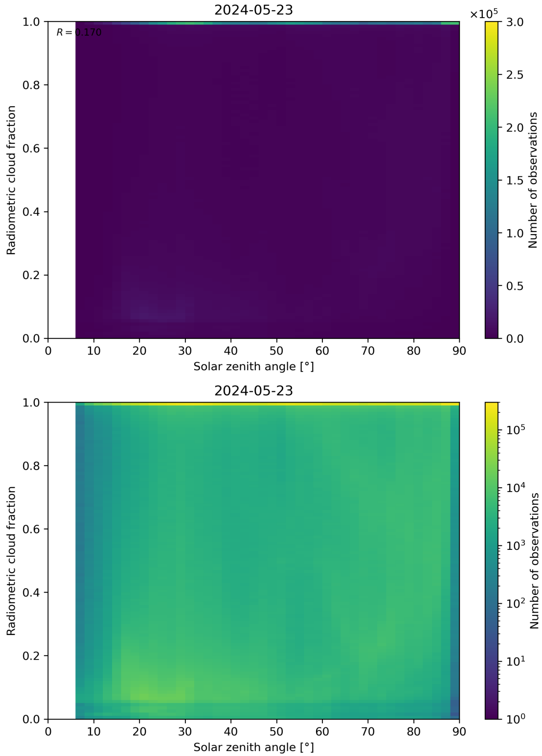
Figure 99: Scatter density plot of “Solar zenith angle” against “Radiometric cloud fraction” for 2024-05-23 to 2024-05-24.
