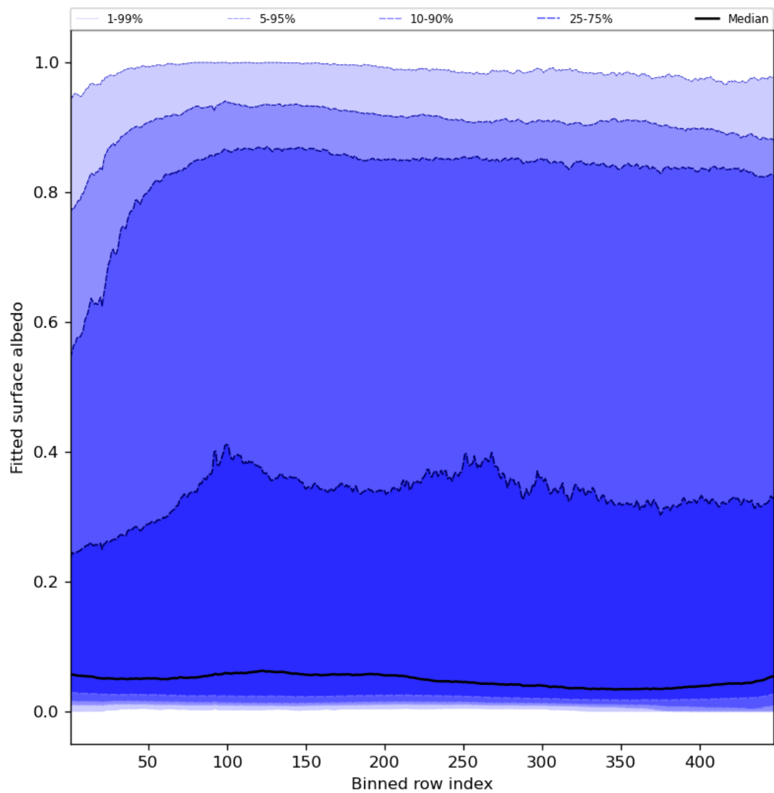
Figure 61: Along track statistics of “Fitted surface albedo” for 2024-05-23 to 2024-05-24
