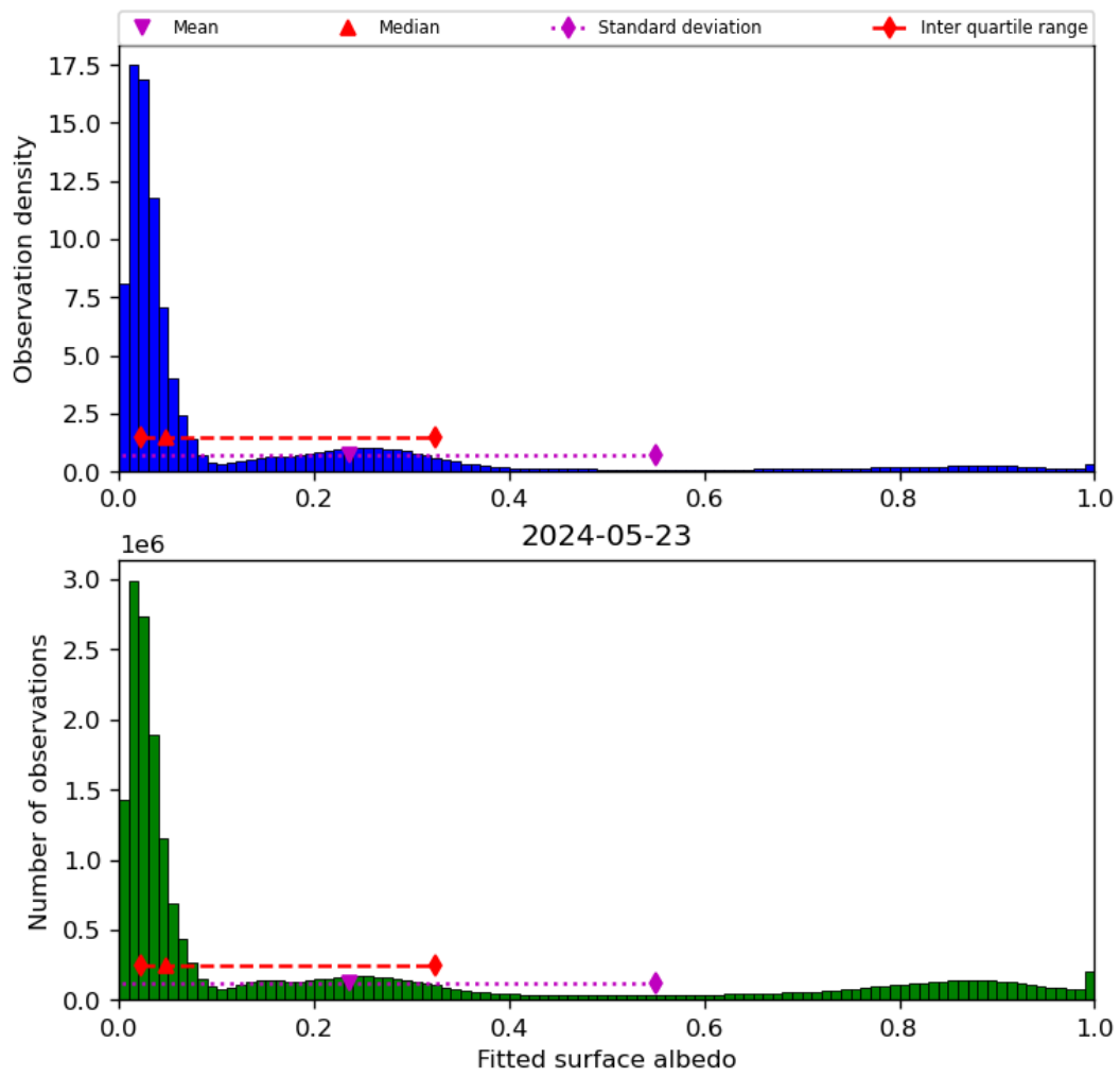
Figure 45: Histogram of “Fitted surface albedo” for 2024-05-23 to 2024-05-24
