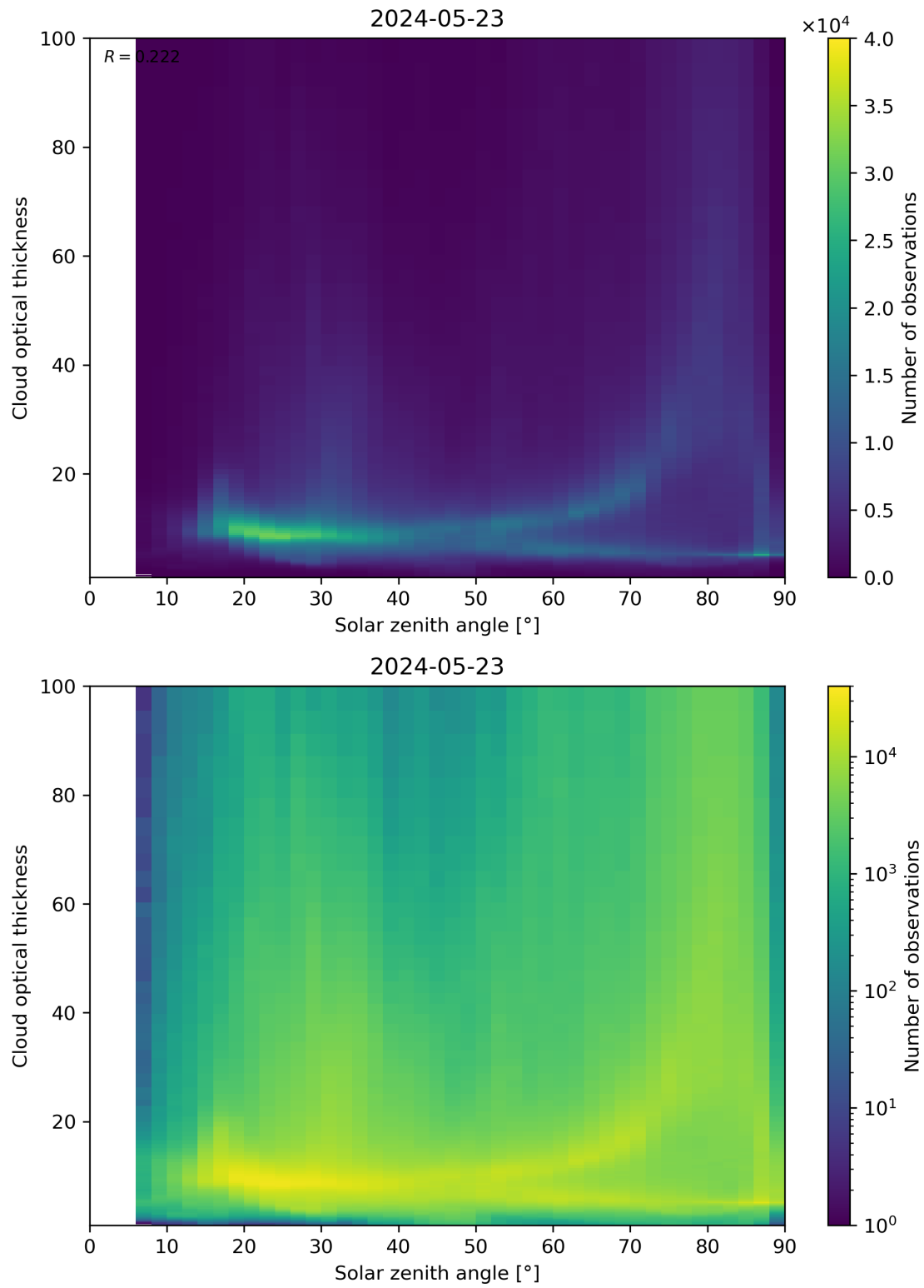
Figure 103: Scatter density plot of “Solar zenith angle” against “Cloud optical thickness” for 2024-05-23 to 2024-05-24.
