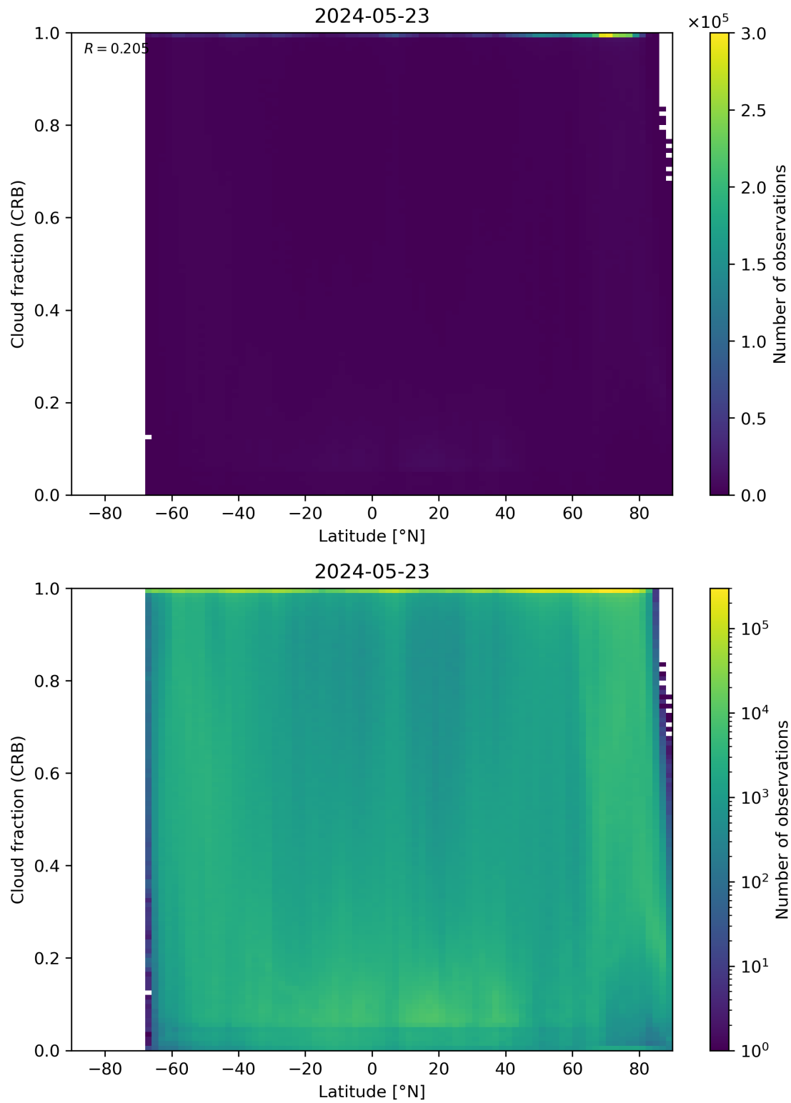
Figure 94: Scatter density plot of “Latitude” against “Cloud fraction (CRB)” for 2024-05-23 to 2024-05-24.
