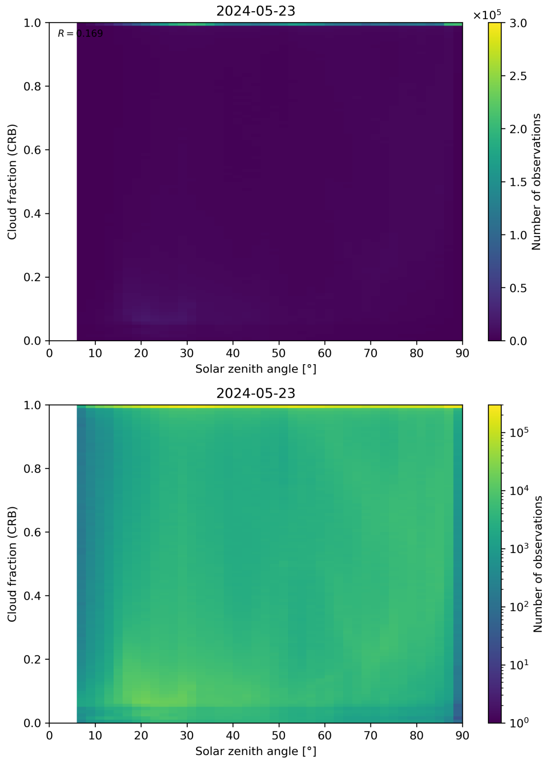
Figure 101: Scatter density plot of “Solar zenith angle” against “Cloud fraction (CRB)” for 2024-05-23 to 2024-05-24.
