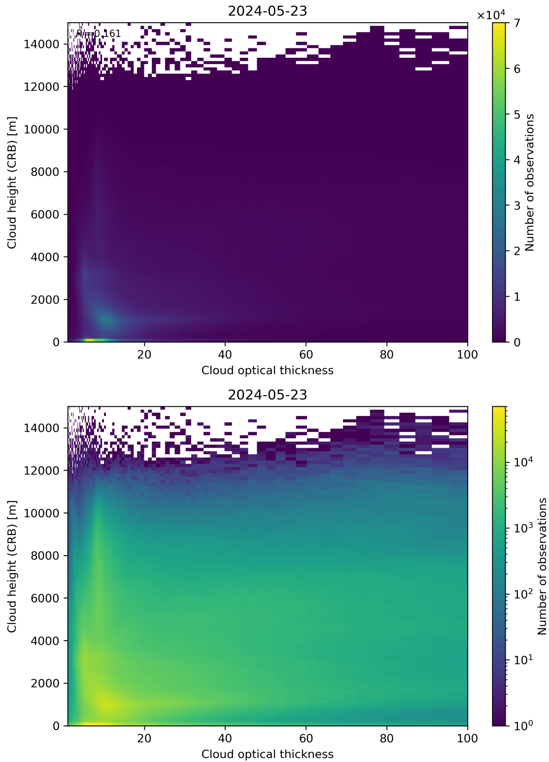
Figure 85: Scatter density plot of “Cloud optical thickness” against “Cloud height (CRB)” for 2024-05-23 to 2024-05-24.
