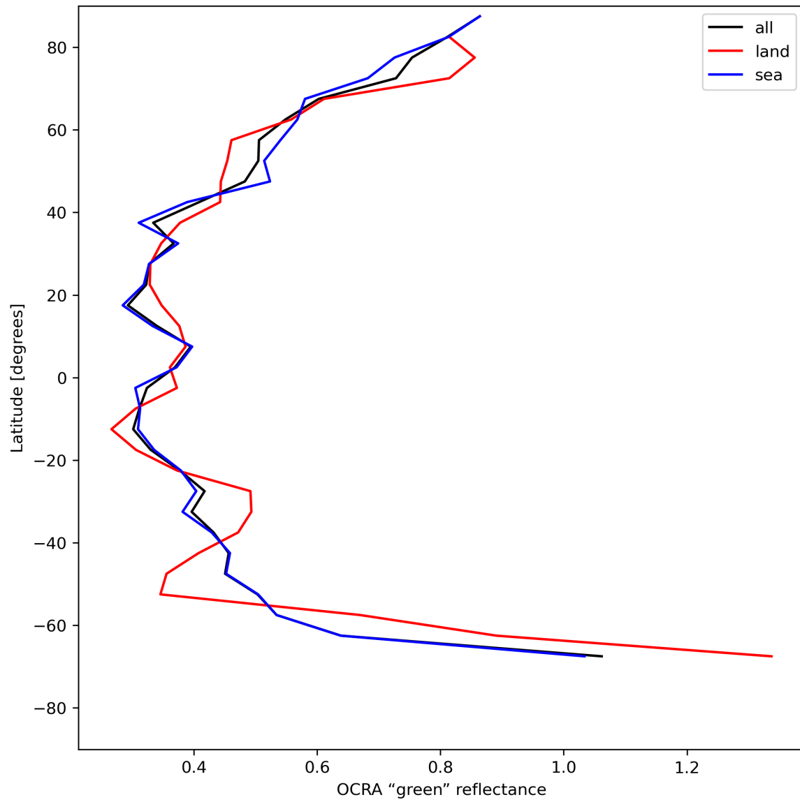
Figure 36: Zonal average of “OCRA “green” reflectance” for 2024-05-23 to 2024-05-24.
