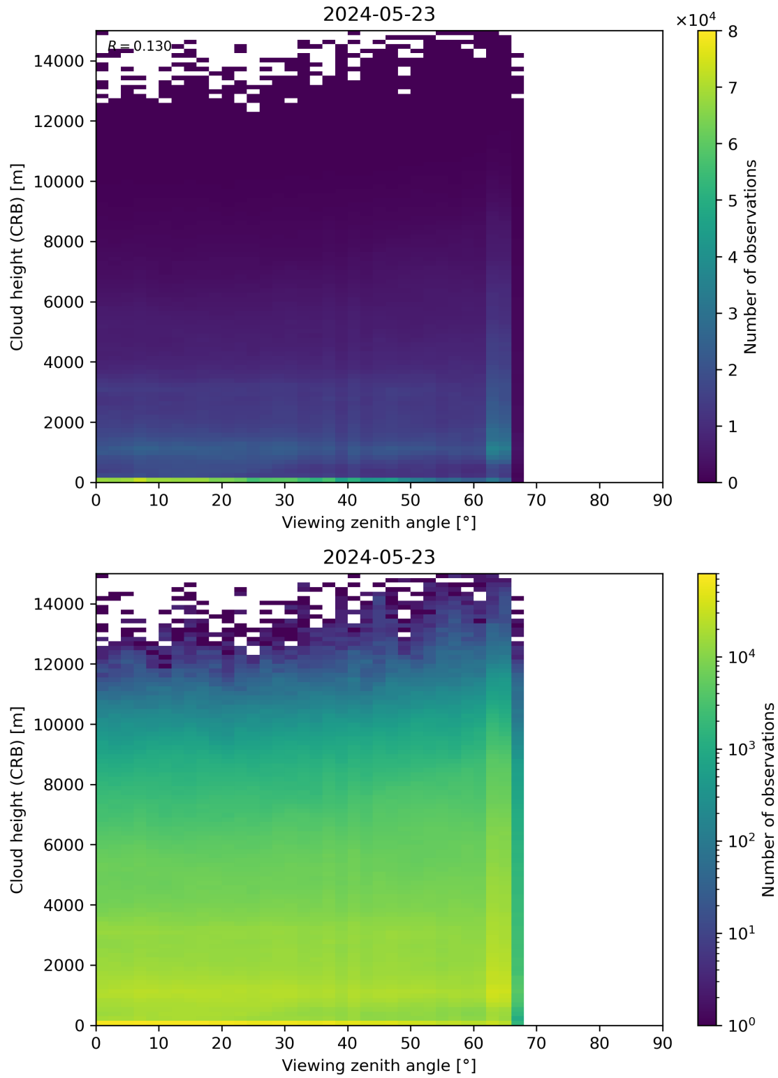
Figure 110: Scatter density plot of “Viewing zenith angle” against “Cloud height (CRB)” for 2024-05-23 to 2024-05-24.
