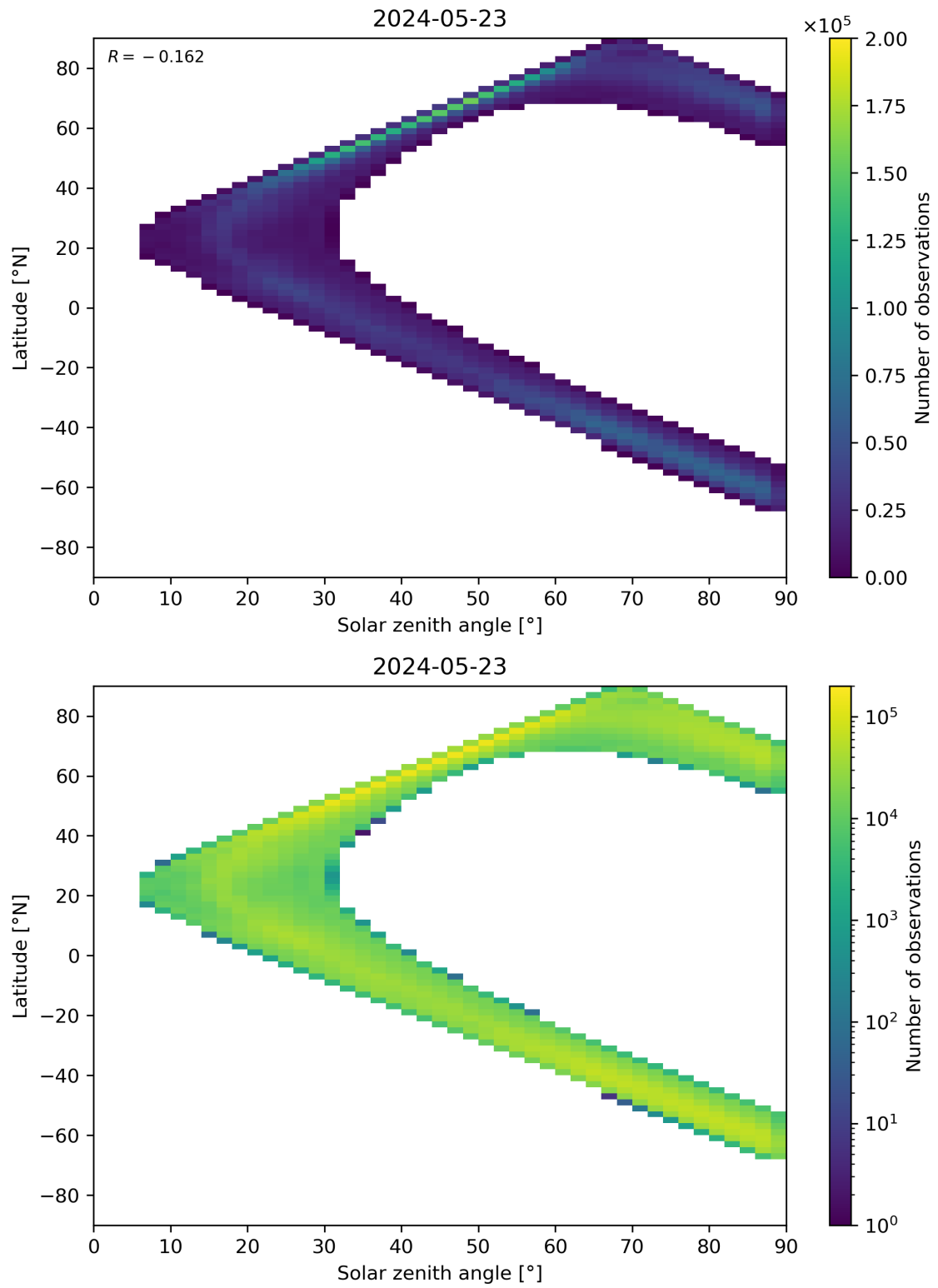
Figure 105: Scatter density plot of “Solar zenith angle” against “Latitude” for 2024-05-23 to 2024-05-24.
