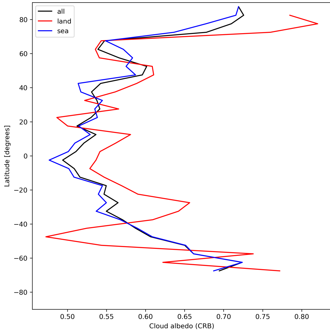
Figure 28: Zonal average of “Cloud albedo (CRB)” for 2024-05-23 to 2024-05-24.
