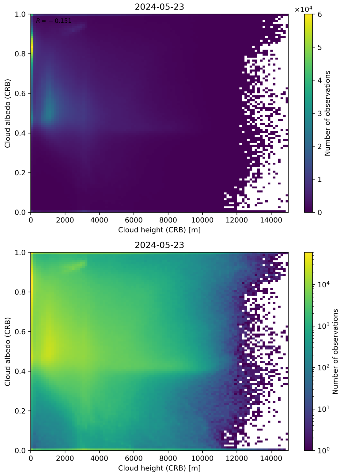
Figure 80: Scatter density plot of “Cloud height (CRB)” against “Cloud albedo (CRB)” for 2024-05-23 to 2024-05-24.
