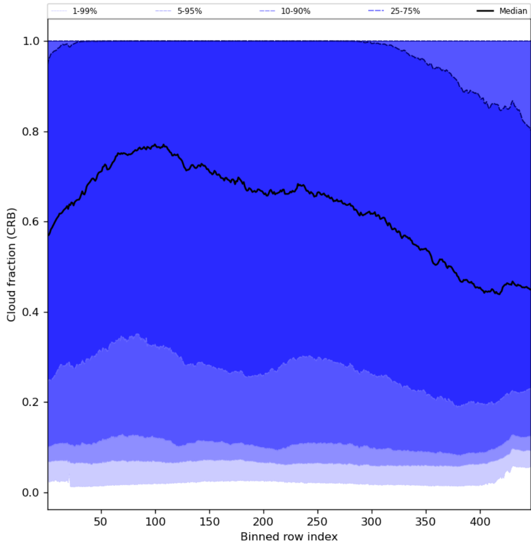
Figure 58: Along track statistics of “Cloud fraction (CRB)” for 2024-05-23 to 2024-05-24
