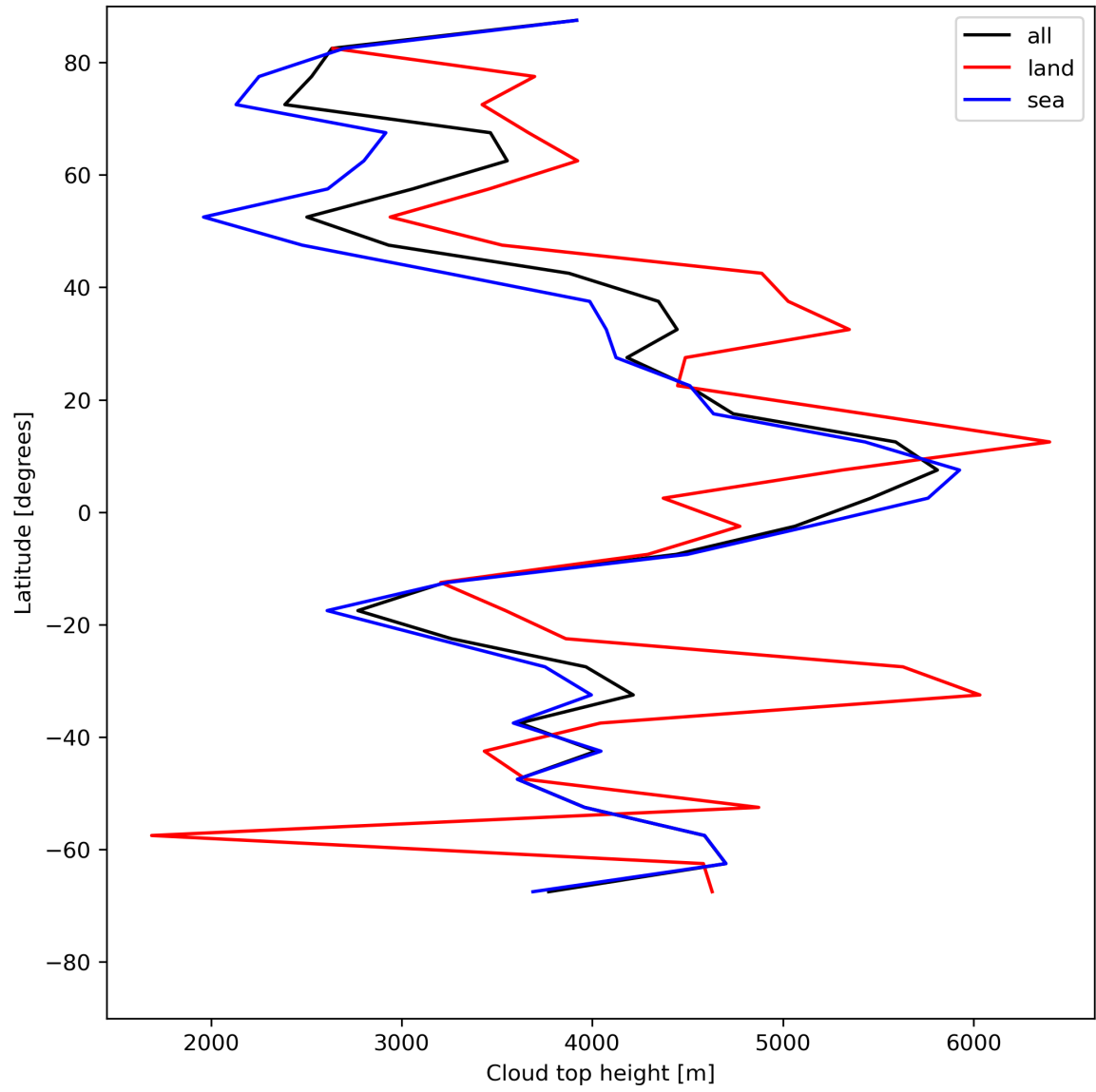
Figure 24: Zonal average of “Cloud top height” for 2024-05-23 to 2024-05-24.
