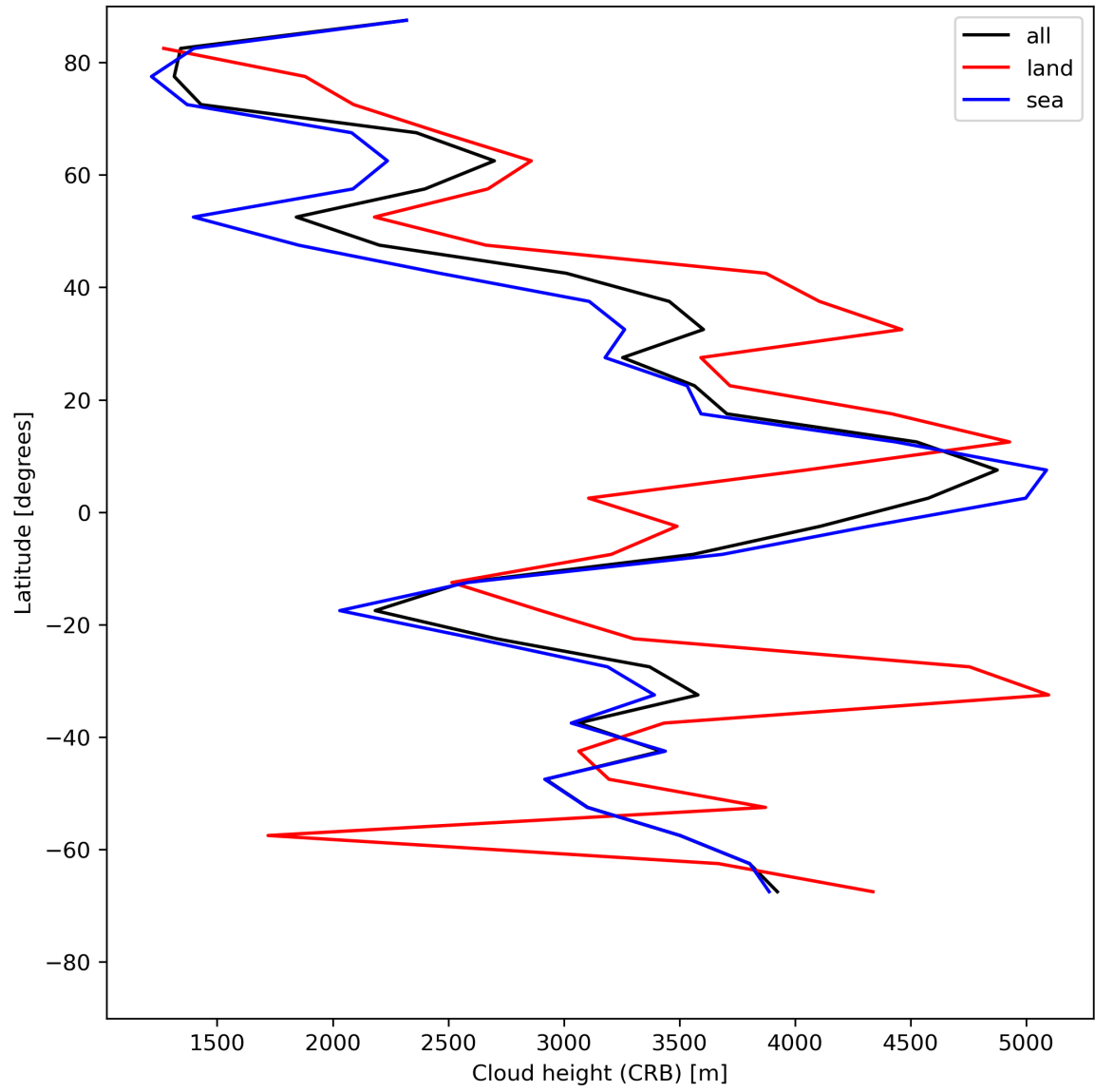
Figure 27: Zonal average of “Cloud height (CRB)” for 2024-05-23 to 2024-05-24.
