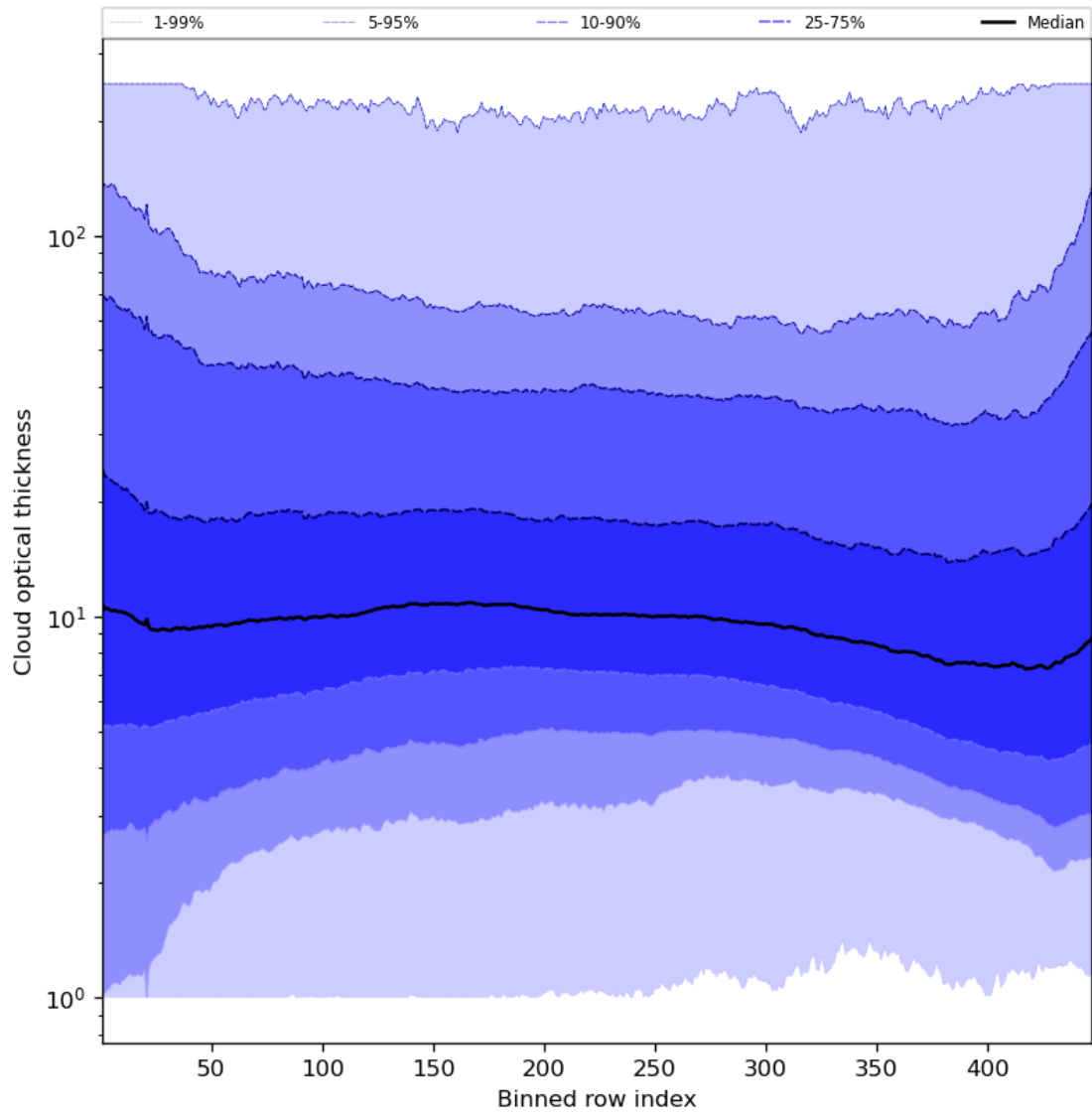
Figure 57: Along track statistics of “Cloud optical thickness” for 2024-05-23 to 2024-05-24
