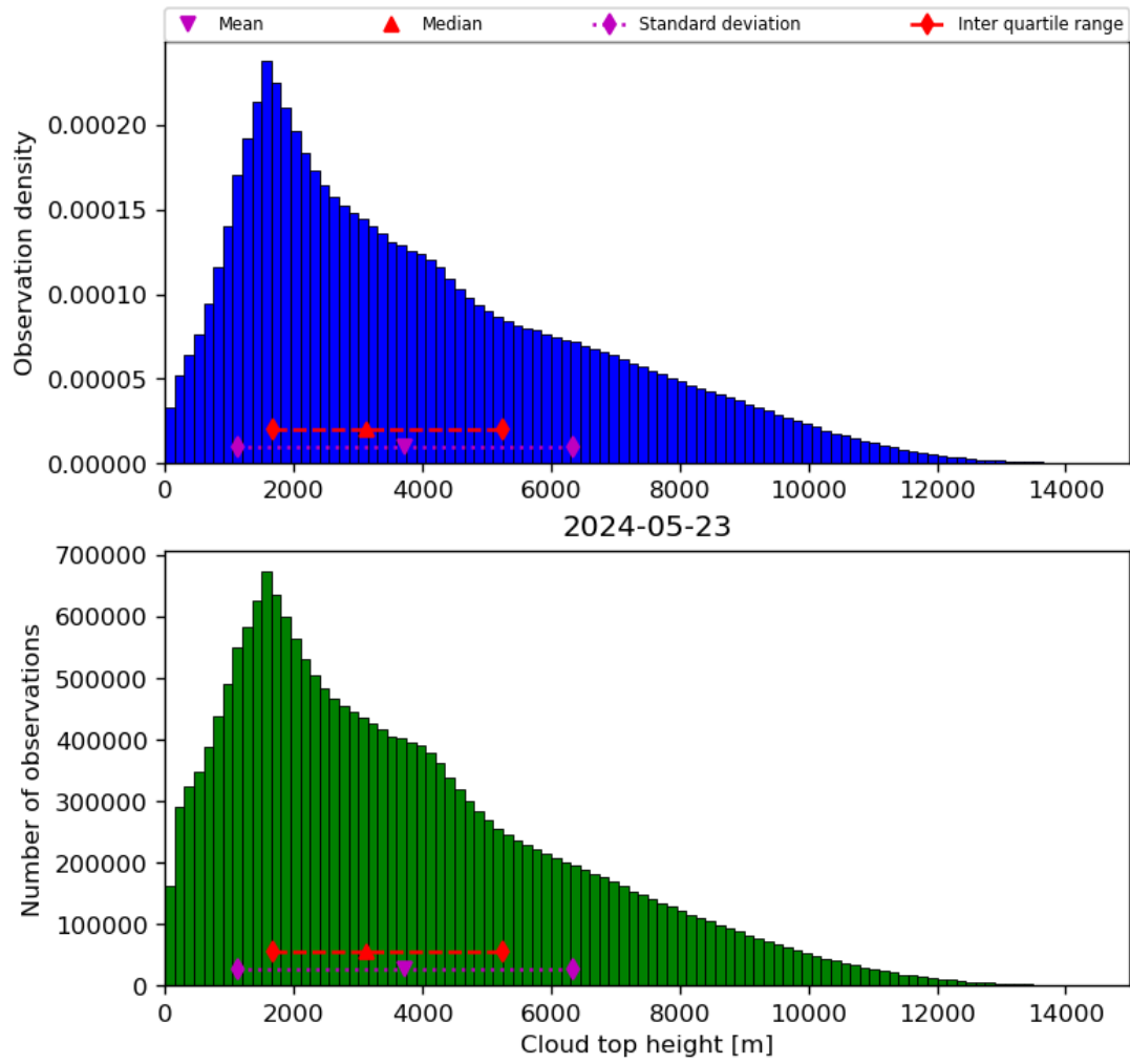
Figure 40: Histogram of “Cloud top height” for 2024-05-23 to 2024-05-24
