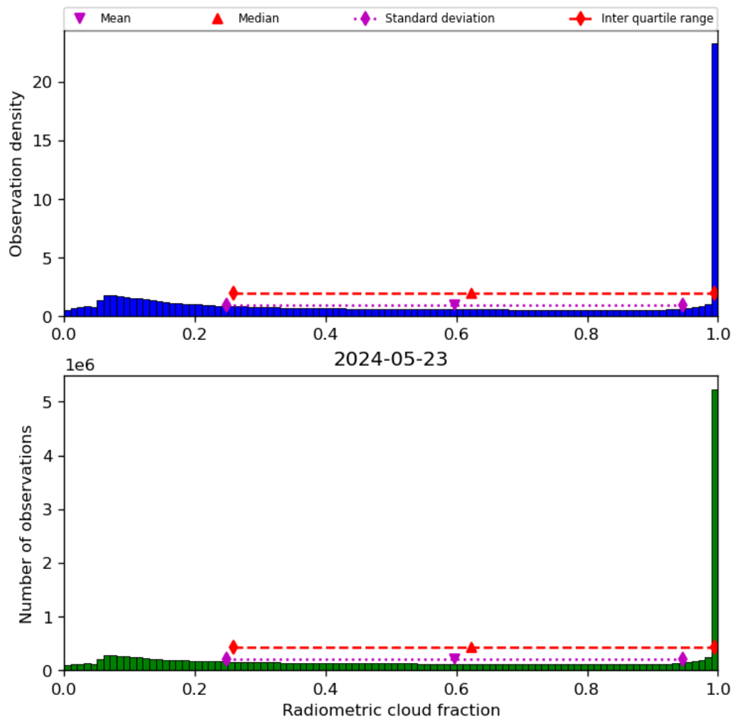
Figure 39: Histogram of “Radiometric cloud fraction” for 2024-05-23 to 2024-05-24
