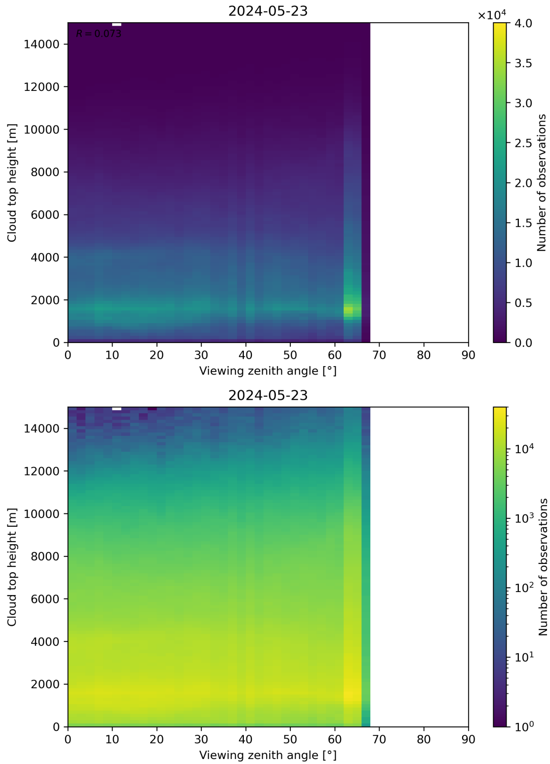
Figure 112: Scatter density plot of “Viewing zenith angle” against “Cloud top height” for 2024-05-23 to 2024-05-24.
