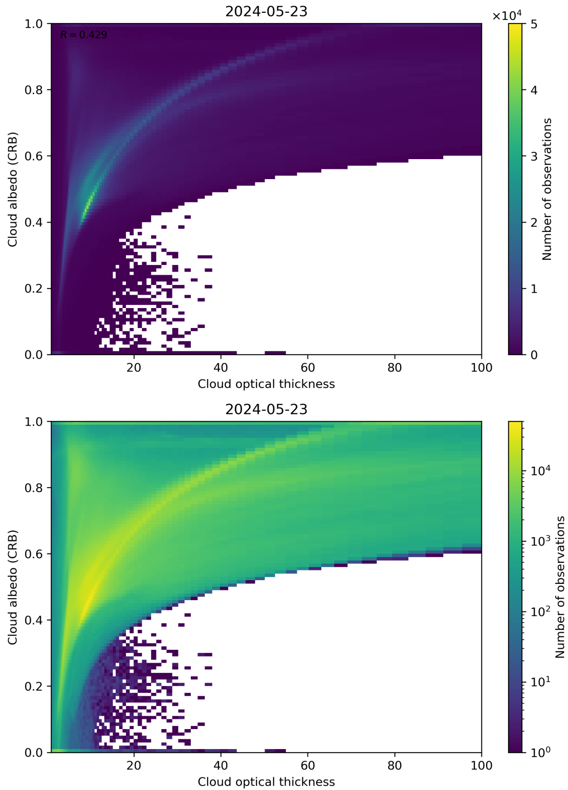
Figure 82: Scatter density plot of “Cloud optical thickness” against “Cloud albedo (CRB)” for 2024-05-23 to 2024-05-24.
