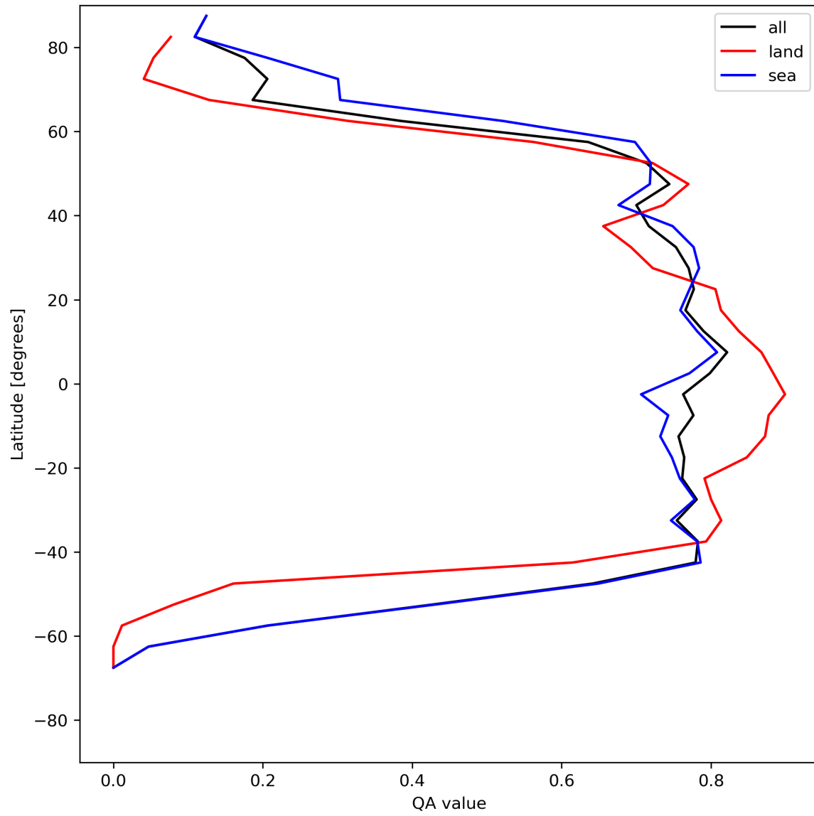
Figure 22: Zonal average of “QA value” for 2024-05-23 to 2024-05-24.
