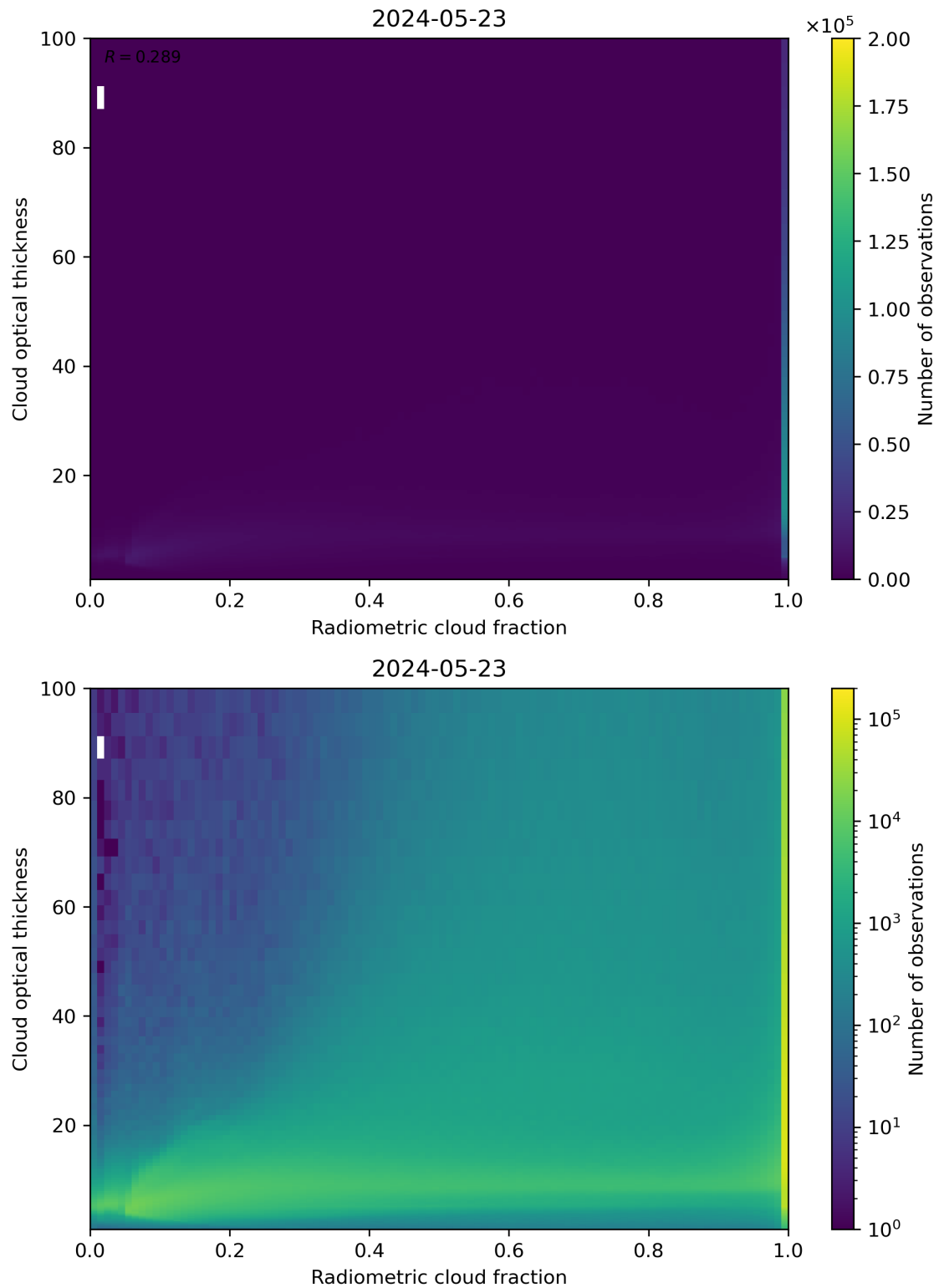
Figure 75: Scatter density plot of “Radiometric cloud fraction” against “Cloud optical thickness” for 2024-05-23 to 2024-05-24.
