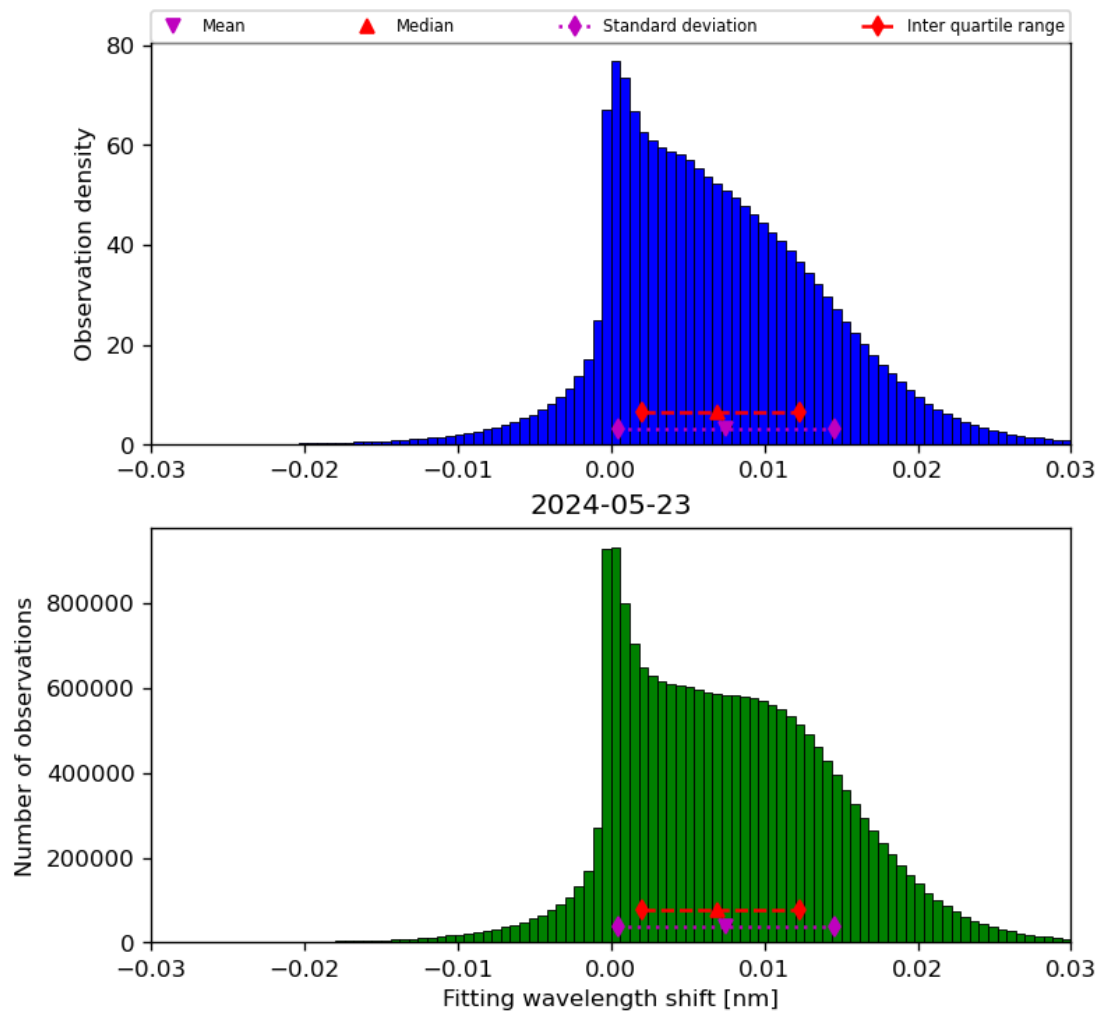
Figure 49: Histogram of “Fitting wavelength shift” for 2024-05-23 to 2024-05-24
