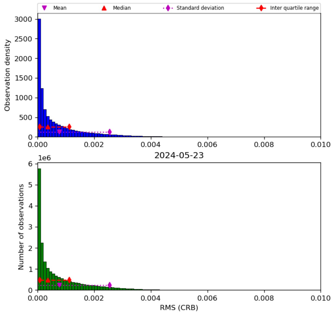
Figure 48: Histogram of “RMS (CRB)” for 2024-05-23 to 2024-05-24
