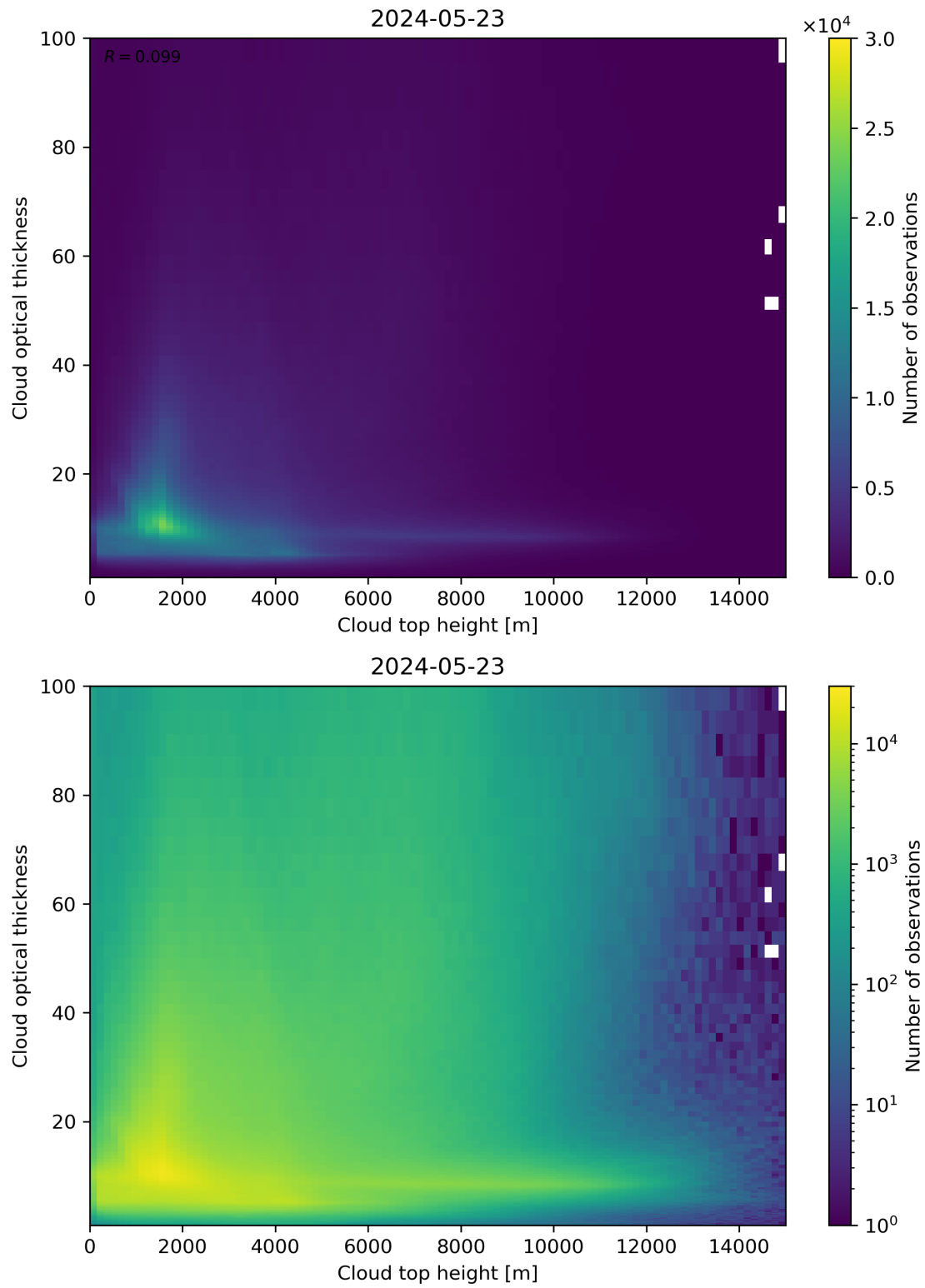
Figure 90: Scatter density plot of “Cloud top height” against “Cloud optical thickness” for 2024-05-23 to 2024-05-24.
