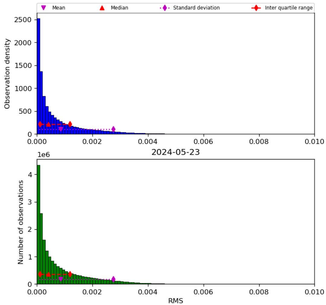
Figure 47: Histogram of “RMS” for 2024-05-23 to 2024-05-24
