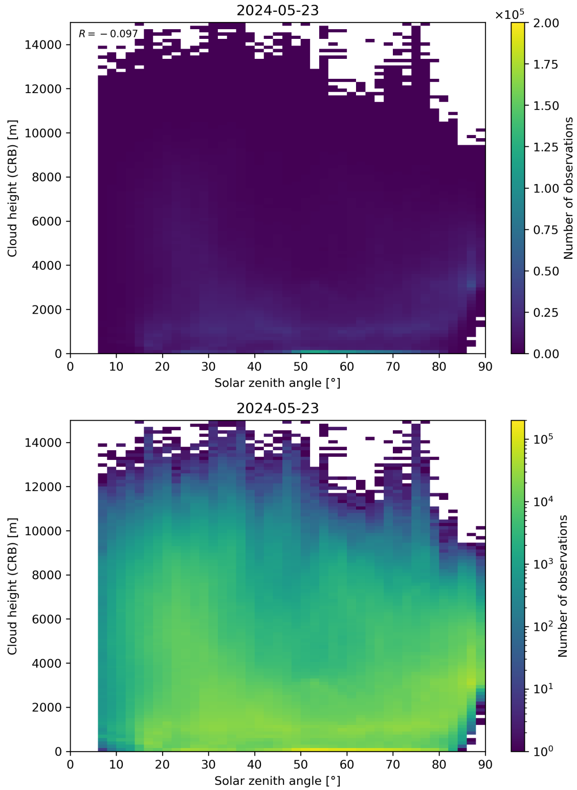
Figure 102: Scatter density plot of “Solar zenith angle” against “Cloud height (CRB)” for 2024-05-23 to 2024-05-24.
