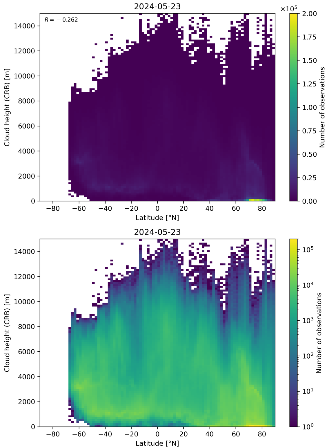
Figure 95: Scatter density plot of “Latitude” against “Cloud height (CRB)” for 2024-05-23 to 2024-05-24.
