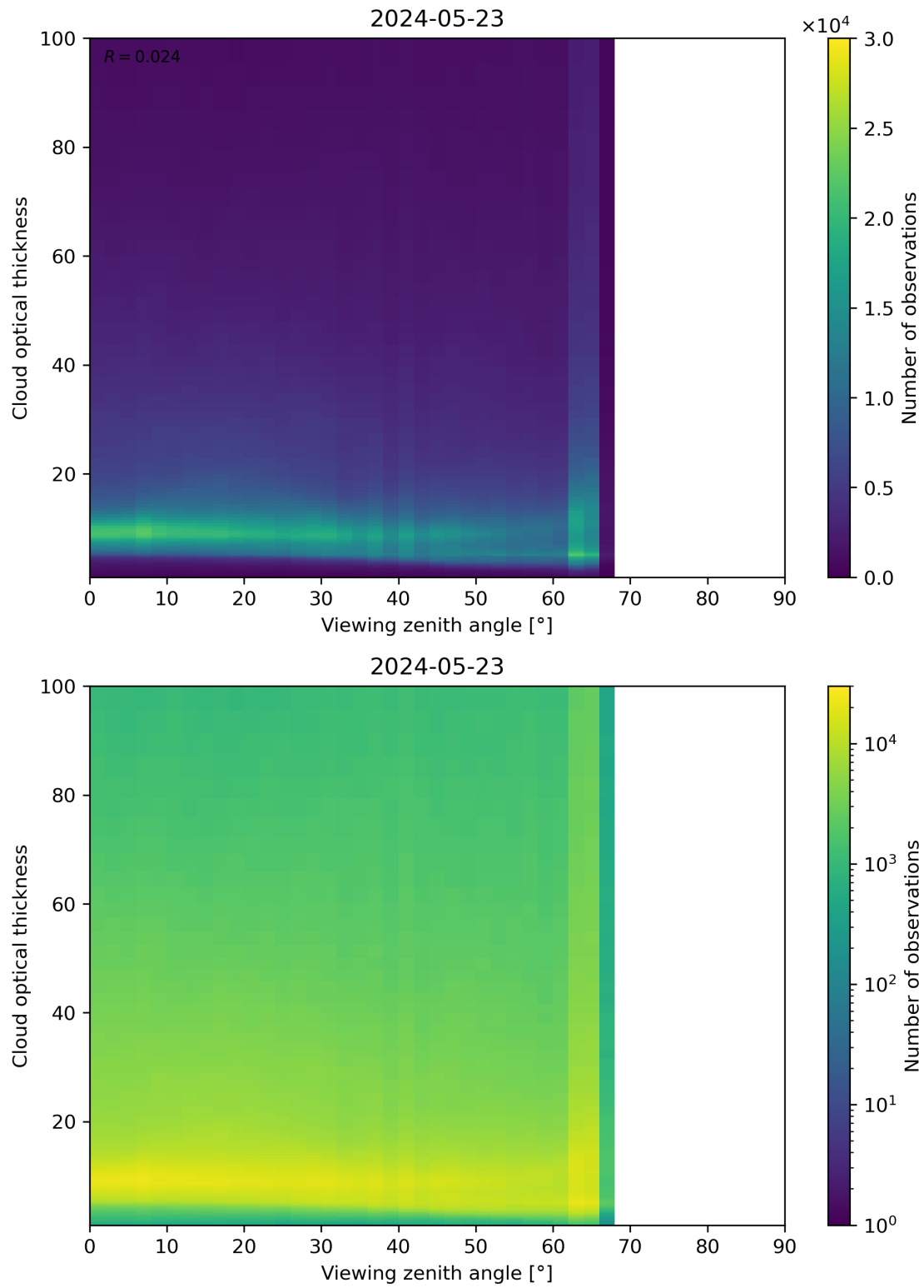
Figure 111: Scatter density plot of “Viewing zenith angle” against “Cloud optical thickness” for 2024-05-23 to 2024-05-24.
