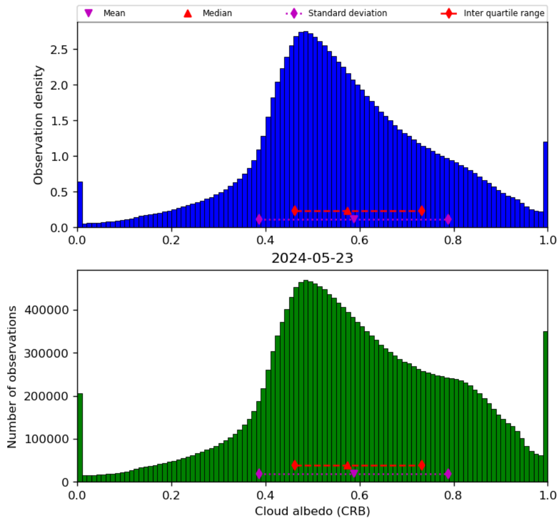
Figure 44: Histogram of “Cloud albedo (CRB)” for 2024-05-23 to 2024-05-24
