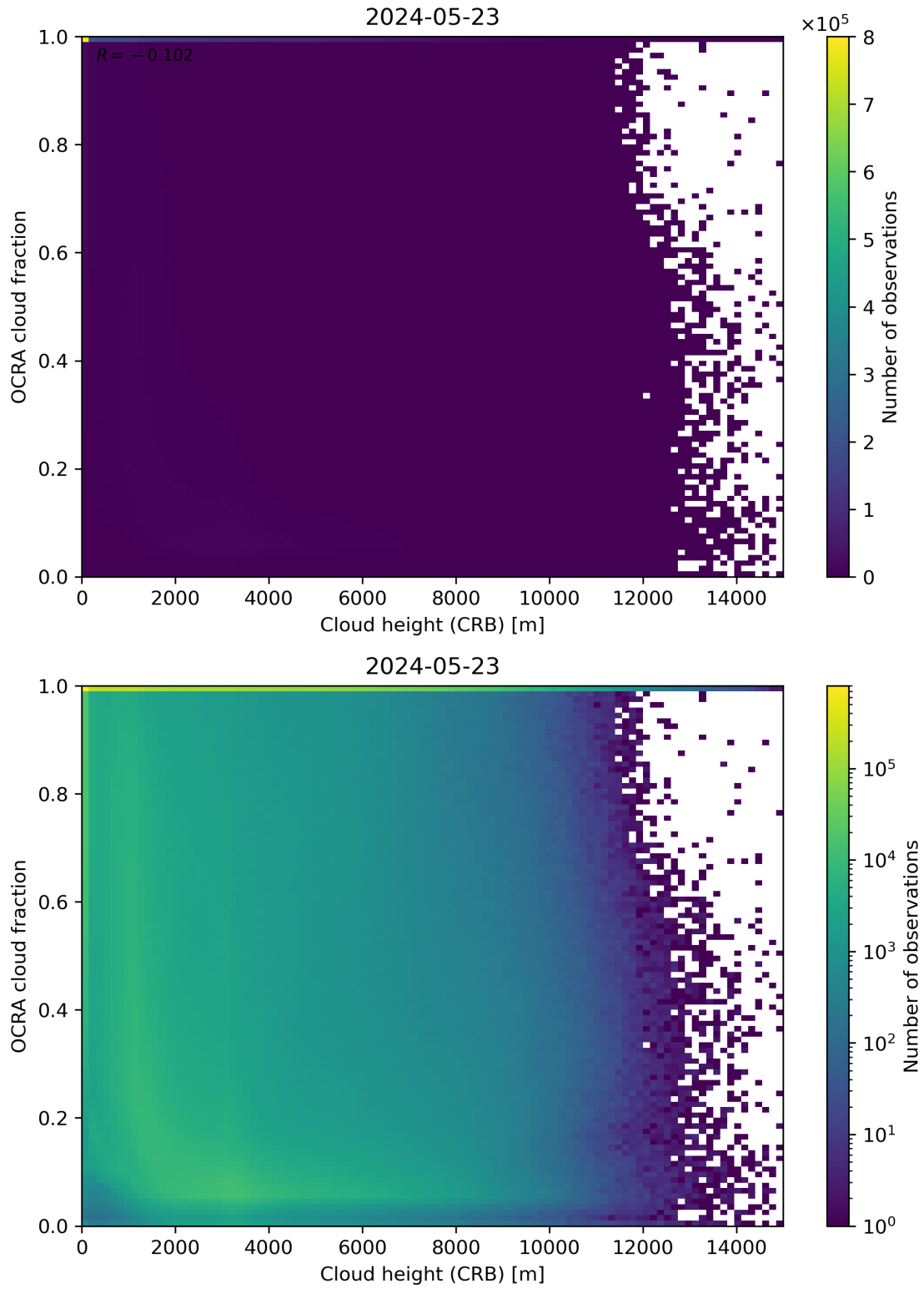
Figure 81: Scatter density plot of “Cloud height (CRB)” against “OCRA cloud fraction” for 2024-05-23 to 2024-05-24.
