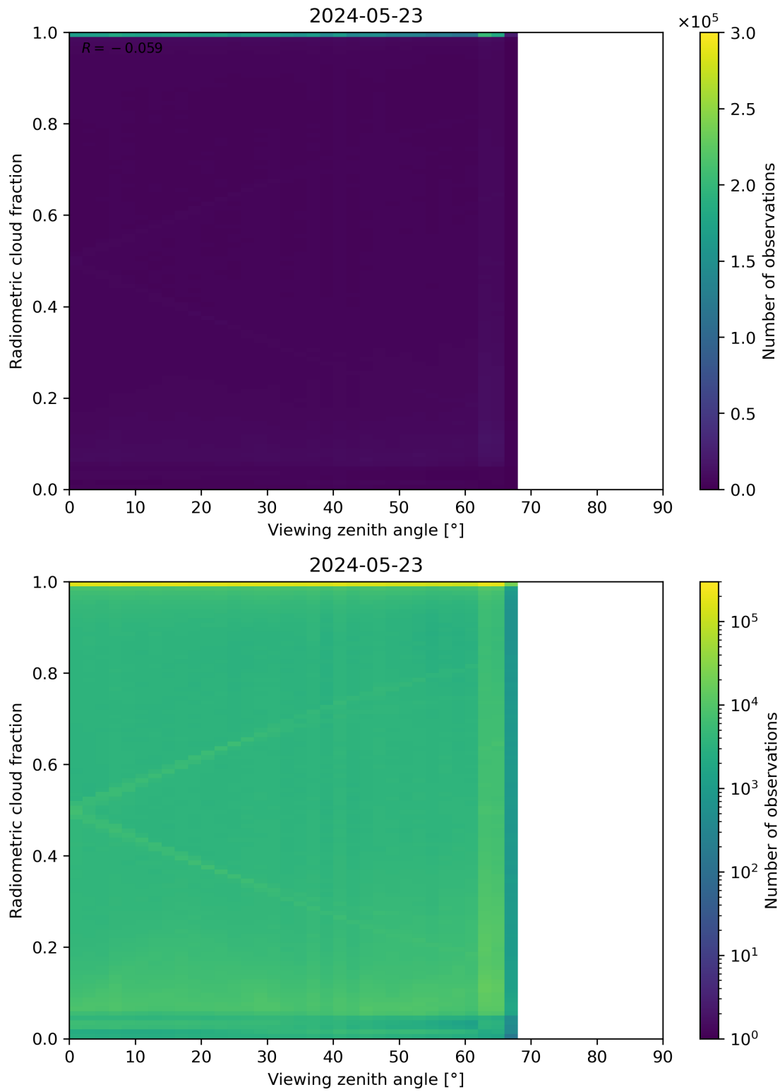
Figure 107: Scatter density plot of “Viewing zenith angle” against “Radiometric cloud fraction” for 2024-05-23 to 2024-05-24.
