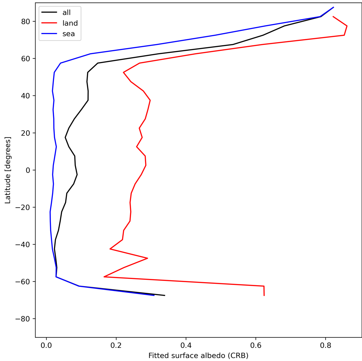
Figure 30: Zonal average of "Fitted surface albedo (CRB)" for 2024-05-23 to 2024-05-24.
