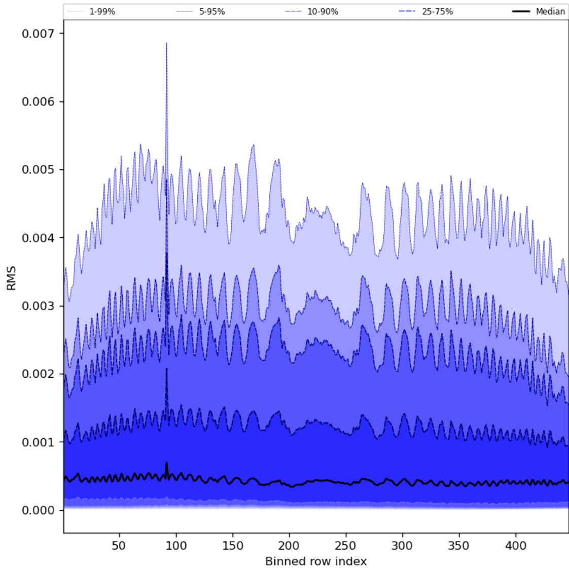
Figure 63: Along track statistics of “RMS” for 2024-05-23 to 2024-05-24
