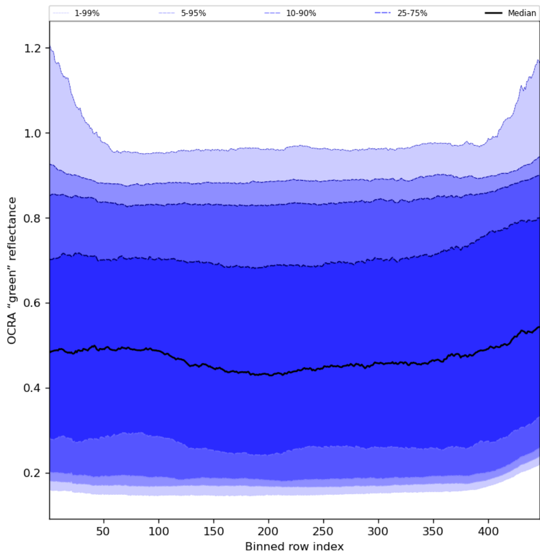
Figure 68: Along track statistics of "OCRA "green" reflectance" for 2024-05-23 to 2024-05-24
