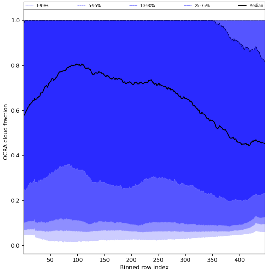
Figure 66: Along track statistics of “OCRA cloud fraction” for 2024-05-23 to 2024-05-24
