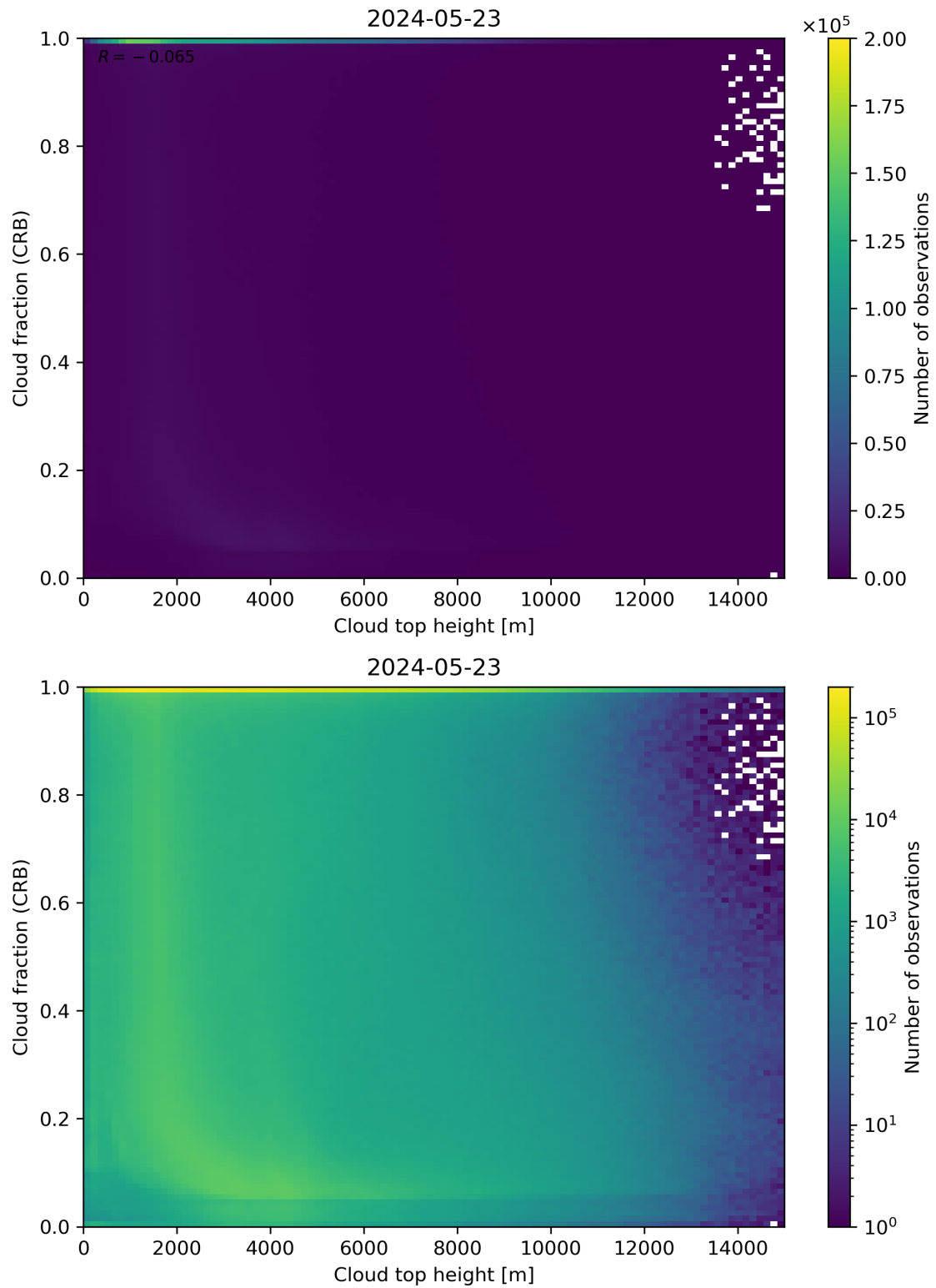
Figure 88: Scatter density plot of “Cloud top height” against “Cloud fraction (CRB)” for 2024-05-23 to 2024-05-24.
