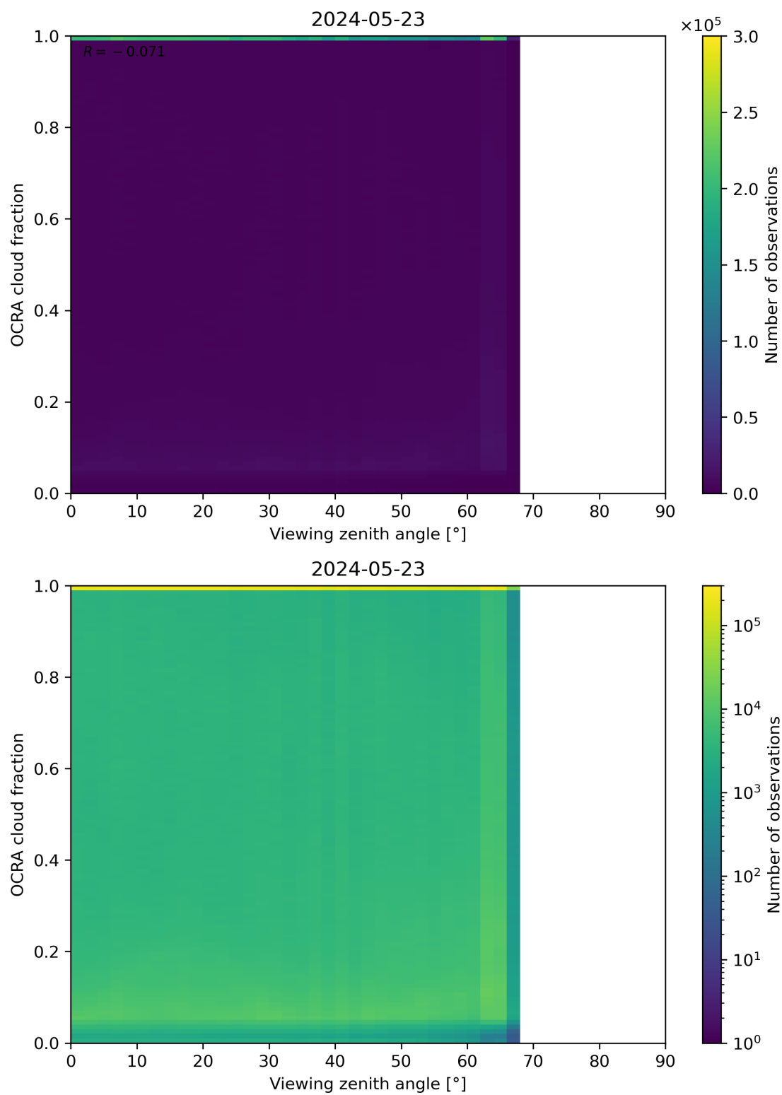
Figure 108: Scatter density plot of “Viewing zenith angle” against “OCRA cloud fraction” for 2024-05-23 to 2024-05-24.
