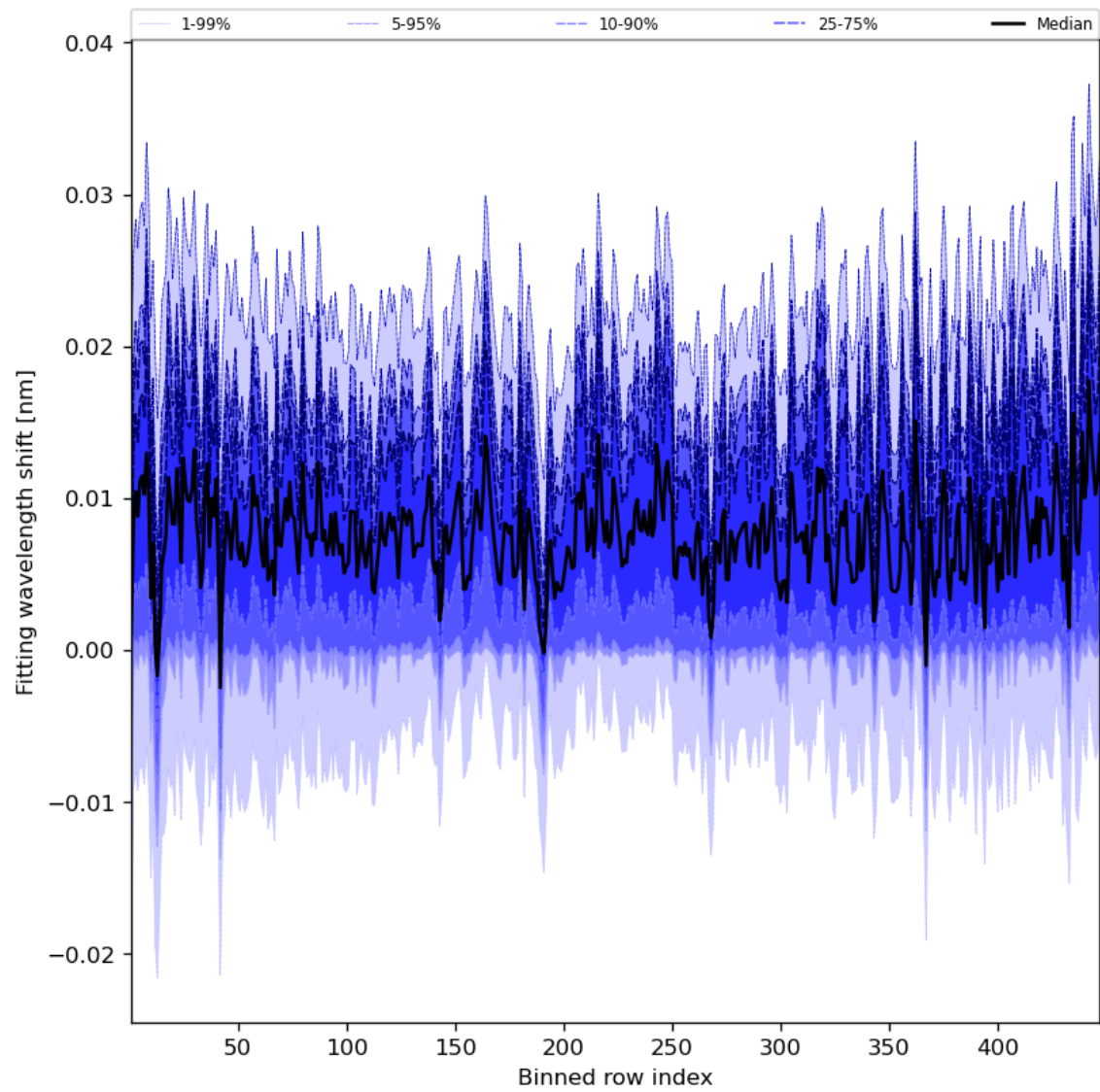
Figure 65: Along track statistics of “Fitting wavelength shift” for 2024-05-23 to 2024-05-24
