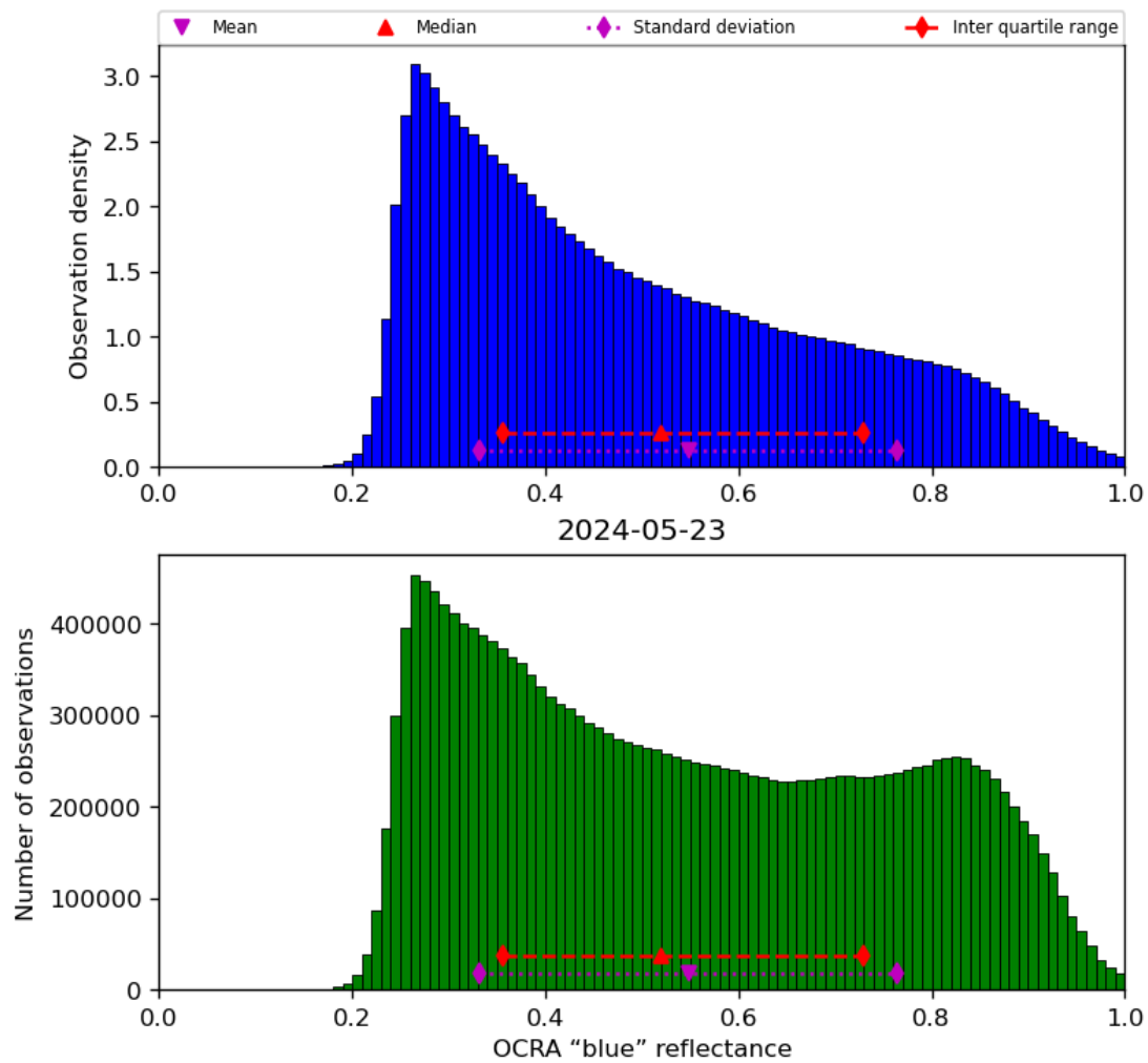
Figure 51: Histogram of “OCRA “blue” reflectance” for 2024-05-23 to 2024-05-24
