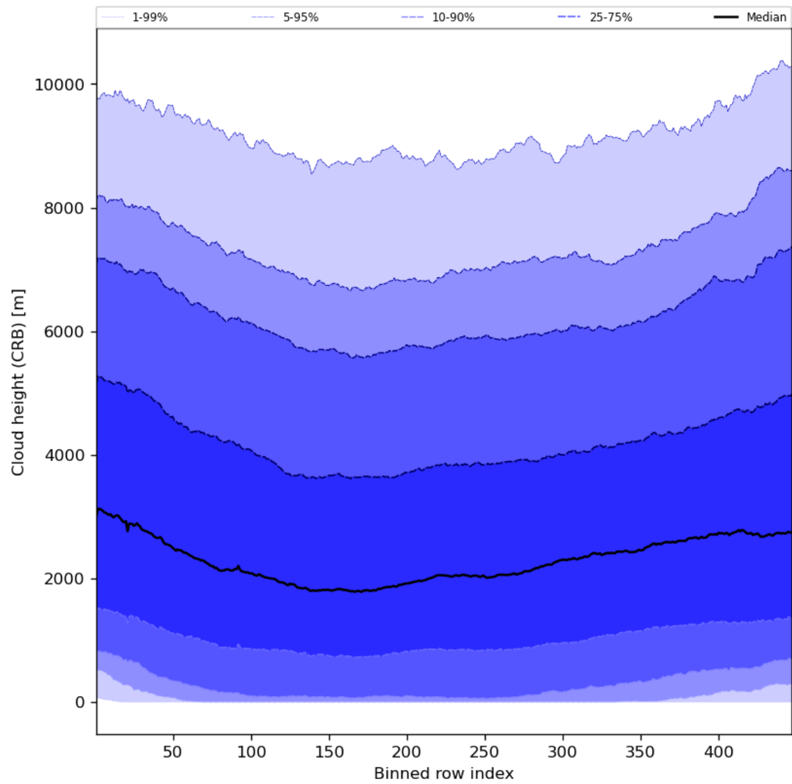
Figure 59: Along track statistics of “Cloud height (CRB)” for 2024-05-23 to 2024-05-24
