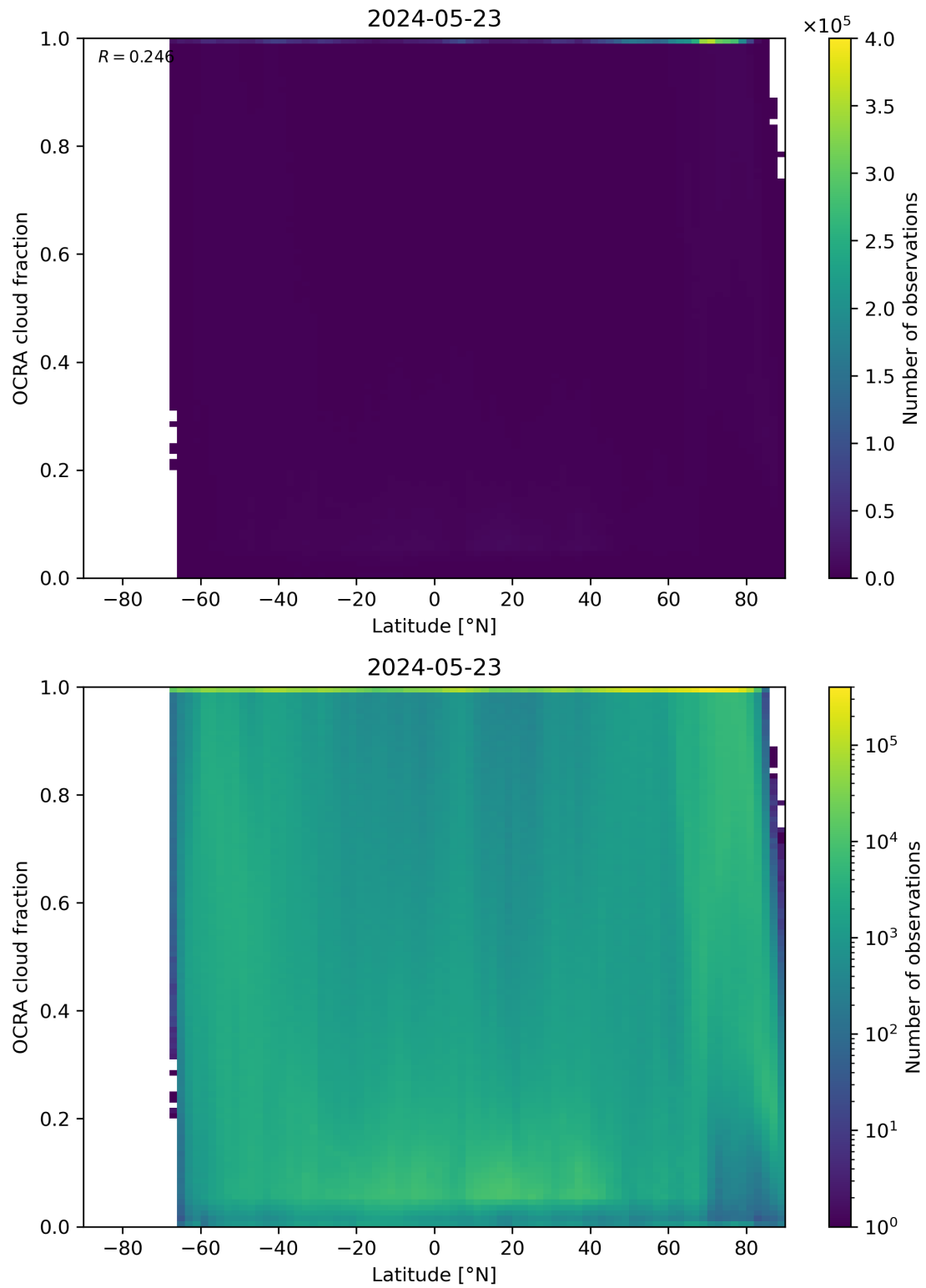
Figure 93: Scatter density plot of “Latitude” against “OCRA cloud fraction” for 2024-05-23 to 2024-05-24.
