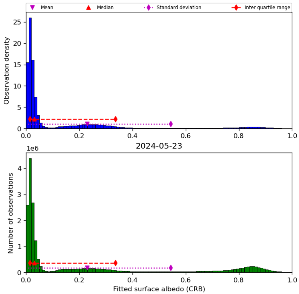
Figure 46: Histogram of “Fitted surface albedo (CRB)” for 2024-05-23 to 2024-05-24
