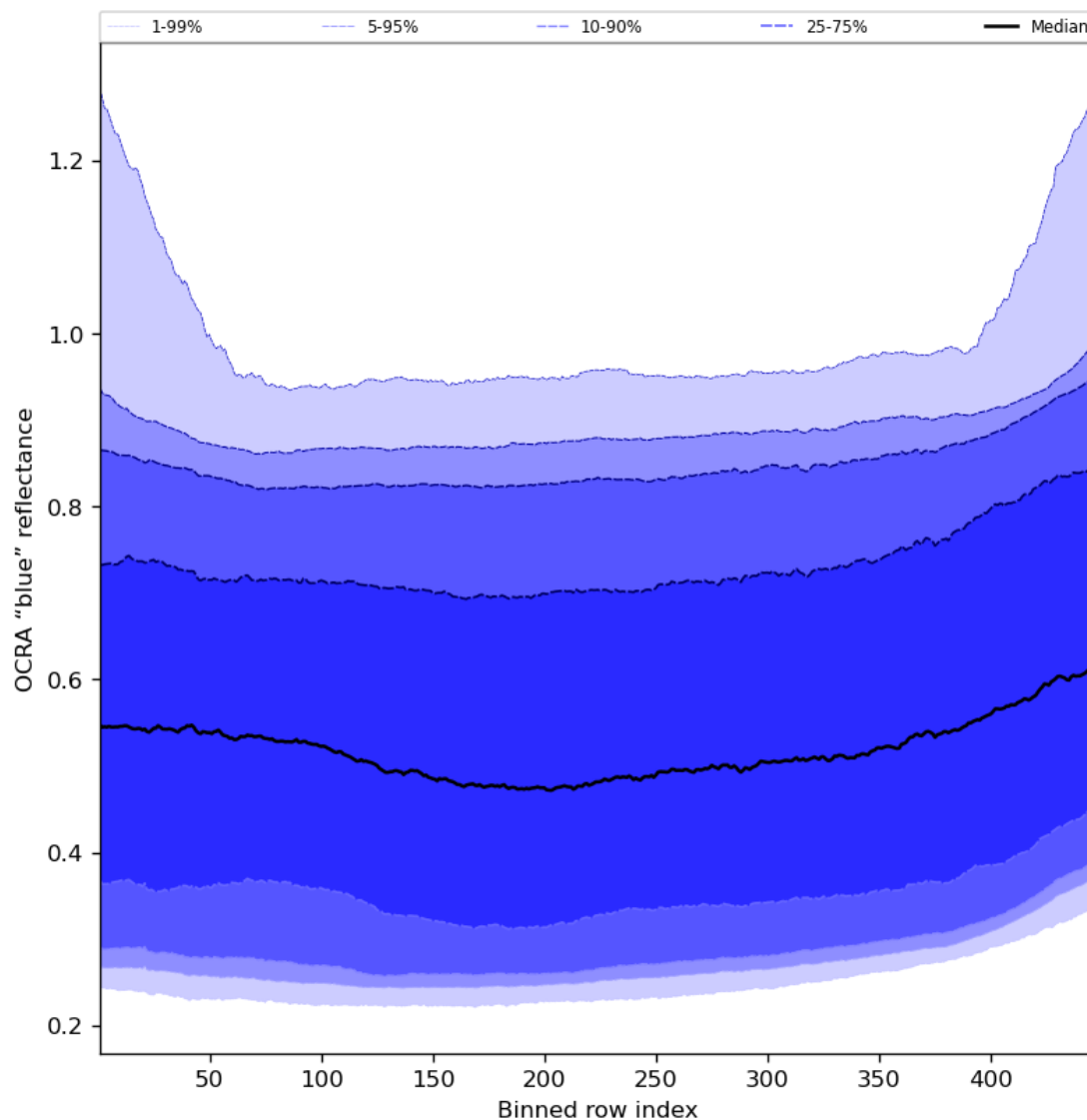
Figure 67: Along track statistics of “OCRA “blue” reflectance” for 2024-05-23 to 2024-05-24
