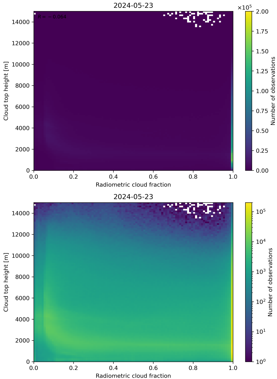
Figure 76: Scatter density plot of “Radiometric cloud fraction” against “Cloud top height” for 2024-05-23 to 2024-05-24.
