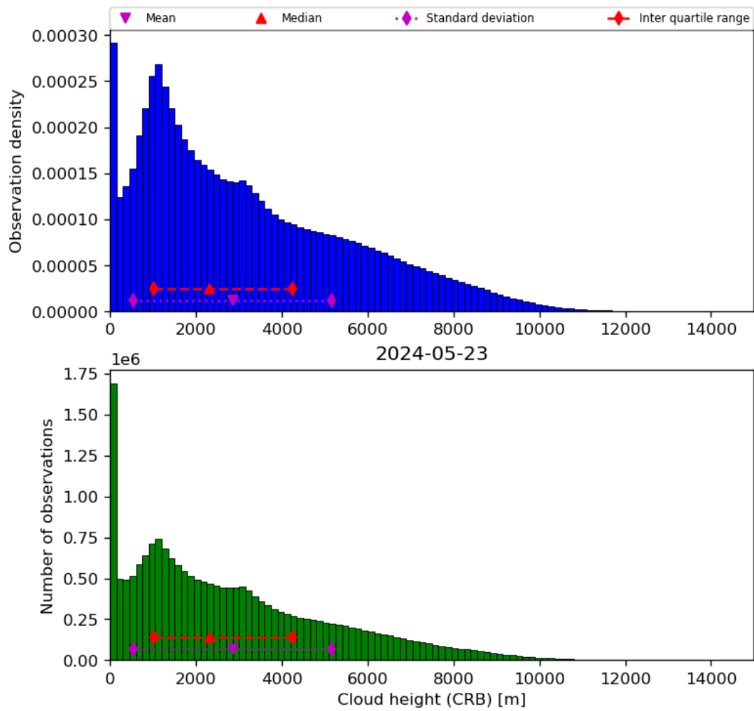
Figure 43: Histogram of “Cloud height (CRB)” for 2024-05-23 to 2024-05-24
