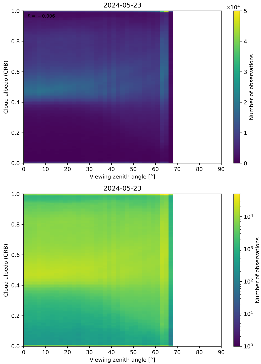
Figure 106: Scatter density plot of “Viewing zenith angle” against “Cloud albedo (CRB)” for 2024-05-23 to 2024-05-24.
