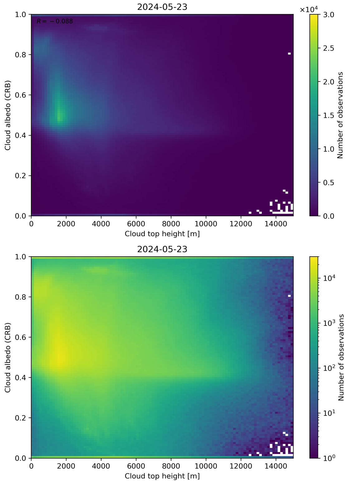
Figure 86: Scatter density plot of “Cloud top height” against “Cloud albedo (CRB)” for 2024-05-23 to 2024-05-24.
