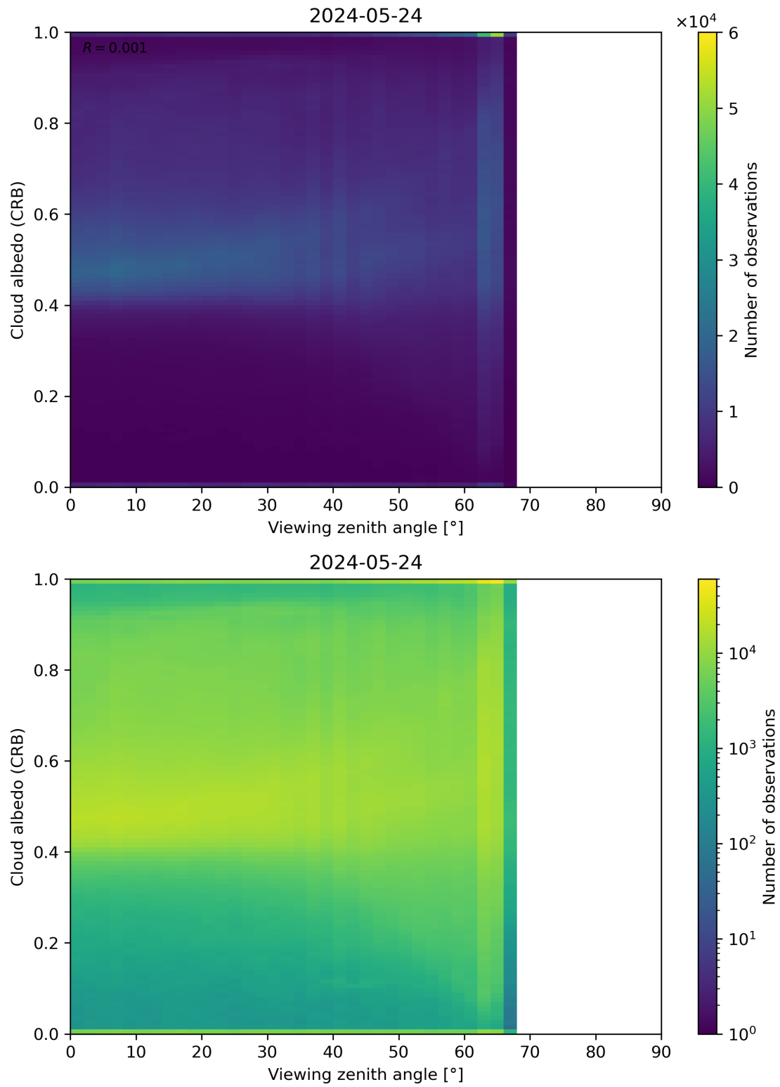
Figure 106: Scatter density plot of “Viewing zenith angle” against “Cloud albedo (CRB)” for 2024-05-23 to 2024-05-25.
