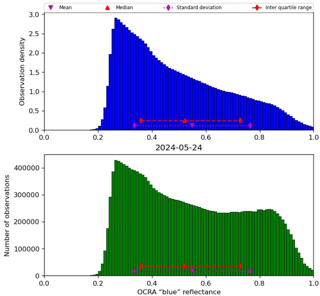
Figure 51: Histogram of “OCRA “blue” reflectance” for 2024-05-23 to 2024-05-25
