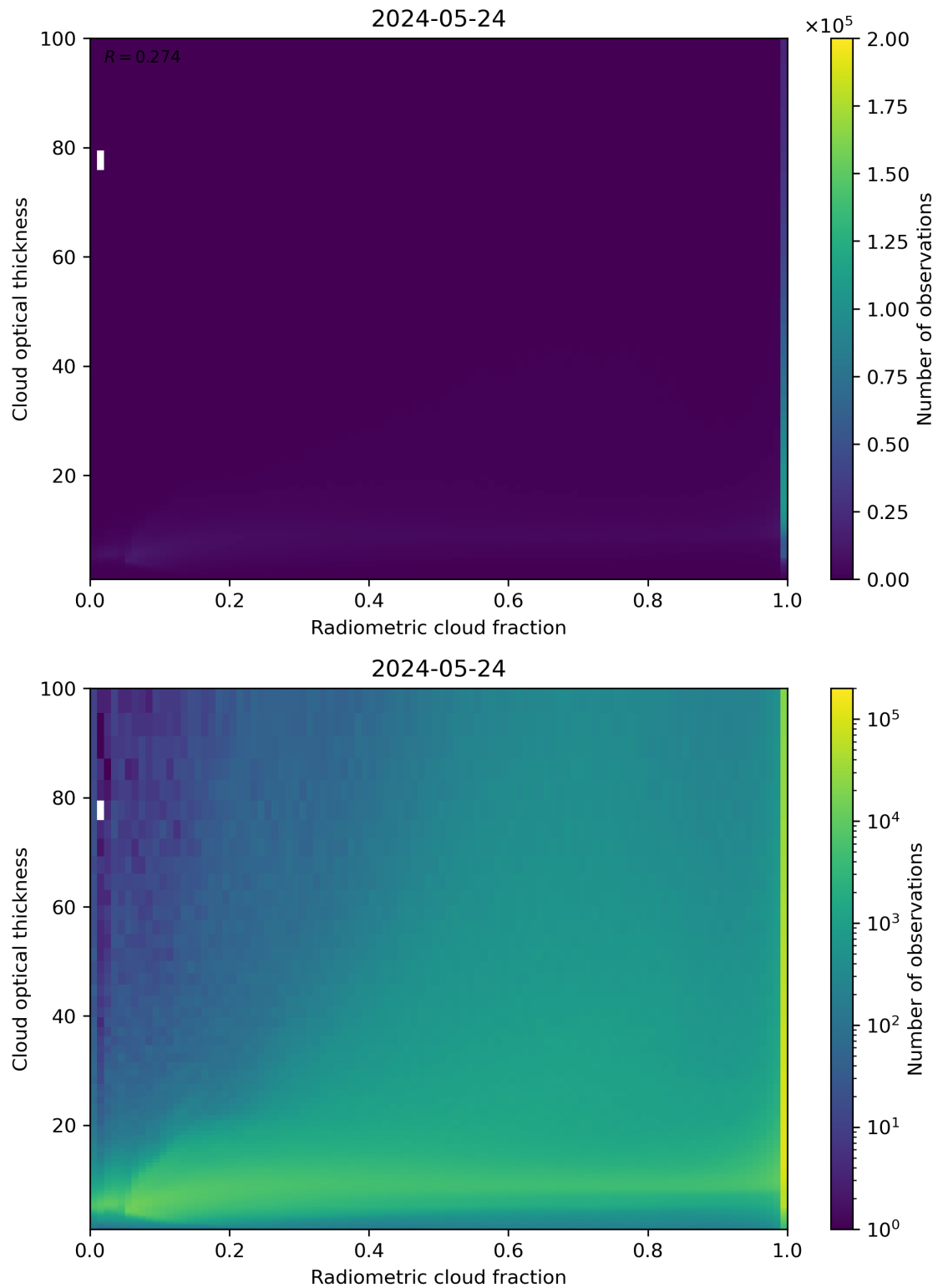
Figure 75: Scatter density plot of “Radiometric cloud fraction” against “Cloud optical thickness” for 2024-05-23 to 2024-05-25.
