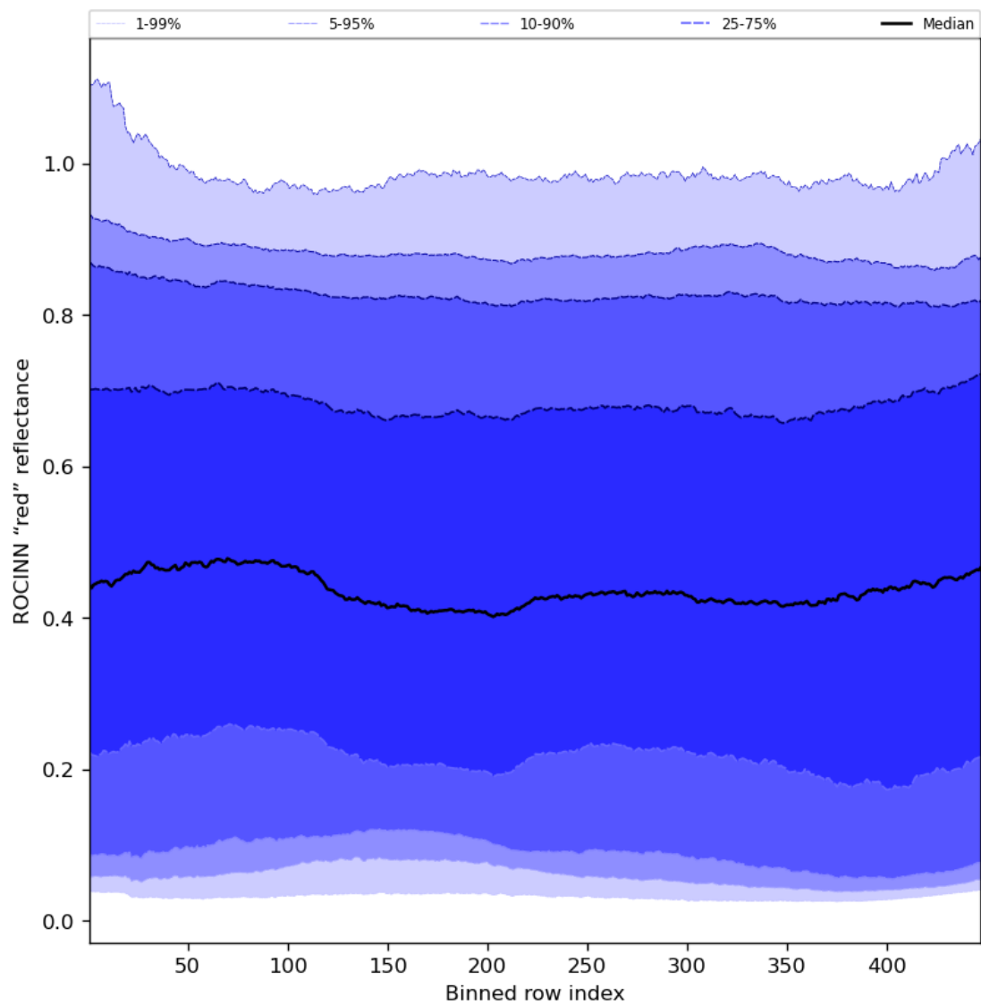
Figure 69: Along track statistics of “ROCINN “red” reflectance” for 2024-05-23 to 2024-05-25
