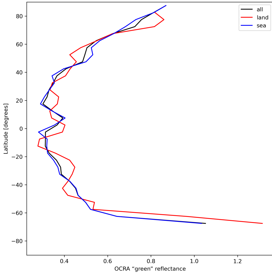
Figure 36: Zonal average of “OCRA “green” reflectance” for 2024-05-23 to 2024-05-25.
