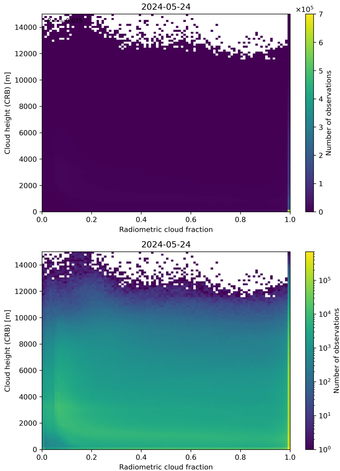
Figure 74: Scatter density plot of “Radiometric cloud fraction” against “Cloud height (CRB)” for 2024-05-23 to 2024-05-25.
