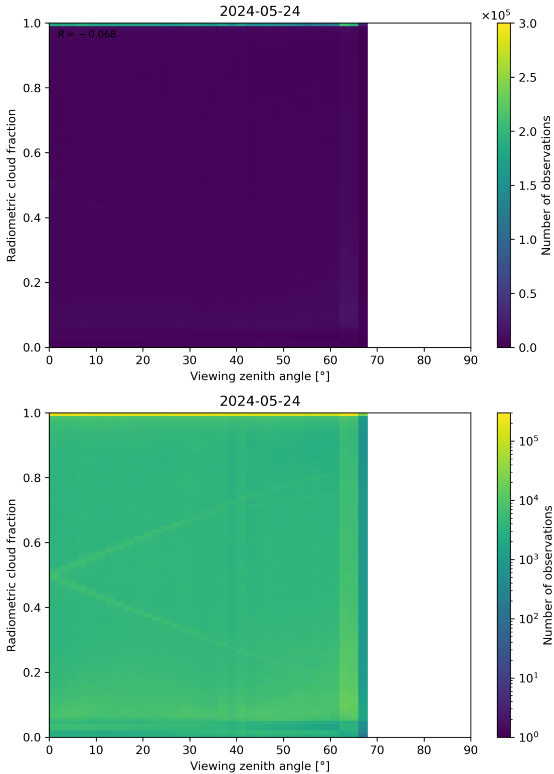
Figure 107: Scatter density plot of “Viewing zenith angle” against “Radiometric cloud fraction” for 2024-05-23 to 2024-05-25.
