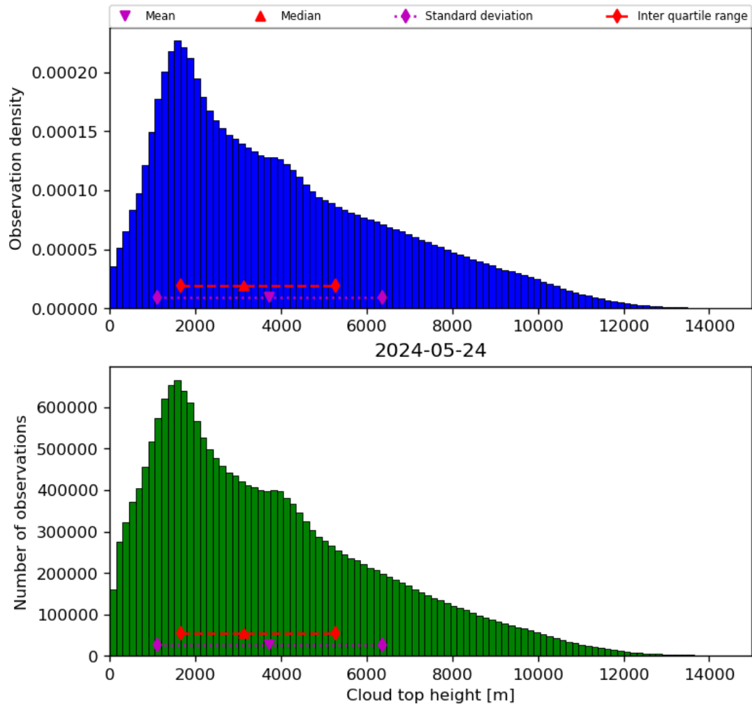
Figure 40: Histogram of “Cloud top height” for 2024-05-23 to 2024-05-25
