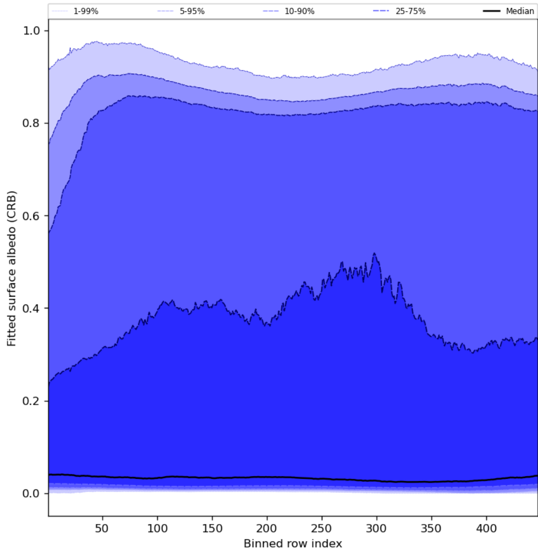
Figure 62: Along track statistics of “Fitted surface albedo (CRB)” for 2024-05-23 to 2024-05-25
