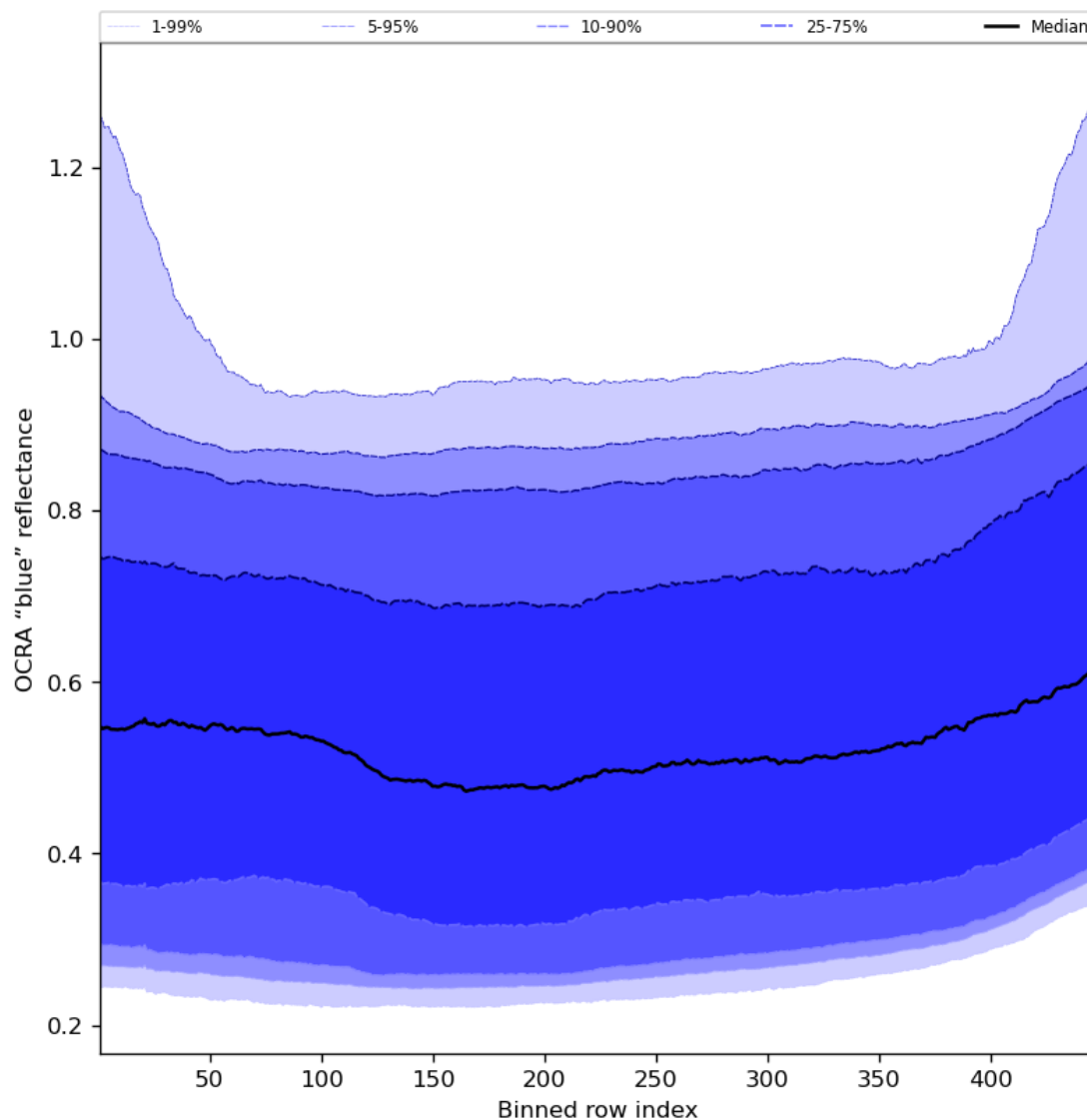
Figure 67: Along track statistics of “OCRA “blue” reflectance” for 2024-05-23 to 2024-05-25
