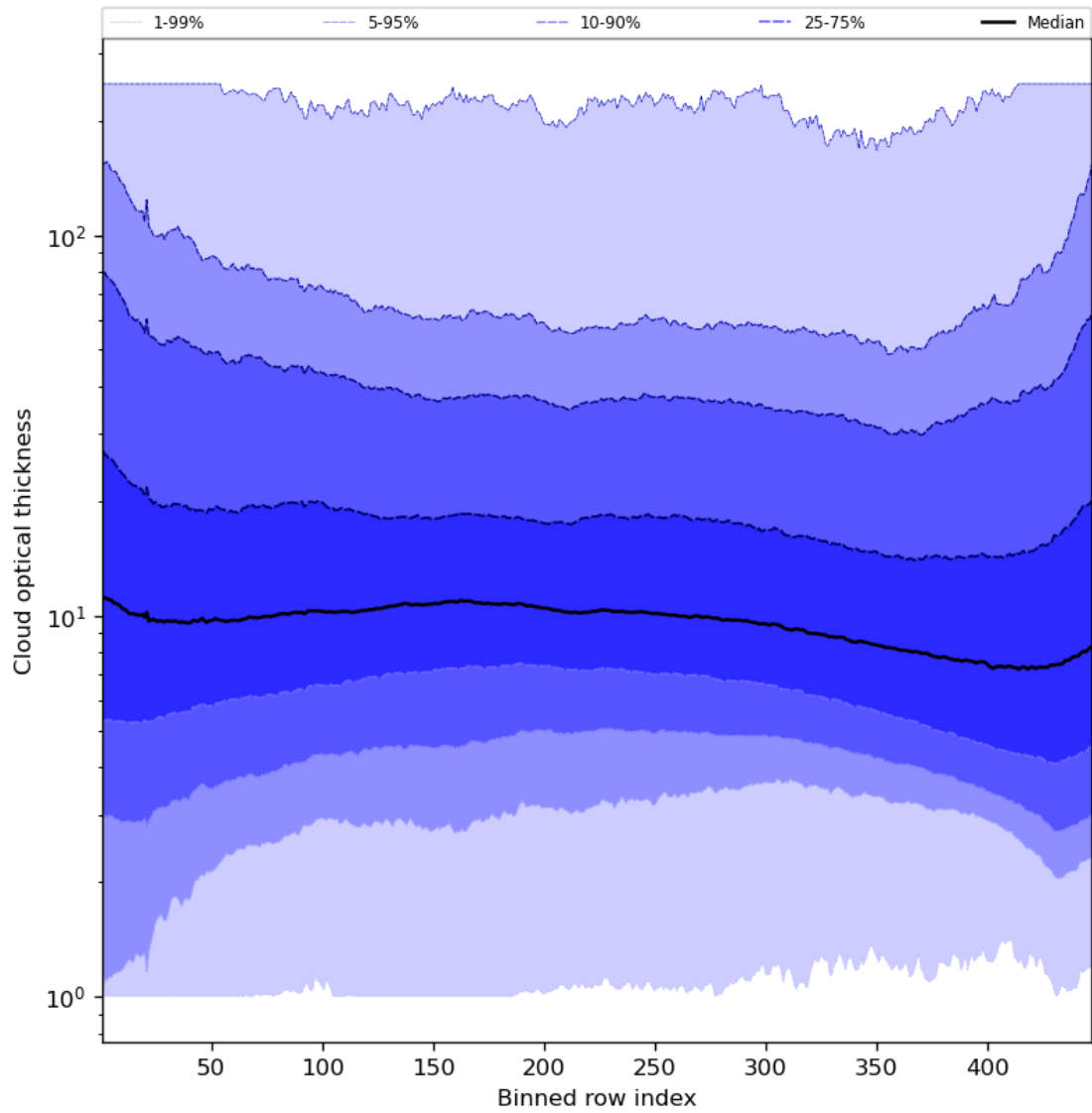
Figure 57: Along track statistics of “Cloud optical thickness” for 2024-05-23 to 2024-05-25
