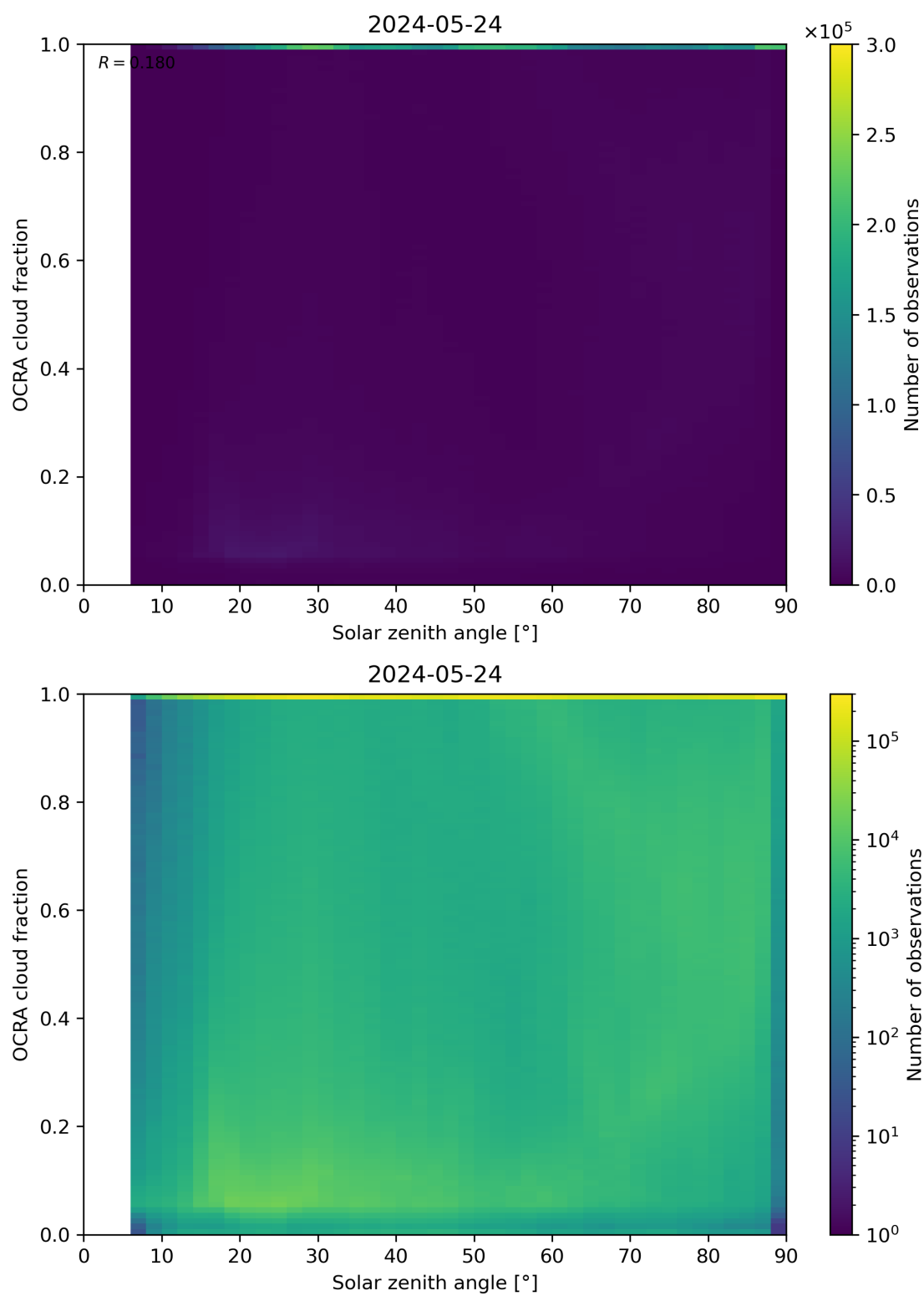
Figure 100: Scatter density plot of “Solar zenith angle” against “OCRA cloud fraction” for 2024-05-23 to 2024-05-25.
