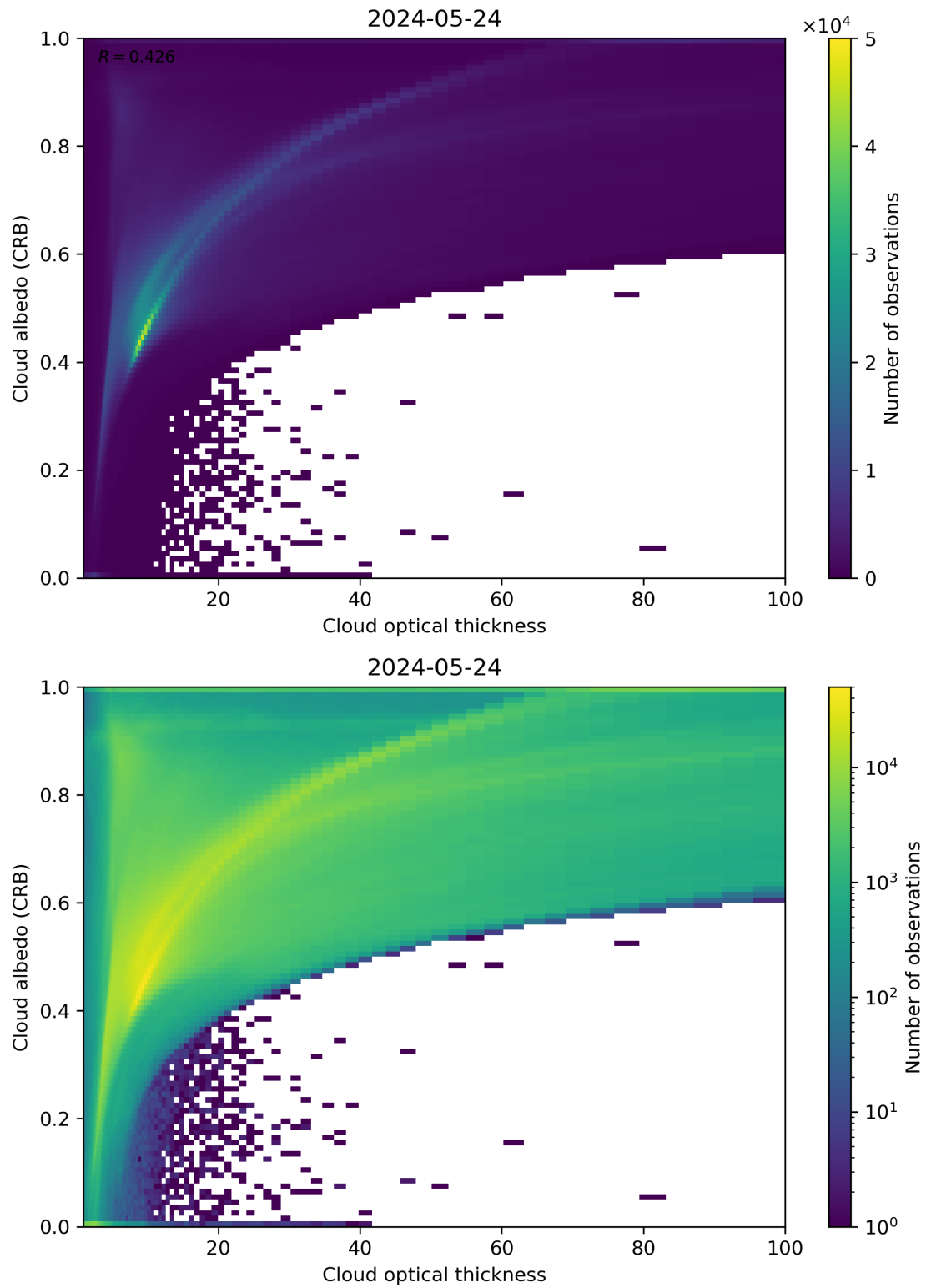
Figure 82: Scatter density plot of “Cloud optical thickness” against “Cloud albedo (CRB)” for 2024-05-23 to 2024-05-25.
