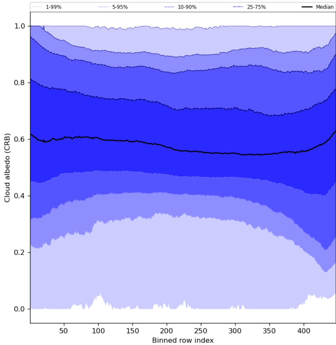
Figure 60: Along track statistics of “Cloud albedo (CRB)” for 2024-05-23 to 2024-05-25
