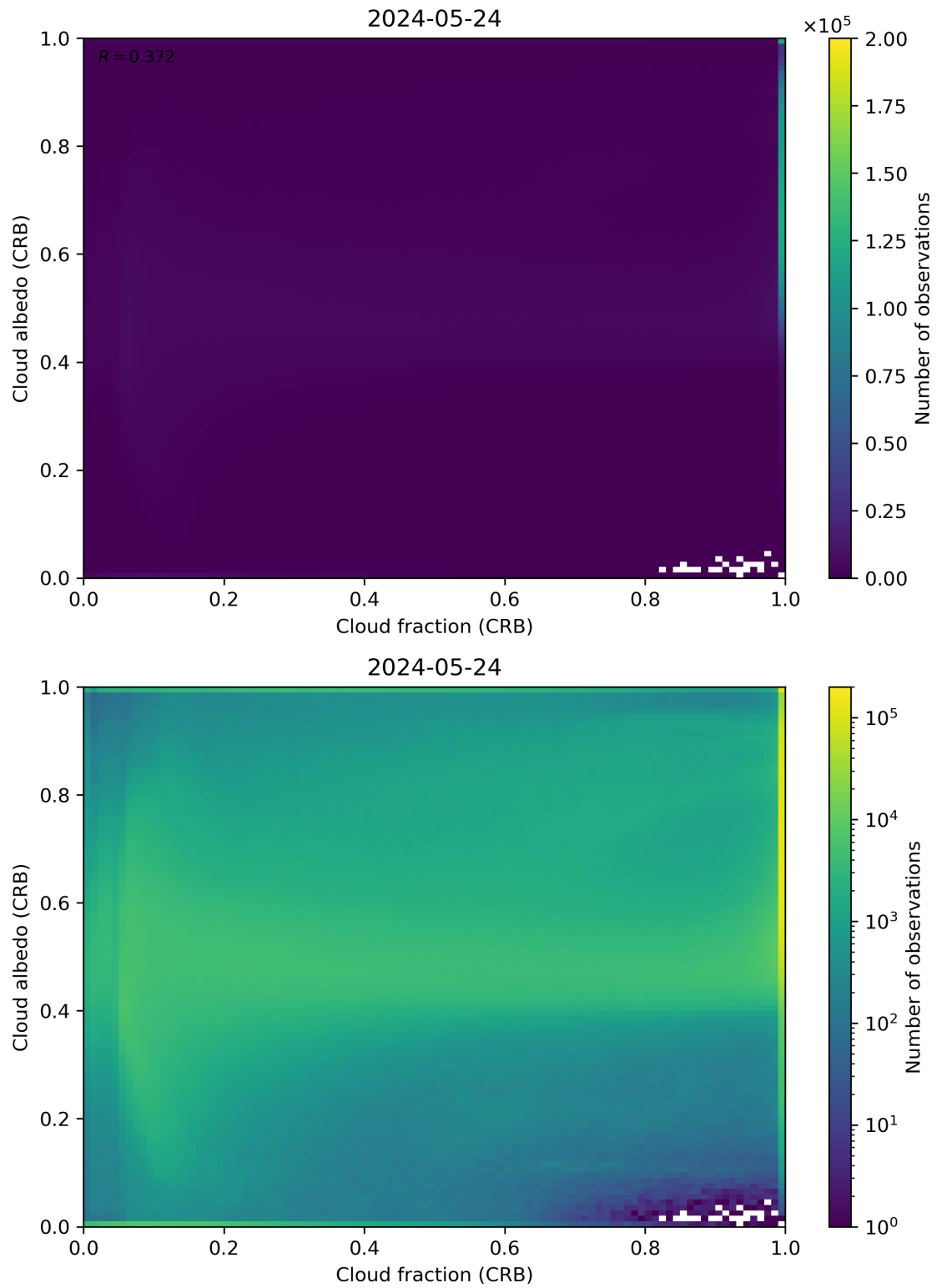
Figure 77: Scatter density plot of “Cloud fraction (CRB)” against “Cloud albedo (CRB)” for 2024-05-23 to 2024-05-25.
