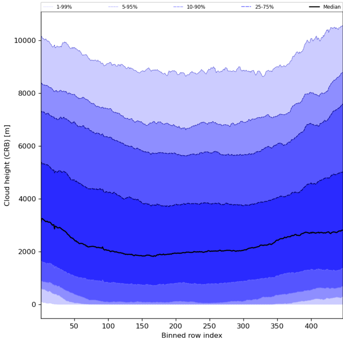
Figure 59: Along track statistics of "Cloud height (CRB)" for 2024-05-23 to 2024-05-25
