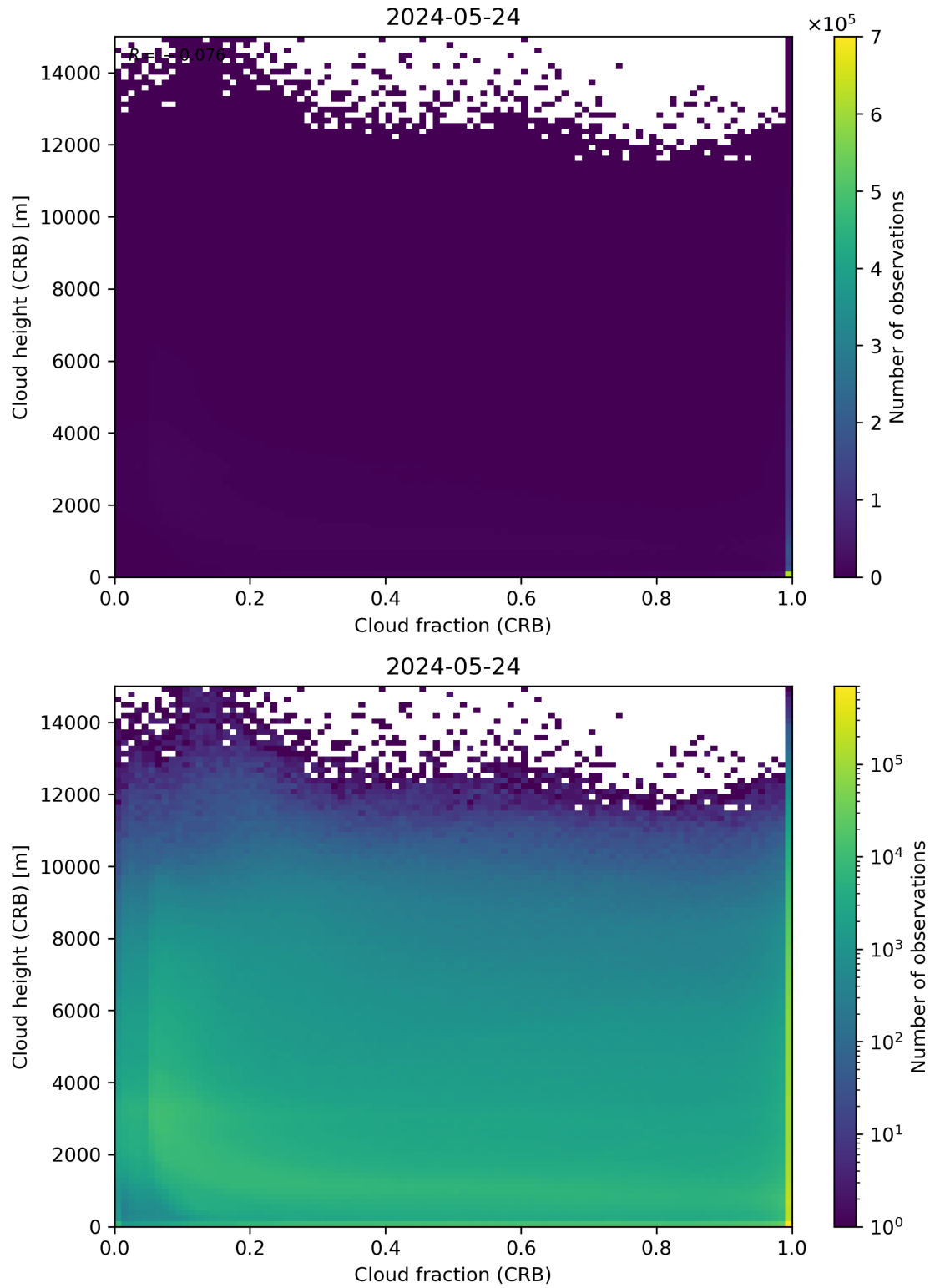
Figure 79: Scatter density plot of “Cloud fraction (CRB)” against “Cloud height (CRB)” for 2024-05-23 to 2024-05-25.
