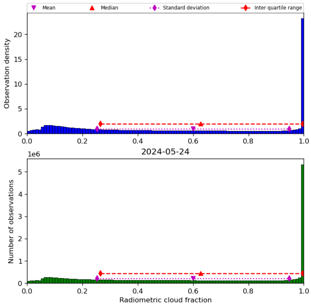
Figure 39: Histogram of “Radiometric cloud fraction” for 2024-05-23 to 2024-05-25
