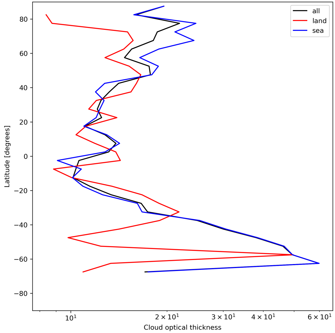
Figure 25: Zonal average of “Cloud optical thickness” for 2024-05-23 to 2024-05-25.
