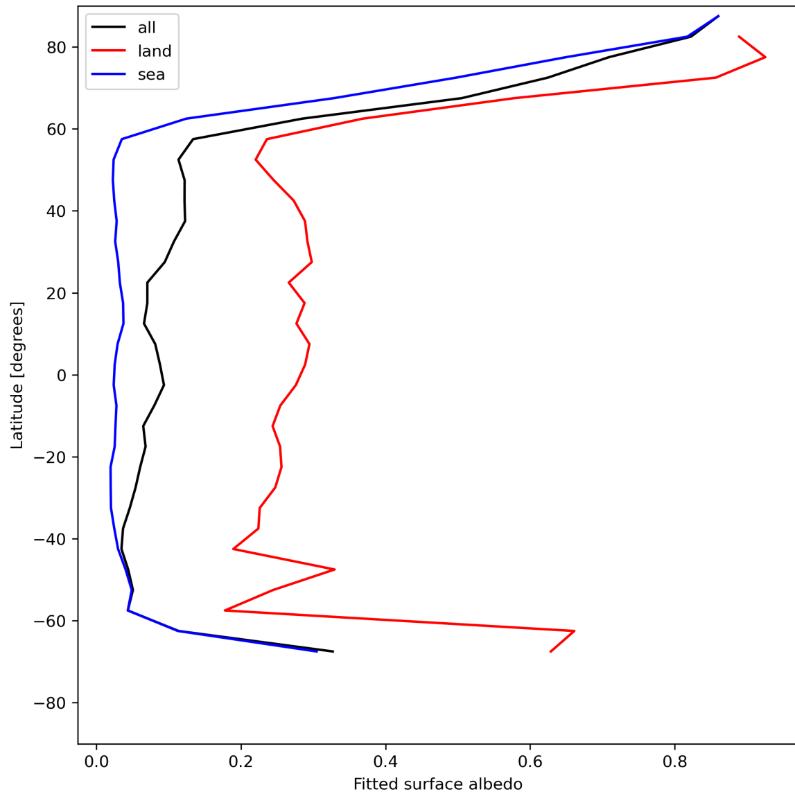
Figure 29: Zonal average of “Fitted surface albedo” for 2024-05-23 to 2024-05-25.
