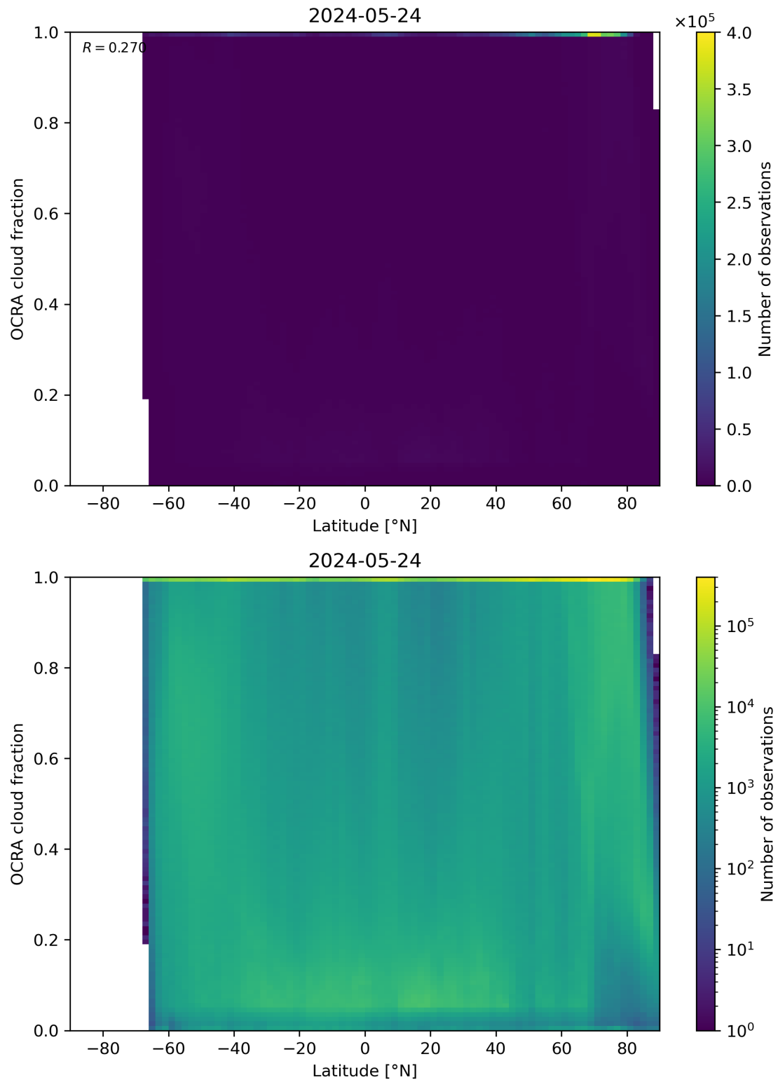
Figure 93: Scatter density plot of “Latitude” against “OCRA cloud fraction” for 2024-05-23 to 2024-05-25.
