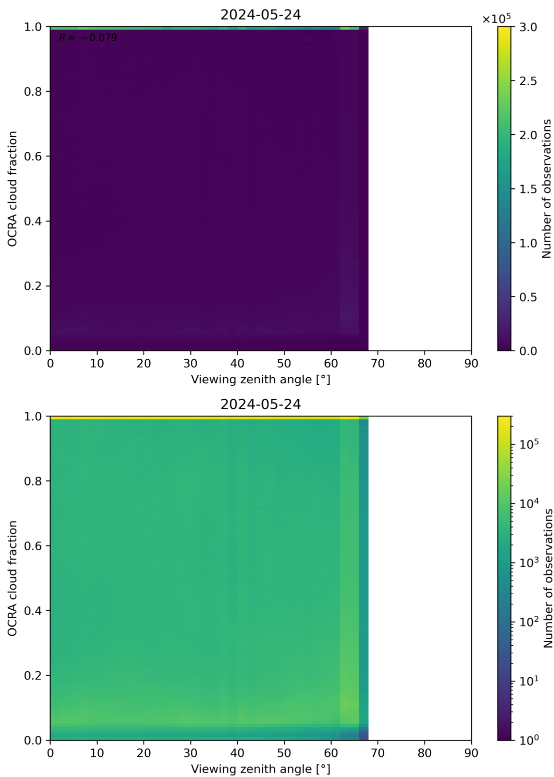
Figure 108: Scatter density plot of “Viewing zenith angle” against “OCRA cloud fraction” for 2024-05-23 to 2024-05-25.
