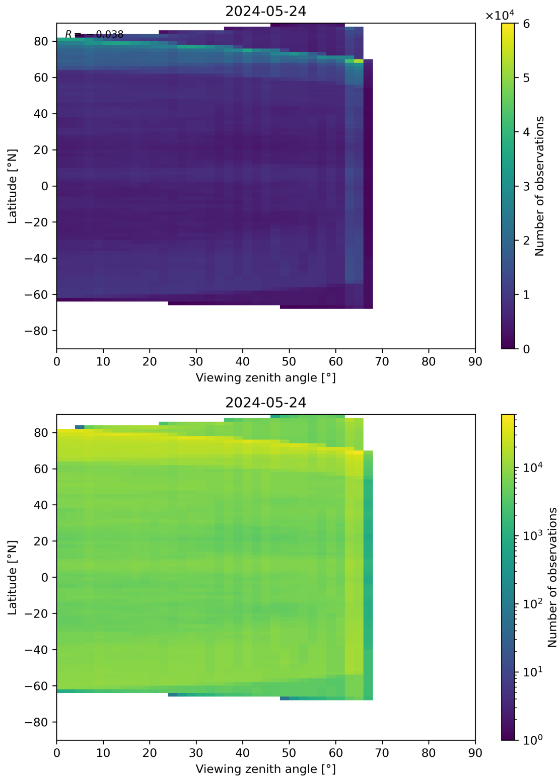
Figure 113: Scatter density plot of “Viewing zenith angle” against “Latitude” for 2024-05-23 to 2024-05-25.
