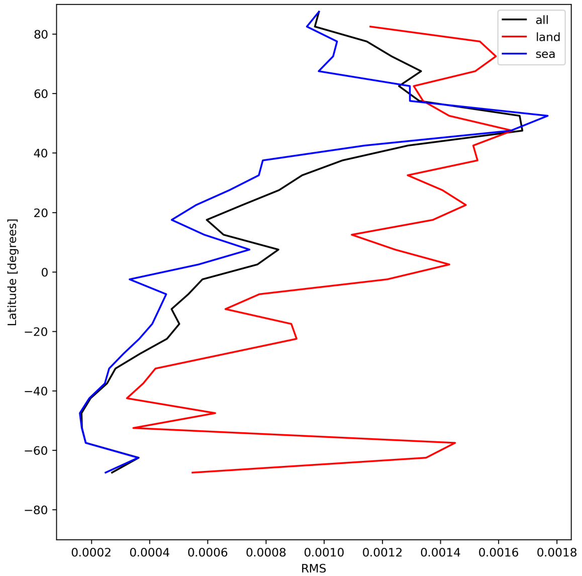
Figure 31: Zonal average of “RMS” for 2024-05-23 to 2024-05-25.
