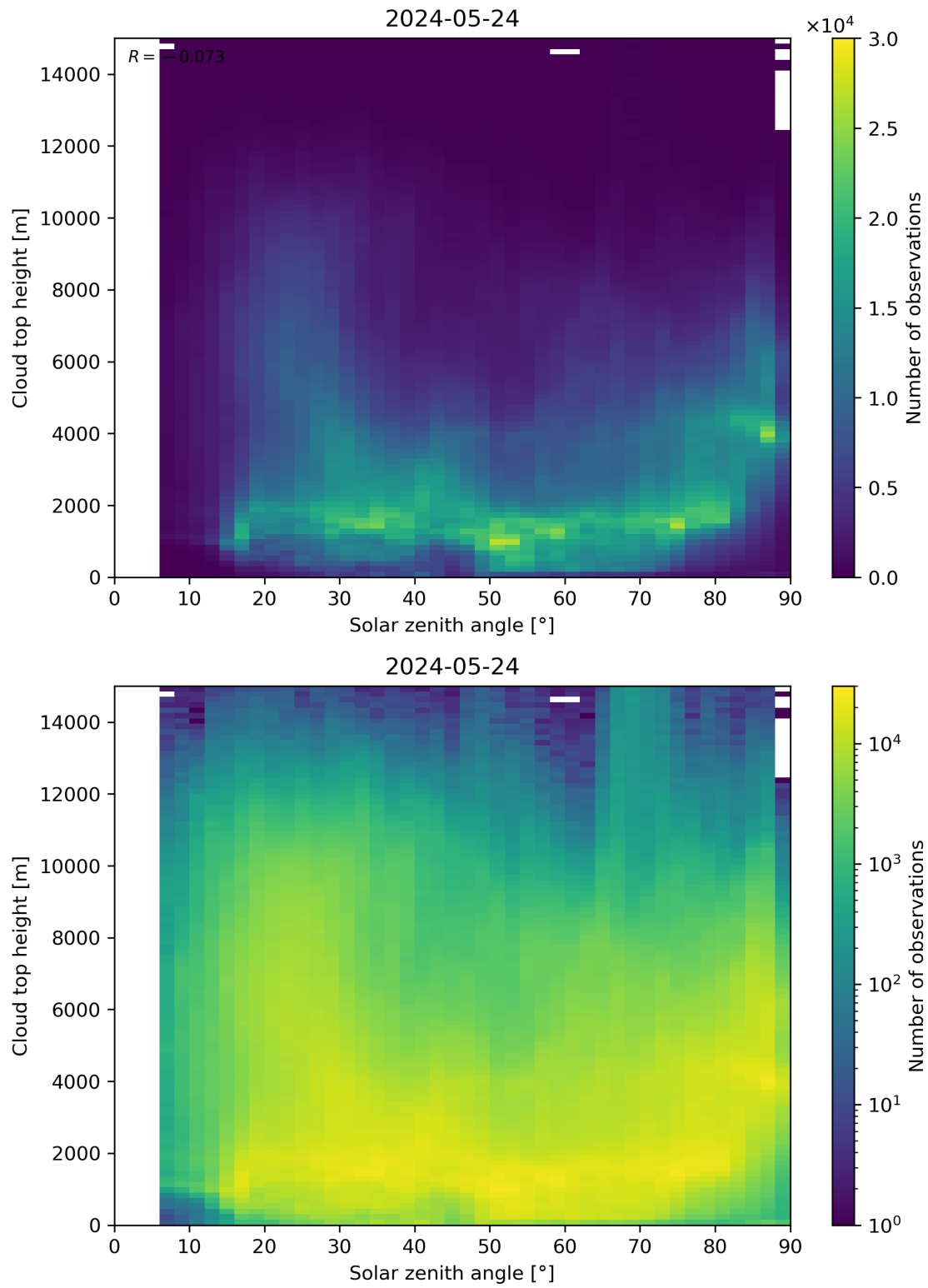
Figure 104: Scatter density plot of “Solar zenith angle” against “Cloud top height” for 2024-05-23 to 2024-05-25.
