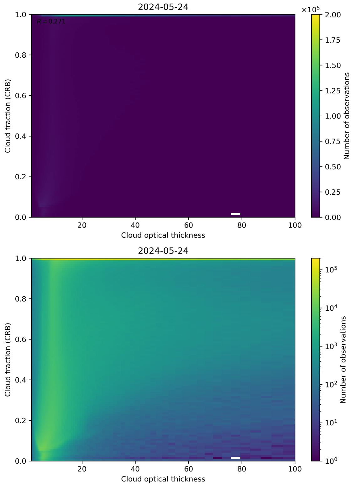
Figure 84: Scatter density plot of “Cloud optical thickness” against “Cloud fraction (CRB)” for 2024-05-23 to 2024-05-25.
