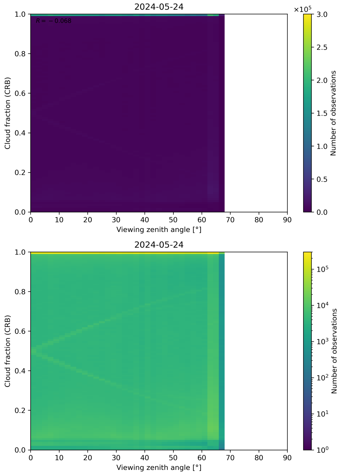
Figure 109: Scatter density plot of “Viewing zenith angle” against “Cloud fraction (CRB)” for 2024-05-23 to 2024-05-25.
