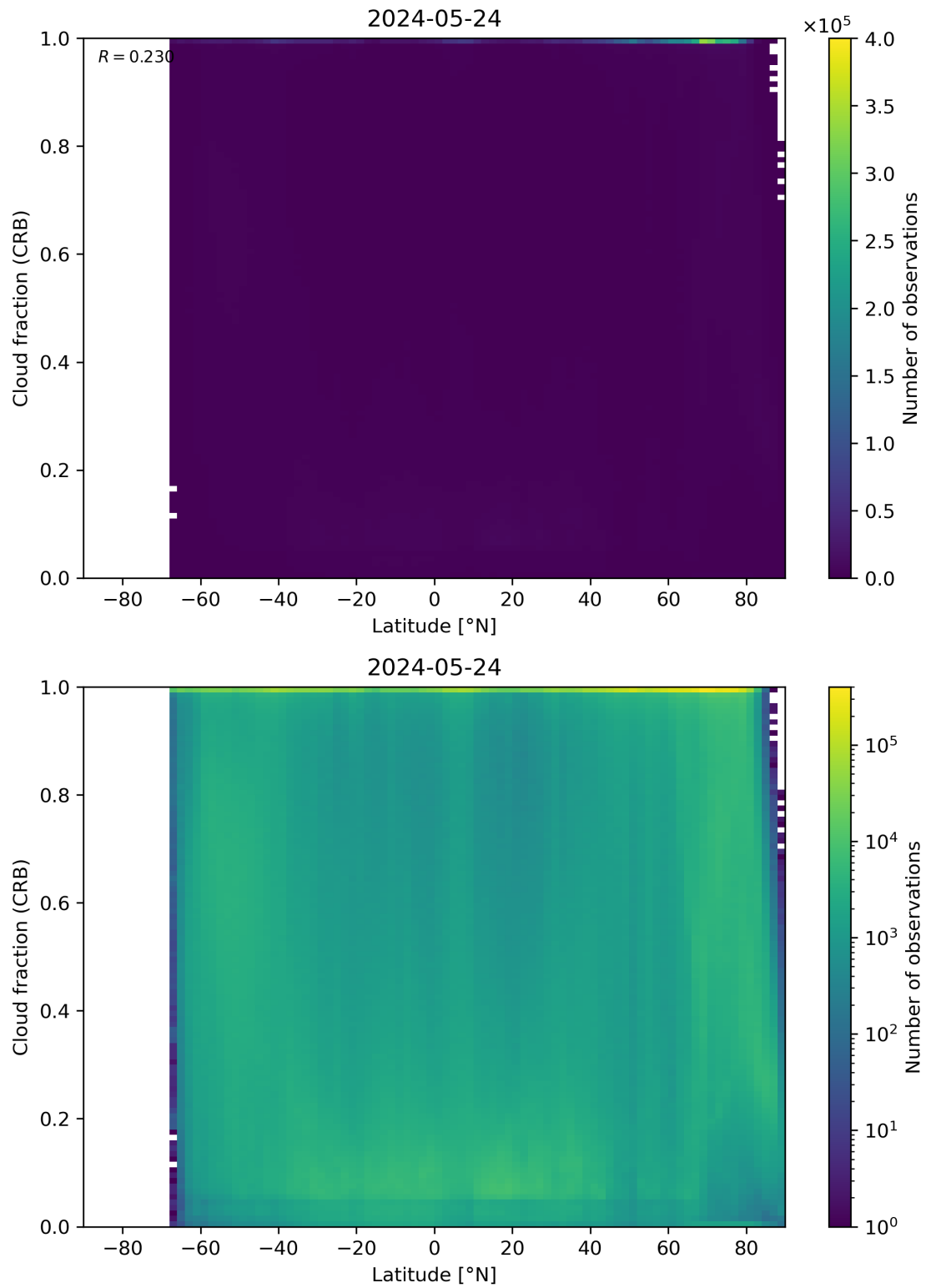
Figure 94: Scatter density plot of “Latitude” against “Cloud fraction (CRB)” for 2024-05-23 to 2024-05-25.
