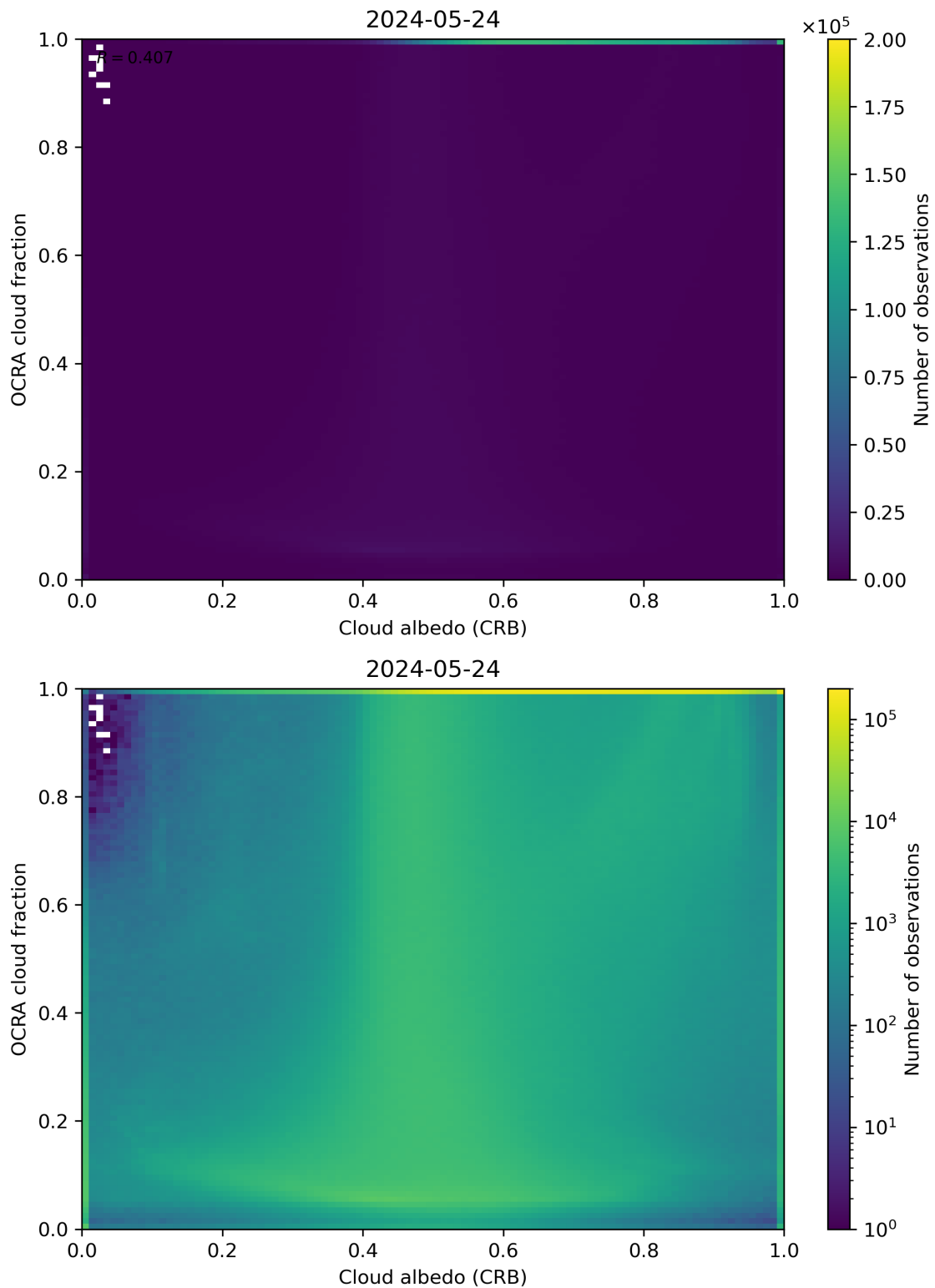
Figure 70: Scatter density plot of “Cloud albedo (CRB)” against “OCRA cloud fraction” for 2024-05-23 to 2024-05-25.
