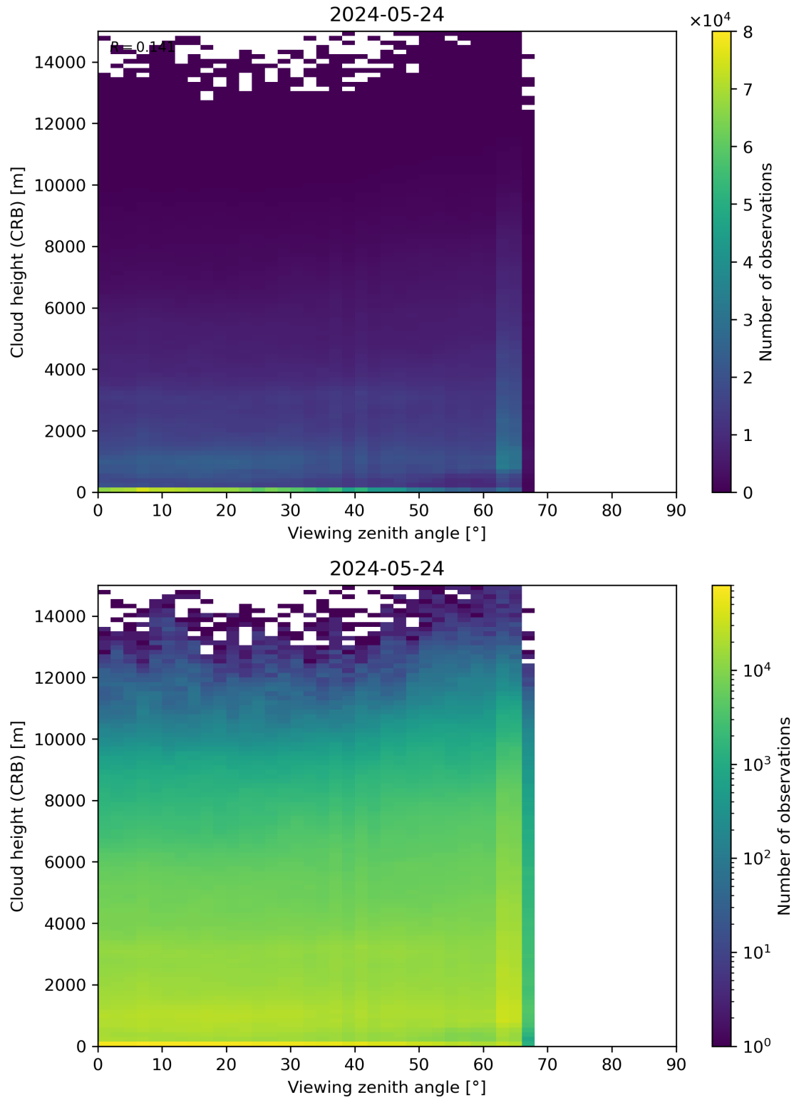
Figure 110: Scatter density plot of “Viewing zenith angle” against “Cloud height (CRB)” for 2024-05-23 to 2024-05-25.
