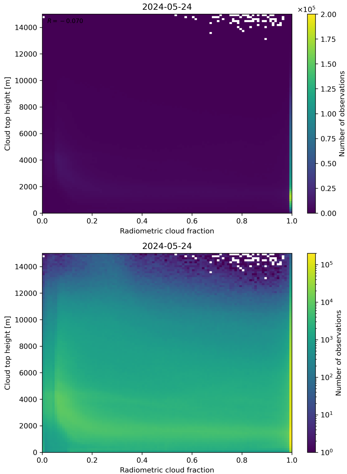
Figure 76: Scatter density plot of “Radiometric cloud fraction” against “Cloud top height” for 2024-05-23 to 2024-05-25.
