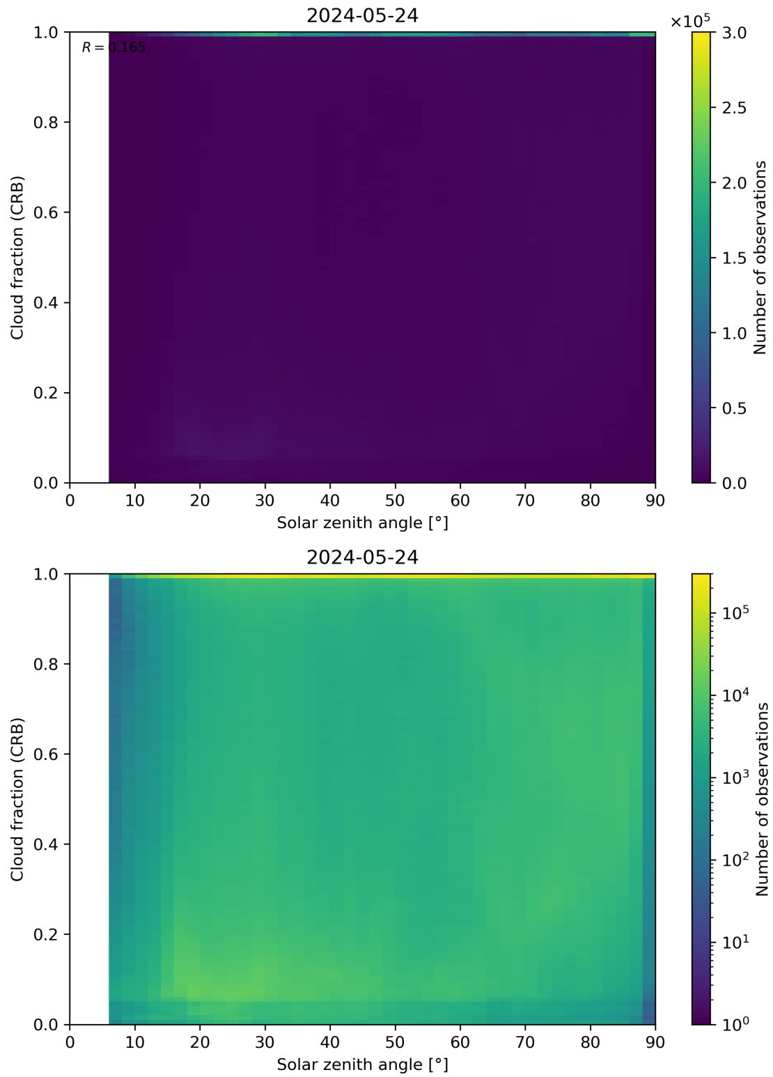
Figure 101: Scatter density plot of “Solar zenith angle” against “Cloud fraction (CRB)” for 2024-05-23 to 2024-05-25.
