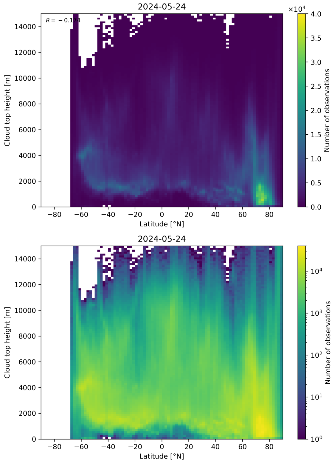
Figure 97: Scatter density plot of “Latitude” against “Cloud top height” for 2024-05-23 to 2024-05-25.
