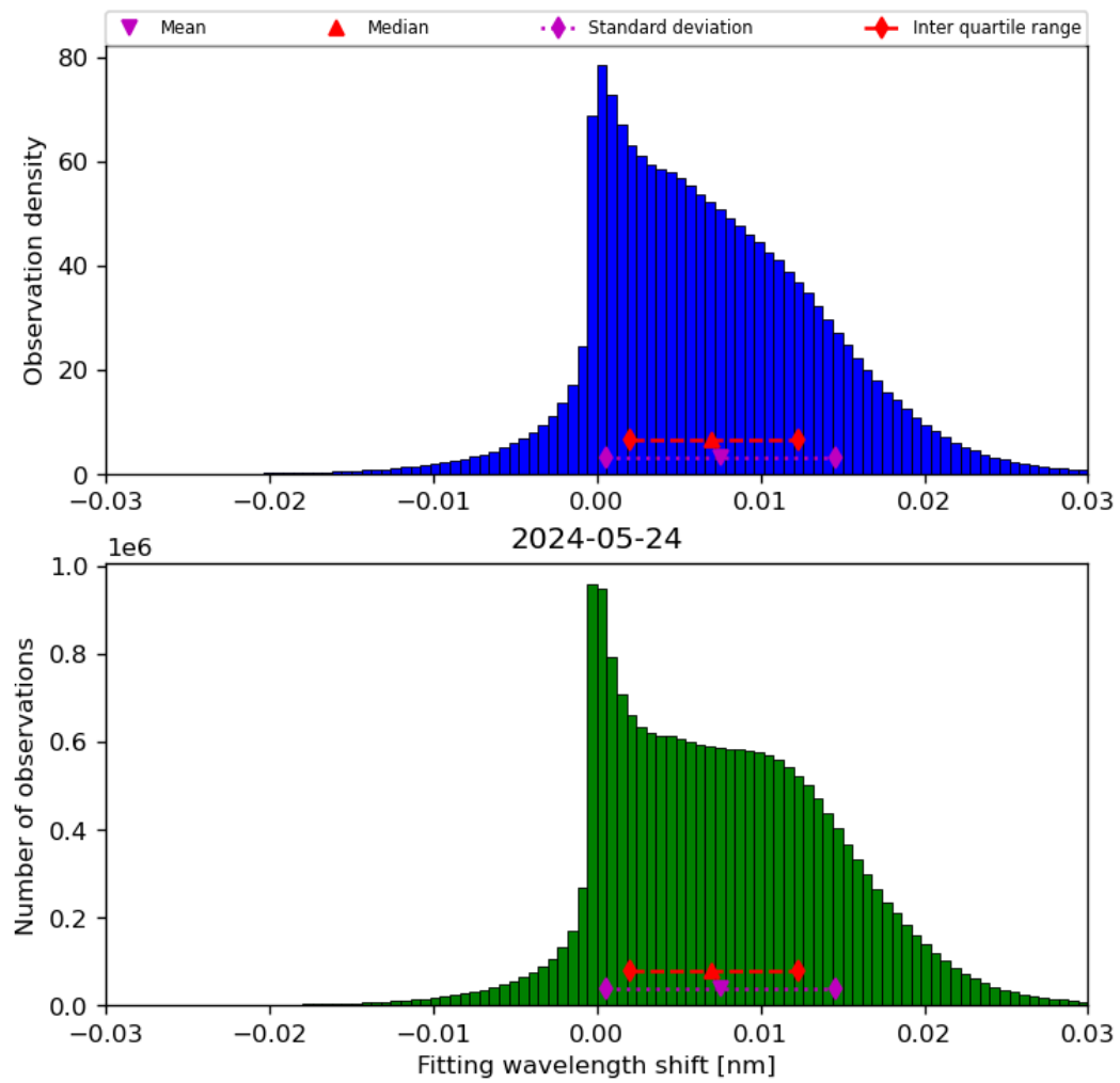
Figure 49: Histogram of “Fitting wavelength shift” for 2024-05-23 to 2024-05-25
