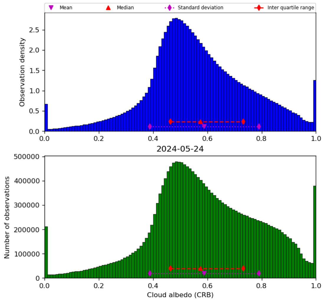
Figure 44: Histogram of “Cloud albedo (CRB)” for 2024-05-23 to 2024-05-25
