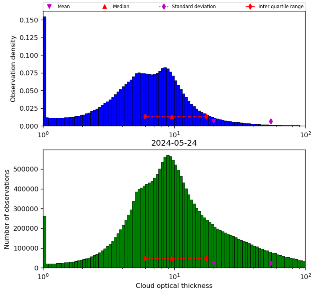
Figure 41: Histogram of “Cloud optical thickness” for 2024-05-23 to 2024-05-25
