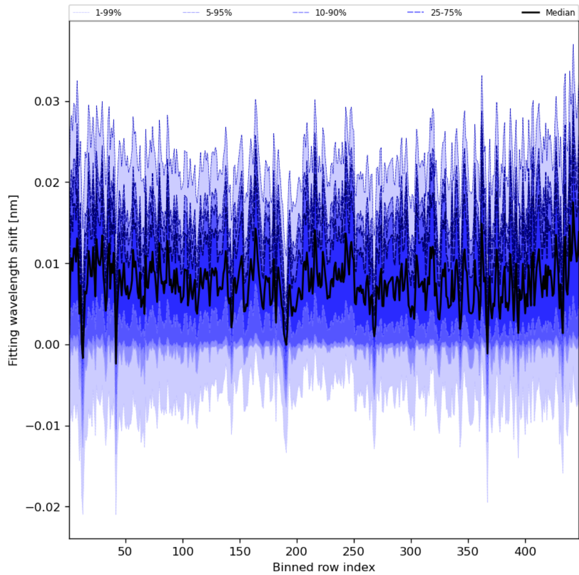
Figure 65: Along track statistics of “Fitting wavelength shift” for 2024-05-23 to 2024-05-25
