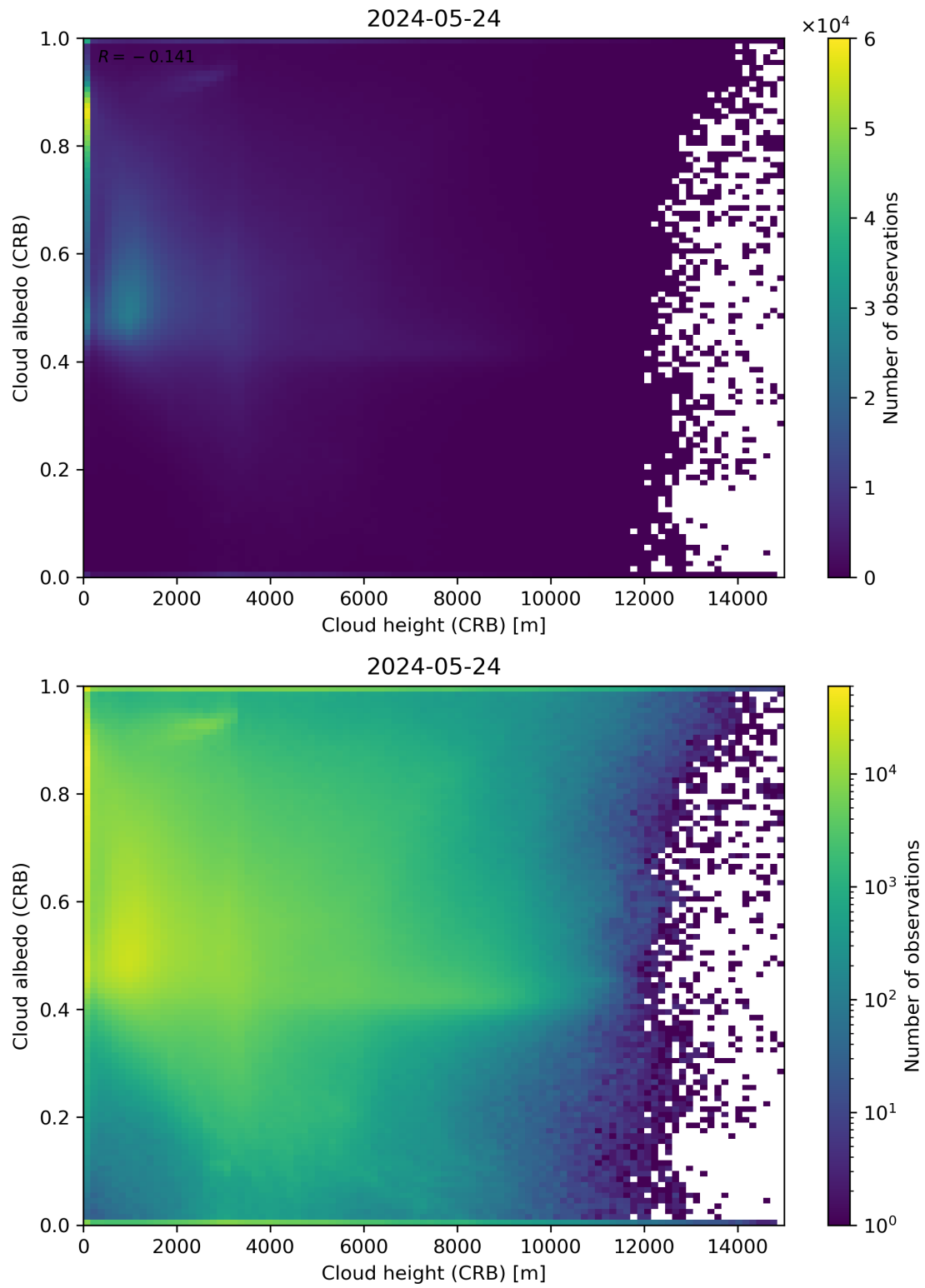
Figure 80: Scatter density plot of “Cloud height (CRB)” against “Cloud albedo (CRB)” for 2024-05-23 to 2024-05-25.
