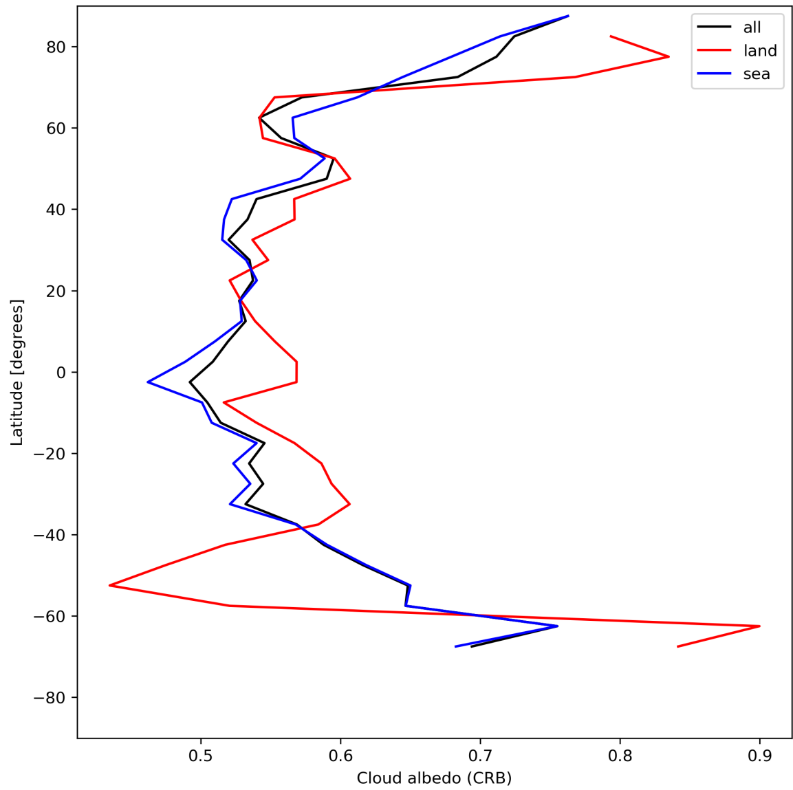
Figure 28: Zonal average of “Cloud albedo (CRB)” for 2024-05-23 to 2024-05-25.
