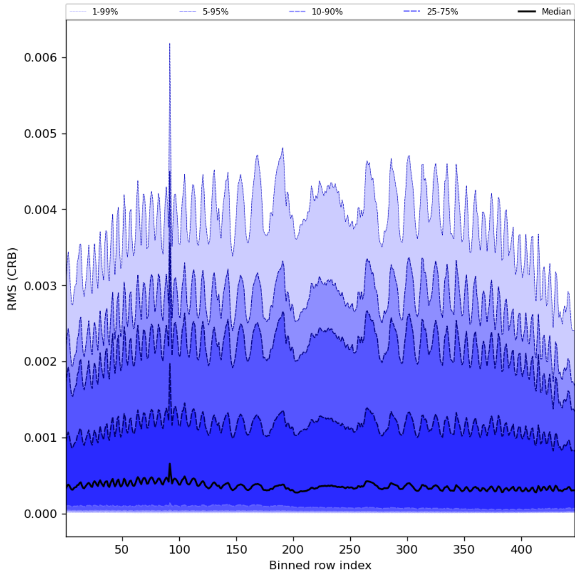
Figure 64: Along track statistics of “RMS (CRB)” for 2024-05-23 to 2024-05-25
