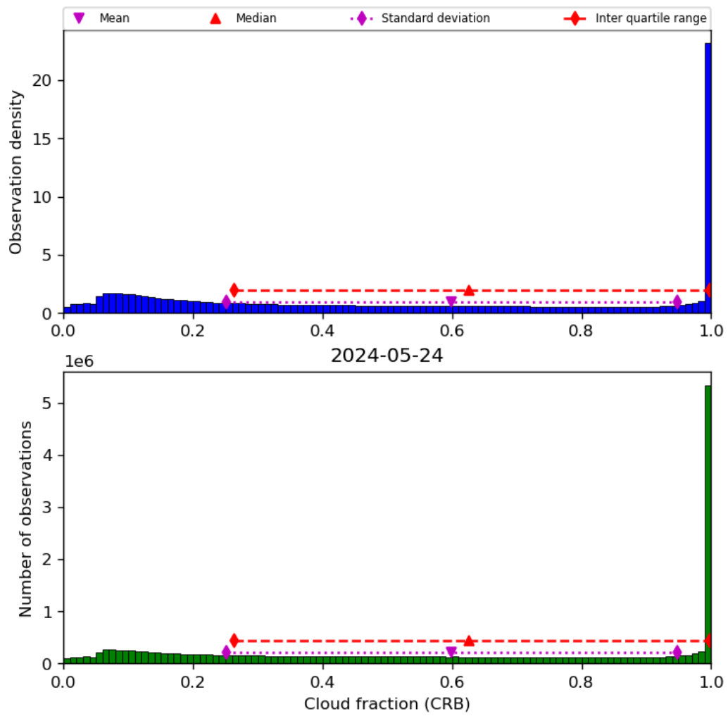
Figure 42: Histogram of “Cloud fraction (CRB)” for 2024-05-23 to 2024-05-25
