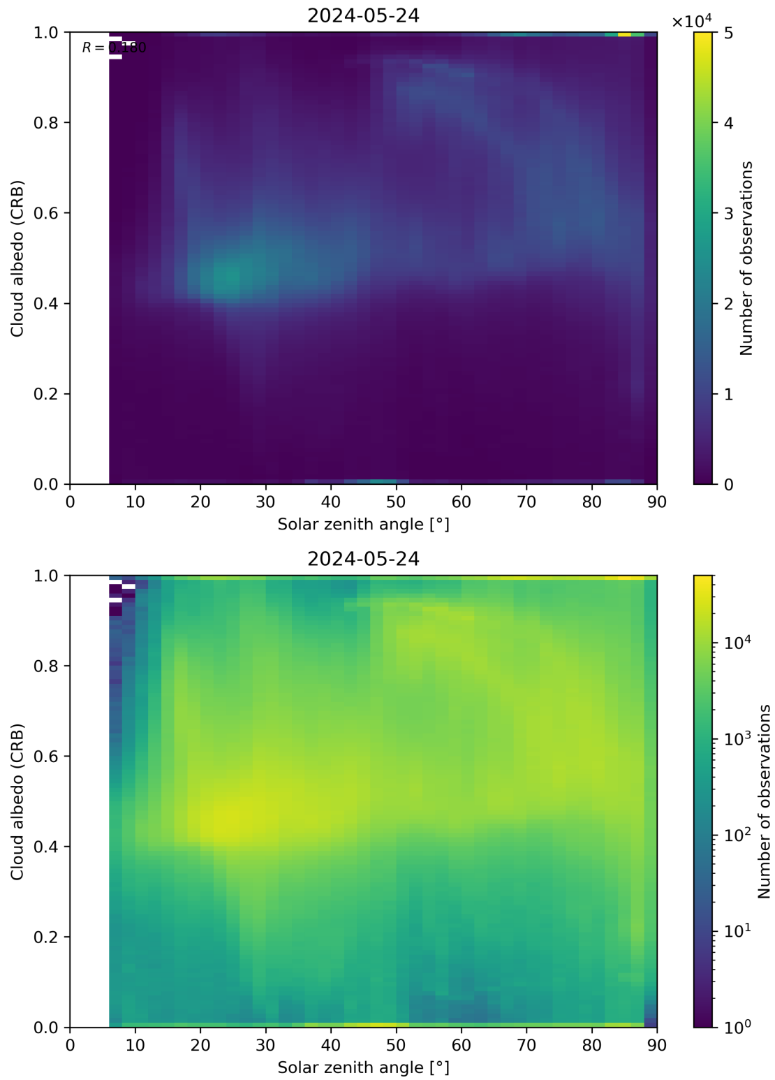
Figure 98: Scatter density plot of “Solar zenith angle” against “Cloud albedo (CRB)” for 2024-05-23 to 2024-05-25.
