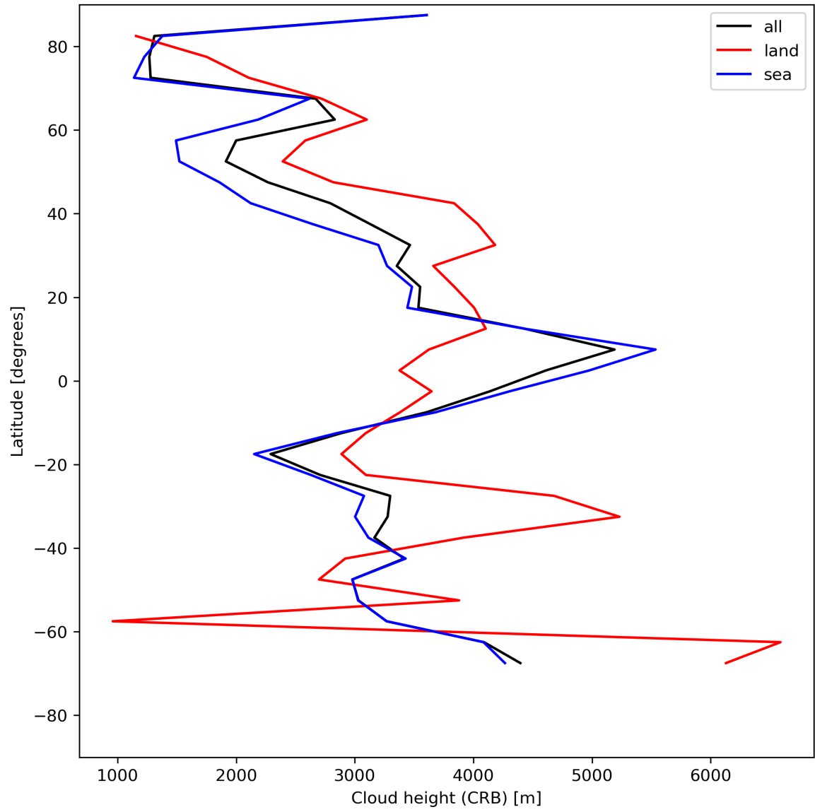
Figure 27: Zonal average of “Cloud height (CRB)” for 2024-05-23 to 2024-05-25.
