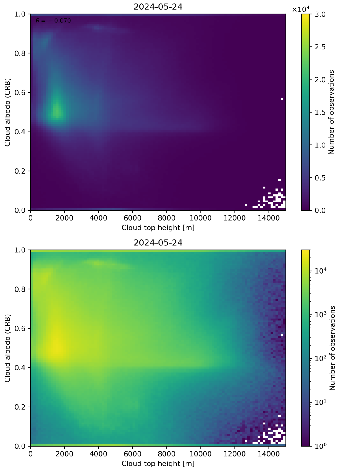
Figure 86: Scatter density plot of “Cloud top height” against “Cloud albedo (CRB)” for 2024-05-23 to 2024-05-25.
