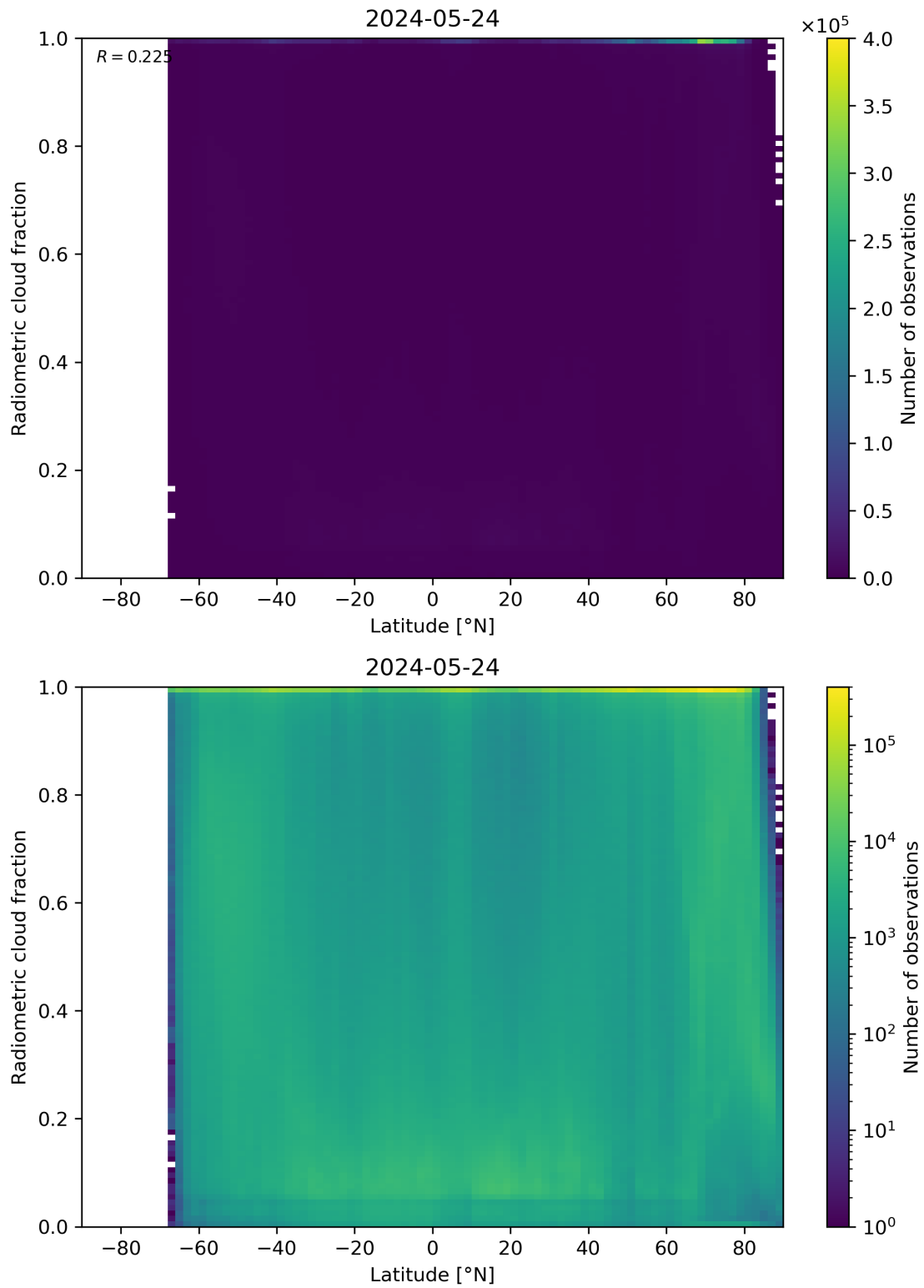
Figure 92: Scatter density plot of “Latitude” against “Radiometric cloud fraction” for 2024-05-23 to 2024-05-25.
