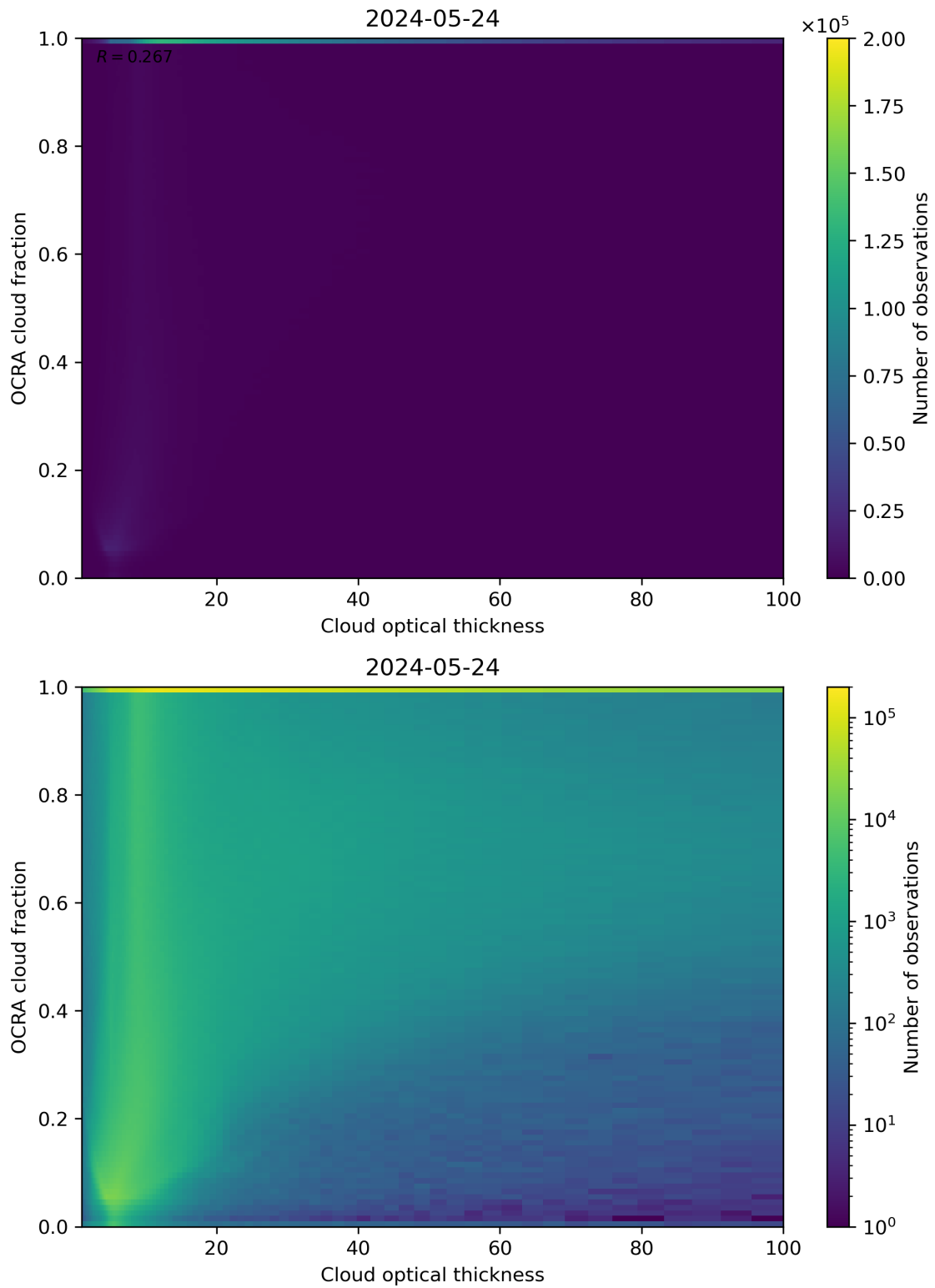
Figure 83: Scatter density plot of “Cloud optical thickness” against “OCRA cloud fraction” for 2024-05-23 to 2024-05-25.
