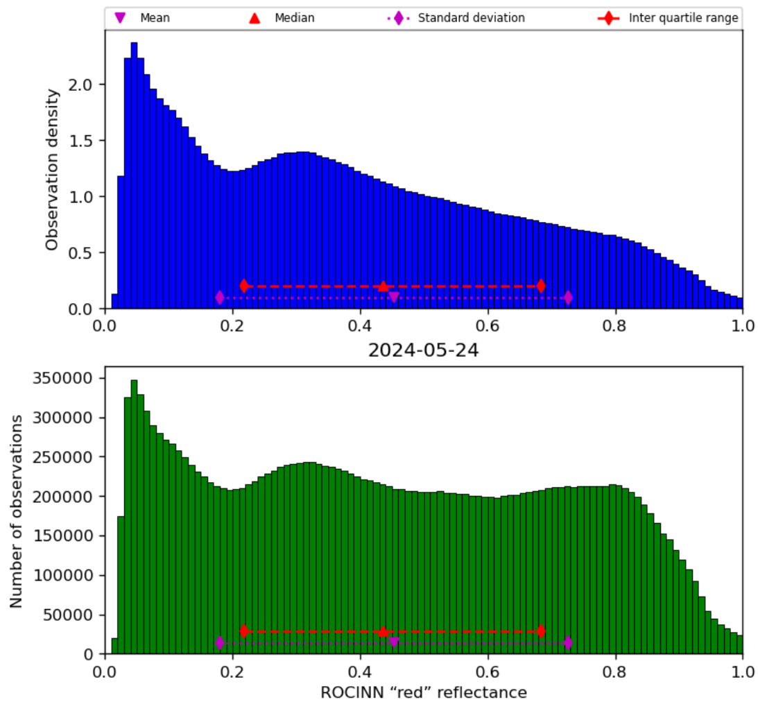
Figure 53: Histogram of “ROCINN “red” reflectance” for 2024-05-23 to 2024-05-25
