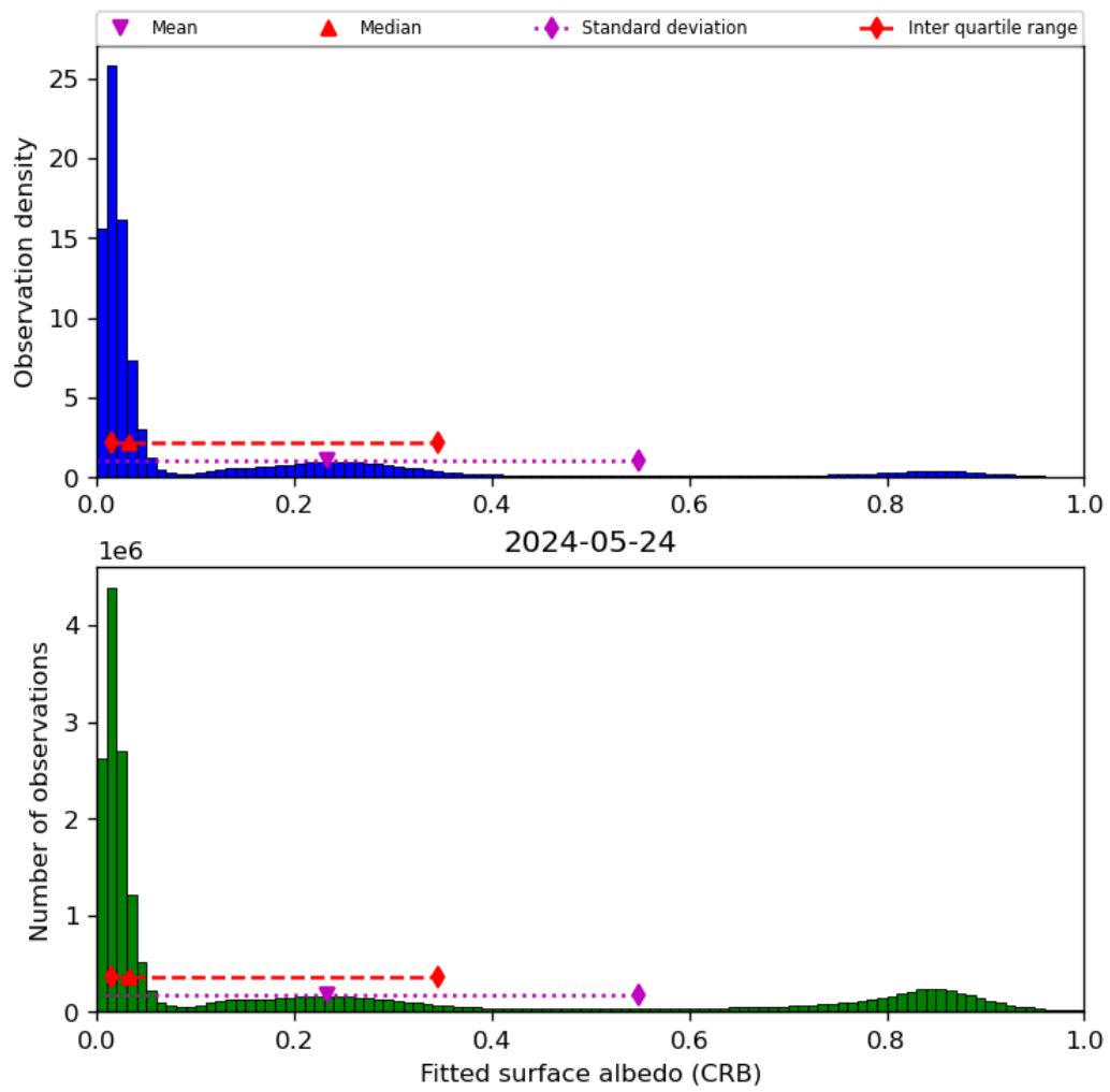
Figure 46: Histogram of “Fitted surface albedo (CRB)” for 2024-05-23 to 2024-05-25
