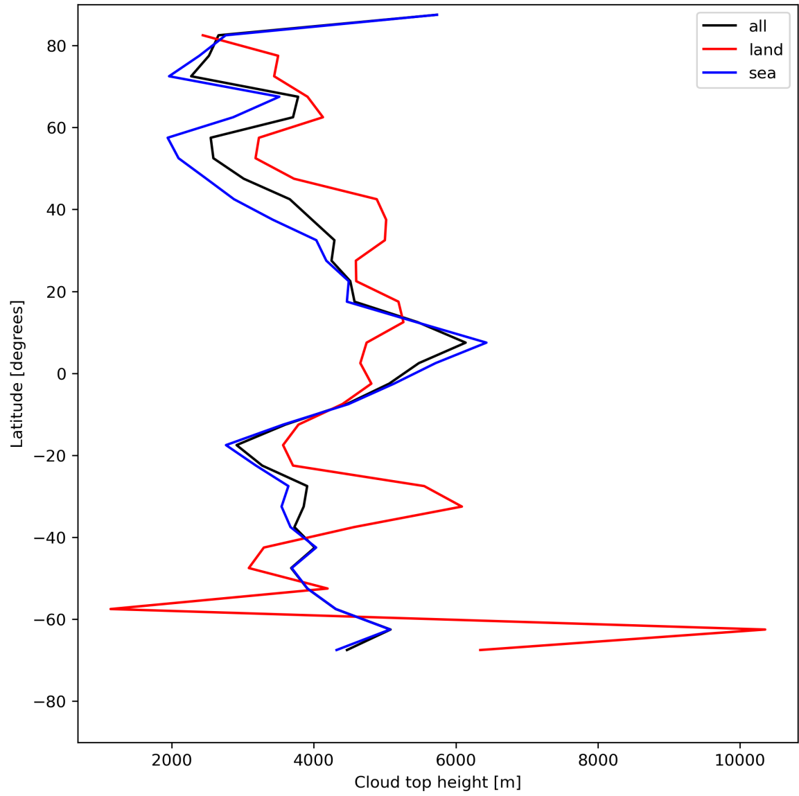
Figure 24: Zonal average of “Cloud top height” for 2024-05-23 to 2024-05-25.
