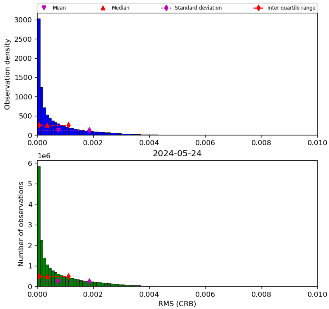
Figure 48: Histogram of “RMS (CRB)” for 2024-05-23 to 2024-05-25
