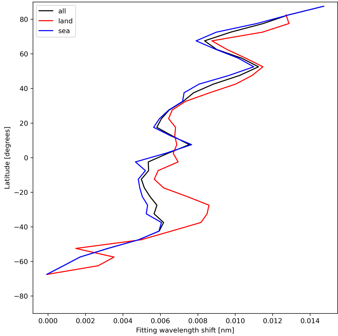
Figure 33: Zonal average of “Fitting wavelength shift” for 2024-05-23 to 2024-05-25.
