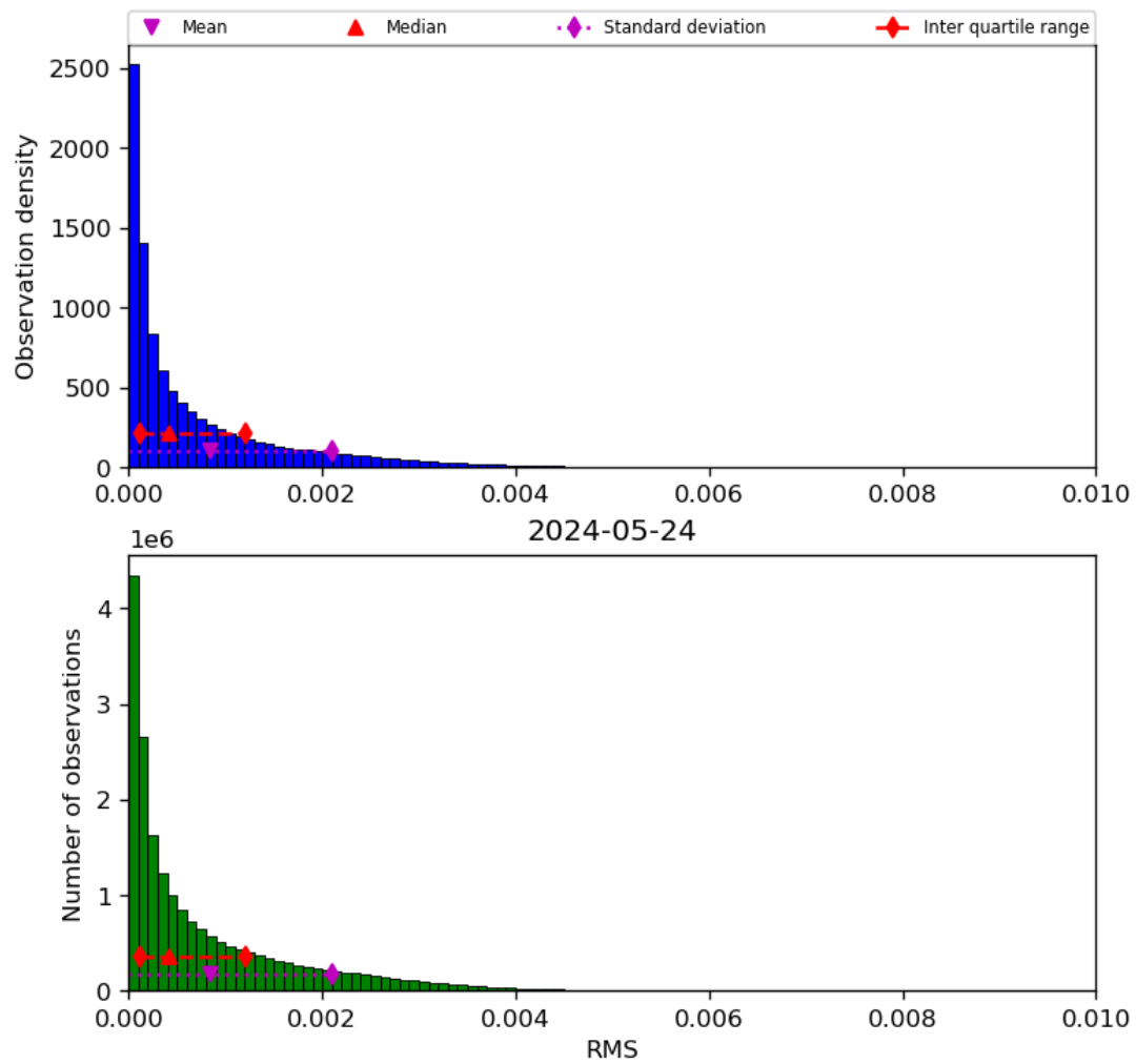
Figure 47: Histogram of “RMS” for 2024-05-23 to 2024-05-25
