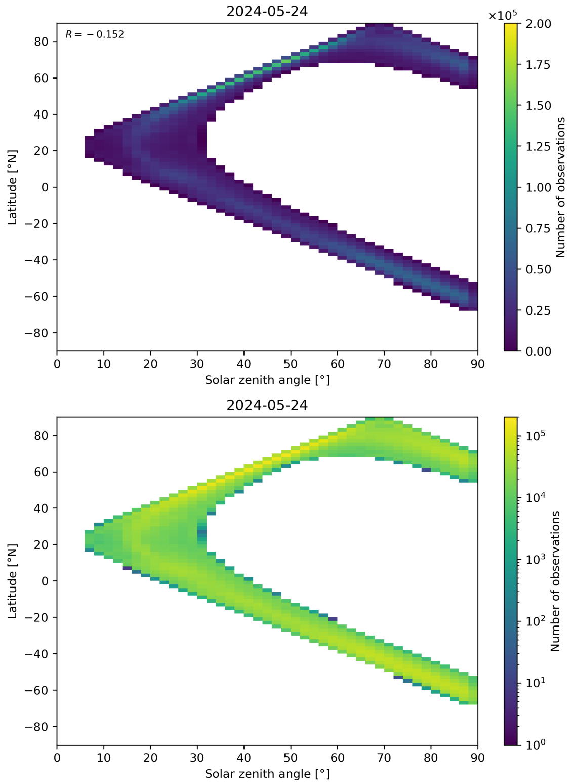
Figure 105: Scatter density plot of “Solar zenith angle” against “Latitude” for 2024-05-23 to 2024-05-25.
