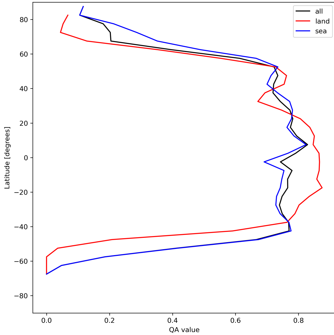
Figure 22: Zonal average of “QA value” for 2024-05-23 to 2024-05-25.
