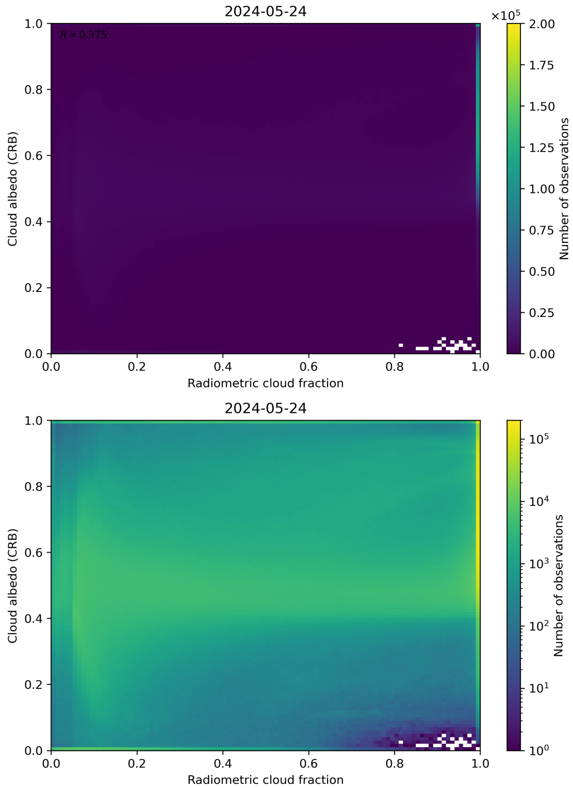
Figure 71: Scatter density plot of “Radiometric cloud fraction” against “Cloud albedo (CRB)” for 2024-05-23 to 2024-05-25.
