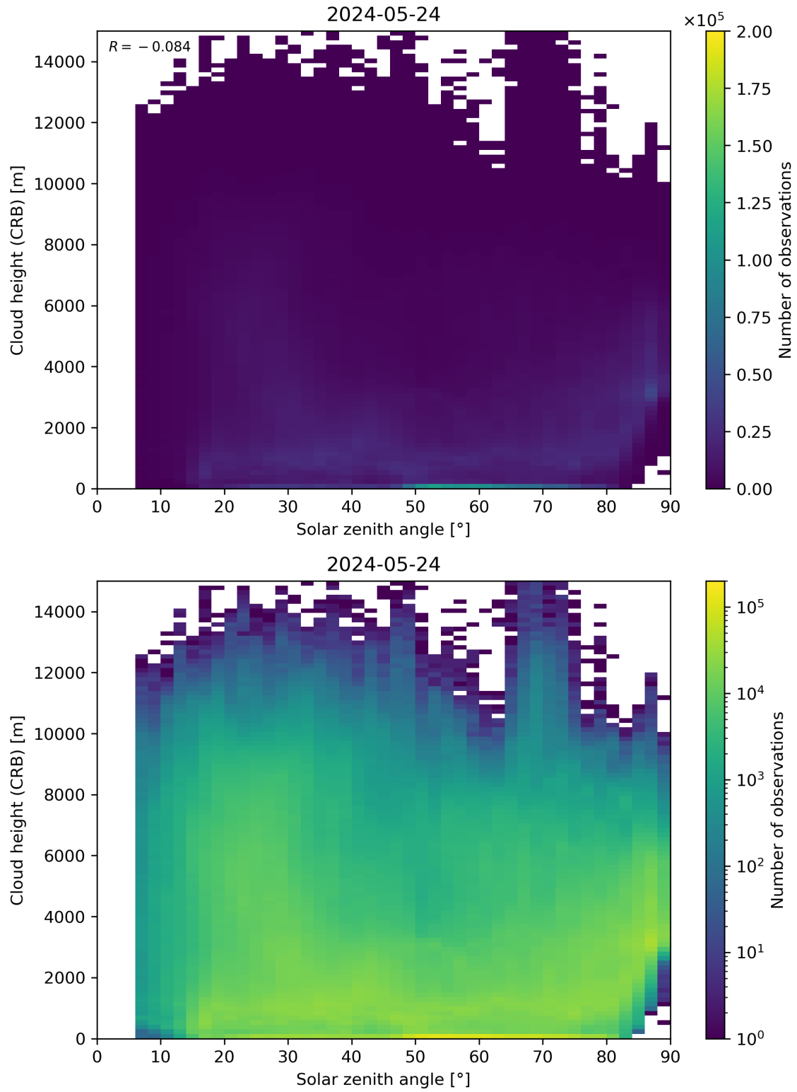
Figure 102: Scatter density plot of “Solar zenith angle” against “Cloud height (CRB)” for 2024-05-23 to 2024-05-25.
