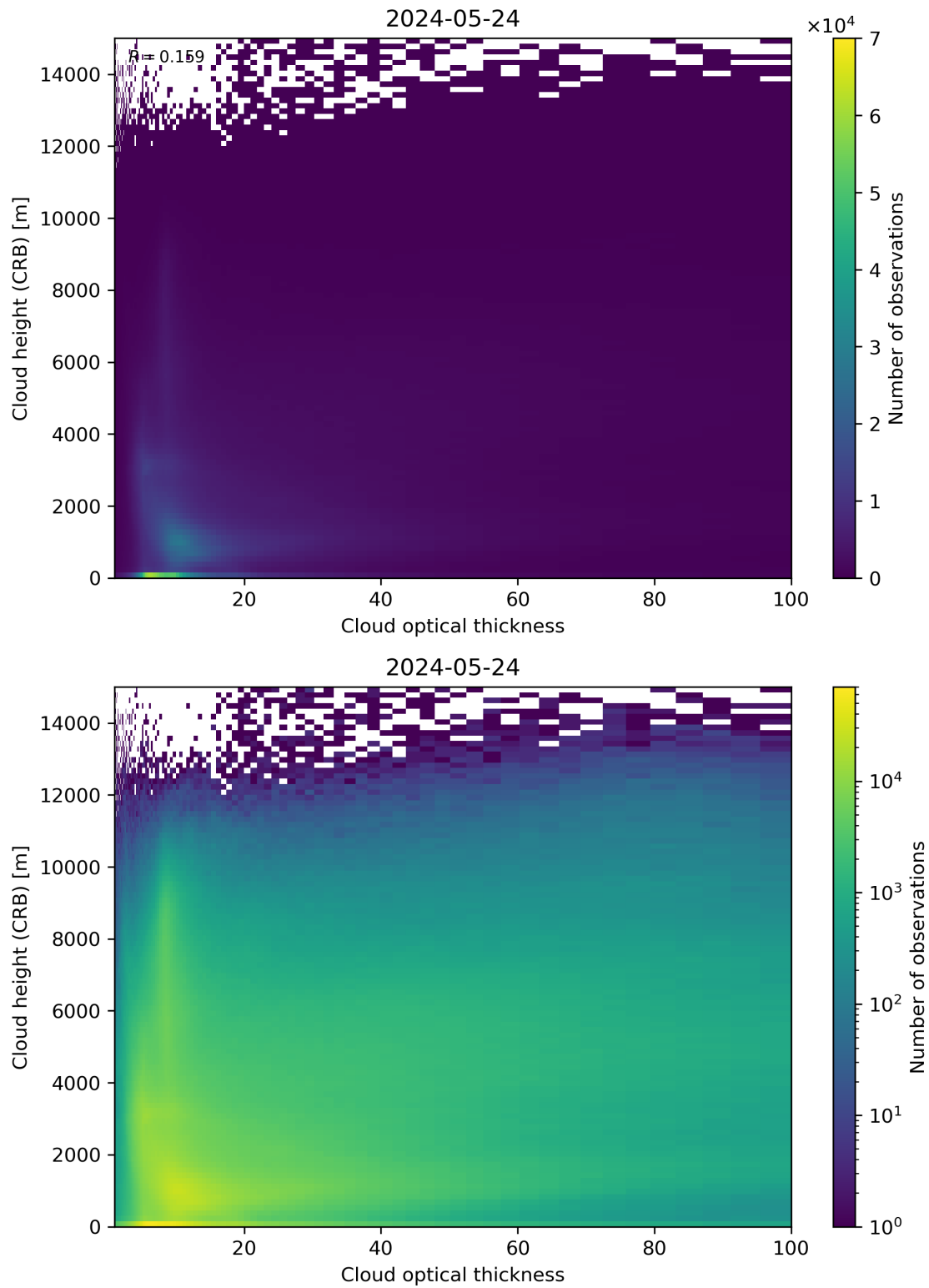
Figure 85: Scatter density plot of “Cloud optical thickness” against “Cloud height (CRB)” for 2024-05-23 to 2024-05-25.
