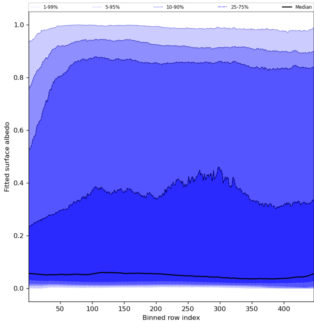
Figure 61: Along track statistics of “Fitted surface albedo” for 2024-05-23 to 2024-05-25
