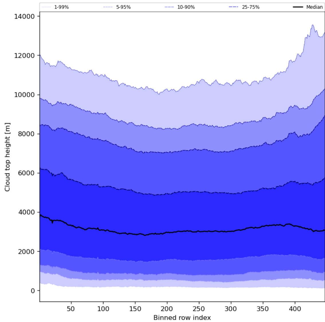
Figure 56: Along track statistics of “Cloud top height” for 2024-05-23 to 2024-05-25
