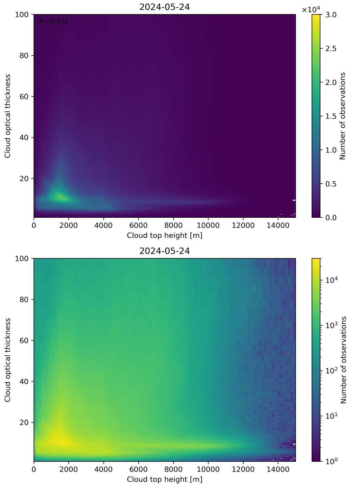
Figure 90: Scatter density plot of “Cloud top height” against “Cloud optical thickness” for 2024-05-23 to 2024-05-25.
