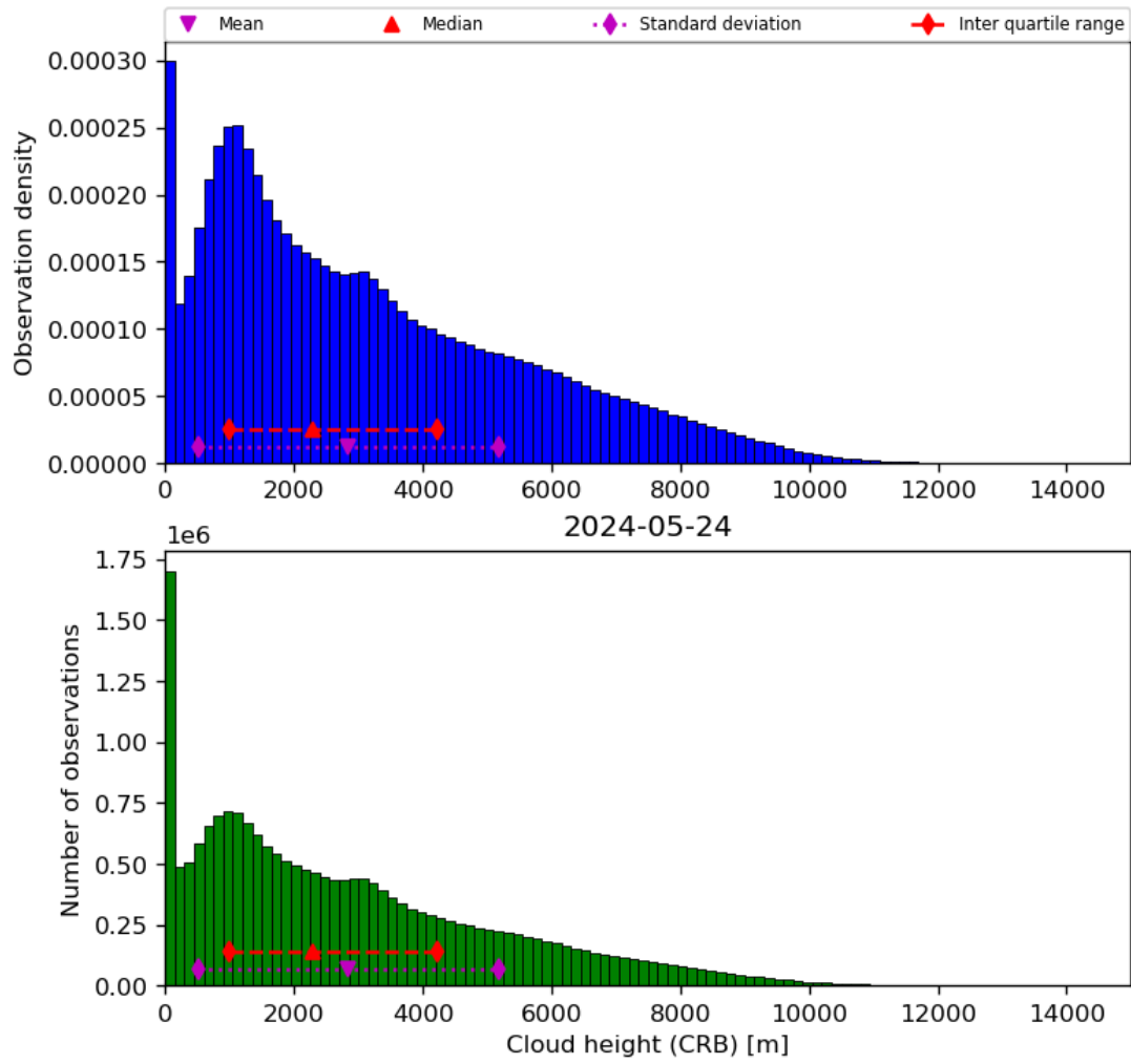
Figure 43: Histogram of “Cloud height (CRB)” for 2024-05-23 to 2024-05-25
