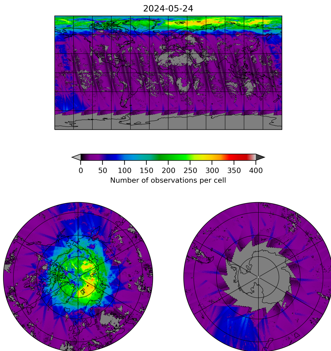
Figure 21: Map of the number of observations for 2024-05-23 to 2024-05-25
