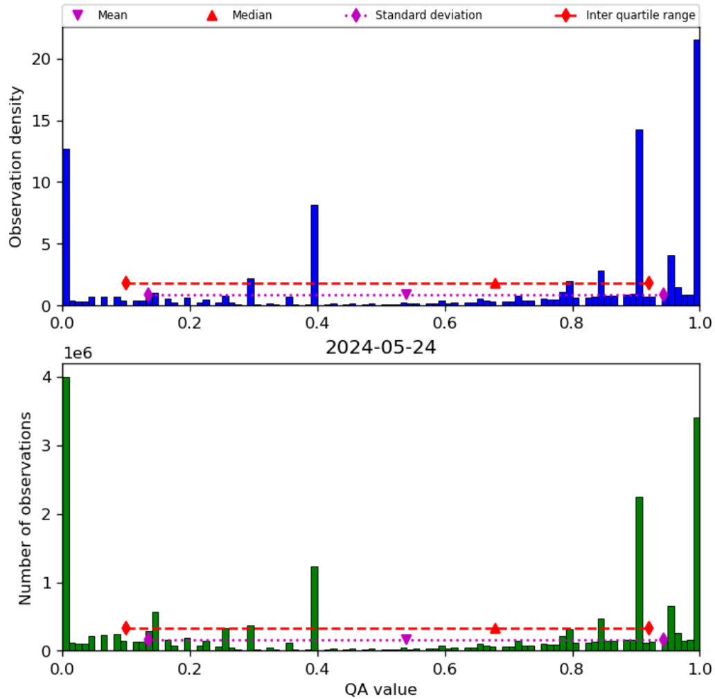
Figure 38: Histogram of “QA value” for 2024-05-23 to 2024-05-25
