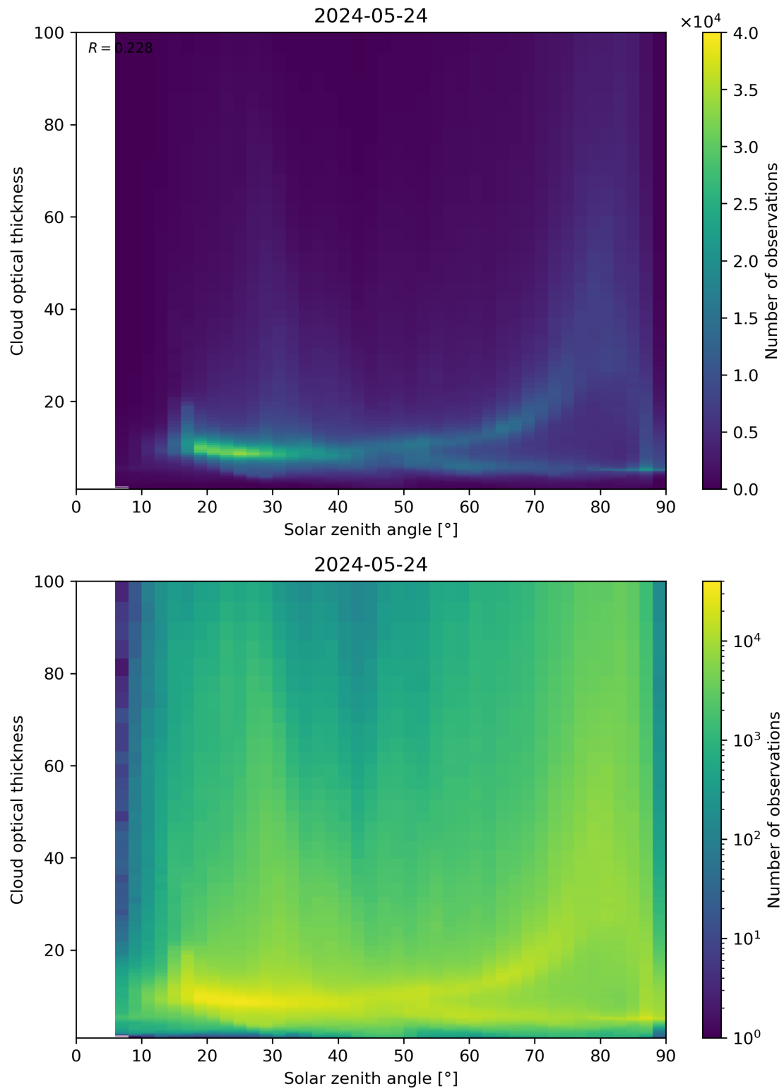
Figure 103: Scatter density plot of “Solar zenith angle” against “Cloud optical thickness” for 2024-05-23 to 2024-05-25.
