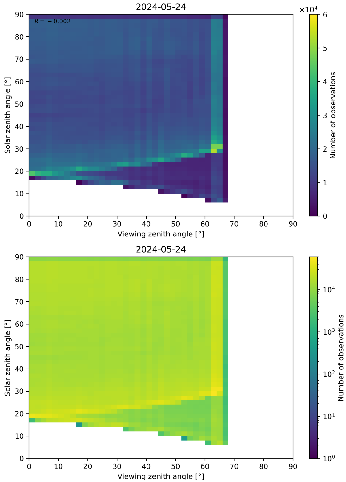
Figure 114: Scatter density plot of “Viewing zenith angle” against “Solar zenith angle” for 2024-05-23 to 2024-05-25.
