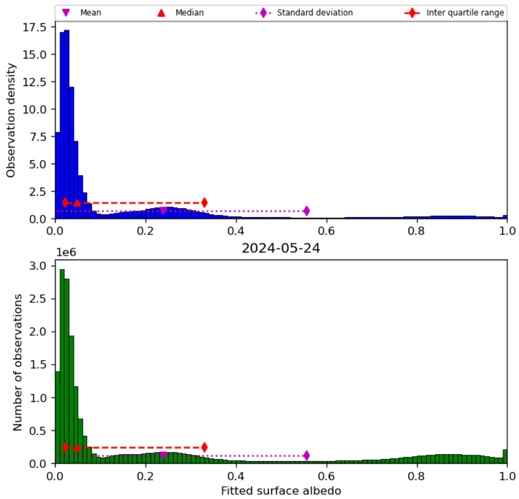
Figure 45: Histogram of “Fitted surface albedo” for 2024-05-23 to 2024-05-25
