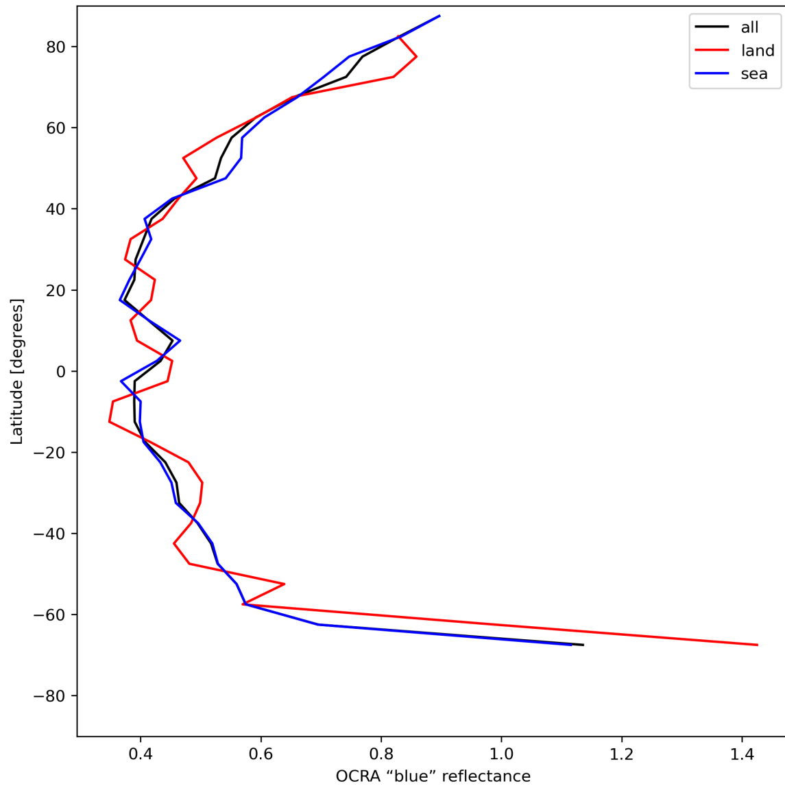
Figure 35: Zonal average of “OCRA “blue” reflectance” for 2024-05-23 to 2024-05-25.
