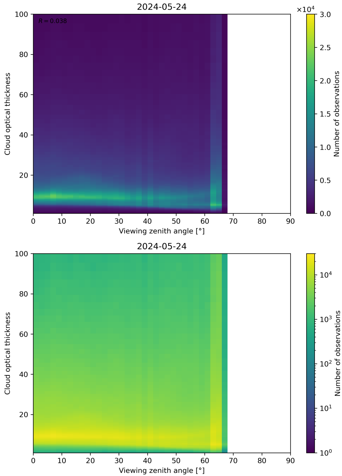
Figure 111: Scatter density plot of “Viewing zenith angle” against “Cloud optical thickness” for 2024-05-23 to 2024-05-25.
