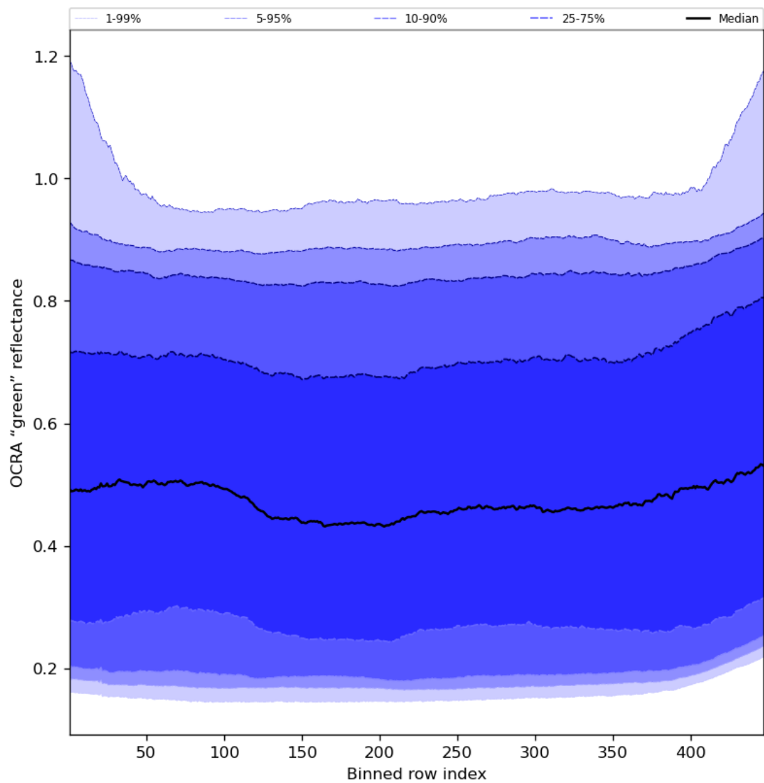
Figure 68: Along track statistics of “OCRA “green” reflectance” for 2024-05-23 to 2024-05-25
