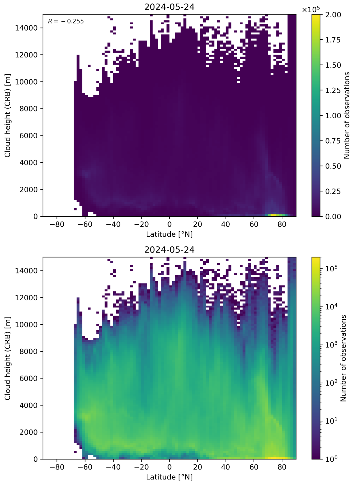
Figure 95: Scatter density plot of “Latitude” against “Cloud height (CRB)” for 2024-05-23 to 2024-05-25.
