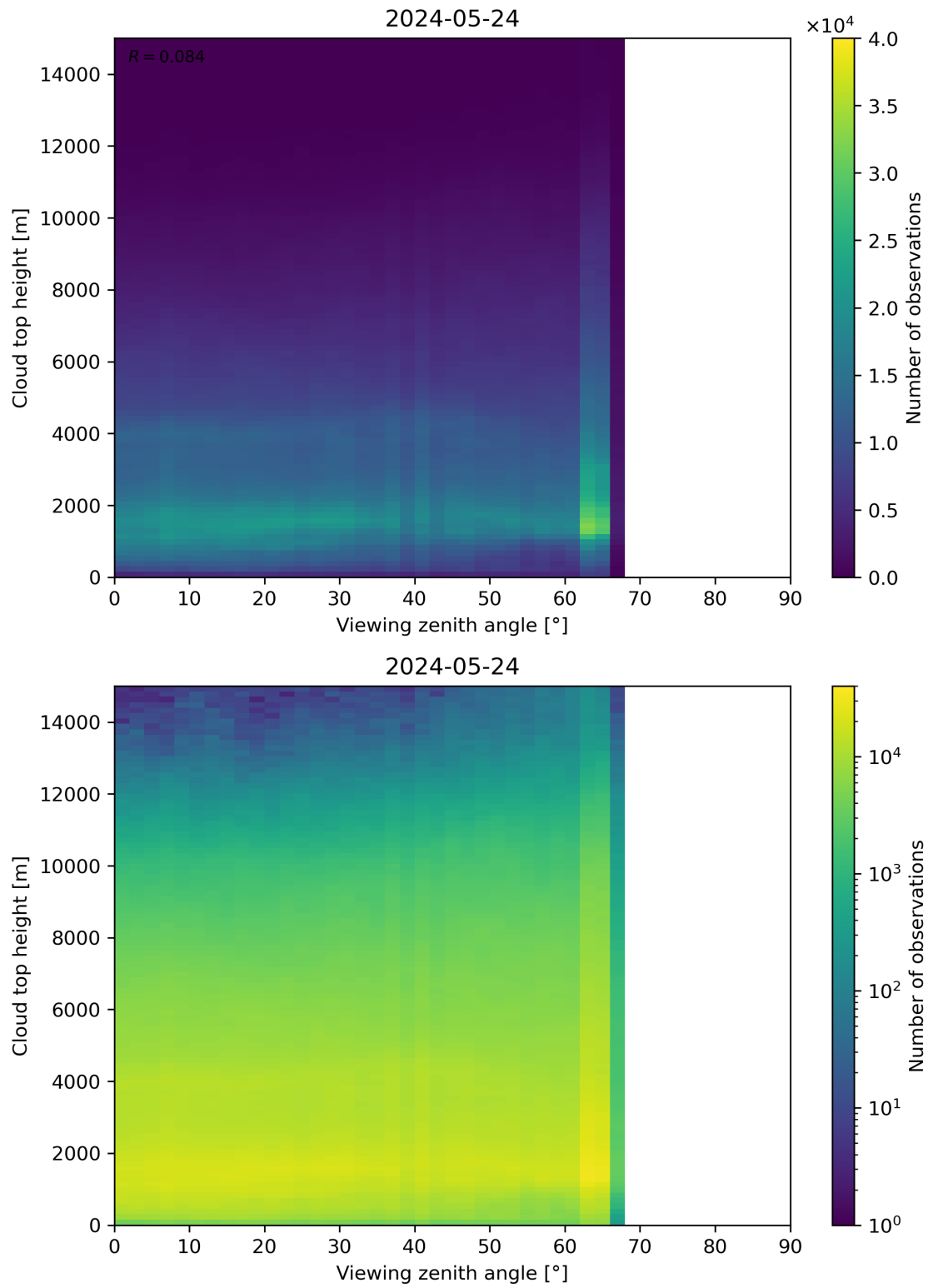
Figure 112: Scatter density plot of “Viewing zenith angle” against “Cloud top height” for 2024-05-23 to 2024-05-25.
