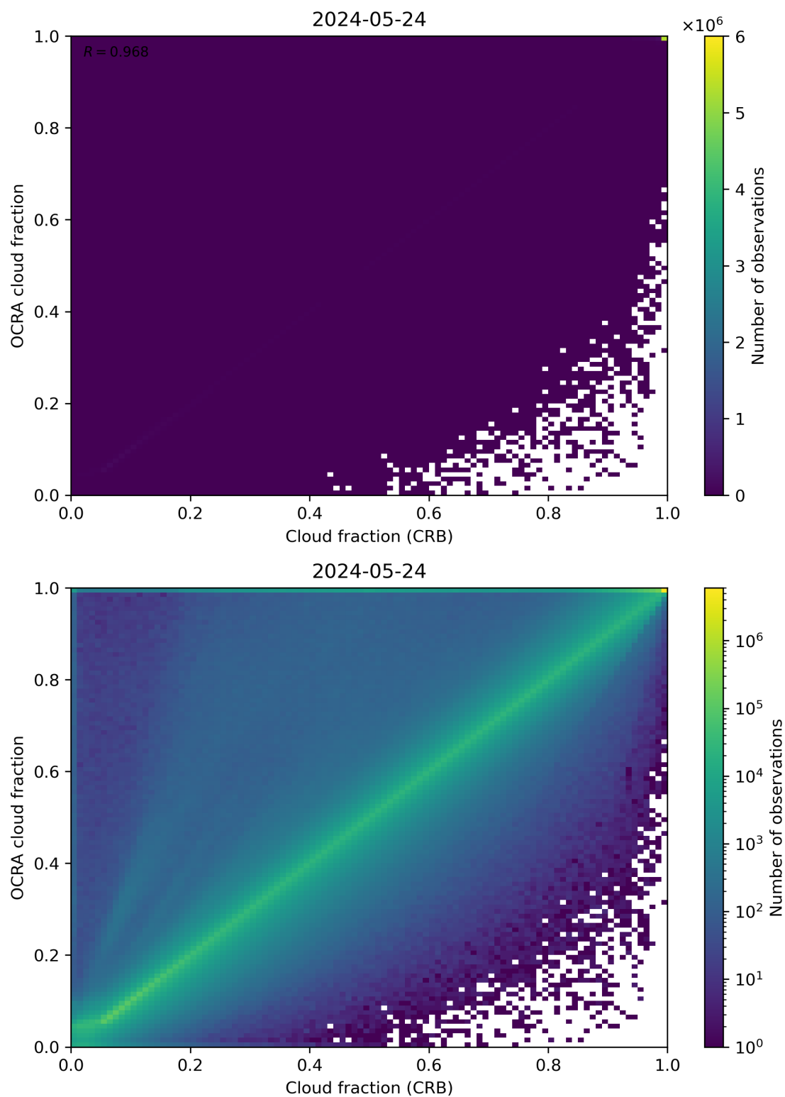
Figure 78: Scatter density plot of “Cloud fraction (CRB)” against “OCRA cloud fraction” for 2024-05-23 to 2024-05-25.
