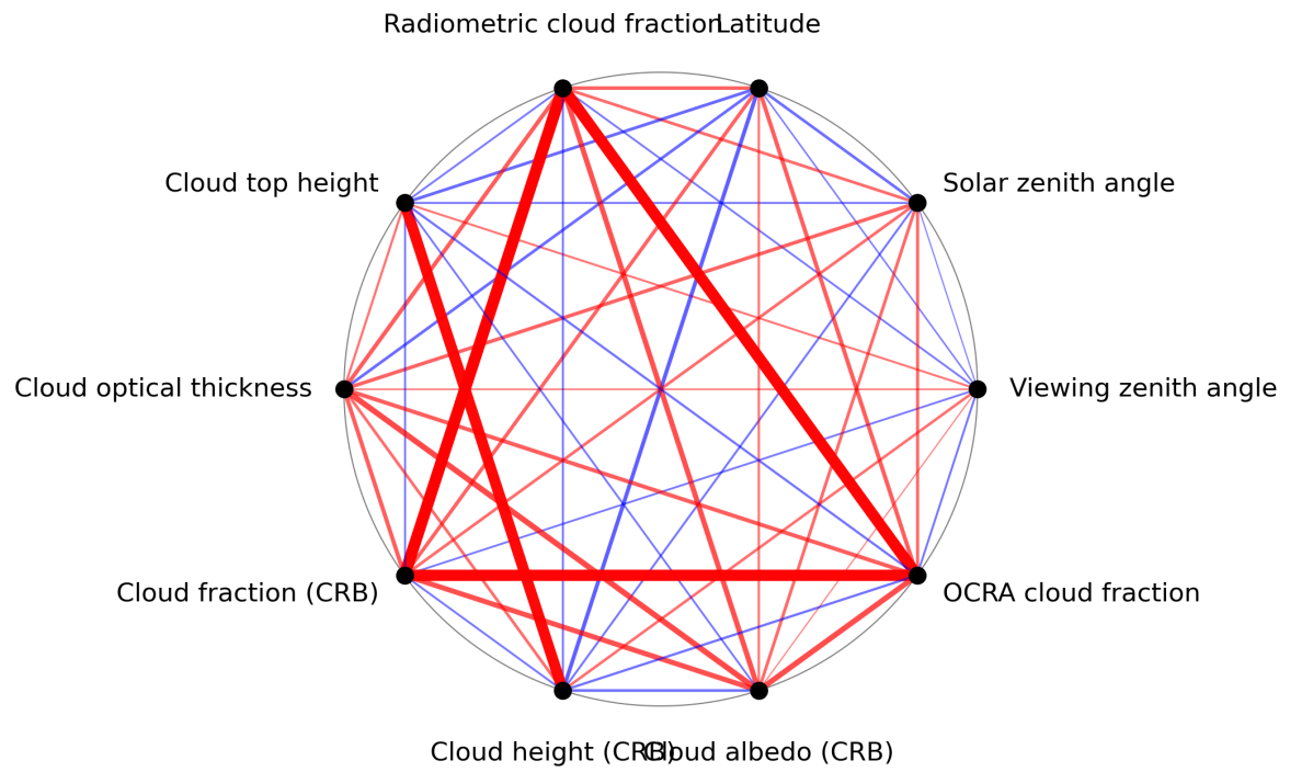
Figure 1: Map of correlation graph for 2024-05-23 to 2024-05-25.
