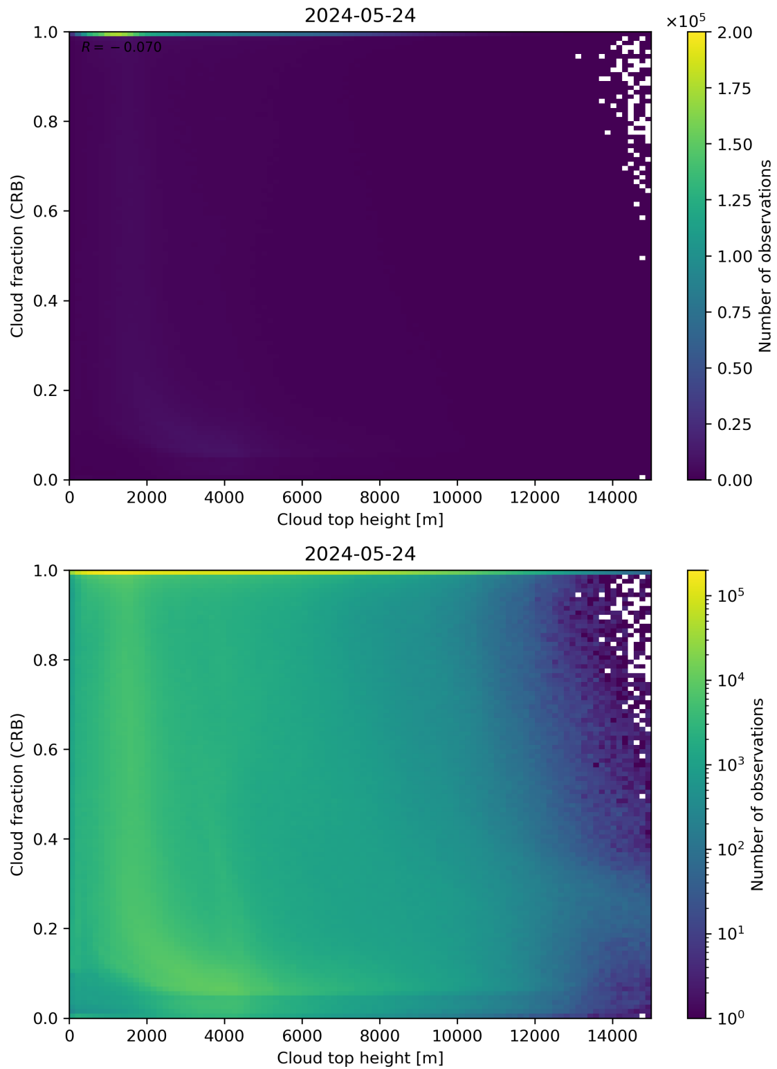
Figure 88: Scatter density plot of “Cloud top height” against “Cloud fraction (CRB)” for 2024-05-23 to 2024-05-25.
