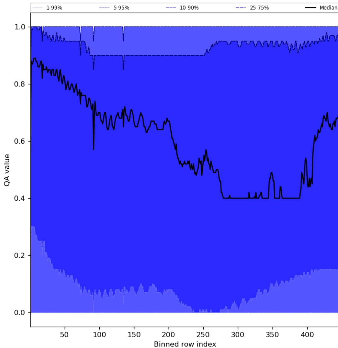
Figure 54: Along track statistics of “QA value” for 2024-05-23 to 2024-05-25
