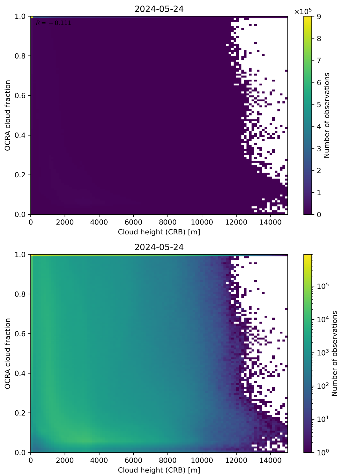
Figure 81: Scatter density plot of “Cloud height (CRB)” against “OCRA cloud fraction” for 2024-05-23 to 2024-05-25.
