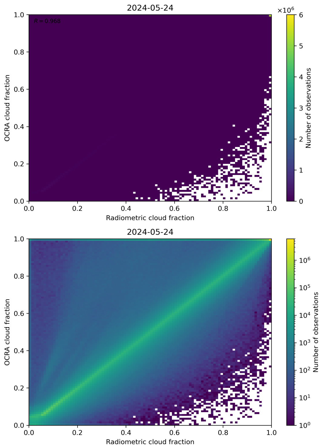
Figure 72: Scatter density plot of “Radiometric cloud fraction” against “OCRA cloud fraction” for 2024-05-23 to 2024-05-25.
