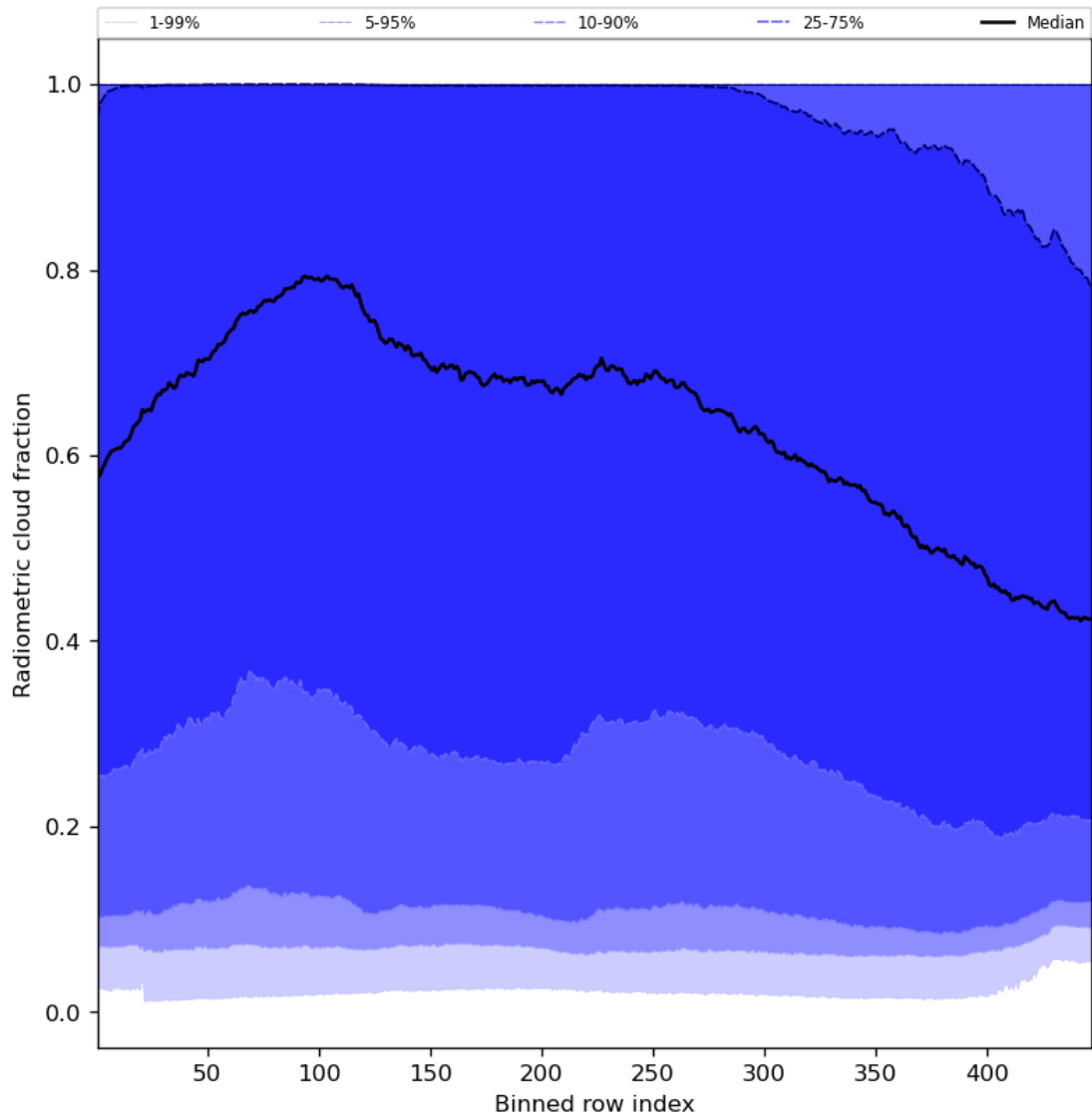
Figure 55: Along track statistics of “Radiometric cloud fraction” for 2024-05-23 to 2024-05-25
