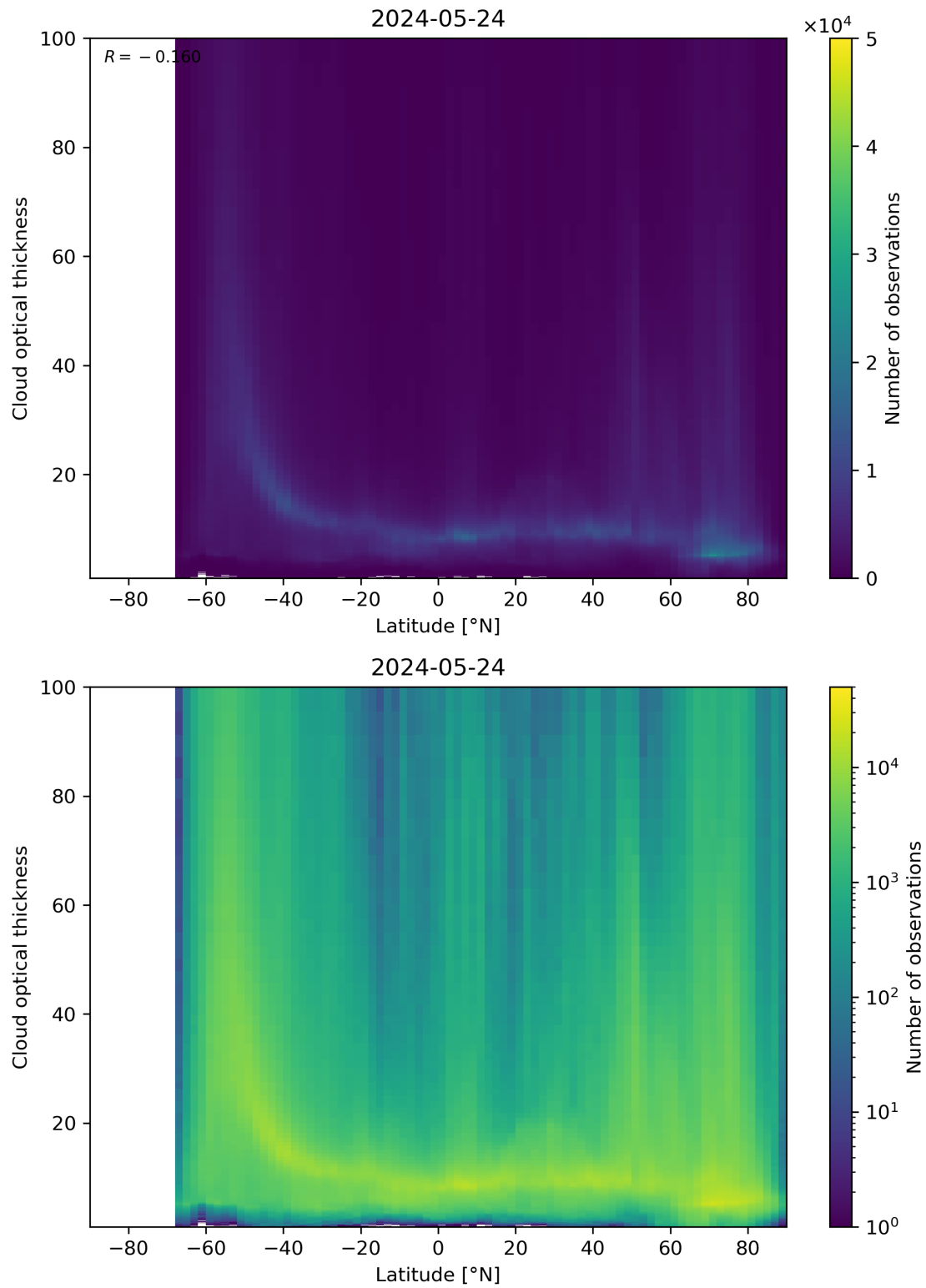
Figure 96: Scatter density plot of “Latitude” against “Cloud optical thickness” for 2024-05-23 to 2024-05-25.
