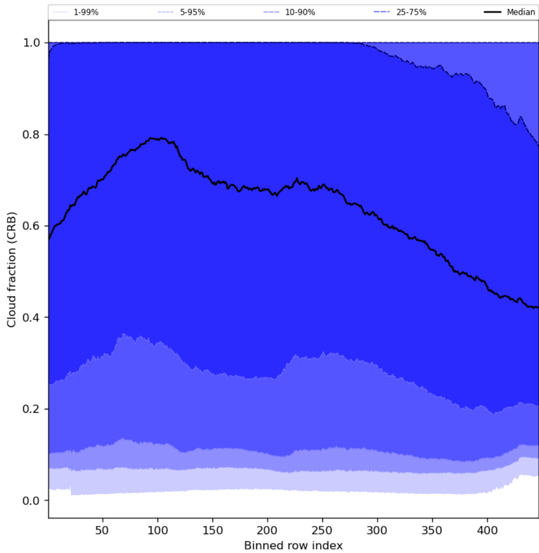
Figure 58: Along track statistics of “Cloud fraction (CRB)” for 2024-05-23 to 2024-05-25
