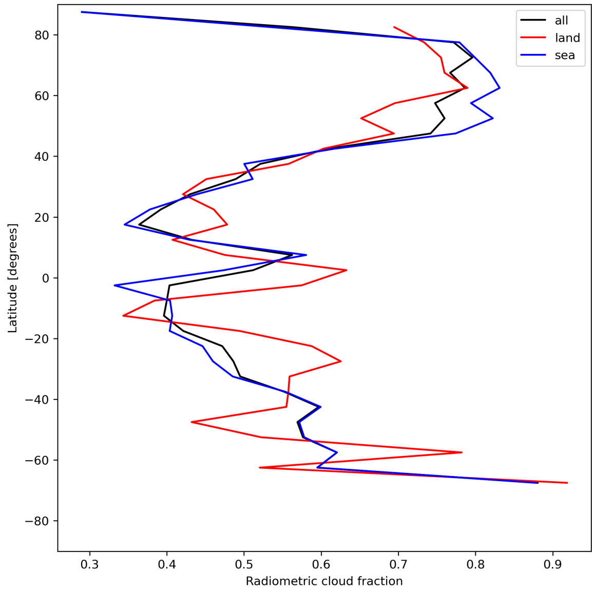
Figure 23: Zonal average of “Radiometric cloud fraction” for 2024-05-23 to 2024-05-25.
