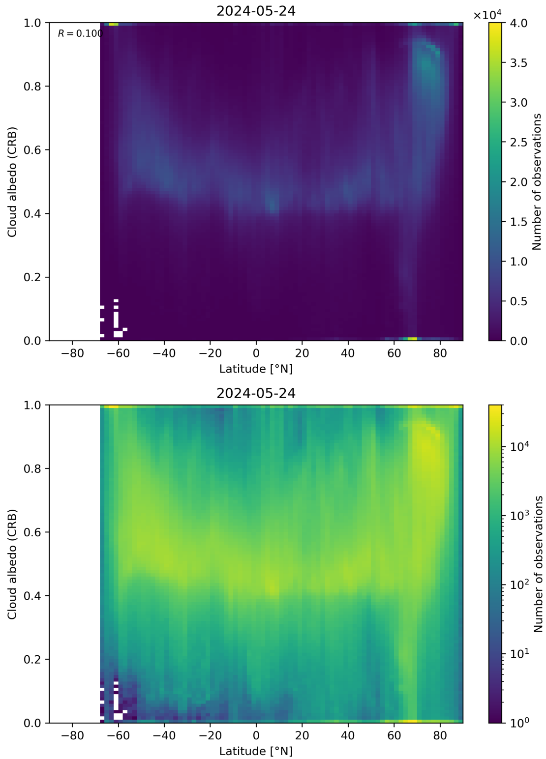
Figure 91: Scatter density plot of “Latitude” against “Cloud albedo (CRB)” for 2024-05-23 to 2024-05-25.
