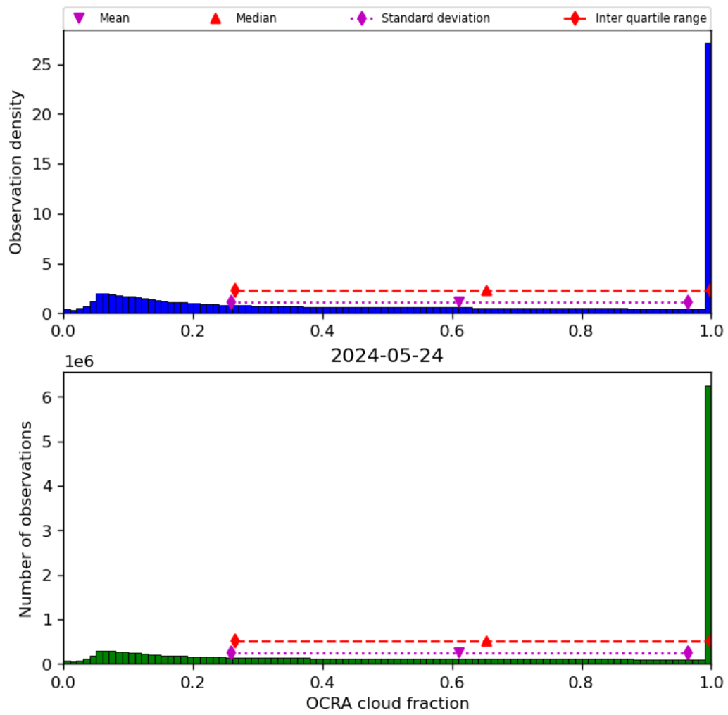
Figure 50: Histogram of “OCRA cloud fraction” for 2024-05-23 to 2024-05-25
