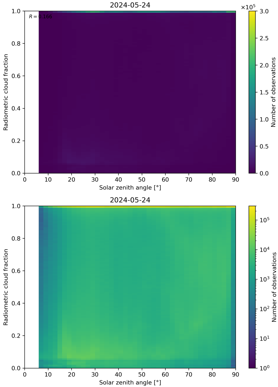
Figure 99: Scatter density plot of “Solar zenith angle” against “Radiometric cloud fraction” for 2024-05-23 to 2024-05-25.
