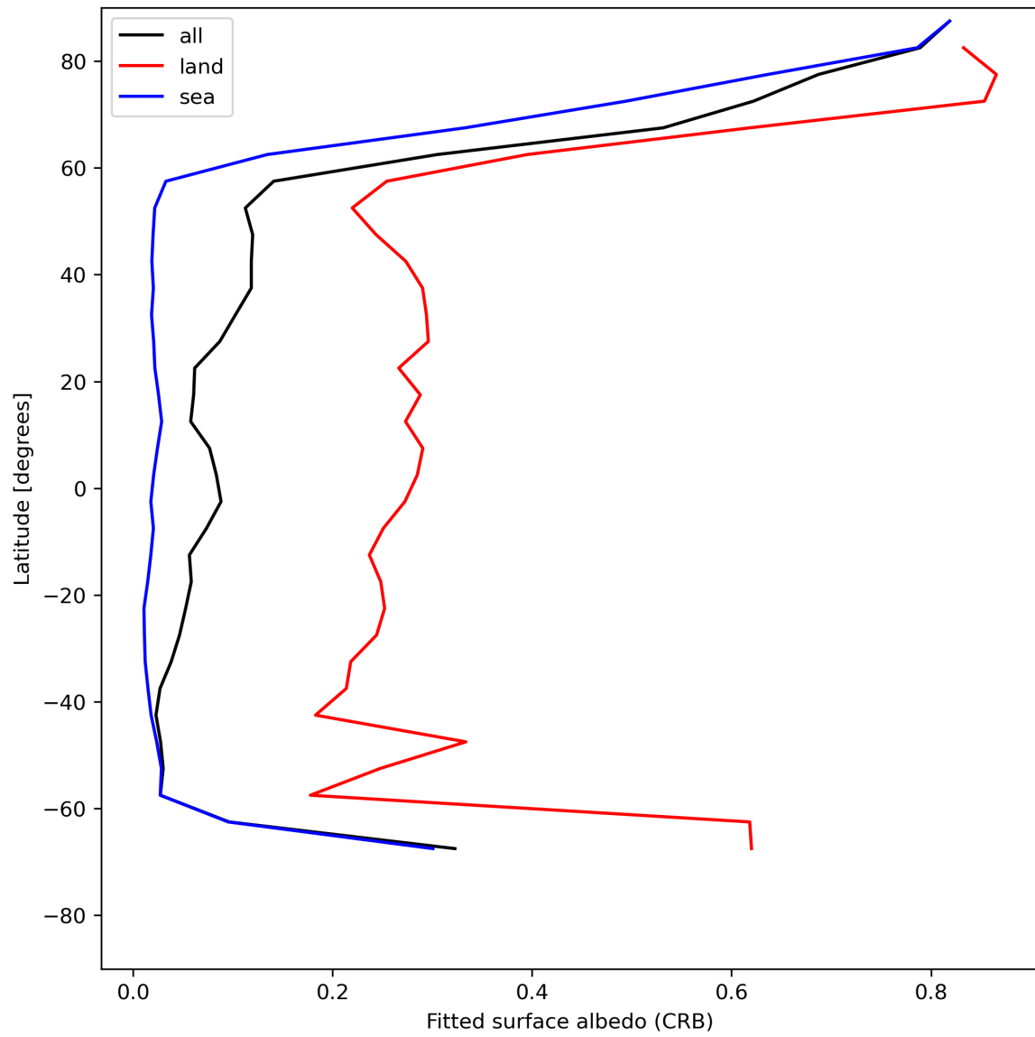
Figure 30: Zonal average of “Fitted surface albedo (CRB)” for 2024-05-23 to 2024-05-25.
