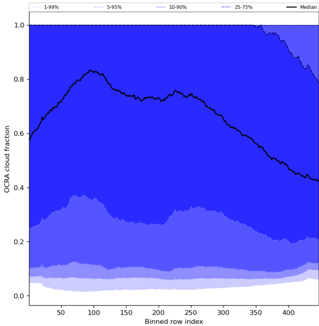
Figure 66: Along track statistics of “OCRA cloud fraction” for 2024-05-23 to 2024-05-25
