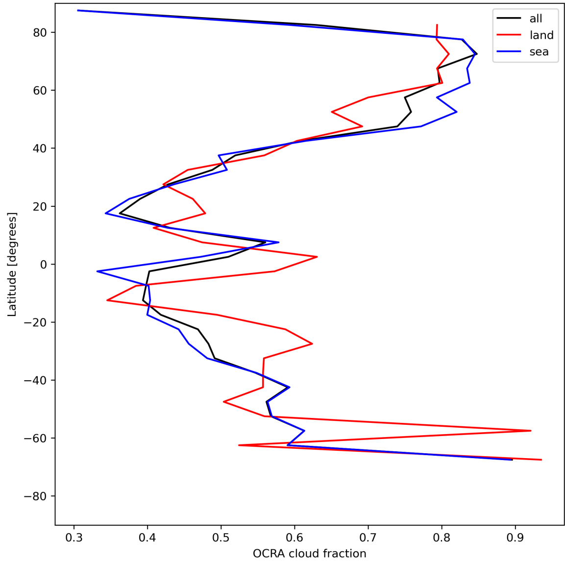
Figure 34: Zonal average of “OCRA cloud fraction” for 2024-05-23 to 2024-05-25.
