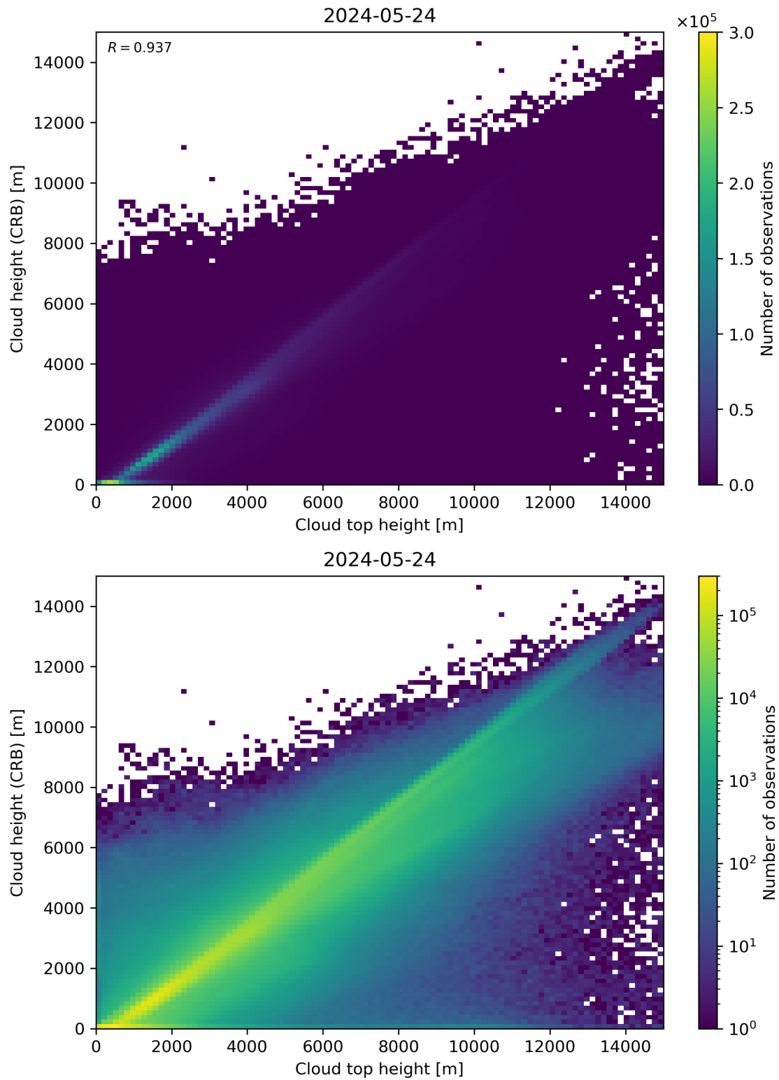
Figure 89: Scatter density plot of “Cloud top height” against “Cloud height (CRB)” for 2024-05-23 to 2024-05-25.
