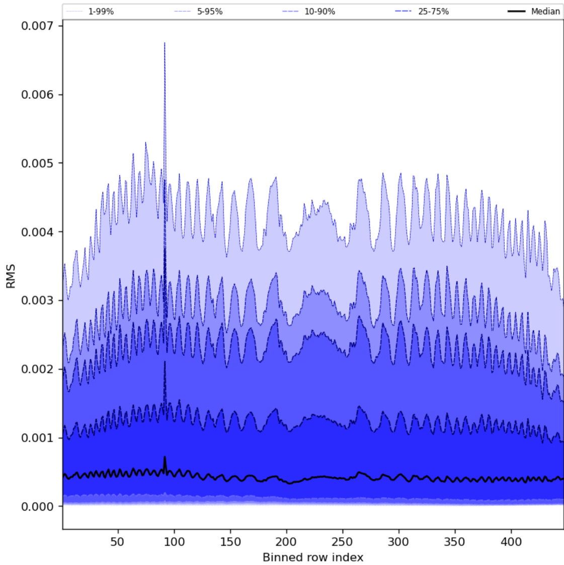
Figure 63: Along track statistics of “RMS” for 2024-05-23 to 2024-05-25
