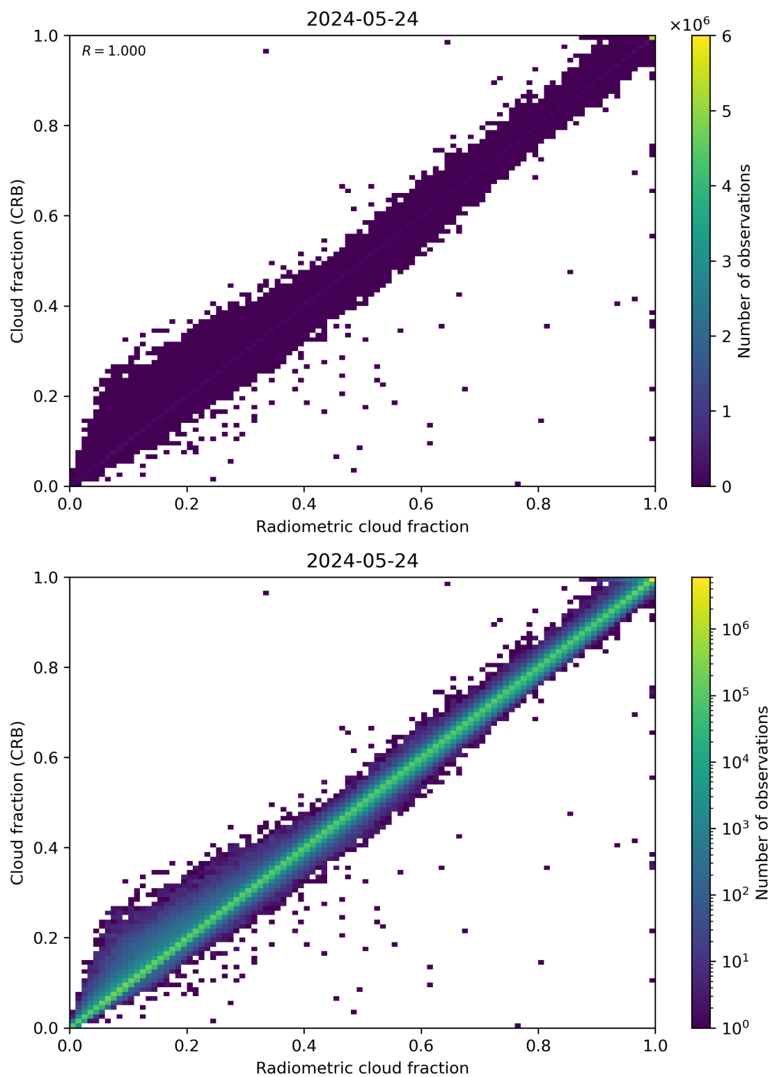
Figure 73: Scatter density plot of “Radiometric cloud fraction” against “Cloud fraction (CRB)” for 2024-05-23 to 2024-05-25.
