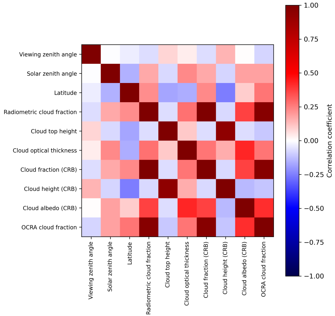
Figure 2: Map of correlation matrix for 2024-05-23 to 2024-05-25.
