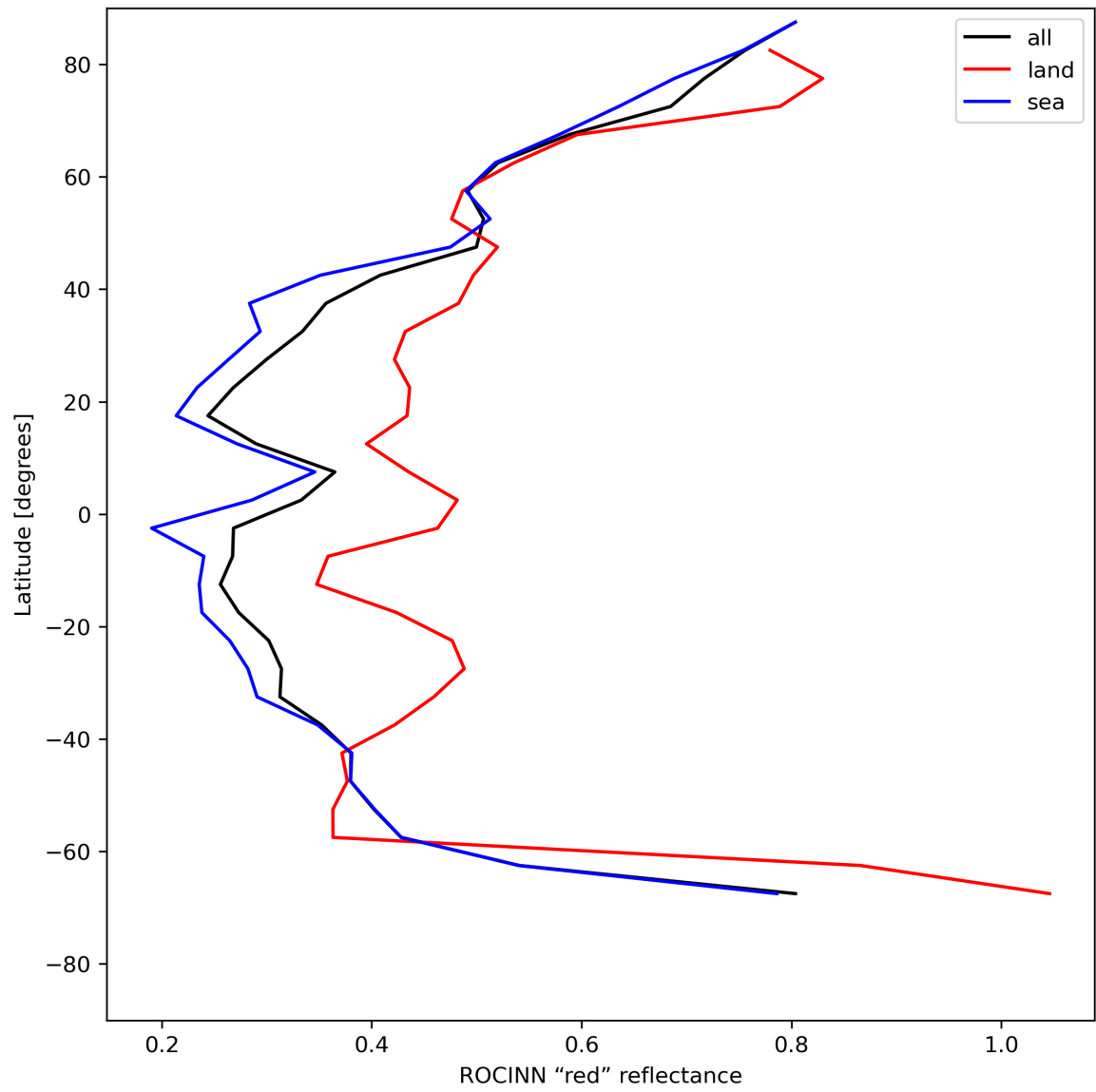
Figure 37: Zonal average of "ROCINN "red" reflectance" for 2024-05-23 to 2024-05-25.
