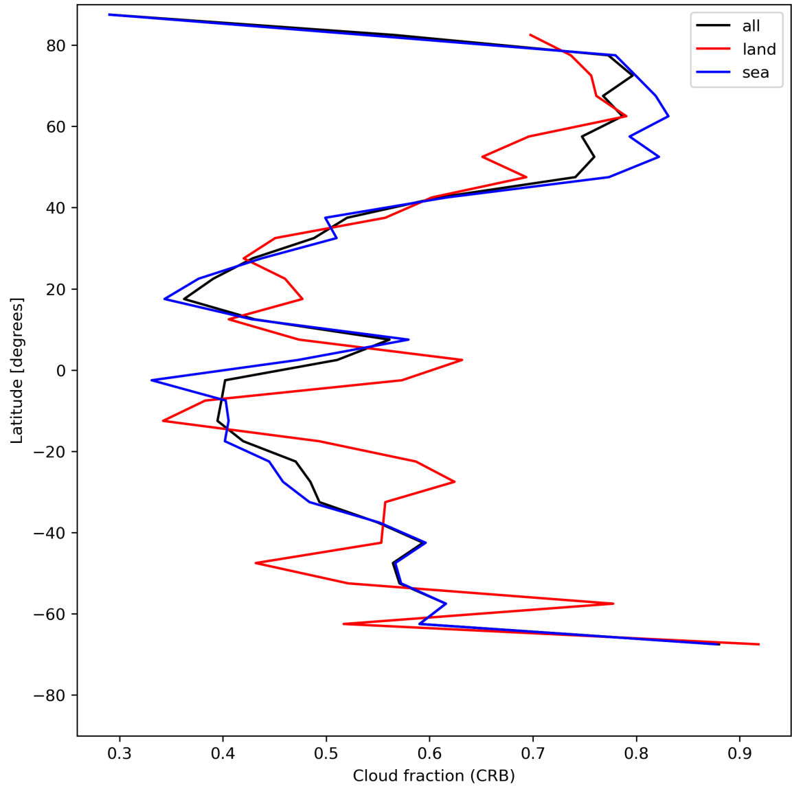
Figure 26: Zonal average of “Cloud fraction (CRB)” for 2024-05-23 to 2024-05-25.
