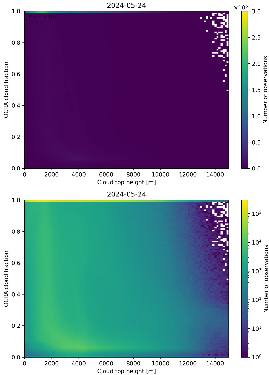
Figure 87: Scatter density plot of “Cloud top height” against “OCRA cloud fraction” for 2024-05-23 to 2024-05-25.
