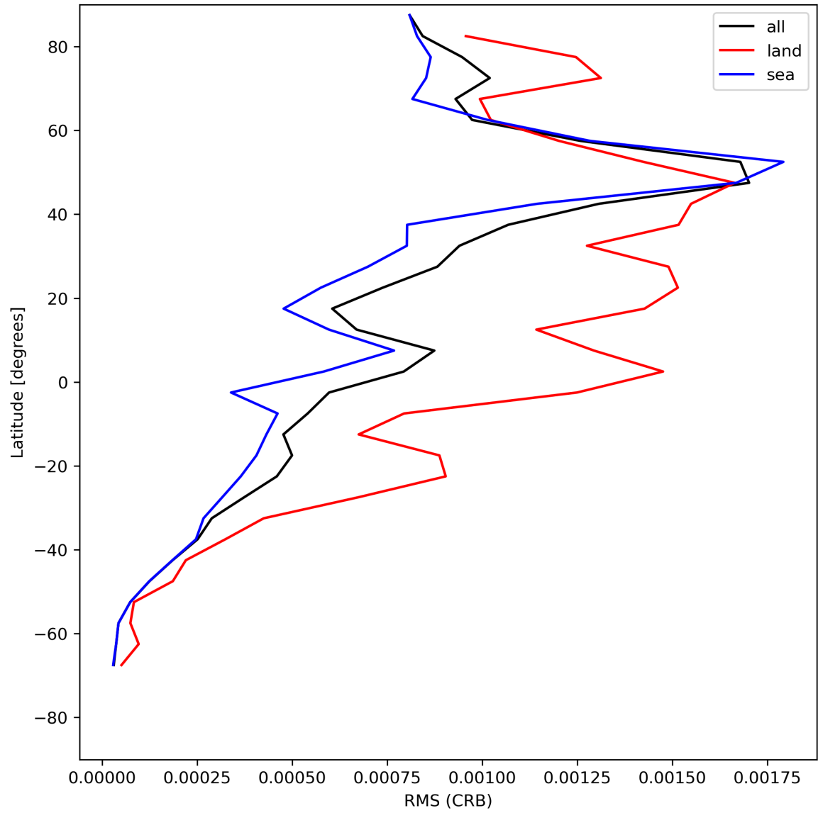
Figure 32: Zonal average of “RMS (CRB)” for 2024-05-23 to 2024-05-25.
