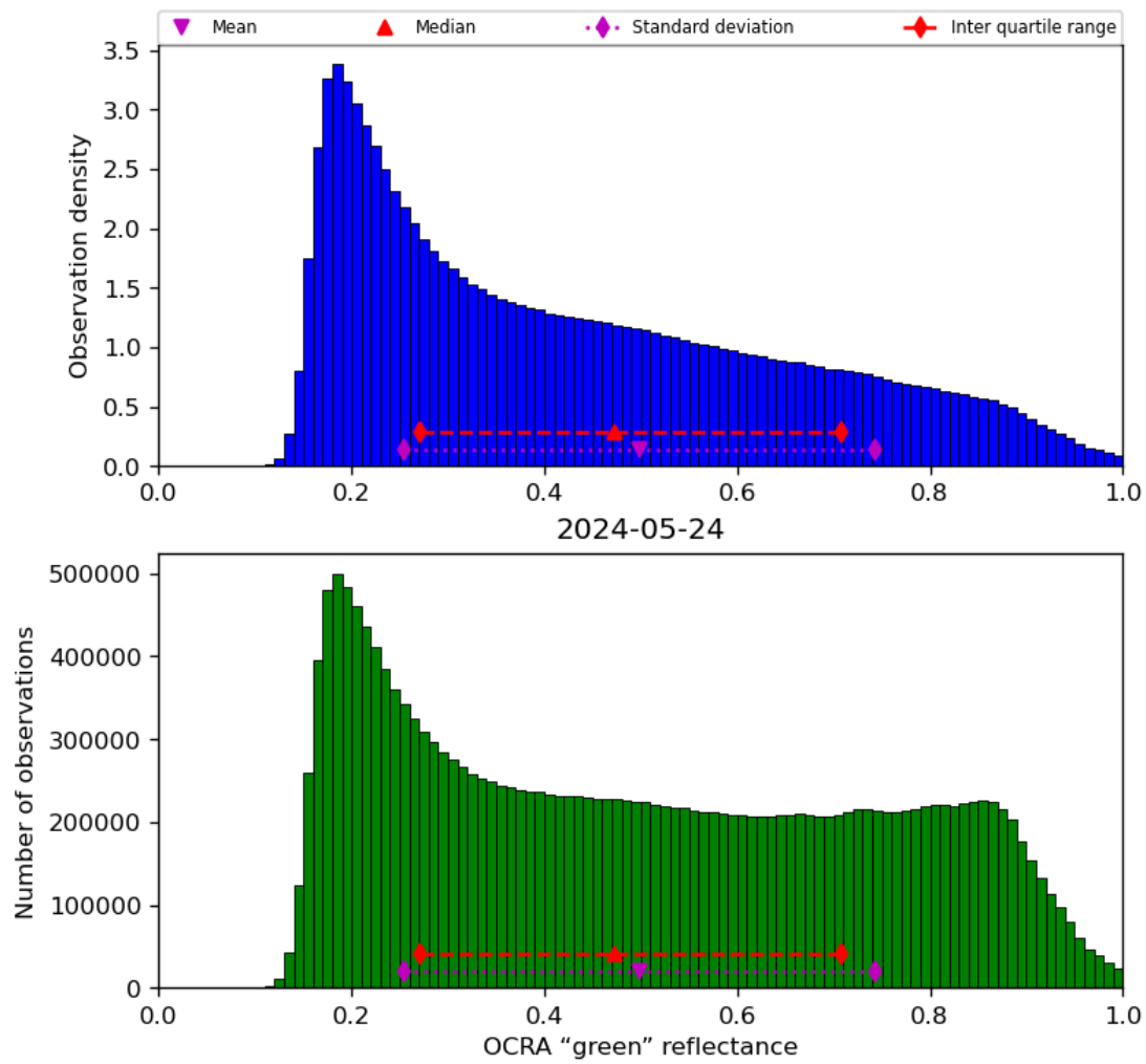
Figure 52: Histogram of “OCRA “green” reflectance” for 2024-05-23 to 2024-05-25
