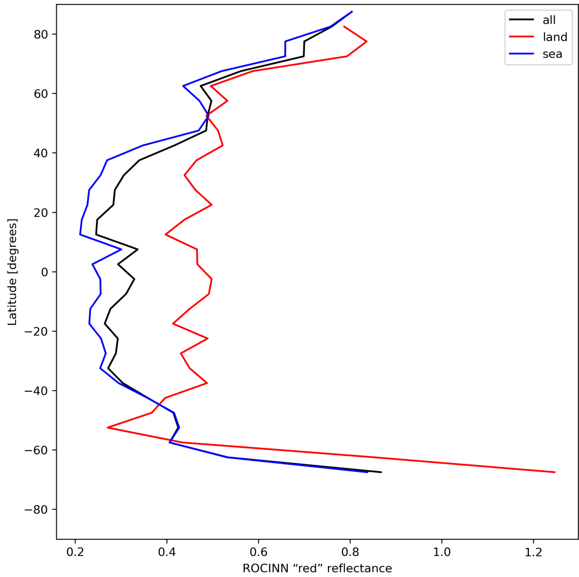
Figure 37: Zonal average of “ROCINN “red” reflectance” for 2024-05-25 to 2024-05-27.
