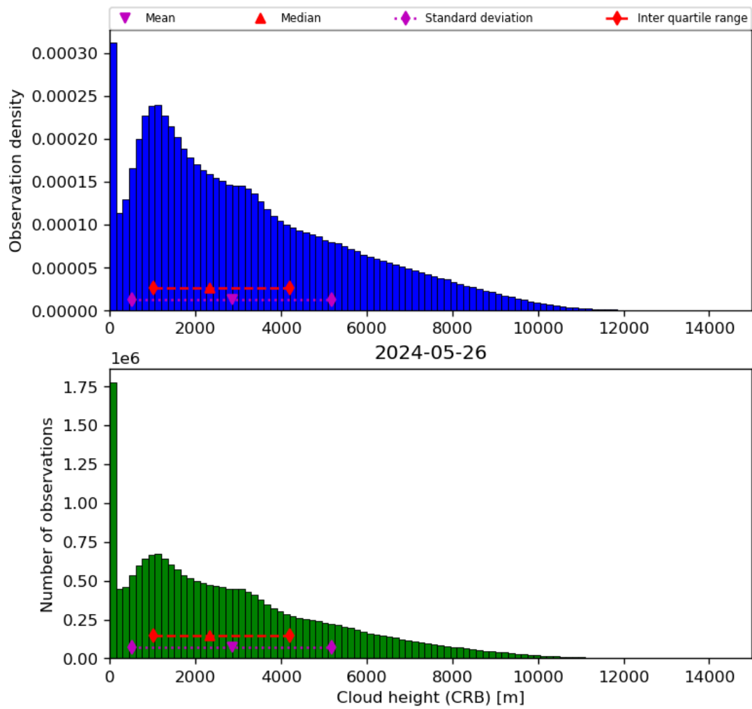
Figure 43: Histogram of “Cloud height (CRB)” for 2024-05-25 to 2024-05-27
