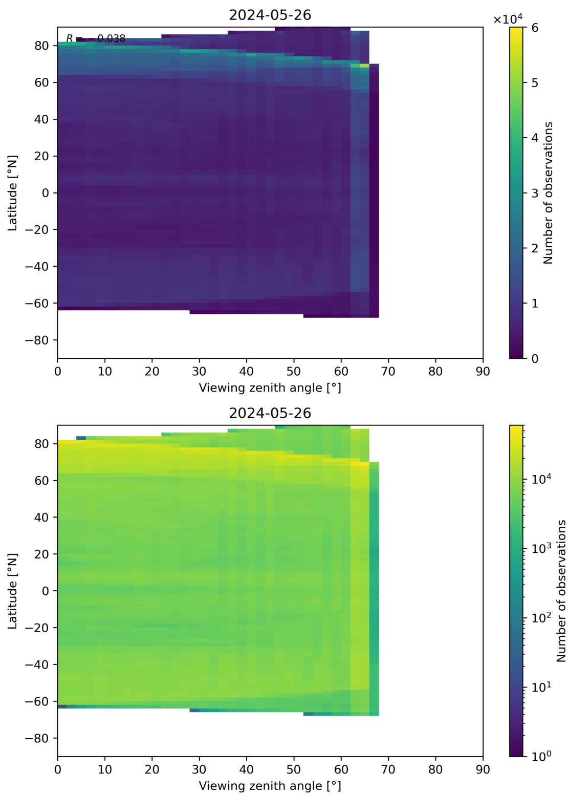
Figure 113: Scatter density plot of “Viewing zenith angle” against “Latitude” for 2024-05-25 to 2024-05-27.
