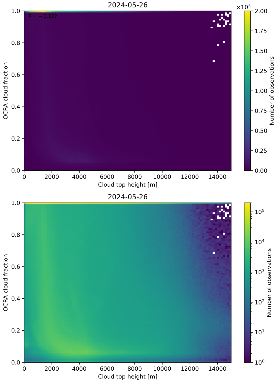
Figure 87: Scatter density plot of “Cloud top height” against “OCRA cloud fraction” for 2024-05-25 to 2024-05-27.
