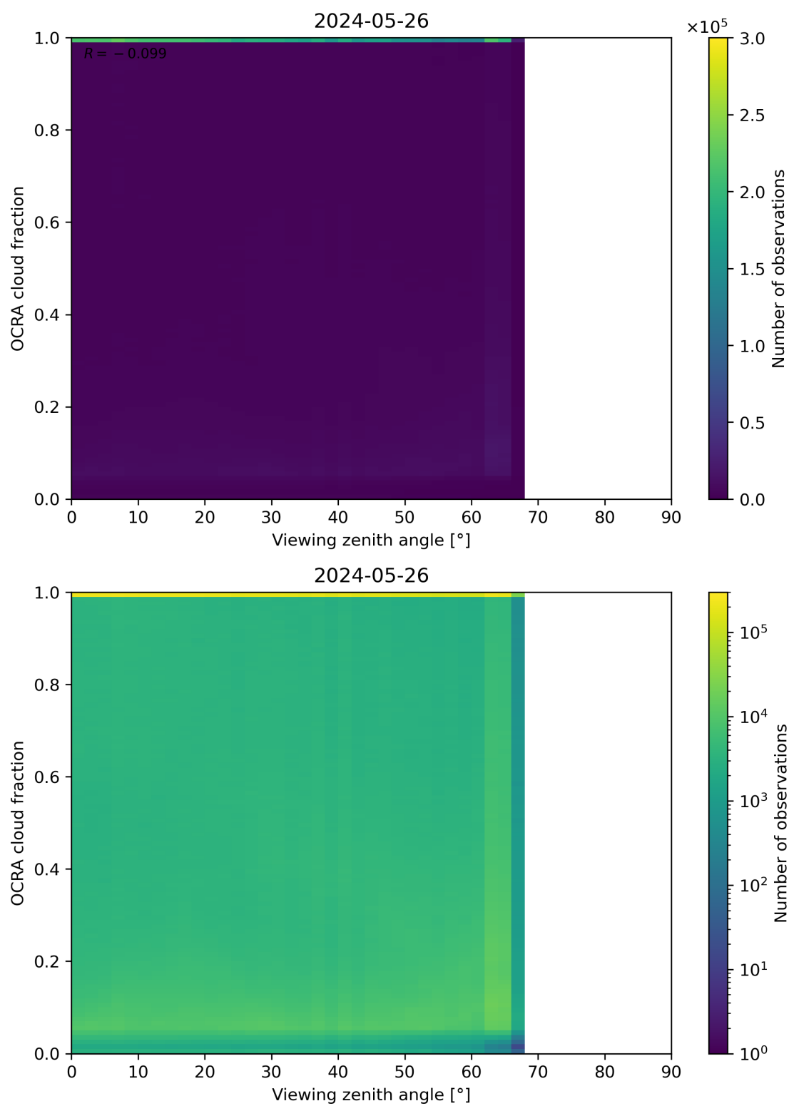
Figure 108: Scatter density plot of “Viewing zenith angle” against “OCRA cloud fraction” for 2024-05-25 to 2024-05-27.
