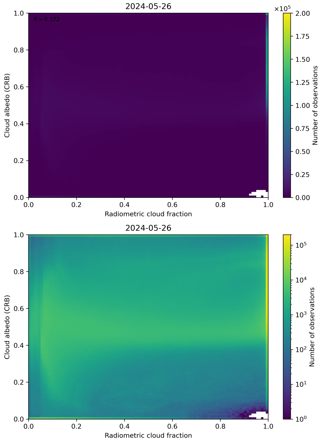
Figure 71: Scatter density plot of “Radiometric cloud fraction” against “Cloud albedo (CRB)” for 2024-05-25 to 2024-05-27.
