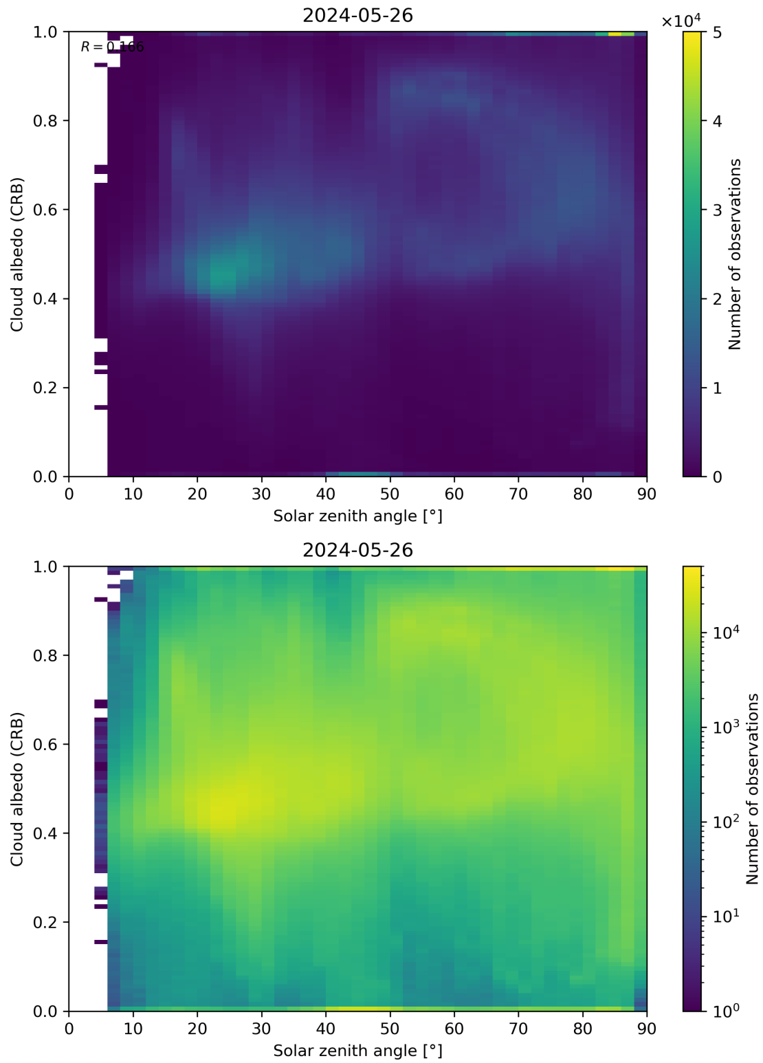
Figure 98: Scatter density plot of “Solar zenith angle” against “Cloud albedo (CRB)” for 2024-05-25 to 2024-05-27.
