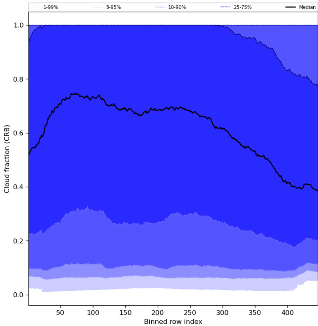
Figure 58: Along track statistics of “Cloud fraction (CRB)” for 2024-05-25 to 2024-05-27
