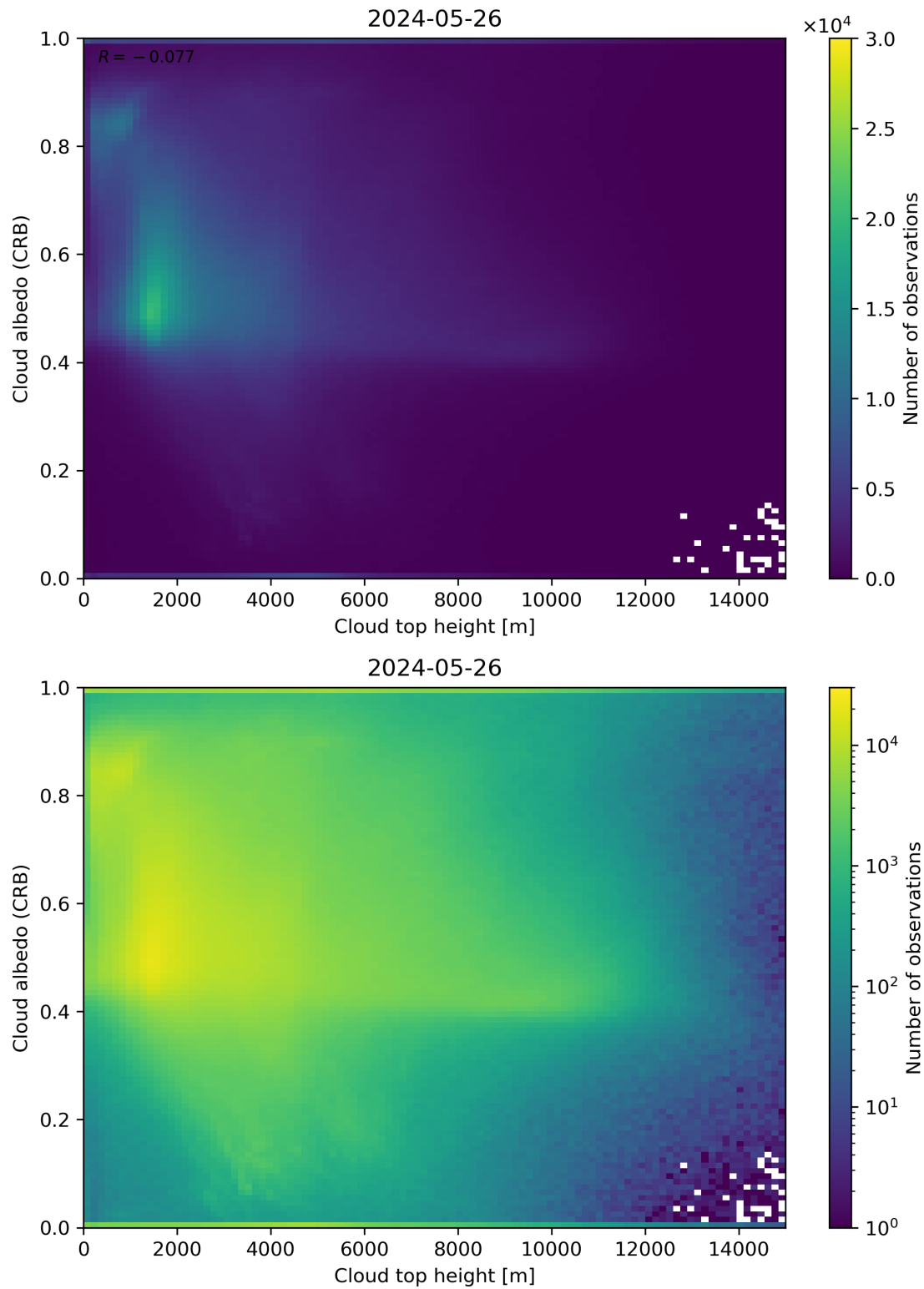
Figure 86: Scatter density plot of “Cloud top height” against “Cloud albedo (CRB)” for 2024-05-25 to 2024-05-27.
