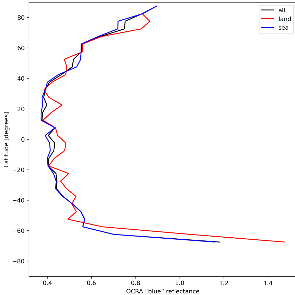
Figure 35: Zonal average of “OCRA “blue” reflectance” for 2024-05-25 to 2024-05-27.
