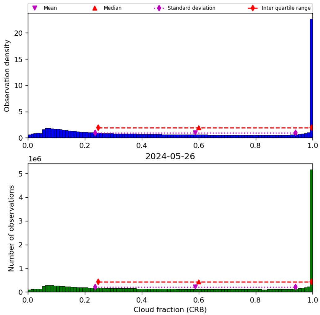
Figure 42: Histogram of “Cloud fraction (CRB)” for 2024-05-25 to 2024-05-27
