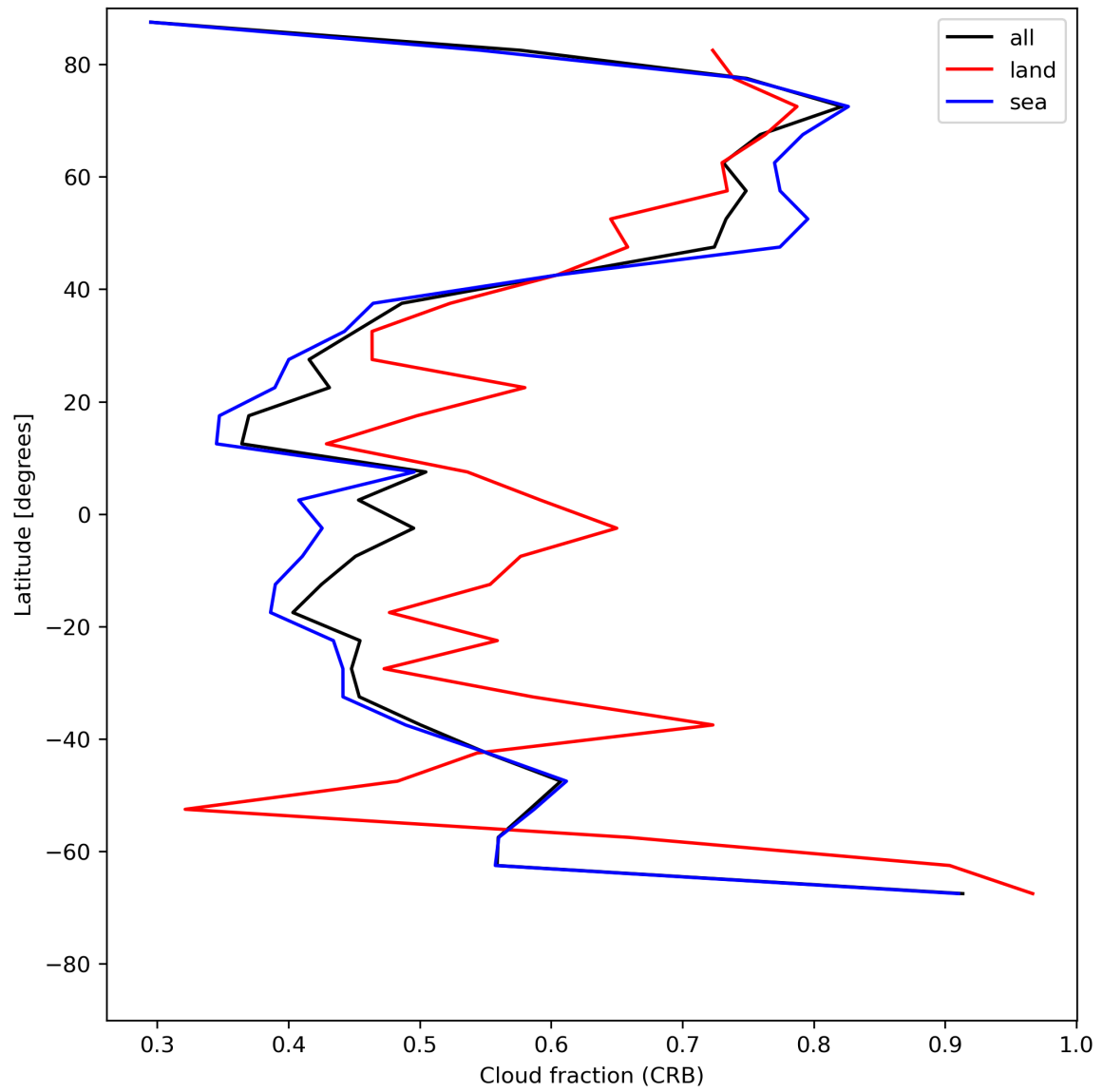
Figure 26: Zonal average of “Cloud fraction (CRB)” for 2024-05-25 to 2024-05-27.
