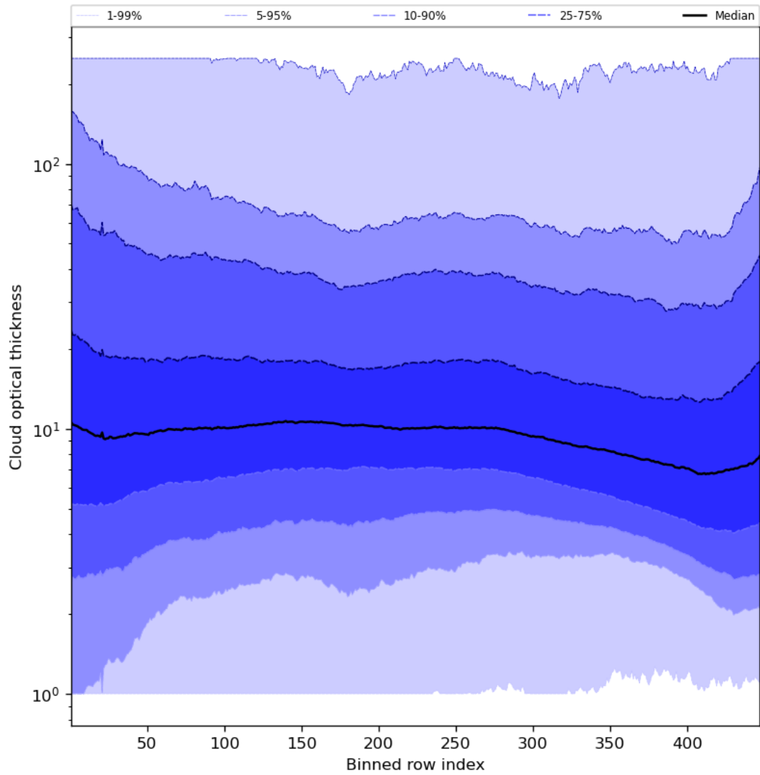
Figure 57: Along track statistics of “Cloud optical thickness” for 2024-05-25 to 2024-05-27
