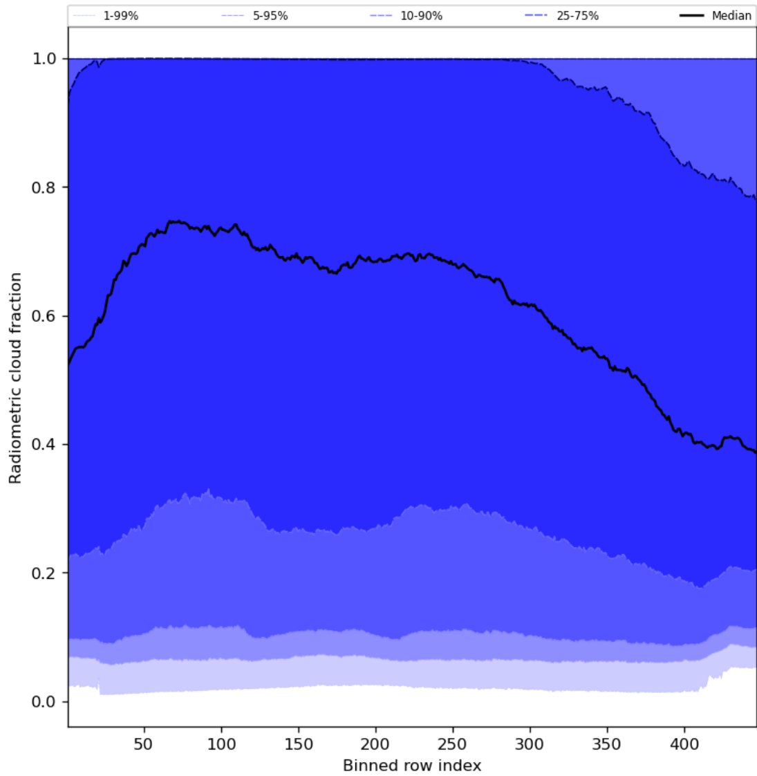
Figure 55: Along track statistics of “Radiometric cloud fraction” for 2024-05-25 to 2024-05-27
