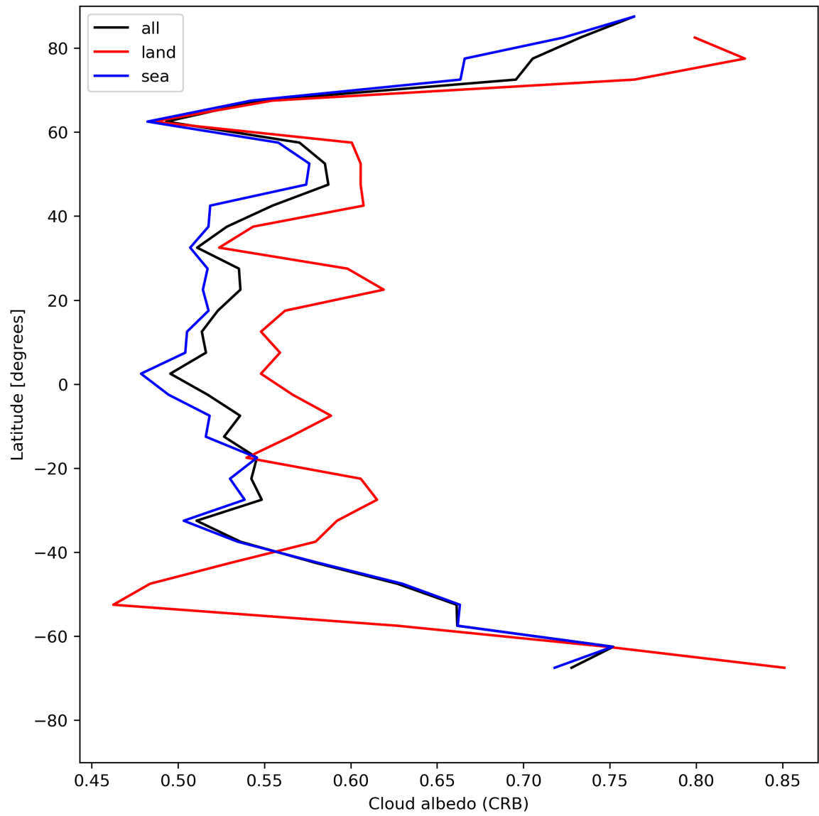
Figure 28: Zonal average of “Cloud albedo (CRB)” for 2024-05-25 to 2024-05-27.
