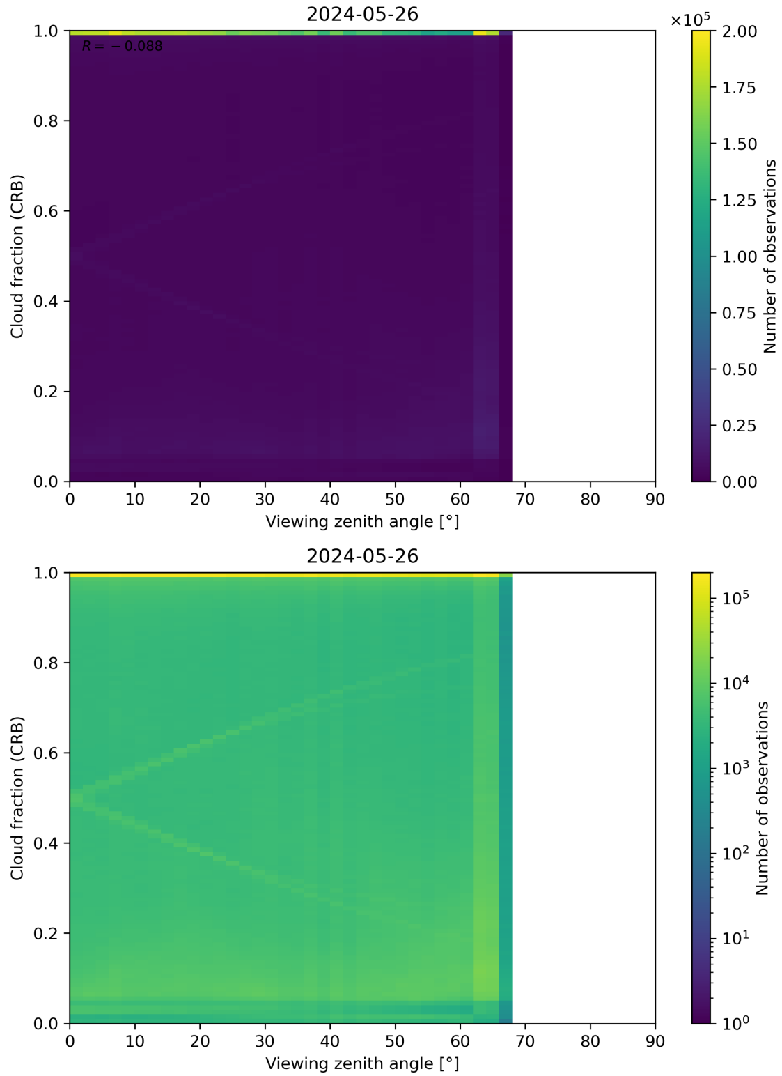
Figure 109: Scatter density plot of “Viewing zenith angle” against “Cloud fraction (CRB)” for 2024-05-25 to 2024-05-27.
