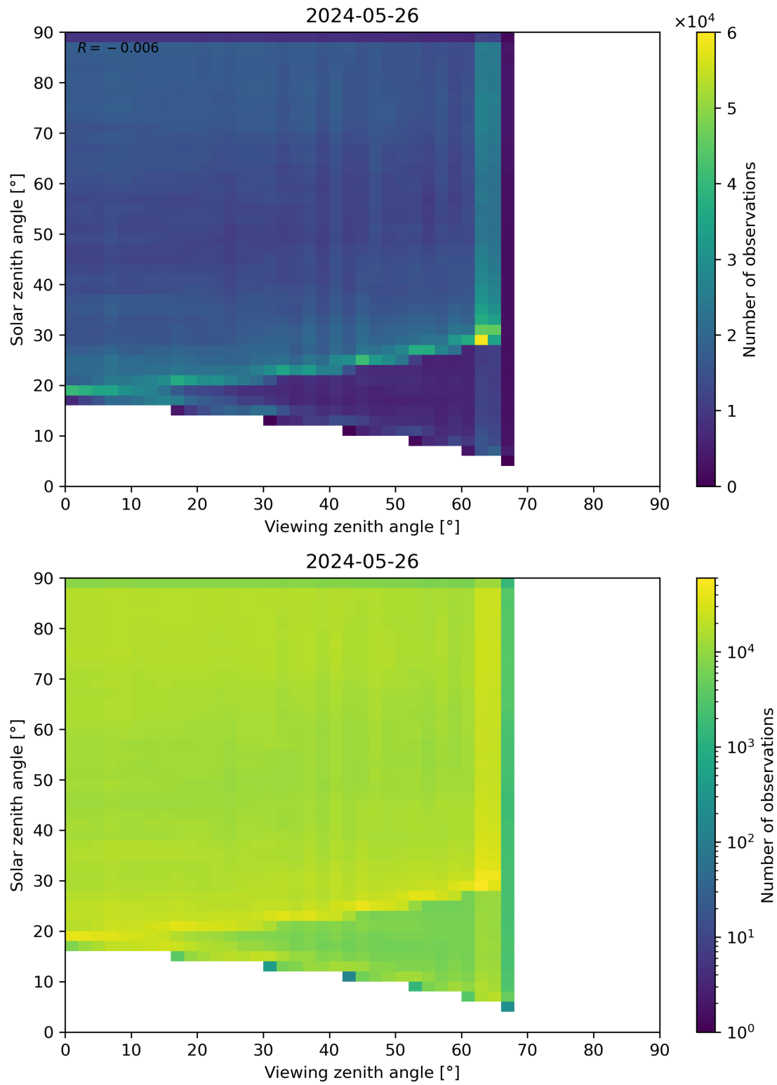
Figure 114: Scatter density plot of “Viewing zenith angle” against “Solar zenith angle” for 2024-05-25 to 2024-05-27.
