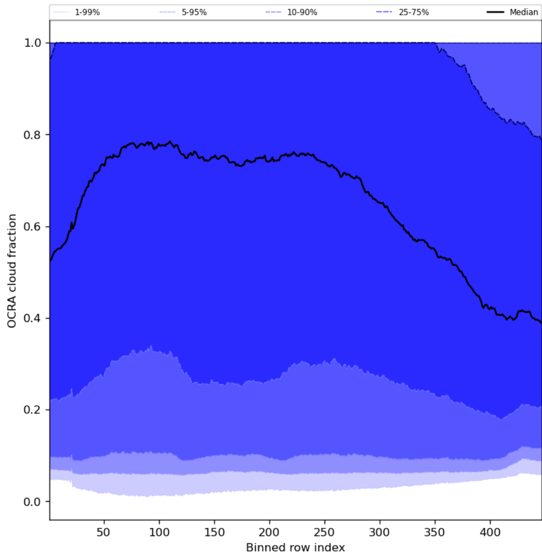
Figure 66: Along track statistics of “OCRA cloud fraction” for 2024-05-25 to 2024-05-27
