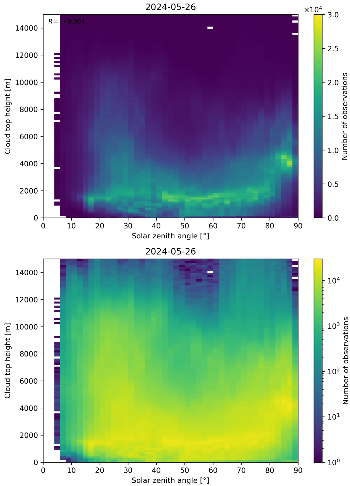
Figure 104: Scatter density plot of “Solar zenith angle” against “Cloud top height” for 2024-05-25 to 2024-05-27.
