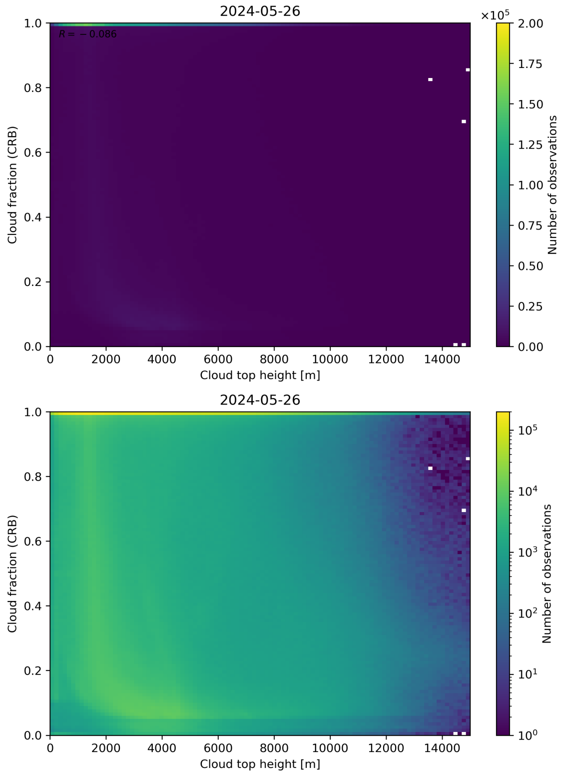
Figure 88: Scatter density plot of “Cloud top height” against “Cloud fraction (CRB)” for 2024-05-25 to 2024-05-27.
