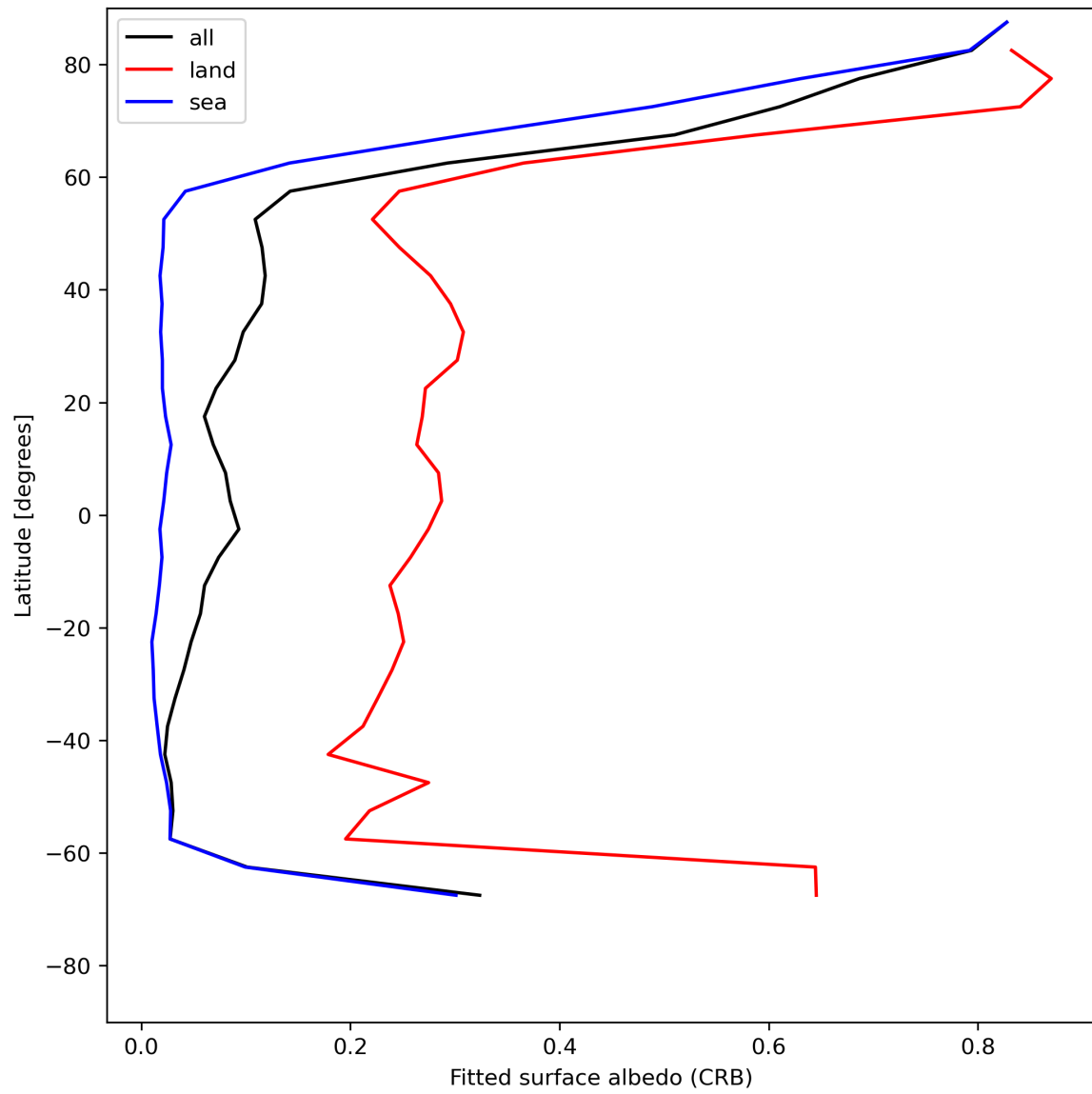
Figure 30: Zonal average of “Fitted surface albedo (CRB)” for 2024-05-25 to 2024-05-27.
