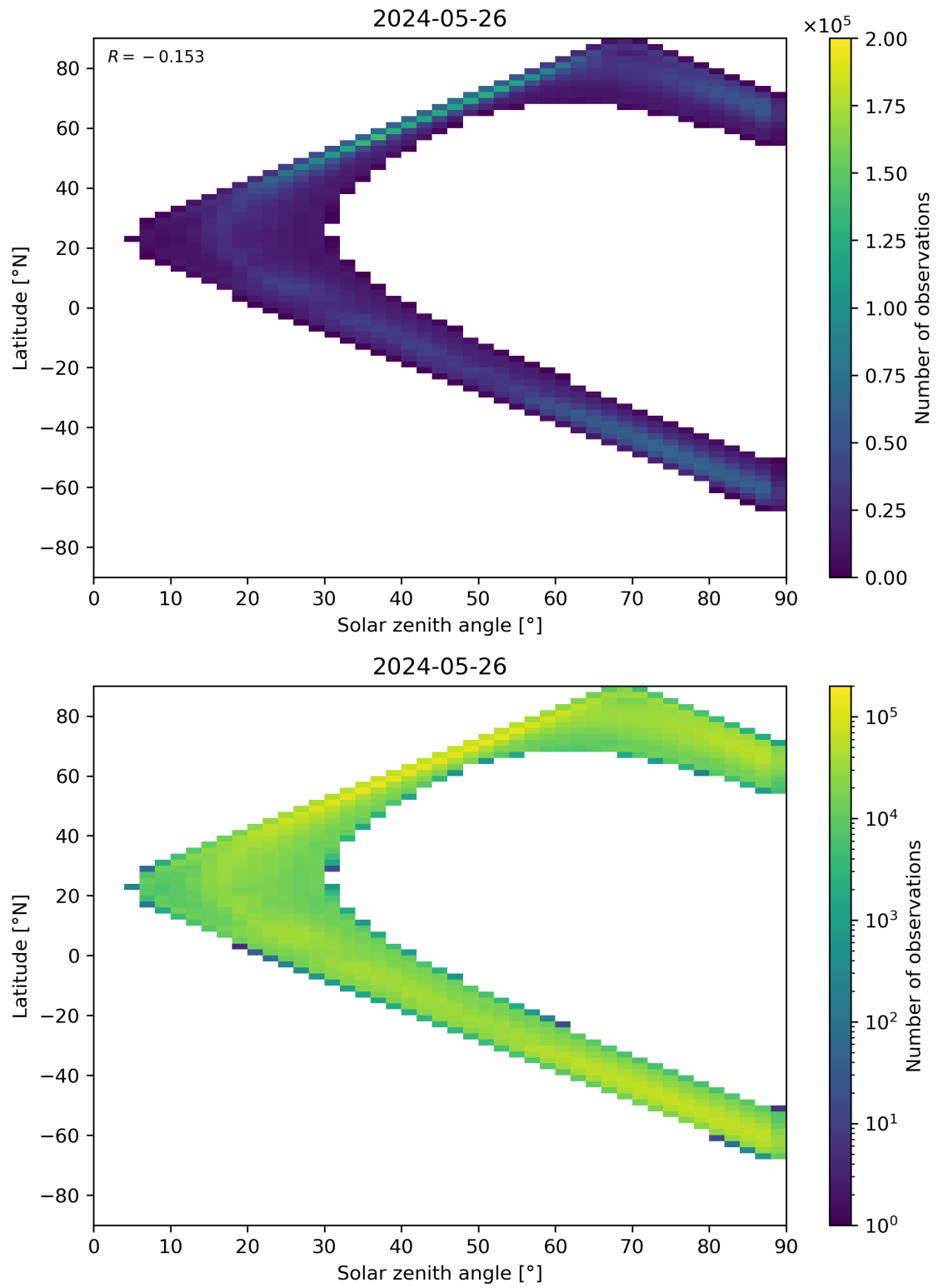
Figure 105: Scatter density plot of “Solar zenith angle” against “Latitude” for 2024-05-25 to 2024-05-27.
