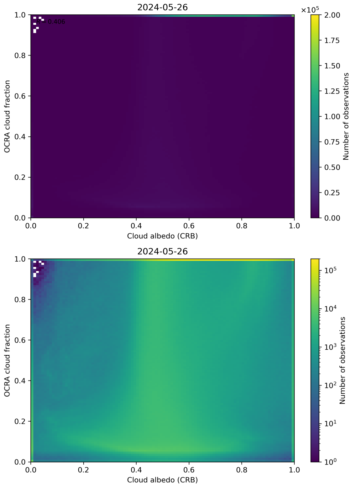
Figure 70: Scatter density plot of “Cloud albedo (CRB)” against “OCRA cloud fraction” for 2024-05-25 to 2024-05-27.
