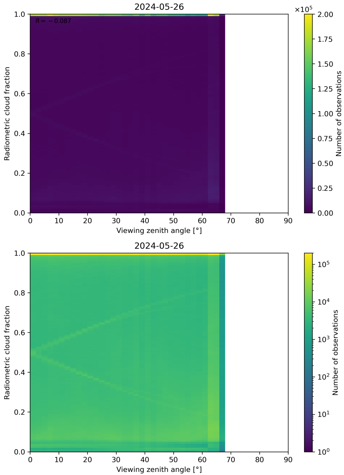
Figure 107: Scatter density plot of “Viewing zenith angle” against “Radiometric cloud fraction” for 2024-05-25 to 2024-05-27.
