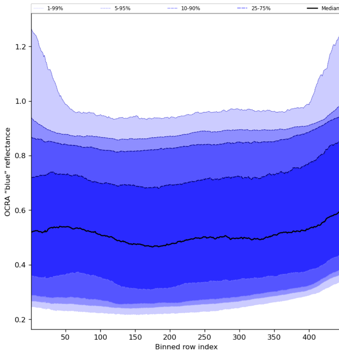
Figure 67: Along track statistics of “OCRA “blue” reflectance” for 2024-05-25 to 2024-05-27
