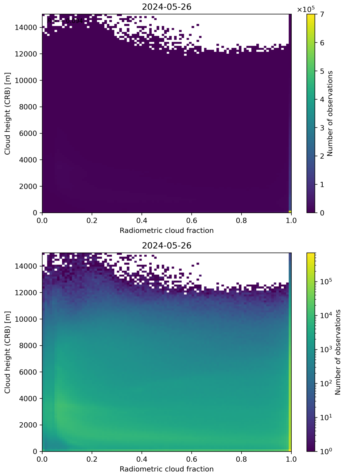
Figure 74: Scatter density plot of “Radiometric cloud fraction” against “Cloud height (CRB)” for 2024-05-25 to 2024-05-27.
