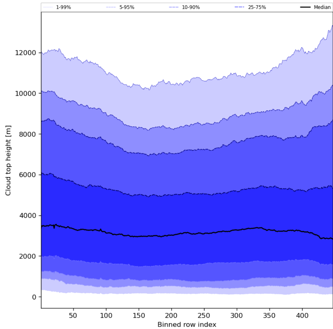
Figure 56: Along track statistics of “Cloud top height” for 2024-05-25 to 2024-05-27
