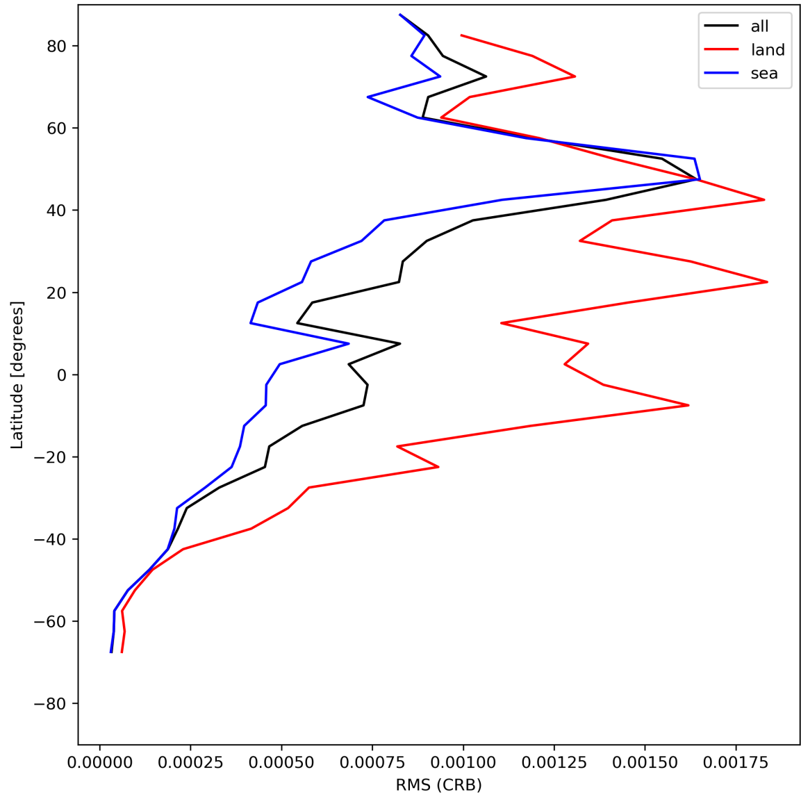
Figure 32: Zonal average of “RMS (CRB)” for 2024-05-25 to 2024-05-27.
