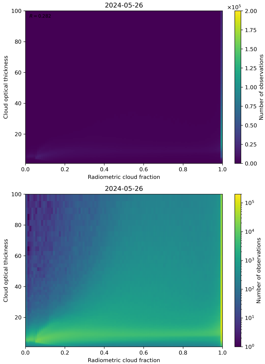
Figure 75: Scatter density plot of “Radiometric cloud fraction” against “Cloud optical thickness” for 2024-05-25 to 2024-05-27.
