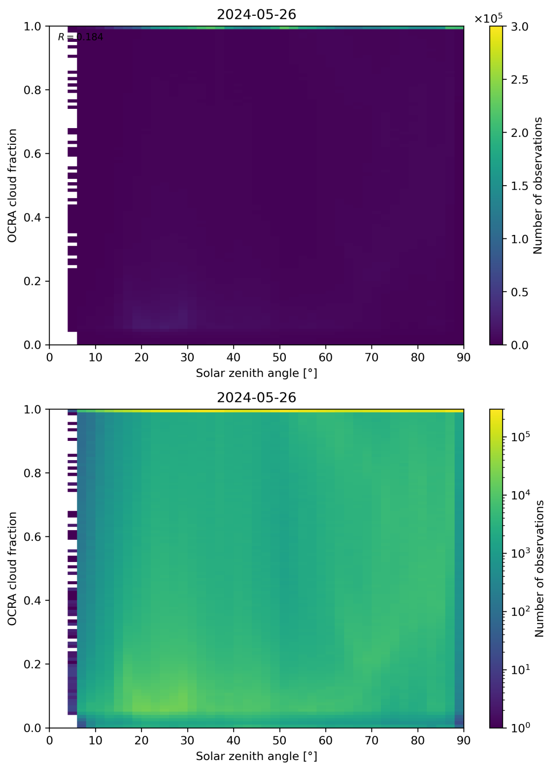
Figure 100: Scatter density plot of “Solar zenith angle” against “OCRA cloud fraction” for 2024-05-25 to 2024-05-27.
