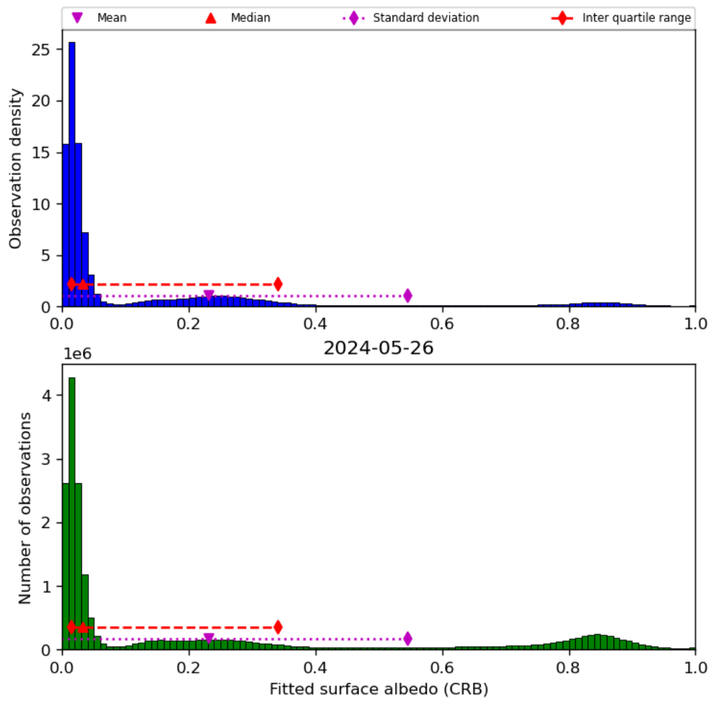
Figure 46: Histogram of “Fitted surface albedo (CRB)” for 2024-05-25 to 2024-05-27
