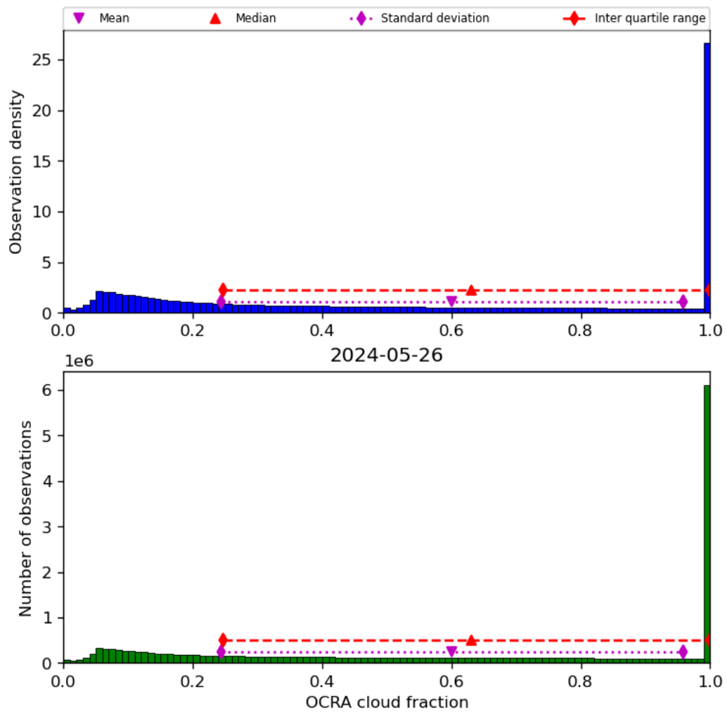
Figure 50: Histogram of “OCRA cloud fraction” for 2024-05-25 to 2024-05-27
