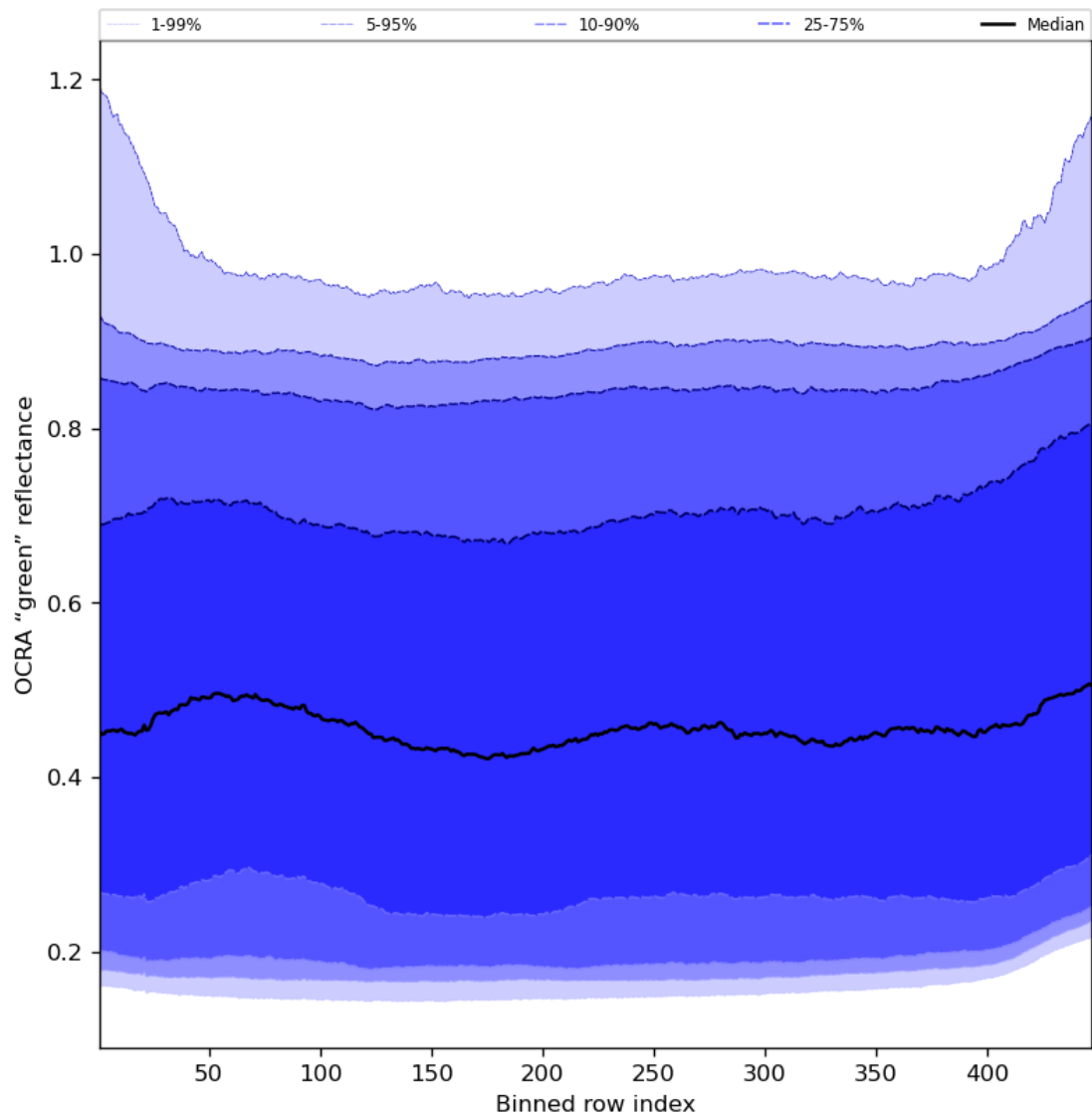
Figure 68: Along track statistics of “OCRA “green” reflectance” for 2024-05-25 to 2024-05-27
