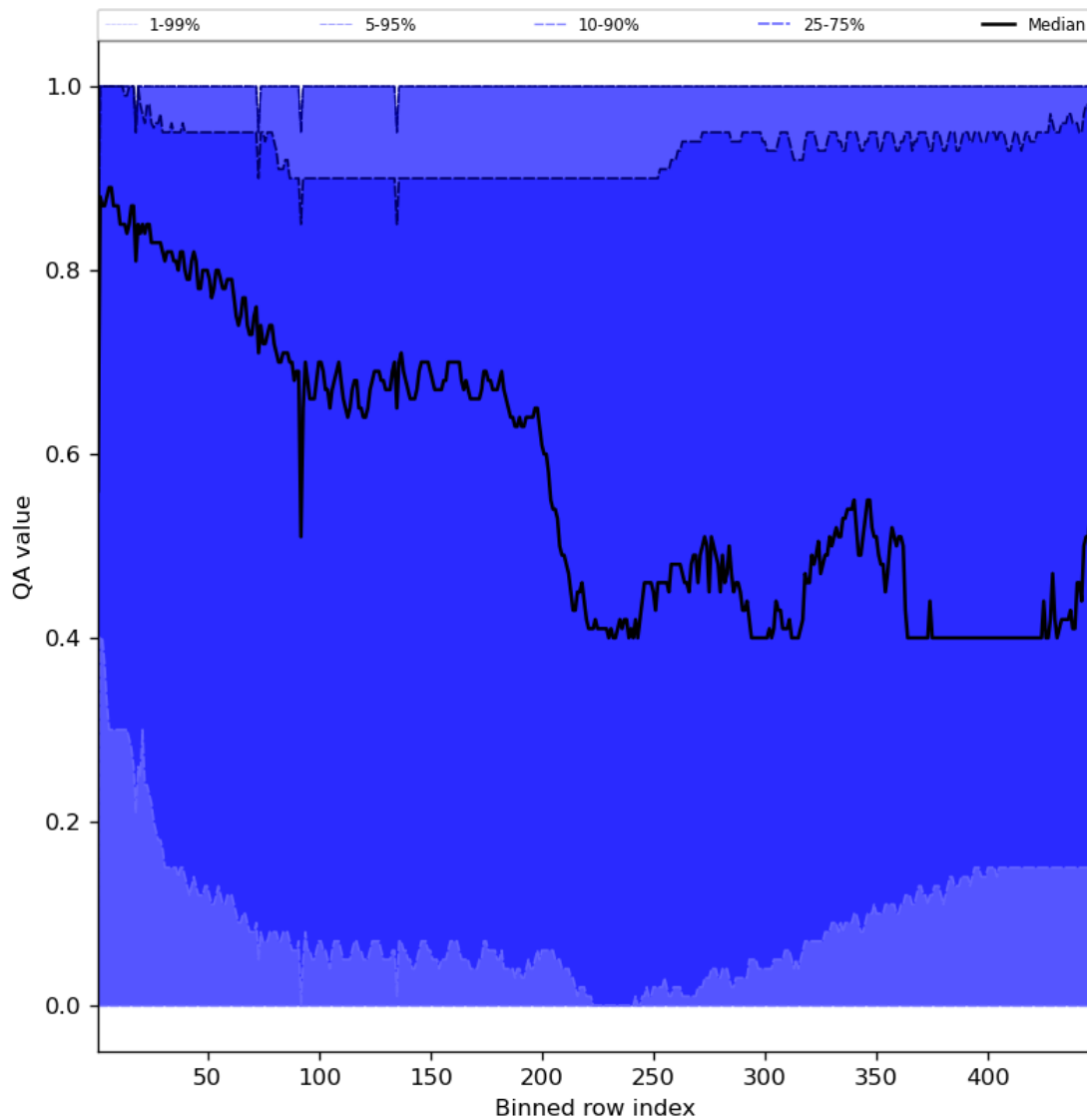
Figure 54: Along track statistics of “QA value” for 2024-05-25 to 2024-05-27
