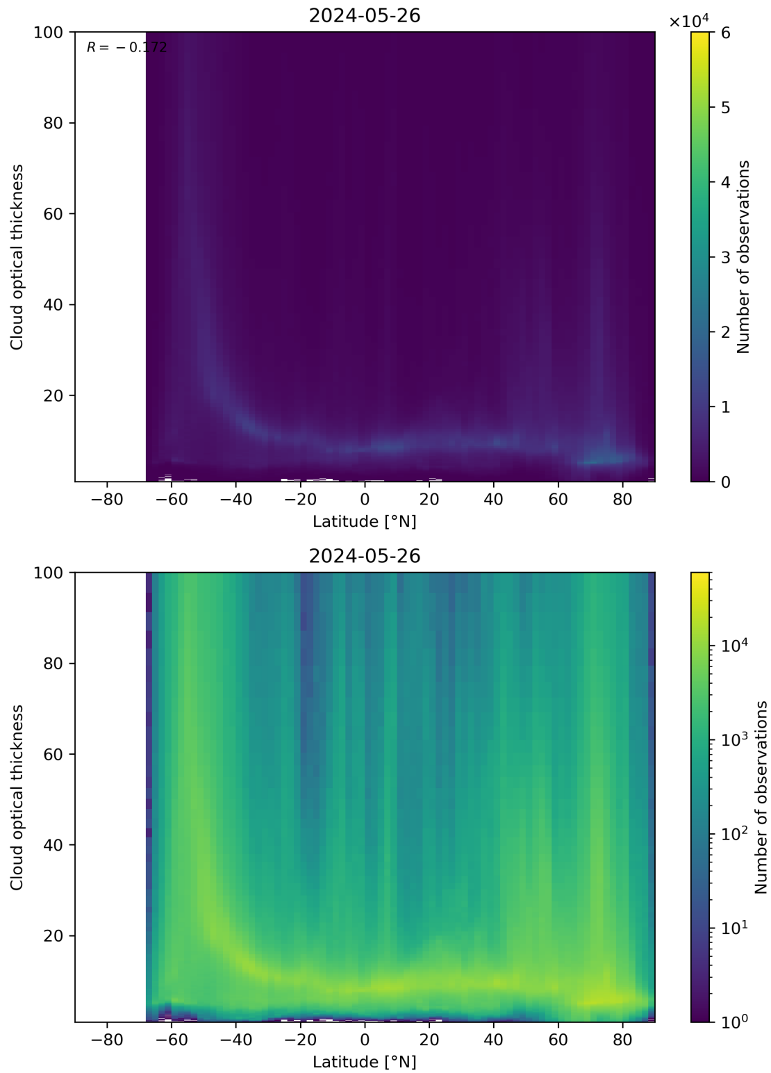
Figure 96: Scatter density plot of “Latitude” against “Cloud optical thickness” for 2024-05-25 to 2024-05-27.
