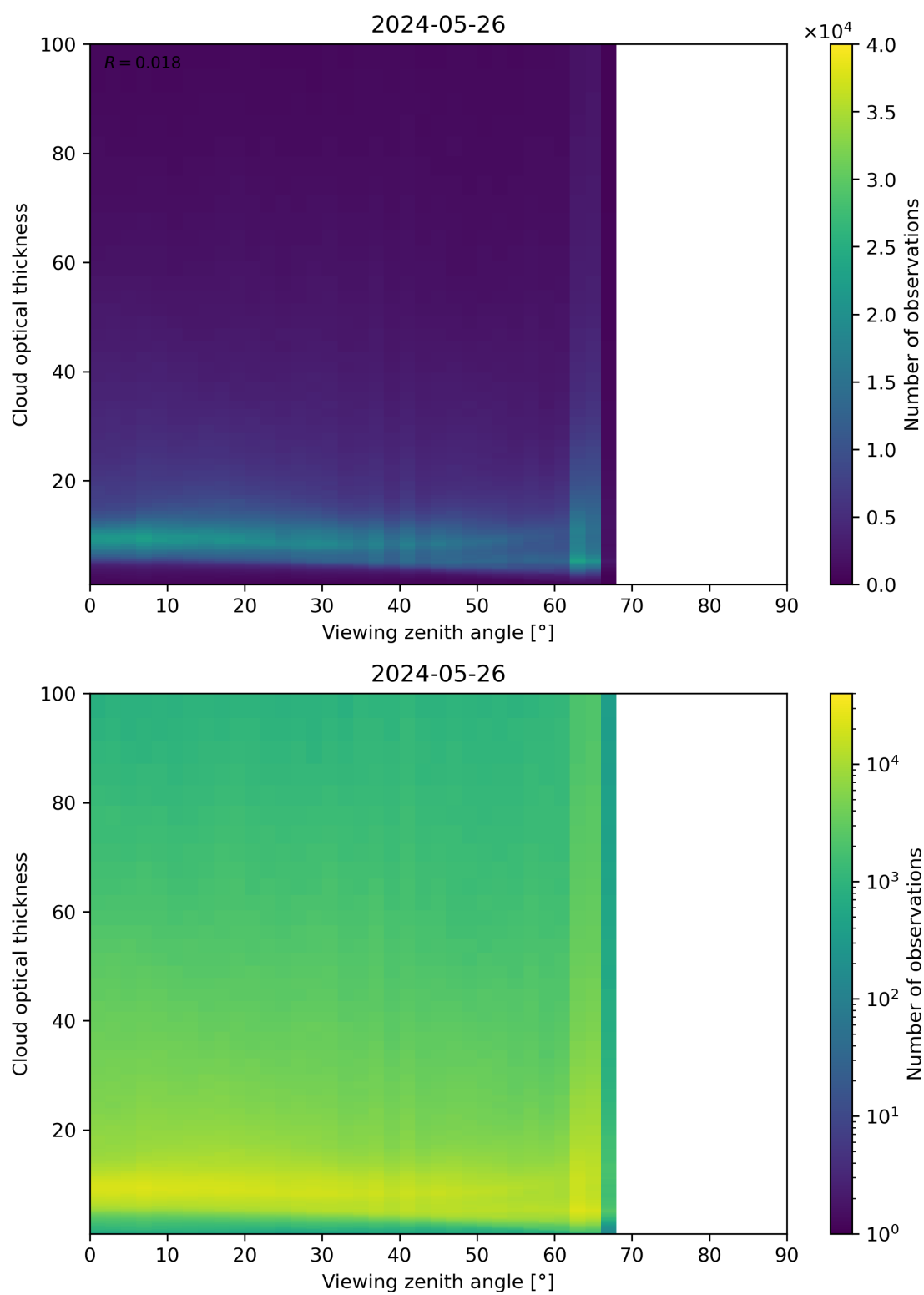
Figure 111: Scatter density plot of “Viewing zenith angle” against “Cloud optical thickness” for 2024-05-25 to 2024-05-27.
