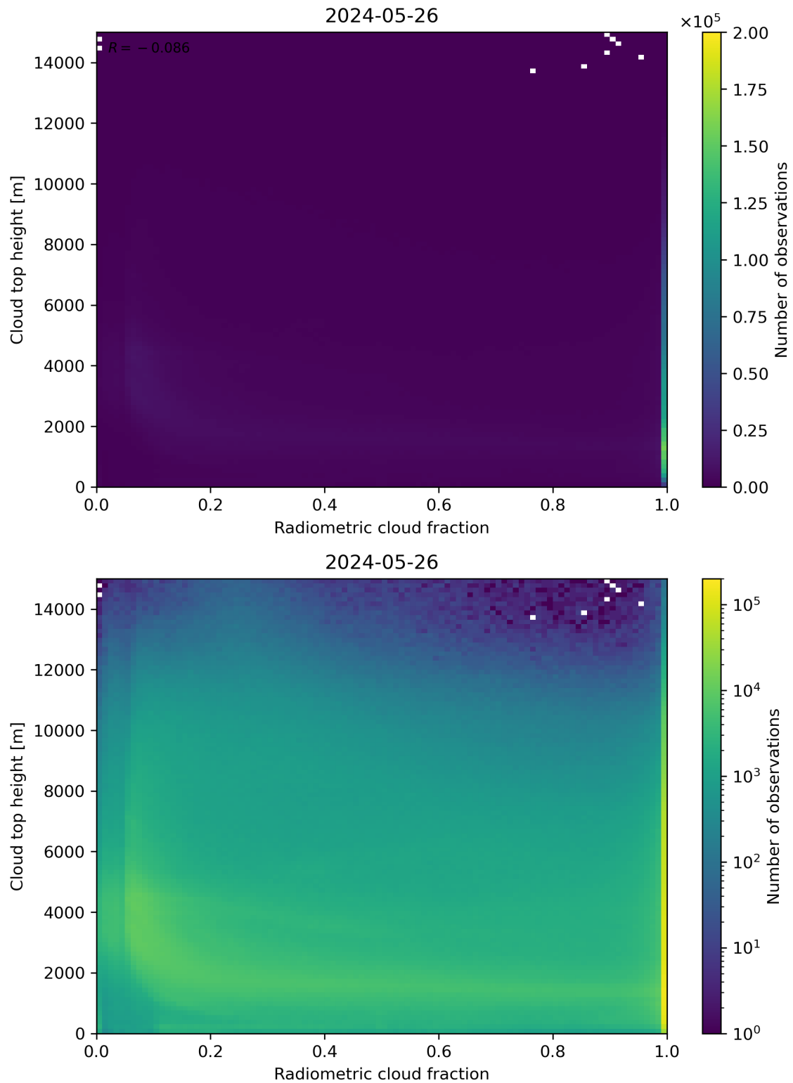
Figure 76: Scatter density plot of “Radiometric cloud fraction” against “Cloud top height” for 2024-05-25 to 2024-05-27.
