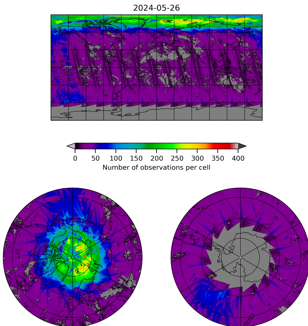
Figure 21: Map of the number of observations for 2024-05-25 to 2024-05-27
