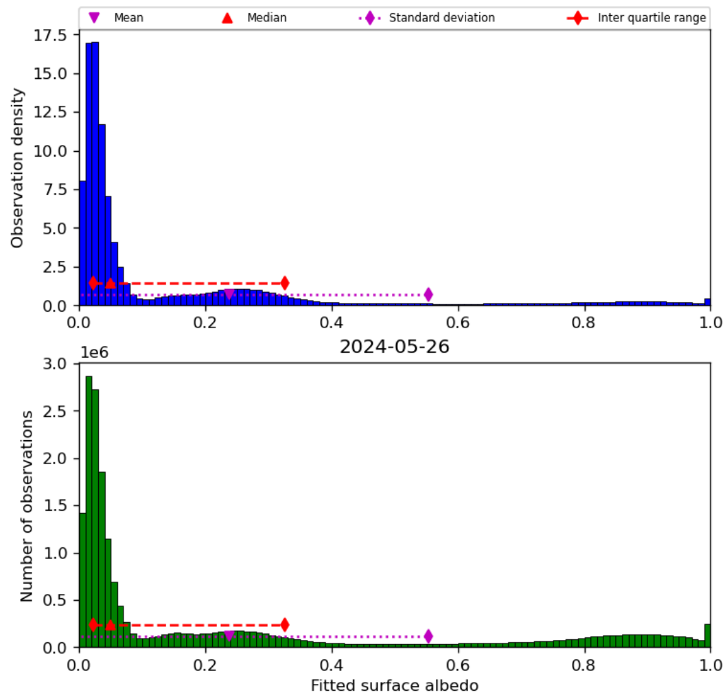
Figure 45: Histogram of “Fitted surface albedo” for 2024-05-25 to 2024-05-27
