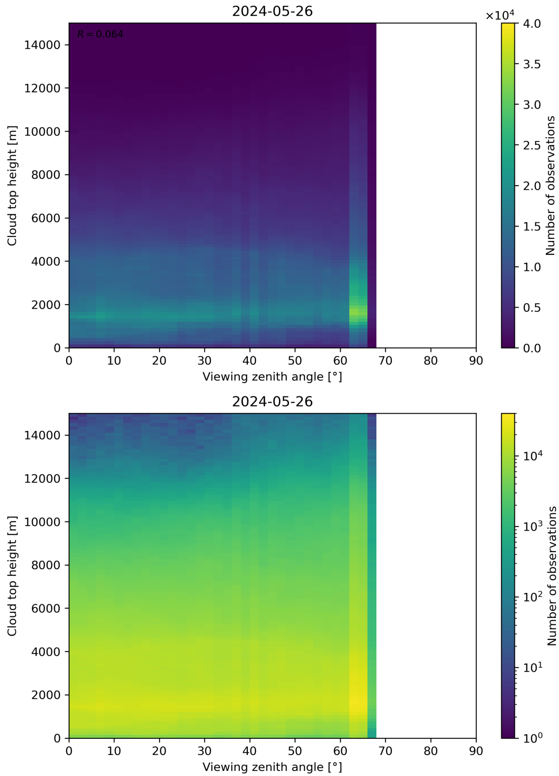
Figure 112: Scatter density plot of “Viewing zenith angle” against “Cloud top height” for 2024-05-25 to 2024-05-27.
