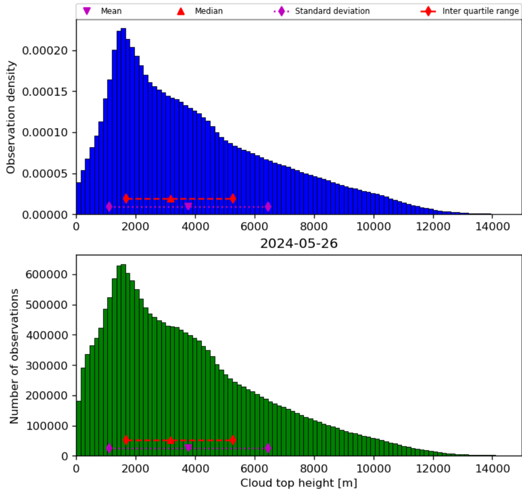
Figure 40: Histogram of “Cloud top height” for 2024-05-25 to 2024-05-27
