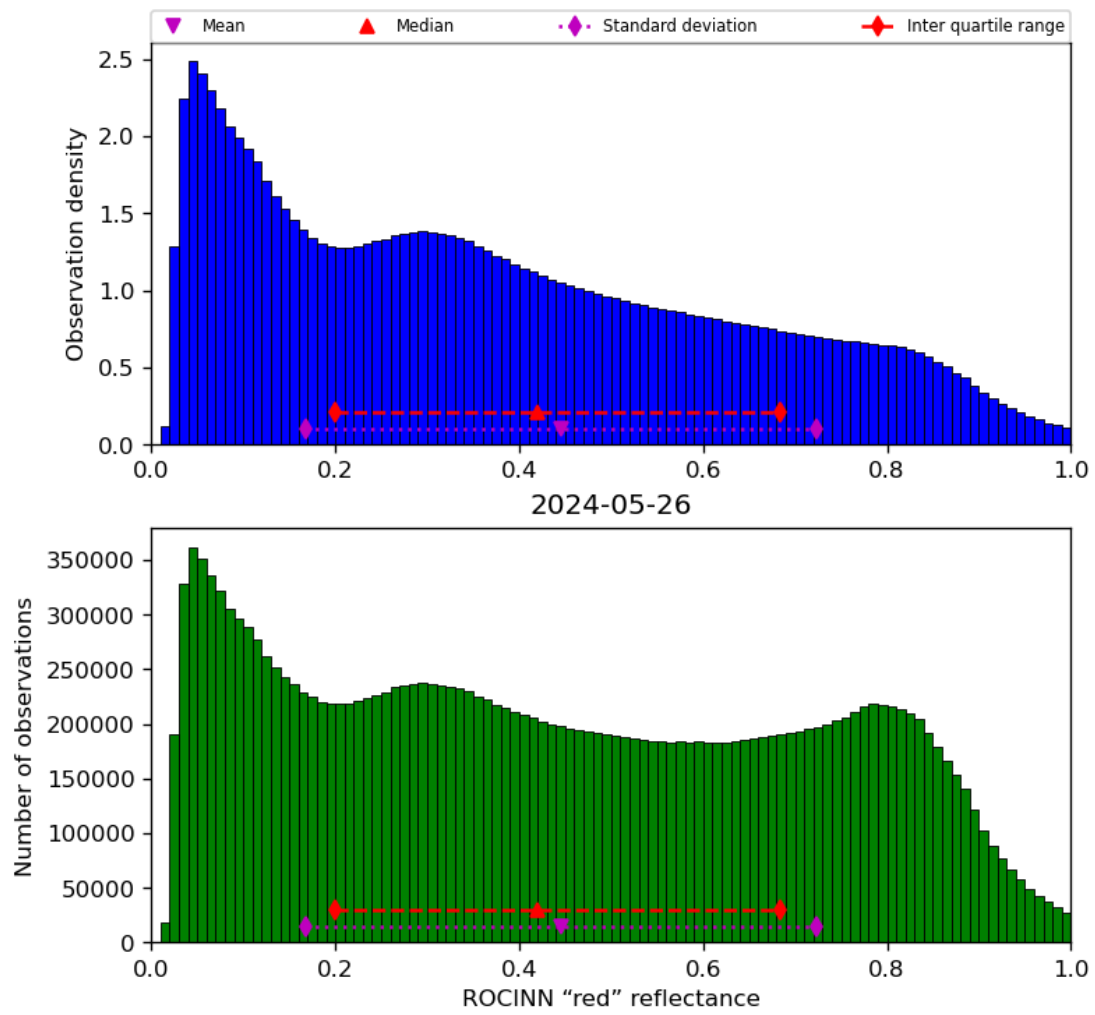
Figure 53: Histogram of “ROCINN “red” reflectance” for 2024-05-25 to 2024-05-27
