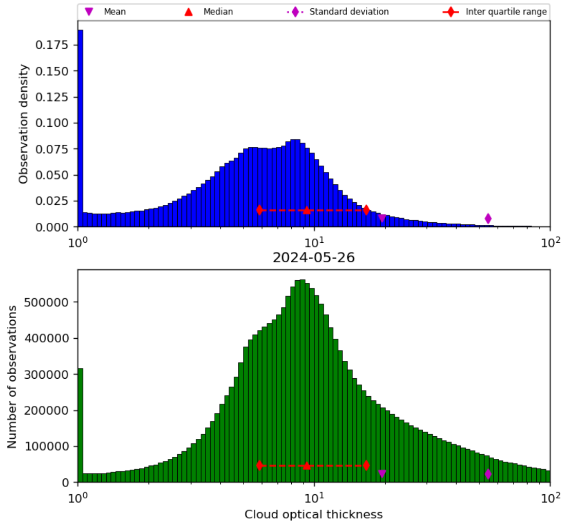
Figure 41: Histogram of “Cloud optical thickness” for 2024-05-25 to 2024-05-27
