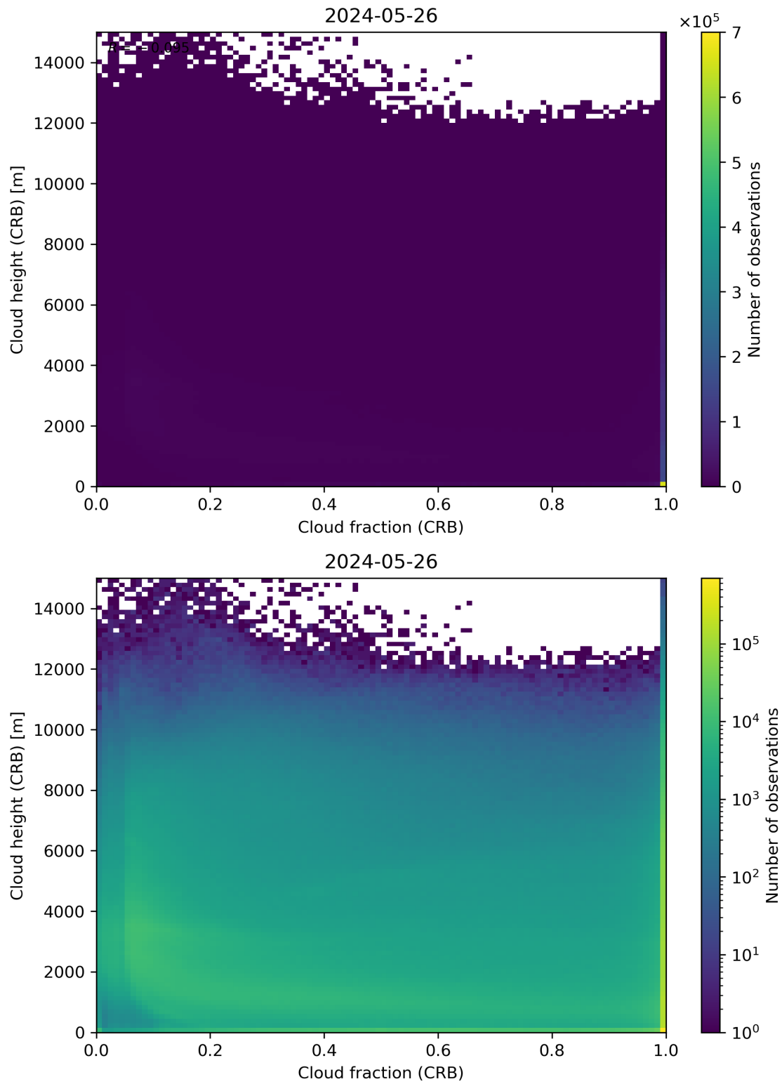
Figure 79: Scatter density plot of “Cloud fraction (CRB)” against “Cloud height (CRB)” for 2024-05-25 to 2024-05-27.
