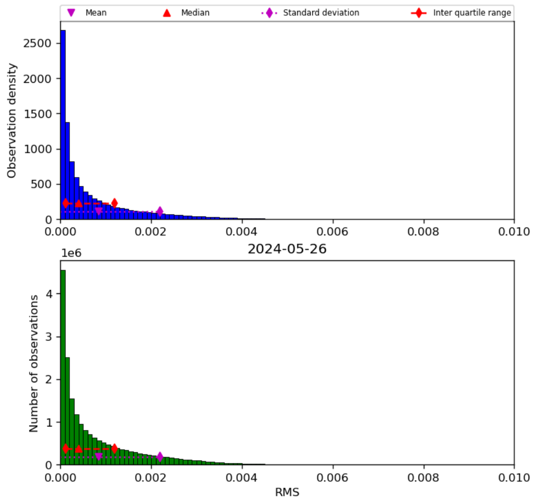
Figure 47: Histogram of “RMS” for 2024-05-25 to 2024-05-27
