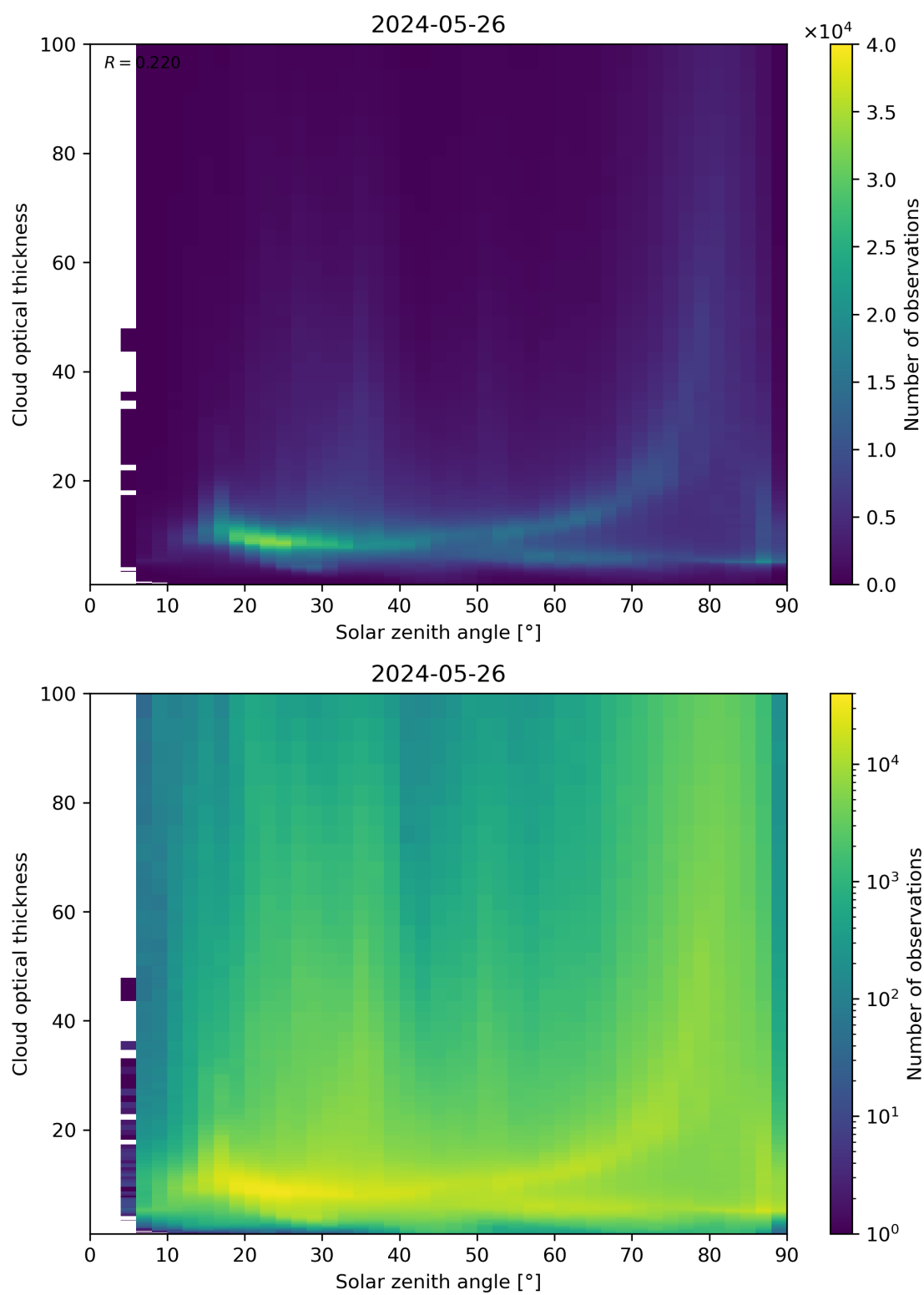
Figure 103: Scatter density plot of “Solar zenith angle” against “Cloud optical thickness” for 2024-05-25 to 2024-05-27.
