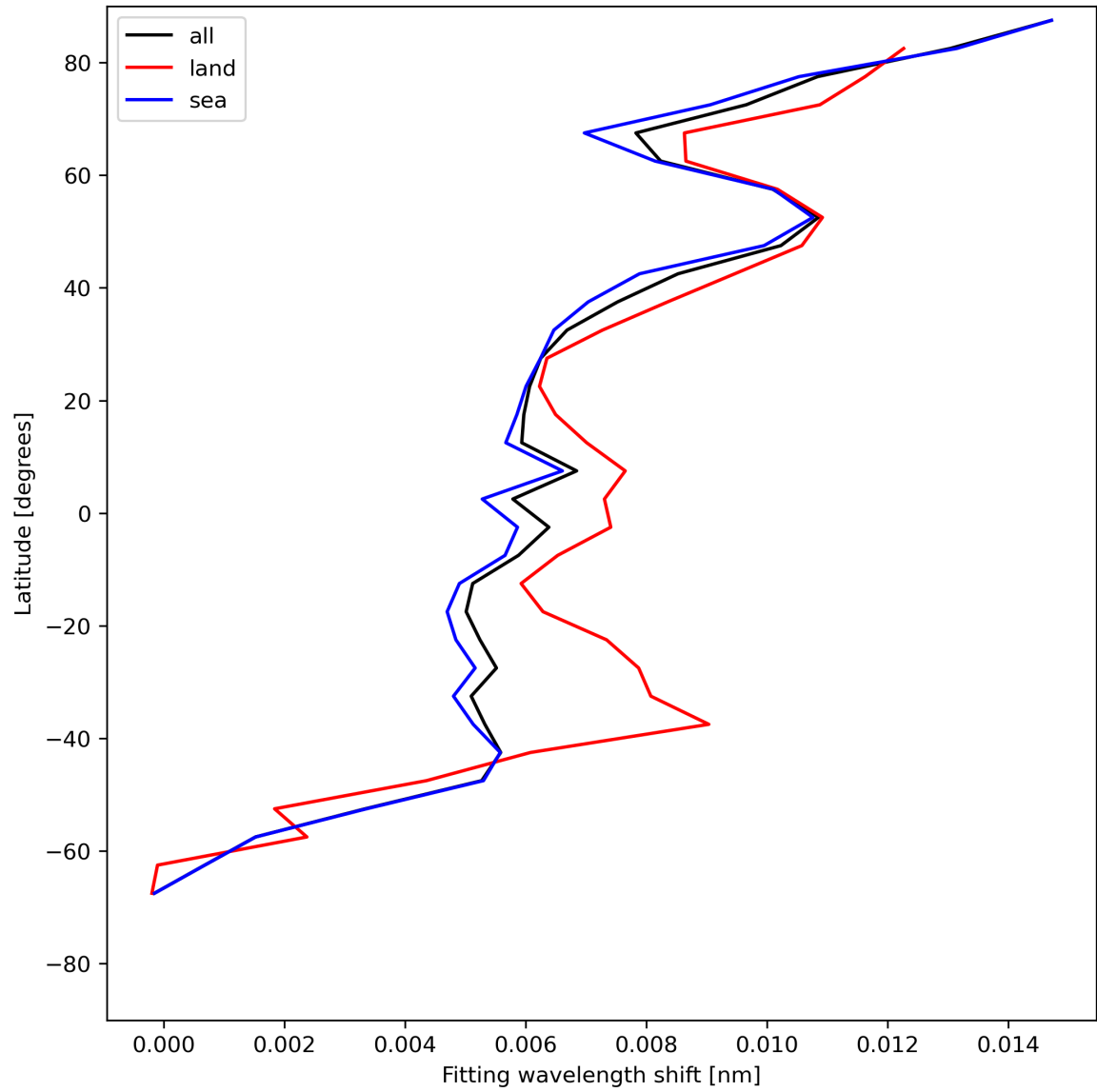
Figure 33: Zonal average of “Fitting wavelength shift” for 2024-05-25 to 2024-05-27.
