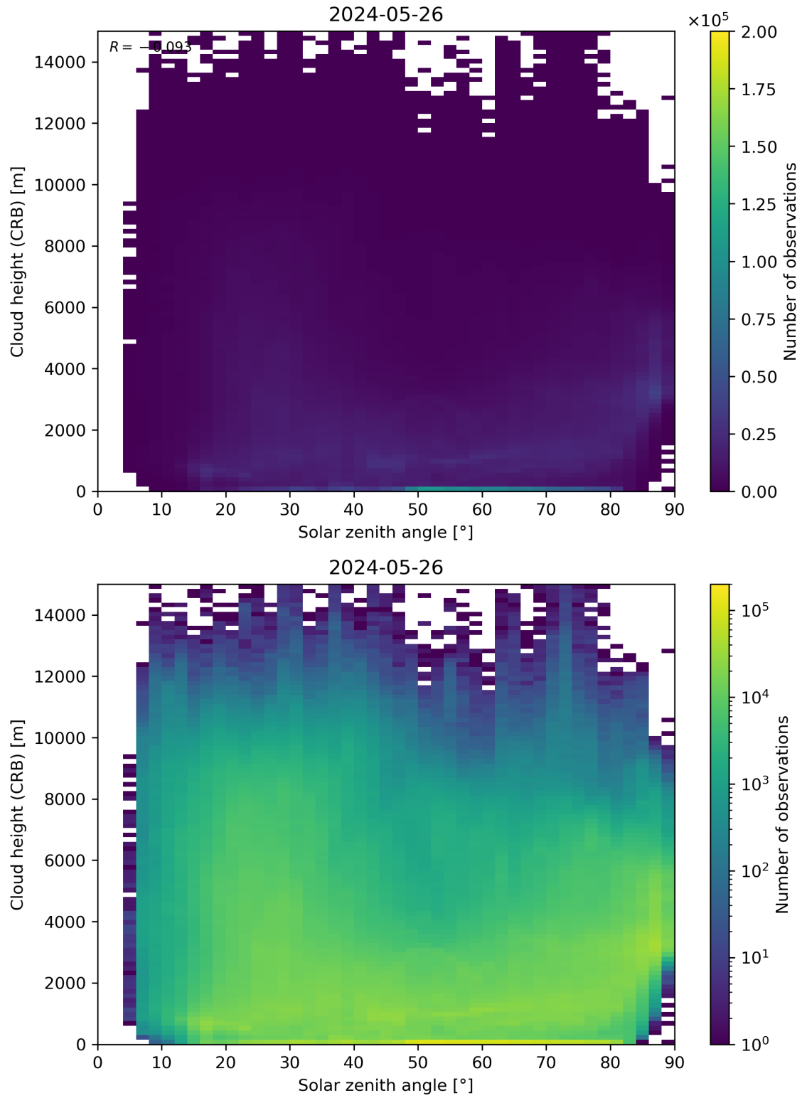
Figure 102: Scatter density plot of “Solar zenith angle” against “Cloud height (CRB)” for 2024-05-25 to 2024-05-27.
