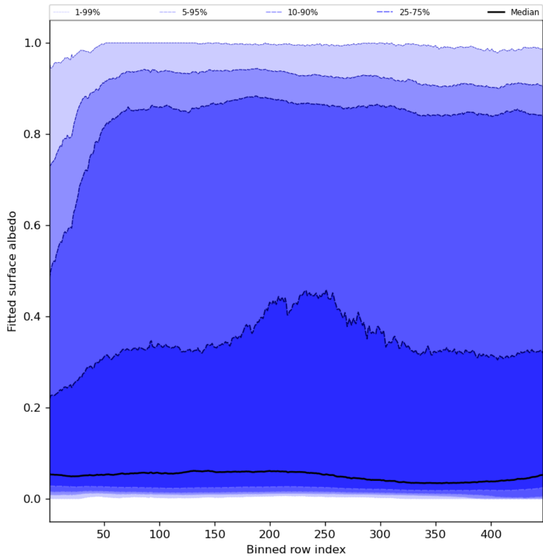
Figure 61: Along track statistics of “Fitted surface albedo” for 2024-05-25 to 2024-05-27
