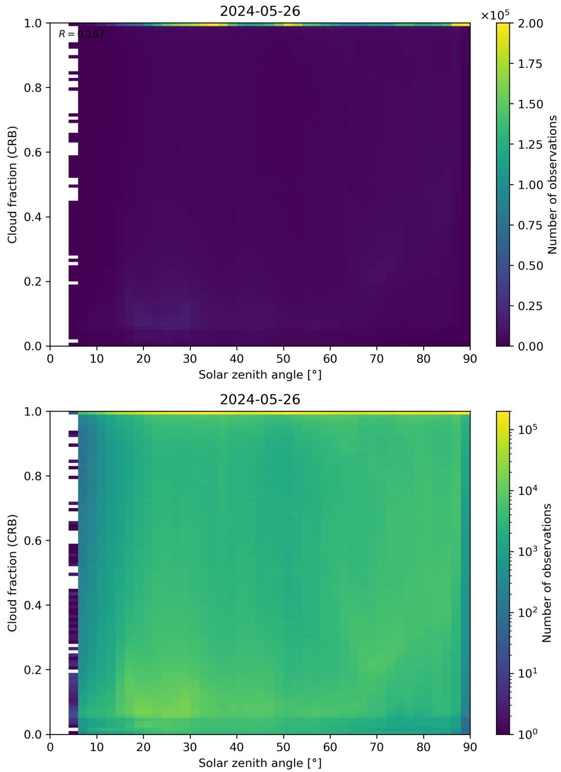
Figure 101: Scatter density plot of “Solar zenith angle” against “Cloud fraction (CRB)” for 2024-05-25 to 2024-05-27.
