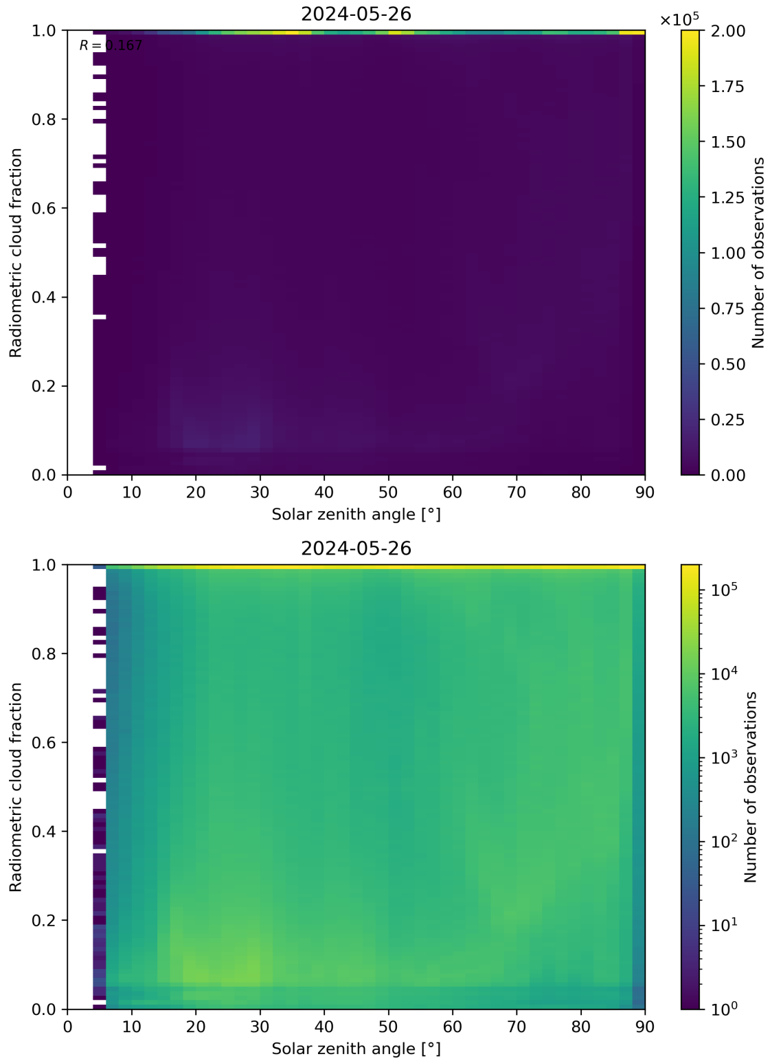
Figure 99: Scatter density plot of “Solar zenith angle” against “Radiometric cloud fraction” for 2024-05-25 to 2024-05-27.
