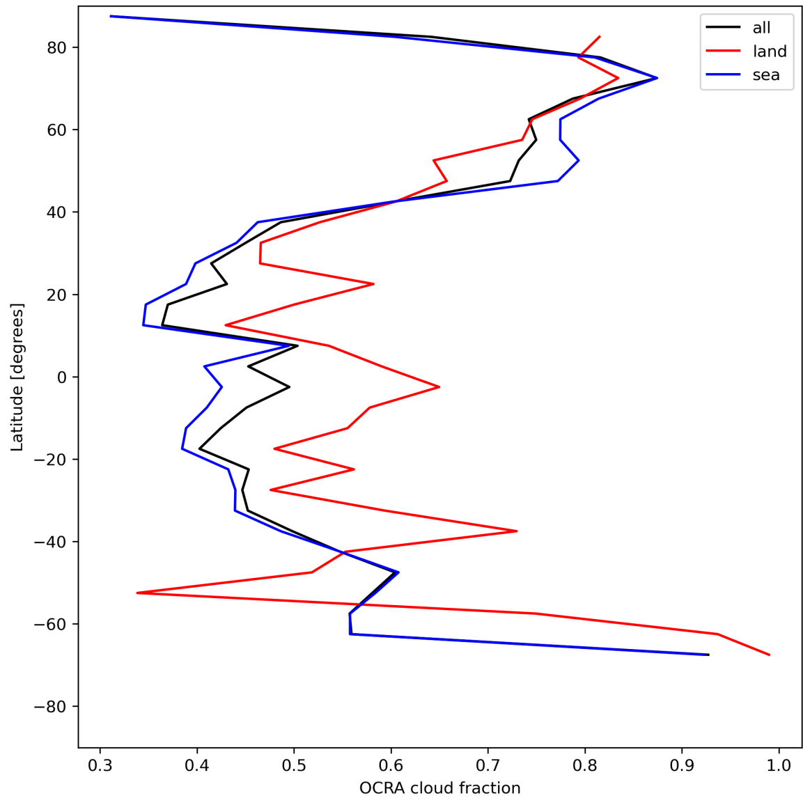
Figure 34: Zonal average of “OCRA cloud fraction” for 2024-05-25 to 2024-05-27.
