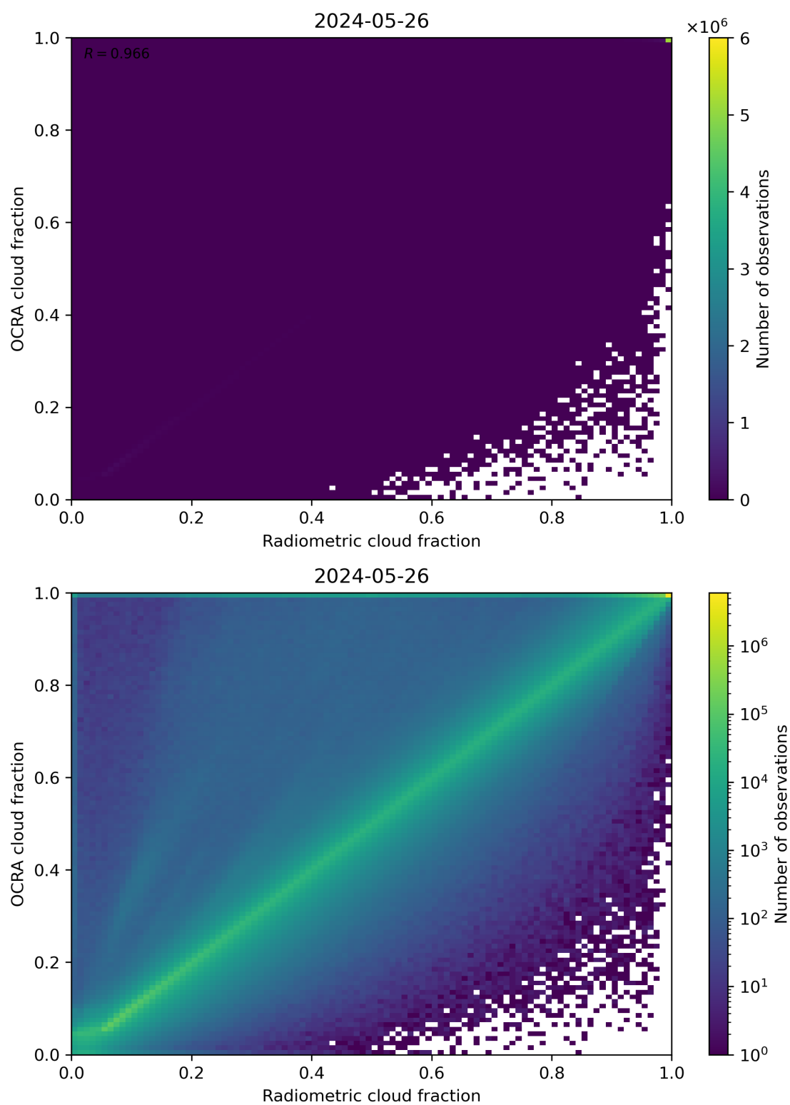
Figure 72: Scatter density plot of “Radiometric cloud fraction” against “OCRA cloud fraction” for 2024-05-25 to 2024-05-27.
