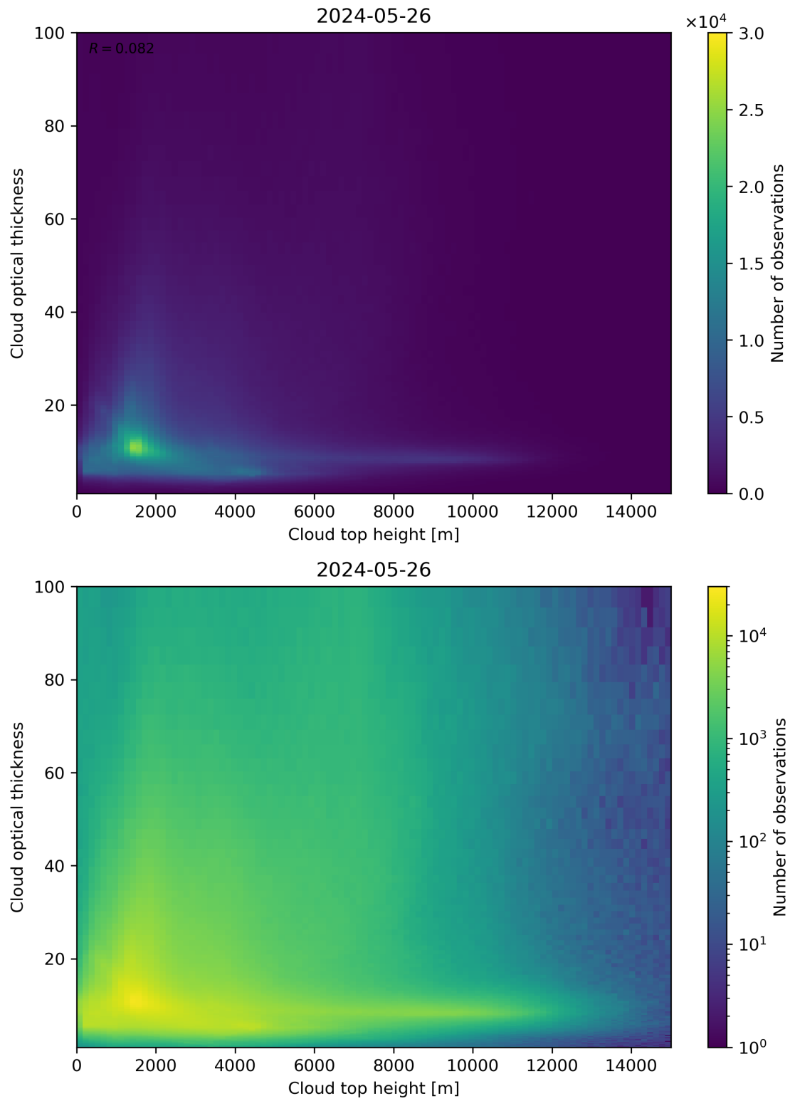
Figure 90: Scatter density plot of “Cloud top height” against “Cloud optical thickness” for 2024-05-25 to 2024-05-27.
