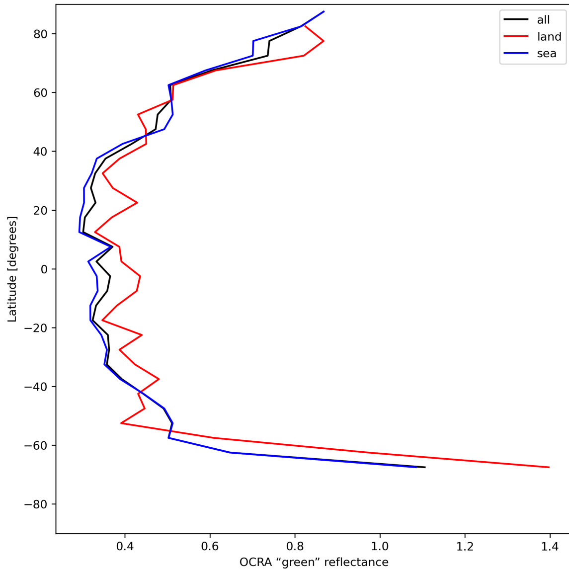
Figure 36: Zonal average of “OCRA “green” reflectance” for 2024-05-25 to 2024-05-27.
