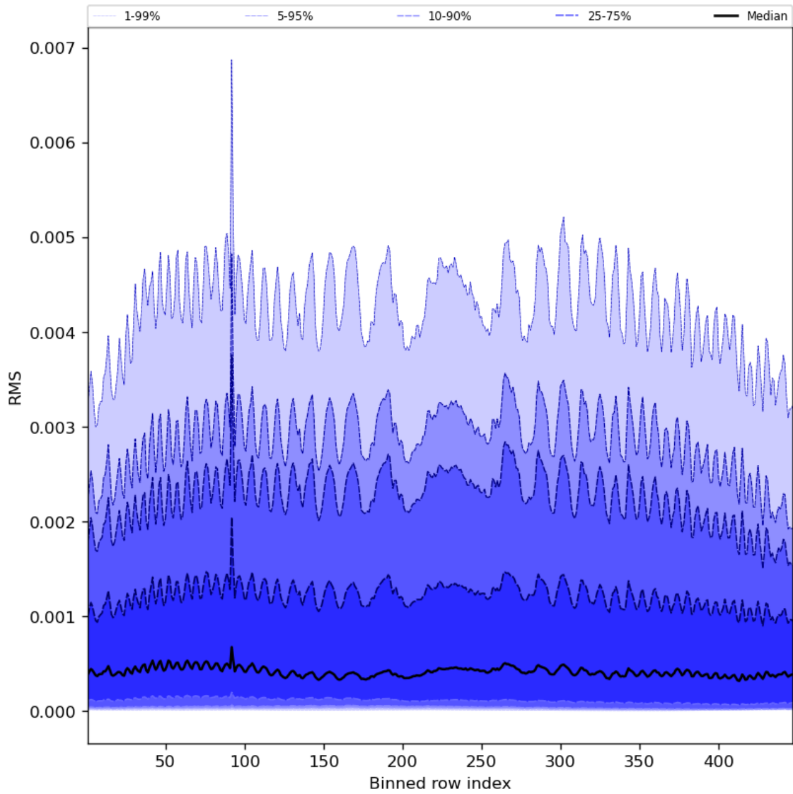
Figure 63: Along track statistics of “RMS” for 2024-05-25 to 2024-05-27
