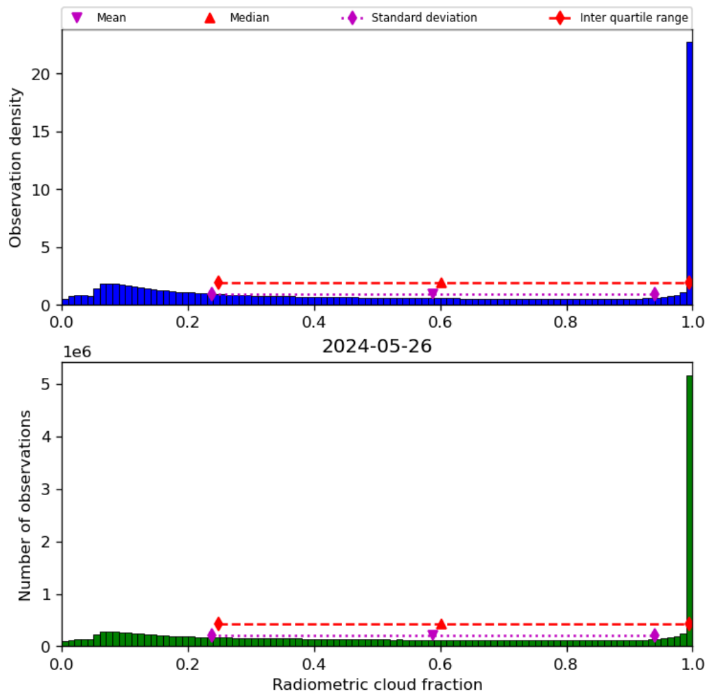
Figure 39: Histogram of “Radiometric cloud fraction” for 2024-05-25 to 2024-05-27
