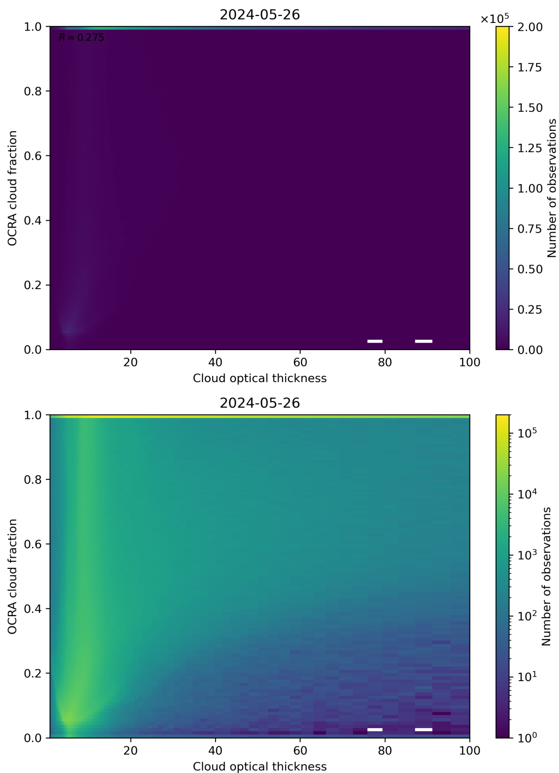
Figure 83: Scatter density plot of “Cloud optical thickness” against “OCRA cloud fraction” for 2024-05-25 to 2024-05-27.
