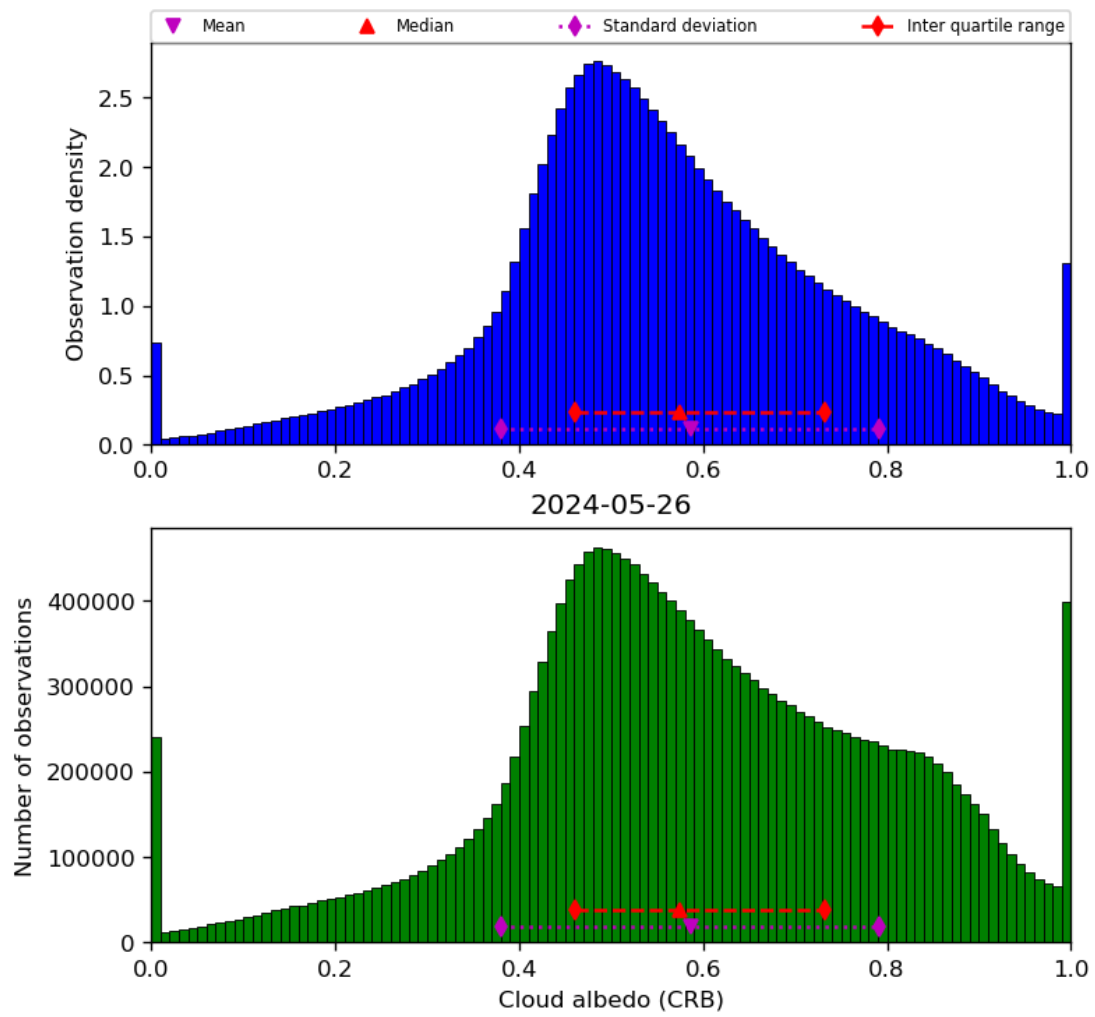
Figure 44: Histogram of “Cloud albedo (CRB)” for 2024-05-25 to 2024-05-27
