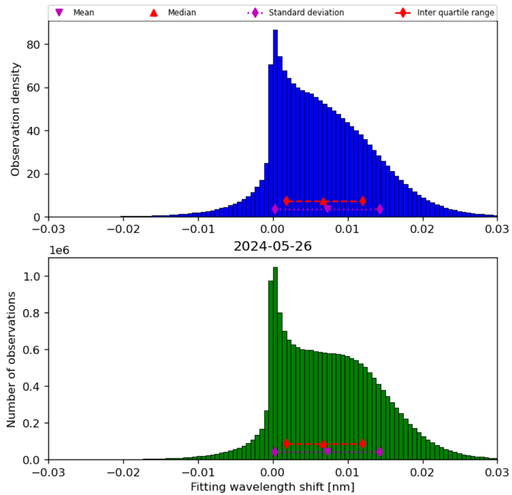
Figure 49: Histogram of “Fitting wavelength shift” for 2024-05-25 to 2024-05-27
