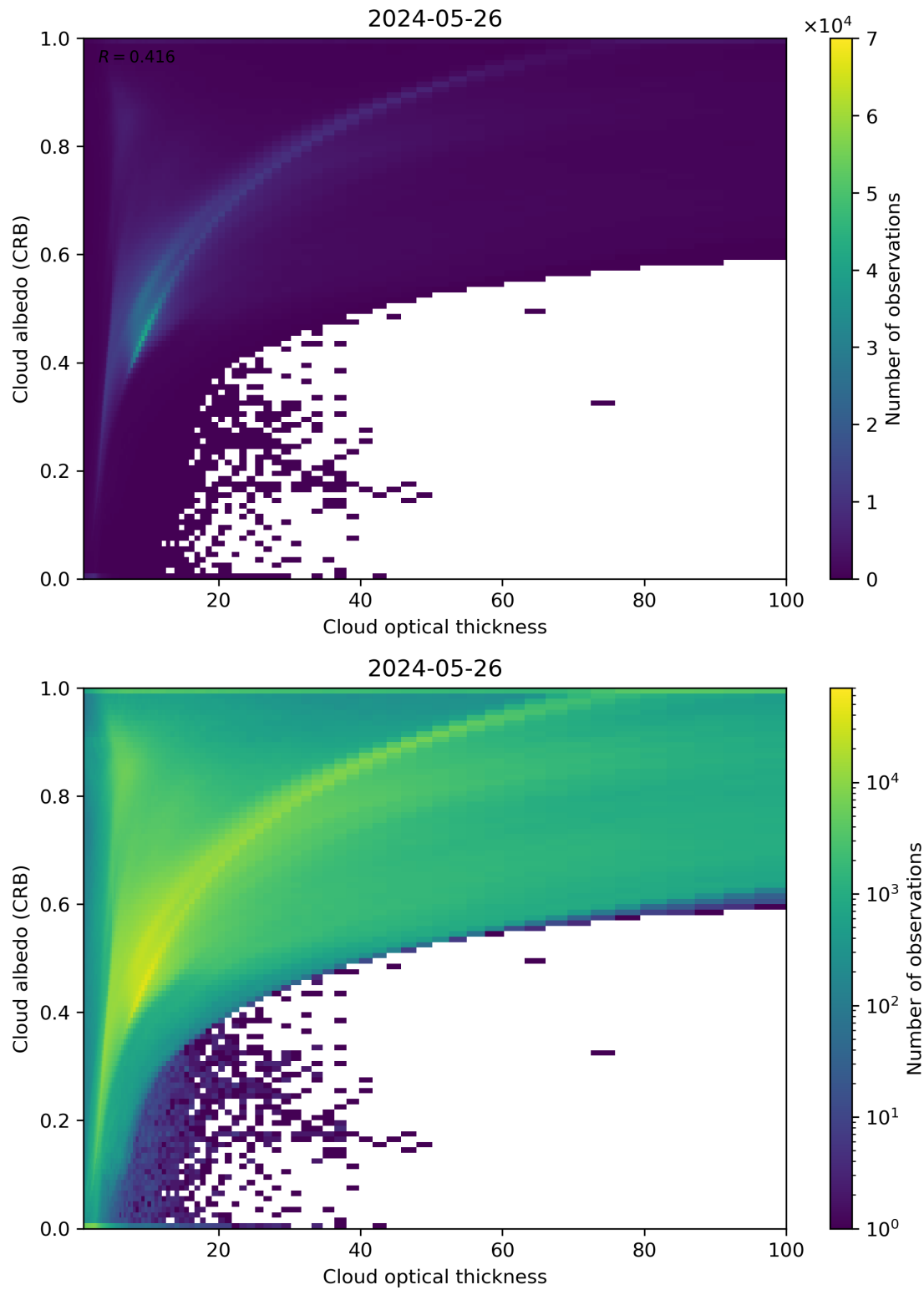
Figure 82: Scatter density plot of “Cloud optical thickness” against “Cloud albedo (CRB)” for 2024-05-25 to 2024-05-27.
