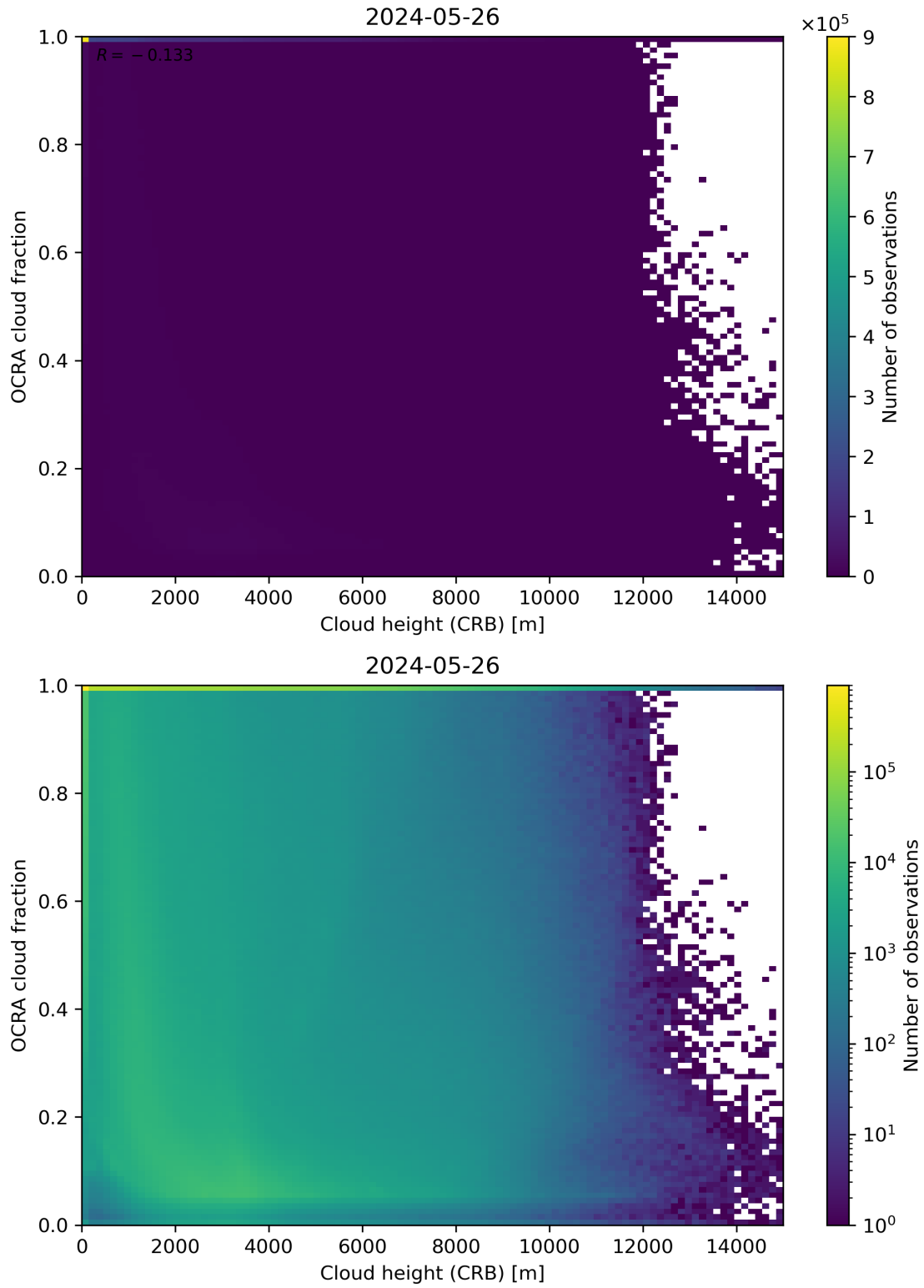
Figure 81: Scatter density plot of “Cloud height (CRB)” against “OCRA cloud fraction” for 2024-05-25 to 2024-05-27.
