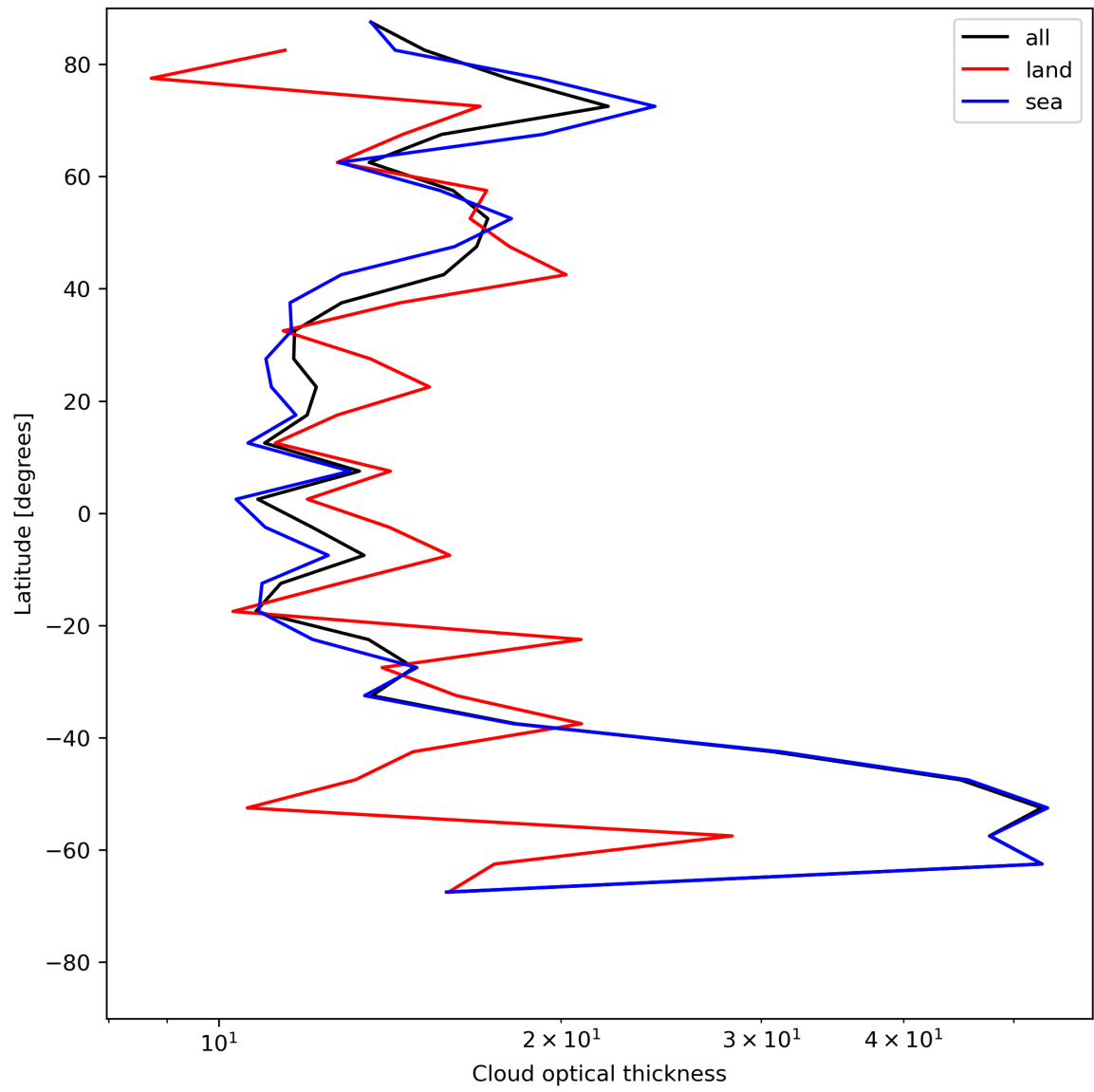
Figure 25: Zonal average of “Cloud optical thickness” for 2024-05-25 to 2024-05-27.
