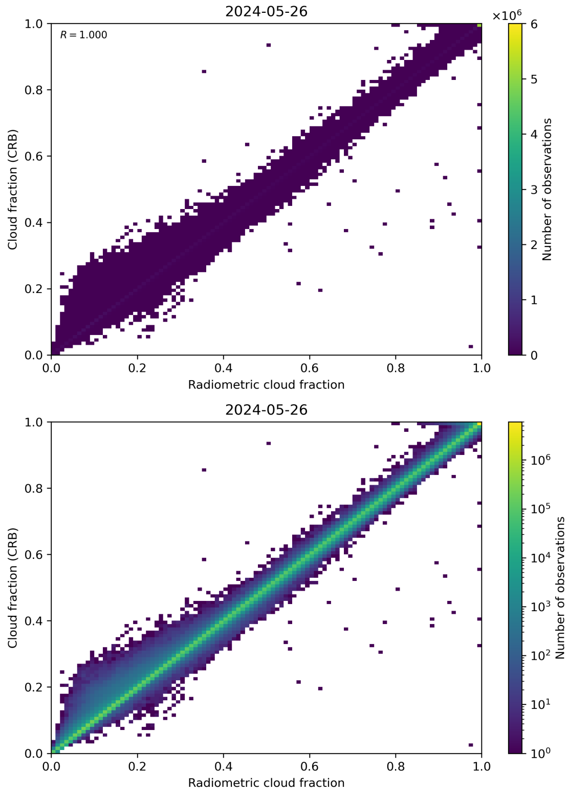
Figure 73: Scatter density plot of “Radiometric cloud fraction” against “Cloud fraction (CRB)” for 2024-05-25 to 2024-05-27.
