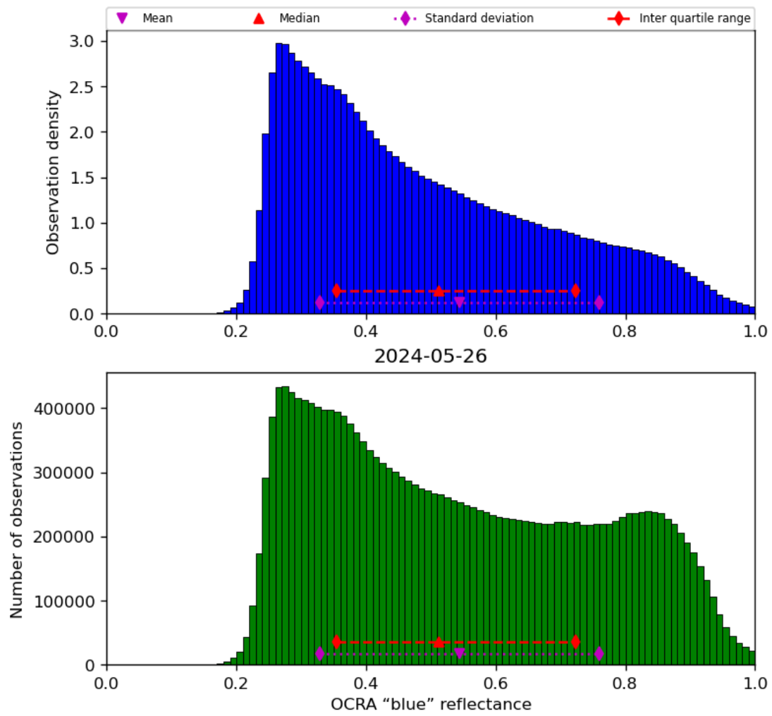
Figure 51: Histogram of “OCRA “blue” reflectance” for 2024-05-25 to 2024-05-27
