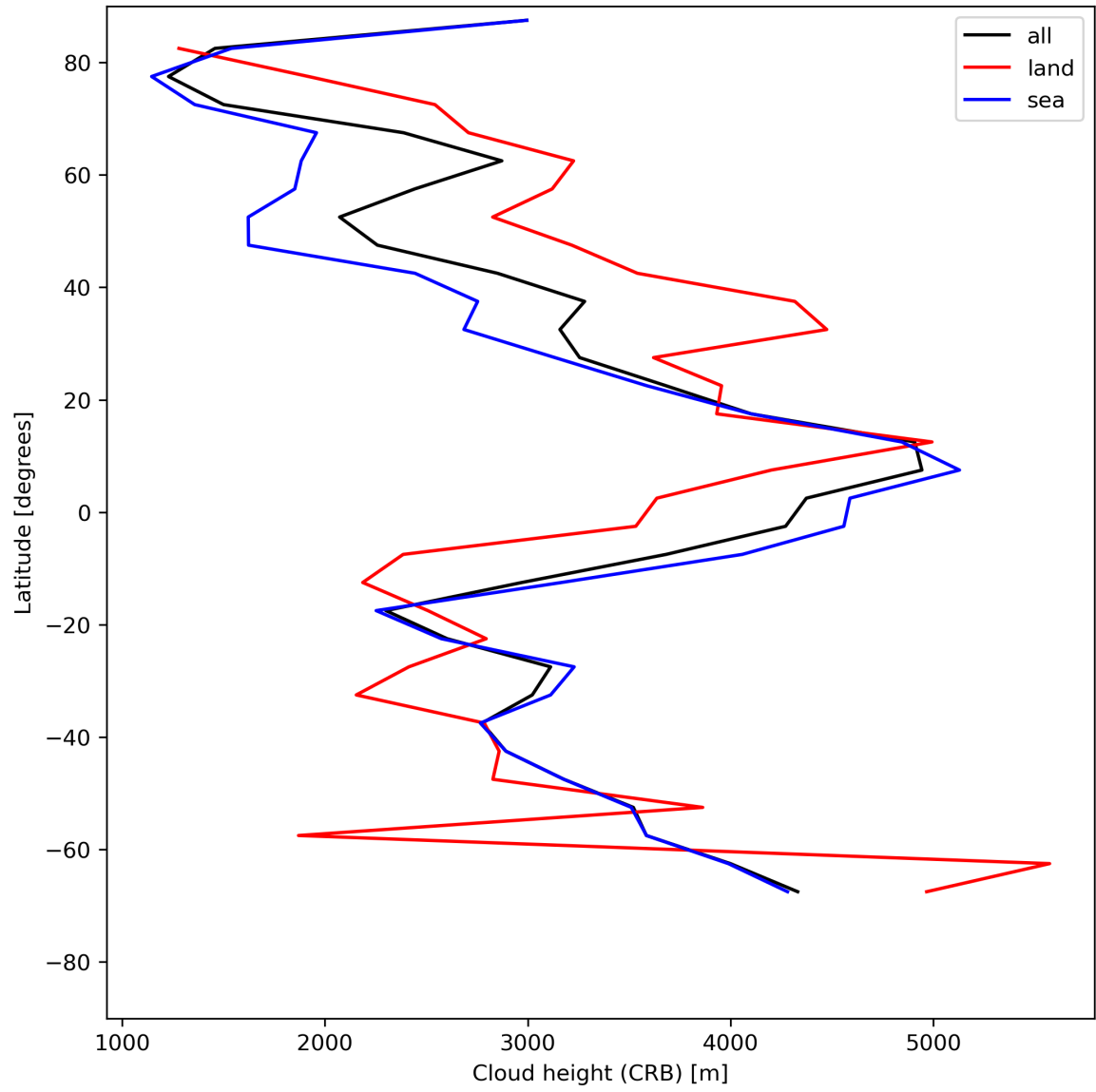
Figure 27: Zonal average of “Cloud height (CRB)” for 2024-05-25 to 2024-05-27.
