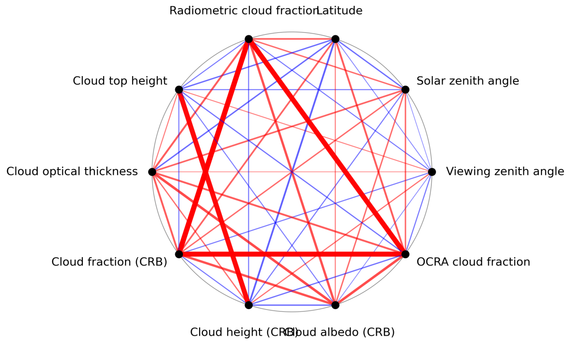
Figure 1: Map of correlation graph for 2024-05-25 to 2024-05-27.
