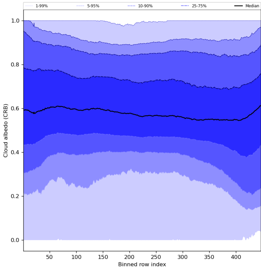
Figure 60: Along track statistics of “Cloud albedo (CRB)” for 2024-05-25 to 2024-05-27
