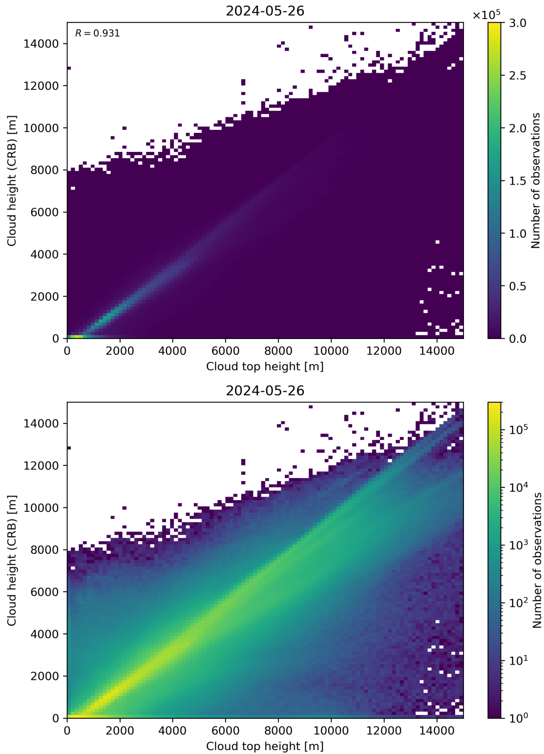
Figure 89: Scatter density plot of “Cloud top height” against “Cloud height (CRB)” for 2024-05-25 to 2024-05-27.
