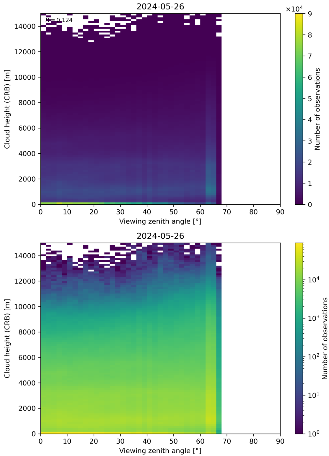
Figure 110: Scatter density plot of “Viewing zenith angle” against “Cloud height (CRB)” for 2024-05-25 to 2024-05-27.
