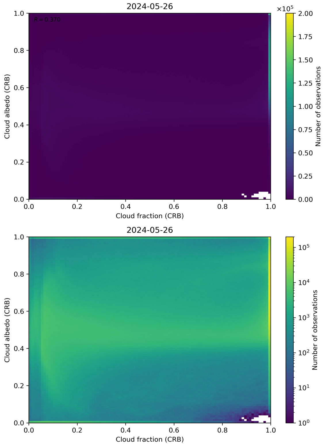
Figure 77: Scatter density plot of “Cloud fraction (CRB)” against “Cloud albedo (CRB)” for 2024-05-25 to 2024-05-27.
