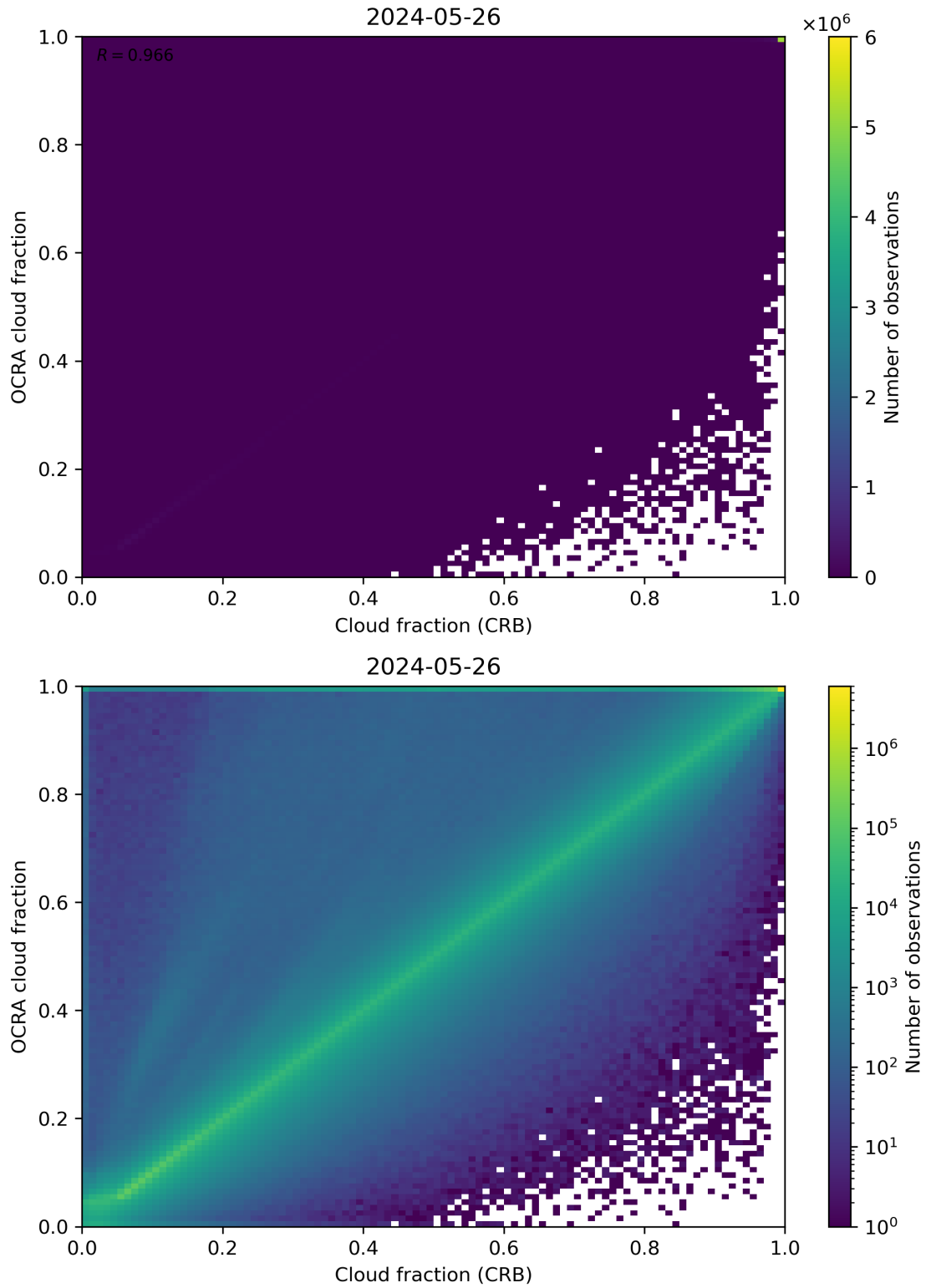
Figure 78: Scatter density plot of “Cloud fraction (CRB)” against “OCRA cloud fraction” for 2024-05-25 to 2024-05-27.
