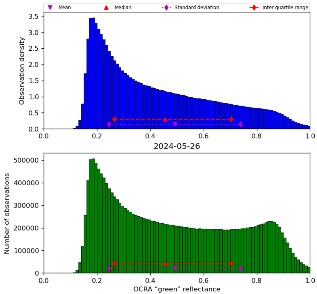
Figure 52: Histogram of “OCRA “green” reflectance” for 2024-05-25 to 2024-05-27
