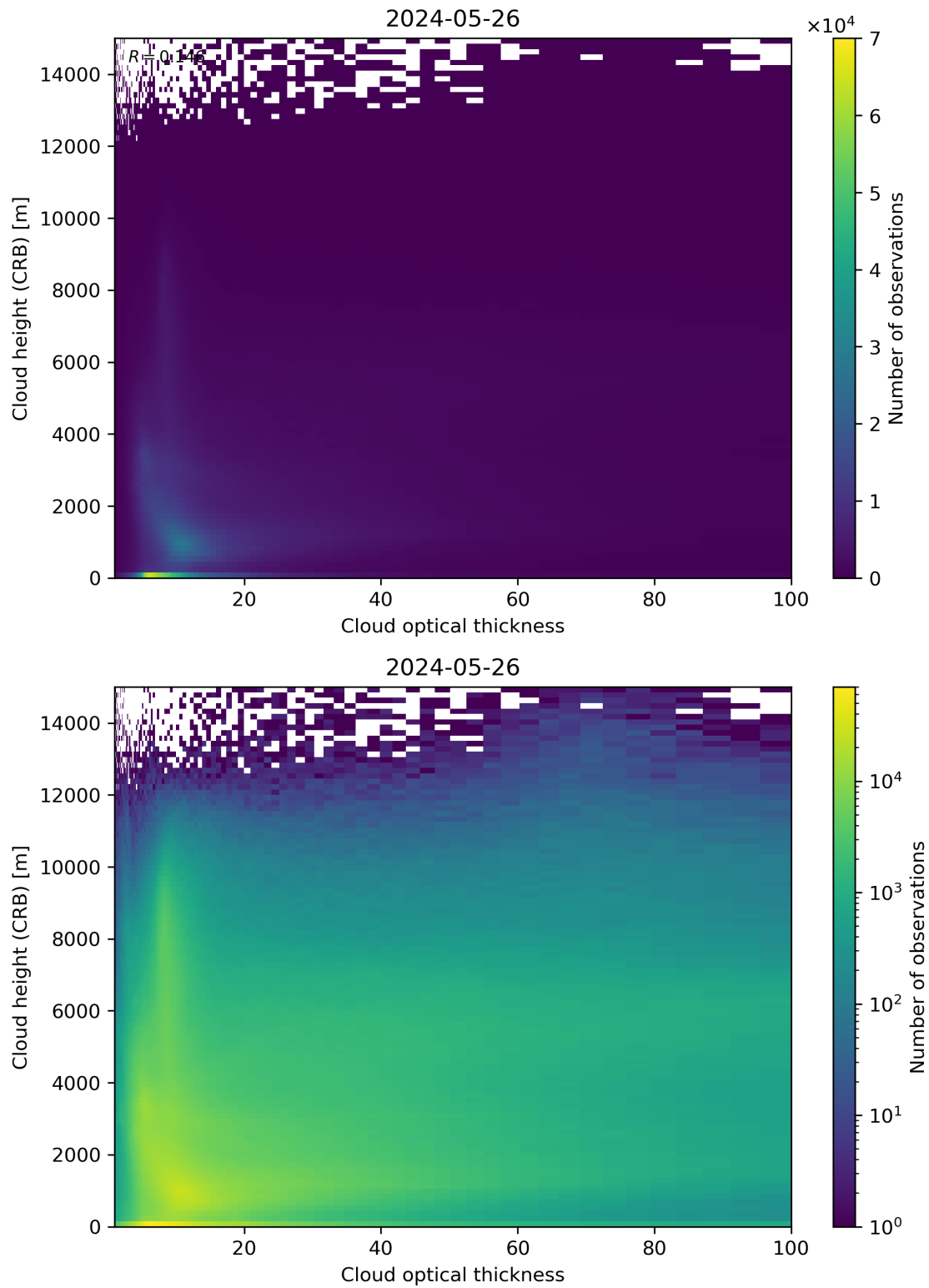
Figure 85: Scatter density plot of “Cloud optical thickness” against “Cloud height (CRB)” for 2024-05-25 to 2024-05-27.
