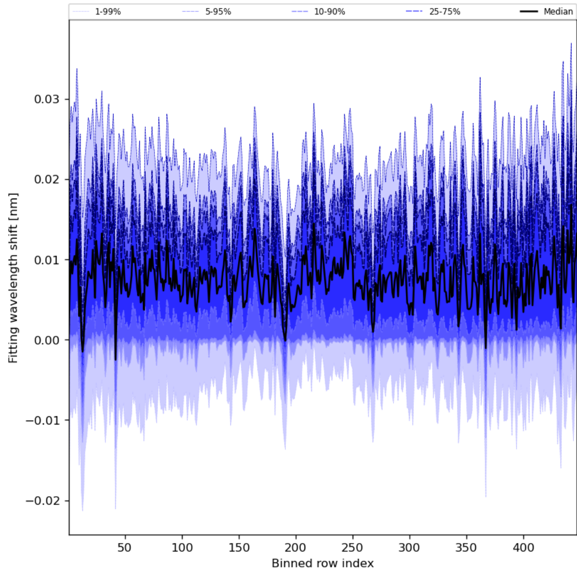
Figure 65: Along track statistics of “Fitting wavelength shift” for 2024-05-25 to 2024-05-27
