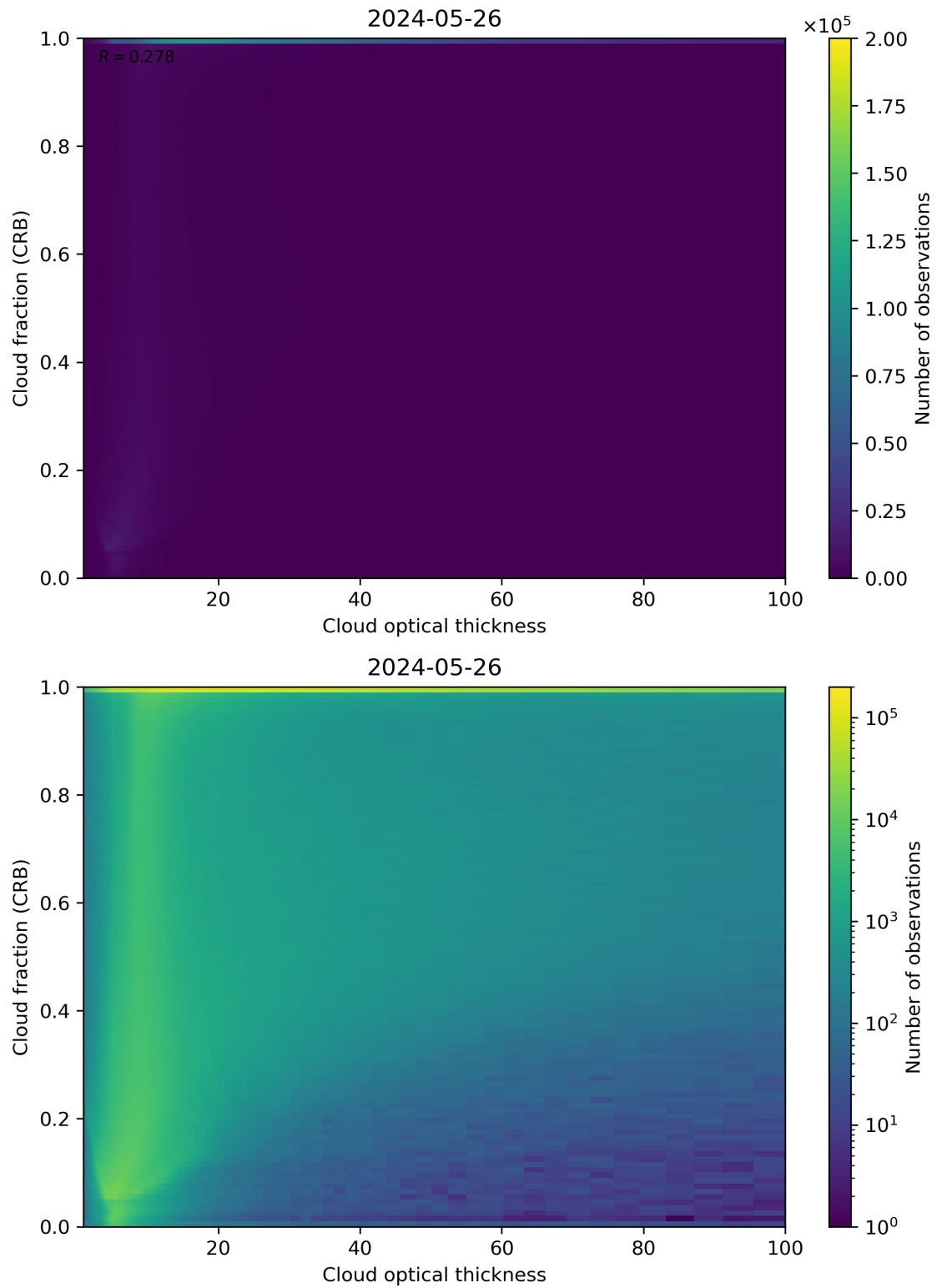
Figure 84: Scatter density plot of “Cloud optical thickness” against “Cloud fraction (CRB)” for 2024-05-25 to 2024-05-27.
