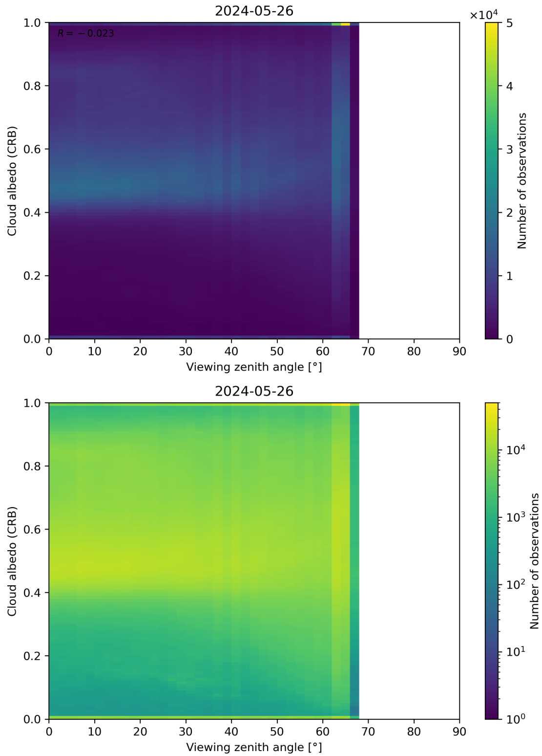
Figure 106: Scatter density plot of “Viewing zenith angle” against “Cloud albedo (CRB)” for 2024-05-25 to 2024-05-27.
