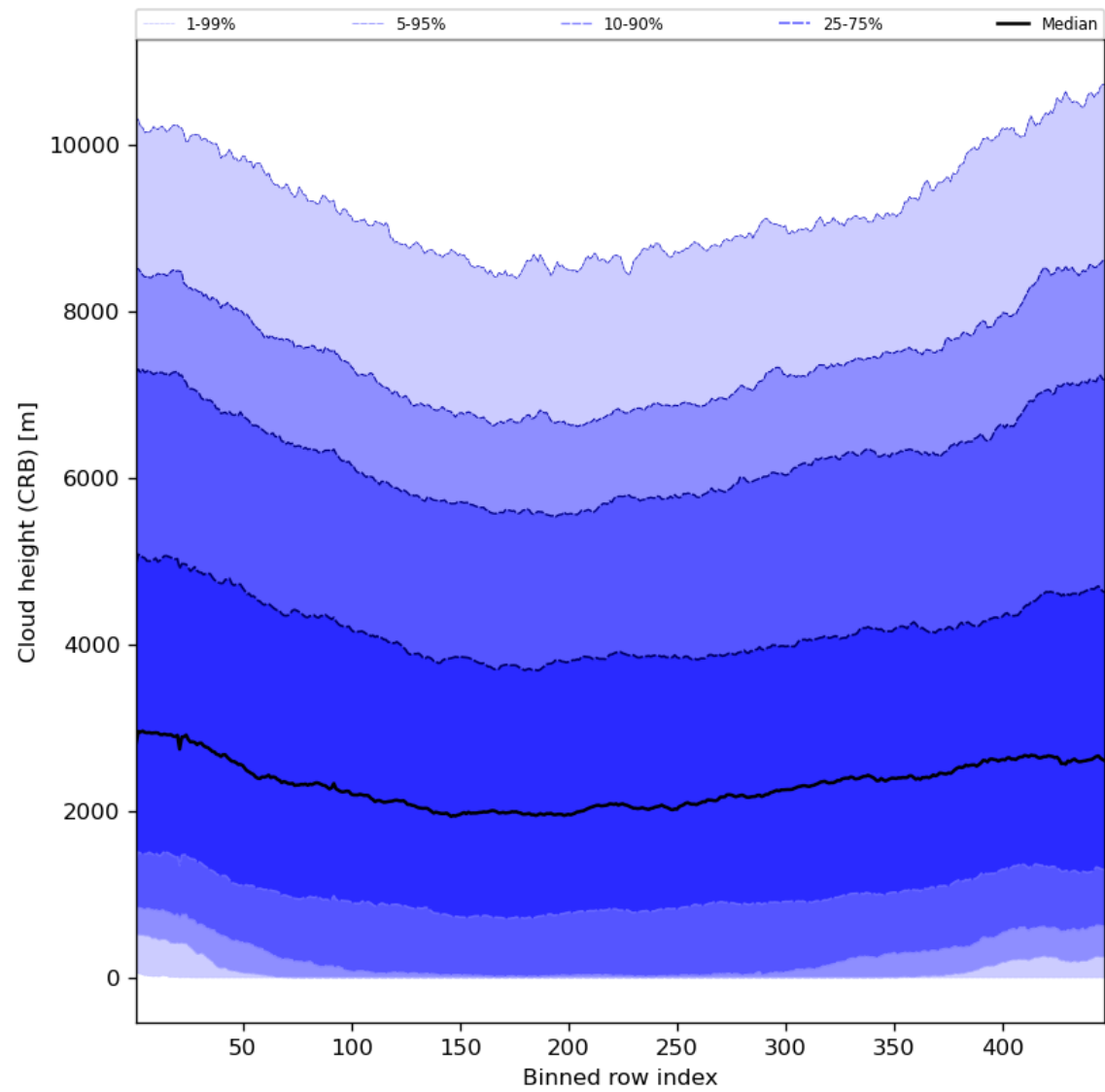
Figure 59: Along track statistics of “Cloud height (CRB)” for 2024-05-25 to 2024-05-27
