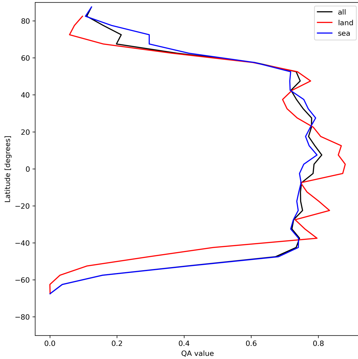
Figure 22: Zonal average of “QA value” for 2024-05-25 to 2024-05-27.
