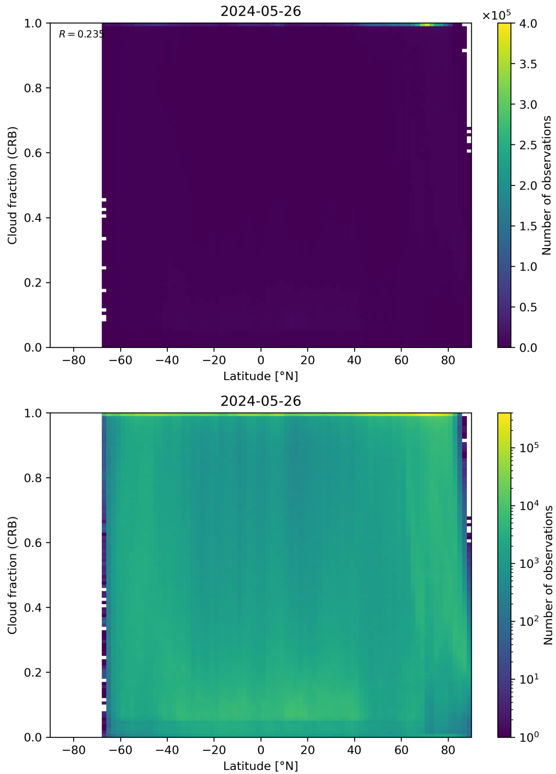
Figure 94: Scatter density plot of “Latitude” against “Cloud fraction (CRB)” for 2024-05-25 to 2024-05-27.
