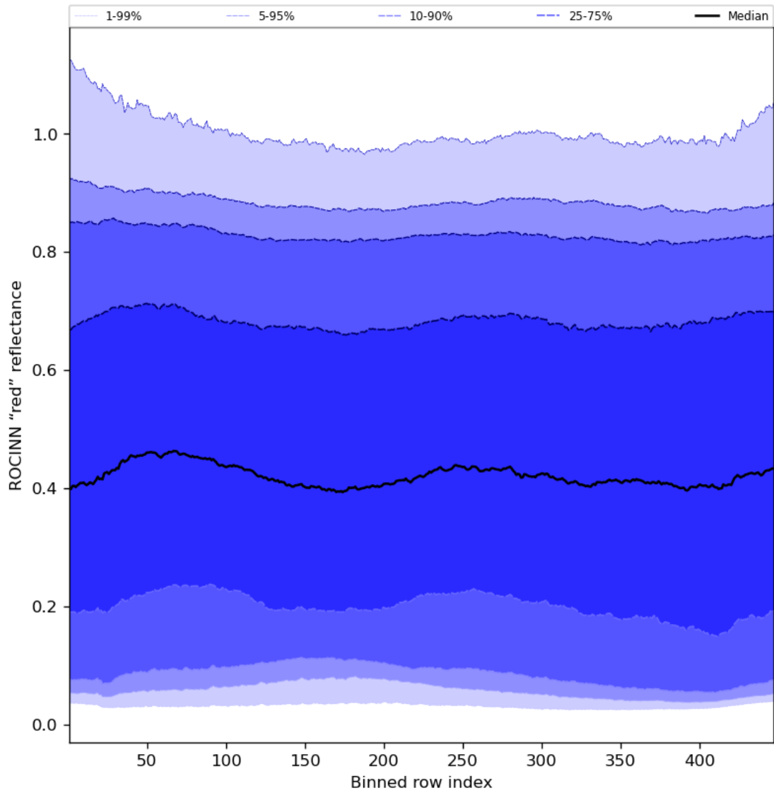
Figure 69: Along track statistics of "ROCINN "red" reflectance" for 2024-05-25 to 2024-05-27
