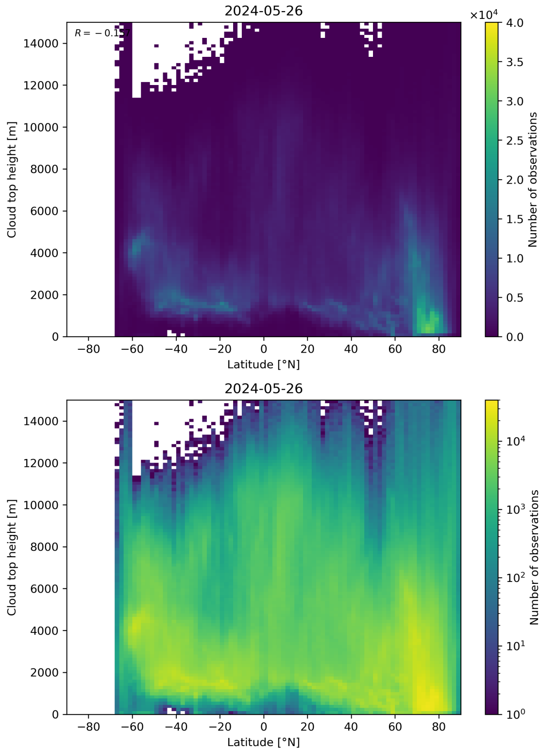
Figure 97: Scatter density plot of “Latitude” against “Cloud top height” for 2024-05-25 to 2024-05-27.
