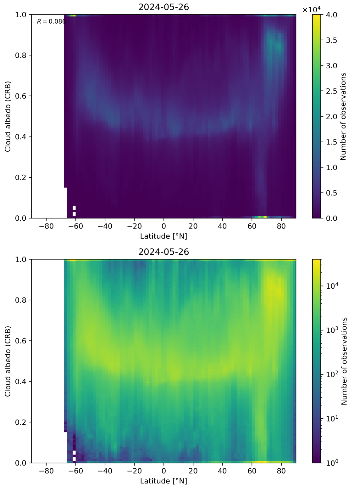
Figure 91: Scatter density plot of “Latitude” against “Cloud albedo (CRB)” for 2024-05-25 to 2024-05-27.
