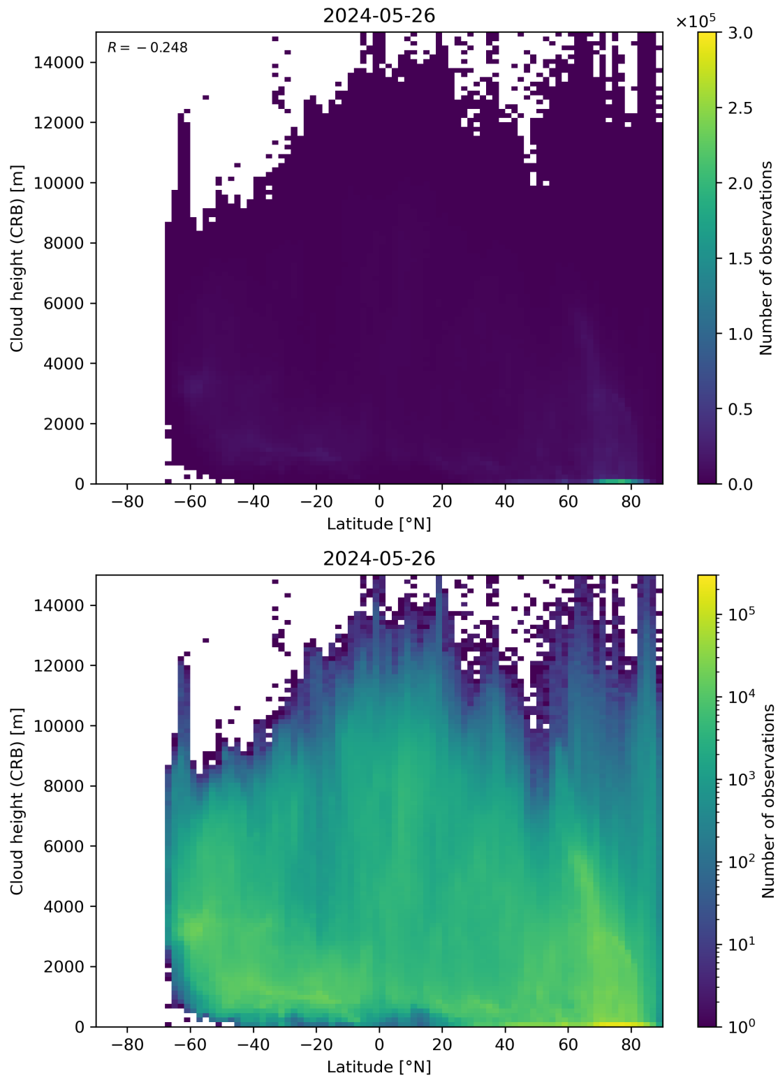
Figure 95: Scatter density plot of “Latitude” against “Cloud height (CRB)” for 2024-05-25 to 2024-05-27.
