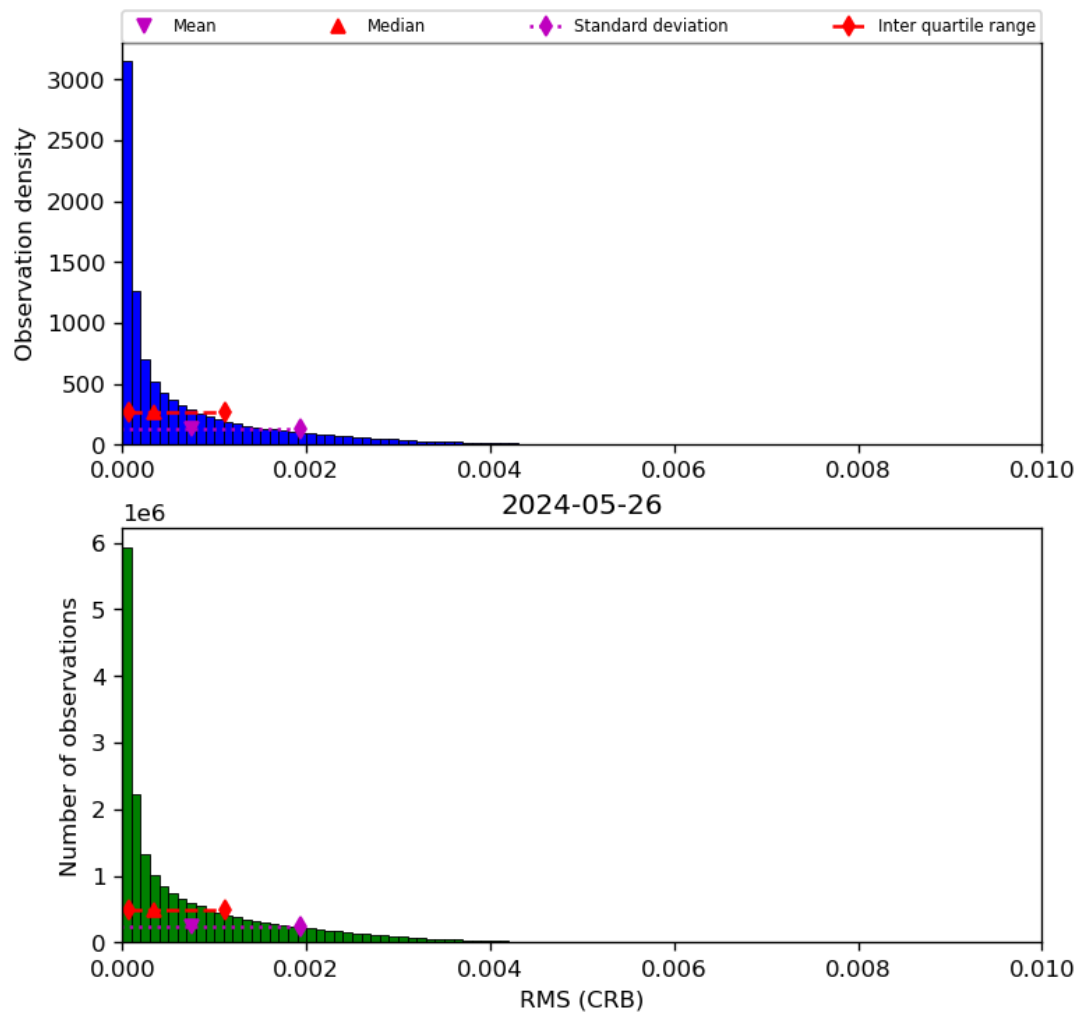
Figure 48: Histogram of “RMS (CRB)” for 2024-05-25 to 2024-05-27
