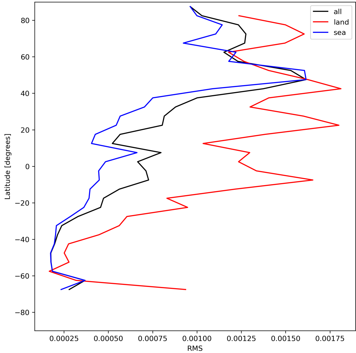
Figure 31: Zonal average of “RMS” for 2024-05-25 to 2024-05-27.
