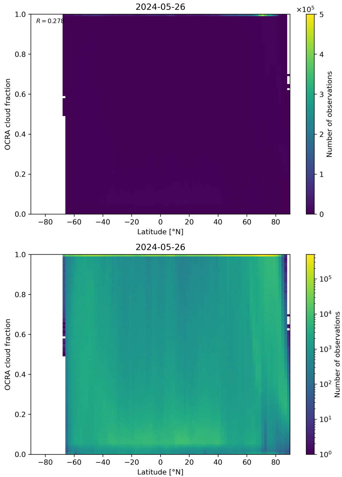
Figure 93: Scatter density plot of “Latitude” against “OCRA cloud fraction” for 2024-05-25 to 2024-05-27.
