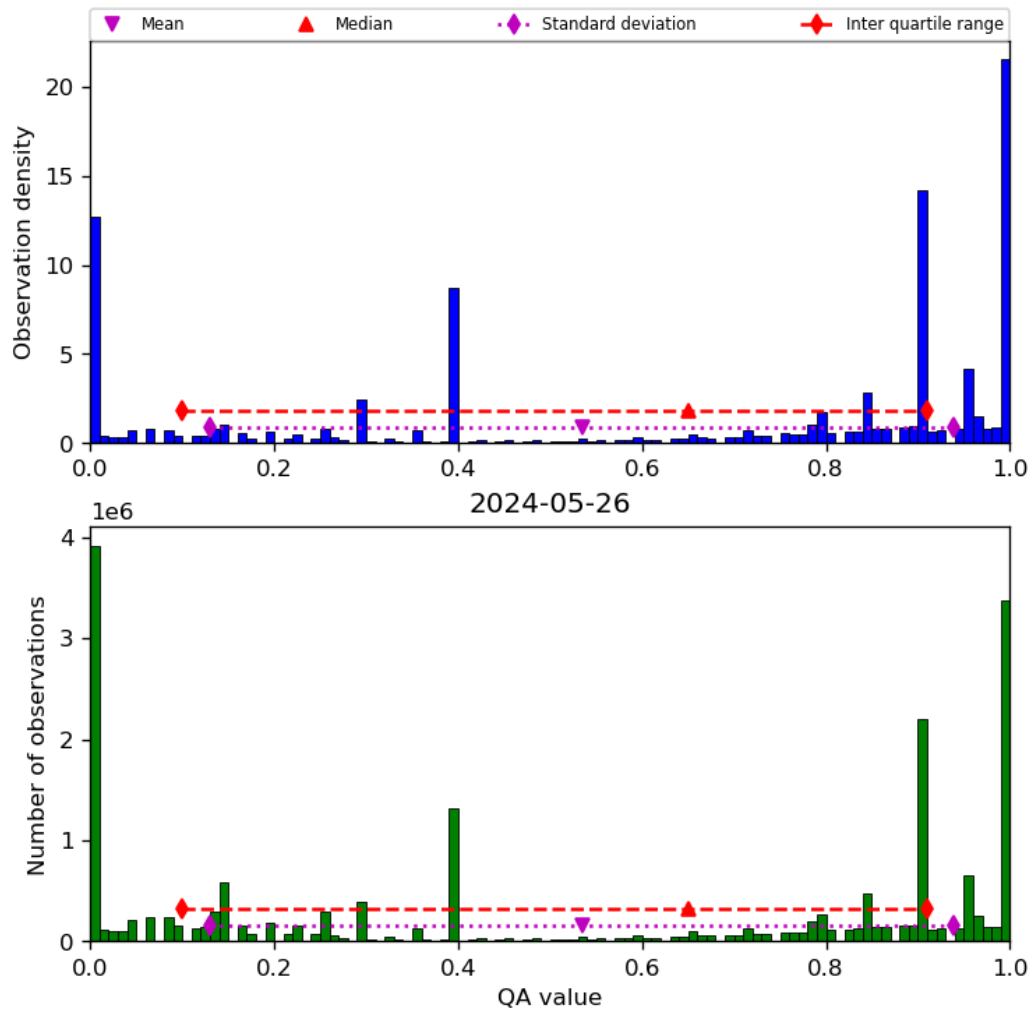
Figure 38: Histogram of “QA value” for 2024-05-25 to 2024-05-27
