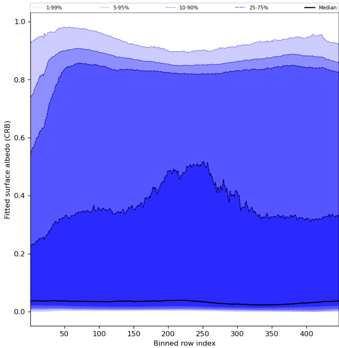
Figure 62: Along track statistics of “Fitted surface albedo (CRB)” for 2024-05-25 to 2024-05-27
