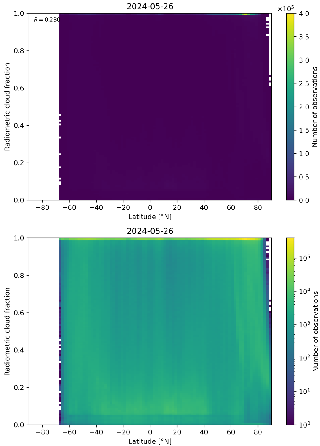
Figure 92: Scatter density plot of “Latitude” against “Radiometric cloud fraction” for 2024-05-25 to 2024-05-27.
