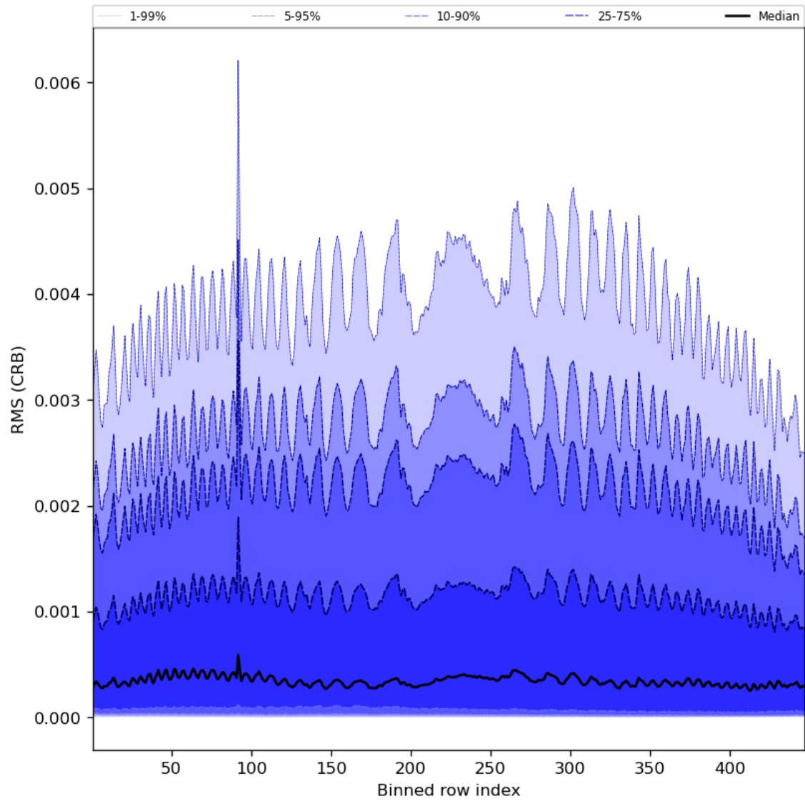
Figure 64: Along track statistics of “RMS (CRB)” for 2024-05-25 to 2024-05-27
