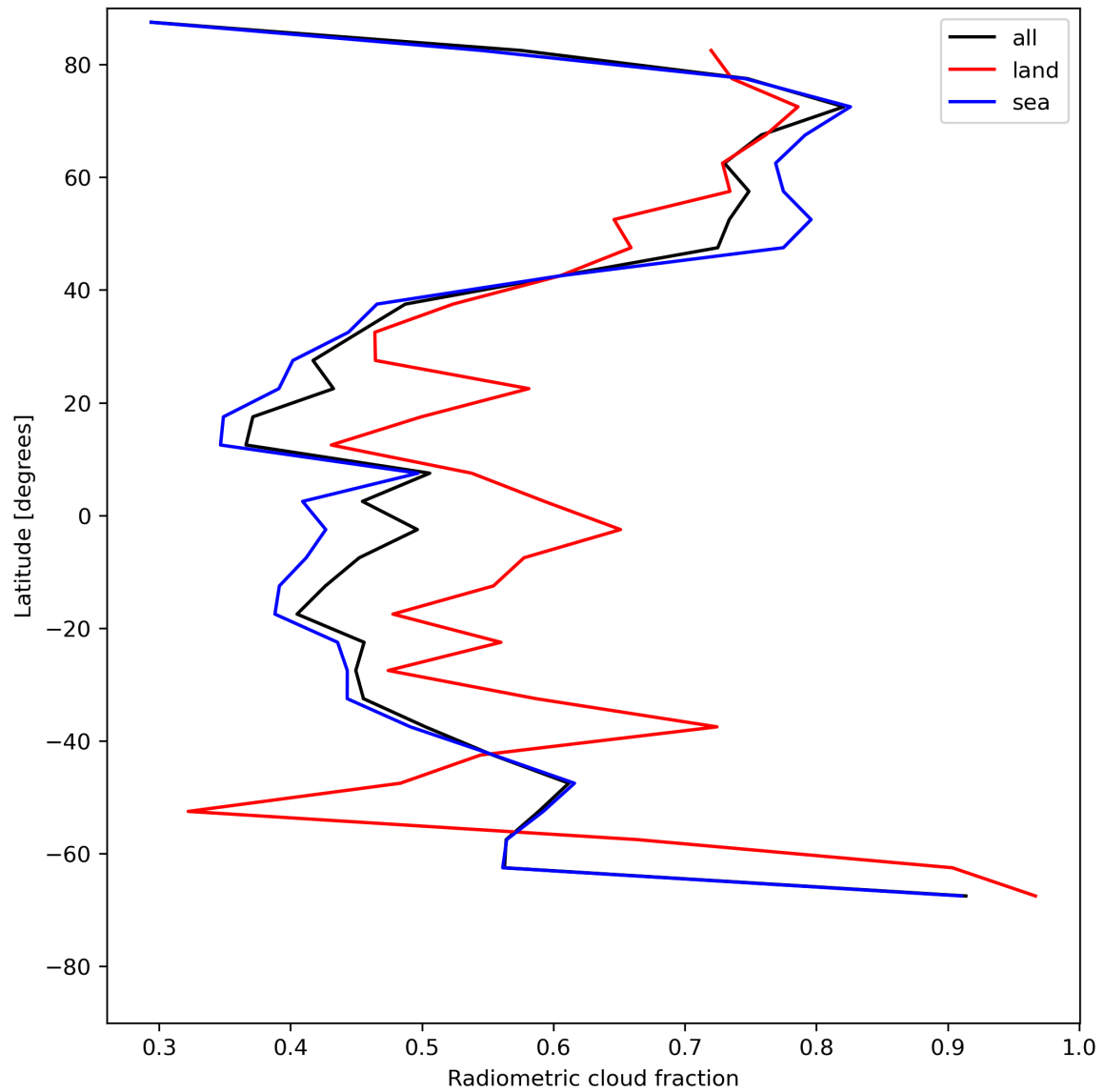
Figure 23: Zonal average of “Radiometric cloud fraction” for 2024-05-25 to 2024-05-27.
