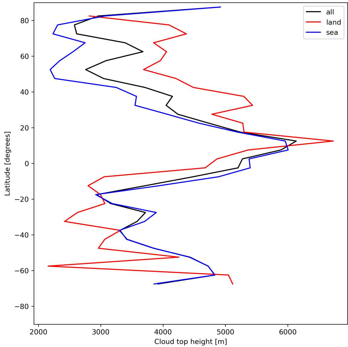
Figure 24: Zonal average of “Cloud top height” for 2024-05-25 to 2024-05-27.
