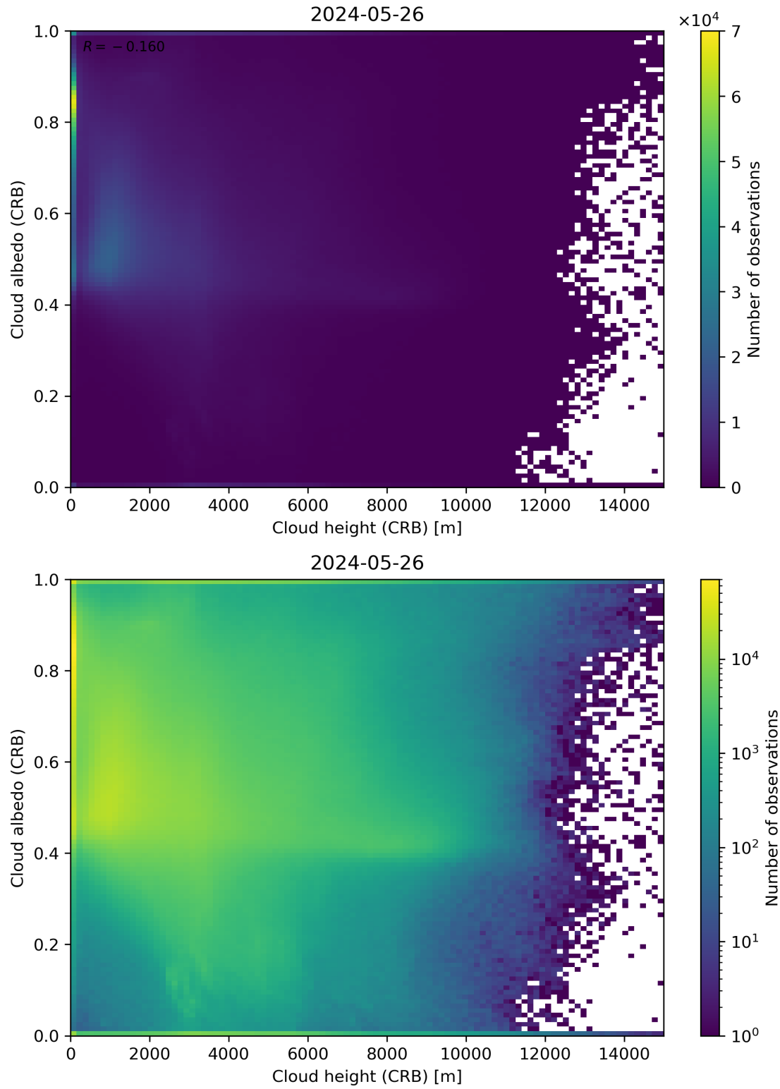
Figure 80: Scatter density plot of “Cloud height (CRB)” against “Cloud albedo (CRB)” for 2024-05-25 to 2024-05-27.
