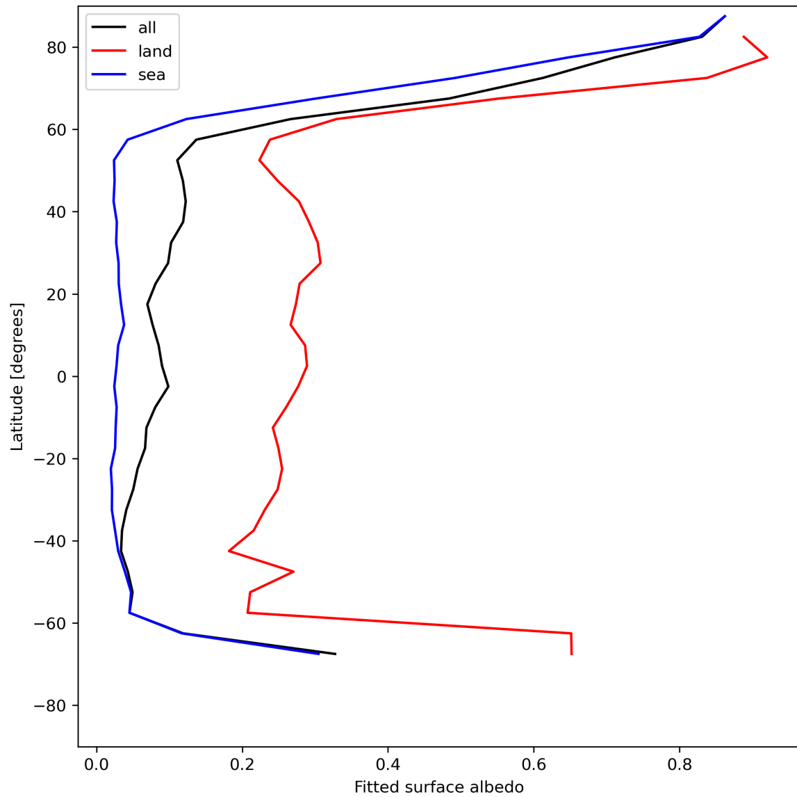
Figure 29: Zonal average of “Fitted surface albedo” for 2024-05-25 to 2024-05-27.
