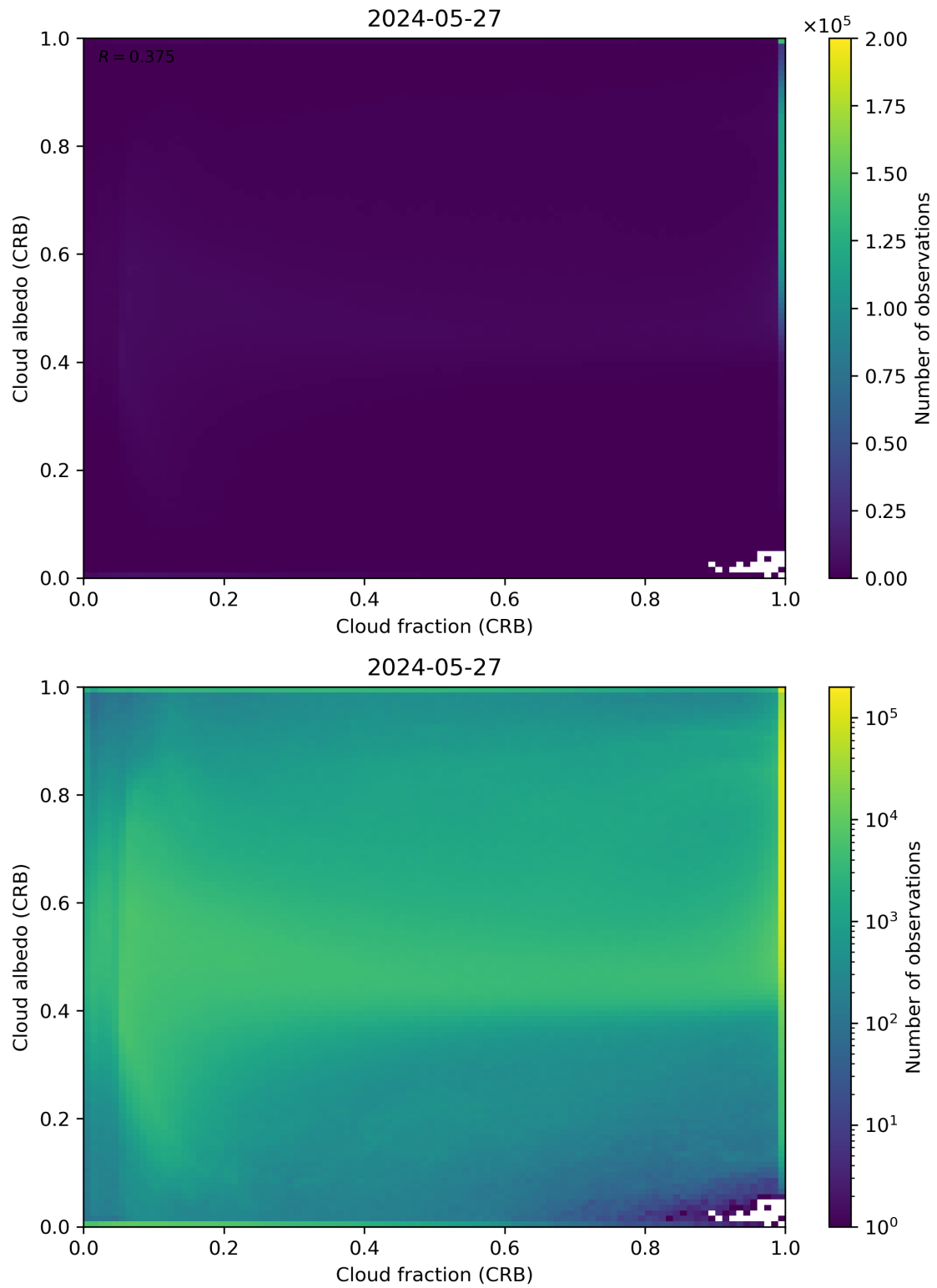
Figure 77: Scatter density plot of “Cloud fraction (CRB)” against “Cloud albedo (CRB)” for 2024-05-26 to 2024-05-28.
