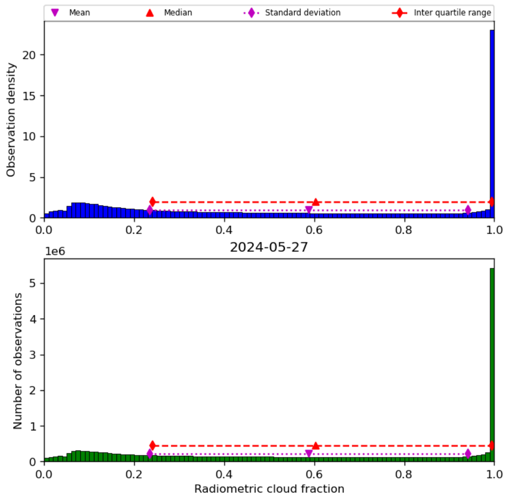
Figure 39: Histogram of “Radiometric cloud fraction” for 2024-05-26 to 2024-05-28
