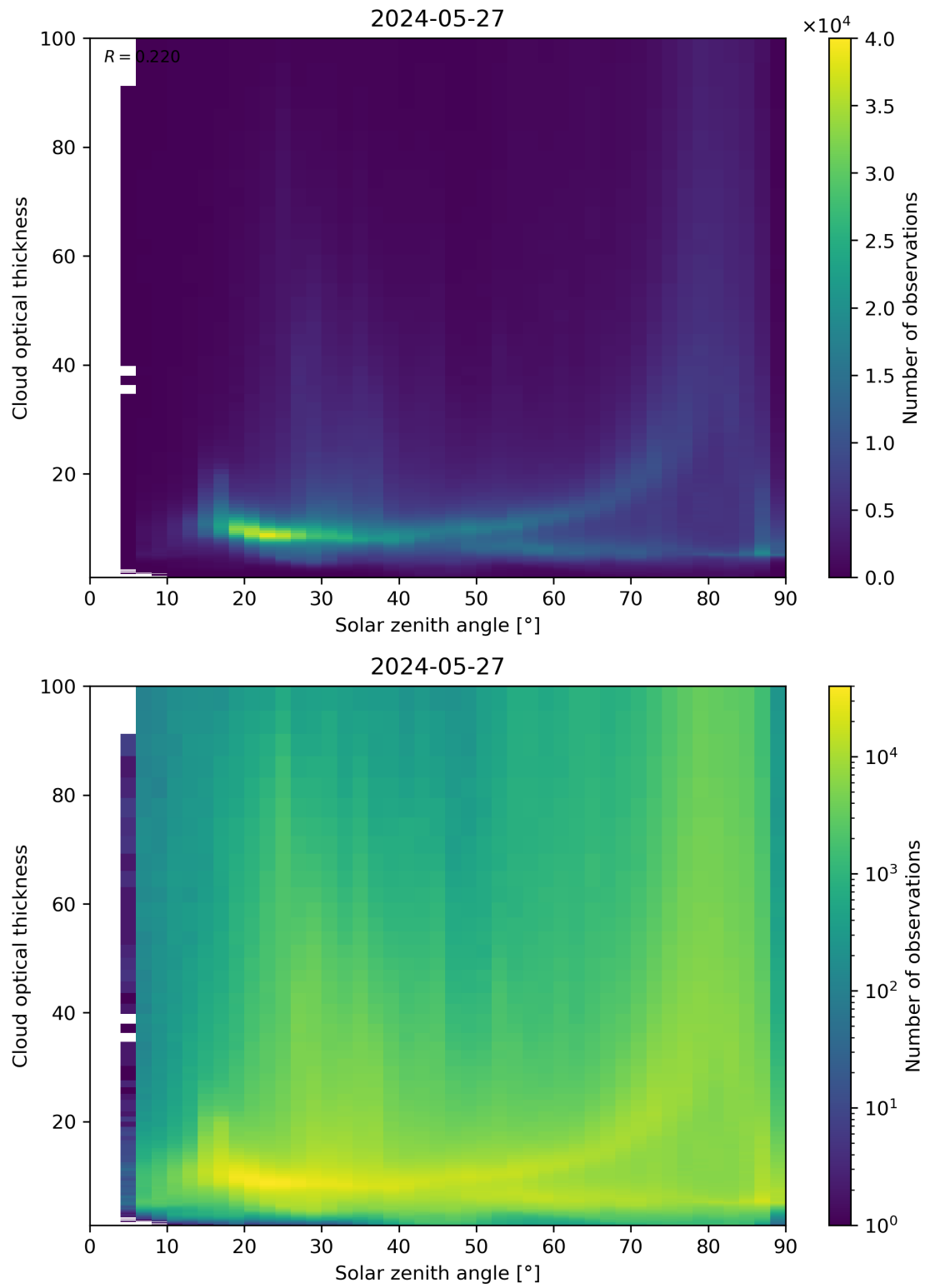
Figure 103: Scatter density plot of “Solar zenith angle” against “Cloud optical thickness” for 2024-05-26 to 2024-05-28.
