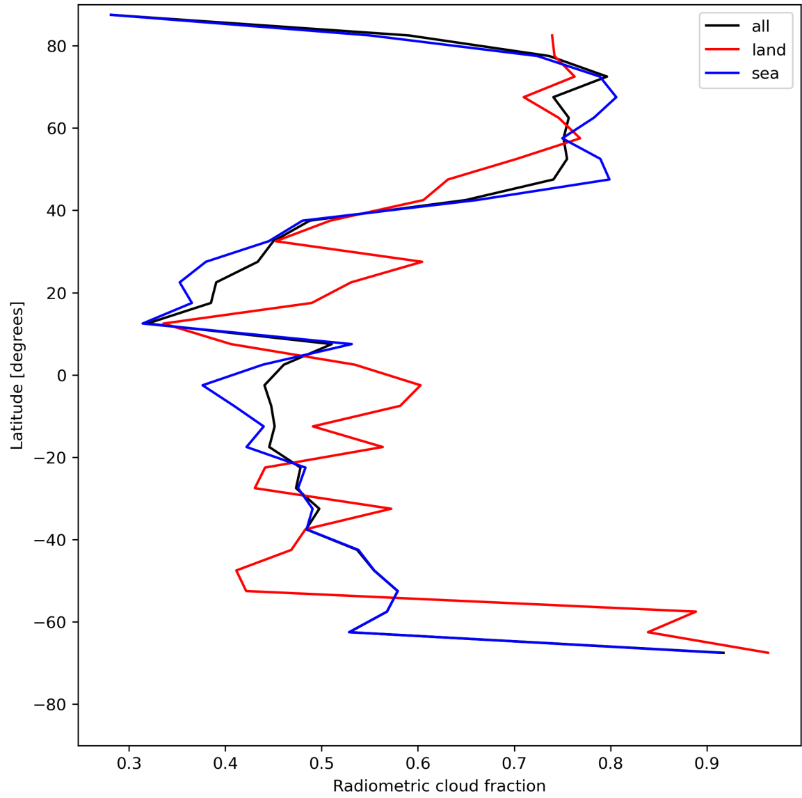
Figure 23: Zonal average of “Radiometric cloud fraction” for 2024-05-26 to 2024-05-28.
