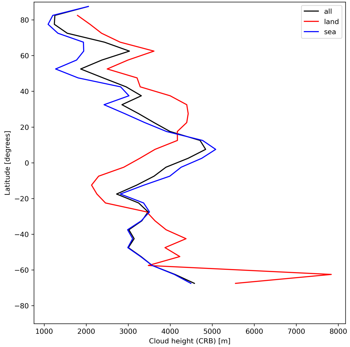
Figure 27: Zonal average of “Cloud height (CRB)” for 2024-05-26 to 2024-05-28.
