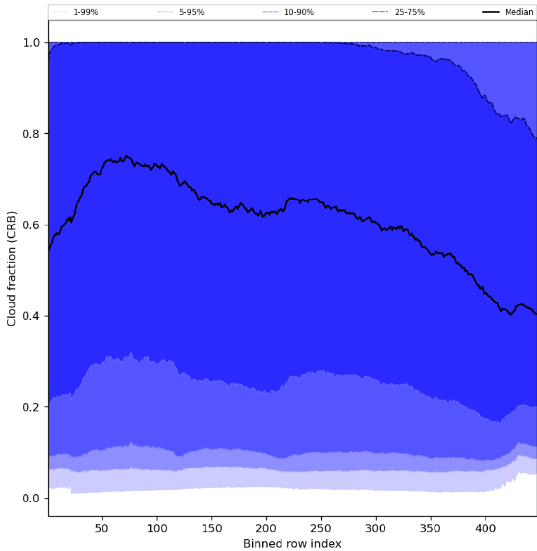
Figure 58: Along track statistics of “Cloud fraction (CRB)” for 2024-05-26 to 2024-05-28
