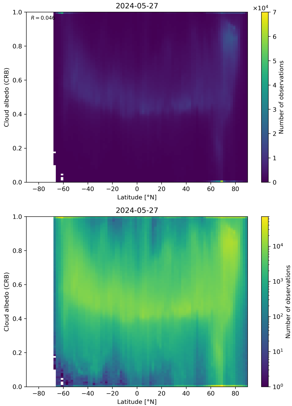
Figure 91: Scatter density plot of “Latitude” against “Cloud albedo (CRB)” for 2024-05-26 to 2024-05-28.
