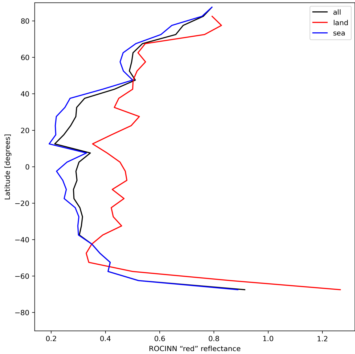
Figure 37: Zonal average of “ROCINN “red” reflectance” for 2024-05-26 to 2024-05-28.
