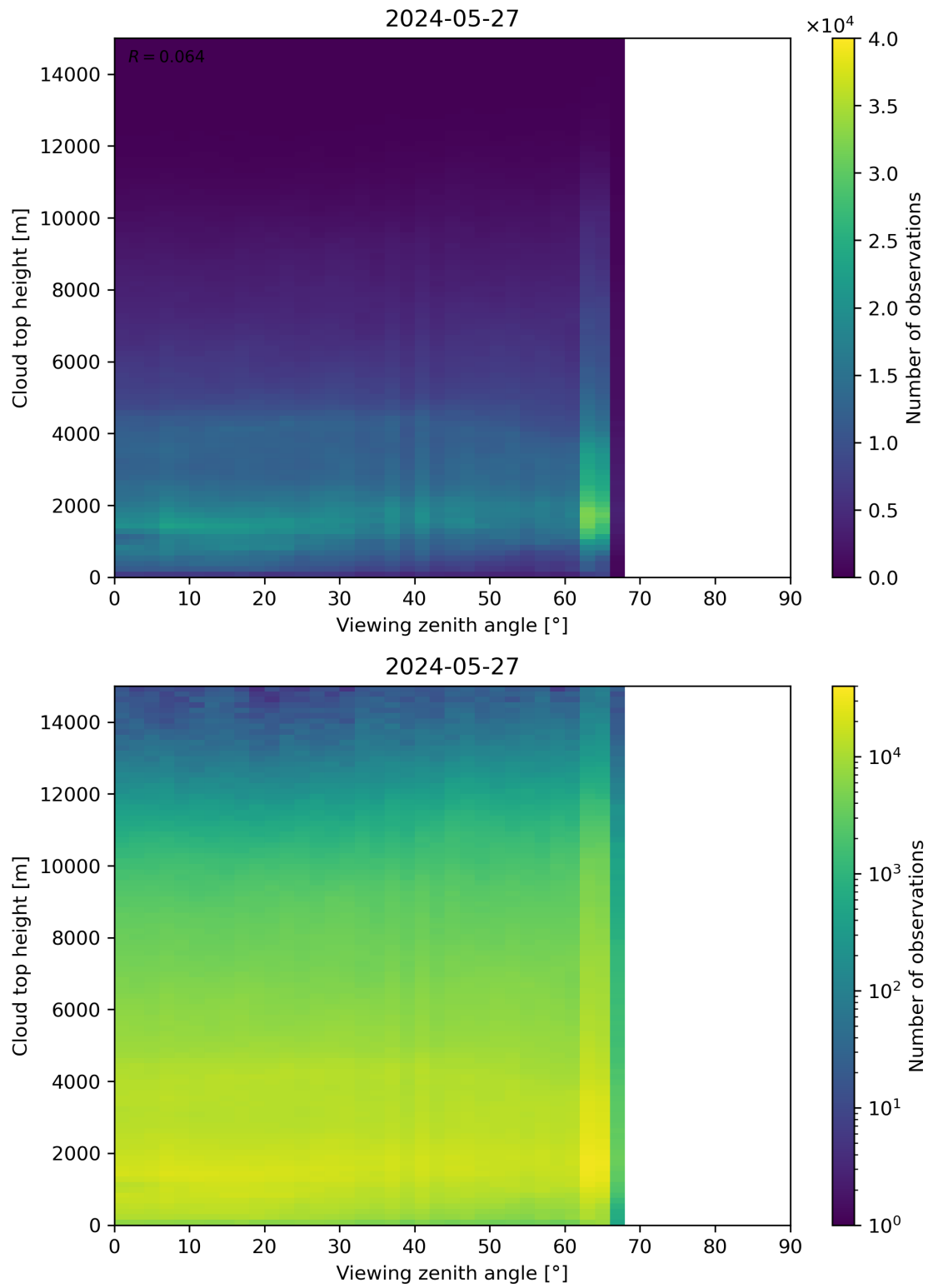
Figure 112: Scatter density plot of “Viewing zenith angle” against “Cloud top height” for 2024-05-26 to 2024-05-28.
