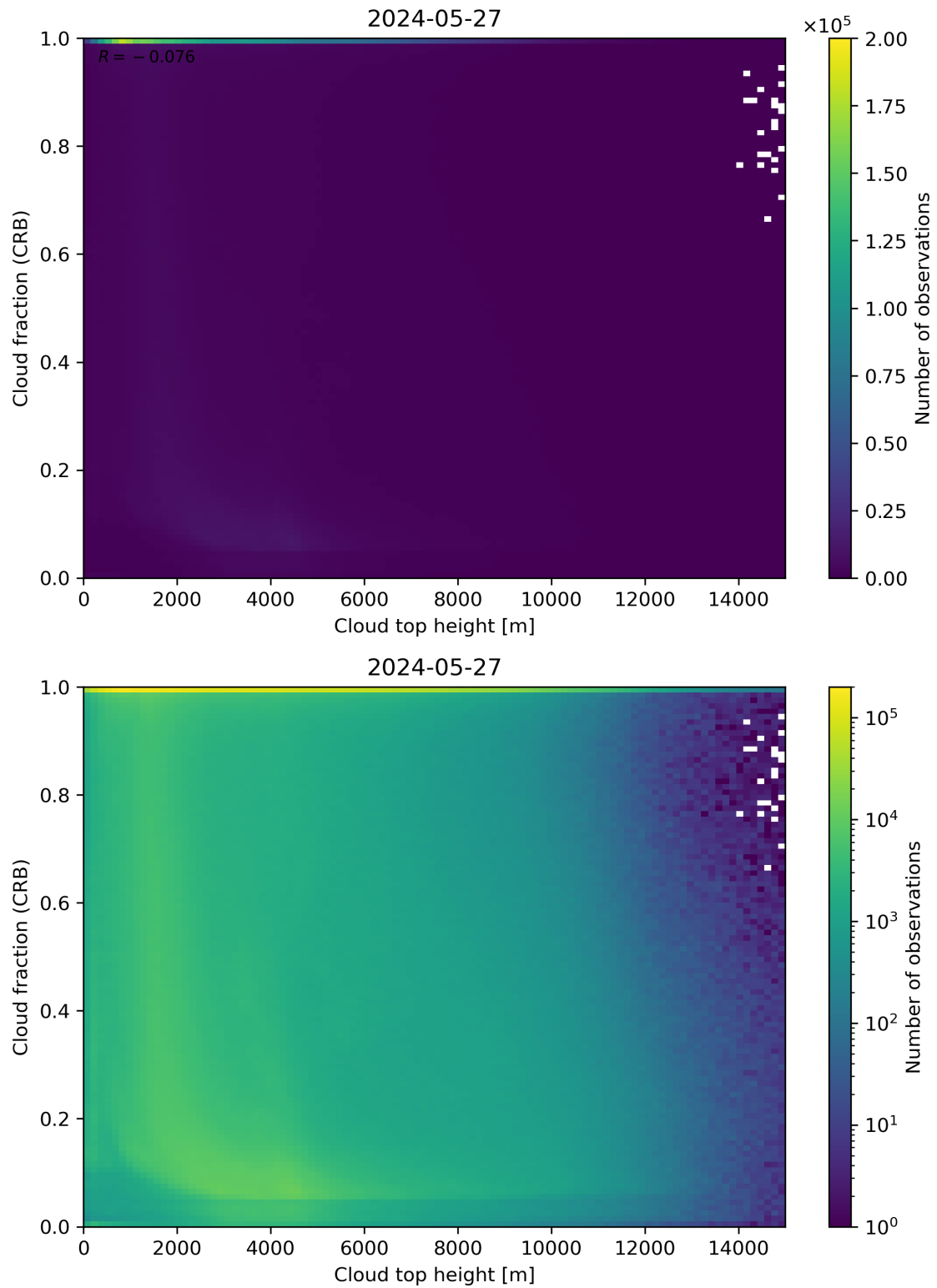
Figure 88: Scatter density plot of “Cloud top height” against “Cloud fraction (CRB)” for 2024-05-26 to 2024-05-28.
