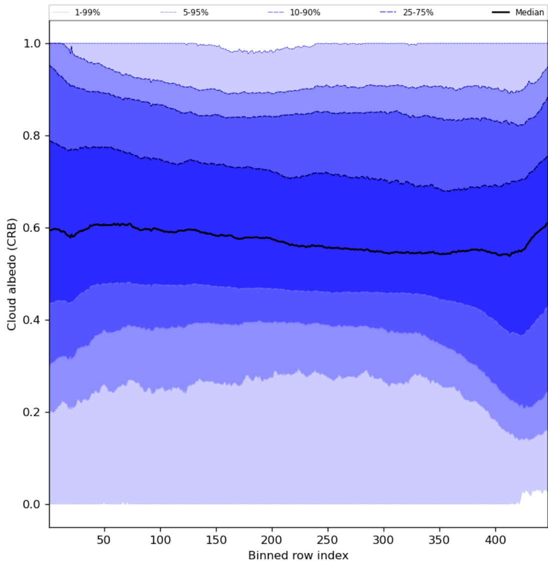
Figure 60: Along track statistics of “Cloud albedo (CRB)” for 2024-05-26 to 2024-05-28
