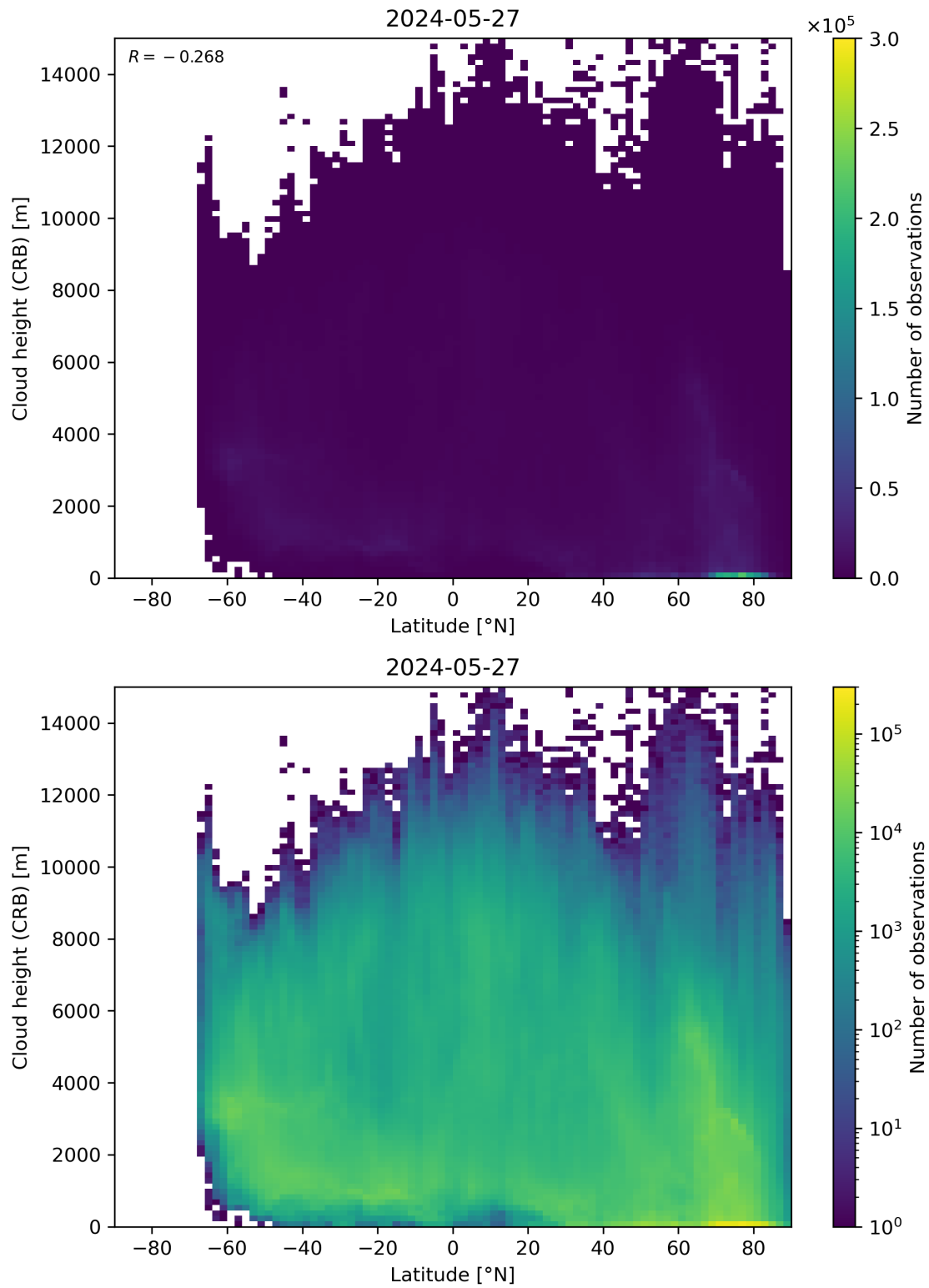
Figure 95: Scatter density plot of “Latitude” against “Cloud height (CRB)” for 2024-05-26 to 2024-05-28.
