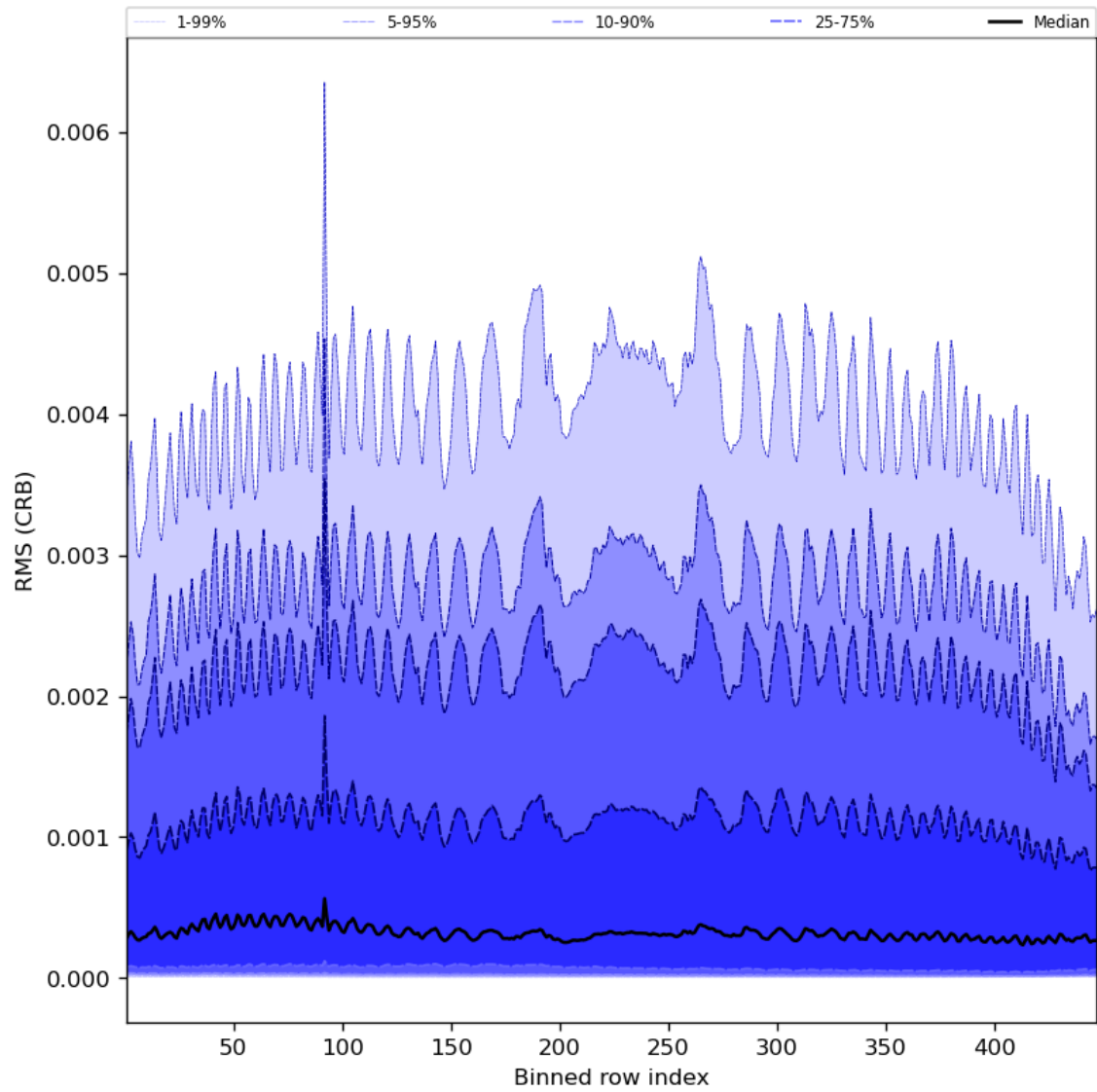
Figure 64: Along track statistics of “RMS (CRB)” for 2024-05-26 to 2024-05-28
