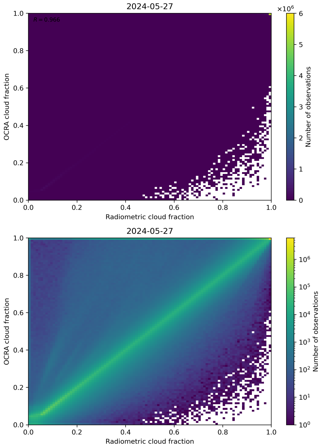
Figure 72: Scatter density plot of “Radiometric cloud fraction” against “OCRA cloud fraction” for 2024-05-26 to 2024-05-28.
