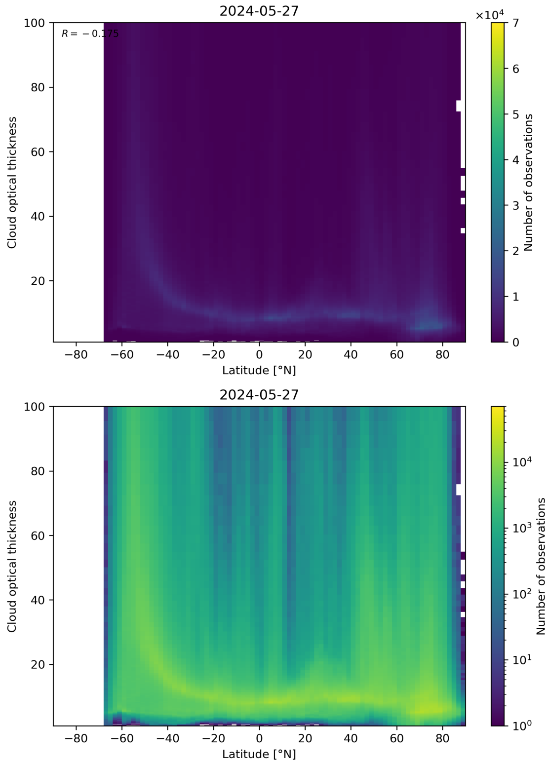
Figure 96: Scatter density plot of “Latitude” against “Cloud optical thickness” for 2024-05-26 to 2024-05-28.
