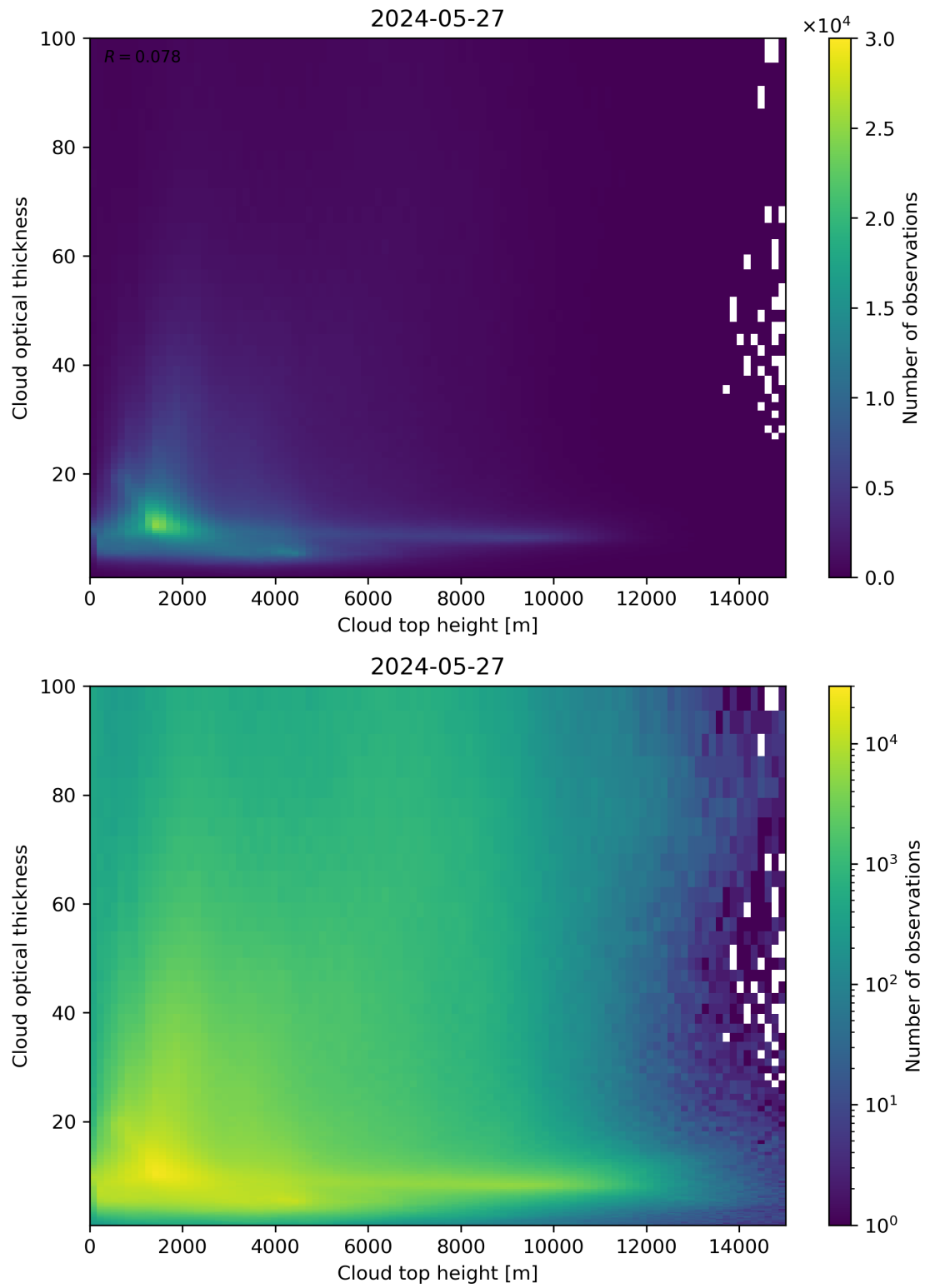
Figure 90: Scatter density plot of “Cloud top height” against “Cloud optical thickness” for 2024-05-26 to 2024-05-28.
