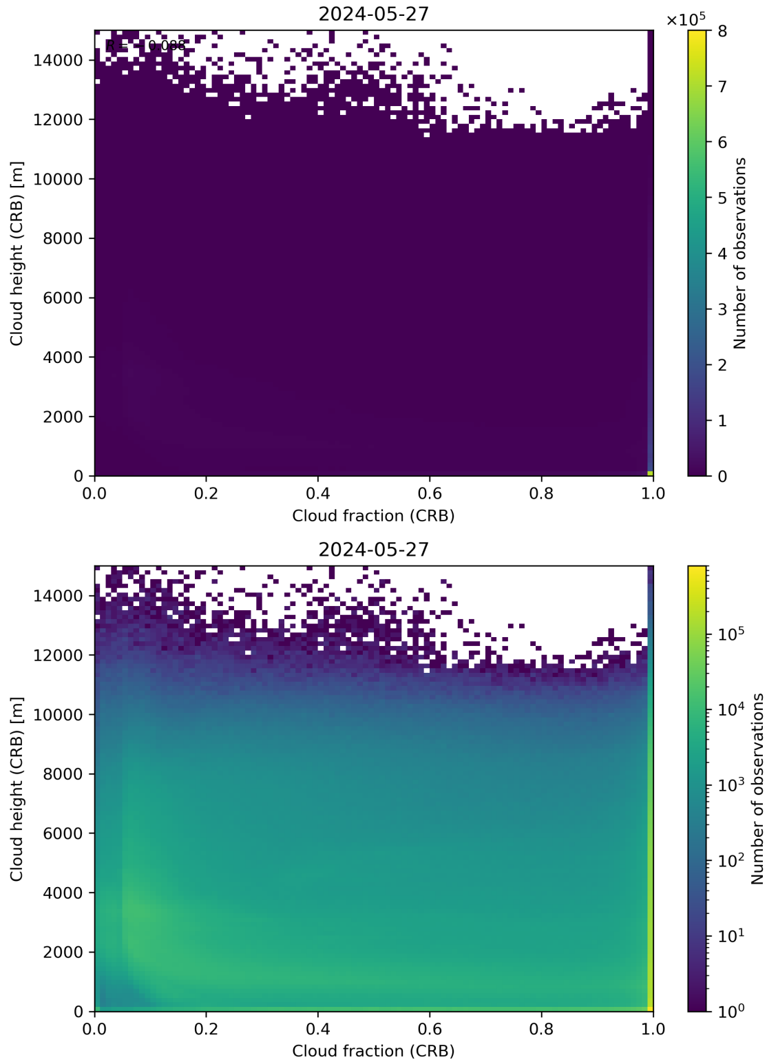
Figure 79: Scatter density plot of “Cloud fraction (CRB)” against “Cloud height (CRB)” for 2024-05-26 to 2024-05-28.
