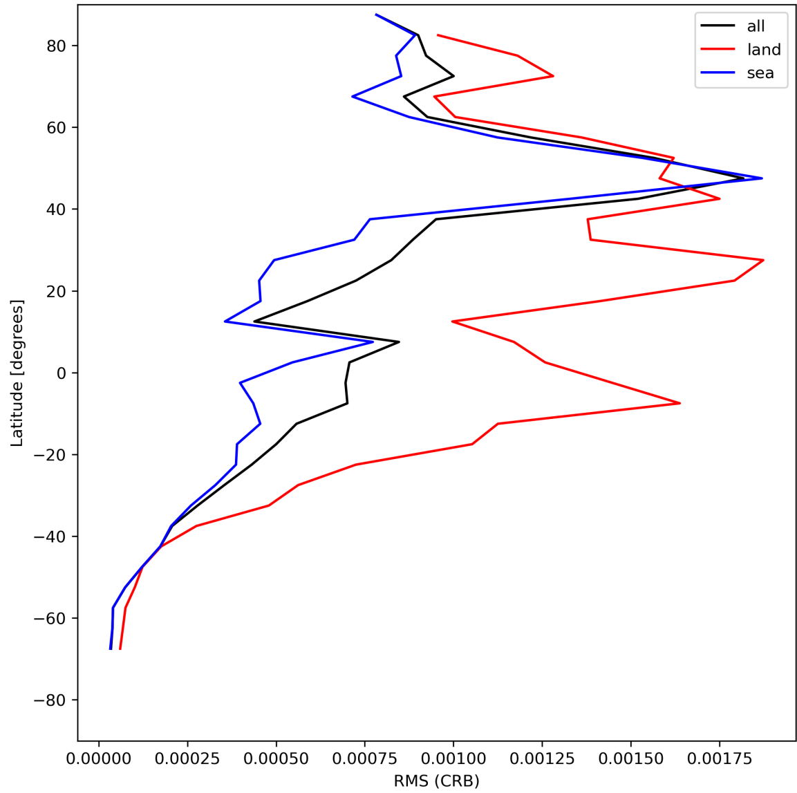
Figure 32: Zonal average of “RMS (CRB)” for 2024-05-26 to 2024-05-28.
