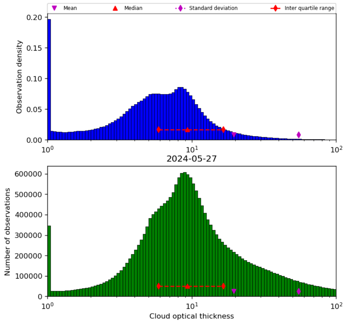
Figure 41: Histogram of “Cloud optical thickness” for 2024-05-26 to 2024-05-28
