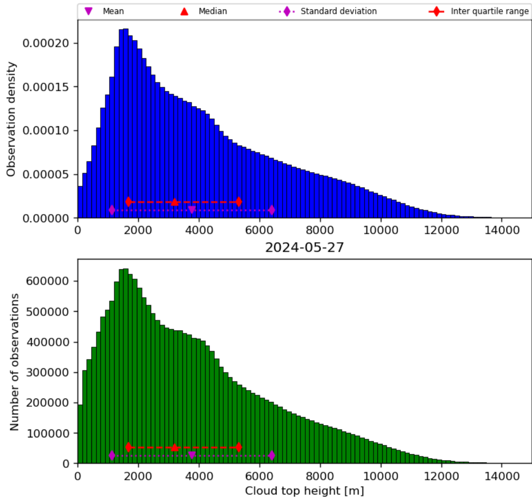
Figure 40: Histogram of “Cloud top height” for 2024-05-26 to 2024-05-28
