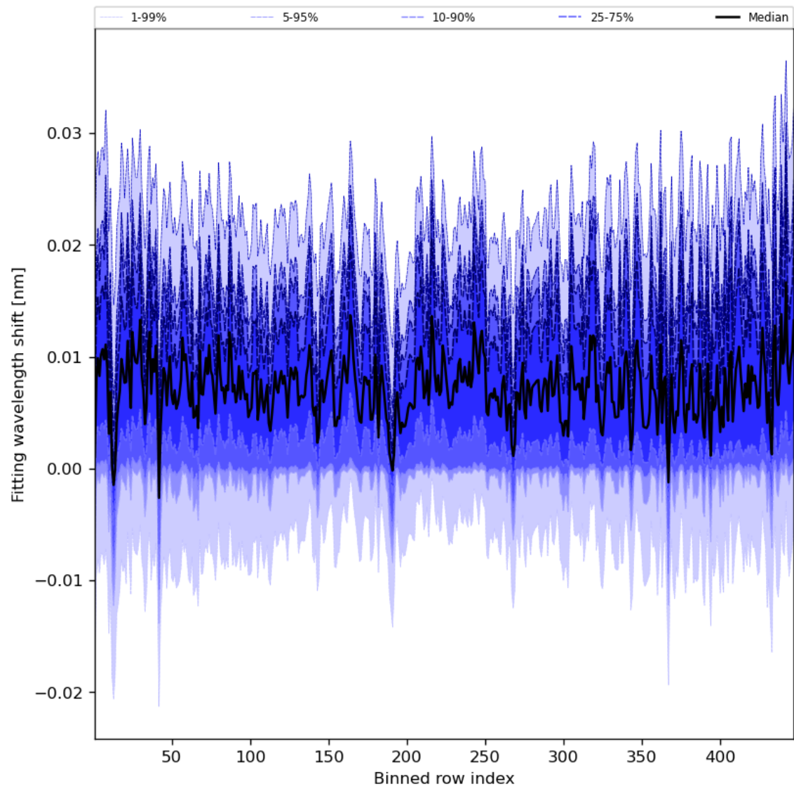
Figure 65: Along track statistics of “Fitting wavelength shift” for 2024-05-26 to 2024-05-28
