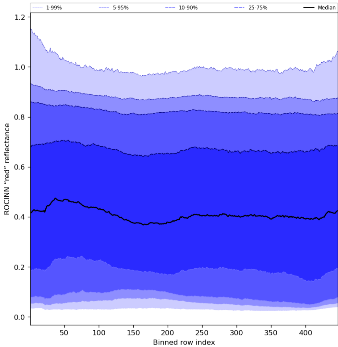
Figure 69: Along track statistics of "ROCINN "red" reflectance" for 2024-05-26 to 2024-05-28
