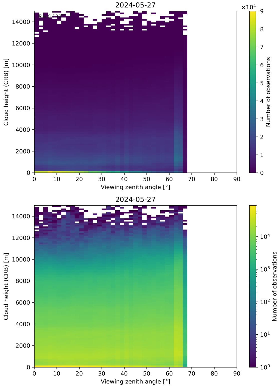
Figure 110: Scatter density plot of “Viewing zenith angle” against “Cloud height (CRB)” for 2024-05-26 to 2024-05-28.
