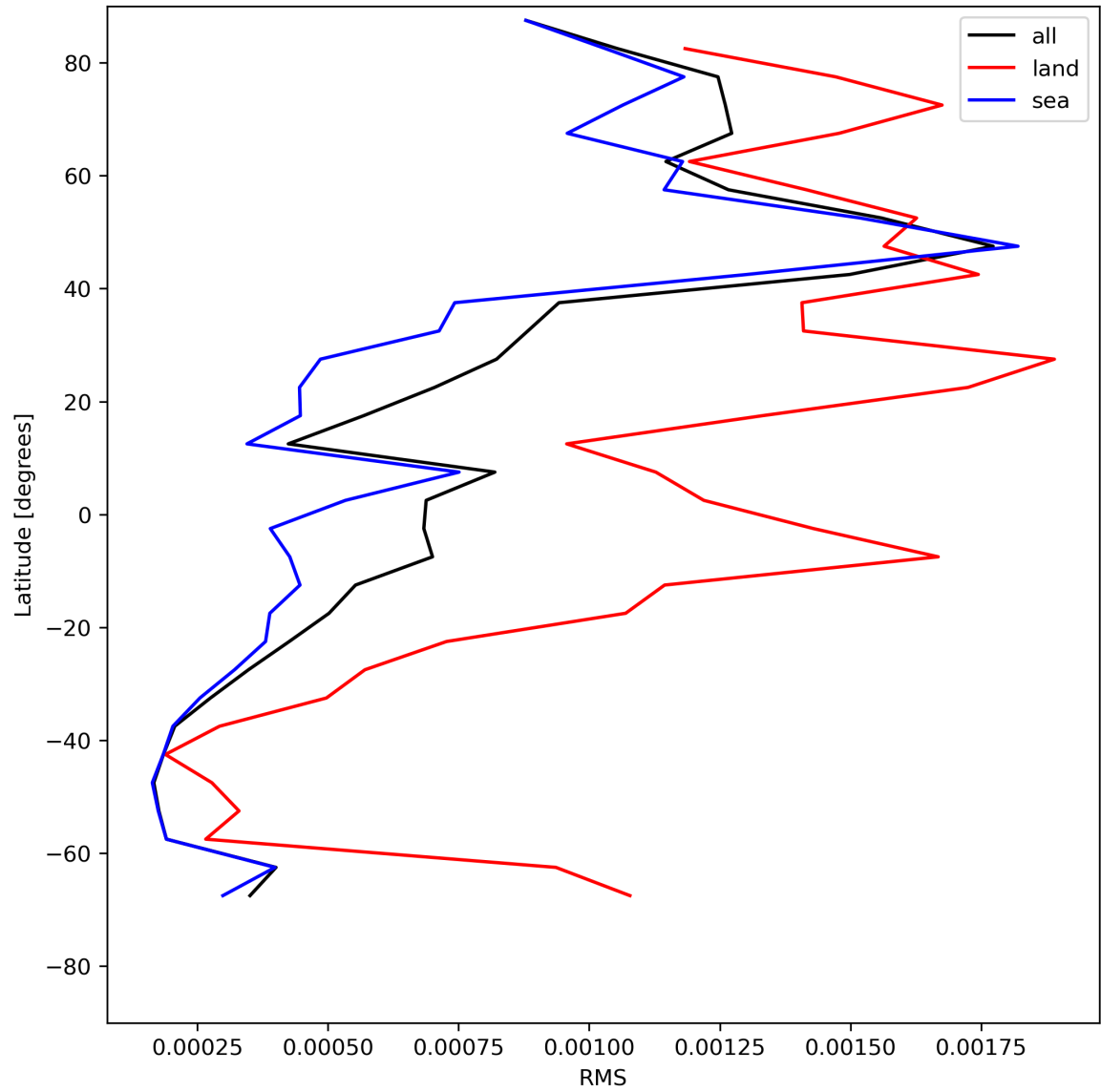
Figure 31: Zonal average of “RMS” for 2024-05-26 to 2024-05-28.
