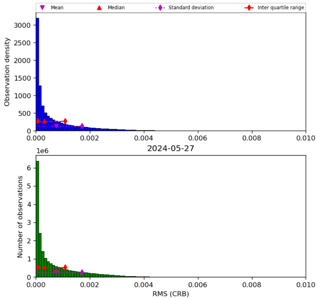
Figure 48: Histogram of “RMS (CRB)” for 2024-05-26 to 2024-05-28
