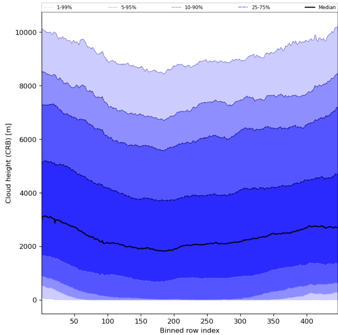
Figure 59: Along track statistics of “Cloud height (CRB)” for 2024-05-26 to 2024-05-28
