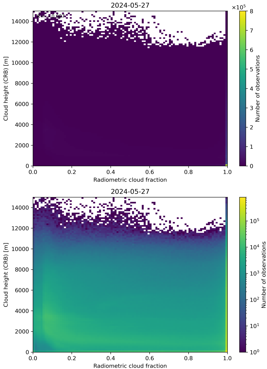
Figure 74: Scatter density plot of “Radiometric cloud fraction” against “Cloud height (CRB)” for 2024-05-26 to 2024-05-28.
