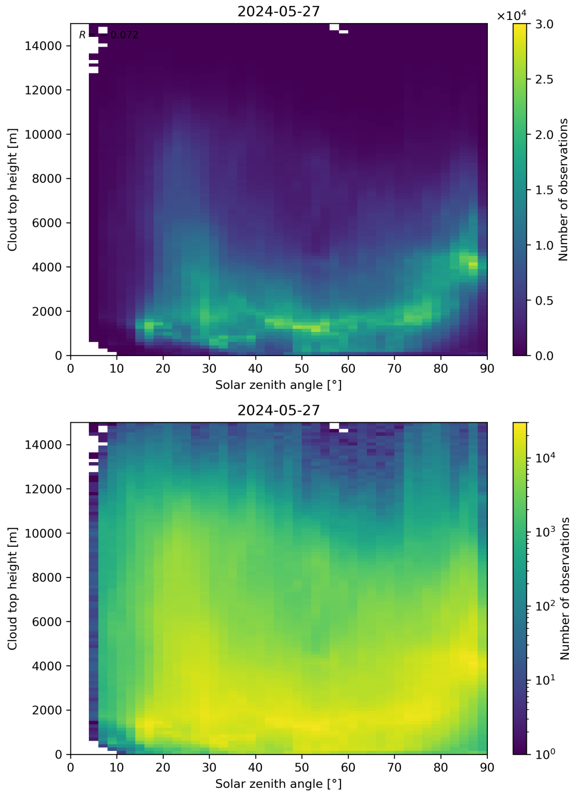
Figure 104: Scatter density plot of “Solar zenith angle” against “Cloud top height” for 2024-05-26 to 2024-05-28.
