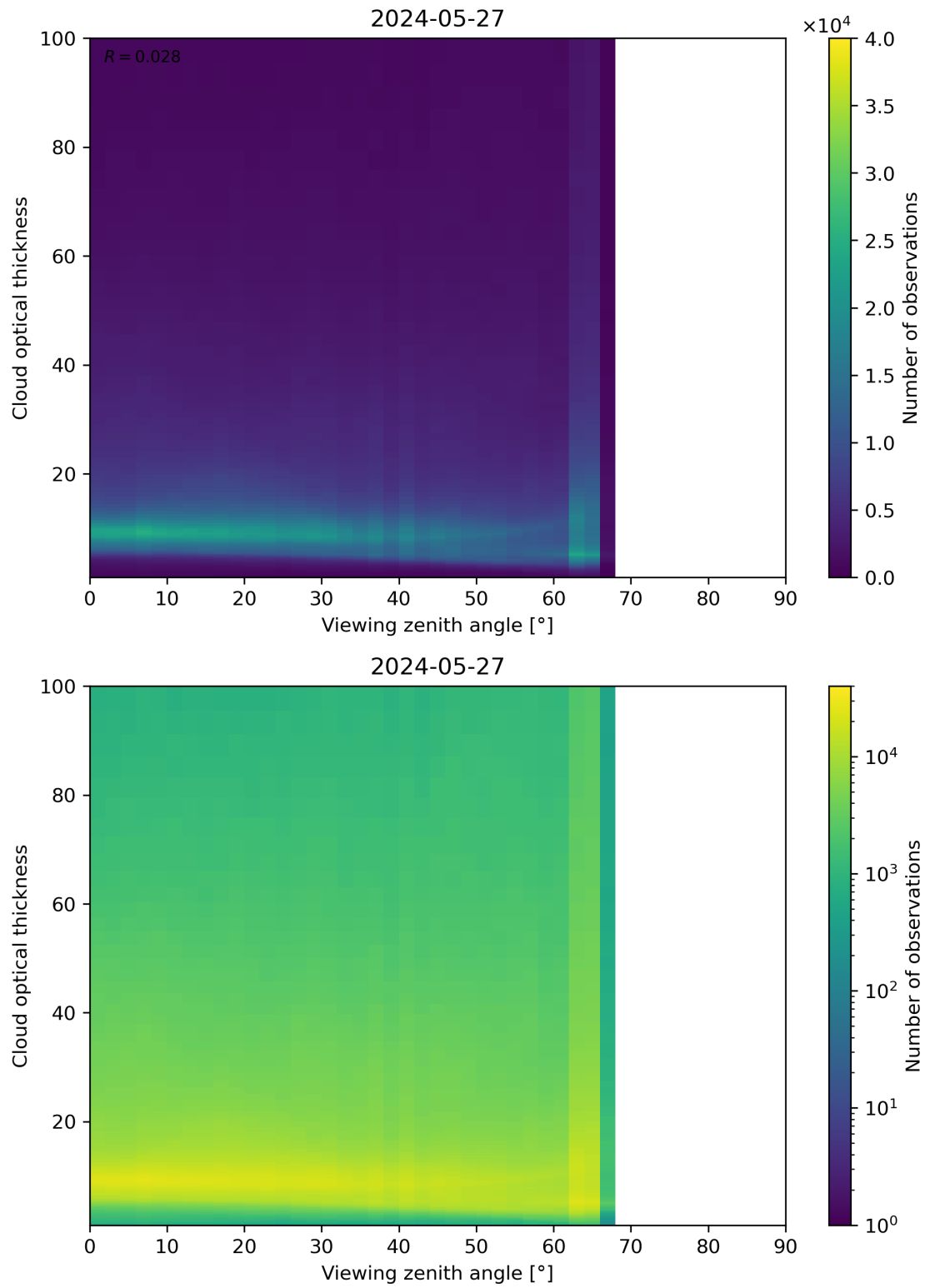
Figure 111: Scatter density plot of “Viewing zenith angle” against “Cloud optical thickness” for 2024-05-26 to 2024-05-28.
