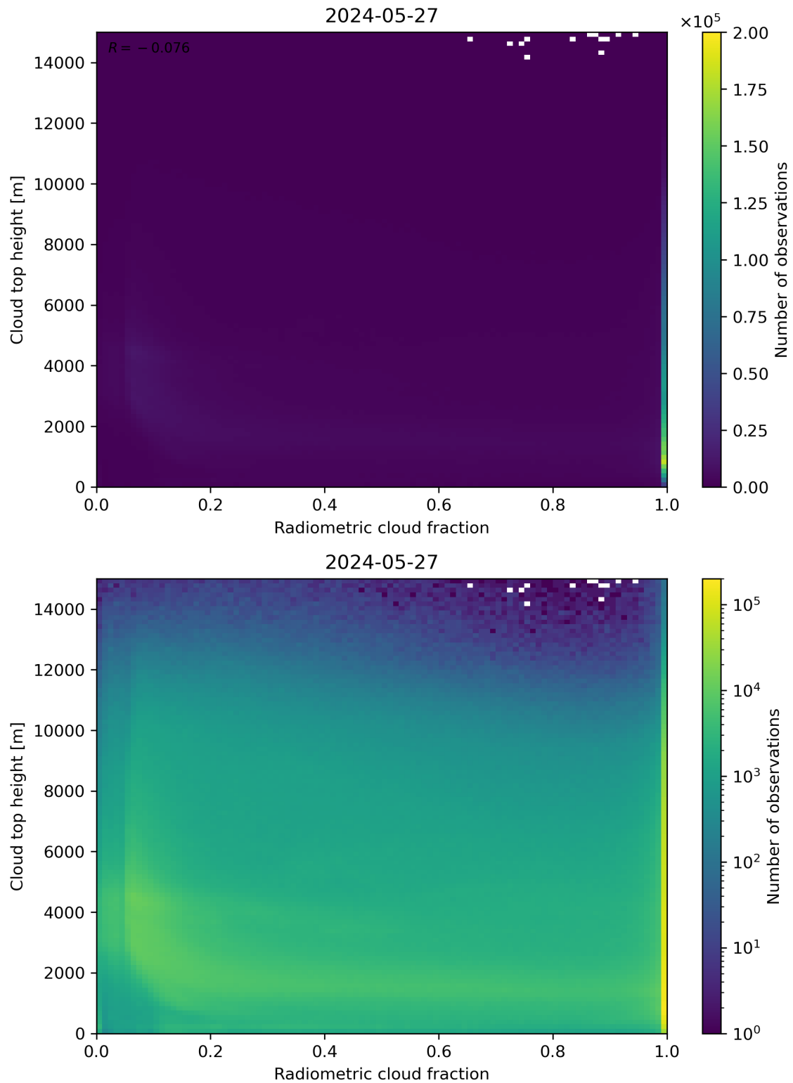
Figure 76: Scatter density plot of “Radiometric cloud fraction” against “Cloud top height” for 2024-05-26 to 2024-05-28.
