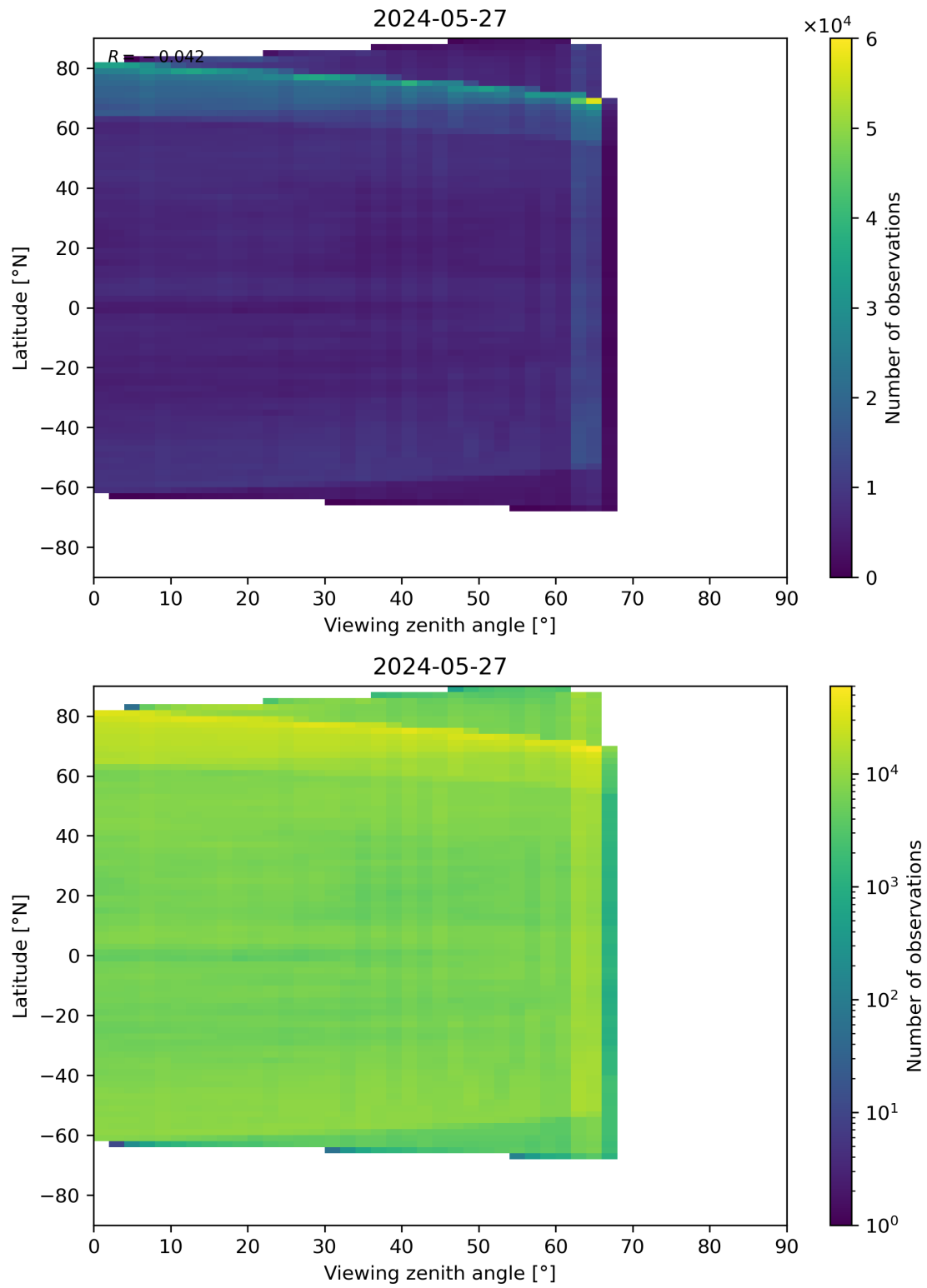
Figure 113: Scatter density plot of “Viewing zenith angle” against “Latitude” for 2024-05-26 to 2024-05-28.
