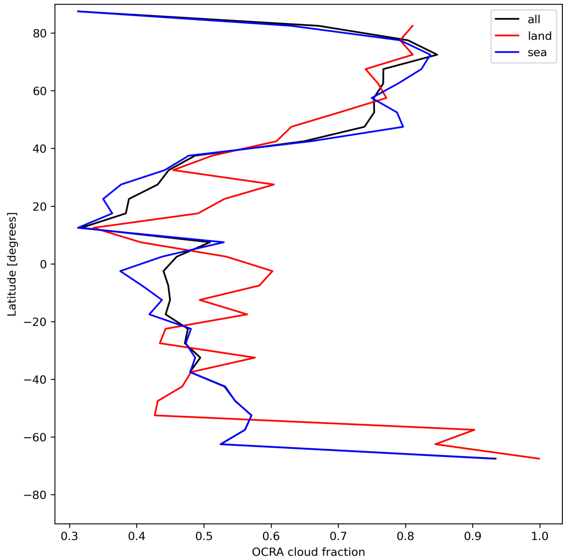
Figure 34: Zonal average of “OCRA cloud fraction” for 2024-05-26 to 2024-05-28.
