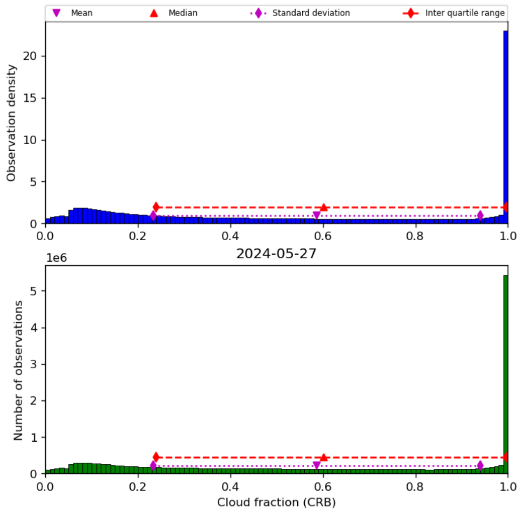
Figure 42: Histogram of “Cloud fraction (CRB)” for 2024-05-26 to 2024-05-28
