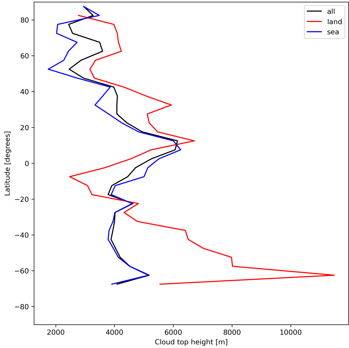
Figure 24: Zonal average of “Cloud top height” for 2024-05-28 to 2024-05-29.
