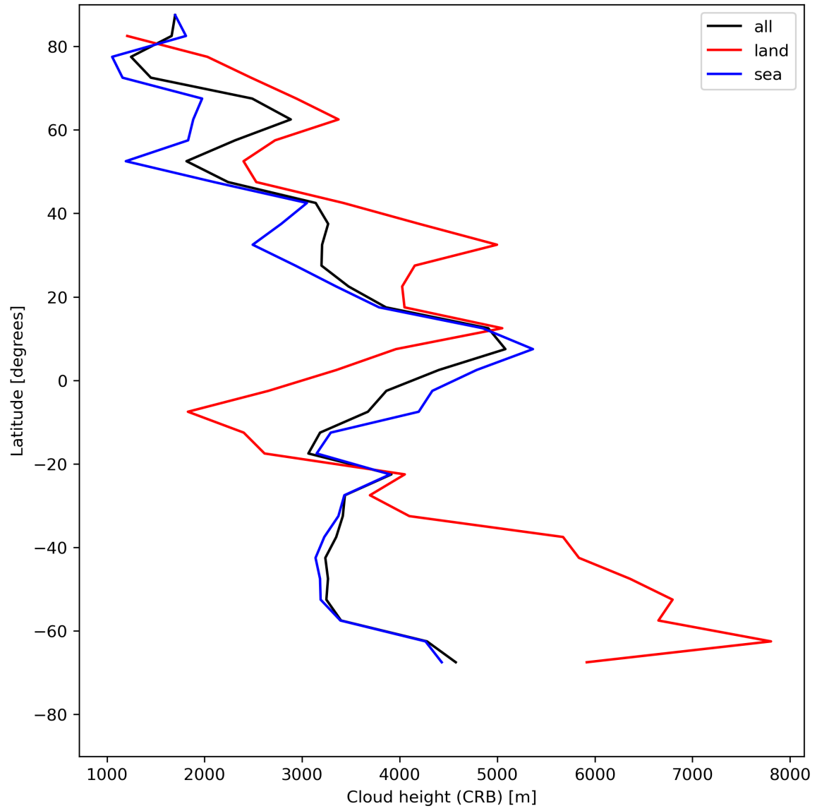
Figure 27: Zonal average of “Cloud height (CRB)” for 2024-05-28 to 2024-05-29.
