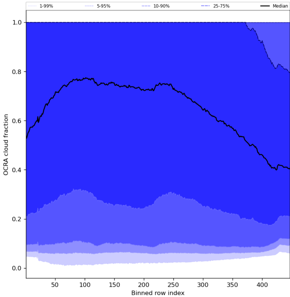
Figure 66: Along track statistics of “OCRA cloud fraction” for 2024-05-28 to 2024-05-29
