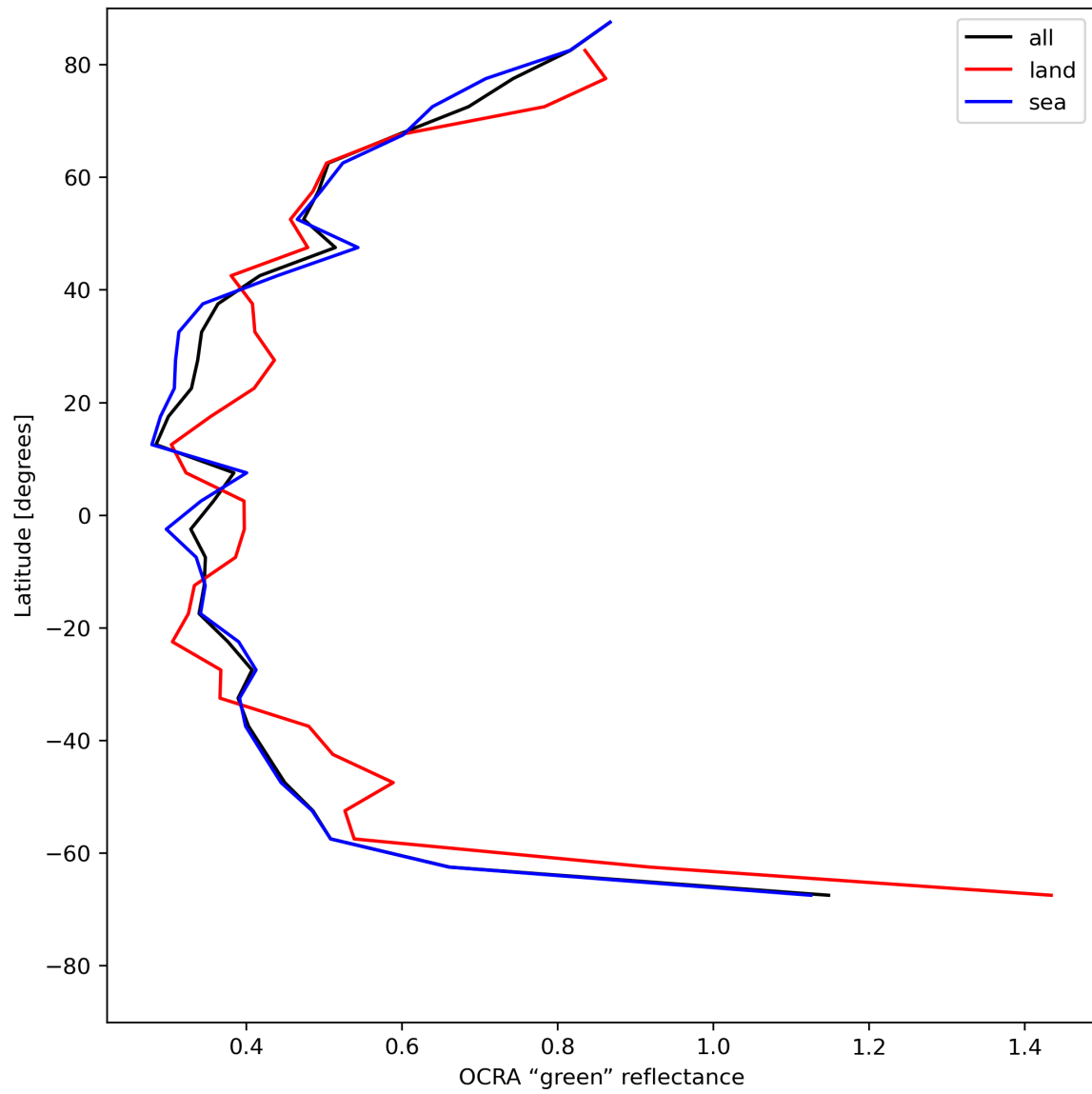
Figure 36: Zonal average of “OCRA “green” reflectance” for 2024-05-28 to 2024-05-29.
