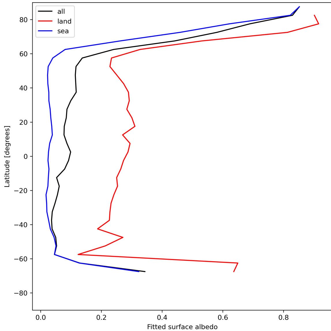
Figure 29: Zonal average of “Fitted surface albedo” for 2024-05-28 to 2024-05-29.
