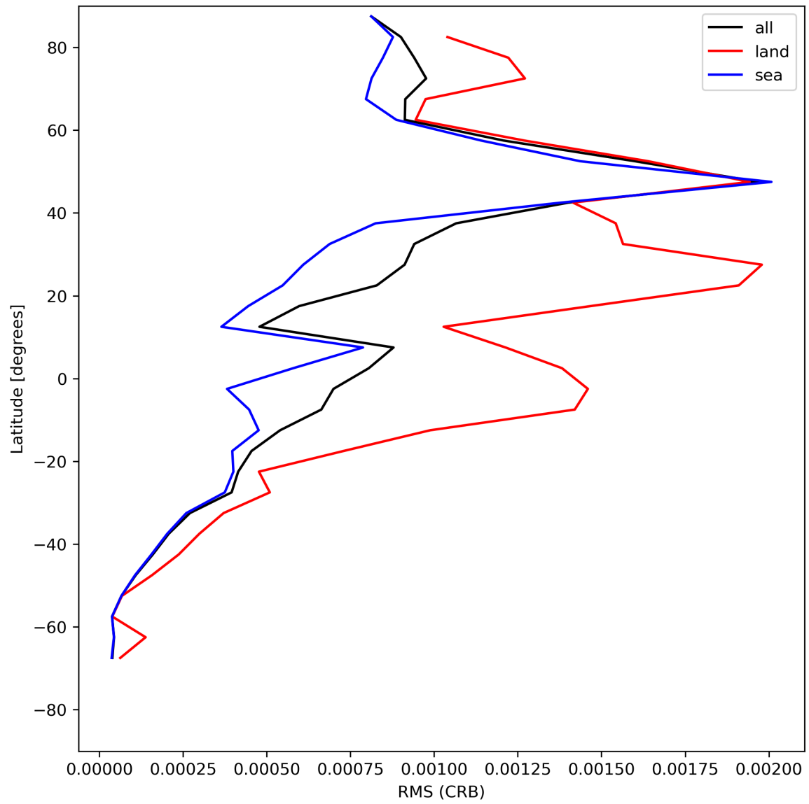
Figure 32: Zonal average of “RMS (CRB)” for 2024-05-28 to 2024-05-29.
