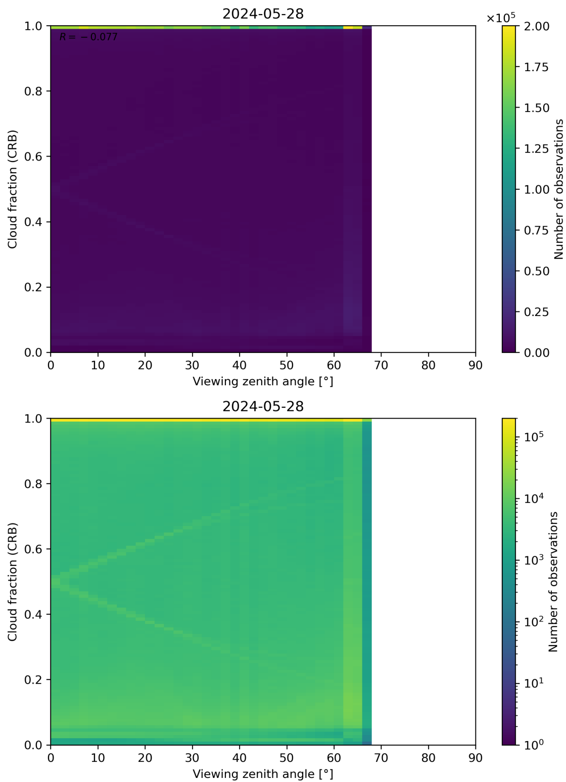
Figure 109: Scatter density plot of “Viewing zenith angle” against “Cloud fraction (CRB)” for 2024-05-28 to 2024-05-29.
