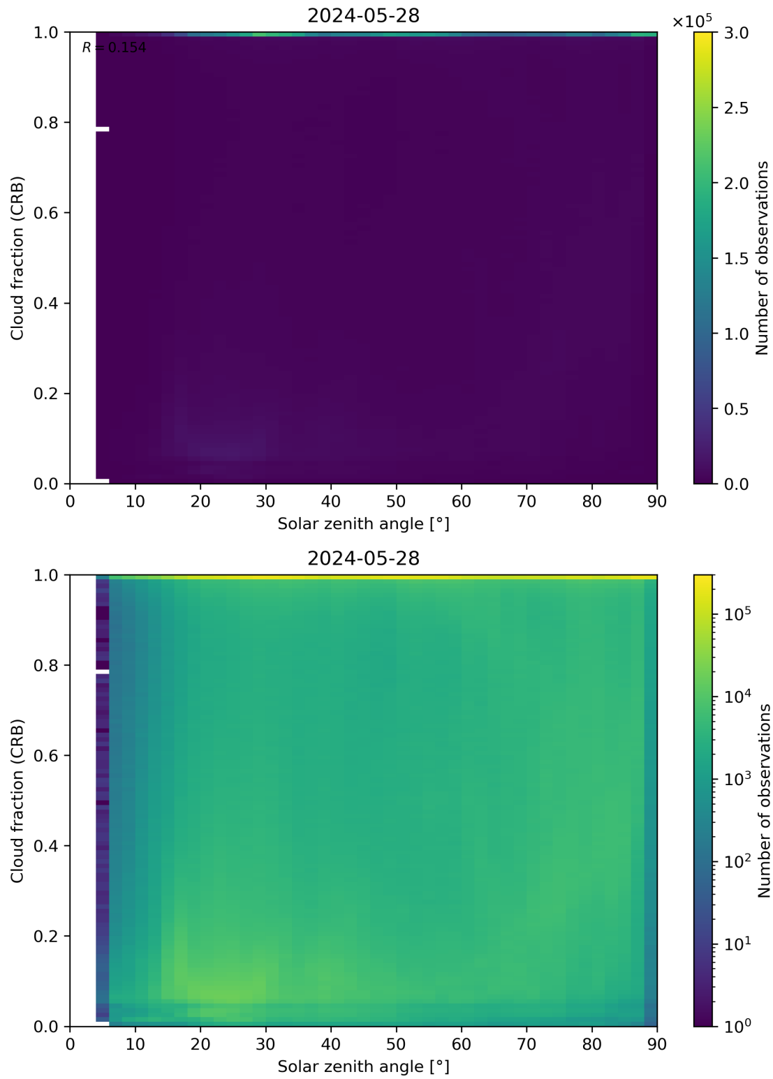
Figure 101: Scatter density plot of “Solar zenith angle” against “Cloud fraction (CRB)” for 2024-05-28 to 2024-05-29.
