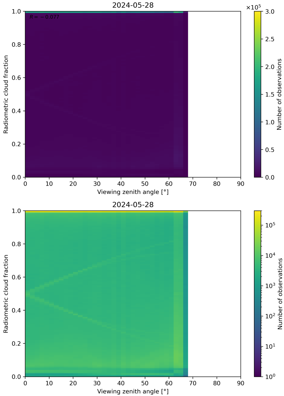
Figure 107: Scatter density plot of “Viewing zenith angle” against “Radiometric cloud fraction” for 2024-05-28 to 2024-05-29.
