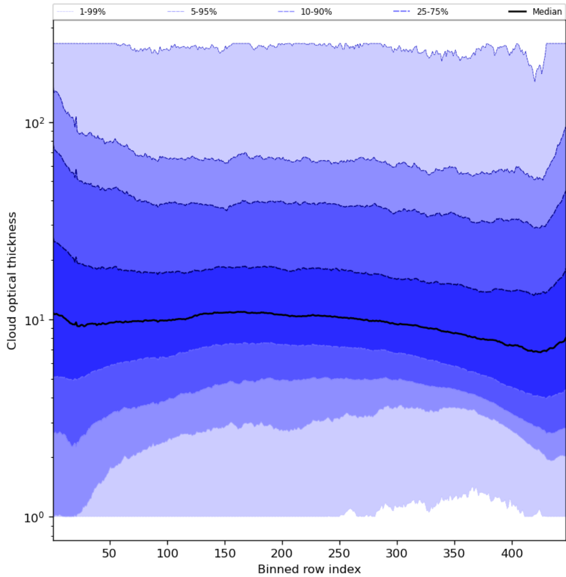
Figure 57: Along track statistics of “Cloud optical thickness” for 2024-05-28 to 2024-05-29
