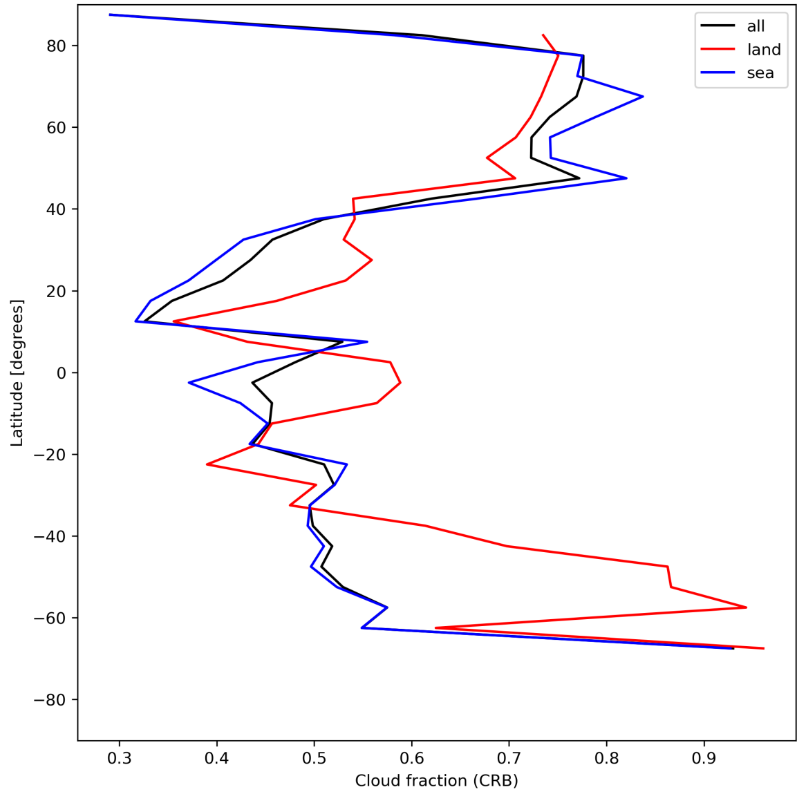
Figure 26: Zonal average of “Cloud fraction (CRB)” for 2024-05-28 to 2024-05-29.
