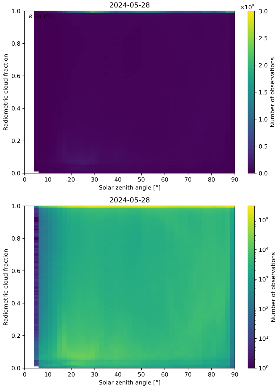
Figure 99: Scatter density plot of “Solar zenith angle” against “Radiometric cloud fraction” for 2024-05-28 to 2024-05-29.
