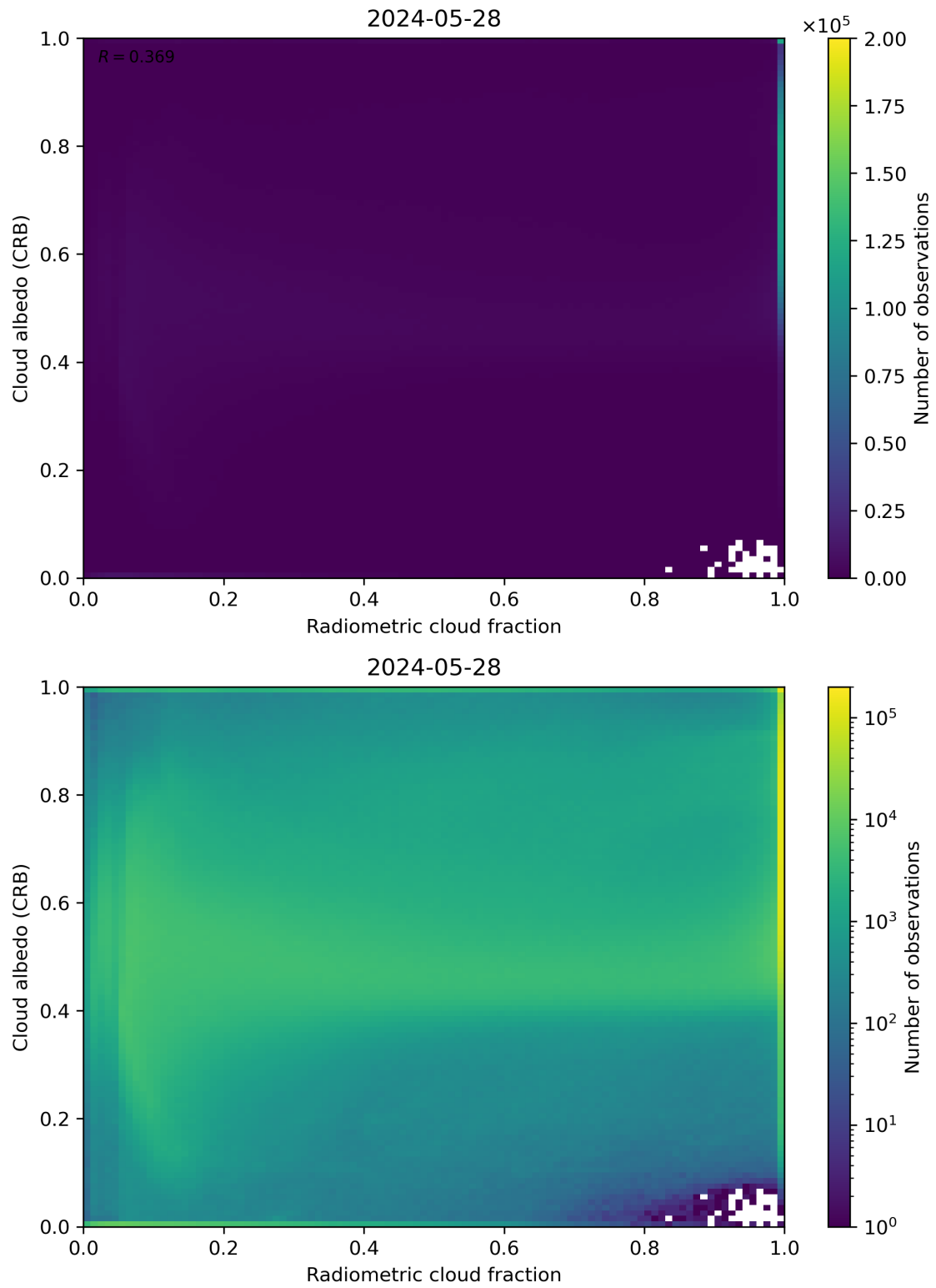
Figure 71: Scatter density plot of “Radiometric cloud fraction” against “Cloud albedo (CRB)” for 2024-05-28 to 2024-05-29.
