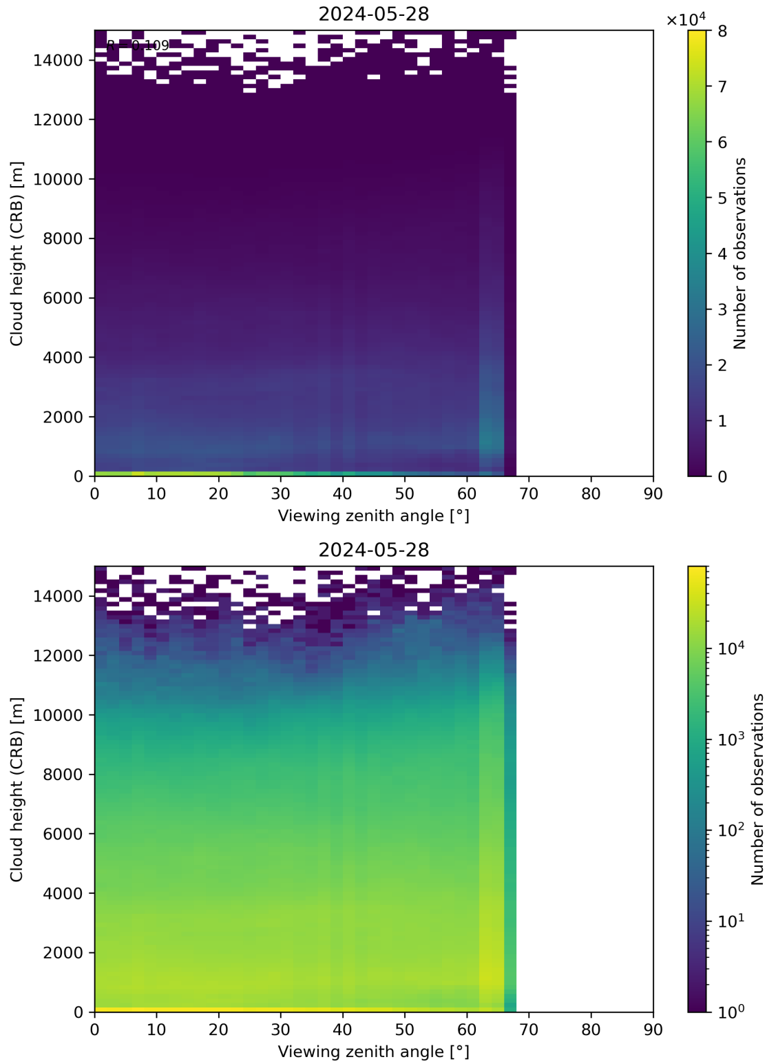
Figure 110: Scatter density plot of “Viewing zenith angle” against “Cloud height (CRB)” for 2024-05-28 to 2024-05-29.
