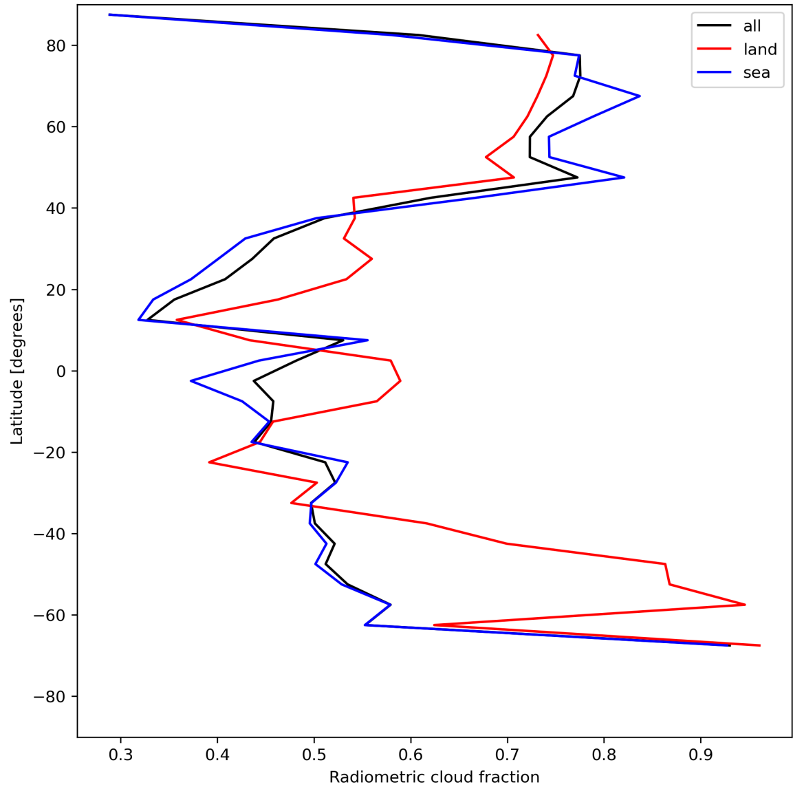
Figure 23: Zonal average of “Radiometric cloud fraction” for 2024-05-28 to 2024-05-29.
