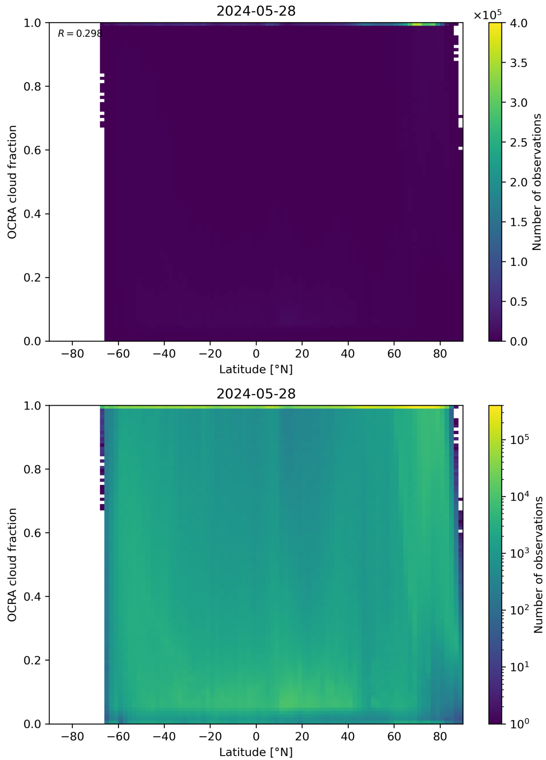
Figure 93: Scatter density plot of “Latitude” against “OCRA cloud fraction” for 2024-05-28 to 2024-05-29.
