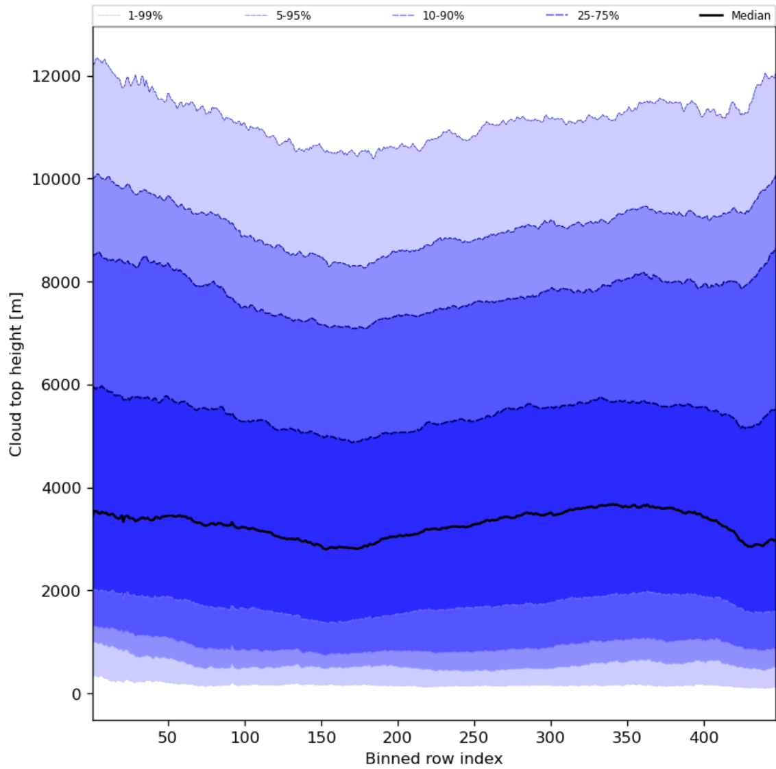
Figure 56: Along track statistics of “Cloud top height” for 2024-05-28 to 2024-05-29
