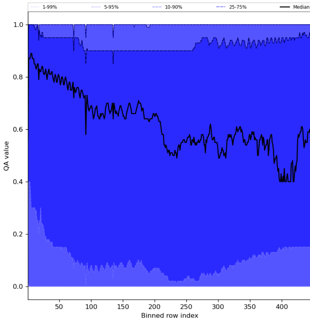
Figure 54: Along track statistics of “QA value” for 2024-05-28 to 2024-05-29
