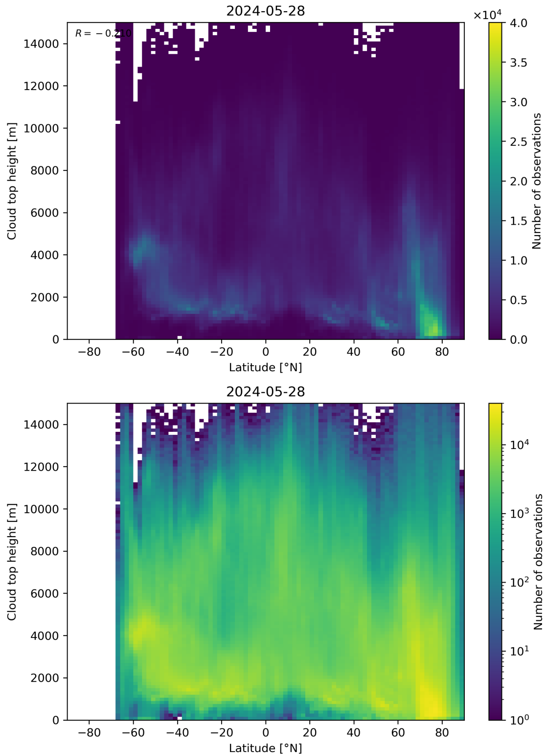
Figure 97: Scatter density plot of “Latitude” against “Cloud top height” for 2024-05-28 to 2024-05-29.
