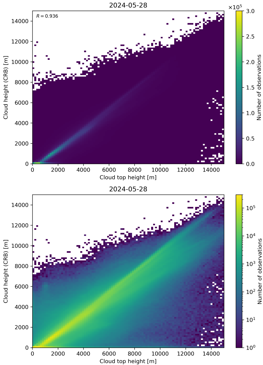
Figure 89: Scatter density plot of “Cloud top height” against “Cloud height (CRB)” for 2024-05-28 to 2024-05-29.
