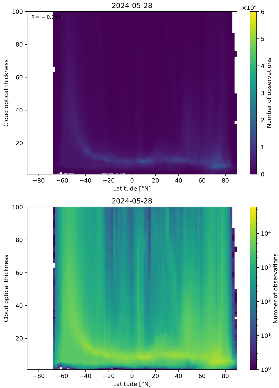
Figure 96: Scatter density plot of “Latitude” against “Cloud optical thickness” for 2024-05-28 to 2024-05-29.
