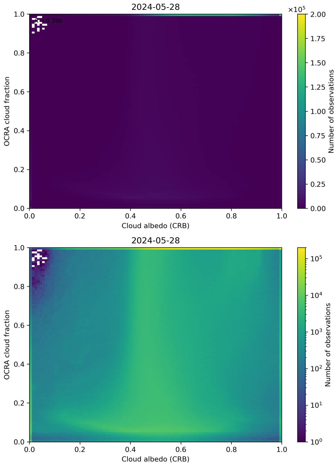
Figure 70: Scatter density plot of “Cloud albedo (CRB)” against “OCRA cloud fraction” for 2024-05-28 to 2024-05-29.
