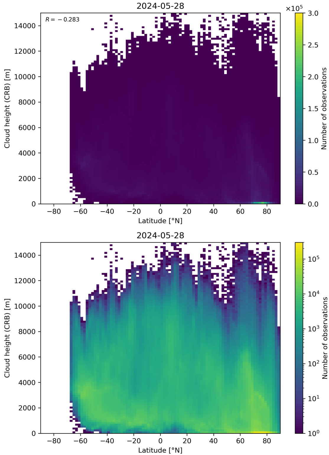
Figure 95: Scatter density plot of “Latitude” against “Cloud height (CRB)” for 2024-05-28 to 2024-05-29.
