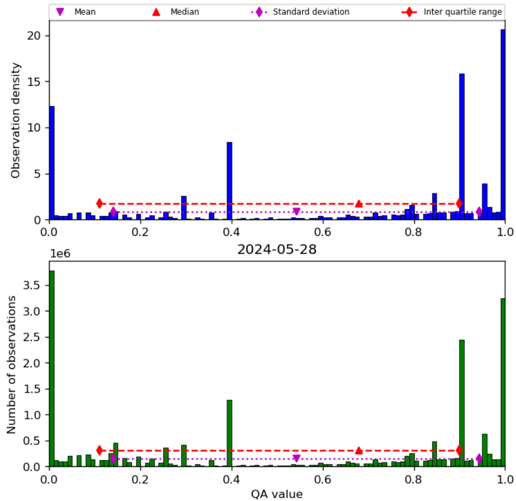
Figure 38: Histogram of “QA value” for 2024-05-28 to 2024-05-29
