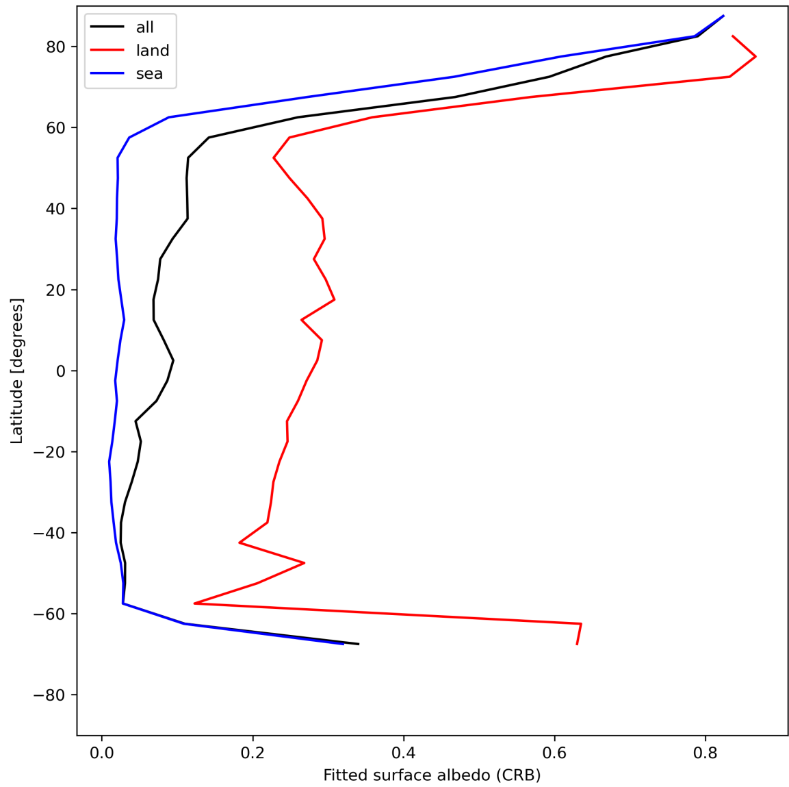
Figure 30: Zonal average of “Fitted surface albedo (CRB)” for 2024-05-28 to 2024-05-29.
