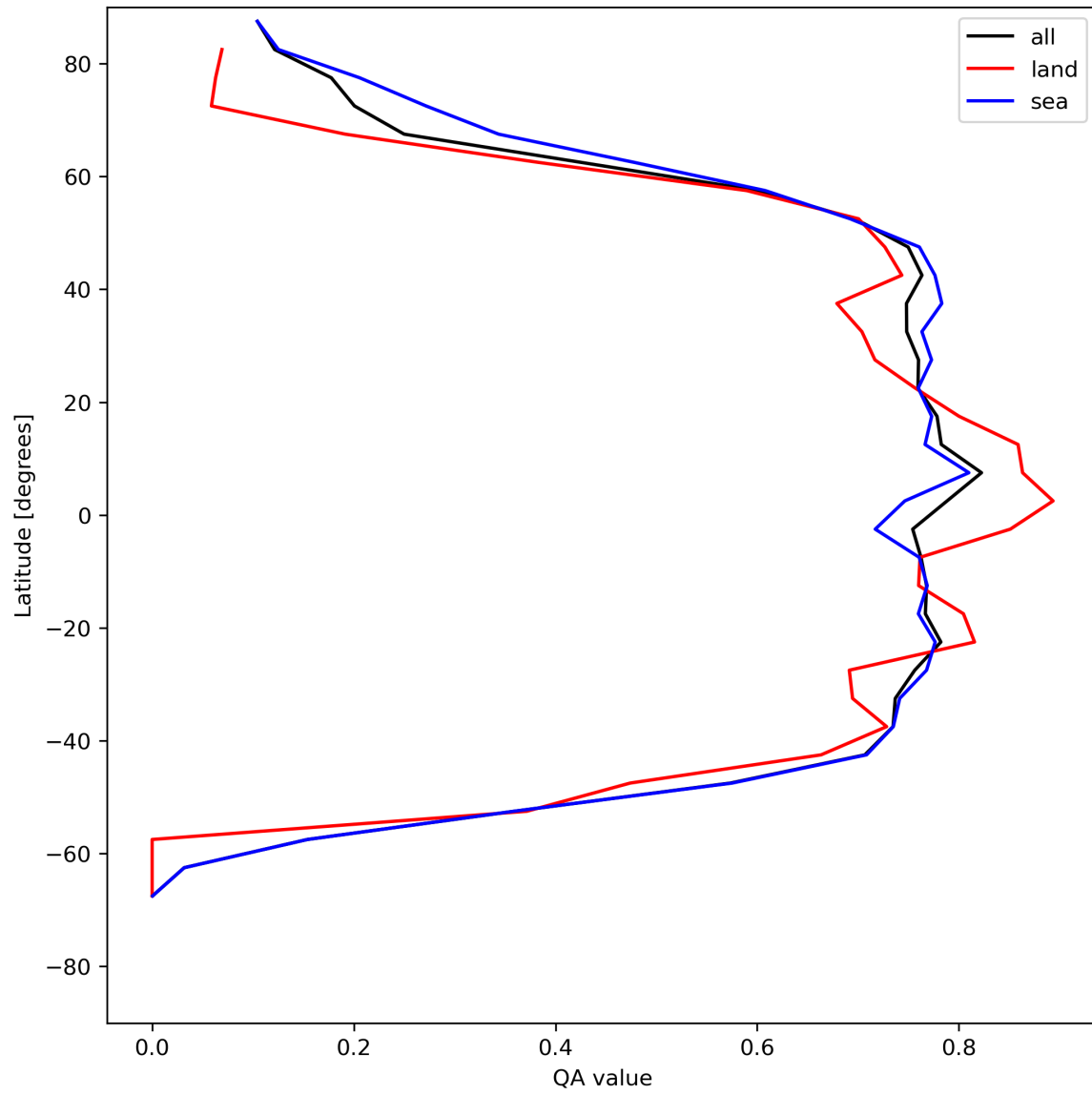
Figure 22: Zonal average of “QA value” for 2024-05-28 to 2024-05-29.
