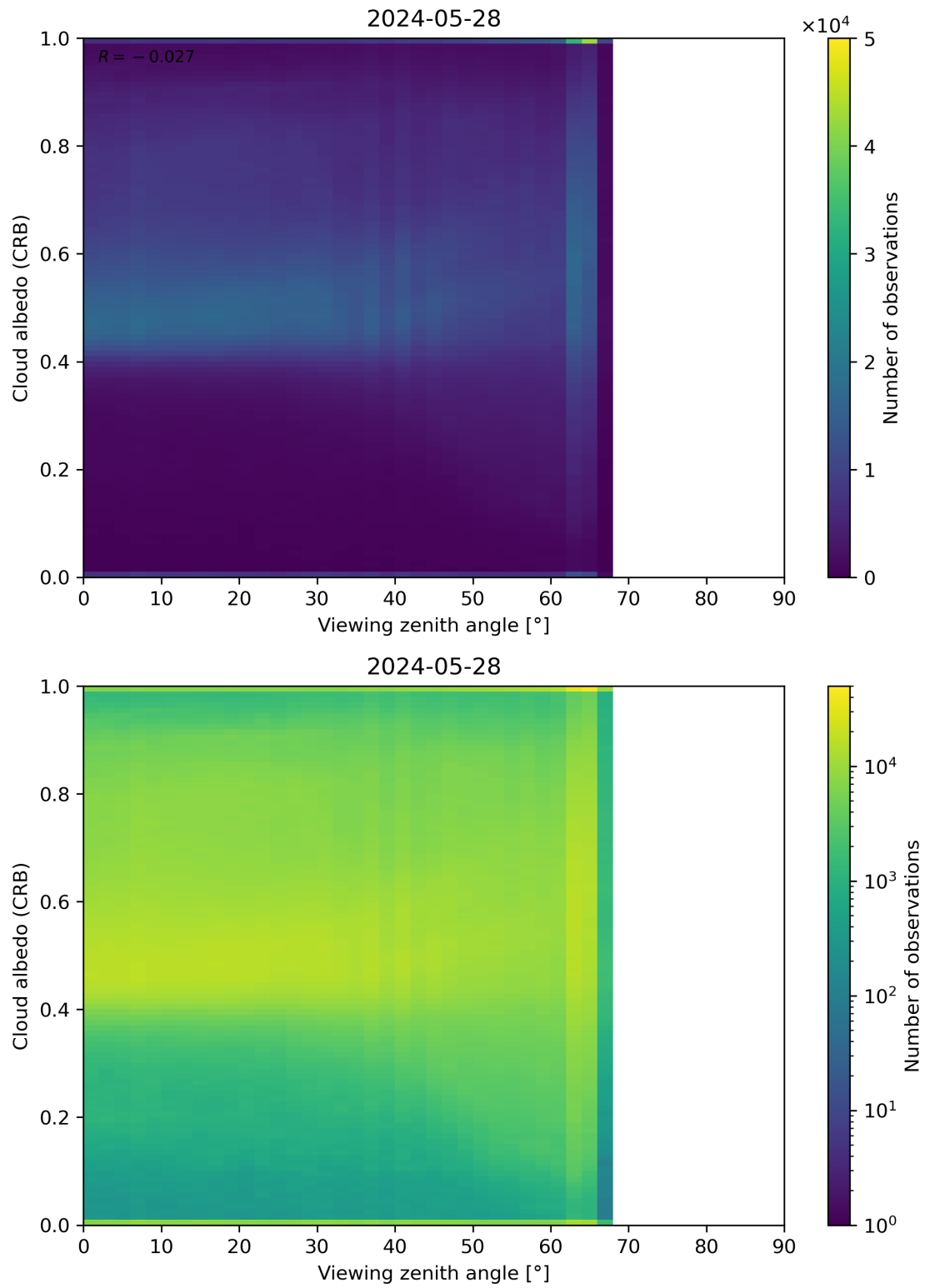
Figure 106: Scatter density plot of “Viewing zenith angle” against “Cloud albedo (CRB)” for 2024-05-28 to 2024-05-29.
