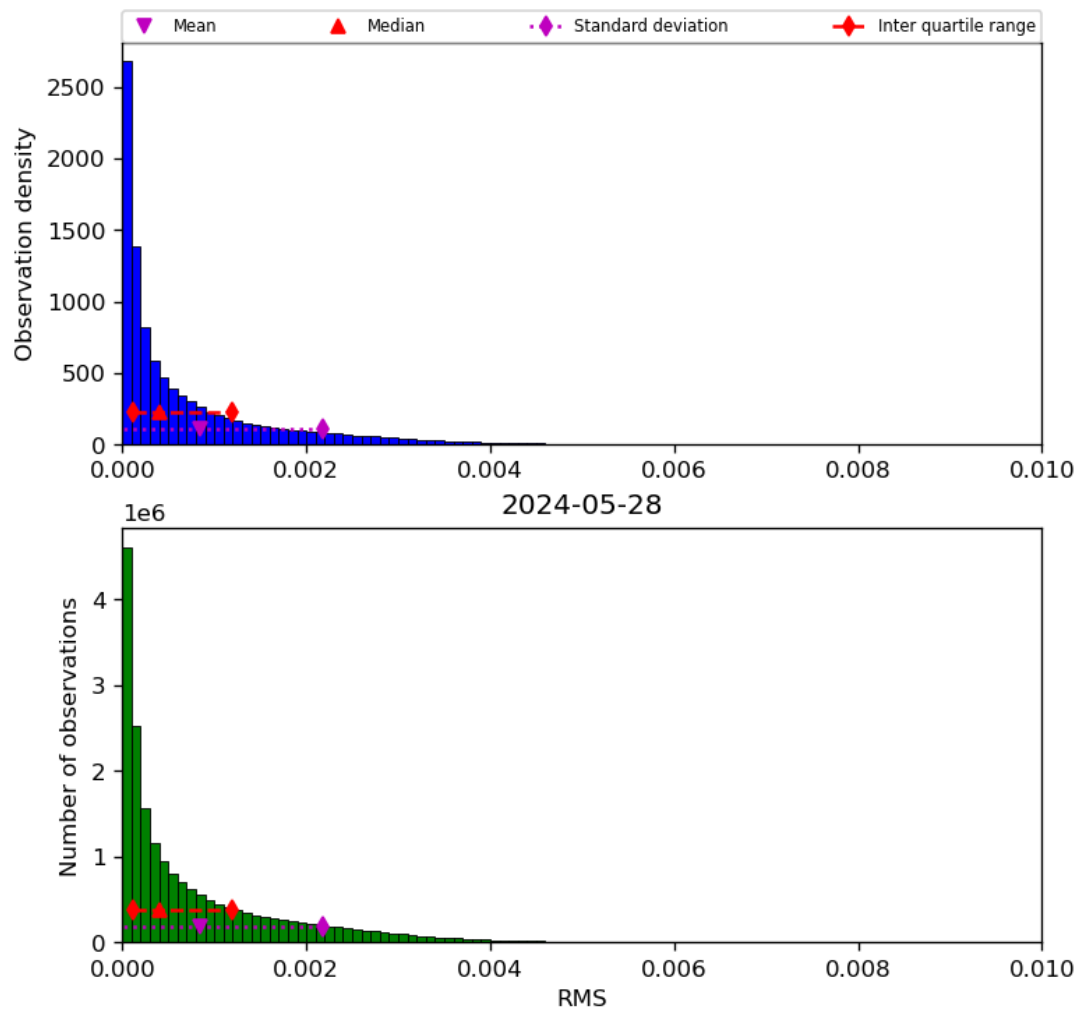
Figure 47: Histogram of “RMS” for 2024-05-28 to 2024-05-29
