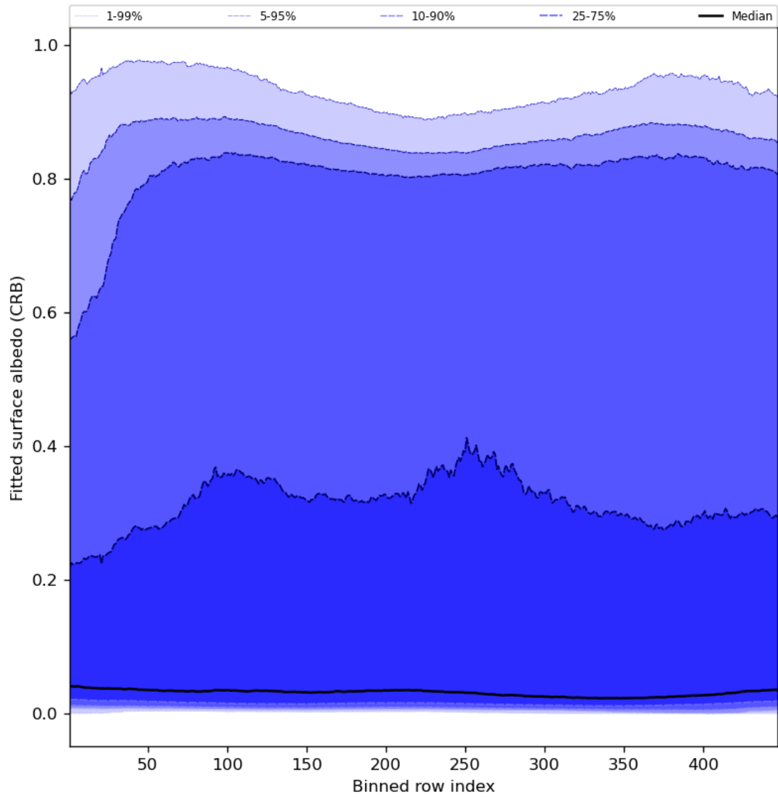
Figure 62: Along track statistics of “Fitted surface albedo (CRB)” for 2024-05-28 to 2024-05-29
