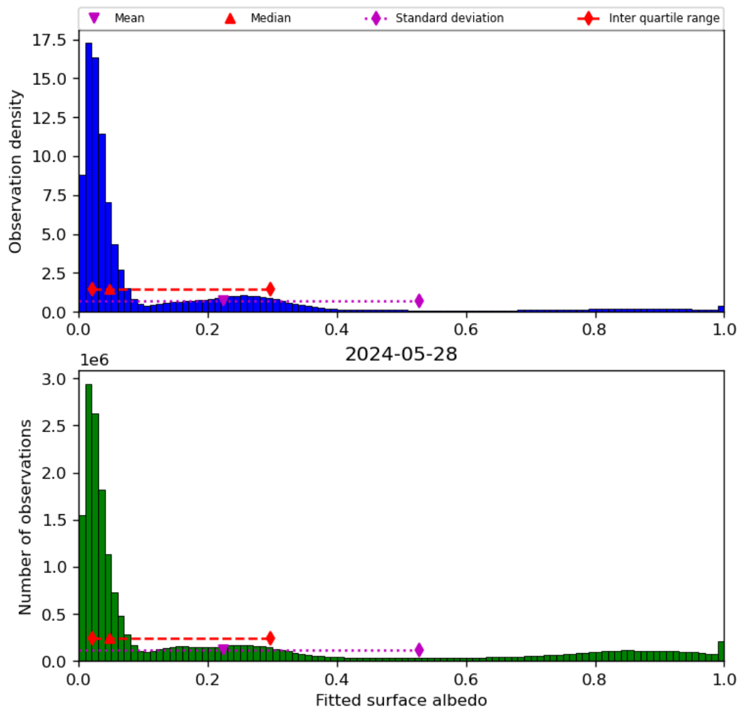
Figure 45: Histogram of “Fitted surface albedo” for 2024-05-28 to 2024-05-29
