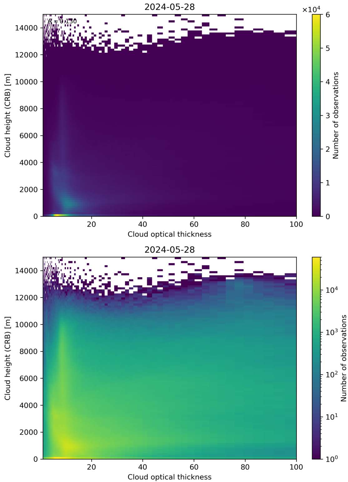
Figure 85: Scatter density plot of “Cloud optical thickness” against “Cloud height (CRB)” for 2024-05-28 to 2024-05-29.
