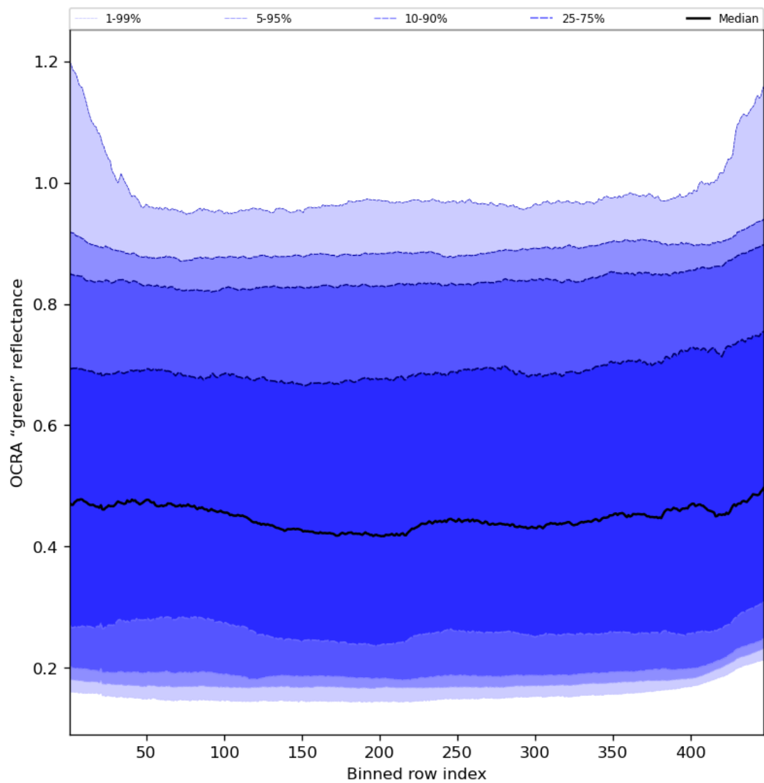
Figure 68: Along track statistics of “OCRA “green” reflectance” for 2024-05-28 to 2024-05-29
