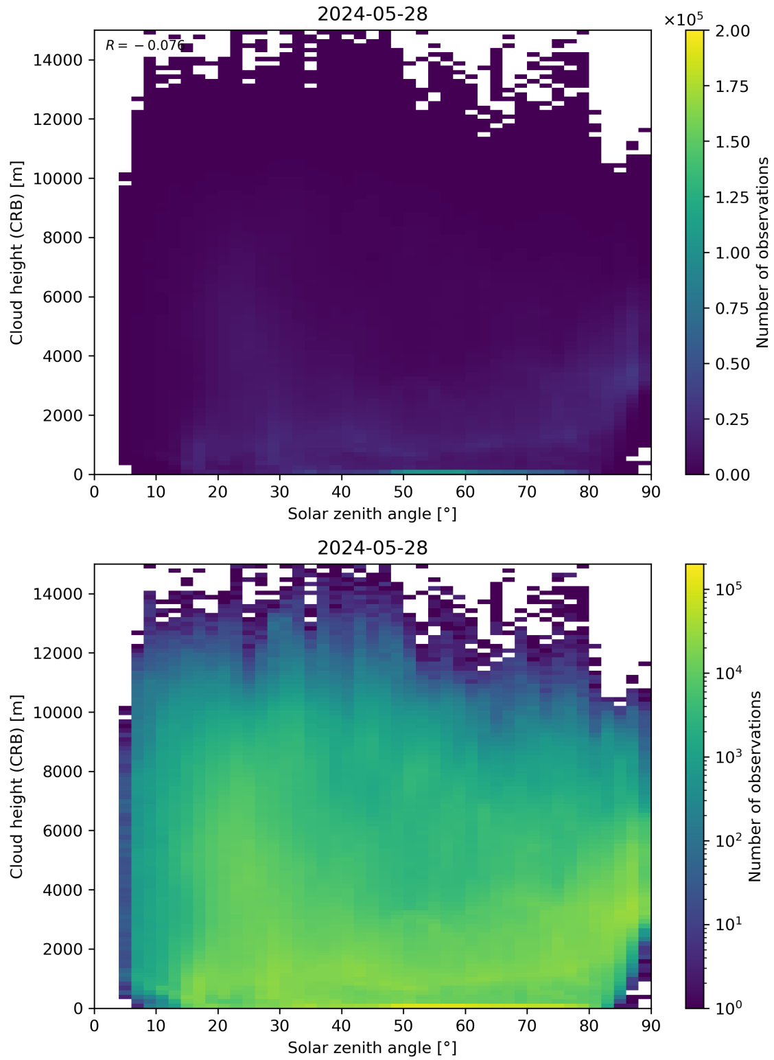
Figure 102: Scatter density plot of “Solar zenith angle” against “Cloud height (CRB)” for 2024-05-28 to 2024-05-29.
