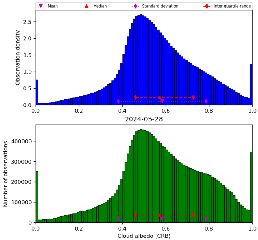
Figure 44: Histogram of “Cloud albedo (CRB)” for 2024-05-28 to 2024-05-29
