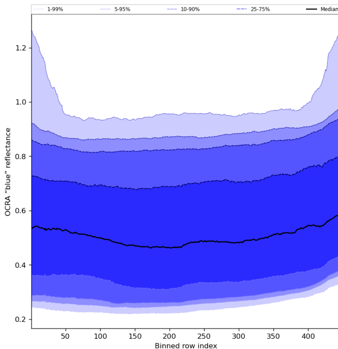
Figure 67: Along track statistics of “OCRA “blue” reflectance” for 2024-05-28 to 2024-05-29
