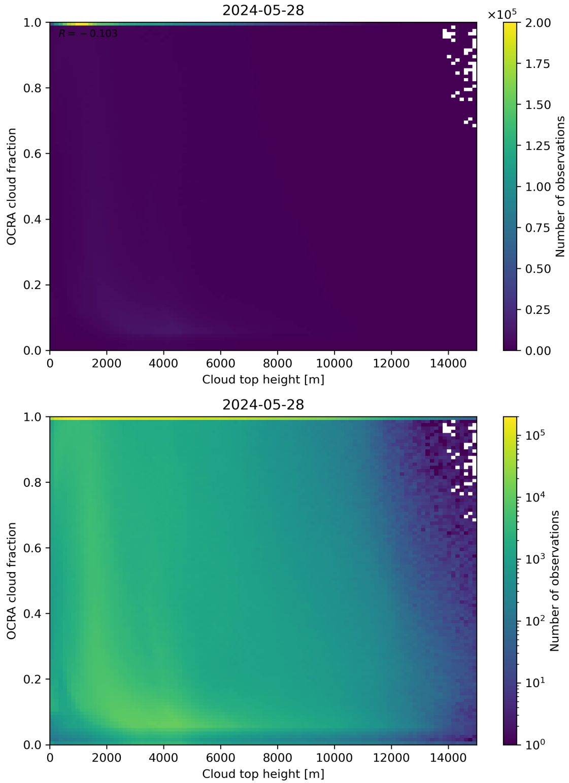
Figure 87: Scatter density plot of “Cloud top height” against “OCRA cloud fraction” for 2024-05-28 to 2024-05-29.
