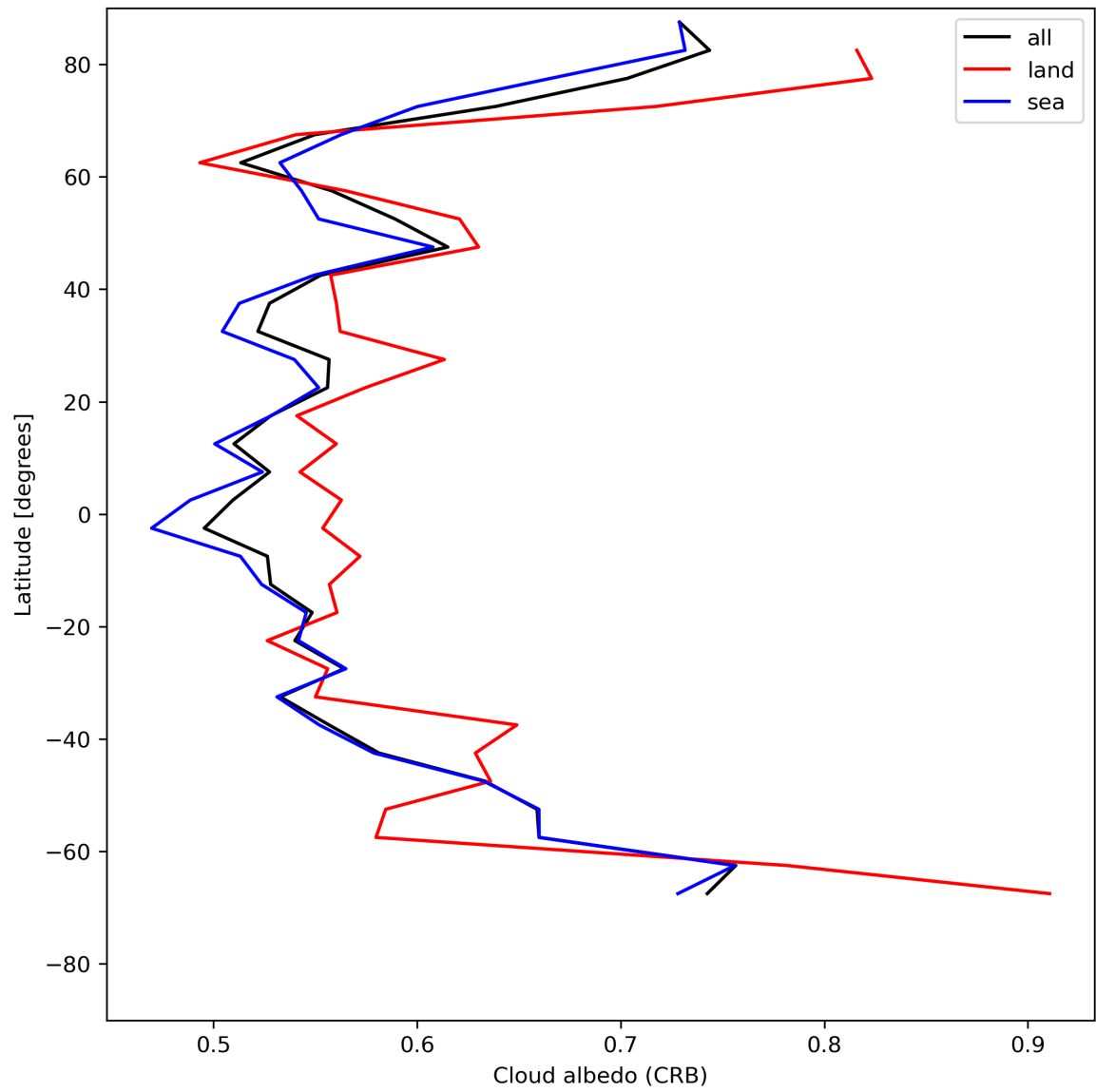
Figure 28: Zonal average of “Cloud albedo (CRB)” for 2024-05-28 to 2024-05-29.
