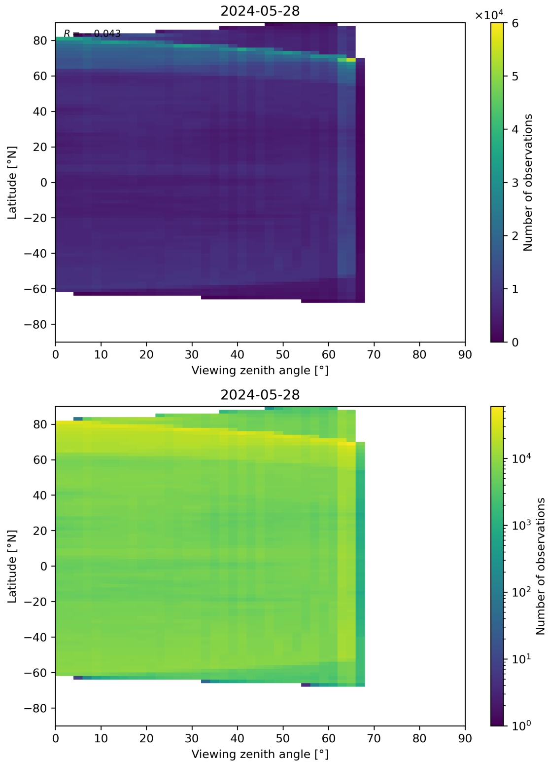
Figure 113: Scatter density plot of “Viewing zenith angle” against “Latitude” for 2024-05-28 to 2024-05-29.
