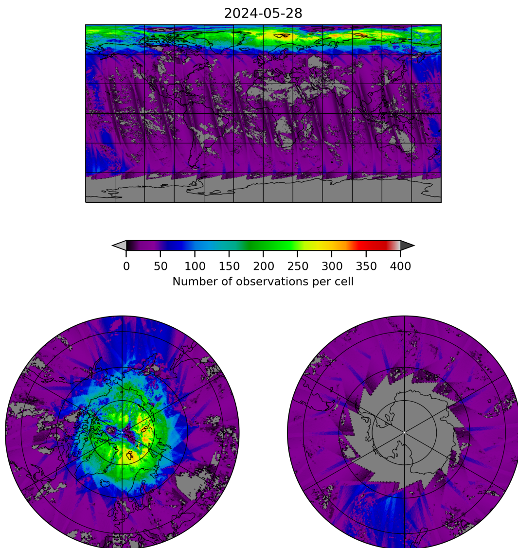
Figure 21: Map of the number of observations for 2024-05-28 to 2024-05-29
