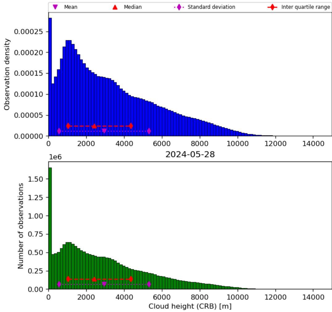
Figure 43: Histogram of “Cloud height (CRB)” for 2024-05-28 to 2024-05-29
