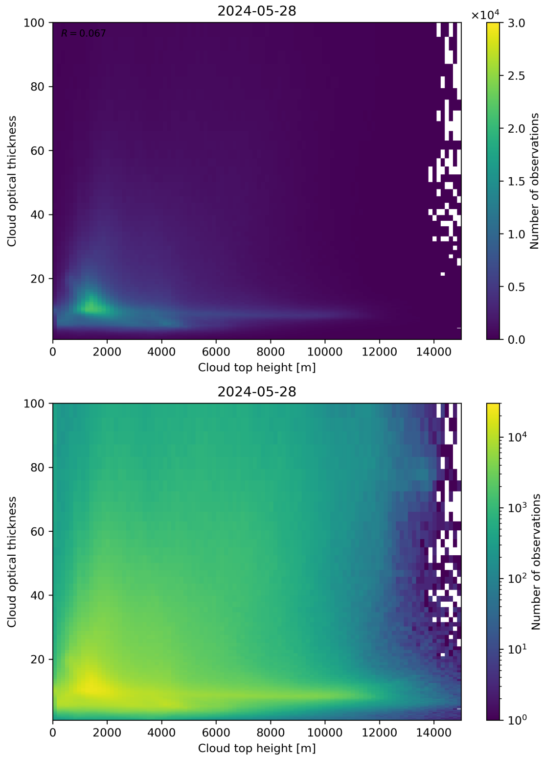
Figure 90: Scatter density plot of “Cloud top height” against “Cloud optical thickness” for 2024-05-28 to 2024-05-29.
