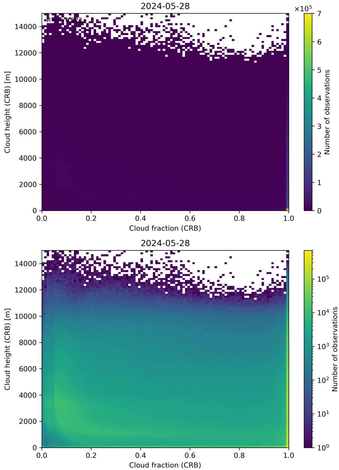
Figure 79: Scatter density plot of “Cloud fraction (CRB)” against “Cloud height (CRB)” for 2024-05-28 to 2024-05-29.
