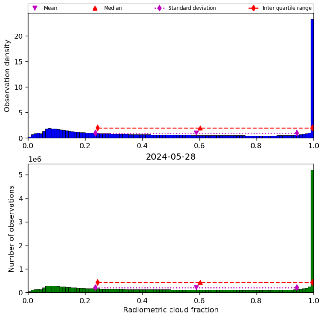
Figure 39: Histogram of “Radiometric cloud fraction” for 2024-05-28 to 2024-05-29
