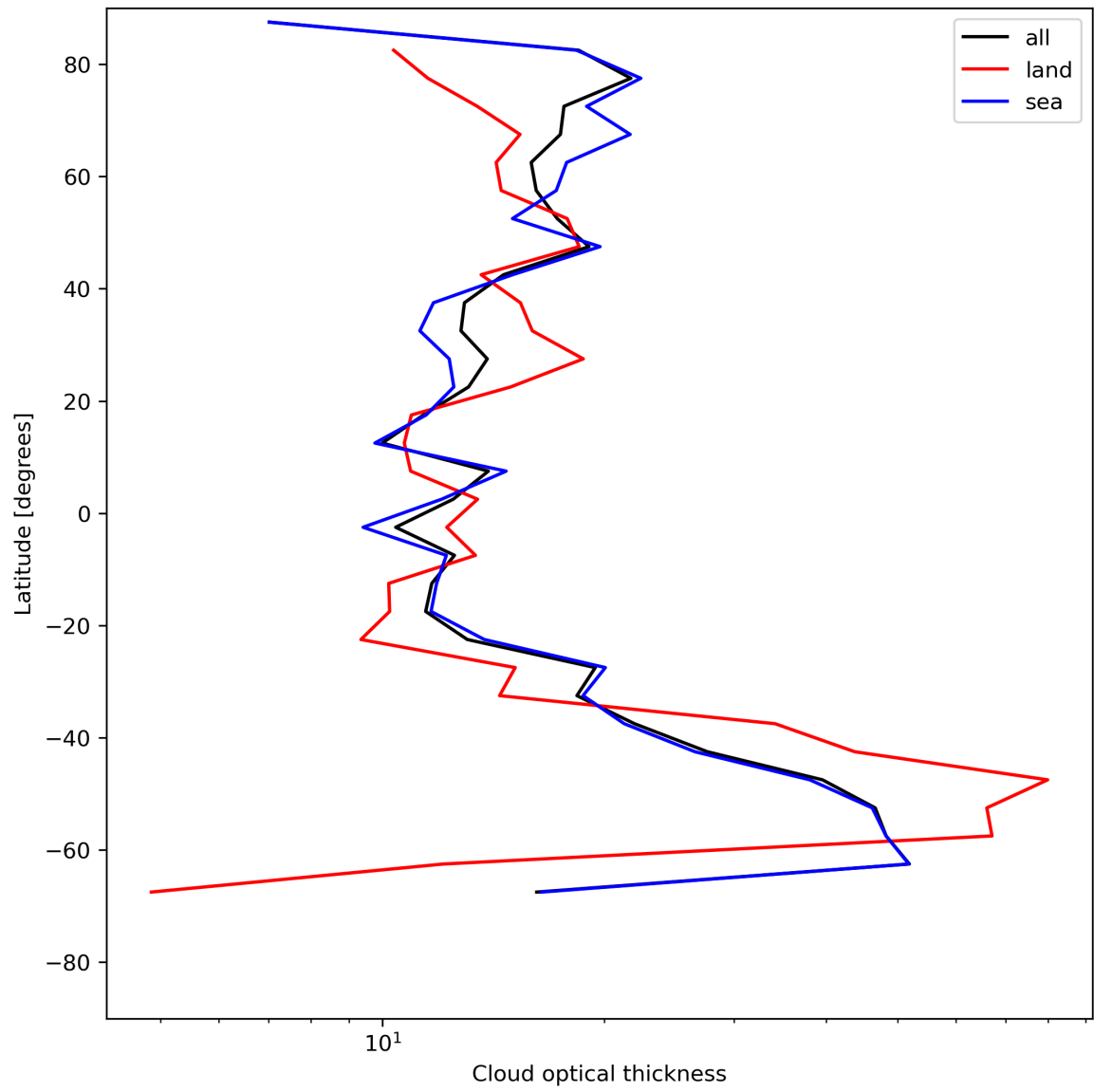
Figure 25: Zonal average of “Cloud optical thickness” for 2024-05-28 to 2024-05-29.
