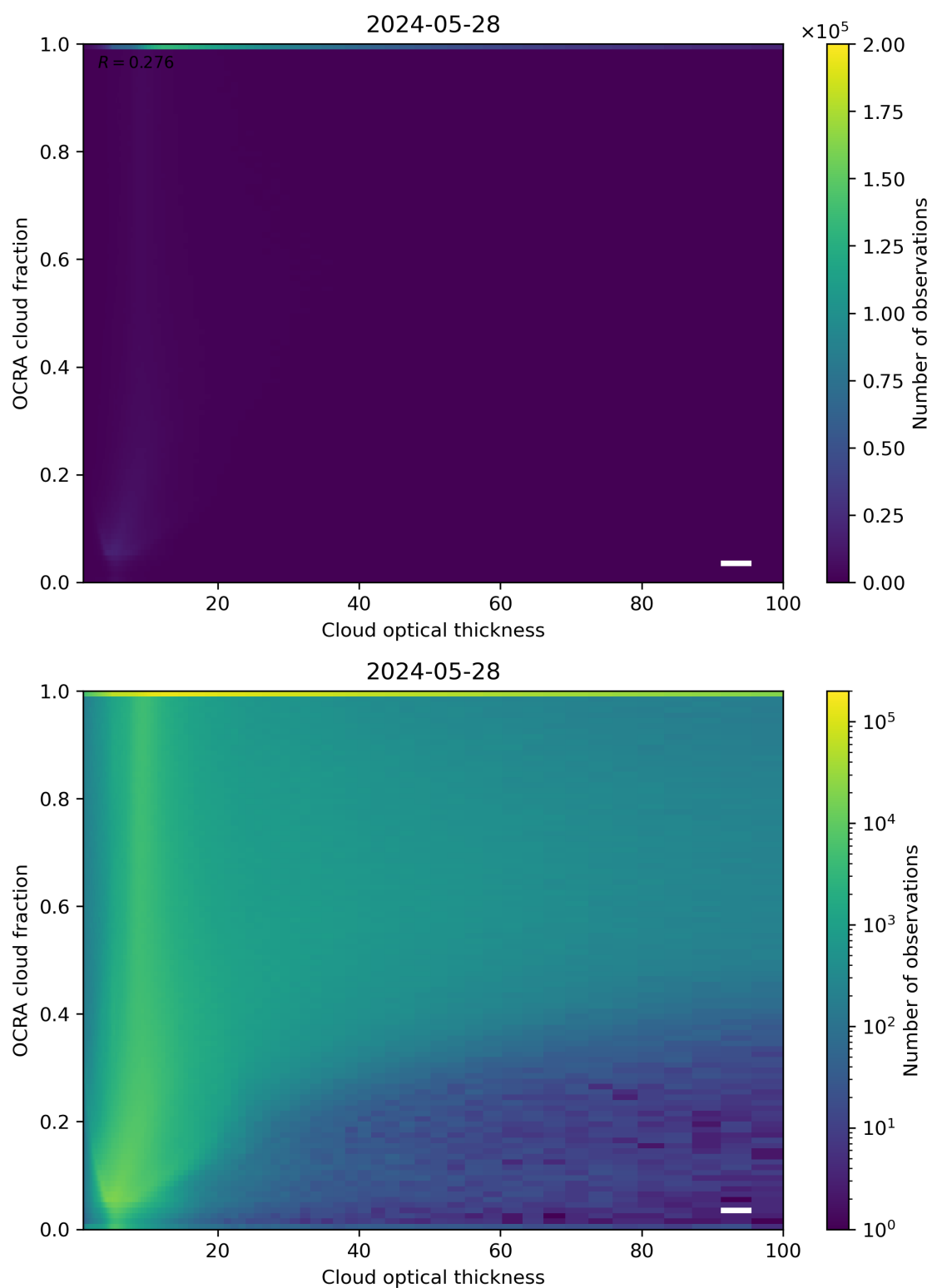
Figure 83: Scatter density plot of “Cloud optical thickness” against “OCRA cloud fraction” for 2024-05-28 to 2024-05-29.
