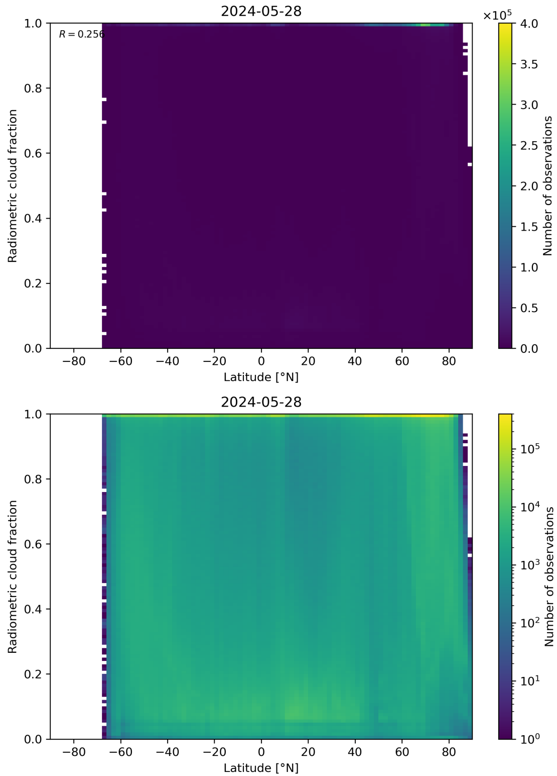
Figure 92: Scatter density plot of “Latitude” against “Radiometric cloud fraction” for 2024-05-28 to 2024-05-29.
