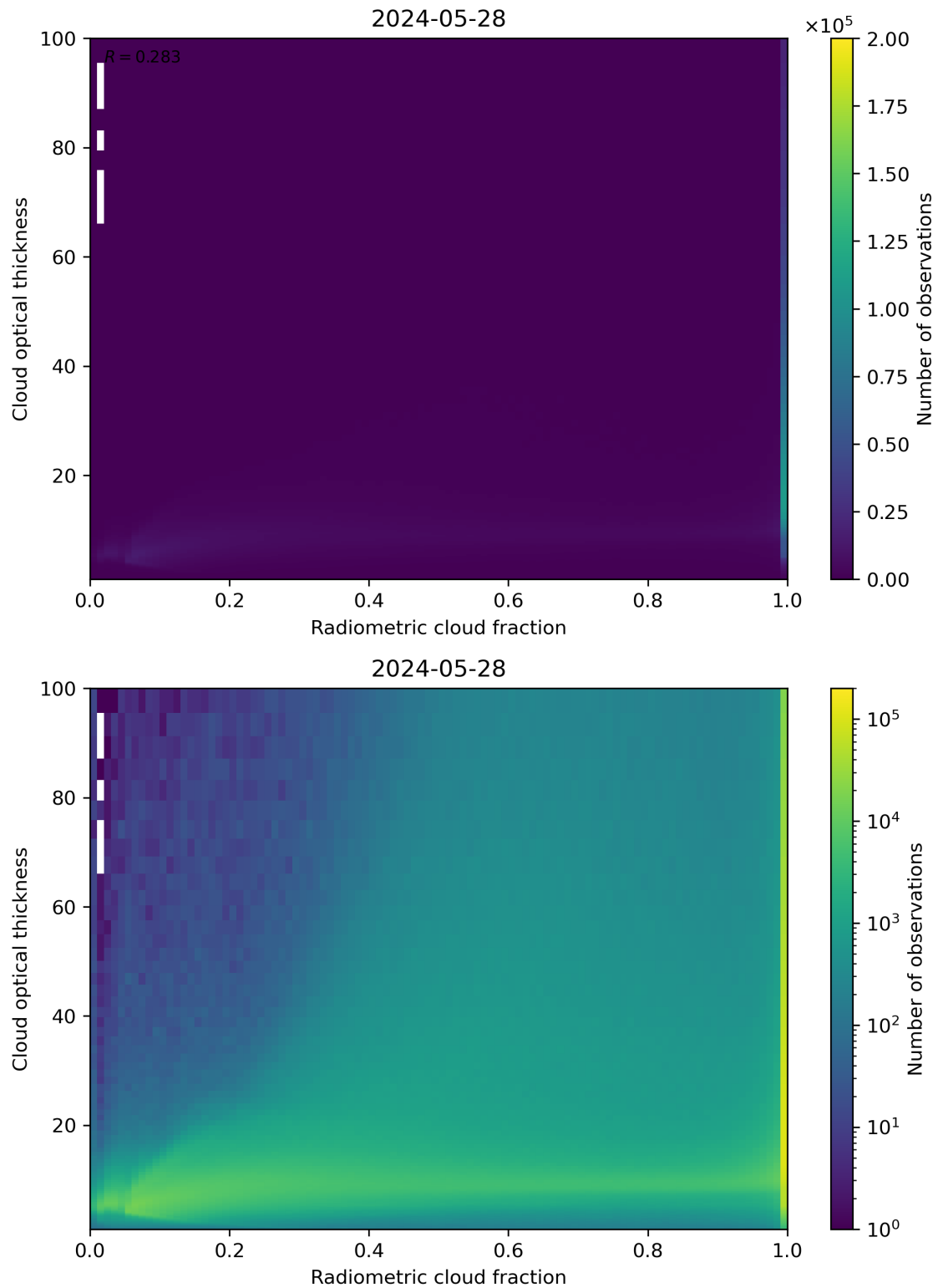
Figure 75: Scatter density plot of “Radiometric cloud fraction” against “Cloud optical thickness” for 2024-05-28 to 2024-05-29.
