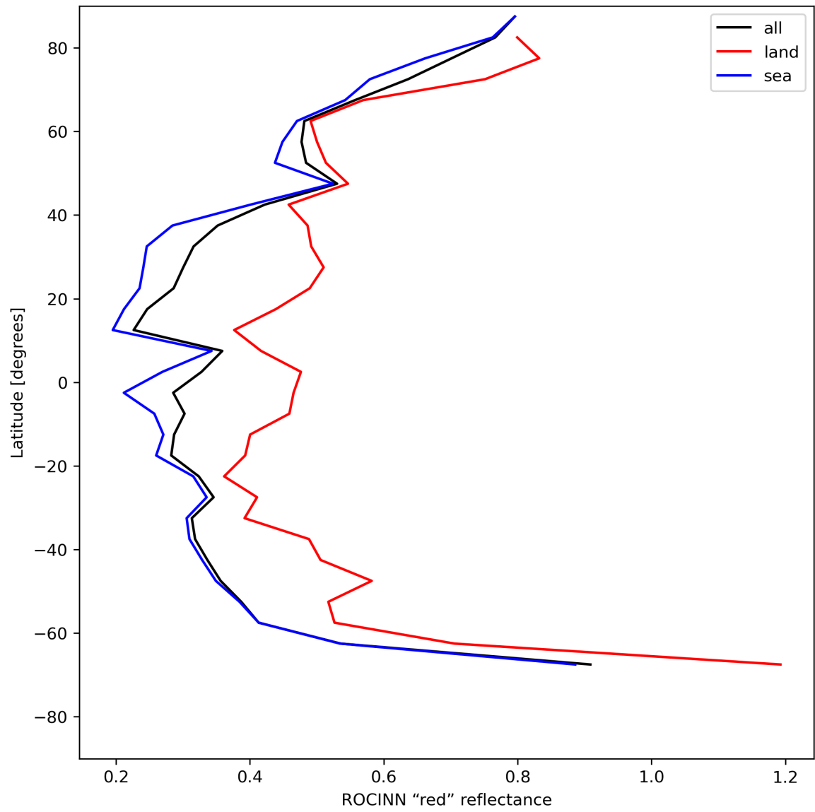
Figure 37: Zonal average of “ROCINN “red” reflectance” for 2024-05-28 to 2024-05-29.
