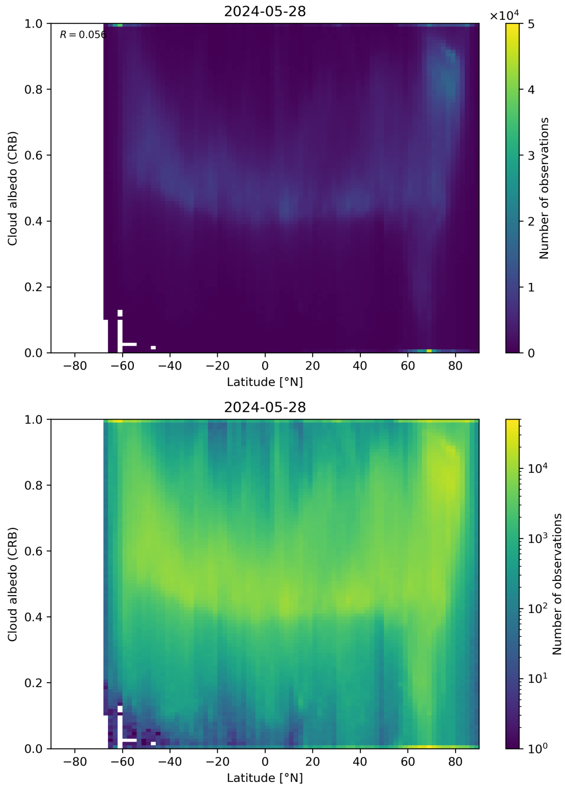
Figure 91: Scatter density plot of “Latitude” against “Cloud albedo (CRB)” for 2024-05-28 to 2024-05-29.
