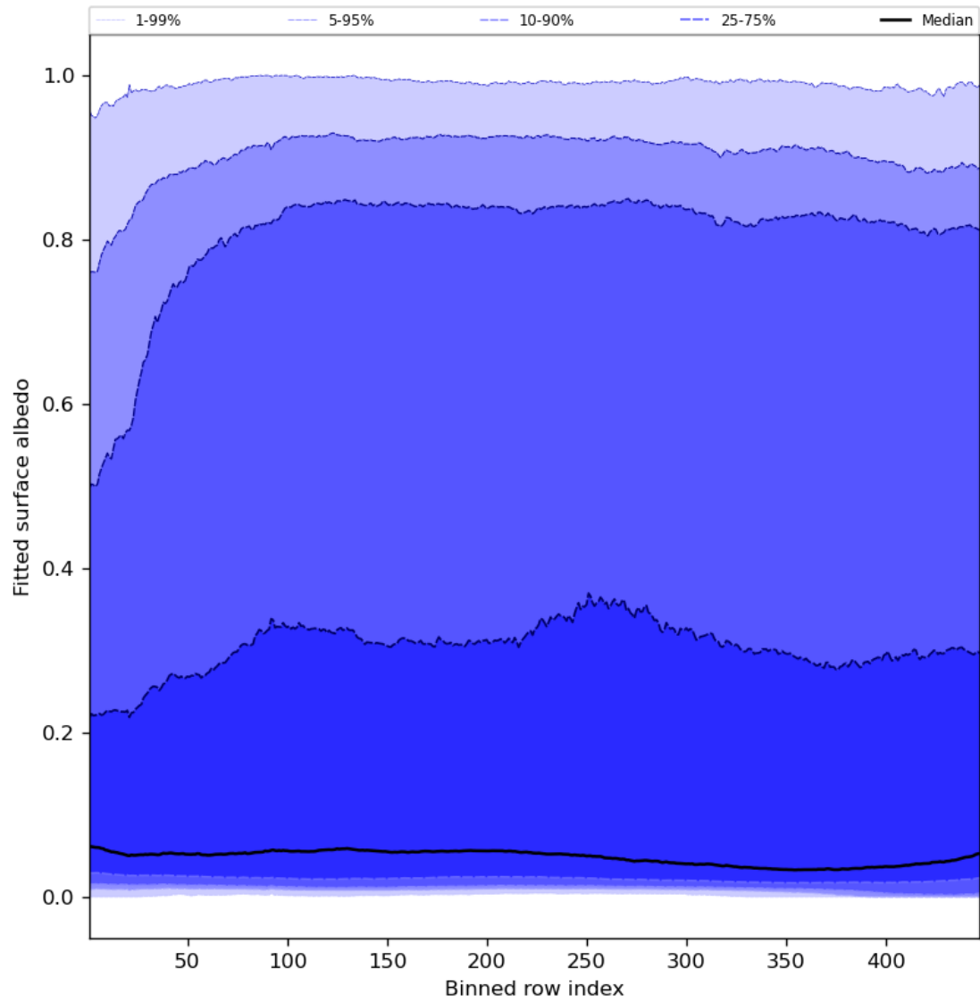
Figure 61: Along track statistics of “Fitted surface albedo” for 2024-05-28 to 2024-05-29
