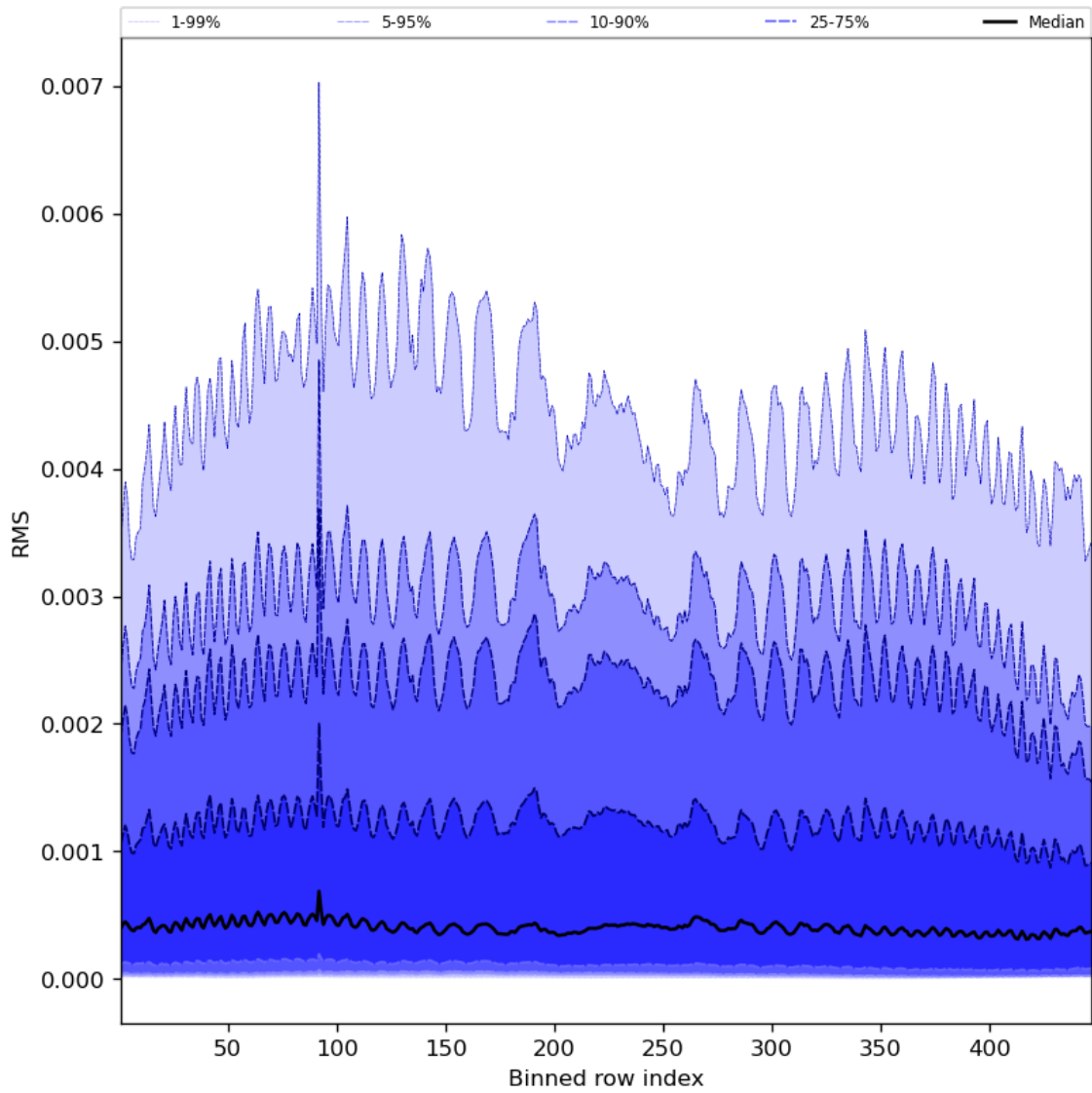
Figure 63: Along track statistics of “RMS” for 2024-05-28 to 2024-05-29
