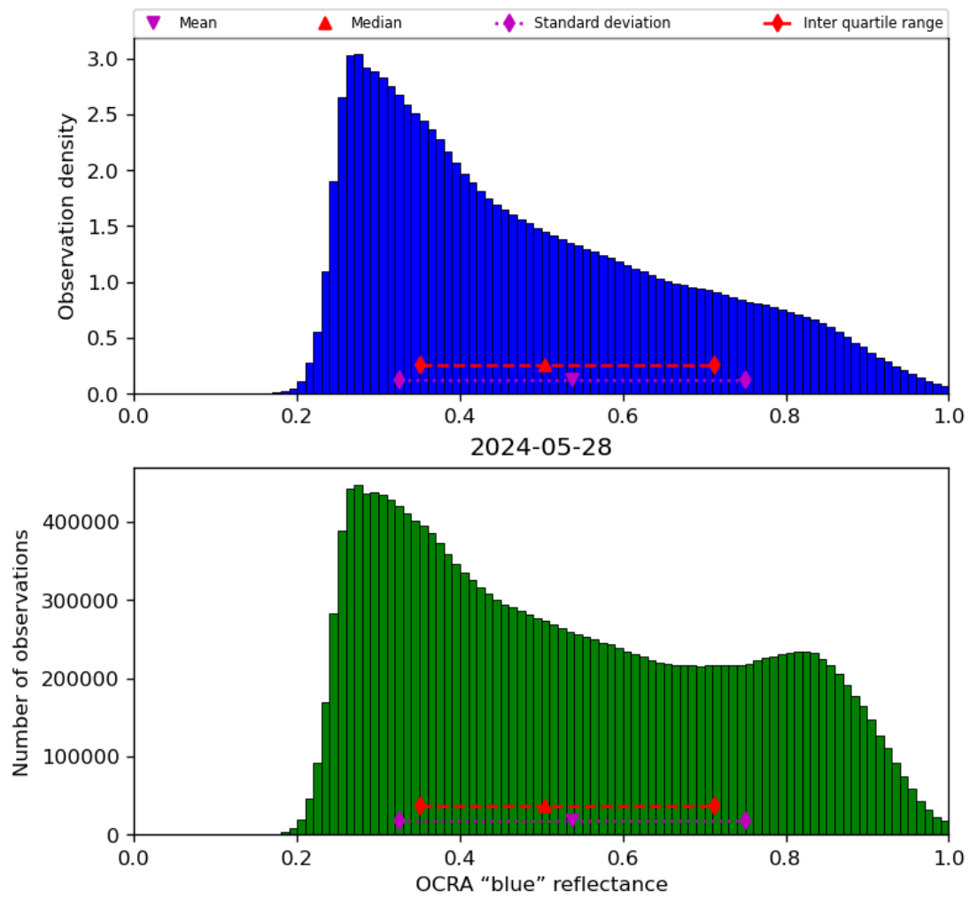
Figure 51: Histogram of “OCRA “blue” reflectance” for 2024-05-28 to 2024-05-29
