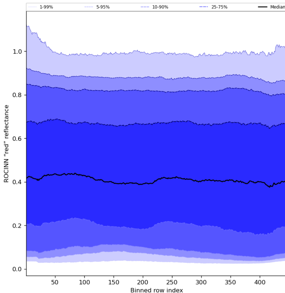
Figure 69: Along track statistics of “ROCINN “red” reflectance” for 2024-05-28 to 2024-05-29
