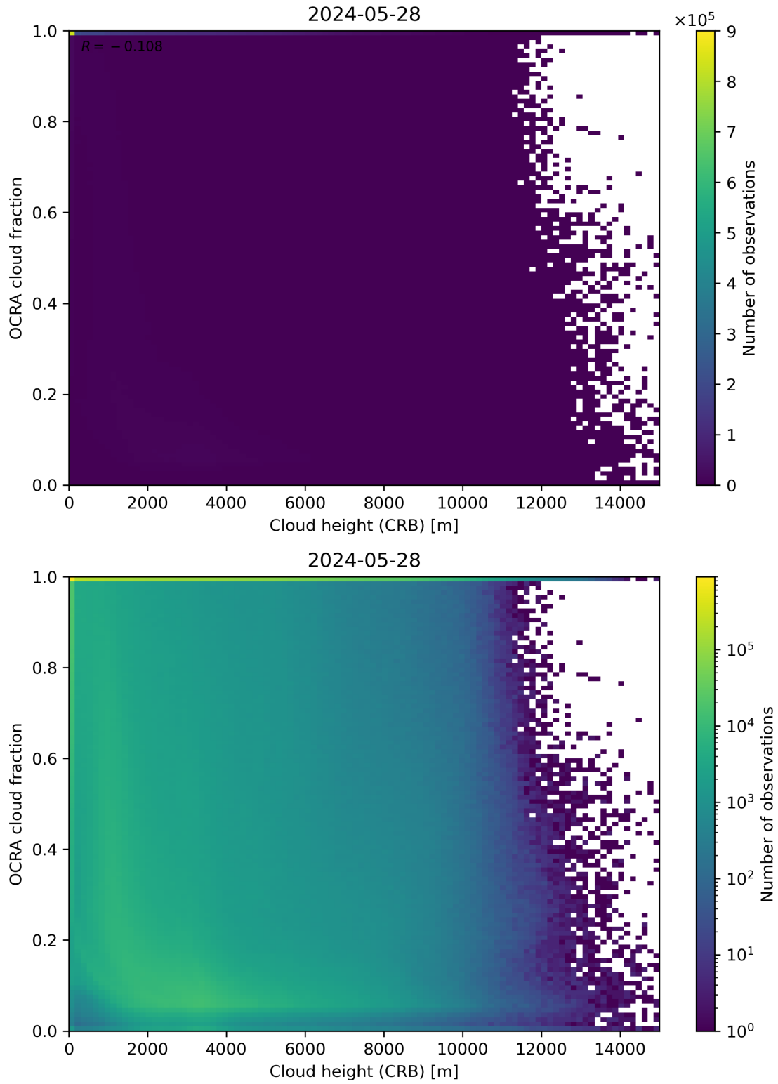
Figure 81: Scatter density plot of “Cloud height (CRB)” against “OCRA cloud fraction” for 2024-05-28 to 2024-05-29.
