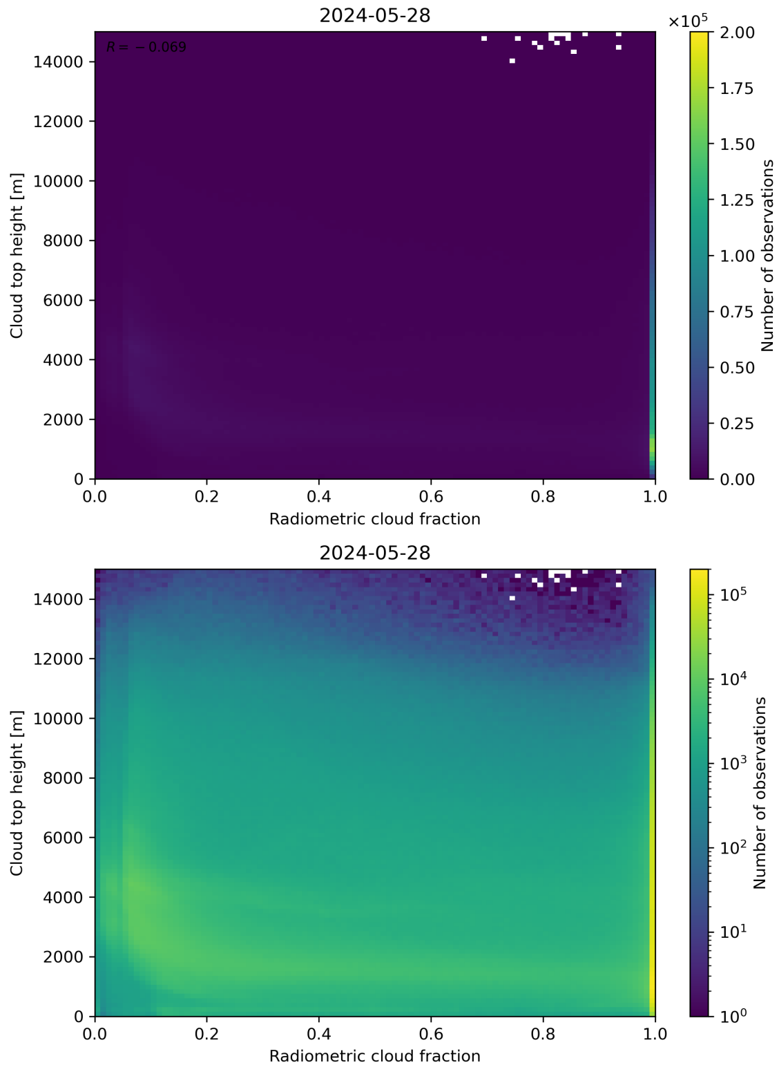
Figure 76: Scatter density plot of “Radiometric cloud fraction” against “Cloud top height” for 2024-05-28 to 2024-05-29.
