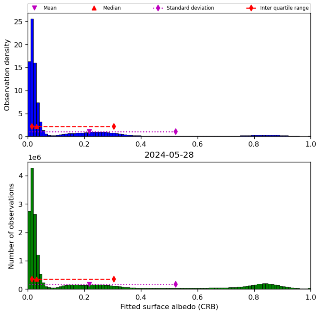
Figure 46: Histogram of “Fitted surface albedo (CRB)” for 2024-05-28 to 2024-05-29
