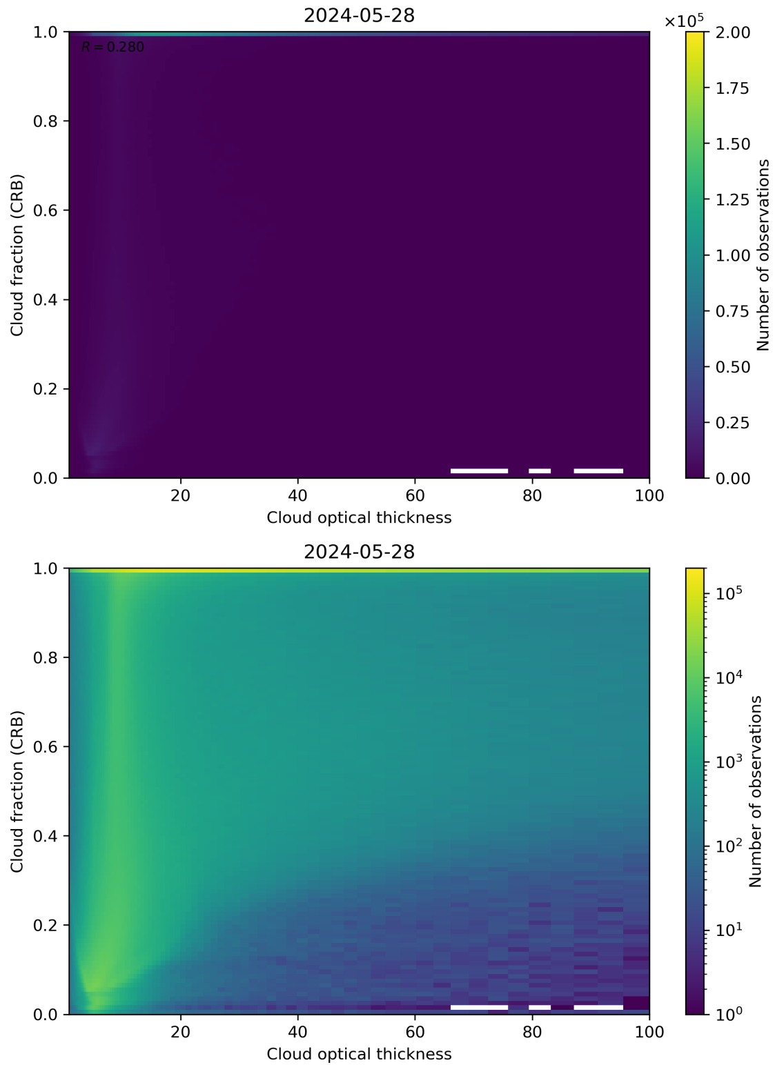
Figure 84: Scatter density plot of “Cloud optical thickness” against “Cloud fraction (CRB)” for 2024-05-28 to 2024-05-29.
