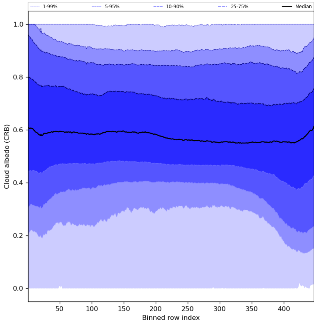
Figure 60: Along track statistics of “Cloud albedo (CRB)” for 2024-05-28 to 2024-05-29
