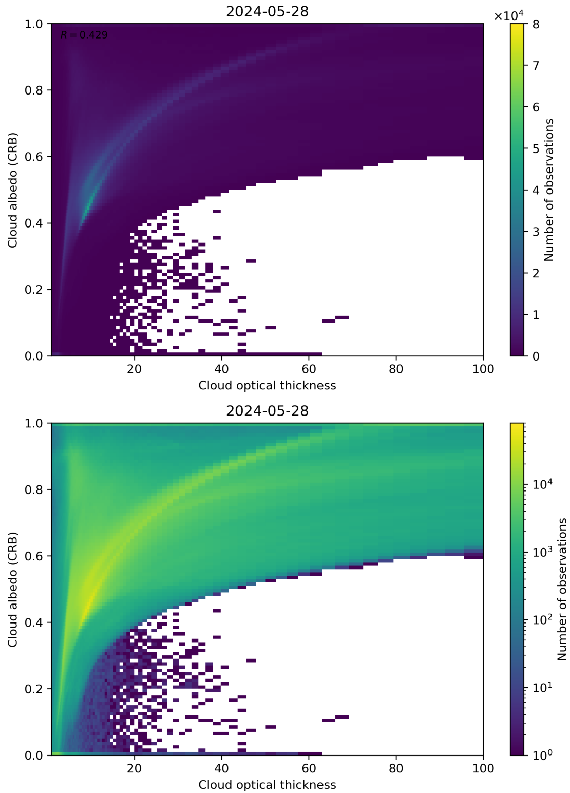
Figure 82: Scatter density plot of “Cloud optical thickness” against “Cloud albedo (CRB)” for 2024-05-28 to 2024-05-29.
