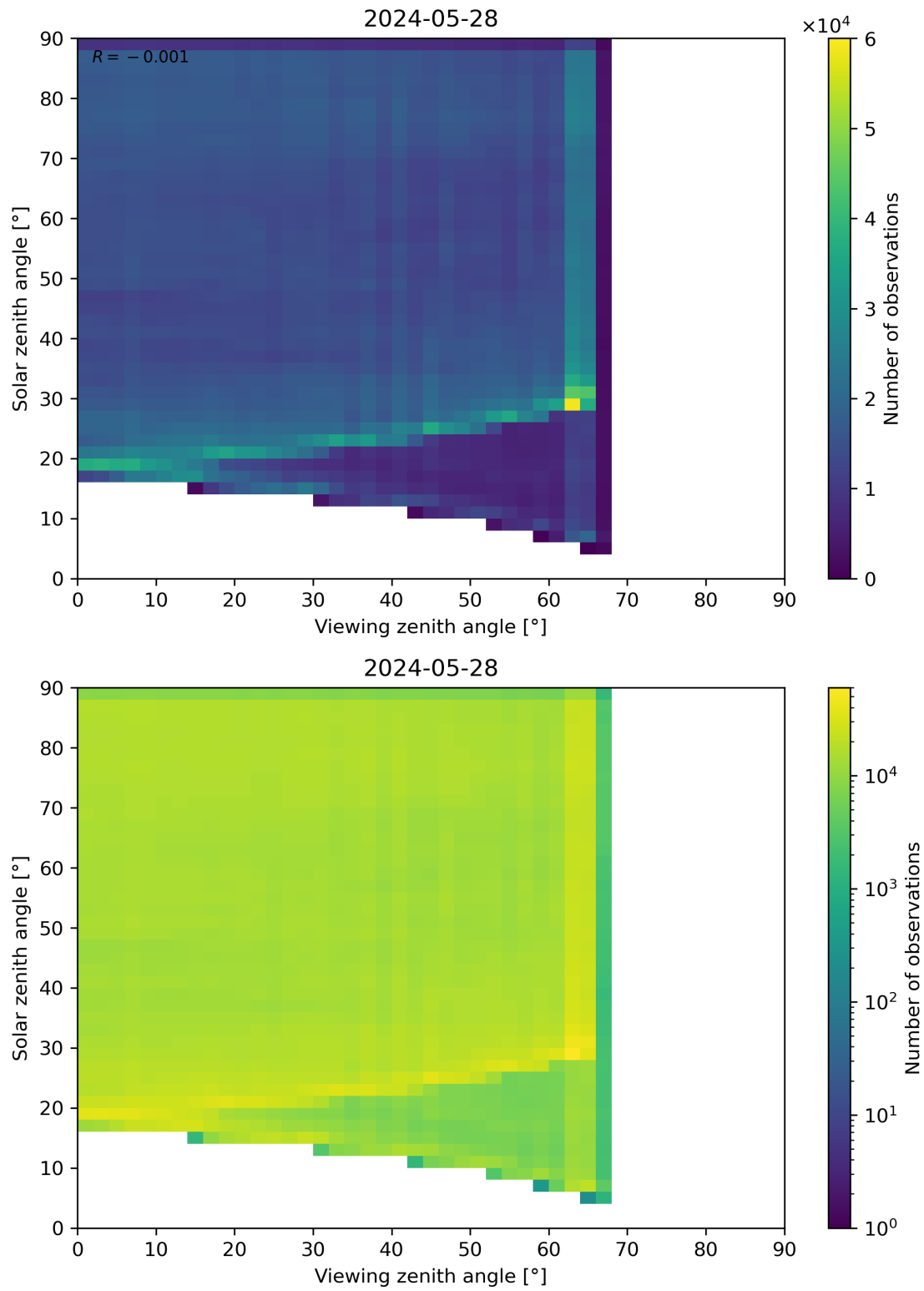
Figure 114: Scatter density plot of “Viewing zenith angle” against “Solar zenith angle” for 2024-05-28 to 2024-05-29.
