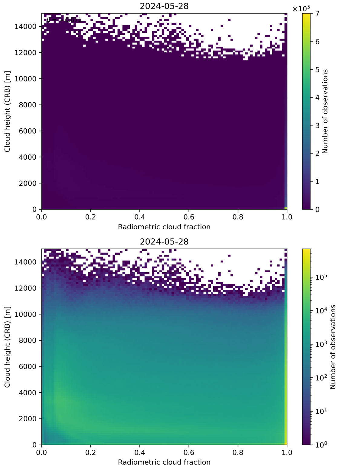
Figure 74: Scatter density plot of “Radiometric cloud fraction” against “Cloud height (CRB)” for 2024-05-28 to 2024-05-29.
