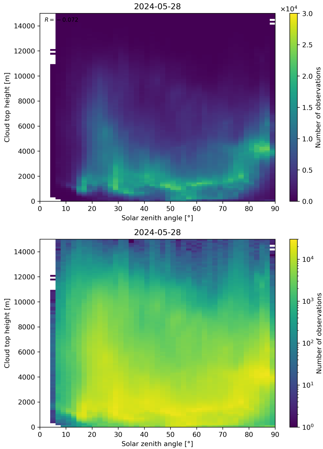
Figure 104: Scatter density plot of “Solar zenith angle” against “Cloud top height” for 2024-05-28 to 2024-05-29.
