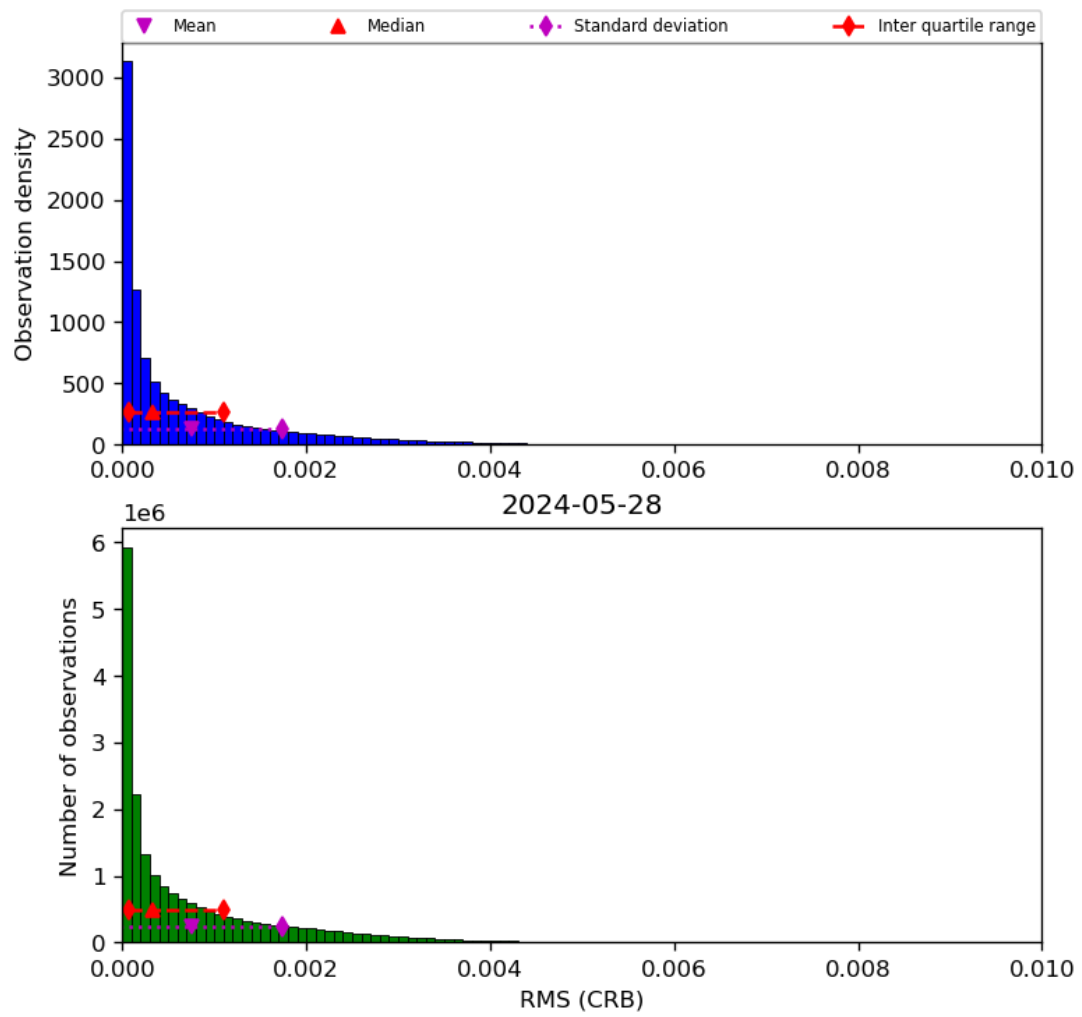
Figure 48: Histogram of "RMS (CRB)" for 2024-05-28 to 2024-05-29
