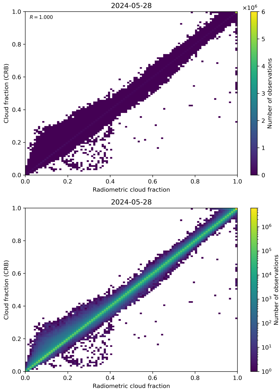
Figure 73: Scatter density plot of “Radiometric cloud fraction” against “Cloud fraction (CRB)” for 2024-05-28 to 2024-05-29.
