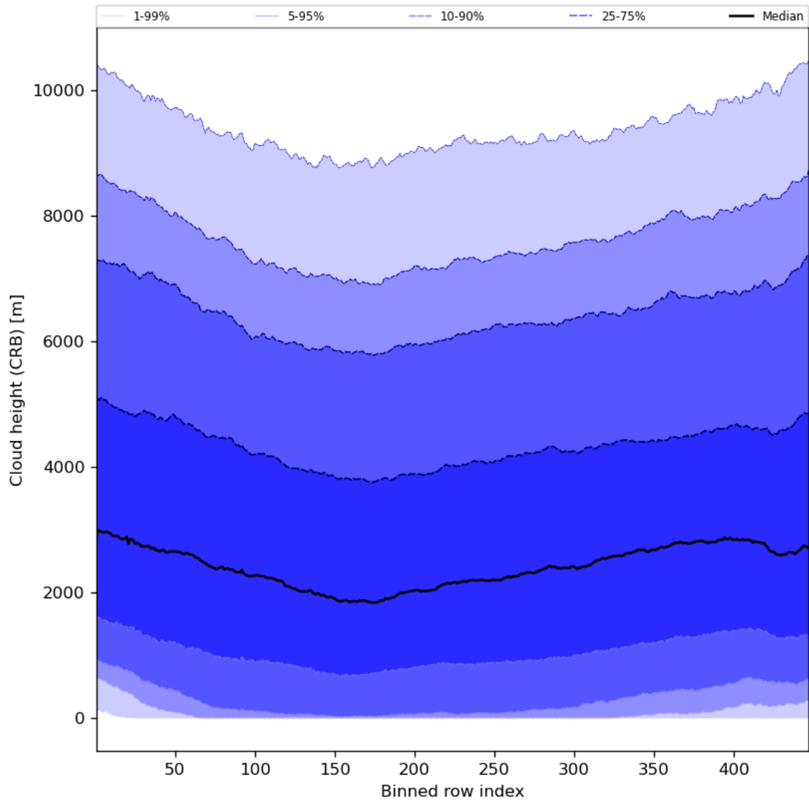
Figure 59: Along track statistics of “Cloud height (CRB)” for 2024-05-28 to 2024-05-29
