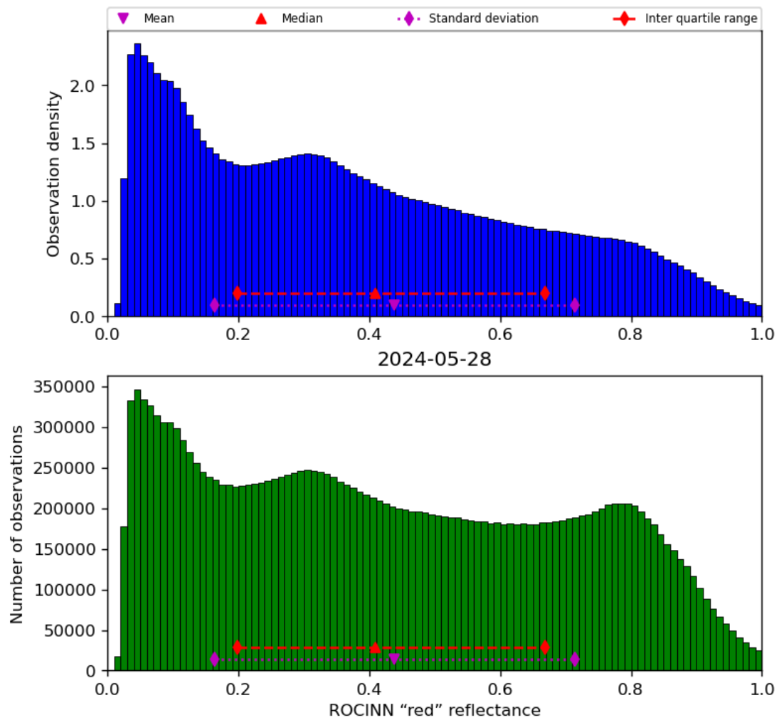
Figure 53: Histogram of “ROCINN “red” reflectance” for 2024-05-28 to 2024-05-29
