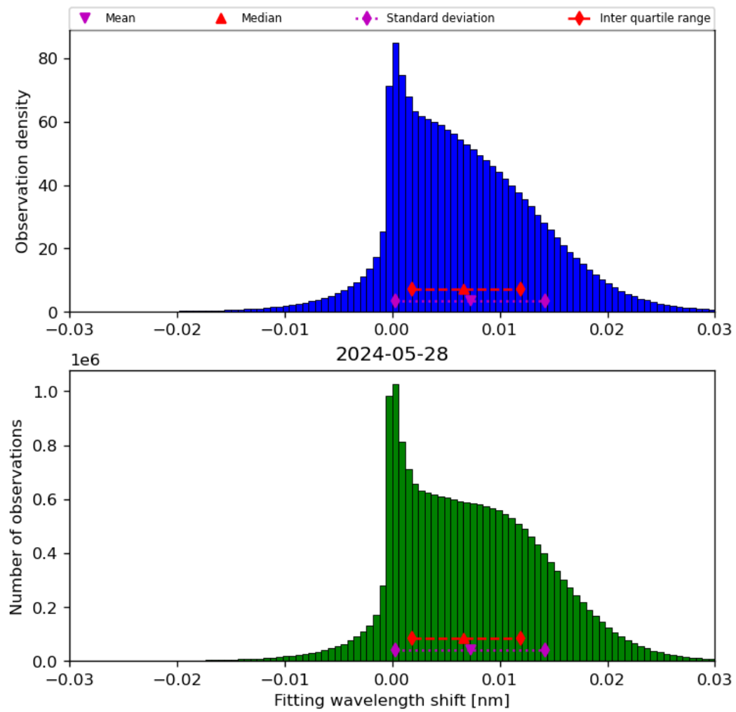
Figure 49: Histogram of “Fitting wavelength shift” for 2024-05-28 to 2024-05-29
