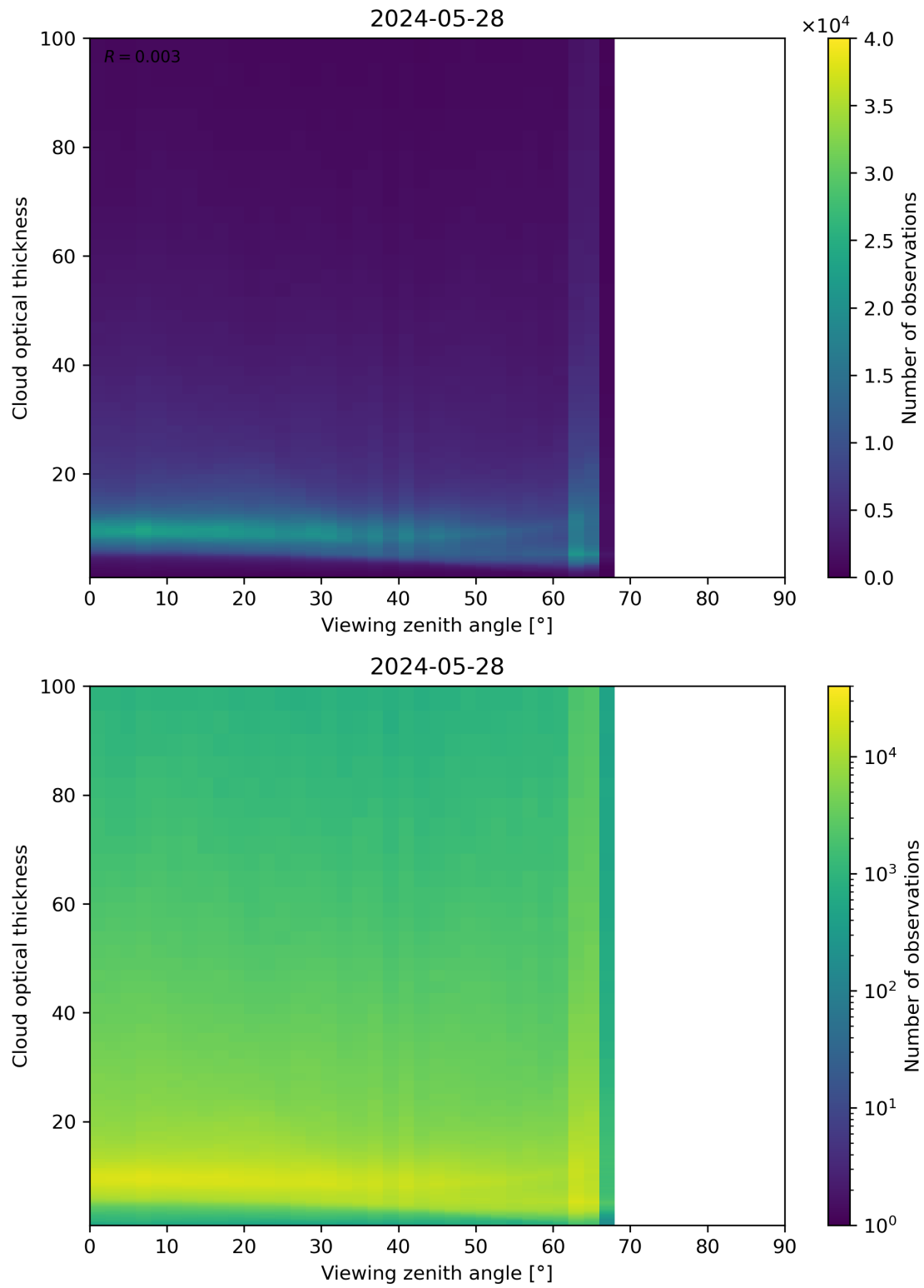
Figure 111: Scatter density plot of “Viewing zenith angle” against “Cloud optical thickness” for 2024-05-28 to 2024-05-29.
