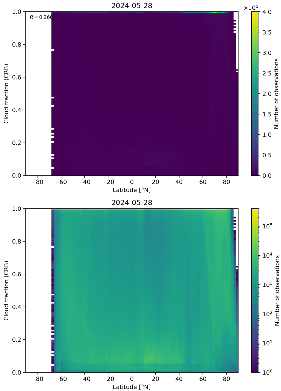
Figure 94: Scatter density plot of “Latitude” against “Cloud fraction (CRB)” for 2024-05-28 to 2024-05-29.
