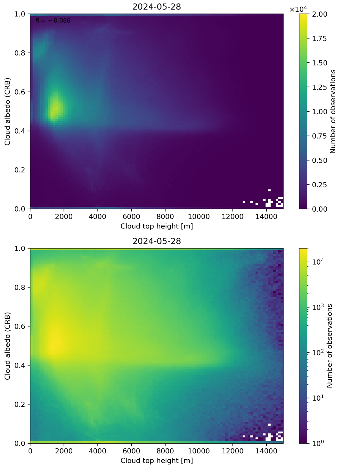
Figure 86: Scatter density plot of “Cloud top height” against “Cloud albedo (CRB)” for 2024-05-28 to 2024-05-29.
