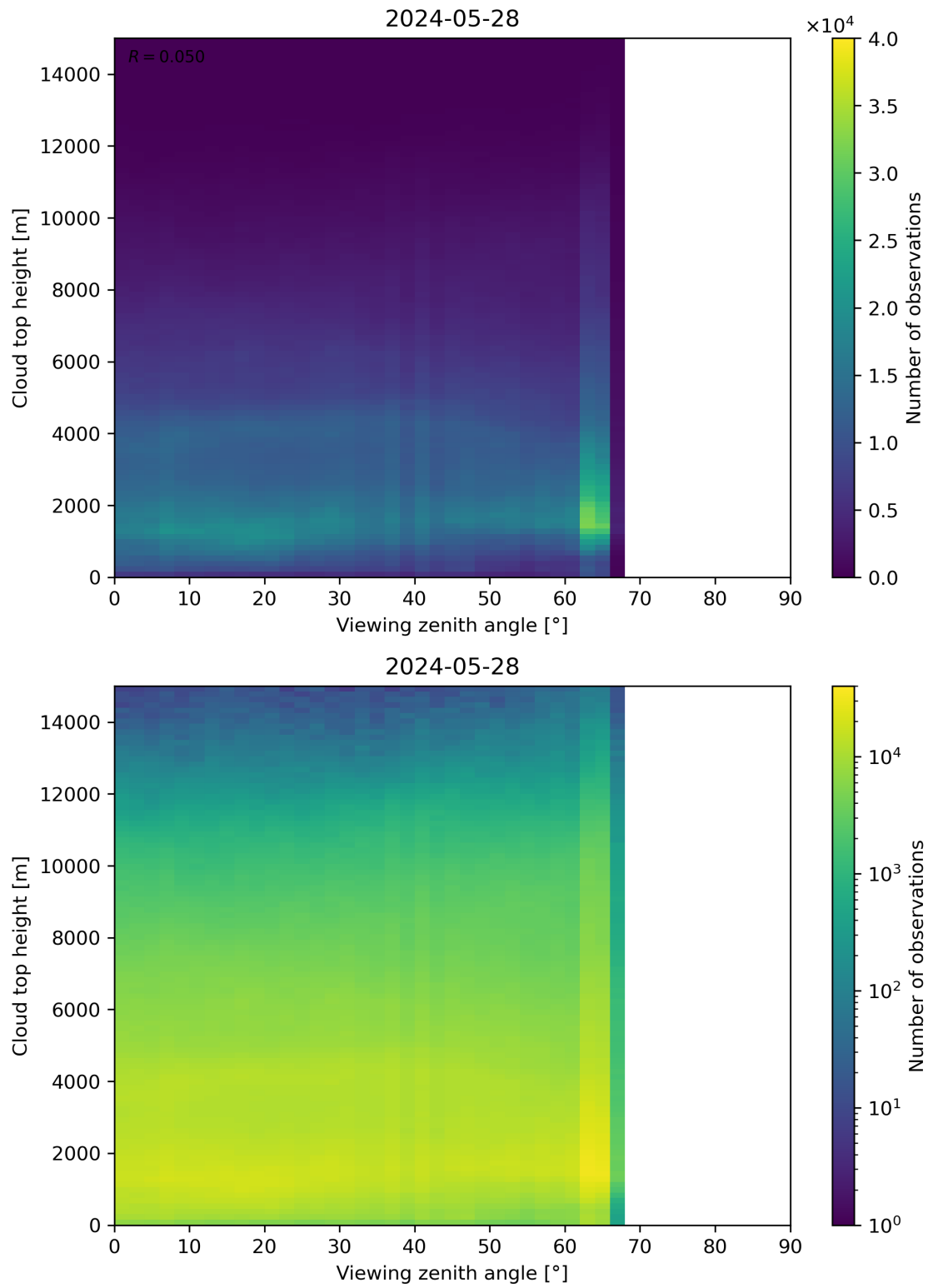
Figure 112: Scatter density plot of “Viewing zenith angle” against “Cloud top height” for 2024-05-28 to 2024-05-29.
