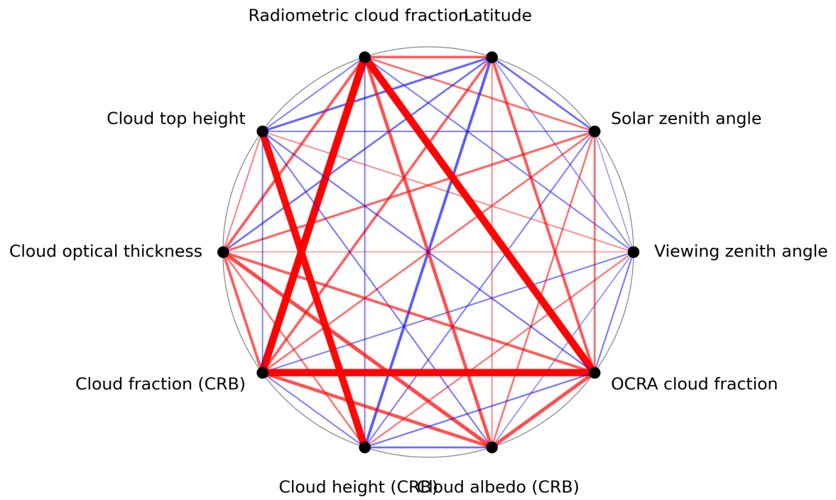
Figure 1: Map of correlation graph for 2024-05-28 to 2024-05-29.
