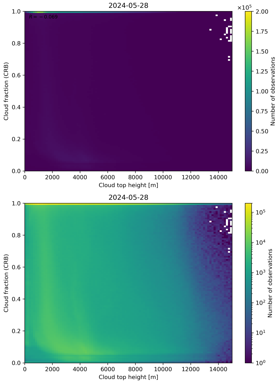
Figure 88: Scatter density plot of “Cloud top height” against “Cloud fraction (CRB)” for 2024-05-28 to 2024-05-29.
