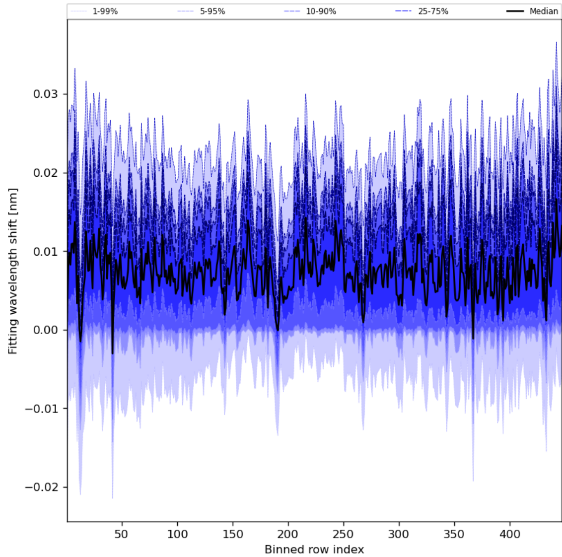
Figure 65: Along track statistics of “Fitting wavelength shift” for 2024-05-28 to 2024-05-29
