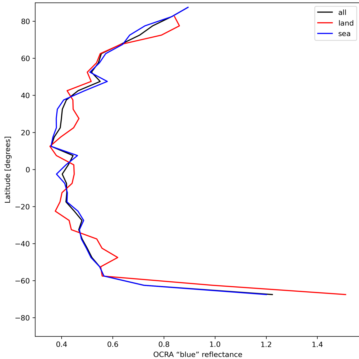
Figure 35: Zonal average of “OCRA “blue” reflectance” for 2024-05-28 to 2024-05-29.
