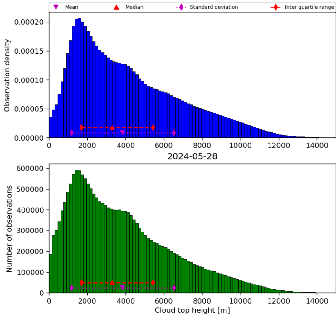
Figure 40: Histogram of “Cloud top height” for 2024-05-28 to 2024-05-29
