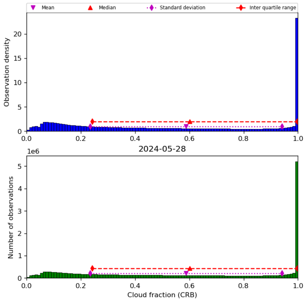
Figure 42: Histogram of “Cloud fraction (CRB)” for 2024-05-28 to 2024-05-29
