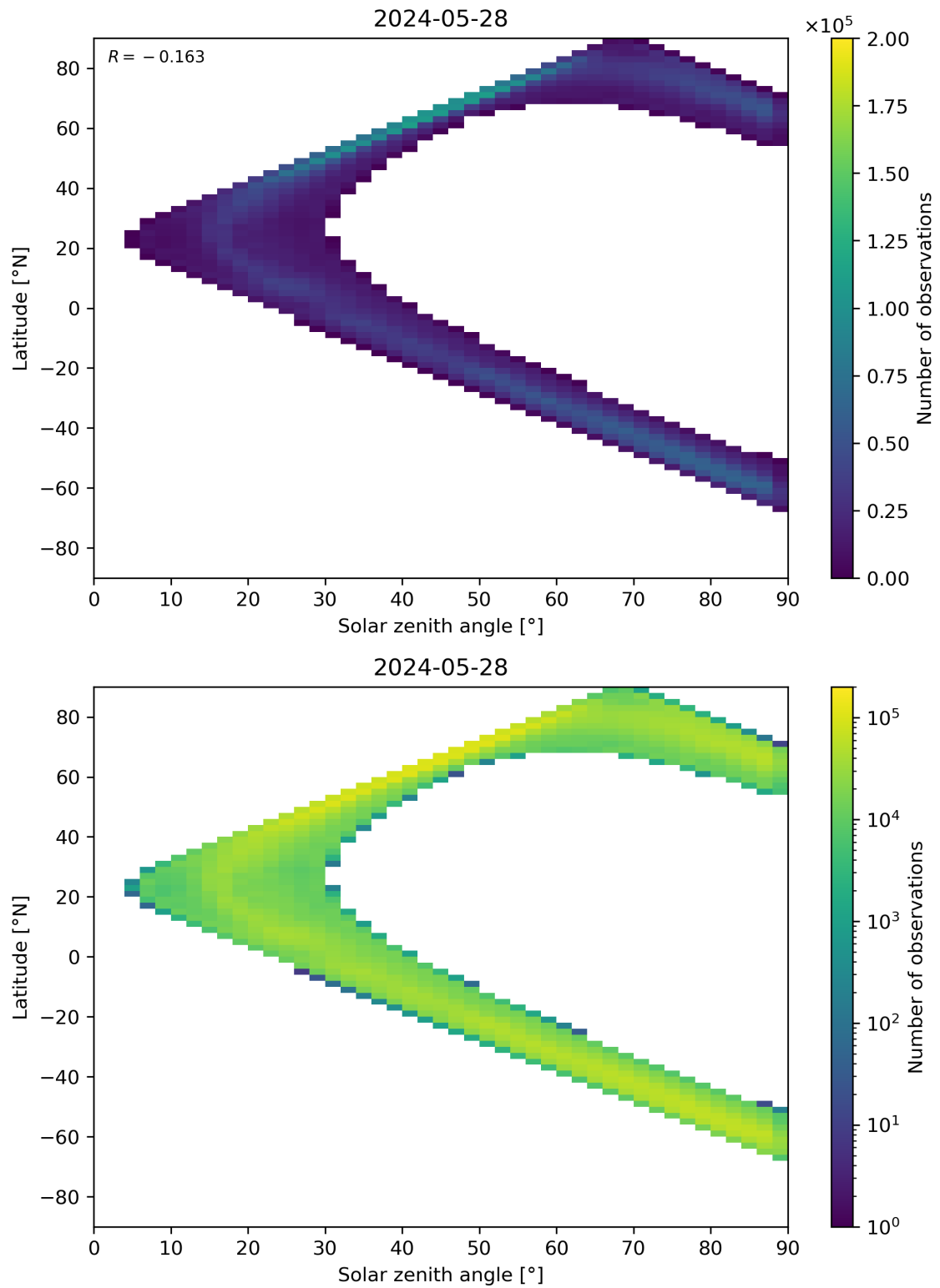
Figure 105: Scatter density plot of “Solar zenith angle” against “Latitude” for 2024-05-28 to 2024-05-29.
