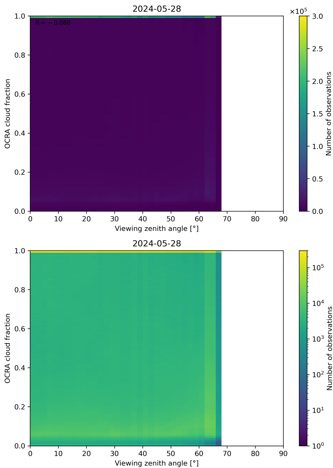
Figure 108: Scatter density plot of “Viewing zenith angle” against “OCRA cloud fraction” for 2024-05-28 to 2024-05-29.
