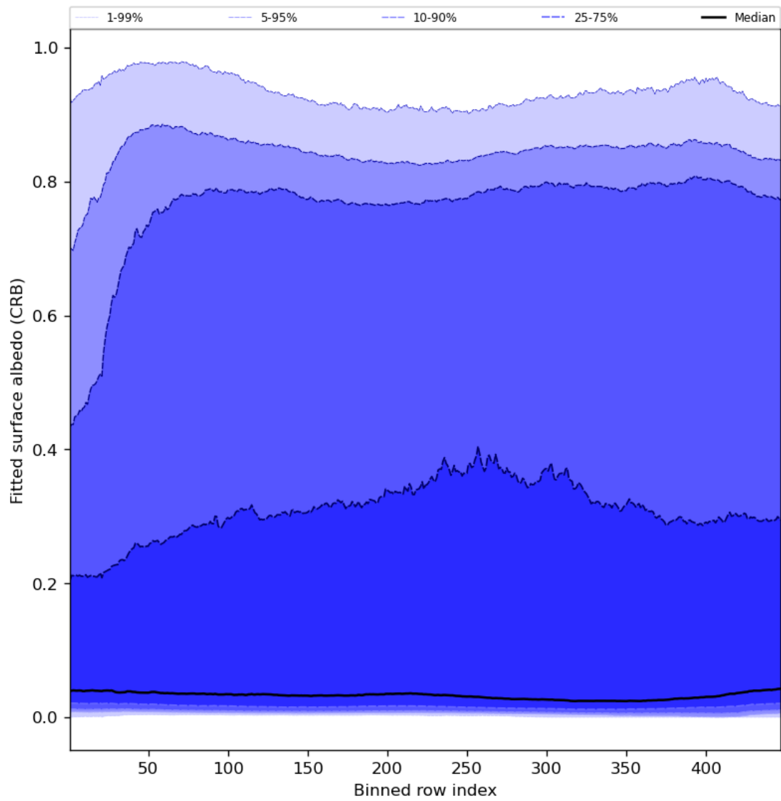
Figure 62: Along track statistics of “Fitted surface albedo (CRB)” for 2024-05-29 to 2024-05-31
