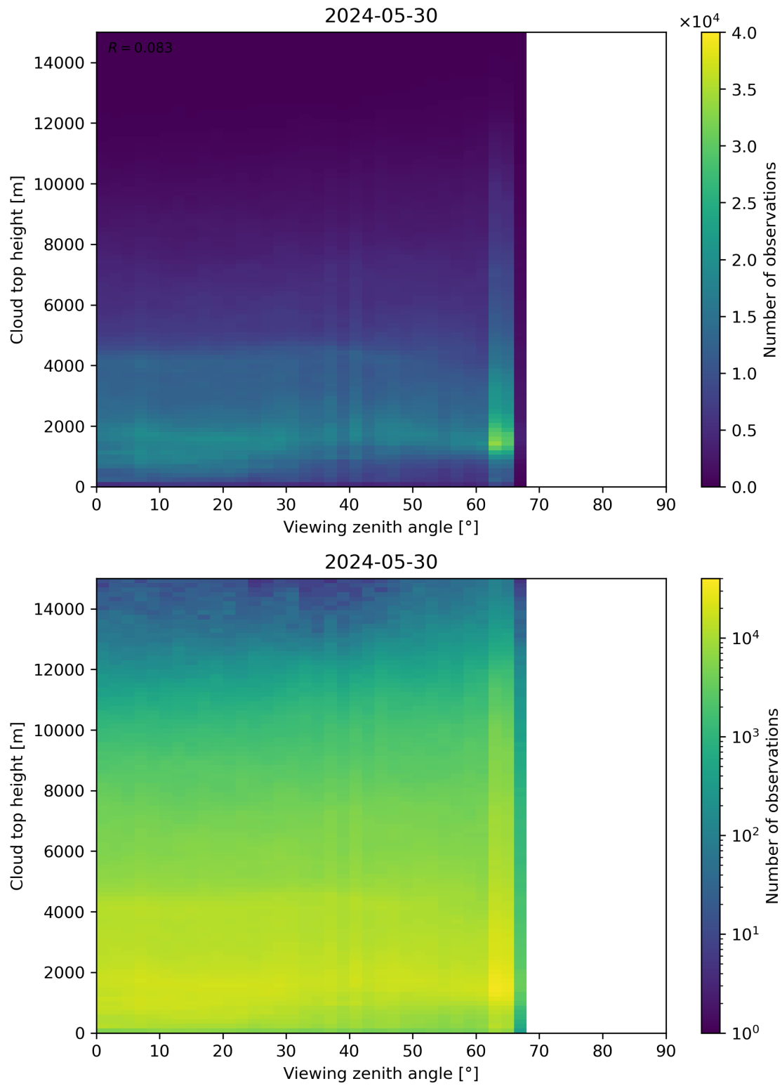
Figure 112: Scatter density plot of “Viewing zenith angle” against “Cloud top height” for 2024-05-29 to 2024-05-31.
