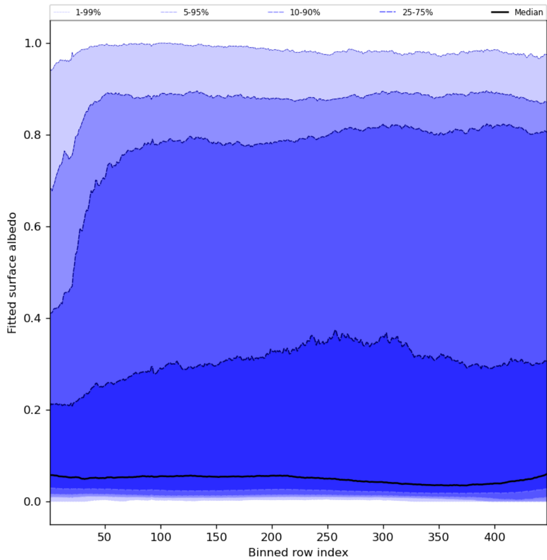
Figure 61: Along track statistics of “Fitted surface albedo” for 2024-05-29 to 2024-05-31
