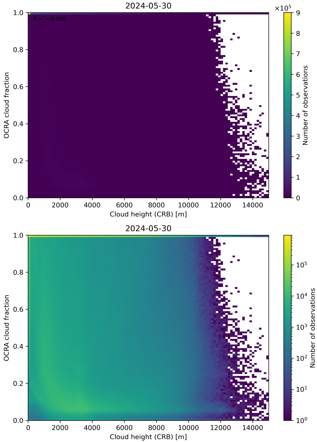
Figure 81: Scatter density plot of “Cloud height (CRB)” against “OCRA cloud fraction” for 2024-05-29 to 2024-05-31.
