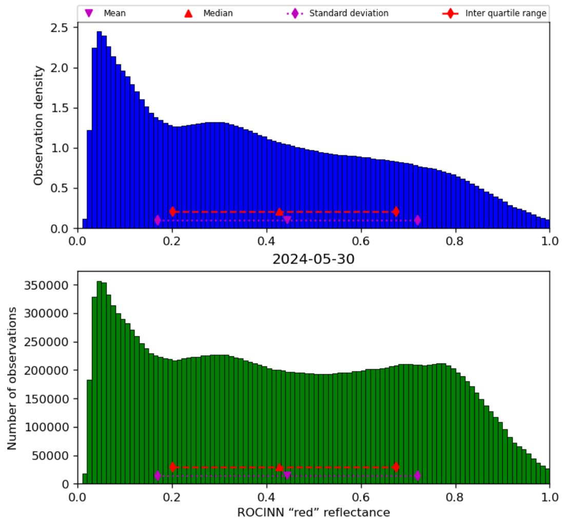
Figure 53: Histogram of “ROCINN “red” reflectance” for 2024-05-29 to 2024-05-31
