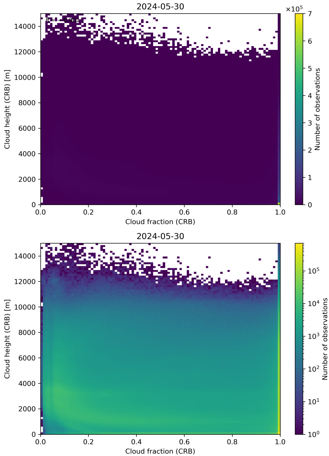
Figure 79: Scatter density plot of “Cloud fraction (CRB)” against “Cloud height (CRB)” for 2024-05-29 to 2024-05-31.
