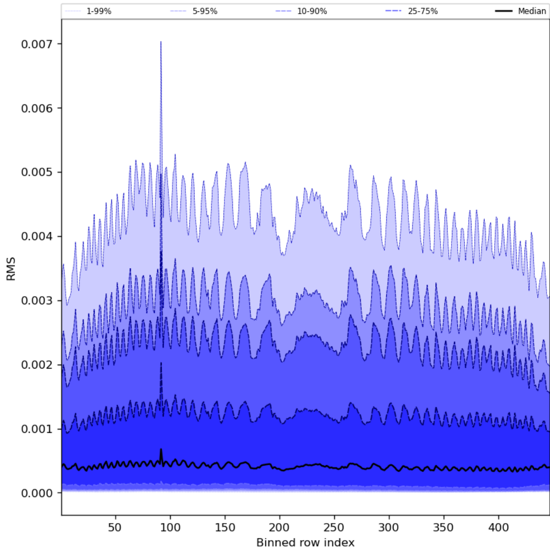
Figure 63: Along track statistics of “RMS” for 2024-05-29 to 2024-05-31
