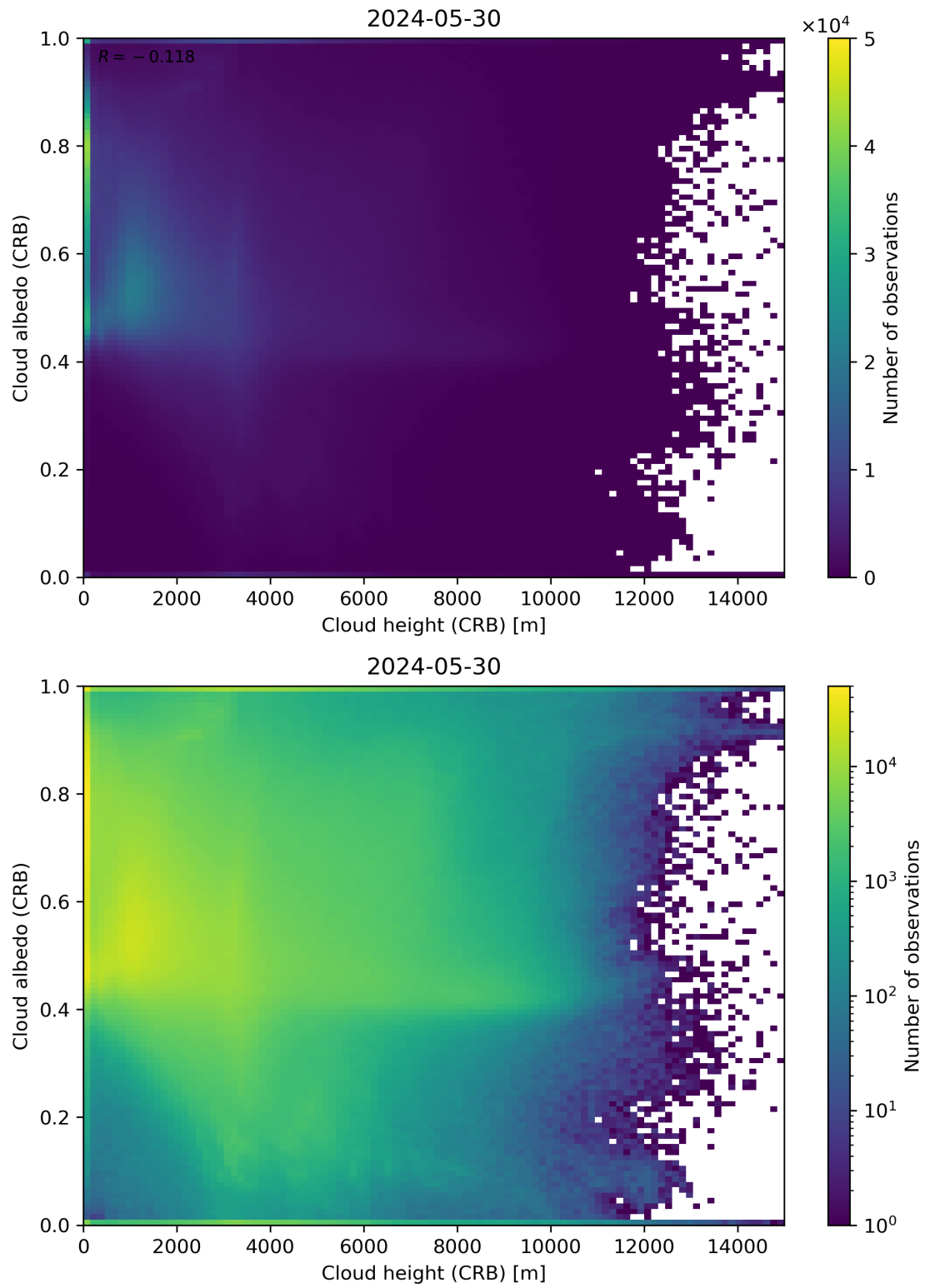
Figure 80: Scatter density plot of “Cloud height (CRB)” against “Cloud albedo (CRB)” for 2024-05-29 to 2024-05-31.
