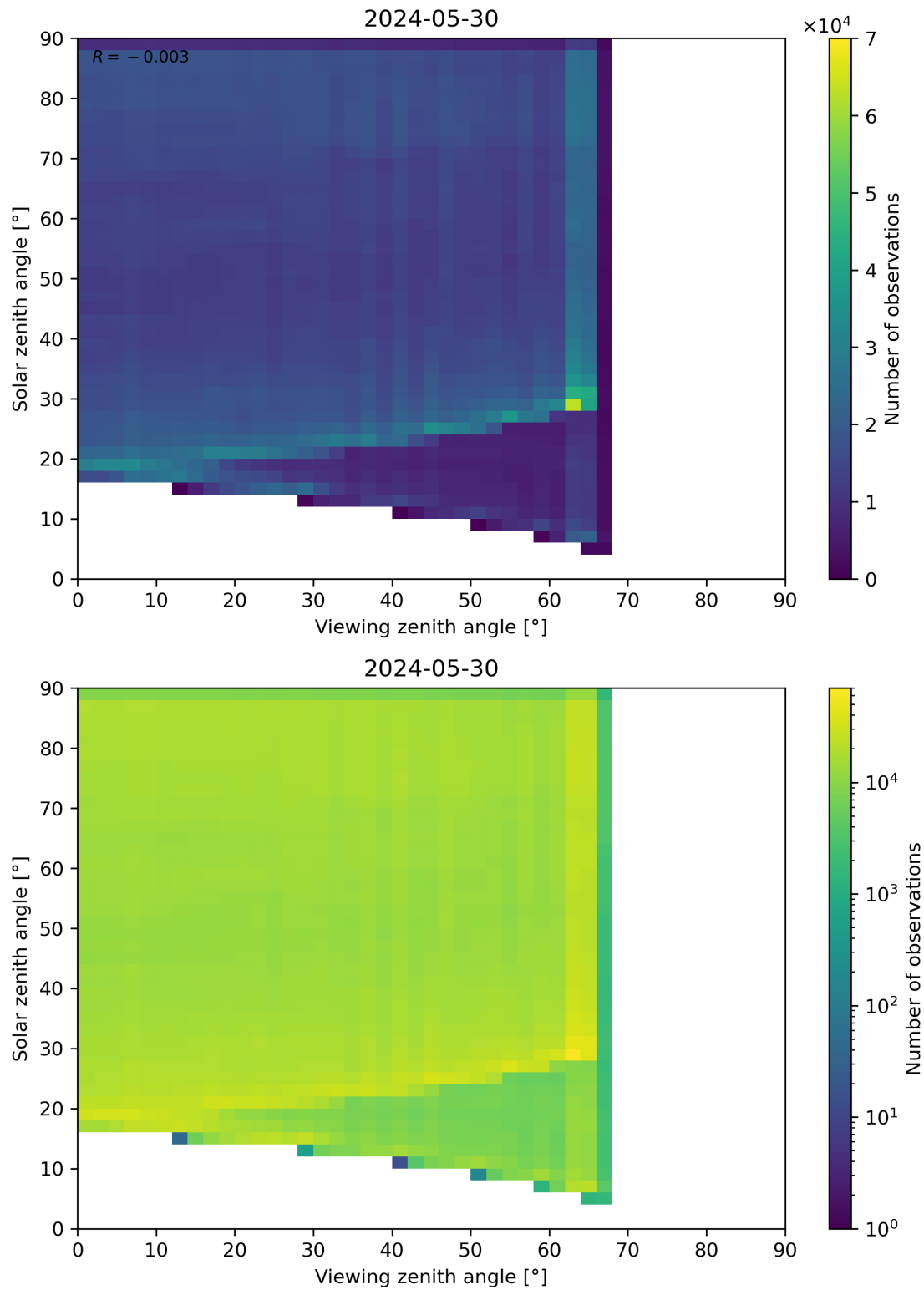
Figure 114: Scatter density plot of “Viewing zenith angle” against “Solar zenith angle” for 2024-05-29 to 2024-05-31.
