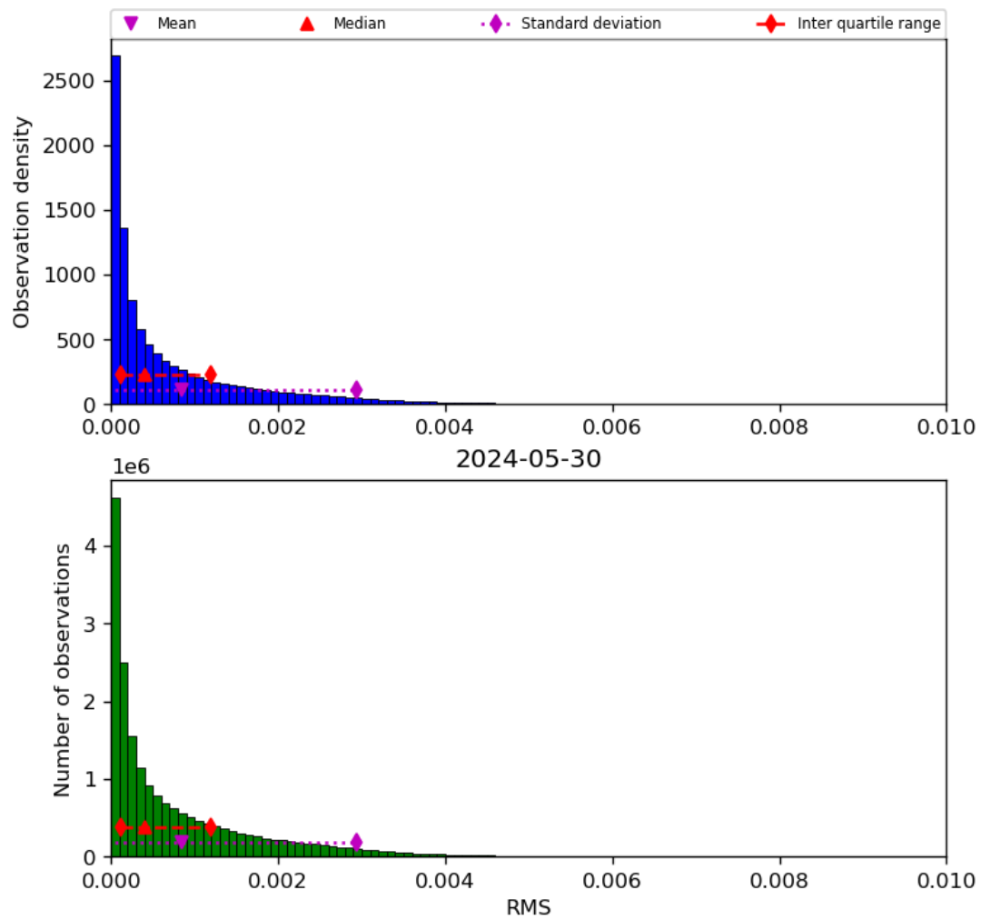
Figure 47: Histogram of “RMS” for 2024-05-29 to 2024-05-31
