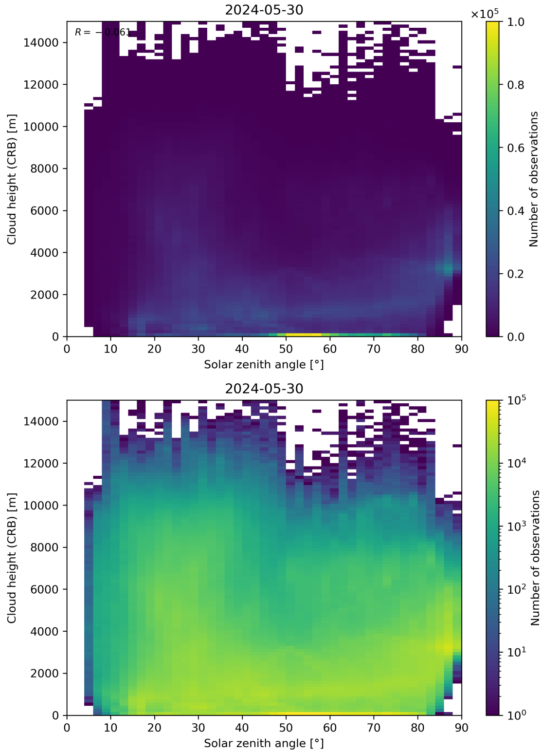
Figure 102: Scatter density plot of “Solar zenith angle” against “Cloud height (CRB)” for 2024-05-29 to 2024-05-31.
