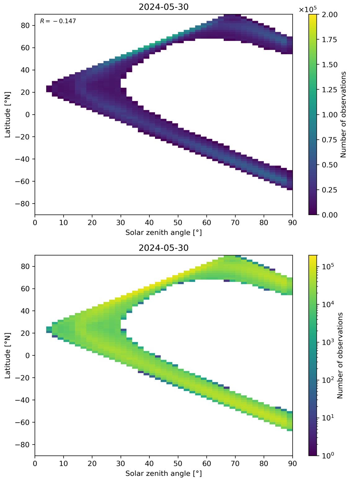
Figure 105: Scatter density plot of “Solar zenith angle” against “Latitude” for 2024-05-29 to 2024-05-31.
