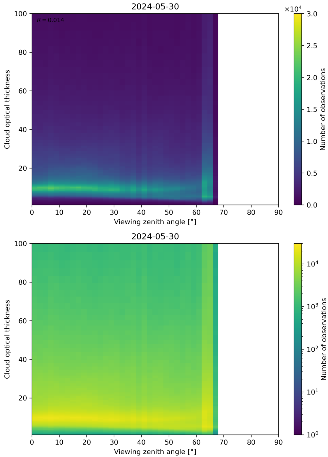
Figure 111: Scatter density plot of “Viewing zenith angle” against “Cloud optical thickness” for 2024-05-29 to 2024-05-31.
