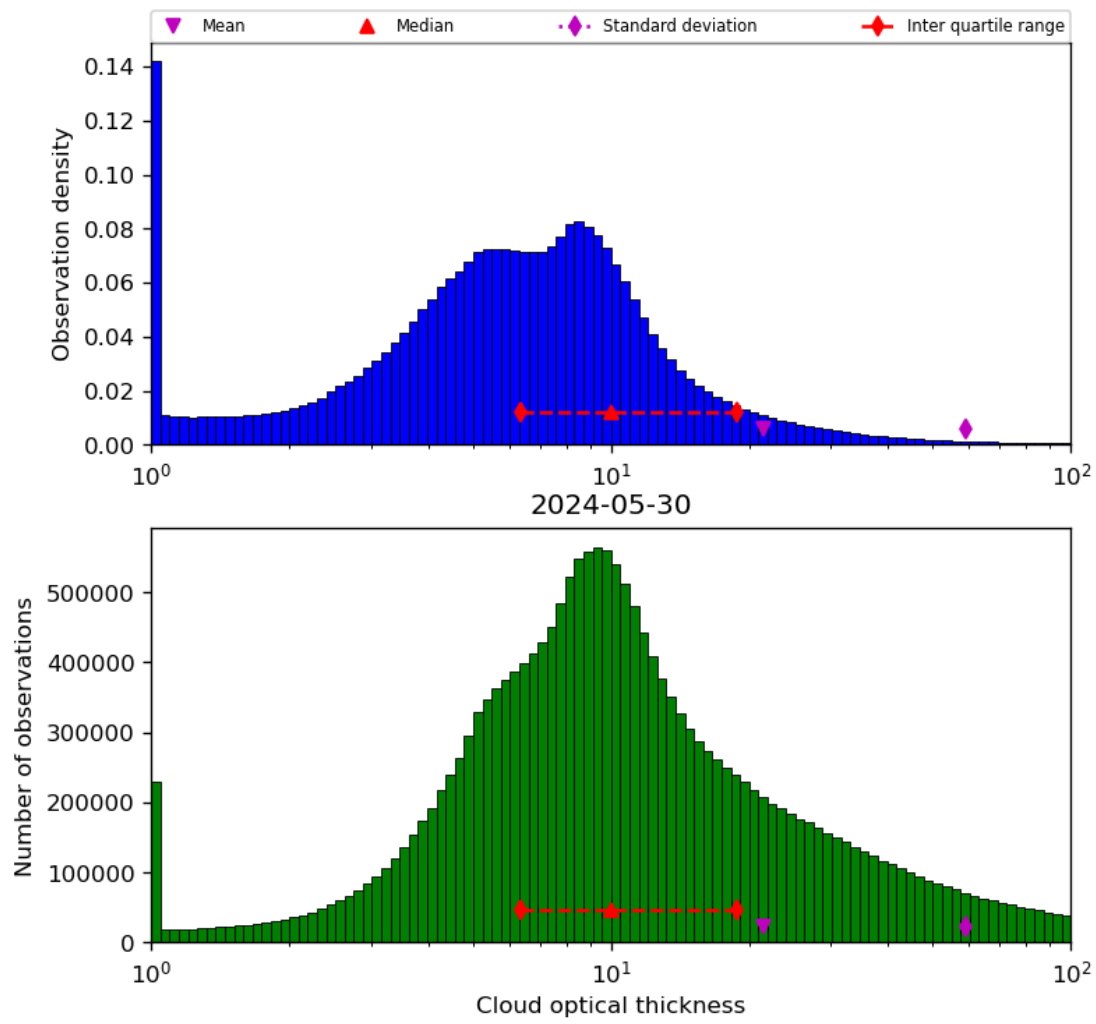
Figure 41: Histogram of “Cloud optical thickness” for 2024-05-29 to 2024-05-31
