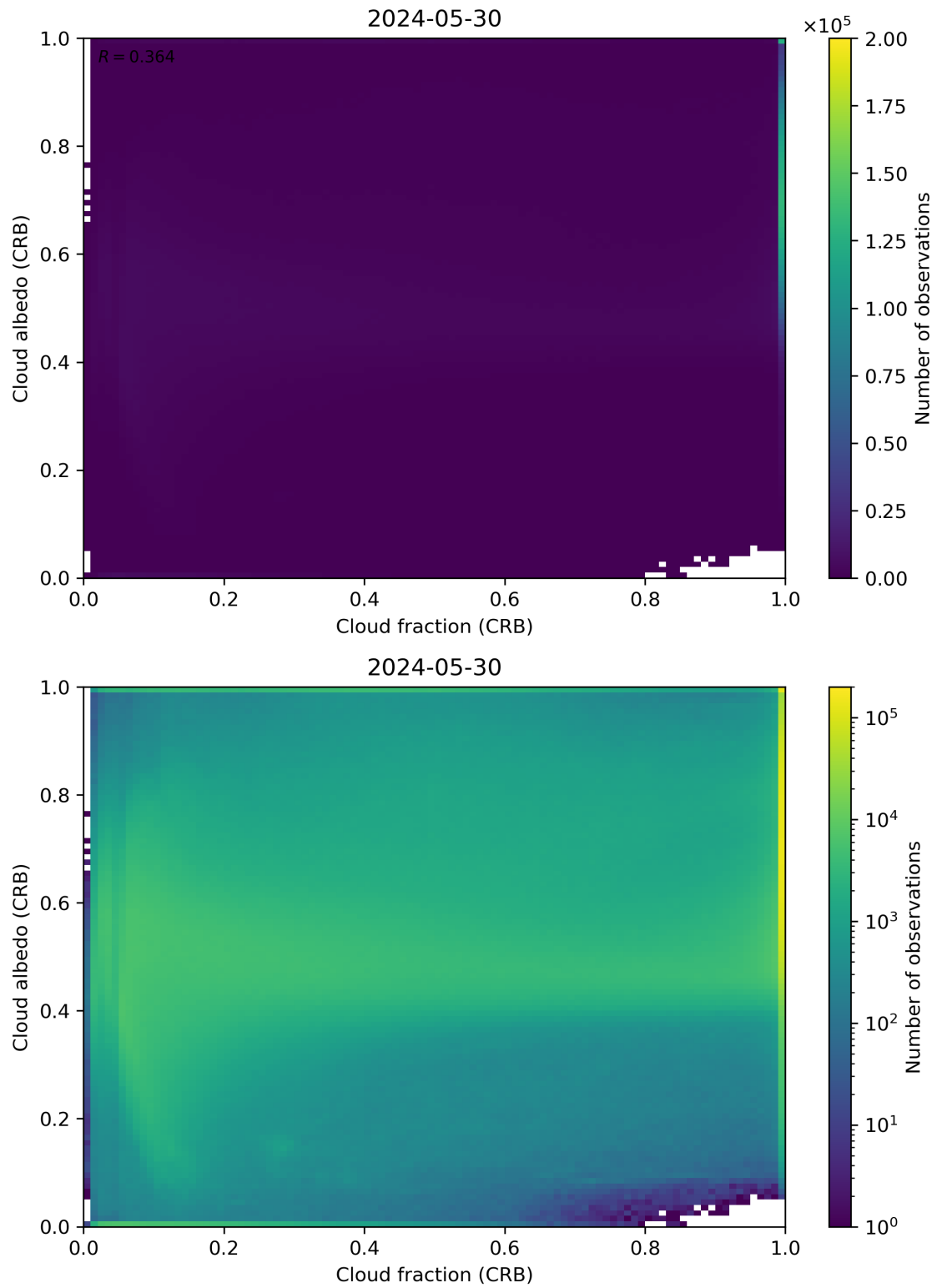
Figure 77: Scatter density plot of “Cloud fraction (CRB)” against “Cloud albedo (CRB)” for 2024-05-29 to 2024-05-31.
