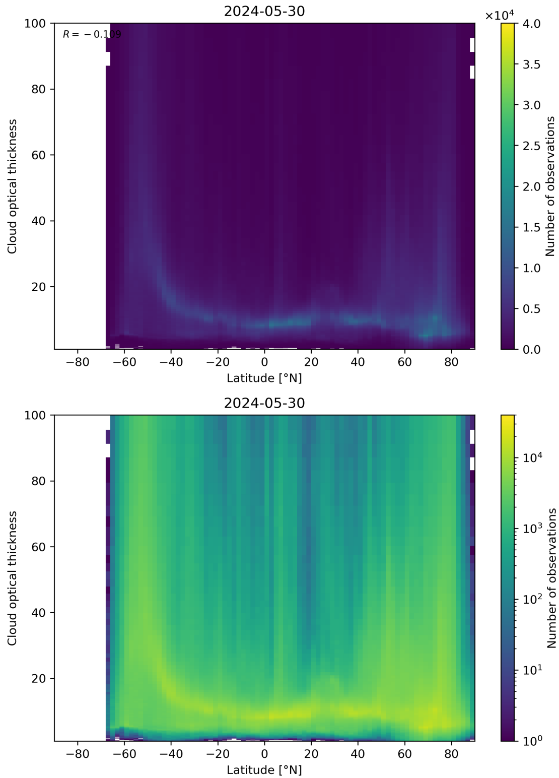
Figure 96: Scatter density plot of “Latitude” against “Cloud optical thickness” for 2024-05-29 to 2024-05-31.
