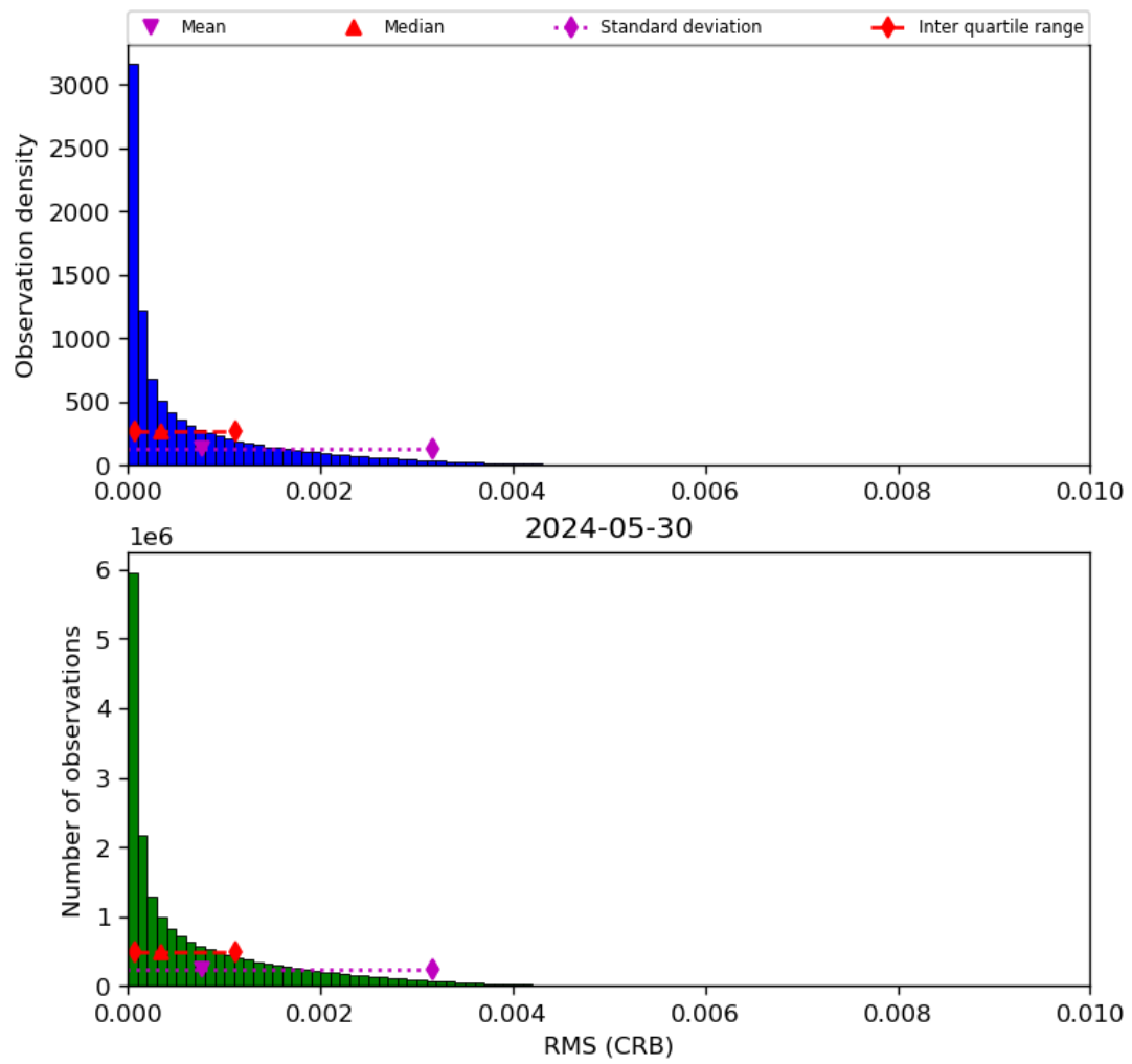
Figure 48: Histogram of “RMS (CRB)” for 2024-05-29 to 2024-05-31
