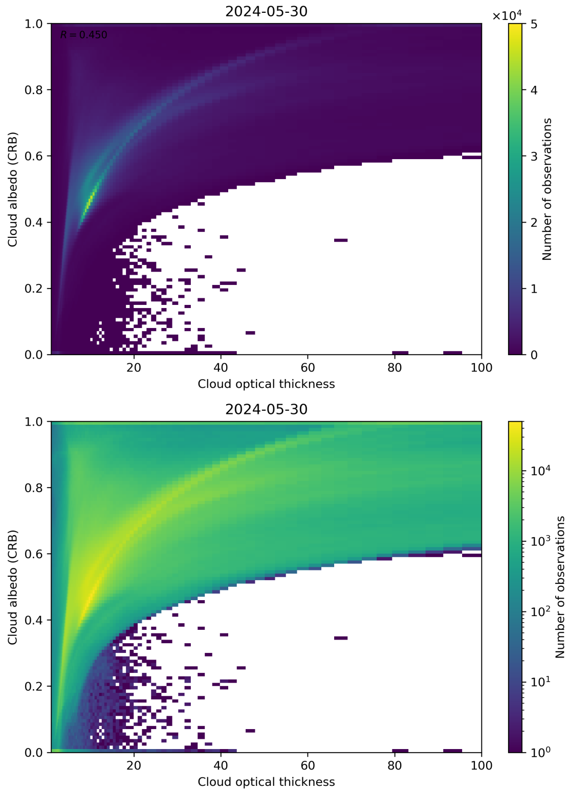
Figure 82: Scatter density plot of “Cloud optical thickness” against “Cloud albedo (CRB)” for 2024-05-29 to 2024-05-31.
