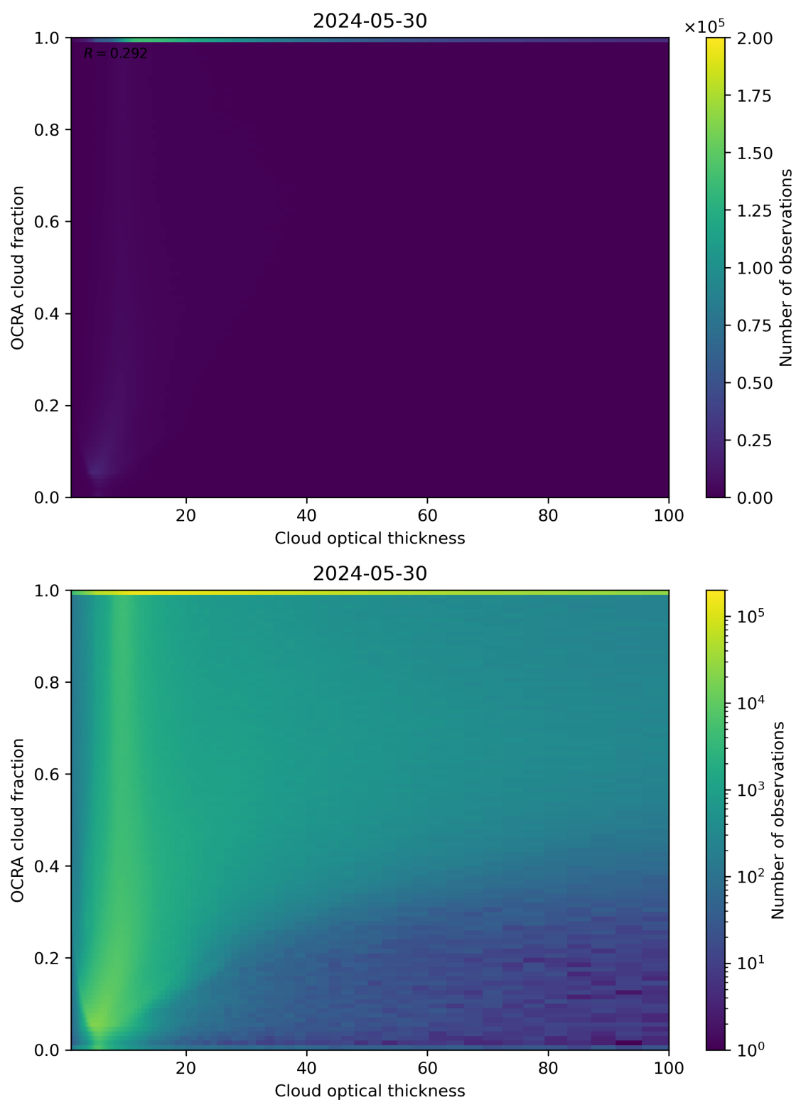
Figure 83: Scatter density plot of “Cloud optical thickness” against “OCRA cloud fraction” for 2024-05-29 to 2024-05-31.
