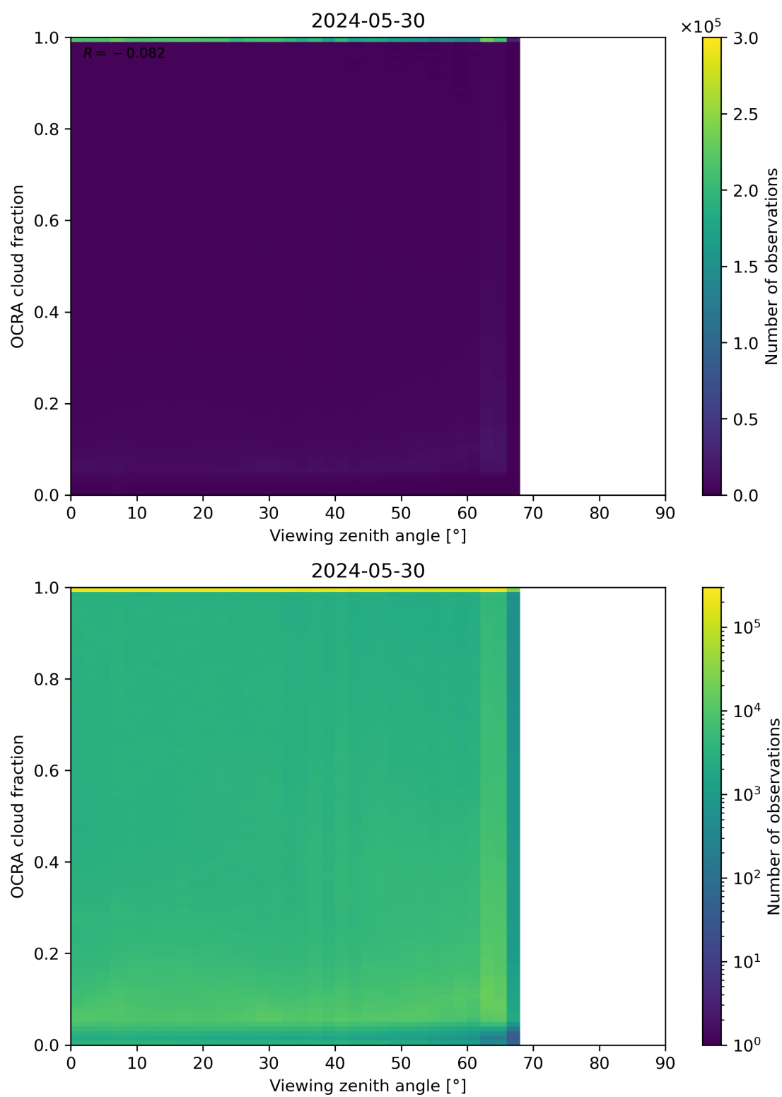
Figure 108: Scatter density plot of “Viewing zenith angle” against “OCRA cloud fraction” for 2024-05-29 to 2024-05-31.
