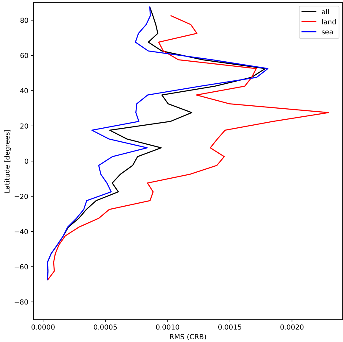
Figure 32: Zonal average of “RMS (CRB)” for 2024-05-29 to 2024-05-31.
