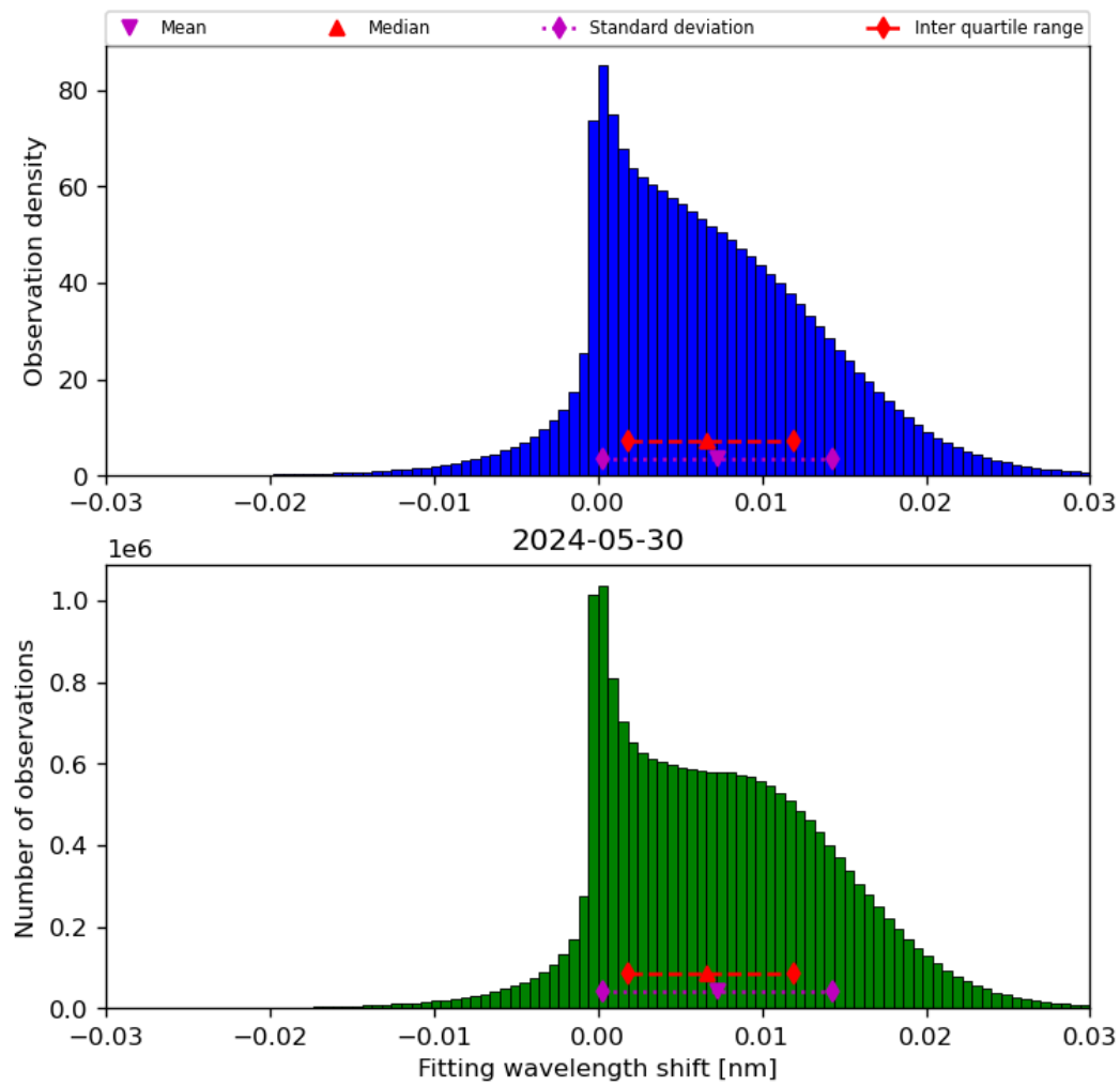
Figure 49: Histogram of “Fitting wavelength shift” for 2024-05-29 to 2024-05-31
