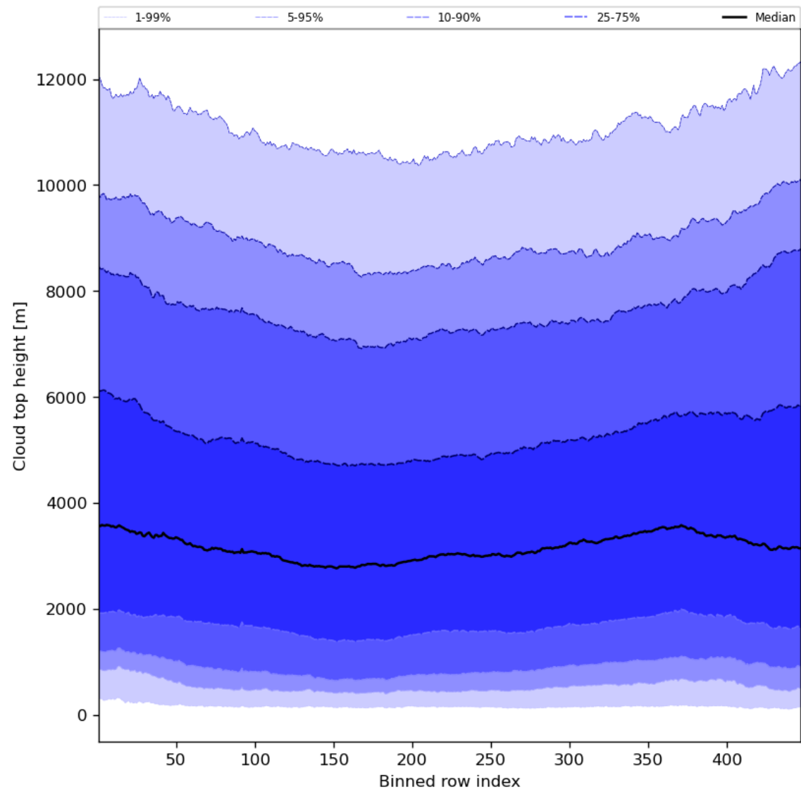
Figure 56: Along track statistics of “Cloud top height” for 2024-05-29 to 2024-05-31
