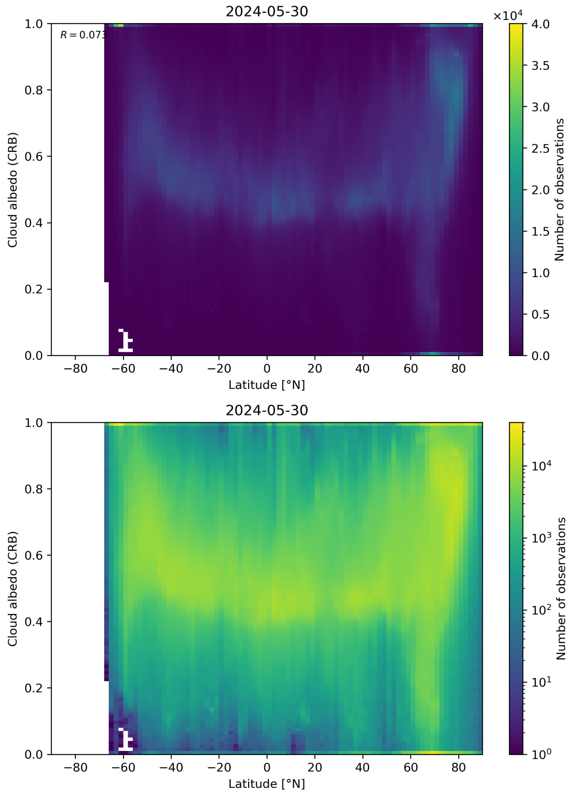
Figure 91: Scatter density plot of “Latitude” against “Cloud albedo (CRB)” for 2024-05-29 to 2024-05-31.
