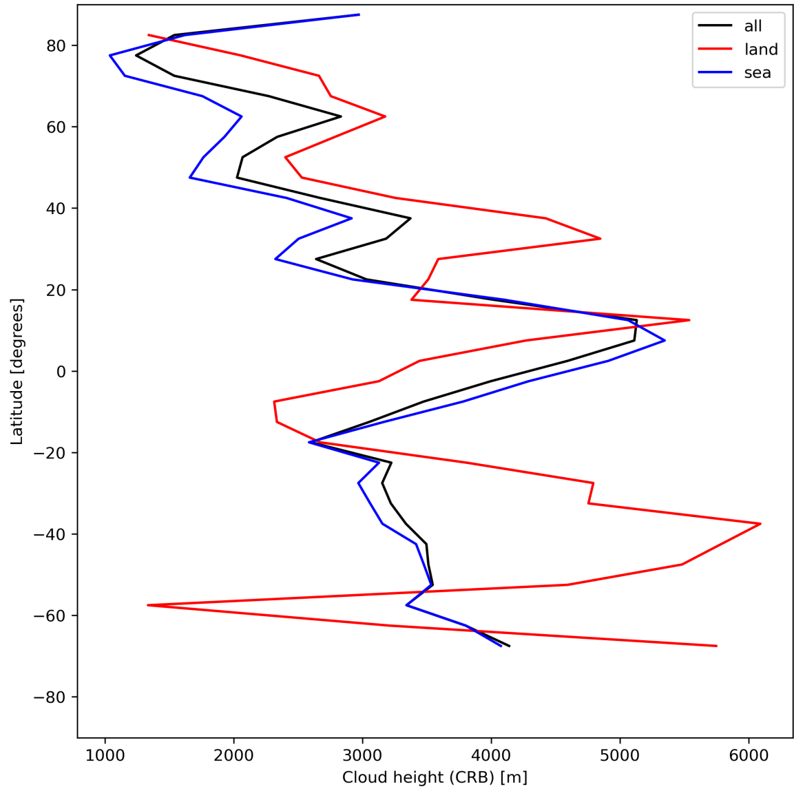
Figure 27: Zonal average of “Cloud height (CRB)” for 2024-05-29 to 2024-05-31.
