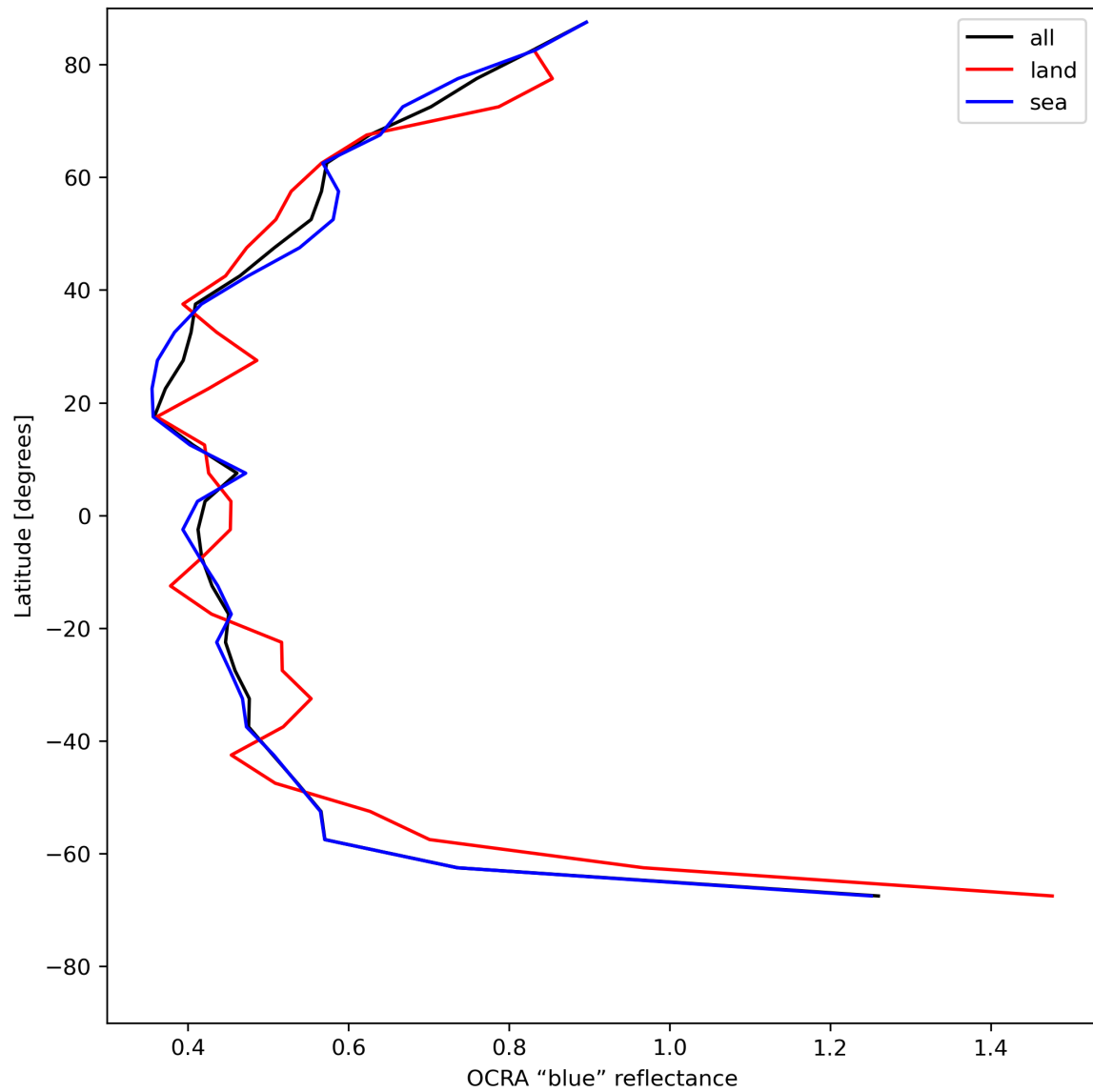
Figure 35: Zonal average of “OCRA “blue” reflectance” for 2024-05-29 to 2024-05-31.
