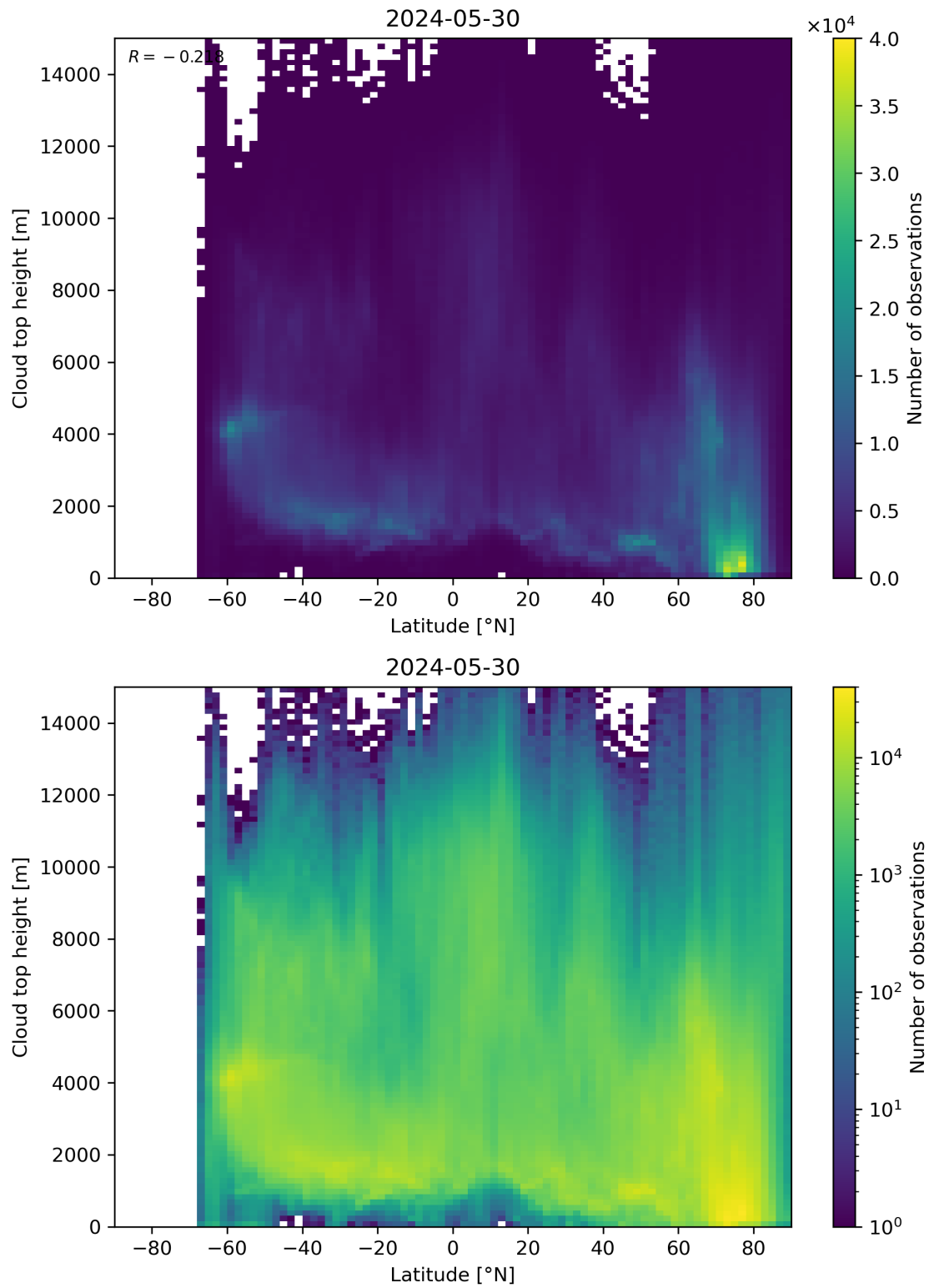
Figure 97: Scatter density plot of “Latitude” against “Cloud top height” for 2024-05-29 to 2024-05-31.
