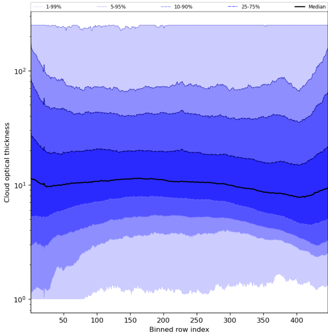
Figure 57: Along track statistics of “Cloud optical thickness” for 2024-05-29 to 2024-05-31
