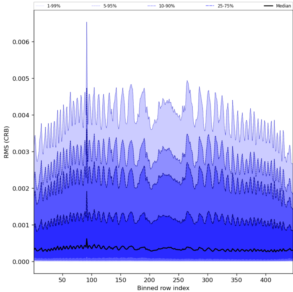
Figure 64: Along track statistics of “RMS (CRB)” for 2024-05-29 to 2024-05-31
