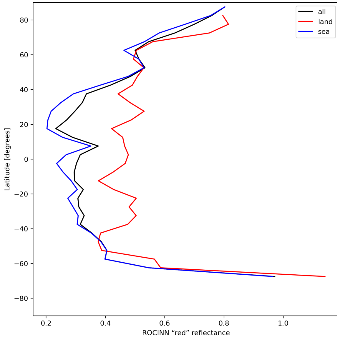
Figure 37: Zonal average of “ROCINN “red” reflectance” for 2024-05-29 to 2024-05-31.
