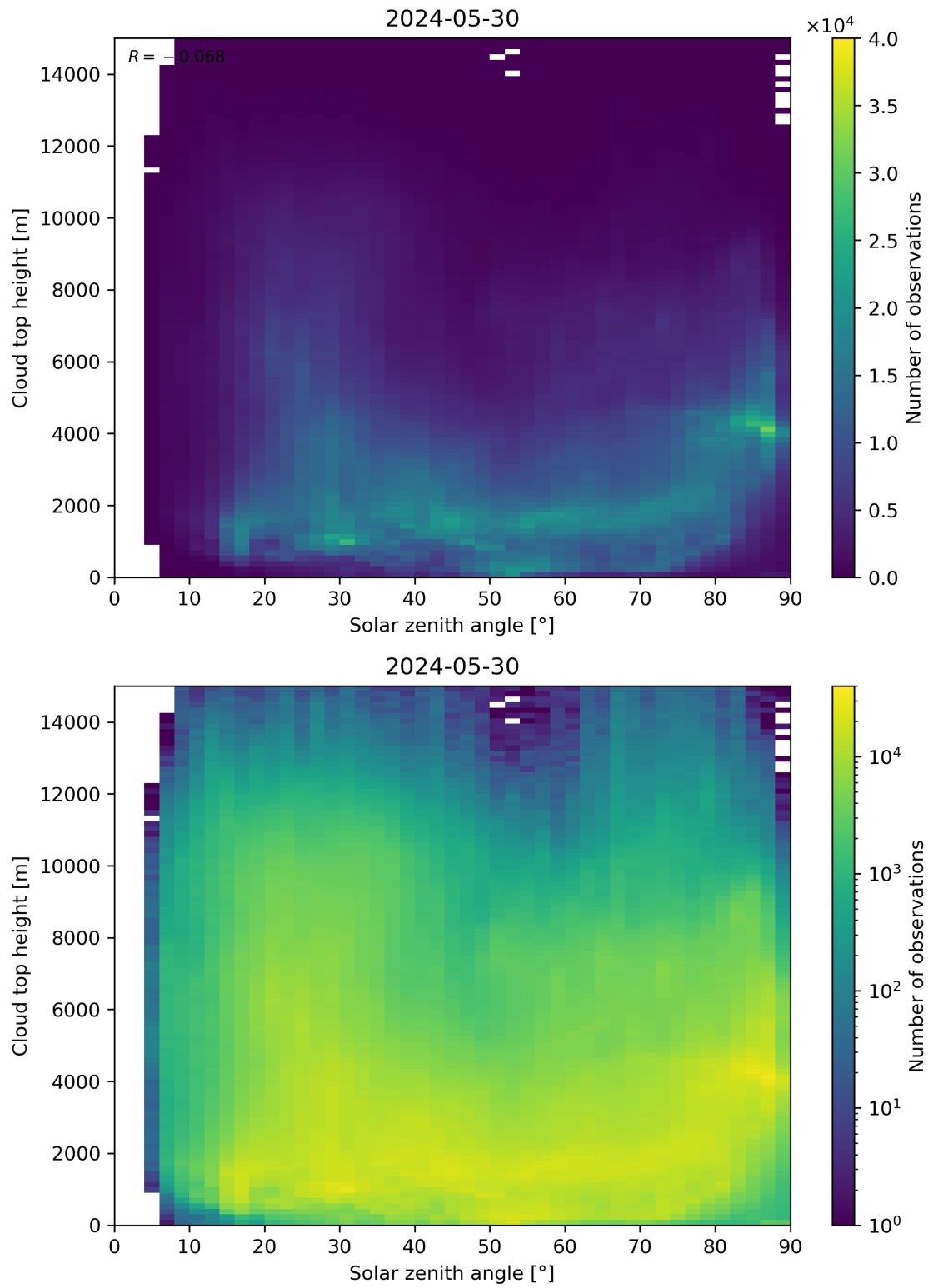
Figure 104: Scatter density plot of “Solar zenith angle” against “Cloud top height” for 2024-05-29 to 2024-05-31.
