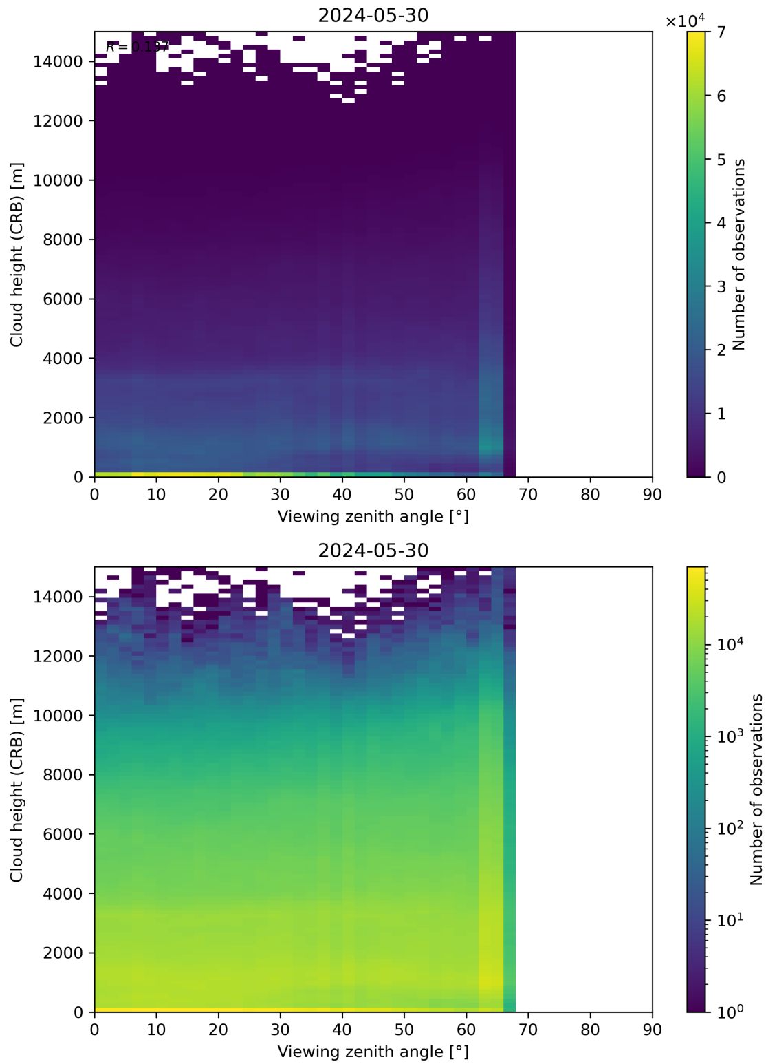
Figure 110: Scatter density plot of “Viewing zenith angle” against “Cloud height (CRB)” for 2024-05-29 to 2024-05-31.
