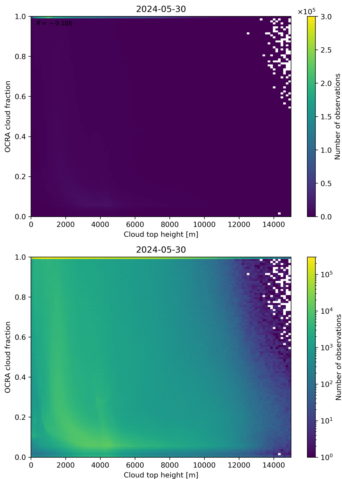
Figure 87: Scatter density plot of “Cloud top height” against “OCRA cloud fraction” for 2024-05-29 to 2024-05-31.
