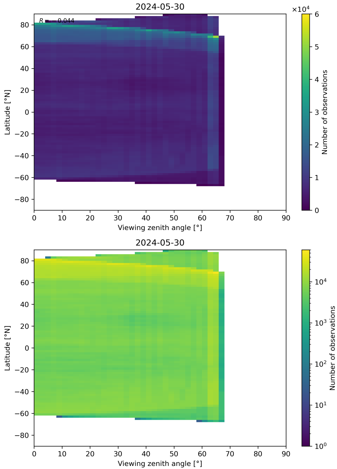
Figure 113: Scatter density plot of “Viewing zenith angle” against “Latitude” for 2024-05-29 to 2024-05-31.
