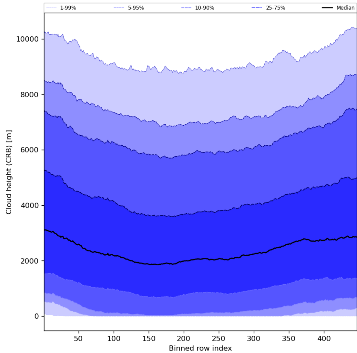
Figure 59: Along track statistics of “Cloud height (CRB)” for 2024-05-29 to 2024-05-31
