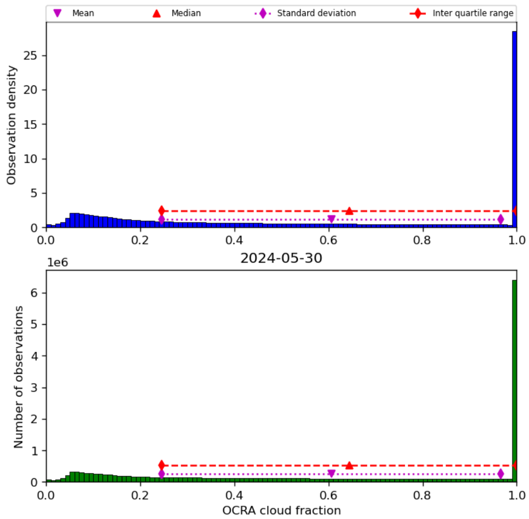
Figure 50: Histogram of “OCRA cloud fraction” for 2024-05-29 to 2024-05-31
