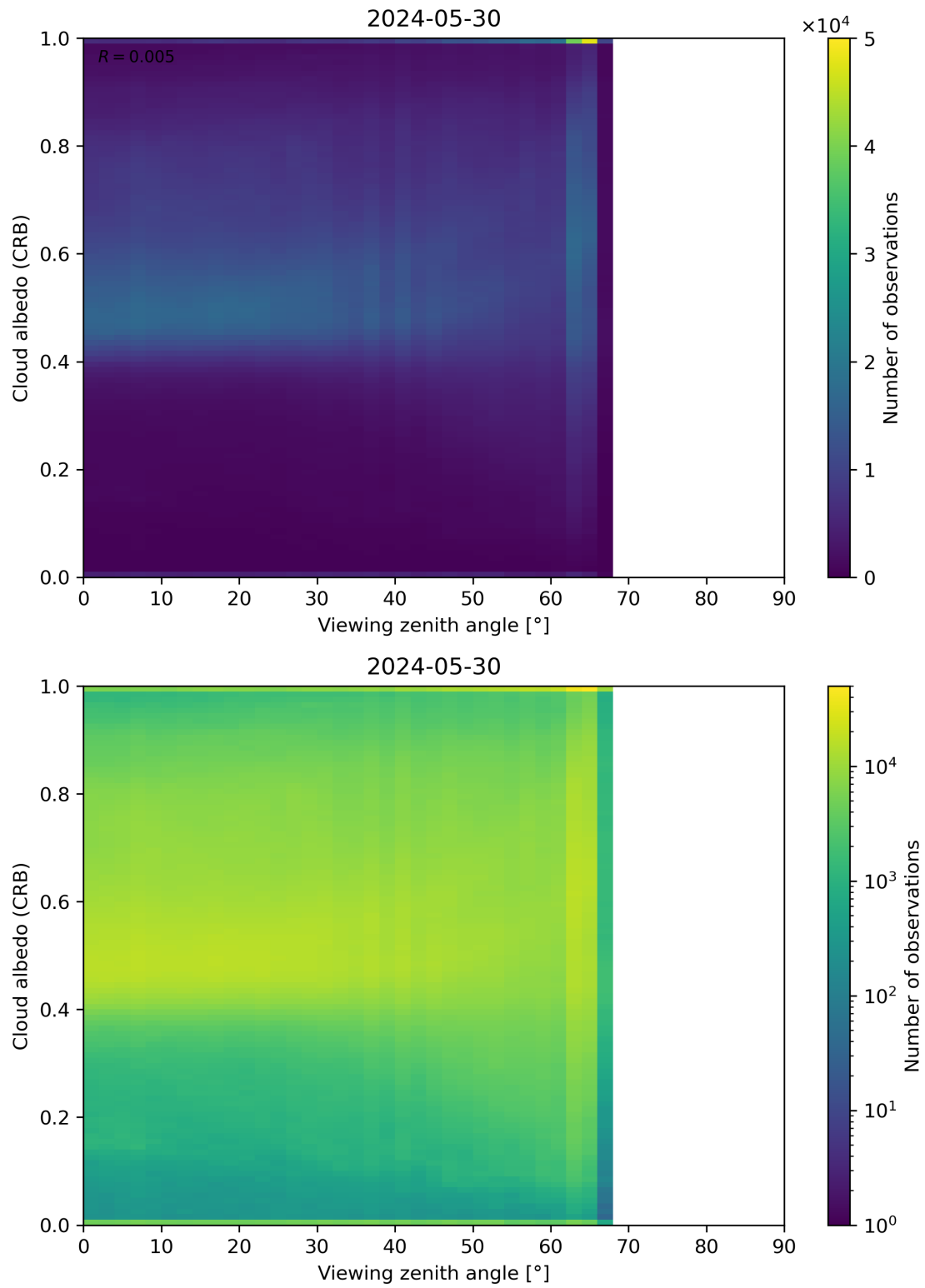
Figure 106: Scatter density plot of “Viewing zenith angle” against “Cloud albedo (CRB)” for 2024-05-29 to 2024-05-31.
