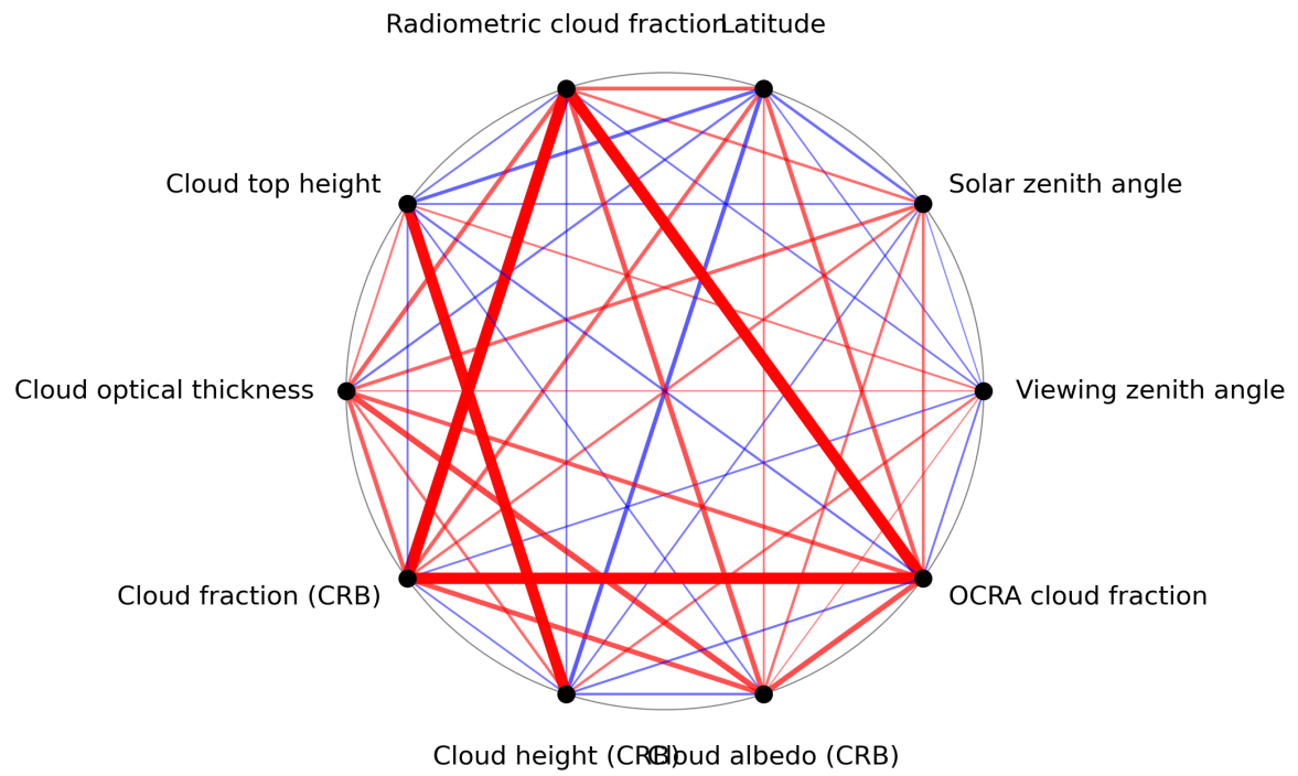
Figure 1: Map of correlation graph for 2024-05-29 to 2024-05-31.
