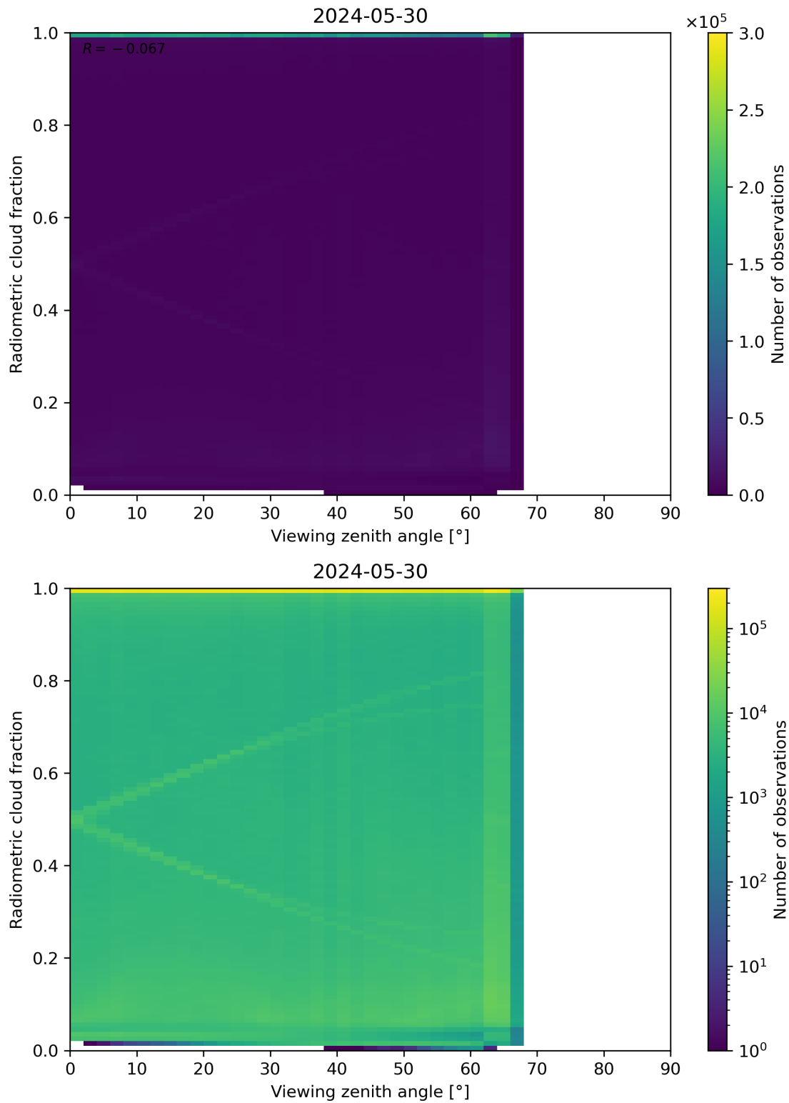
Figure 107: Scatter density plot of “Viewing zenith angle” against “Radiometric cloud fraction” for 2024-05-29 to 2024-05-31.
