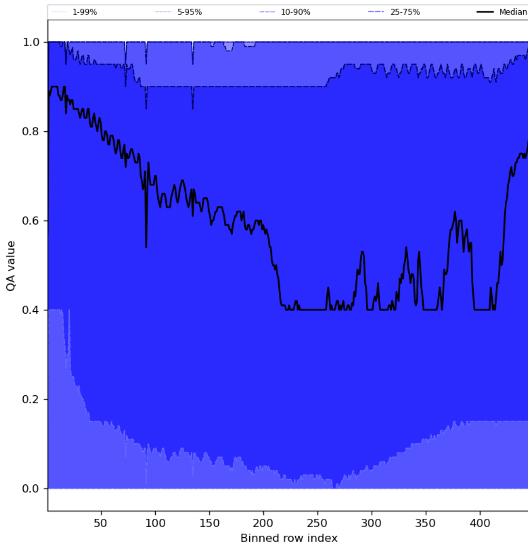
Figure 54: Along track statistics of “QA value” for 2024-05-29 to 2024-05-31
