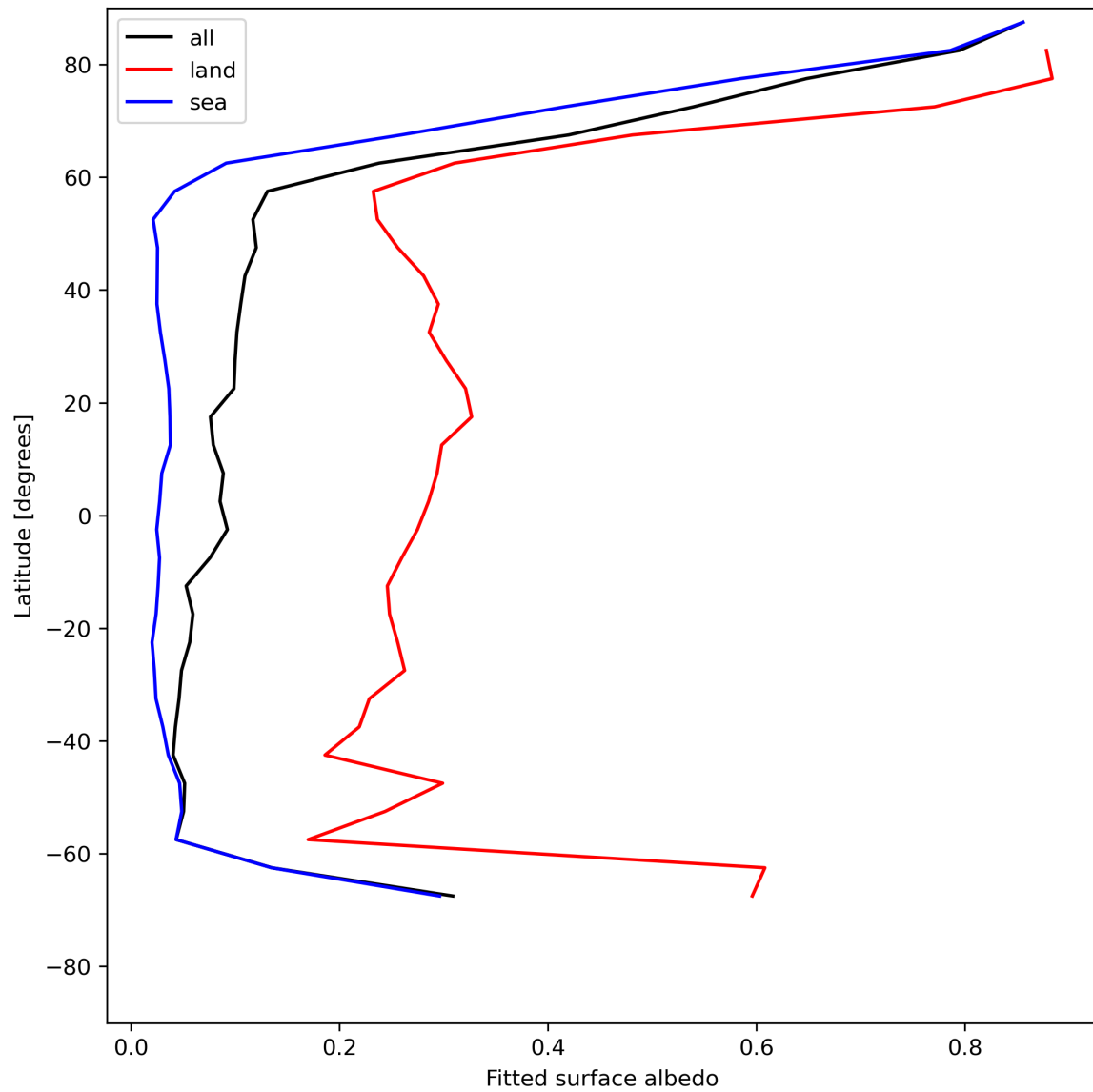
Figure 29: Zonal average of “Fitted surface albedo” for 2024-05-29 to 2024-05-31.
