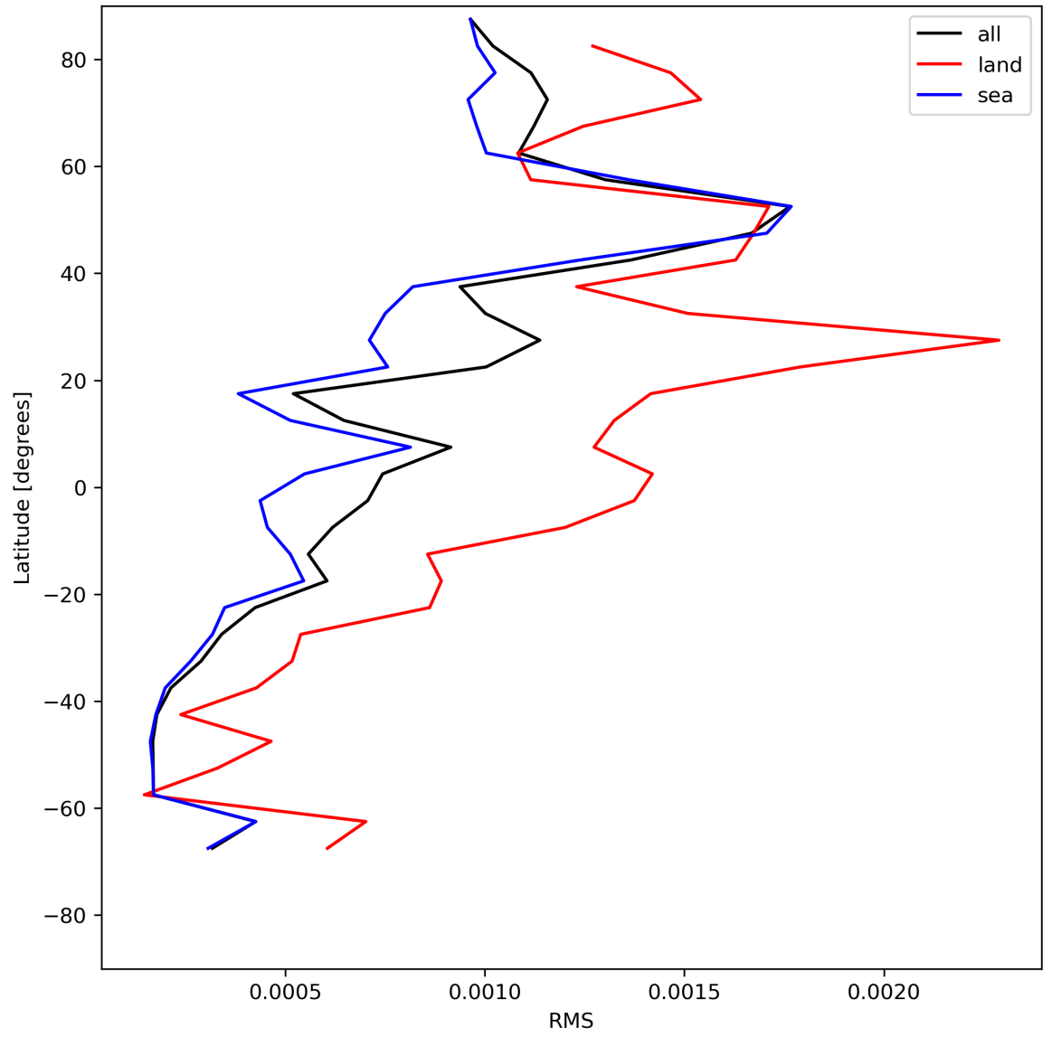
Figure 31: Zonal average of “RMS” for 2024-05-29 to 2024-05-31.
