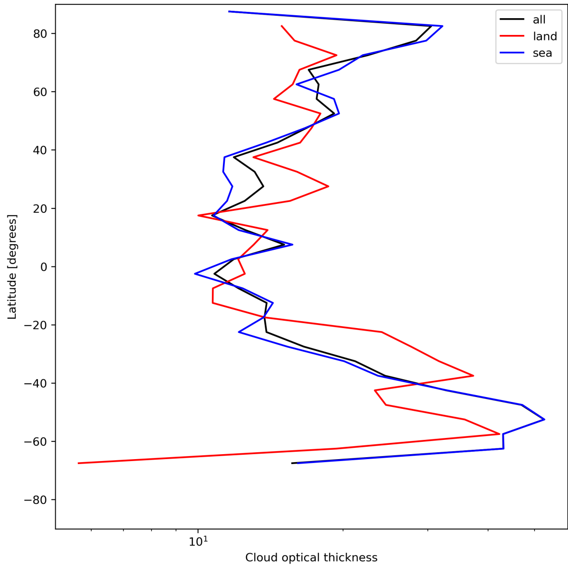
Figure 25: Zonal average of “Cloud optical thickness” for 2024-05-29 to 2024-05-31.
