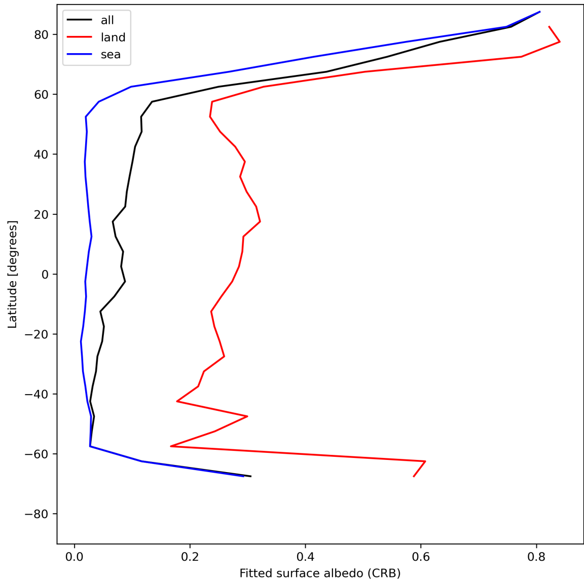
Figure 30: Zonal average of “Fitted surface albedo (CRB)” for 2024-05-29 to 2024-05-31.
