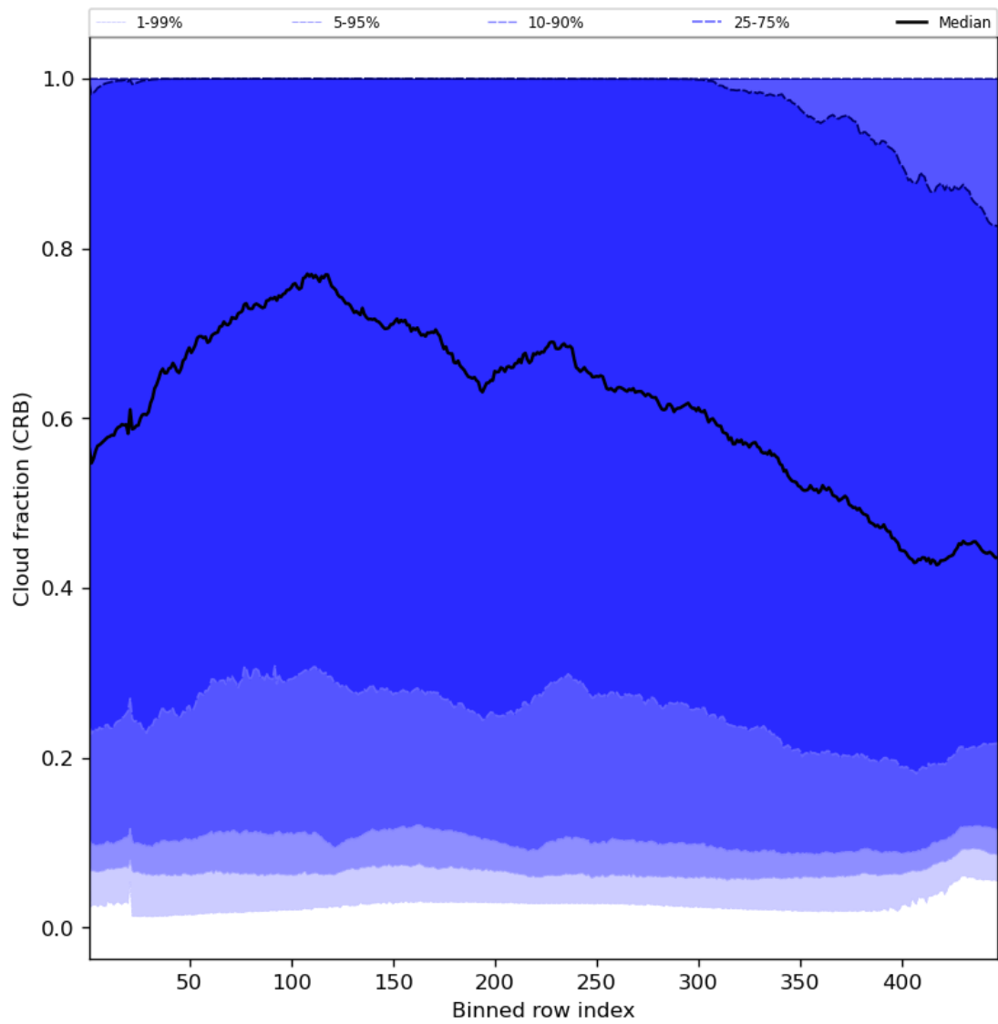
Figure 58: Along track statistics of “Cloud fraction (CRB)” for 2024-05-29 to 2024-05-31
