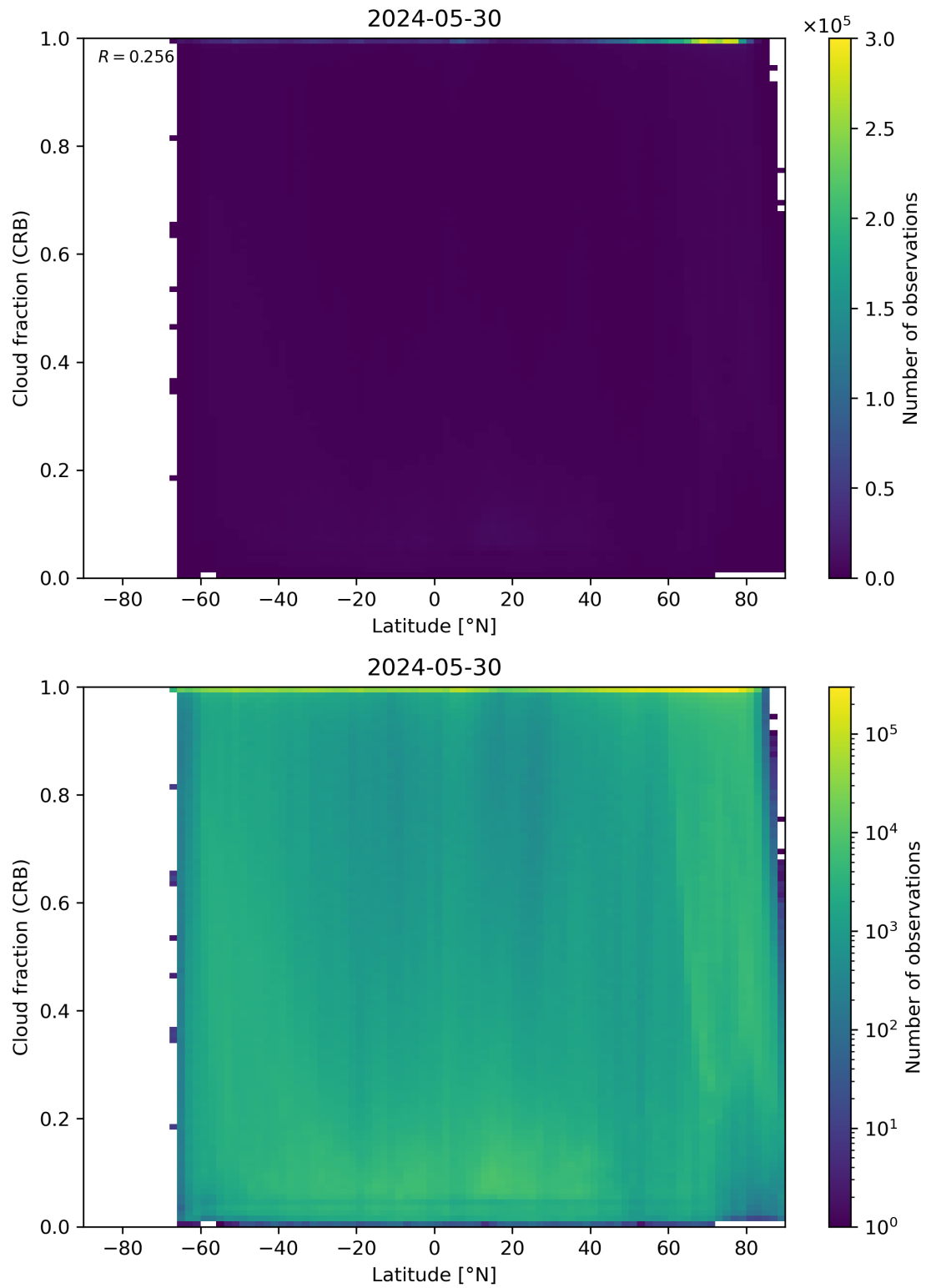
Figure 94: Scatter density plot of “Latitude” against “Cloud fraction (CRB)” for 2024-05-29 to 2024-05-31.
