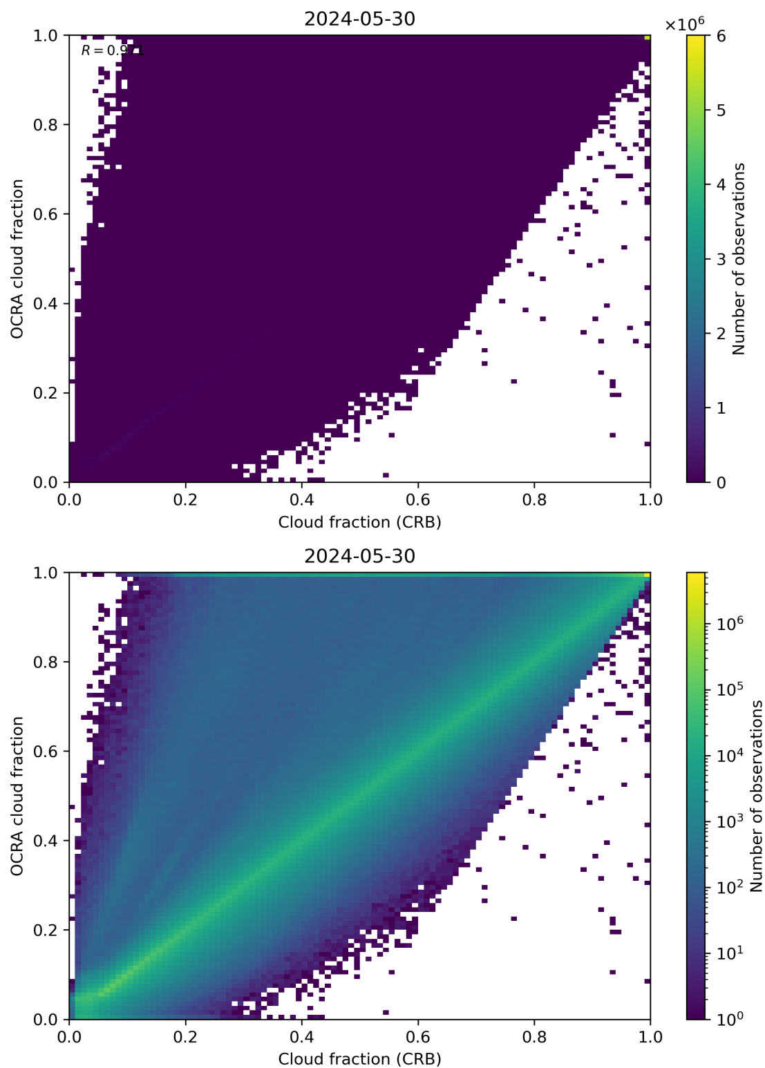
Figure 78: Scatter density plot of “Cloud fraction (CRB)” against “OCRA cloud fraction” for 2024-05-29 to 2024-05-31.
