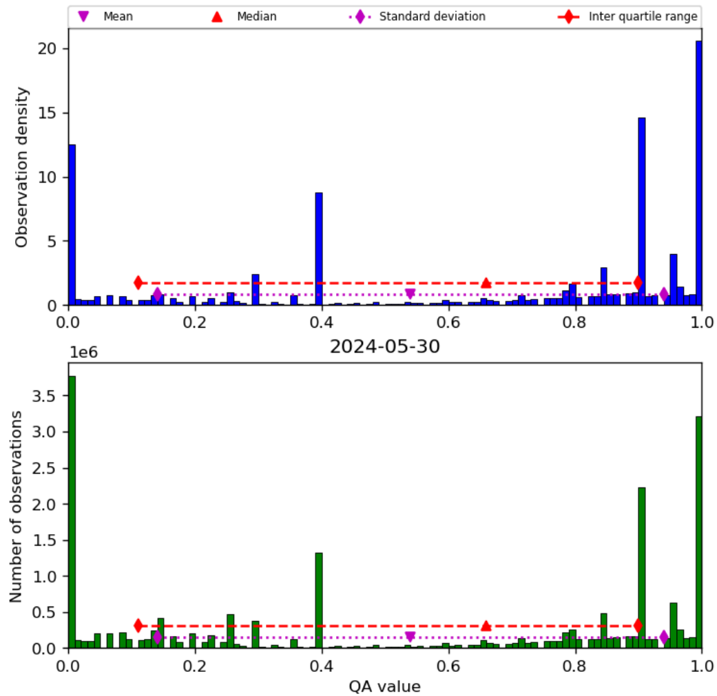
Figure 38: Histogram of “QA value” for 2024-05-29 to 2024-05-31
