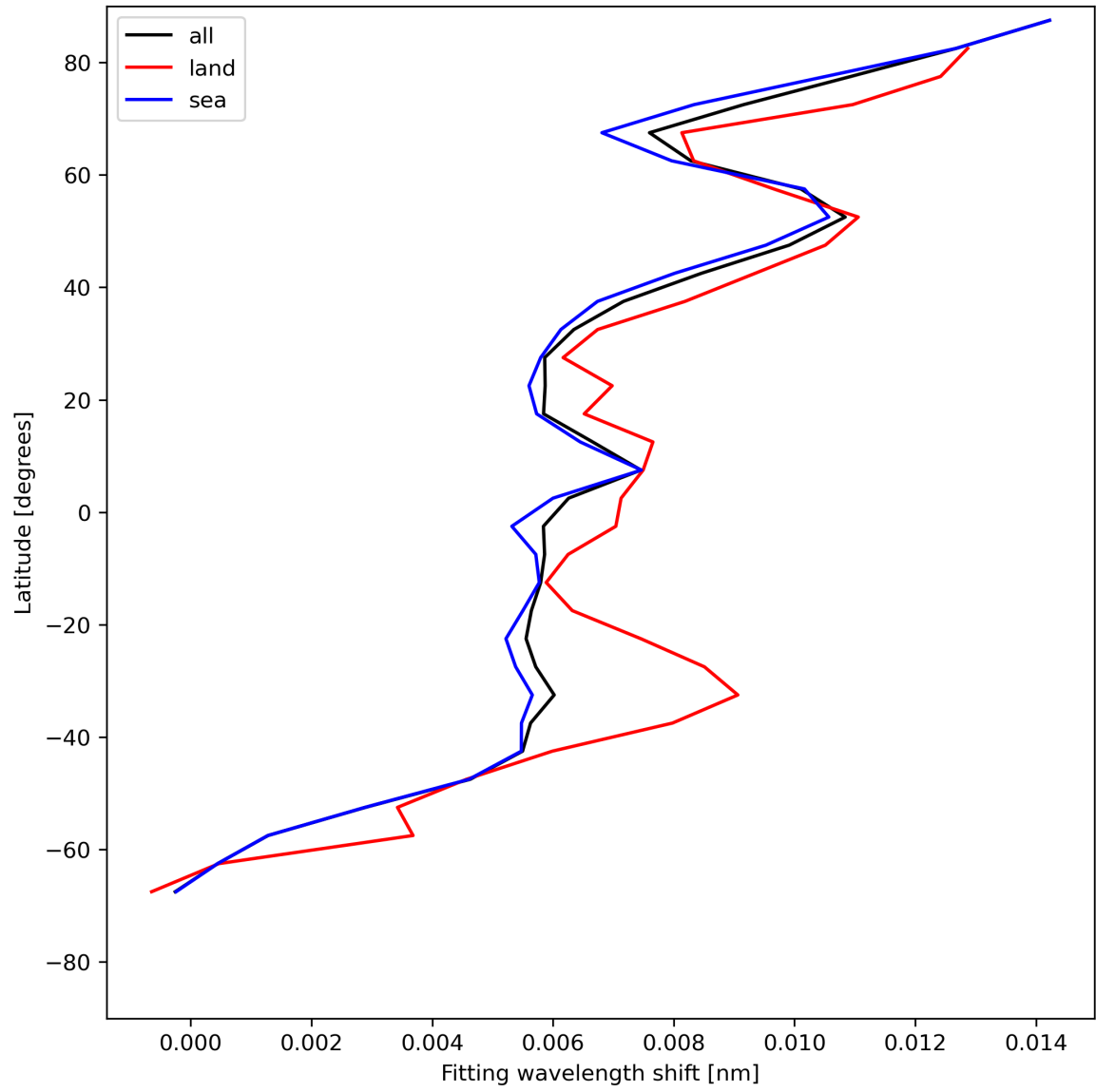
Figure 33: Zonal average of “Fitting wavelength shift” for 2024-05-29 to 2024-05-31.
