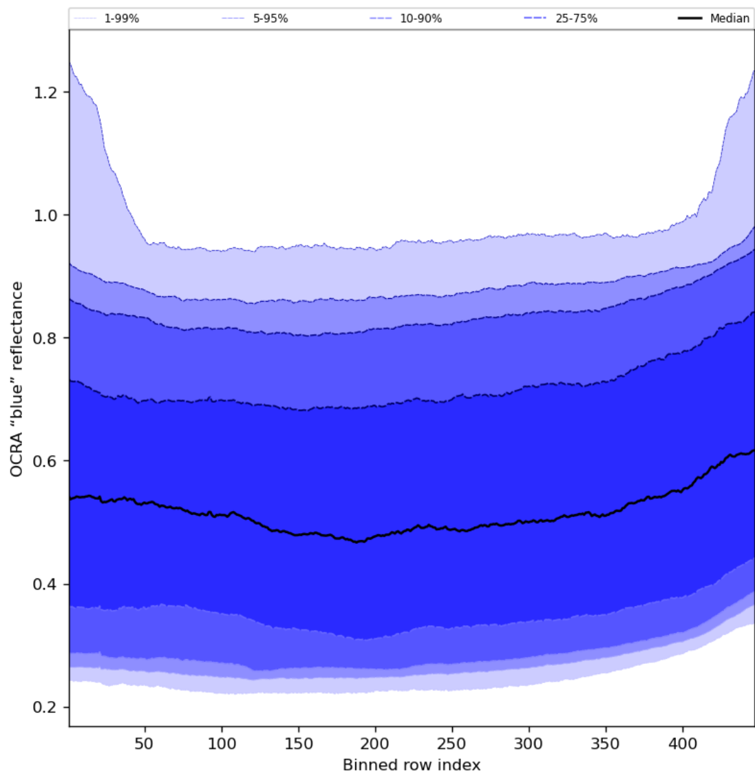
Figure 67: Along track statistics of "OCRA "blue" reflectance" for 2024-05-29 to 2024-05-31
