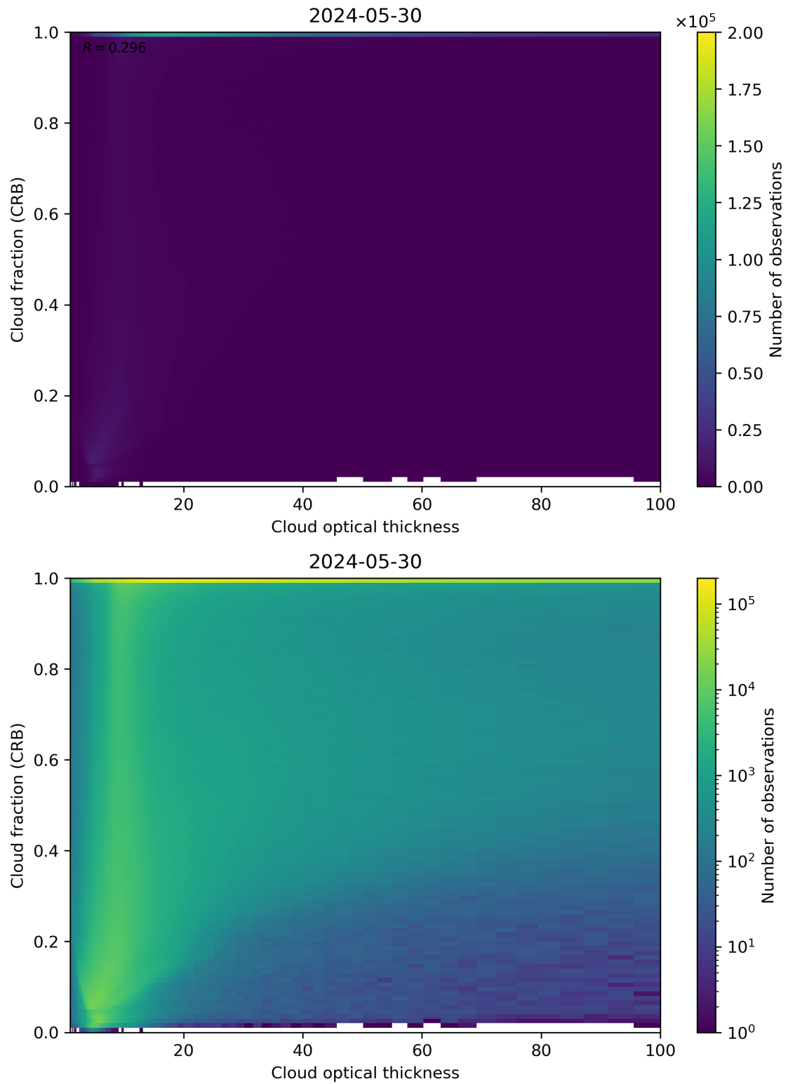
Figure 84: Scatter density plot of “Cloud optical thickness” against “Cloud fraction (CRB)” for 2024-05-29 to 2024-05-31.
