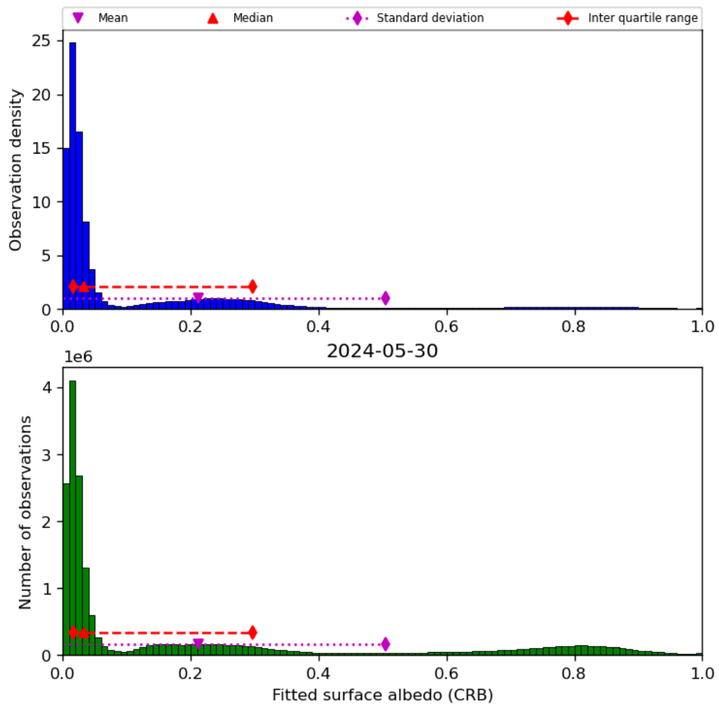
Figure 46: Histogram of “Fitted surface albedo (CRB)” for 2024-05-29 to 2024-05-31
