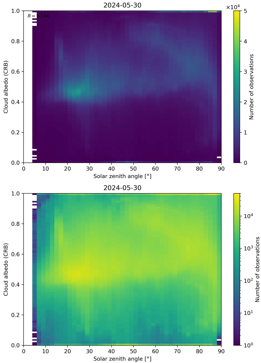
Figure 98: Scatter density plot of “Solar zenith angle” against “Cloud albedo (CRB)” for 2024-05-29 to 2024-05-31.
