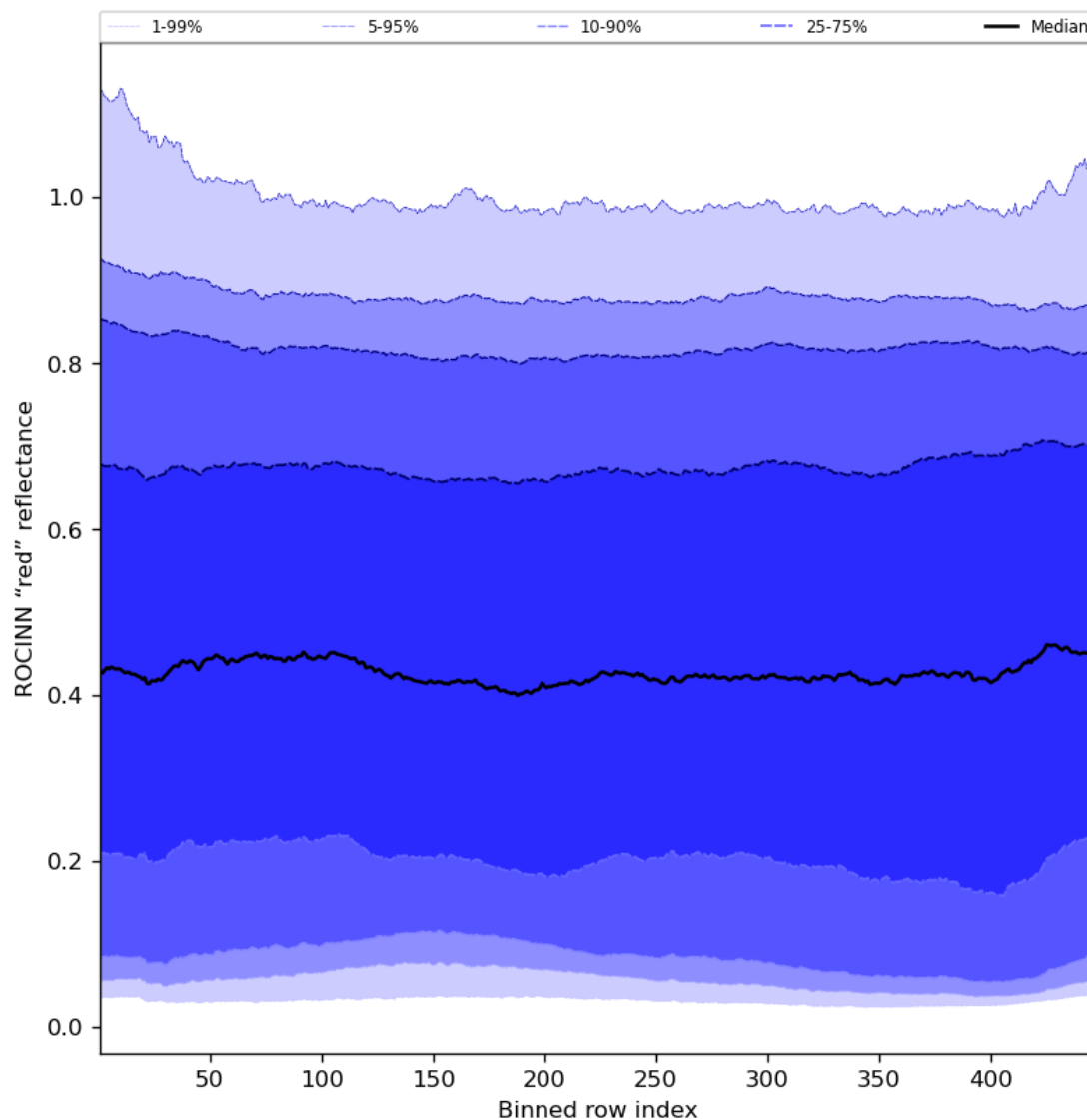
Figure 69: Along track statistics of “ROCINN “red” reflectance” for 2024-05-29 to 2024-05-31
