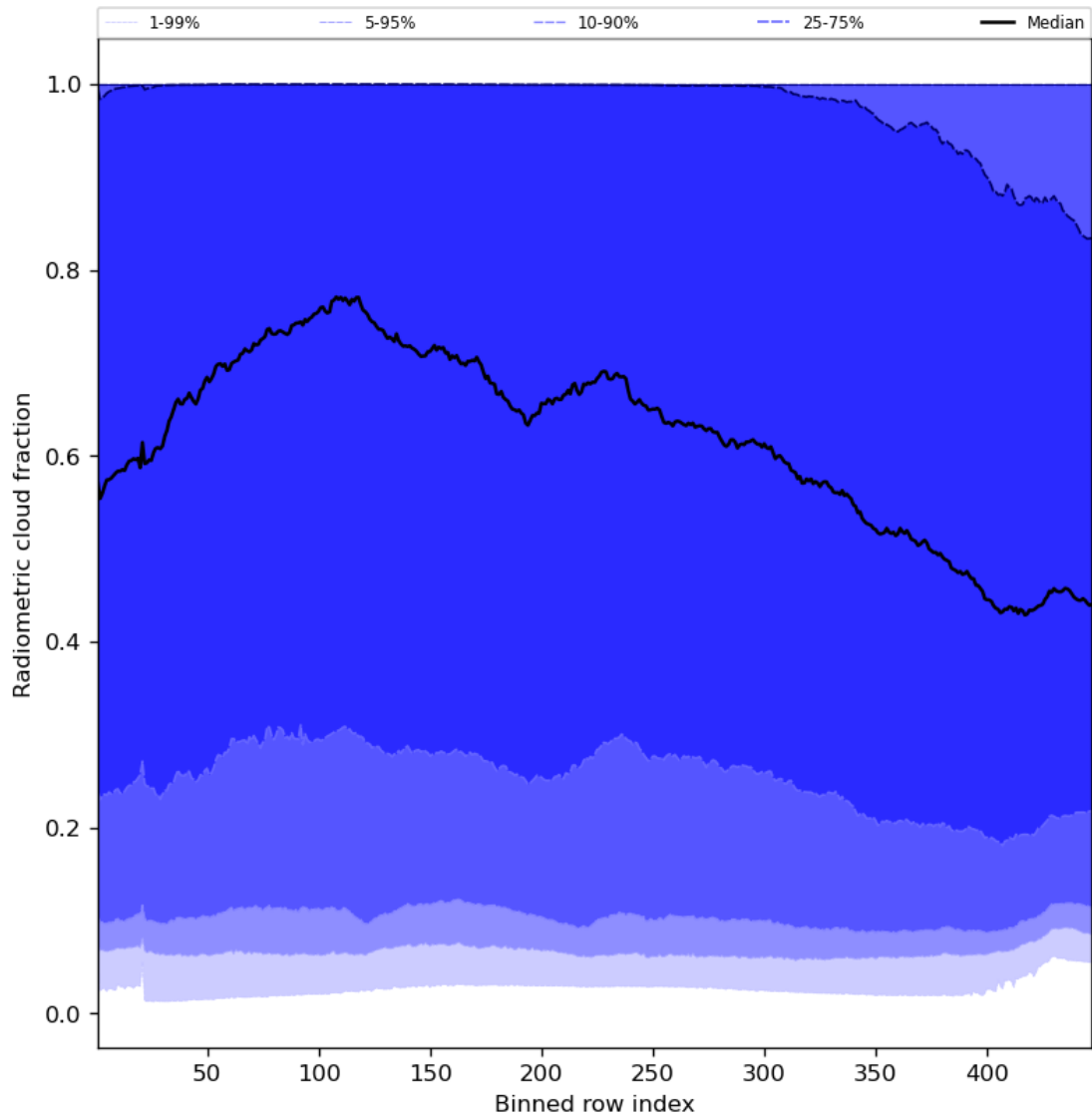
Figure 55: Along track statistics of “Radiometric cloud fraction” for 2024-05-29 to 2024-05-31
