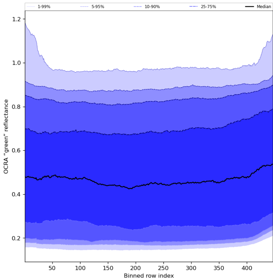
Figure 68: Along track statistics of “OCRA “green” reflectance” for 2024-05-29 to 2024-05-31
