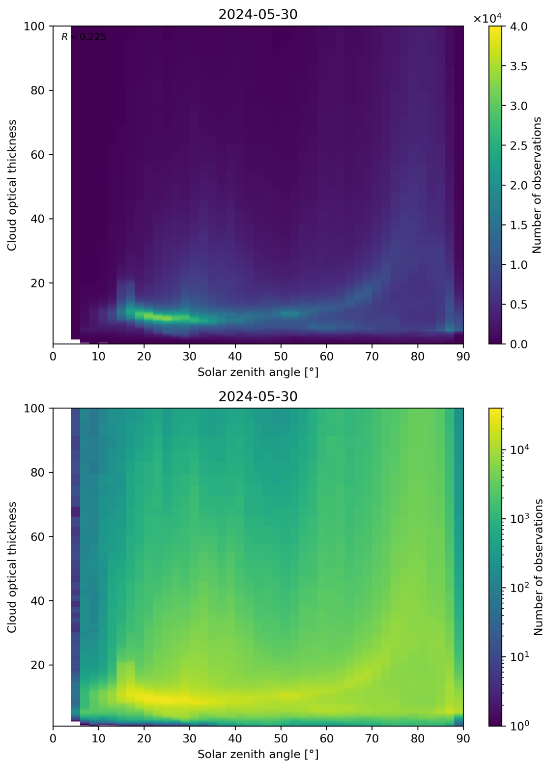
Figure 103: Scatter density plot of “Solar zenith angle” against “Cloud optical thickness” for 2024-05-29 to 2024-05-31.
