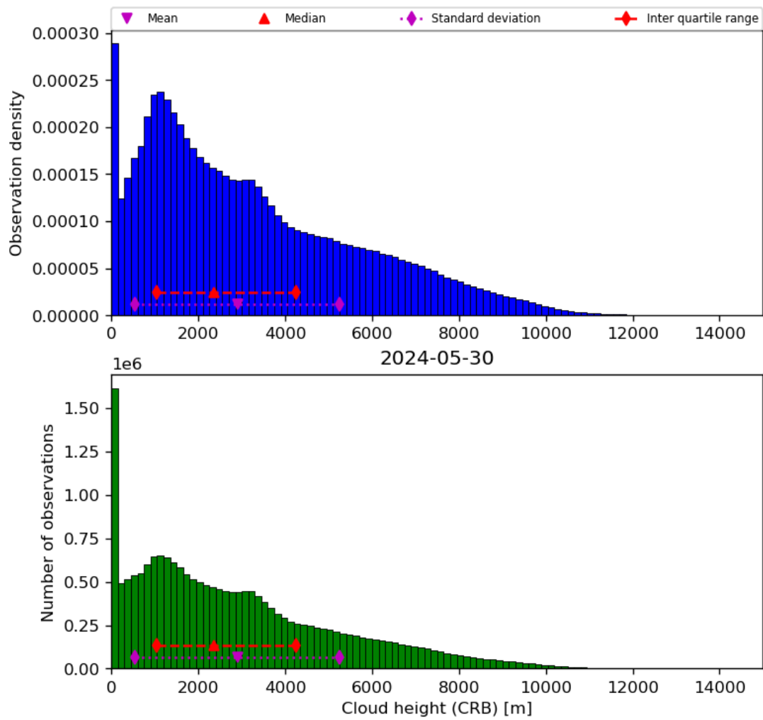
Figure 43: Histogram of “Cloud height (CRB)” for 2024-05-29 to 2024-05-31
