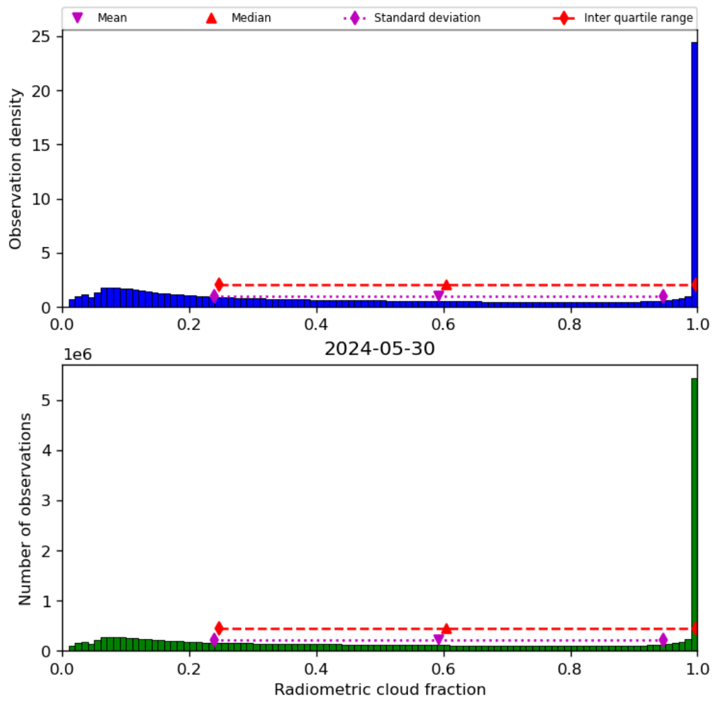
Figure 39: Histogram of “Radiometric cloud fraction” for 2024-05-29 to 2024-05-31
