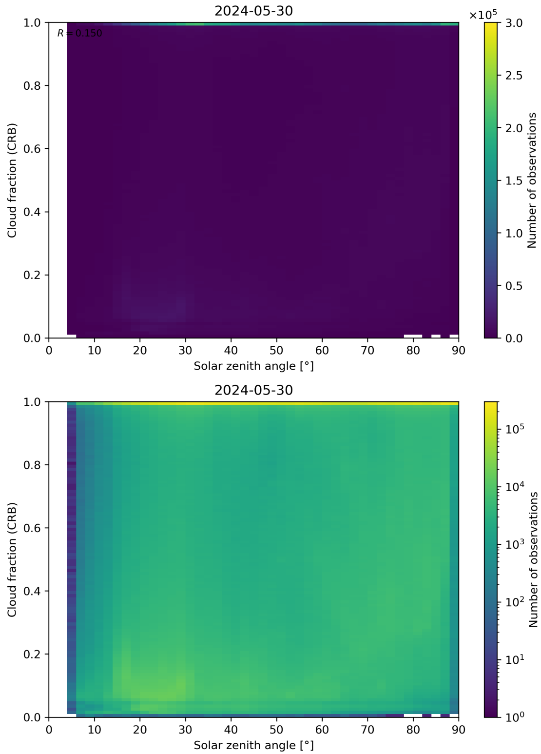
Figure 101: Scatter density plot of “Solar zenith angle” against “Cloud fraction (CRB)” for 2024-05-29 to 2024-05-31.
