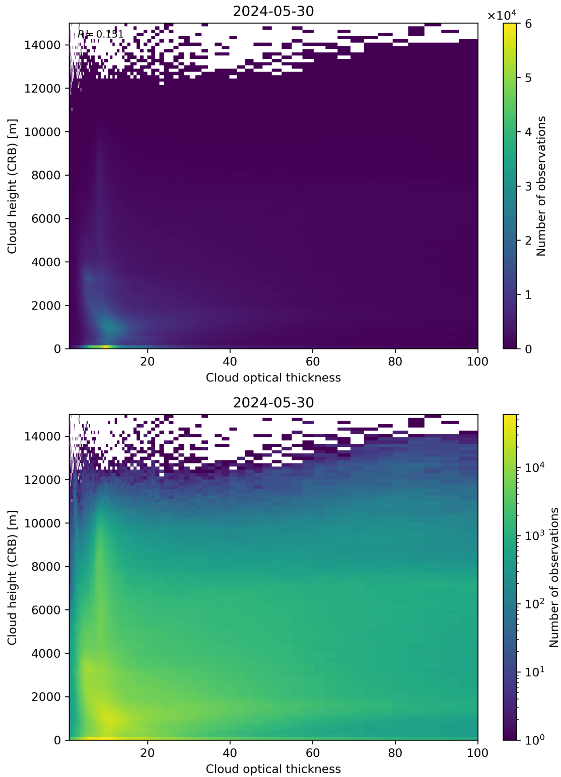
Figure 85: Scatter density plot of “Cloud optical thickness” against “Cloud height (CRB)” for 2024-05-29 to 2024-05-31.
