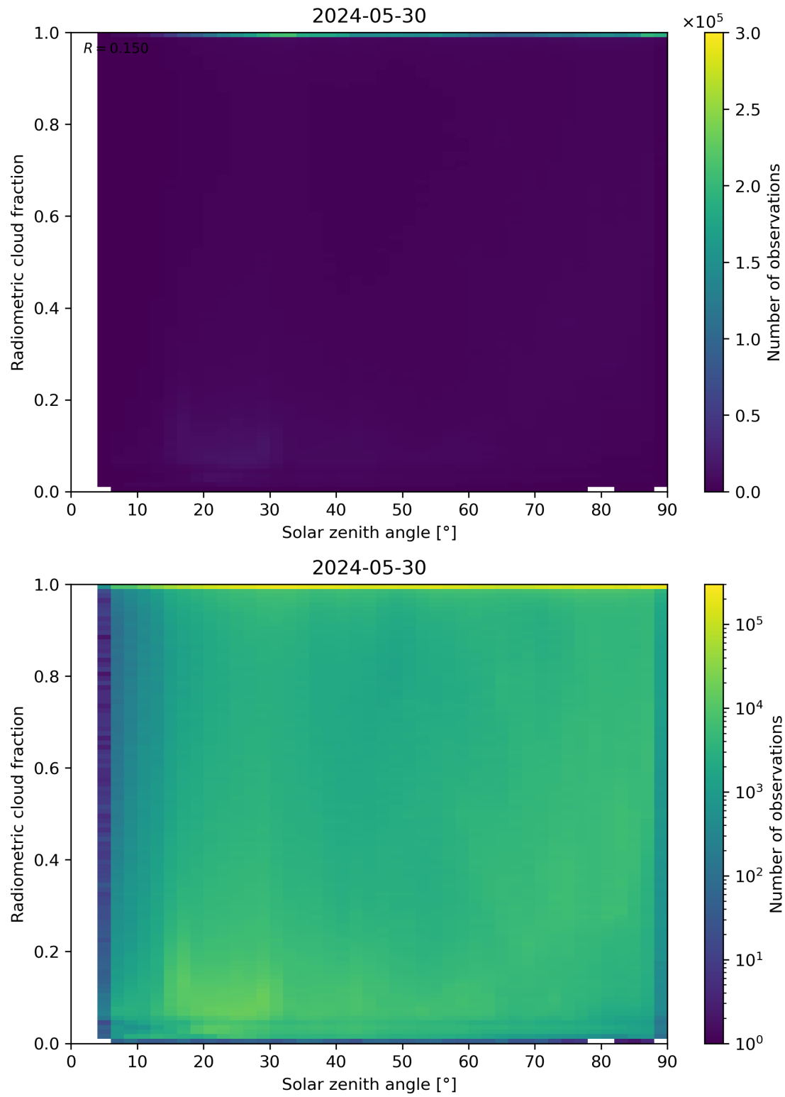
Figure 99: Scatter density plot of “Solar zenith angle” against “Radiometric cloud fraction” for 2024-05-29 to 2024-05-31.
