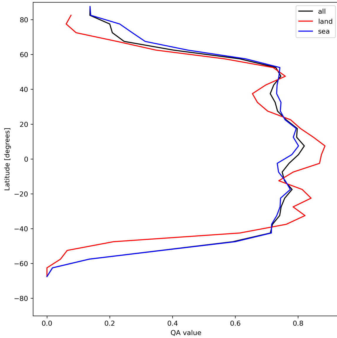
Figure 22: Zonal average of “QA value” for 2024-05-29 to 2024-05-31.
