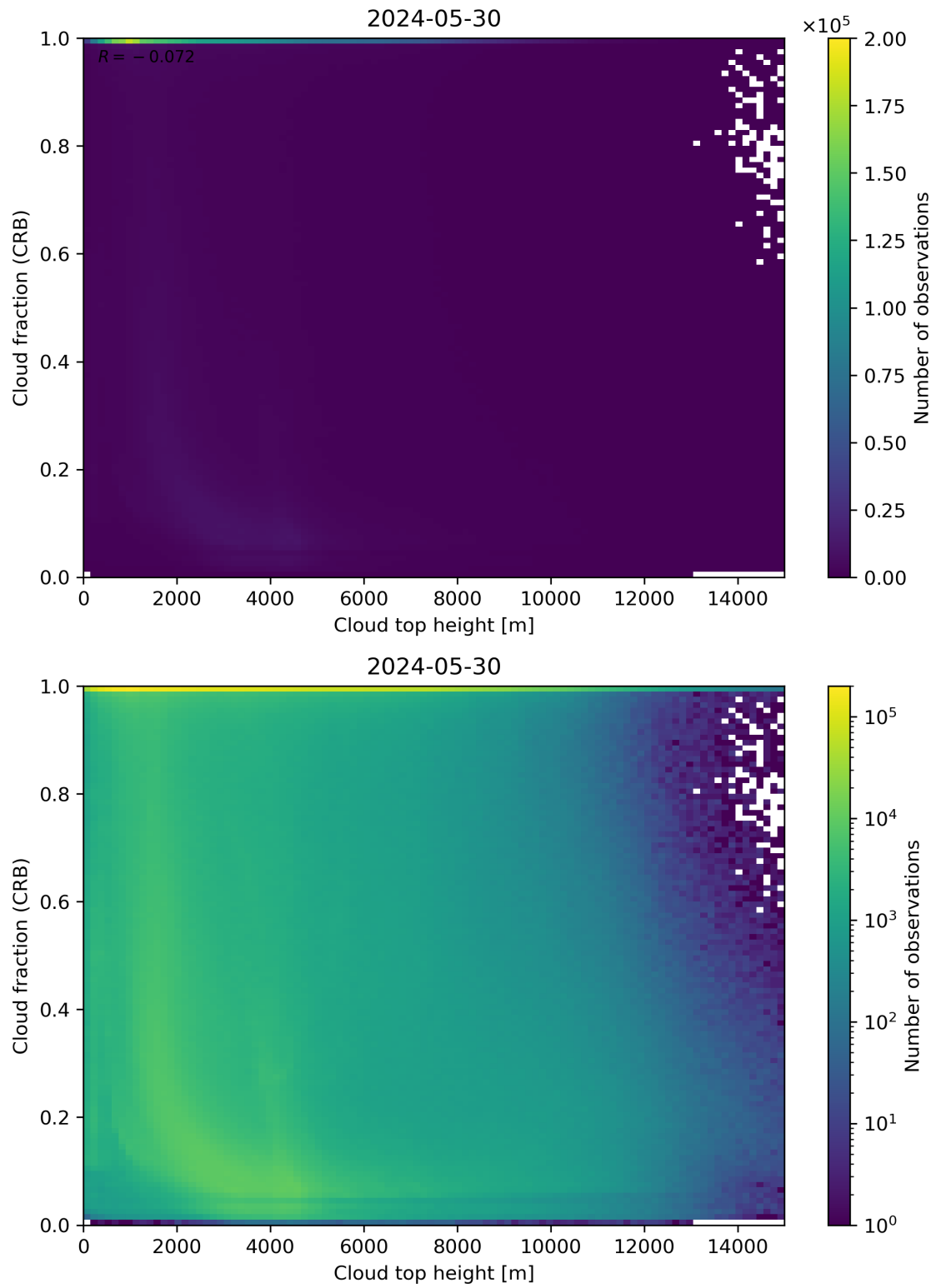
Figure 88: Scatter density plot of “Cloud top height” against “Cloud fraction (CRB)” for 2024-05-29 to 2024-05-31.
