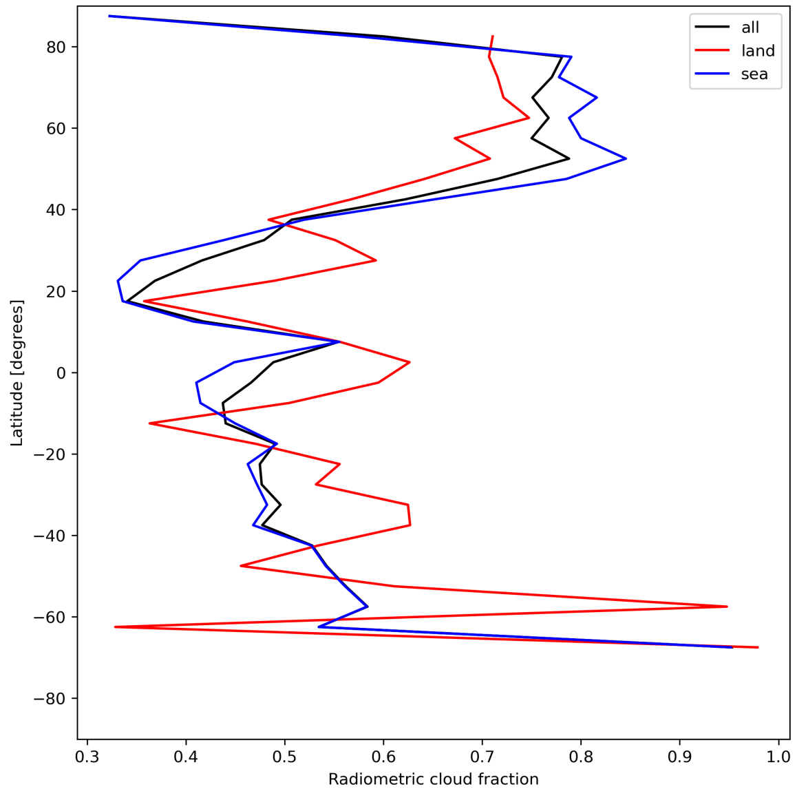
Figure 23: Zonal average of “Radiometric cloud fraction” for 2024-05-29 to 2024-05-31.
