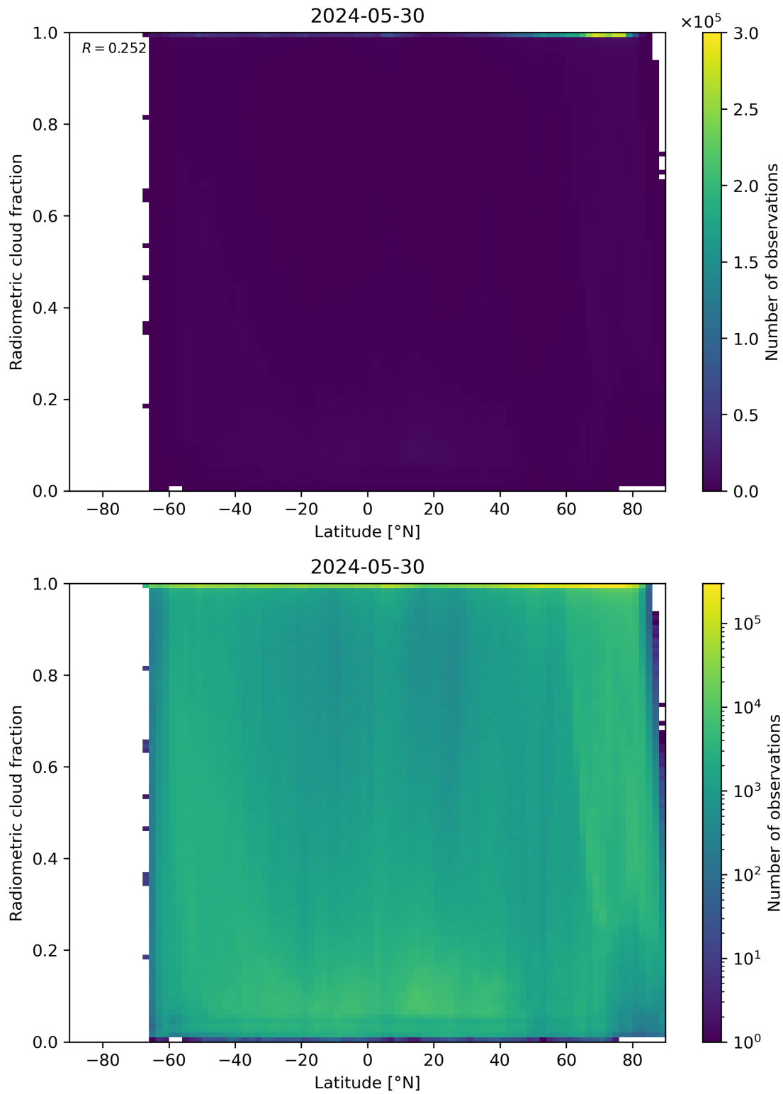
Figure 92: Scatter density plot of “Latitude” against “Radiometric cloud fraction” for 2024-05-29 to 2024-05-31.
