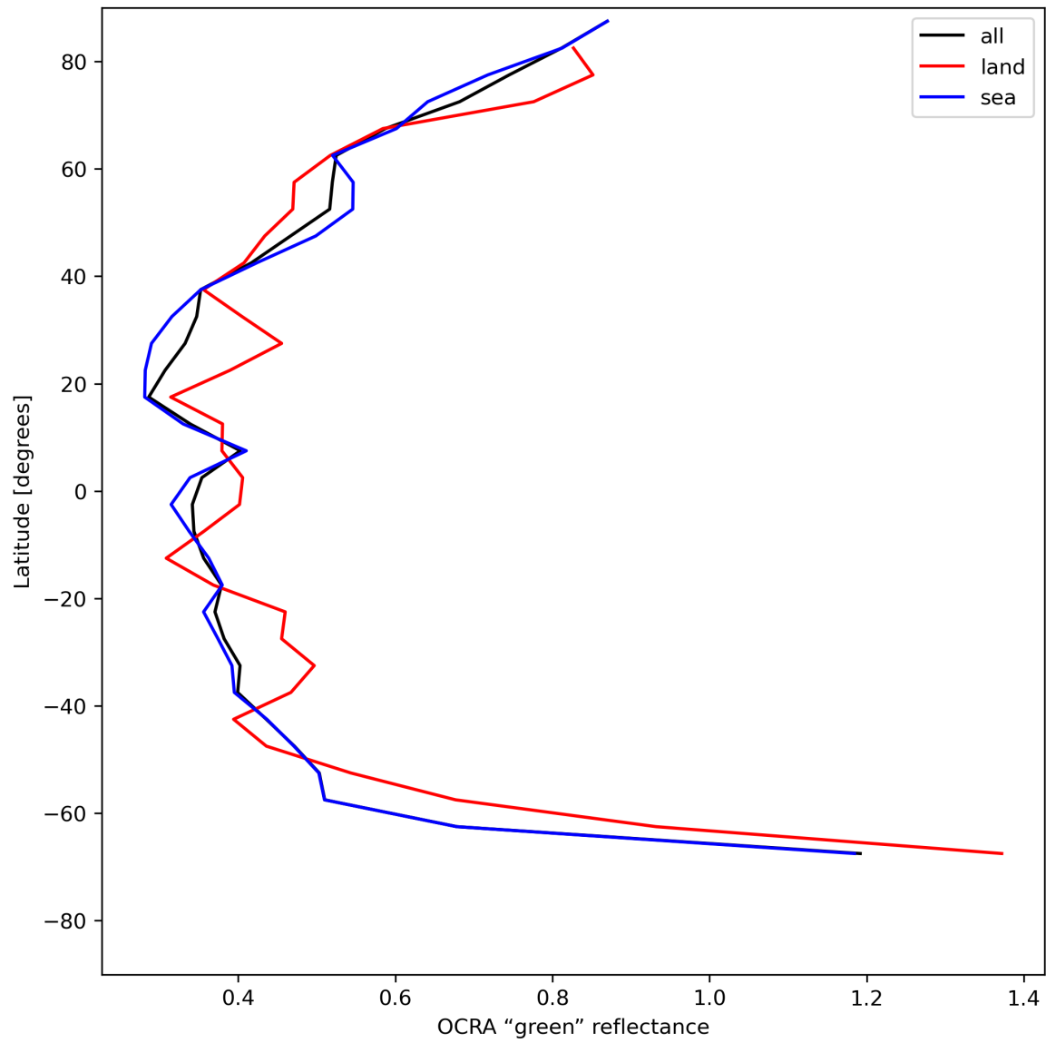
Figure 36: Zonal average of “OCRA “green” reflectance” for 2024-05-29 to 2024-05-31.
