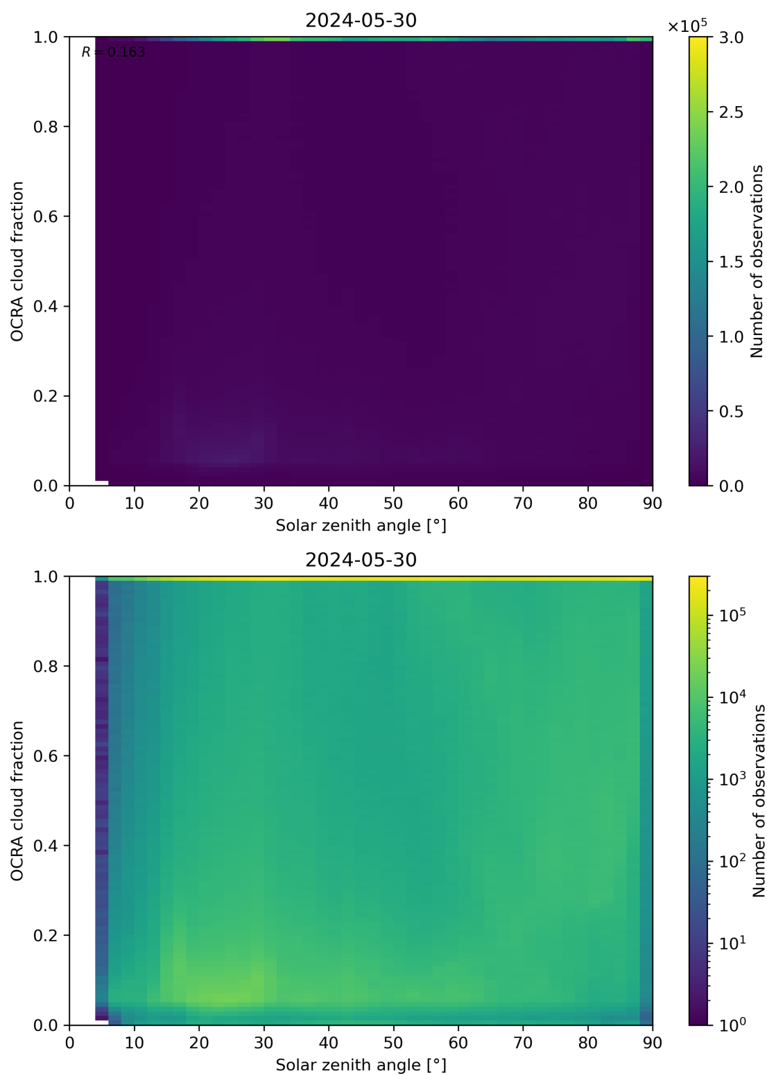
Figure 100: Scatter density plot of “Solar zenith angle” against “OCRA cloud fraction” for 2024-05-29 to 2024-05-31.
