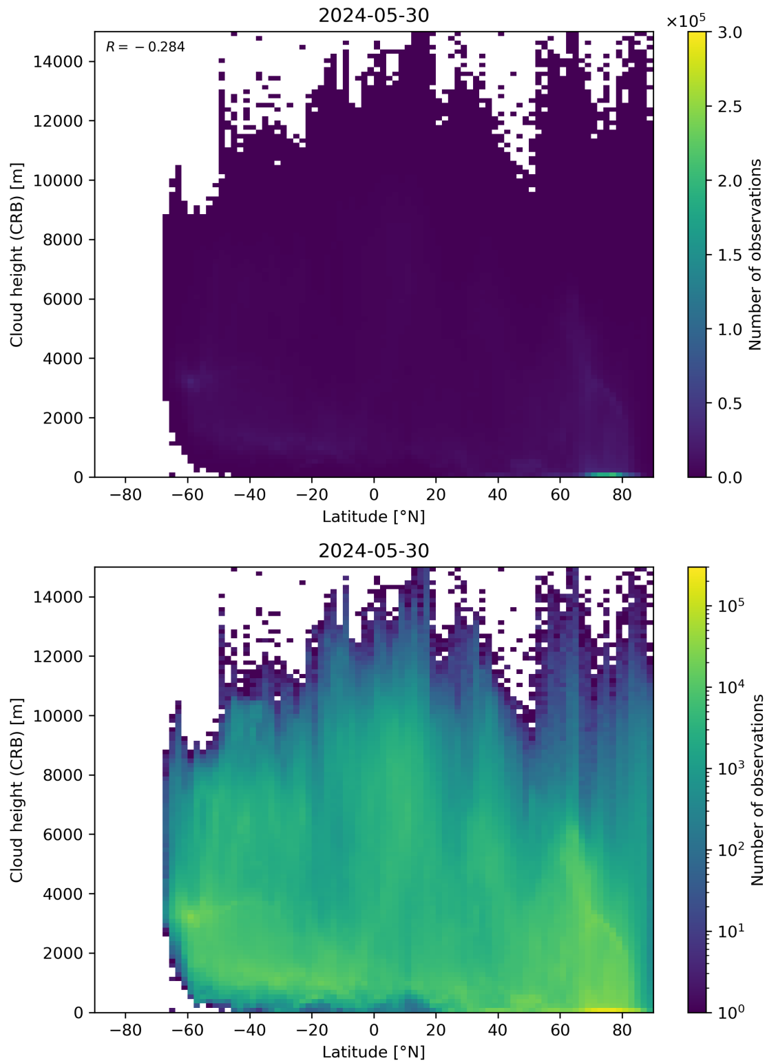
Figure 95: Scatter density plot of “Latitude” against “Cloud height (CRB)” for 2024-05-29 to 2024-05-31.
