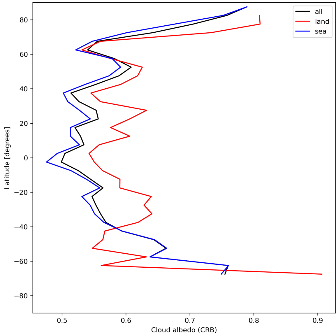
Figure 28: Zonal average of “Cloud albedo (CRB)” for 2024-05-29 to 2024-05-31.
