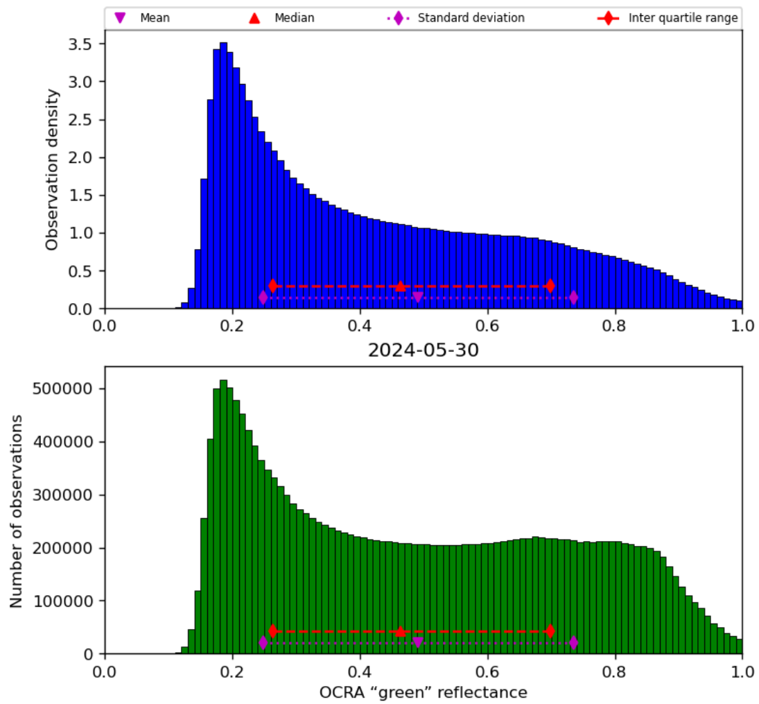
Figure 52: Histogram of “OCRA “green” reflectance” for 2024-05-29 to 2024-05-31
