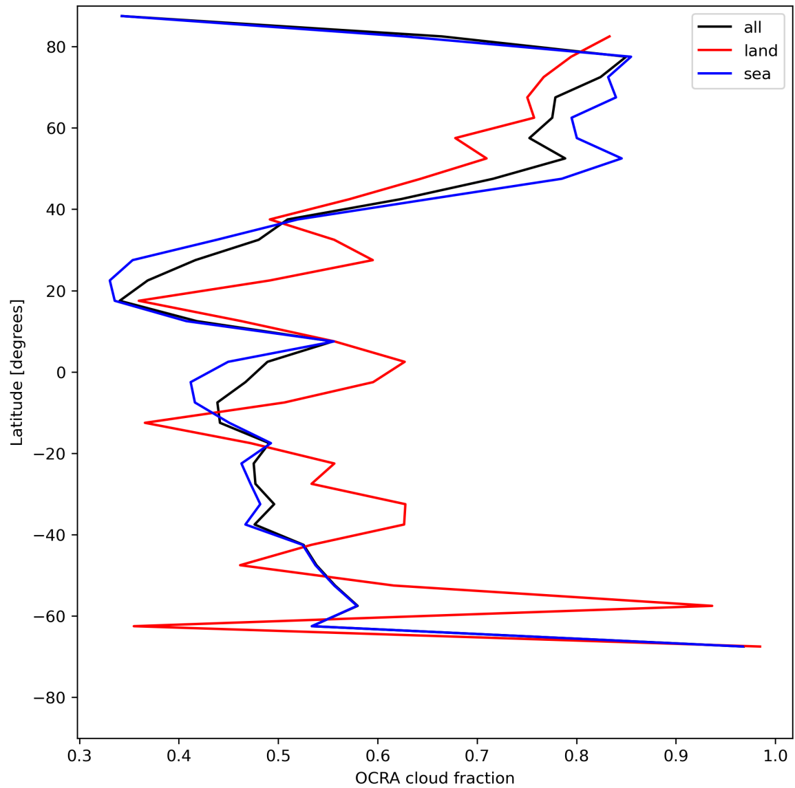
Figure 34: Zonal average of “OCRA cloud fraction” for 2024-05-29 to 2024-05-31.
