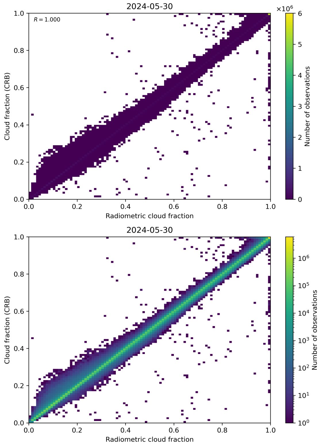
Figure 73: Scatter density plot of “Radiometric cloud fraction” against “Cloud fraction (CRB)” for 2024-05-29 to 2024-05-31.
