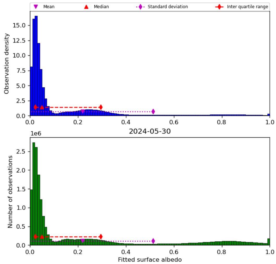
Figure 45: Histogram of “Fitted surface albedo” for 2024-05-29 to 2024-05-31
