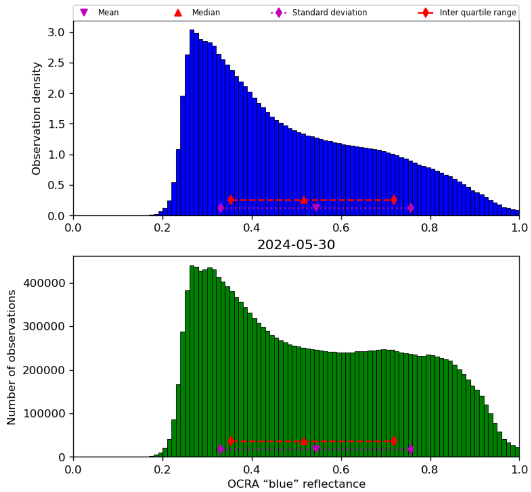
Figure 51: Histogram of “OCRA “blue” reflectance” for 2024-05-29 to 2024-05-31
