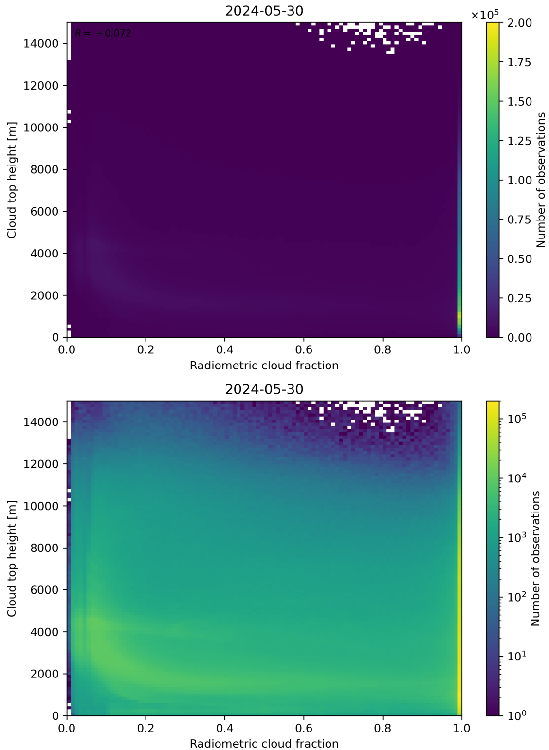
Figure 76: Scatter density plot of “Radiometric cloud fraction” against “Cloud top height” for 2024-05-29 to 2024-05-31.
