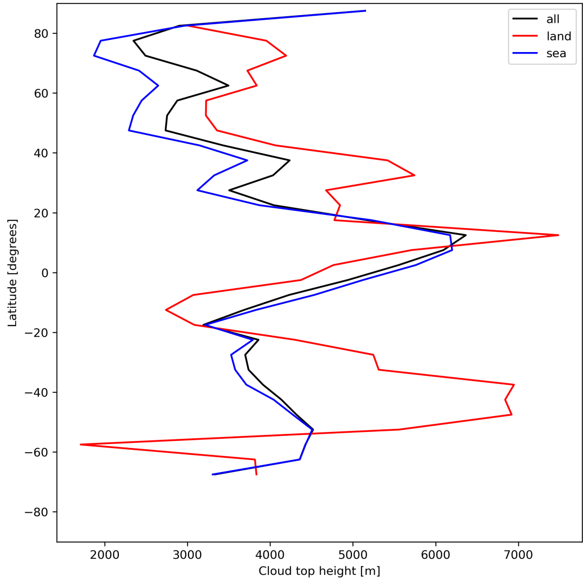
Figure 24: Zonal average of “Cloud top height” for 2024-05-29 to 2024-05-31.
