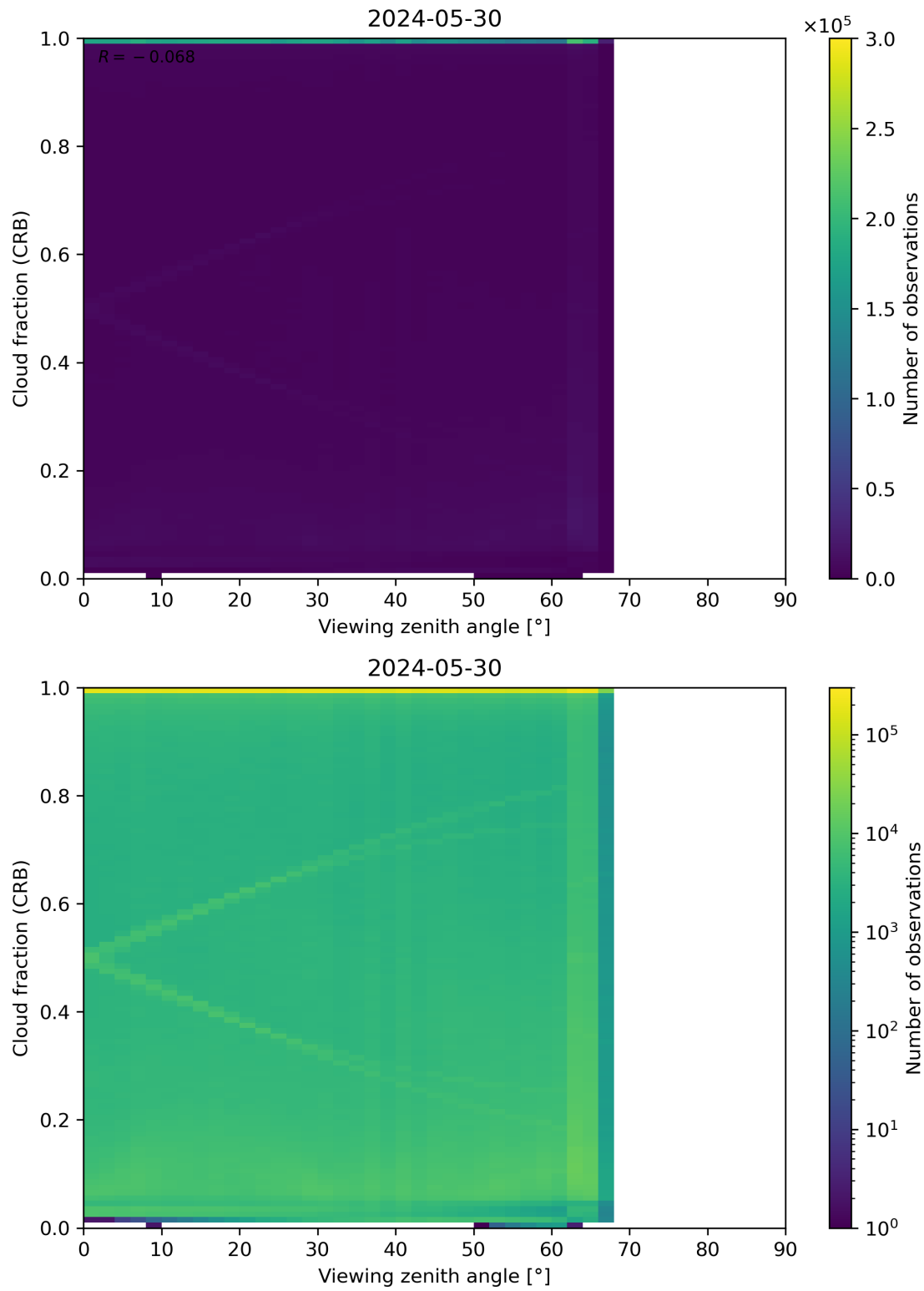
Figure 109: Scatter density plot of “Viewing zenith angle” against “Cloud fraction (CRB)” for 2024-05-29 to 2024-05-31.
