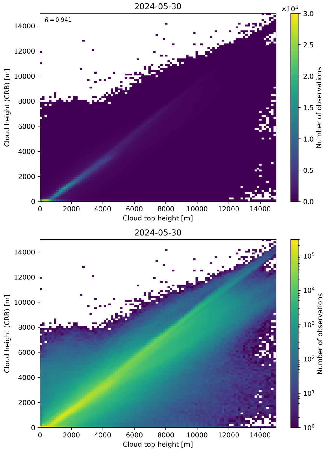
Figure 89: Scatter density plot of “Cloud top height” against “Cloud height (CRB)” for 2024-05-29 to 2024-05-31.
