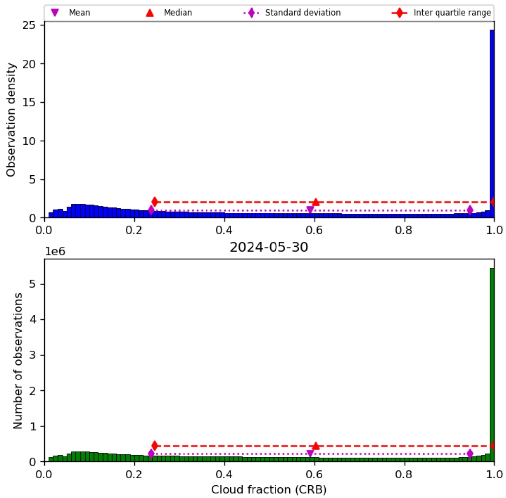
Figure 42: Histogram of “Cloud fraction (CRB)” for 2024-05-29 to 2024-05-31
