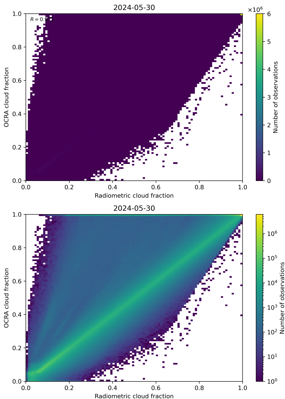
Figure 72: Scatter density plot of “Radiometric cloud fraction” against “OCRA cloud fraction” for 2024-05-29 to 2024-05-31.
