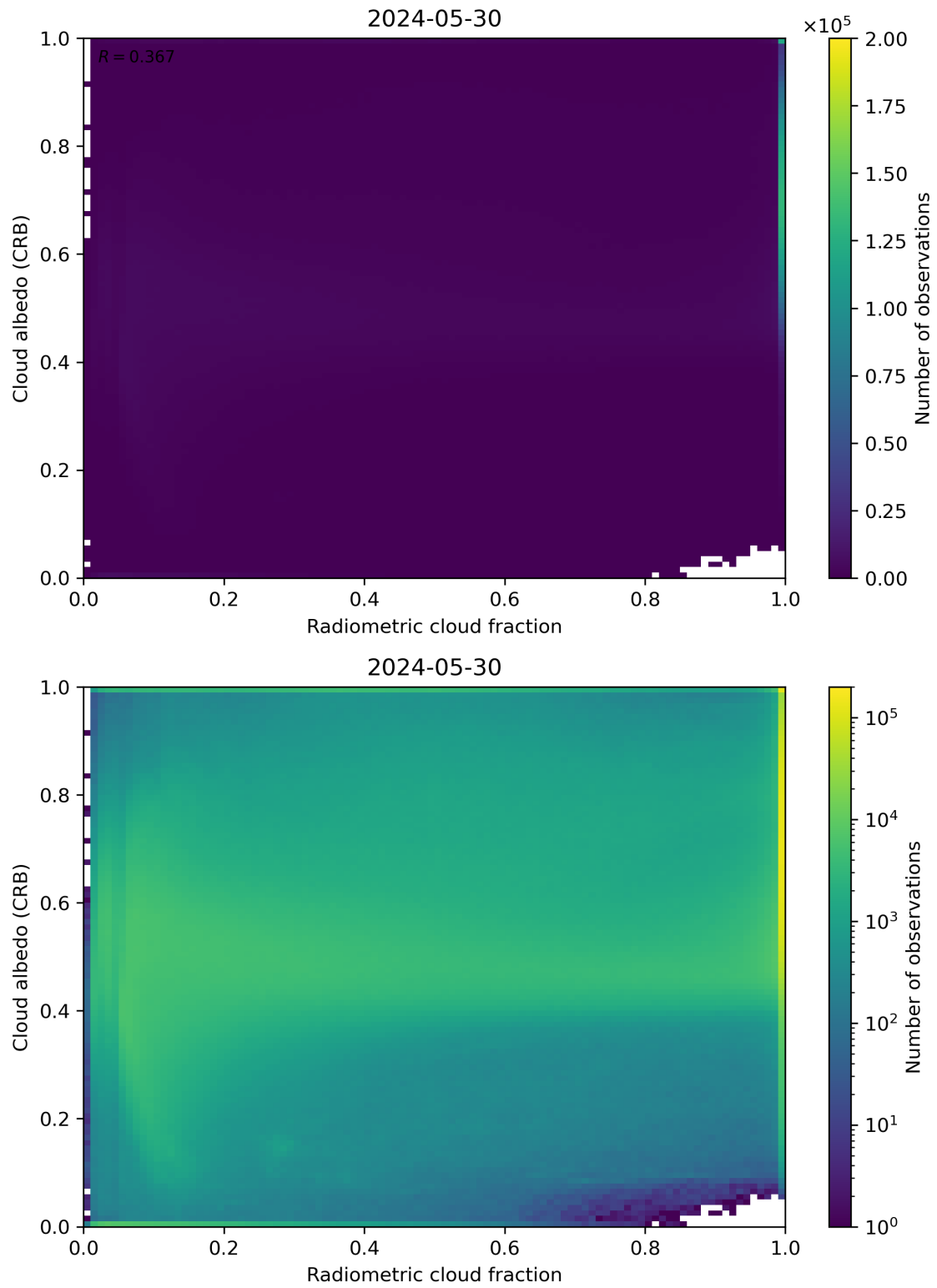
Figure 71: Scatter density plot of “Radiometric cloud fraction” against “Cloud albedo (CRB)” for 2024-05-29 to 2024-05-31.
