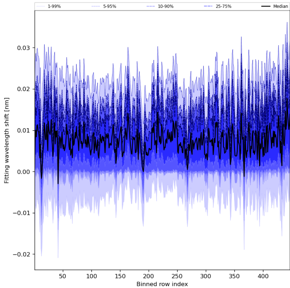
Figure 65: Along track statistics of “Fitting wavelength shift” for 2024-05-29 to 2024-05-31
