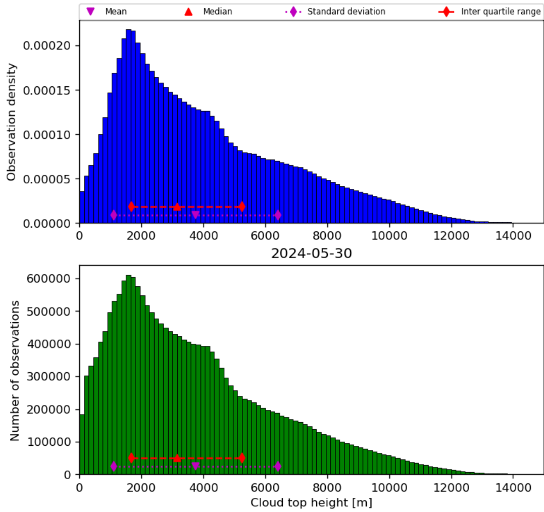
Figure 40: Histogram of “Cloud top height” for 2024-05-29 to 2024-05-31
