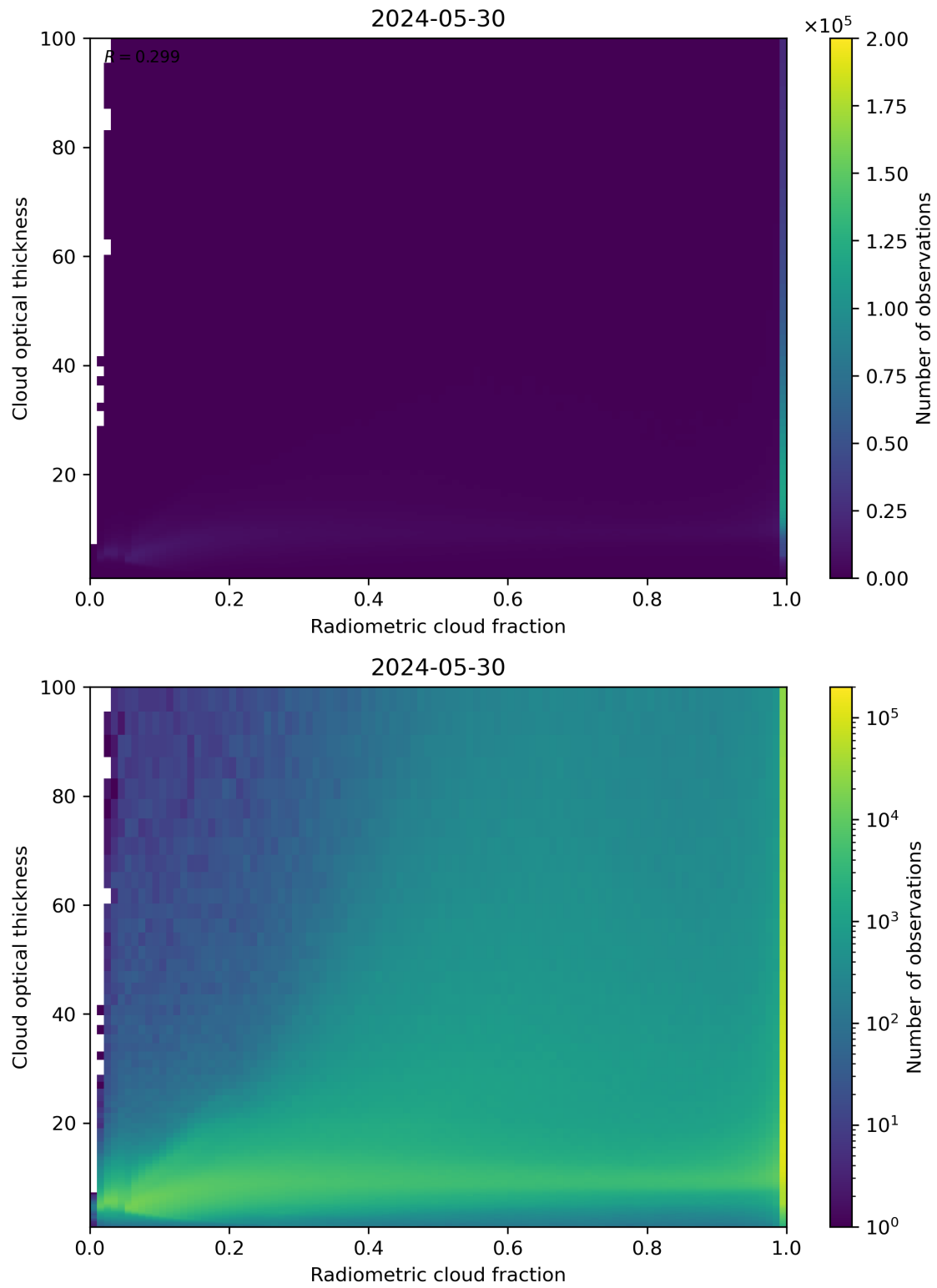
Figure 75: Scatter density plot of “Radiometric cloud fraction” against “Cloud optical thickness” for 2024-05-29 to 2024-05-31.
