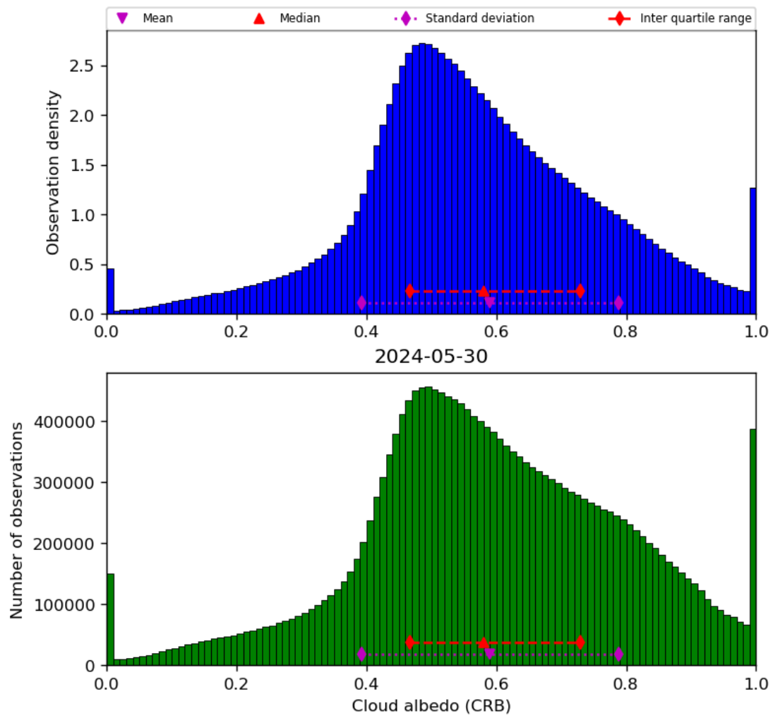
Figure 44: Histogram of “Cloud albedo (CRB)” for 2024-05-29 to 2024-05-31
