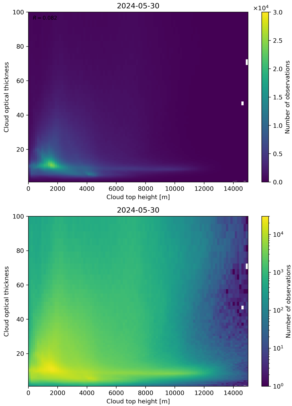
Figure 90: Scatter density plot of “Cloud top height” against “Cloud optical thickness” for 2024-05-29 to 2024-05-31.
