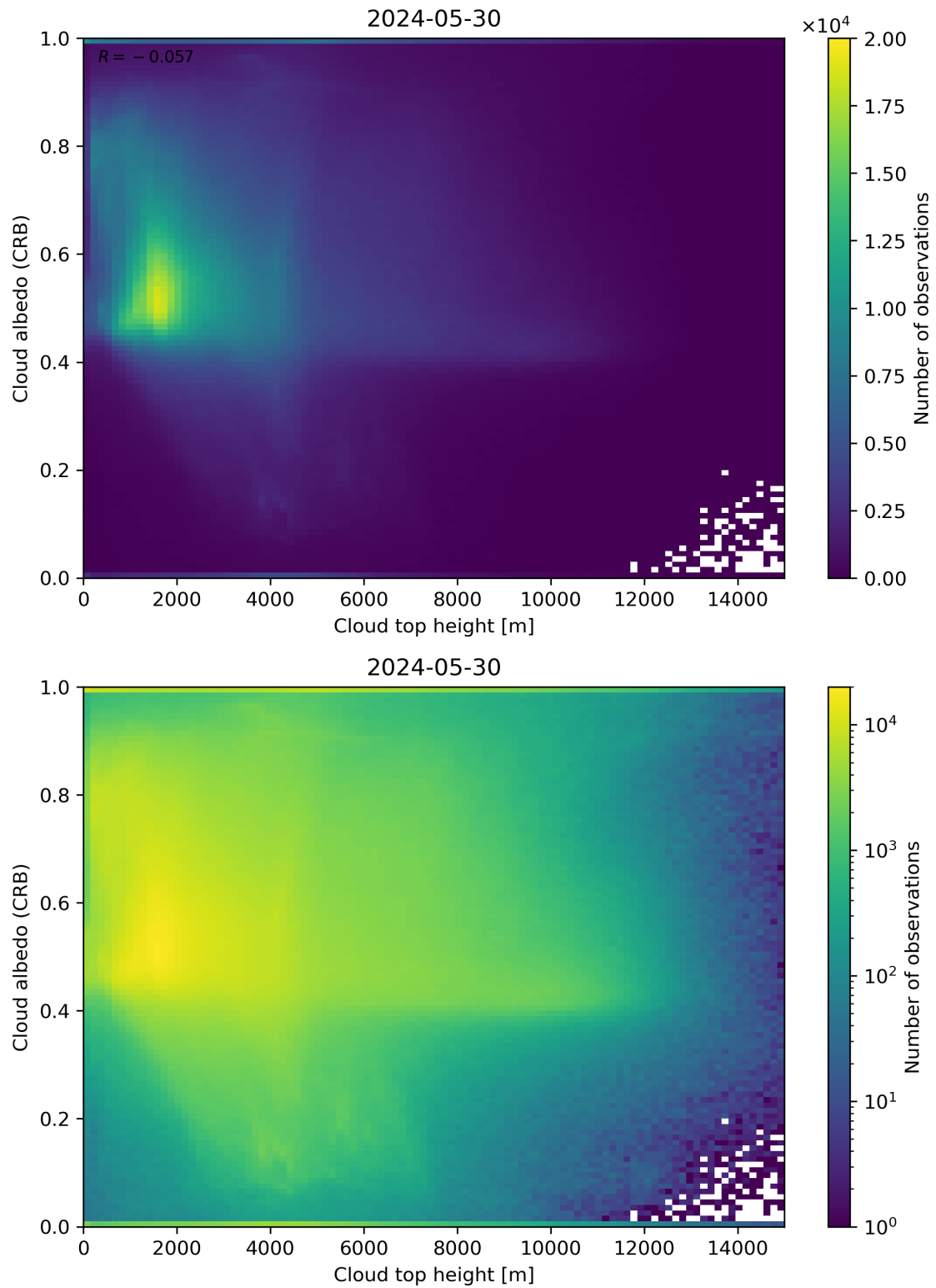
Figure 86: Scatter density plot of “Cloud top height” against “Cloud albedo (CRB)” for 2024-05-29 to 2024-05-31.
