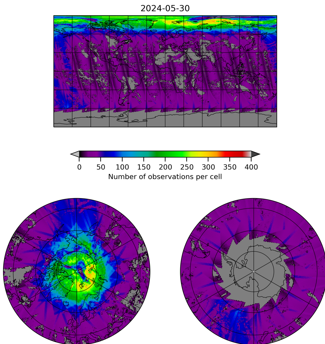
Figure 21: Map of the number of observations for 2024-05-29 to 2024-05-31
