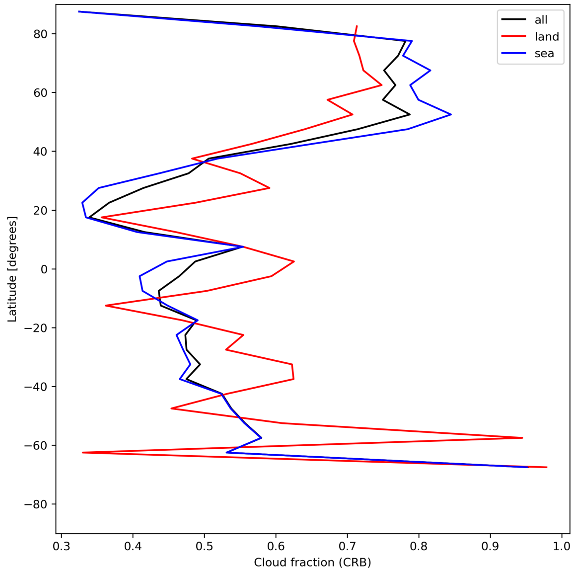
Figure 26: Zonal average of “Cloud fraction (CRB)” for 2024-05-29 to 2024-05-31.
