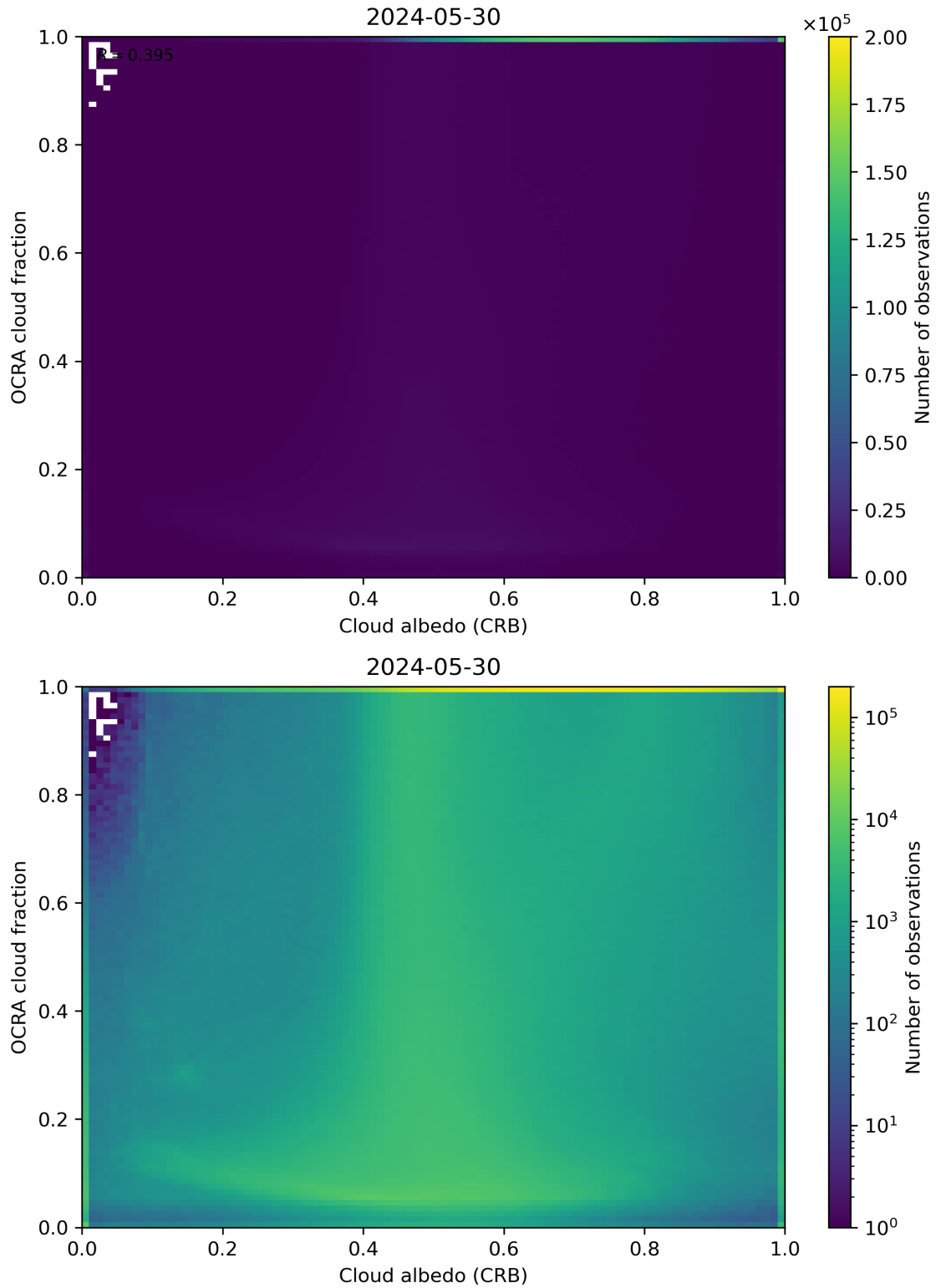
Figure 70: Scatter density plot of “Cloud albedo (CRB)” against “OCRA cloud fraction” for 2024-05-29 to 2024-05-31.
