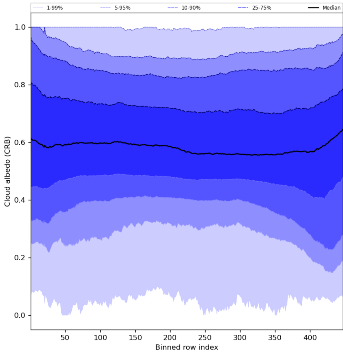
Figure 60: Along track statistics of “Cloud albedo (CRB)” for 2024-05-29 to 2024-05-31
