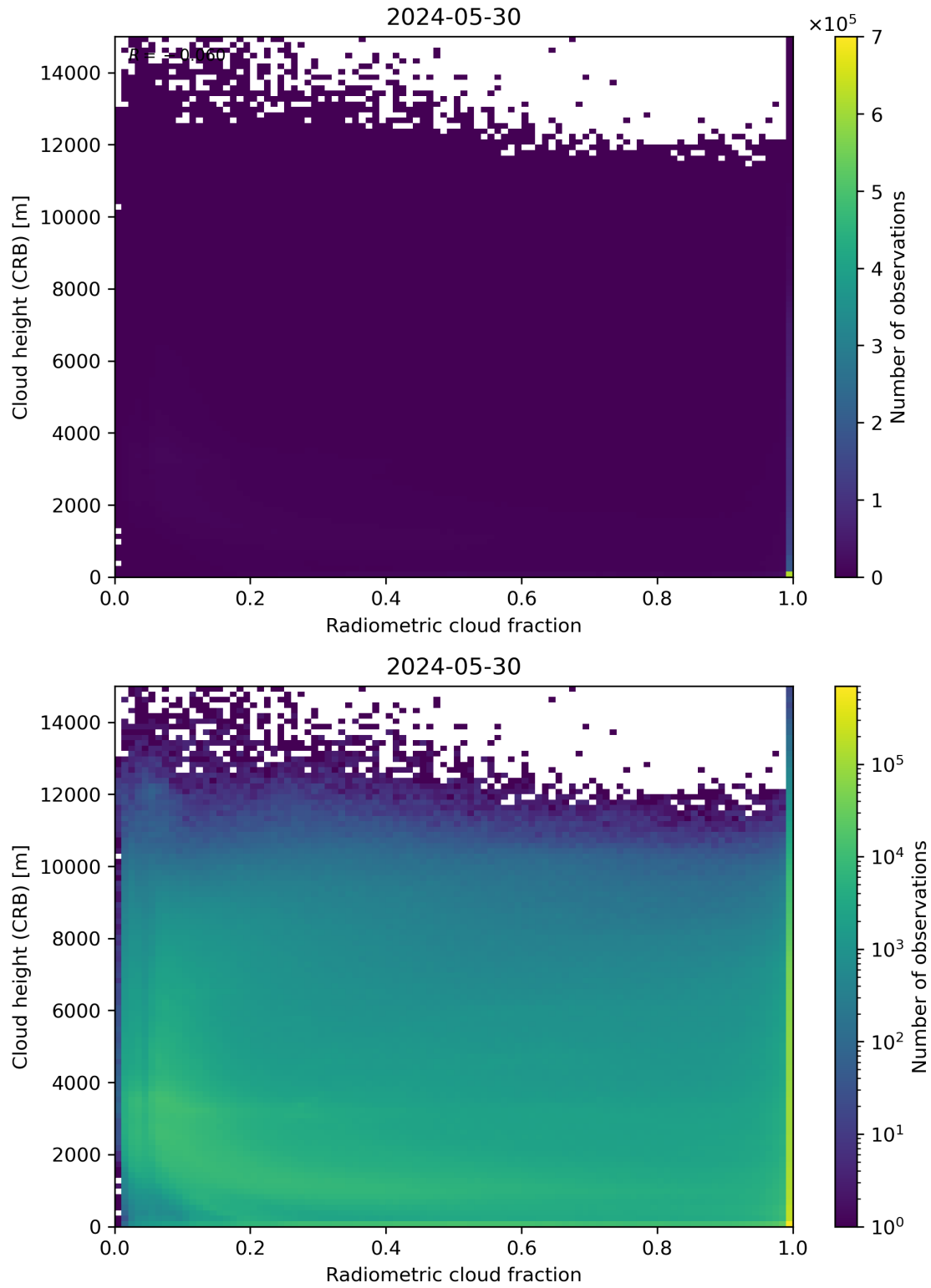
Figure 74: Scatter density plot of “Radiometric cloud fraction” against “Cloud height (CRB)” for 2024-05-29 to 2024-05-31.
