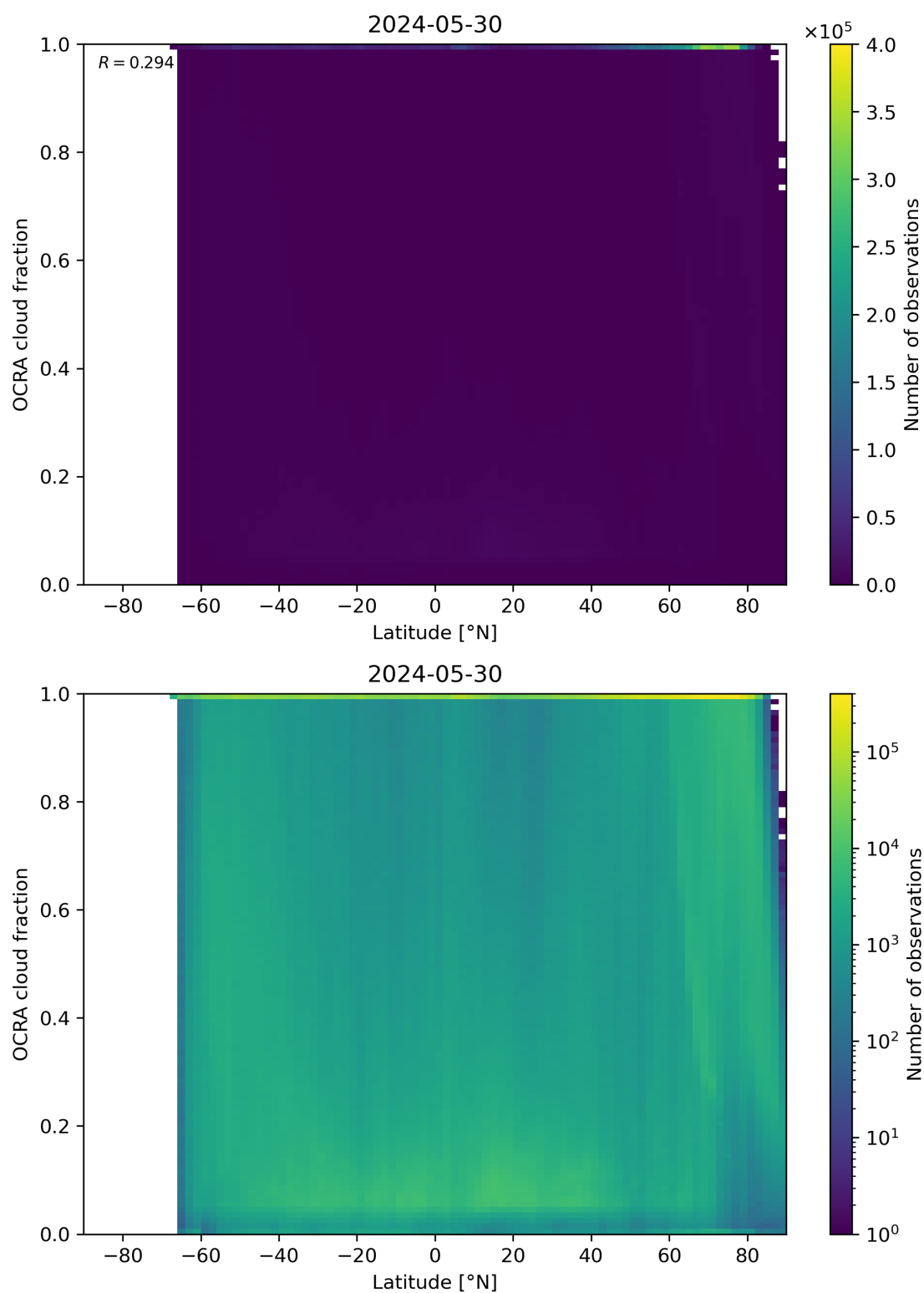
Figure 93: Scatter density plot of “Latitude” against “OCRA cloud fraction” for 2024-05-29 to 2024-05-31.
