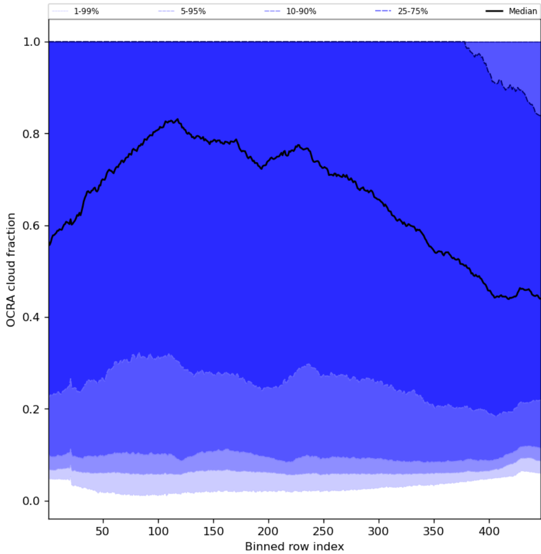
Figure 66: Along track statistics of “OCRA cloud fraction” for 2024-05-29 to 2024-05-31
