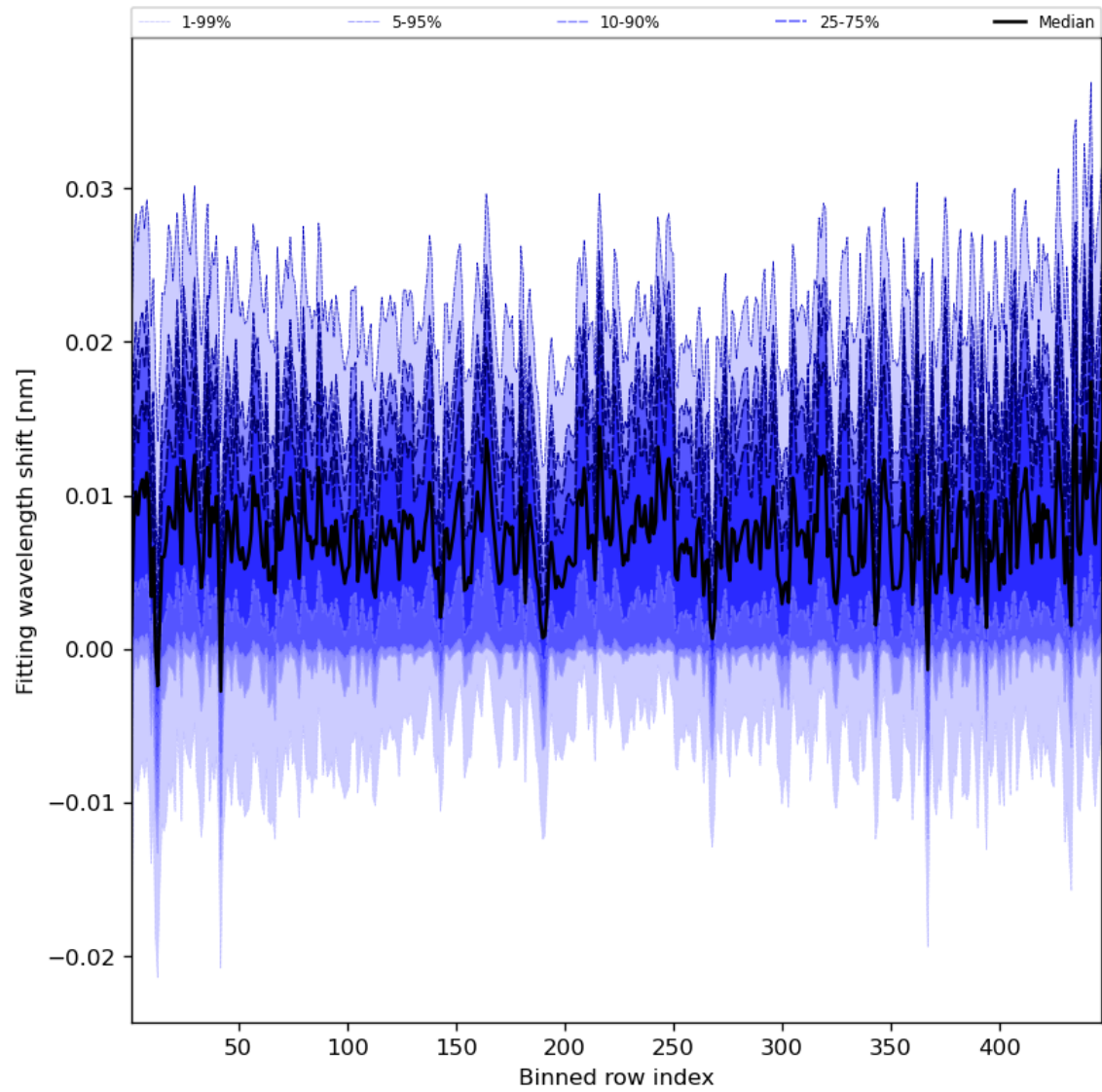
Figure 65: Along track statistics of “Fitting wavelength shift” for 2024-05-31 to 2024-06-02
