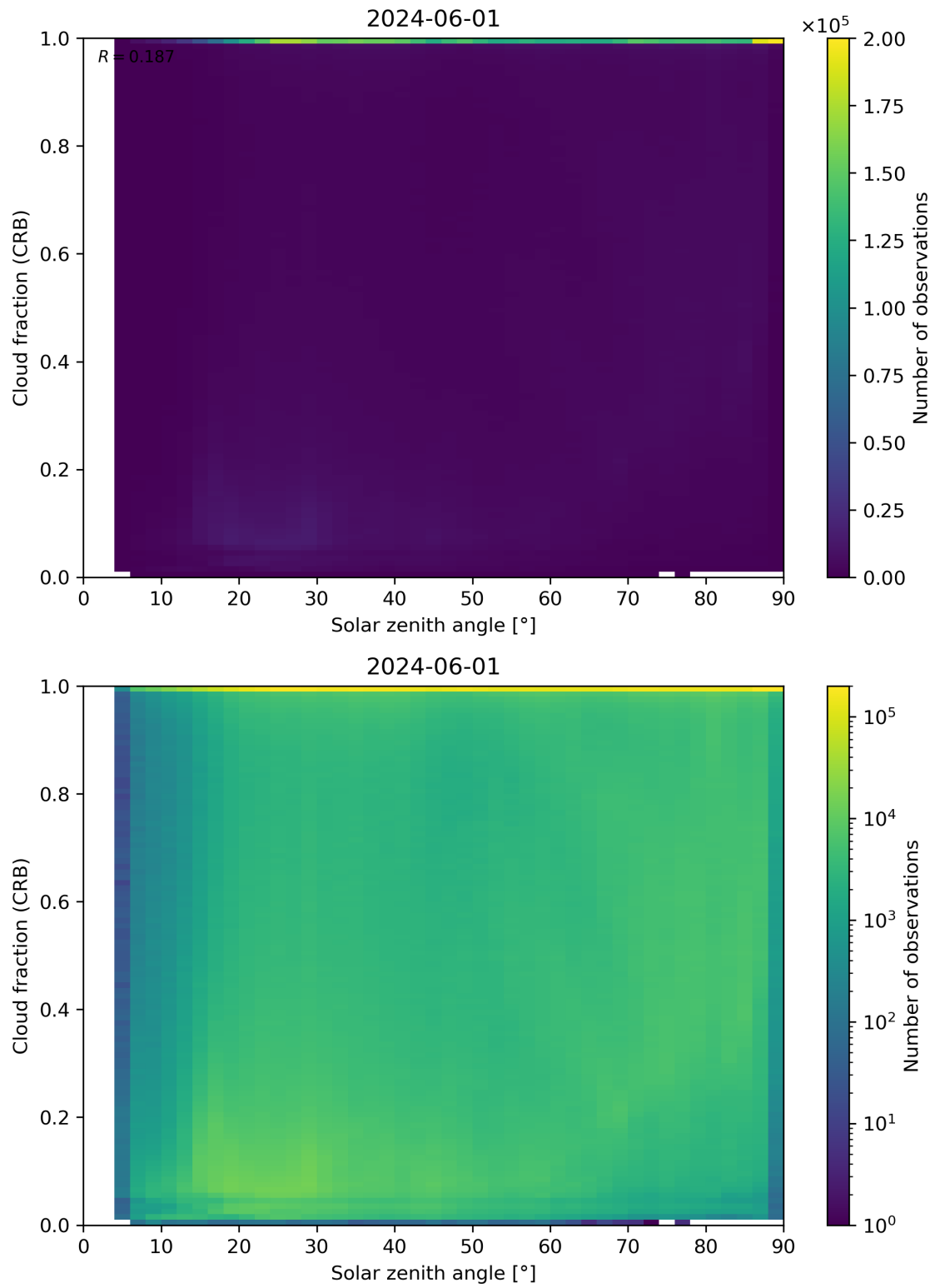
Figure 101: Scatter density plot of “Solar zenith angle” against “Cloud fraction (CRB)” for 2024-05-31 to 2024-06-02.
