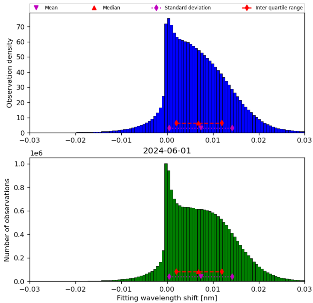
Figure 49: Histogram of “Fitting wavelength shift” for 2024-05-31 to 2024-06-02
