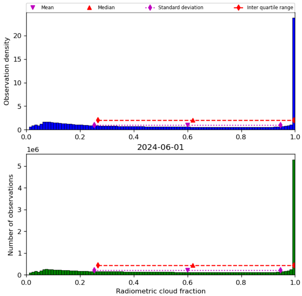
Figure 39: Histogram of “Radiometric cloud fraction” for 2024-05-31 to 2024-06-02
