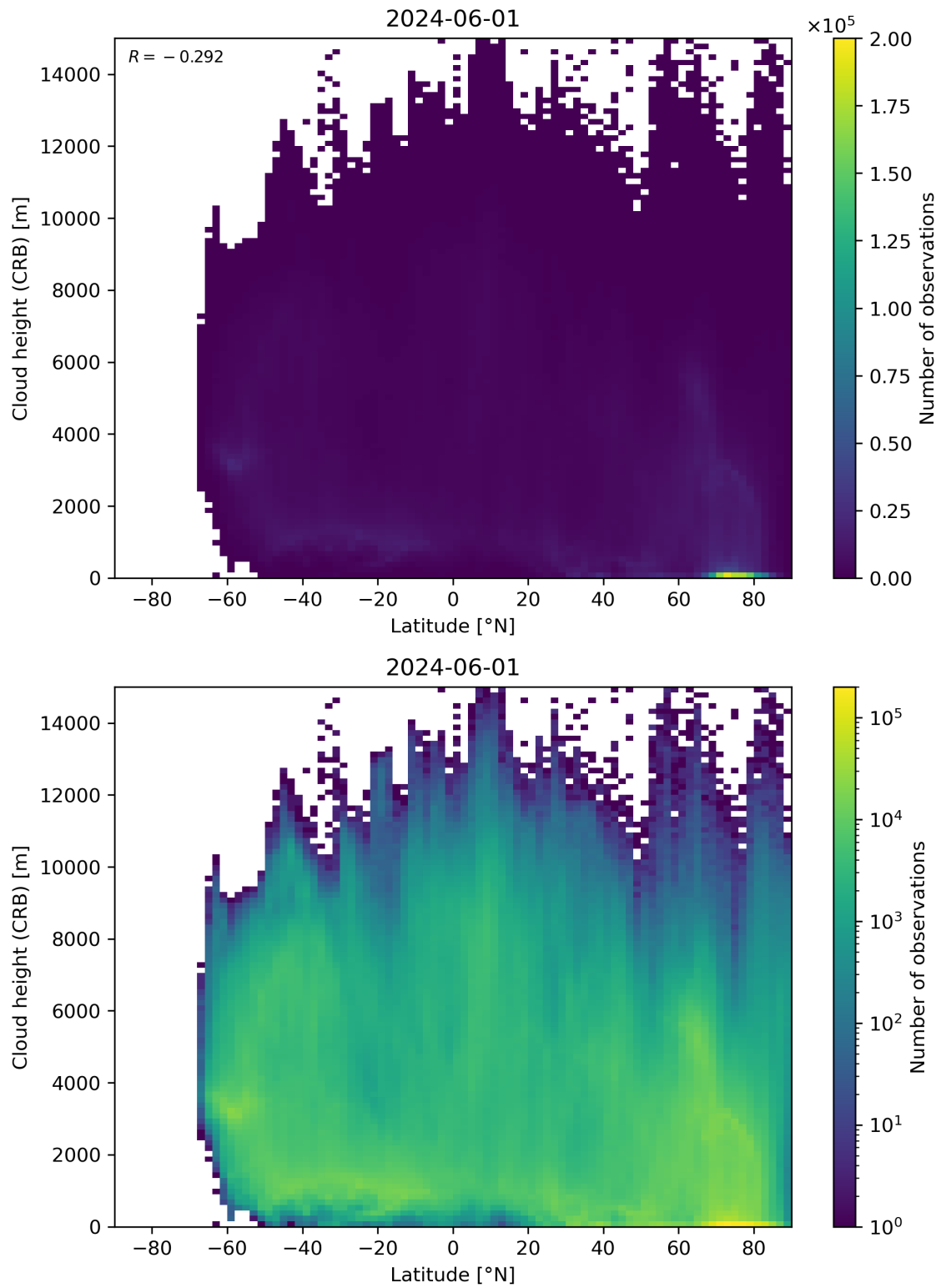
Figure 95: Scatter density plot of “Latitude” against “Cloud height (CRB)” for 2024-05-31 to 2024-06-02.
