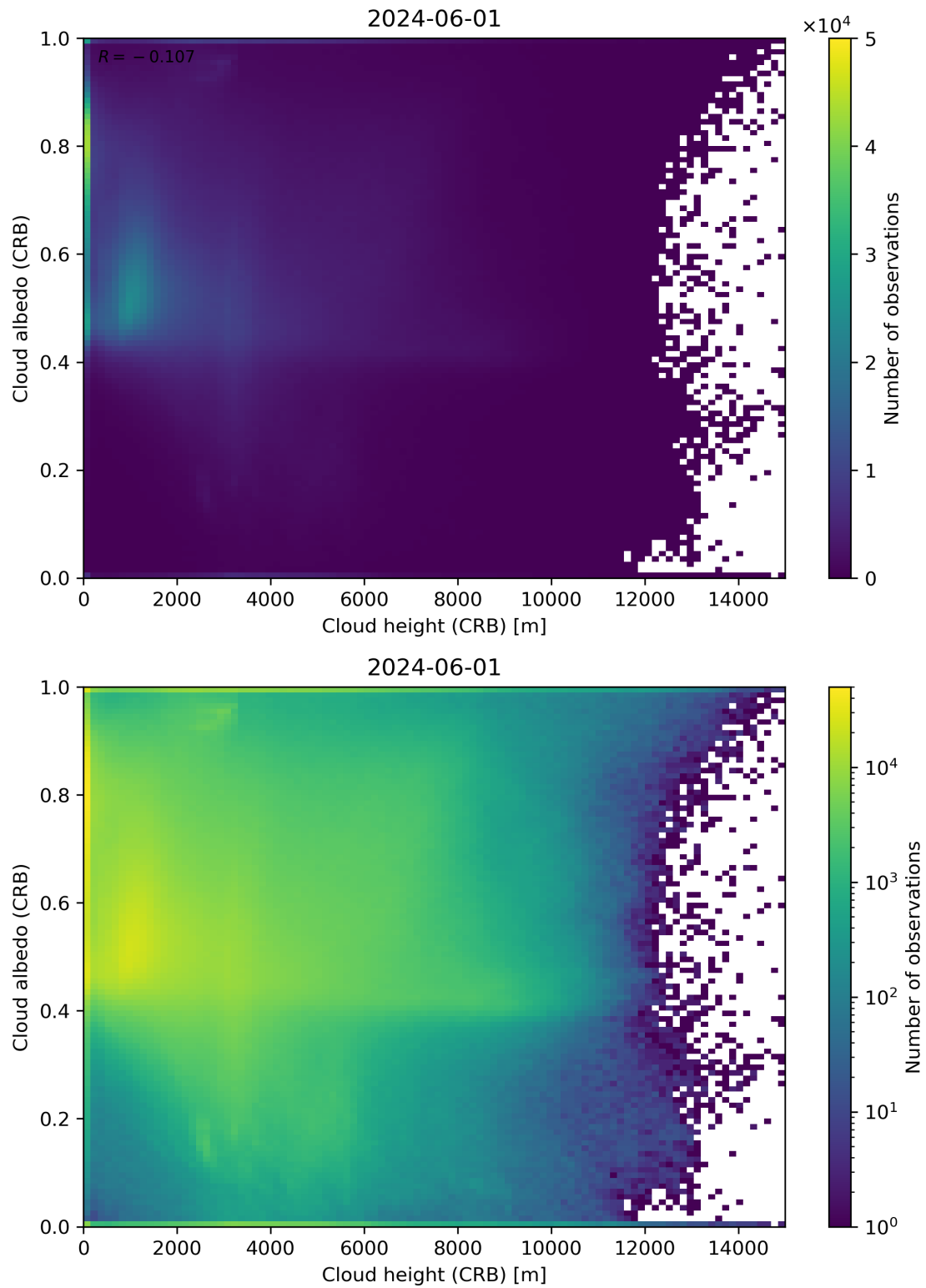
Figure 80: Scatter density plot of “Cloud height (CRB)” against “Cloud albedo (CRB)” for 2024-05-31 to 2024-06-02.
