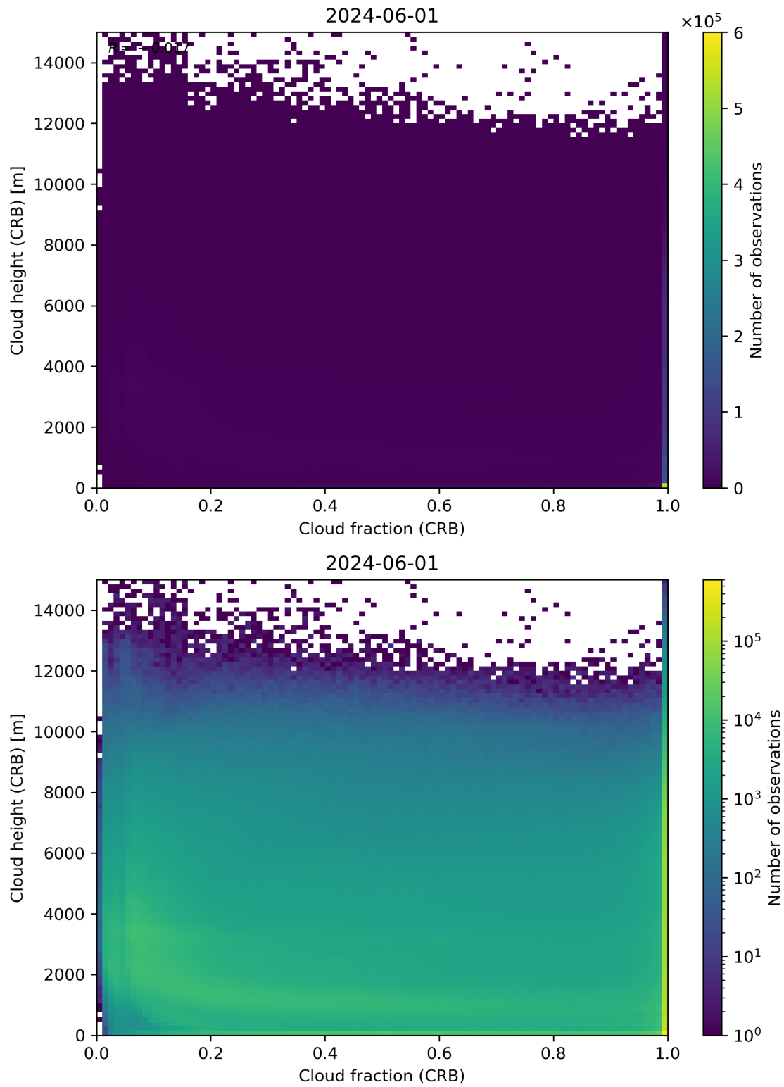
Figure 79: Scatter density plot of “Cloud fraction (CRB)” against “Cloud height (CRB)” for 2024-05-31 to 2024-06-02.
