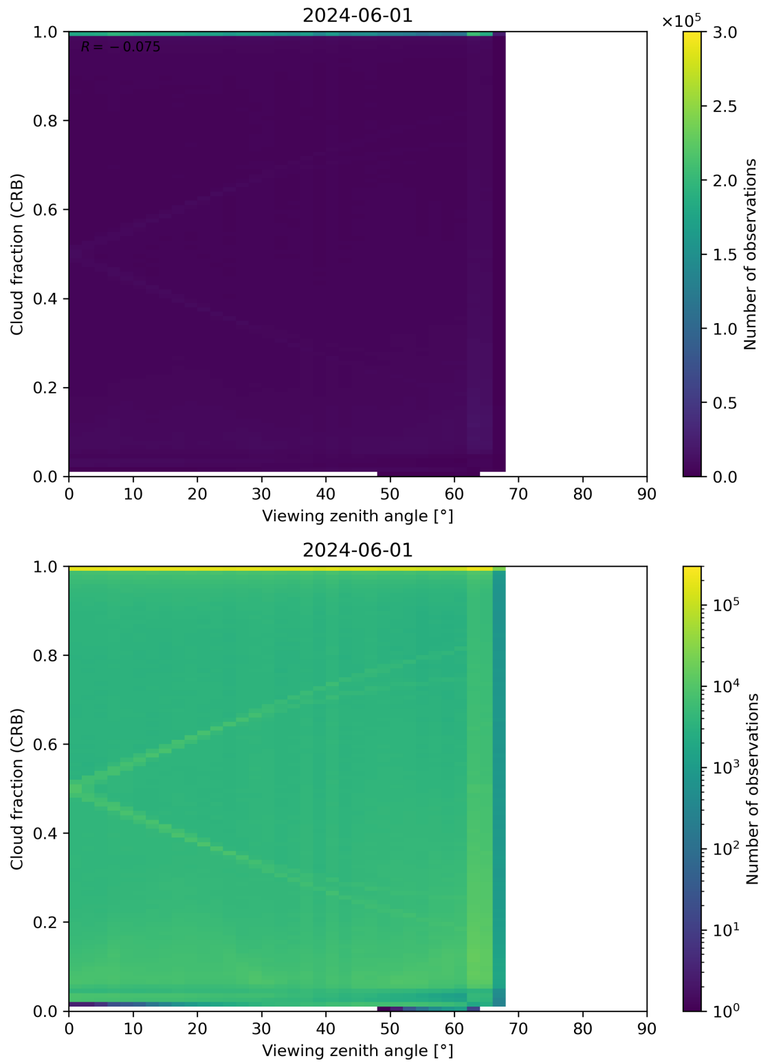
Figure 109: Scatter density plot of “Viewing zenith angle” against “Cloud fraction (CRB)” for 2024-05-31 to 2024-06-02.
