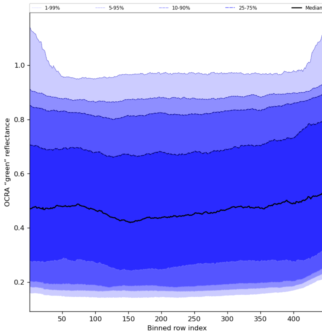
Figure 68: Along track statistics of “OCRA “green” reflectance” for 2024-05-31 to 2024-06-02
