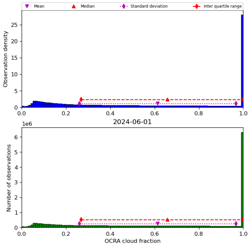
Figure 50: Histogram of “OCRA cloud fraction” for 2024-05-31 to 2024-06-02
