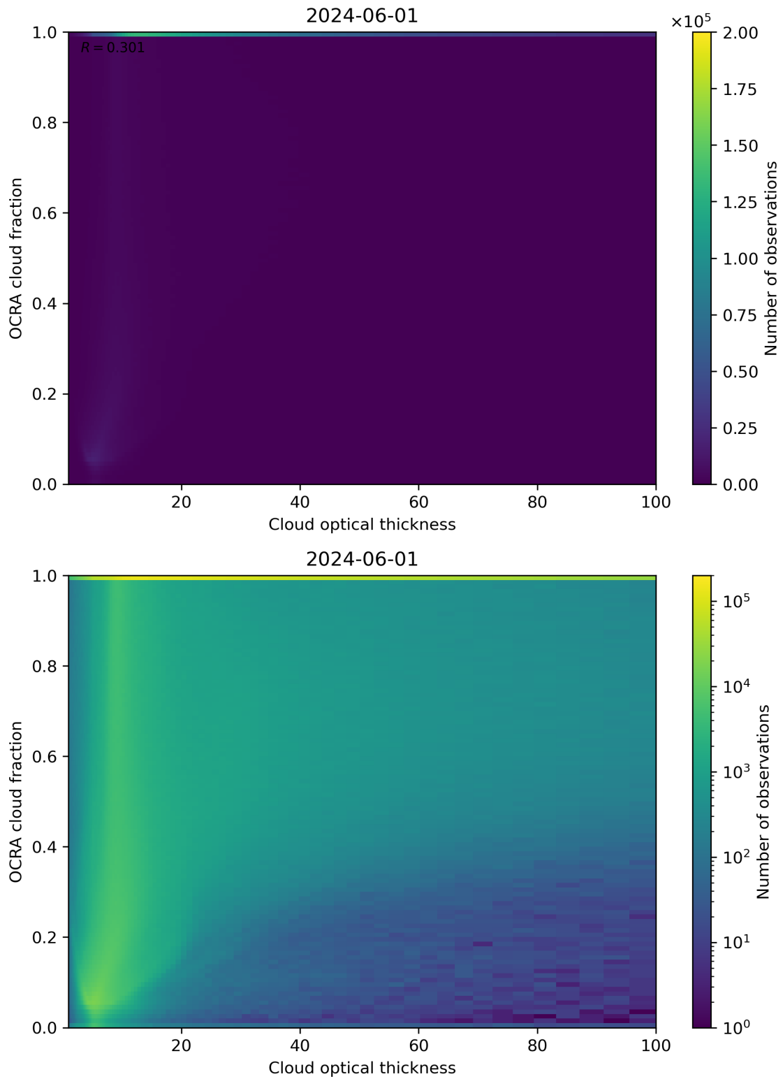
Figure 83: Scatter density plot of “Cloud optical thickness” against “OCRA cloud fraction” for 2024-05-31 to 2024-06-02.
