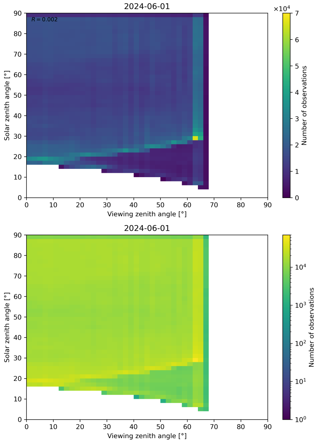
Figure 114: Scatter density plot of “Viewing zenith angle” against “Solar zenith angle” for 2024-05-31 to 2024-06-02.
