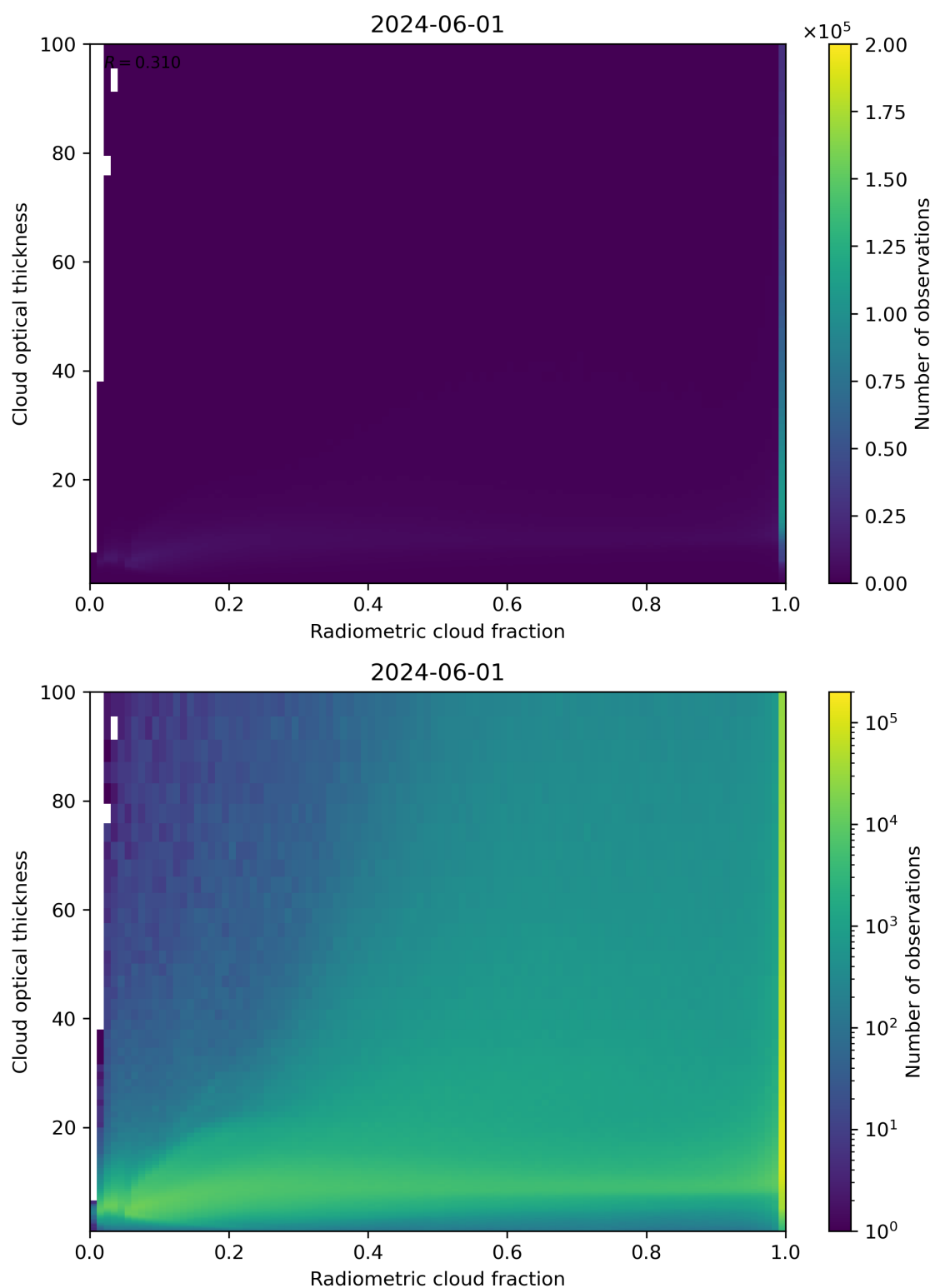
Figure 75: Scatter density plot of “Radiometric cloud fraction” against “Cloud optical thickness” for 2024-05-31 to 2024-06-02.
