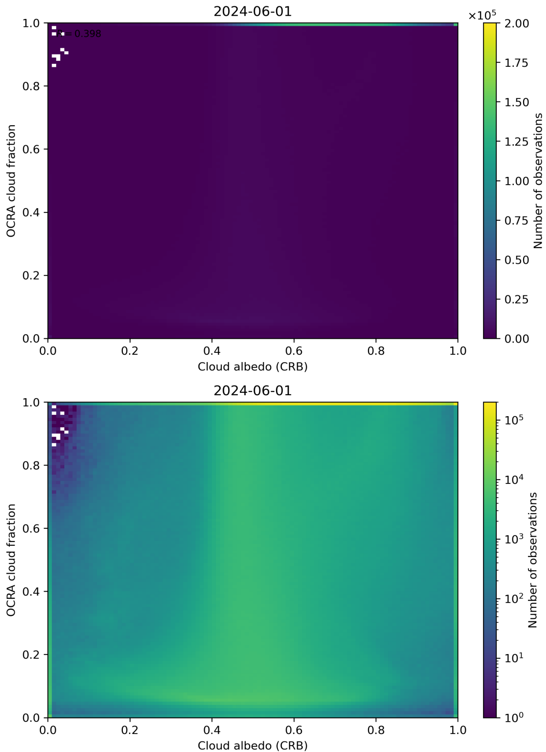
Figure 70: Scatter density plot of “Cloud albedo (CRB)” against “OCRA cloud fraction” for 2024-05-31 to 2024-06-02.
