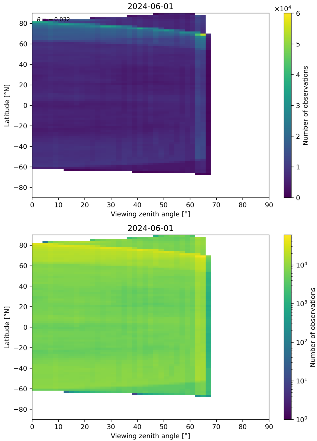
Figure 113: Scatter density plot of “Viewing zenith angle” against “Latitude” for 2024-05-31 to 2024-06-02.
