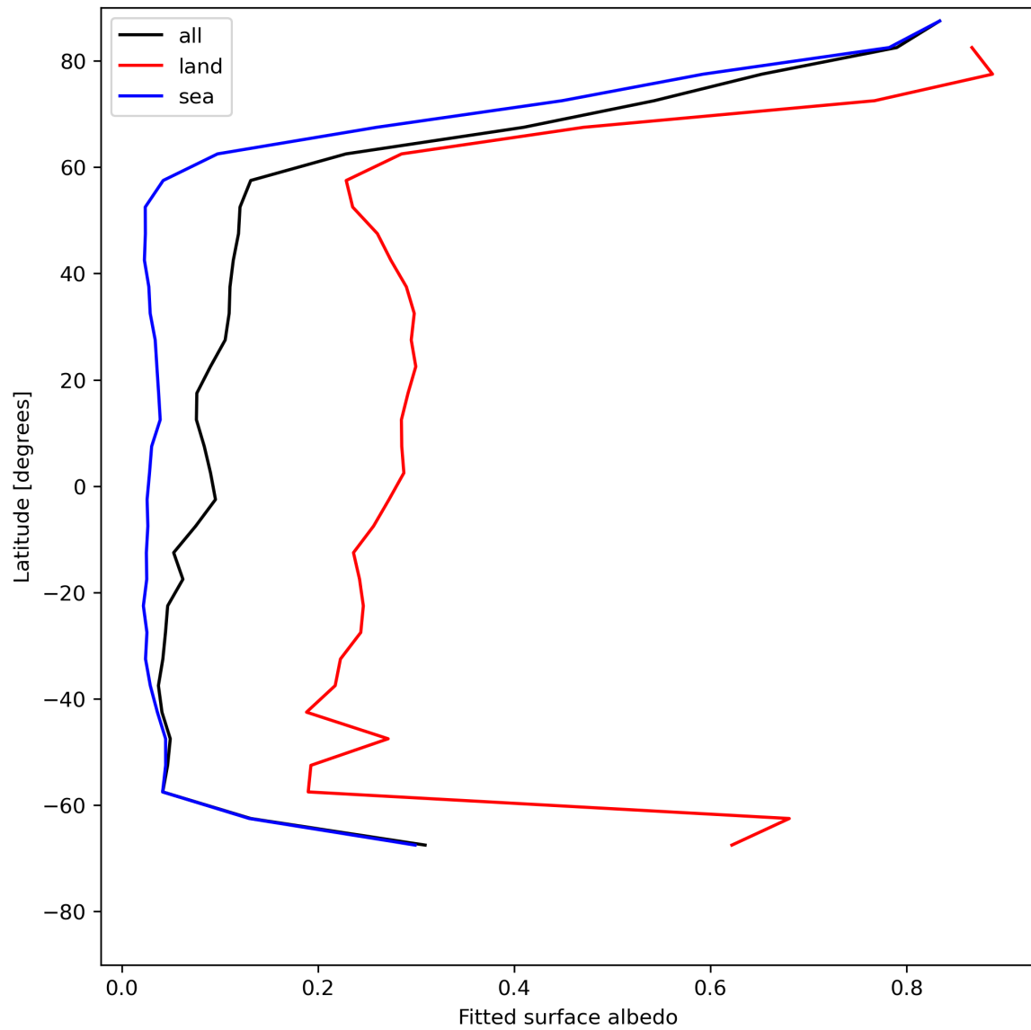
Figure 29: Zonal average of “Fitted surface albedo” for 2024-05-31 to 2024-06-02.
