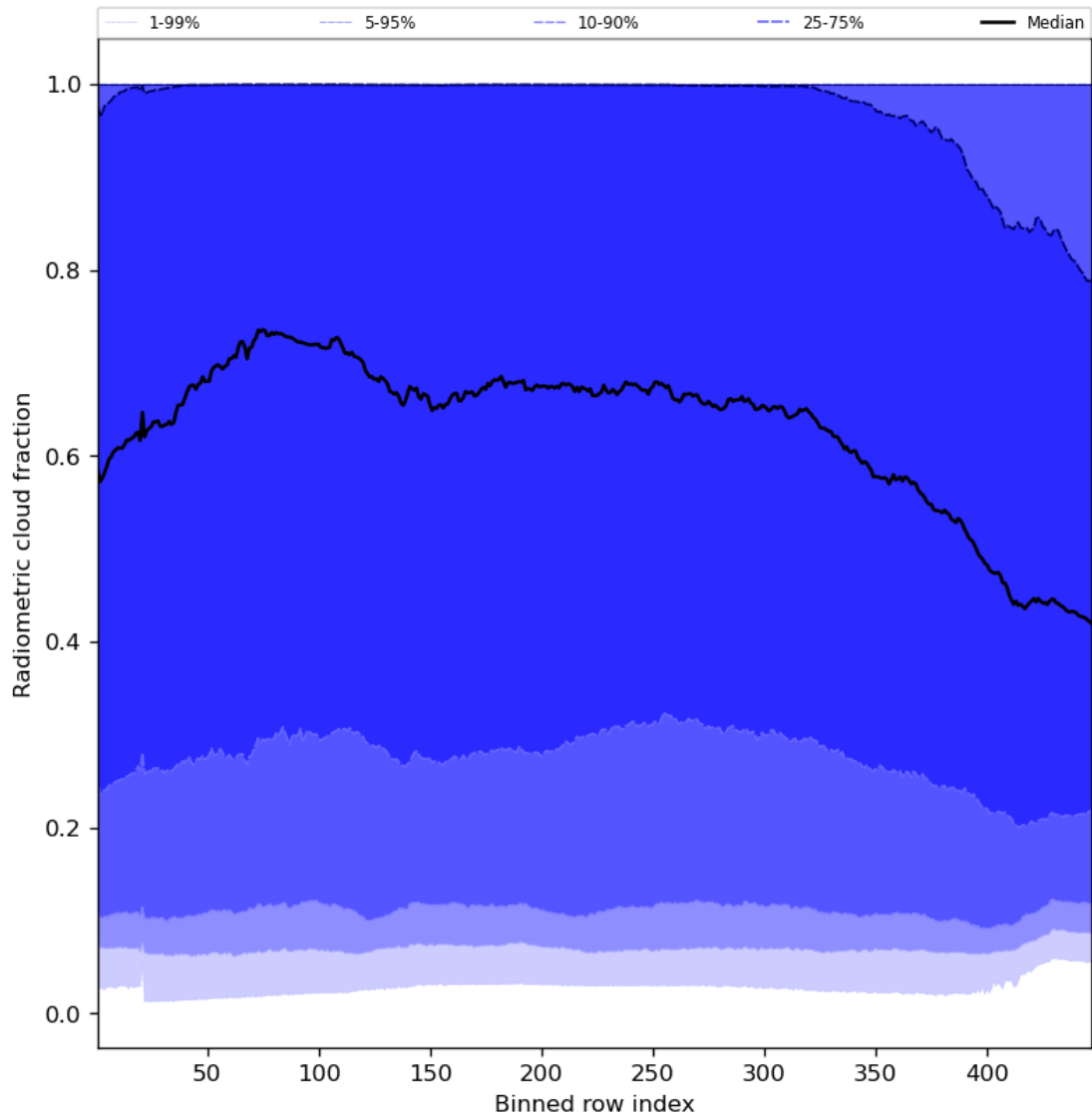
Figure 55: Along track statistics of “Radiometric cloud fraction” for 2024-05-31 to 2024-06-02
