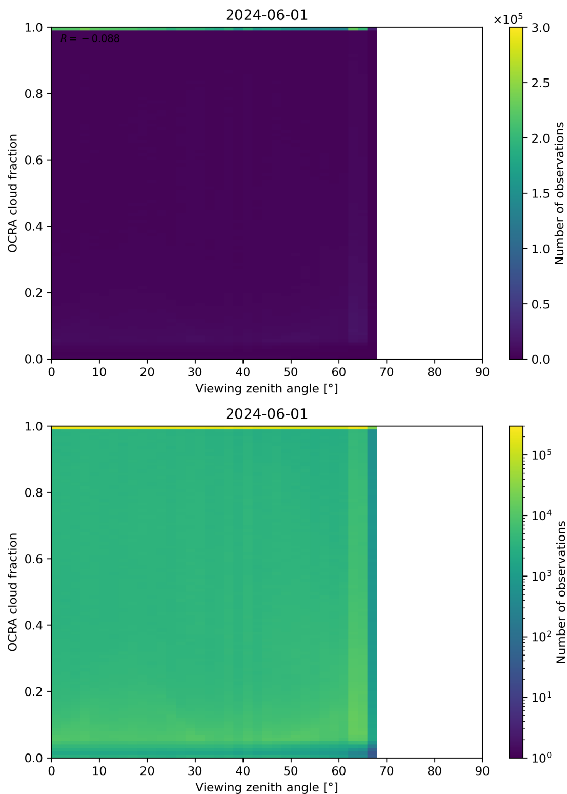
Figure 108: Scatter density plot of “Viewing zenith angle” against “OCRA cloud fraction” for 2024-05-31 to 2024-06-02.
