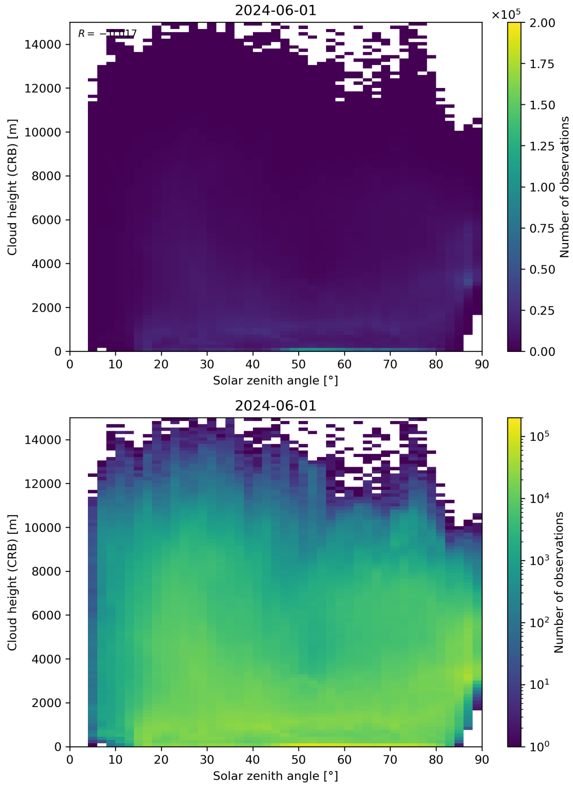
Figure 102: Scatter density plot of “Solar zenith angle” against “Cloud height (CRB)” for 2024-05-31 to 2024-06-02.
