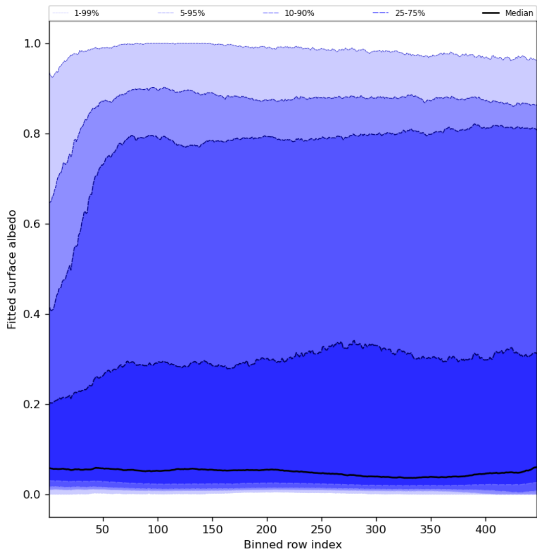
Figure 61: Along track statistics of “Fitted surface albedo” for 2024-05-31 to 2024-06-02
