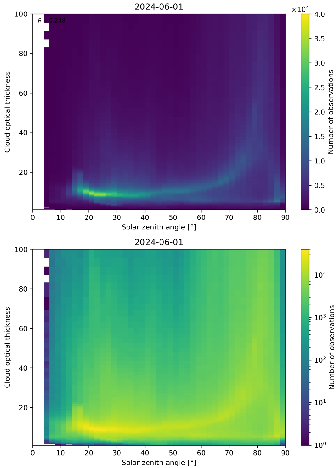
Figure 103: Scatter density plot of “Solar zenith angle” against “Cloud optical thickness” for 2024-05-31 to 2024-06-02.
