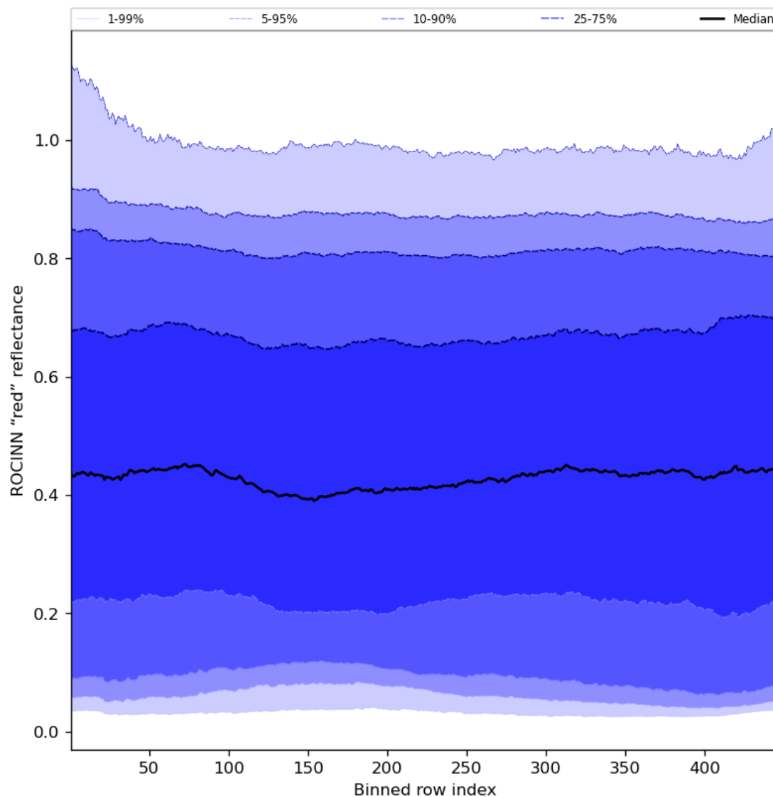
Figure 69: Along track statistics of "ROCINN "red" reflectance" for 2024-05-31 to 2024-06-02
