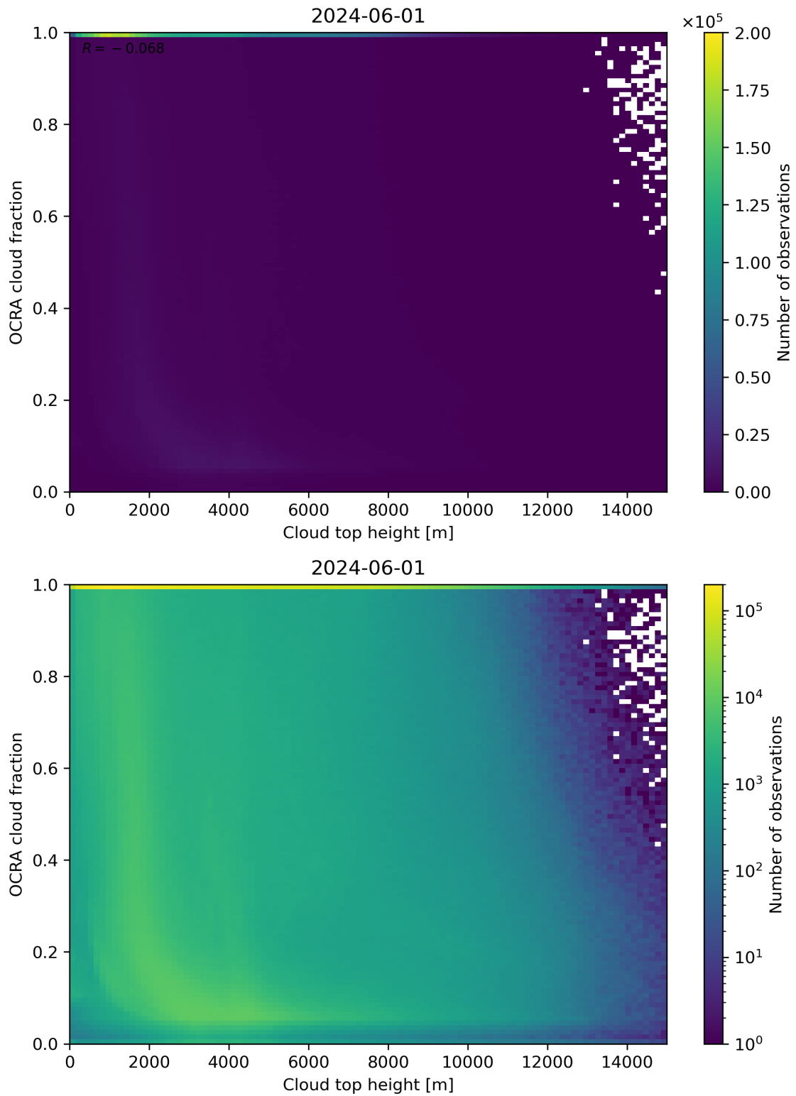
Figure 87: Scatter density plot of “Cloud top height” against “OCRA cloud fraction” for 2024-05-31 to 2024-06-02.
