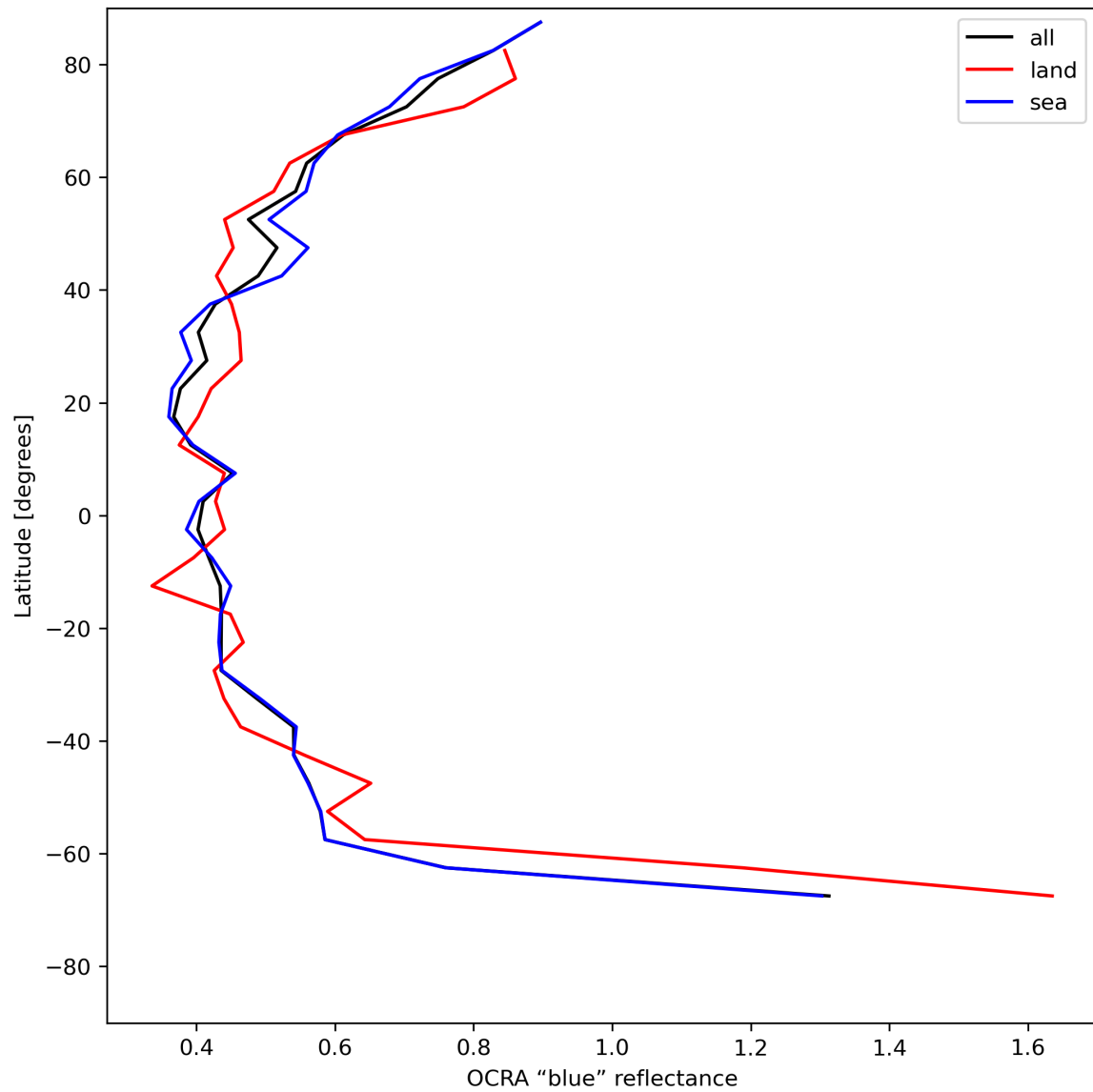
Figure 35: Zonal average of “OCRA “blue” reflectance” for 2024-05-31 to 2024-06-02.
