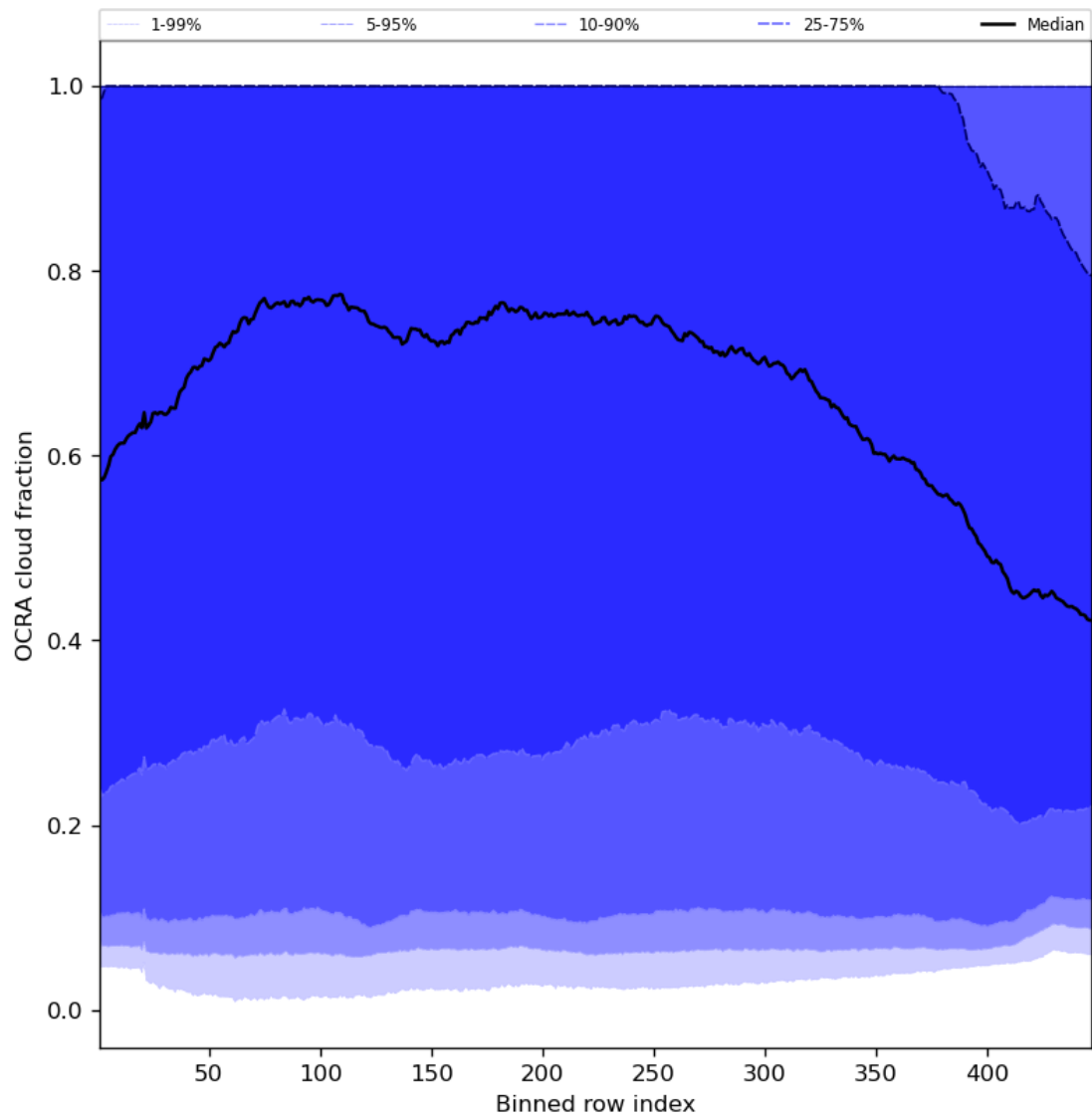
Figure 66: Along track statistics of “OCRA cloud fraction” for 2024-05-31 to 2024-06-02
