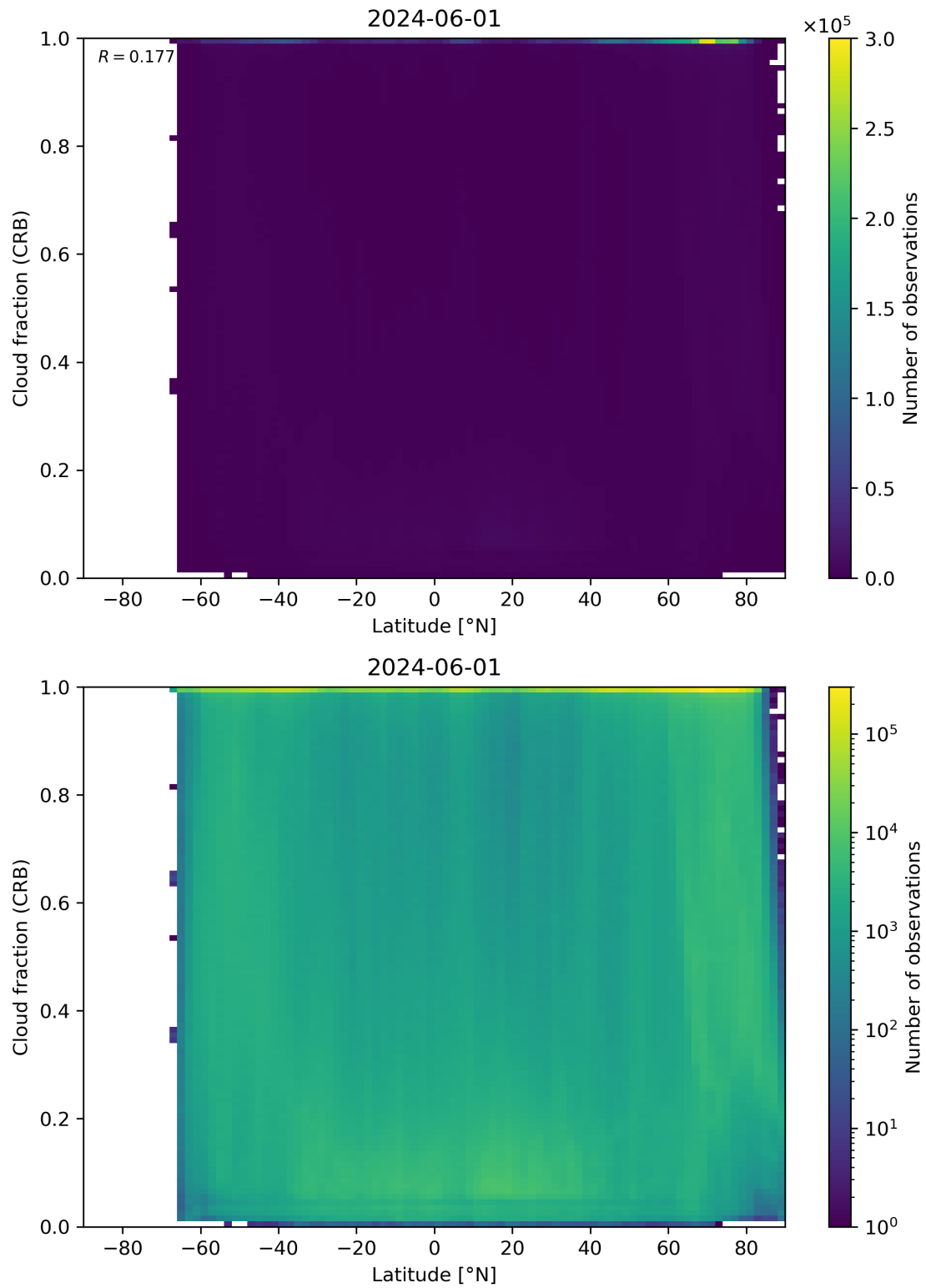
Figure 94: Scatter density plot of “Latitude” against “Cloud fraction (CRB)” for 2024-05-31 to 2024-06-02.
