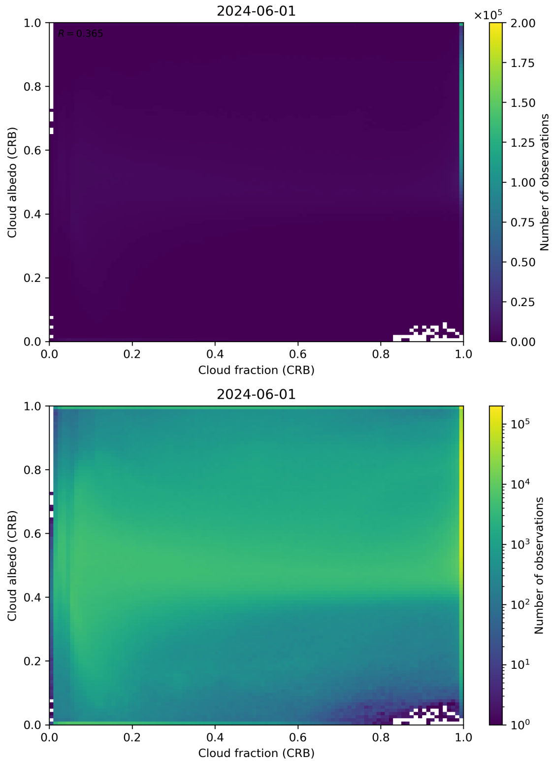
Figure 77: Scatter density plot of “Cloud fraction (CRB)” against “Cloud albedo (CRB)” for 2024-05-31 to 2024-06-02.
