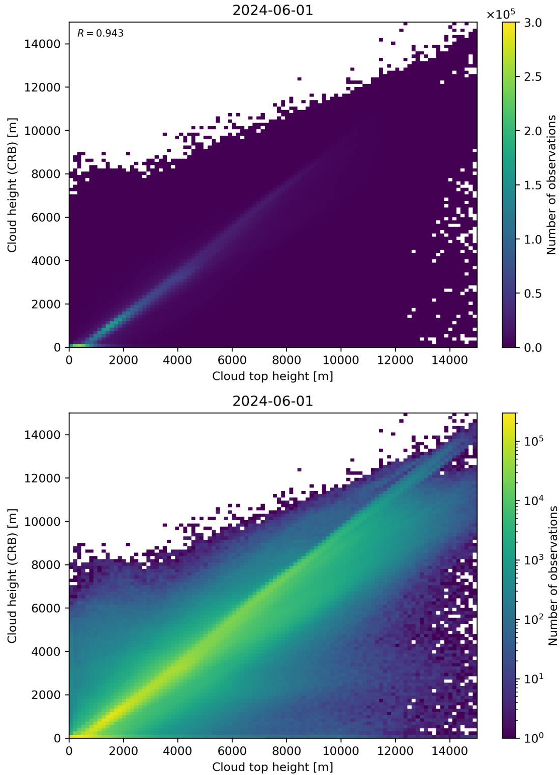
Figure 89: Scatter density plot of “Cloud top height” against “Cloud height (CRB)” for 2024-05-31 to 2024-06-02.
