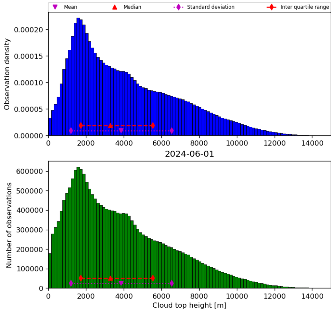
Figure 40: Histogram of “Cloud top height” for 2024-05-31 to 2024-06-02
