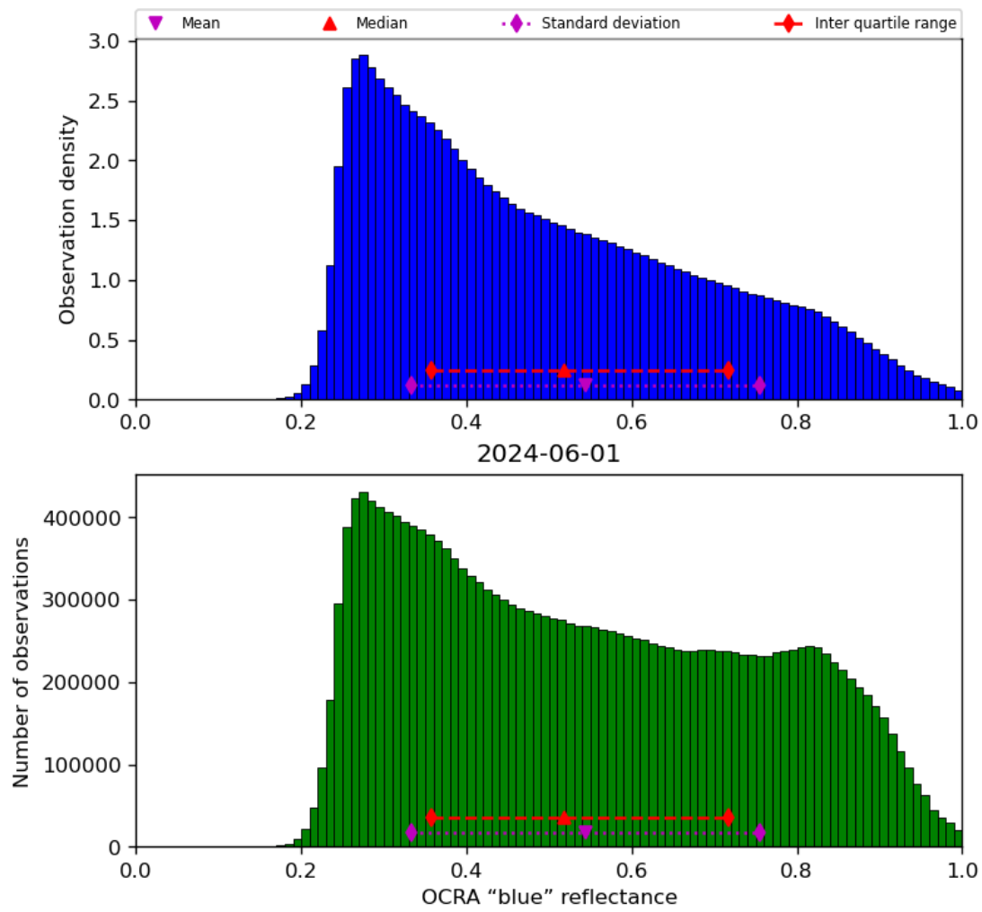
Figure 51: Histogram of “OCRA “blue” reflectance” for 2024-05-31 to 2024-06-02
