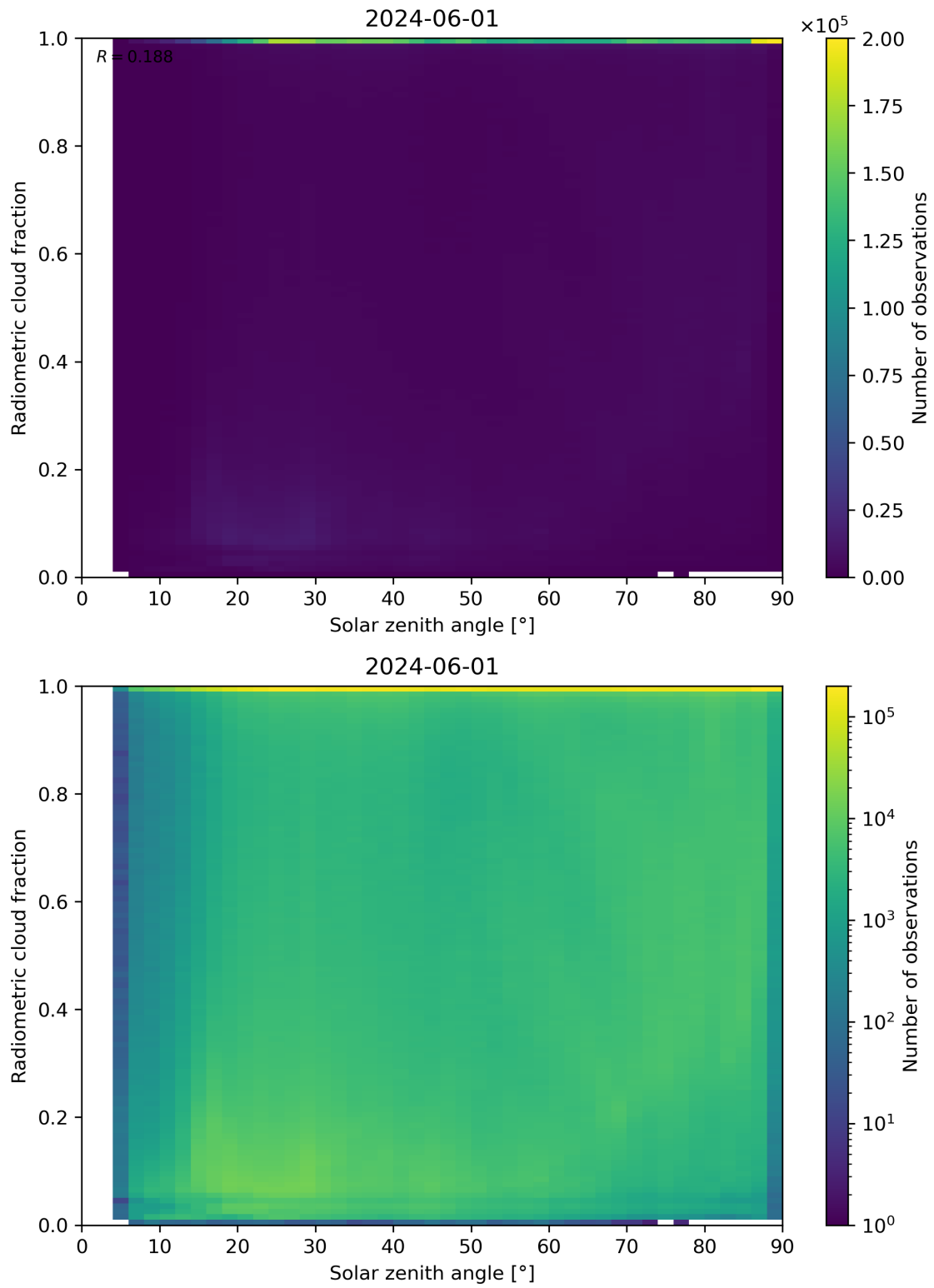
Figure 99: Scatter density plot of “Solar zenith angle” against “Radiometric cloud fraction” for 2024-05-31 to 2024-06-02.
