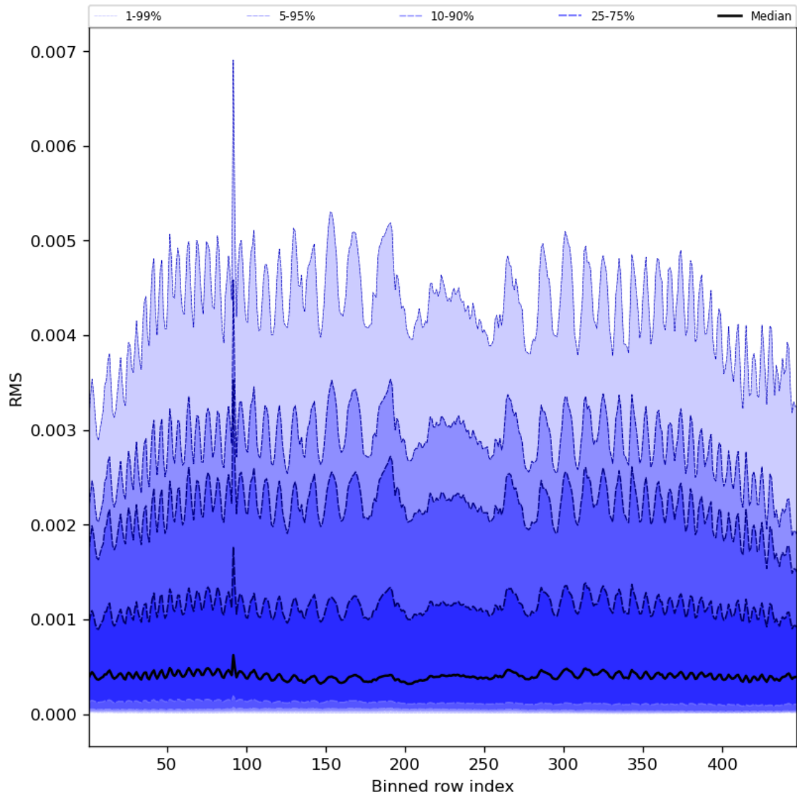
Figure 63: Along track statistics of “RMS” for 2024-05-31 to 2024-06-02
