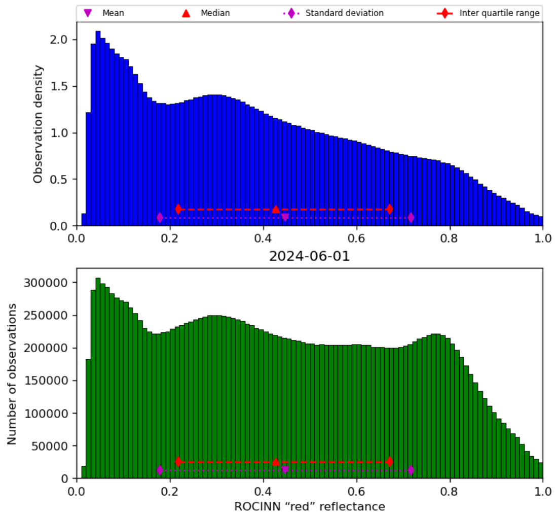
Figure 53: Histogram of “ROCINN “red” reflectance” for 2024-05-31 to 2024-06-02
