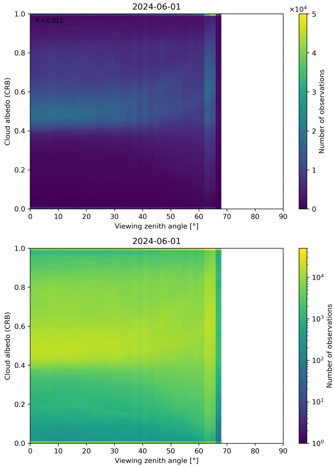
Figure 106: Scatter density plot of “Viewing zenith angle” against “Cloud albedo (CRB)” for 2024-05-31 to 2024-06-02.
