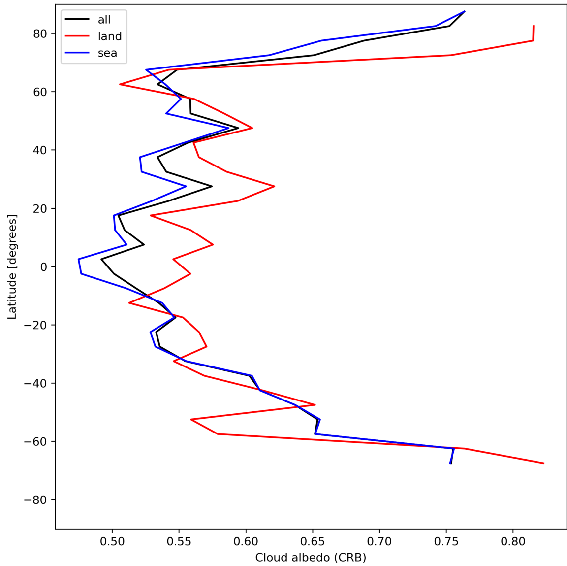
Figure 28: Zonal average of “Cloud albedo (CRB)” for 2024-05-31 to 2024-06-02.
