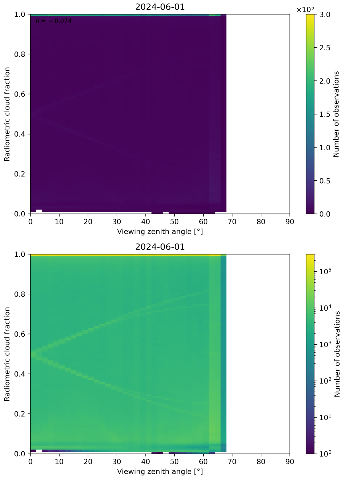
Figure 107: Scatter density plot of “Viewing zenith angle” against “Radiometric cloud fraction” for 2024-05-31 to 2024-06-02.
