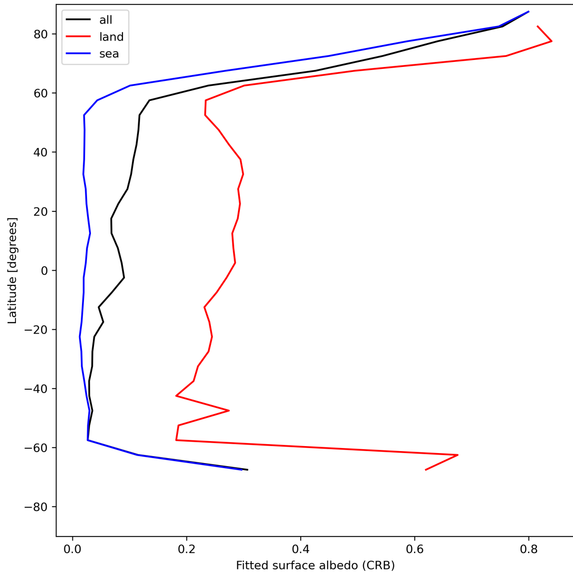
Figure 30: Zonal average of “Fitted surface albedo (CRB)” for 2024-05-31 to 2024-06-02.
