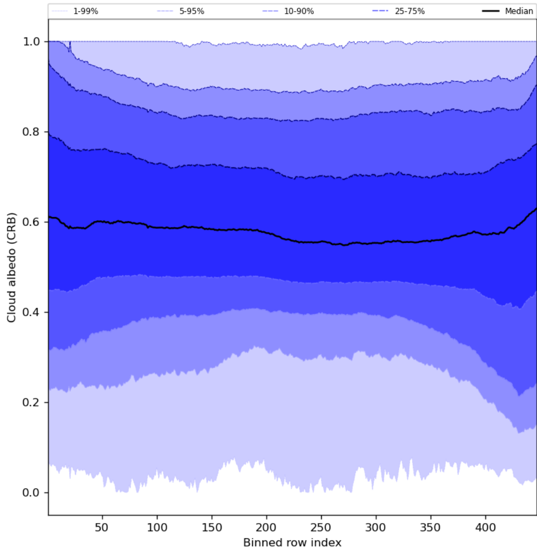
Figure 60: Along track statistics of “Cloud albedo (CRB)” for 2024-05-31 to 2024-06-02
