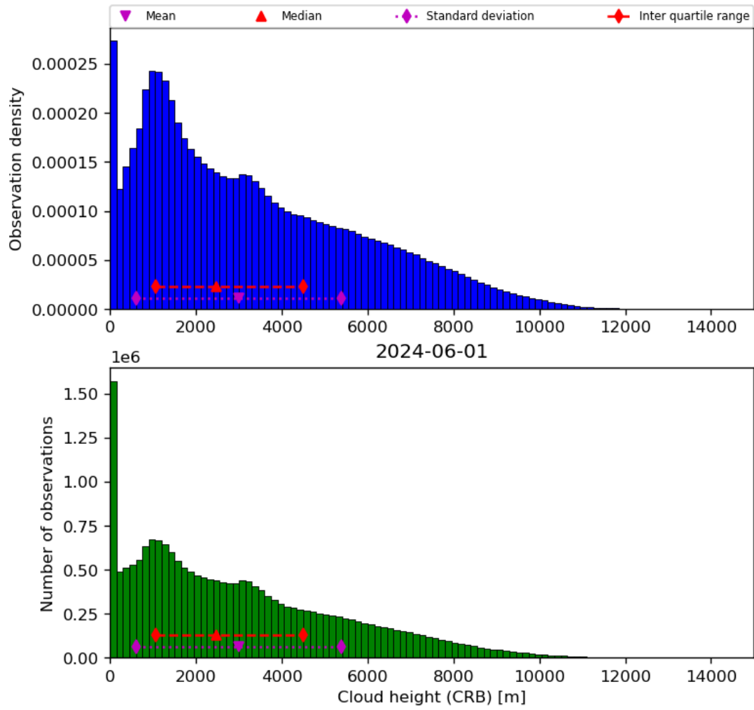
Figure 43: Histogram of “Cloud height (CRB)” for 2024-05-31 to 2024-06-02
