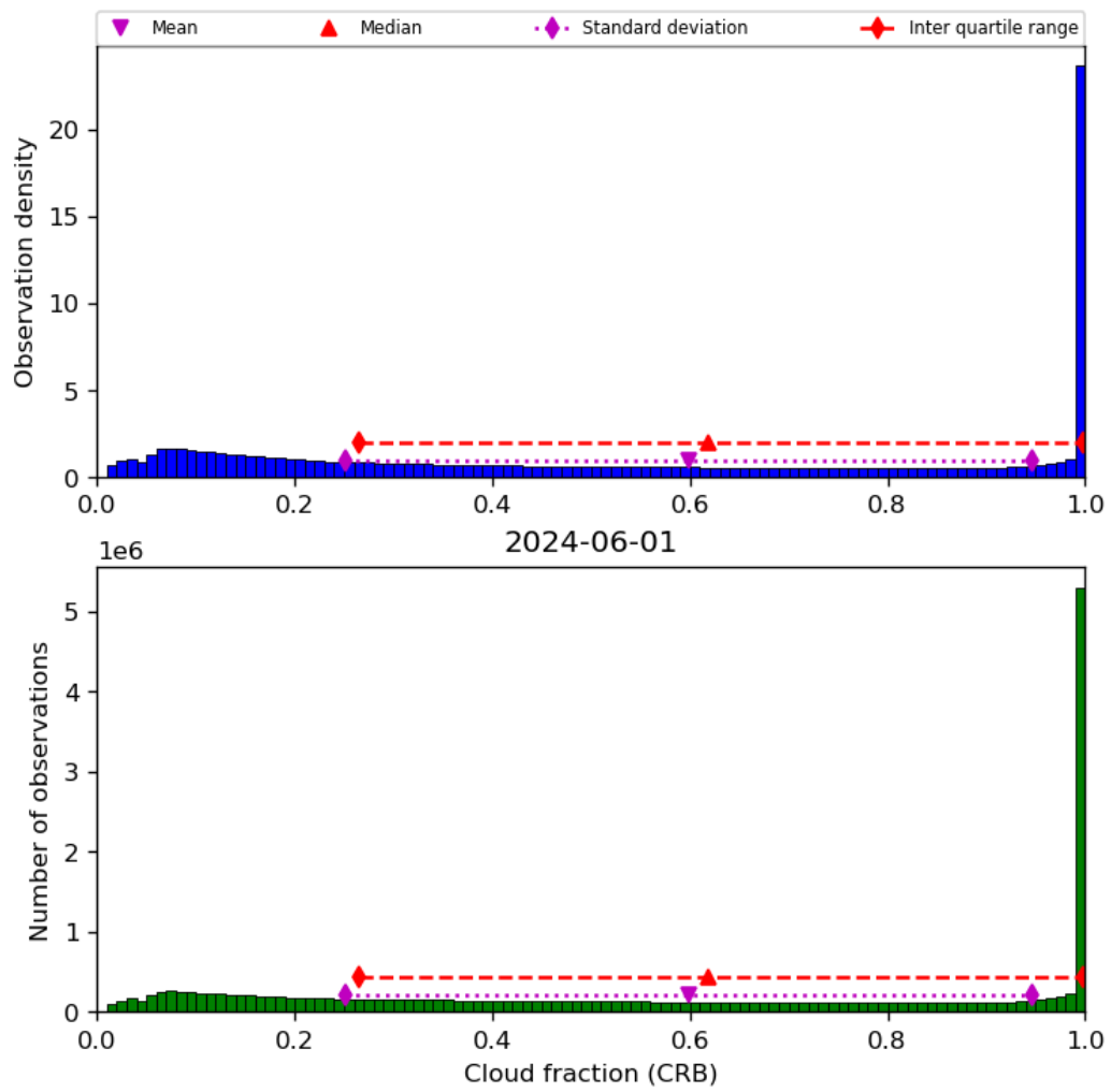
Figure 42: Histogram of “Cloud fraction (CRB)” for 2024-05-31 to 2024-06-02
