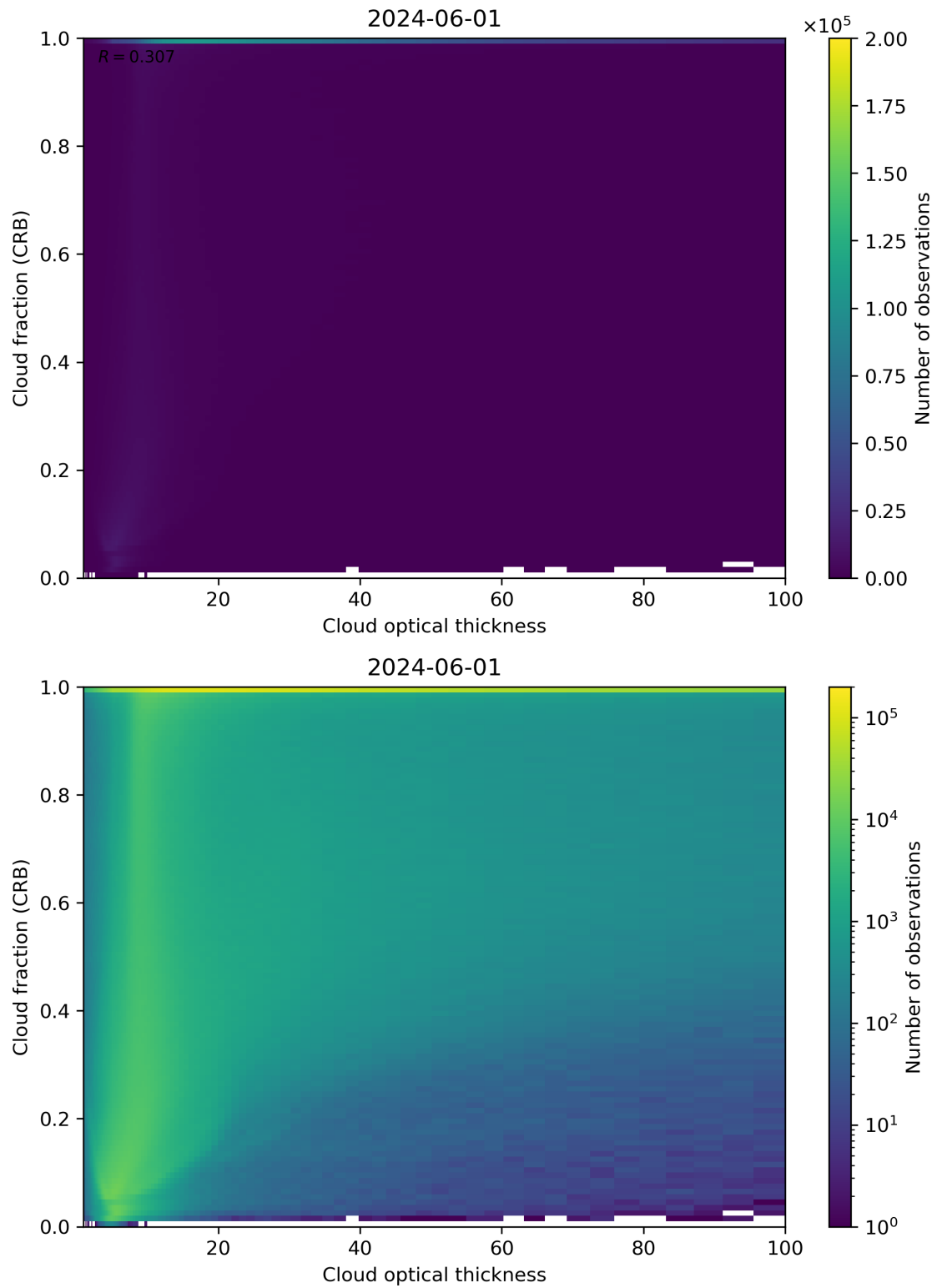
Figure 84: Scatter density plot of “Cloud optical thickness” against “Cloud fraction (CRB)” for 2024-05-31 to 2024-06-02.
