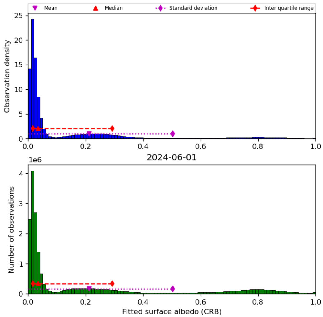
Figure 46: Histogram of “Fitted surface albedo (CRB)” for 2024-05-31 to 2024-06-02
