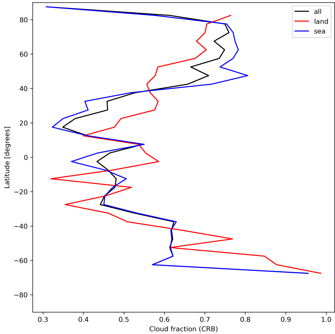
Figure 26: Zonal average of “Cloud fraction (CRB)” for 2024-05-31 to 2024-06-02.
