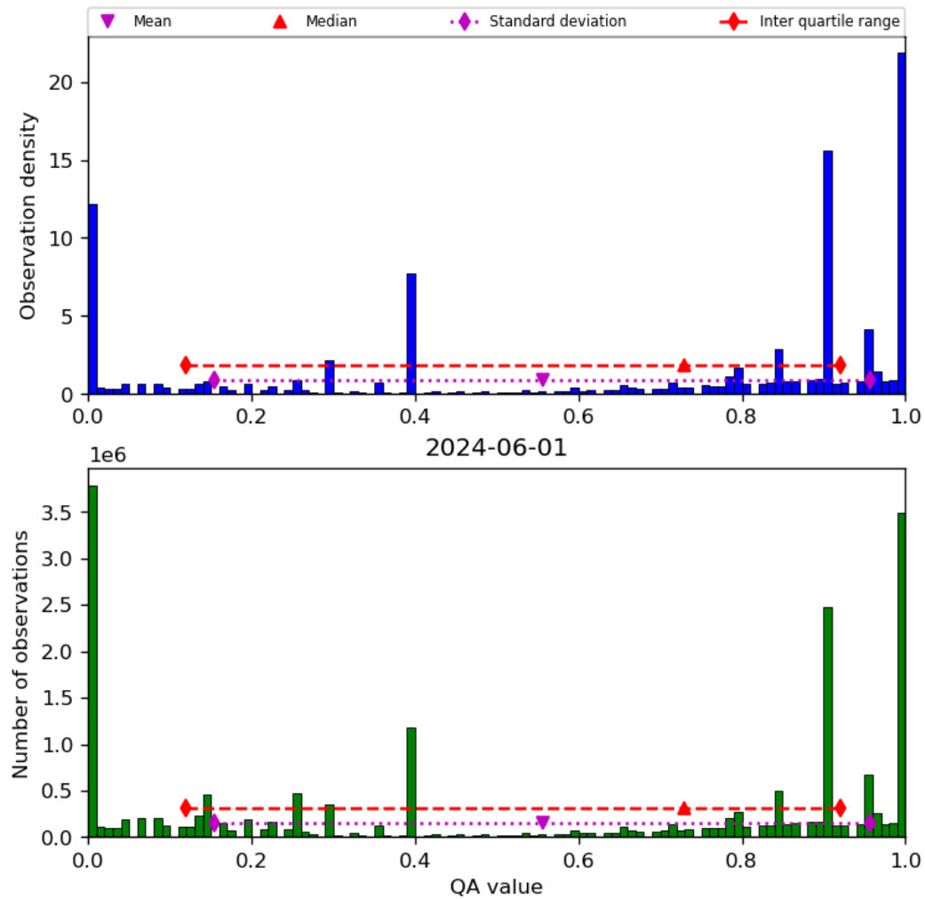
Figure 38: Histogram of “QA value” for 2024-05-31 to 2024-06-02
