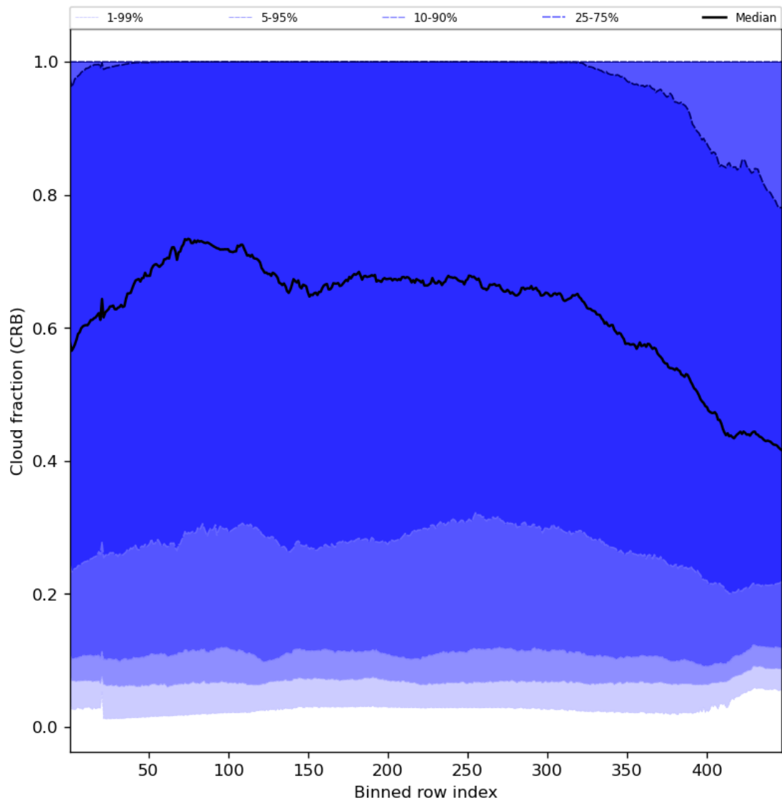
Figure 58: Along track statistics of “Cloud fraction (CRB)” for 2024-05-31 to 2024-06-02
