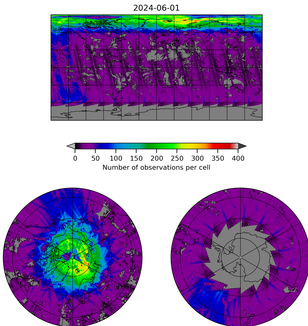
Figure 21: Map of the number of observations for 2024-05-31 to 2024-06-02
