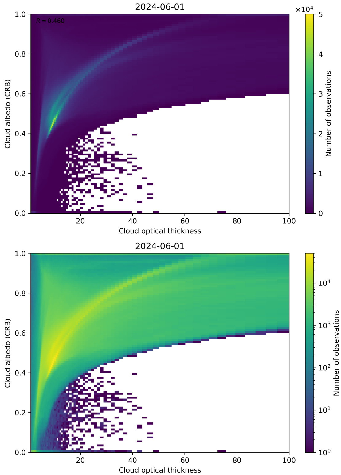
Figure 82: Scatter density plot of “Cloud optical thickness” against “Cloud albedo (CRB)” for 2024-05-31 to 2024-06-02.
