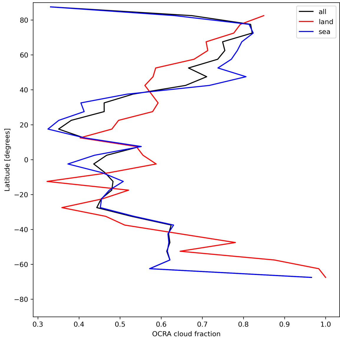
Figure 34: Zonal average of “OCRA cloud fraction” for 2024-05-31 to 2024-06-02.
