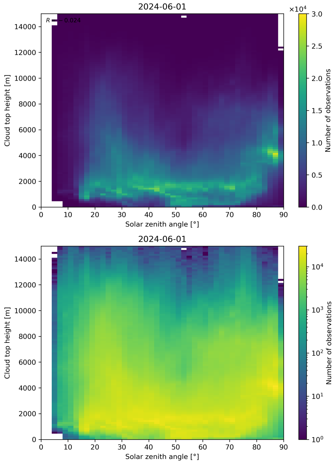
Figure 104: Scatter density plot of “Solar zenith angle” against “Cloud top height” for 2024-05-31 to 2024-06-02.
