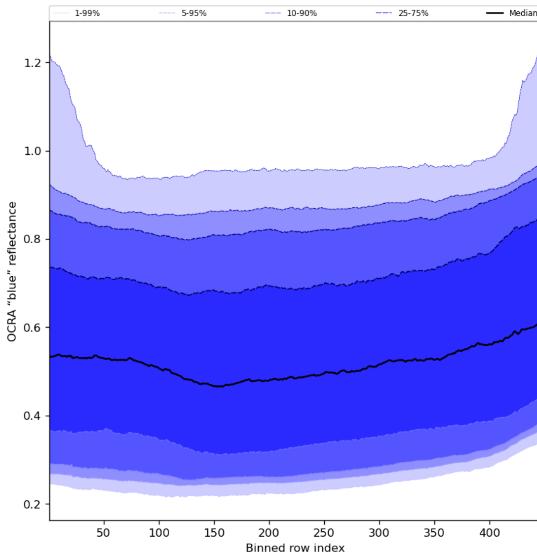
Figure 67: Along track statistics of "OCRA "blue" reflectance" for 2024-05-31 to 2024-06-02
