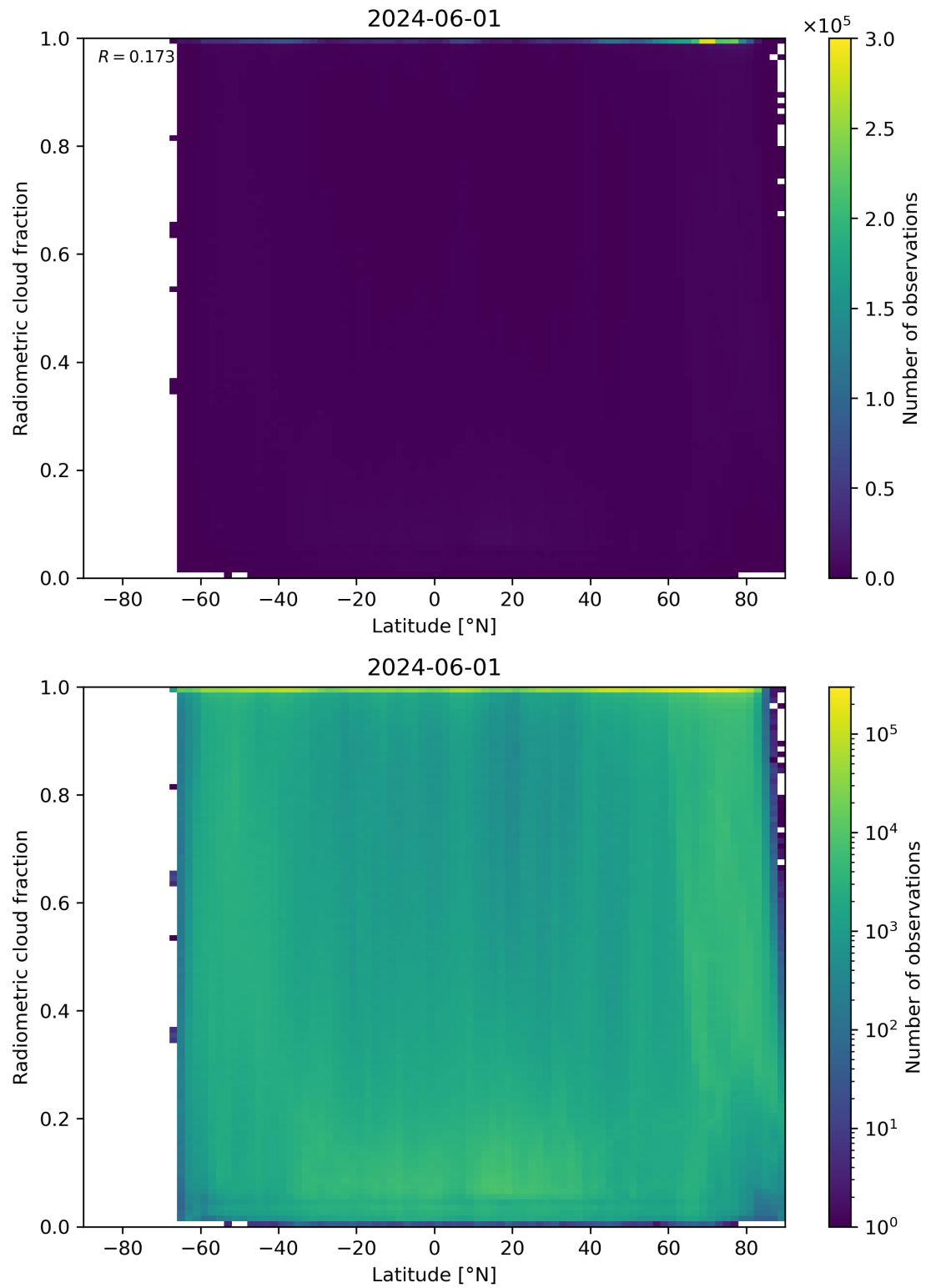
Figure 92: Scatter density plot of “Latitude” against “Radiometric cloud fraction” for 2024-05-31 to 2024-06-02.
