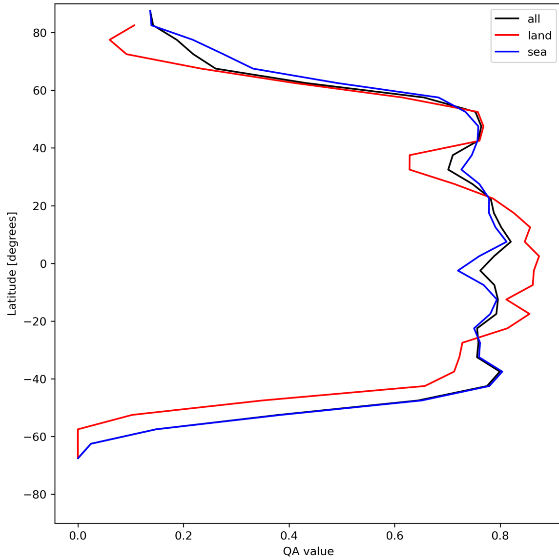
Figure 22: Zonal average of “QA value” for 2024-05-31 to 2024-06-02.
