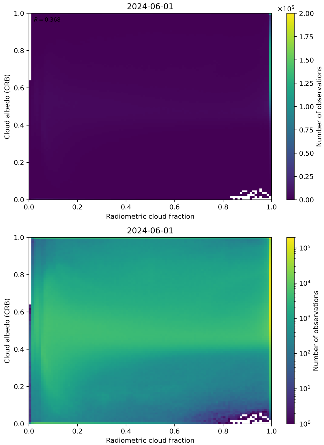
Figure 71: Scatter density plot of “Radiometric cloud fraction” against “Cloud albedo (CRB)” for 2024-05-31 to 2024-06-02.
