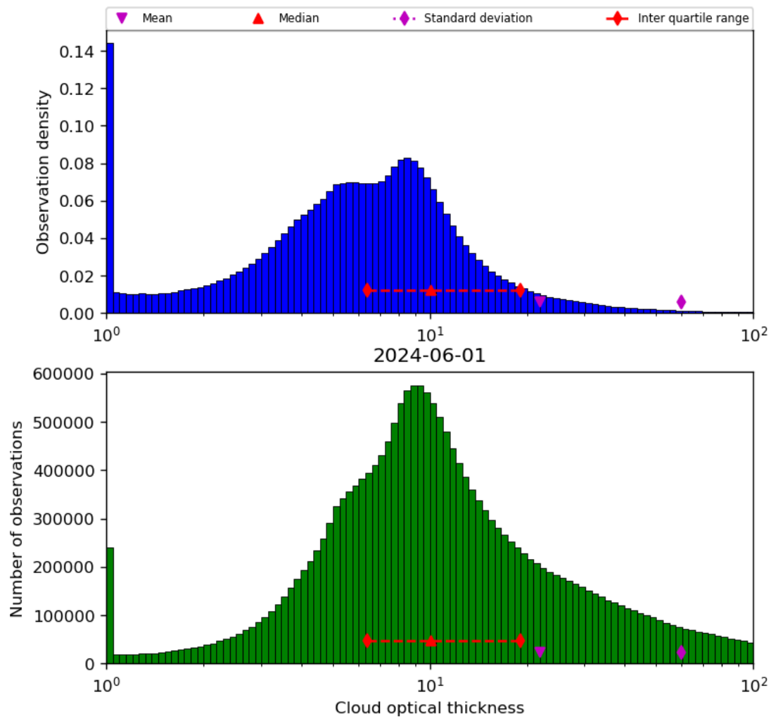
Figure 41: Histogram of “Cloud optical thickness” for 2024-05-31 to 2024-06-02
