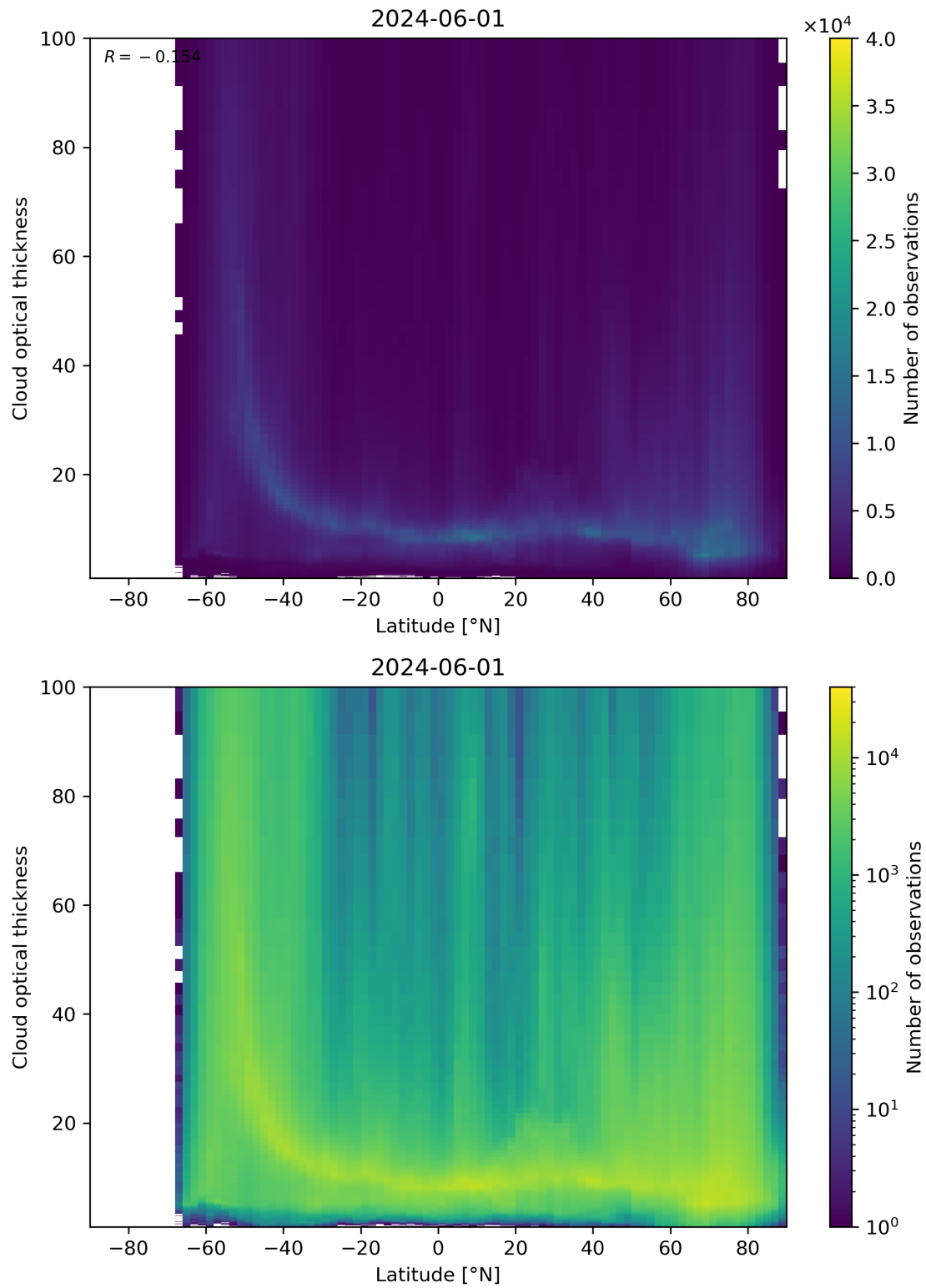
Figure 96: Scatter density plot of “Latitude” against “Cloud optical thickness” for 2024-05-31 to 2024-06-02.
