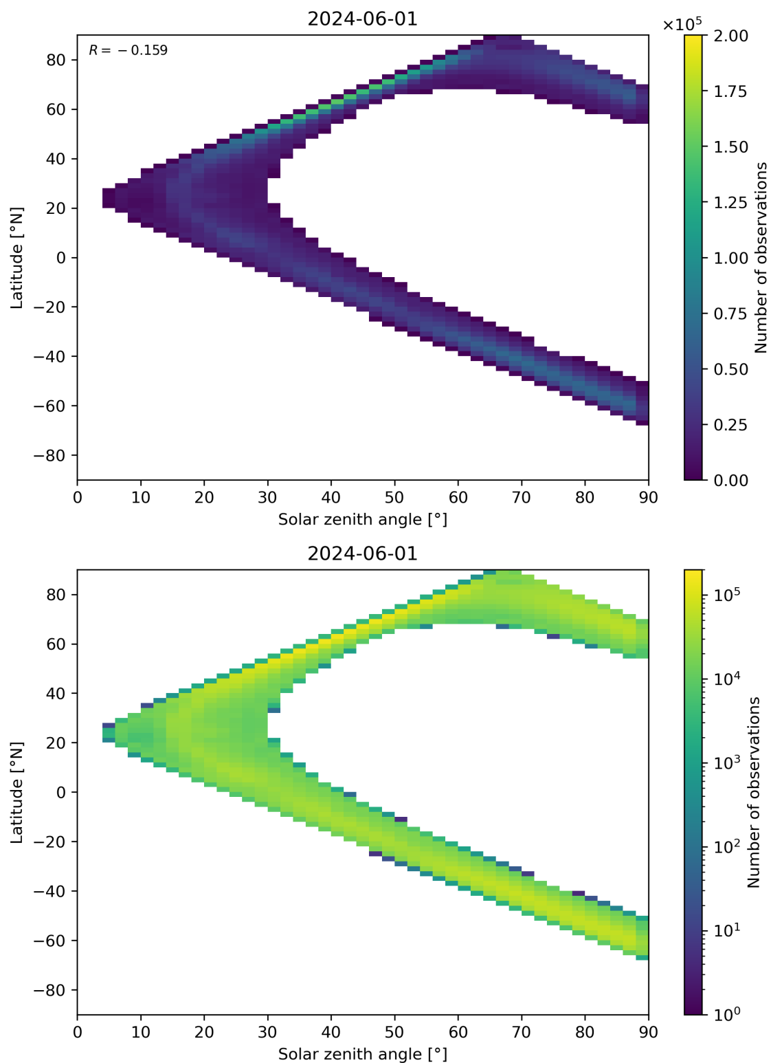
Figure 105: Scatter density plot of “Solar zenith angle” against “Latitude” for 2024-05-31 to 2024-06-02.
