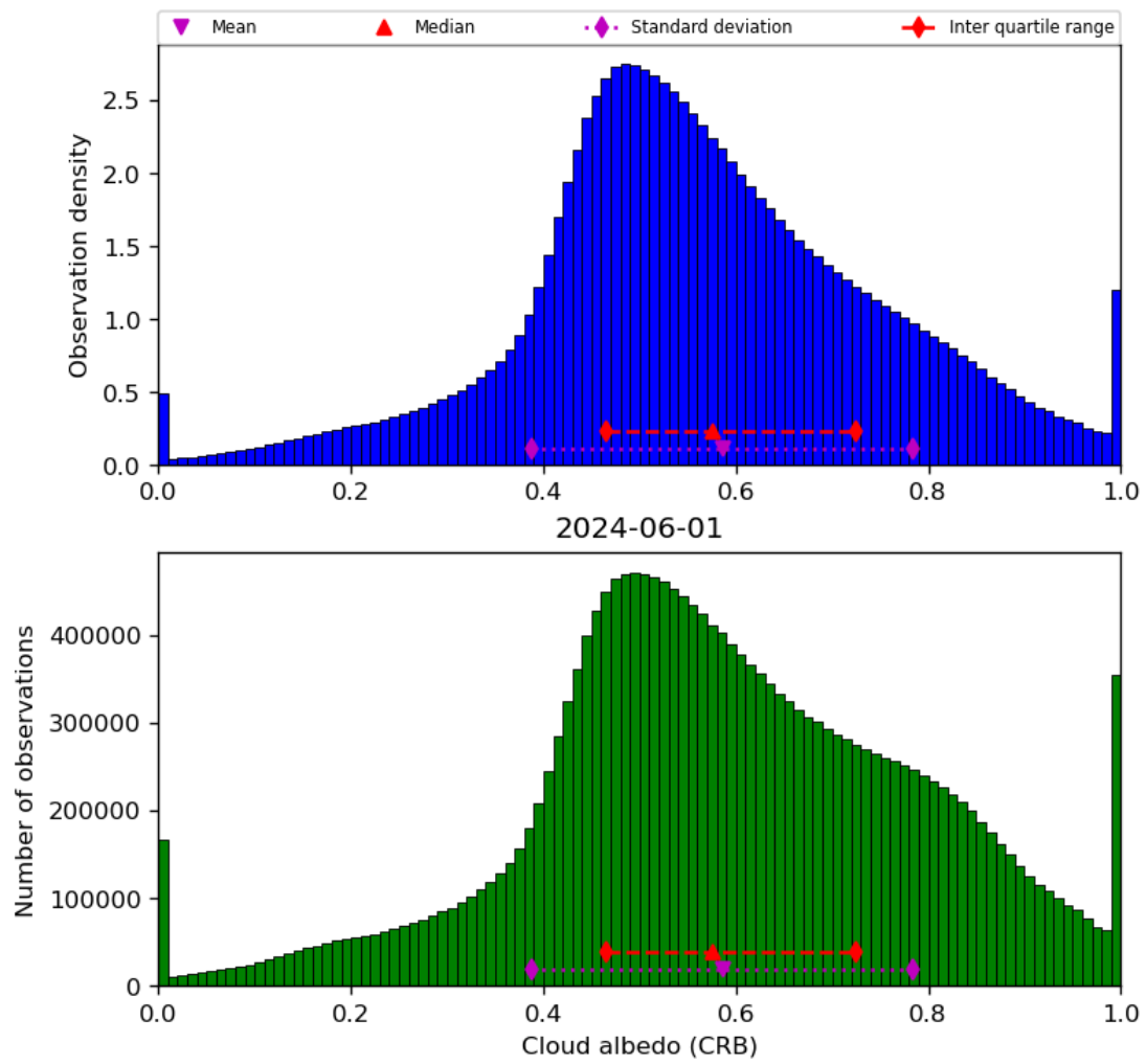
Figure 44: Histogram of “Cloud albedo (CRB)” for 2024-05-31 to 2024-06-02
