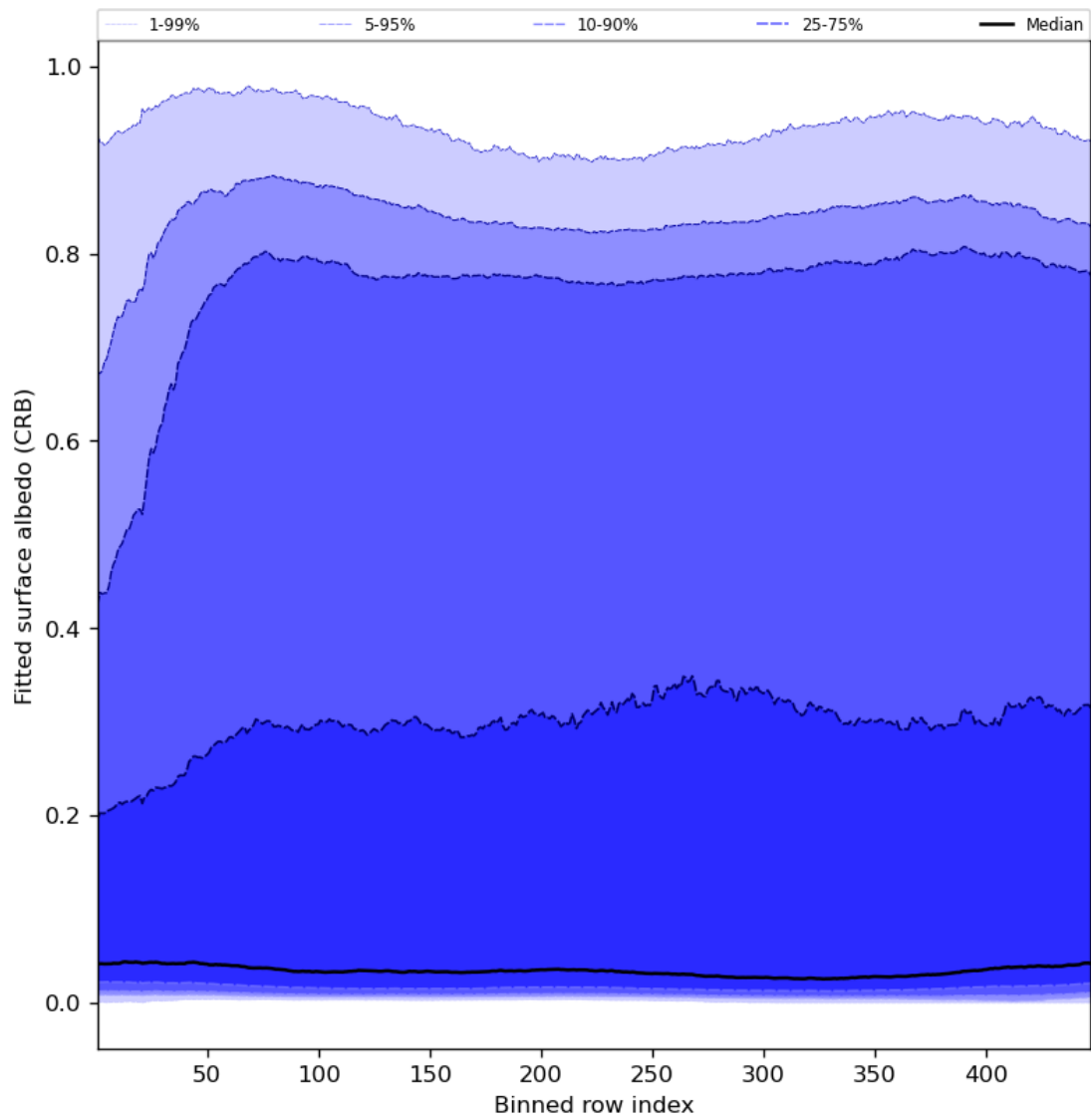
Figure 62: Along track statistics of “Fitted surface albedo (CRB)” for 2024-05-31 to 2024-06-02
