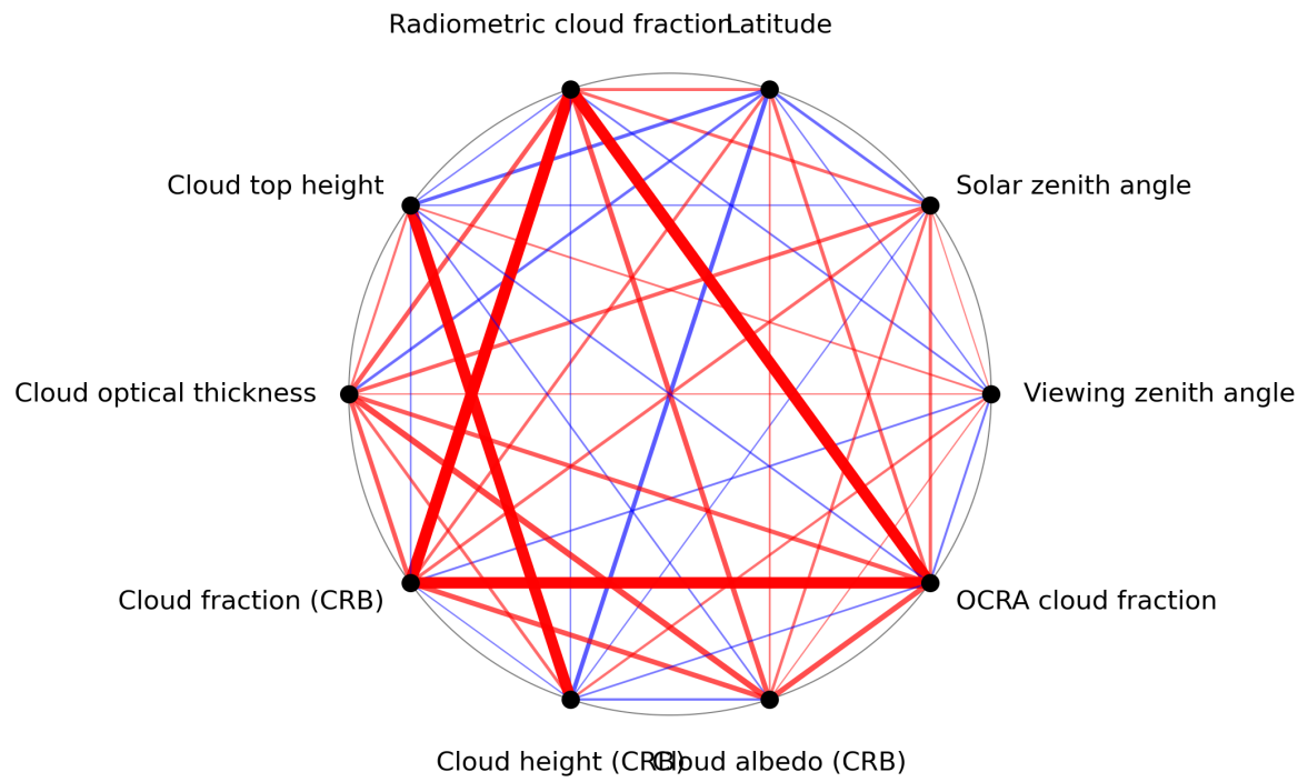
Figure 1: Map of correlation graph for 2024-05-31 to 2024-06-02.
