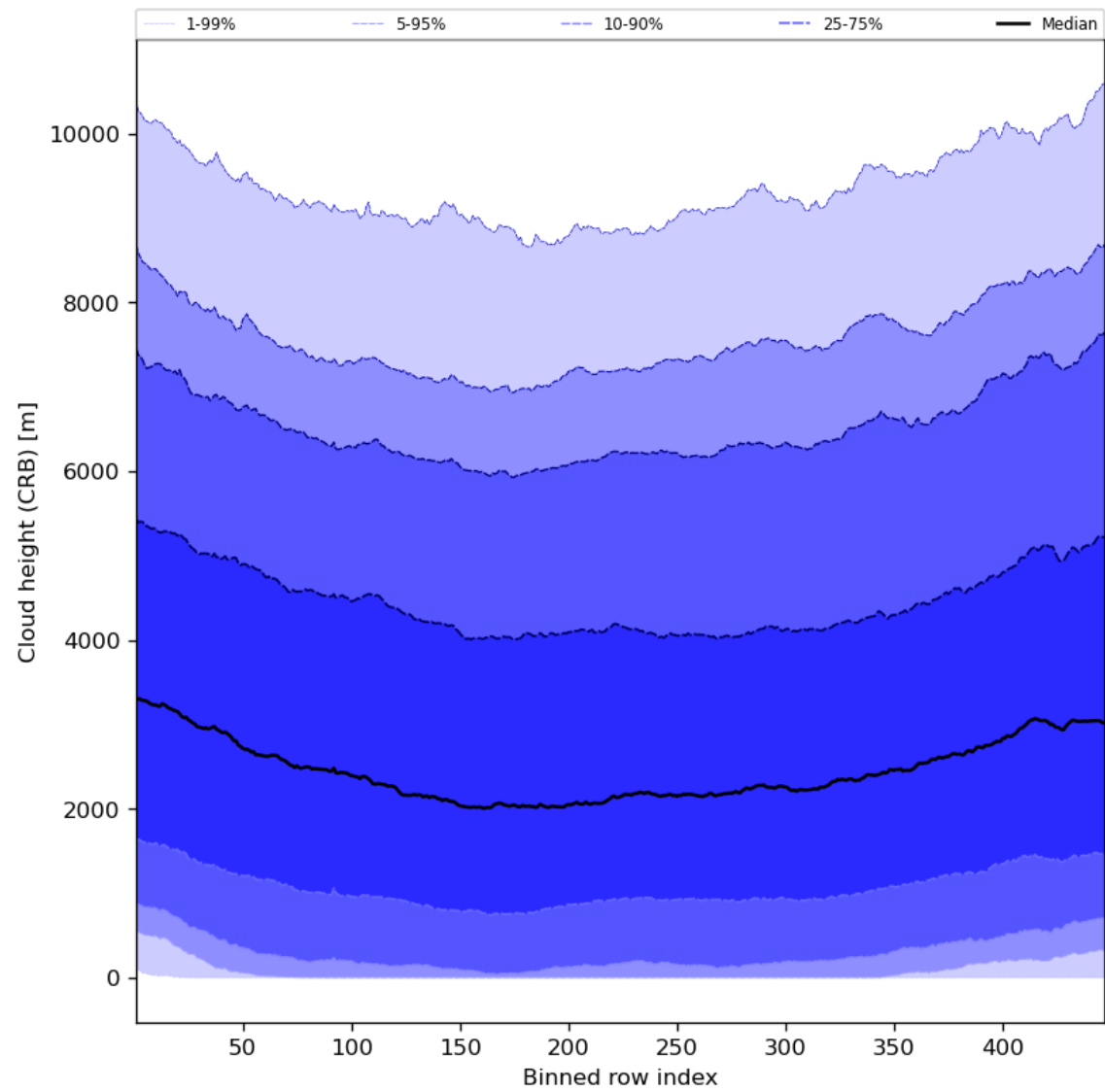
Figure 59: Along track statistics of “Cloud height (CRB)” for 2024-05-31 to 2024-06-02
