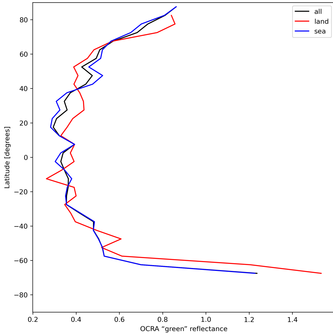
Figure 36: Zonal average of “OCRA “green” reflectance” for 2024-05-31 to 2024-06-02.
