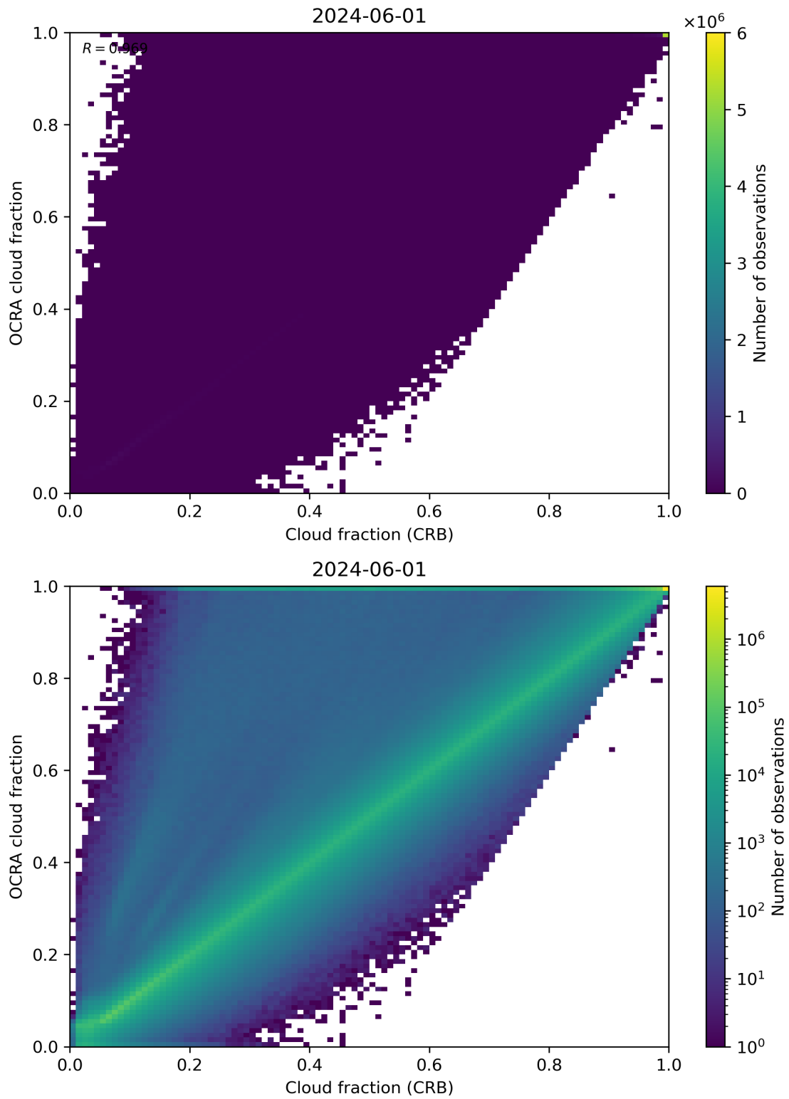
Figure 78: Scatter density plot of “Cloud fraction (CRB)” against “OCRA cloud fraction” for 2024-05-31 to 2024-06-02.
