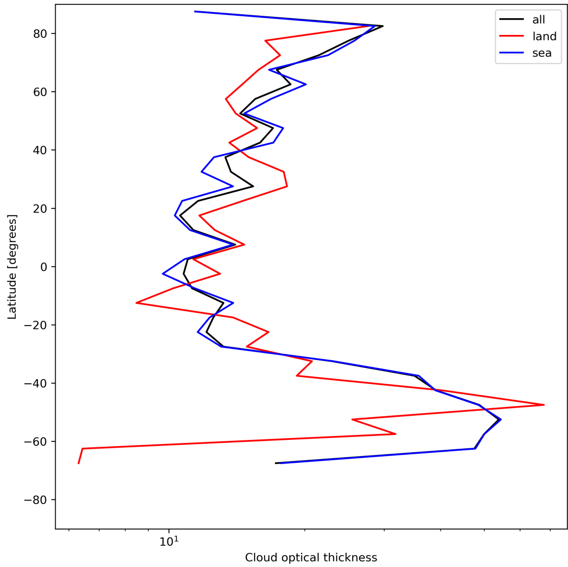
Figure 25: Zonal average of “Cloud optical thickness” for 2024-05-31 to 2024-06-02.
