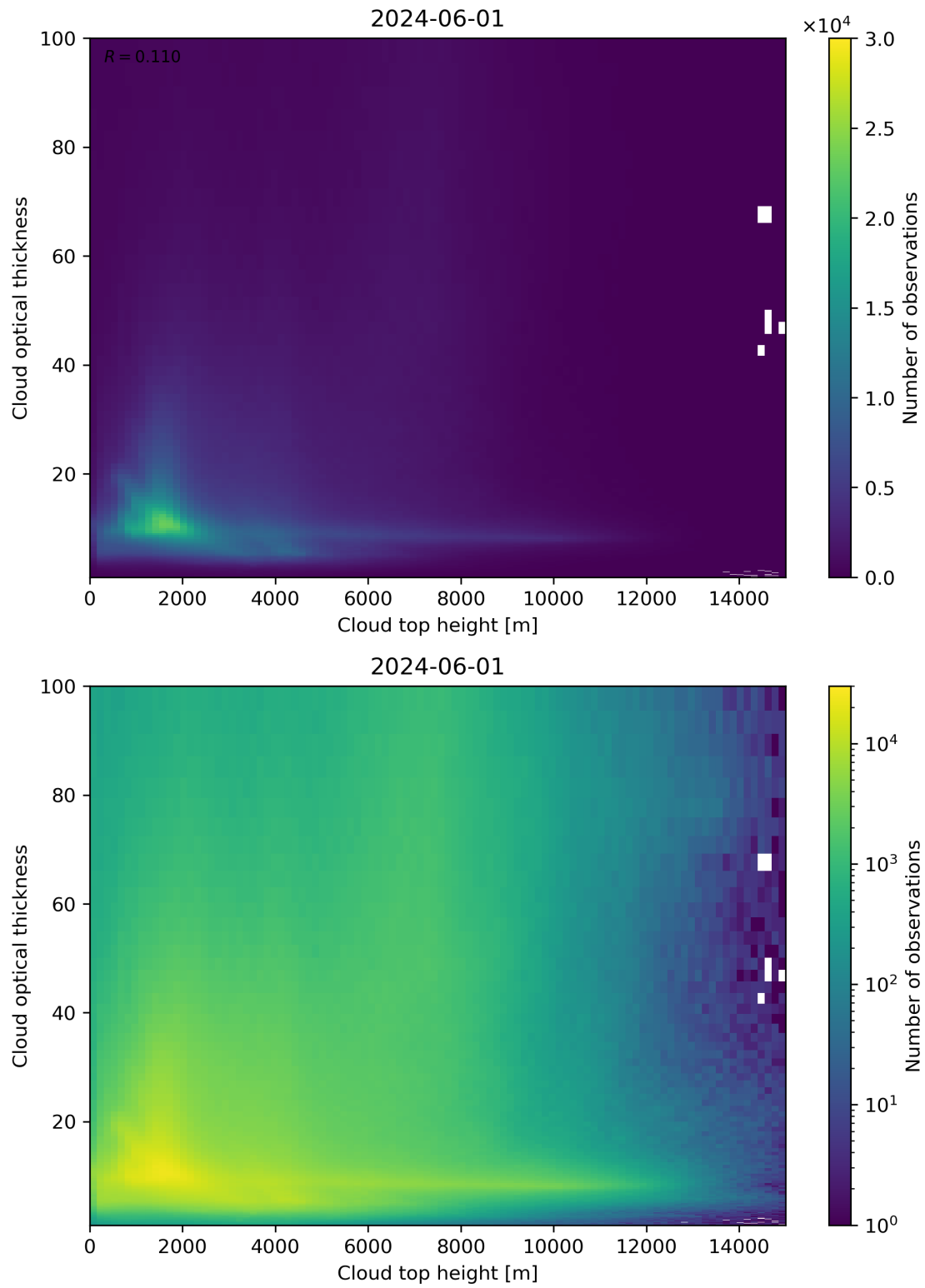
Figure 90: Scatter density plot of “Cloud top height” against “Cloud optical thickness” for 2024-05-31 to 2024-06-02.
