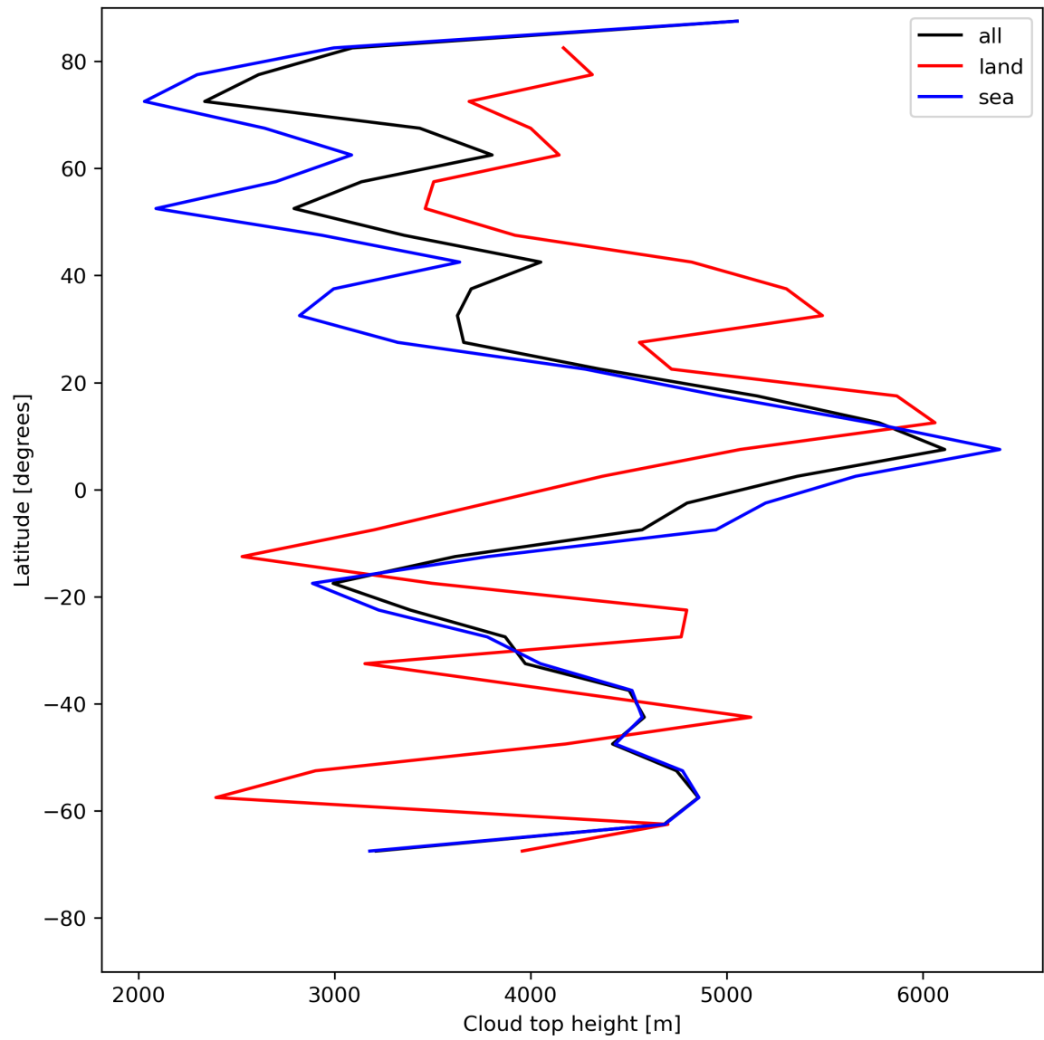
Figure 24: Zonal average of “Cloud top height” for 2024-05-31 to 2024-06-02.
