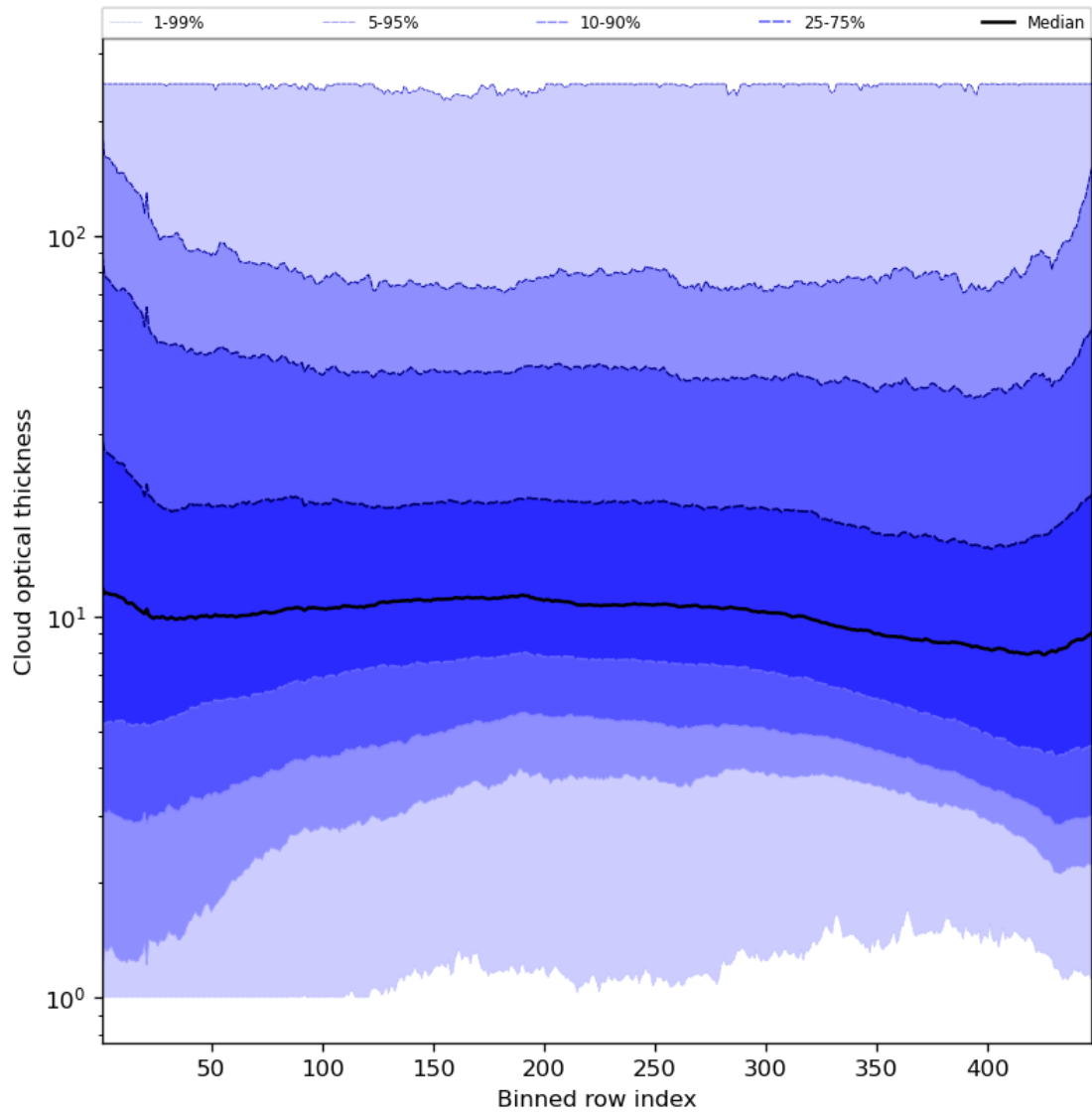
Figure 57: Along track statistics of “Cloud optical thickness” for 2024-05-31 to 2024-06-02
