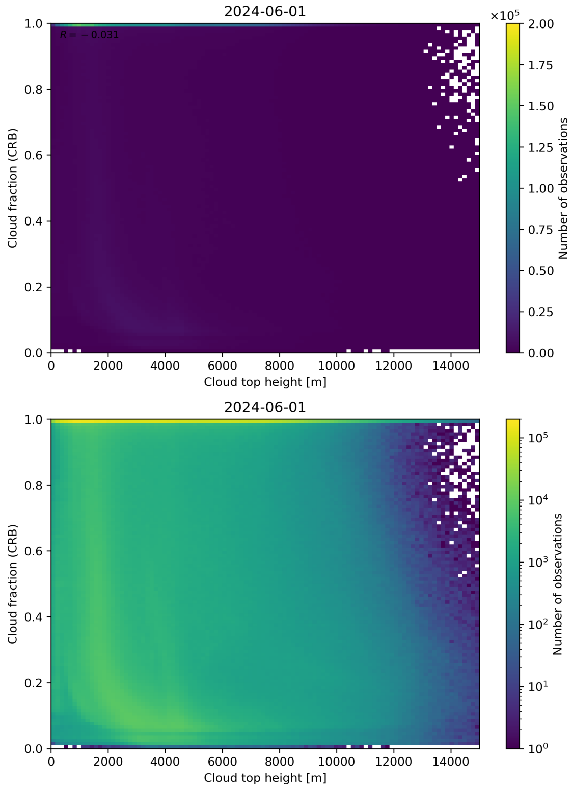
Figure 88: Scatter density plot of “Cloud top height” against “Cloud fraction (CRB)” for 2024-05-31 to 2024-06-02.
