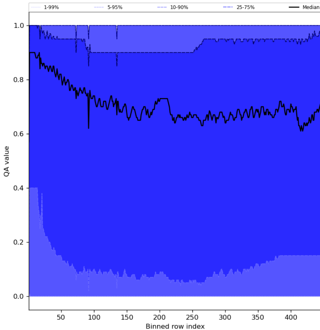
Figure 54: Along track statistics of “QA value” for 2024-05-31 to 2024-06-02
