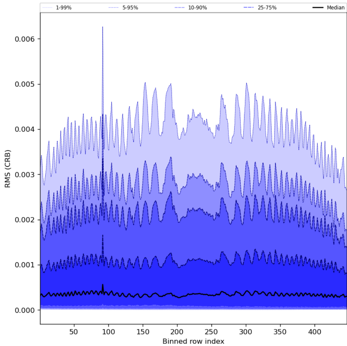
Figure 64: Along track statistics of “RMS (CRB)” for 2024-05-31 to 2024-06-02
