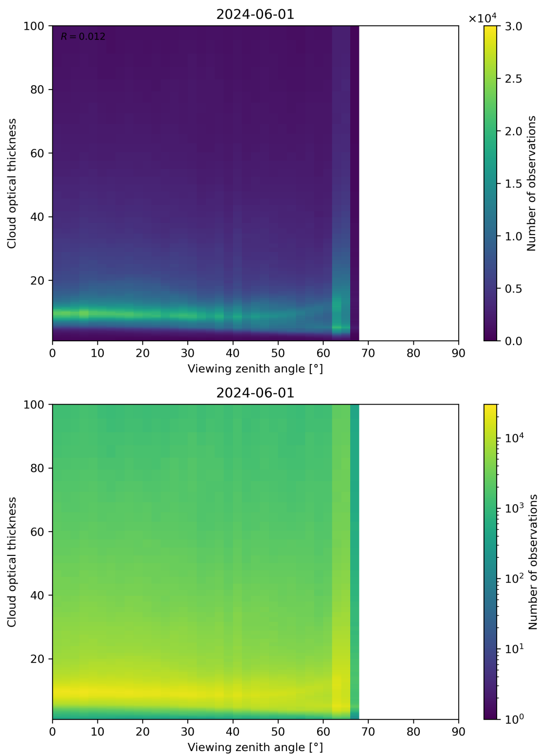
Figure 111: Scatter density plot of “Viewing zenith angle” against “Cloud optical thickness” for 2024-05-31 to 2024-06-02.
