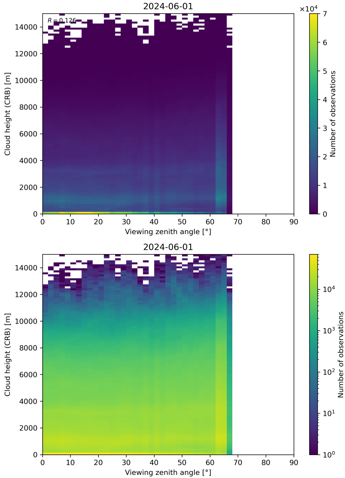
Figure 110: Scatter density plot of “Viewing zenith angle” against “Cloud height (CRB)” for 2024-05-31 to 2024-06-02.
