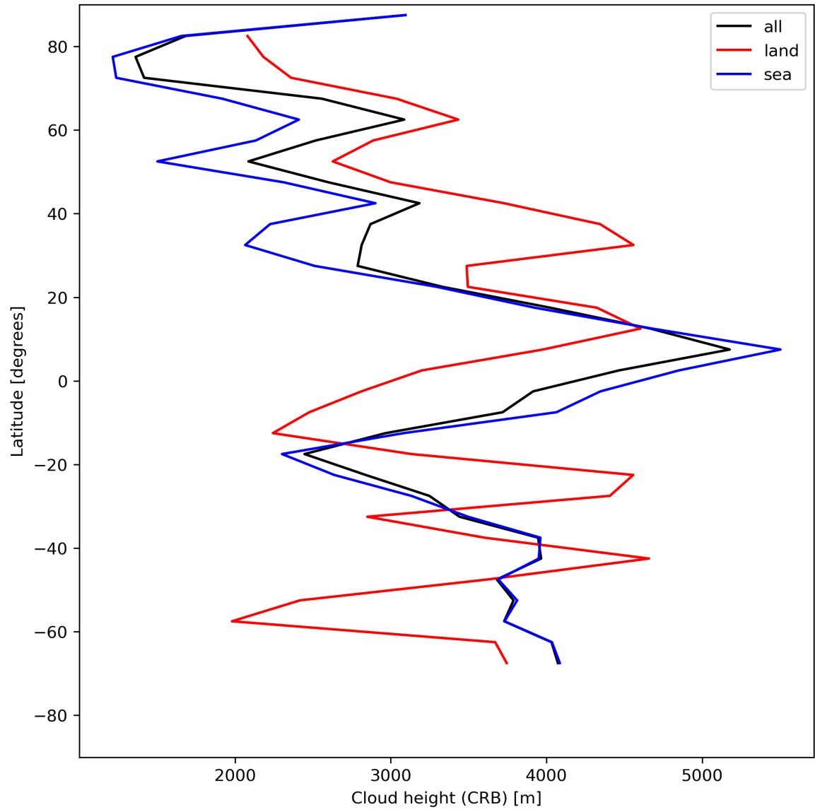
Figure 27: Zonal average of “Cloud height (CRB)” for 2024-05-31 to 2024-06-02.
