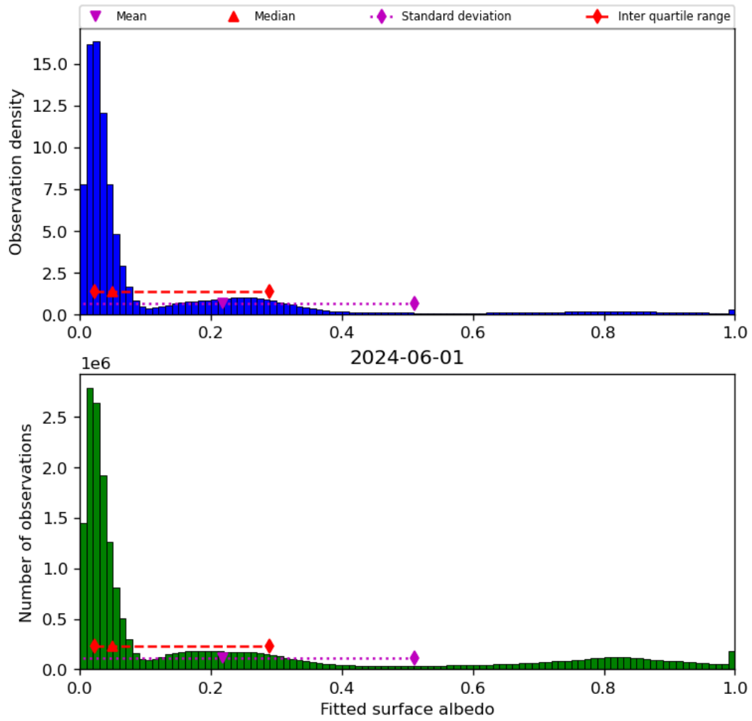
Figure 45: Histogram of “Fitted surface albedo” for 2024-05-31 to 2024-06-02
