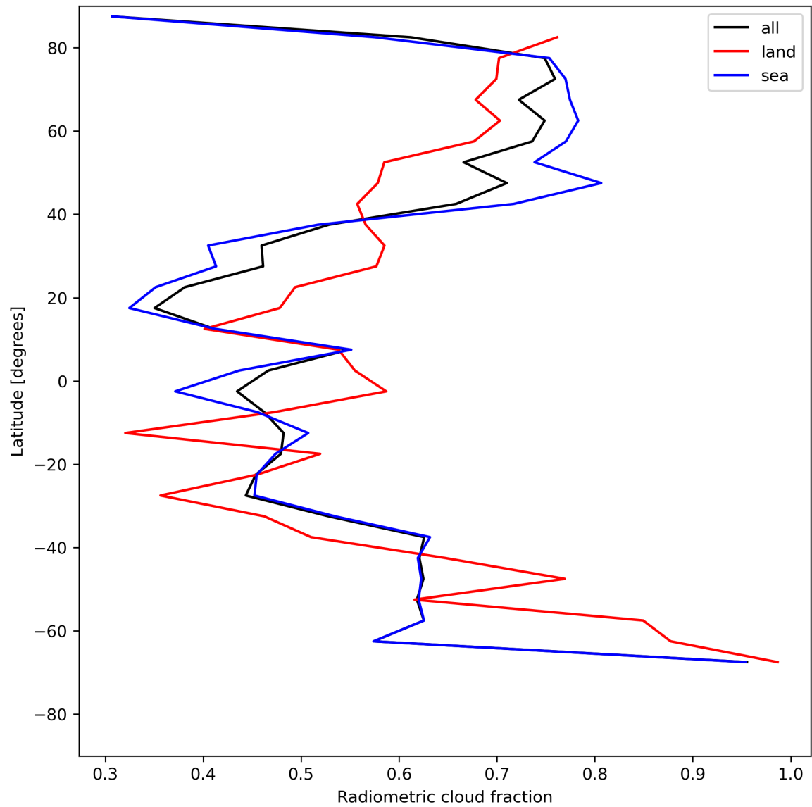
Figure 23: Zonal average of “Radiometric cloud fraction” for 2024-05-31 to 2024-06-02.
