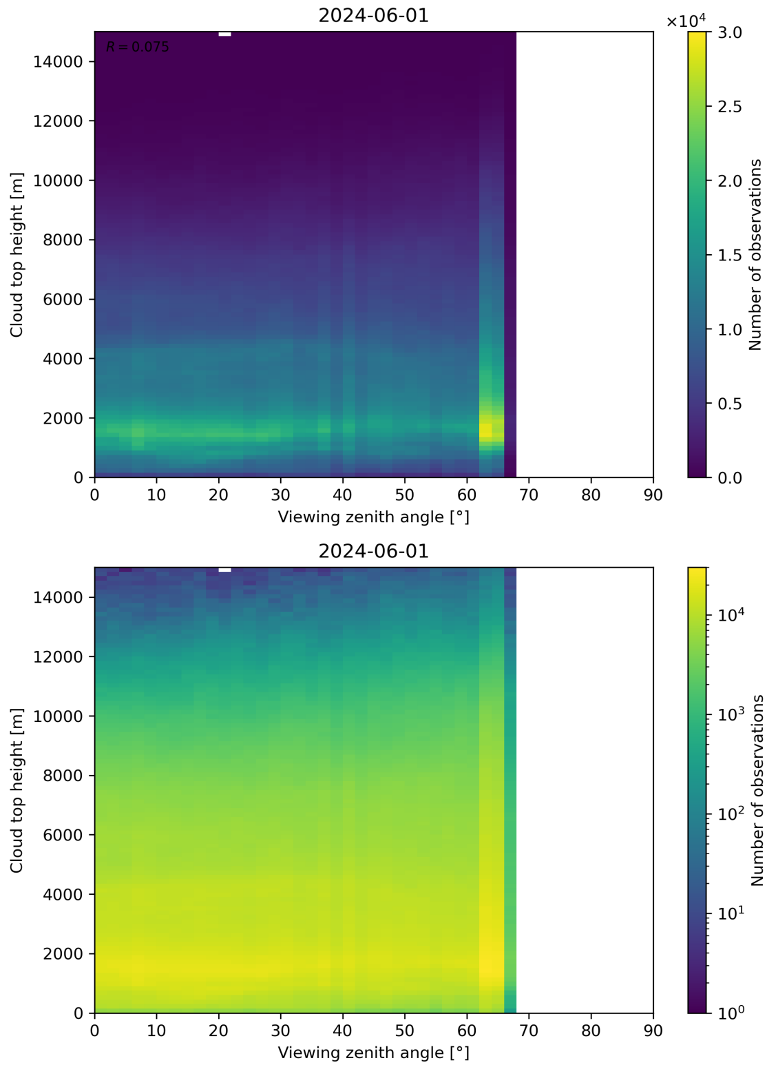
Figure 112: Scatter density plot of “Viewing zenith angle” against “Cloud top height” for 2024-05-31 to 2024-06-02.
