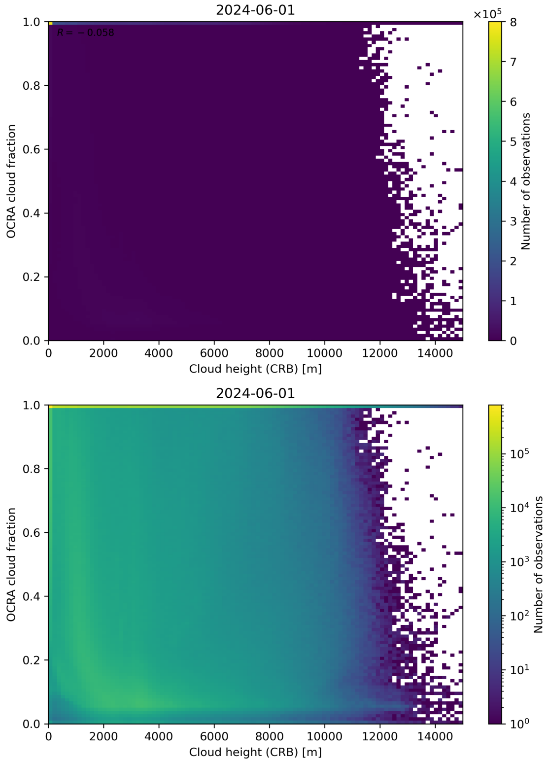
Figure 81: Scatter density plot of “Cloud height (CRB)” against “OCRA cloud fraction” for 2024-05-31 to 2024-06-02.
