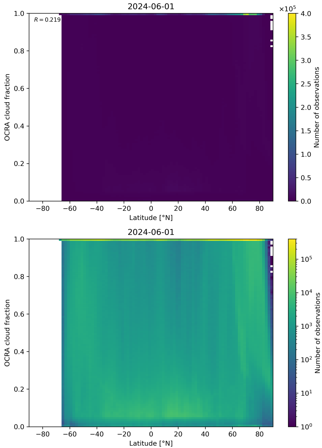
Figure 93: Scatter density plot of “Latitude” against “OCRA cloud fraction” for 2024-05-31 to 2024-06-02.
