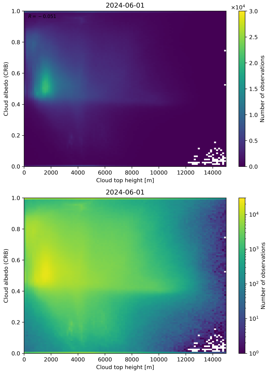
Figure 86: Scatter density plot of “Cloud top height” against “Cloud albedo (CRB)” for 2024-05-31 to 2024-06-02.
