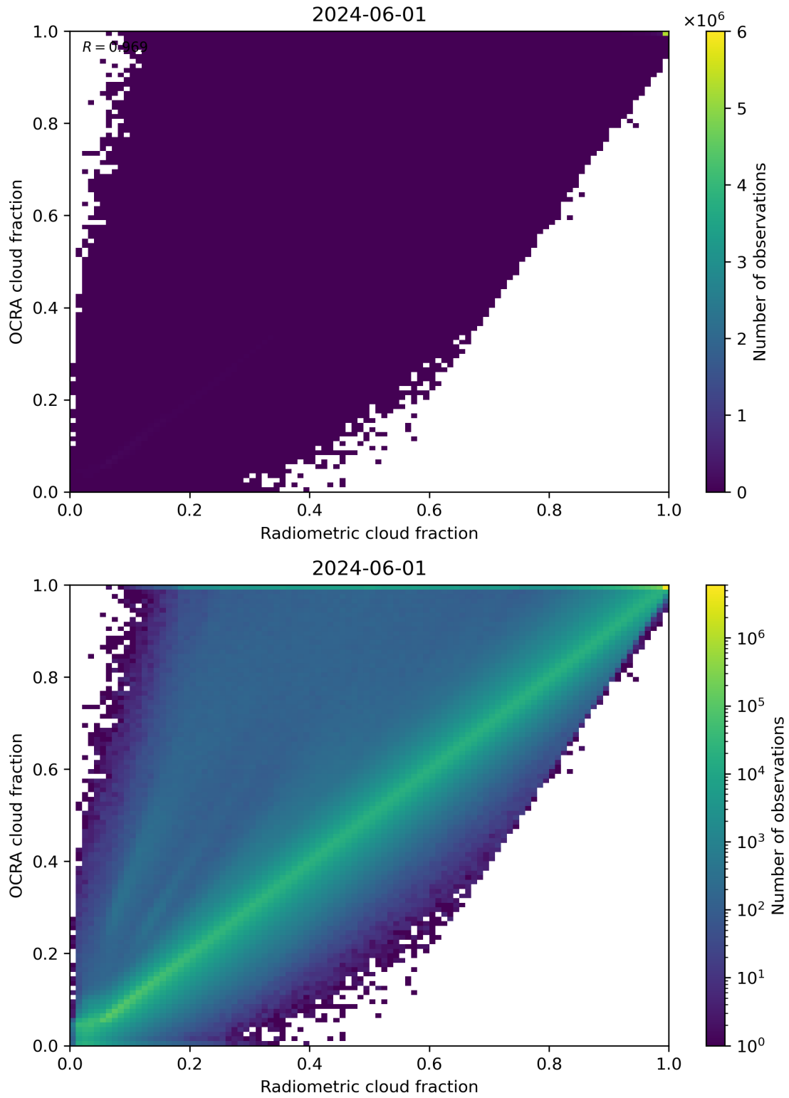
Figure 72: Scatter density plot of “Radiometric cloud fraction” against “OCRA cloud fraction” for 2024-05-31 to 2024-06-02.
