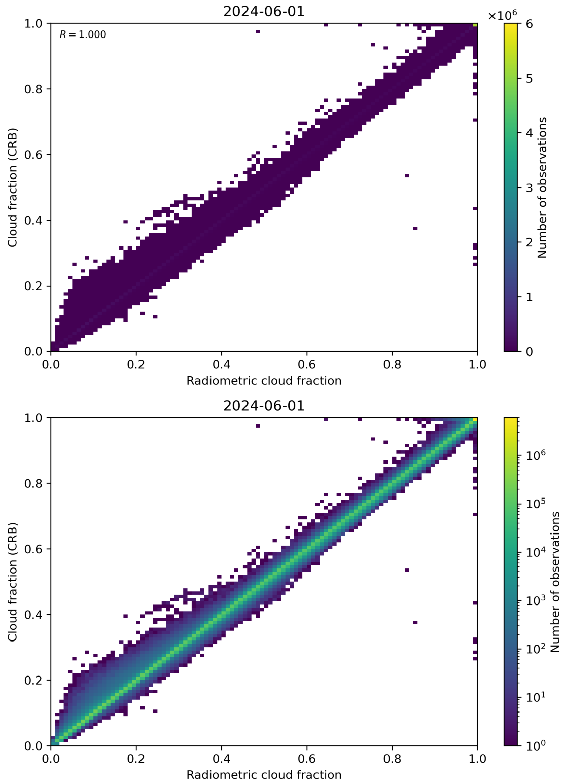
Figure 73: Scatter density plot of “Radiometric cloud fraction” against “Cloud fraction (CRB)” for 2024-05-31 to 2024-06-02.
