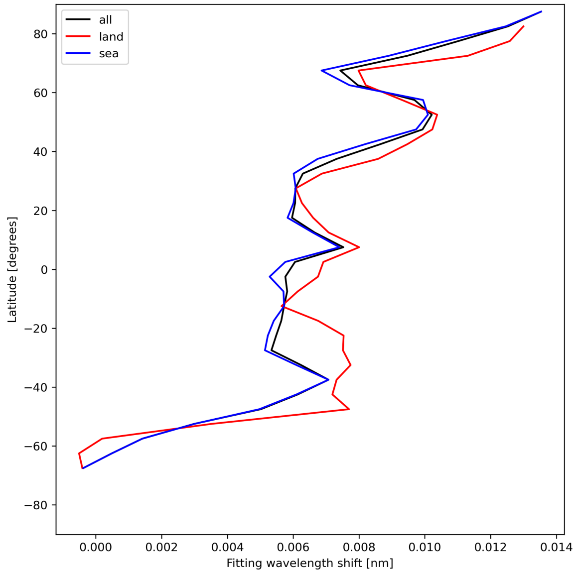
Figure 33: Zonal average of “Fitting wavelength shift” for 2024-05-31 to 2024-06-02.
