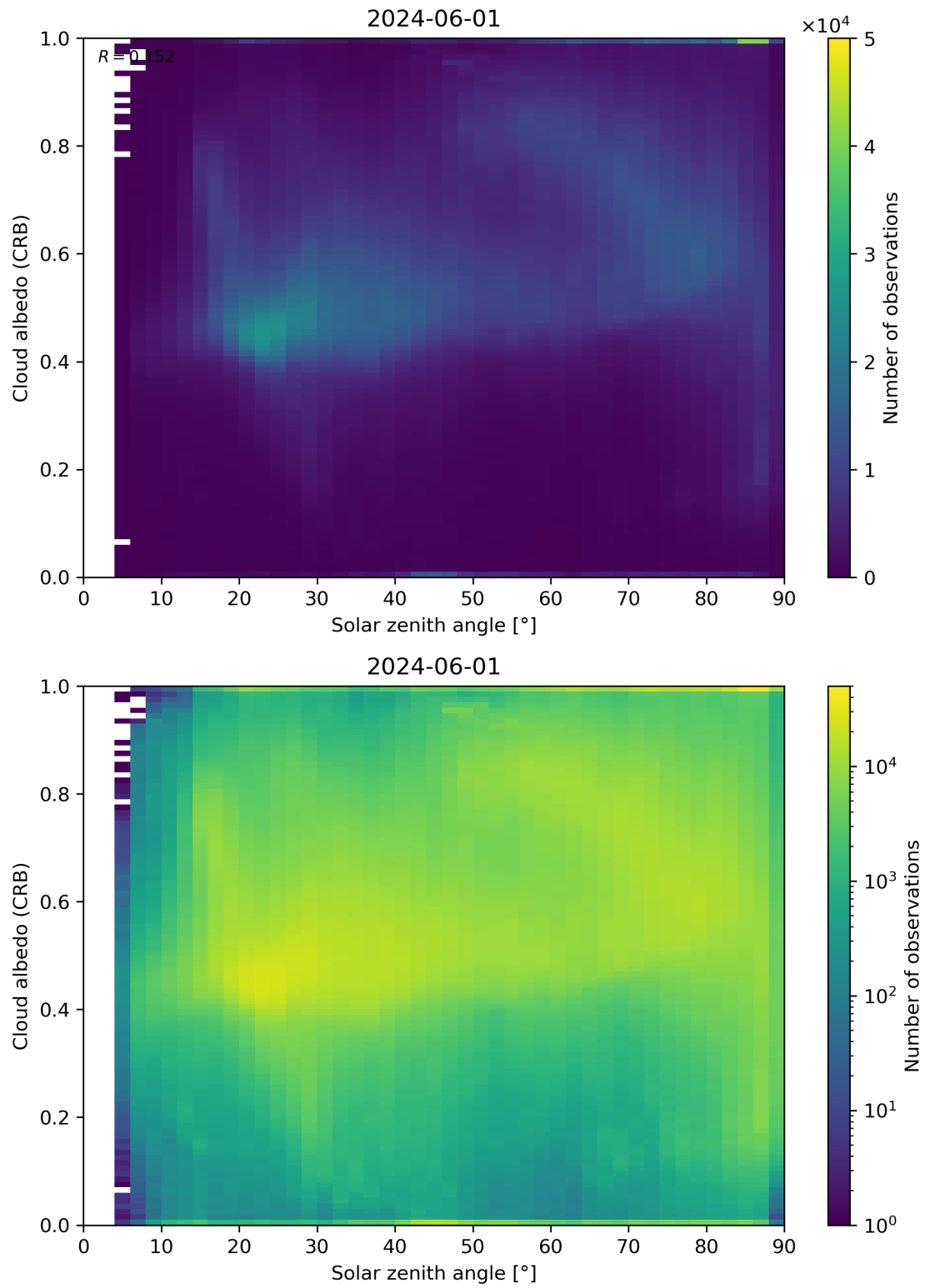
Figure 98: Scatter density plot of “Solar zenith angle” against “Cloud albedo (CRB)” for 2024-05-31 to 2024-06-02.
