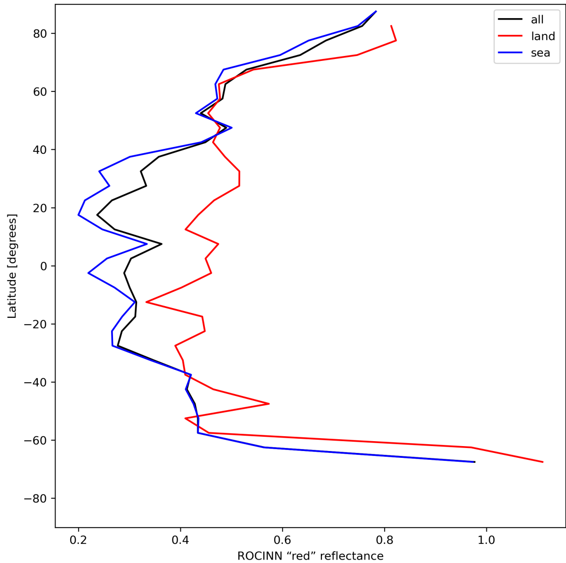
Figure 37: Zonal average of “ROCINN “red” reflectance” for 2024-05-31 to 2024-06-02.
