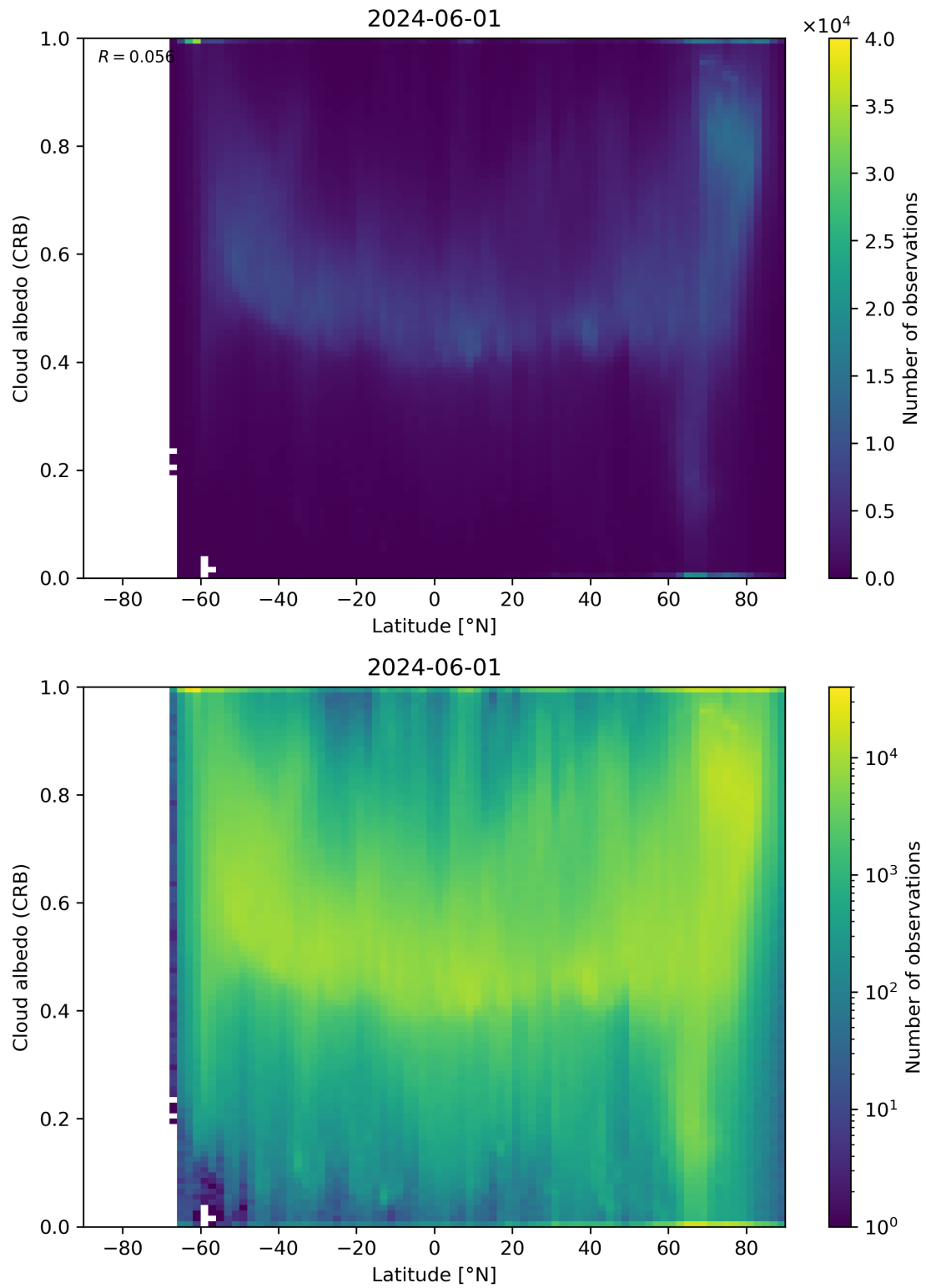
Figure 91: Scatter density plot of “Latitude” against “Cloud albedo (CRB)” for 2024-05-31 to 2024-06-02.
