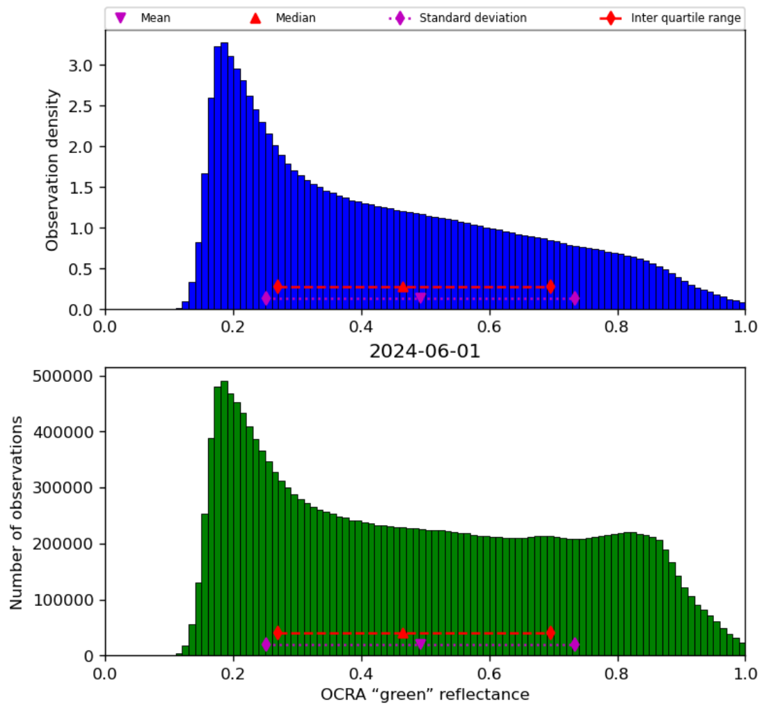
Figure 52: Histogram of “OCRA “green” reflectance” for 2024-05-31 to 2024-06-02
