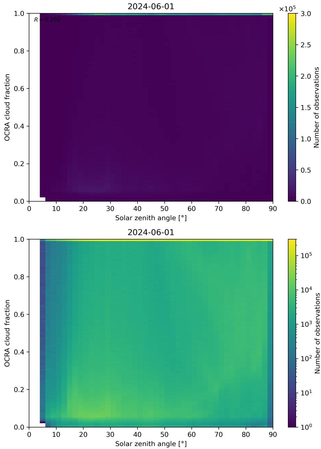
Figure 100: Scatter density plot of “Solar zenith angle” against “OCRA cloud fraction” for 2024-05-31 to 2024-06-02.
