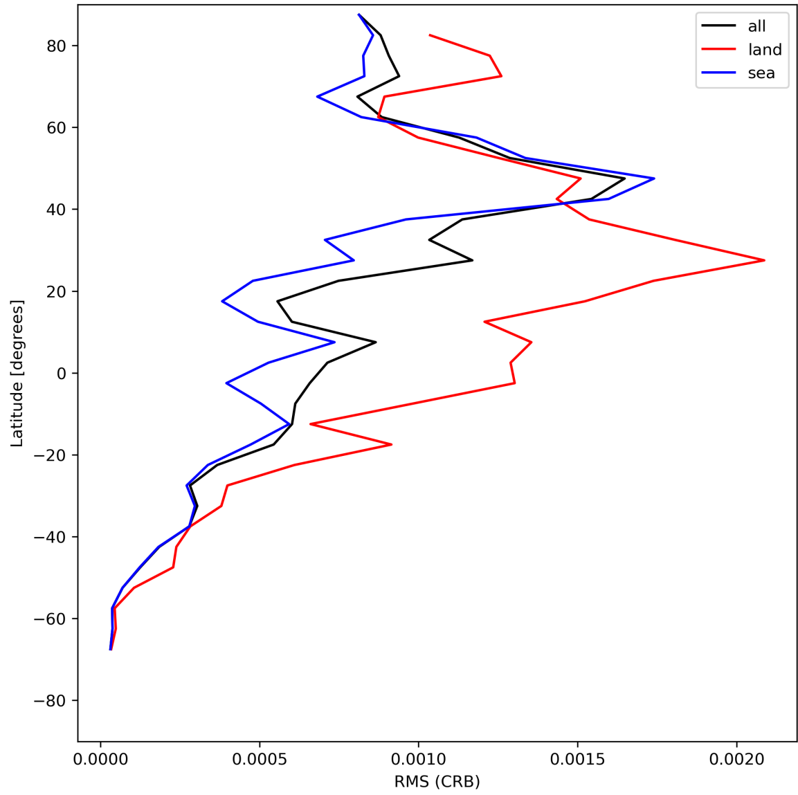
Figure 32: Zonal average of “RMS (CRB)” for 2024-05-31 to 2024-06-02.
