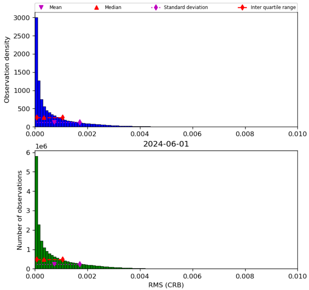
Figure 48: Histogram of “RMS (CRB)” for 2024-05-31 to 2024-06-02
