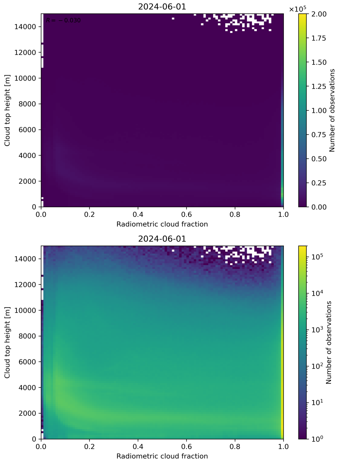
Figure 76: Scatter density plot of “Radiometric cloud fraction” against “Cloud top height” for 2024-05-31 to 2024-06-02.
