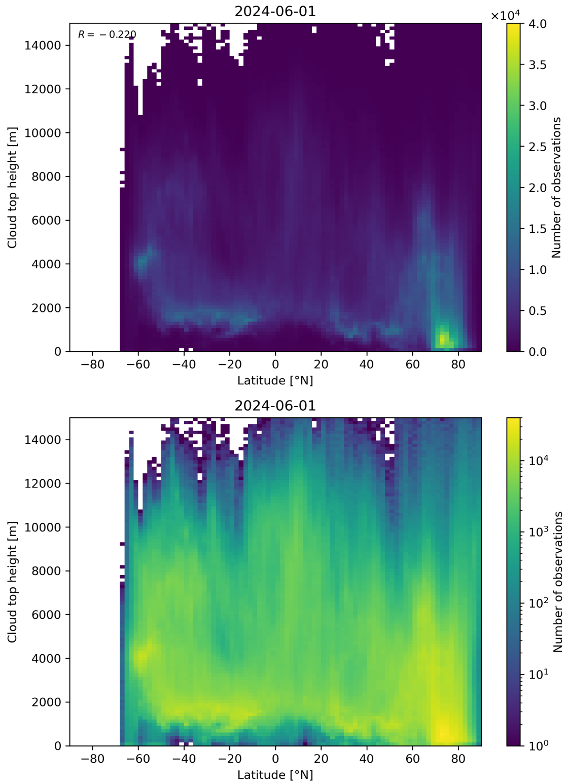
Figure 97: Scatter density plot of “Latitude” against “Cloud top height” for 2024-05-31 to 2024-06-02.
