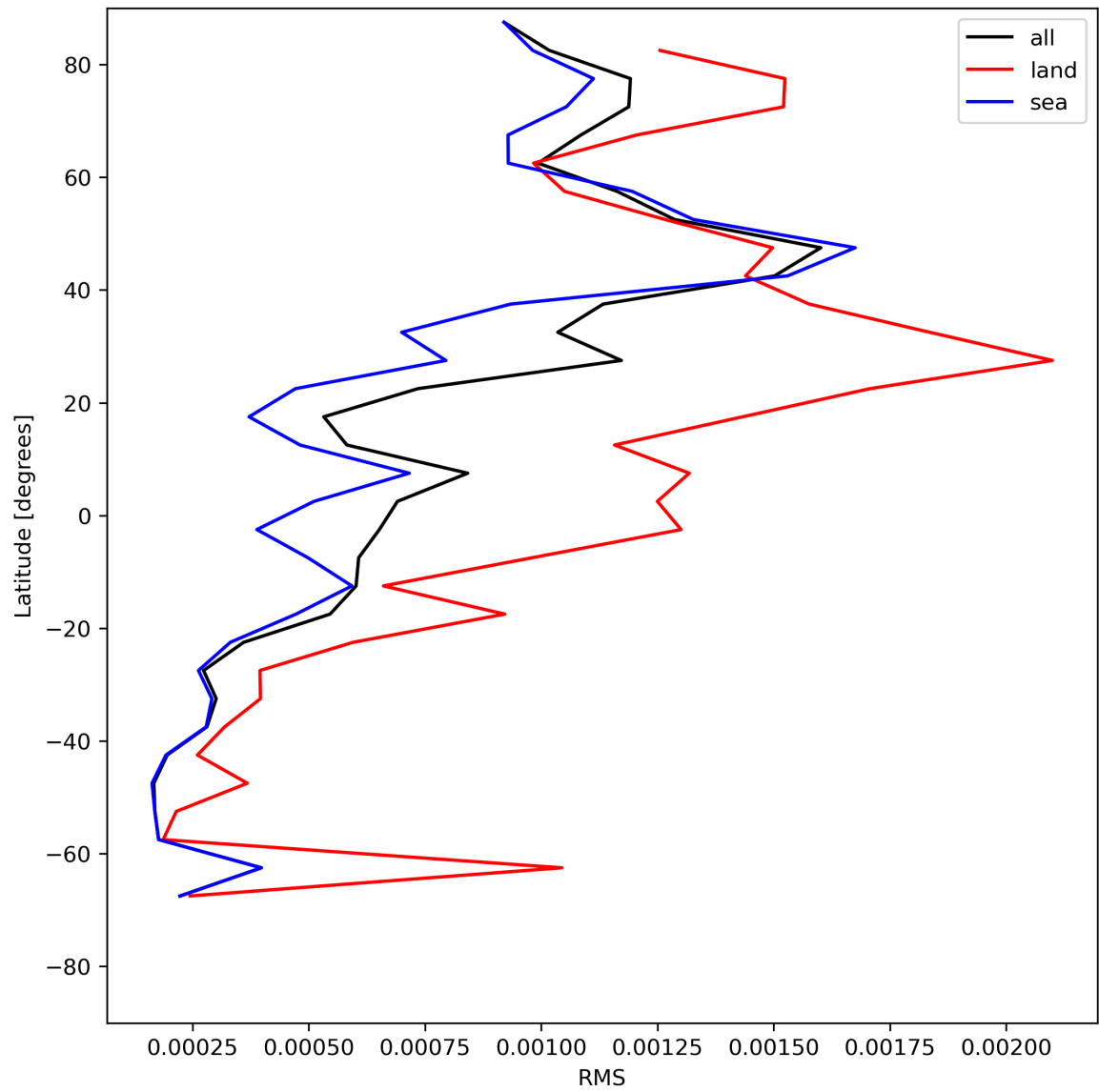
Figure 31: Zonal average of “RMS” for 2024-05-31 to 2024-06-02.
