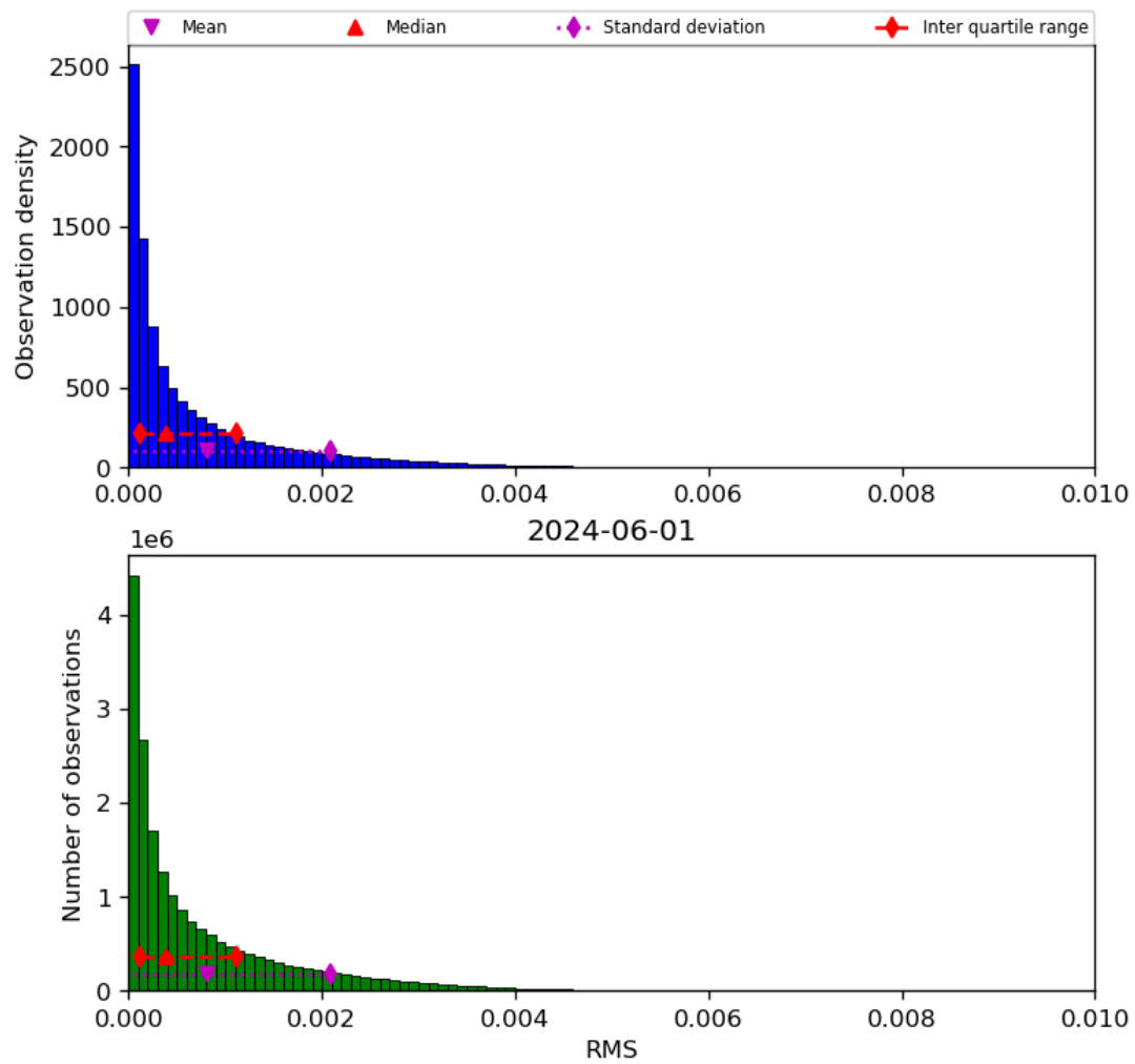
Figure 47: Histogram of “RMS” for 2024-05-31 to 2024-06-02
