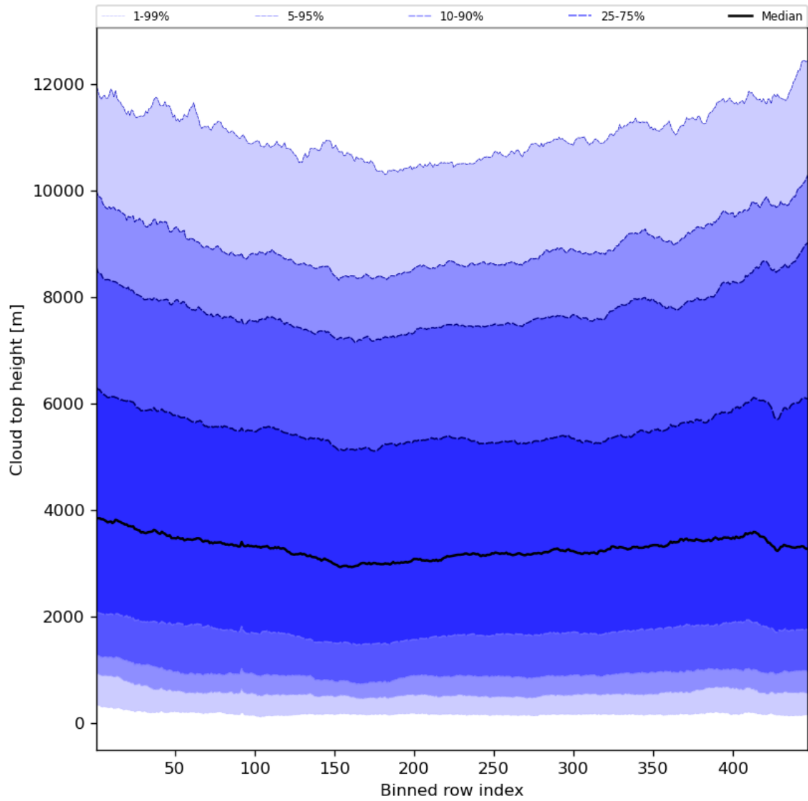
Figure 56: Along track statistics of “Cloud top height” for 2024-05-31 to 2024-06-02
