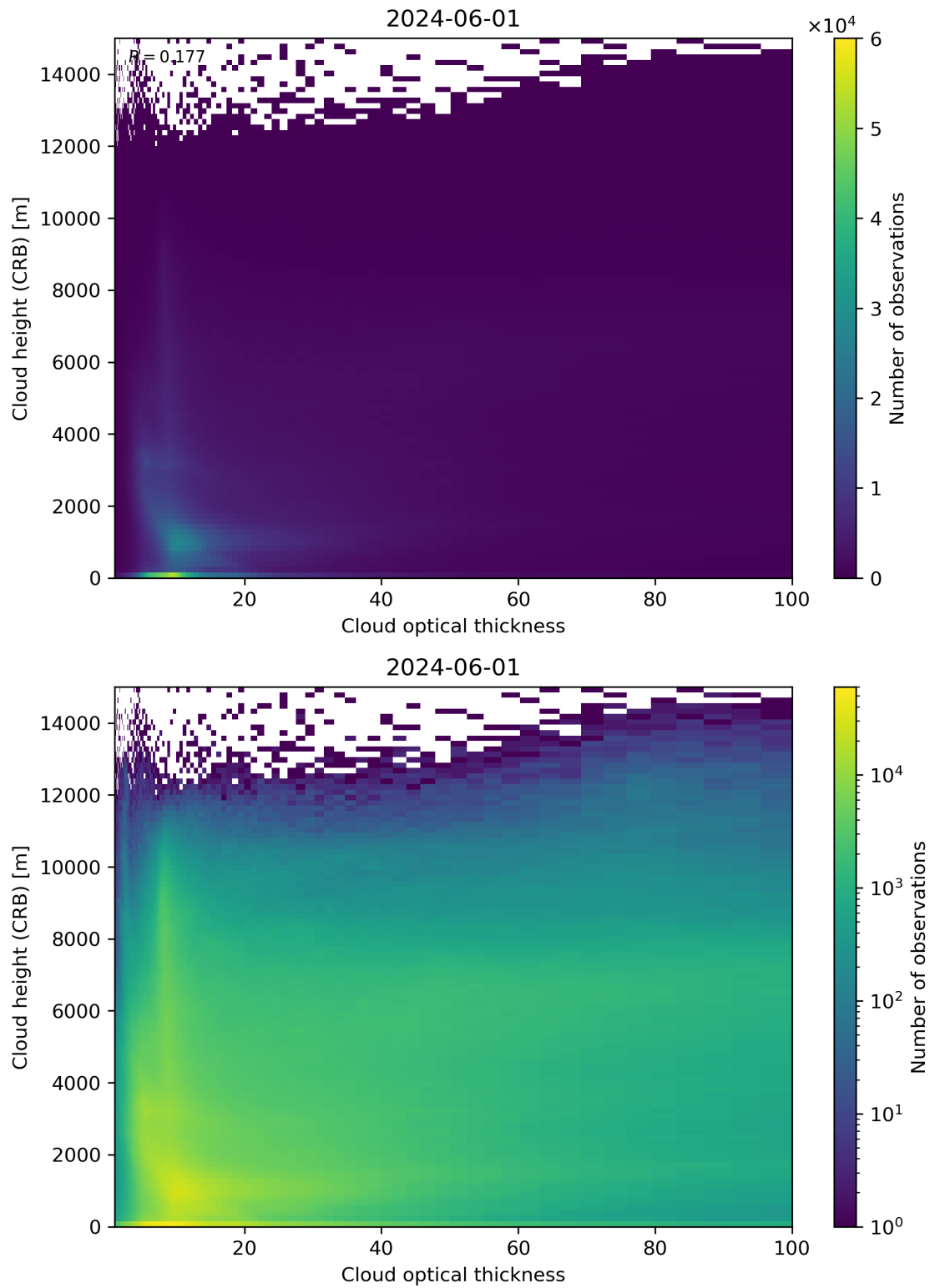
Figure 85: Scatter density plot of “Cloud optical thickness” against “Cloud height (CRB)” for 2024-05-31 to 2024-06-02.
