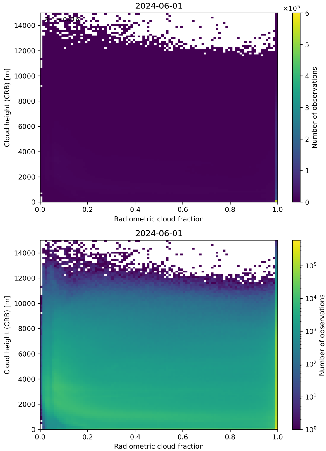
Figure 74: Scatter density plot of “Radiometric cloud fraction” against “Cloud height (CRB)” for 2024-05-31 to 2024-06-02.
