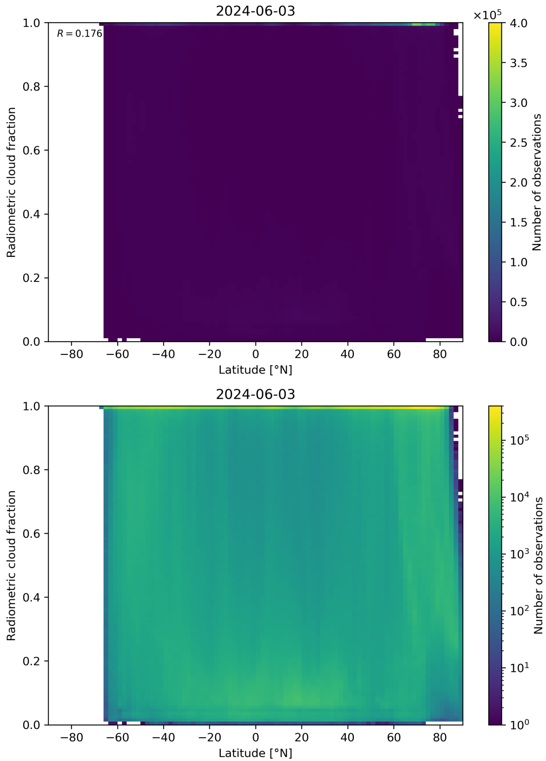
Figure 92: Scatter density plot of “Latitude” against “Radiometric cloud fraction” for 2024-06-03 to 2024-06-04.
