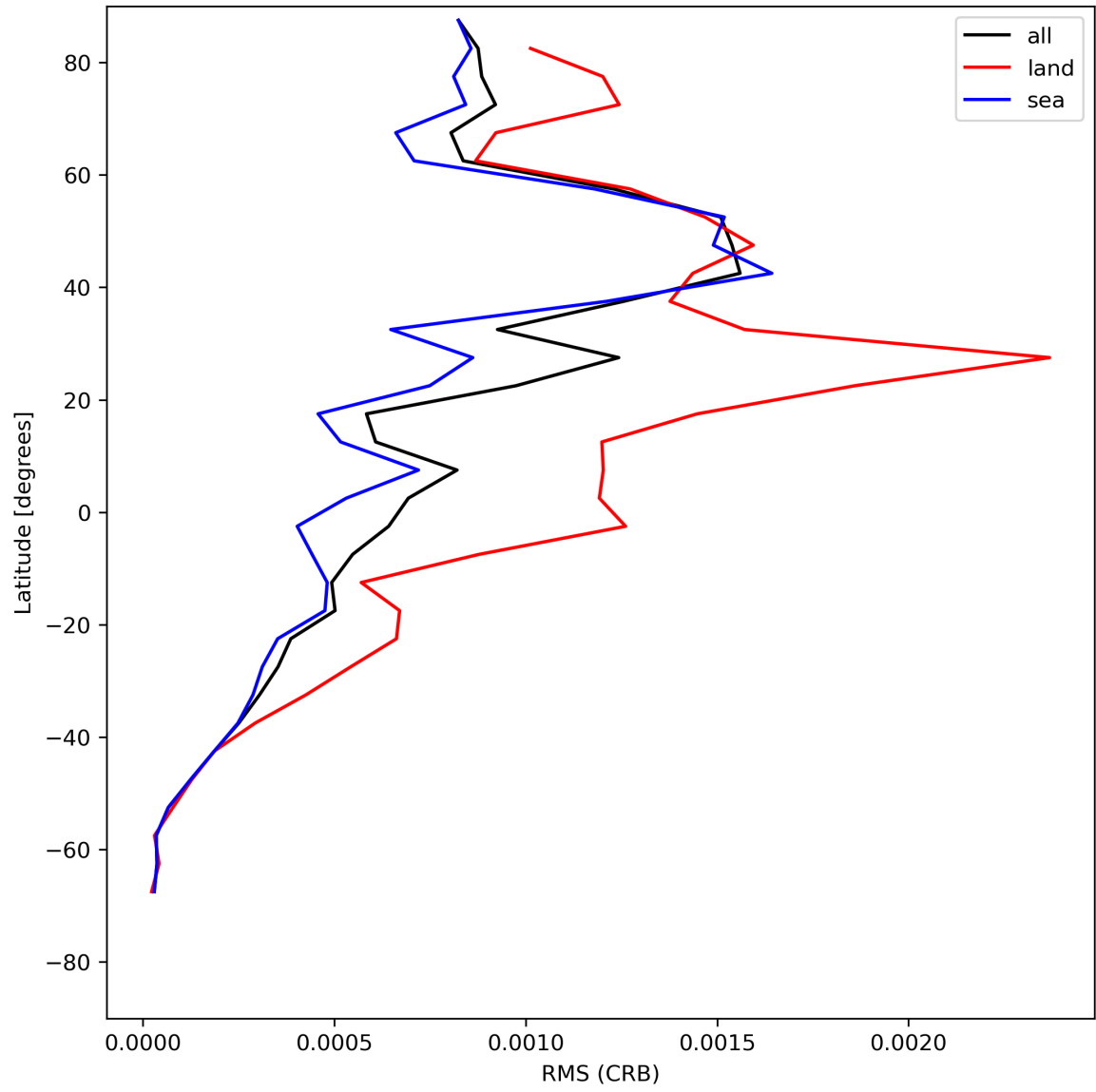
Figure 32: Zonal average of “RMS (CRB)” for 2024-06-03 to 2024-06-04.
