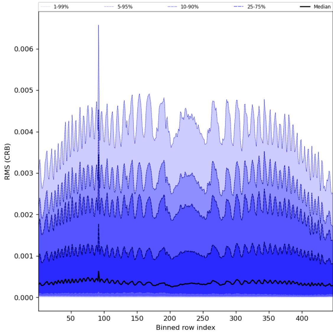
Figure 64: Along track statistics of “RMS (CRB)” for 2024-06-03 to 2024-06-04
