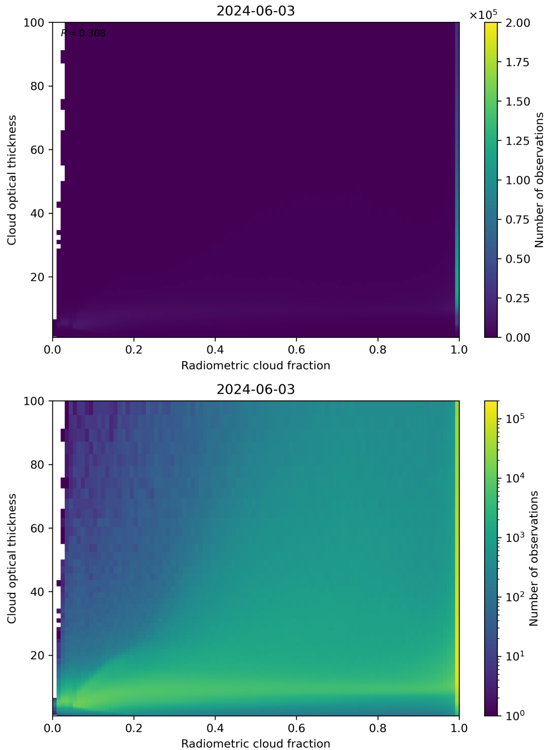
Figure 75: Scatter density plot of “Radiometric cloud fraction” against “Cloud optical thickness” for 2024-06-03 to 2024-06-04.
