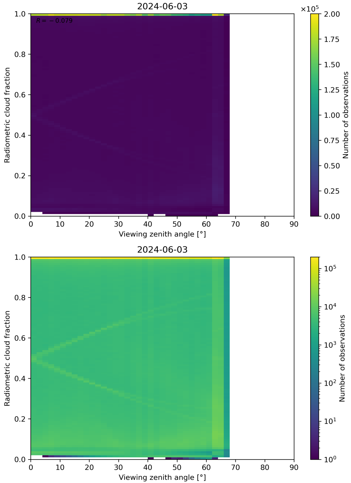
Figure 107: Scatter density plot of “Viewing zenith angle” against “Radiometric cloud fraction” for 2024-06-03 to 2024-06-04.
