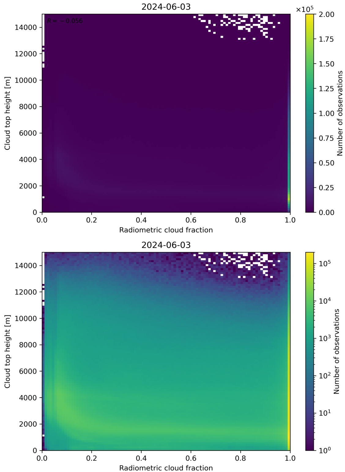
Figure 76: Scatter density plot of “Radiometric cloud fraction” against “Cloud top height” for 2024-06-03 to 2024-06-04.
