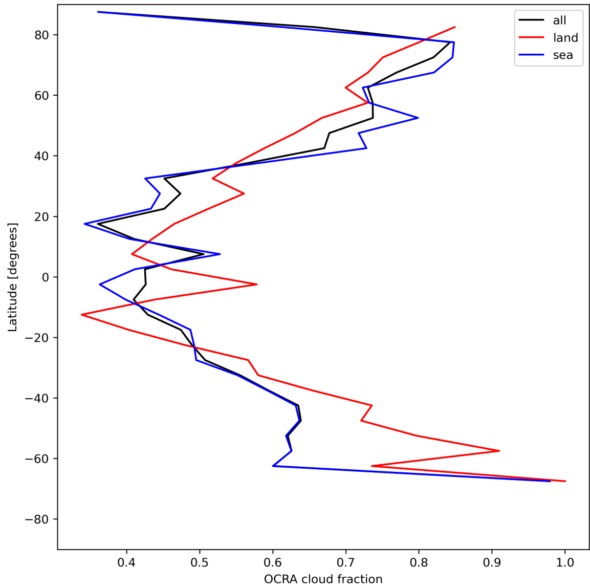
Figure 34: Zonal average of “OCRA cloud fraction” for 2024-06-03 to 2024-06-04.
