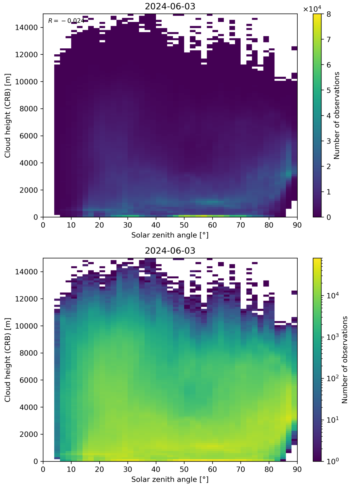
Figure 102: Scatter density plot of “Solar zenith angle” against “Cloud height (CRB)” for 2024-06-03 to 2024-06-04.
