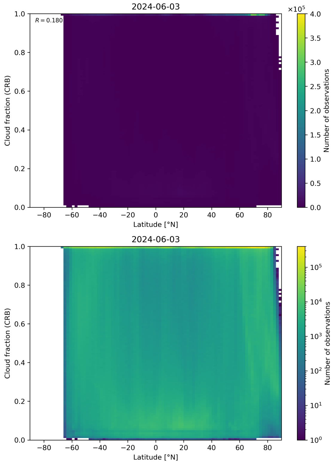
Figure 94: Scatter density plot of “Latitude” against “Cloud fraction (CRB)” for 2024-06-03 to 2024-06-04.
