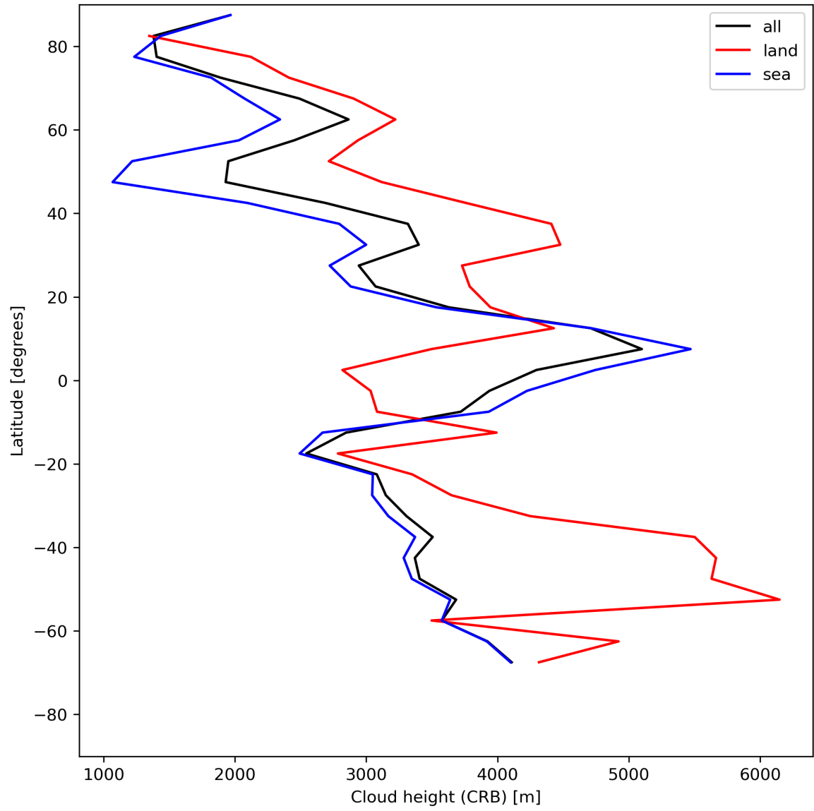
Figure 27: Zonal average of “Cloud height (CRB)” for 2024-06-03 to 2024-06-04.
