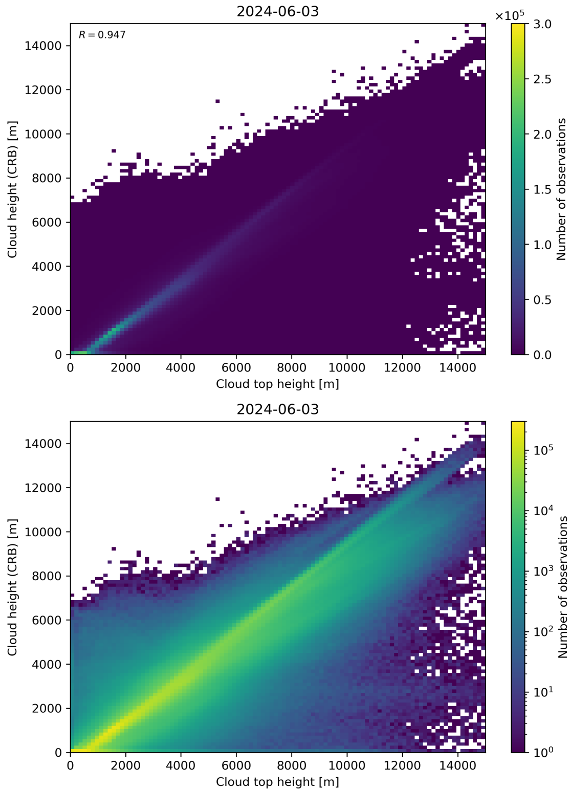
Figure 89: Scatter density plot of “Cloud top height” against “Cloud height (CRB)” for 2024-06-03 to 2024-06-04.
