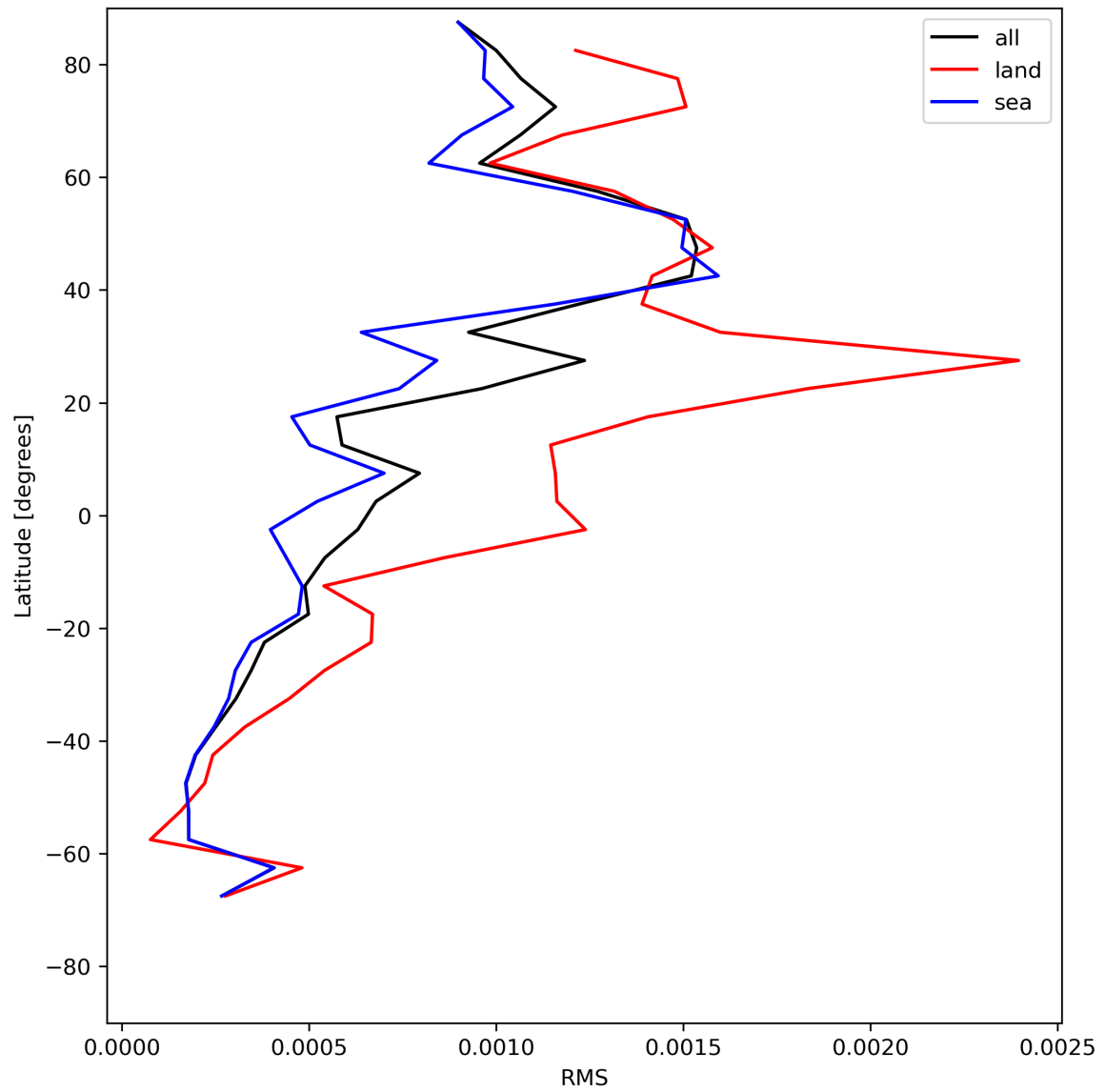
Figure 31: Zonal average of “RMS” for 2024-06-03 to 2024-06-04.
