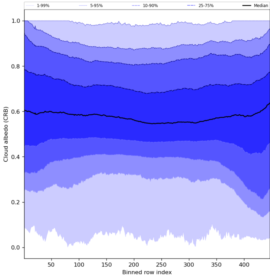
Figure 60: Along track statistics of “Cloud albedo (CRB)” for 2024-06-03 to 2024-06-04
