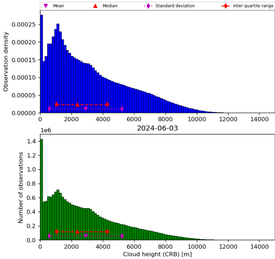
Figure 43: Histogram of “Cloud height (CRB)” for 2024-06-03 to 2024-06-04
