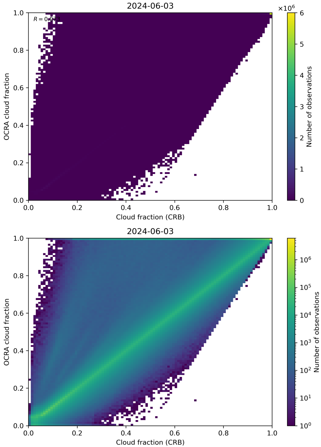
Figure 78: Scatter density plot of “Cloud fraction (CRB)” against “OCRA cloud fraction” for 2024-06-03 to 2024-06-04.
