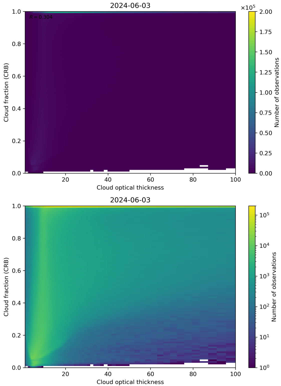
Figure 84: Scatter density plot of “Cloud optical thickness” against “Cloud fraction (CRB)” for 2024-06-03 to 2024-06-04.
