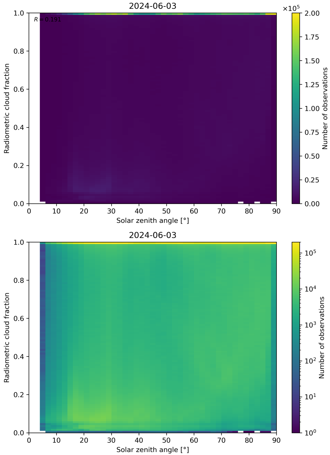
Figure 99: Scatter density plot of “Solar zenith angle” against “Radiometric cloud fraction” for 2024-06-03 to 2024-06-04.
