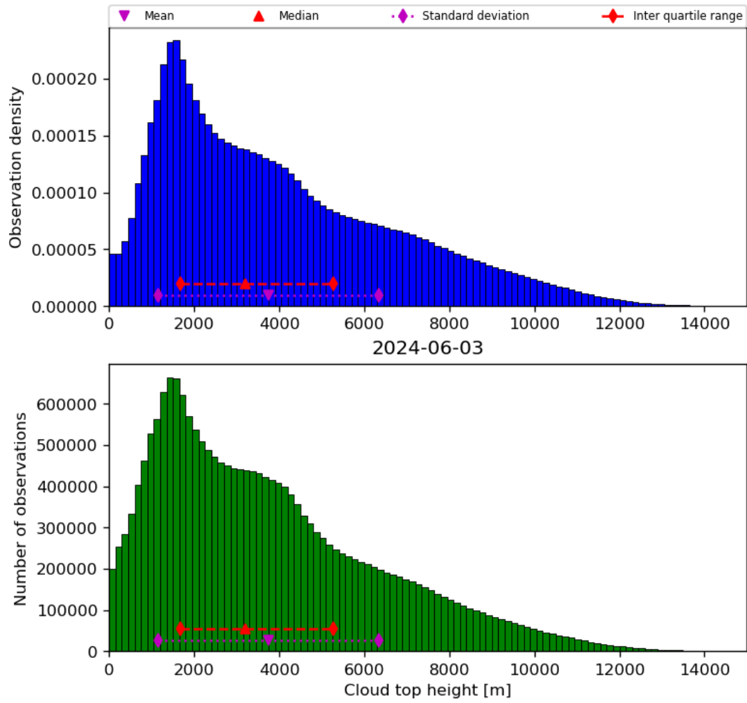
Figure 40: Histogram of “Cloud top height” for 2024-06-03 to 2024-06-04
