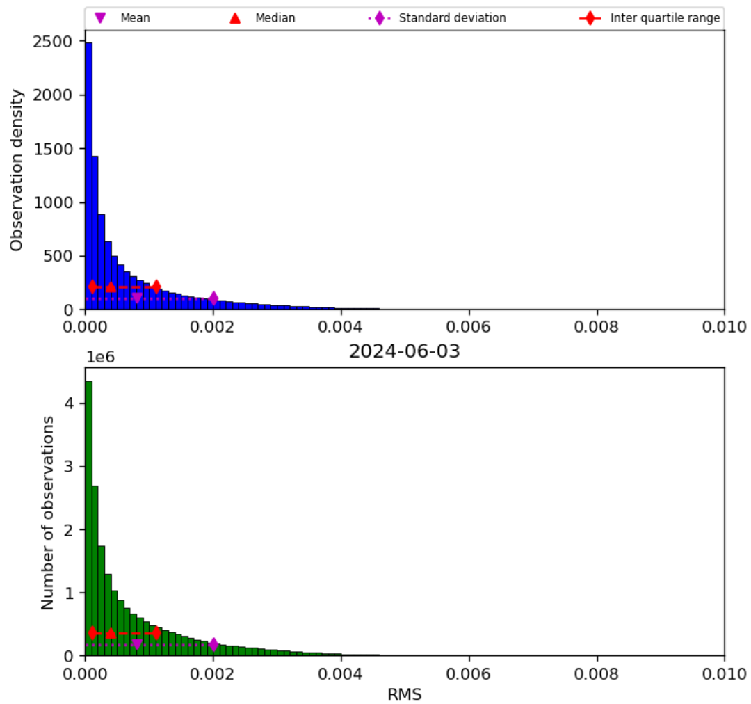
Figure 47: Histogram of “RMS” for 2024-06-03 to 2024-06-04
