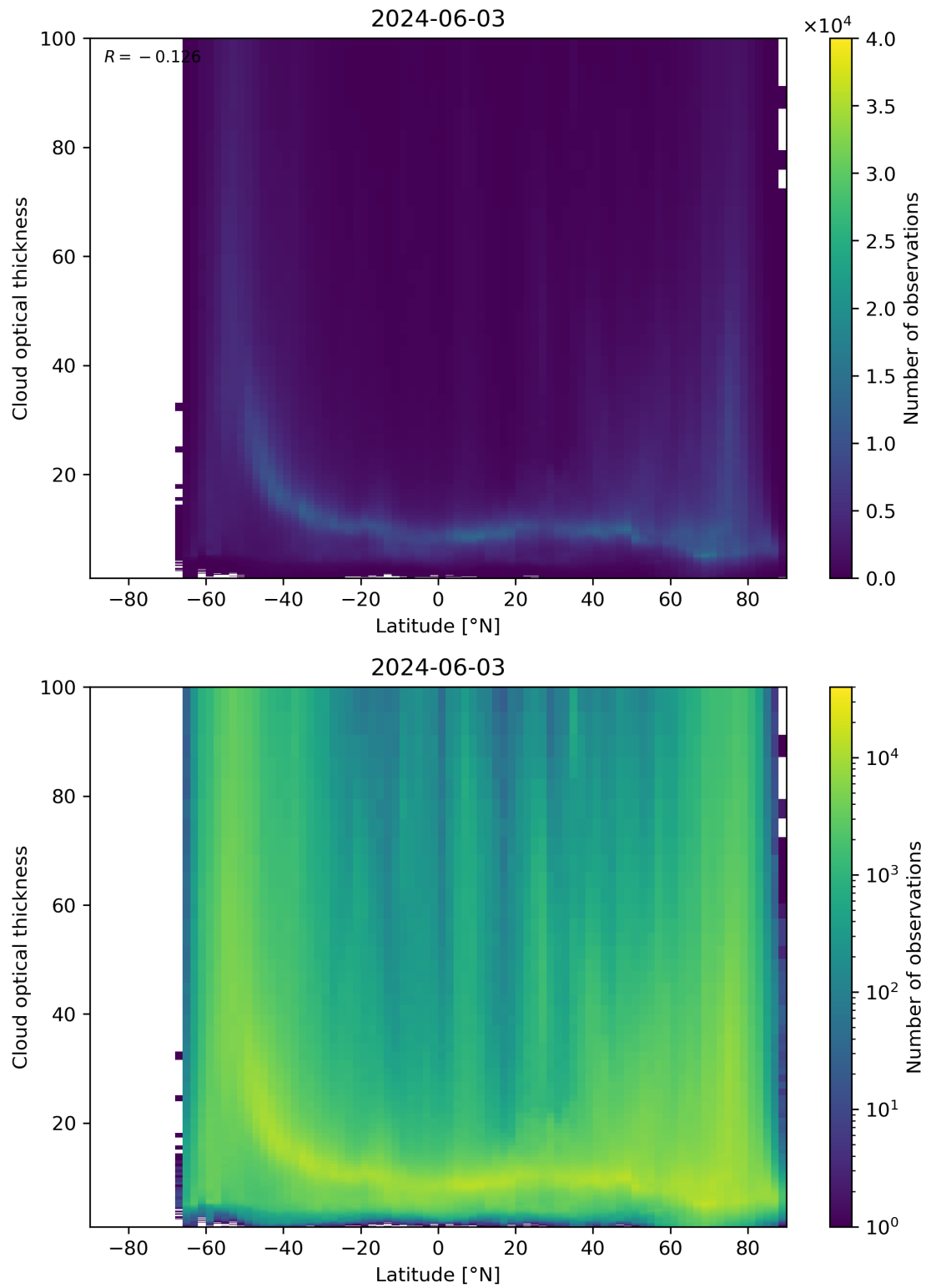
Figure 96: Scatter density plot of “Latitude” against “Cloud optical thickness” for 2024-06-03 to 2024-06-04.
