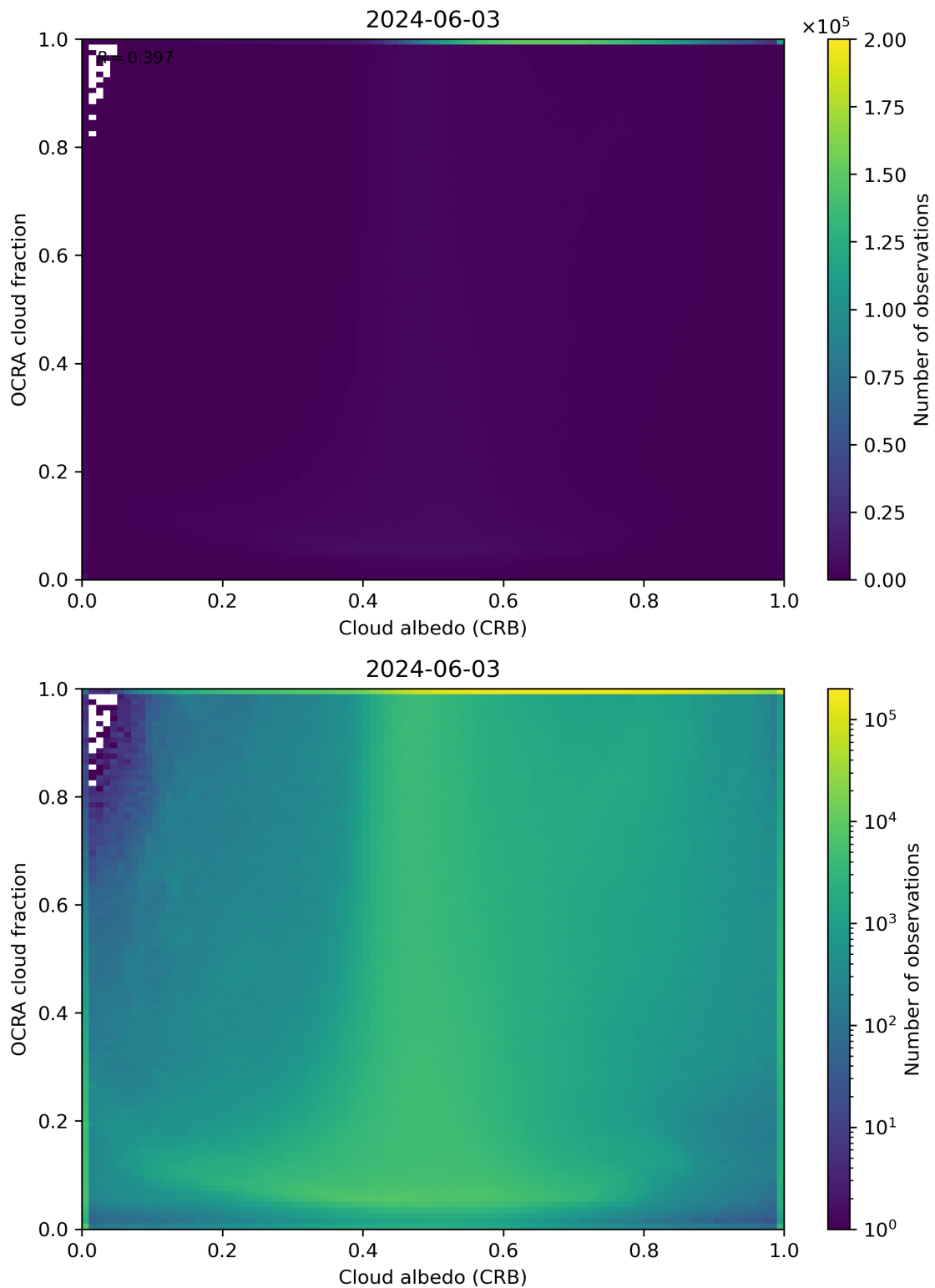
Figure 70: Scatter density plot of “Cloud albedo (CRB)” against “OCRA cloud fraction” for 2024-06-03 to 2024-06-04.
