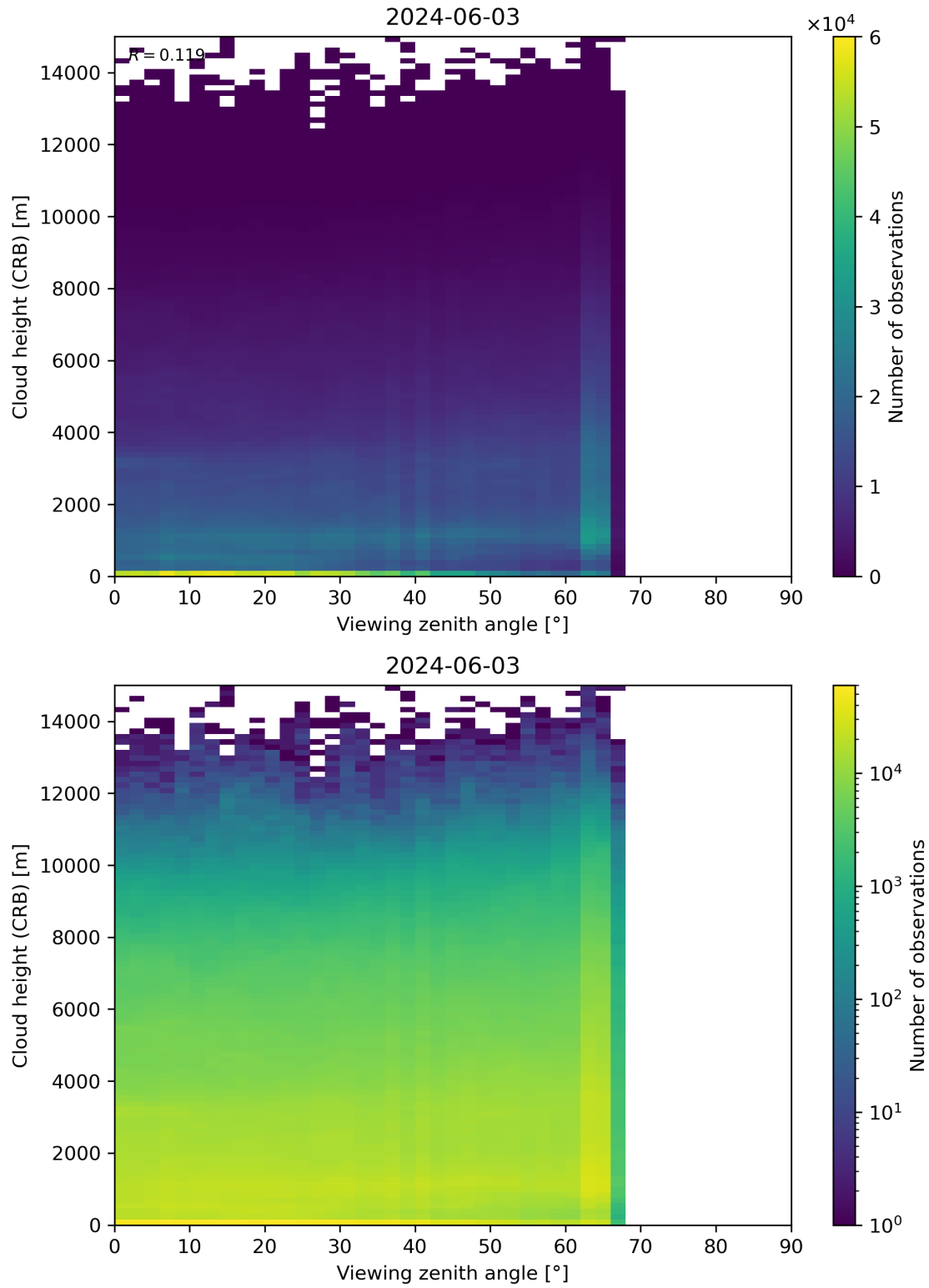
Figure 110: Scatter density plot of “Viewing zenith angle” against “Cloud height (CRB)” for 2024-06-03 to 2024-06-04.
