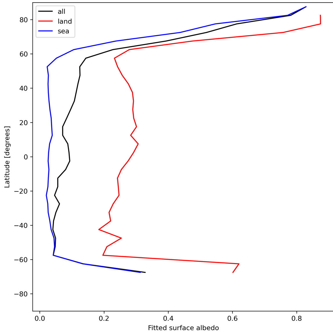
Figure 29: Zonal average of “Fitted surface albedo” for 2024-06-03 to 2024-06-04.
