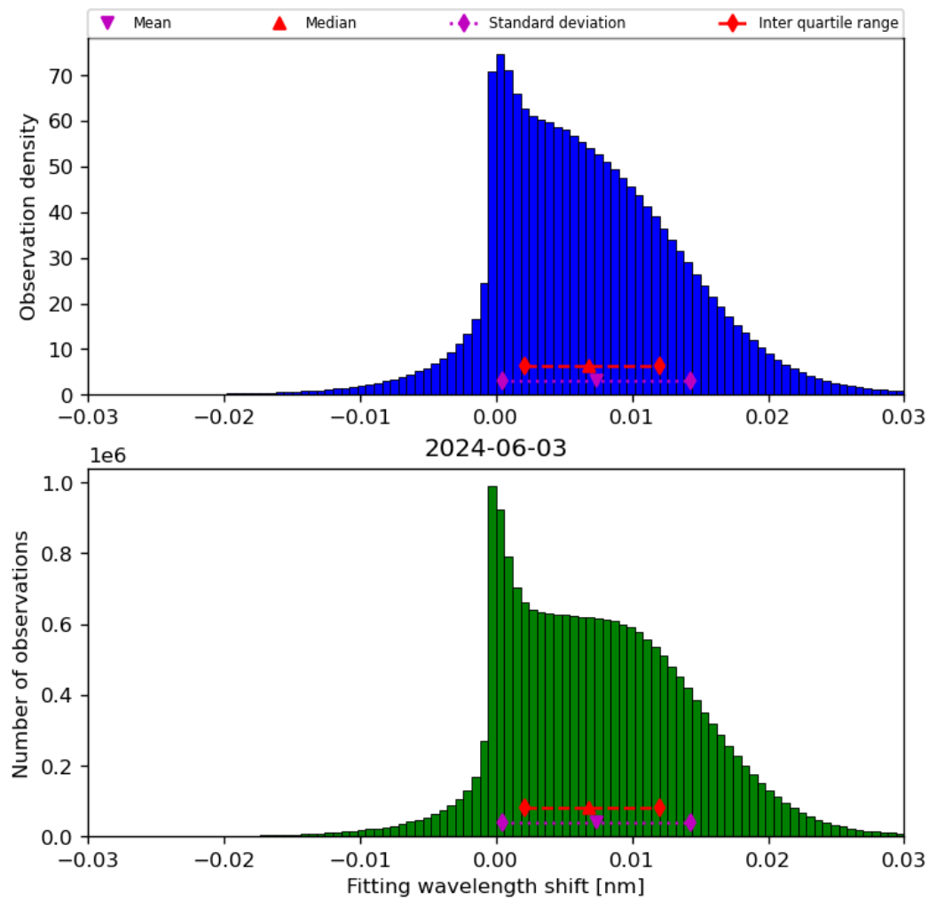
Figure 49: Histogram of “Fitting wavelength shift” for 2024-06-03 to 2024-06-04
