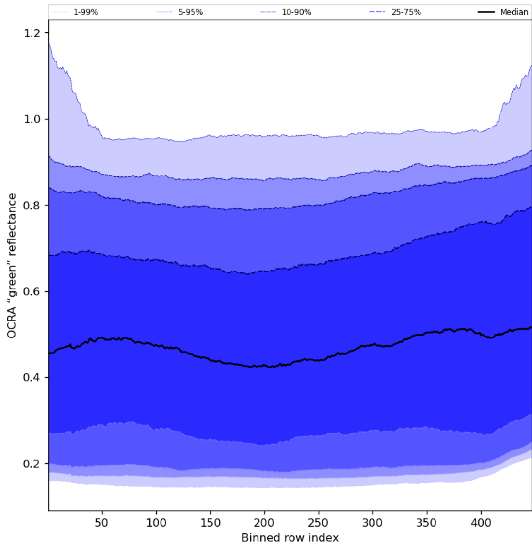
Figure 68: Along track statistics of "OCRA "green" reflectance" for 2024-06-03 to 2024-06-04
