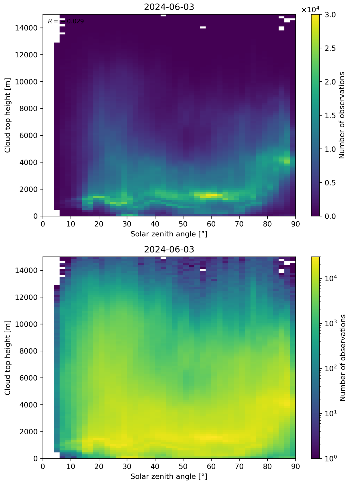
Figure 104: Scatter density plot of “Solar zenith angle” against “Cloud top height” for 2024-06-03 to 2024-06-04.
