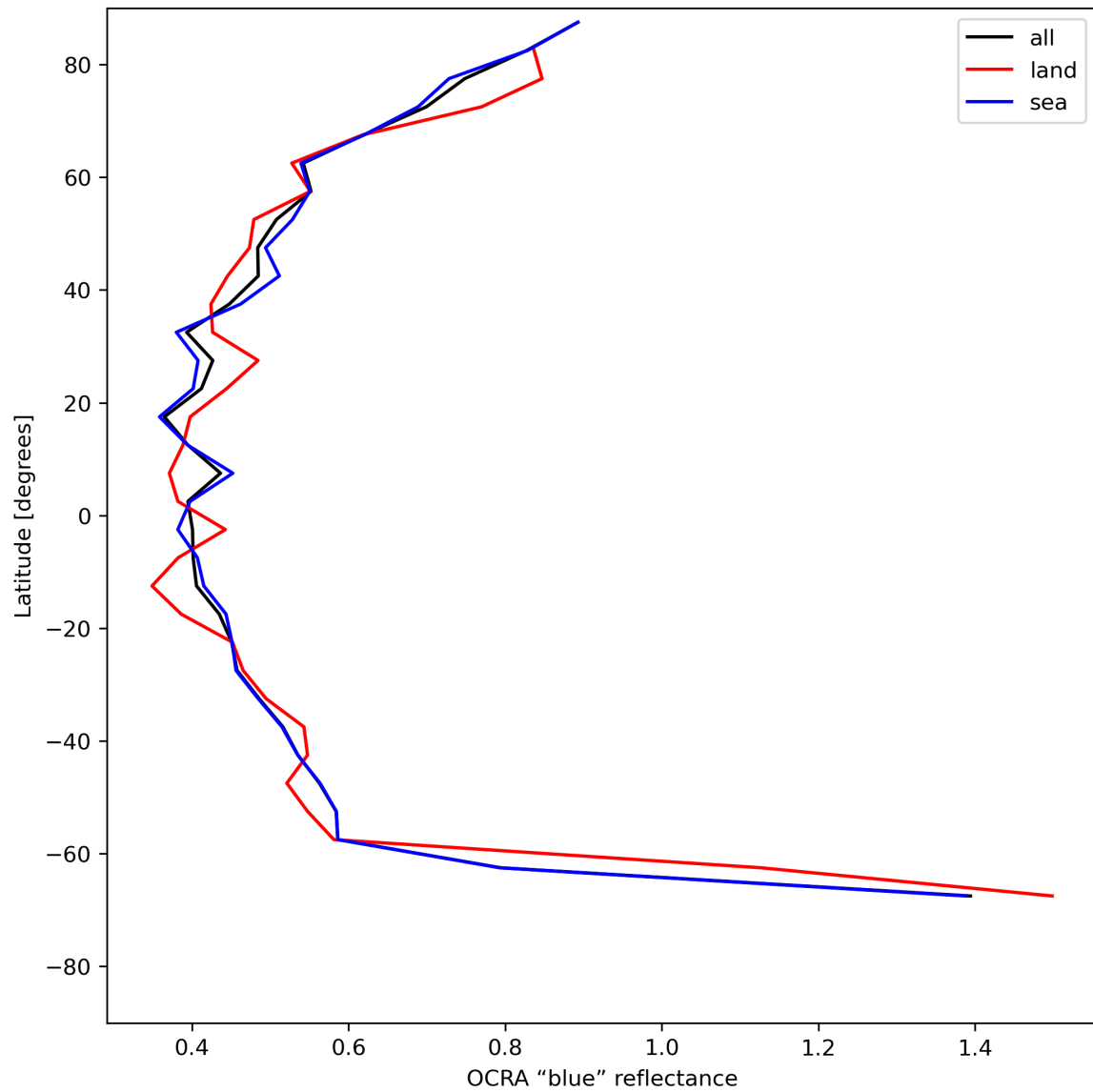
Figure 35: Zonal average of “OCRA “blue” reflectance” for 2024-06-03 to 2024-06-04.
