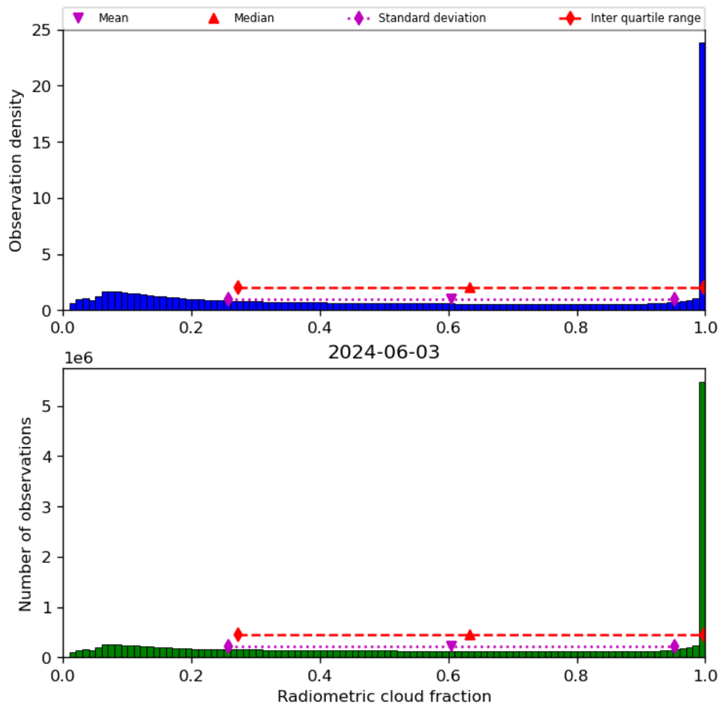
Figure 39: Histogram of “Radiometric cloud fraction” for 2024-06-03 to 2024-06-04
