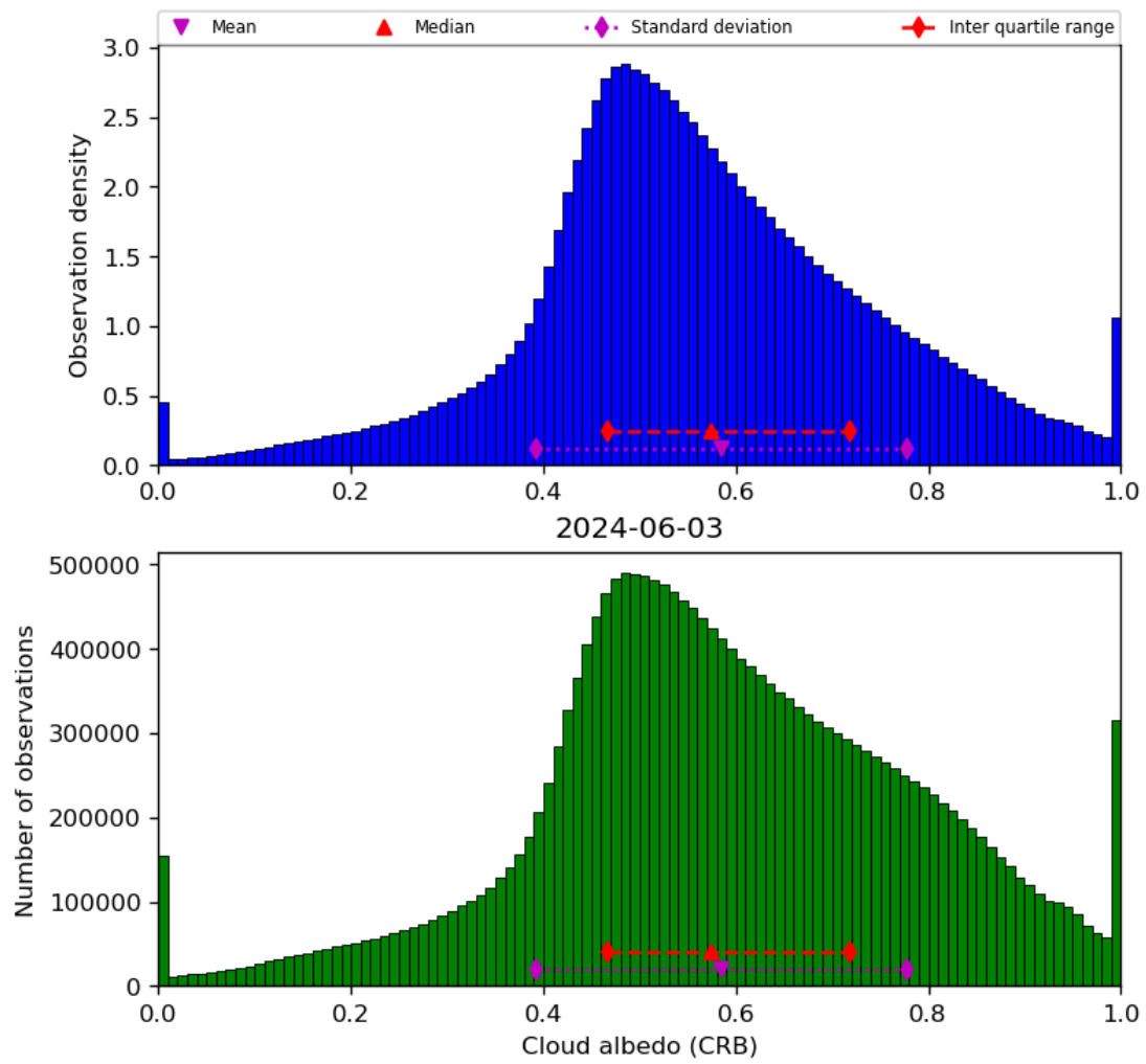
Figure 44: Histogram of “Cloud albedo (CRB)” for 2024-06-03 to 2024-06-04
