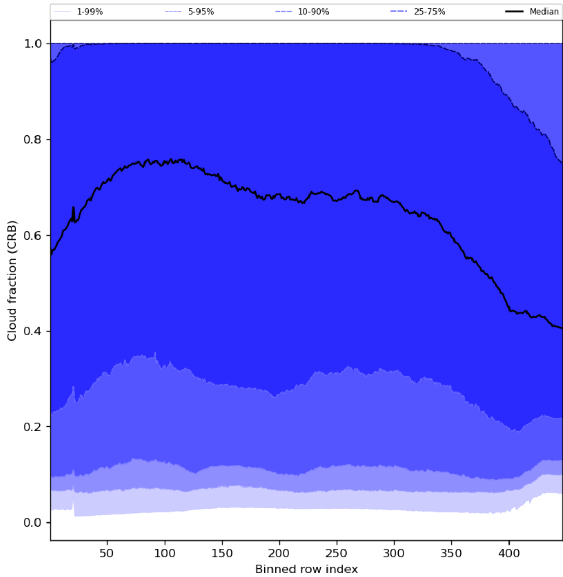
Figure 58: Along track statistics of “Cloud fraction (CRB)” for 2024-06-03 to 2024-06-04
