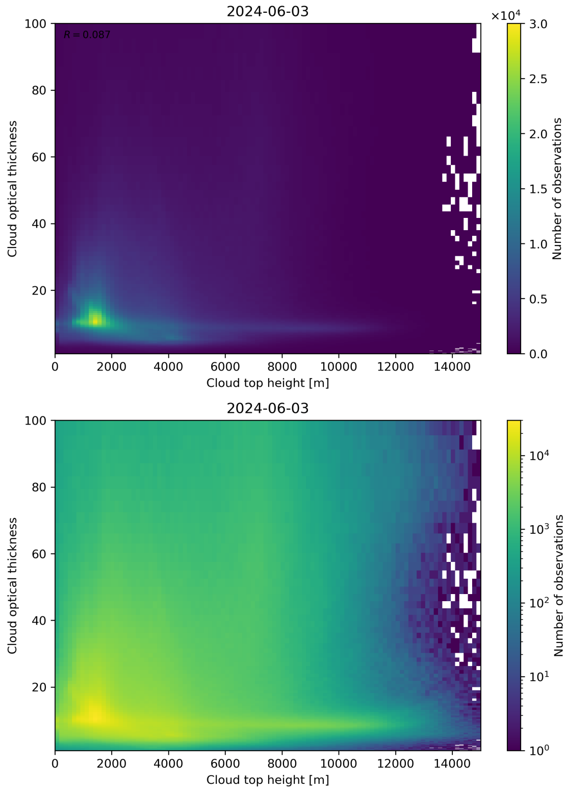
Figure 90: Scatter density plot of “Cloud top height” against “Cloud optical thickness” for 2024-06-03 to 2024-06-04.
