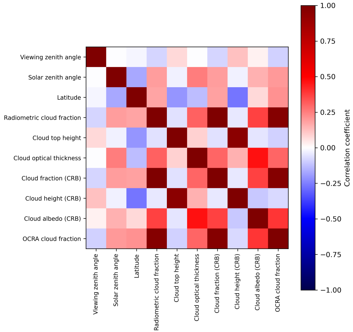
Figure 2: Map of correlation matrix for 2024-06-03 to 2024-06-04.
