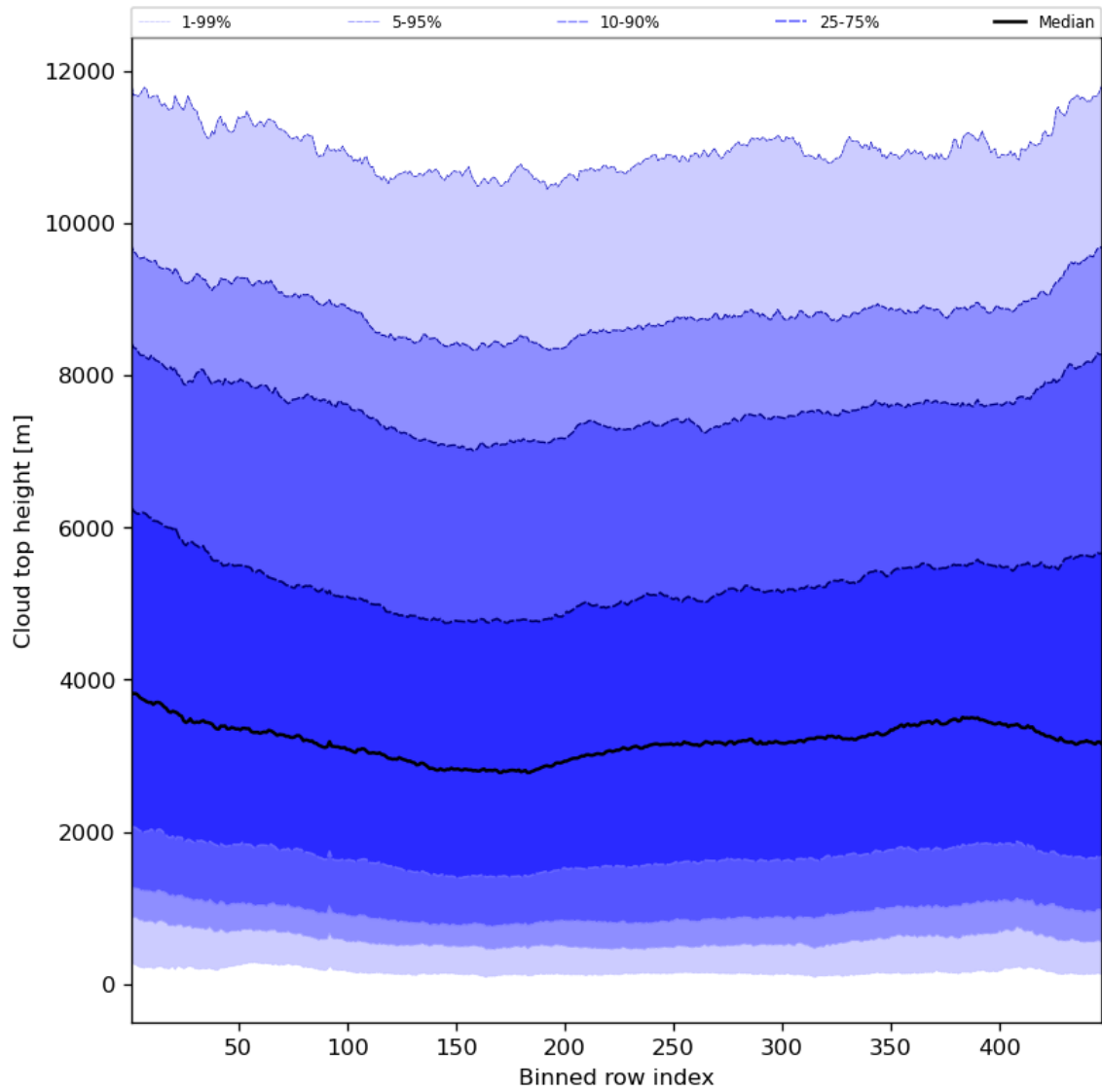
Figure 56: Along track statistics of “Cloud top height” for 2024-06-03 to 2024-06-04
