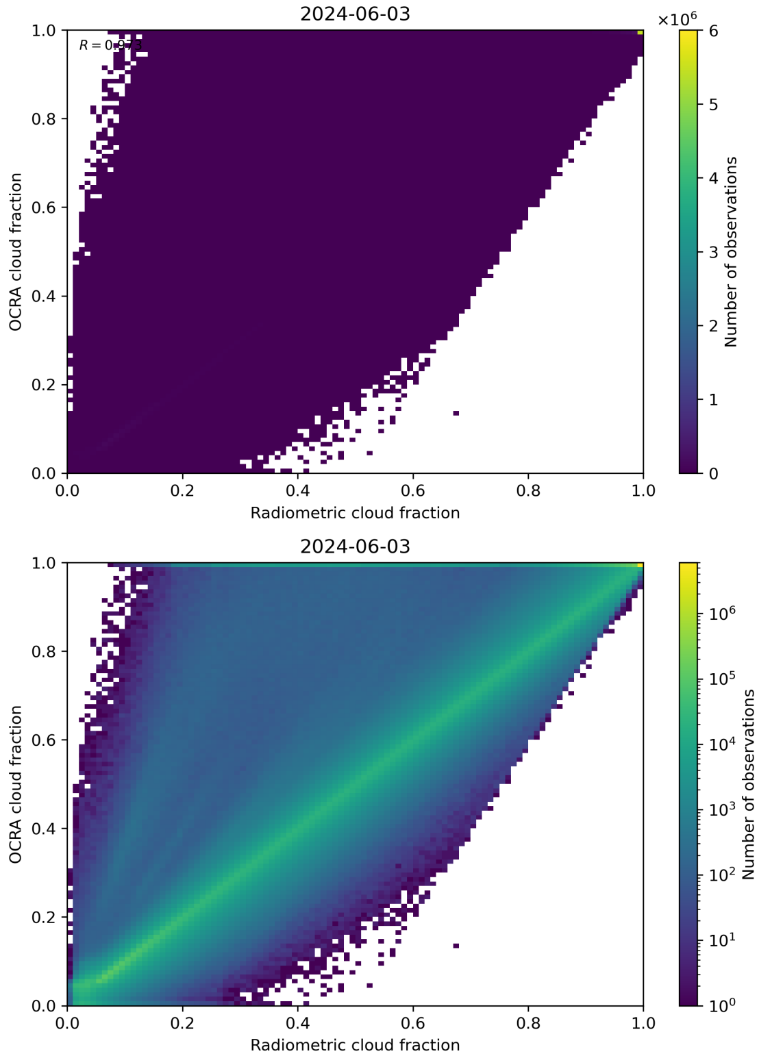
Figure 72: Scatter density plot of “Radiometric cloud fraction” against “OCRA cloud fraction” for 2024-06-03 to 2024-06-04.
