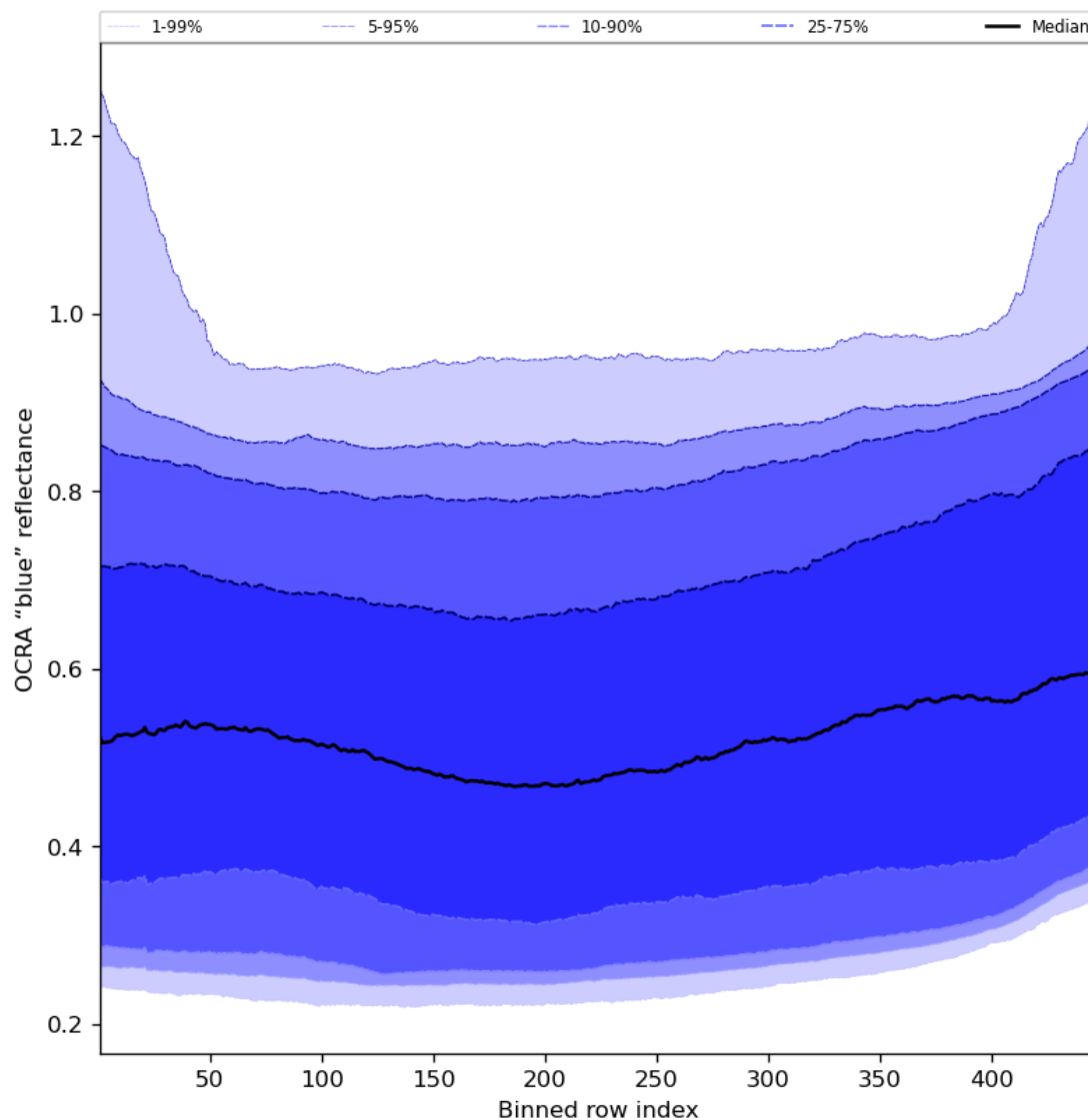
Figure 67: Along track statistics of “OCRA “blue” reflectance” for 2024-06-03 to 2024-06-04
