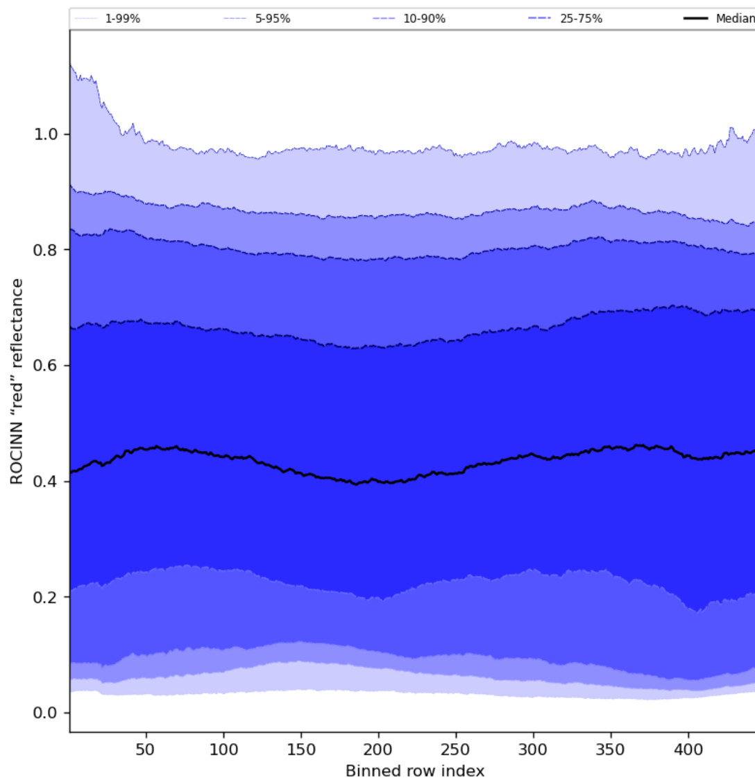
Figure 69: Along track statistics of “ROCINN “red” reflectance” for 2024-06-03 to 2024-06-04
