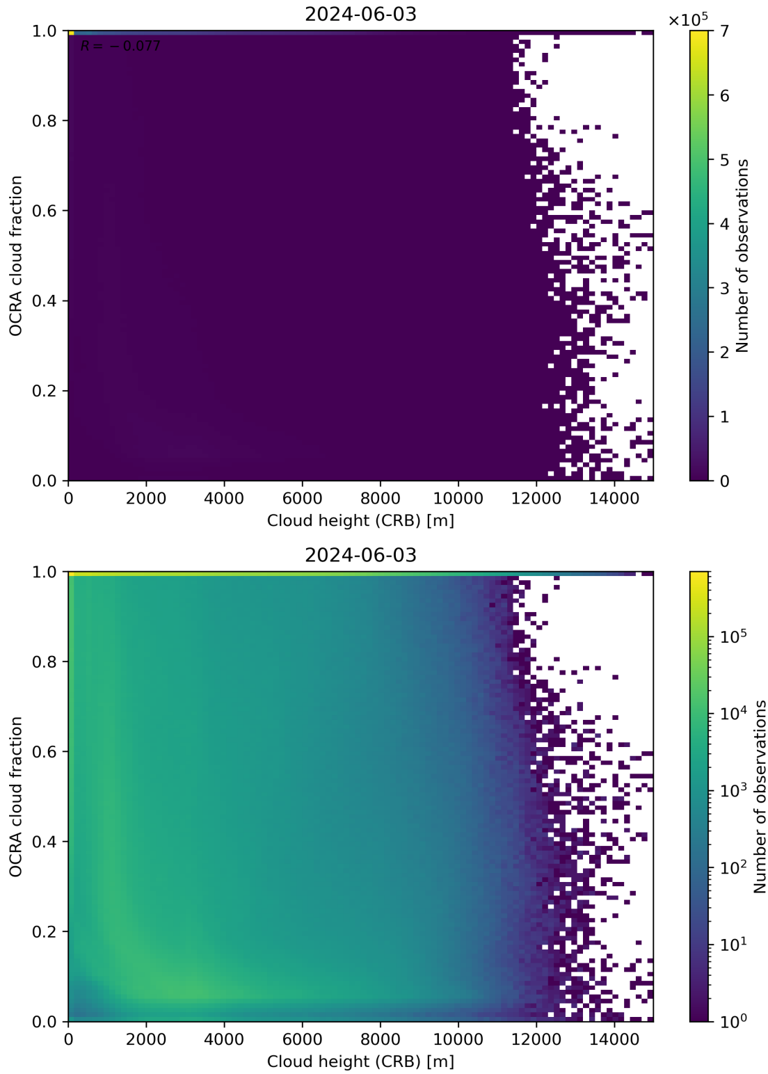
Figure 81: Scatter density plot of “Cloud height (CRB)” against “OCRA cloud fraction” for 2024-06-03 to 2024-06-04.
