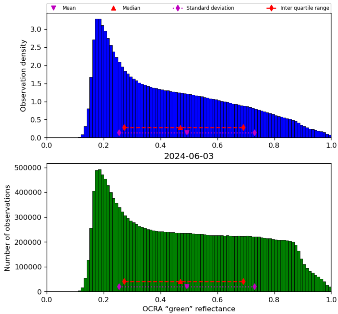
Figure 52: Histogram of “OCRA “green” reflectance” for 2024-06-03 to 2024-06-04
