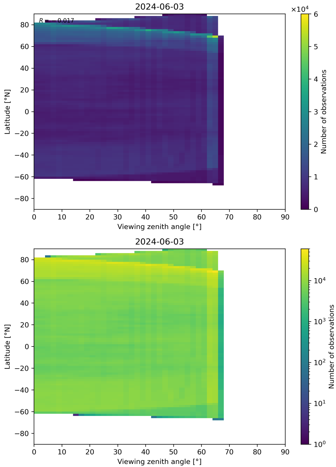
Figure 113: Scatter density plot of “Viewing zenith angle” against “Latitude” for 2024-06-03 to 2024-06-04.
