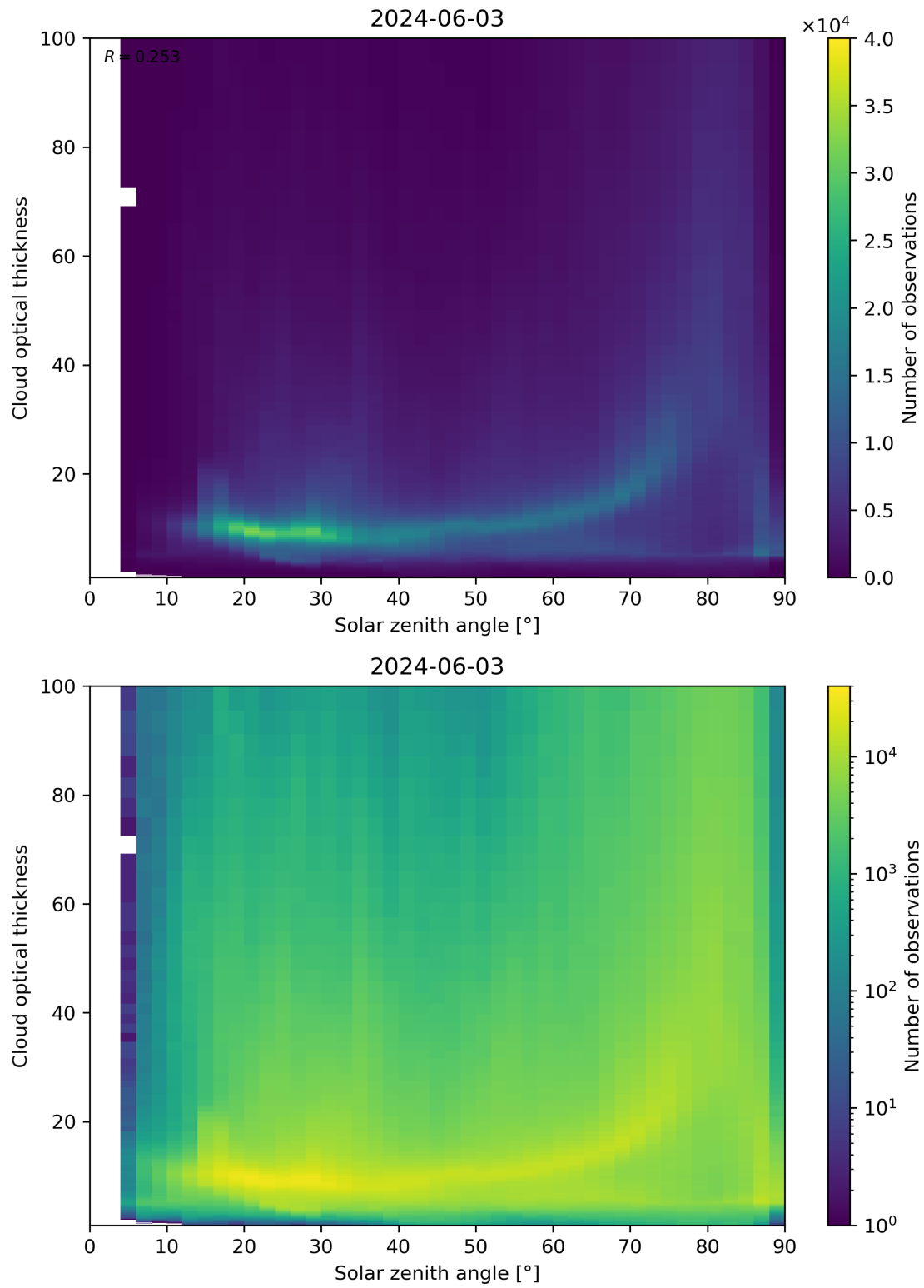
Figure 103: Scatter density plot of “Solar zenith angle” against “Cloud optical thickness” for 2024-06-03 to 2024-06-04.
