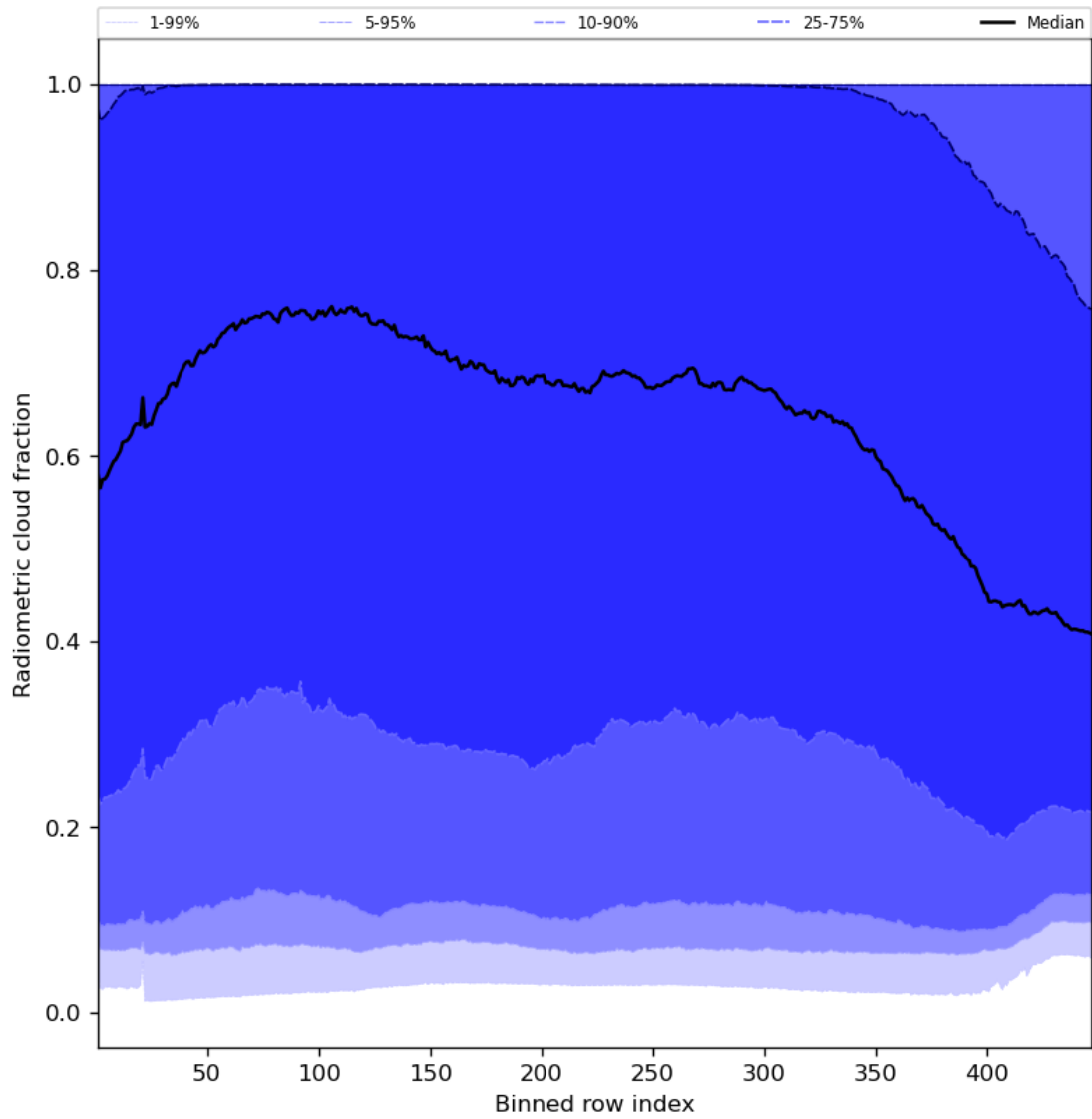
Figure 55: Along track statistics of "Radiometric cloud fraction" for 2024-06-03 to 2024-06-04
