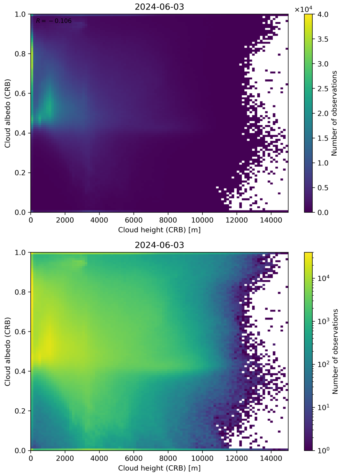
Figure 80: Scatter density plot of “Cloud height (CRB)” against “Cloud albedo (CRB)” for 2024-06-03 to 2024-06-04.
