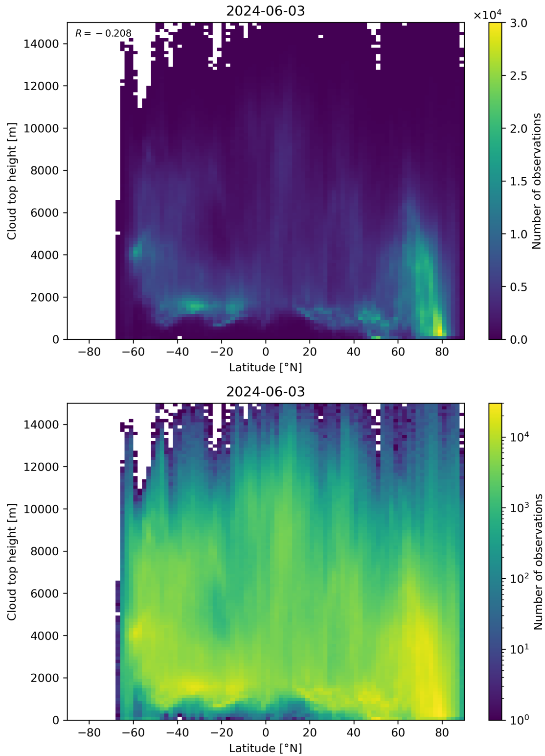
Figure 97: Scatter density plot of “Latitude” against “Cloud top height” for 2024-06-03 to 2024-06-04.
