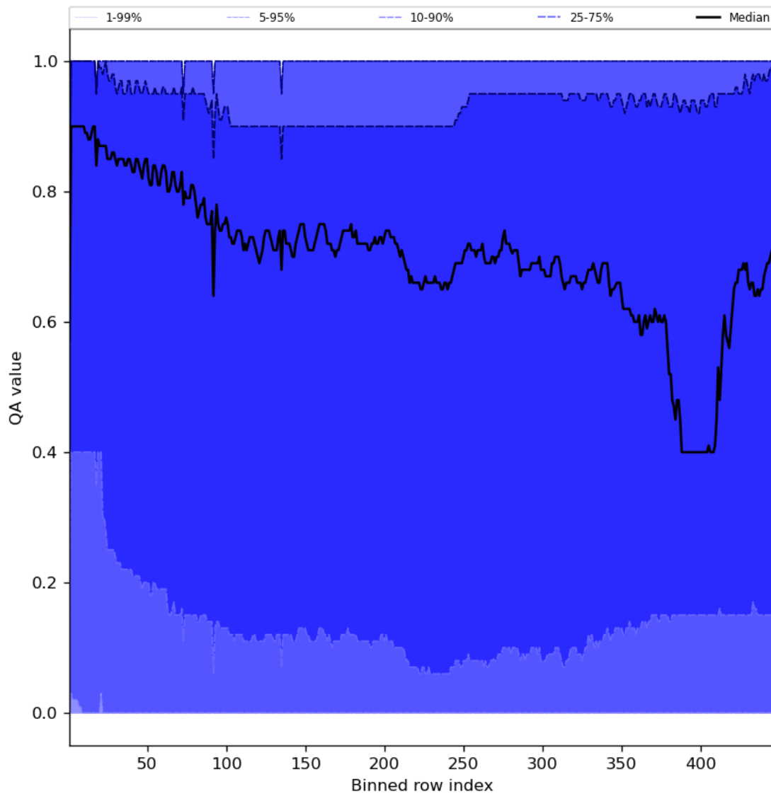
Figure 54: Along track statistics of “QA value” for 2024-06-03 to 2024-06-04
