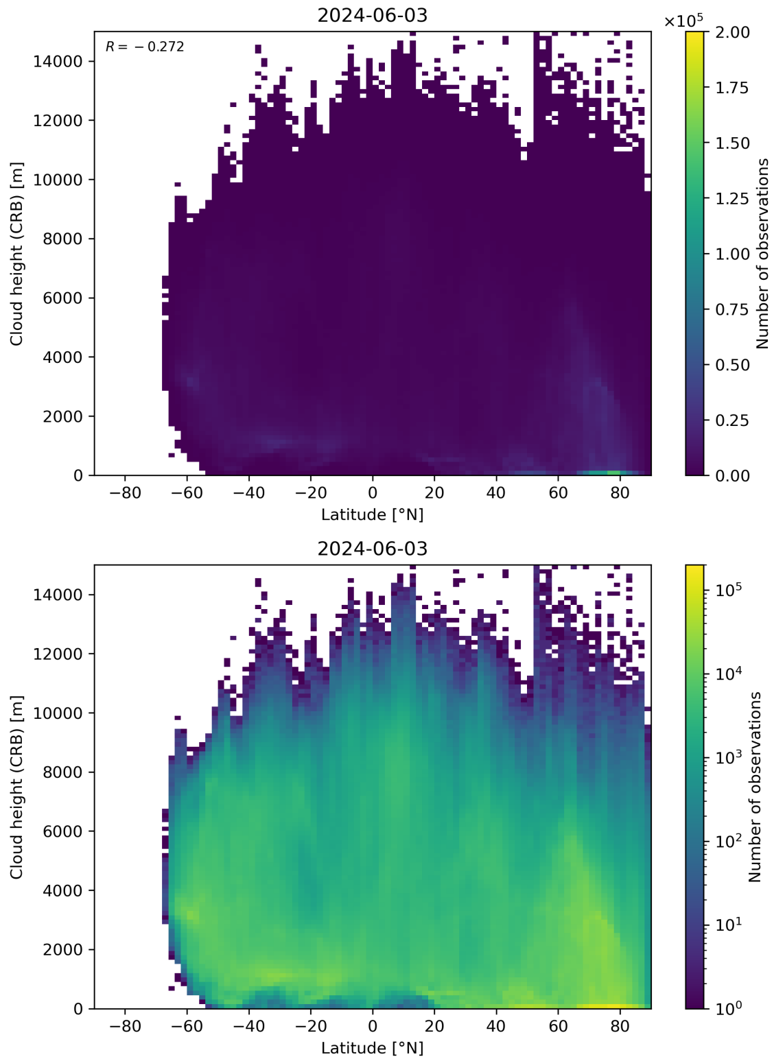
Figure 95: Scatter density plot of “Latitude” against “Cloud height (CRB)” for 2024-06-03 to 2024-06-04.
