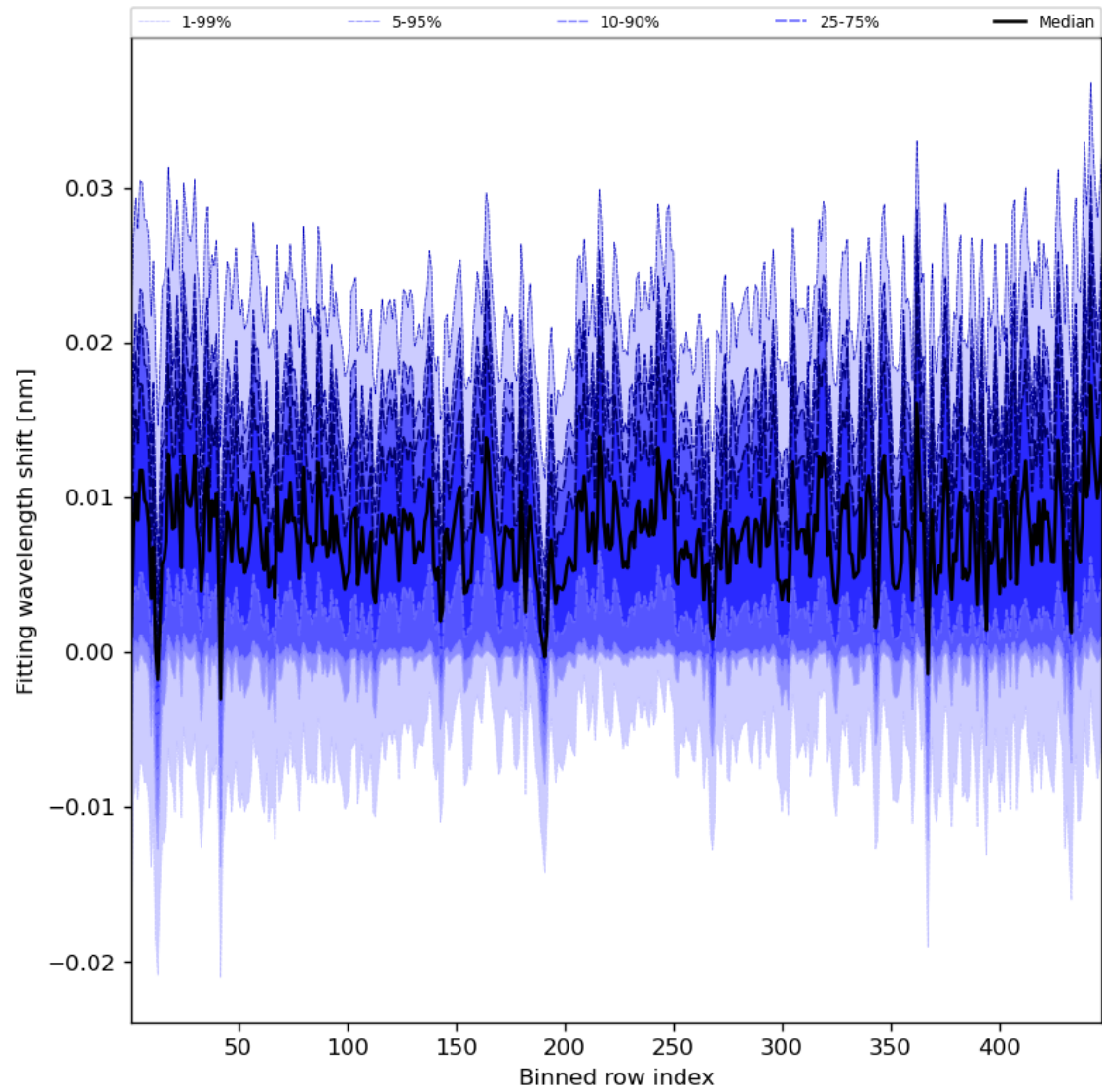
Figure 65: Along track statistics of “Fitting wavelength shift” for 2024-06-03 to 2024-06-04
