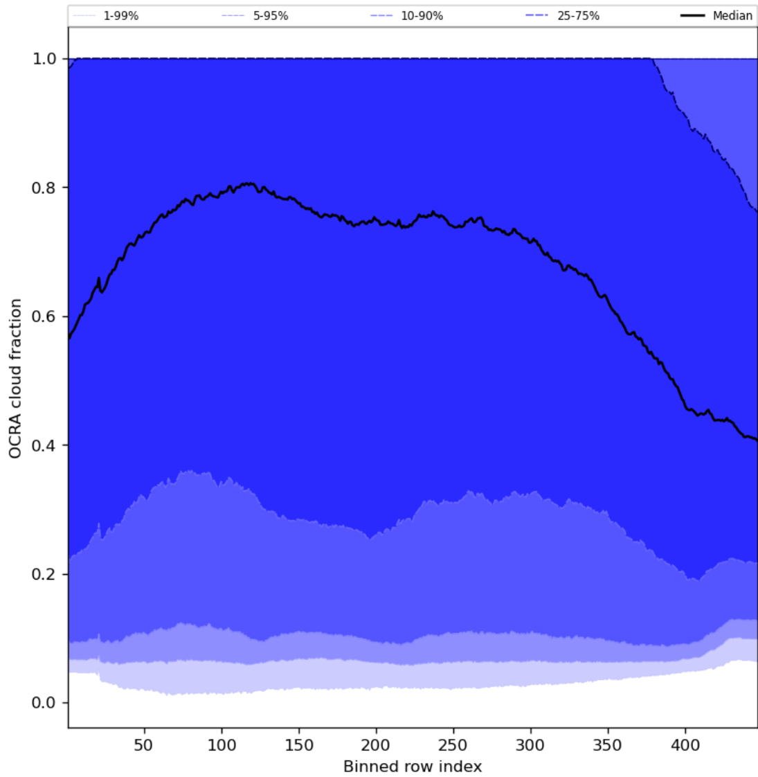
Figure 66: Along track statistics of “OCRA cloud fraction” for 2024-06-03 to 2024-06-04
