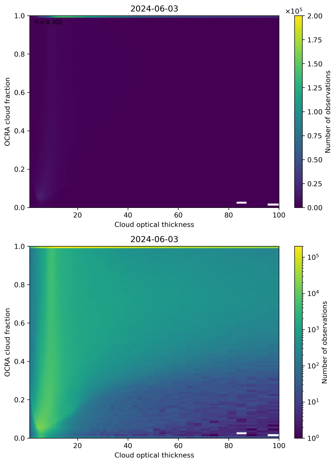
Figure 83: Scatter density plot of “Cloud optical thickness” against “OCRA cloud fraction” for 2024-06-03 to 2024-06-04.
