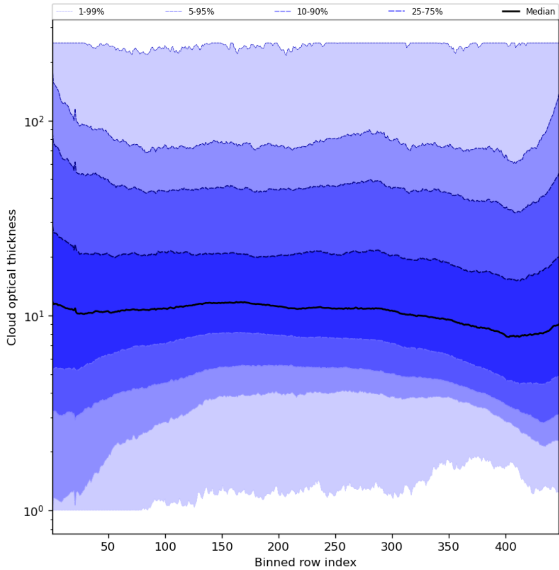
Figure 57: Along track statistics of “Cloud optical thickness” for 2024-06-03 to 2024-06-04
