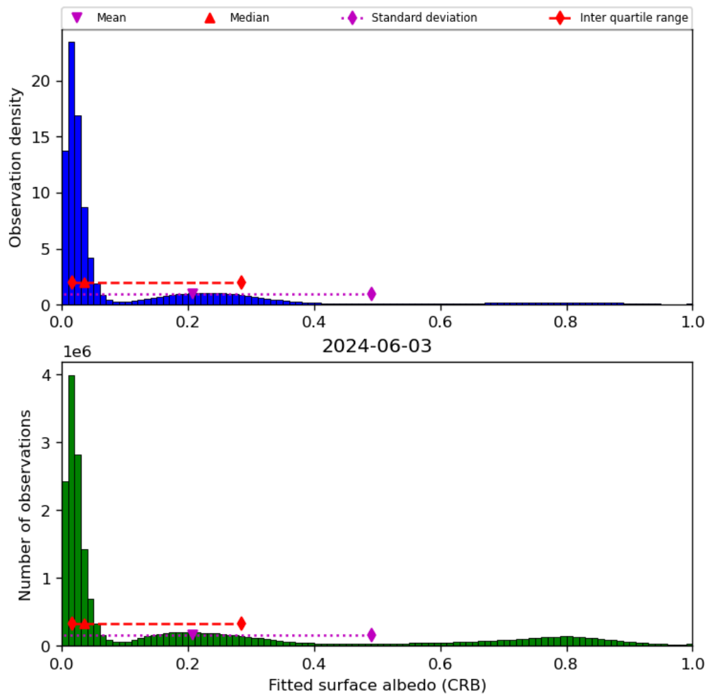
Figure 46: Histogram of “Fitted surface albedo (CRB)” for 2024-06-03 to 2024-06-04
