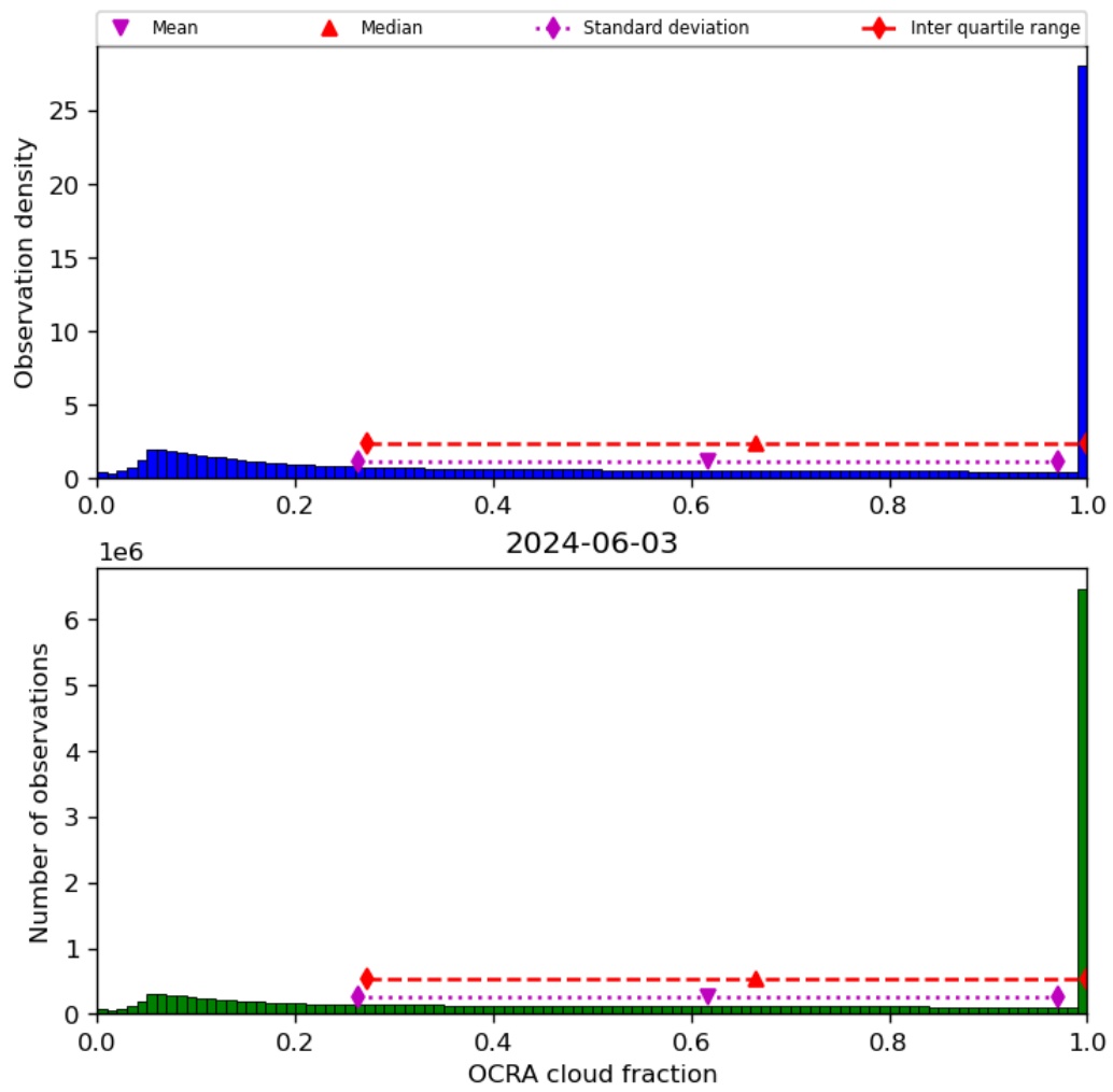
Figure 50: Histogram of “OCRA cloud fraction” for 2024-06-03 to 2024-06-04
