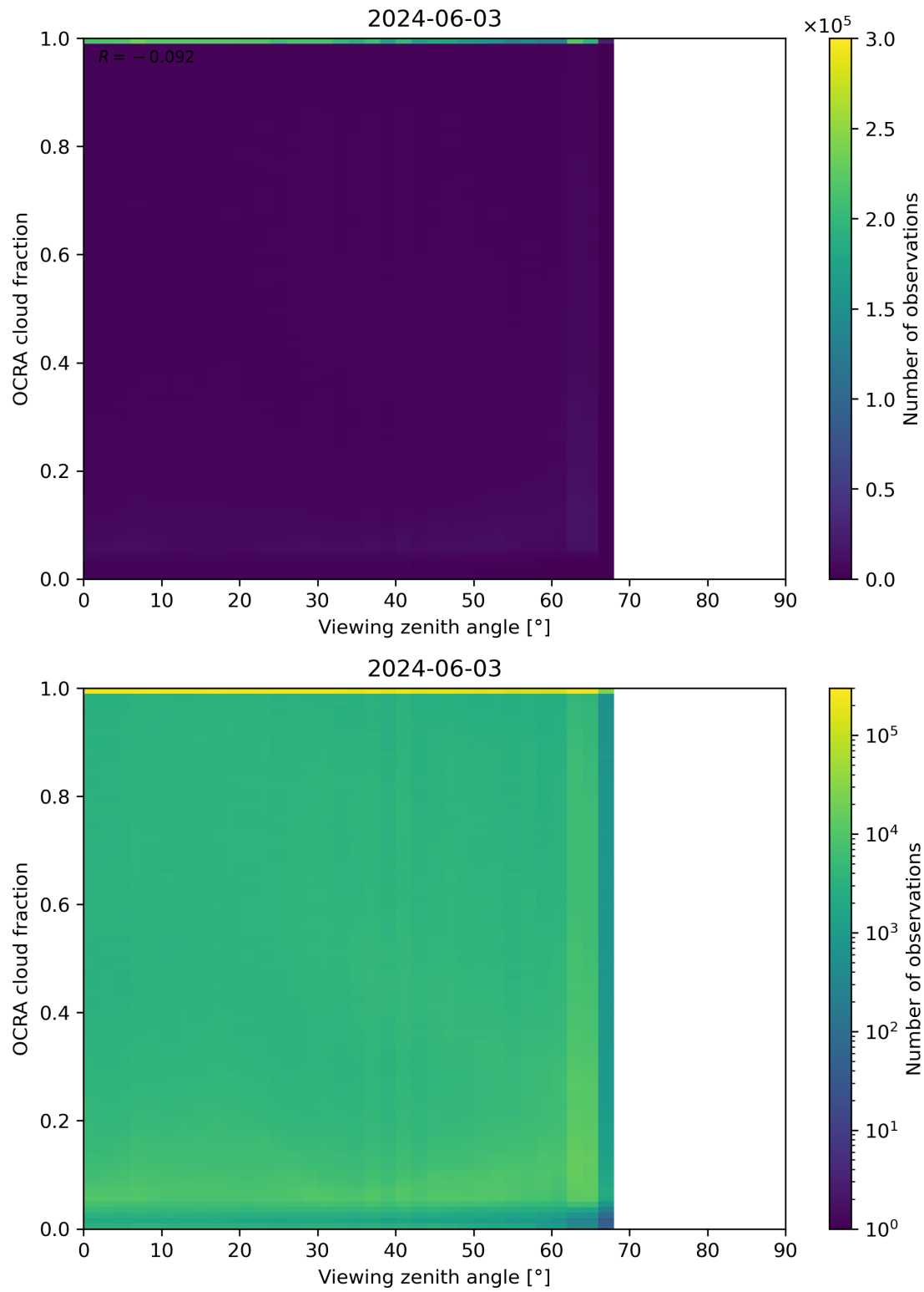
Figure 108: Scatter density plot of “Viewing zenith angle” against “OCRA cloud fraction” for 2024-06-03 to 2024-06-04.
