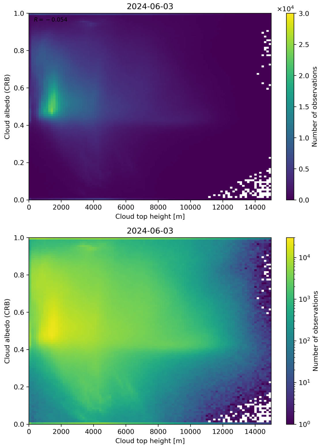
Figure 86: Scatter density plot of “Cloud top height” against “Cloud albedo (CRB)” for 2024-06-03 to 2024-06-04.
