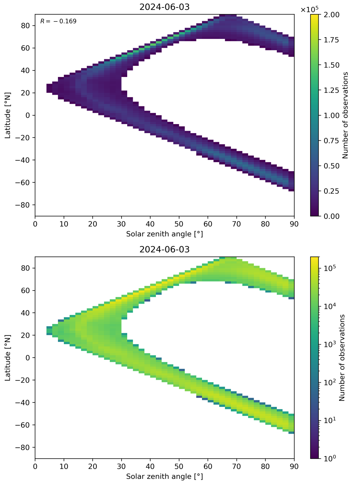
Figure 105: Scatter density plot of “Solar zenith angle” against “Latitude” for 2024-06-03 to 2024-06-04.
