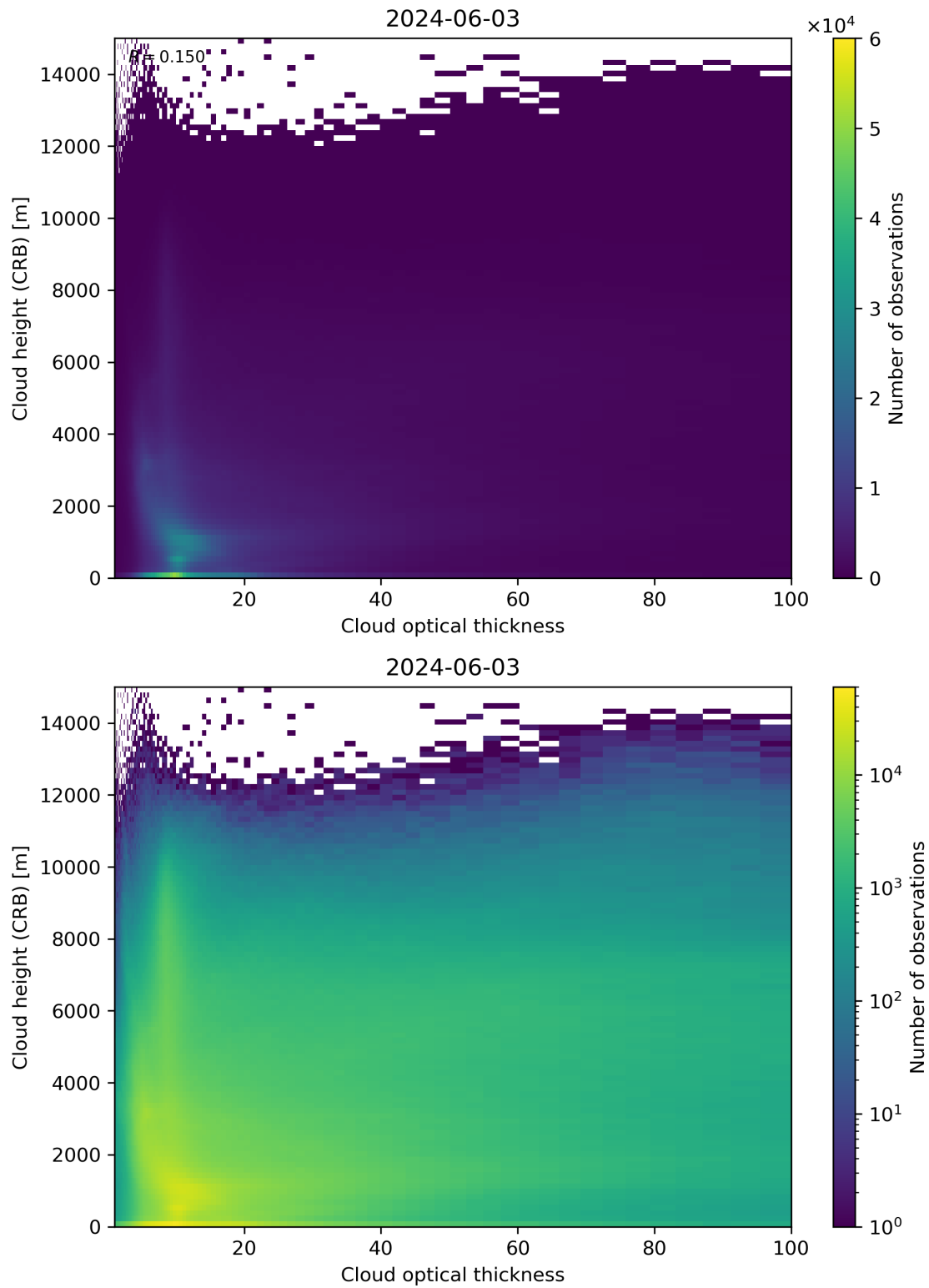
Figure 85: Scatter density plot of “Cloud optical thickness” against “Cloud height (CRB)” for 2024-06-03 to 2024-06-04.
