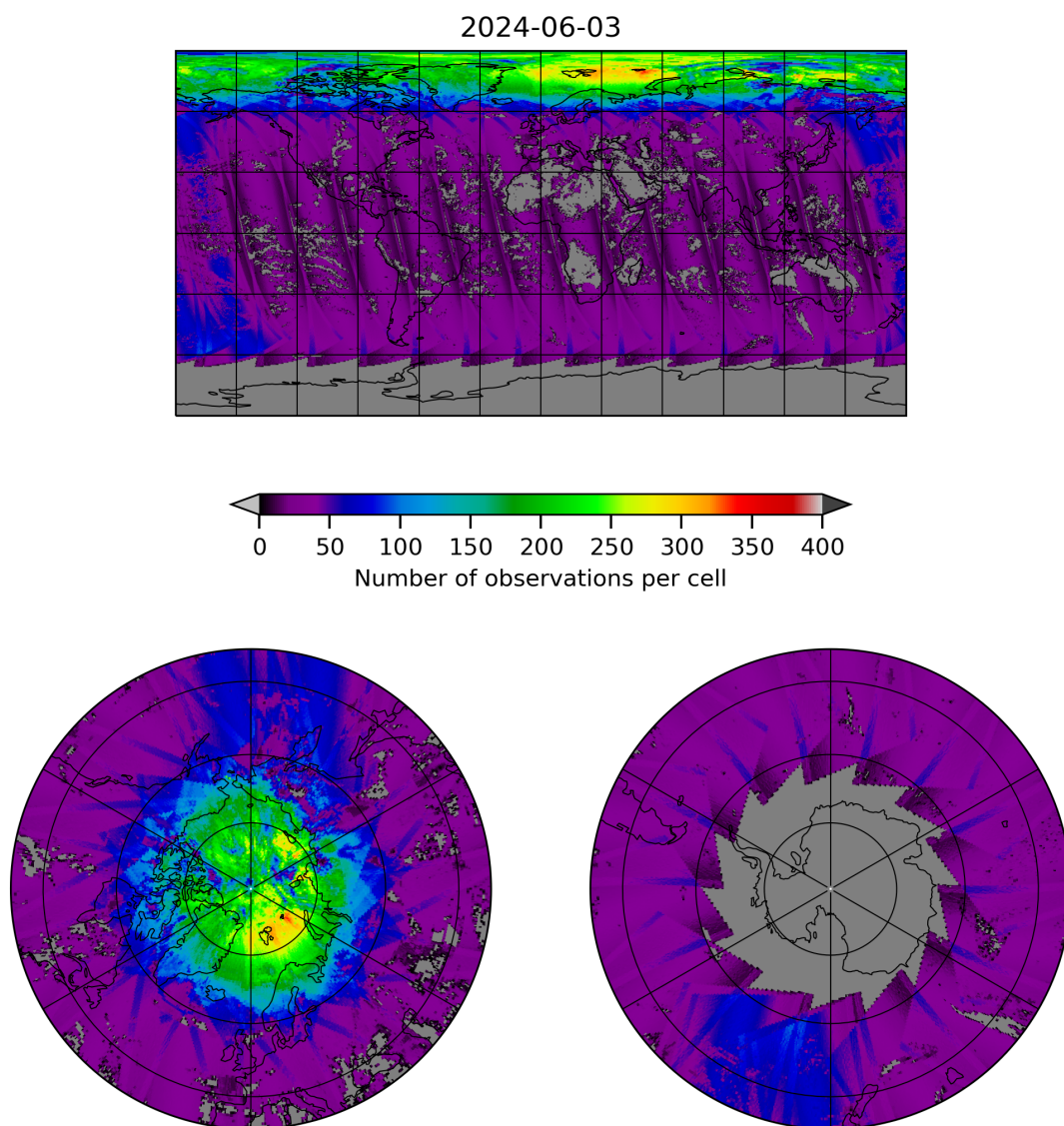
Figure 21: Map of the number of observations for 2024-06-03 to 2024-06-04
