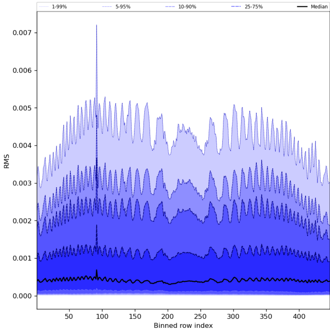
Figure 63: Along track statistics of “RMS” for 2024-06-03 to 2024-06-04
