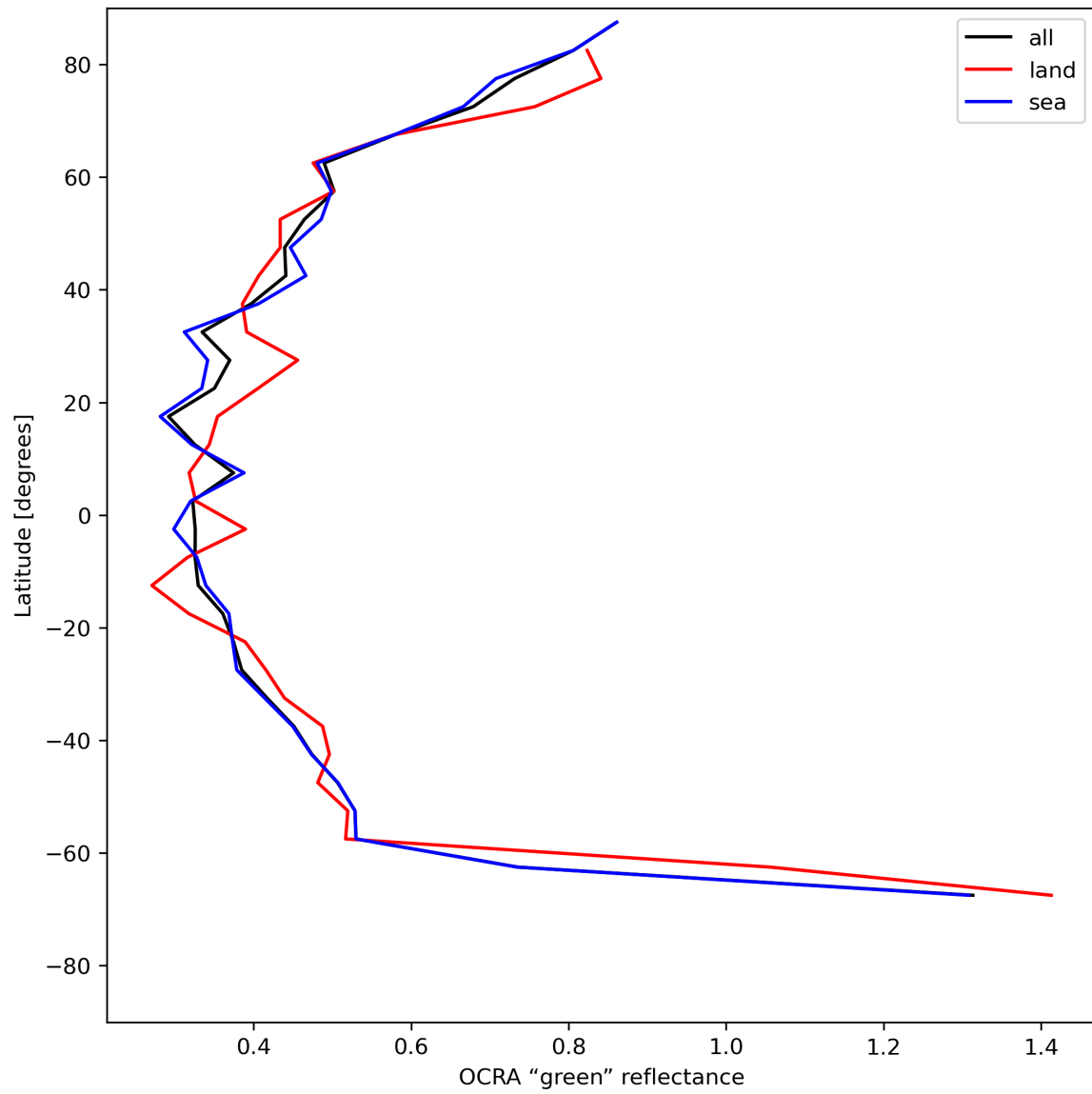
Figure 36: Zonal average of “OCRA “green” reflectance” for 2024-06-03 to 2024-06-04.
