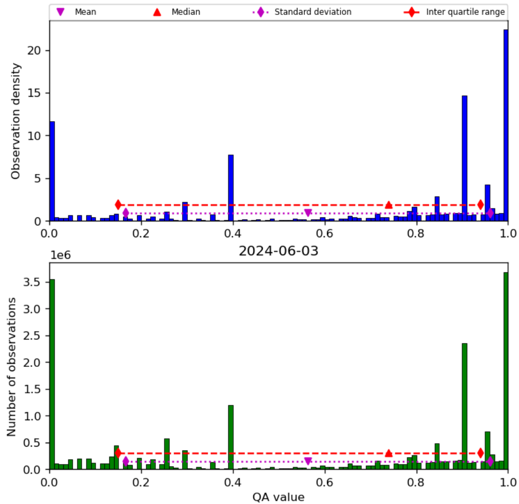
Figure 38: Histogram of “QA value” for 2024-06-03 to 2024-06-04
