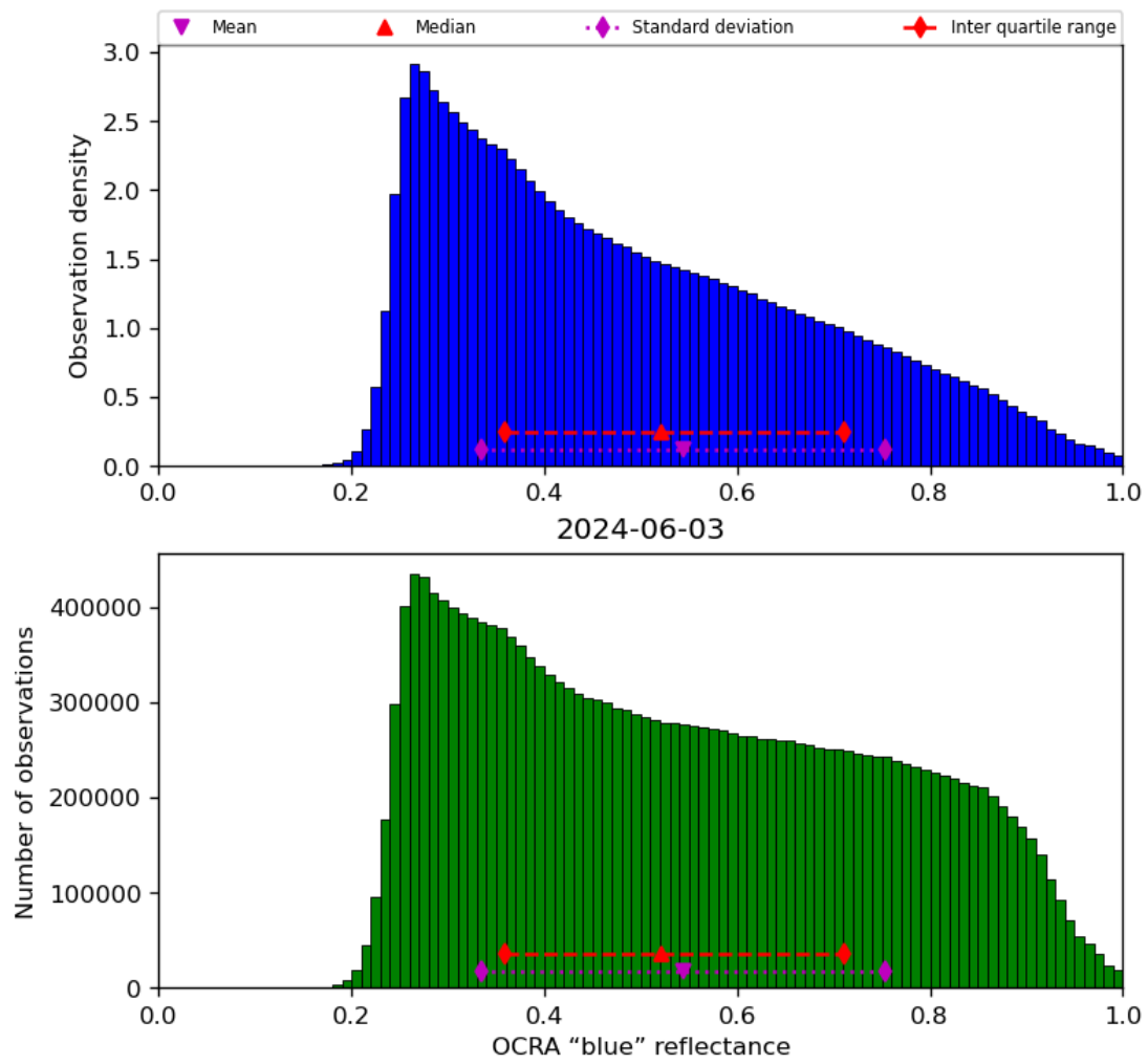
Figure 51: Histogram of “OCRA “blue” reflectance” for 2024-06-03 to 2024-06-04
