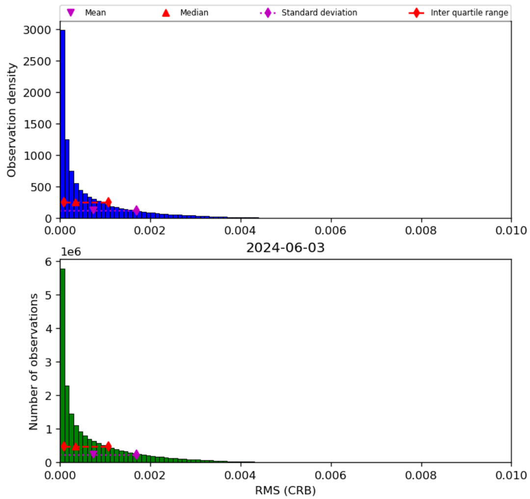
Figure 48: Histogram of “RMS (CRB)” for 2024-06-03 to 2024-06-04
