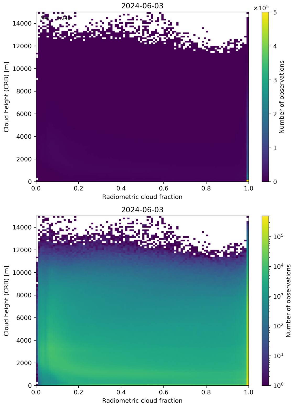
Figure 74: Scatter density plot of “Radiometric cloud fraction” against “Cloud height (CRB)” for 2024-06-03 to 2024-06-04.
