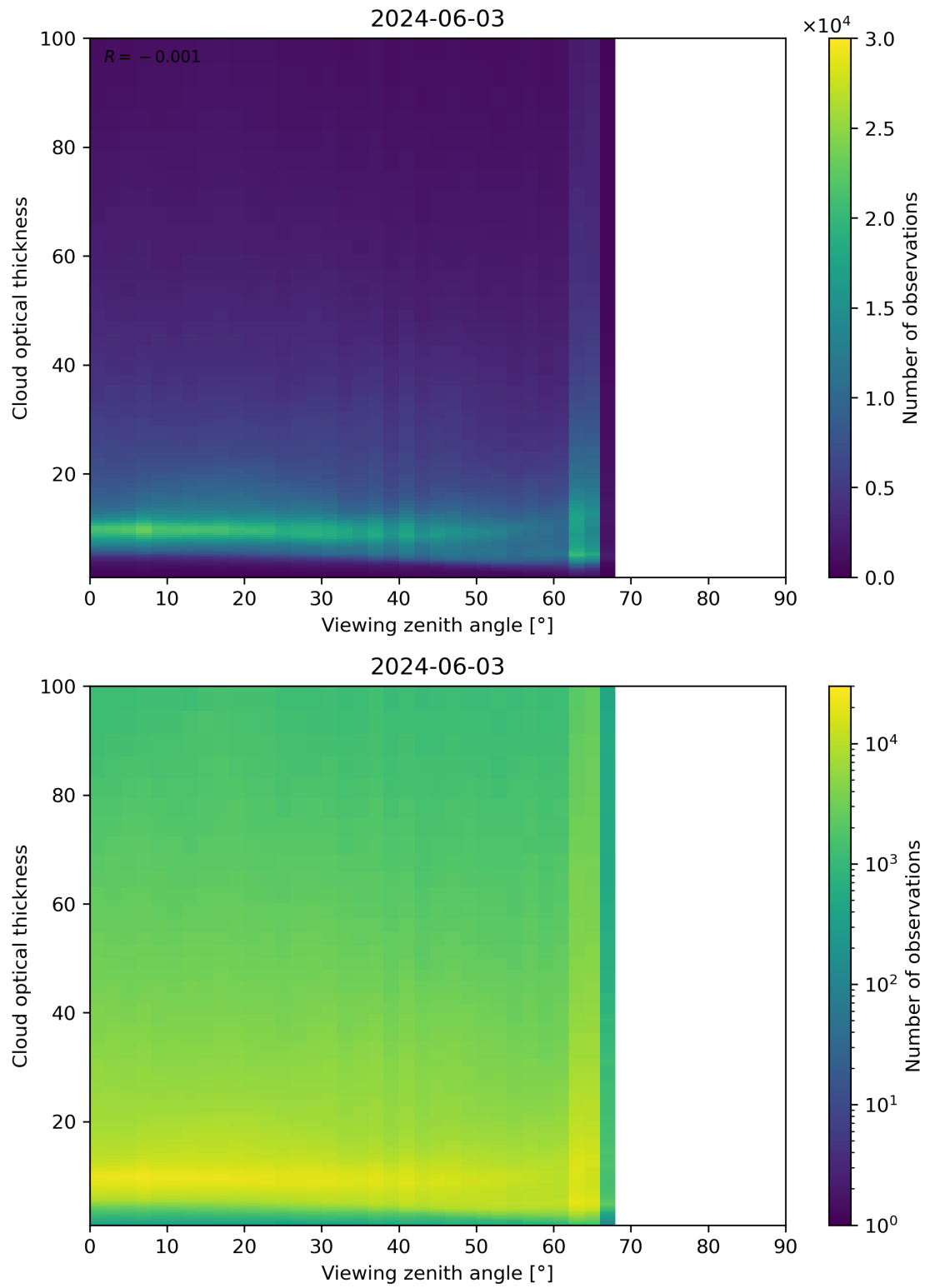
Figure 111: Scatter density plot of “Viewing zenith angle” against “Cloud optical thickness” for 2024-06-03 to 2024-06-04.
