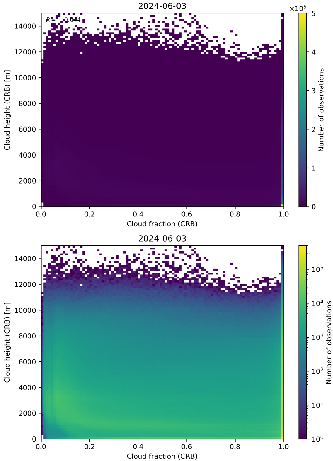
Figure 79: Scatter density plot of “Cloud fraction (CRB)” against “Cloud height (CRB)” for 2024-06-03 to 2024-06-04.
