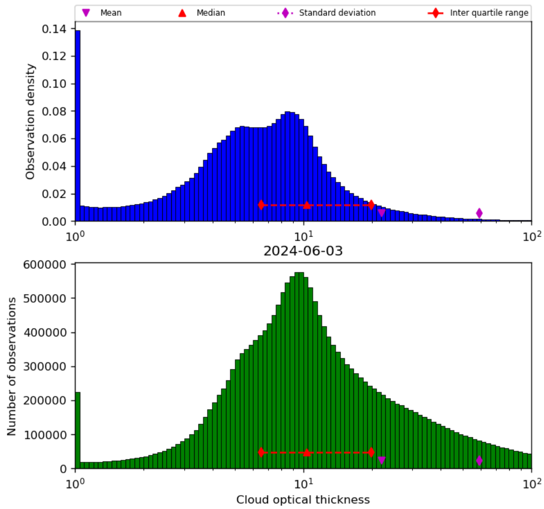
Figure 41: Histogram of “Cloud optical thickness” for 2024-06-03 to 2024-06-04
