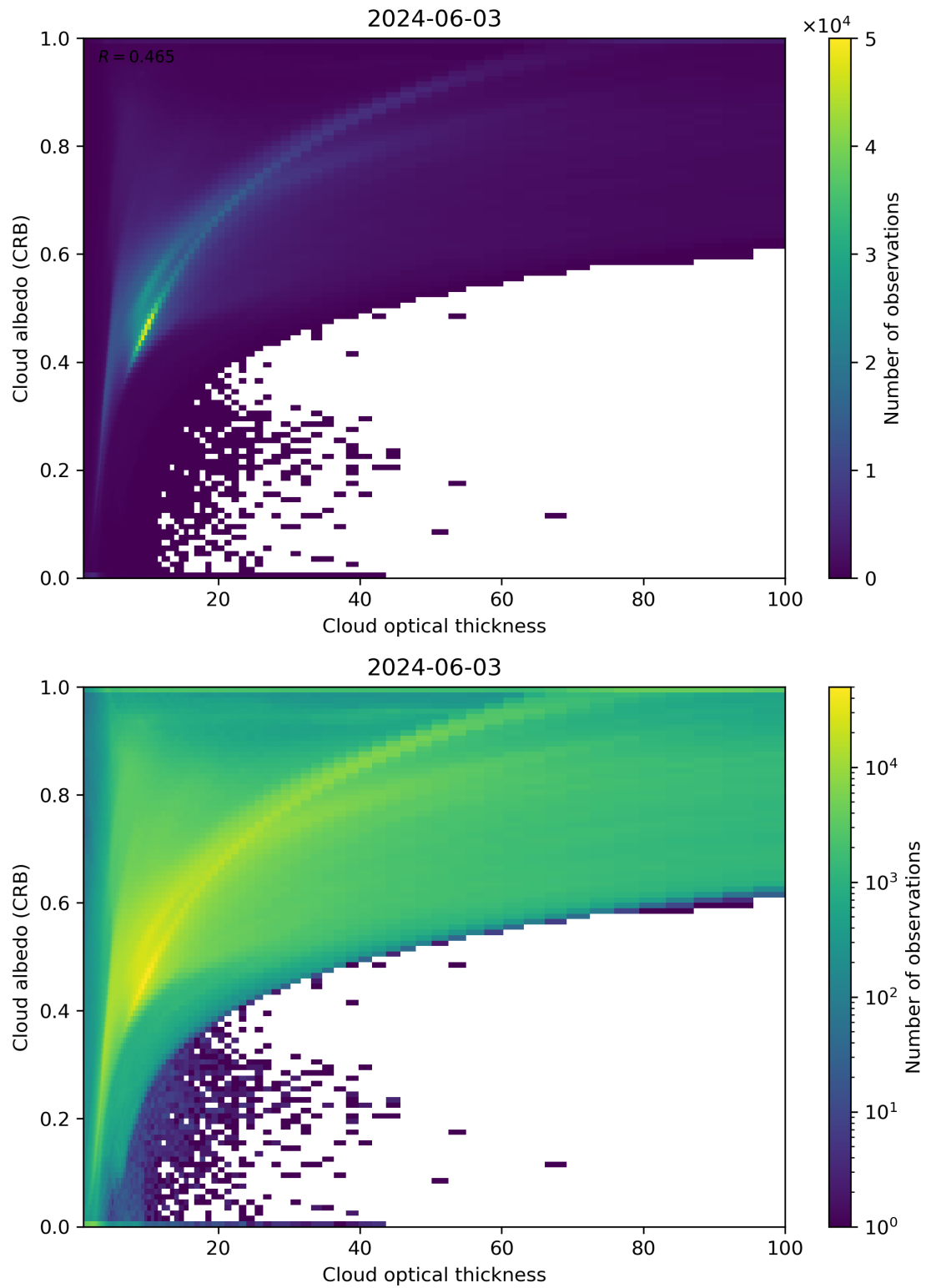
Figure 82: Scatter density plot of “Cloud optical thickness” against “Cloud albedo (CRB)” for 2024-06-03 to 2024-06-04.
