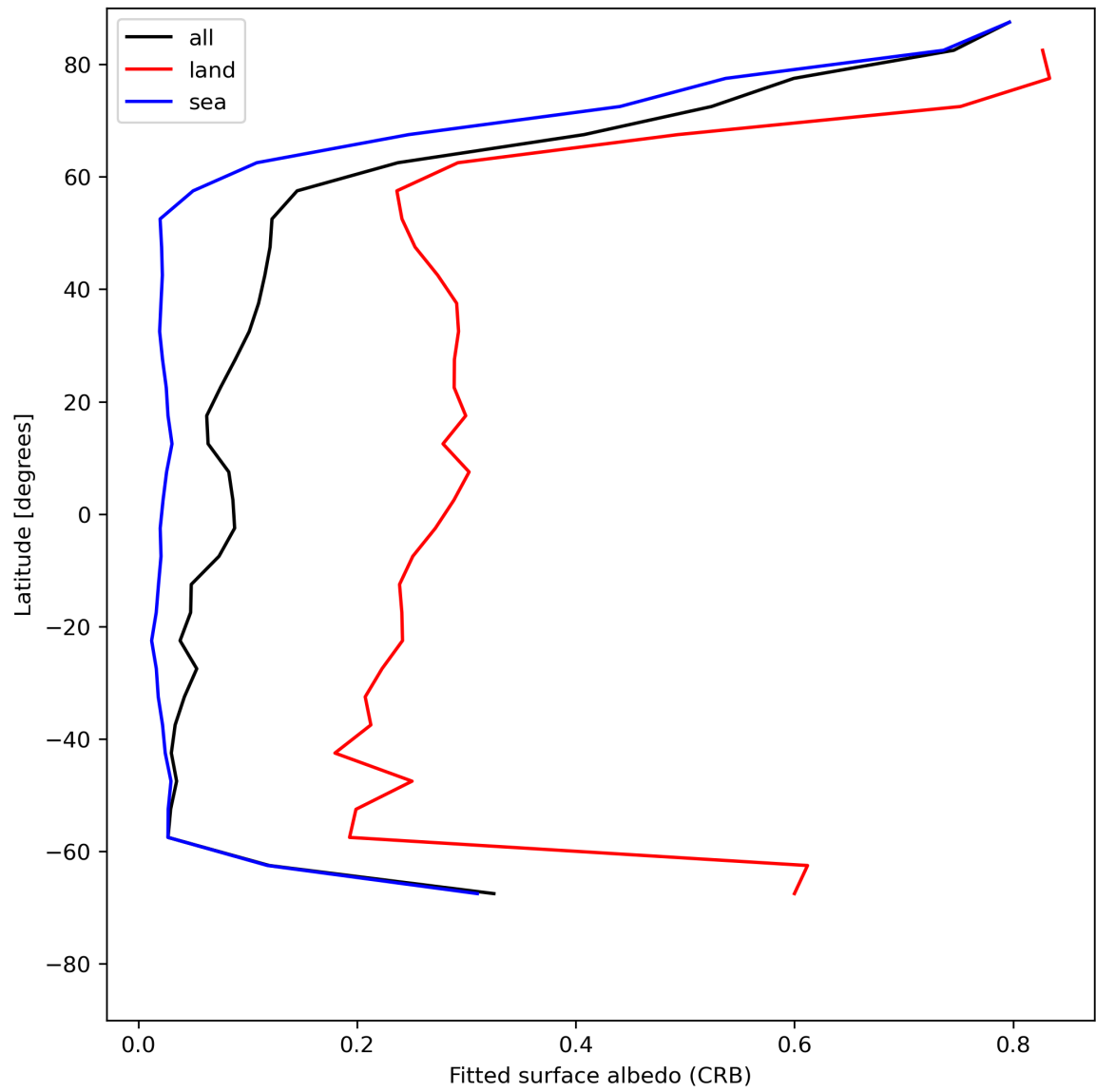
Figure 30: Zonal average of “Fitted surface albedo (CRB)” for 2024-06-03 to 2024-06-04.
