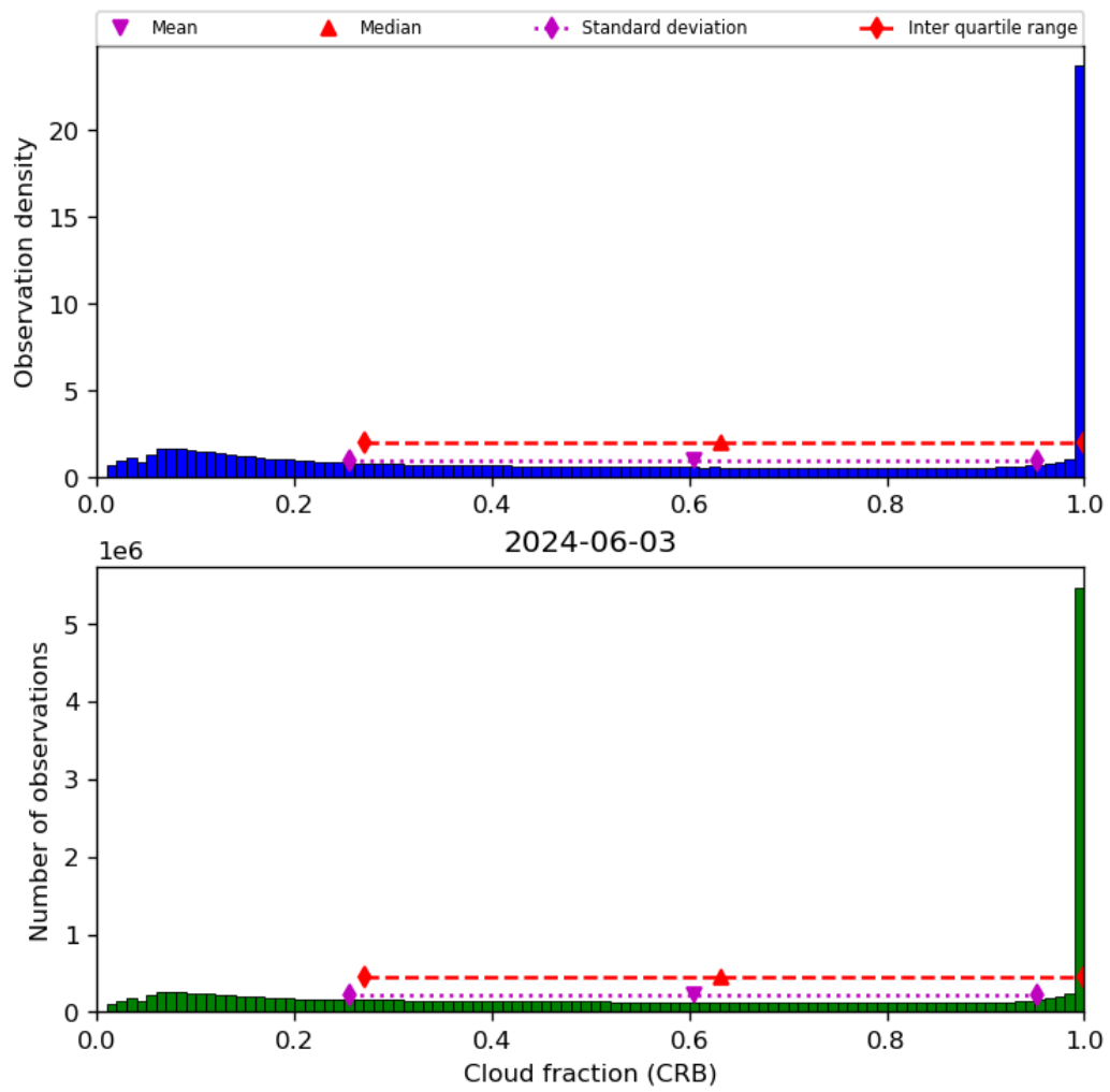
Figure 42: Histogram of “Cloud fraction (CRB)” for 2024-06-03 to 2024-06-04
