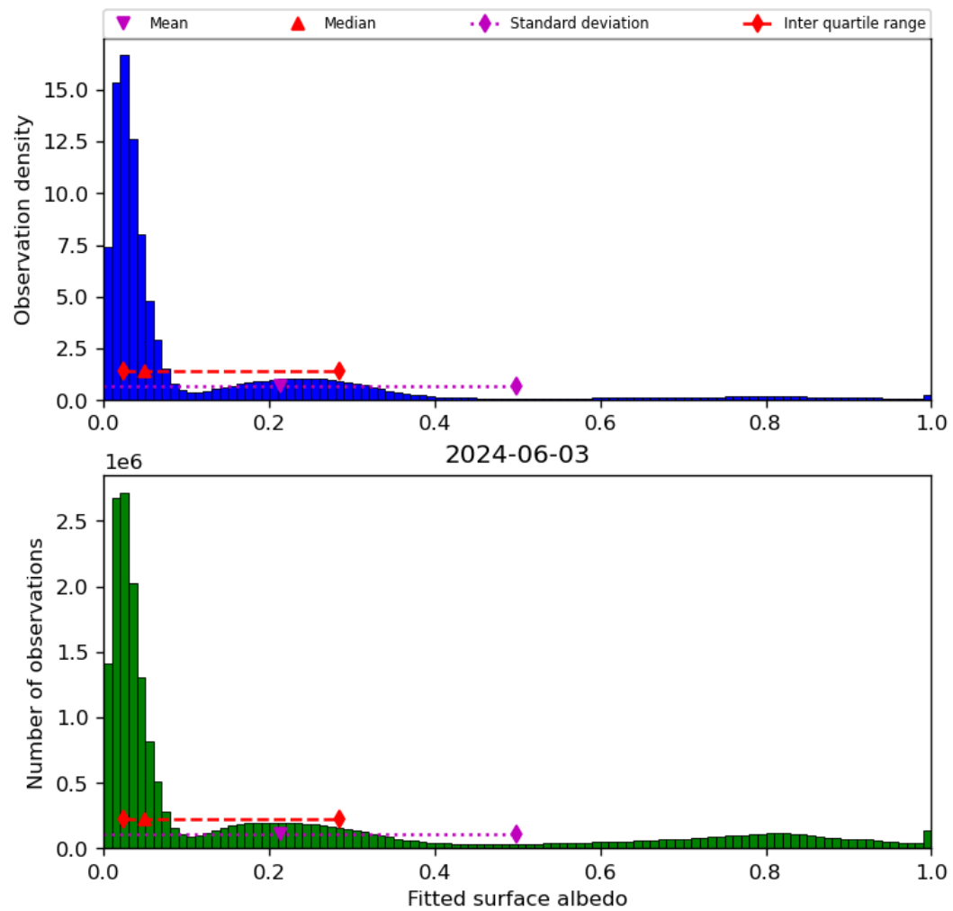
Figure 45: Histogram of “Fitted surface albedo” for 2024-06-03 to 2024-06-04
