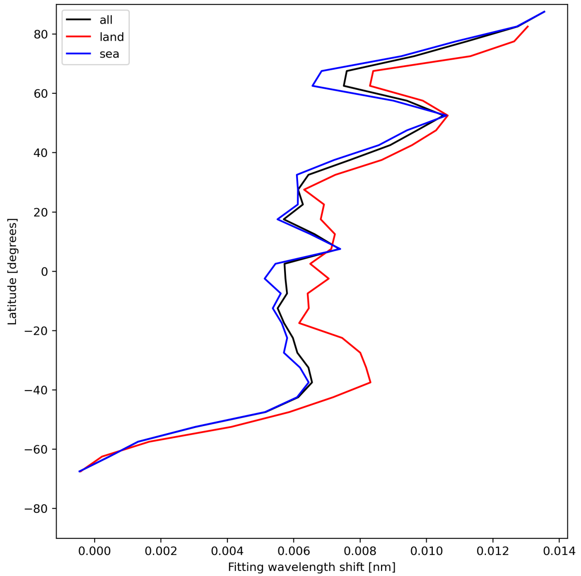
Figure 33: Zonal average of “Fitting wavelength shift” for 2024-06-03 to 2024-06-04.
