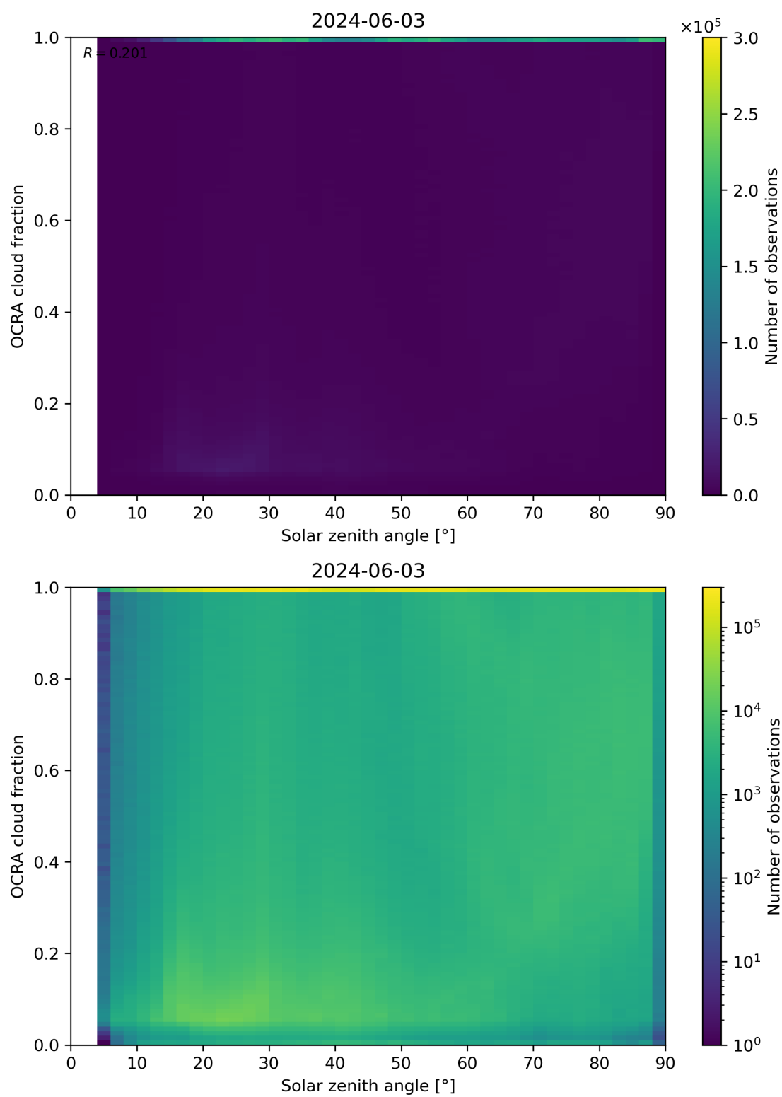
Figure 100: Scatter density plot of “Solar zenith angle” against “OCRA cloud fraction” for 2024-06-03 to 2024-06-04.
