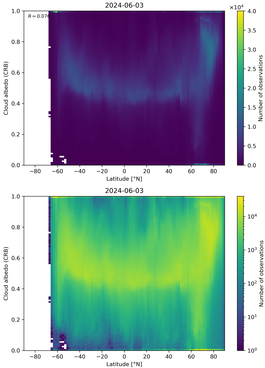
Figure 91: Scatter density plot of “Latitude” against “Cloud albedo (CRB)” for 2024-06-03 to 2024-06-04.
