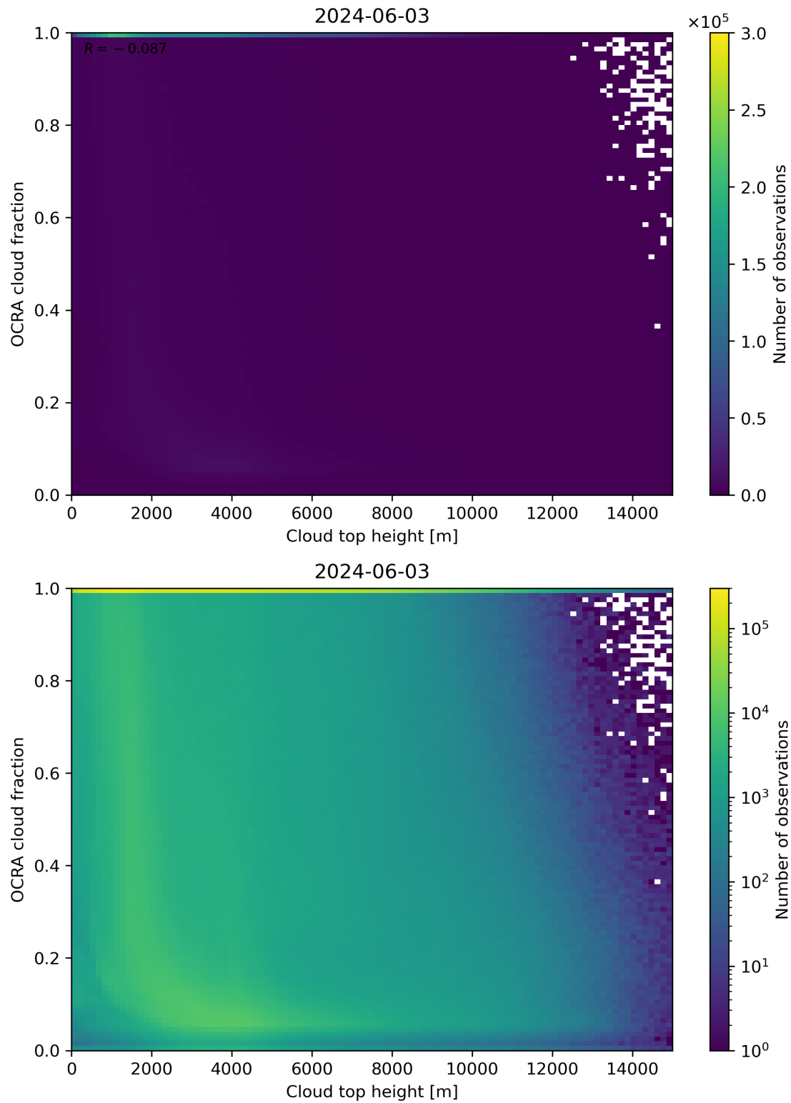
Figure 87: Scatter density plot of “Cloud top height” against “OCRA cloud fraction” for 2024-06-03 to 2024-06-04.
