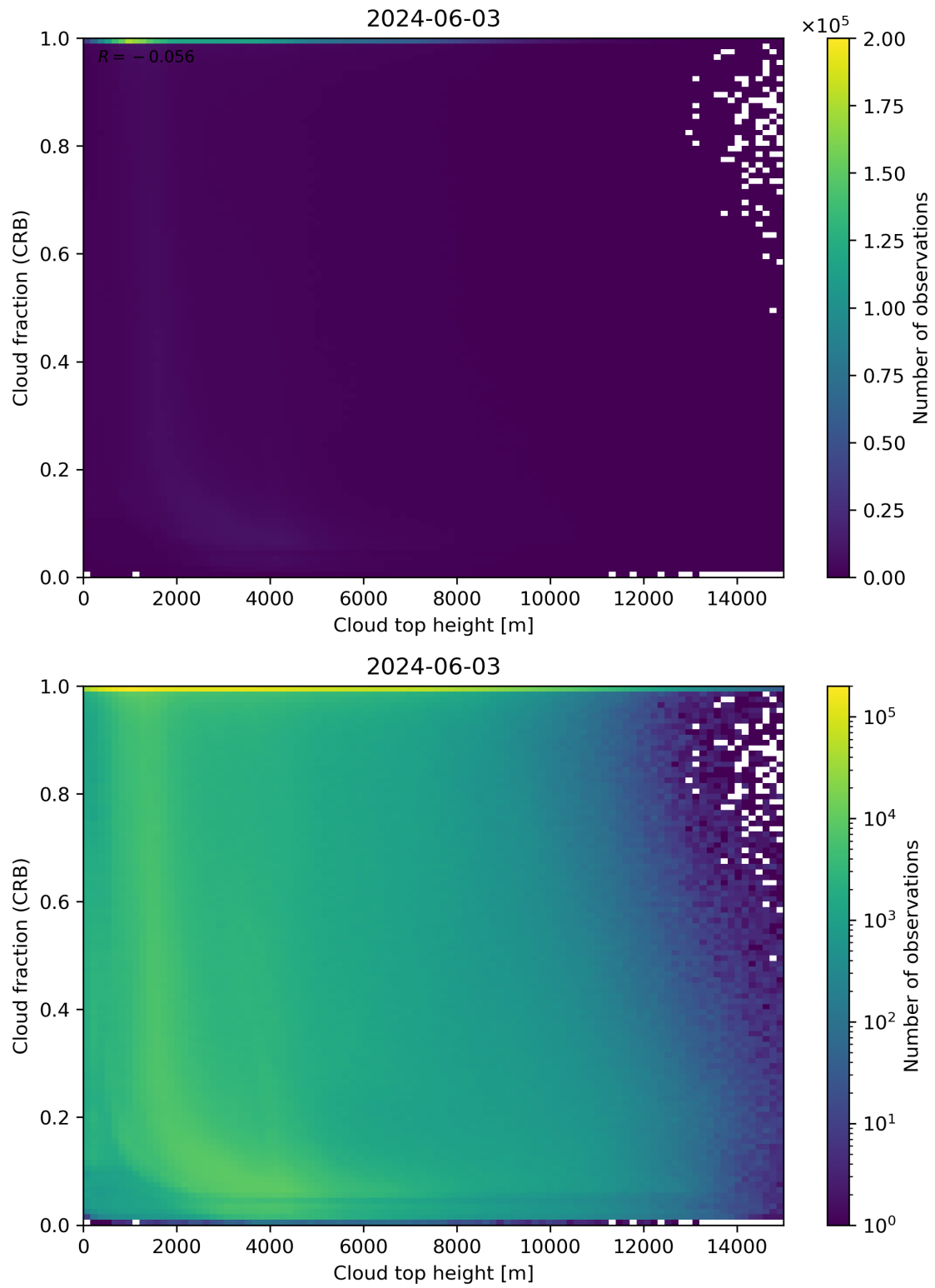
Figure 88: Scatter density plot of “Cloud top height” against “Cloud fraction (CRB)” for 2024-06-03 to 2024-06-04.
