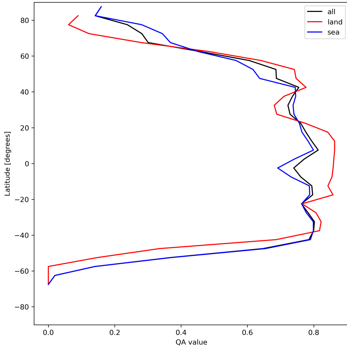
Figure 22: Zonal average of “QA value” for 2024-06-03 to 2024-06-04.
