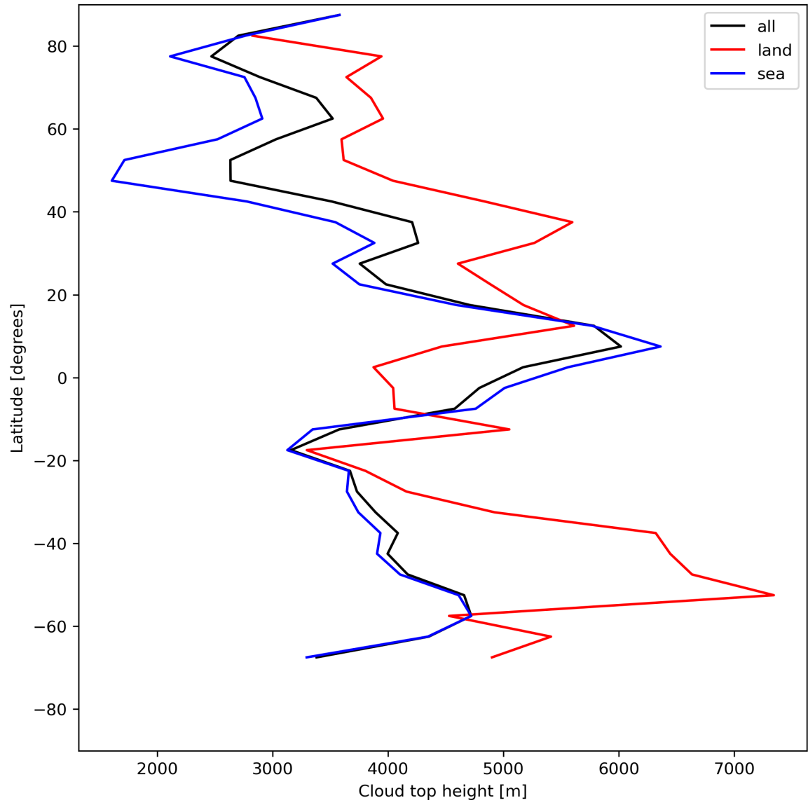
Figure 24: Zonal average of “Cloud top height” for 2024-06-03 to 2024-06-04.
