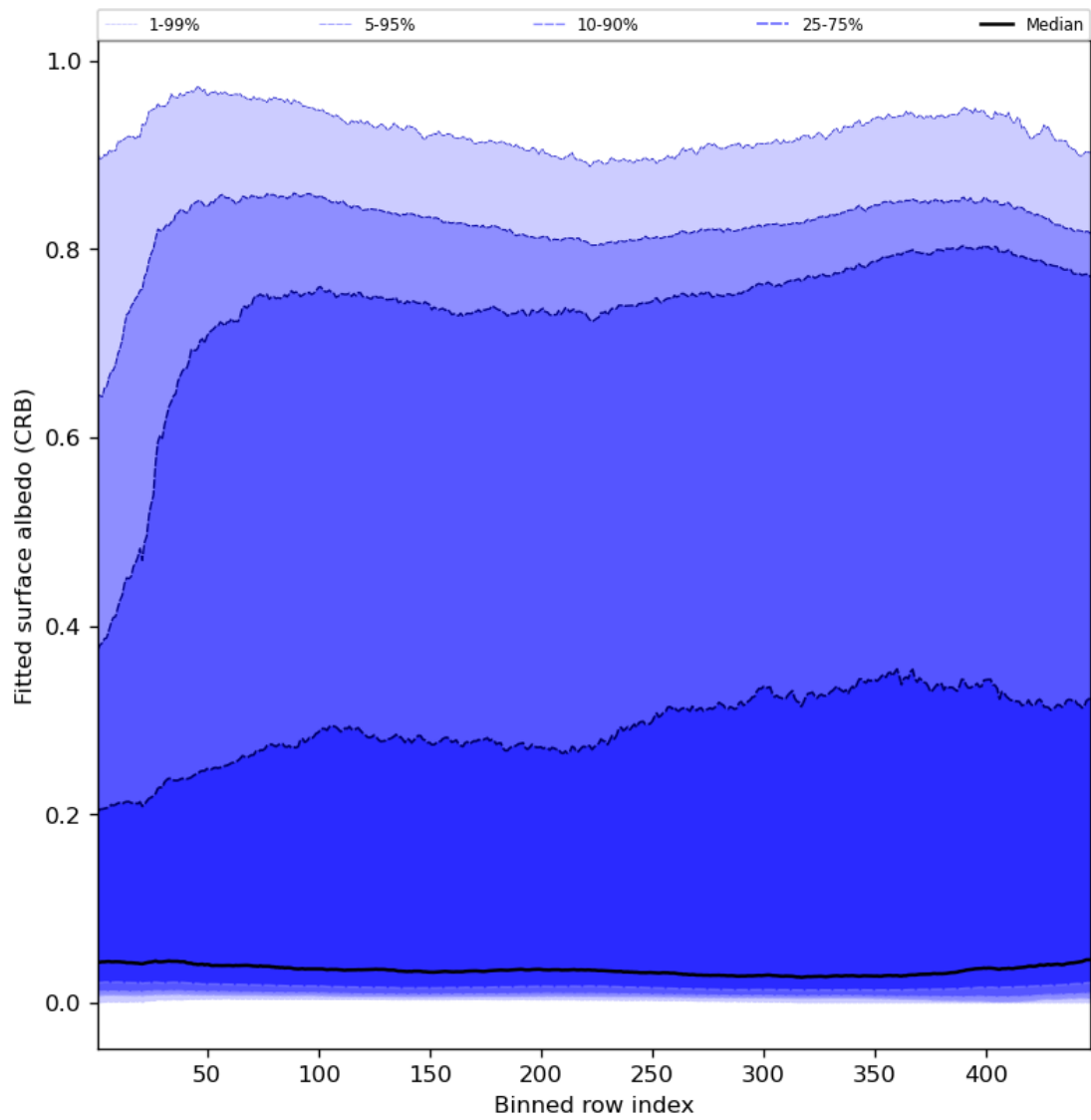
Figure 62: Along track statistics of “Fitted surface albedo (CRB)” for 2024-06-03 to 2024-06-04
