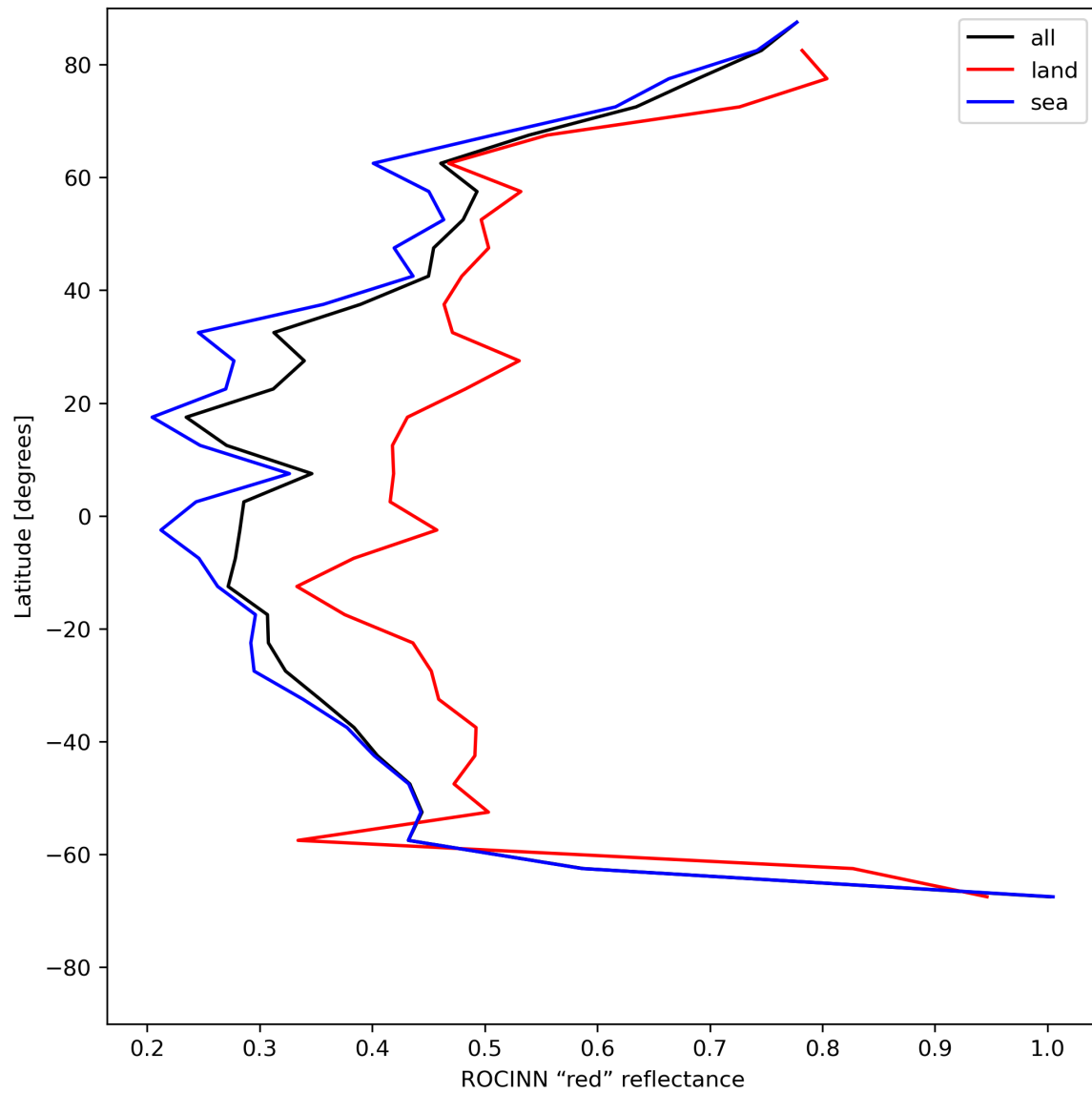
Figure 37: Zonal average of “ROCINN “red” reflectance” for 2024-06-03 to 2024-06-04.
