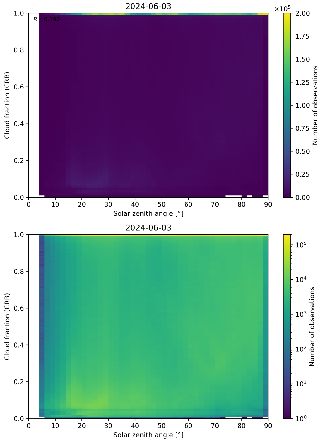
Figure 101: Scatter density plot of “Solar zenith angle” against “Cloud fraction (CRB)” for 2024-06-03 to 2024-06-04.
