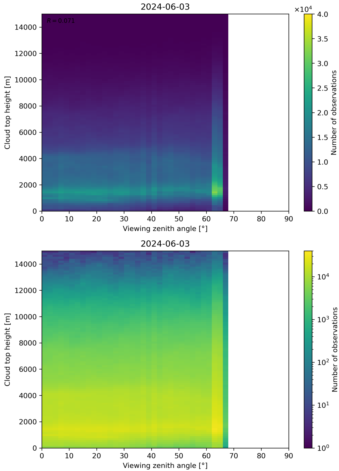
Figure 112: Scatter density plot of “Viewing zenith angle” against “Cloud top height” for 2024-06-03 to 2024-06-04.
