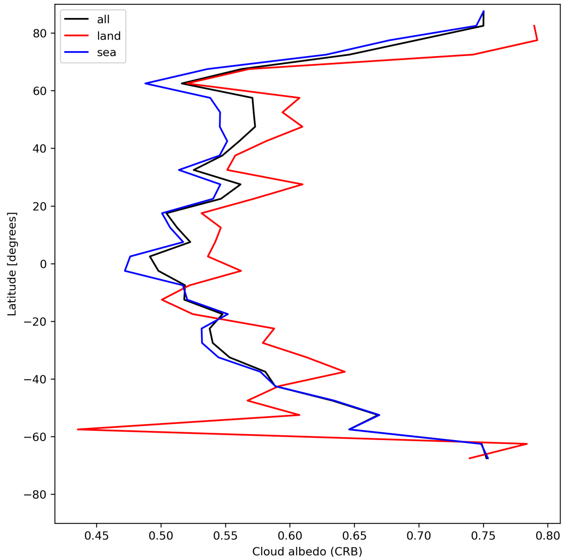
Figure 28: Zonal average of “Cloud albedo (CRB)” for 2024-06-03 to 2024-06-04.
