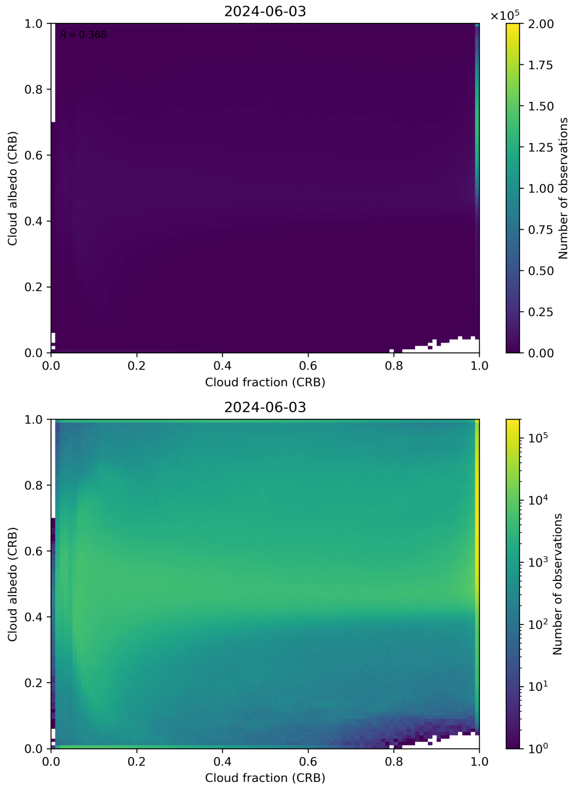
Figure 77: Scatter density plot of “Cloud fraction (CRB)” against “Cloud albedo (CRB)” for 2024-06-03 to 2024-06-04.
