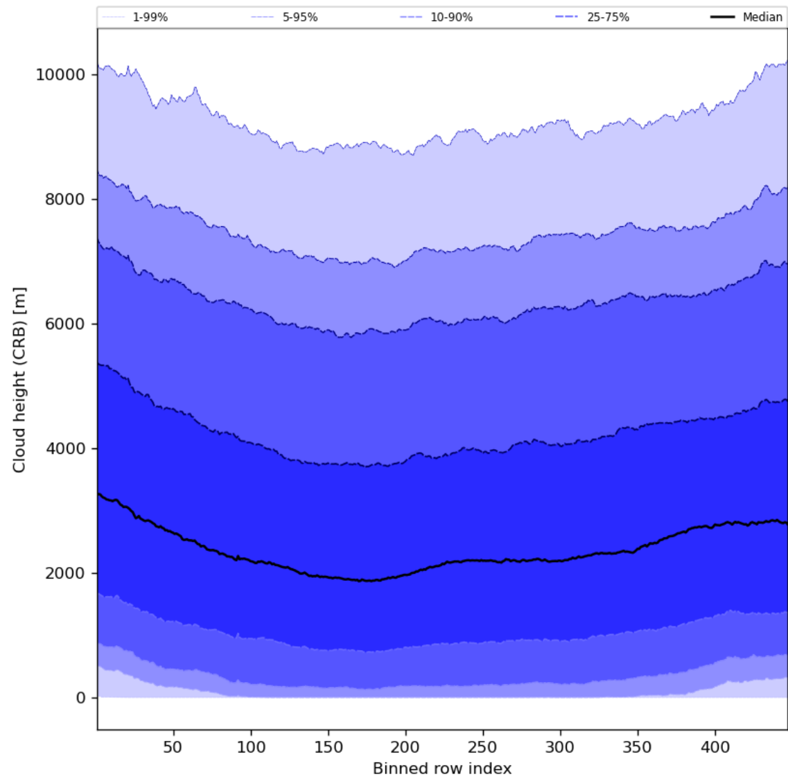
Figure 59: Along track statistics of “Cloud height (CRB)” for 2024-06-03 to 2024-06-04
