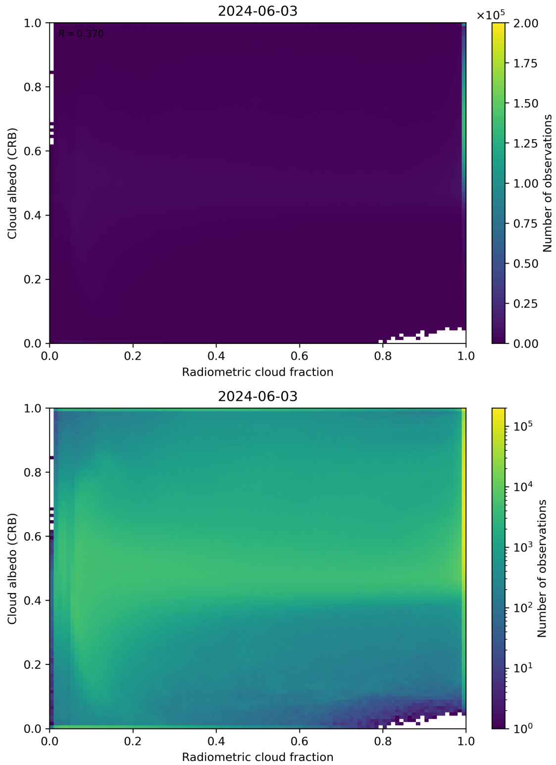
Figure 71: Scatter density plot of “Radiometric cloud fraction” against “Cloud albedo (CRB)” for 2024-06-03 to 2024-06-04.
