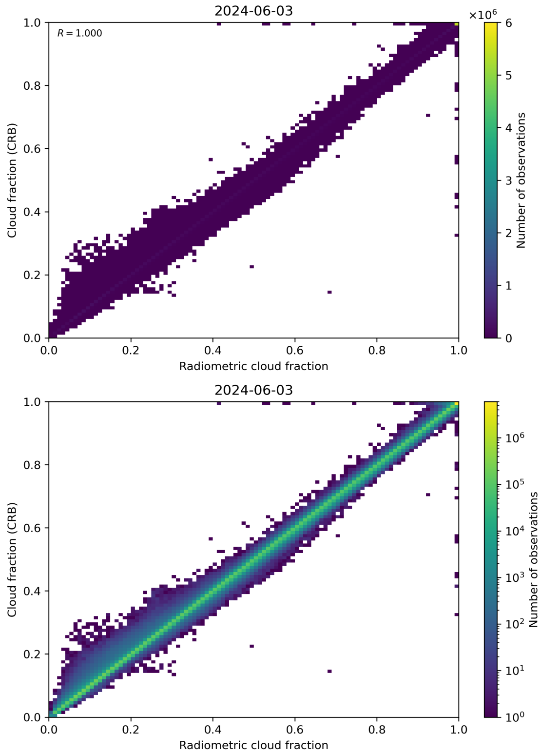
Figure 73: Scatter density plot of “Radiometric cloud fraction” against “Cloud fraction (CRB)” for 2024-06-03 to 2024-06-04.
