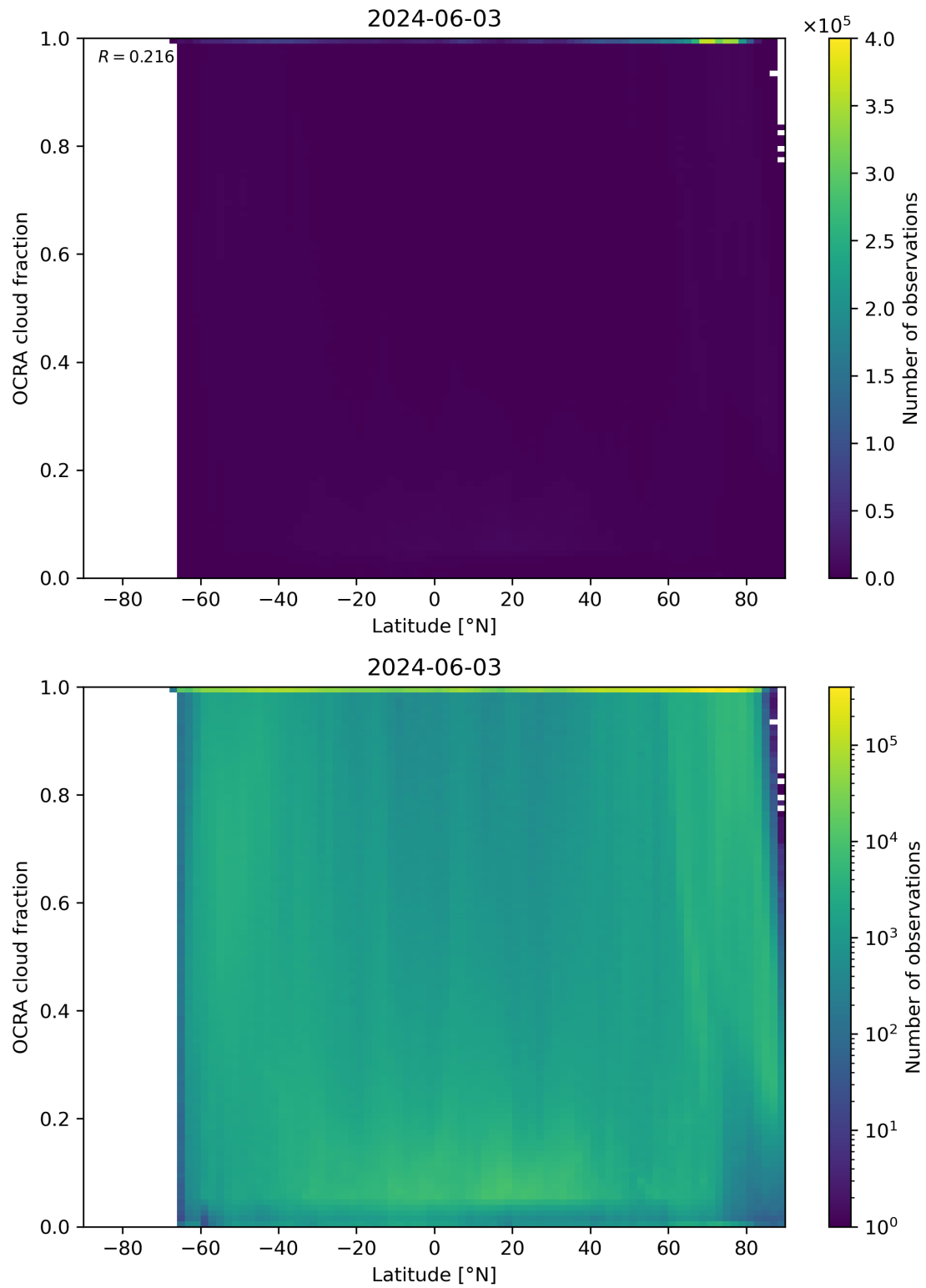
Figure 93: Scatter density plot of “Latitude” against “OCRA cloud fraction” for 2024-06-03 to 2024-06-04.
