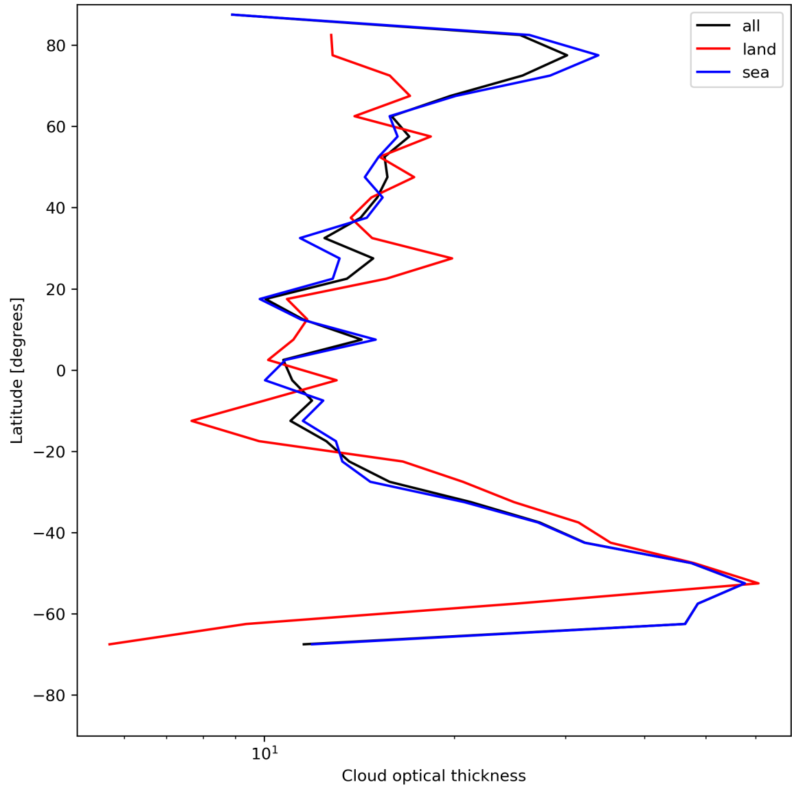
Figure 25: Zonal average of “Cloud optical thickness” for 2024-06-03 to 2024-06-04.
