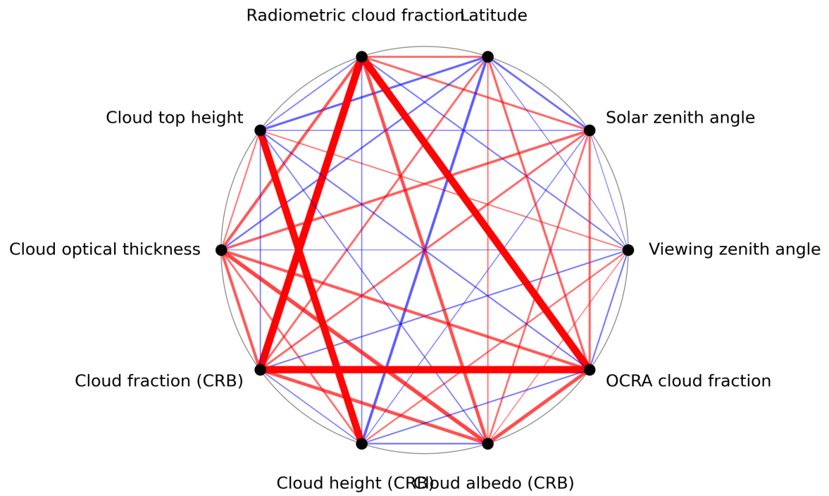
Figure 1: Map of correlation graph for 2024-06-03 to 2024-06-04.
