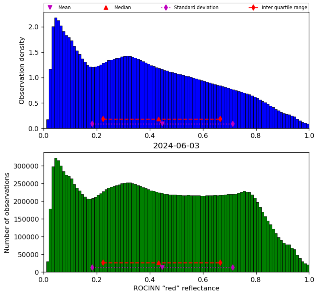
Figure 53: Histogram of “ROCINN “red” reflectance” for 2024-06-03 to 2024-06-04
