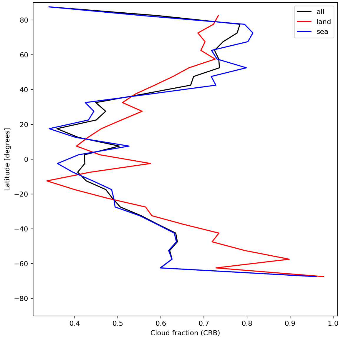
Figure 26: Zonal average of “Cloud fraction (CRB)” for 2024-06-03 to 2024-06-04.
