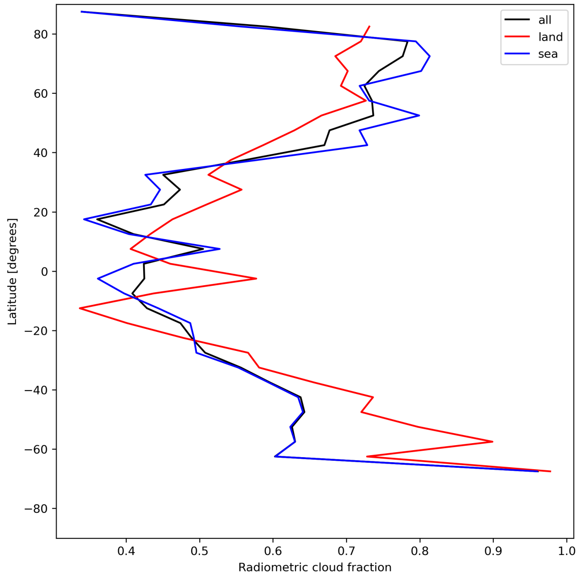
Figure 23: Zonal average of “Radiometric cloud fraction” for 2024-06-03 to 2024-06-04.
