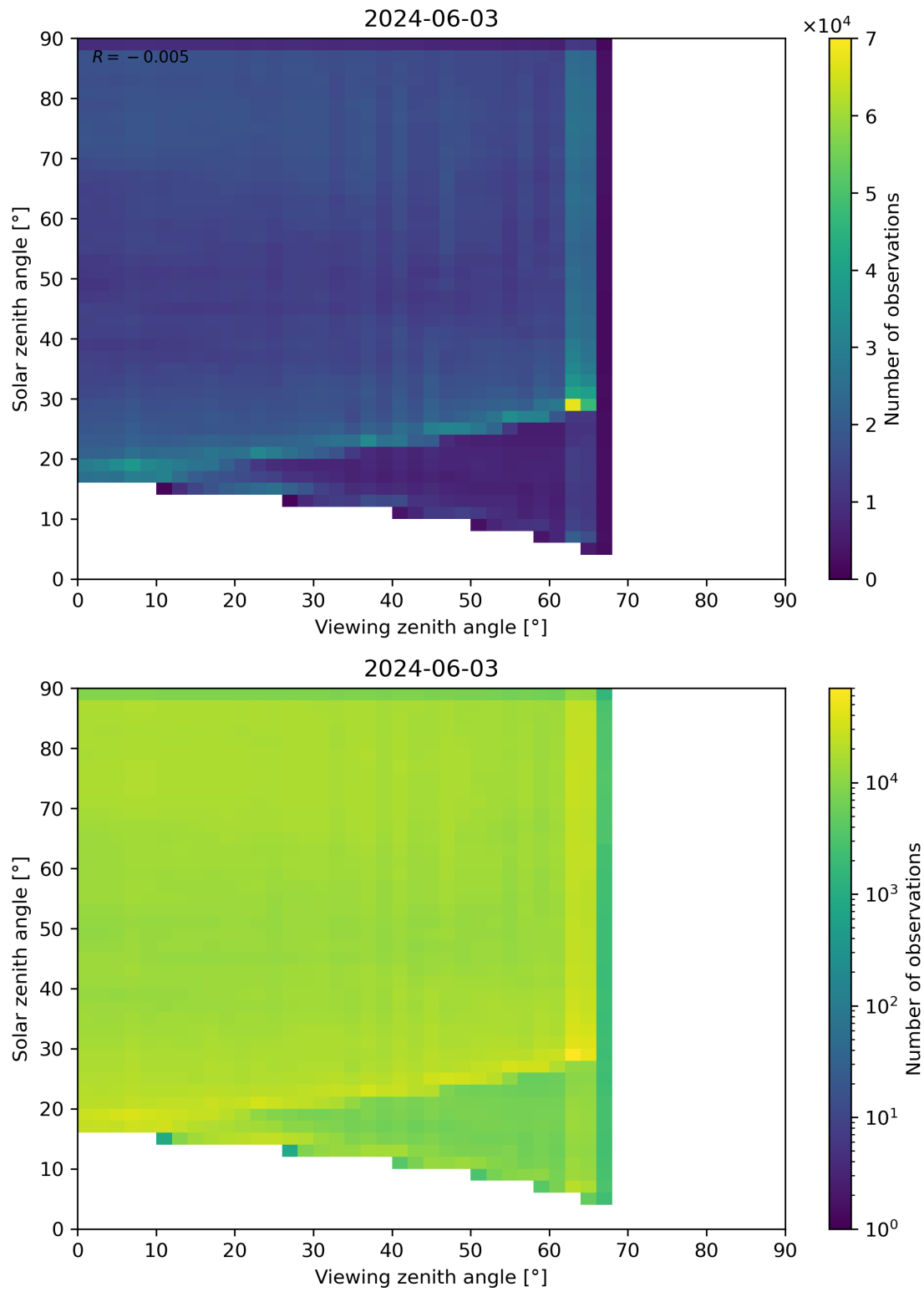
Figure 114: Scatter density plot of “Viewing zenith angle” against “Solar zenith angle” for 2024-06-03 to 2024-06-04.
