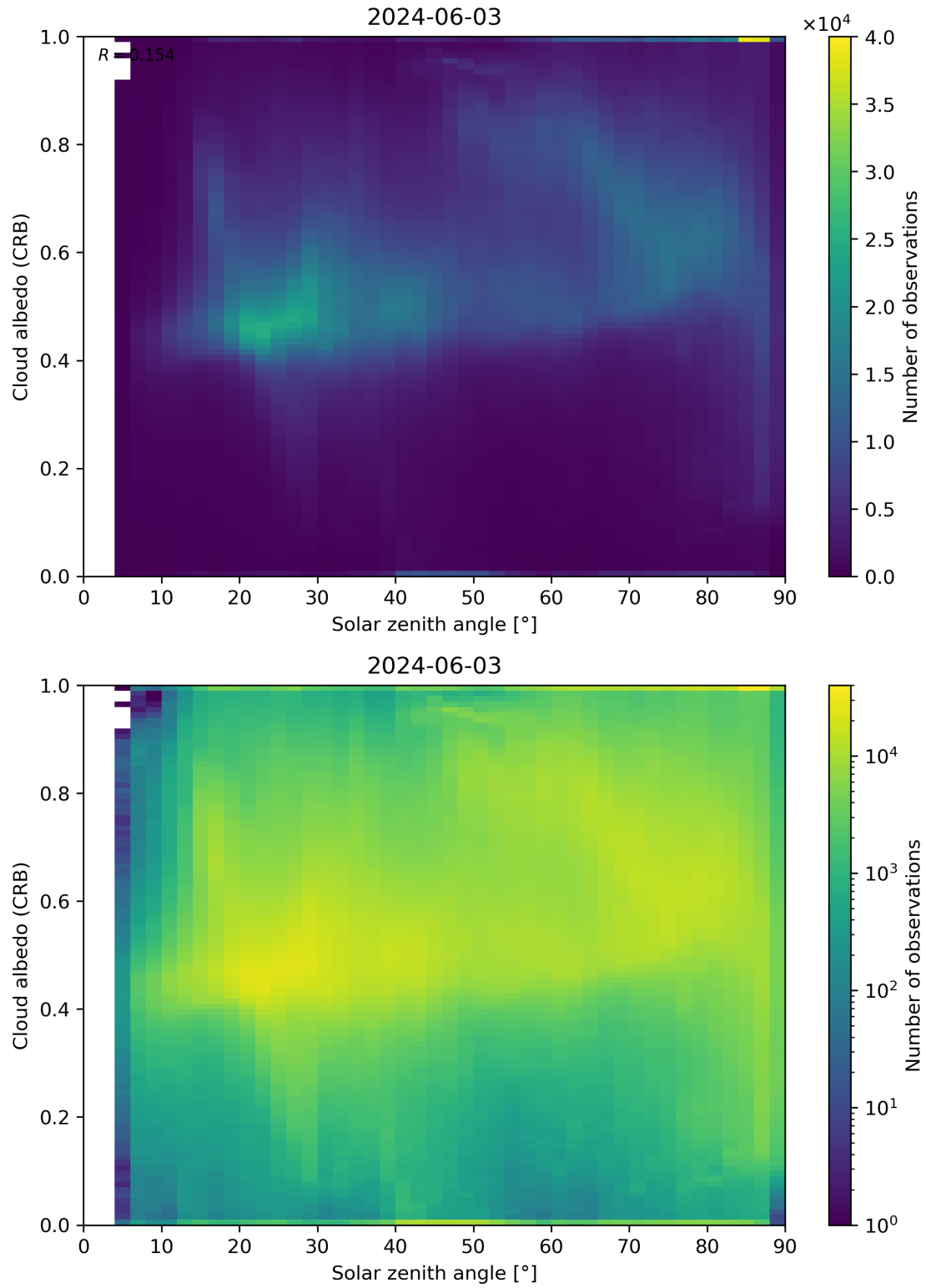
Figure 98: Scatter density plot of “Solar zenith angle” against “Cloud albedo (CRB)” for 2024-06-03 to 2024-06-04.
