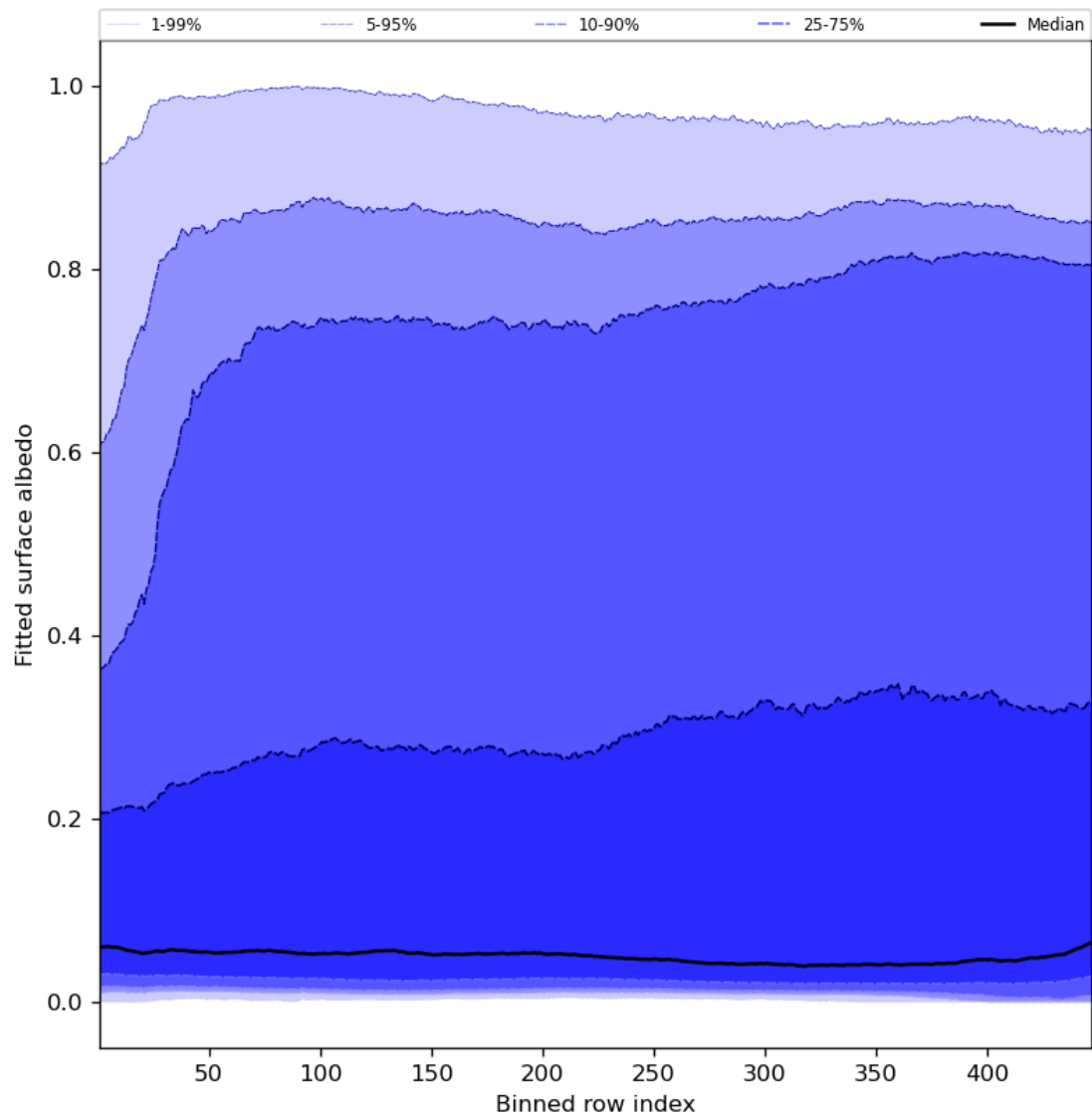
Figure 61: Along track statistics of “Fitted surface albedo” for 2024-06-03 to 2024-06-04
