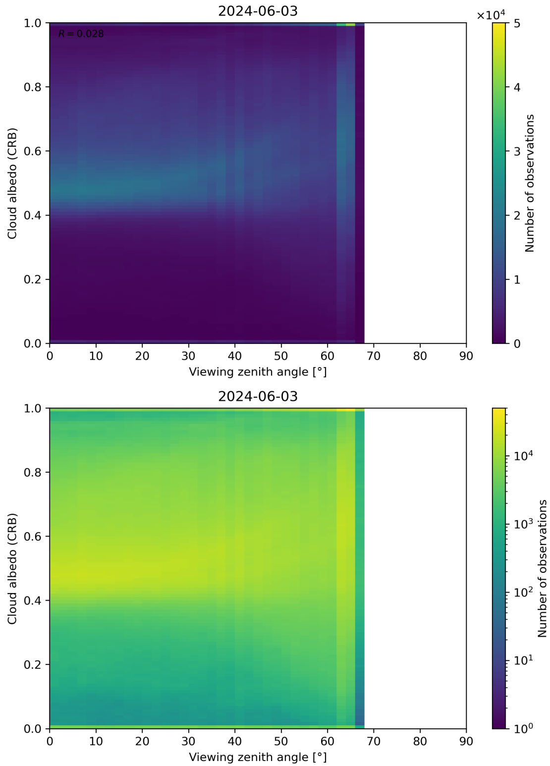
Figure 106: Scatter density plot of “Viewing zenith angle” against “Cloud albedo (CRB)” for 2024-06-03 to 2024-06-04.
