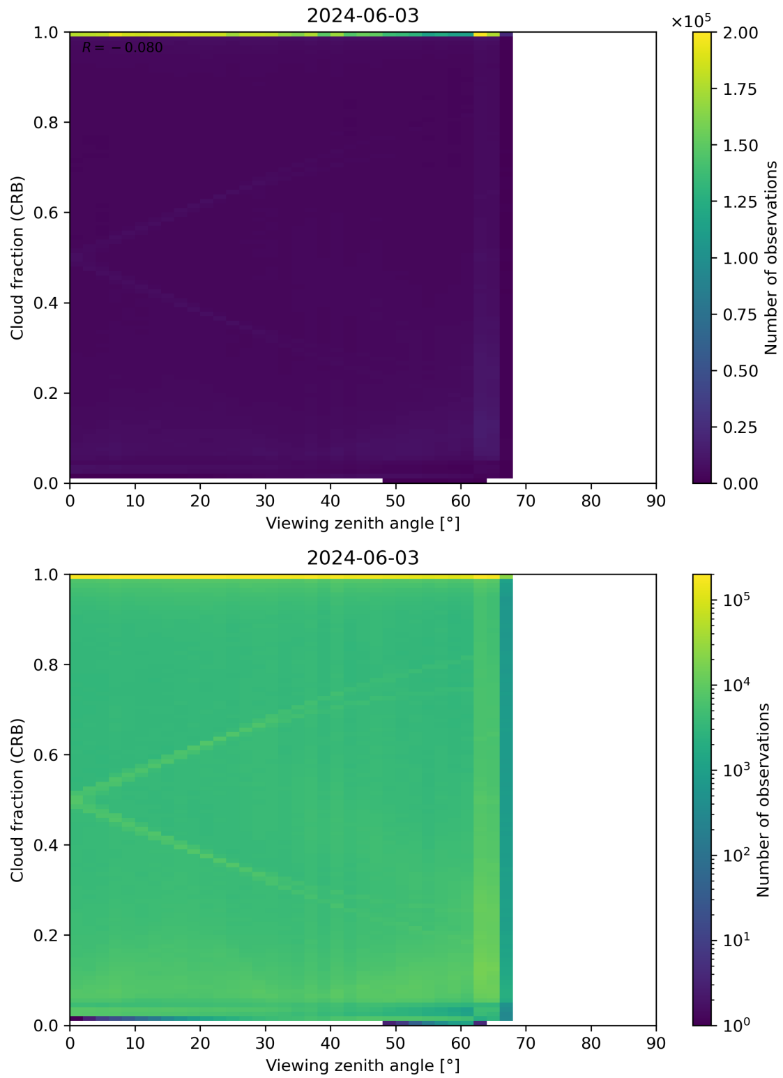
Figure 109: Scatter density plot of “Viewing zenith angle” against “Cloud fraction (CRB)” for 2024-06-03 to 2024-06-04.
