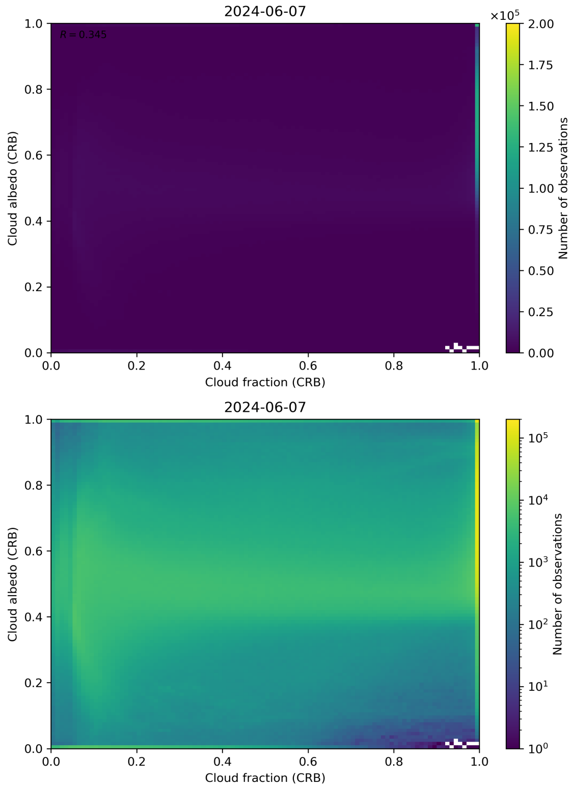
Figure 77: Scatter density plot of “Cloud fraction (CRB)” against “Cloud albedo (CRB)” for 2024-06-06 to 2024-06-08.
