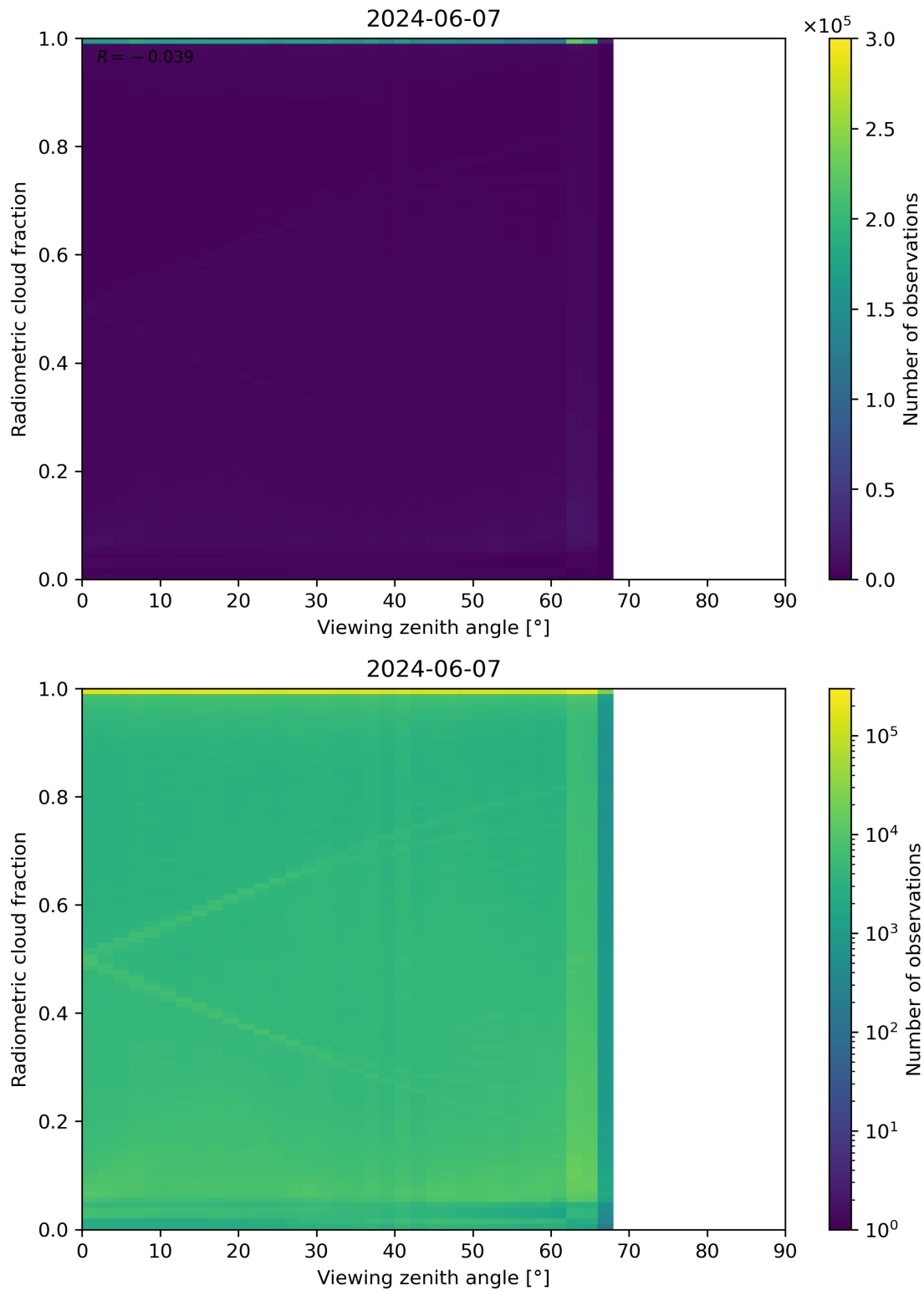
Figure 107: Scatter density plot of “Viewing zenith angle” against “Radiometric cloud fraction” for 2024-06-06 to 2024-06-08.
