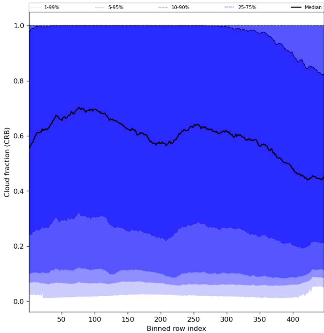
Figure 58: Along track statistics of “Cloud fraction (CRB)” for 2024-06-06 to 2024-06-08
