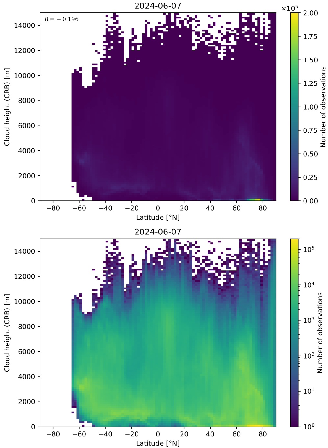
Figure 95: Scatter density plot of “Latitude” against “Cloud height (CRB)” for 2024-06-06 to 2024-06-08.
