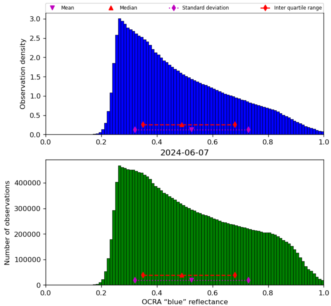
Figure 51: Histogram of “OCRA “blue” reflectance” for 2024-06-06 to 2024-06-08
