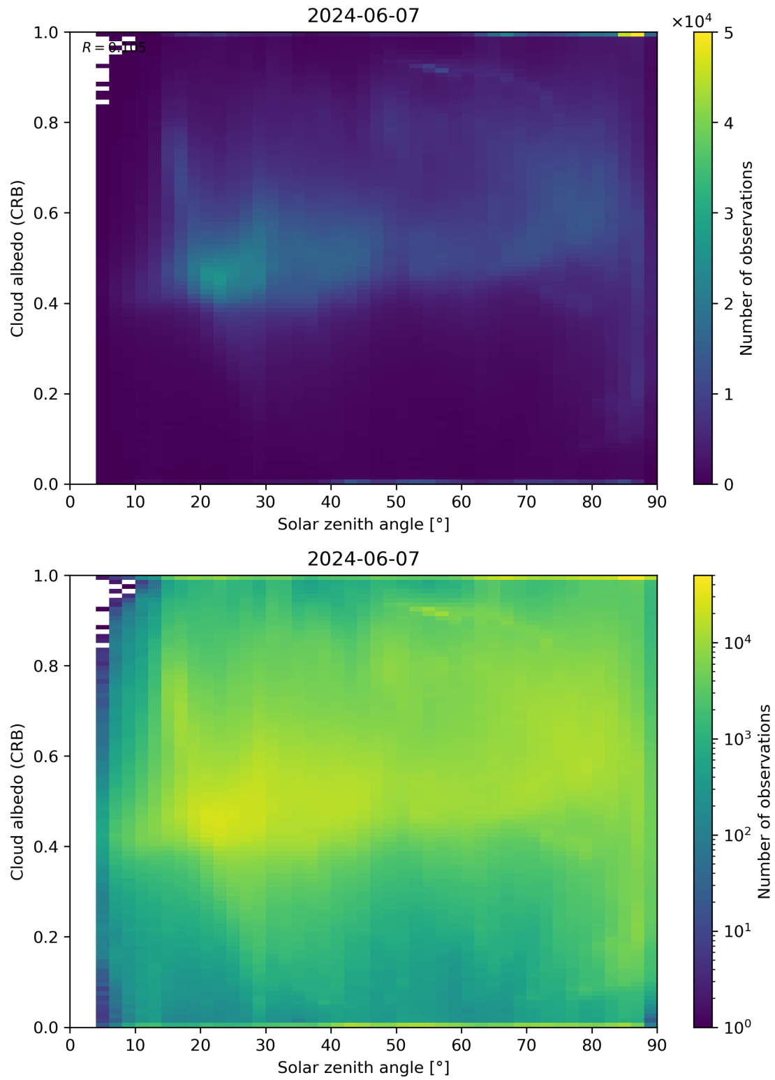
Figure 98: Scatter density plot of “Solar zenith angle” against “Cloud albedo (CRB)” for 2024-06-06 to 2024-06-08.
