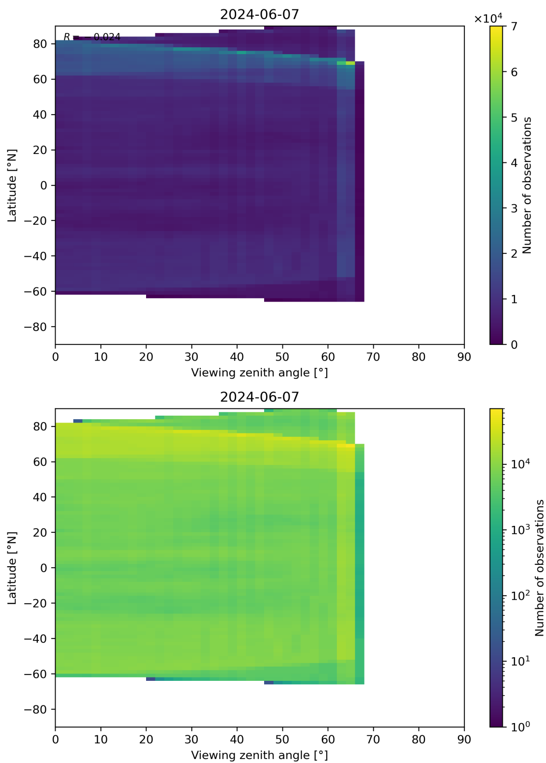
Figure 113: Scatter density plot of “Viewing zenith angle” against “Latitude” for 2024-06-06 to 2024-06-08.
