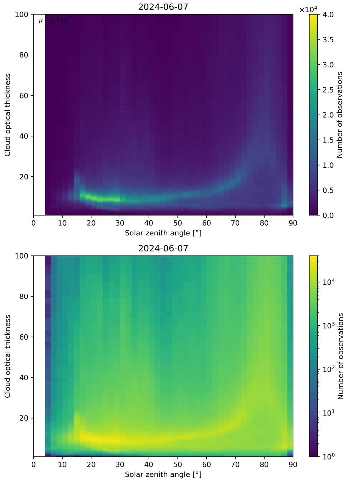
Figure 103: Scatter density plot of “Solar zenith angle” against “Cloud optical thickness” for 2024-06-06 to 2024-06-08.
