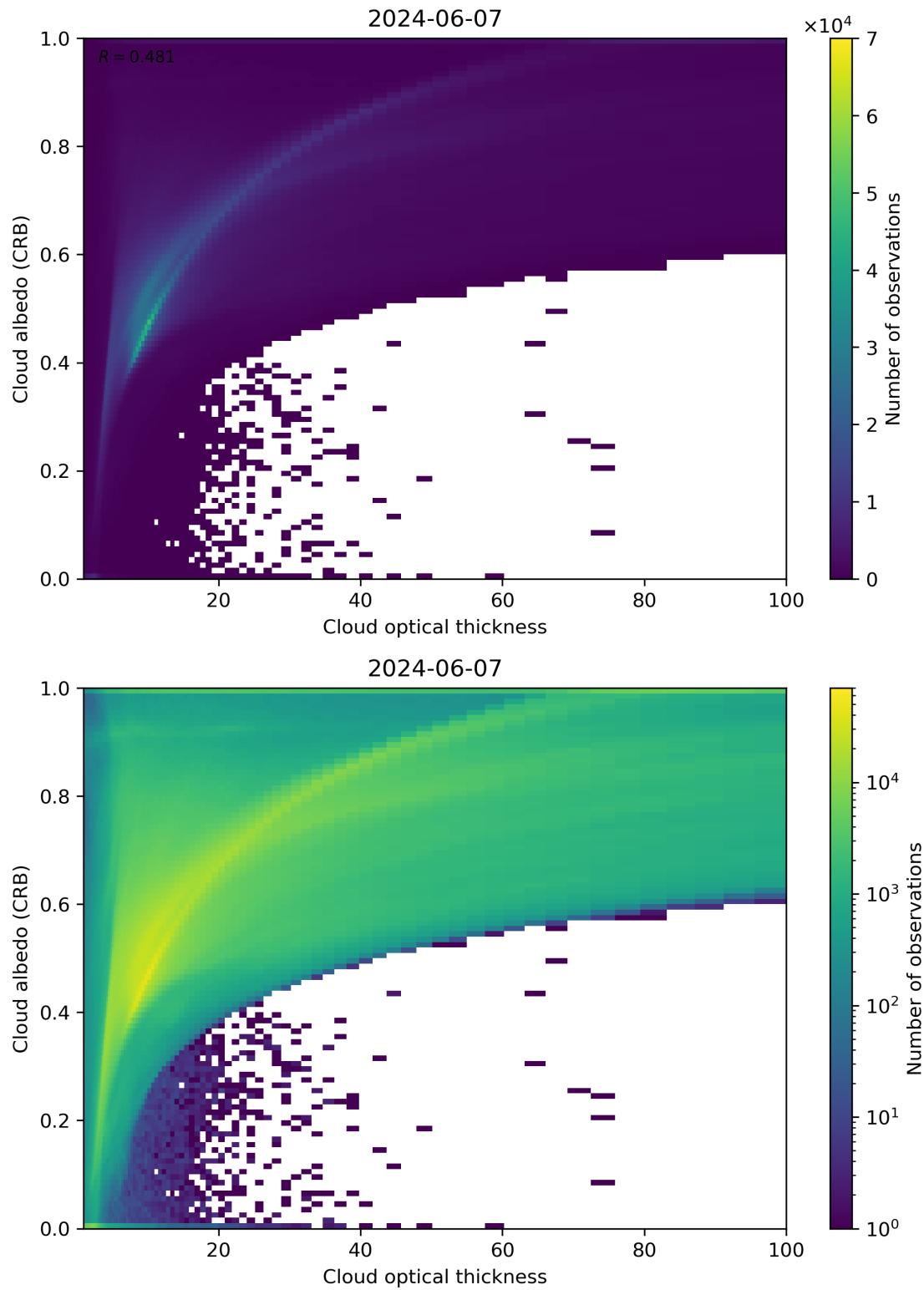
Figure 82: Scatter density plot of “Cloud optical thickness” against “Cloud albedo (CRB)” for 2024-06-06 to 2024-06-08.
