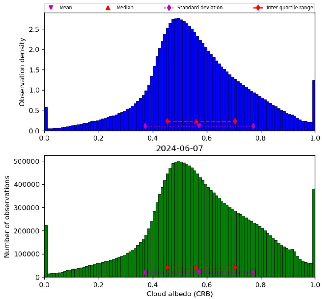
Figure 44: Histogram of “Cloud albedo (CRB)” for 2024-06-06 to 2024-06-08
