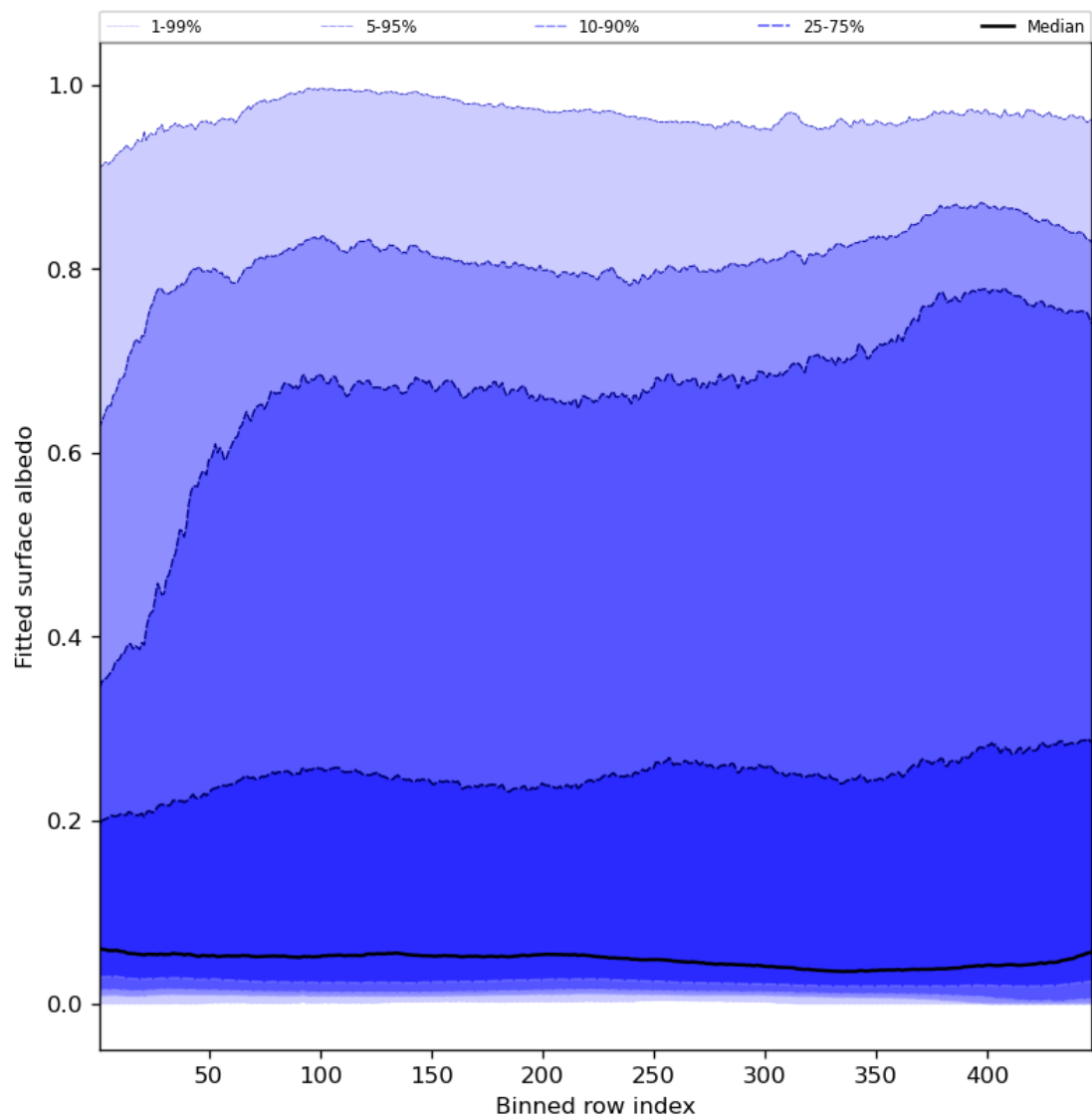
Figure 61: Along track statistics of “Fitted surface albedo” for 2024-06-06 to 2024-06-08
