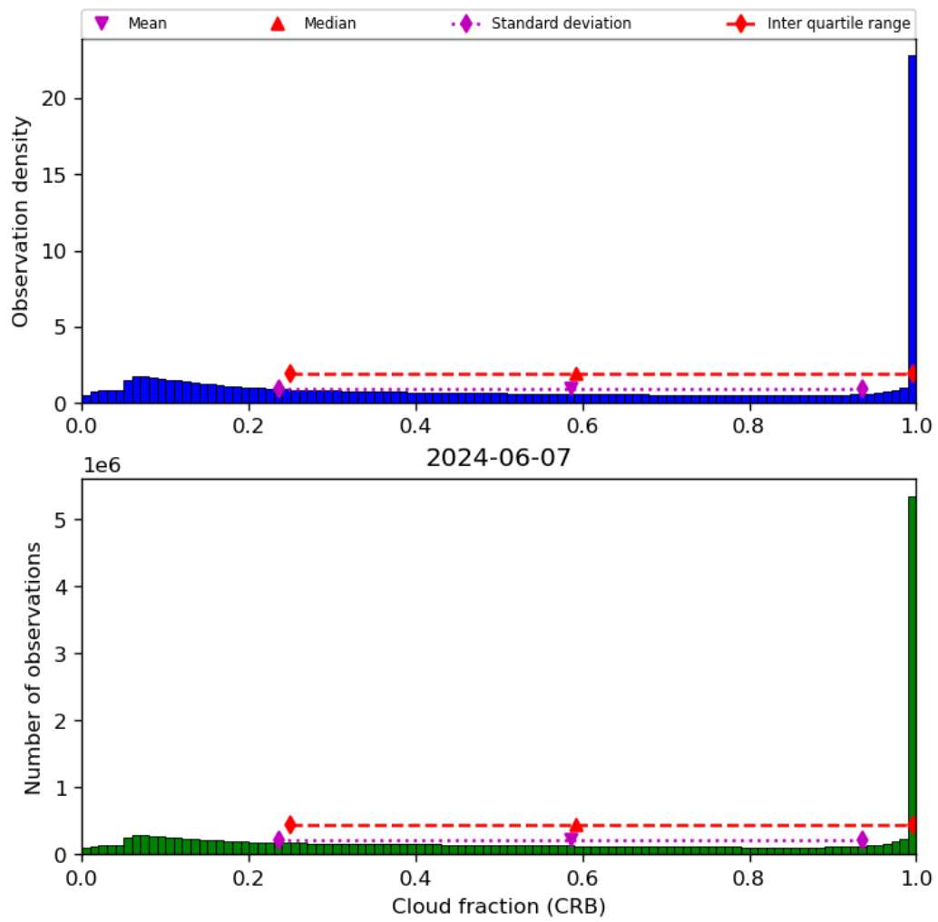
Figure 42: Histogram of “Cloud fraction (CRB)” for 2024-06-06 to 2024-06-08
