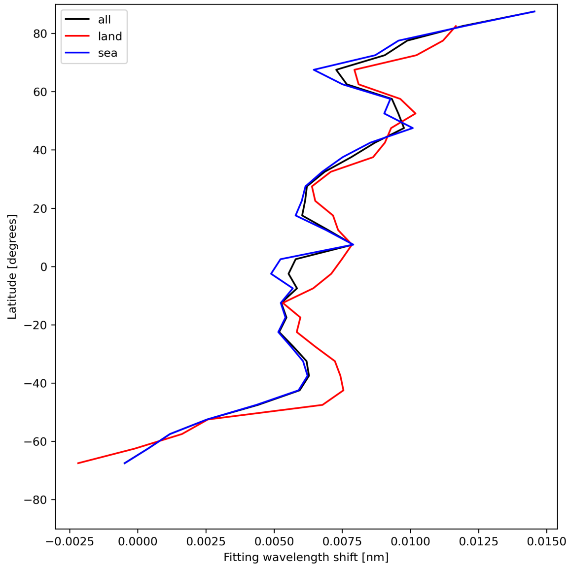
Figure 33: Zonal average of “Fitting wavelength shift” for 2024-06-06 to 2024-06-08.
