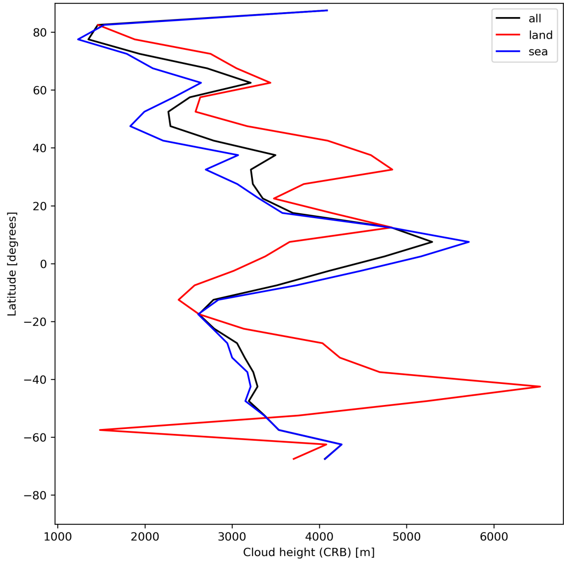
Figure 27: Zonal average of “Cloud height (CRB)” for 2024-06-06 to 2024-06-08.
