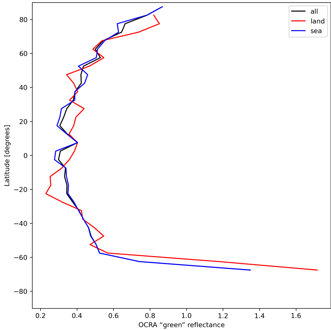
Figure 36: Zonal average of “OCRA “green” reflectance” for 2024-06-06 to 2024-06-08.
