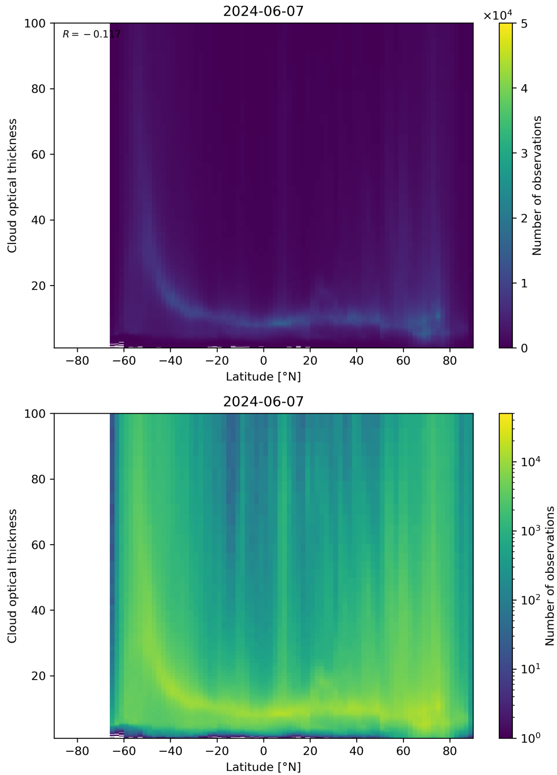
Figure 96: Scatter density plot of “Latitude” against “Cloud optical thickness” for 2024-06-06 to 2024-06-08.
