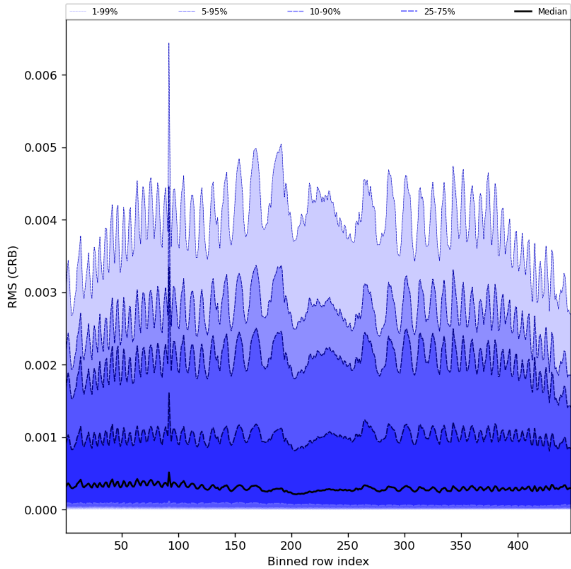
Figure 64: Along track statistics of "RMS (CRB)" for 2024-06-06 to 2024-06-08
