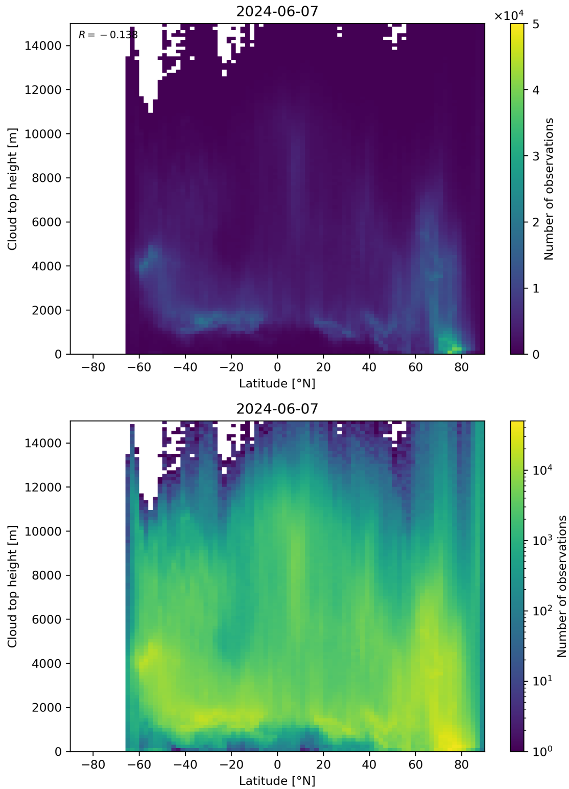
Figure 97: Scatter density plot of “Latitude” against “Cloud top height” for 2024-06-06 to 2024-06-08.
