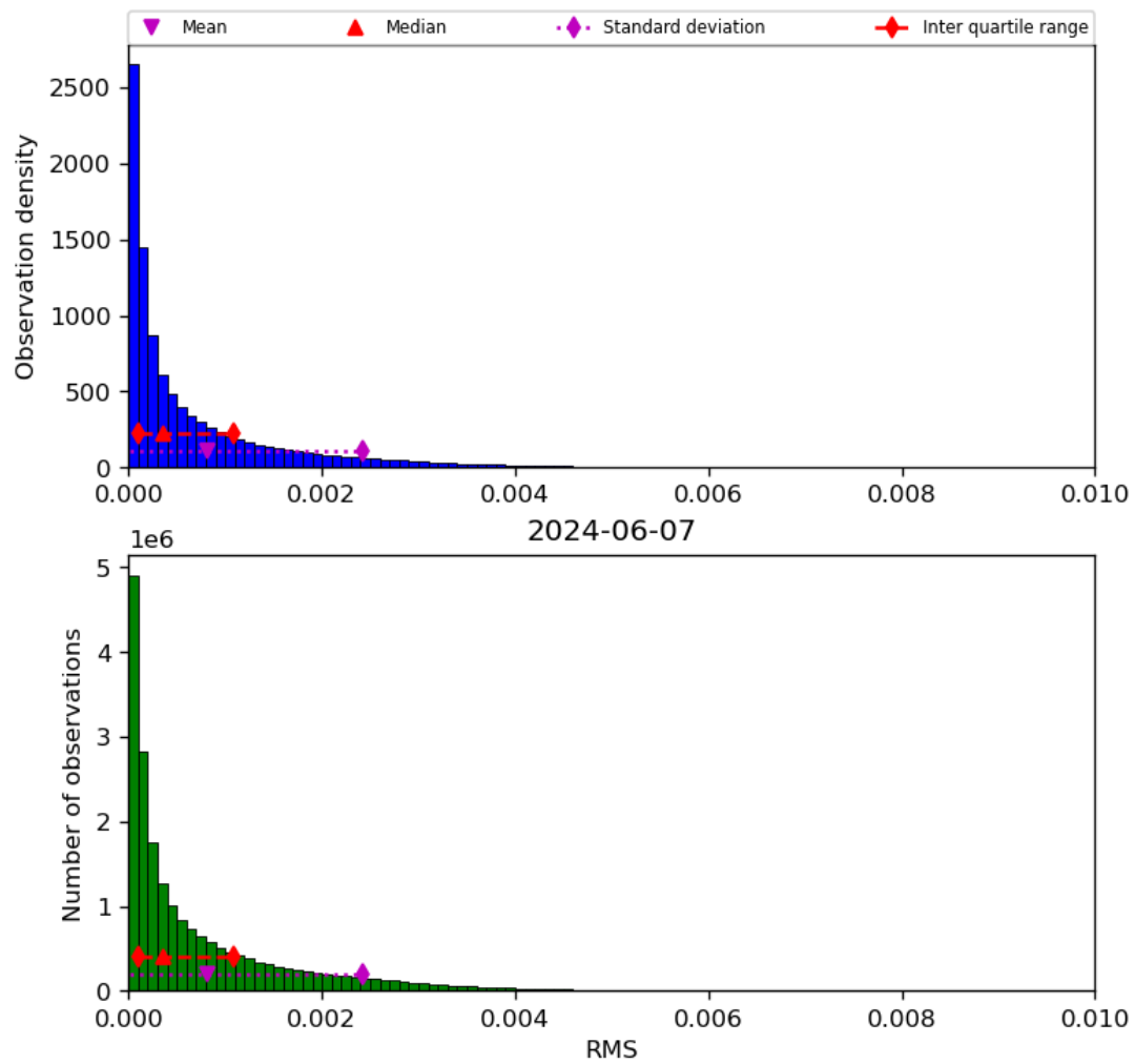
Figure 47: Histogram of “RMS” for 2024-06-06 to 2024-06-08
