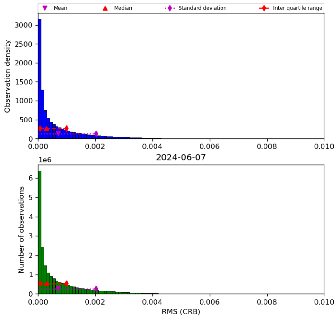
Figure 48: Histogram of “RMS (CRB)” for 2024-06-06 to 2024-06-08
