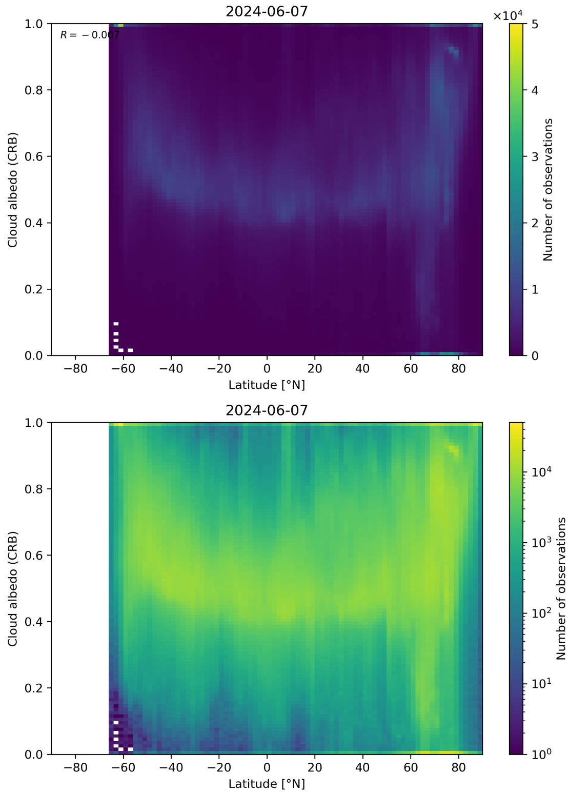
Figure 91: Scatter density plot of “Latitude” against “Cloud albedo (CRB)” for 2024-06-06 to 2024-06-08.
