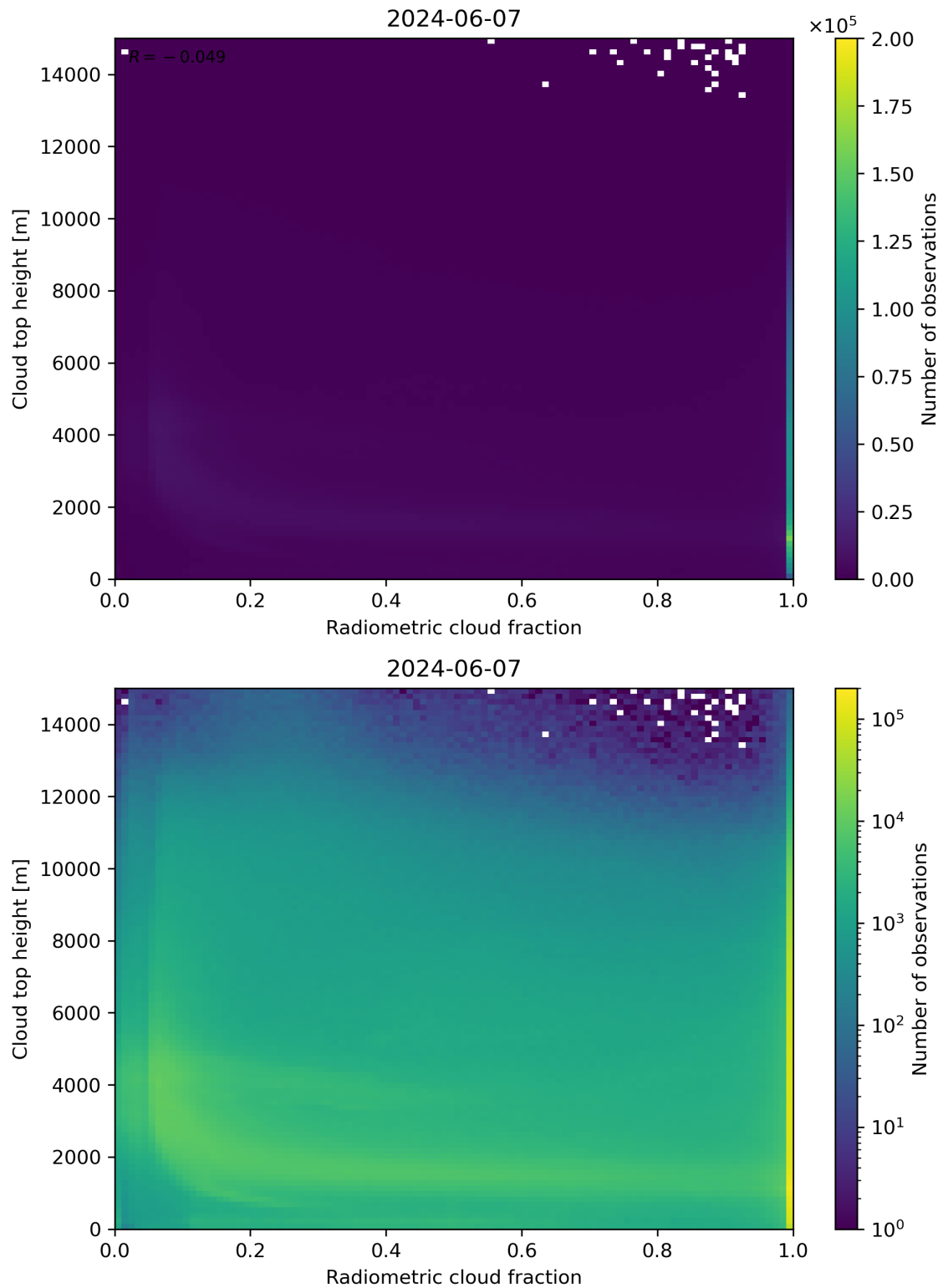
Figure 76: Scatter density plot of “Radiometric cloud fraction” against “Cloud top height” for 2024-06-06 to 2024-06-08.
