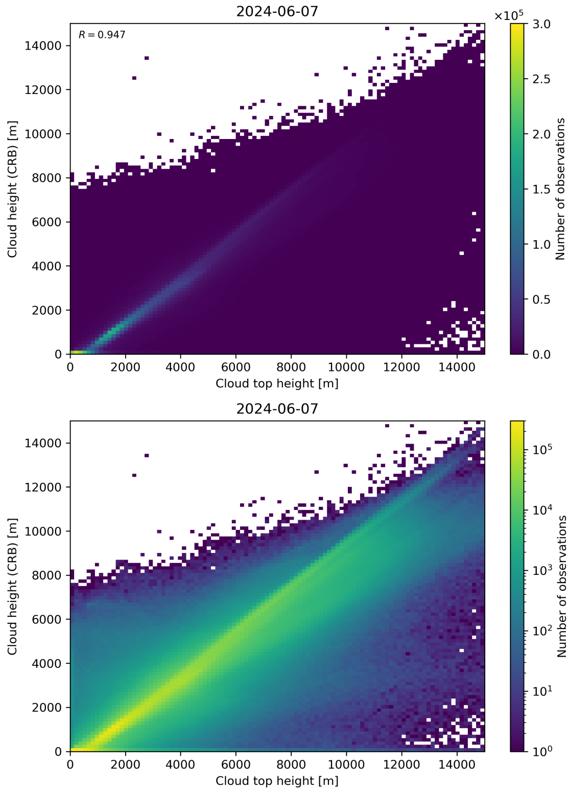
Figure 89: Scatter density plot of “Cloud top height” against “Cloud height (CRB)” for 2024-06-06 to 2024-06-08.
