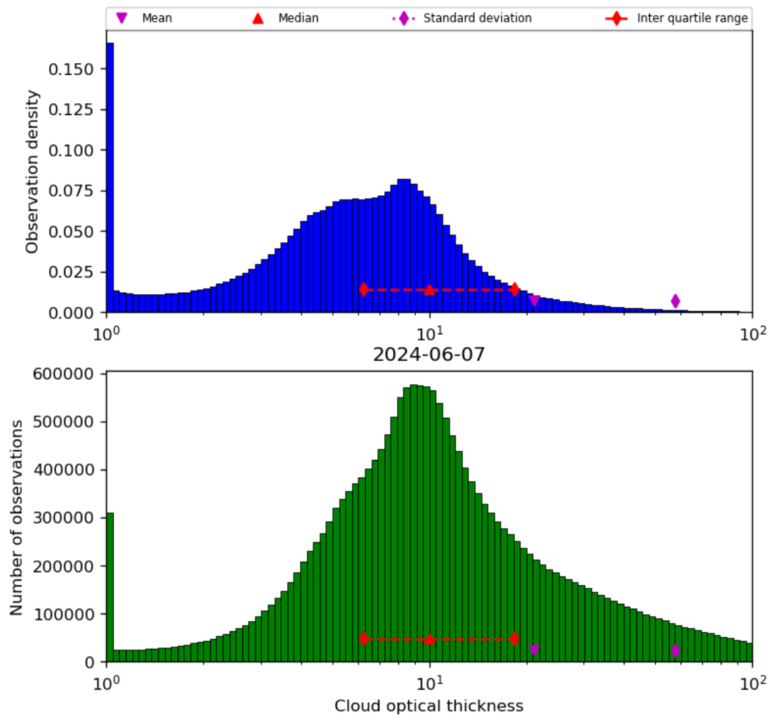
Figure 41: Histogram of “Cloud optical thickness” for 2024-06-06 to 2024-06-08
