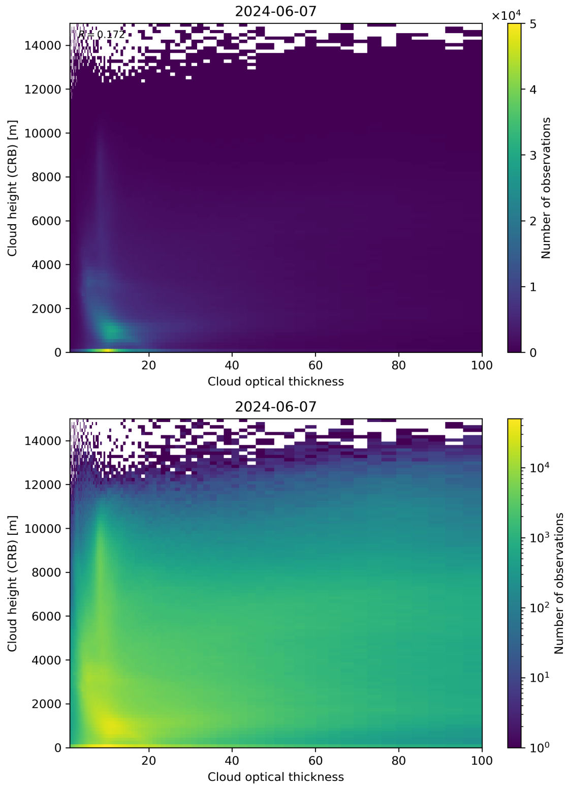
Figure 85: Scatter density plot of “Cloud optical thickness” against “Cloud height (CRB)” for 2024-06-06 to 2024-06-08.
