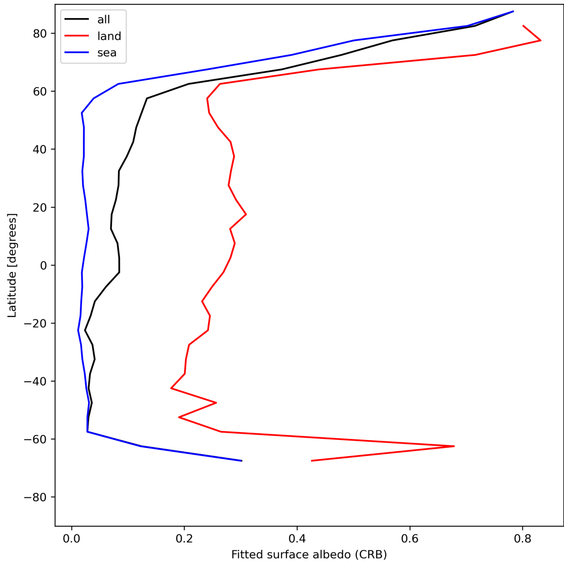
Figure 30: Zonal average of “Fitted surface albedo (CRB)” for 2024-06-06 to 2024-06-08.
