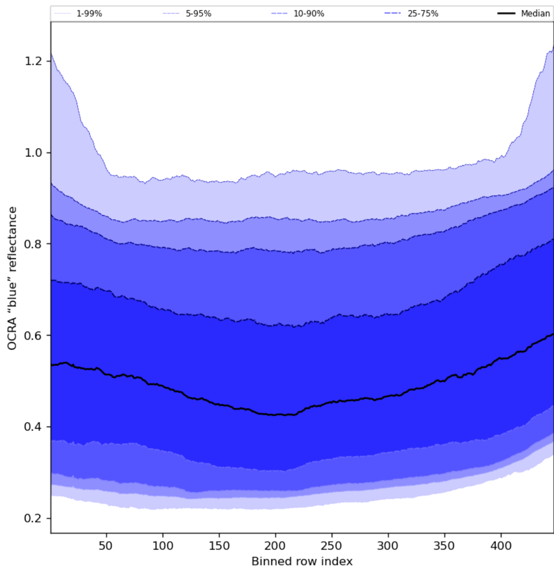
Figure 67: Along track statistics of “OCRA “blue” reflectance” for 2024-06-06 to 2024-06-08
