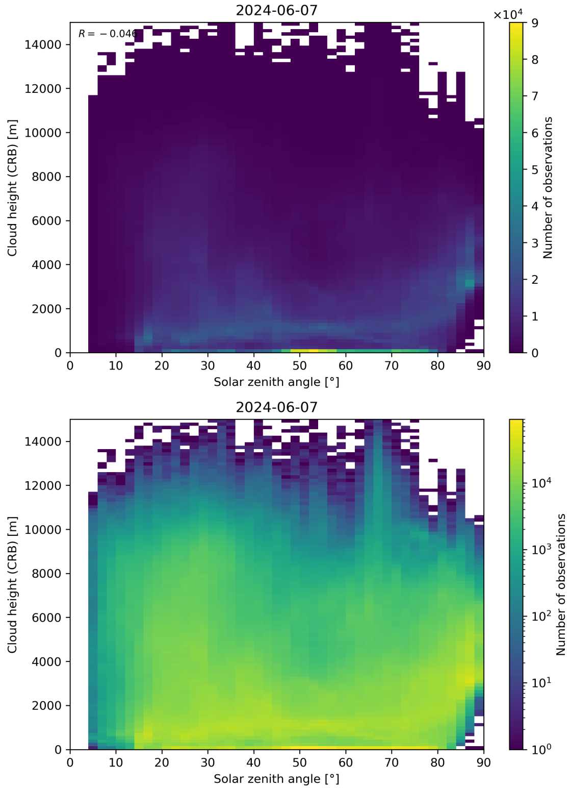
Figure 102: Scatter density plot of “Solar zenith angle” against “Cloud height (CRB)” for 2024-06-06 to 2024-06-08.
