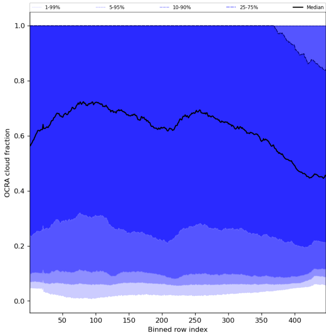
Figure 66: Along track statistics of “OCRA cloud fraction” for 2024-06-06 to 2024-06-08
