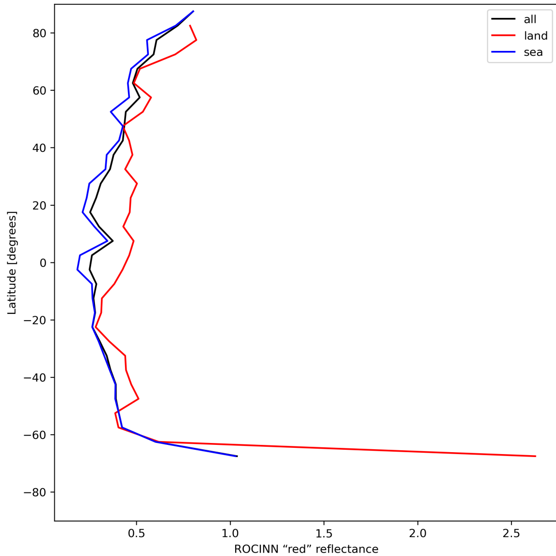
Figure 37: Zonal average of “ROCINN “red” reflectance” for 2024-06-06 to 2024-06-08.
