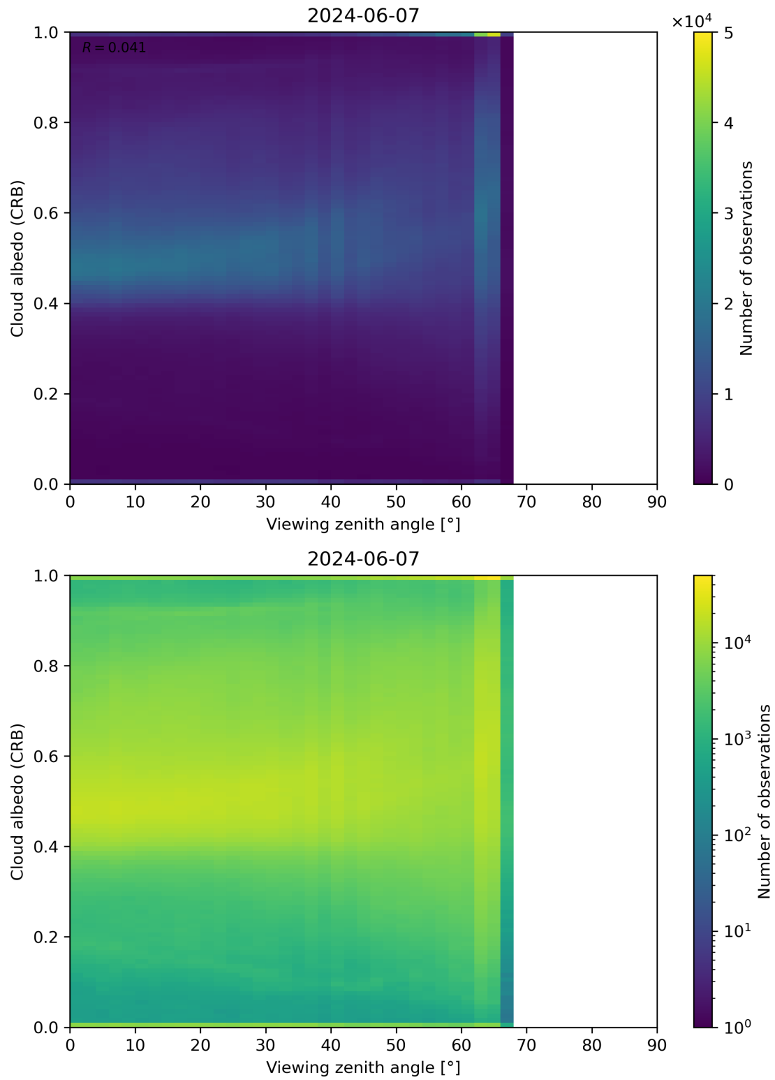
Figure 106: Scatter density plot of “Viewing zenith angle” against “Cloud albedo (CRB)” for 2024-06-06 to 2024-06-08.
