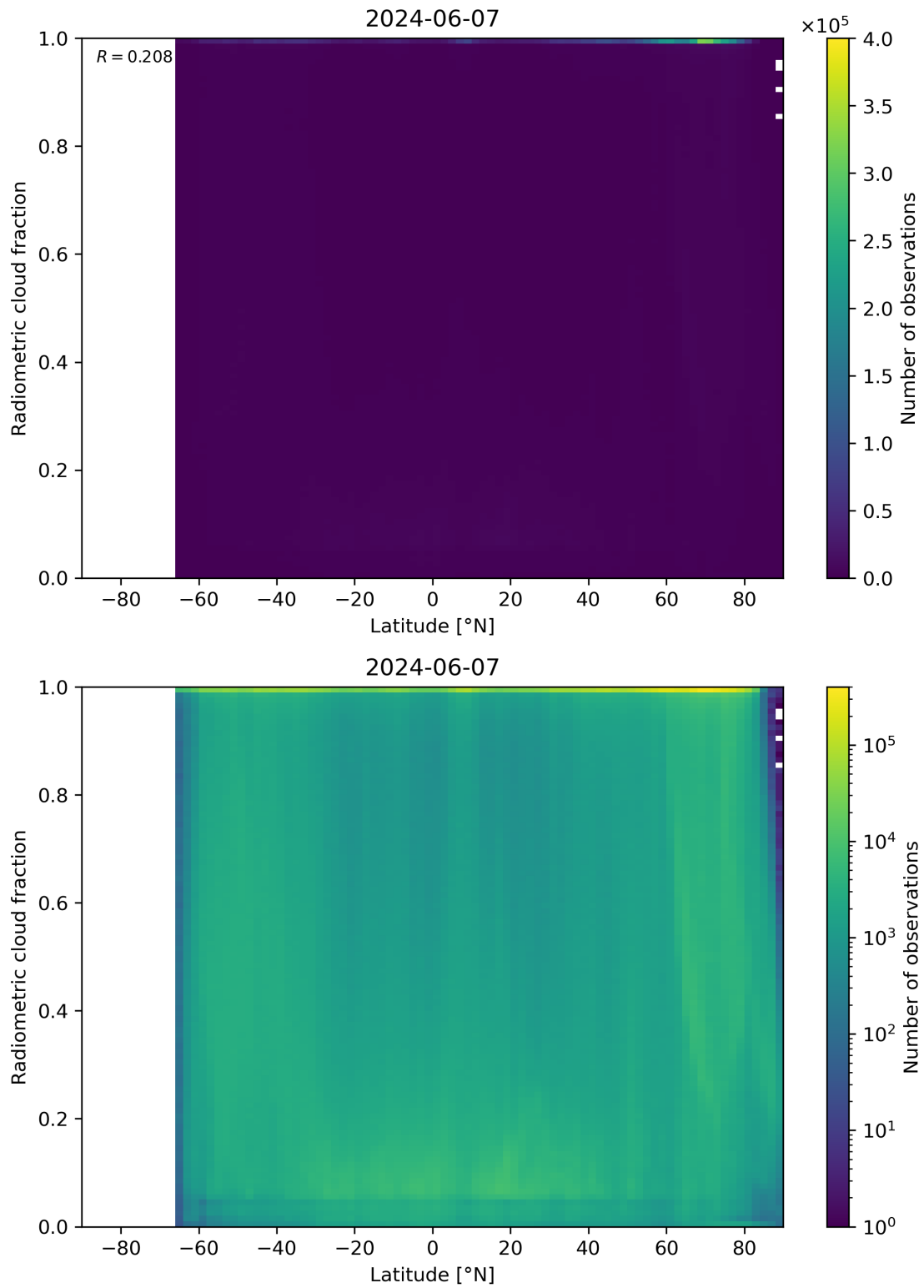
Figure 92: Scatter density plot of “Latitude” against “Radiometric cloud fraction” for 2024-06-06 to 2024-06-08.
