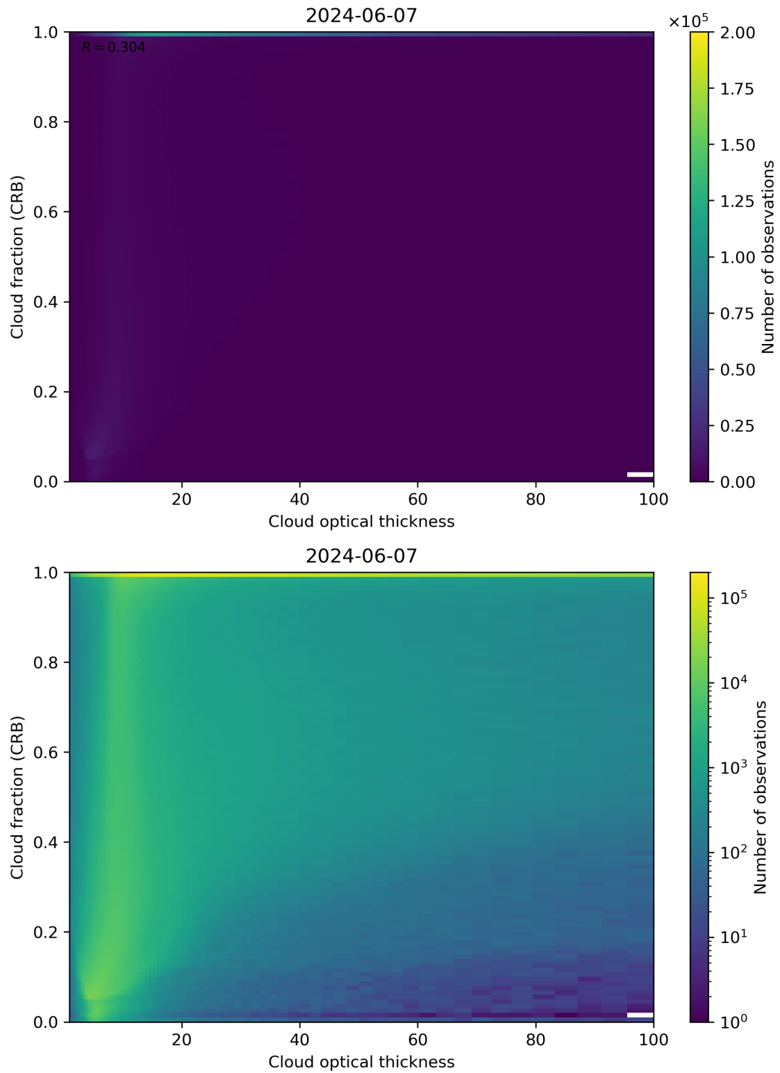
Figure 84: Scatter density plot of “Cloud optical thickness” against “Cloud fraction (CRB)” for 2024-06-06 to 2024-06-08.
