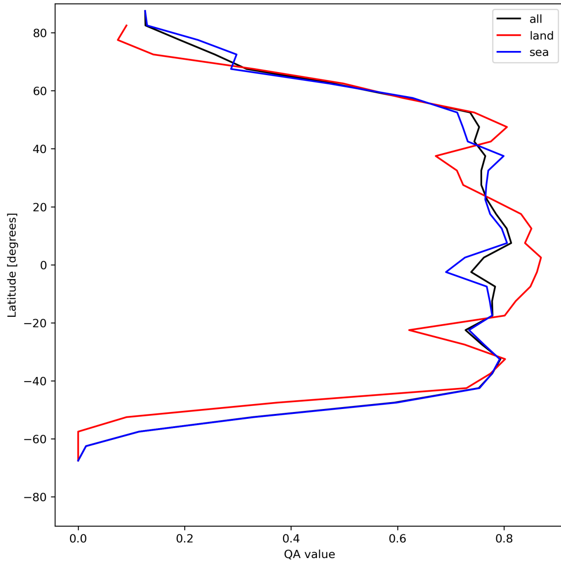
Figure 22: Zonal average of “QA value” for 2024-06-06 to 2024-06-08.
