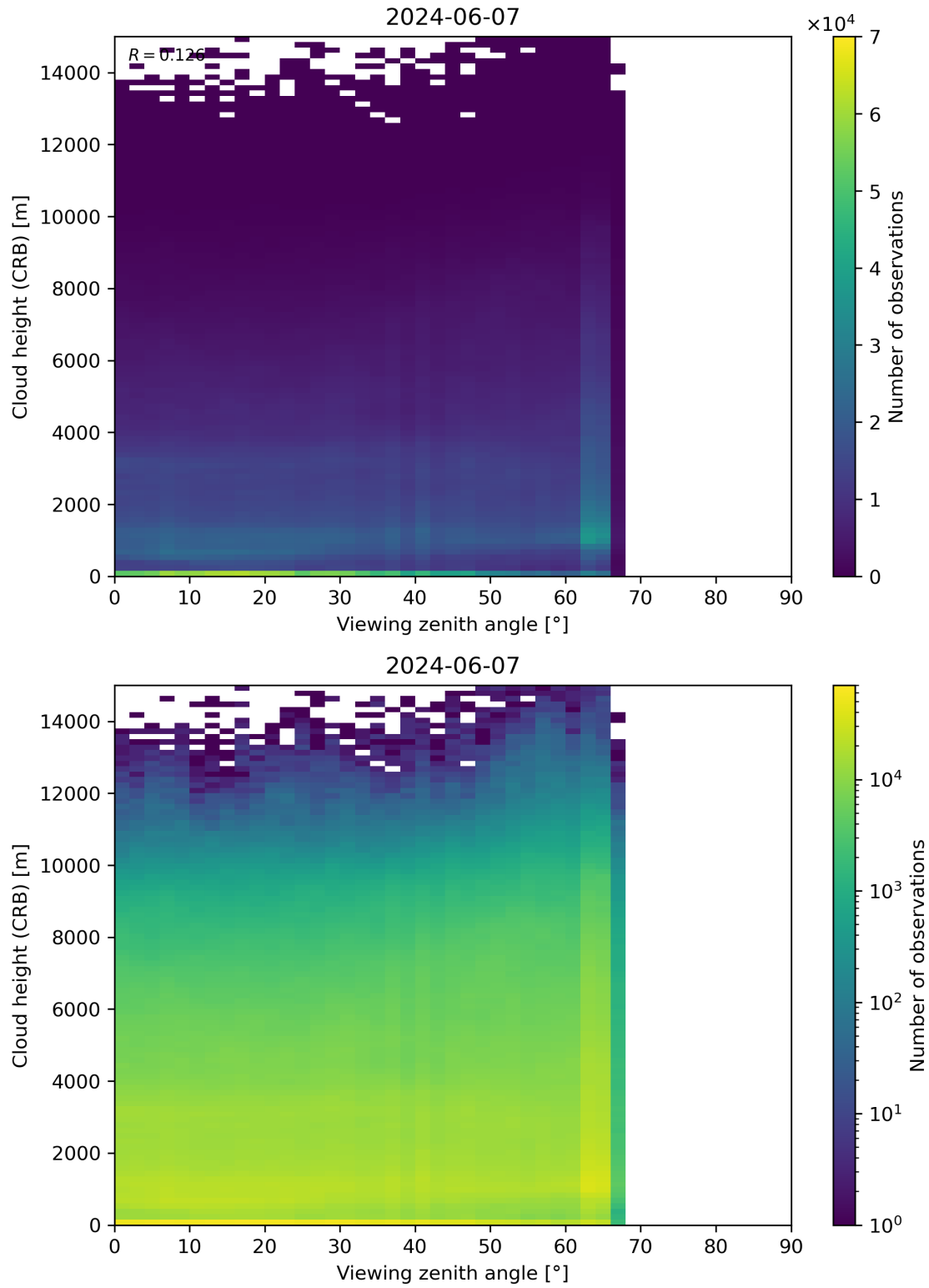
Figure 110: Scatter density plot of “Viewing zenith angle” against “Cloud height (CRB)” for 2024-06-06 to 2024-06-08.
