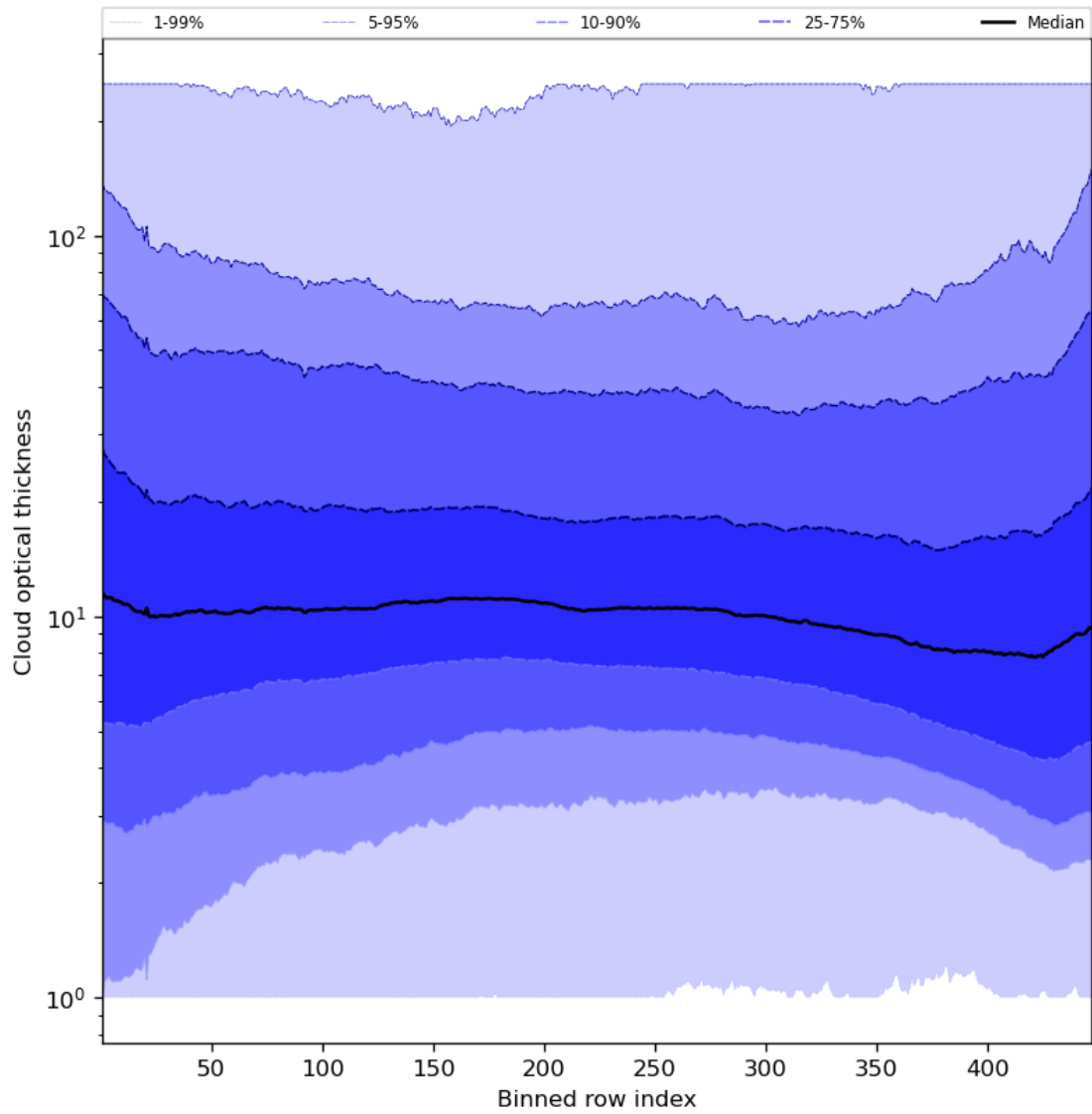
Figure 57: Along track statistics of “Cloud optical thickness” for 2024-06-06 to 2024-06-08
