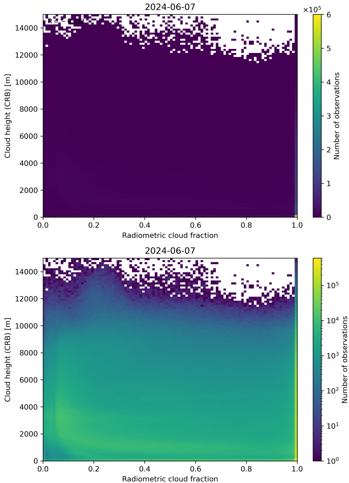
Figure 74: Scatter density plot of “Radiometric cloud fraction” against “Cloud height (CRB)” for 2024-06-06 to 2024-06-08.
