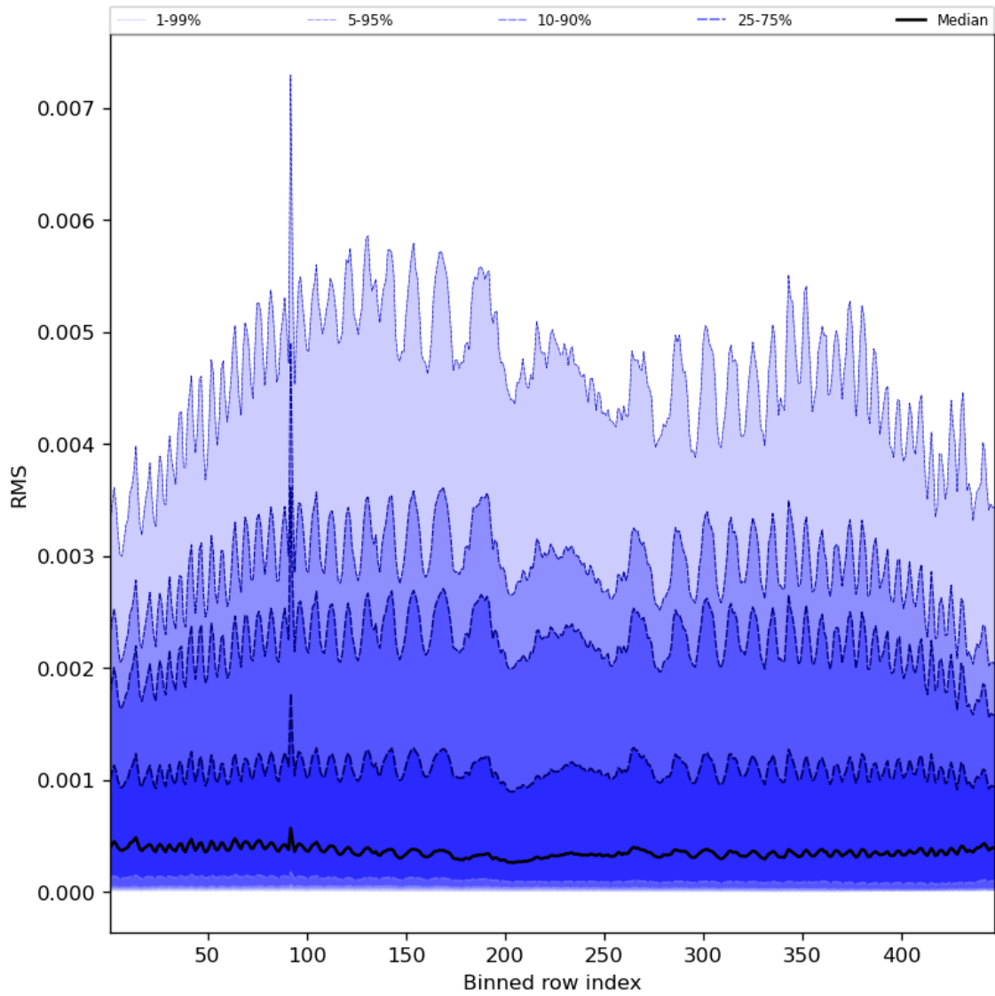
Figure 63: Along track statistics of “RMS” for 2024-06-06 to 2024-06-08
