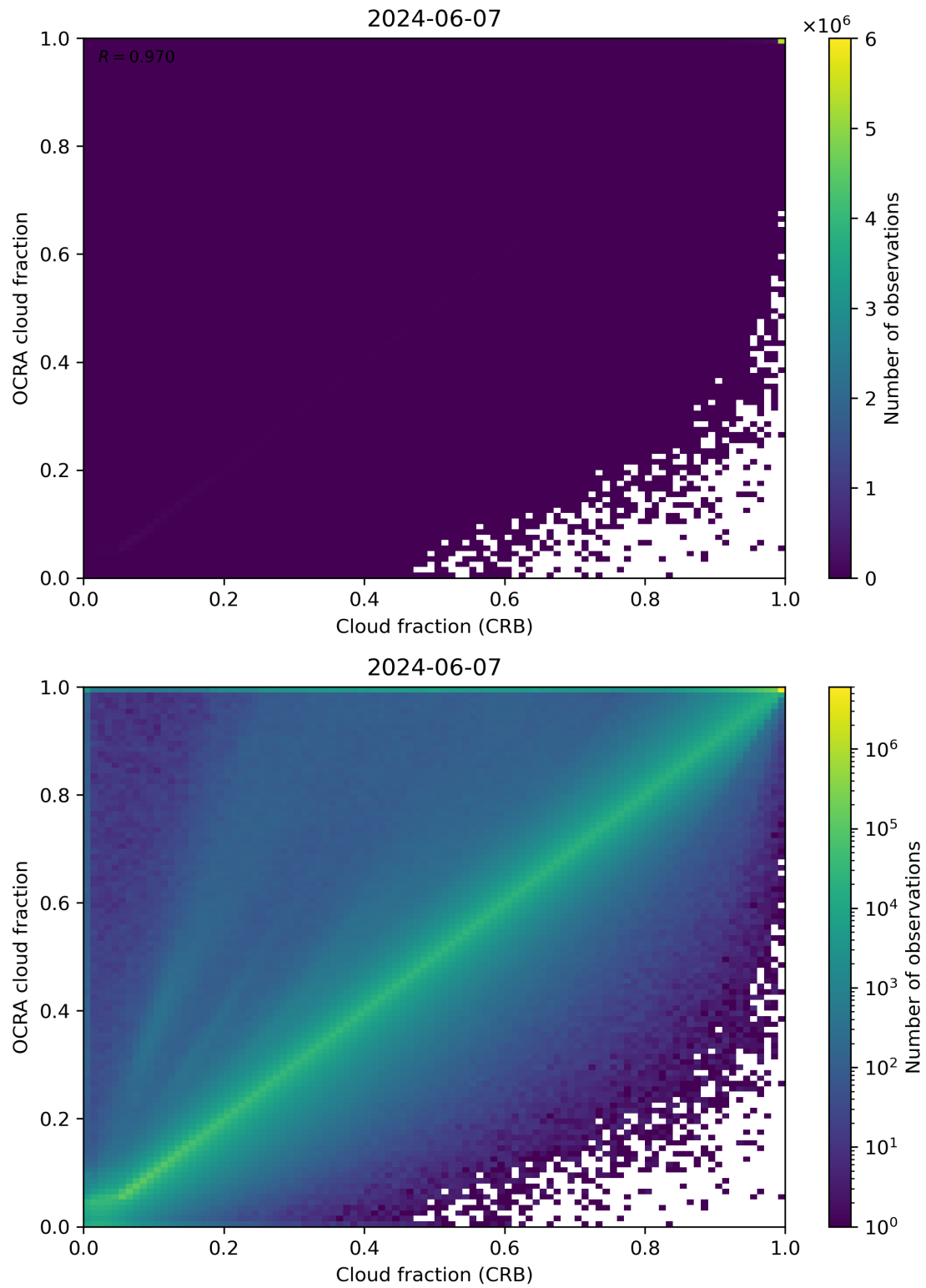
Figure 78: Scatter density plot of “Cloud fraction (CRB)” against “OCRA cloud fraction” for 2024-06-06 to 2024-06-08.
