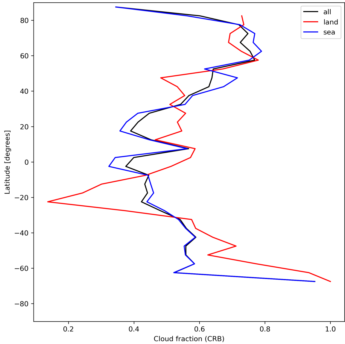
Figure 26: Zonal average of “Cloud fraction (CRB)” for 2024-06-06 to 2024-06-08.
