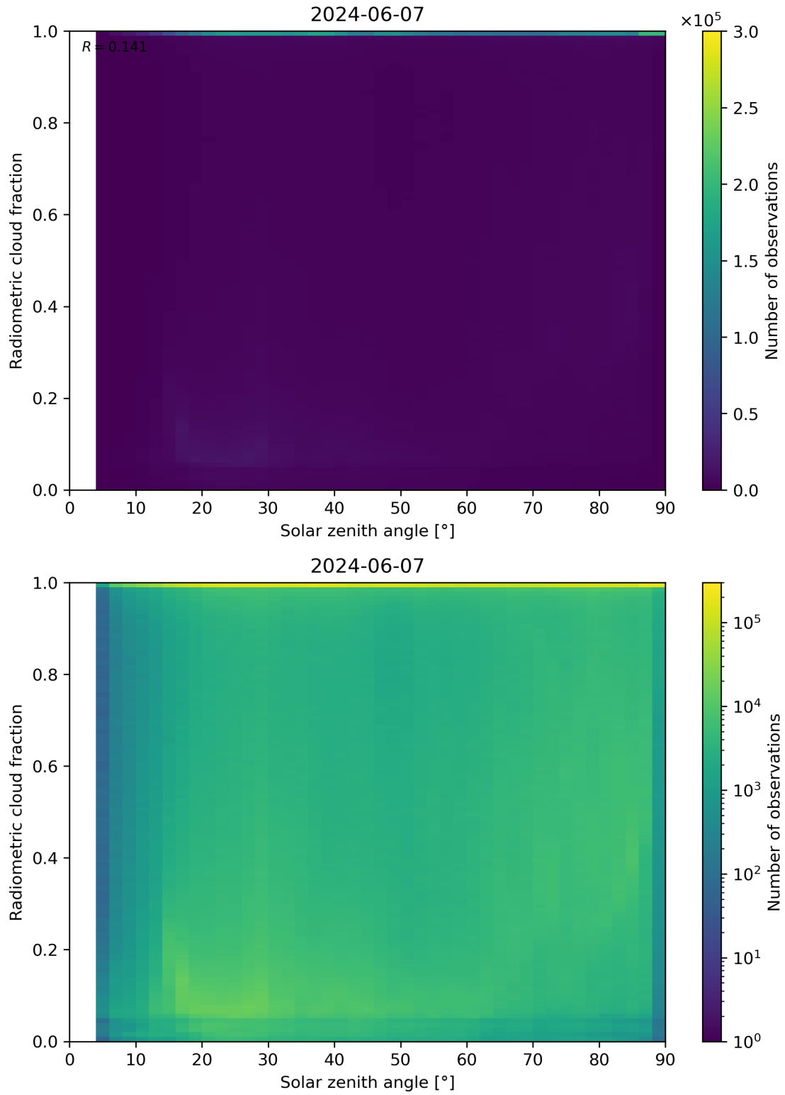
Figure 99: Scatter density plot of “Solar zenith angle” against “Radiometric cloud fraction” for 2024-06-06 to 2024-06-08.
