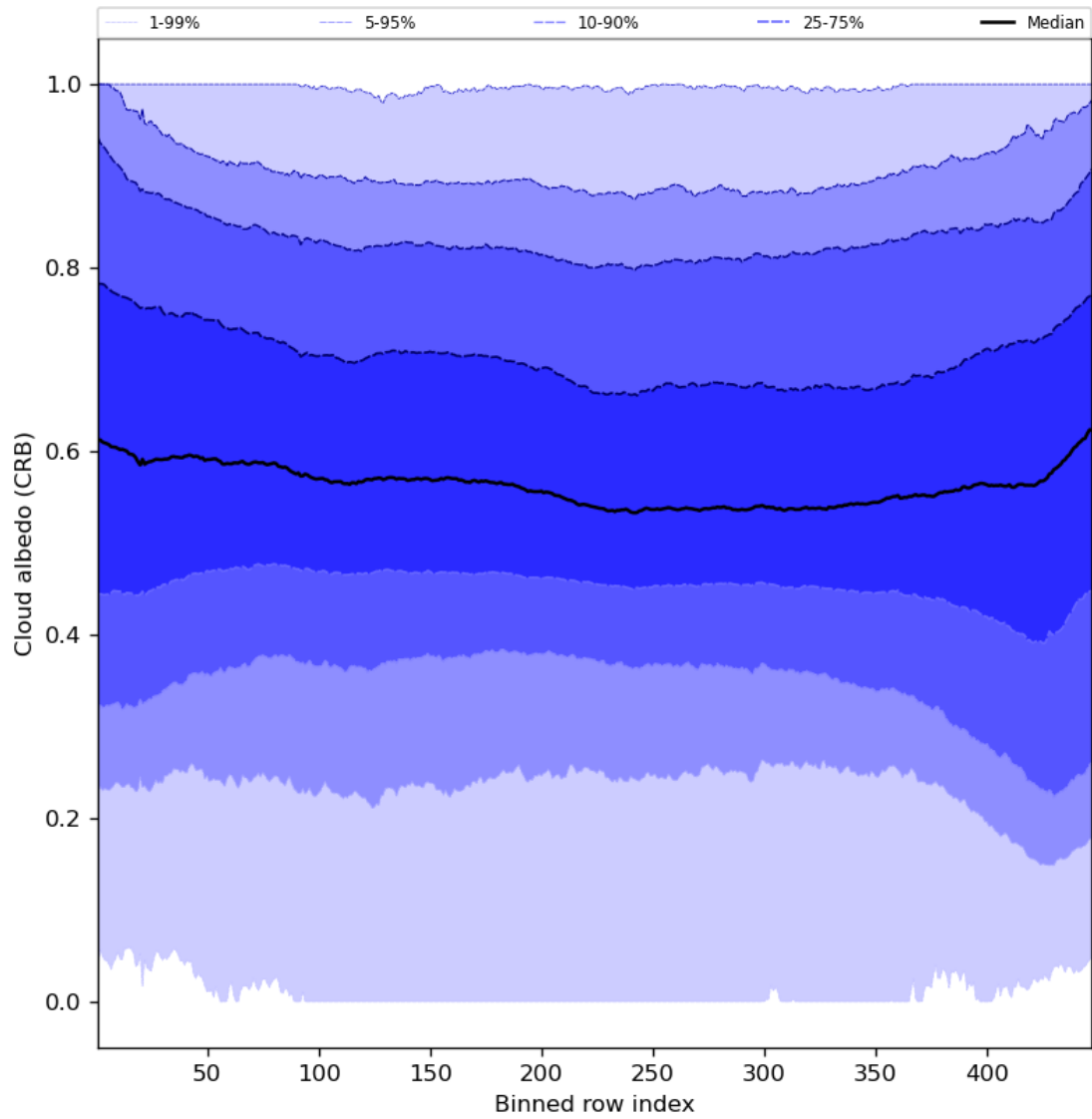
Figure 60: Along track statistics of “Cloud albedo (CRB)” for 2024-06-06 to 2024-06-08
