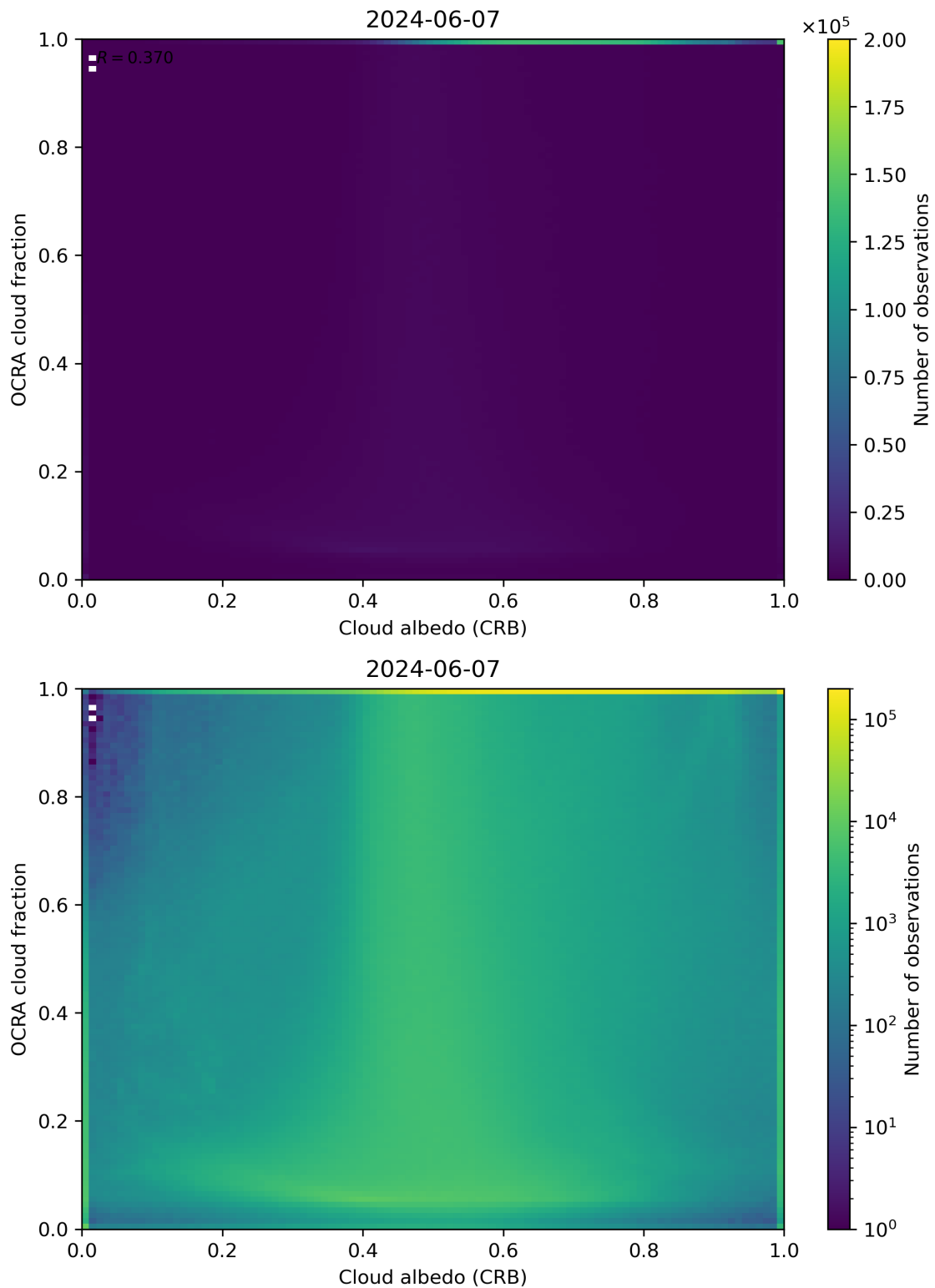
Figure 70: Scatter density plot of “Cloud albedo (CRB)” against “OCRA cloud fraction” for 2024-06-06 to 2024-06-08.
