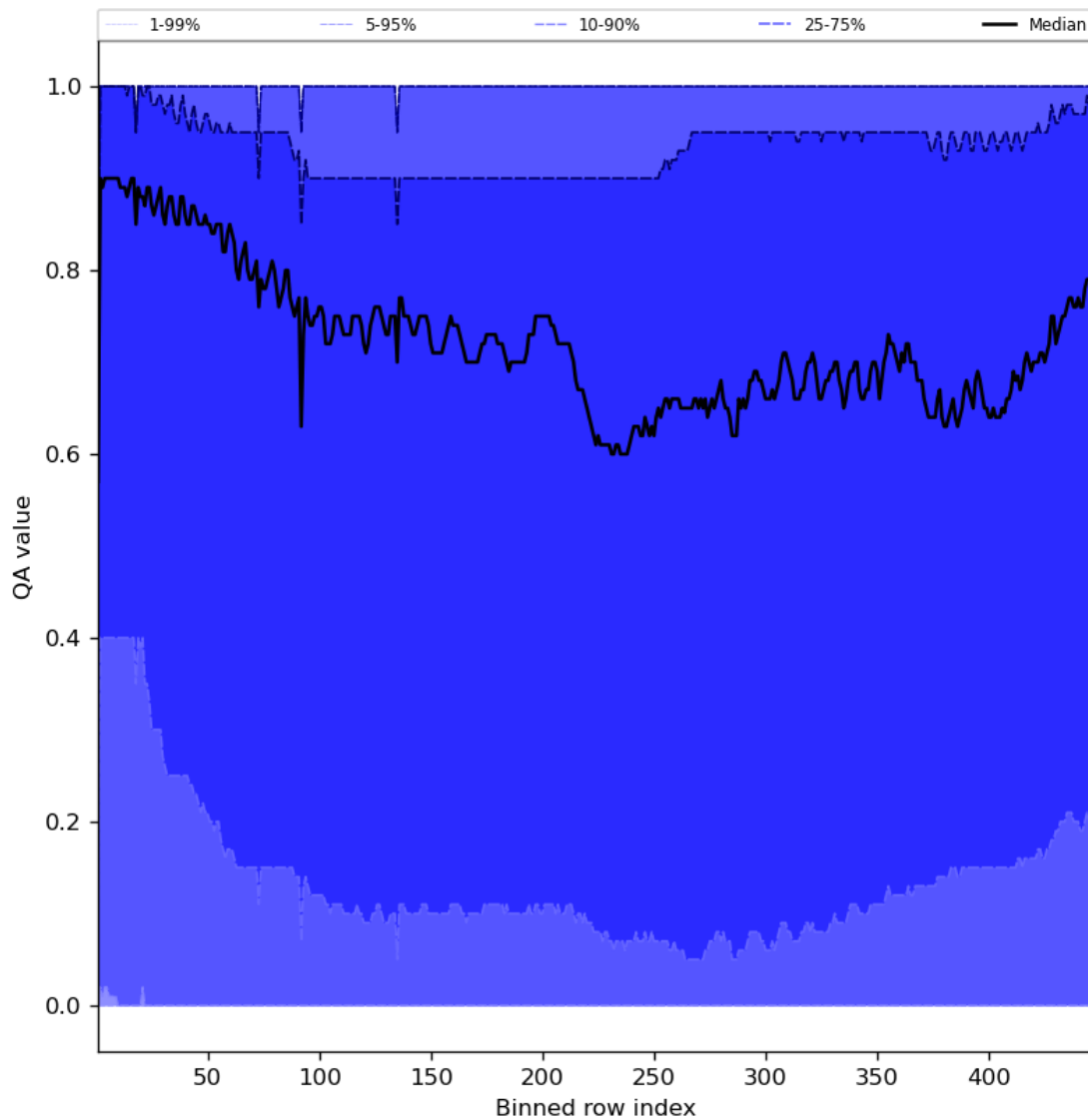
Figure 54: Along track statistics of “QA value” for 2024-06-06 to 2024-06-08
