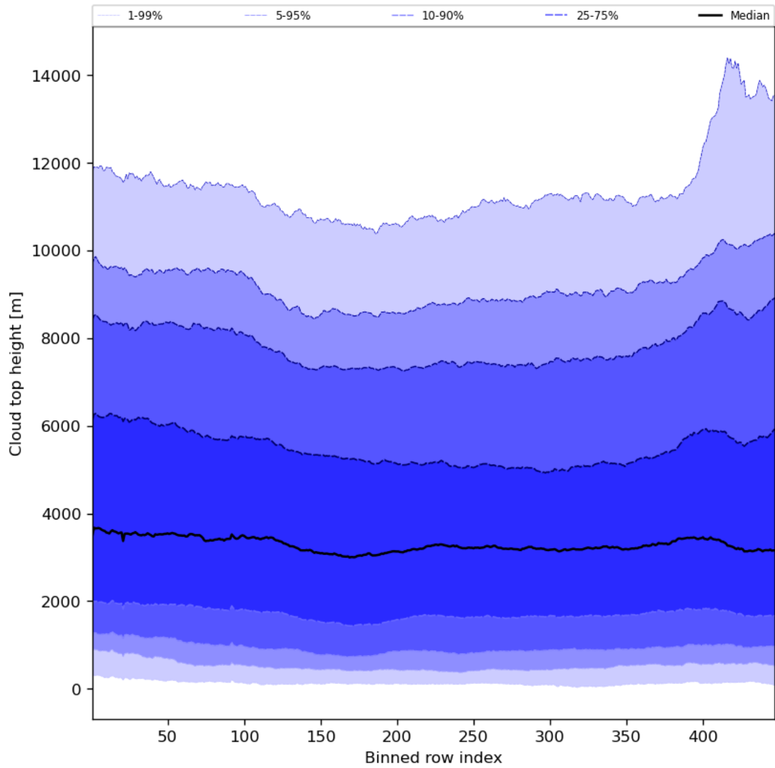
Figure 56: Along track statistics of “Cloud top height” for 2024-06-06 to 2024-06-08
