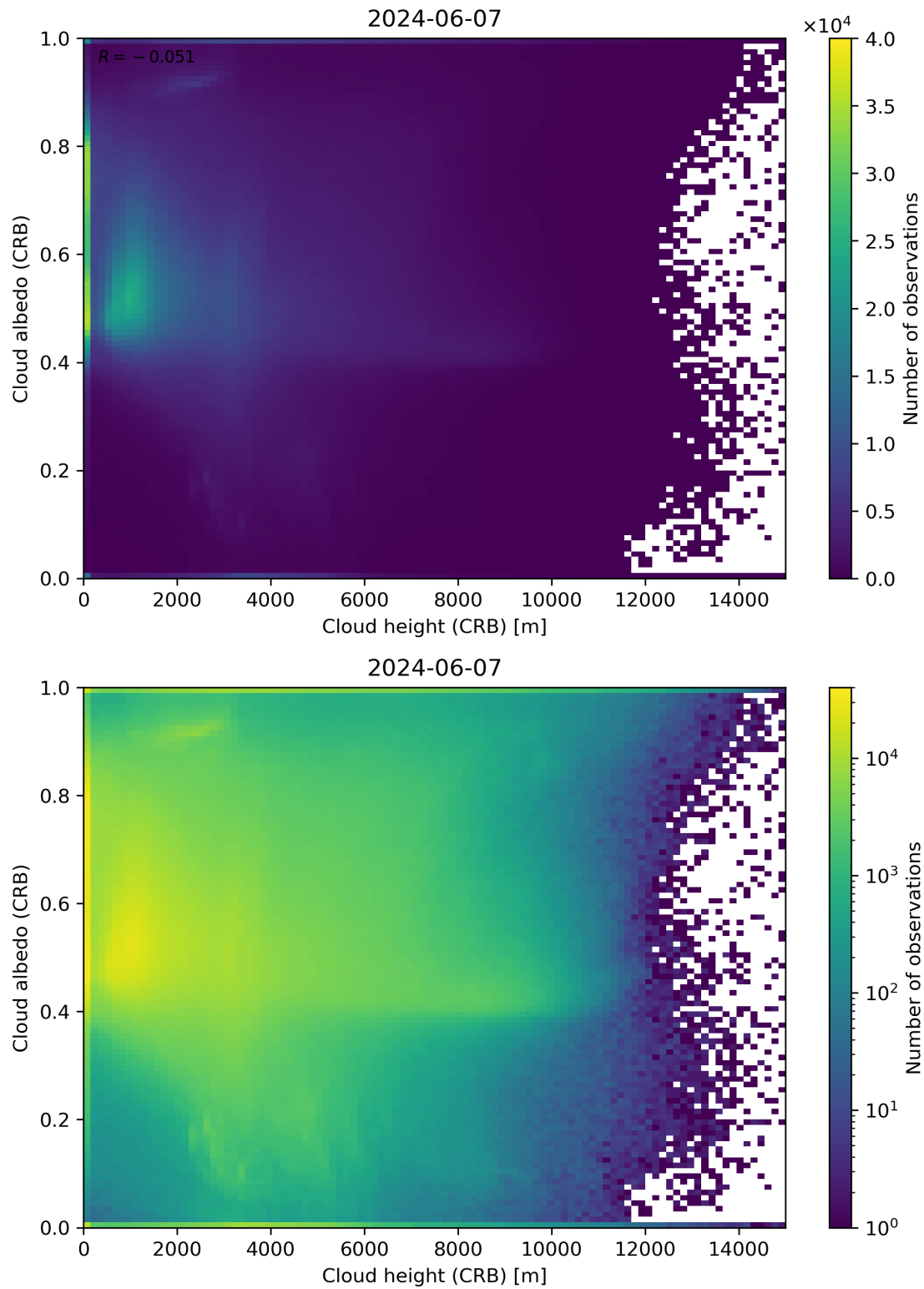
Figure 80: Scatter density plot of “Cloud height (CRB)” against “Cloud albedo (CRB)” for 2024-06-06 to 2024-06-08.
