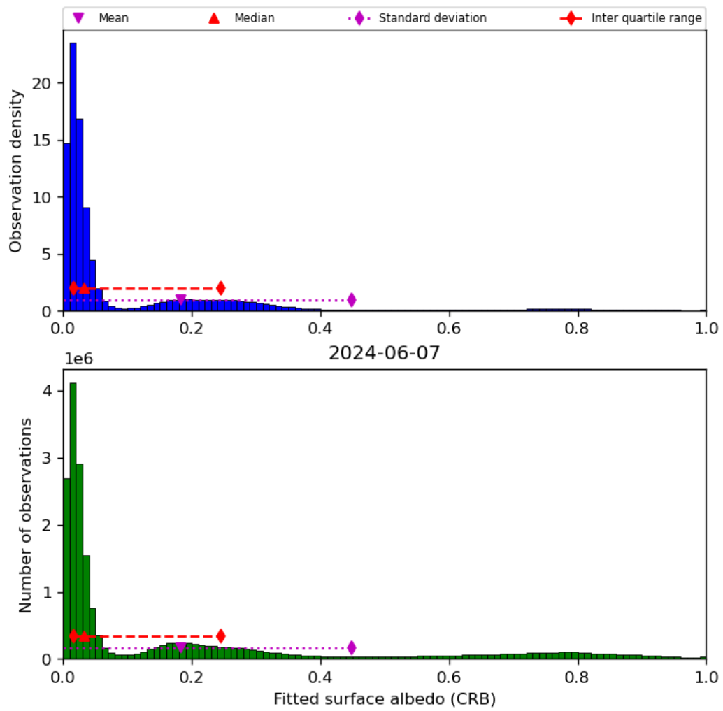
Figure 46: Histogram of “Fitted surface albedo (CRB)” for 2024-06-06 to 2024-06-08
