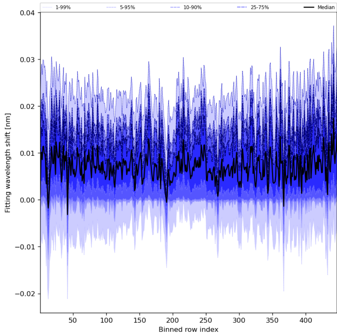
Figure 65: Along track statistics of “Fitting wavelength shift” for 2024-06-06 to 2024-06-08
