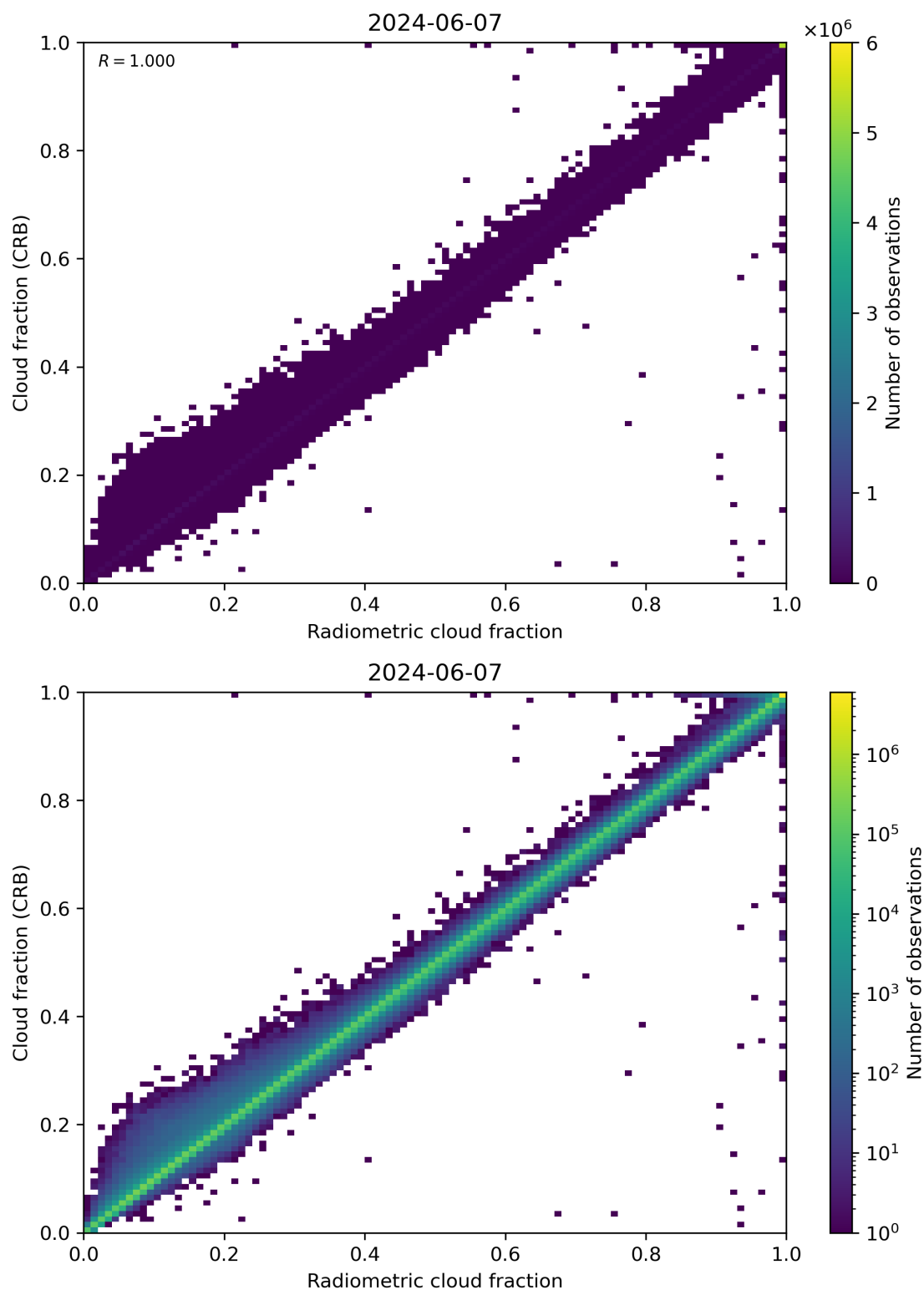
Figure 73: Scatter density plot of “Radiometric cloud fraction” against “Cloud fraction (CRB)” for 2024-06-06 to 2024-06-08.
