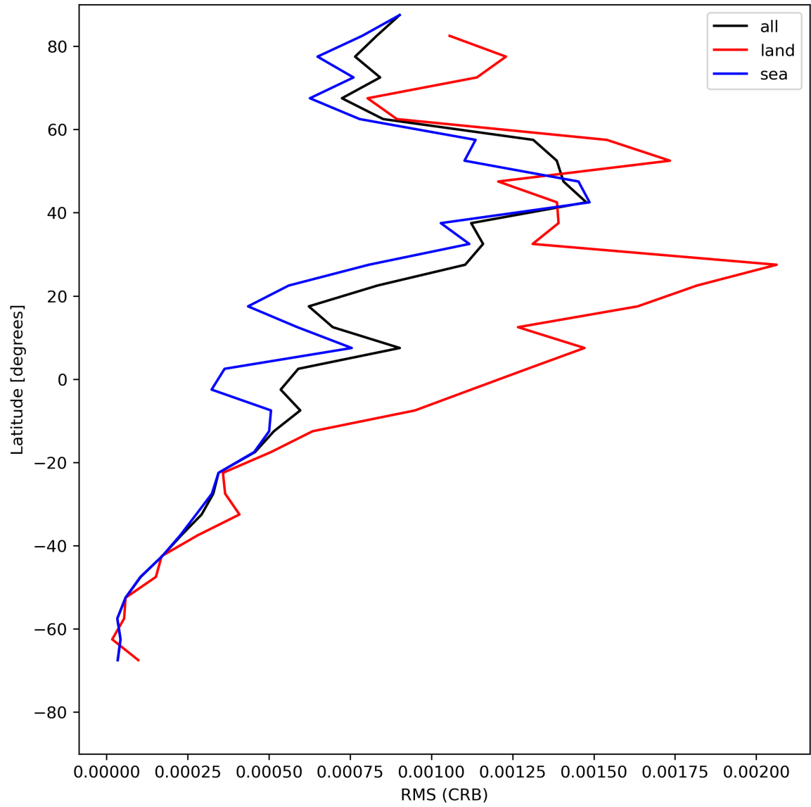
Figure 32: Zonal average of “RMS (CRB)” for 2024-06-06 to 2024-06-08.
