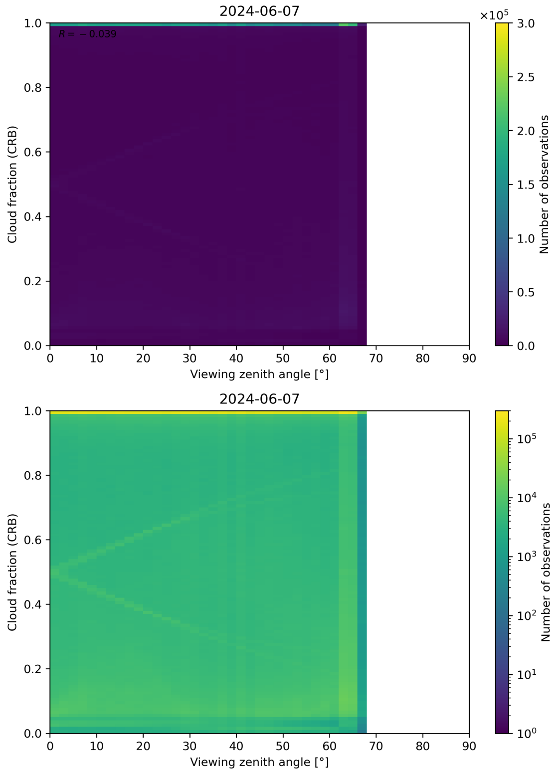
Figure 109: Scatter density plot of “Viewing zenith angle” against “Cloud fraction (CRB)” for 2024-06-06 to 2024-06-08.
