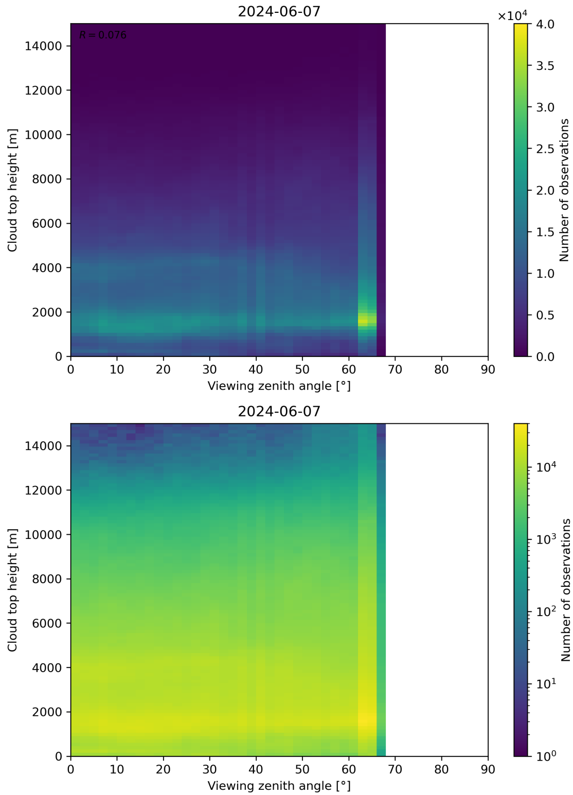
Figure 112: Scatter density plot of “Viewing zenith angle” against “Cloud top height” for 2024-06-06 to 2024-06-08.
