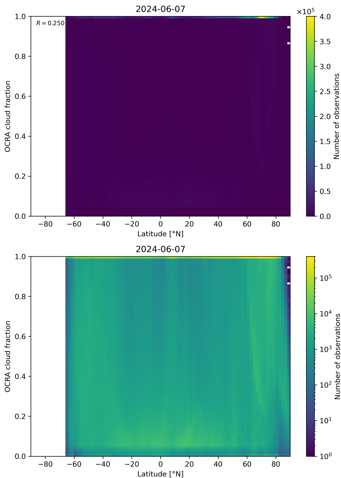
Figure 93: Scatter density plot of “Latitude” against “OCRA cloud fraction” for 2024-06-06 to 2024-06-08.
