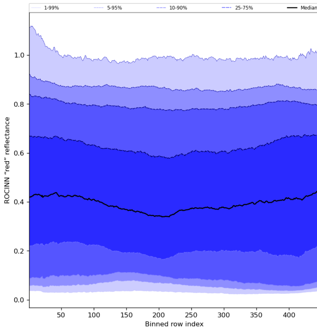
Figure 69: Along track statistics of “ROCINN “red” reflectance” for 2024-06-06 to 2024-06-08
