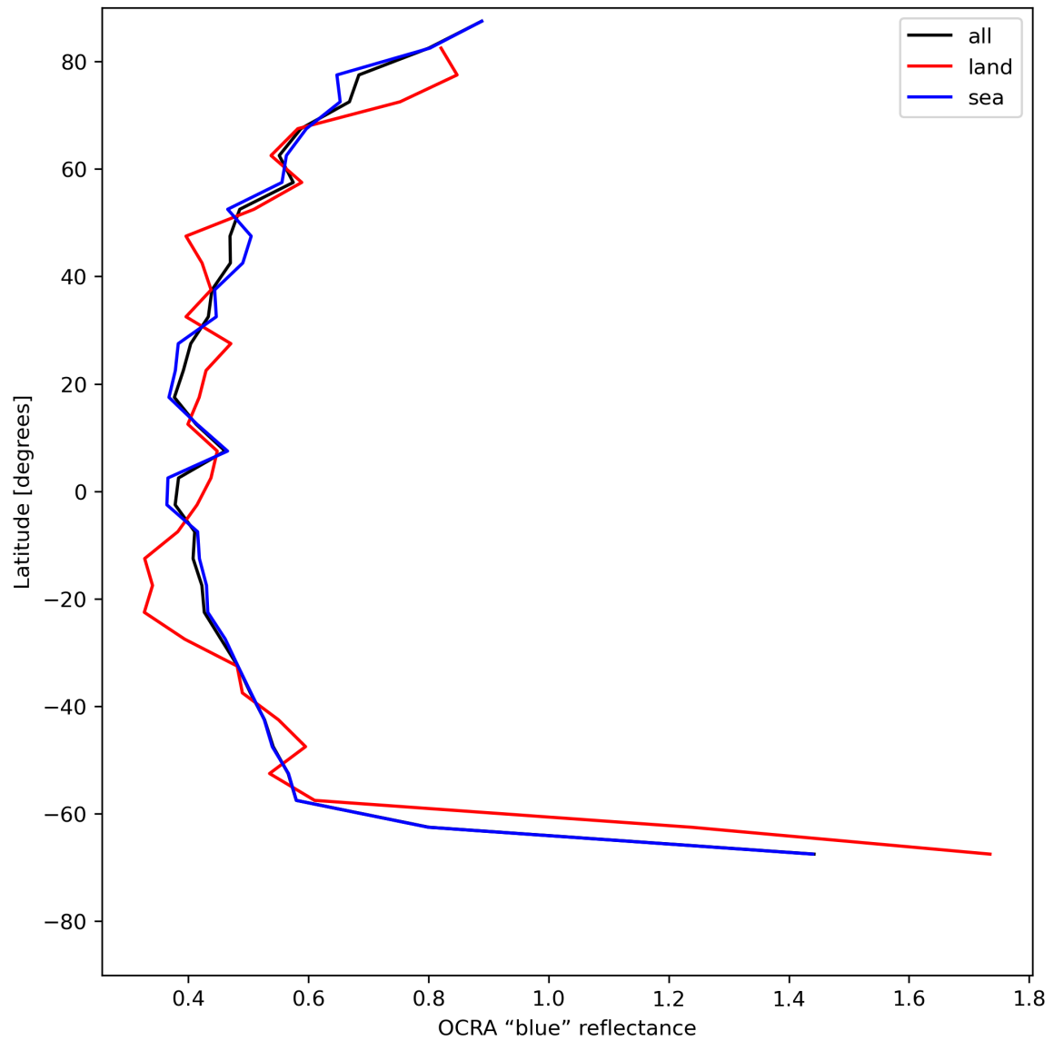
Figure 35: Zonal average of “OCRA “blue” reflectance” for 2024-06-06 to 2024-06-08.
