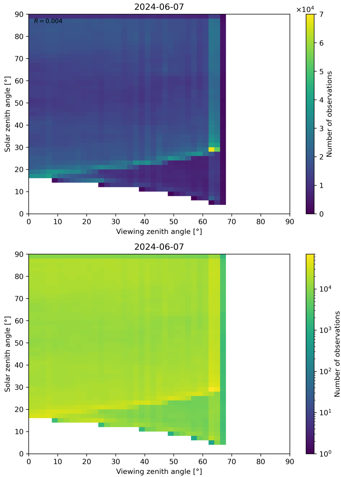
Figure 114: Scatter density plot of “Viewing zenith angle” against “Solar zenith angle” for 2024-06-06 to 2024-06-08.
