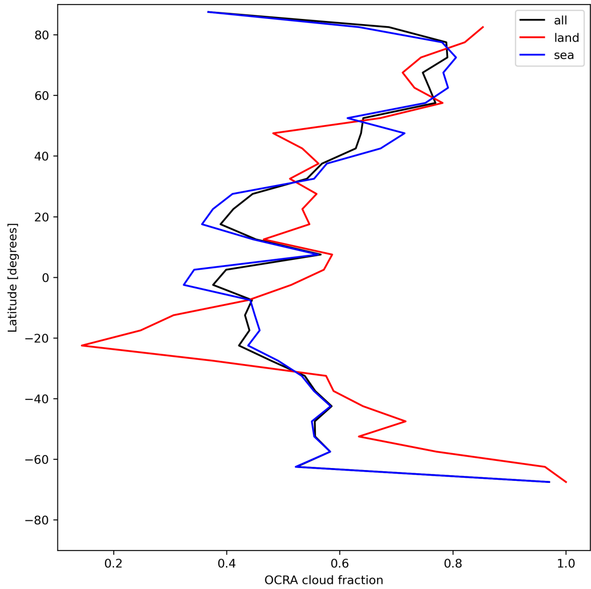
Figure 34: Zonal average of “OCRA cloud fraction” for 2024-06-06 to 2024-06-08.
