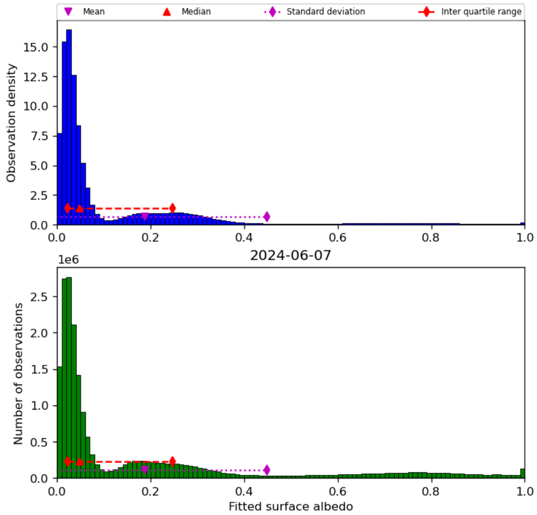
Figure 45: Histogram of “Fitted surface albedo” for 2024-06-06 to 2024-06-08
