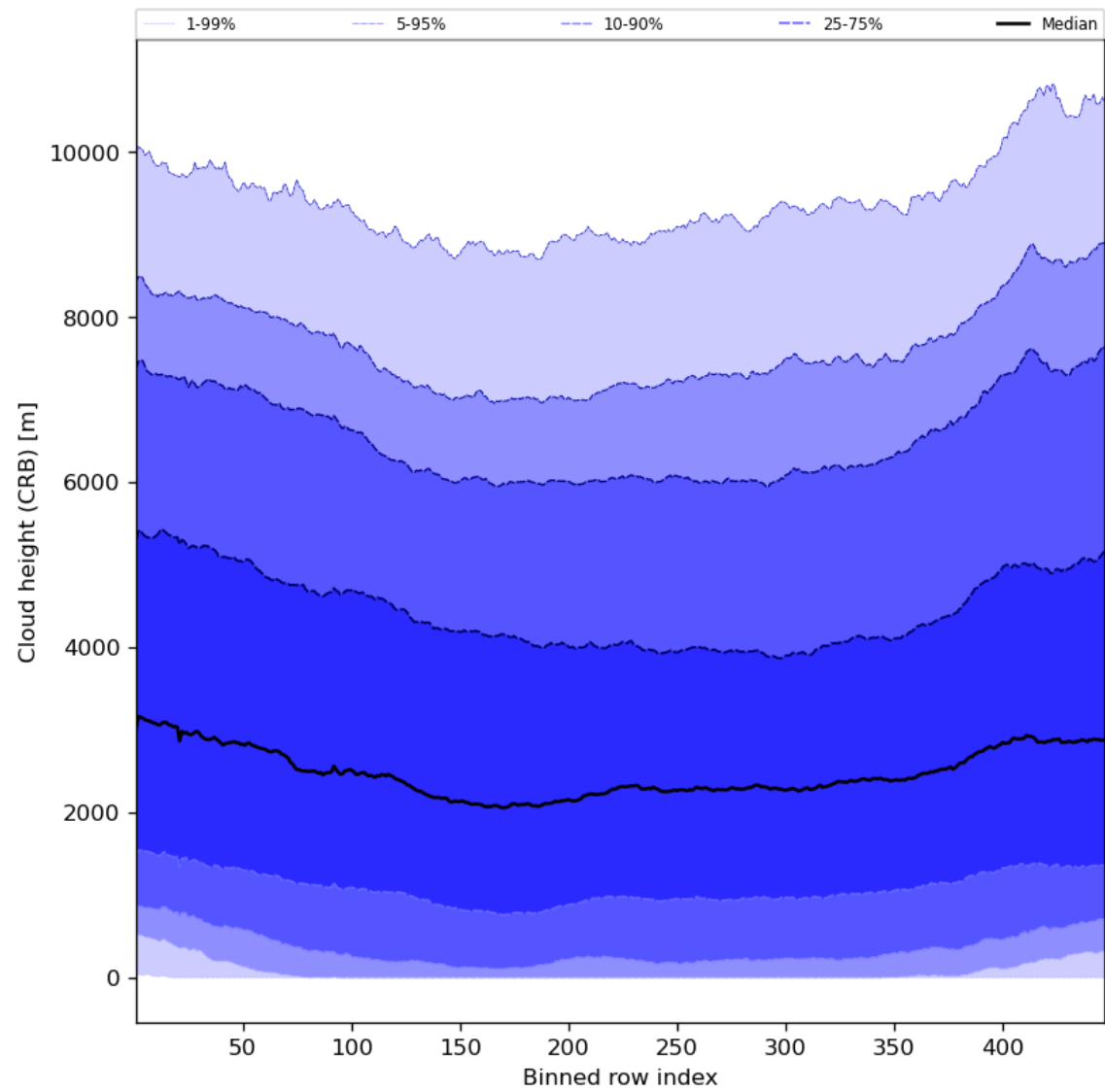
Figure 59: Along track statistics of “Cloud height (CRB)” for 2024-06-06 to 2024-06-08
