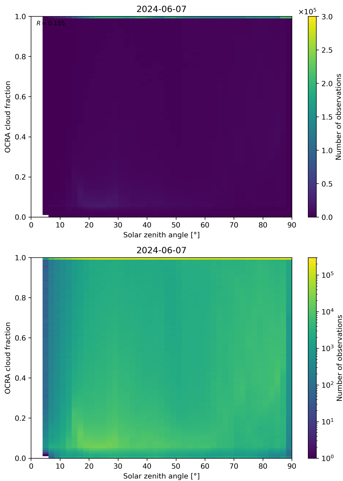
Figure 100: Scatter density plot of “Solar zenith angle” against “OCRA cloud fraction” for 2024-06-06 to 2024-06-08.
