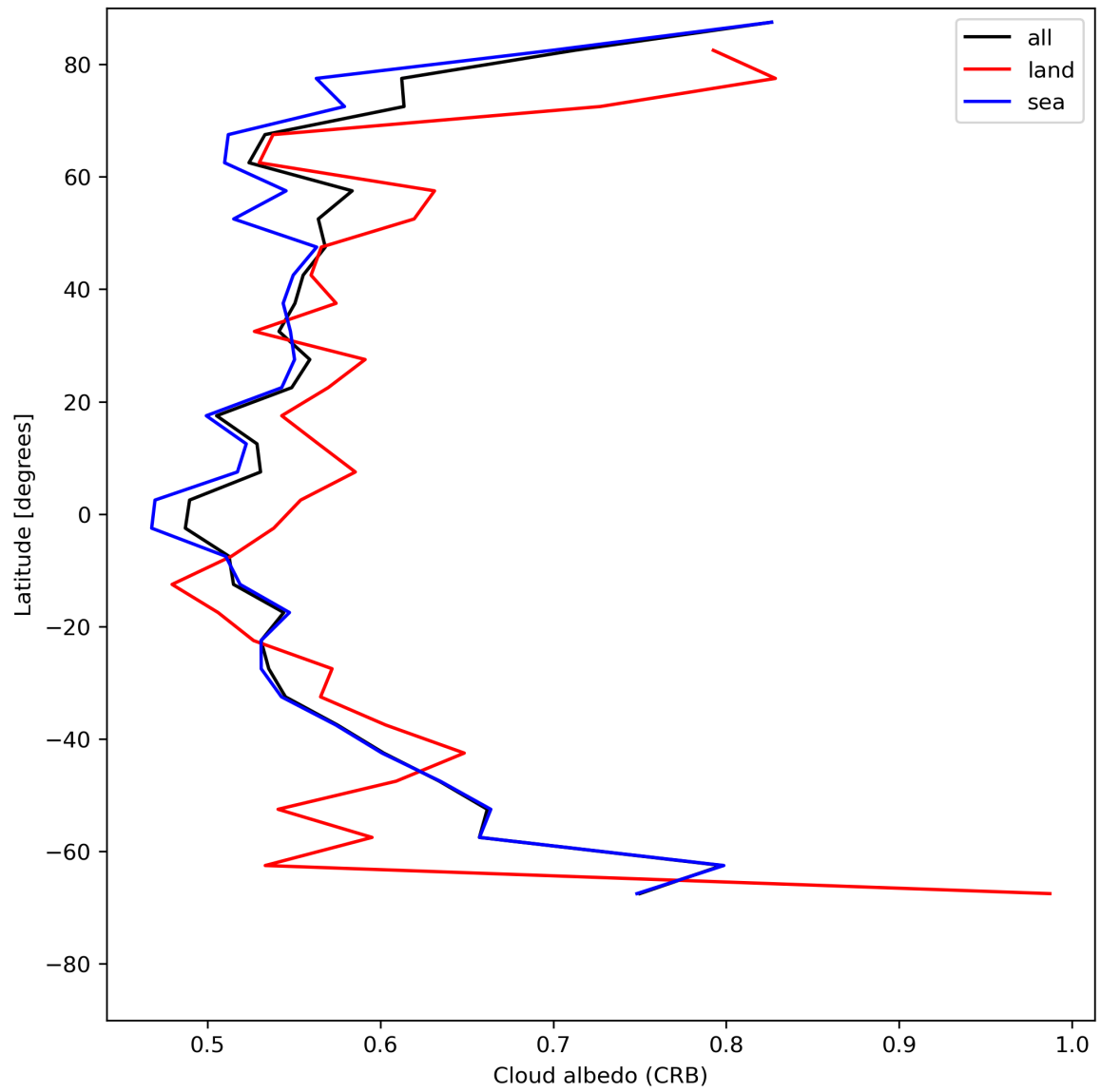
Figure 28: Zonal average of “Cloud albedo (CRB)” for 2024-06-06 to 2024-06-08.
