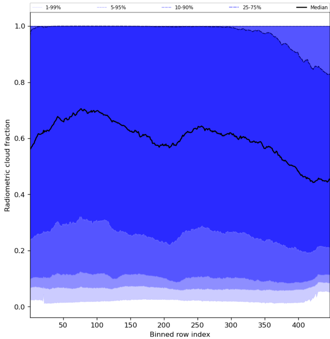
Figure 55: Along track statistics of “Radiometric cloud fraction” for 2024-06-06 to 2024-06-08
