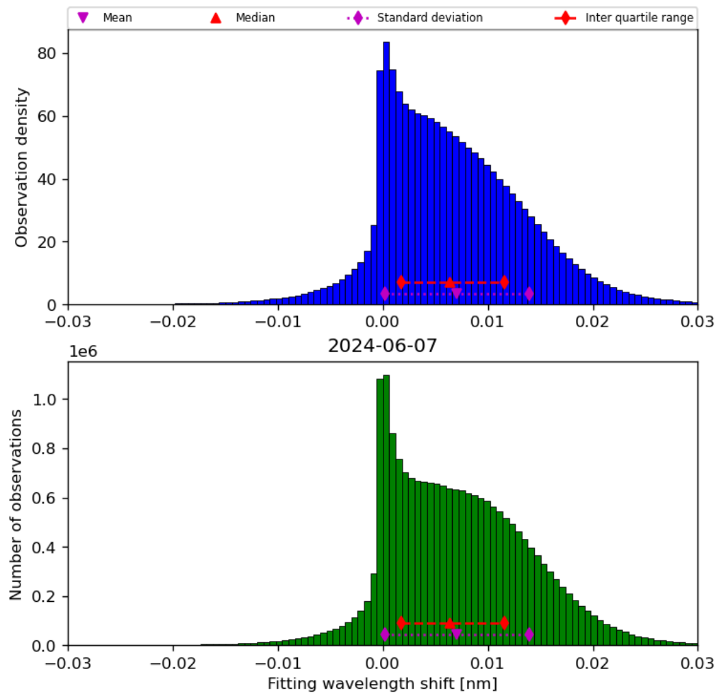
Figure 49: Histogram of “Fitting wavelength shift” for 2024-06-06 to 2024-06-08
