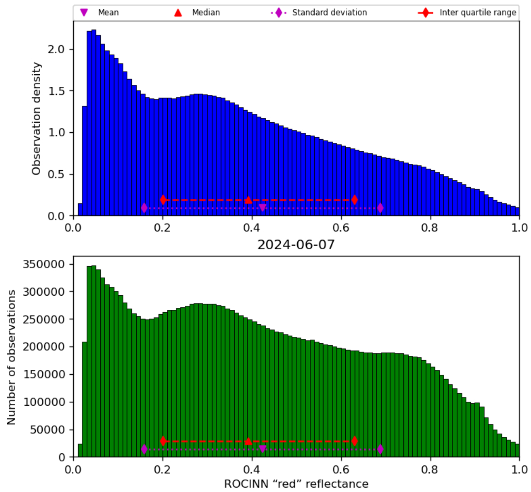
Figure 53: Histogram of “ROCINN “red” reflectance” for 2024-06-06 to 2024-06-08
