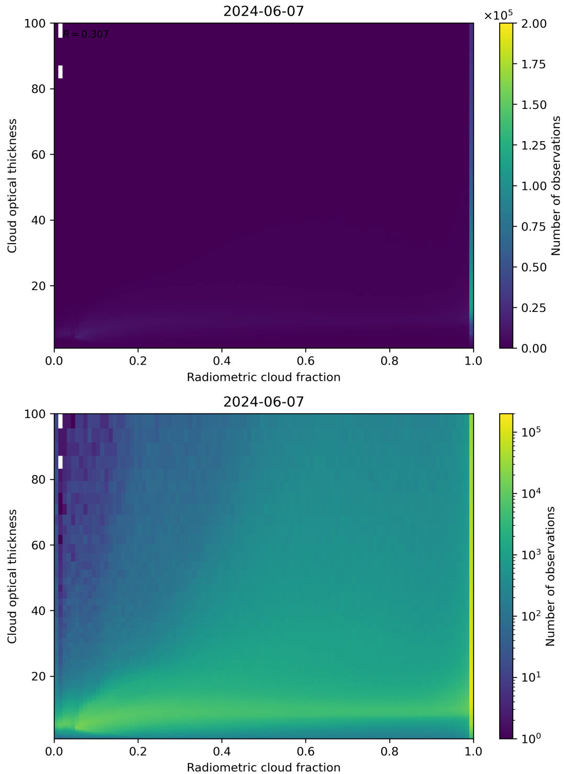
Figure 75: Scatter density plot of “Radiometric cloud fraction” against “Cloud optical thickness” for 2024-06-06 to 2024-06-08.
