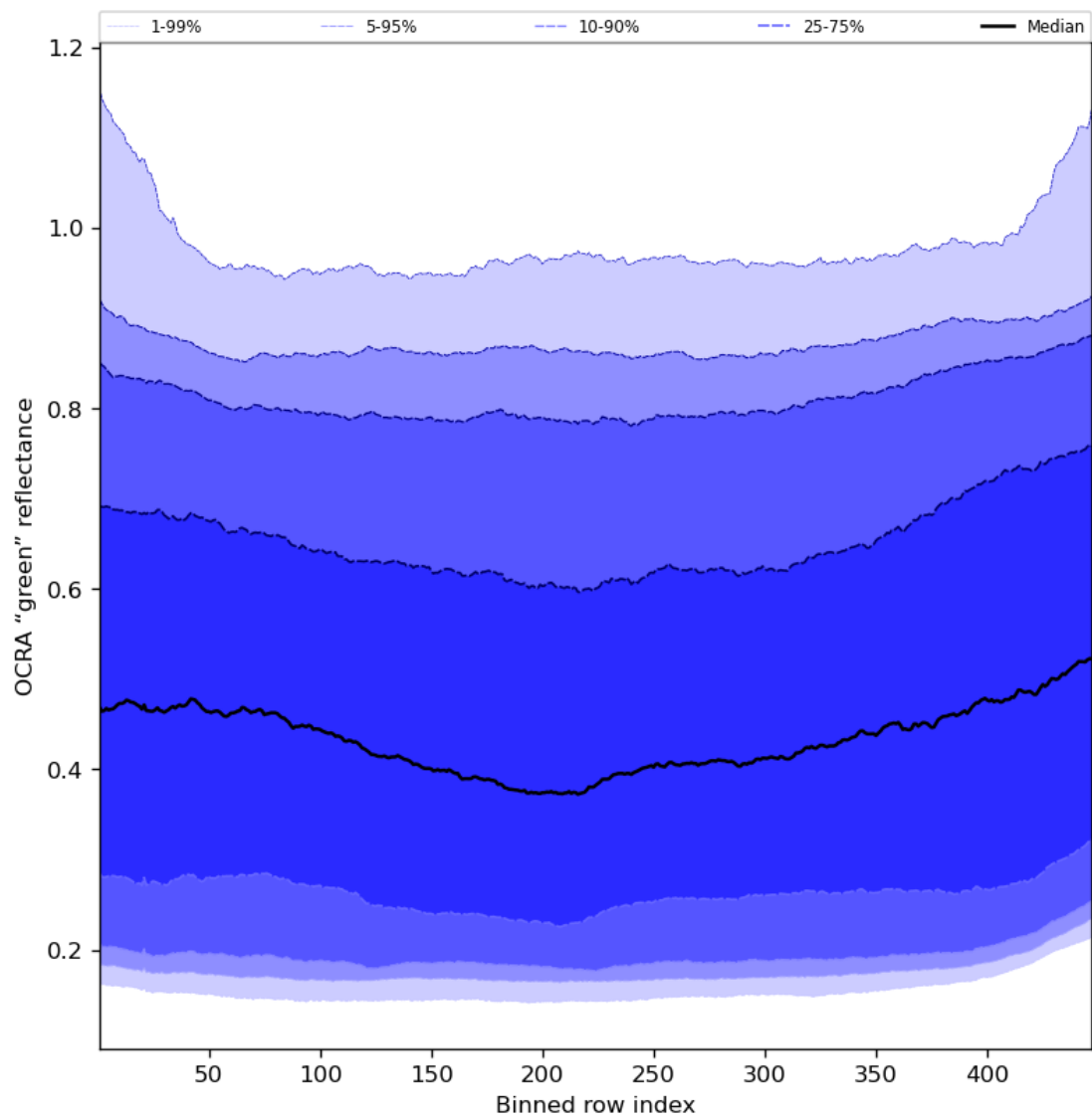
Figure 68: Along track statistics of "OCRA "green" reflectance" for 2024-06-06 to 2024-06-08
