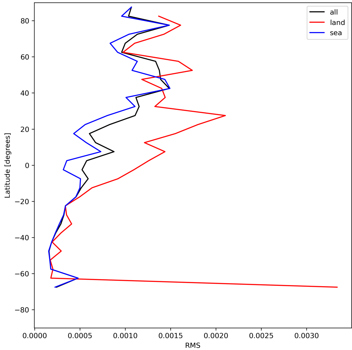
Figure 31: Zonal average of “RMS” for 2024-06-06 to 2024-06-08.
