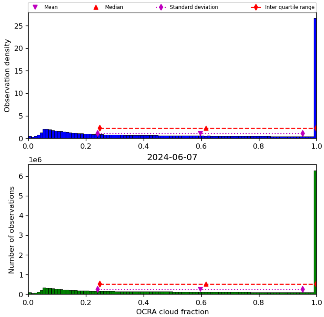
Figure 50: Histogram of “OCRA cloud fraction” for 2024-06-06 to 2024-06-08
