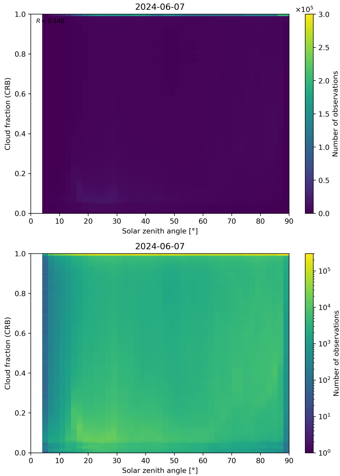
Figure 101: Scatter density plot of “Solar zenith angle” against “Cloud fraction (CRB)” for 2024-06-06 to 2024-06-08.
