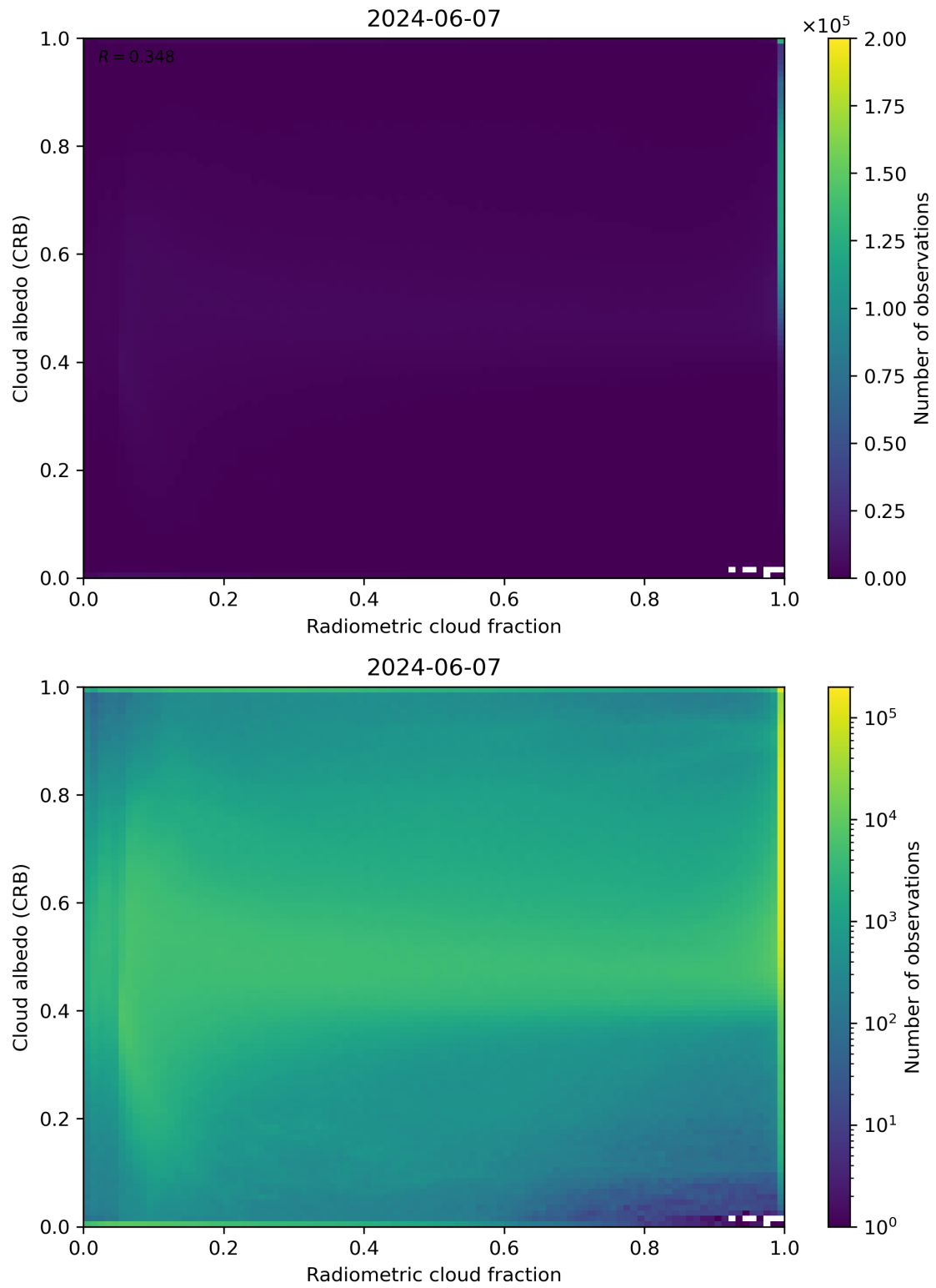
Figure 71: Scatter density plot of “Radiometric cloud fraction” against “Cloud albedo (CRB)” for 2024-06-06 to 2024-06-08.
