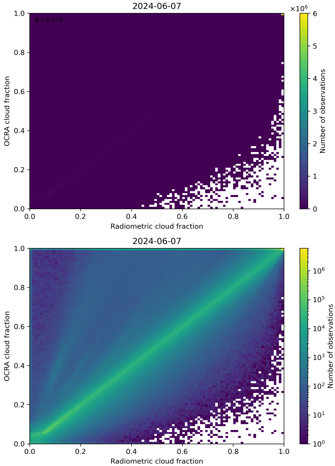
Figure 72: Scatter density plot of “Radiometric cloud fraction” against “OCRA cloud fraction” for 2024-06-06 to 2024-06-08.
