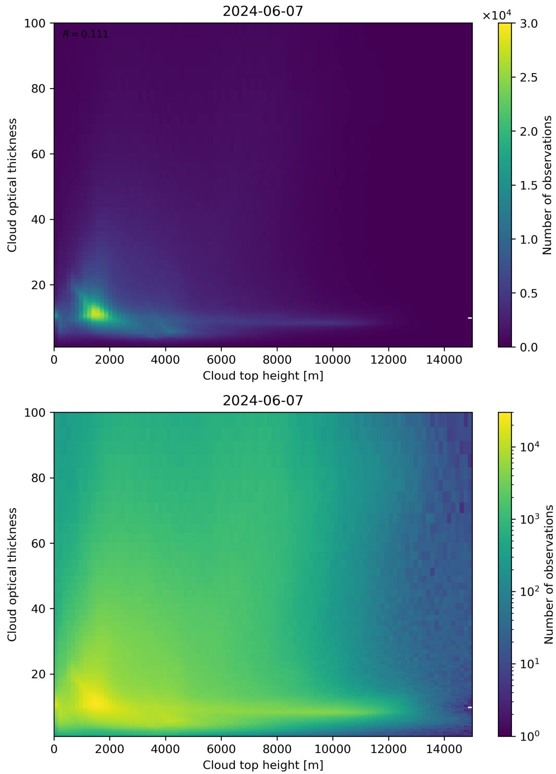
Figure 90: Scatter density plot of “Cloud top height” against “Cloud optical thickness” for 2024-06-06 to 2024-06-08.
