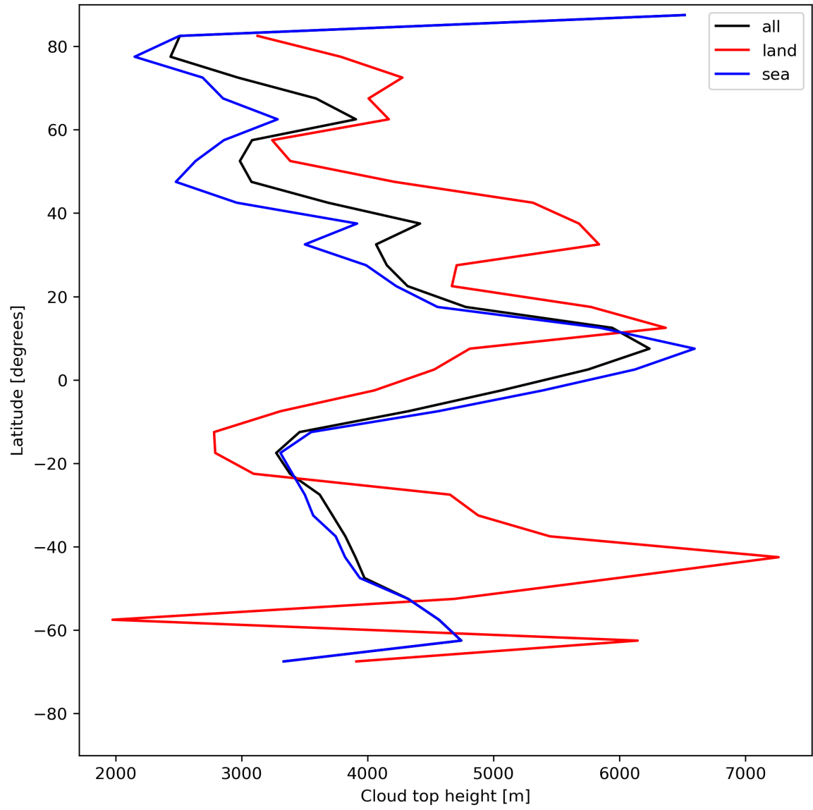
Figure 24: Zonal average of “Cloud top height” for 2024-06-06 to 2024-06-08.
