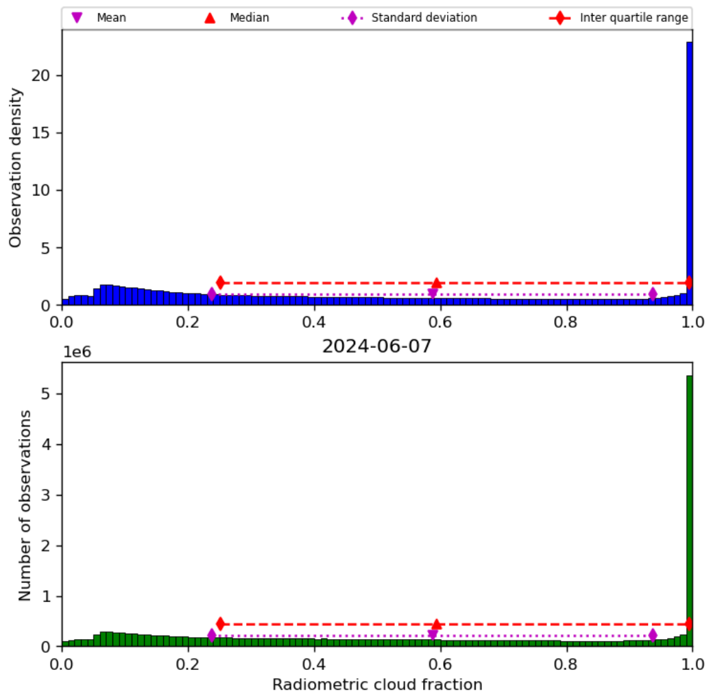
Figure 39: Histogram of “Radiometric cloud fraction” for 2024-06-06 to 2024-06-08
