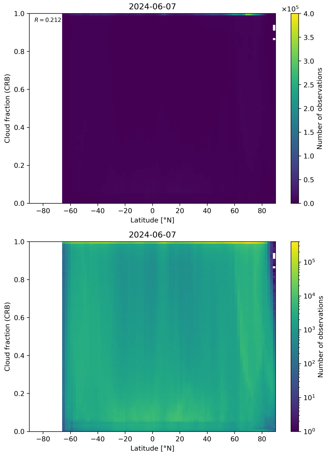
Figure 94: Scatter density plot of “Latitude” against “Cloud fraction (CRB)” for 2024-06-06 to 2024-06-08.
