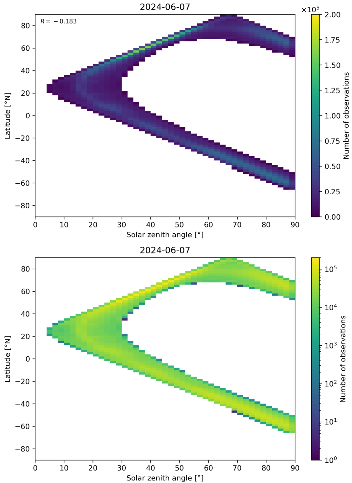
Figure 105: Scatter density plot of “Solar zenith angle” against “Latitude” for 2024-06-06 to 2024-06-08.
