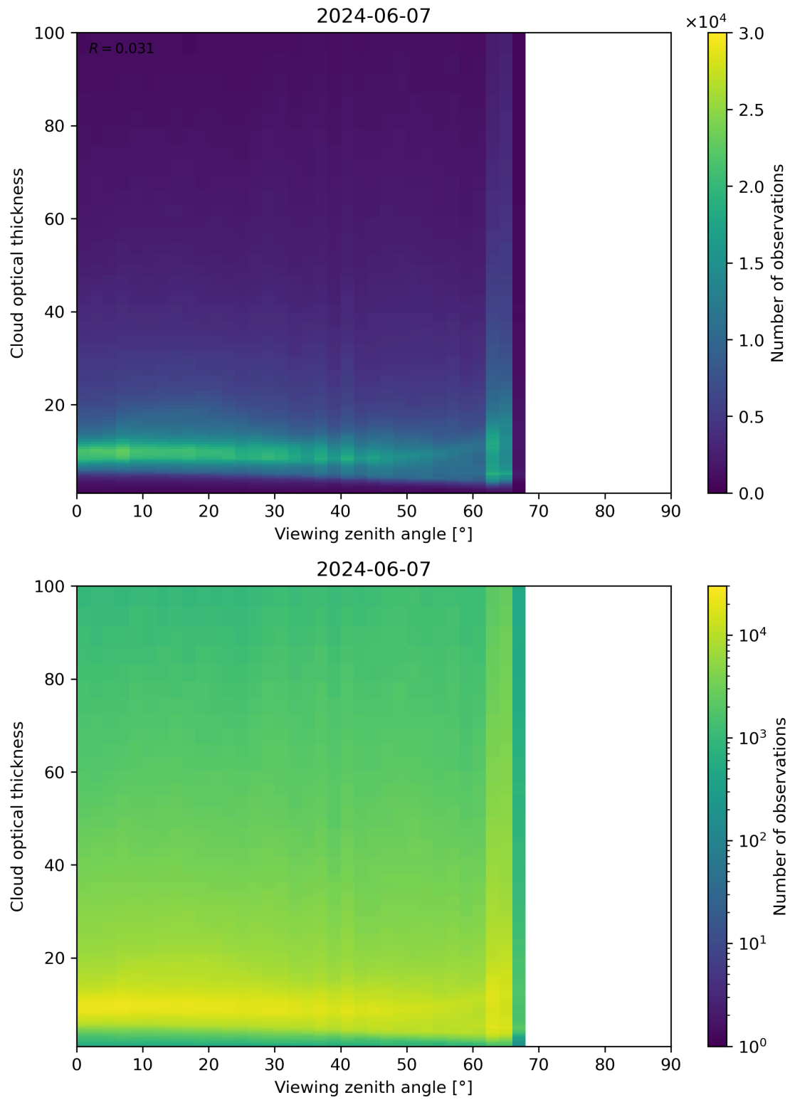
Figure 111: Scatter density plot of “Viewing zenith angle” against “Cloud optical thickness” for 2024-06-06 to 2024-06-08.
