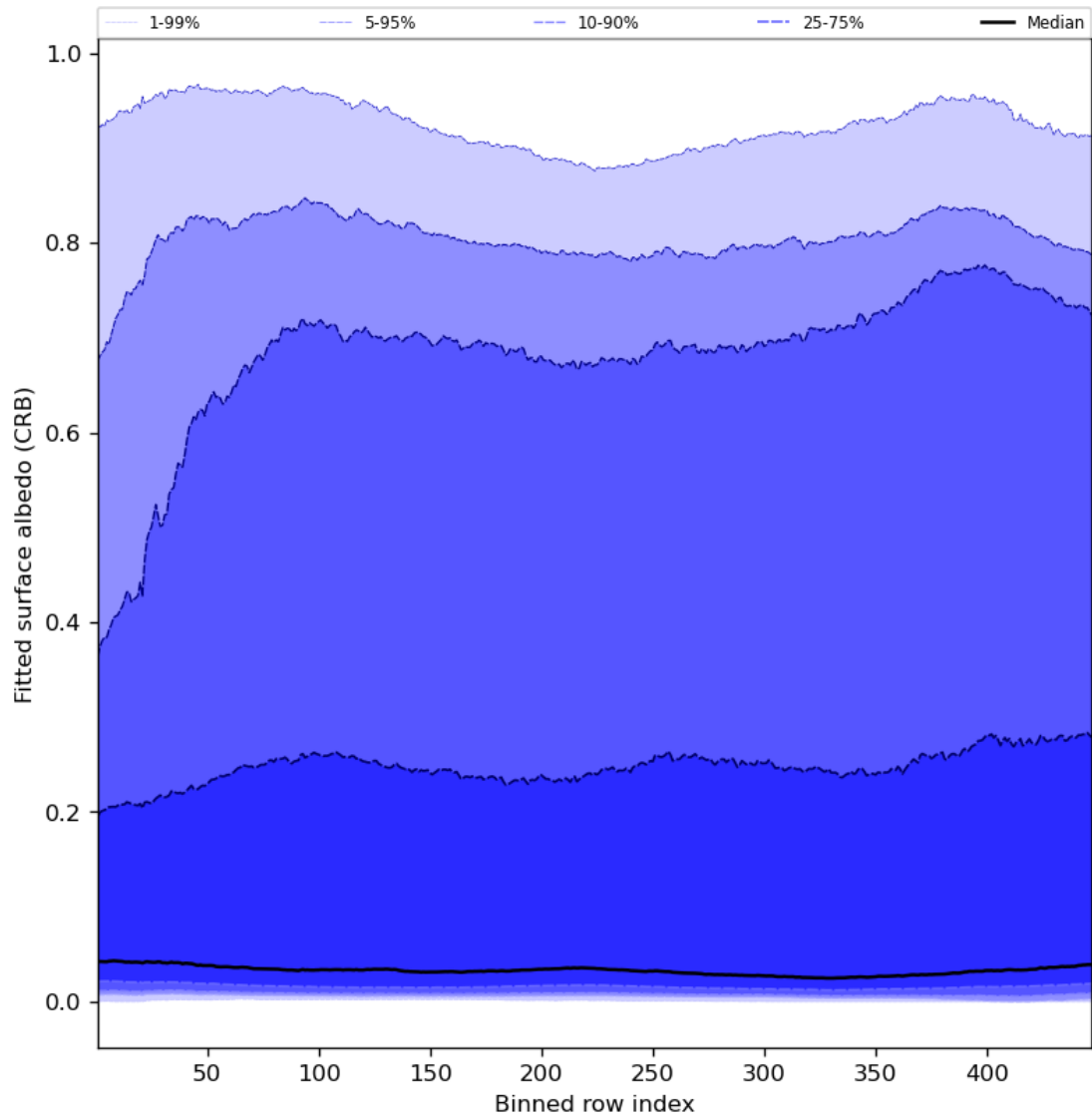
Figure 62: Along track statistics of “Fitted surface albedo (CRB)” for 2024-06-06 to 2024-06-08
