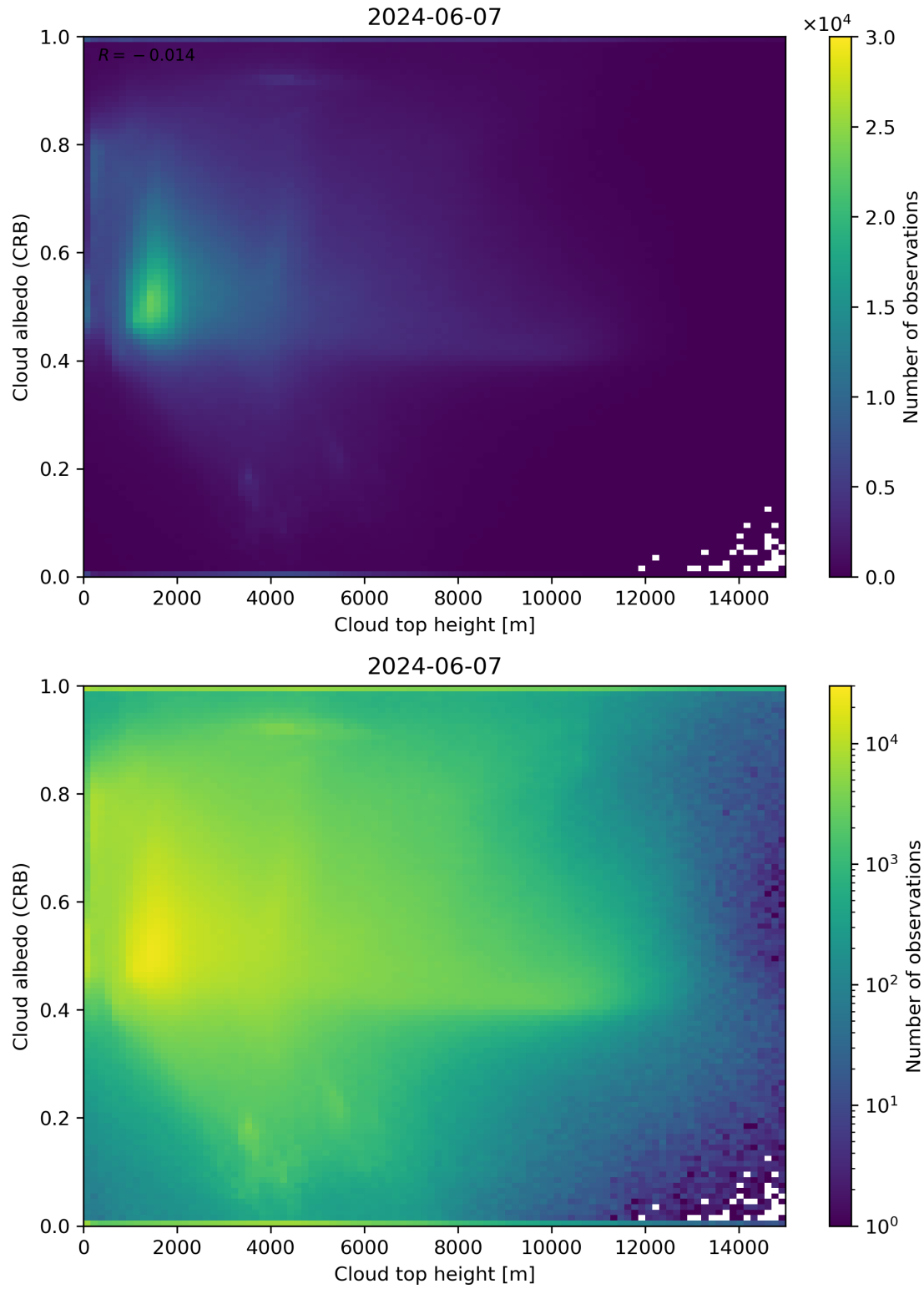
Figure 86: Scatter density plot of “Cloud top height” against “Cloud albedo (CRB)” for 2024-06-06 to 2024-06-08.
