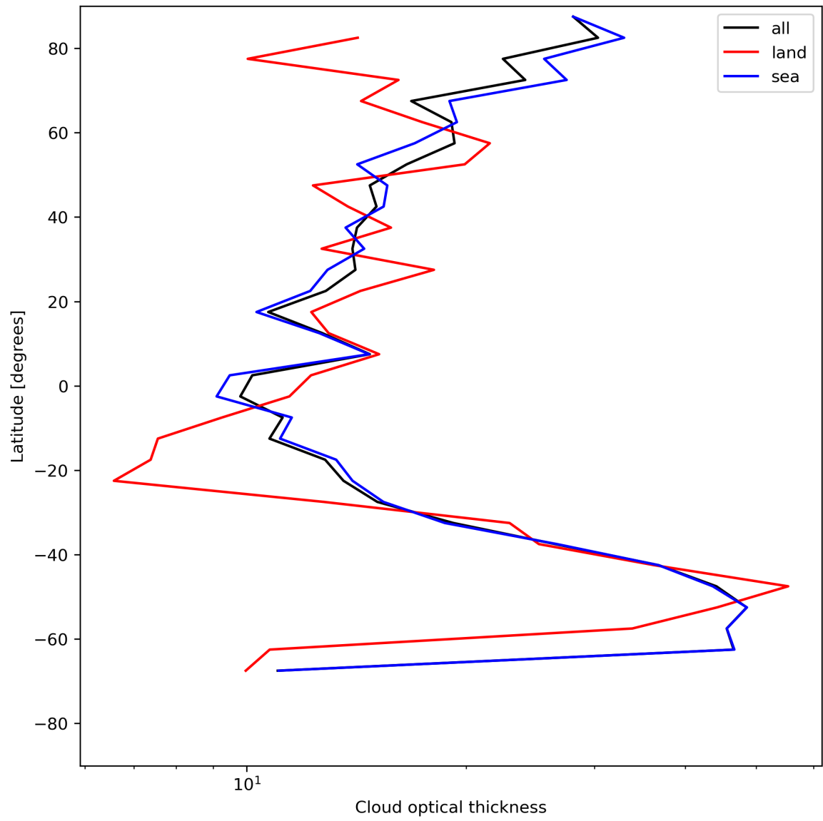
Figure 25: Zonal average of “Cloud optical thickness” for 2024-06-06 to 2024-06-08.
