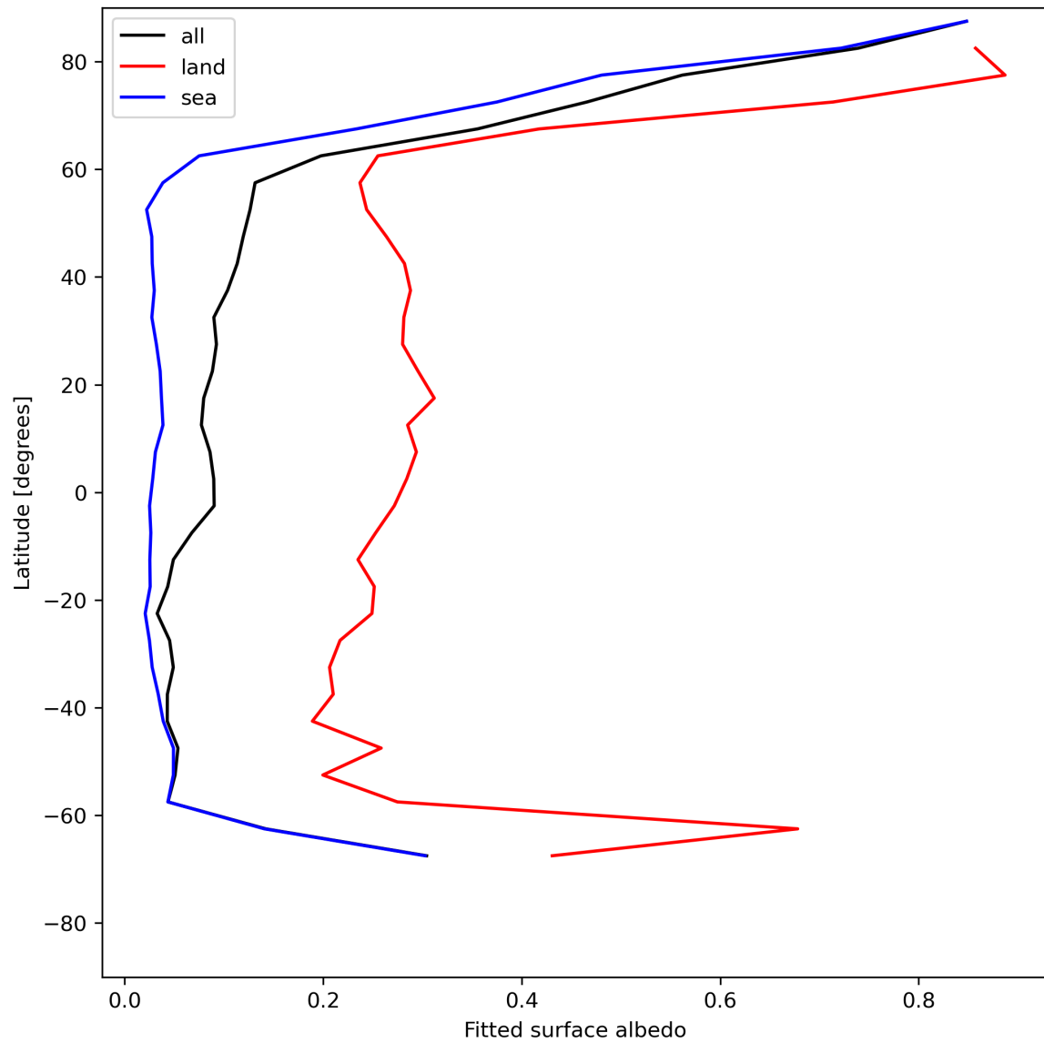
Figure 29: Zonal average of “Fitted surface albedo” for 2024-06-06 to 2024-06-08.
