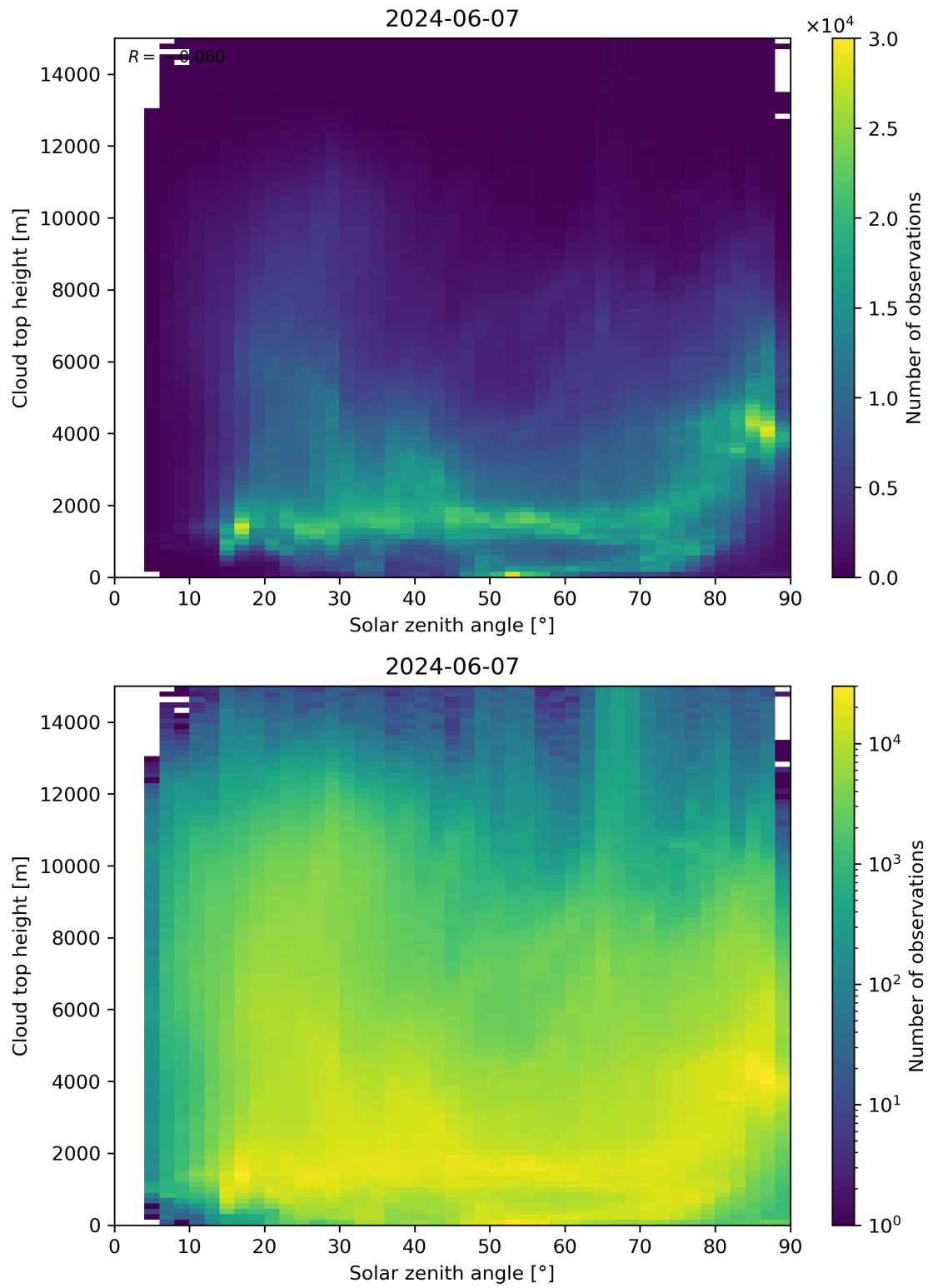
Figure 104: Scatter density plot of “Solar zenith angle” against “Cloud top height” for 2024-06-06 to 2024-06-08.
