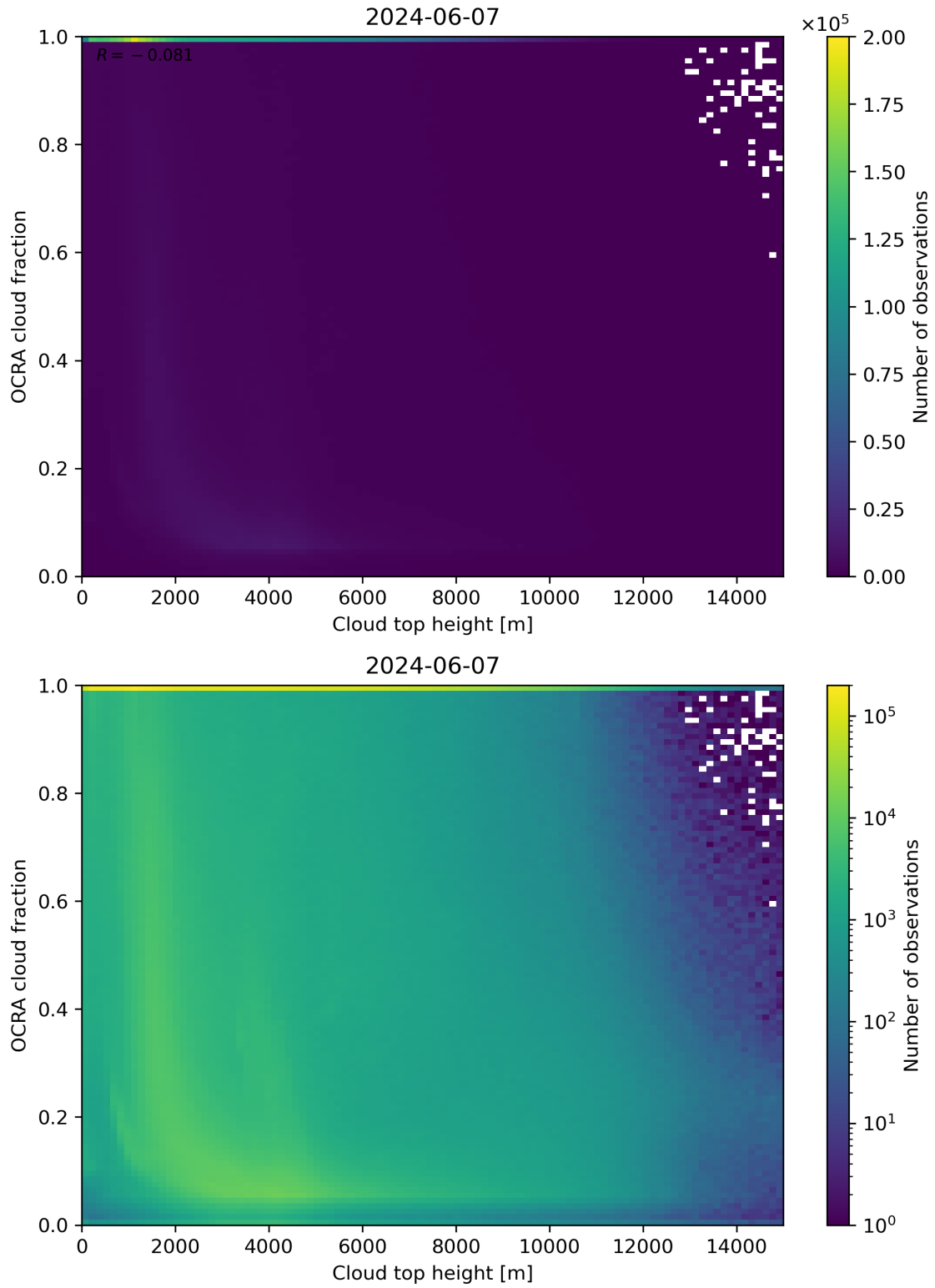
Figure 87: Scatter density plot of “Cloud top height” against “OCRA cloud fraction” for 2024-06-06 to 2024-06-08.
