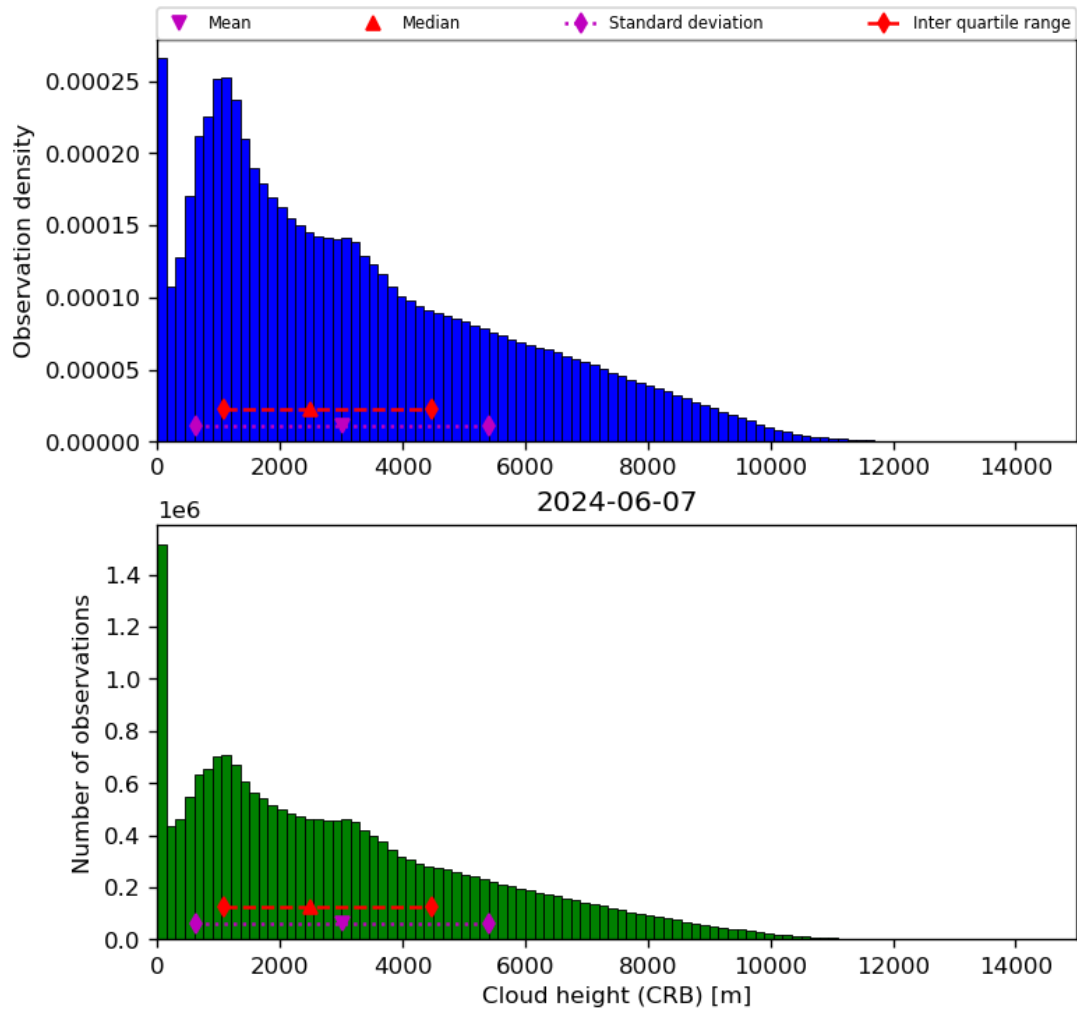
Figure 43: Histogram of “Cloud height (CRB)” for 2024-06-06 to 2024-06-08
