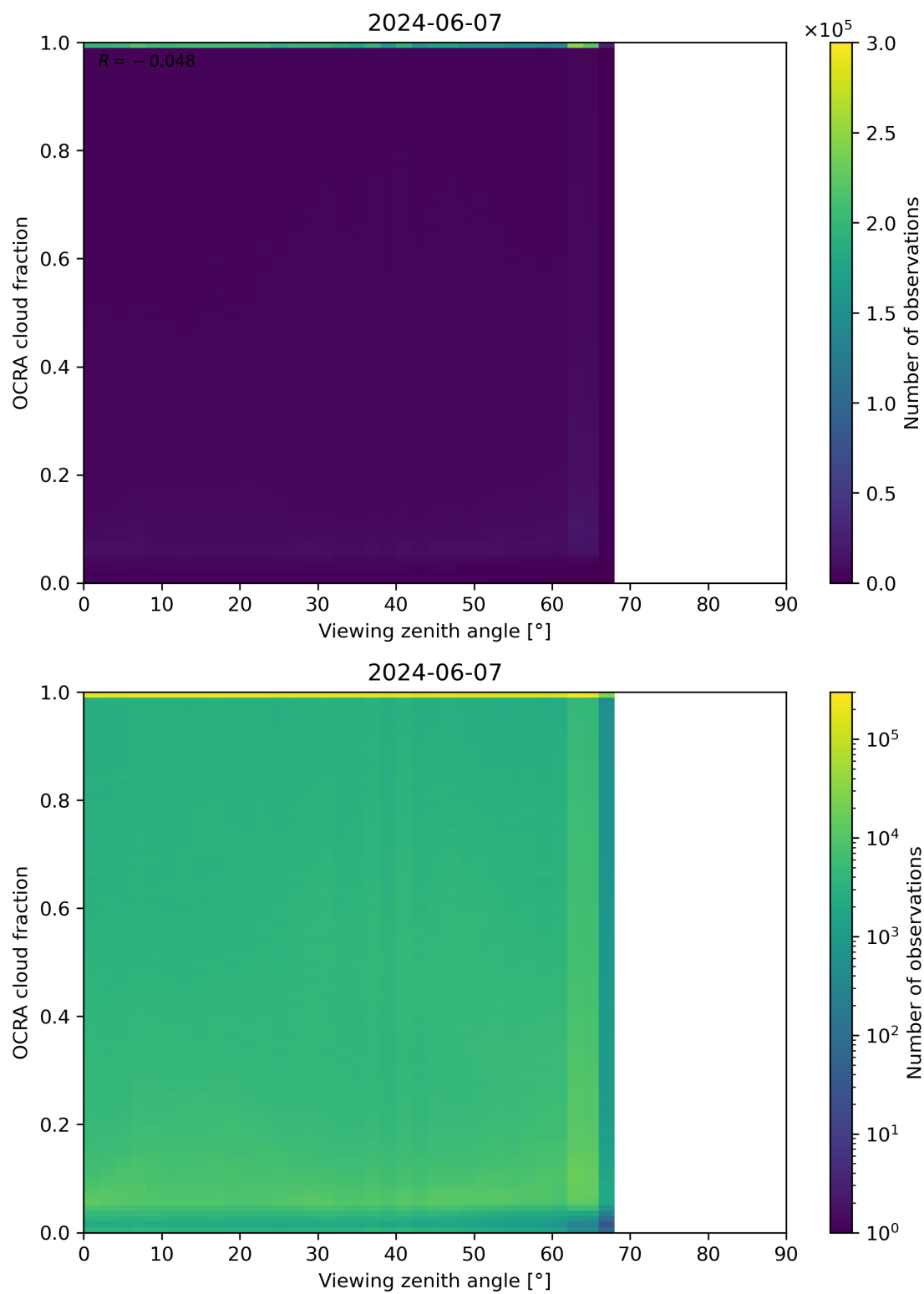
Figure 108: Scatter density plot of “Viewing zenith angle” against “OCRA cloud fraction” for 2024-06-06 to 2024-06-08.
