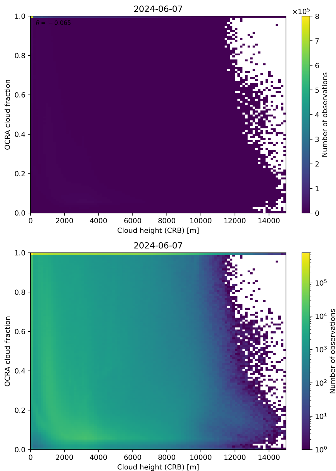
Figure 81: Scatter density plot of “Cloud height (CRB)” against “OCRA cloud fraction” for 2024-06-06 to 2024-06-08.
