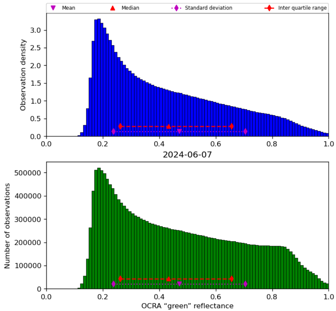
Figure 52: Histogram of “OCRA “green” reflectance” for 2024-06-06 to 2024-06-08
