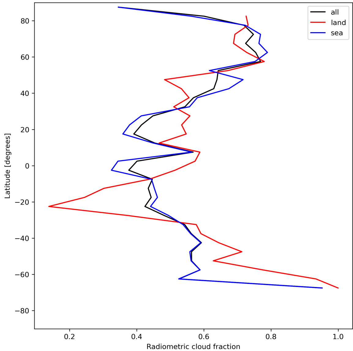
Figure 23: Zonal average of “Radiometric cloud fraction” for 2024-06-06 to 2024-06-08.
