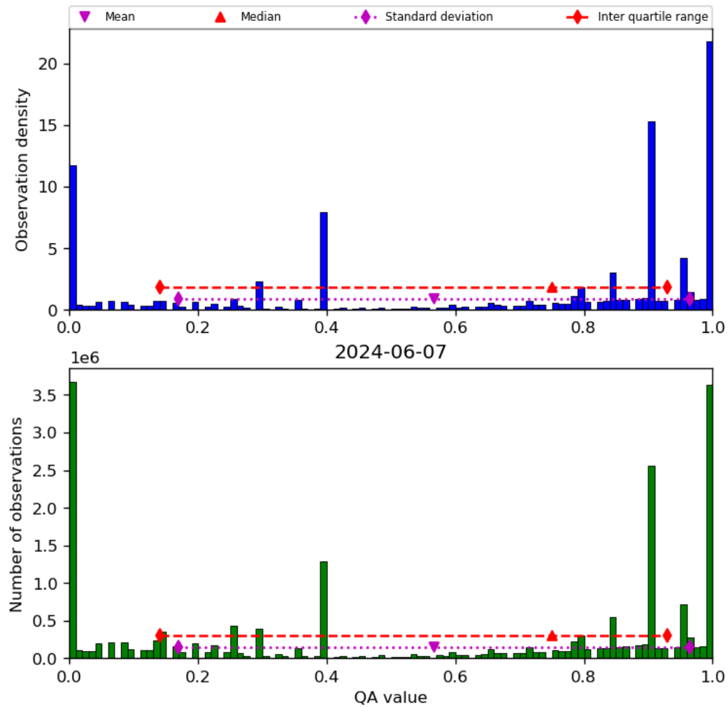
Figure 38: Histogram of “QA value” for 2024-06-06 to 2024-06-08
