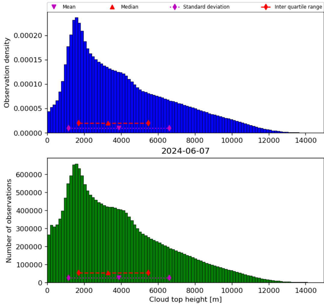
Figure 40: Histogram of “Cloud top height” for 2024-06-06 to 2024-06-08
