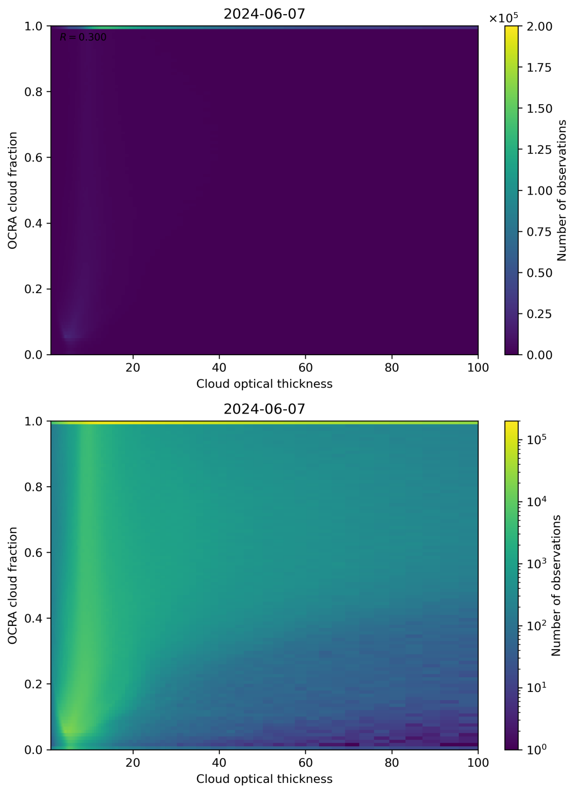
Figure 83: Scatter density plot of “Cloud optical thickness” against “OCRA cloud fraction” for 2024-06-06 to 2024-06-08.
