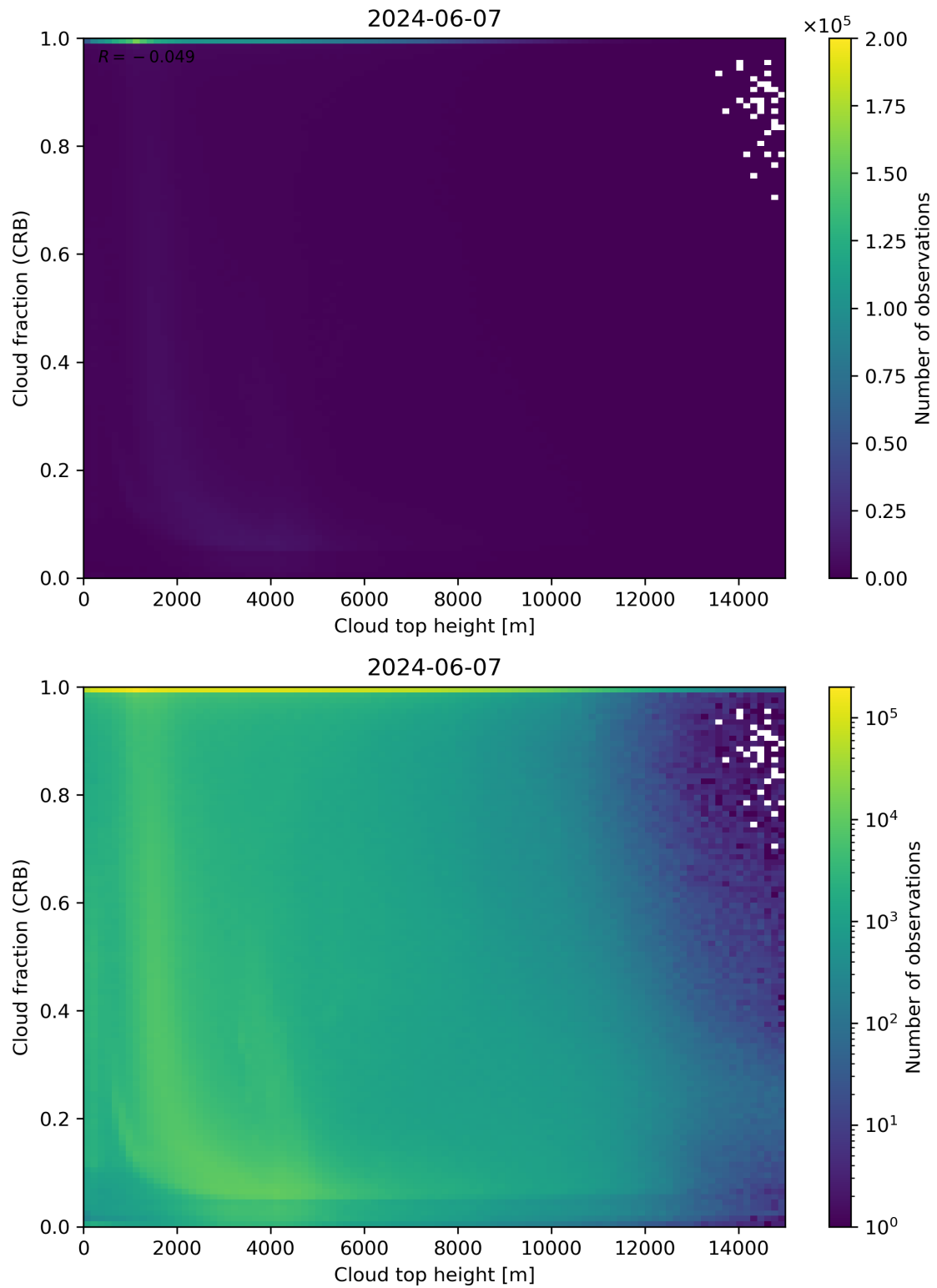
Figure 88: Scatter density plot of “Cloud top height” against “Cloud fraction (CRB)” for 2024-06-06 to 2024-06-08.
