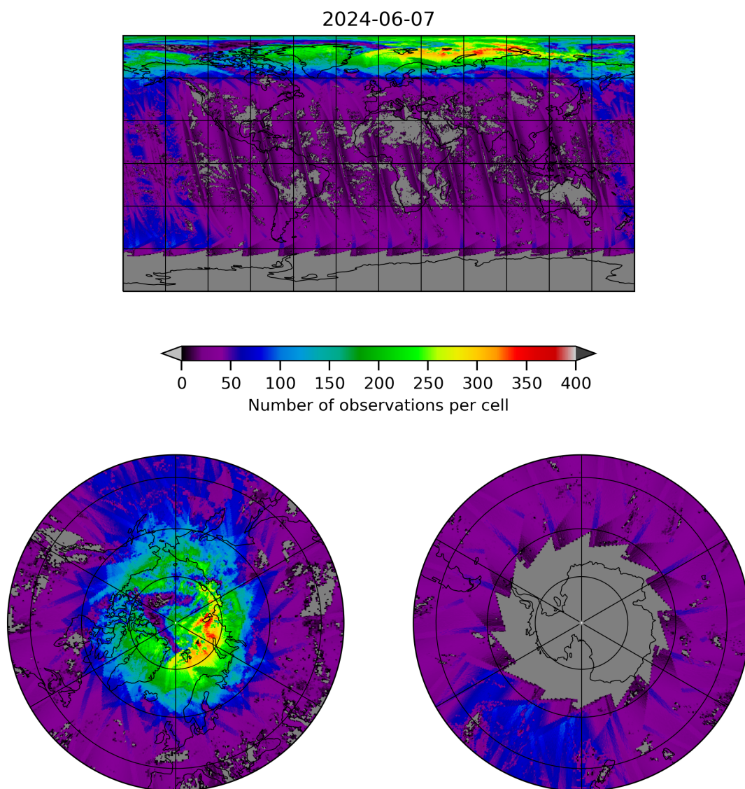
Figure 21: Map of the number of observations for 2024-06-06 to 2024-06-08
