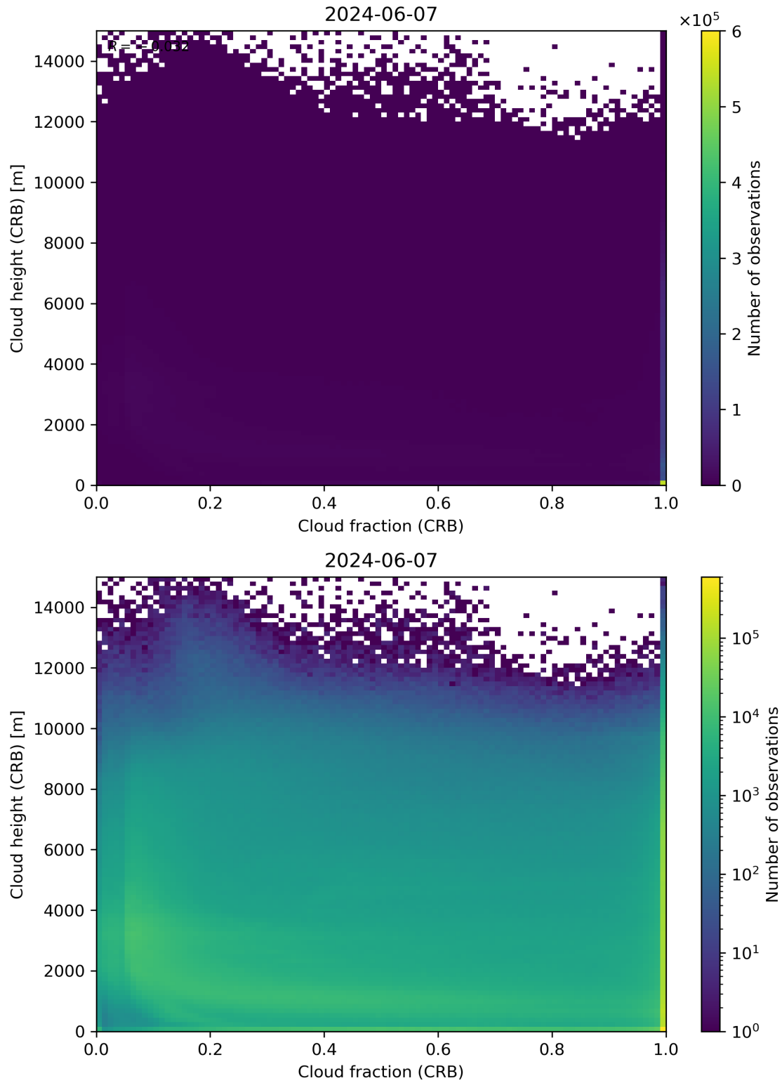
Figure 79: Scatter density plot of “Cloud fraction (CRB)” against “Cloud height (CRB)” for 2024-06-06 to 2024-06-08.
