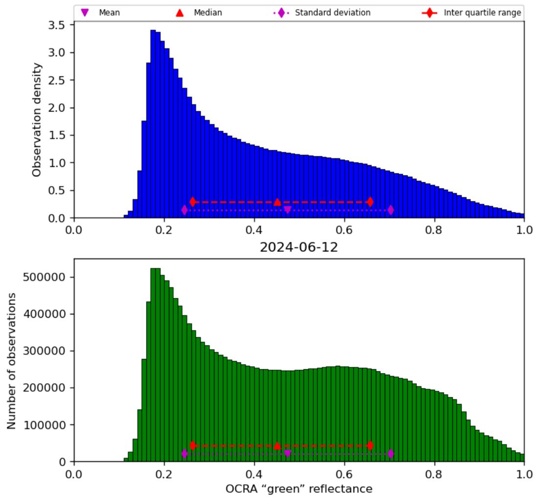
Figure 52: Histogram of “OCRA “green” reflectance” for 2024-06-11 to 2024-06-13
