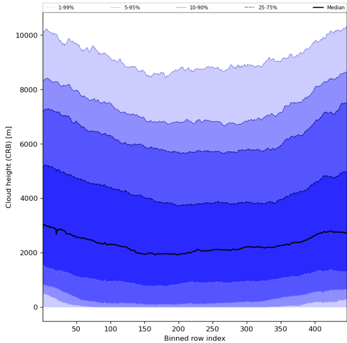
Figure 59: Along track statistics of “Cloud height (CRB)” for 2024-06-11 to 2024-06-13
