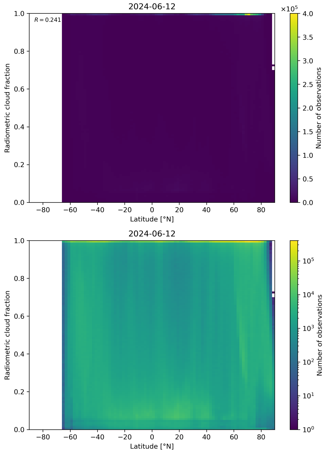
Figure 92: Scatter density plot of “Latitude” against “Radiometric cloud fraction” for 2024-06-11 to 2024-06-13.
