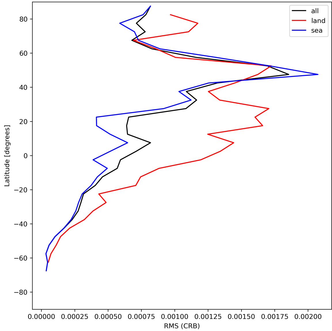
Figure 32: Zonal average of “RMS (CRB)” for 2024-06-11 to 2024-06-13.
