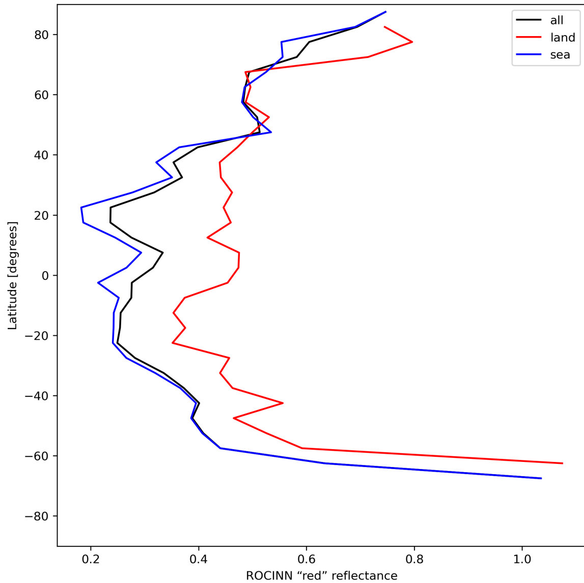
Figure 37: Zonal average of “ROCINN “red” reflectance” for 2024-06-11 to 2024-06-13.
