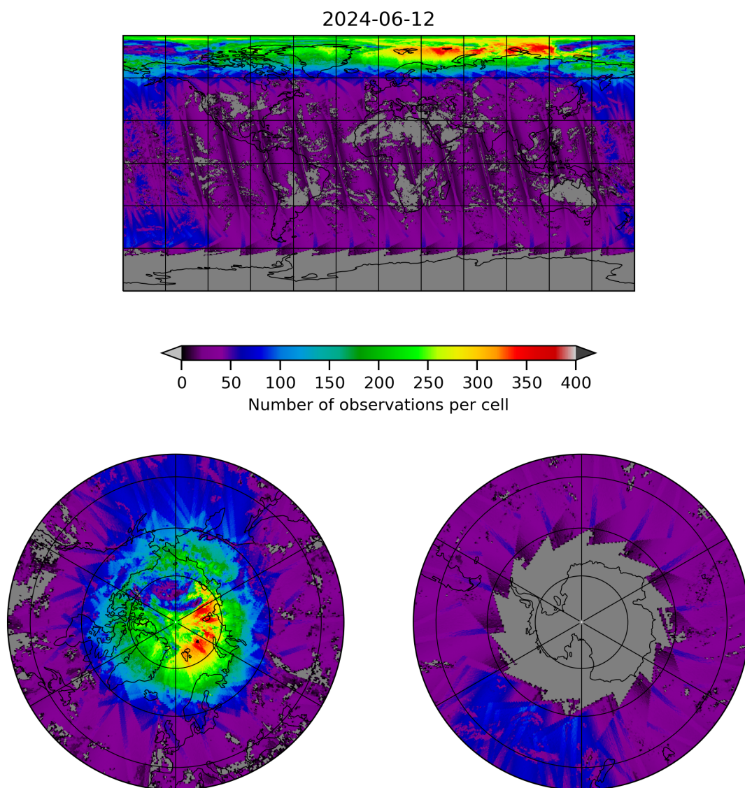
Figure 21: Map of the number of observations for 2024-06-11 to 2024-06-13
