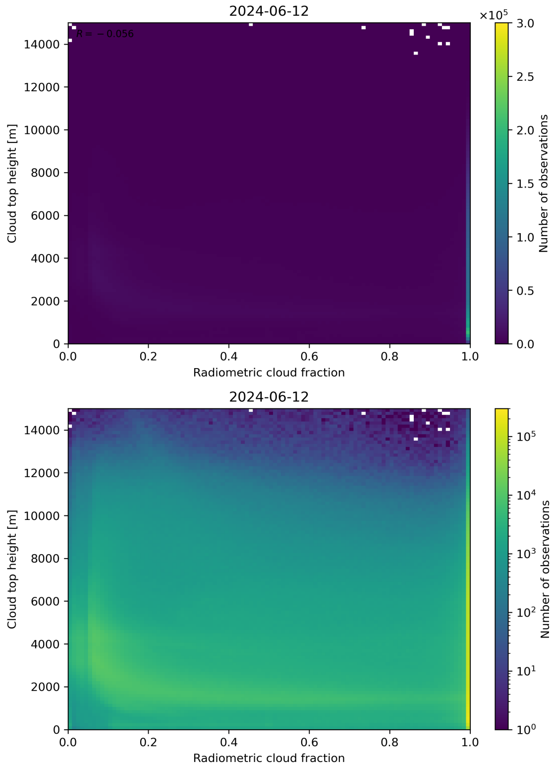
Figure 76: Scatter density plot of “Radiometric cloud fraction” against “Cloud top height” for 2024-06-11 to 2024-06-13.
