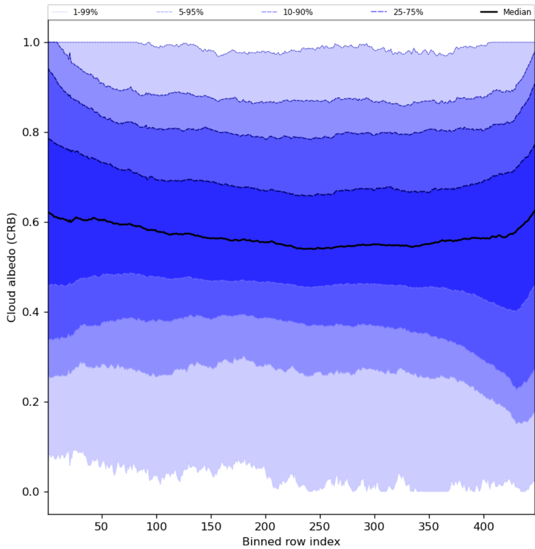
Figure 60: Along track statistics of “Cloud albedo (CRB)” for 2024-06-11 to 2024-06-13
