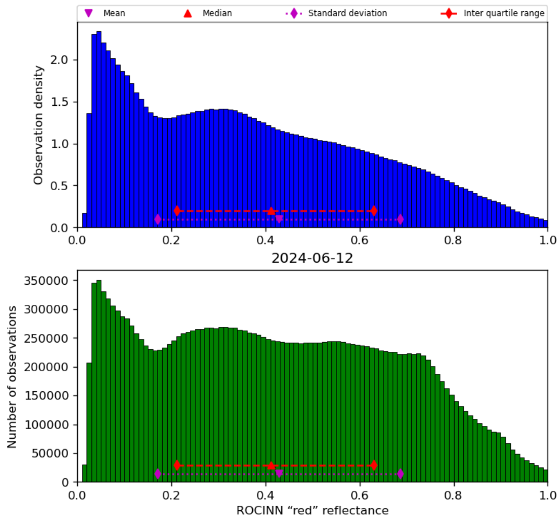
Figure 53: Histogram of “ROCINN “red” reflectance” for 2024-06-11 to 2024-06-13
