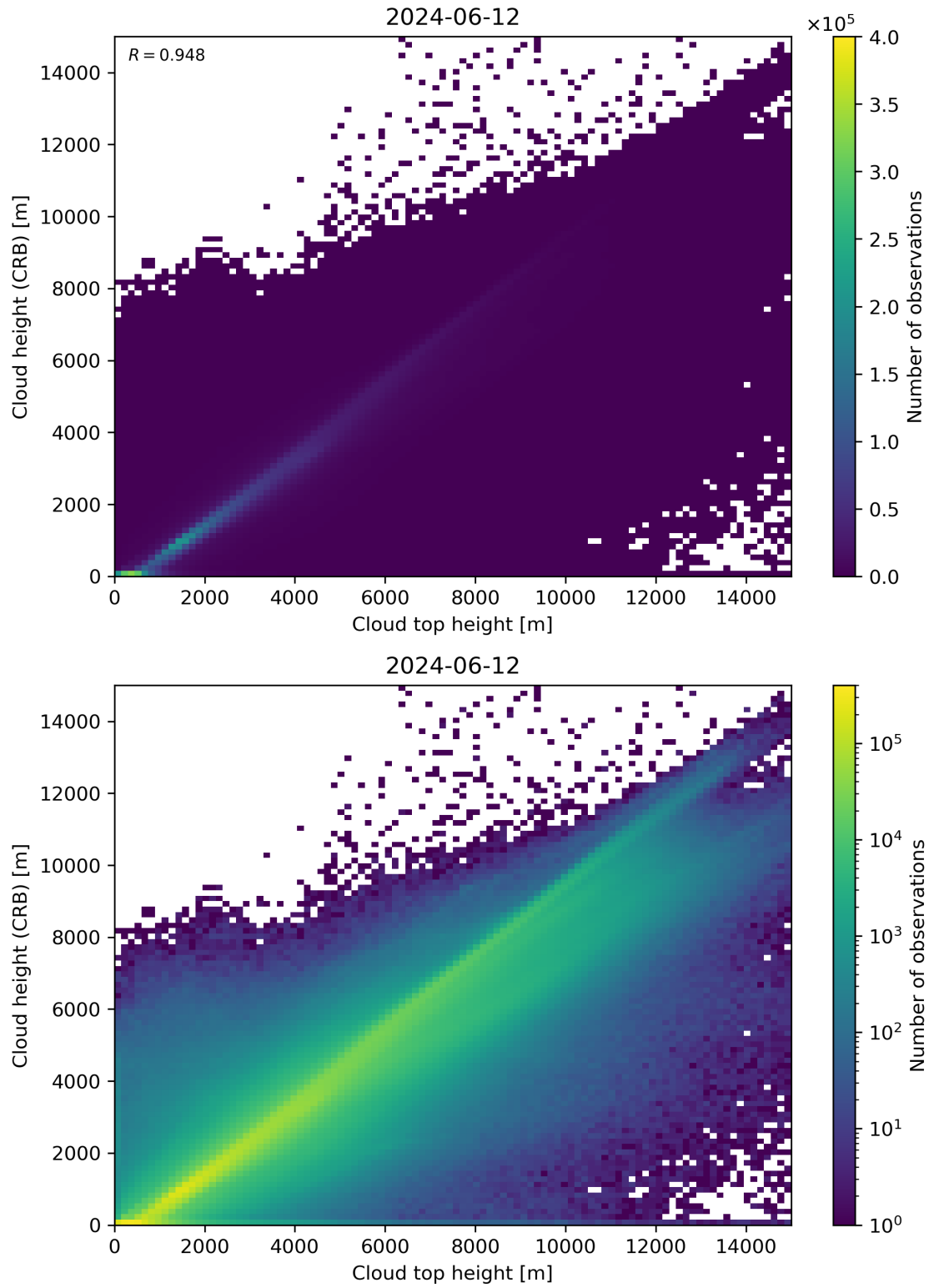
Figure 89: Scatter density plot of “Cloud top height” against “Cloud height (CRB)” for 2024-06-11 to 2024-06-13.
