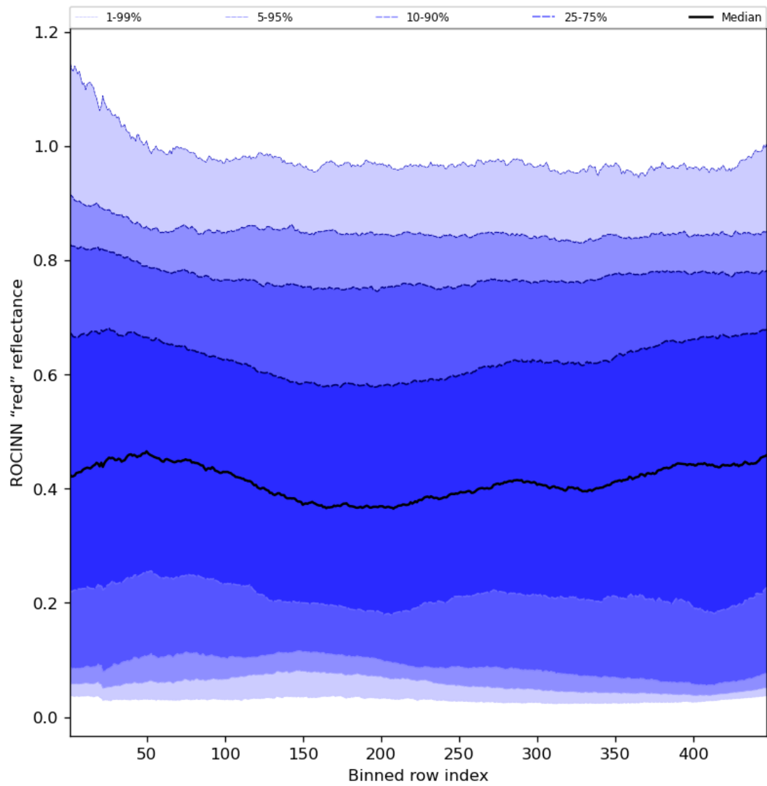
Figure 69: Along track statistics of “ROCINN “red” reflectance” for 2024-06-11 to 2024-06-13
