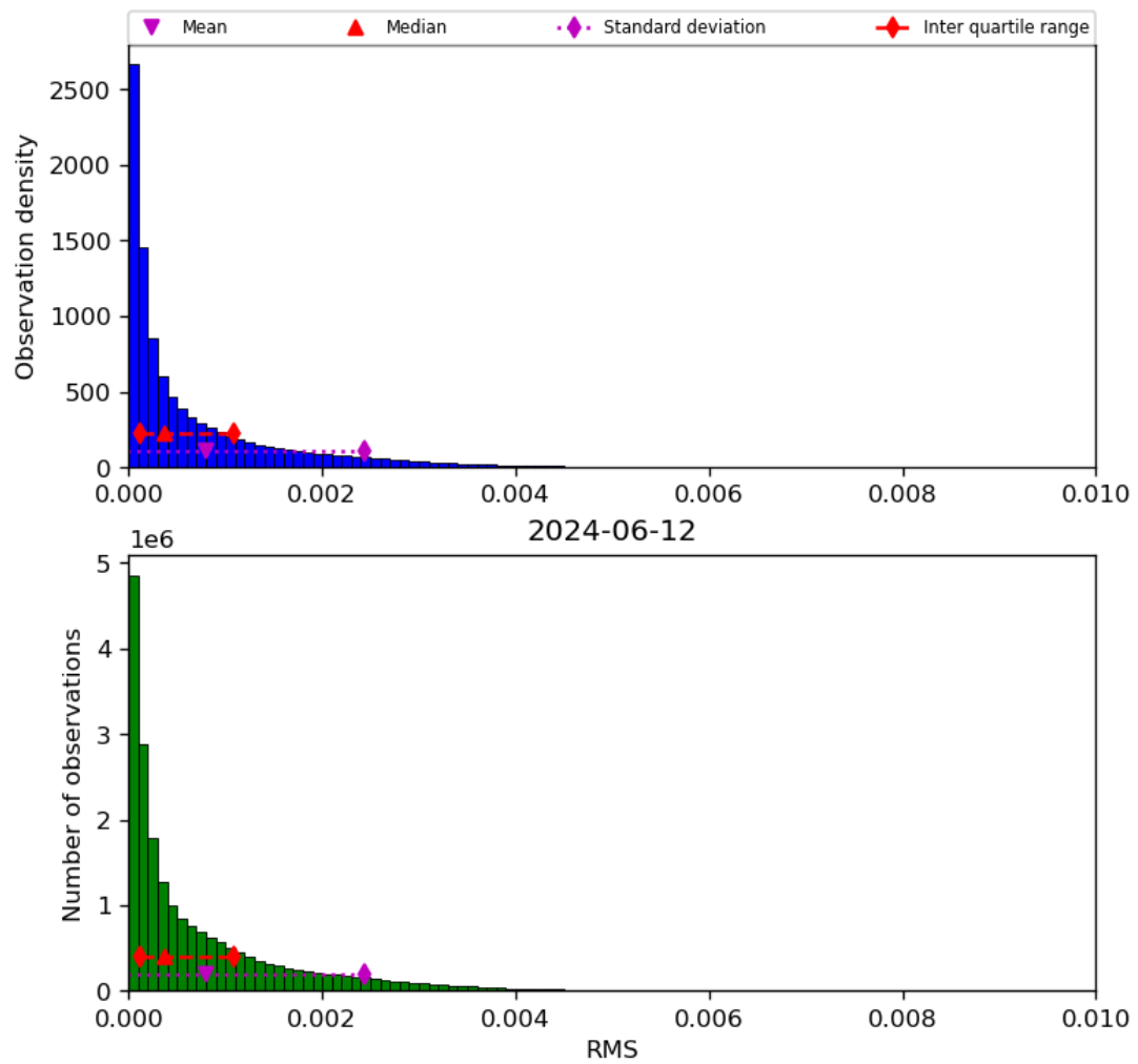
Figure 47: Histogram of “RMS” for 2024-06-11 to 2024-06-13
