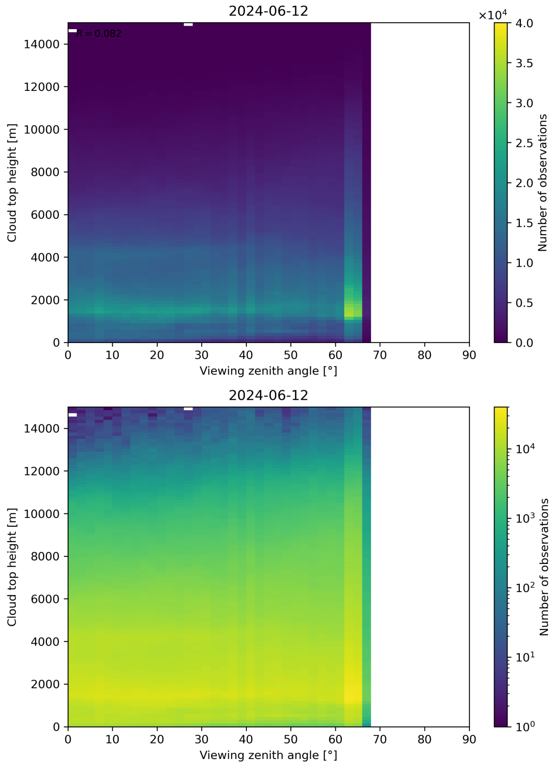
Figure 112: Scatter density plot of “Viewing zenith angle” against “Cloud top height” for 2024-06-11 to 2024-06-13.
