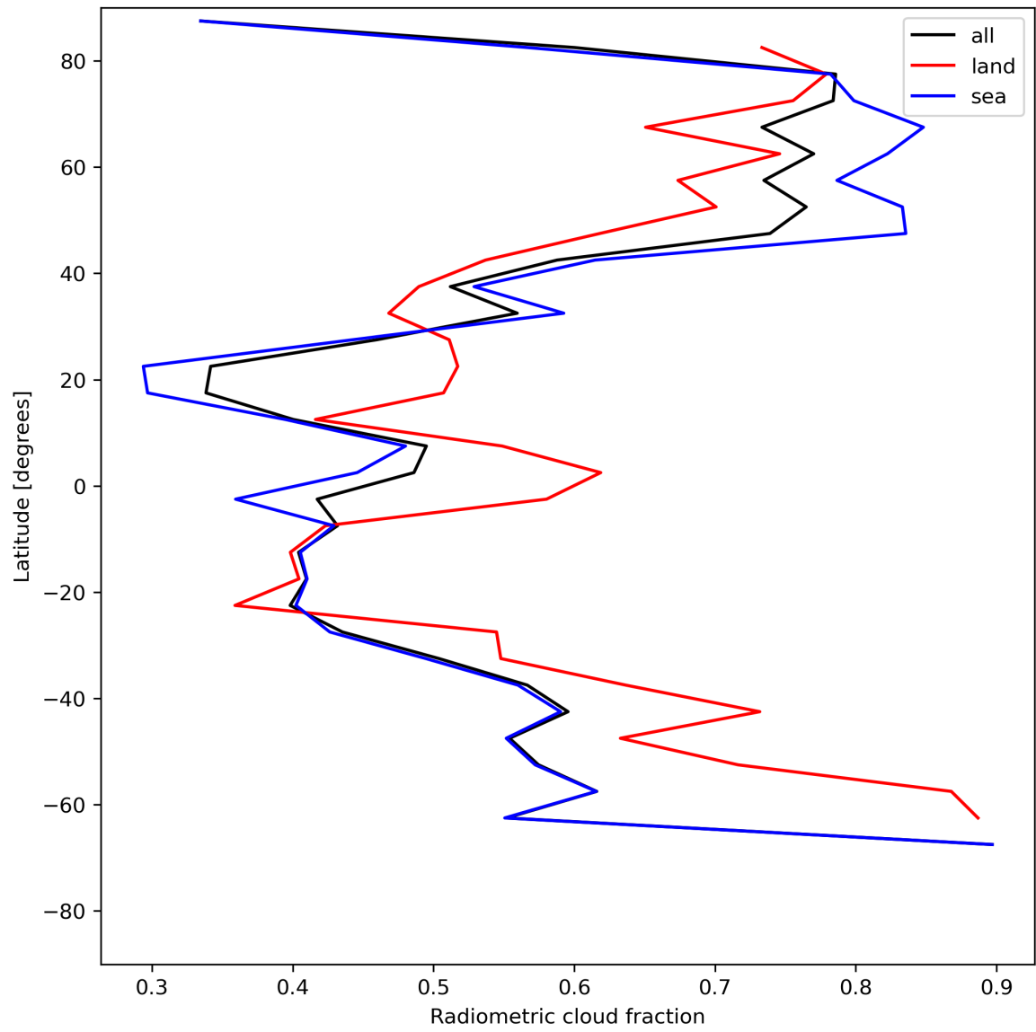
Figure 23: Zonal average of “Radiometric cloud fraction” for 2024-06-11 to 2024-06-13.
