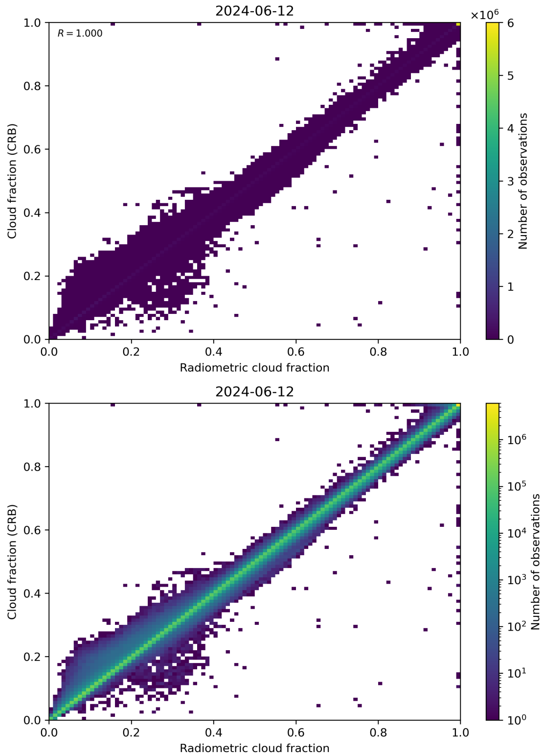
Figure 73: Scatter density plot of “Radiometric cloud fraction” against “Cloud fraction (CRB)” for 2024-06-11 to 2024-06-13.
