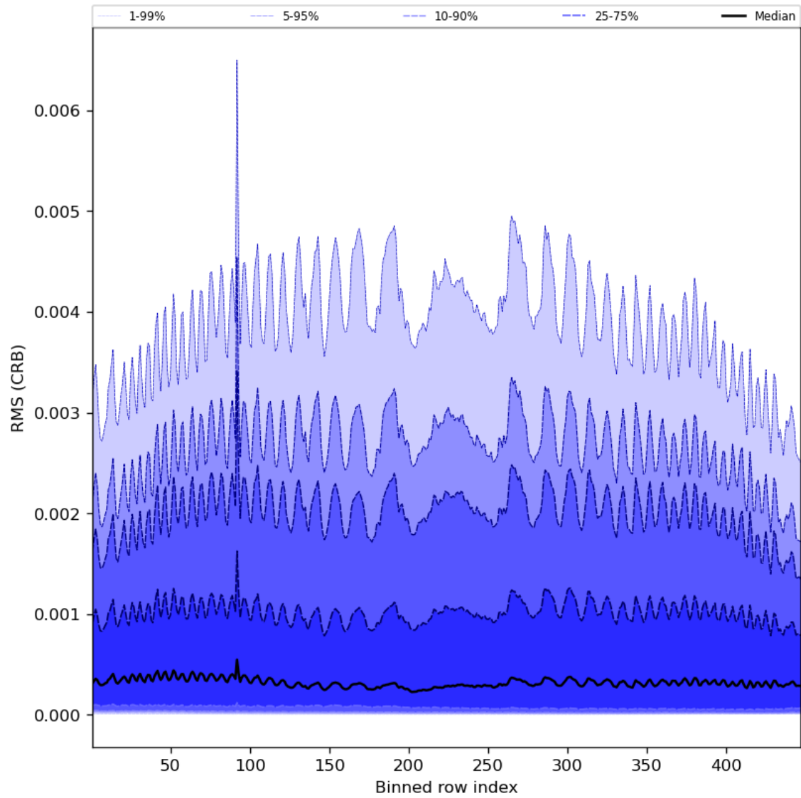
Figure 64: Along track statistics of “RMS (CRB)” for 2024-06-11 to 2024-06-13
