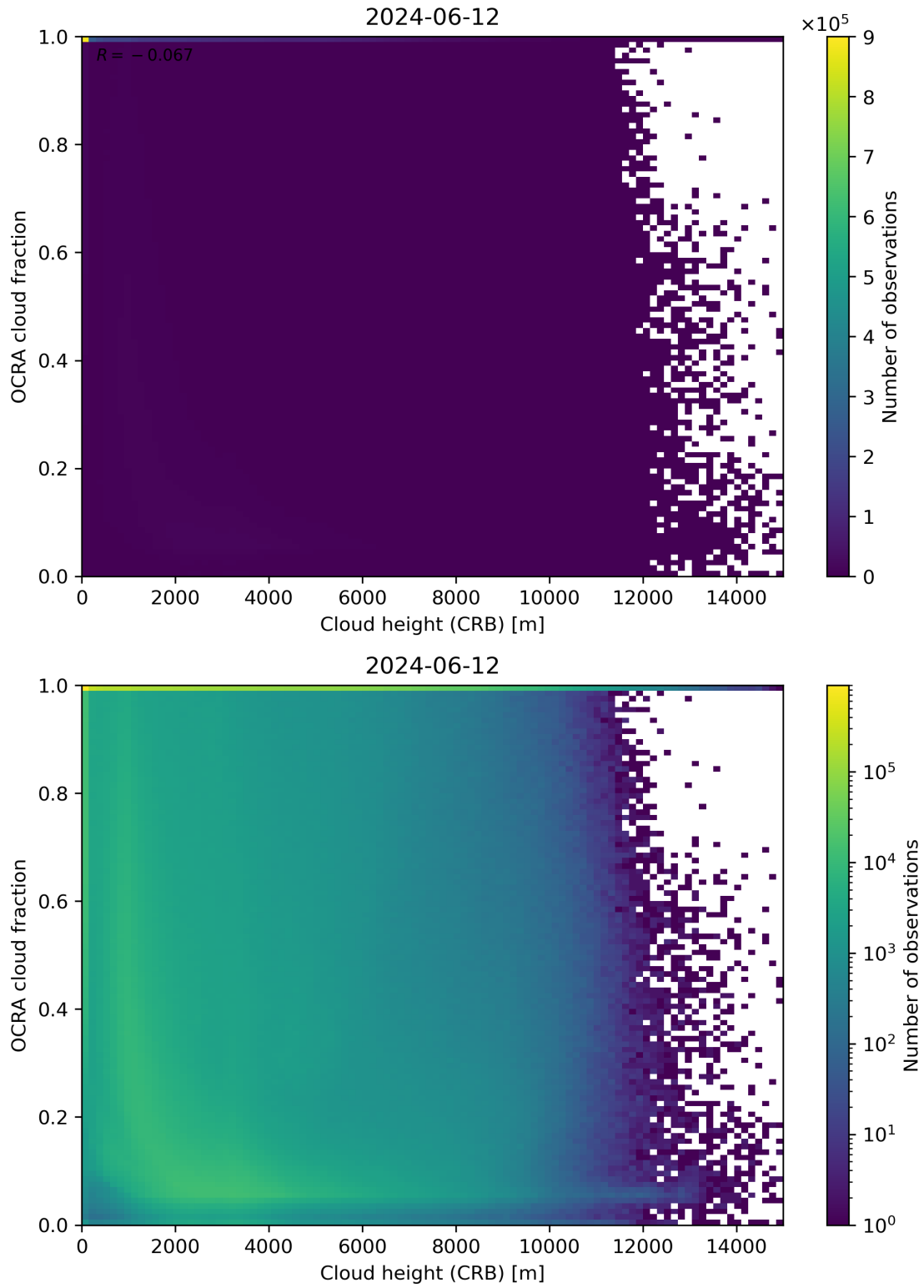
Figure 81: Scatter density plot of “Cloud height (CRB)” against “OCRA cloud fraction” for 2024-06-11 to 2024-06-13.
