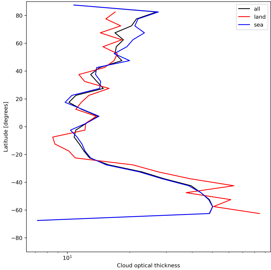
Figure 25: Zonal average of “Cloud optical thickness” for 2024-06-11 to 2024-06-13.
