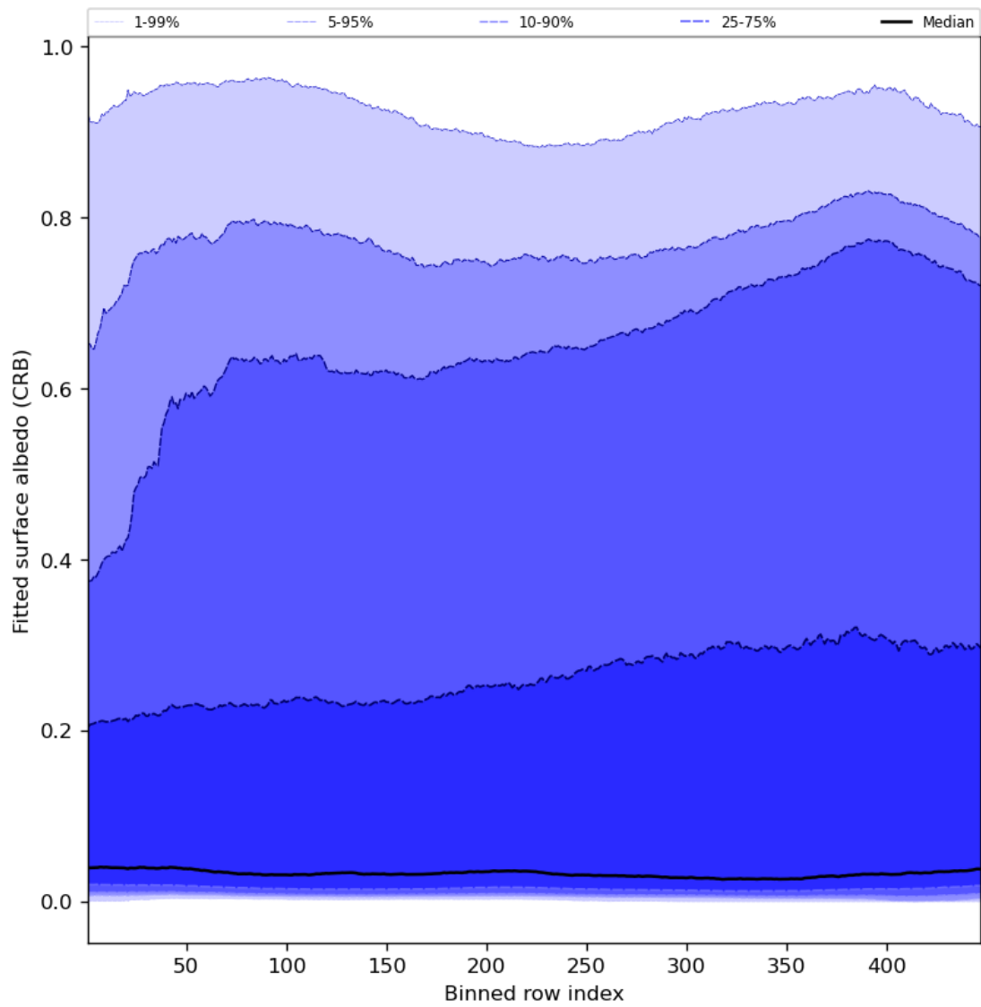
Figure 62: Along track statistics of “Fitted surface albedo (CRB)” for 2024-06-11 to 2024-06-13
