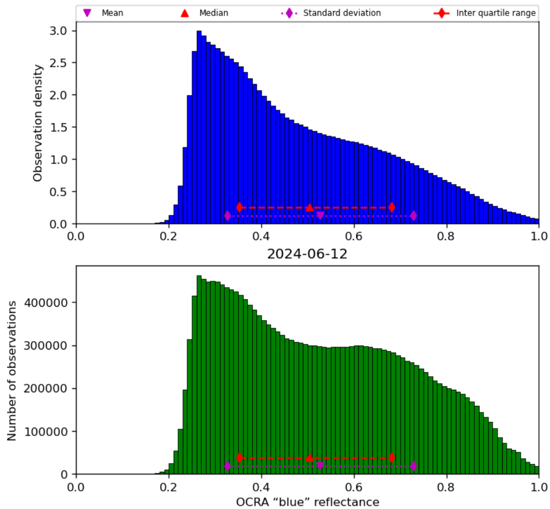
Figure 51: Histogram of “OCRA “blue” reflectance” for 2024-06-11 to 2024-06-13
