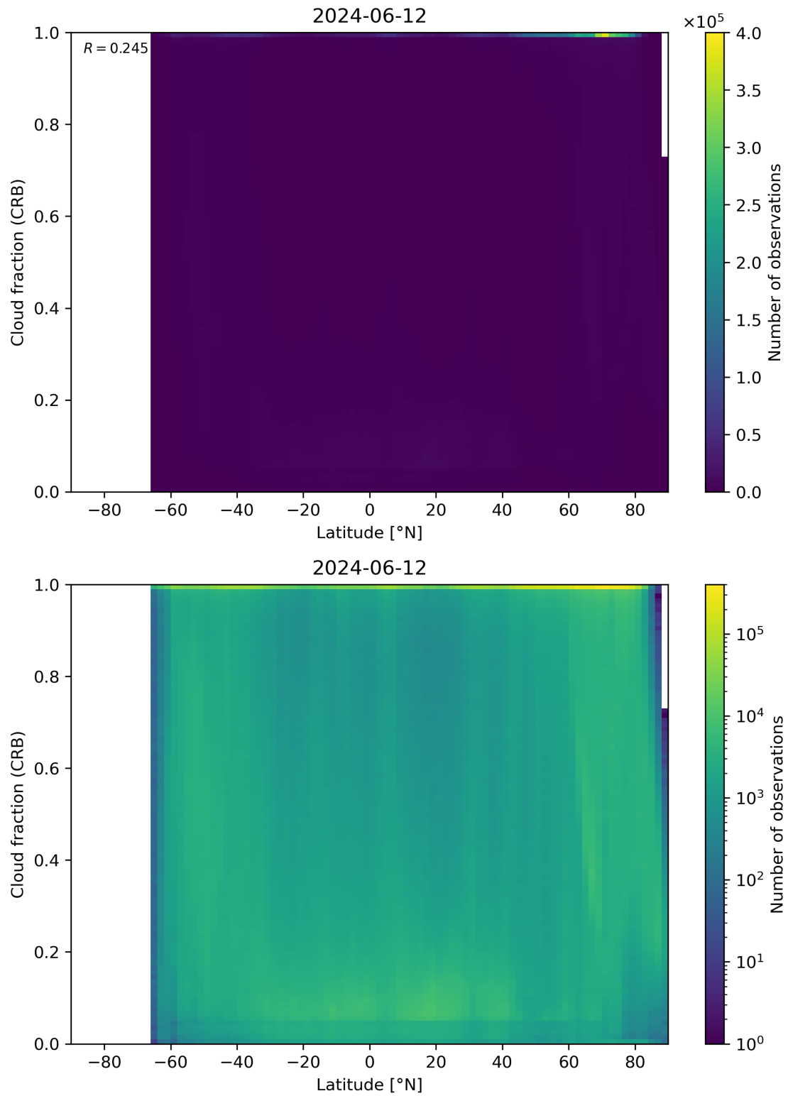
Figure 94: Scatter density plot of “Latitude” against “Cloud fraction (CRB)” for 2024-06-11 to 2024-06-13.
