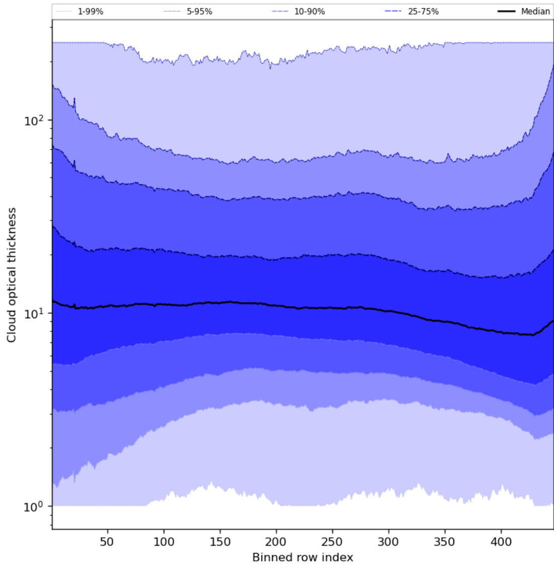
Figure 57: Along track statistics of “Cloud optical thickness” for 2024-06-11 to 2024-06-13
