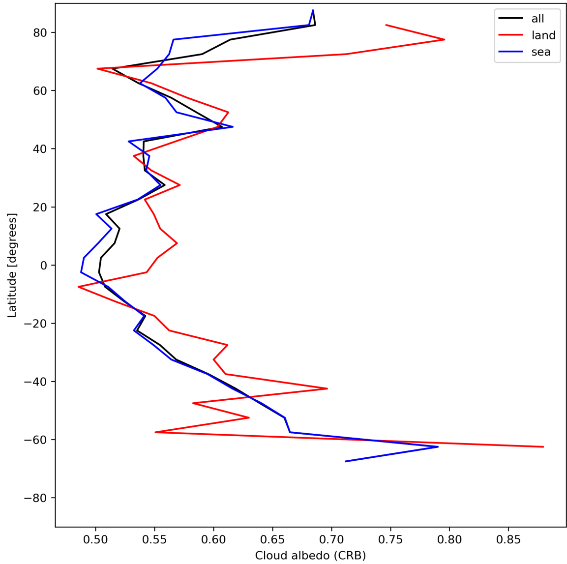
Figure 28: Zonal average of “Cloud albedo (CRB)” for 2024-06-11 to 2024-06-13.
