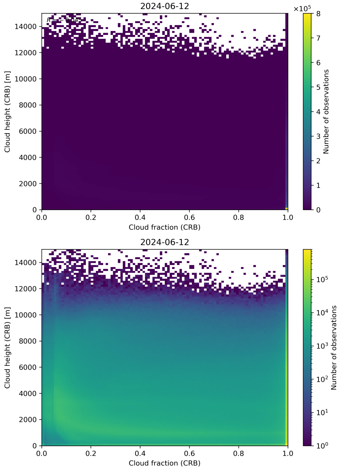
Figure 79: Scatter density plot of “Cloud fraction (CRB)” against “Cloud height (CRB)” for 2024-06-11 to 2024-06-13.
