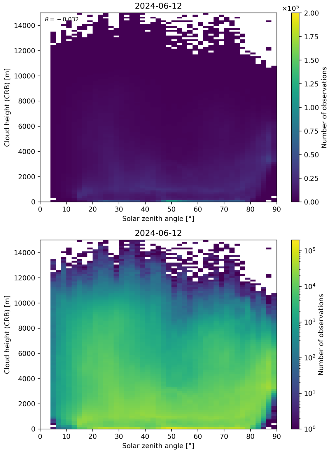
Figure 102: Scatter density plot of “Solar zenith angle” against “Cloud height (CRB)” for 2024-06-11 to 2024-06-13.
