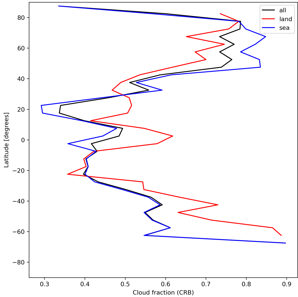
Figure 26: Zonal average of “Cloud fraction (CRB)” for 2024-06-11 to 2024-06-13.
