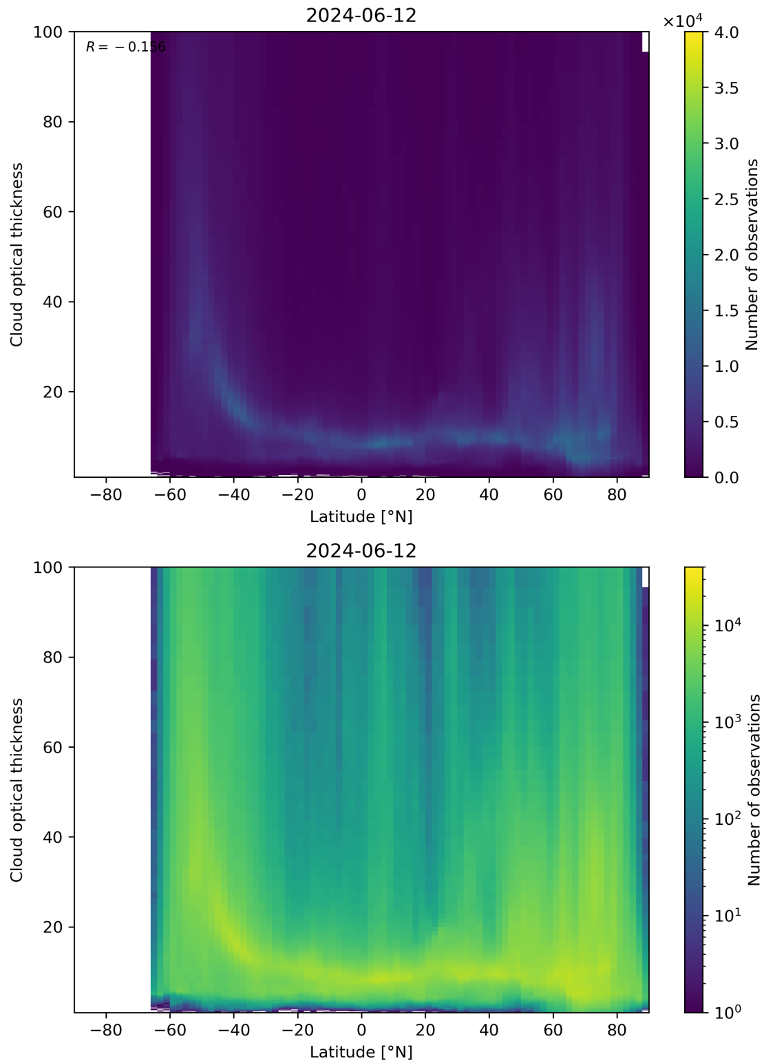
Figure 96: Scatter density plot of “Latitude” against “Cloud optical thickness” for 2024-06-11 to 2024-06-13.
