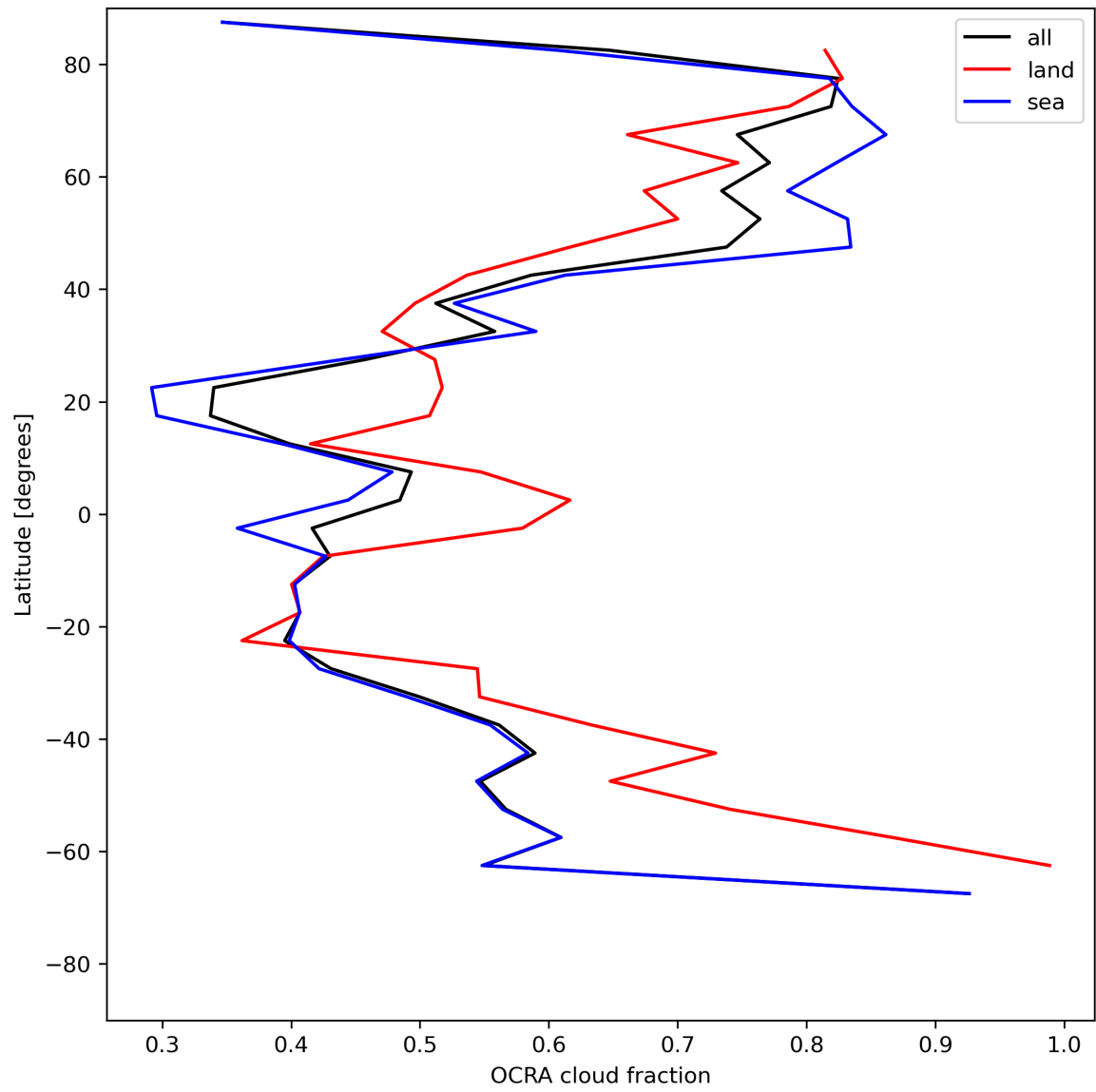
Figure 34: Zonal average of “OCRA cloud fraction” for 2024-06-11 to 2024-06-13.
