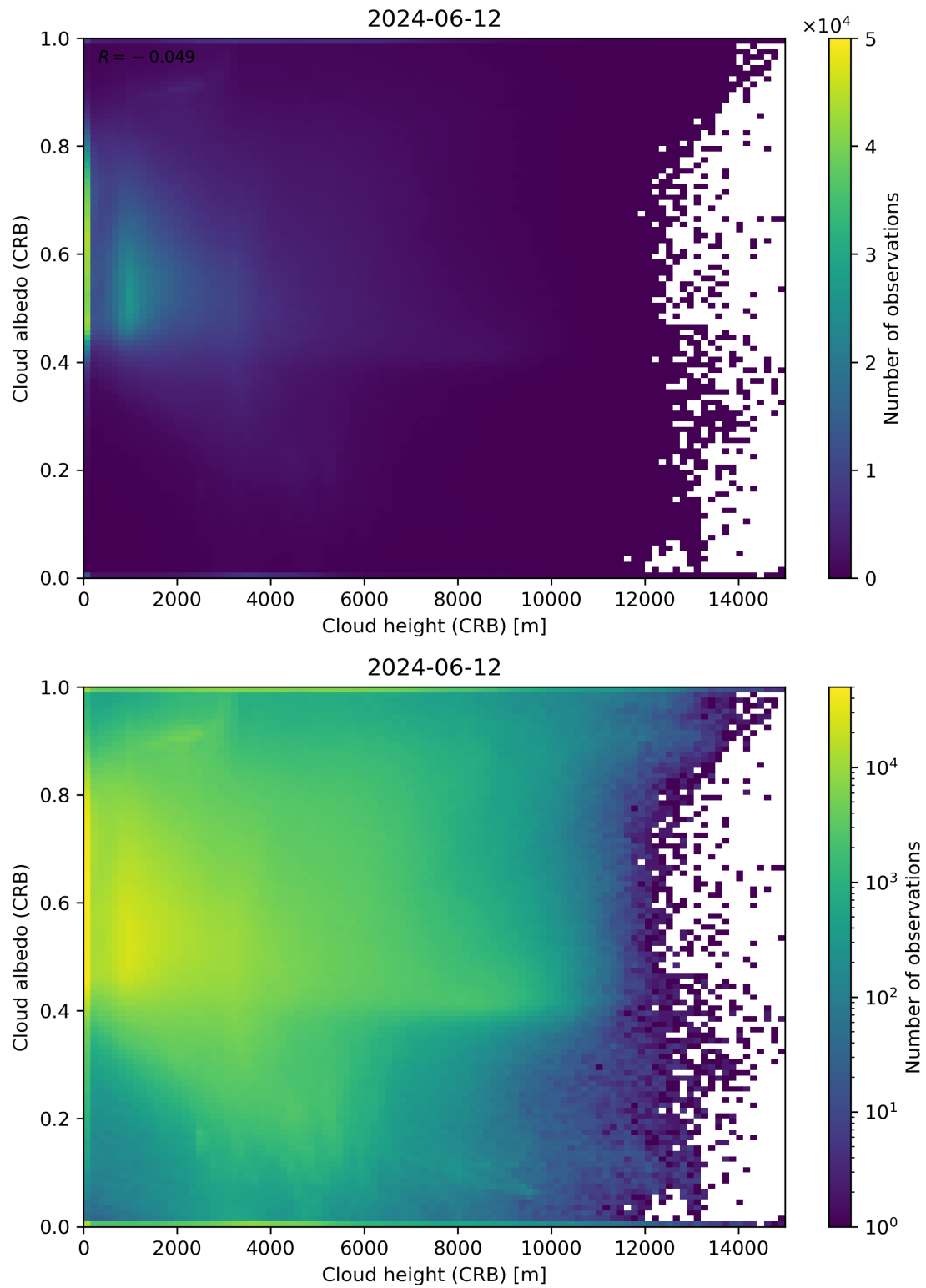
Figure 80: Scatter density plot of “Cloud height (CRB)” against “Cloud albedo (CRB)” for 2024-06-11 to 2024-06-13.
