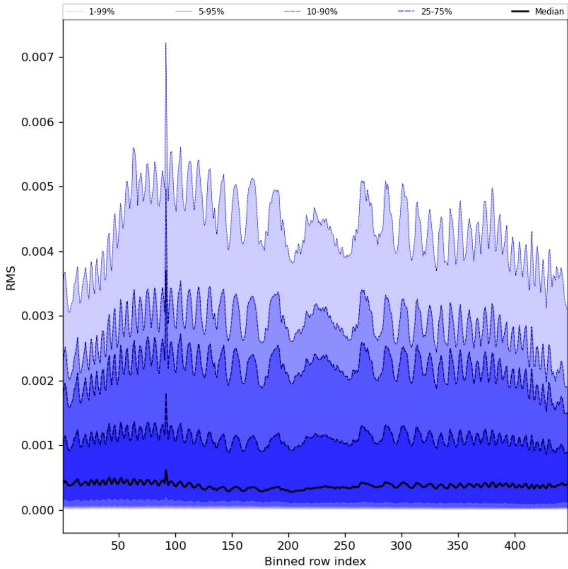
Figure 63: Along track statistics of “RMS” for 2024-06-11 to 2024-06-13
