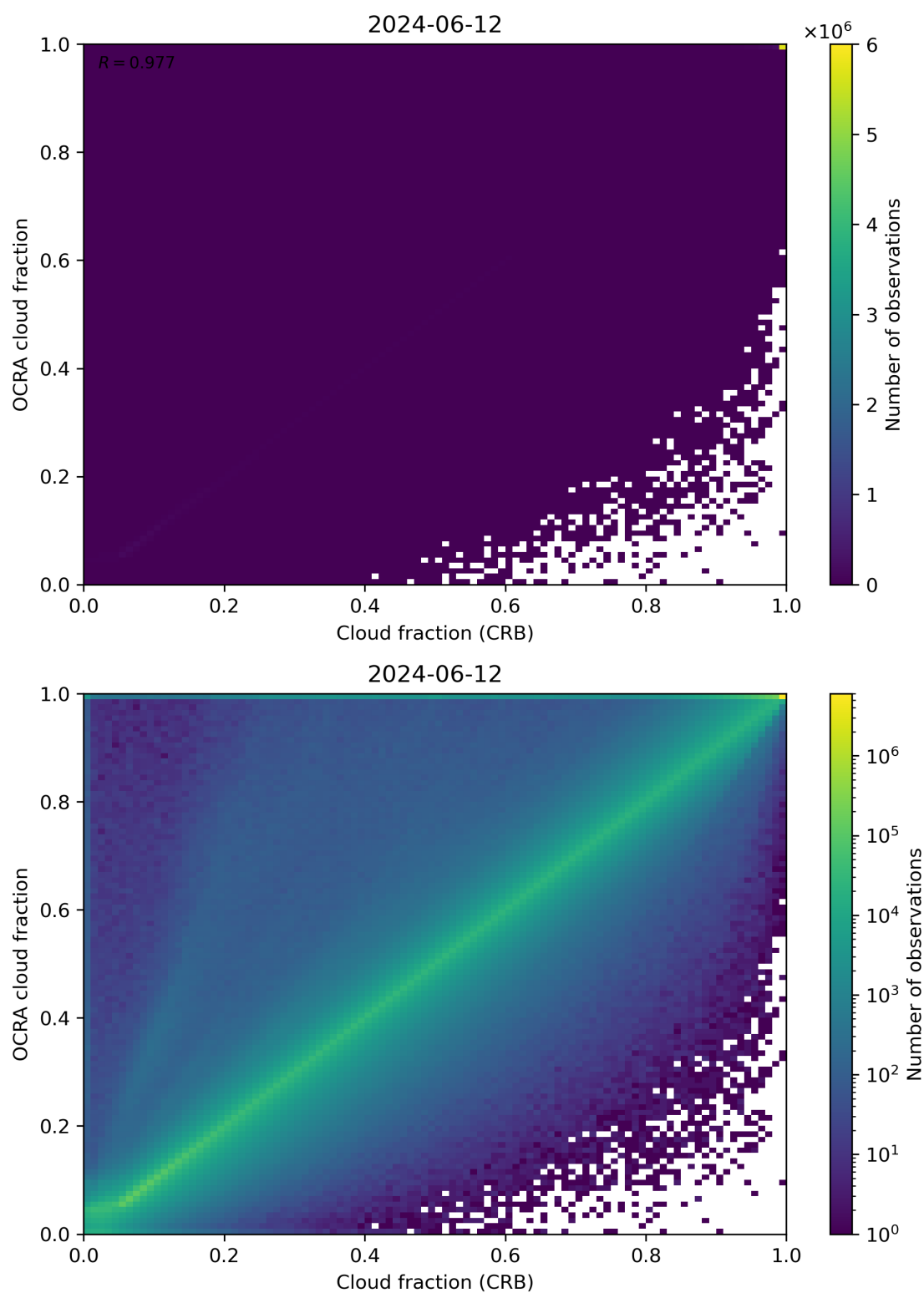
Figure 78: Scatter density plot of “Cloud fraction (CRB)” against “OCRA cloud fraction” for 2024-06-11 to 2024-06-13.
