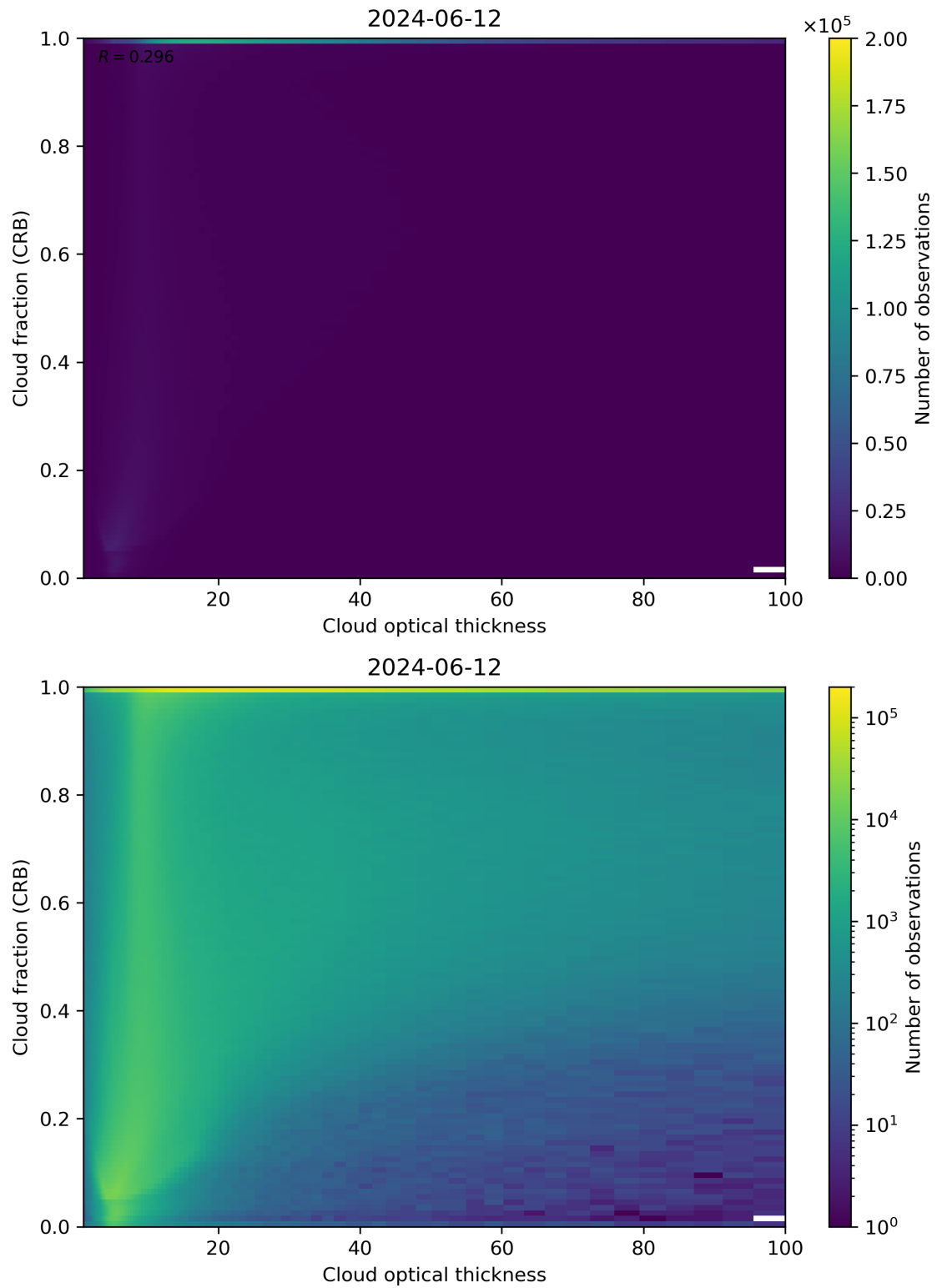
Figure 84: Scatter density plot of “Cloud optical thickness” against “Cloud fraction (CRB)” for 2024-06-11 to 2024-06-13.
