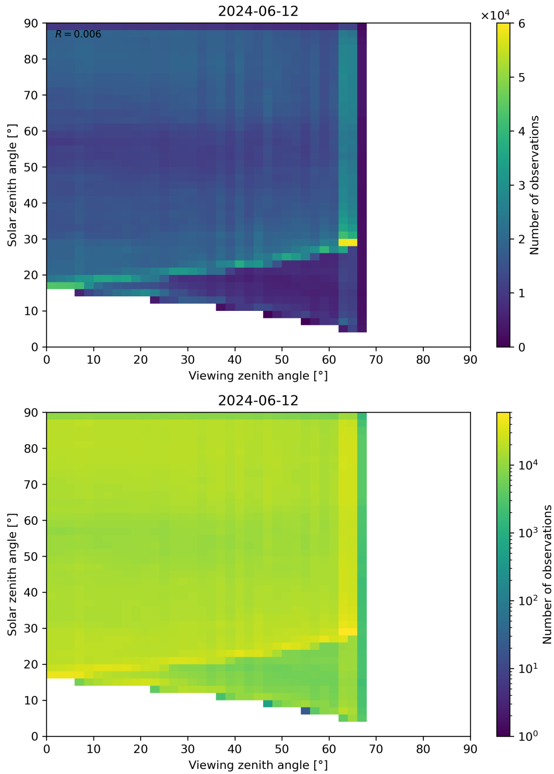
Figure 114: Scatter density plot of “Viewing zenith angle” against “Solar zenith angle” for 2024-06-11 to 2024-06-13.
