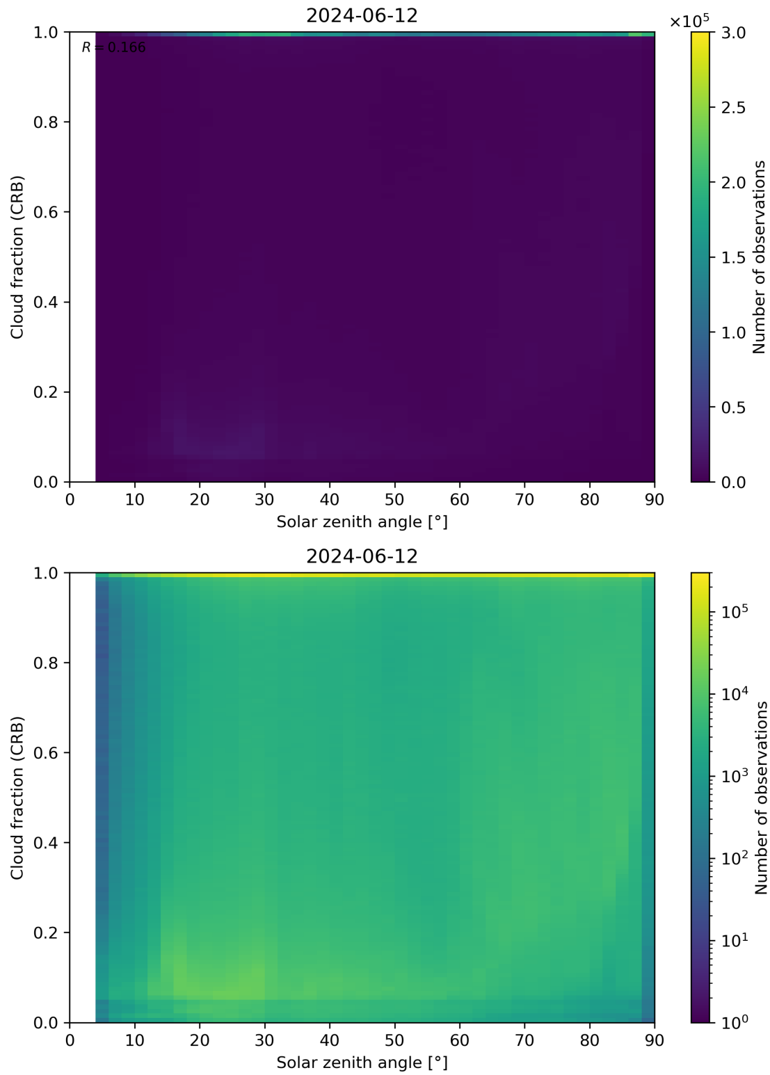
Figure 101: Scatter density plot of “Solar zenith angle” against “Cloud fraction (CRB)” for 2024-06-11 to 2024-06-13.
