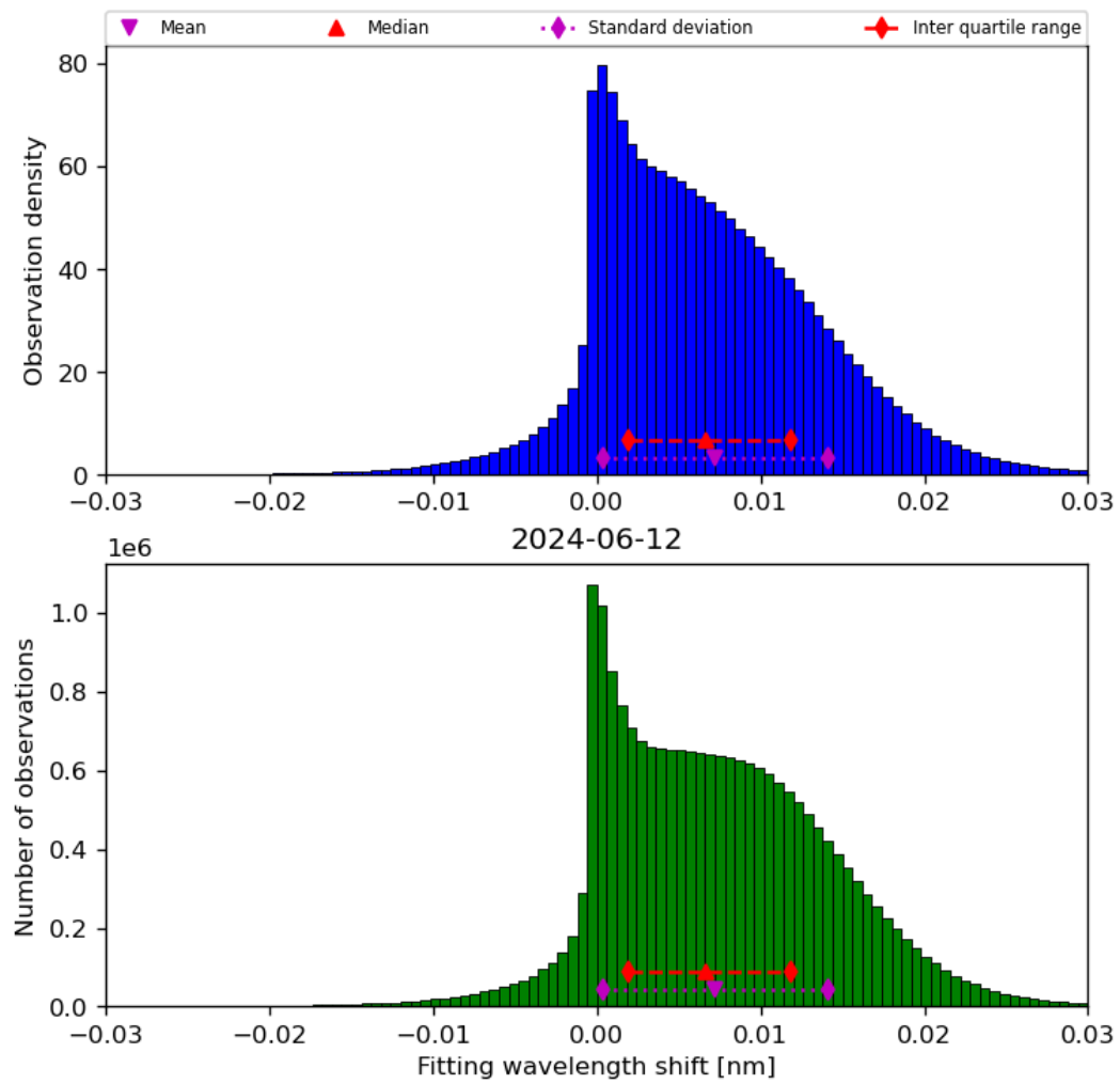
Figure 49: Histogram of “Fitting wavelength shift” for 2024-06-11 to 2024-06-13
