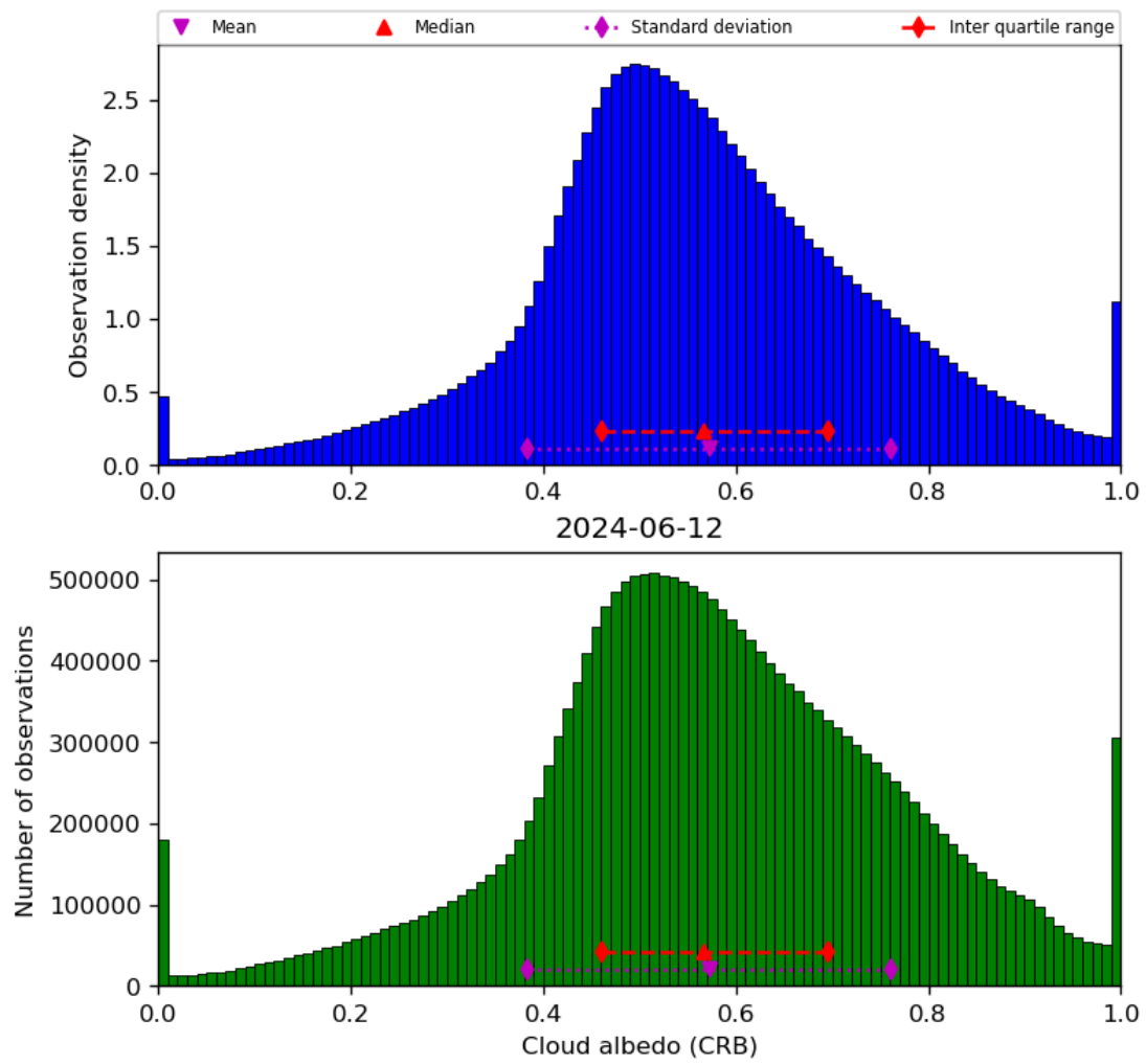
Figure 44: Histogram of “Cloud albedo (CRB)” for 2024-06-11 to 2024-06-13
