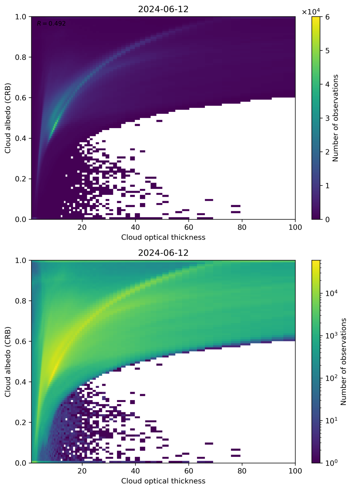
Figure 82: Scatter density plot of “Cloud optical thickness” against “Cloud albedo (CRB)” for 2024-06-11 to 2024-06-13.
