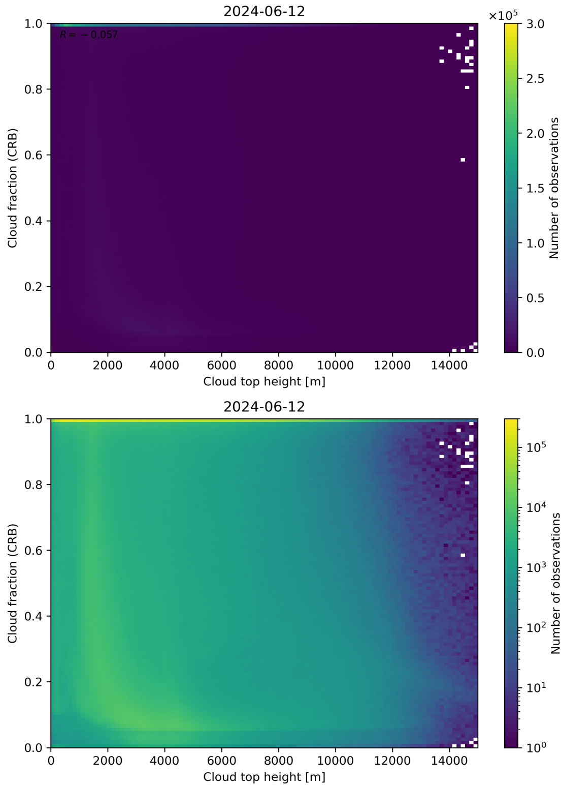
Figure 88: Scatter density plot of “Cloud top height” against “Cloud fraction (CRB)” for 2024-06-11 to 2024-06-13.
