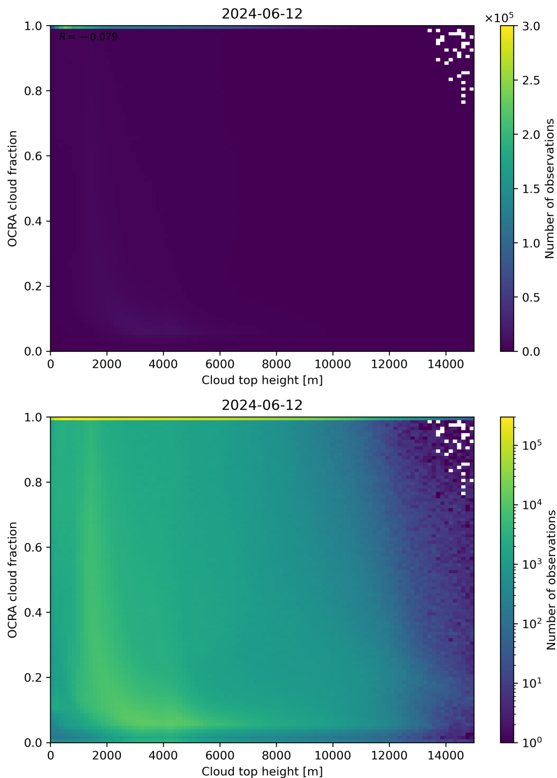
Figure 87: Scatter density plot of “Cloud top height” against “OCRA cloud fraction” for 2024-06-11 to 2024-06-13.
