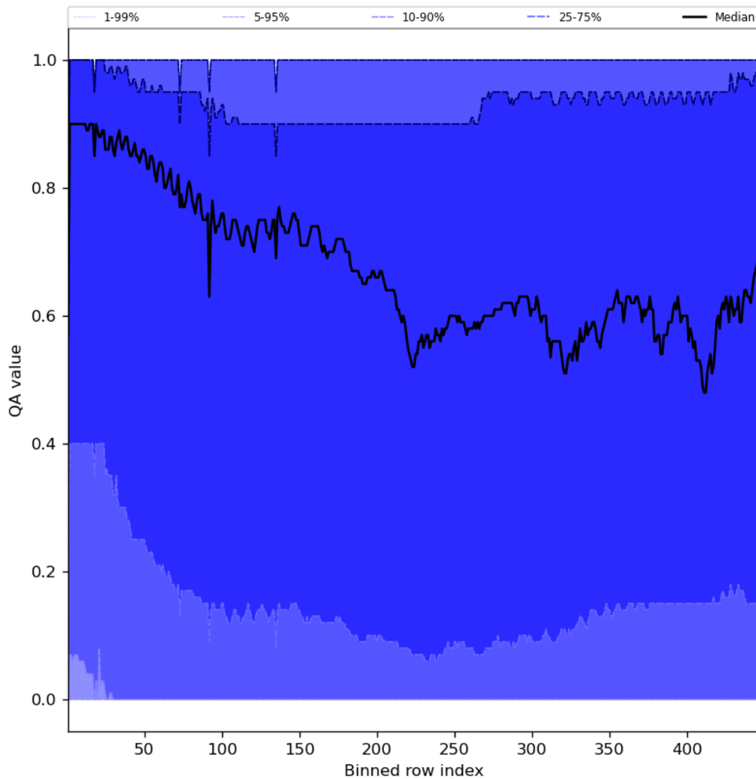
Figure 54: Along track statistics of “QA value” for 2024-06-11 to 2024-06-13
