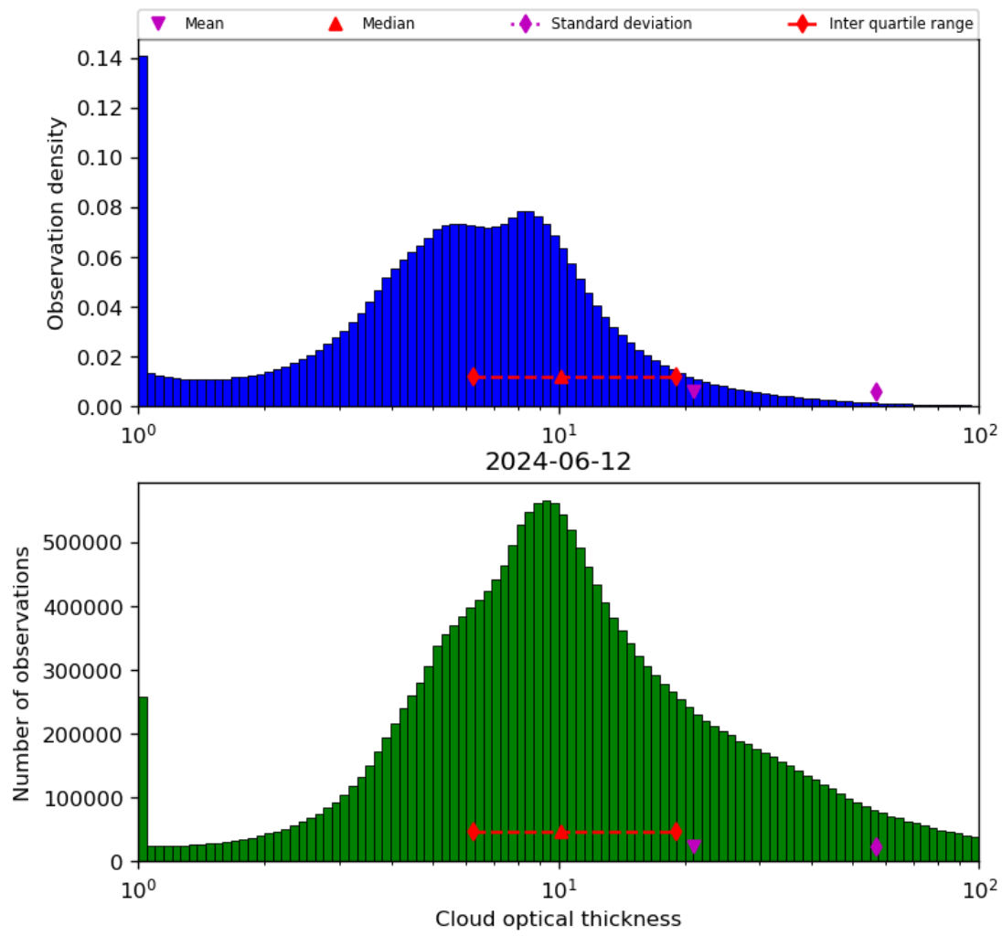
Figure 41: Histogram of “Cloud optical thickness” for 2024-06-11 to 2024-06-13
