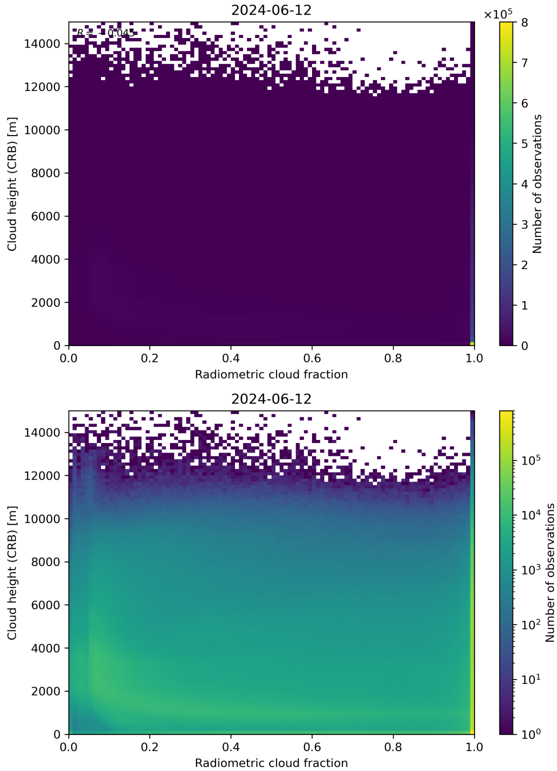
Figure 74: Scatter density plot of “Radiometric cloud fraction” against “Cloud height (CRB)” for 2024-06-11 to 2024-06-13.
