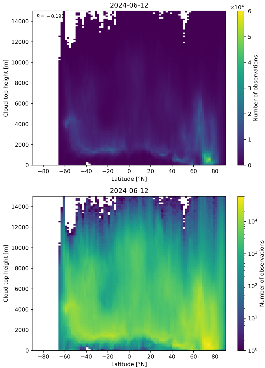
Figure 97: Scatter density plot of “Latitude” against “Cloud top height” for 2024-06-11 to 2024-06-13.
