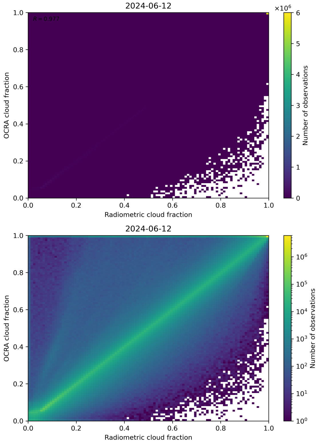
Figure 72: Scatter density plot of “Radiometric cloud fraction” against “OCRA cloud fraction” for 2024-06-11 to 2024-06-13.
