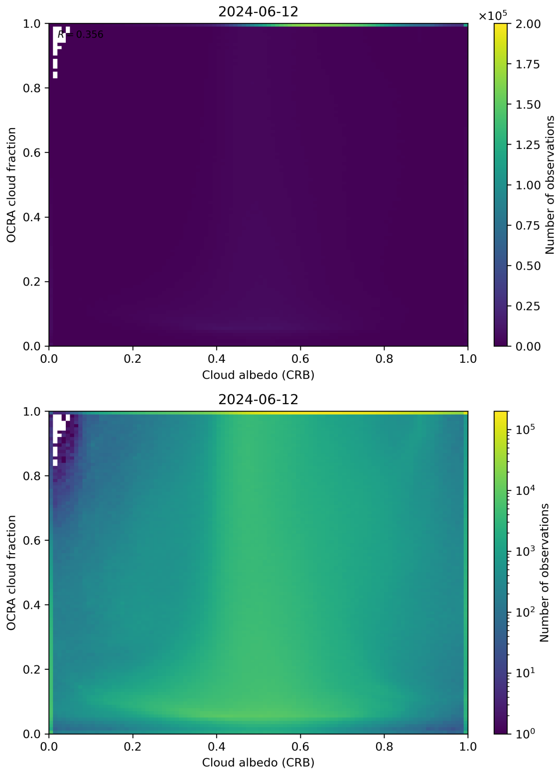
Figure 70: Scatter density plot of “Cloud albedo (CRB)” against “OCRA cloud fraction” for 2024-06-11 to 2024-06-13.
