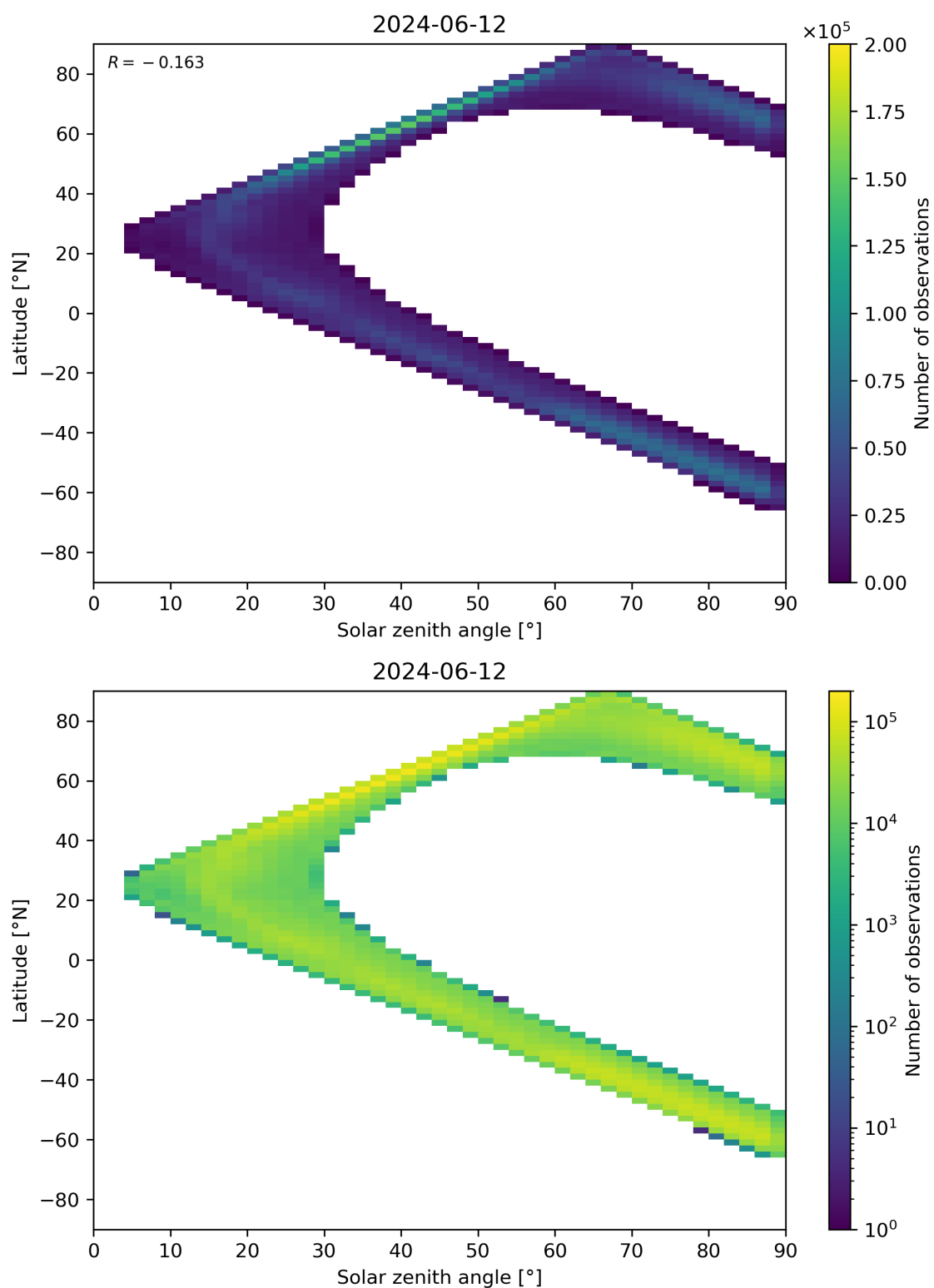
Figure 105: Scatter density plot of “Solar zenith angle” against “Latitude” for 2024-06-11 to 2024-06-13.
