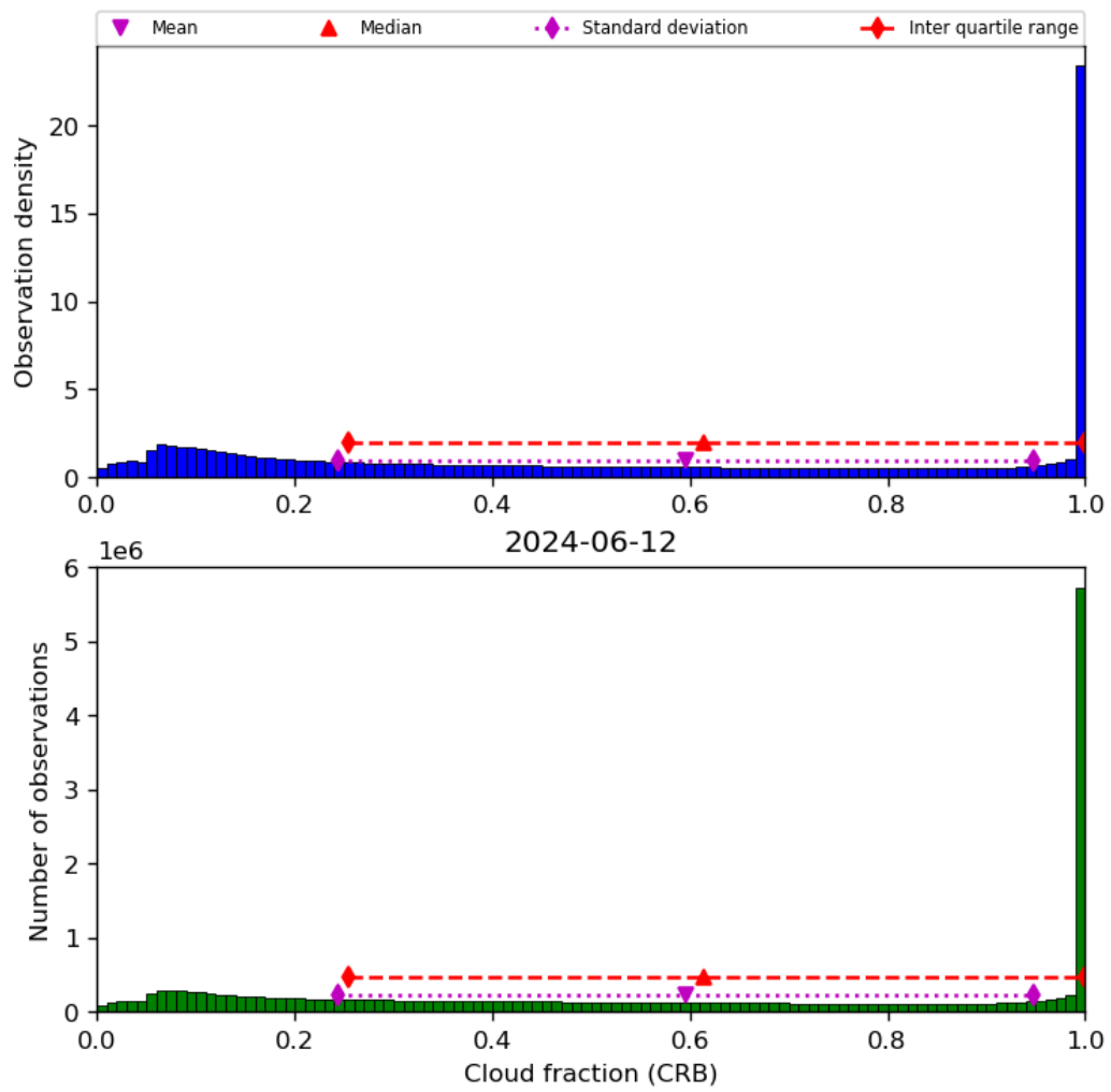
Figure 42: Histogram of “Cloud fraction (CRB)” for 2024-06-11 to 2024-06-13
