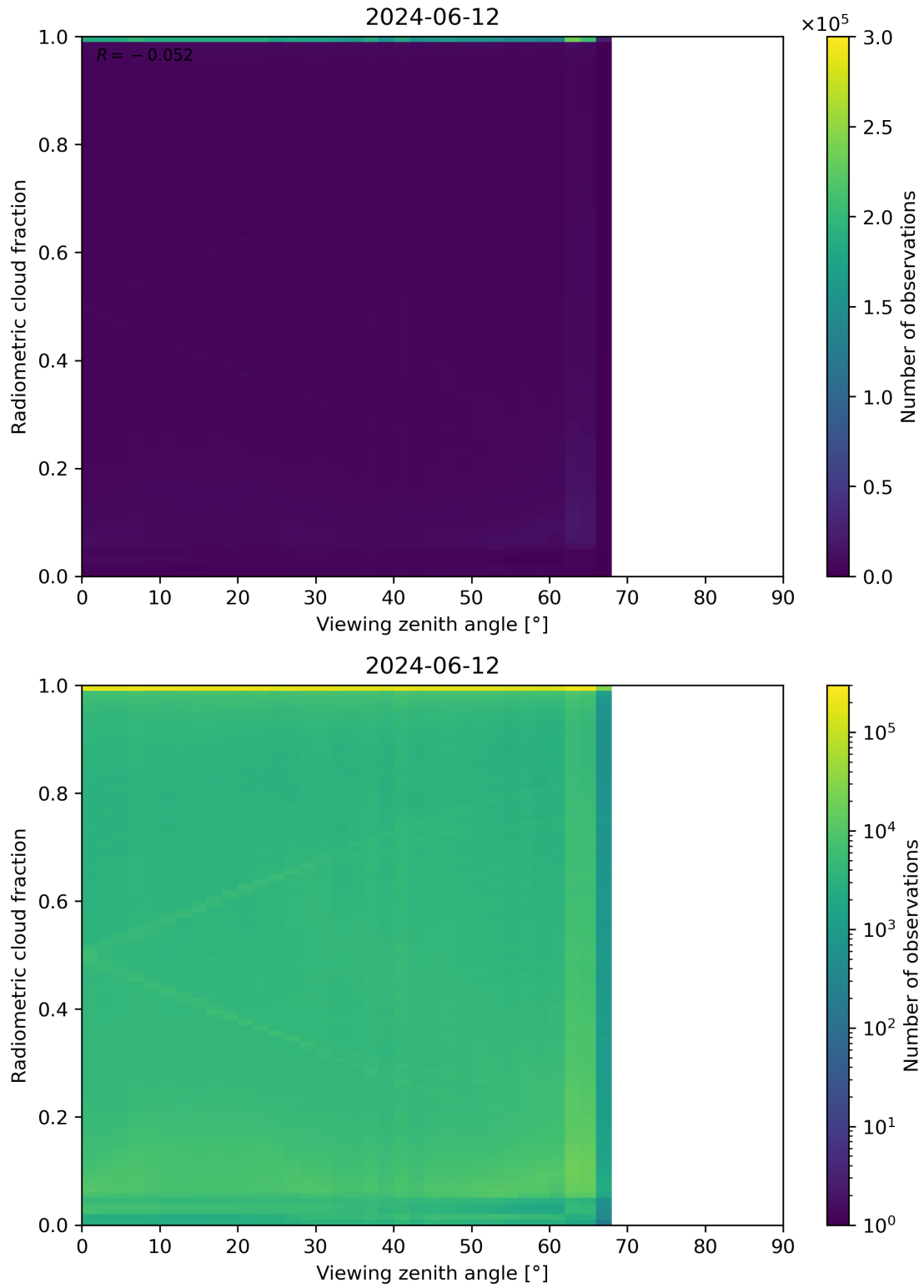
Figure 107: Scatter density plot of “Viewing zenith angle” against “Radiometric cloud fraction” for 2024-06-11 to 2024-06-13.
