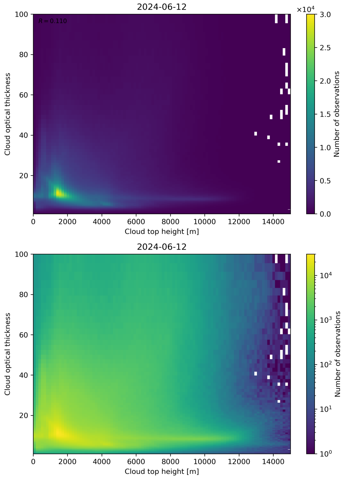
Figure 90: Scatter density plot of “Cloud top height” against “Cloud optical thickness” for 2024-06-11 to 2024-06-13.
