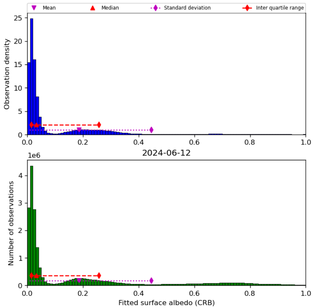
Figure 46: Histogram of “Fitted surface albedo (CRB)” for 2024-06-11 to 2024-06-13
