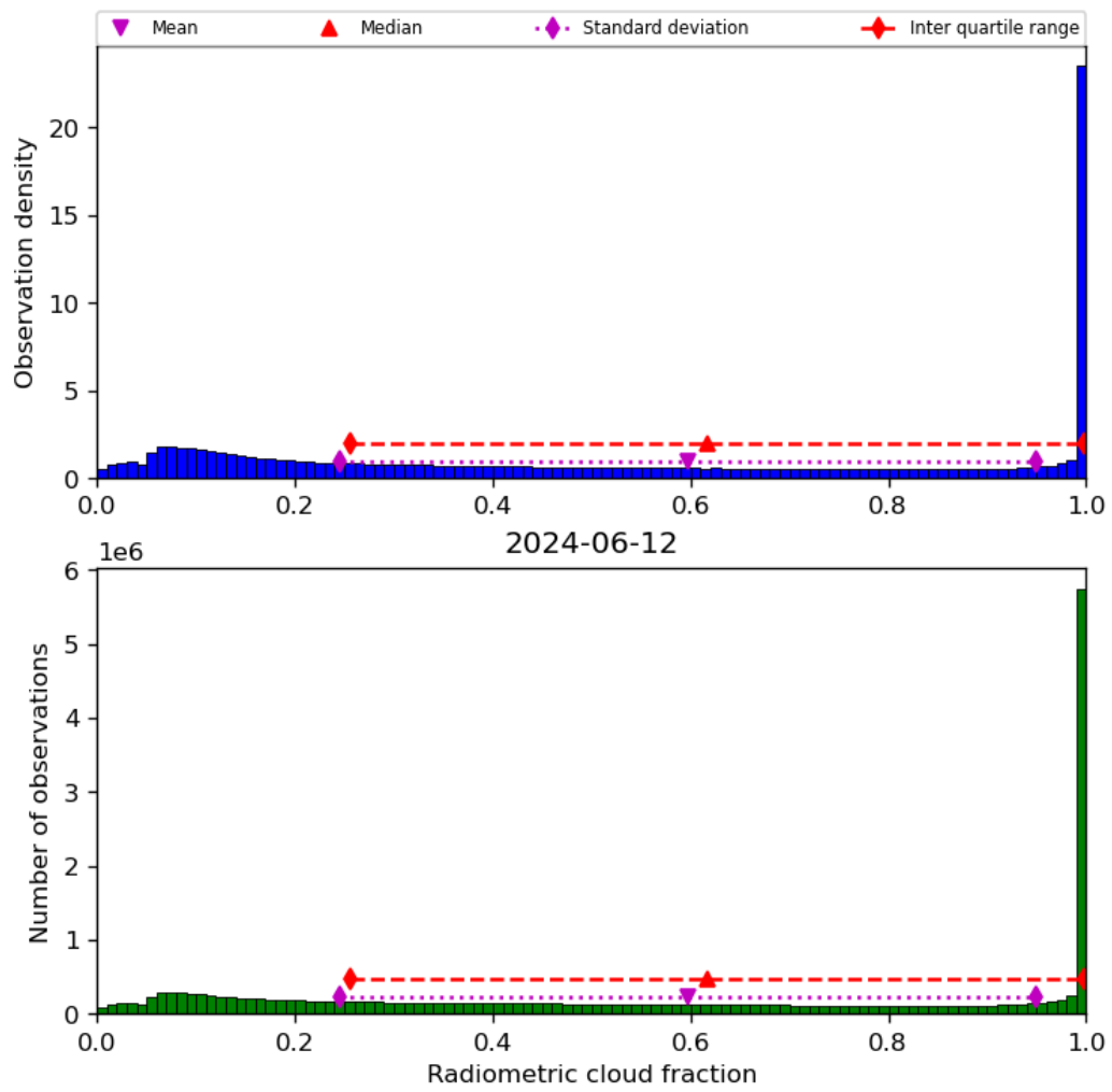
Figure 39: Histogram of “Radiometric cloud fraction” for 2024-06-11 to 2024-06-13
