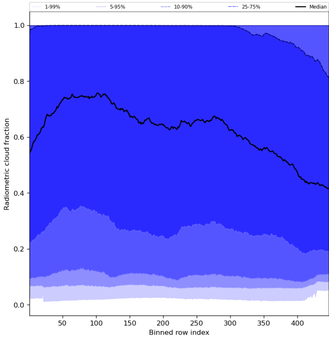
Figure 55: Along track statistics of “Radiometric cloud fraction” for 2024-06-11 to 2024-06-13
