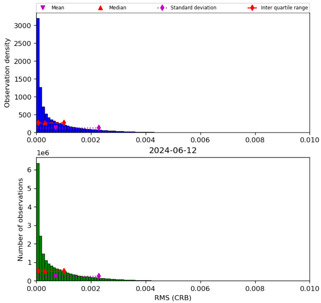
Figure 48: Histogram of “RMS (CRB)” for 2024-06-11 to 2024-06-13
