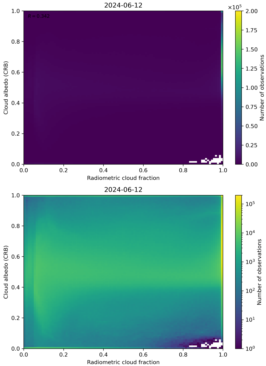
Figure 71: Scatter density plot of “Radiometric cloud fraction” against “Cloud albedo (CRB)” for 2024-06-11 to 2024-06-13.
