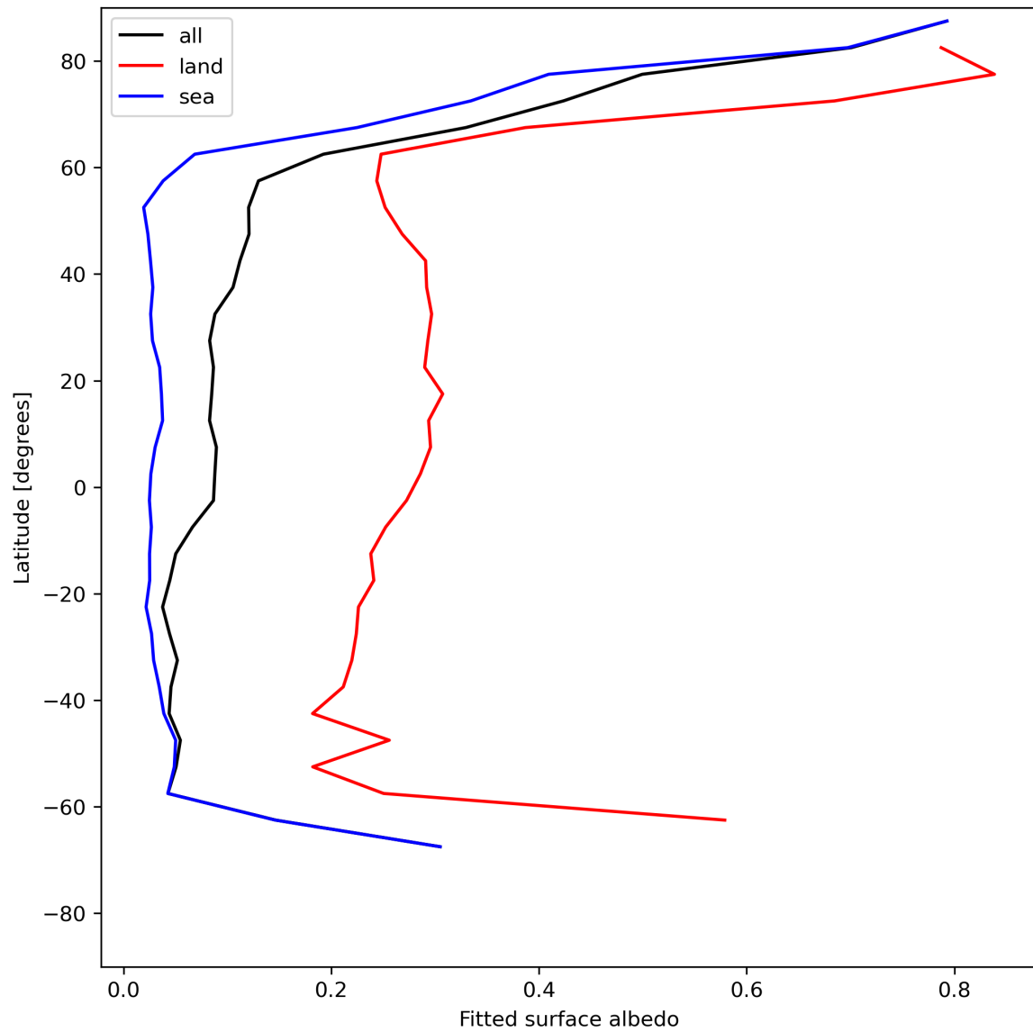
Figure 29: Zonal average of “Fitted surface albedo” for 2024-06-11 to 2024-06-13.
