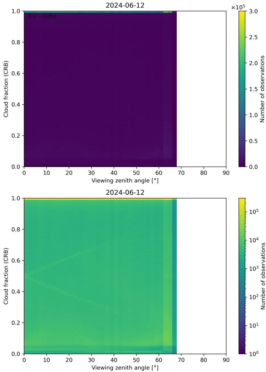
Figure 109: Scatter density plot of “Viewing zenith angle” against “Cloud fraction (CRB)” for 2024-06-11 to 2024-06-13.
