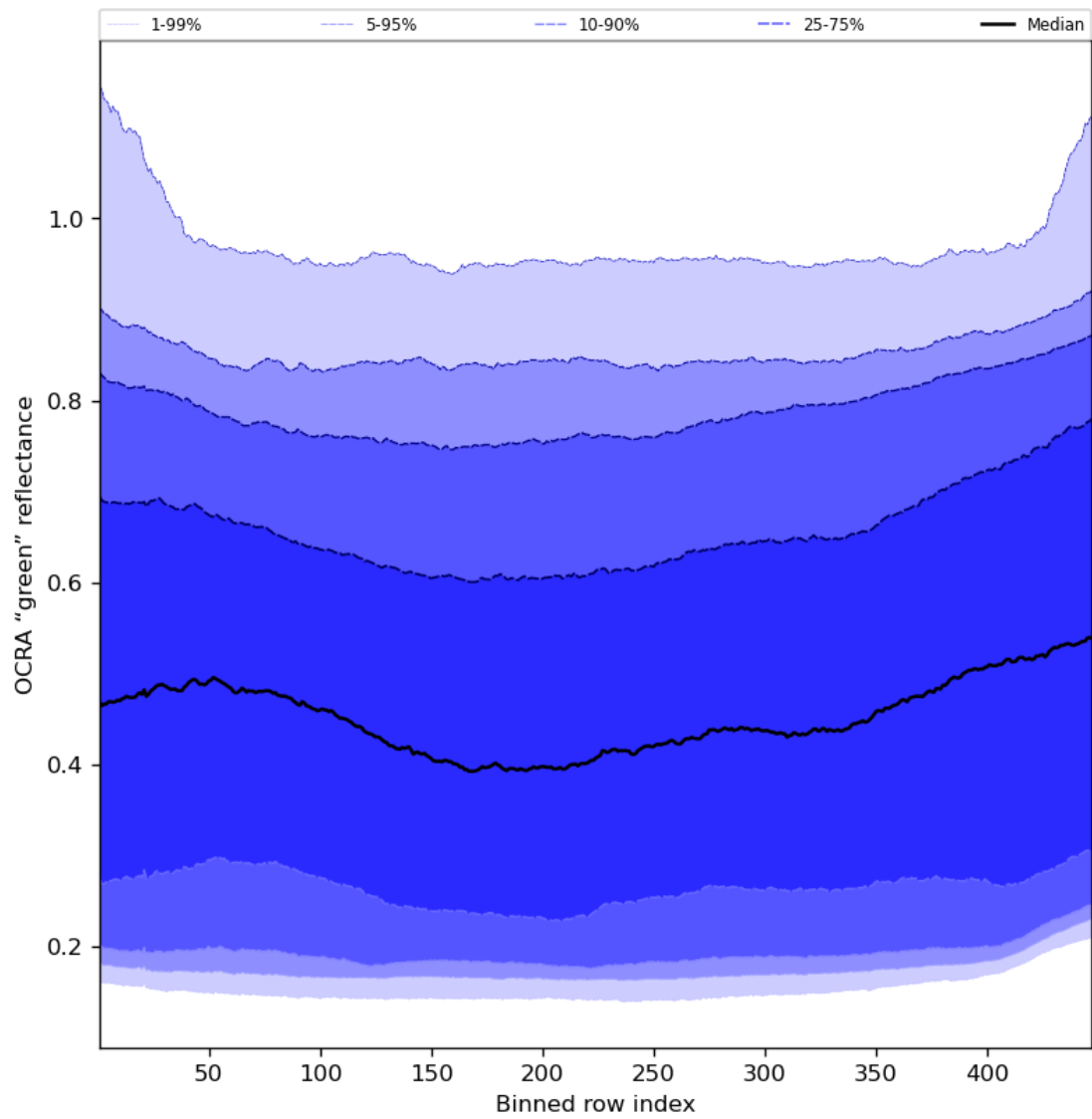
Figure 68: Along track statistics of “OCRA “green” reflectance” for 2024-06-11 to 2024-06-13
