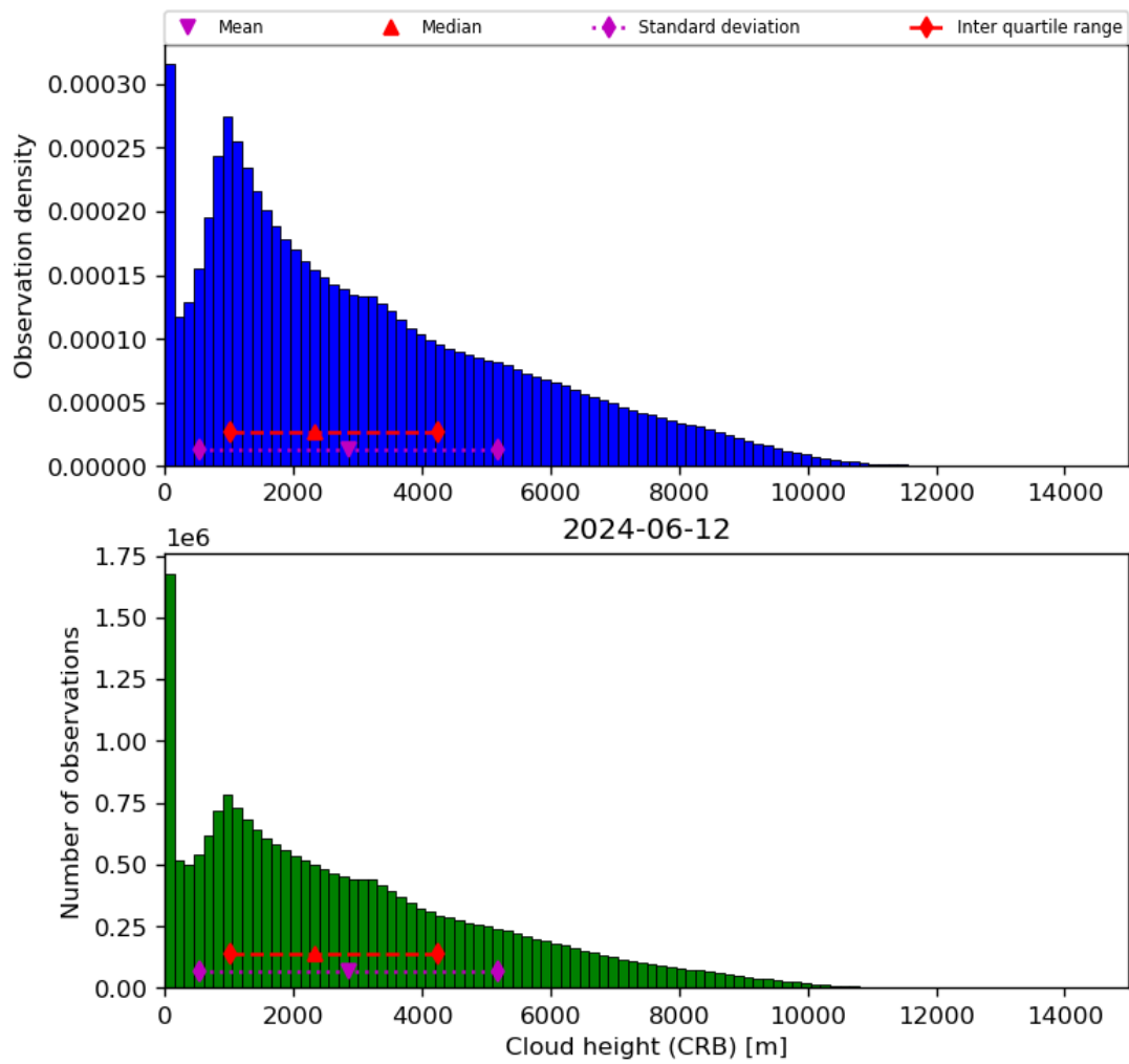
Figure 43: Histogram of “Cloud height (CRB)” for 2024-06-11 to 2024-06-13
