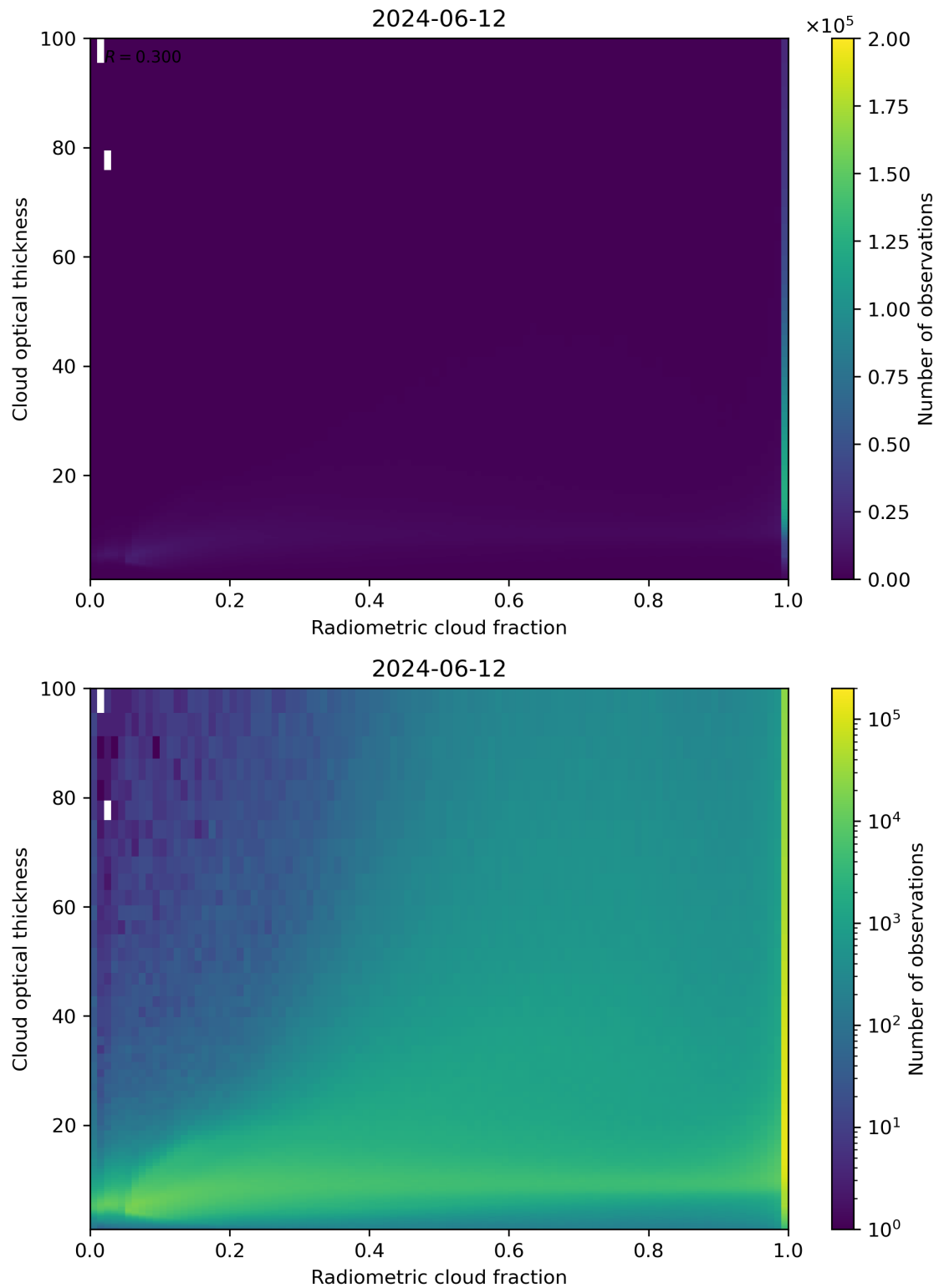
Figure 75: Scatter density plot of “Radiometric cloud fraction” against “Cloud optical thickness” for 2024-06-11 to 2024-06-13.
