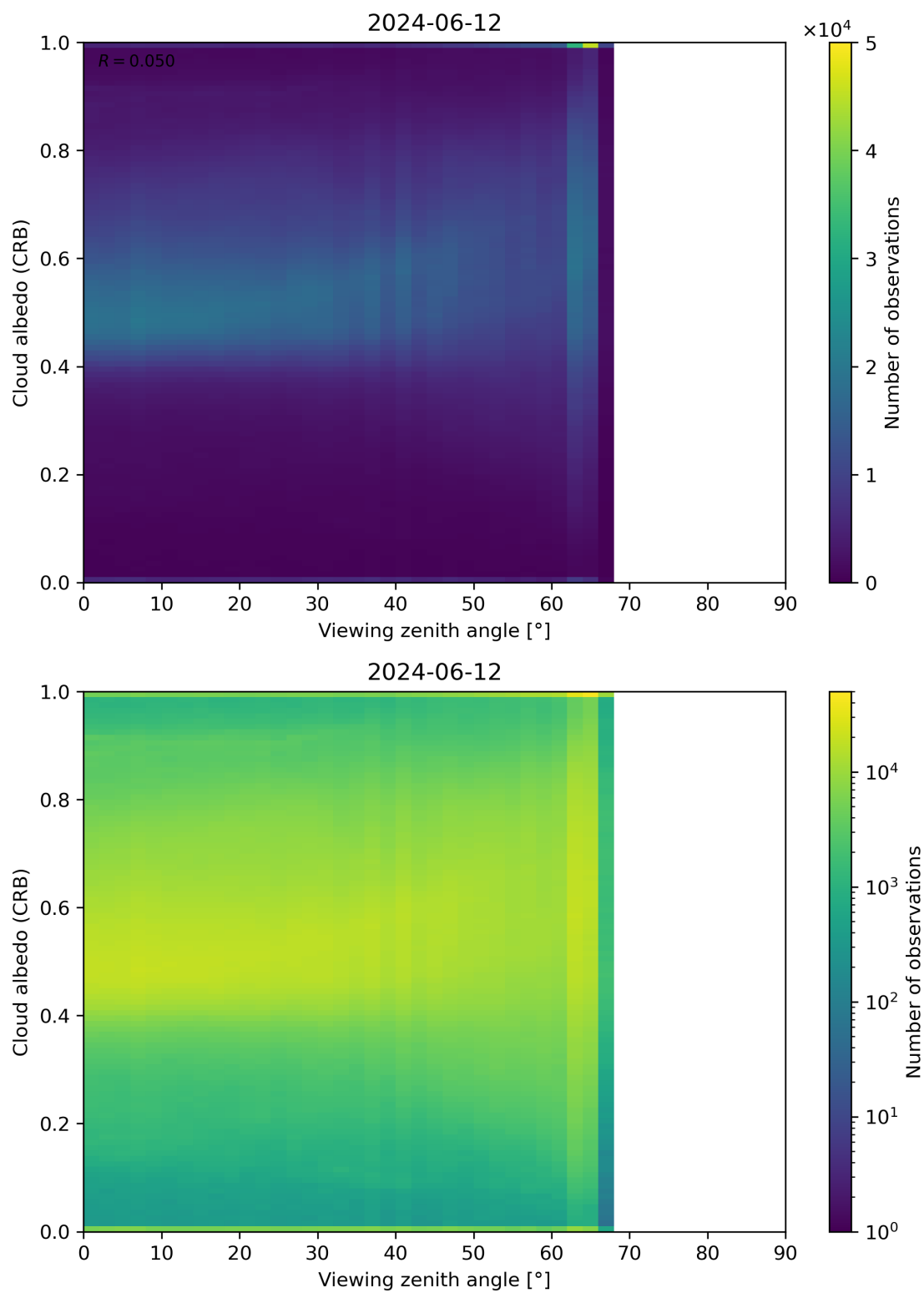
Figure 106: Scatter density plot of “Viewing zenith angle” against “Cloud albedo (CRB)” for 2024-06-11 to 2024-06-13.
