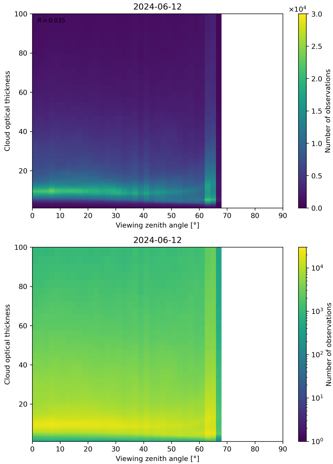
Figure 111: Scatter density plot of “Viewing zenith angle” against “Cloud optical thickness” for 2024-06-11 to 2024-06-13.
