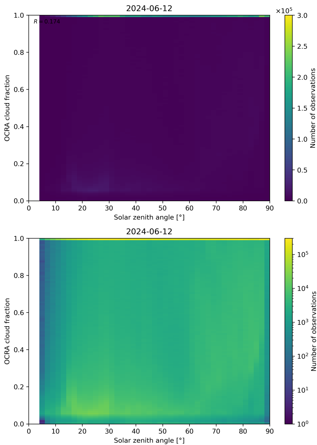
Figure 100: Scatter density plot of “Solar zenith angle” against “OCRA cloud fraction” for 2024-06-11 to 2024-06-13.
