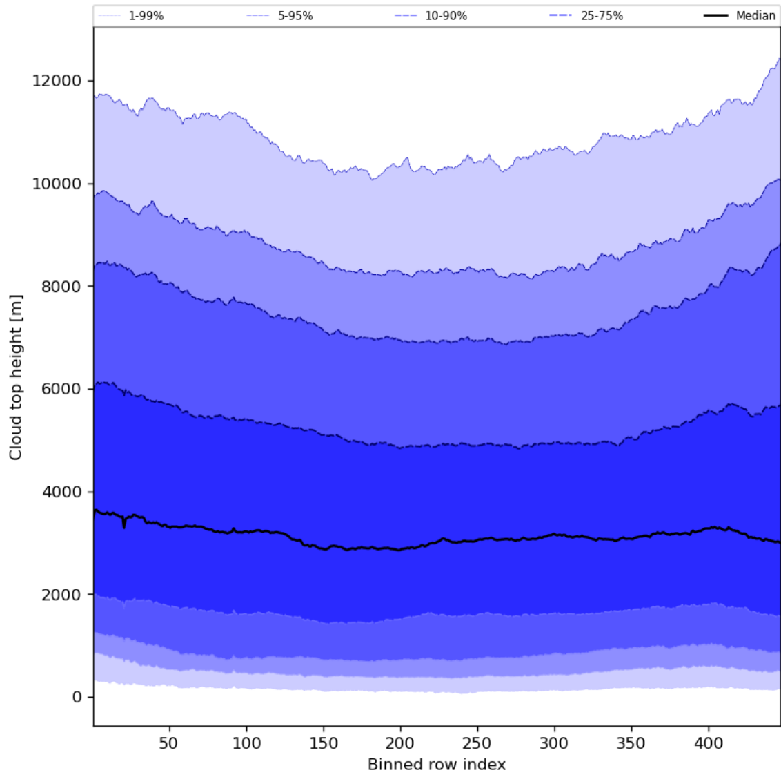
Figure 56: Along track statistics of “Cloud top height” for 2024-06-11 to 2024-06-13
