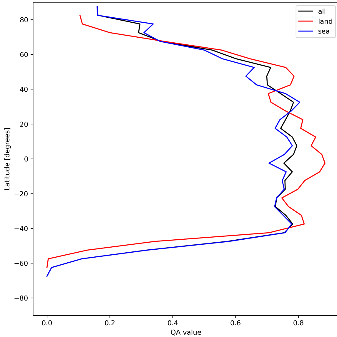
Figure 22: Zonal average of “QA value” for 2024-06-11 to 2024-06-13.
