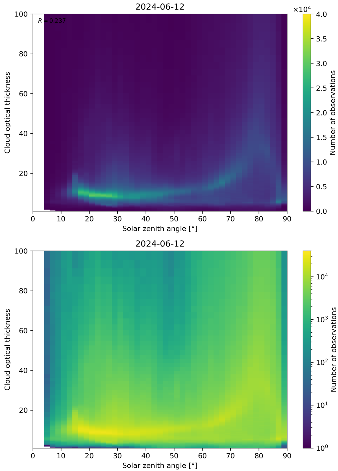
Figure 103: Scatter density plot of “Solar zenith angle” against “Cloud optical thickness” for 2024-06-11 to 2024-06-13.
