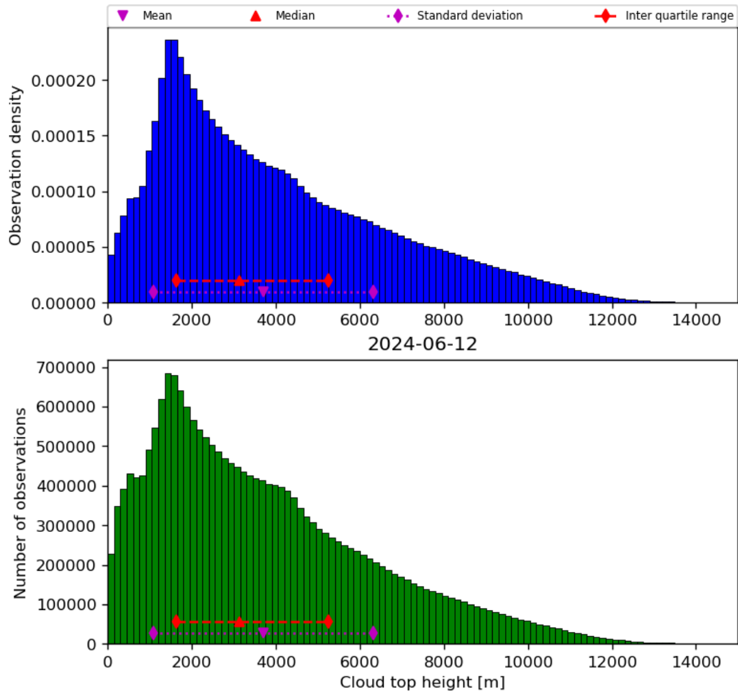
Figure 40: Histogram of “Cloud top height” for 2024-06-11 to 2024-06-13
