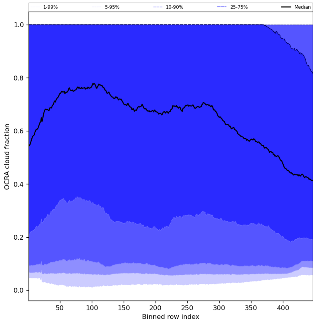
Figure 66: Along track statistics of “OCRA cloud fraction” for 2024-06-11 to 2024-06-13
