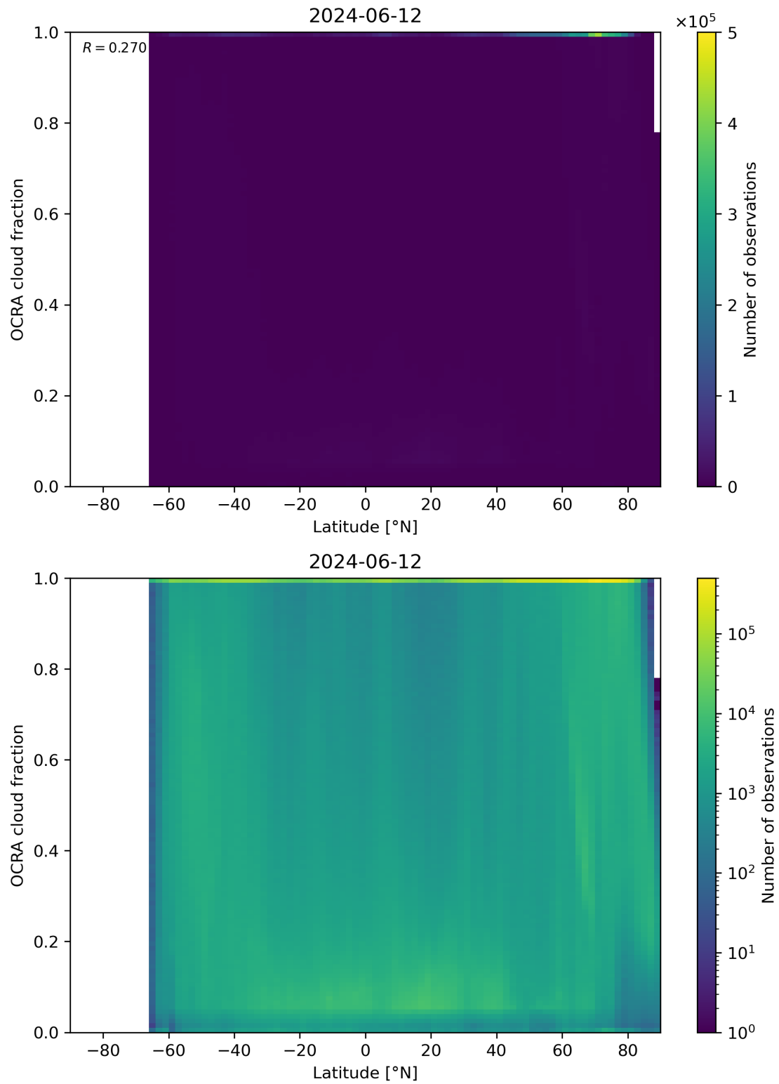
Figure 93: Scatter density plot of “Latitude” against “OCRA cloud fraction” for 2024-06-11 to 2024-06-13.
