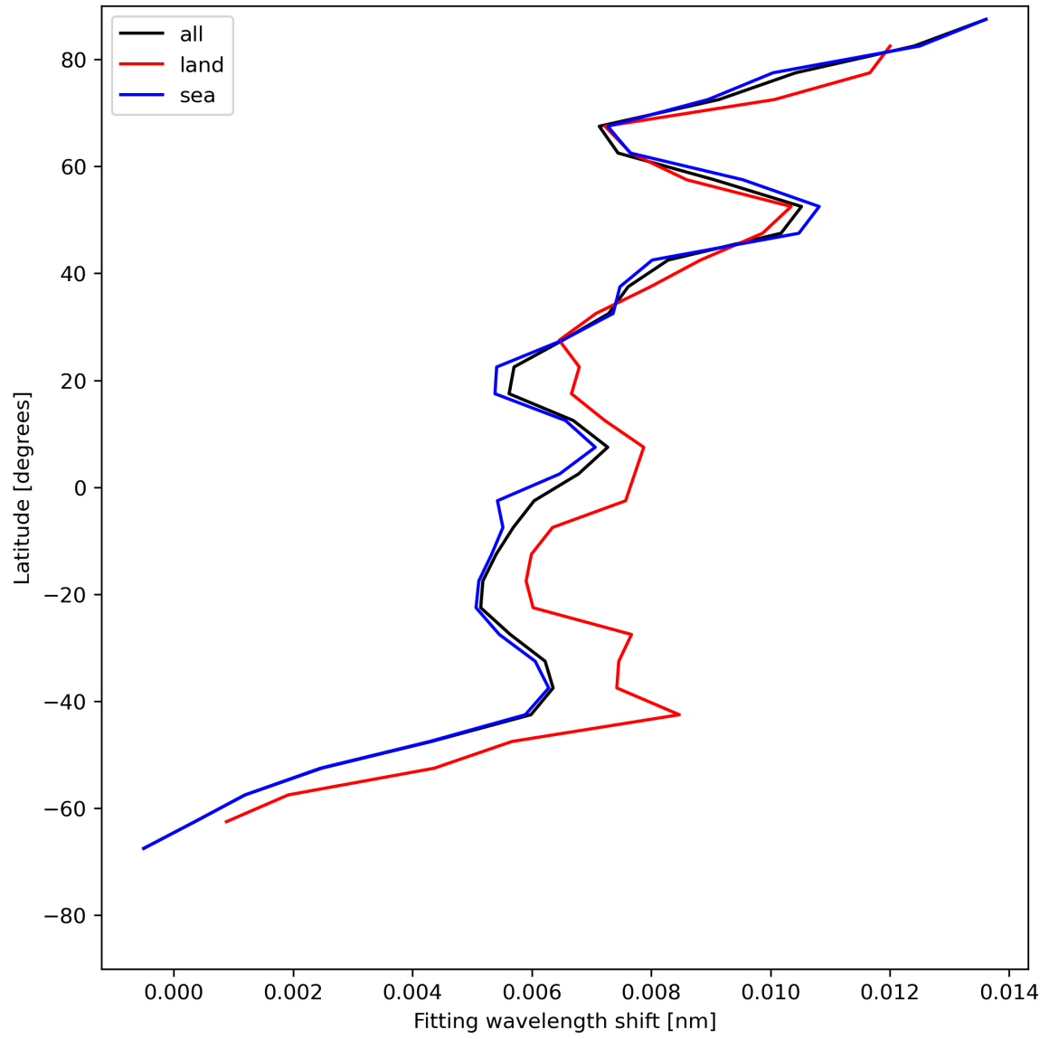
Figure 33: Zonal average of “Fitting wavelength shift” for 2024-06-11 to 2024-06-13.
