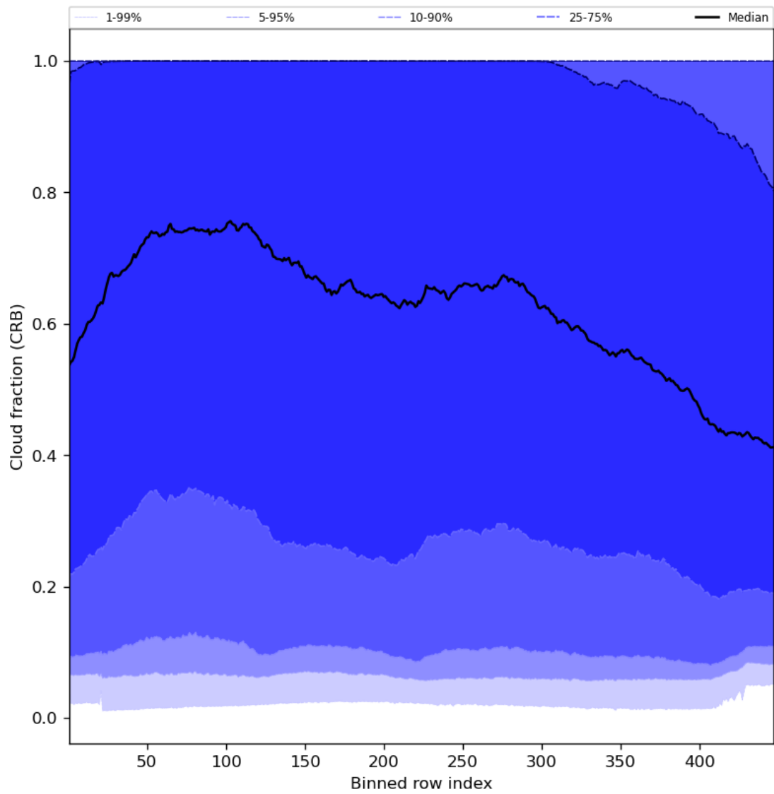
Figure 58: Along track statistics of “Cloud fraction (CRB)” for 2024-06-11 to 2024-06-13
