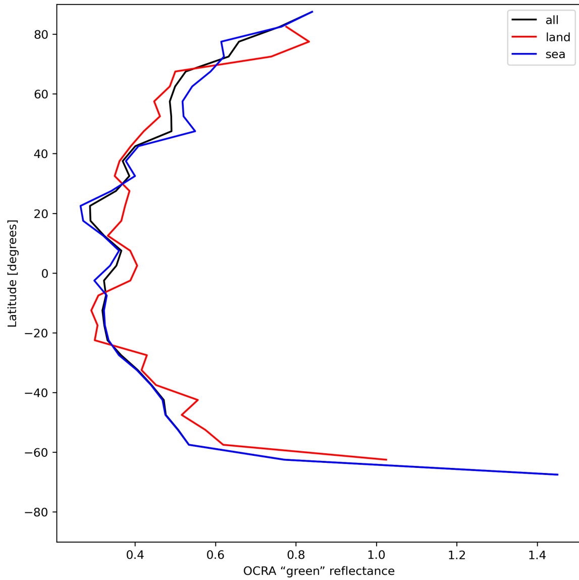
Figure 36: Zonal average of “OCRA “green” reflectance” for 2024-06-11 to 2024-06-13.
