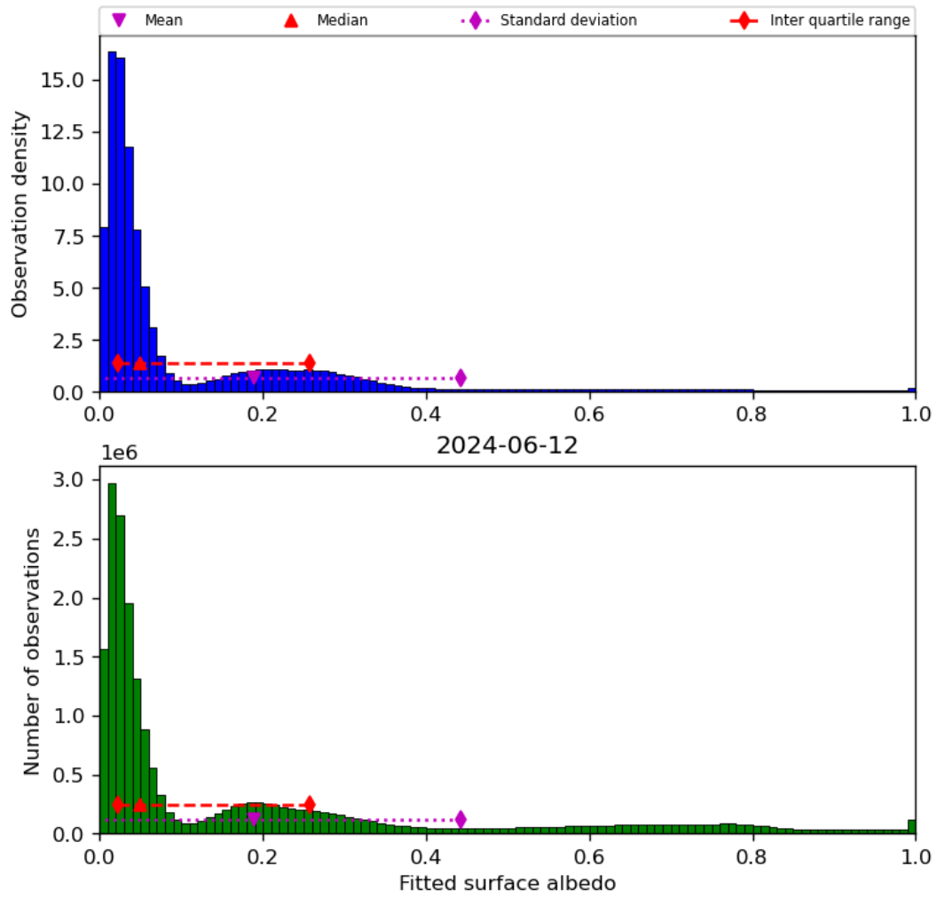
Figure 45: Histogram of “Fitted surface albedo” for 2024-06-11 to 2024-06-13
