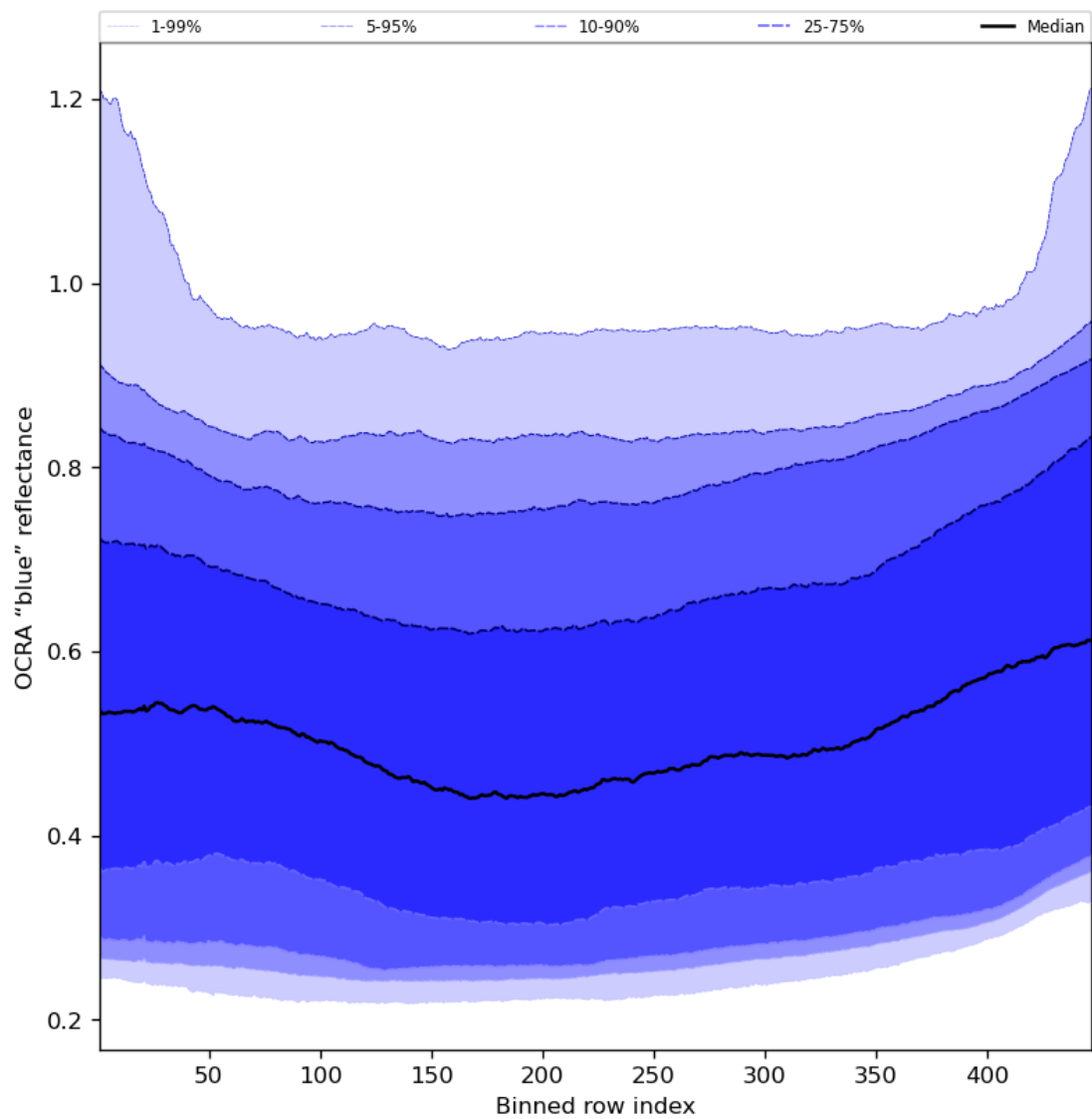
Figure 67: Along track statistics of “OCRA “blue” reflectance” for 2024-06-11 to 2024-06-13
