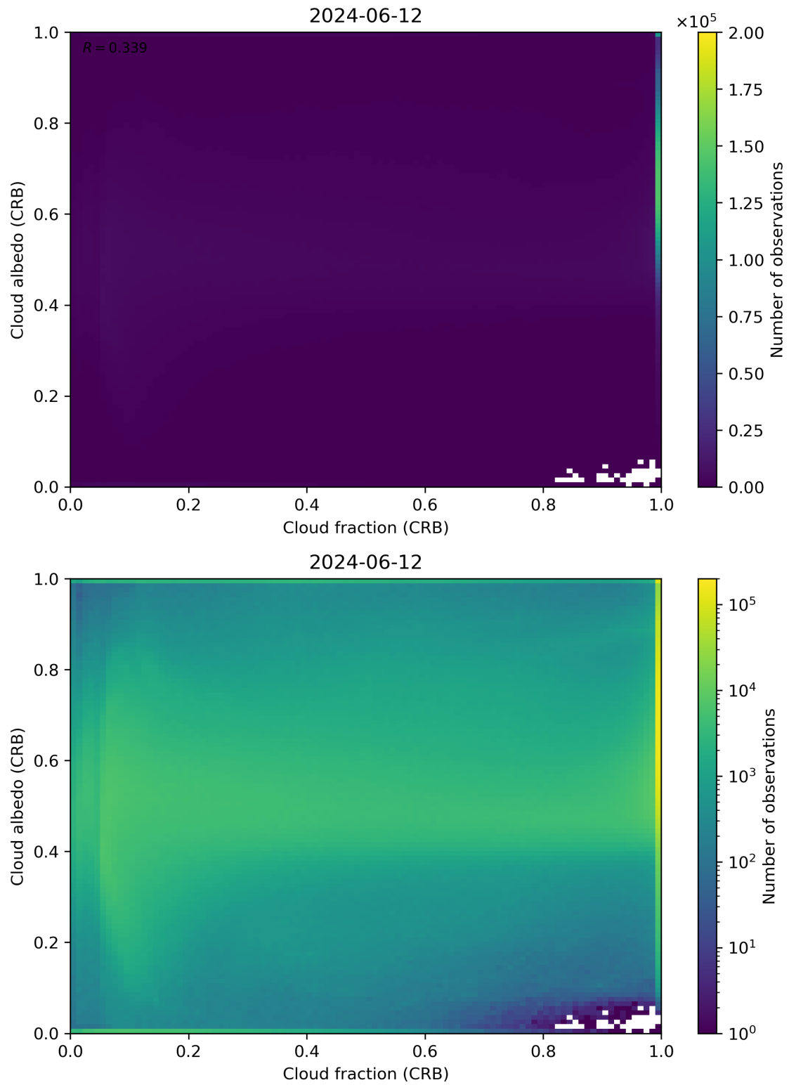
Figure 77: Scatter density plot of “Cloud fraction (CRB)” against “Cloud albedo (CRB)” for 2024-06-11 to 2024-06-13.
