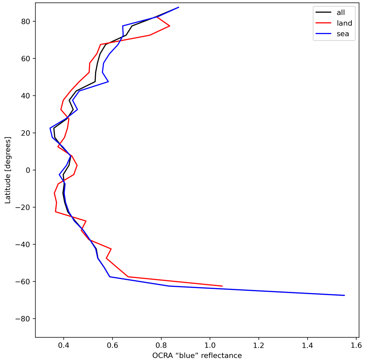
Figure 35: Zonal average of “OCRA “blue” reflectance” for 2024-06-11 to 2024-06-13.
