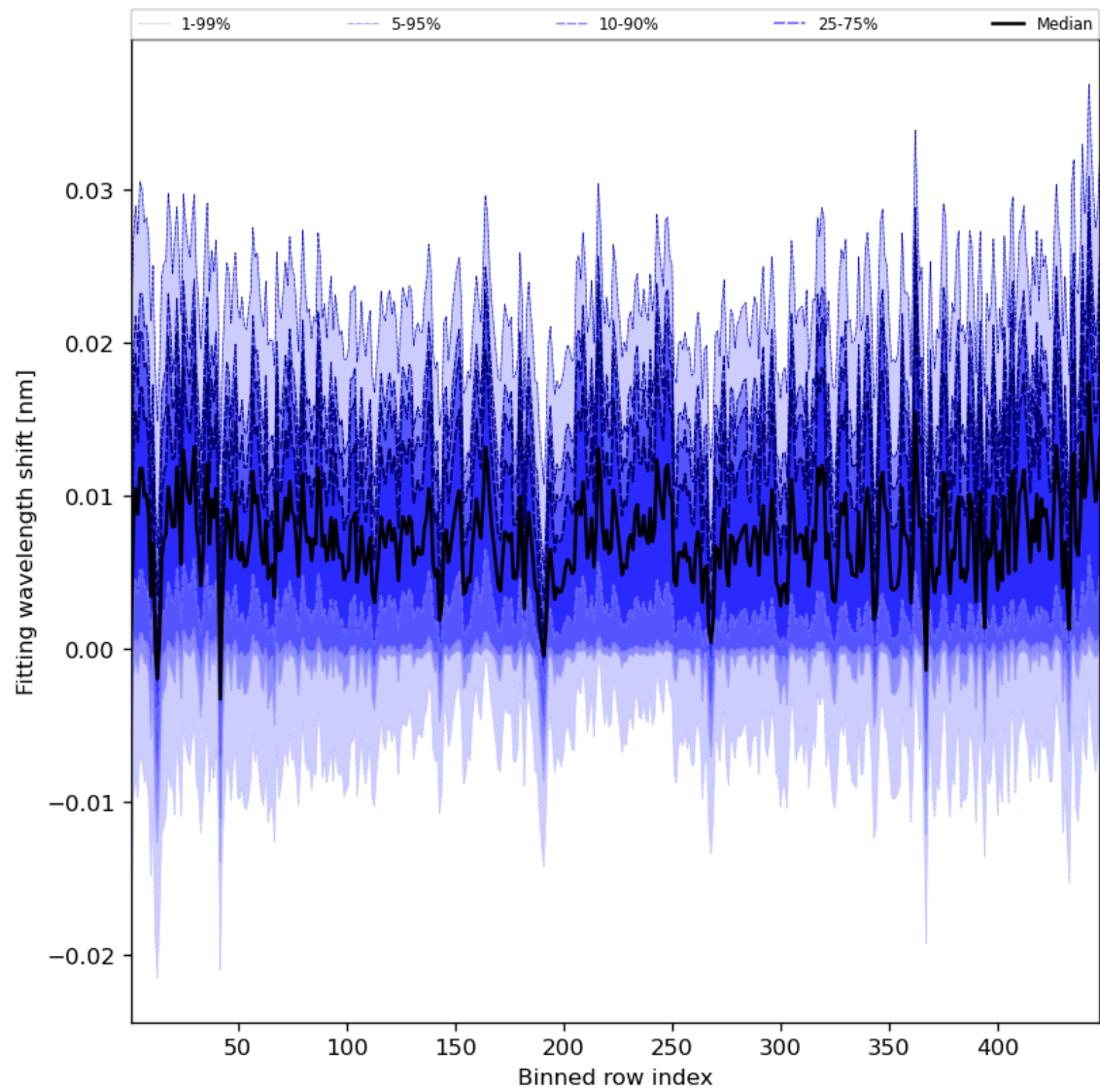
Figure 65: Along track statistics of “Fitting wavelength shift” for 2024-06-11 to 2024-06-13
