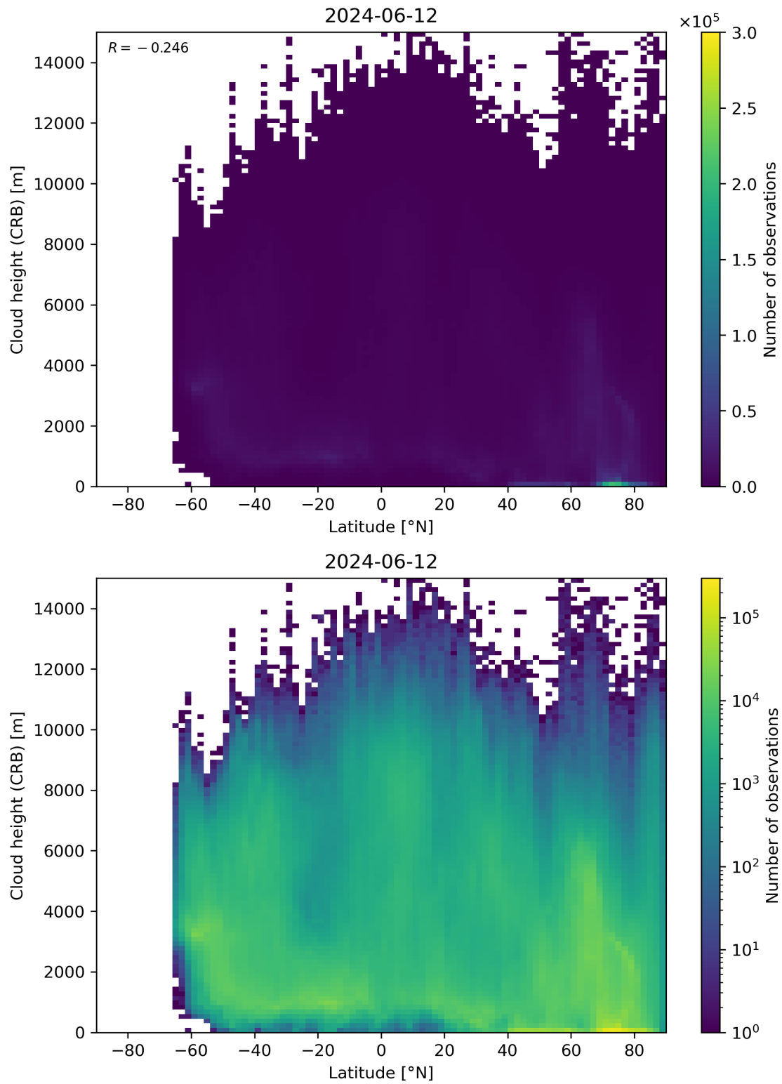
Figure 95: Scatter density plot of “Latitude” against “Cloud height (CRB)” for 2024-06-11 to 2024-06-13.
