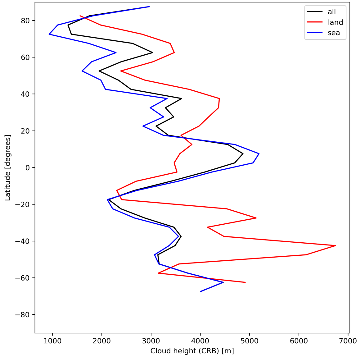
Figure 27: Zonal average of “Cloud height (CRB)” for 2024-06-11 to 2024-06-13.
