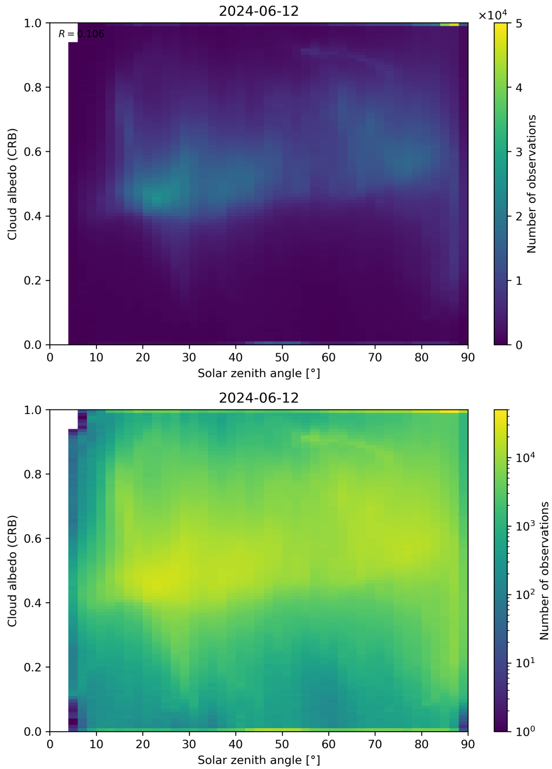
Figure 98: Scatter density plot of “Solar zenith angle” against “Cloud albedo (CRB)” for 2024-06-11 to 2024-06-13.
