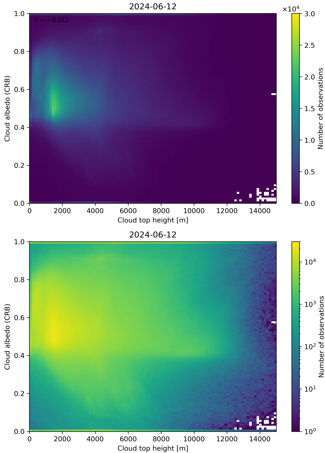
Figure 86: Scatter density plot of “Cloud top height” against “Cloud albedo (CRB)” for 2024-06-11 to 2024-06-13.
