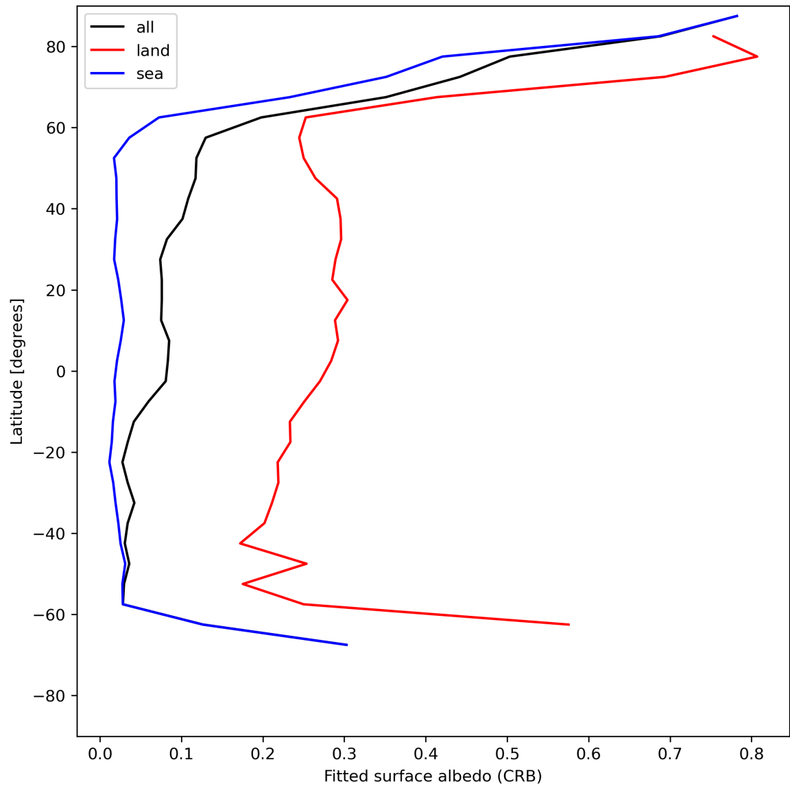
Figure 30: Zonal average of “Fitted surface albedo (CRB)” for 2024-06-11 to 2024-06-13.
