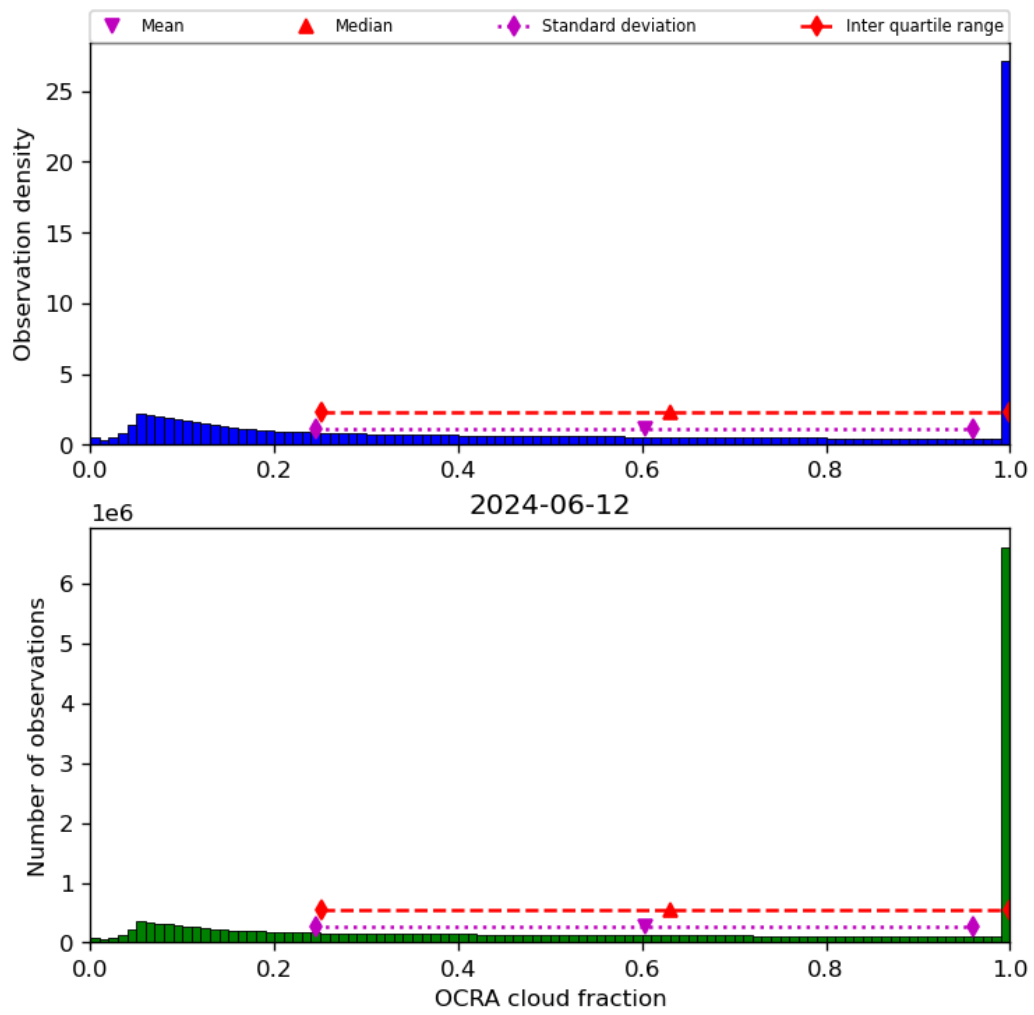
Figure 50: Histogram of “OCRA cloud fraction” for 2024-06-11 to 2024-06-13
