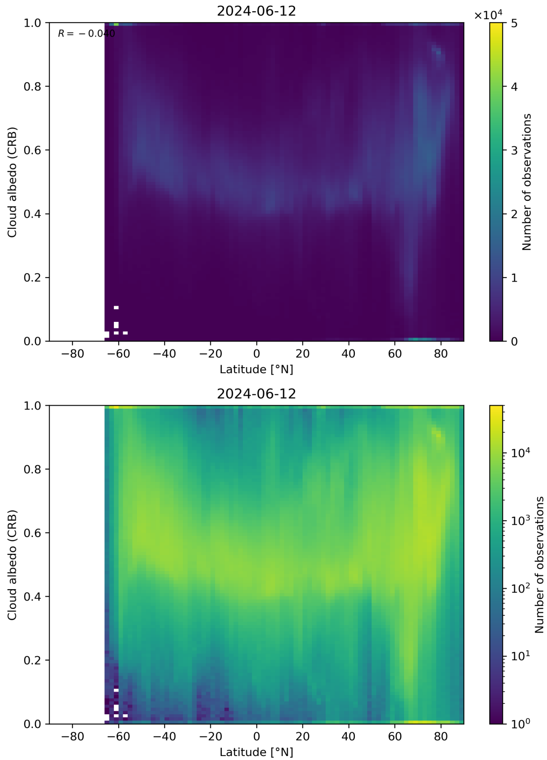
Figure 91: Scatter density plot of “Latitude” against “Cloud albedo (CRB)” for 2024-06-11 to 2024-06-13.
