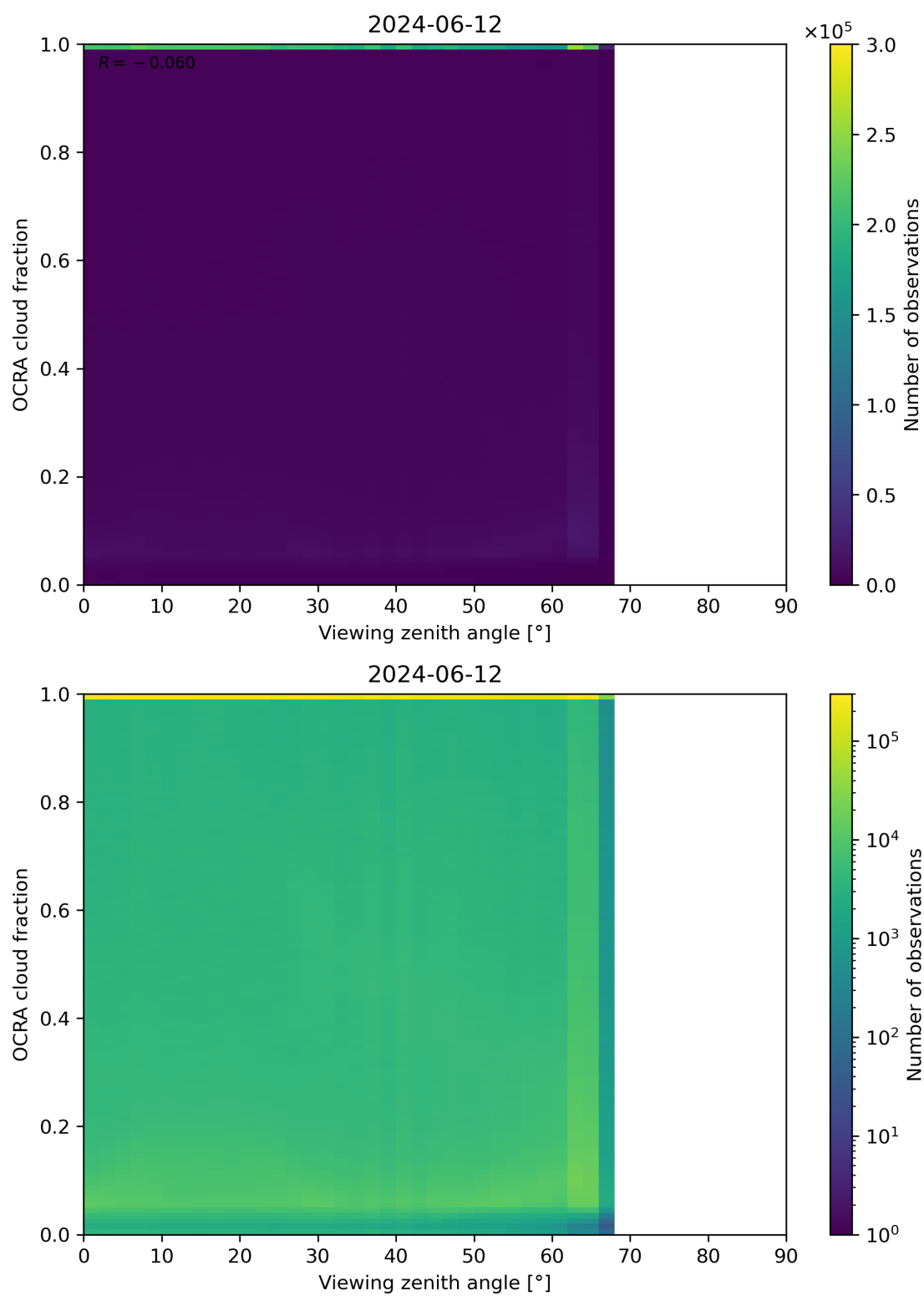
Figure 108: Scatter density plot of “Viewing zenith angle” against “OCRA cloud fraction” for 2024-06-11 to 2024-06-13.
