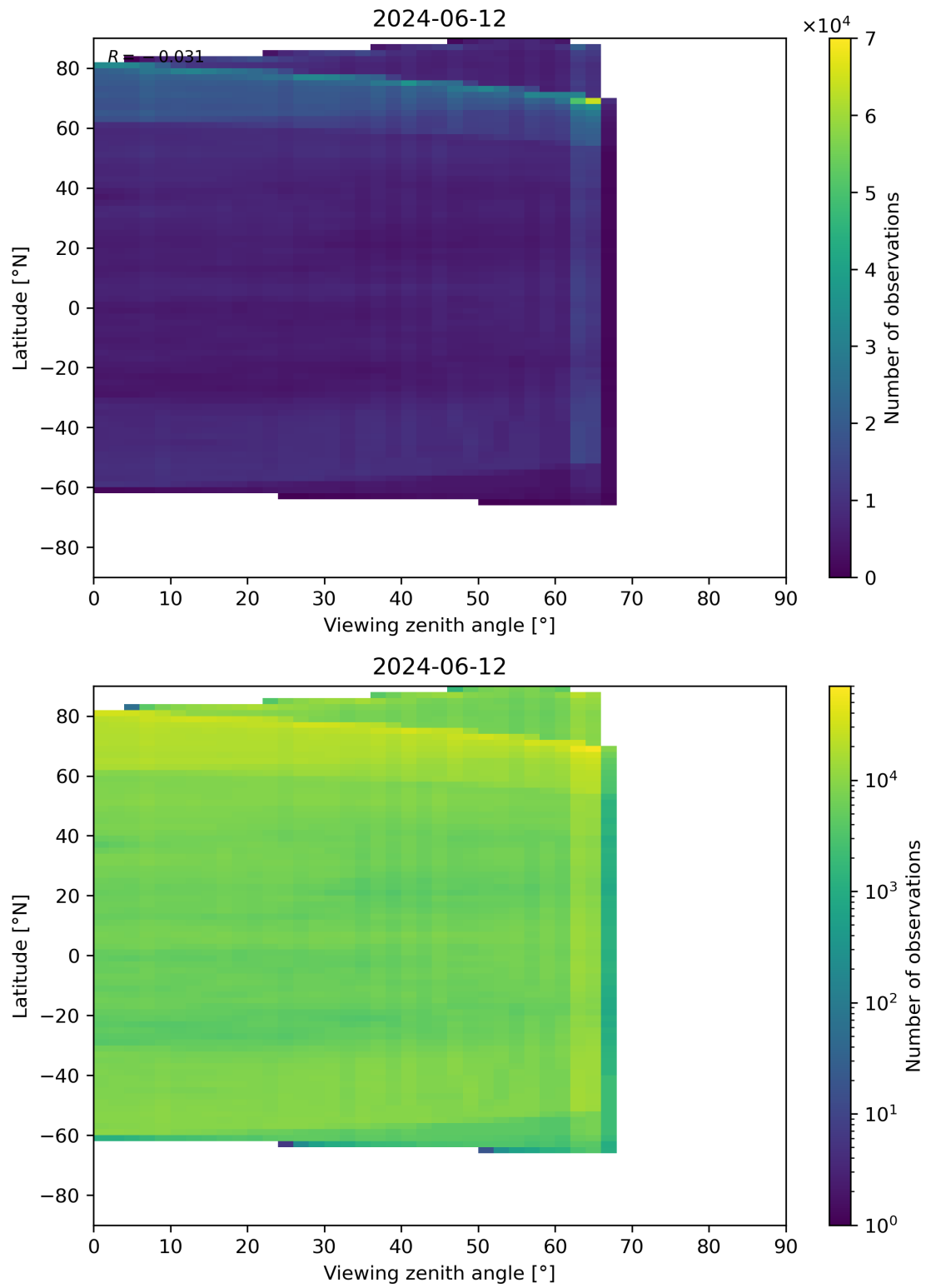
Figure 113: Scatter density plot of “Viewing zenith angle” against “Latitude” for 2024-06-11 to 2024-06-13.
