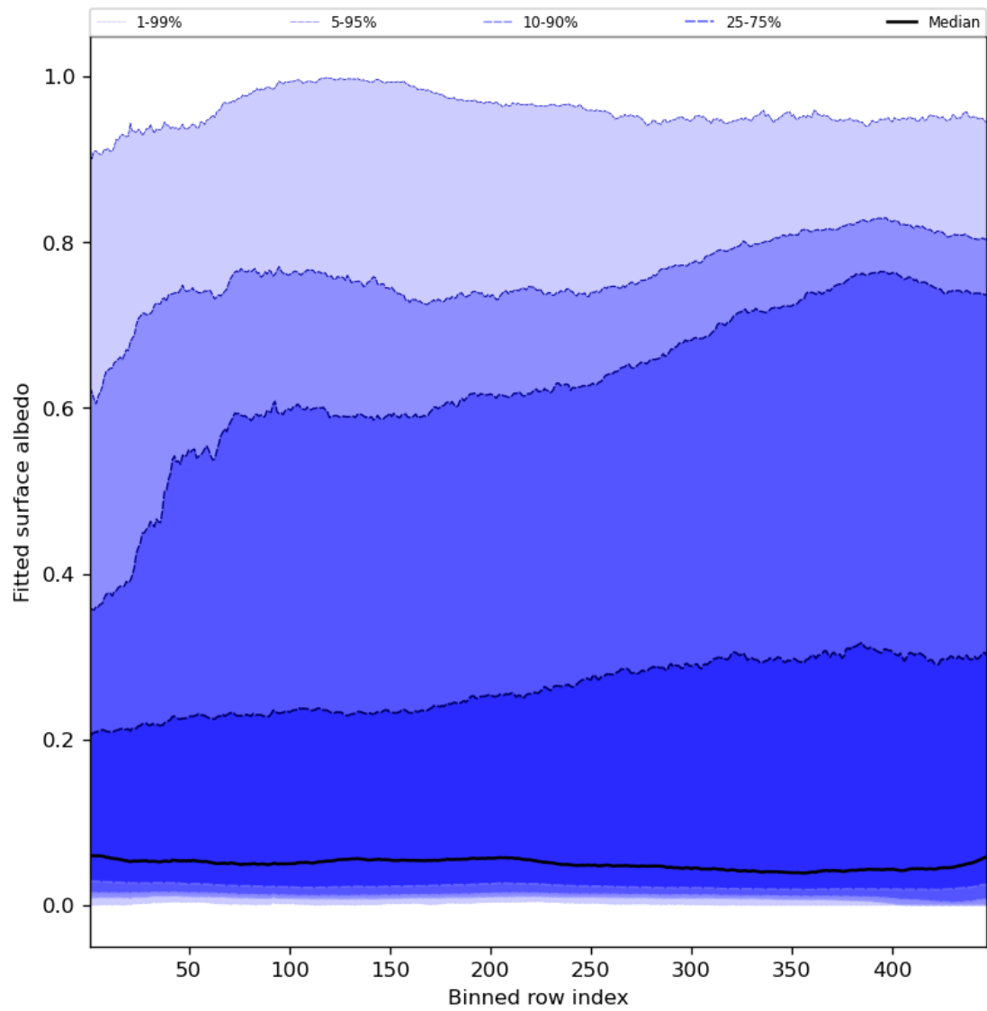
Figure 61: Along track statistics of “Fitted surface albedo” for 2024-06-11 to 2024-06-13
