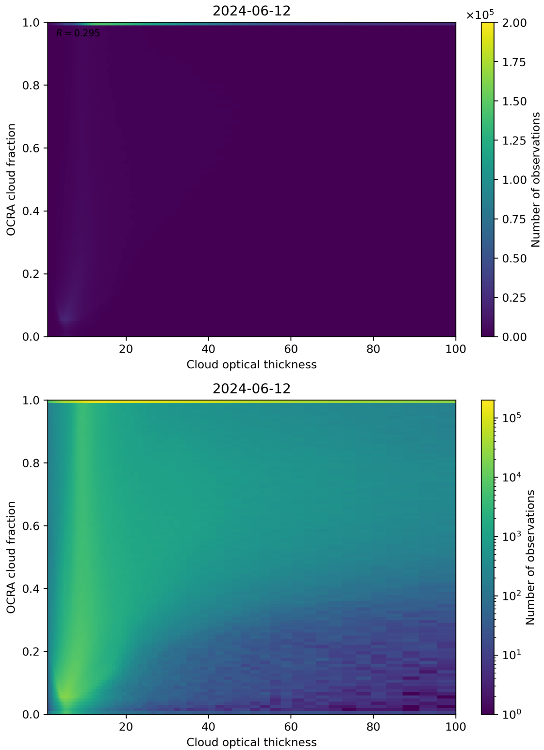
Figure 83: Scatter density plot of “Cloud optical thickness” against “OCRA cloud fraction” for 2024-06-11 to 2024-06-13.
