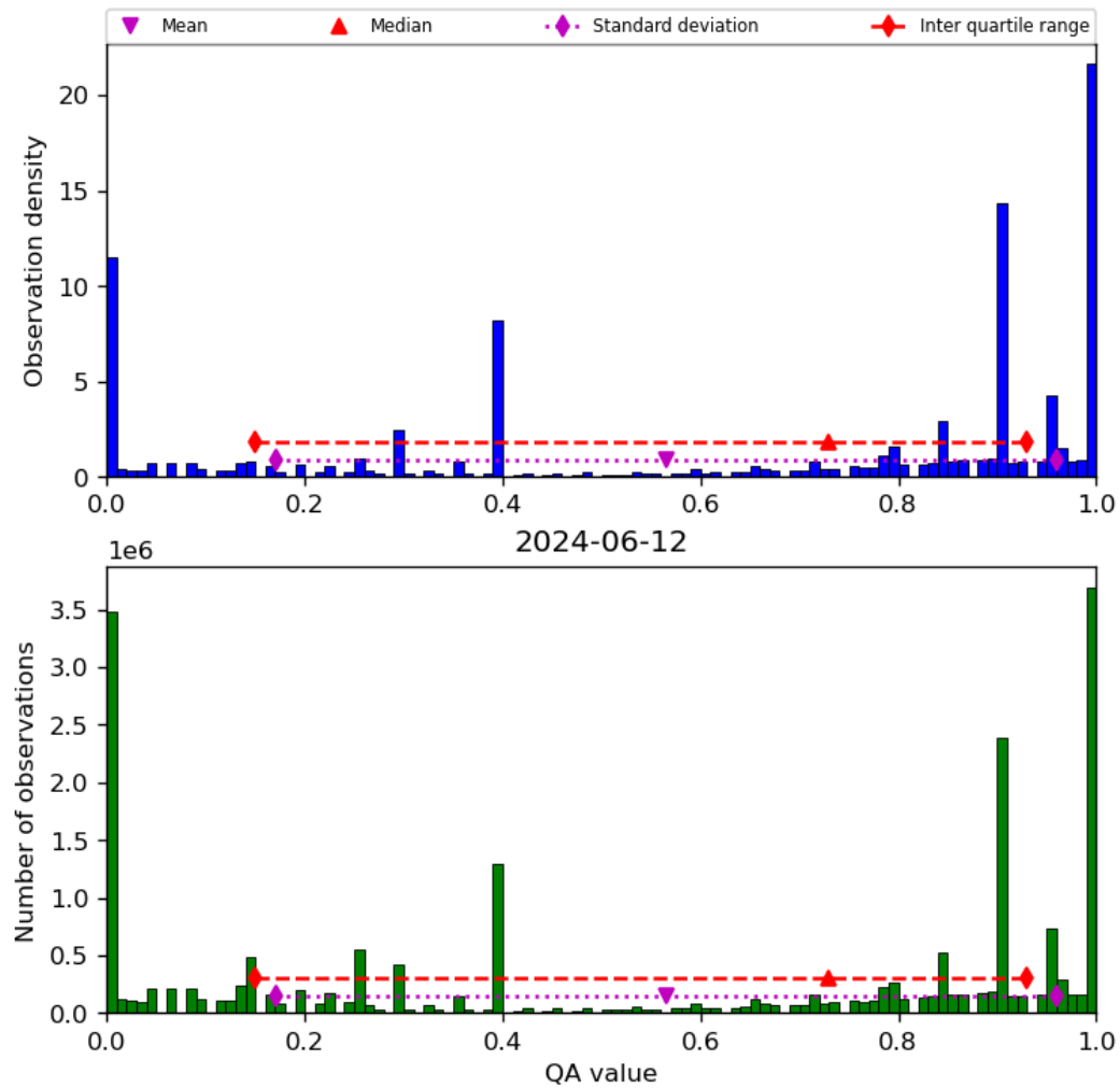
Figure 38: Histogram of “QA value” for 2024-06-11 to 2024-06-13
