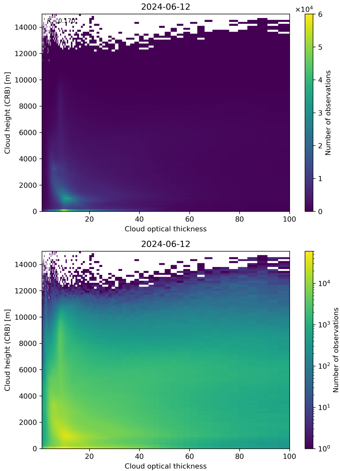
Figure 85: Scatter density plot of “Cloud optical thickness” against “Cloud height (CRB)” for 2024-06-11 to 2024-06-13.
