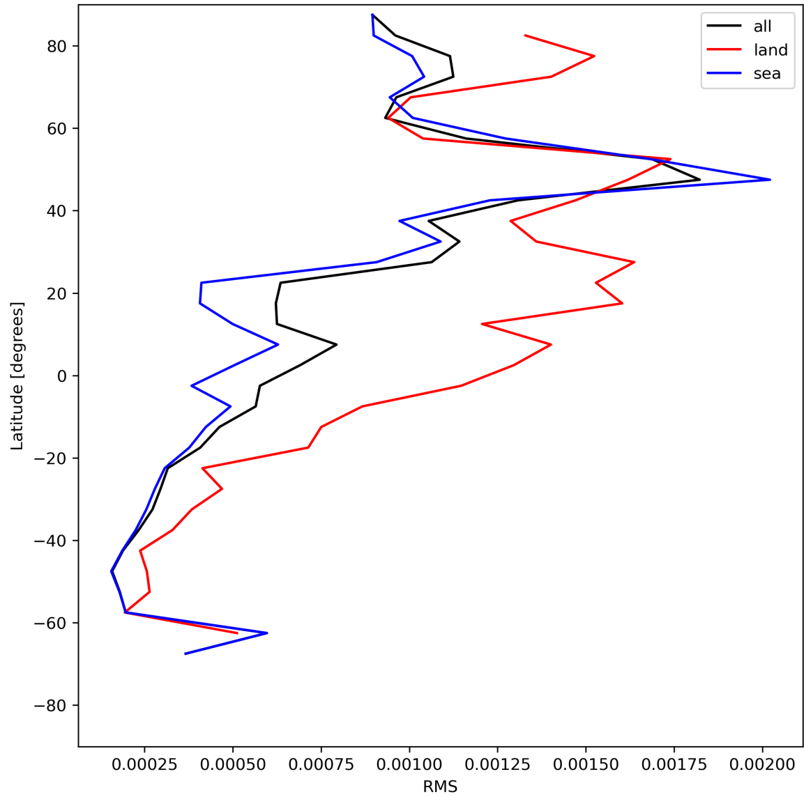
Figure 31: Zonal average of “RMS” for 2024-06-11 to 2024-06-13.
