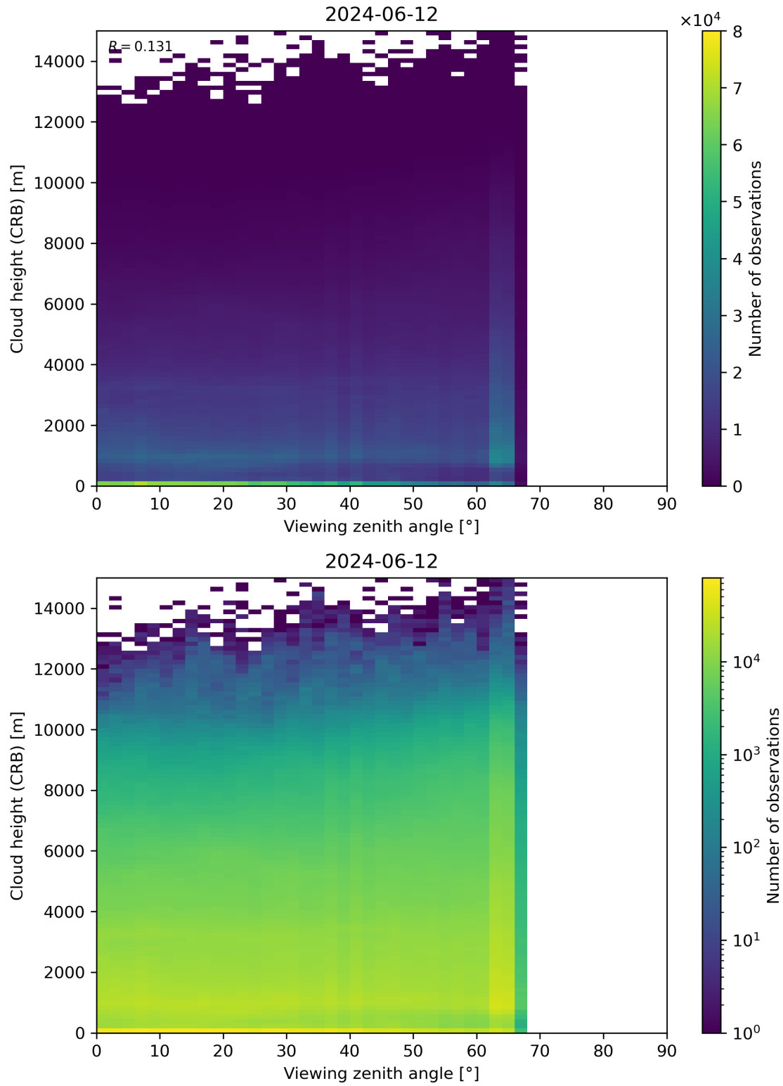
Figure 110: Scatter density plot of “Viewing zenith angle” against “Cloud height (CRB)” for 2024-06-11 to 2024-06-13.
