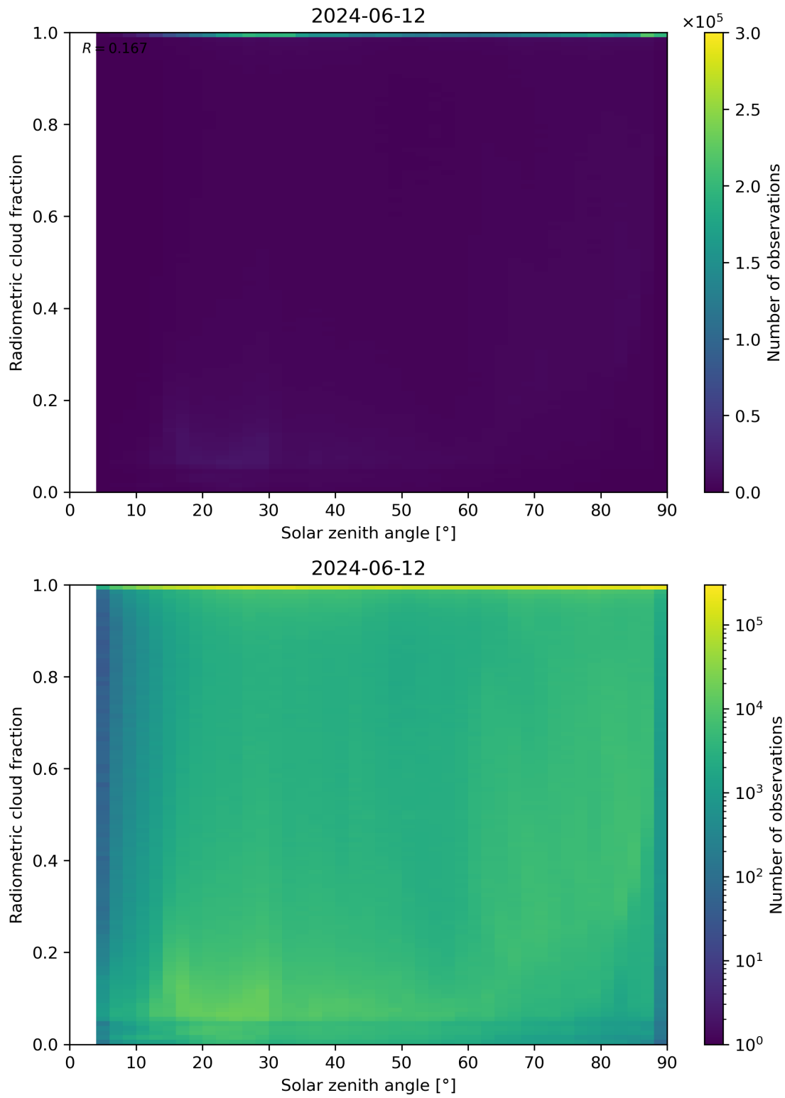
Figure 99: Scatter density plot of “Solar zenith angle” against “Radiometric cloud fraction” for 2024-06-11 to 2024-06-13.
