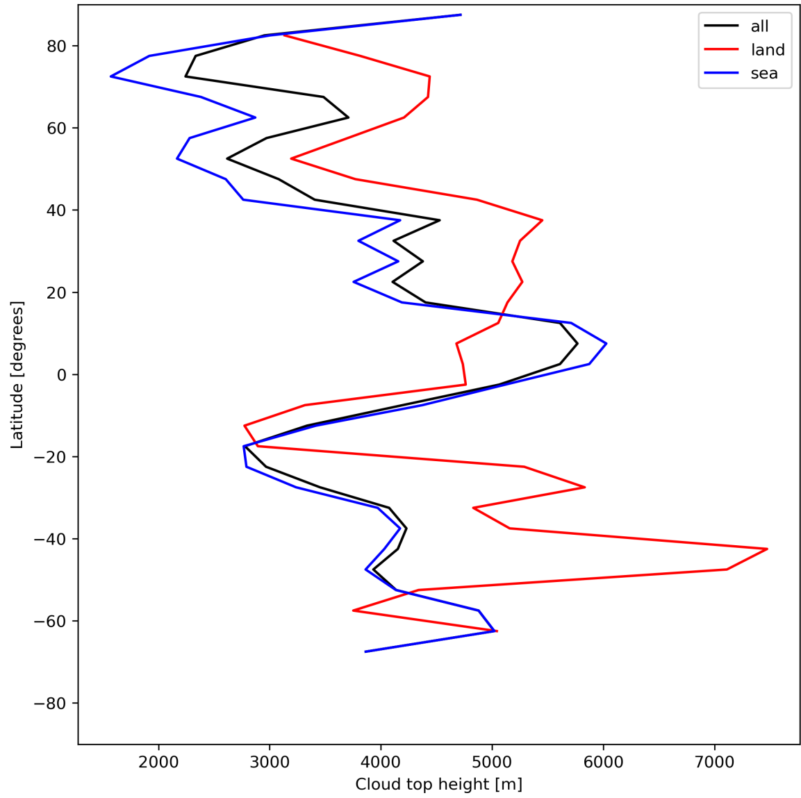
Figure 24: Zonal average of “Cloud top height” for 2024-06-11 to 2024-06-13.
