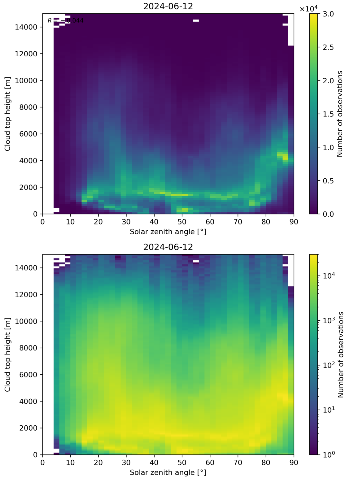
Figure 104: Scatter density plot of “Solar zenith angle” against “Cloud top height” for 2024-06-11 to 2024-06-13.
