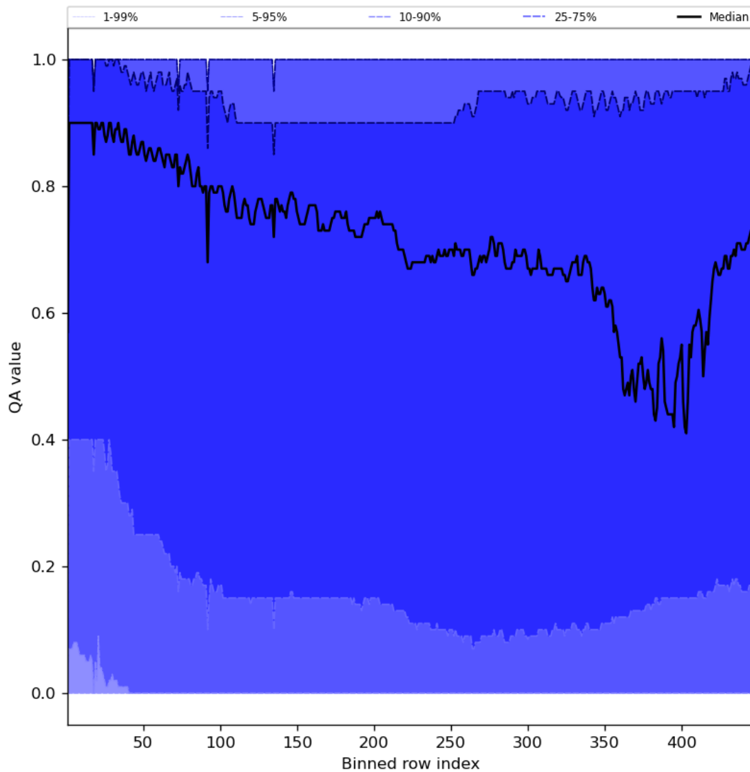
Figure 54: Along track statistics of “QA value” for 2024-06-13 to 2024-06-14
