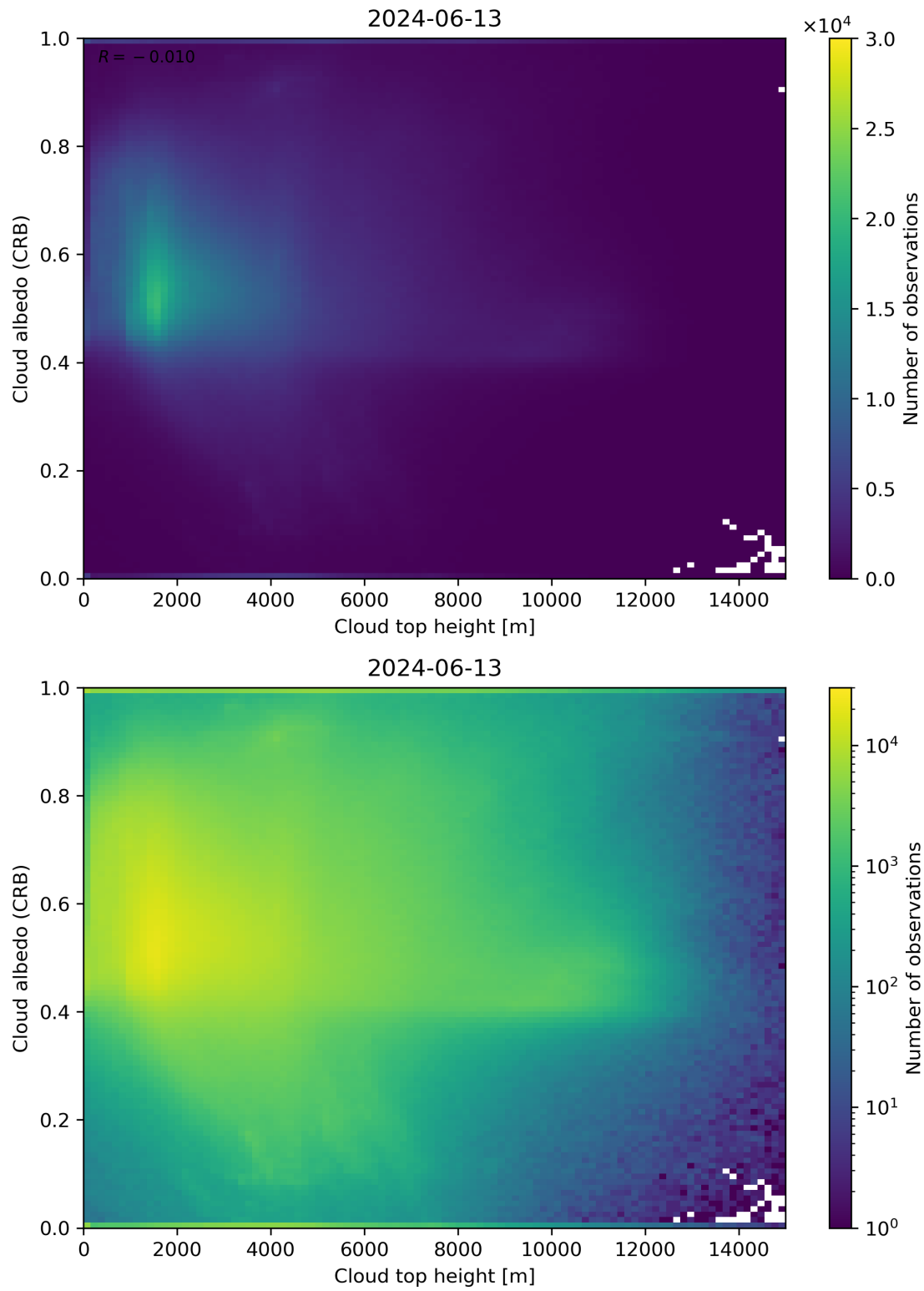
Figure 86: Scatter density plot of “Cloud top height” against “Cloud albedo (CRB)” for 2024-06-13 to 2024-06-14.
