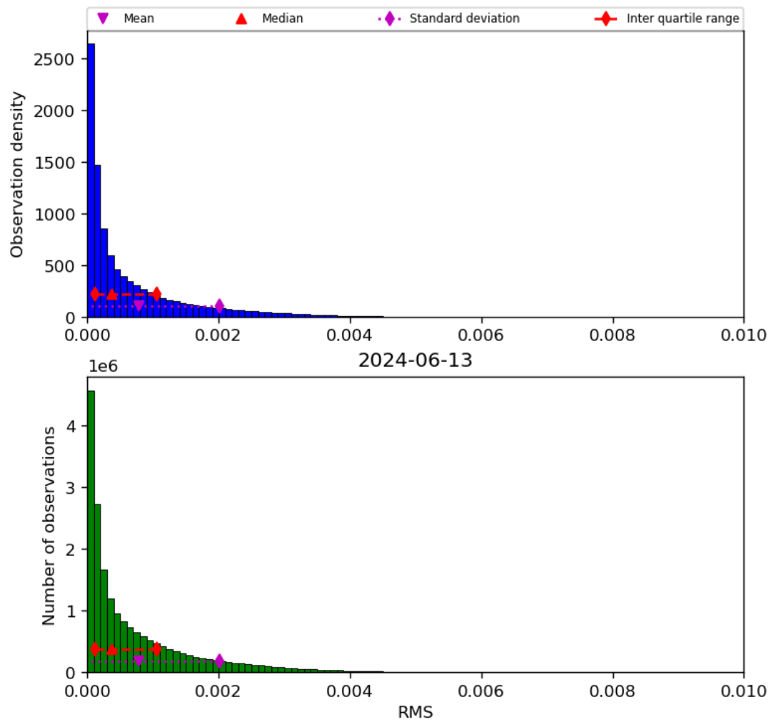
Figure 47: Histogram of “RMS” for 2024-06-13 to 2024-06-14
