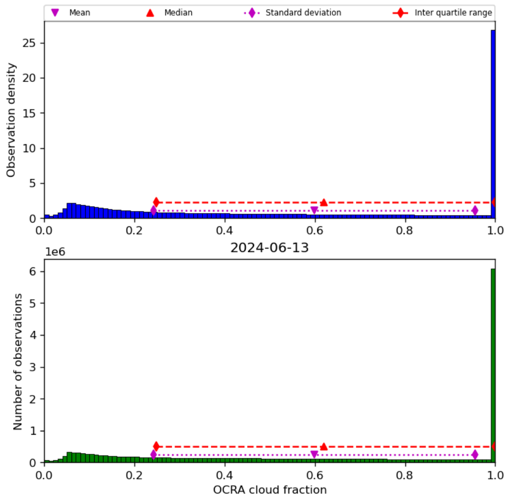
Figure 50: Histogram of “OCRA cloud fraction” for 2024-06-13 to 2024-06-14
