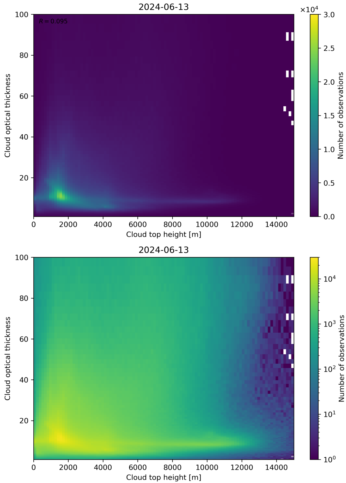
Figure 90: Scatter density plot of “Cloud top height” against “Cloud optical thickness” for 2024-06-13 to 2024-06-14.
