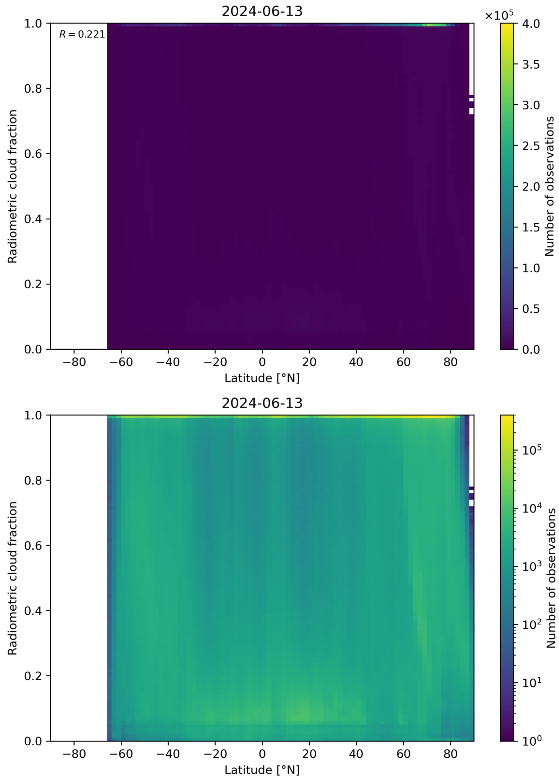
Figure 92: Scatter density plot of “Latitude” against “Radiometric cloud fraction” for 2024-06-13 to 2024-06-14.
