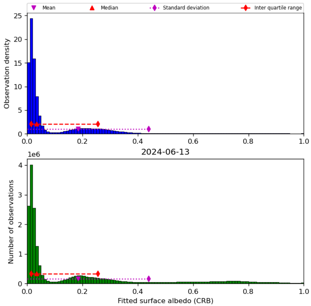
Figure 46: Histogram of “Fitted surface albedo (CRB)” for 2024-06-13 to 2024-06-14
