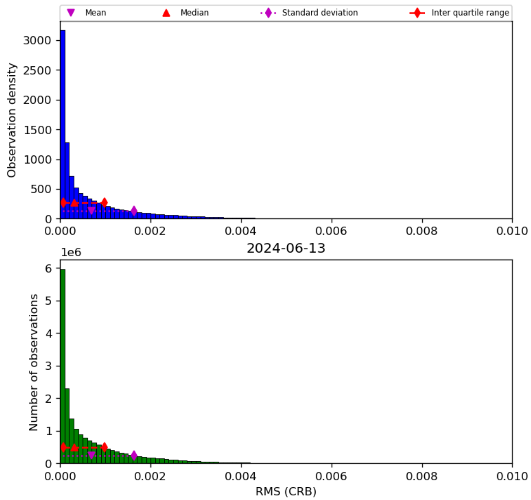
Figure 48: Histogram of "RMS (CRB)" for 2024-06-13 to 2024-06-14
