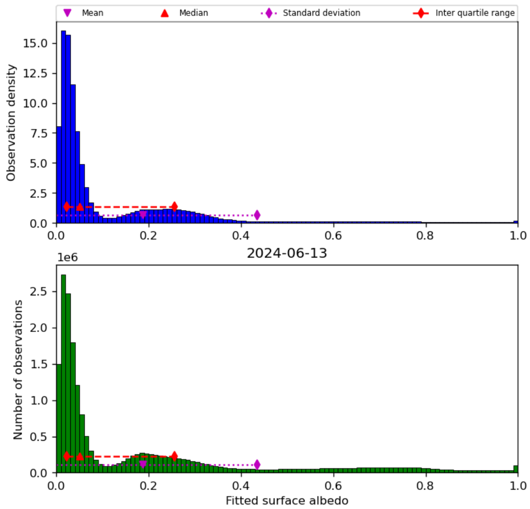
Figure 45: Histogram of “Fitted surface albedo” for 2024-06-13 to 2024-06-14
