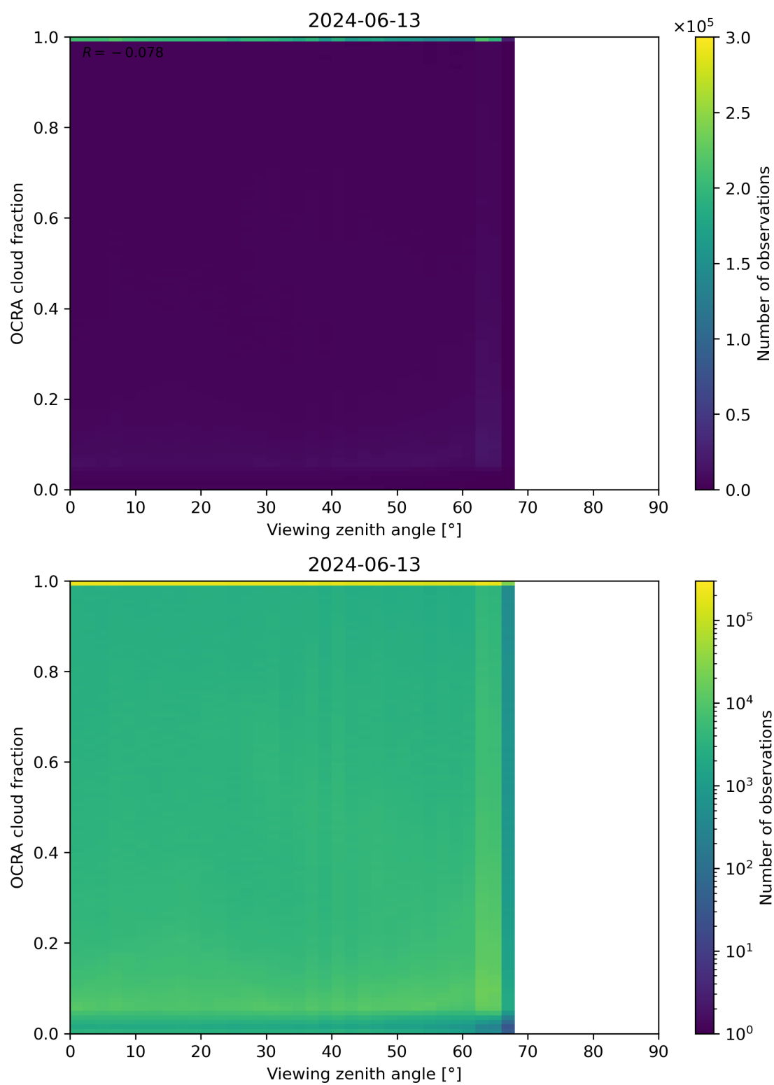
Figure 108: Scatter density plot of “Viewing zenith angle” against “OCRA cloud fraction” for 2024-06-13 to 2024-06-14.
