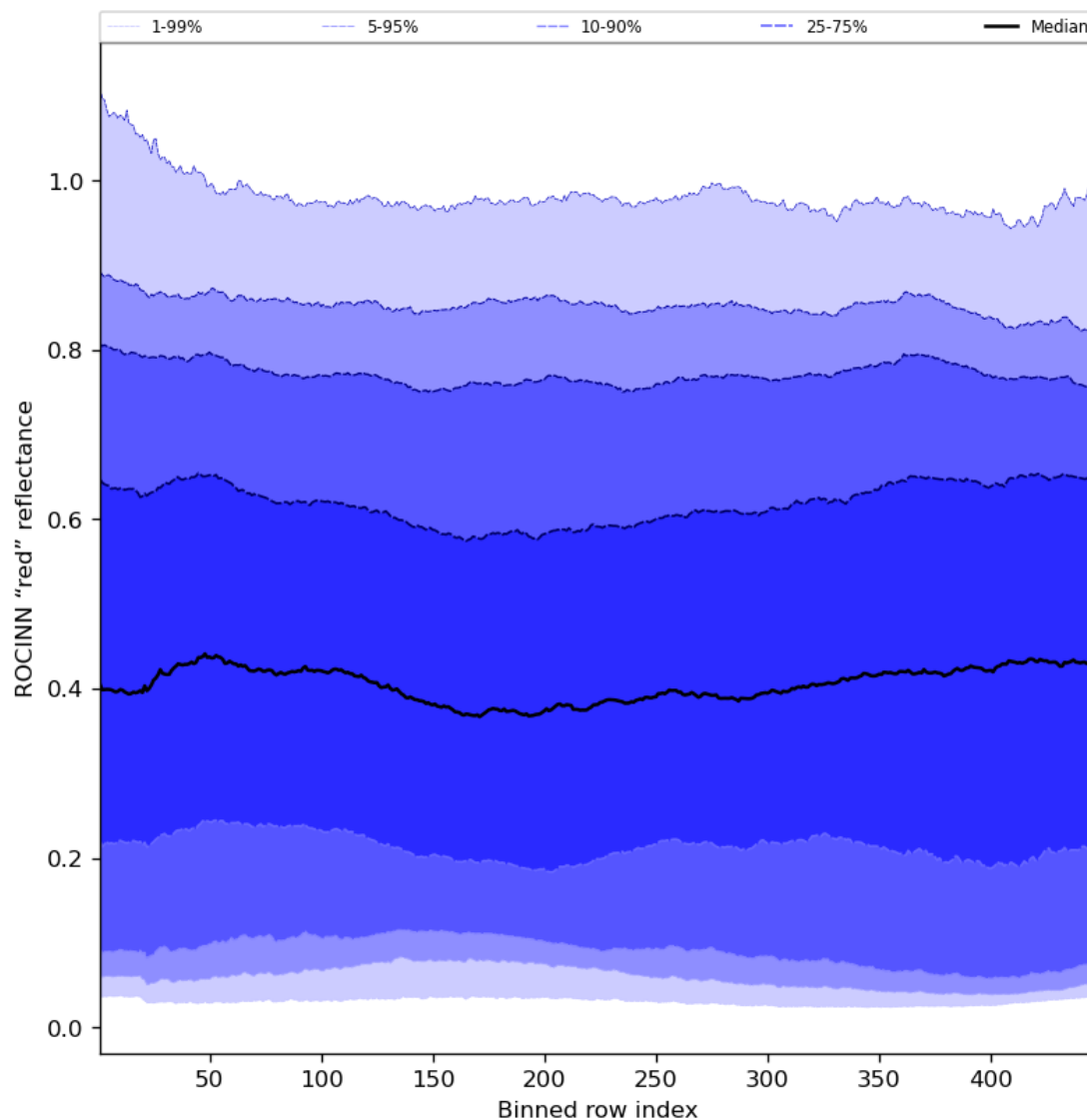
Figure 69: Along track statistics of “ROCINN “red” reflectance” for 2024-06-13 to 2024-06-14
