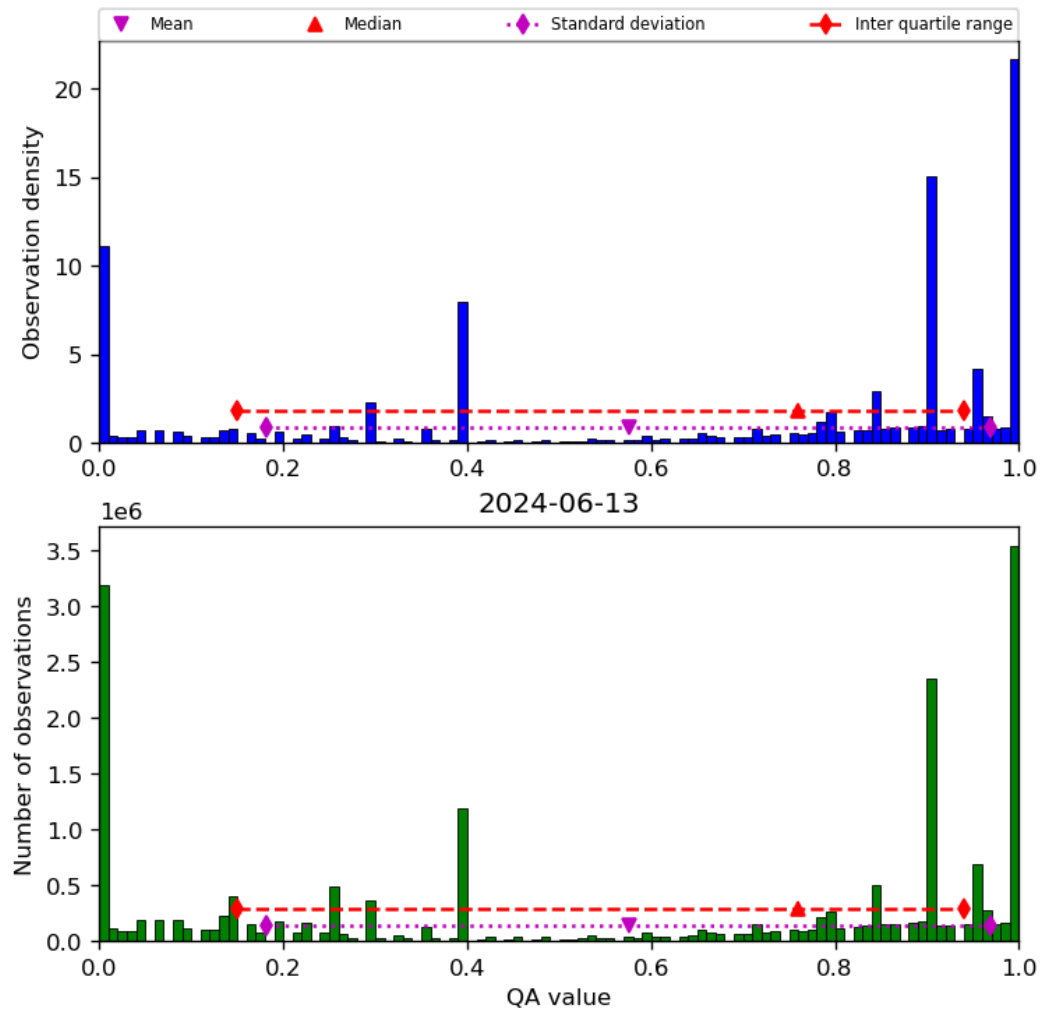
Figure 38: Histogram of “QA value” for 2024-06-13 to 2024-06-14
