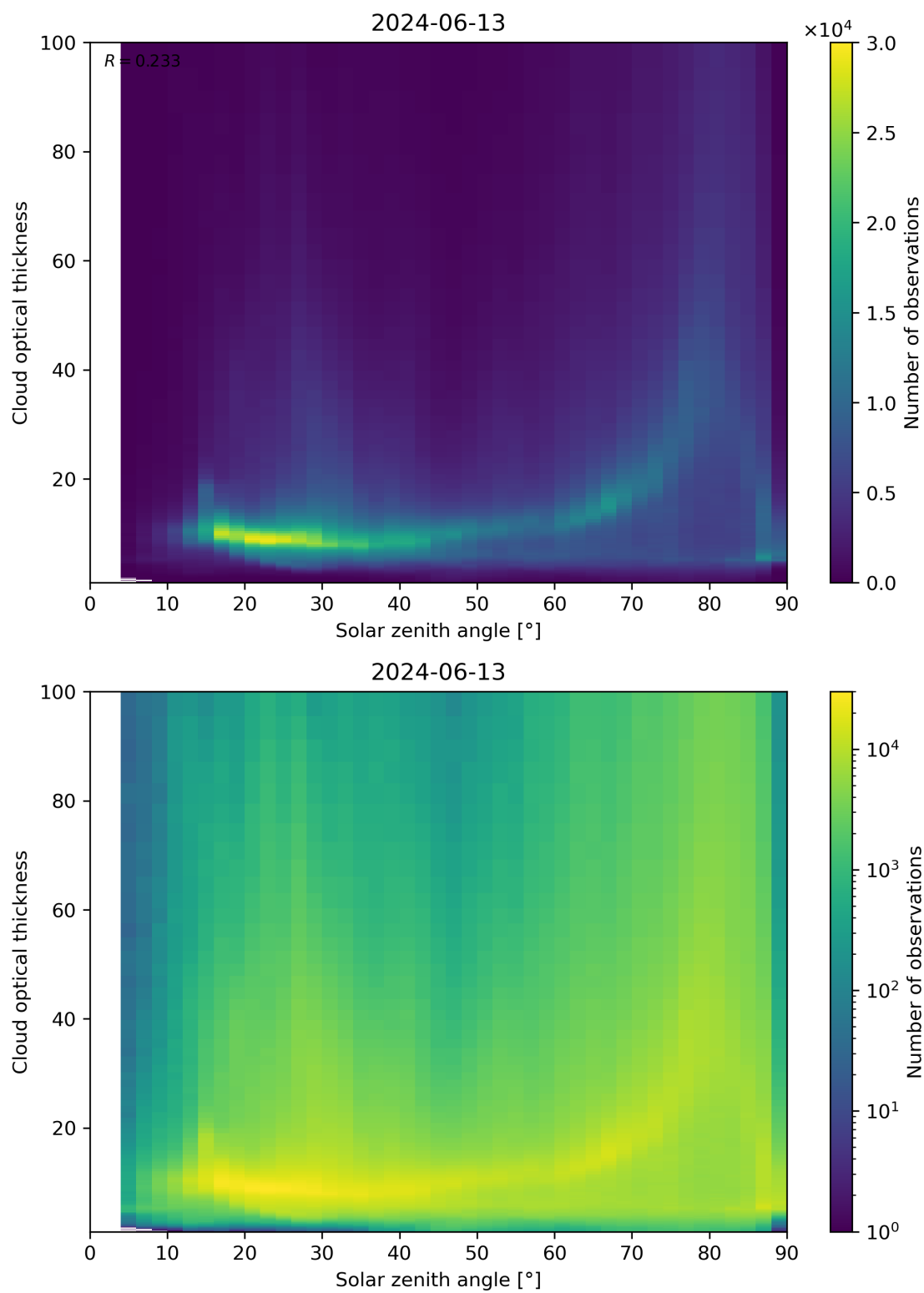
Figure 103: Scatter density plot of “Solar zenith angle” against “Cloud optical thickness” for 2024-06-13 to 2024-06-14.
