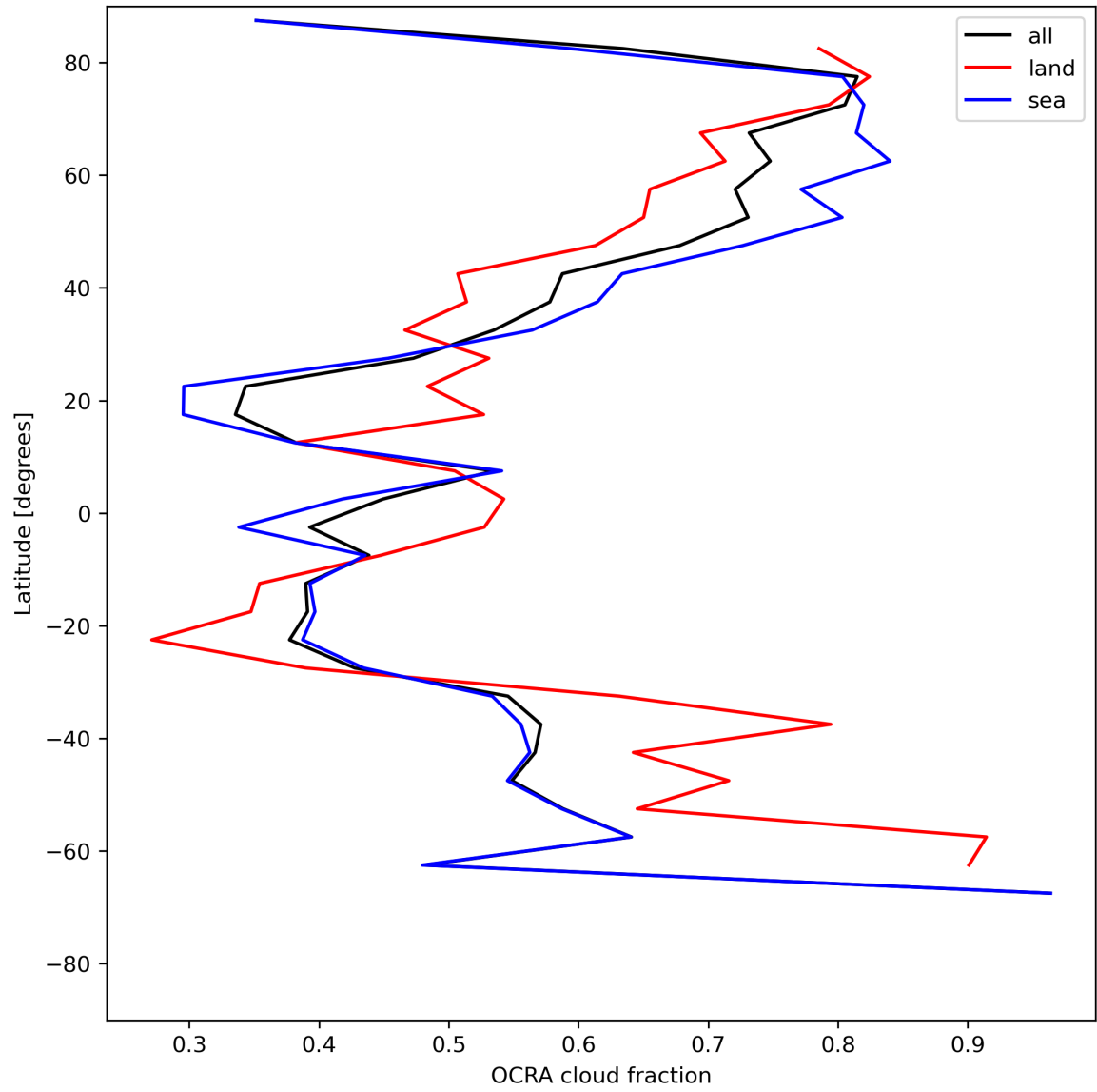
Figure 34: Zonal average of “OCRA cloud fraction” for 2024-06-13 to 2024-06-14.
