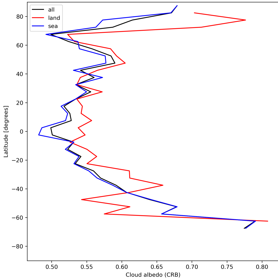
Figure 28: Zonal average of “Cloud albedo (CRB)” for 2024-06-13 to 2024-06-14.
