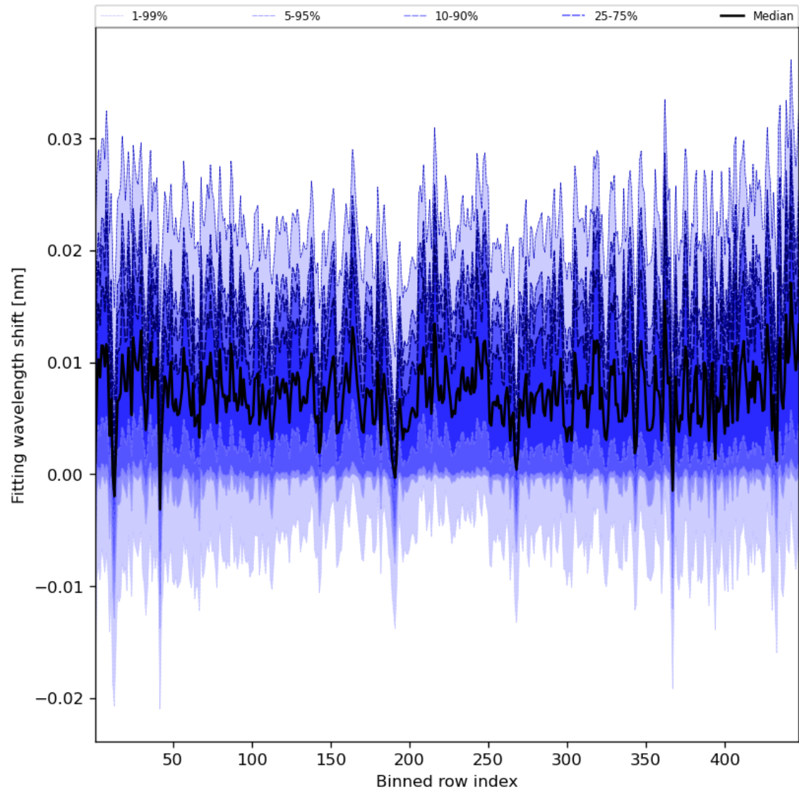
Figure 65: Along track statistics of “Fitting wavelength shift” for 2024-06-13 to 2024-06-14
