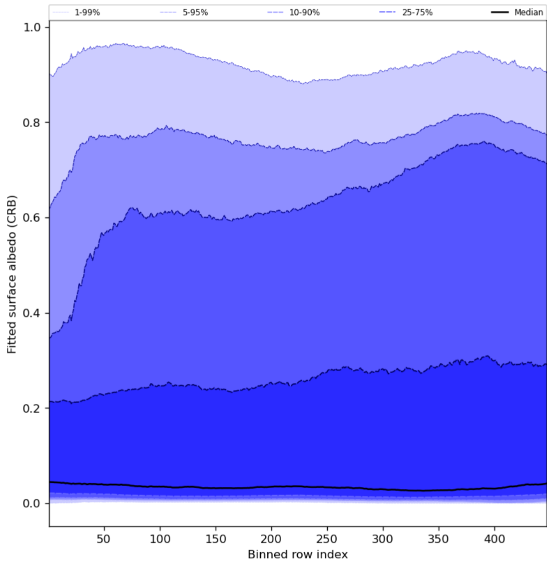
Figure 62: Along track statistics of “Fitted surface albedo (CRB)” for 2024-06-13 to 2024-06-14
