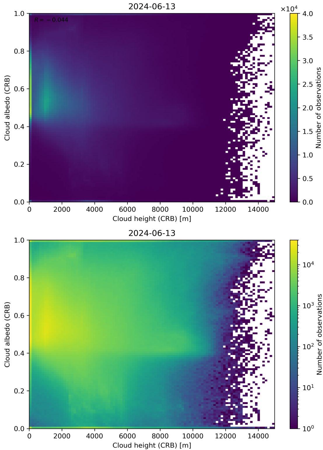
Figure 80: Scatter density plot of “Cloud height (CRB)” against “Cloud albedo (CRB)” for 2024-06-13 to 2024-06-14.
