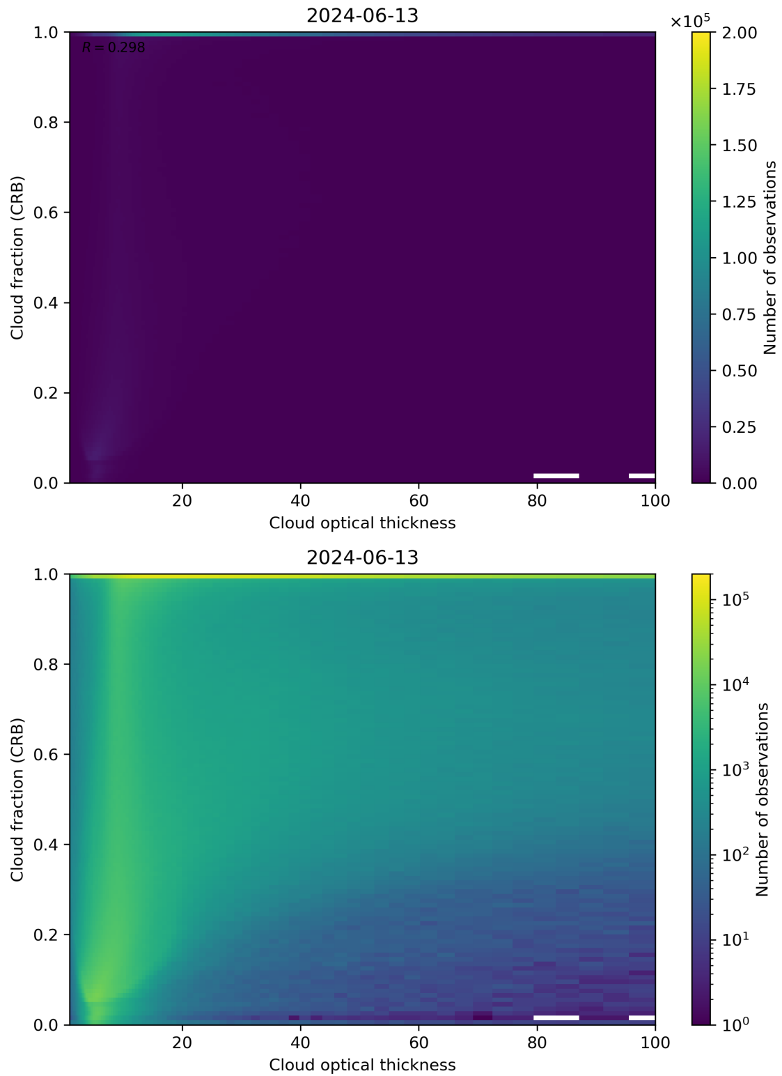
Figure 84: Scatter density plot of “Cloud optical thickness” against “Cloud fraction (CRB)” for 2024-06-13 to 2024-06-14.
