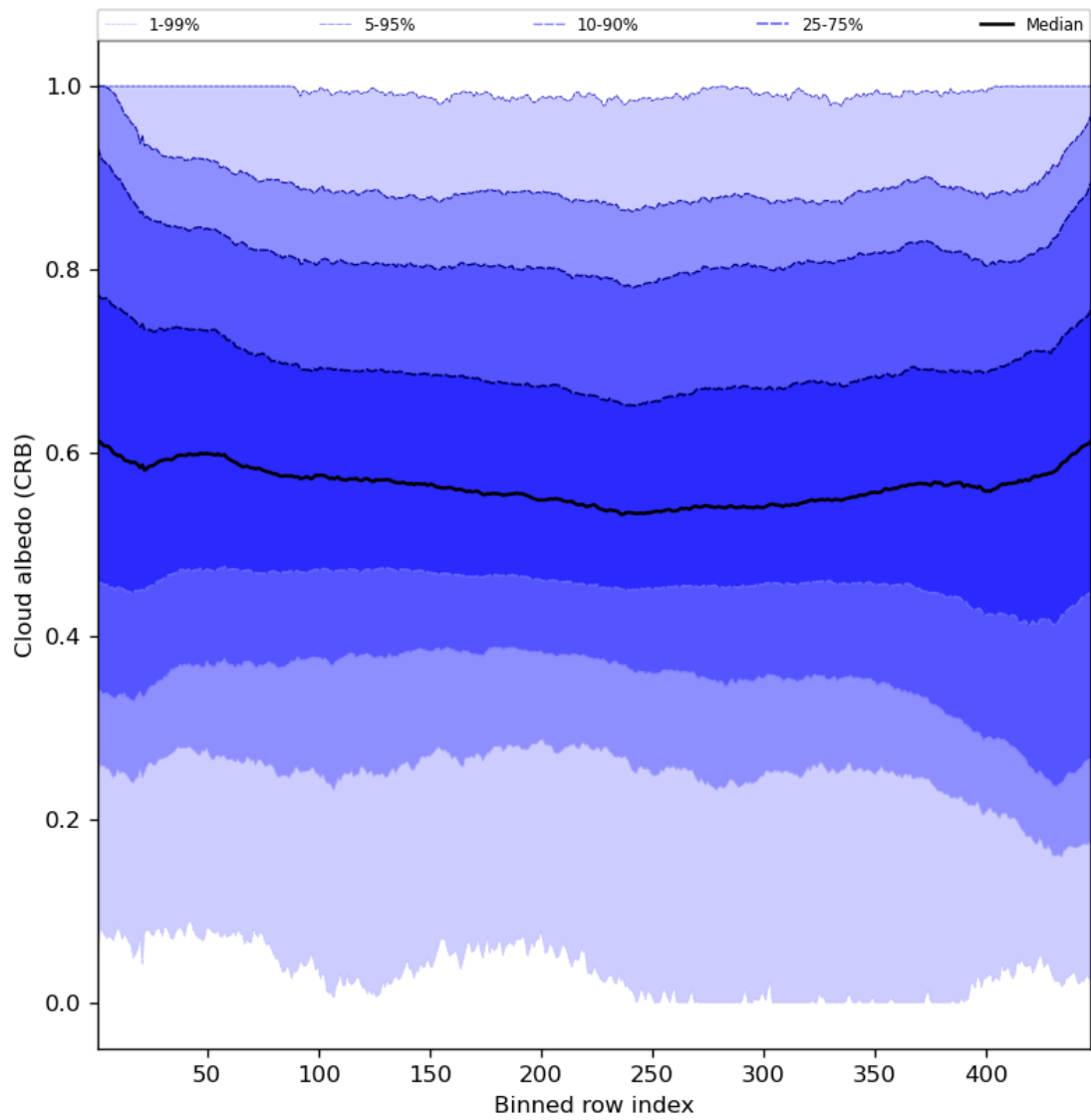
Figure 60: Along track statistics of “Cloud albedo (CRB)” for 2024-06-13 to 2024-06-14
