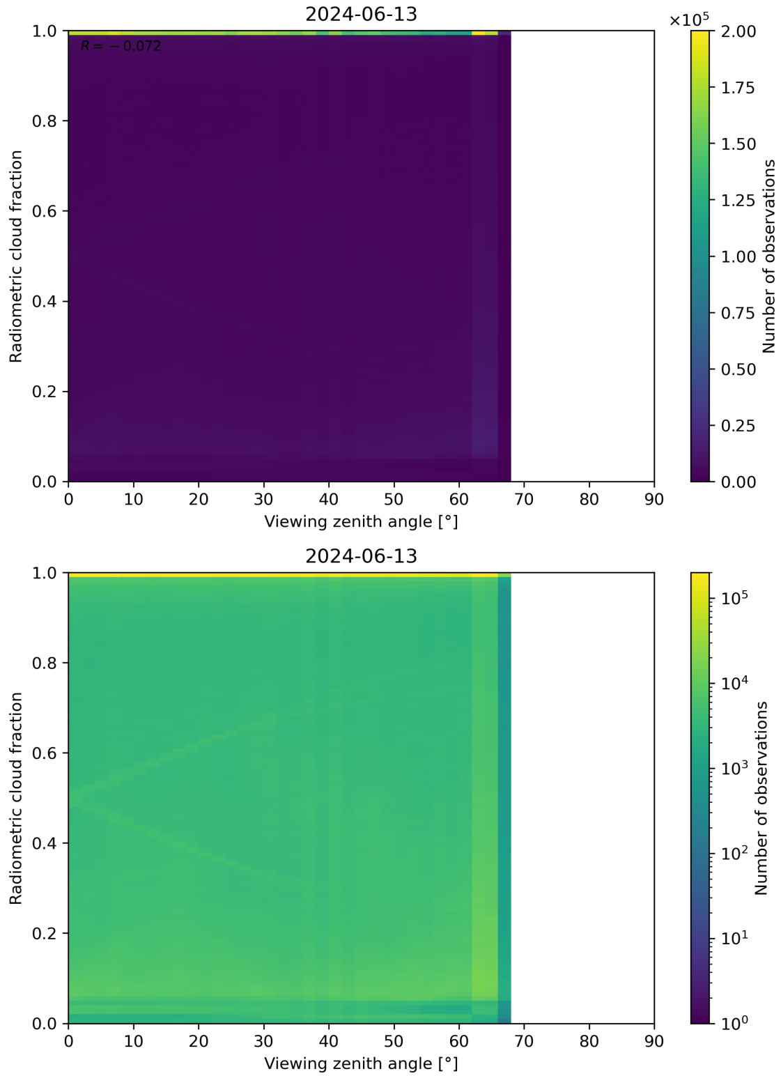
Figure 107: Scatter density plot of “Viewing zenith angle” against “Radiometric cloud fraction” for 2024-06-13 to 2024-06-14.
