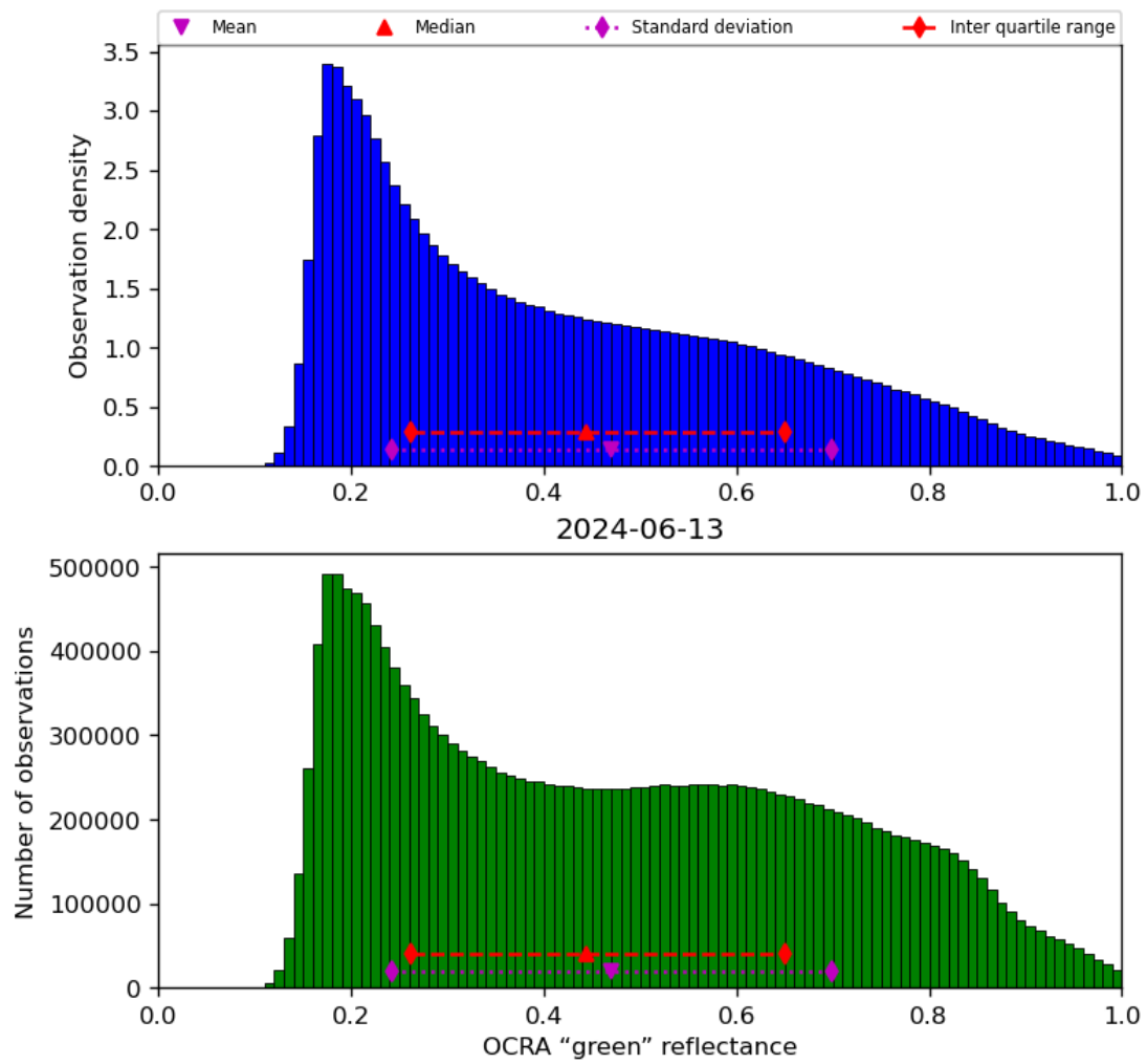
Figure 52: Histogram of “OCRA “green” reflectance” for 2024-06-13 to 2024-06-14
