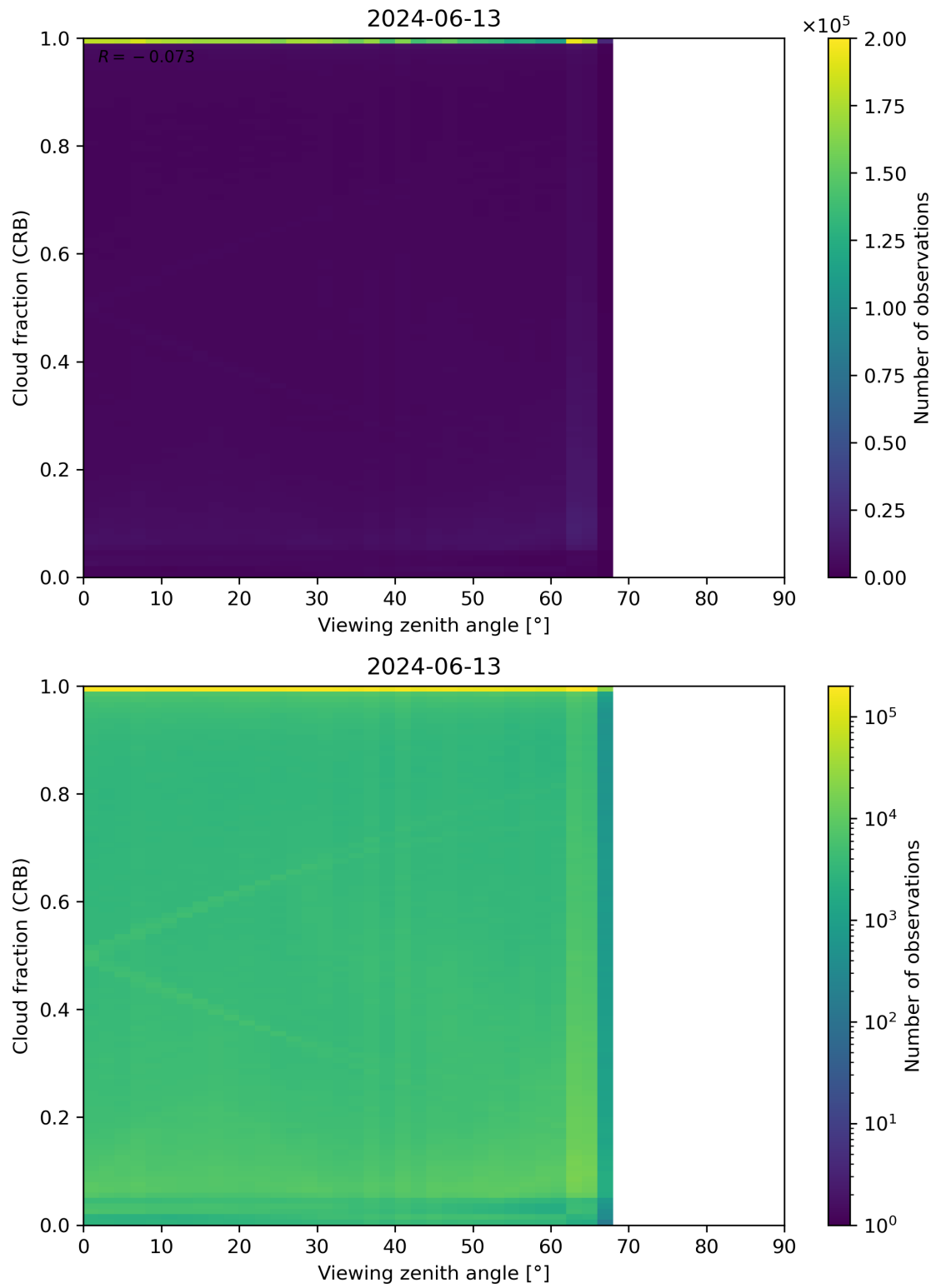
Figure 109: Scatter density plot of “Viewing zenith angle” against “Cloud fraction (CRB)” for 2024-06-13 to 2024-06-14.
