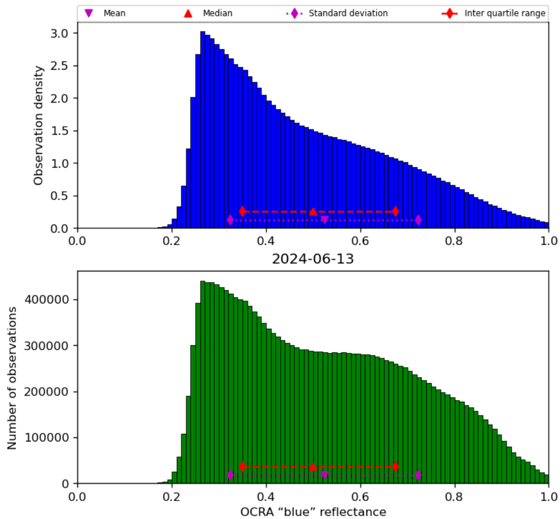
Figure 51: Histogram of “OCRA “blue” reflectance” for 2024-06-13 to 2024-06-14
