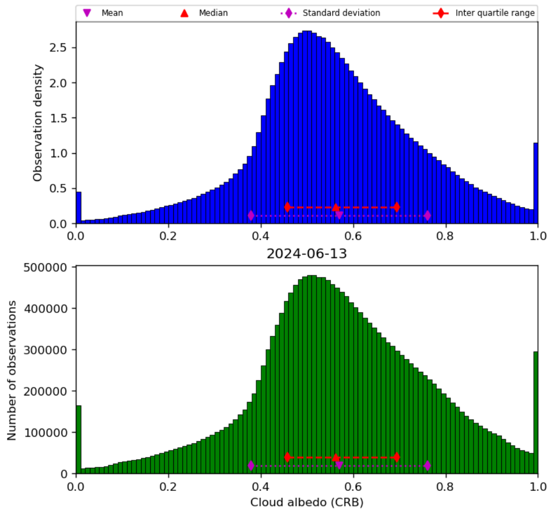
Figure 44: Histogram of “Cloud albedo (CRB)” for 2024-06-13 to 2024-06-14
