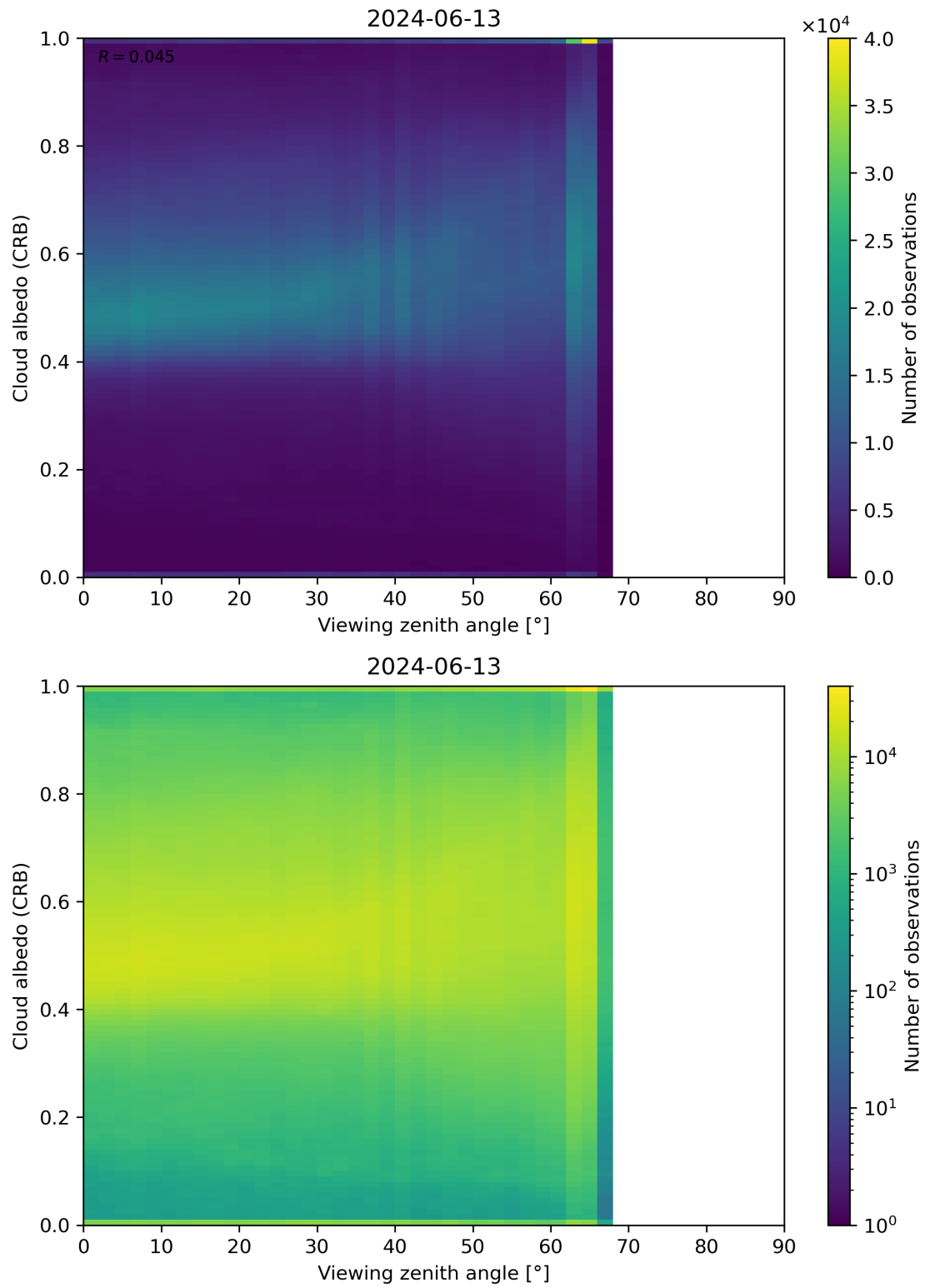
Figure 106: Scatter density plot of “Viewing zenith angle” against “Cloud albedo (CRB)” for 2024-06-13 to 2024-06-14.
