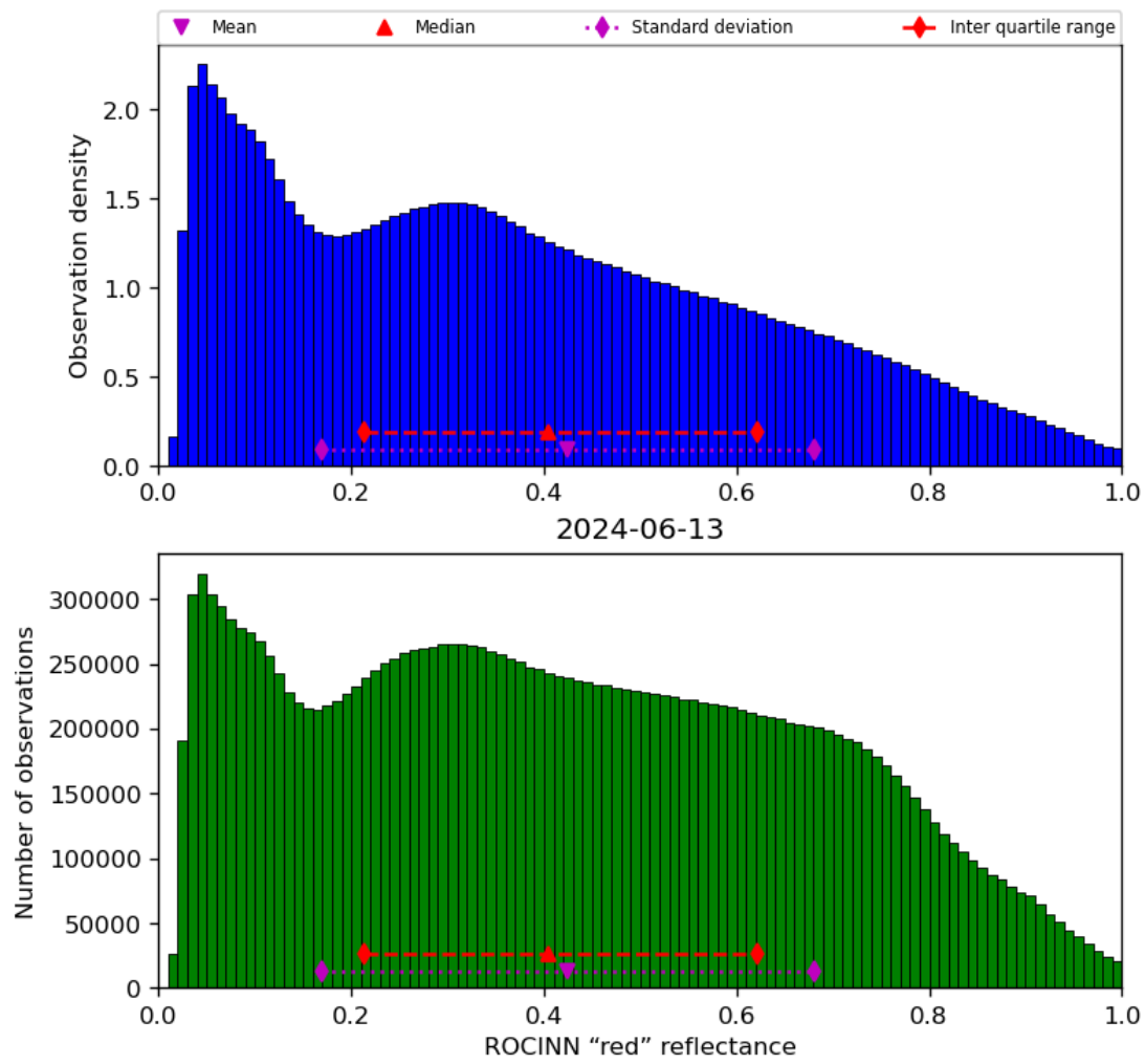
Figure 53: Histogram of “ROCINN “red” reflectance” for 2024-06-13 to 2024-06-14
