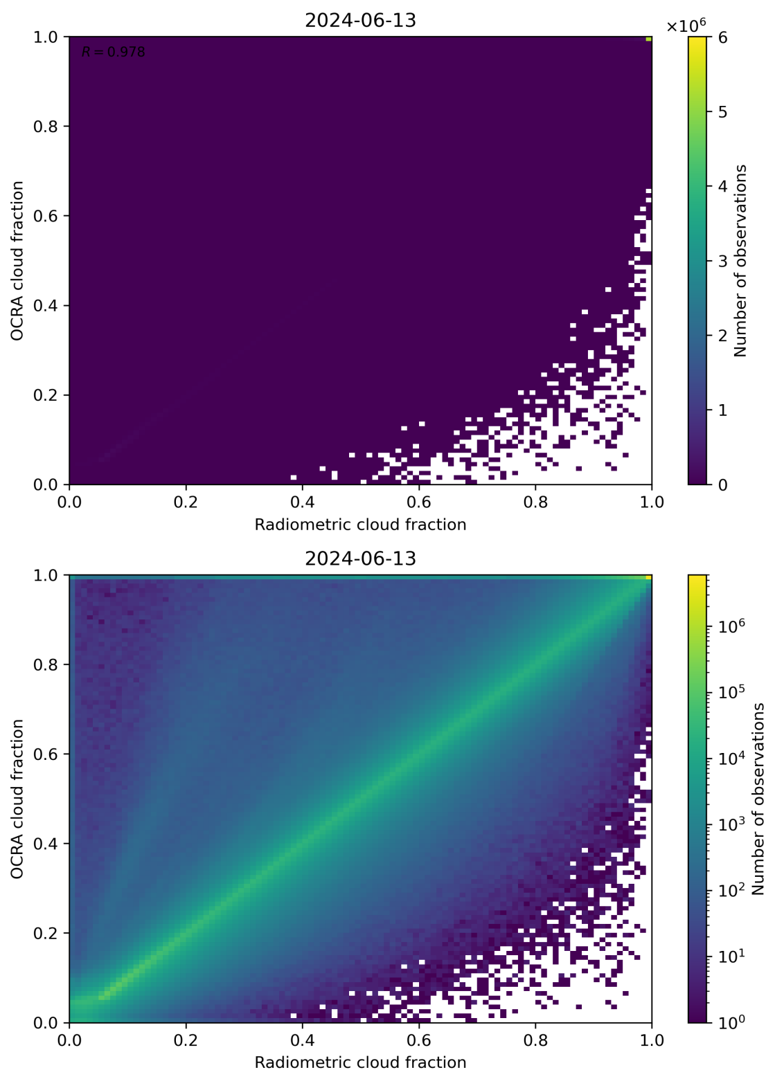
Figure 72: Scatter density plot of “Radiometric cloud fraction” against “OCRA cloud fraction” for 2024-06-13 to 2024-06-14.
