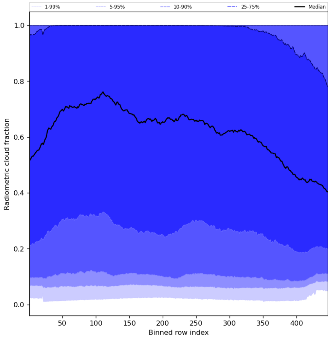
Figure 55: Along track statistics of “Radiometric cloud fraction” for 2024-06-13 to 2024-06-14
