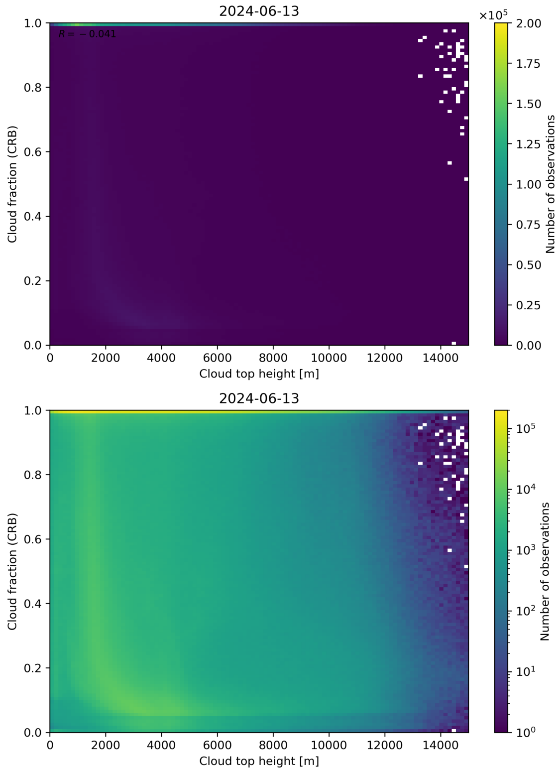
Figure 88: Scatter density plot of “Cloud top height” against “Cloud fraction (CRB)” for 2024-06-13 to 2024-06-14.
