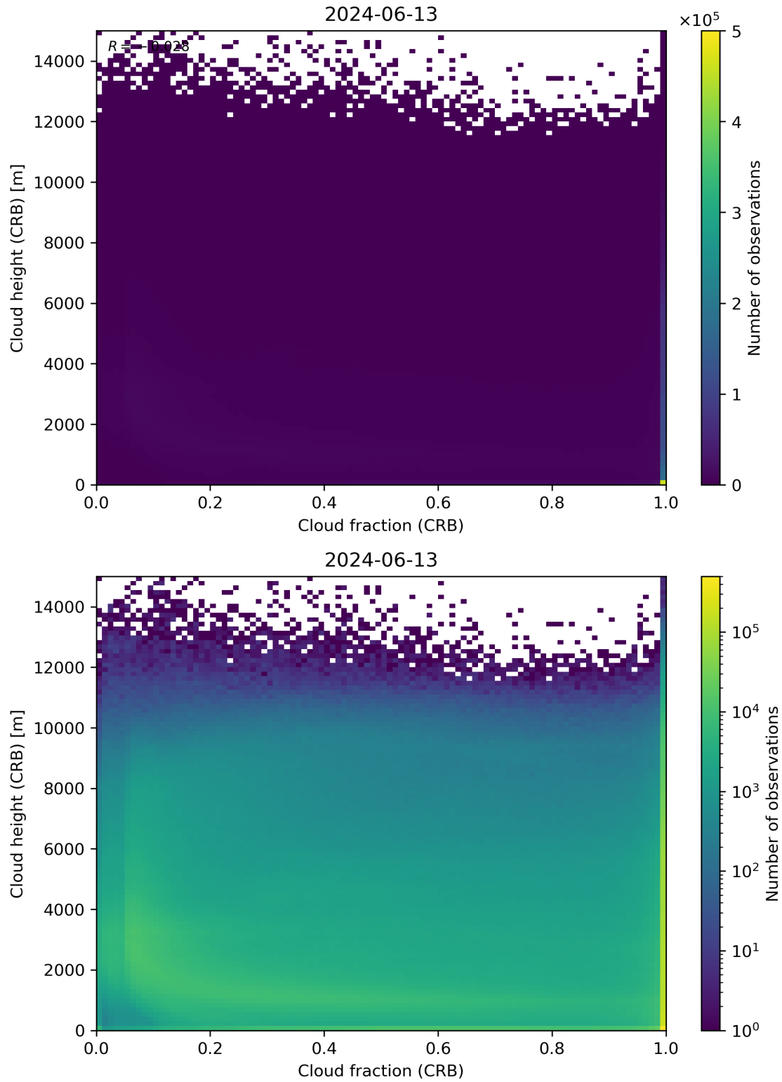
Figure 79: Scatter density plot of “Cloud fraction (CRB)” against “Cloud height (CRB)” for 2024-06-13 to 2024-06-14.
