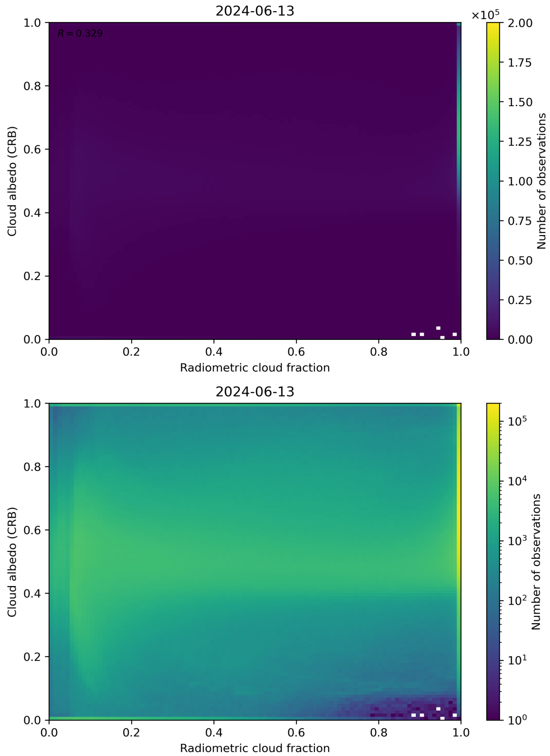
Figure 71: Scatter density plot of “Radiometric cloud fraction” against “Cloud albedo (CRB)” for 2024-06-13 to 2024-06-14.
