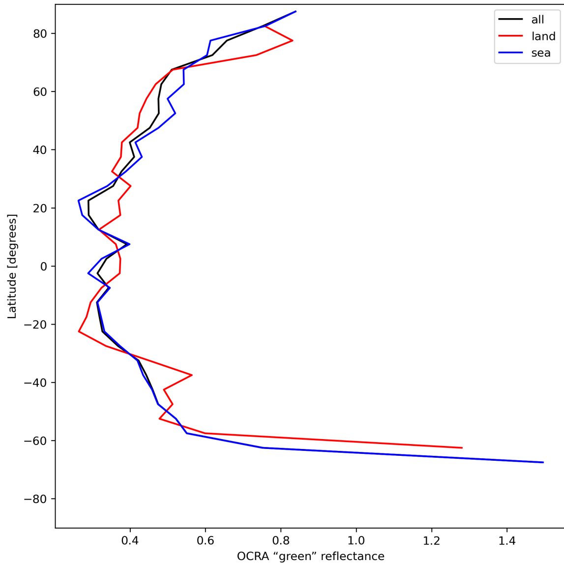
Figure 36: Zonal average of “OCRA “green” reflectance” for 2024-06-13 to 2024-06-14.
