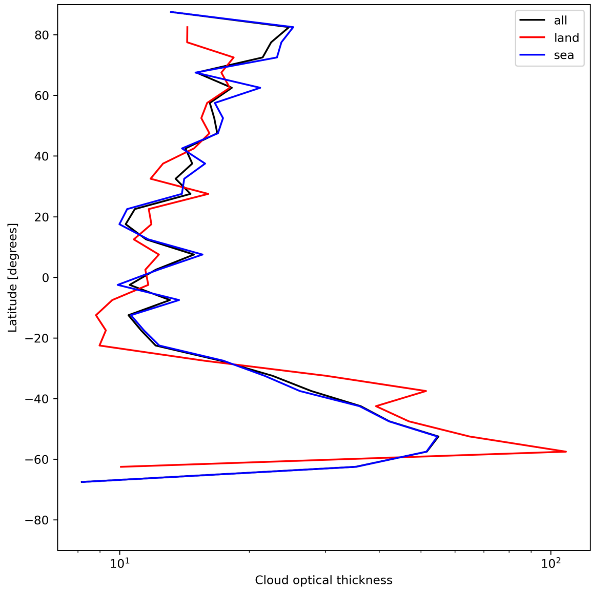
Figure 25: Zonal average of “Cloud optical thickness” for 2024-06-13 to 2024-06-14.
