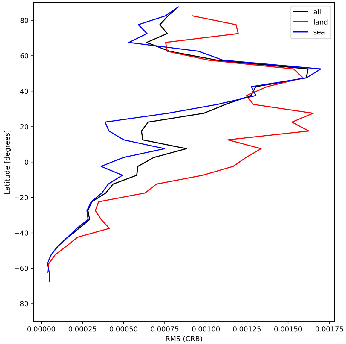
Figure 32: Zonal average of “RMS (CRB)” for 2024-06-13 to 2024-06-14.
