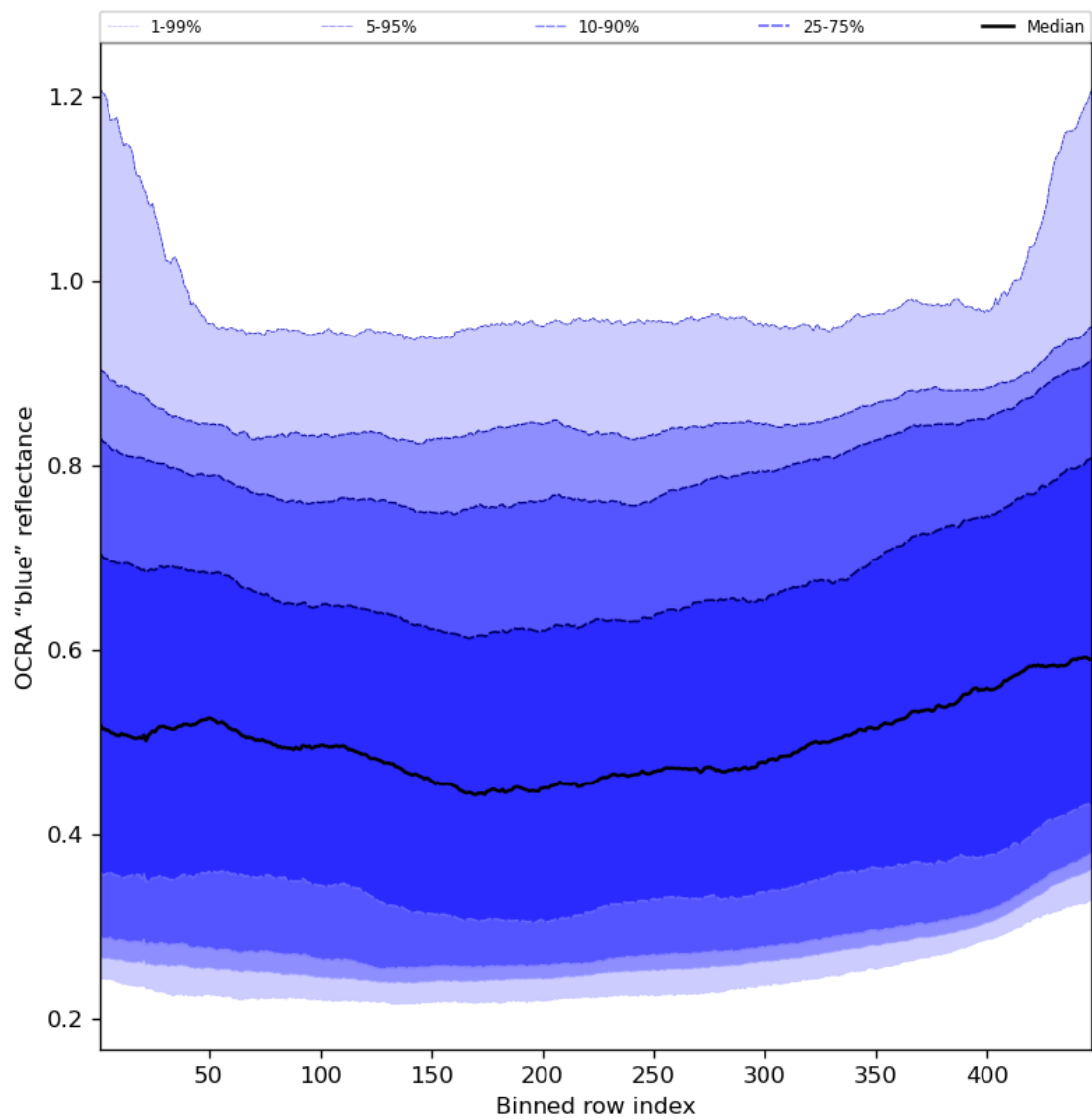
Figure 67: Along track statistics of “OCRA “blue” reflectance” for 2024-06-13 to 2024-06-14
