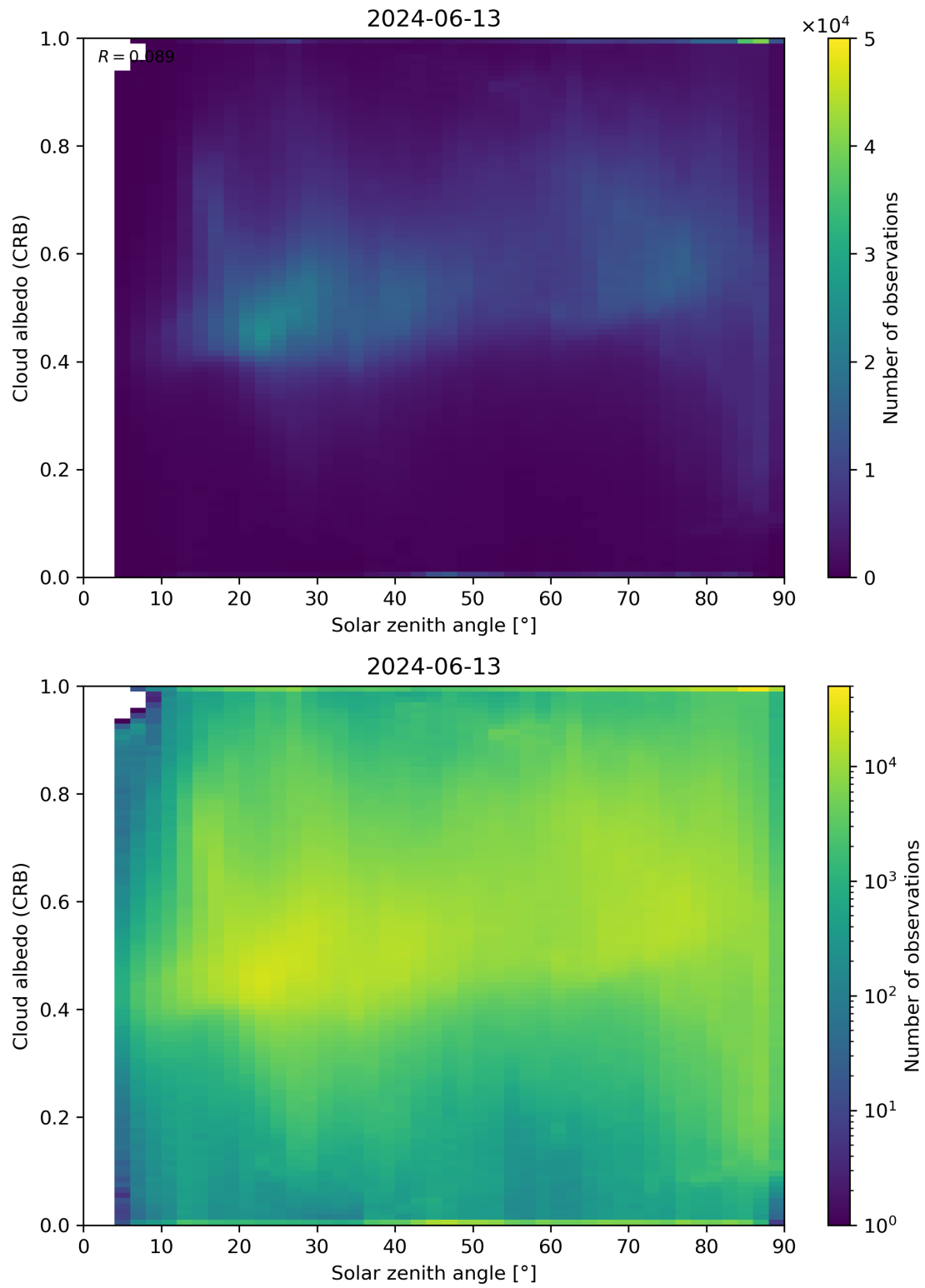
Figure 98: Scatter density plot of “Solar zenith angle” against “Cloud albedo (CRB)” for 2024-06-13 to 2024-06-14.
