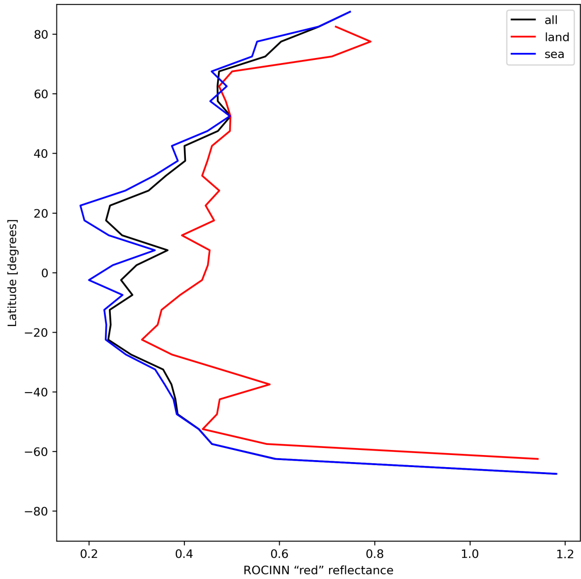
Figure 37: Zonal average of “ROCINN “red” reflectance” for 2024-06-13 to 2024-06-14.
