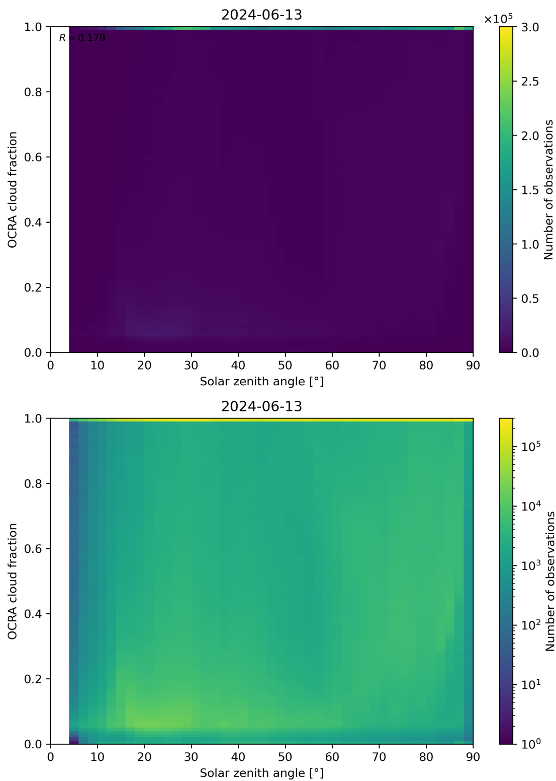
Figure 100: Scatter density plot of “Solar zenith angle” against “OCRA cloud fraction” for 2024-06-13 to 2024-06-14.
