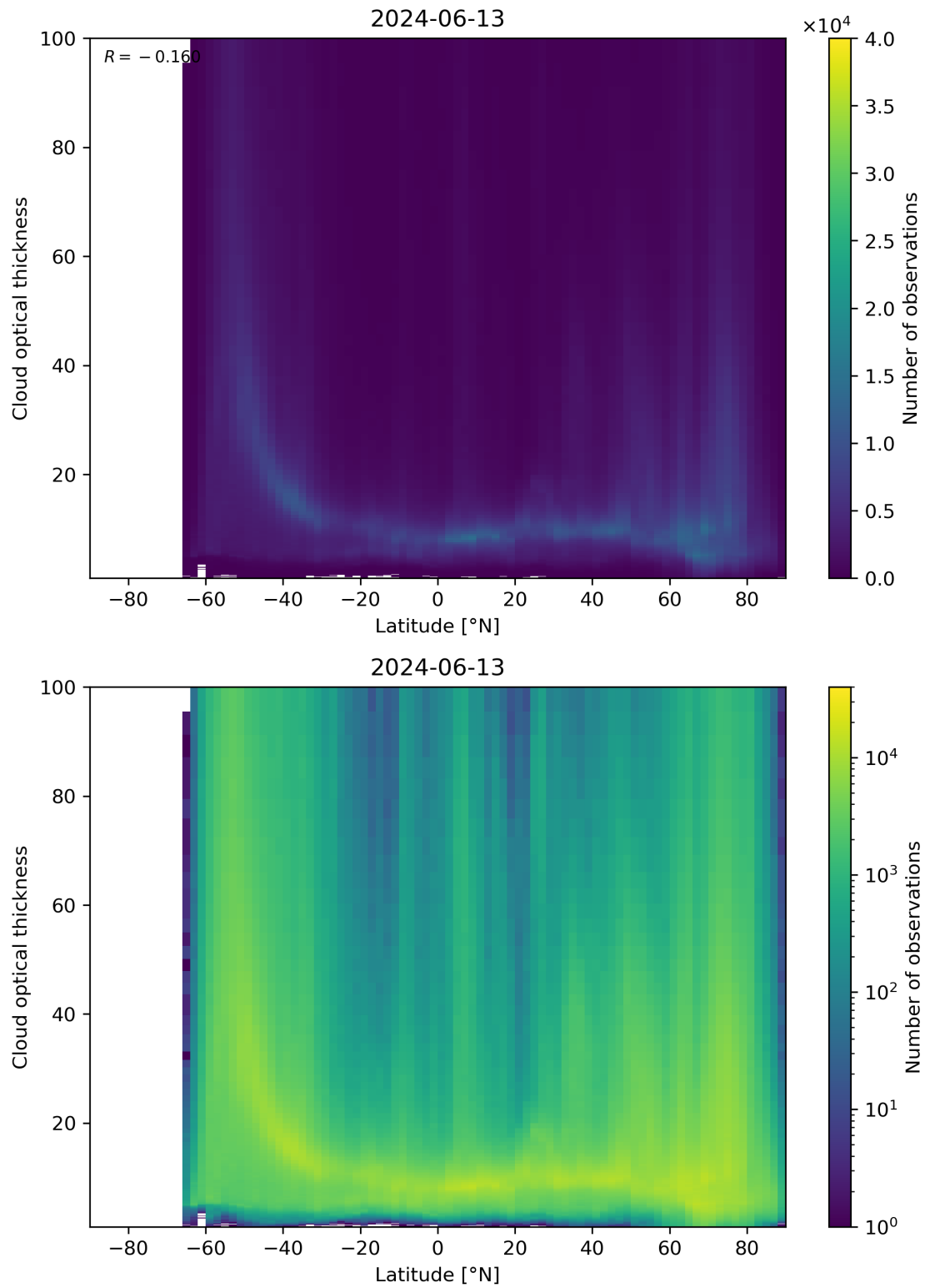
Figure 96: Scatter density plot of “Latitude” against “Cloud optical thickness” for 2024-06-13 to 2024-06-14.
