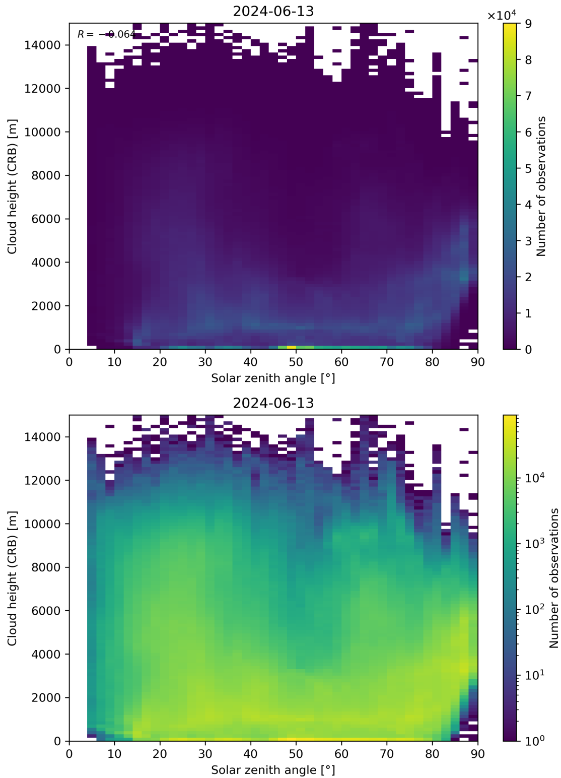
Figure 102: Scatter density plot of “Solar zenith angle” against “Cloud height (CRB)” for 2024-06-13 to 2024-06-14.
