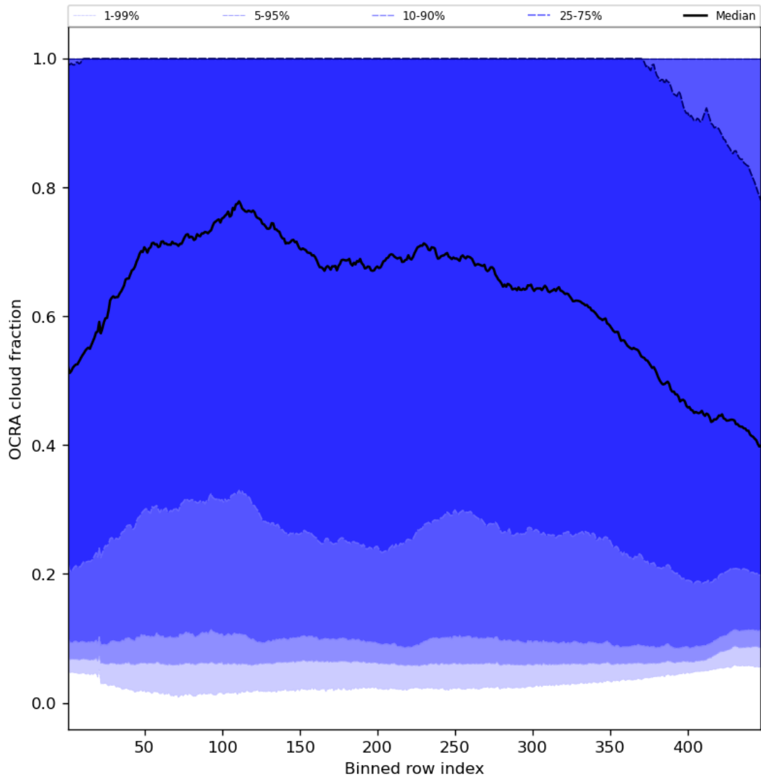
Figure 66: Along track statistics of “OCRA cloud fraction” for 2024-06-13 to 2024-06-14
