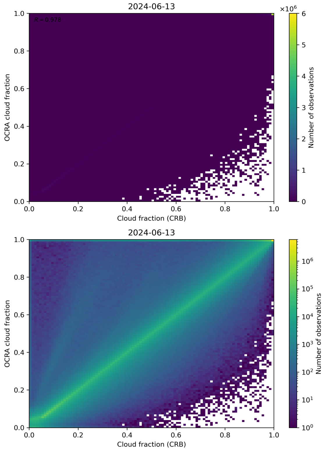
Figure 78: Scatter density plot of “Cloud fraction (CRB)” against “OCRA cloud fraction” for 2024-06-13 to 2024-06-14.
