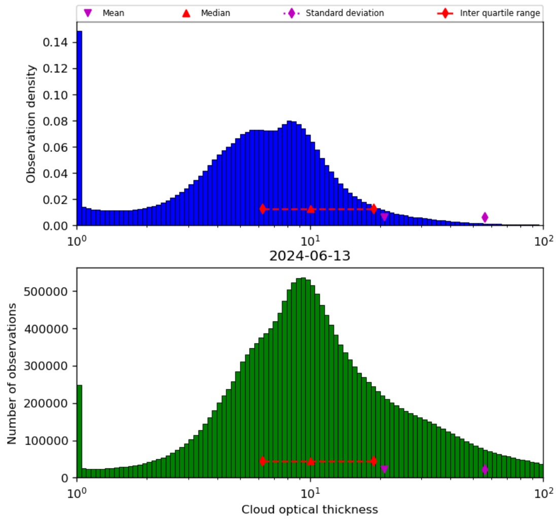
Figure 41: Histogram of “Cloud optical thickness” for 2024-06-13 to 2024-06-14
