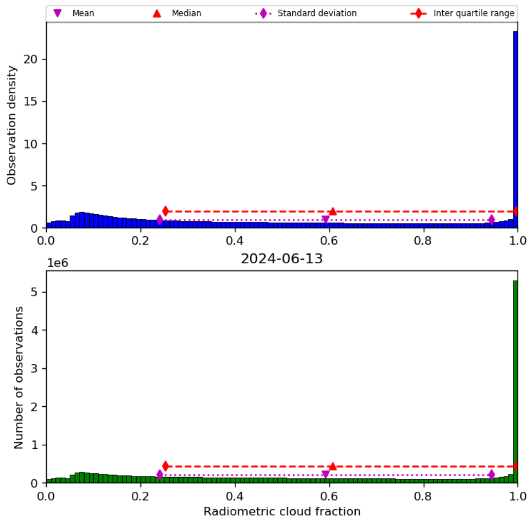
Figure 39: Histogram of “Radiometric cloud fraction” for 2024-06-13 to 2024-06-14
