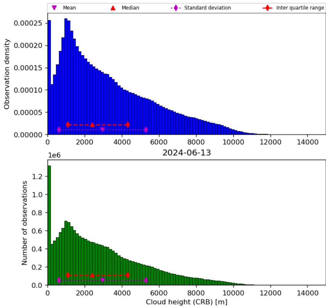
Figure 43: Histogram of “Cloud height (CRB)” for 2024-06-13 to 2024-06-14
