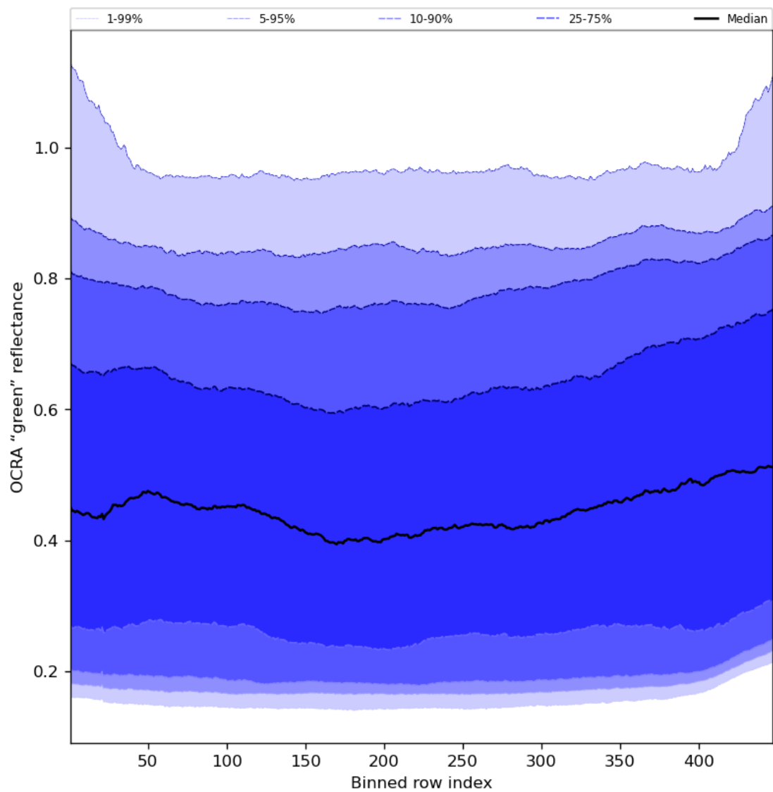
Figure 68: Along track statistics of “OCRA “green” reflectance” for 2024-06-13 to 2024-06-14
