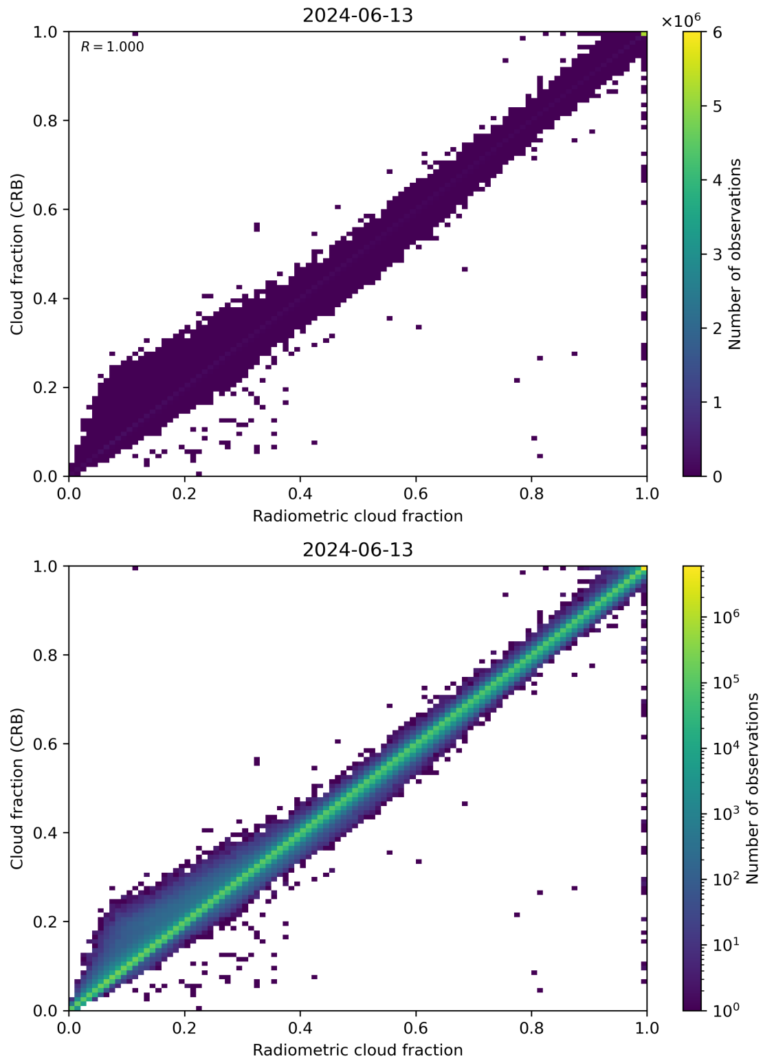
Figure 73: Scatter density plot of “Radiometric cloud fraction” against “Cloud fraction (CRB)” for 2024-06-13 to 2024-06-14.
