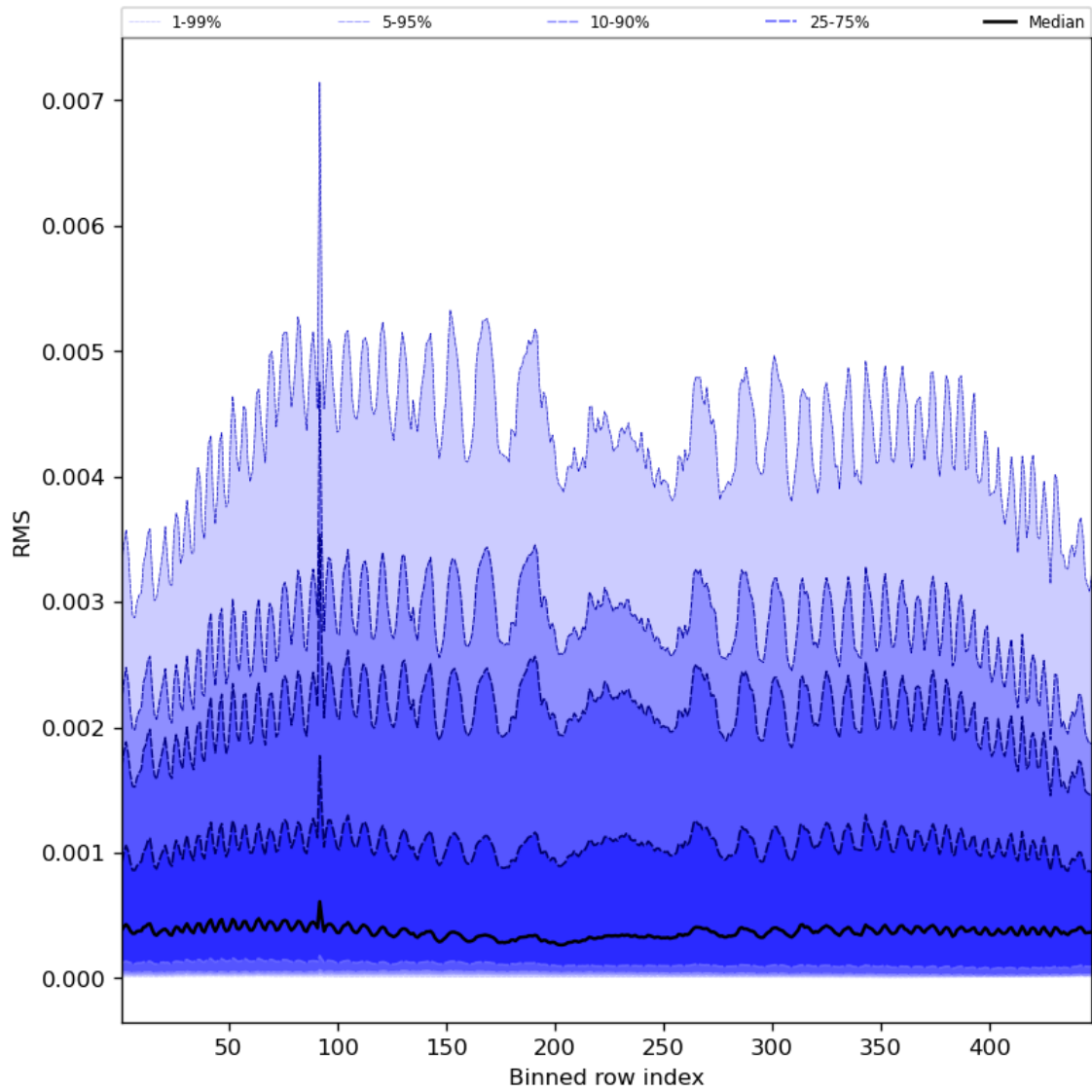
Figure 63: Along track statistics of “RMS” for 2024-06-13 to 2024-06-14
