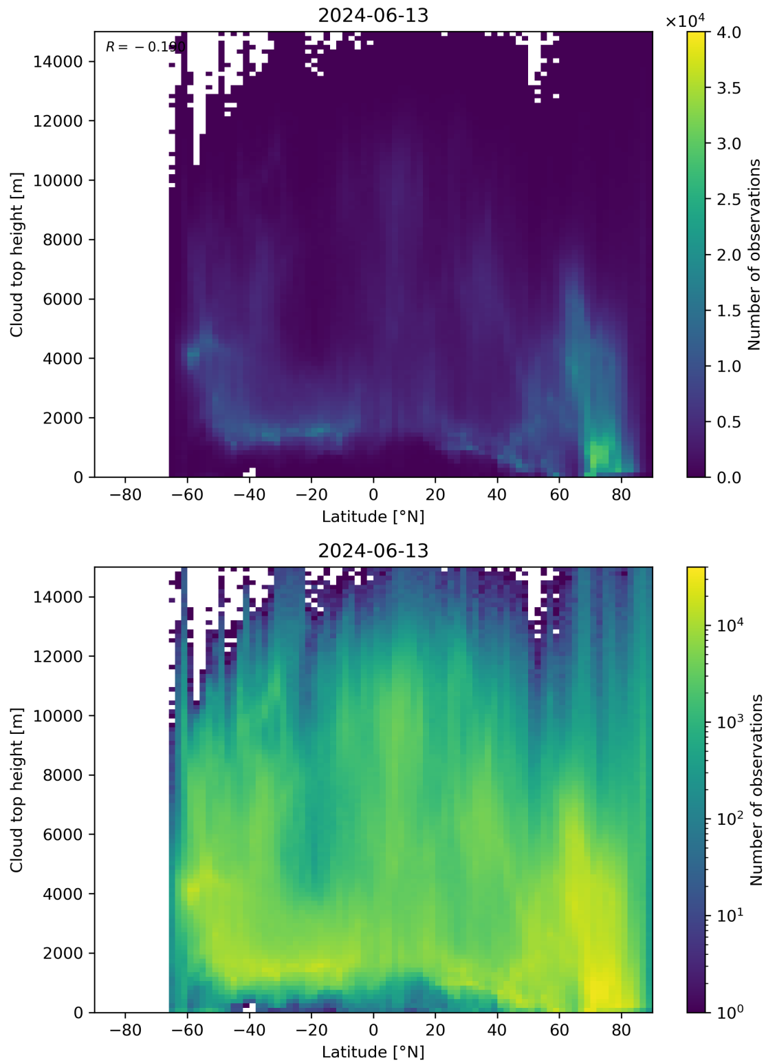
Figure 97: Scatter density plot of “Latitude” against “Cloud top height” for 2024-06-13 to 2024-06-14.
