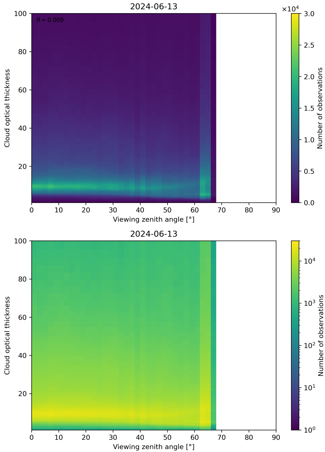
Figure 111: Scatter density plot of “Viewing zenith angle” against “Cloud optical thickness” for 2024-06-13 to 2024-06-14.
