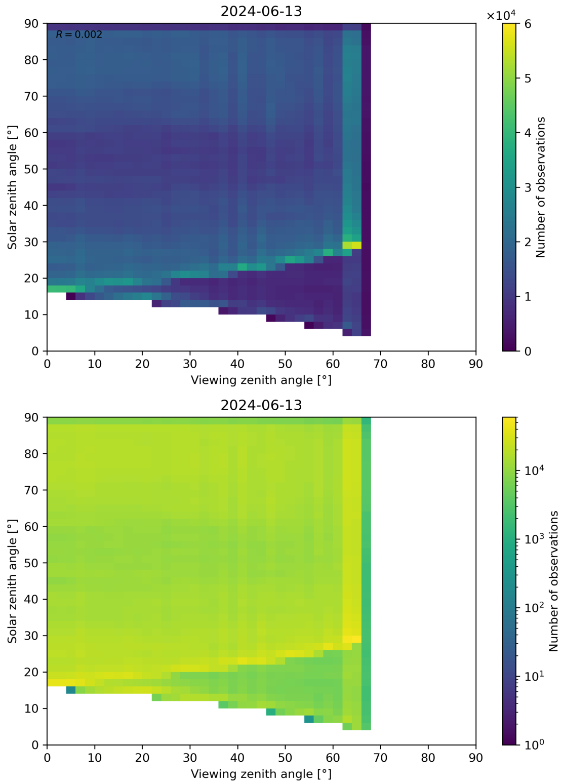
Figure 114: Scatter density plot of “Viewing zenith angle” against “Solar zenith angle” for 2024-06-13 to 2024-06-14.
