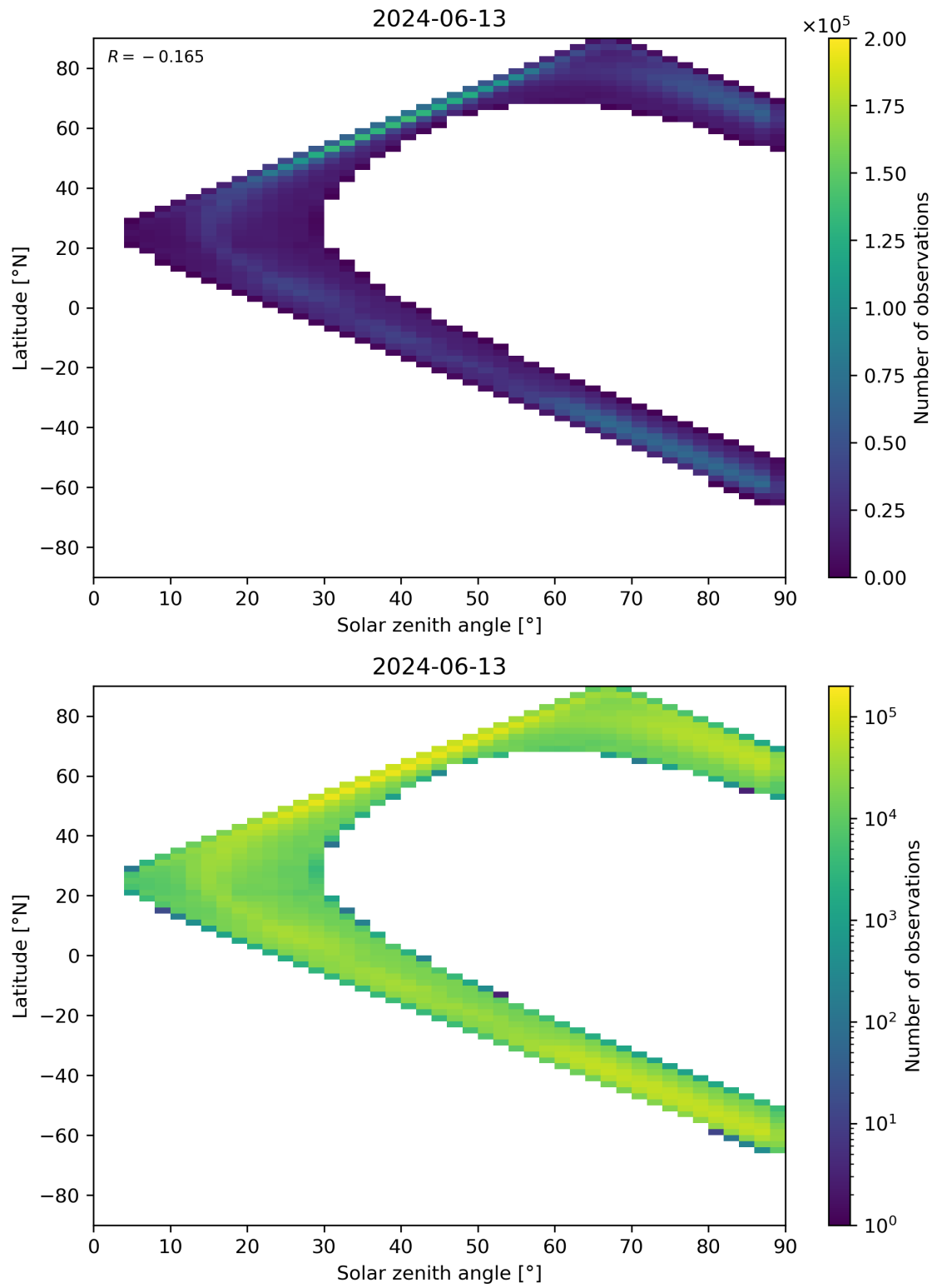
Figure 105: Scatter density plot of “Solar zenith angle” against “Latitude” for 2024-06-13 to 2024-06-14.
