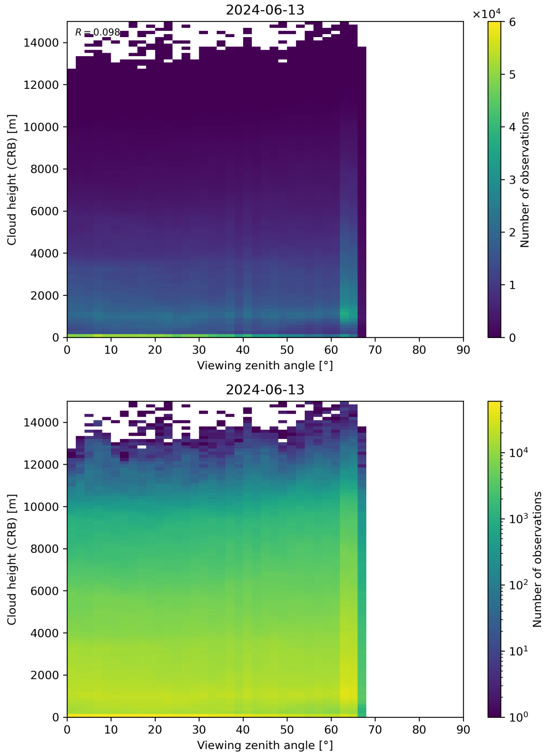
Figure 110: Scatter density plot of “Viewing zenith angle” against “Cloud height (CRB)” for 2024-06-13 to 2024-06-14.
