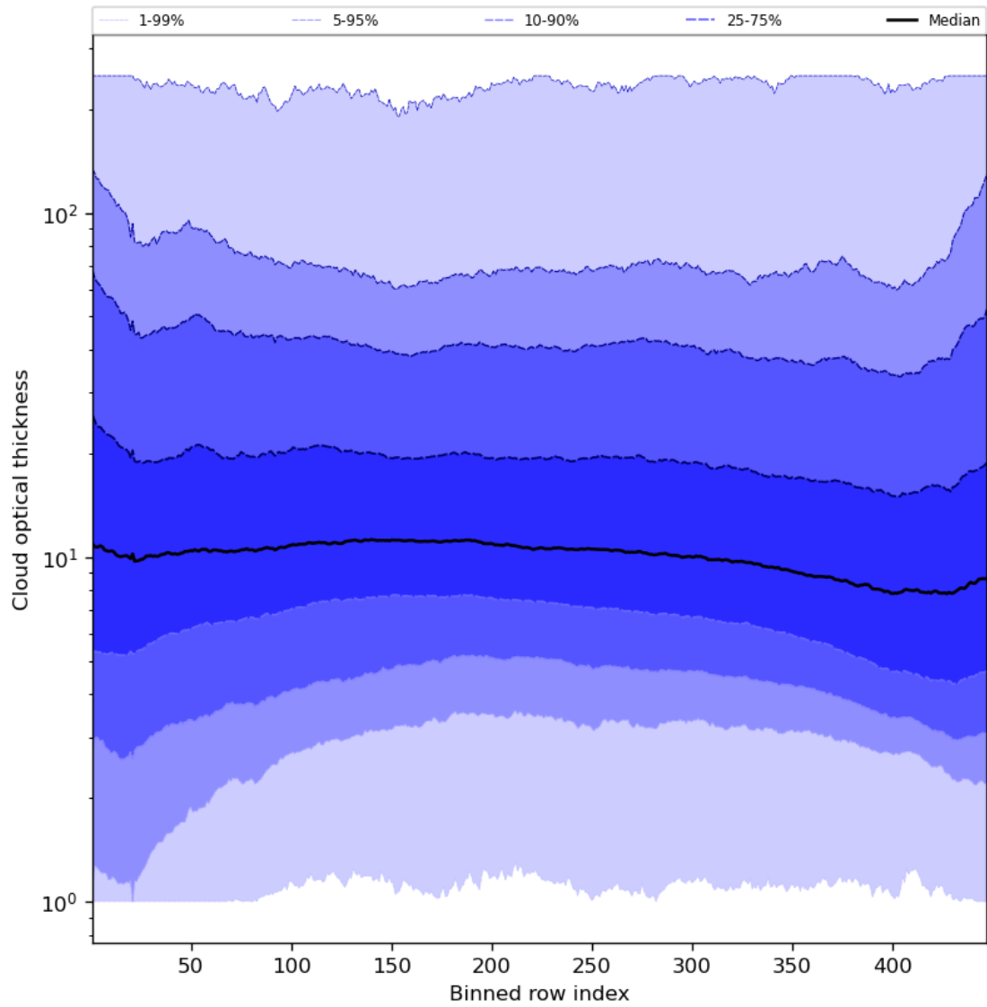
Figure 57: Along track statistics of “Cloud optical thickness” for 2024-06-13 to 2024-06-14
