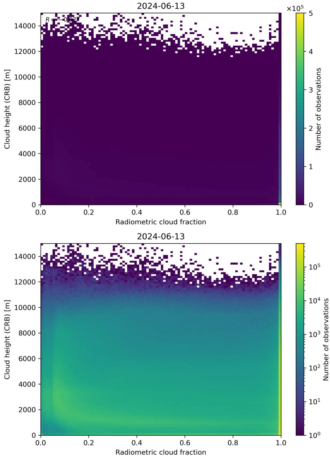
Figure 74: Scatter density plot of “Radiometric cloud fraction” against “Cloud height (CRB)” for 2024-06-13 to 2024-06-14.
