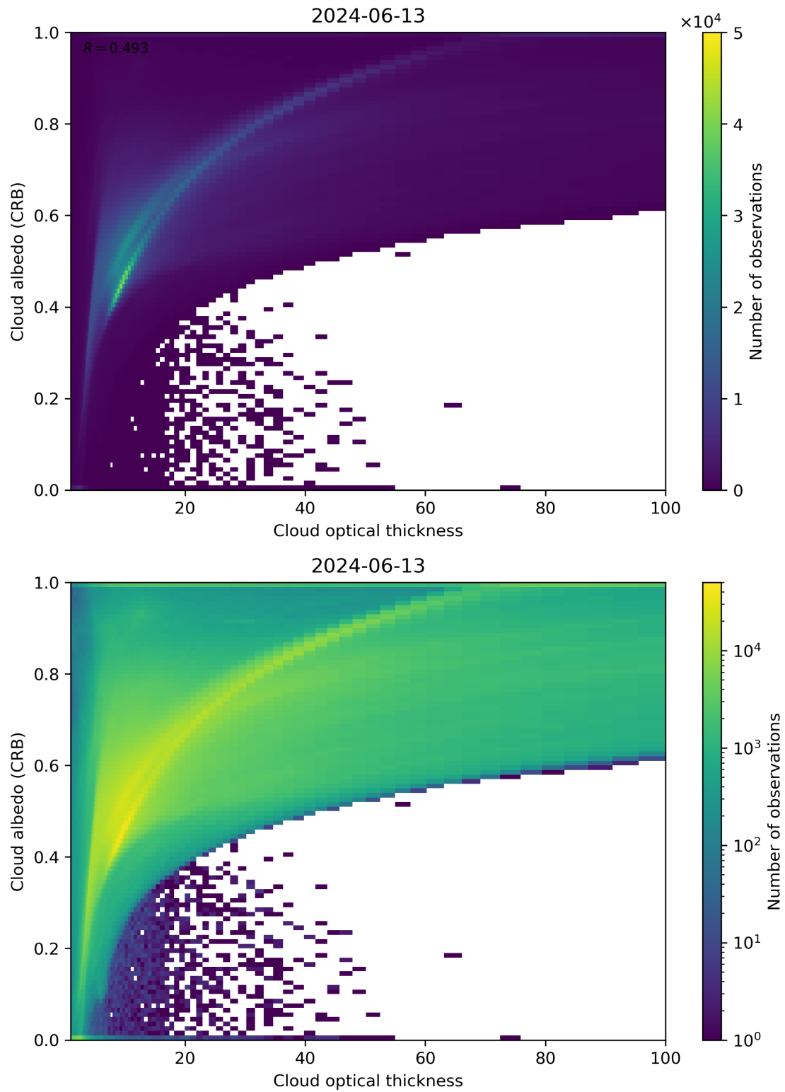
Figure 82: Scatter density plot of “Cloud optical thickness” against “Cloud albedo (CRB)” for 2024-06-13 to 2024-06-14.
