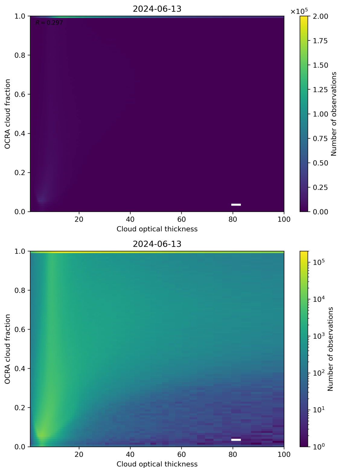
Figure 83: Scatter density plot of “Cloud optical thickness” against “OCRA cloud fraction” for 2024-06-13 to 2024-06-14.
