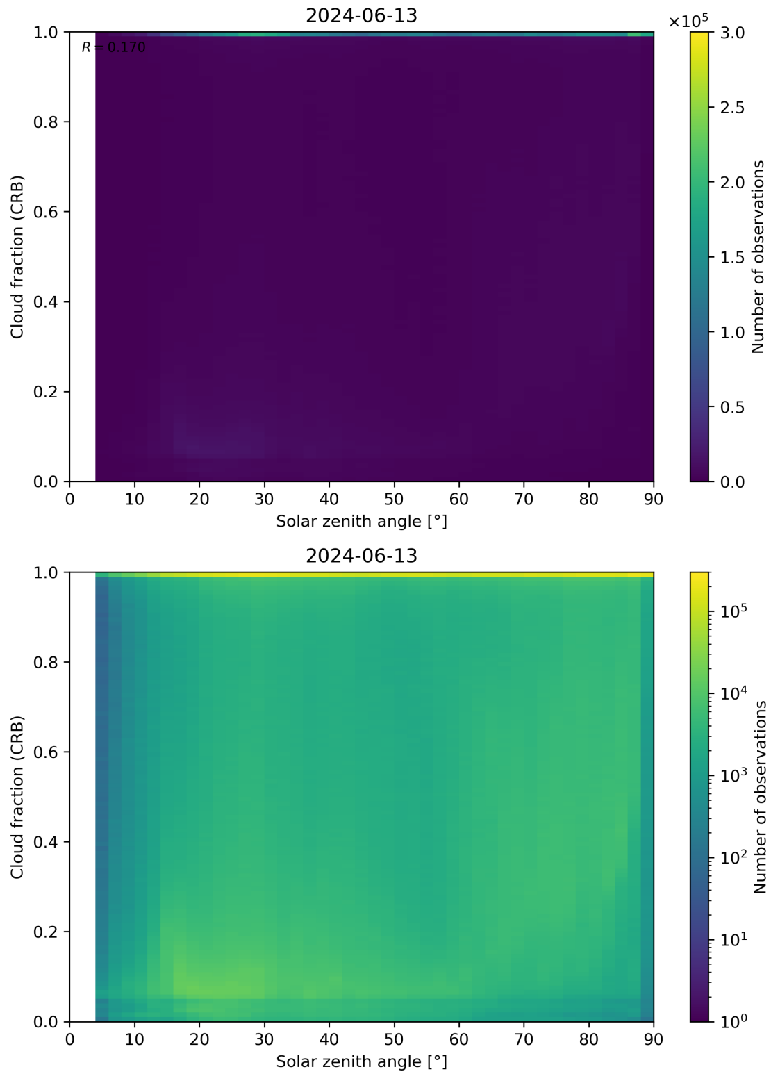
Figure 101: Scatter density plot of “Solar zenith angle” against “Cloud fraction (CRB)” for 2024-06-13 to 2024-06-14.
