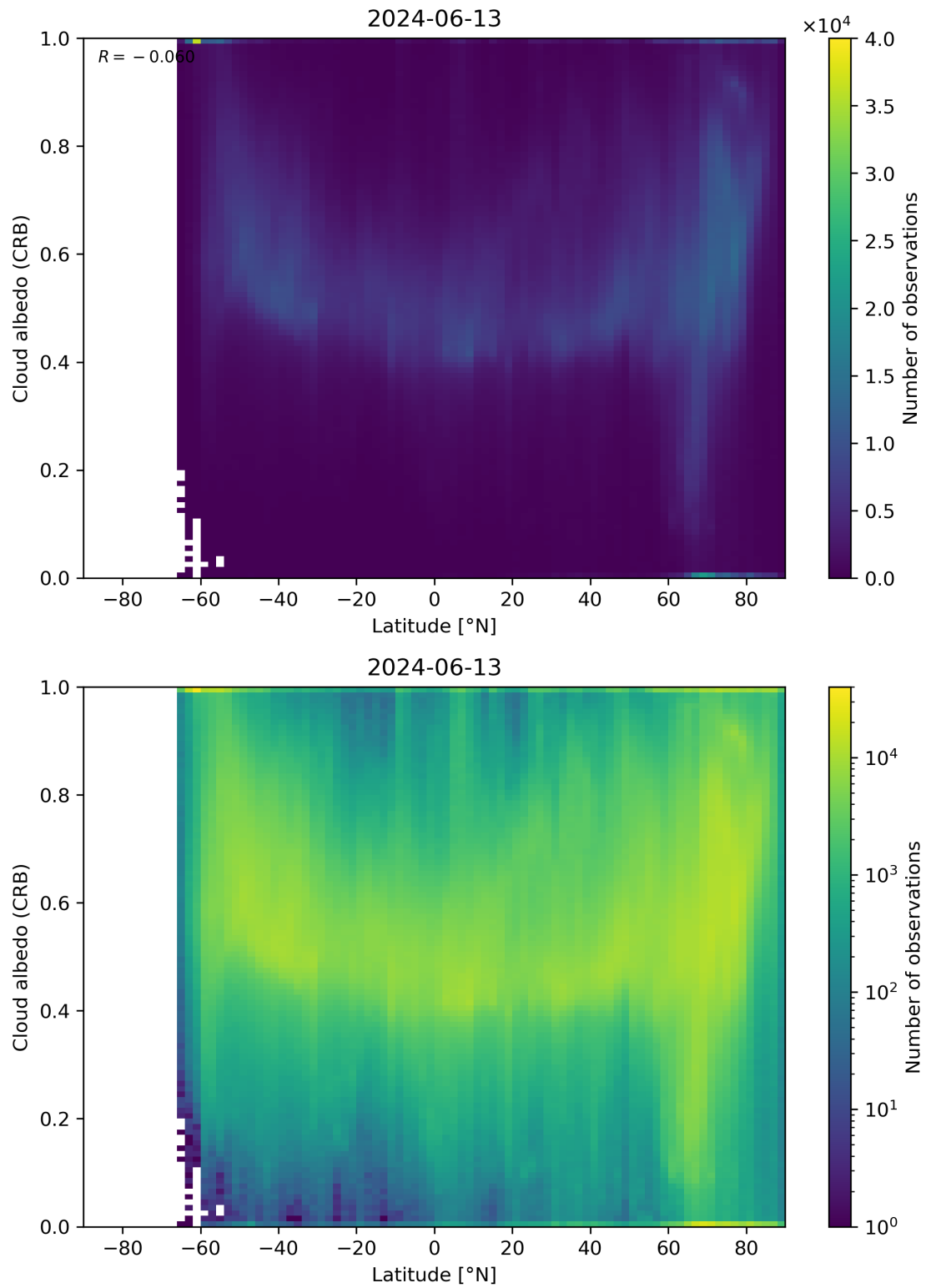
Figure 91: Scatter density plot of “Latitude” against “Cloud albedo (CRB)” for 2024-06-13 to 2024-06-14.
