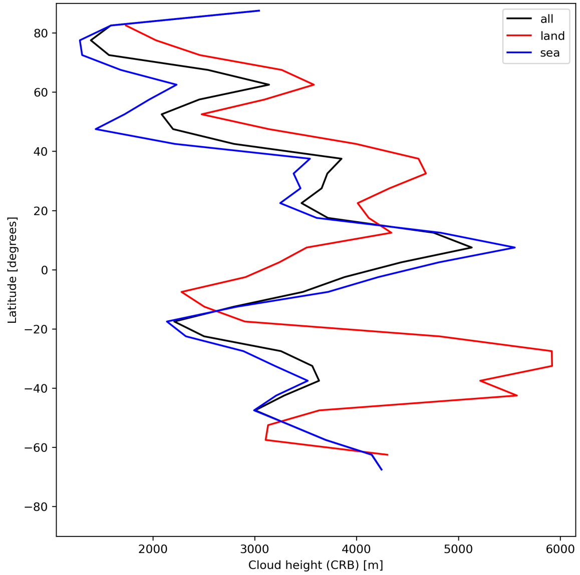
Figure 27: Zonal average of “Cloud height (CRB)” for 2024-06-13 to 2024-06-14.
