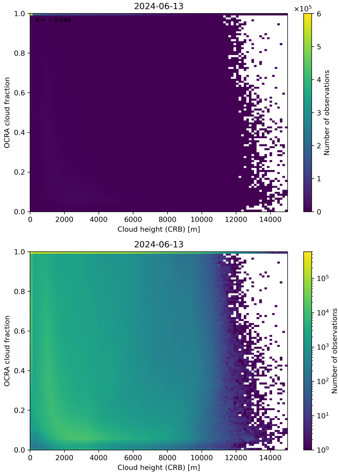
Figure 81: Scatter density plot of “Cloud height (CRB)” against “OCRA cloud fraction” for 2024-06-13 to 2024-06-14.
