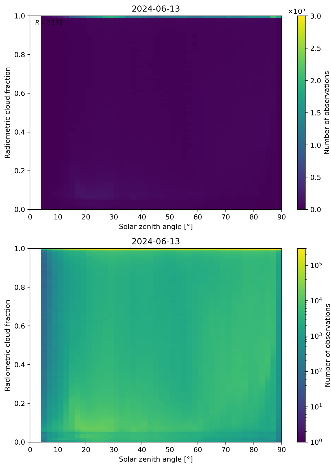
Figure 99: Scatter density plot of “Solar zenith angle” against “Radiometric cloud fraction” for 2024-06-13 to 2024-06-14.
