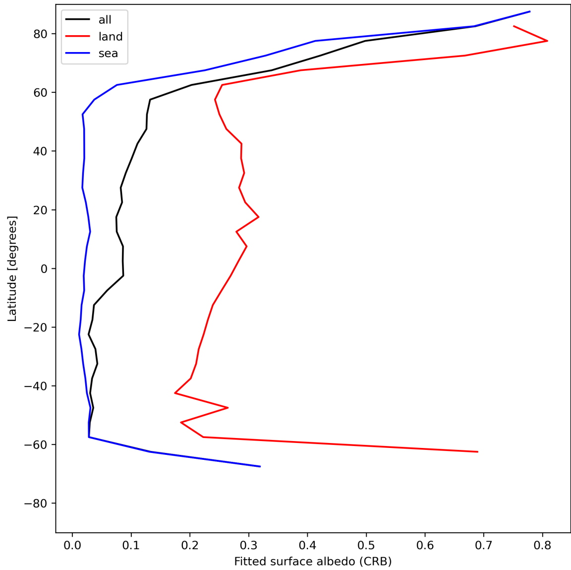
Figure 30: Zonal average of “Fitted surface albedo (CRB)” for 2024-06-13 to 2024-06-14.
