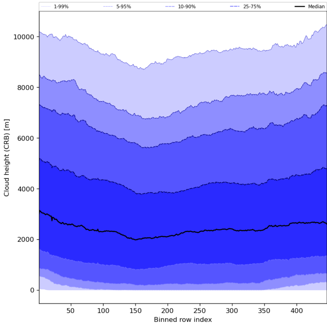
Figure 59: Along track statistics of “Cloud height (CRB)” for 2024-06-13 to 2024-06-14
