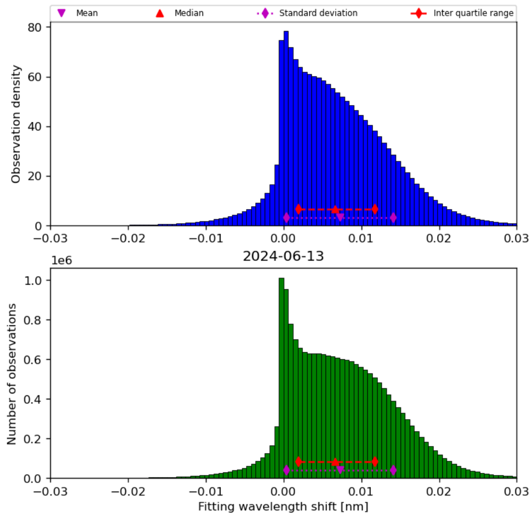
Figure 49: Histogram of “Fitting wavelength shift” for 2024-06-13 to 2024-06-14
