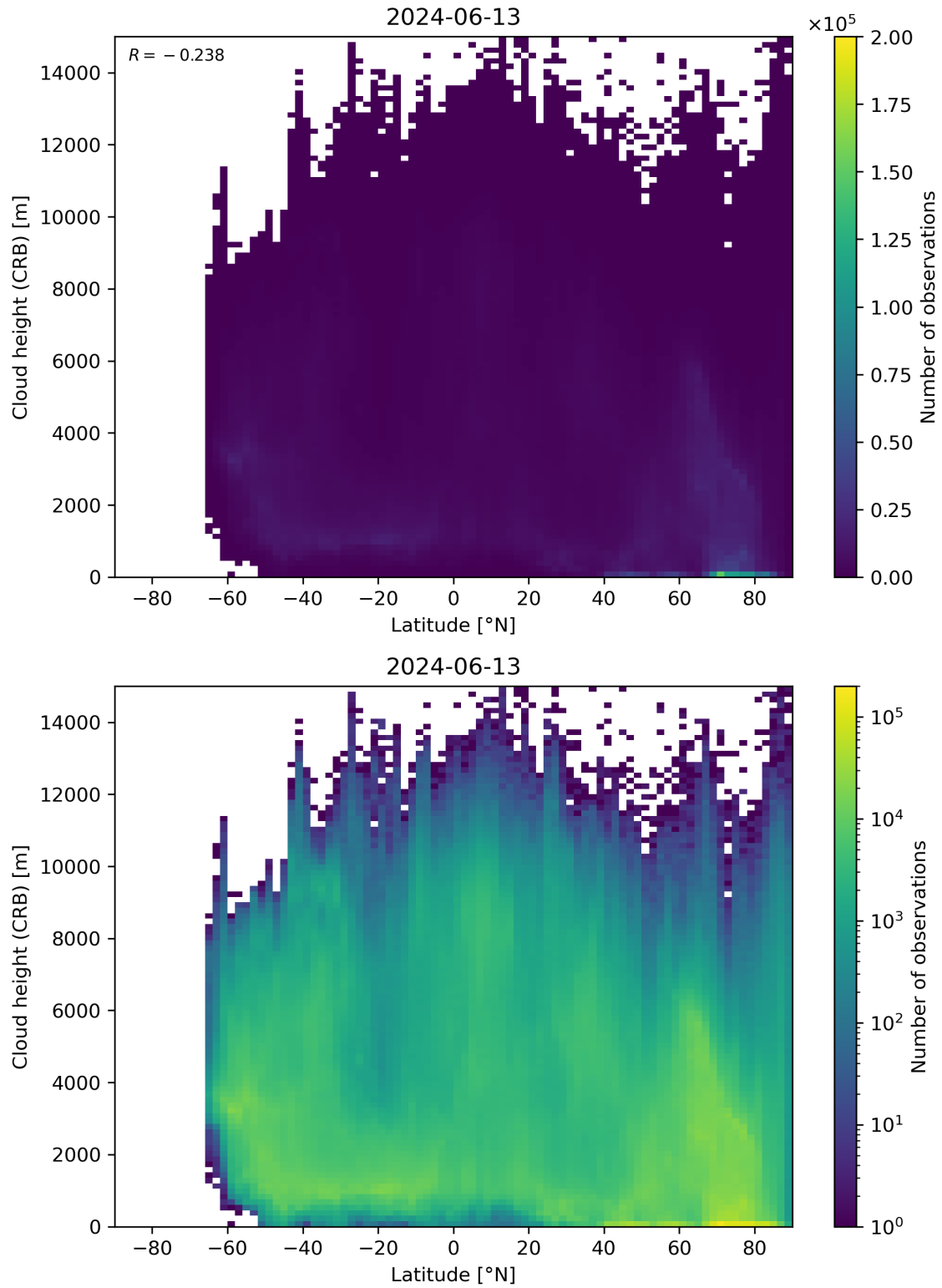
Figure 95: Scatter density plot of “Latitude” against “Cloud height (CRB)” for 2024-06-13 to 2024-06-14.
