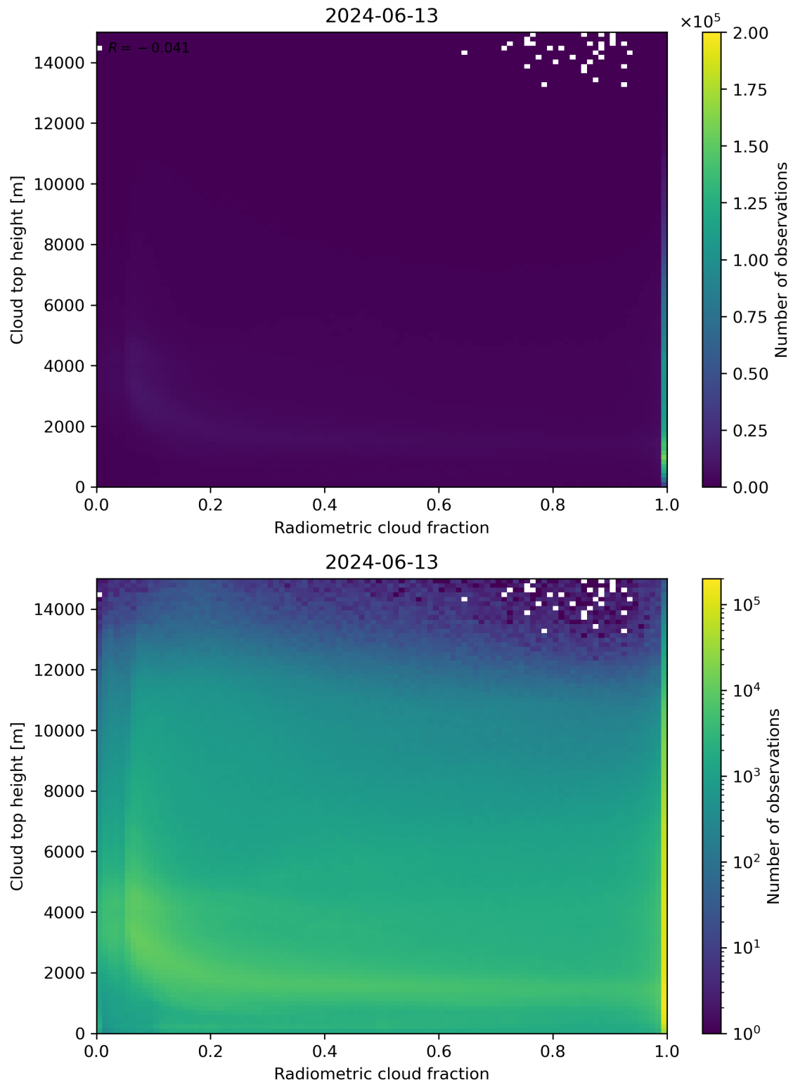
Figure 76: Scatter density plot of “Radiometric cloud fraction” against “Cloud top height” for 2024-06-13 to 2024-06-14.
