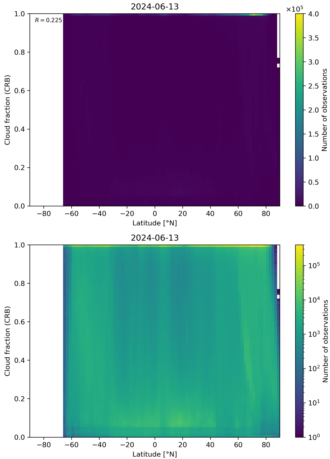
Figure 94: Scatter density plot of “Latitude” against “Cloud fraction (CRB)” for 2024-06-13 to 2024-06-14.
