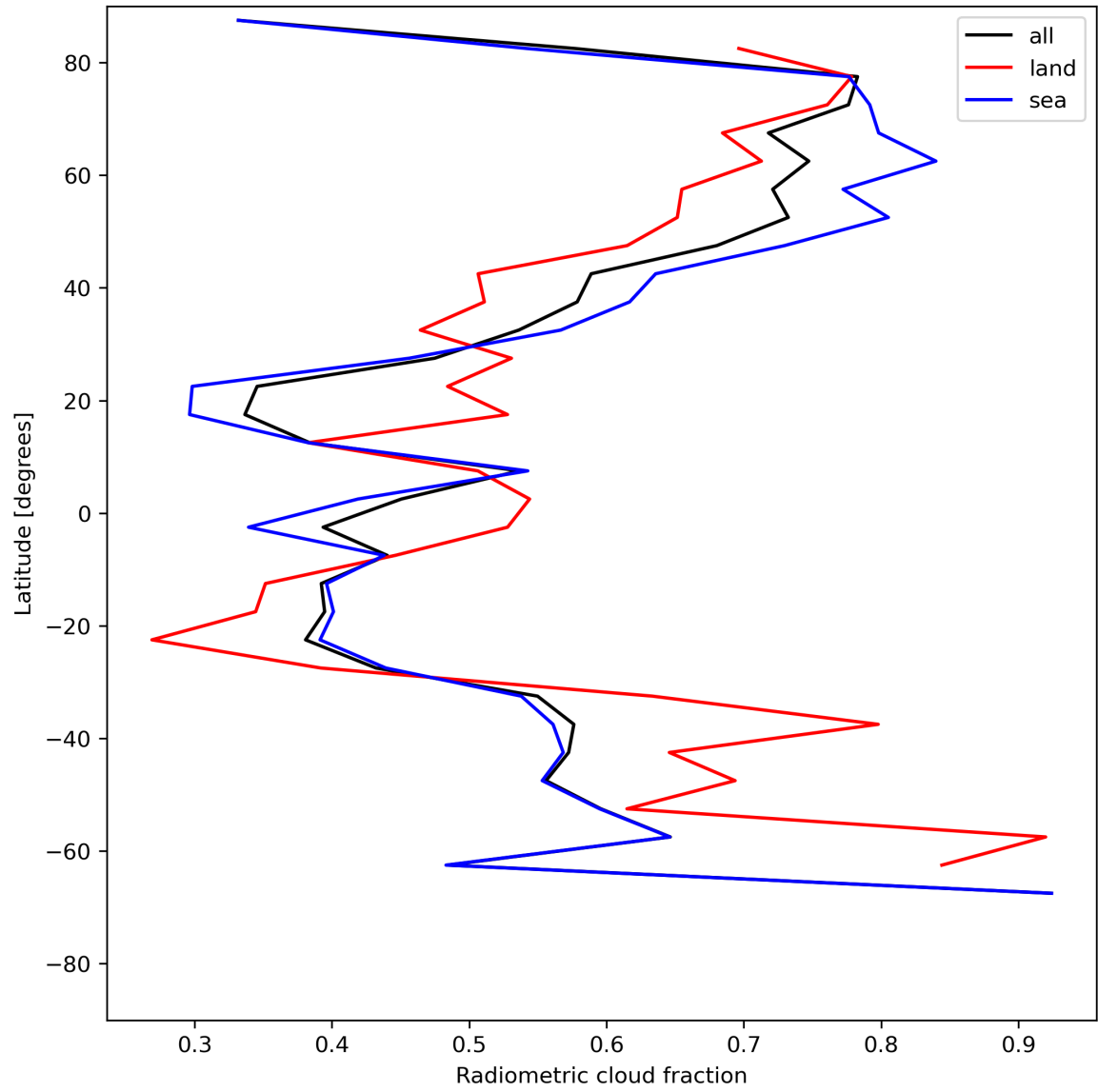
Figure 23: Zonal average of “Radiometric cloud fraction” for 2024-06-13 to 2024-06-14.
