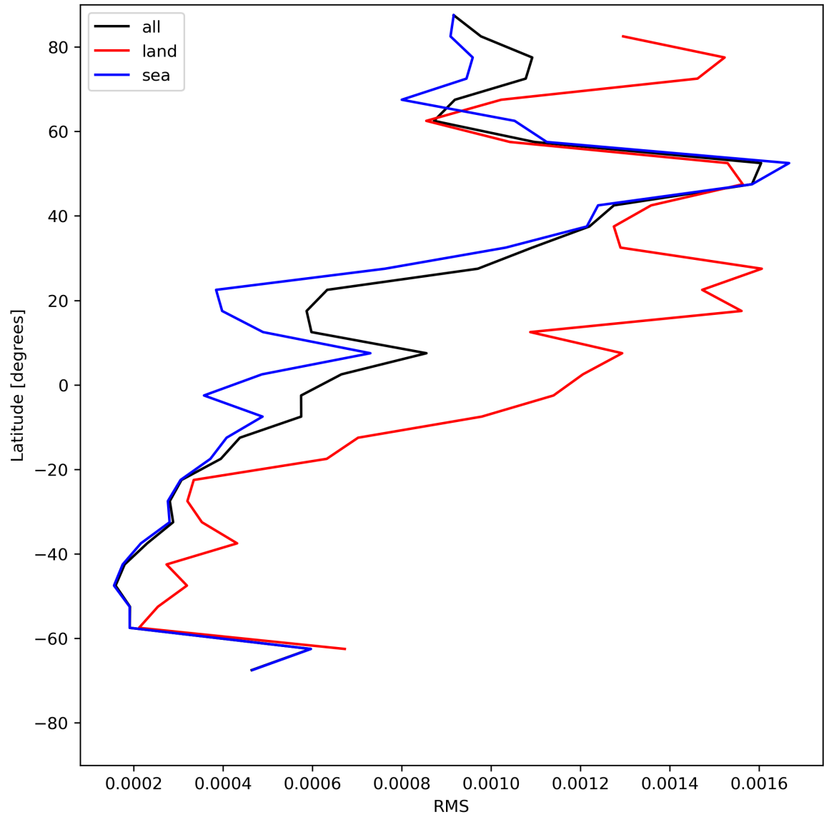
Figure 31: Zonal average of “RMS” for 2024-06-13 to 2024-06-14.
