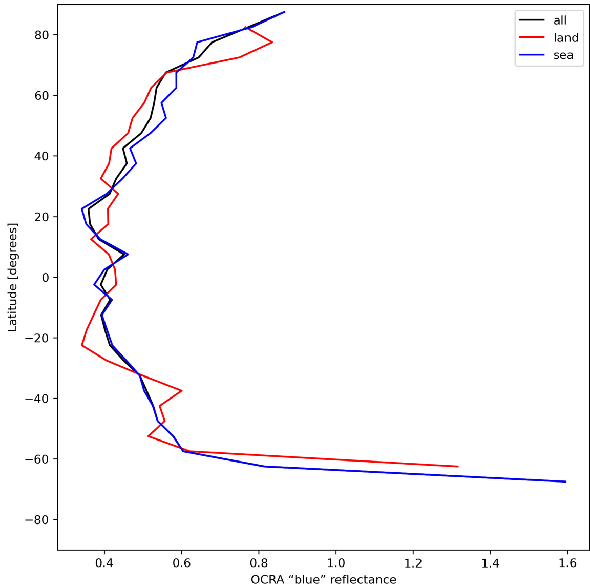
Figure 35: Zonal average of “OCRA “blue” reflectance” for 2024-06-13 to 2024-06-14.
