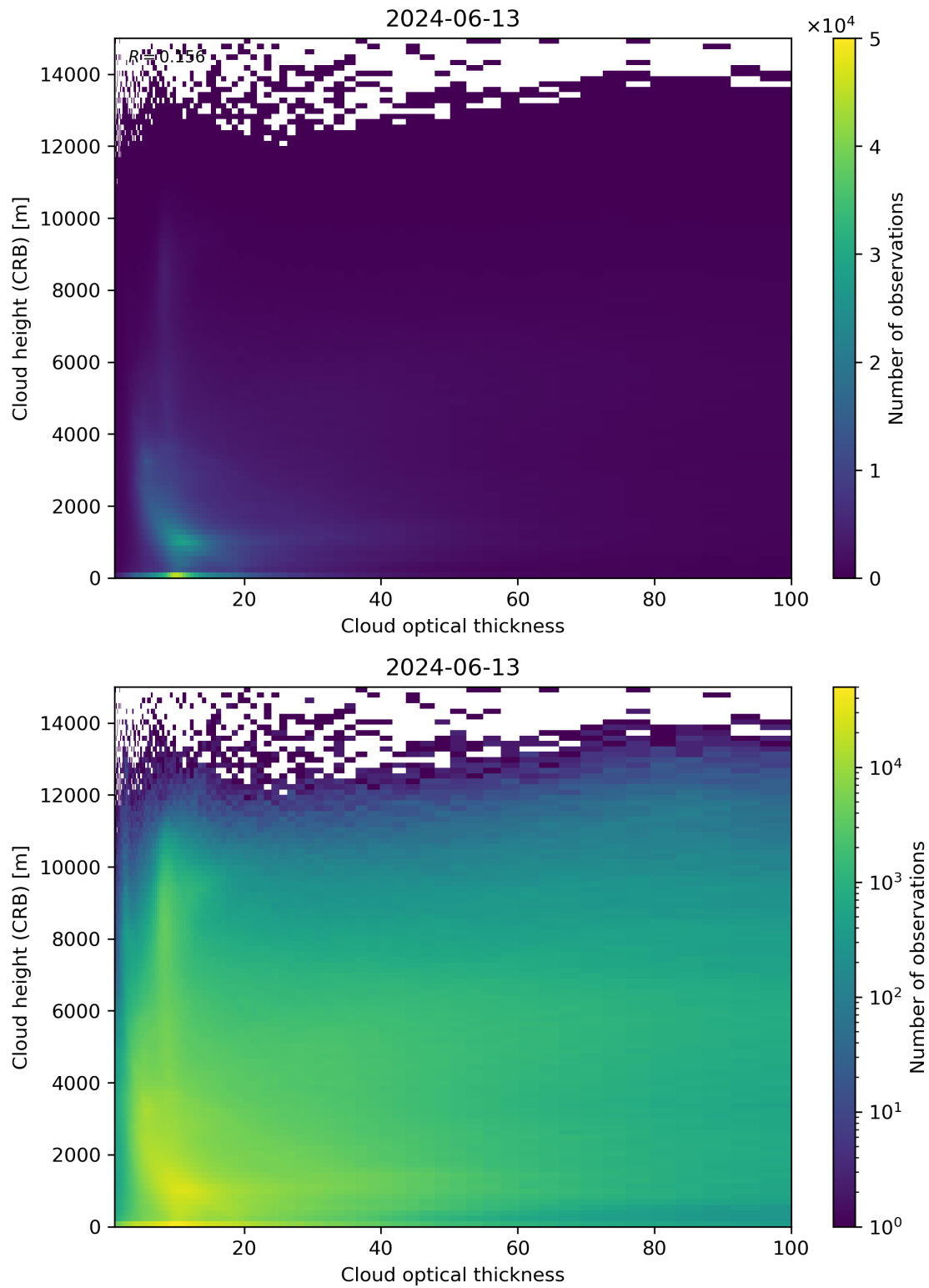
Figure 85: Scatter density plot of “Cloud optical thickness” against “Cloud height (CRB)” for 2024-06-13 to 2024-06-14.
