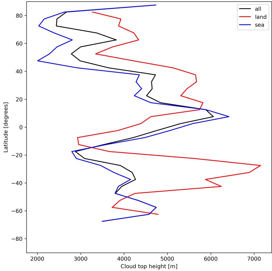
Figure 24: Zonal average of “Cloud top height” for 2024-06-13 to 2024-06-14.
