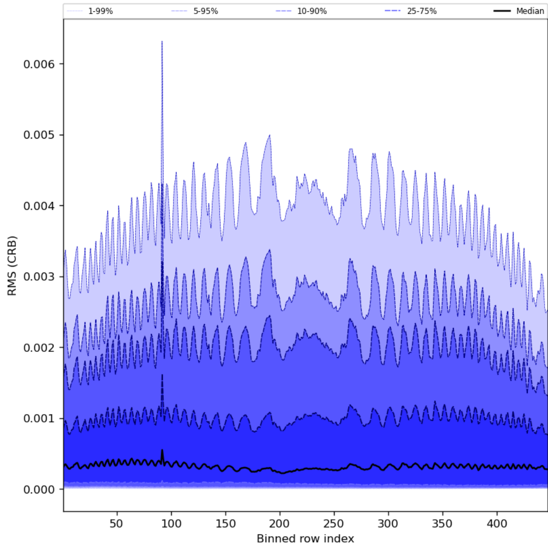
Figure 64: Along track statistics of “RMS (CRB)” for 2024-06-13 to 2024-06-14
