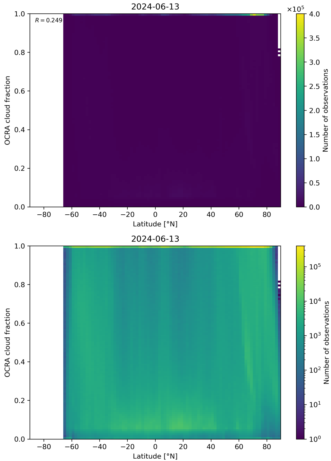
Figure 93: Scatter density plot of “Latitude” against “OCRA cloud fraction” for 2024-06-13 to 2024-06-14.
