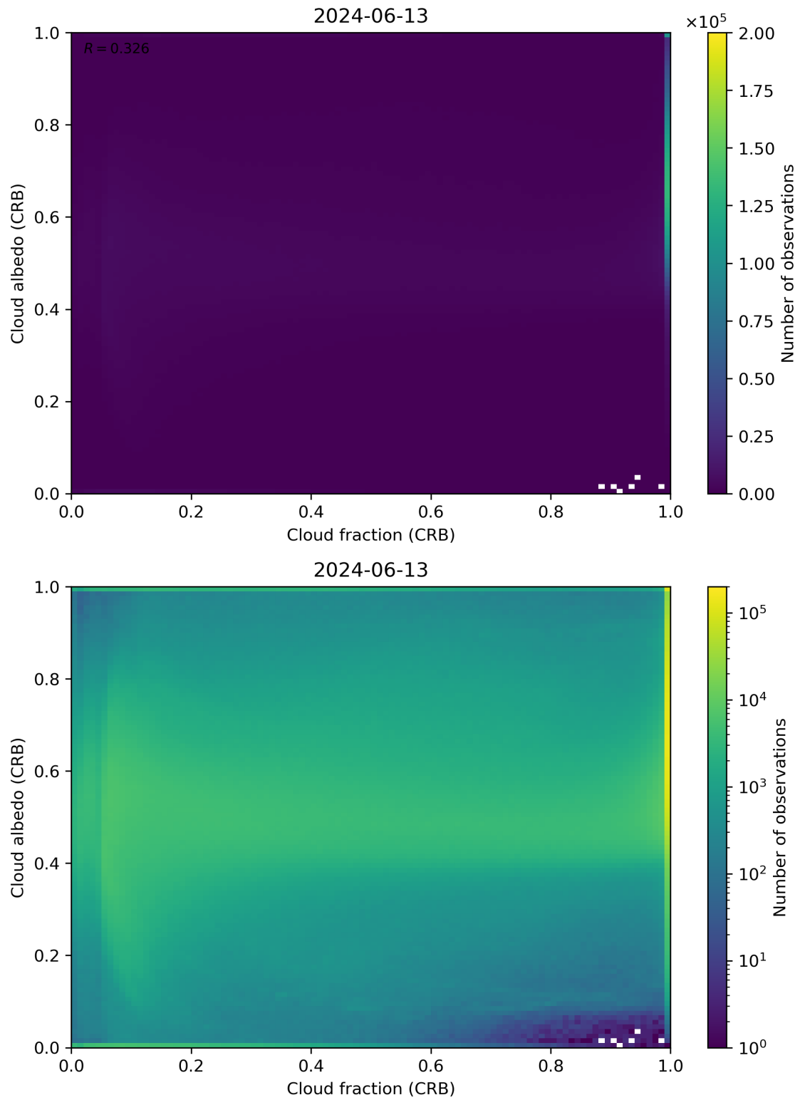
Figure 77: Scatter density plot of “Cloud fraction (CRB)” against “Cloud albedo (CRB)” for 2024-06-13 to 2024-06-14.
