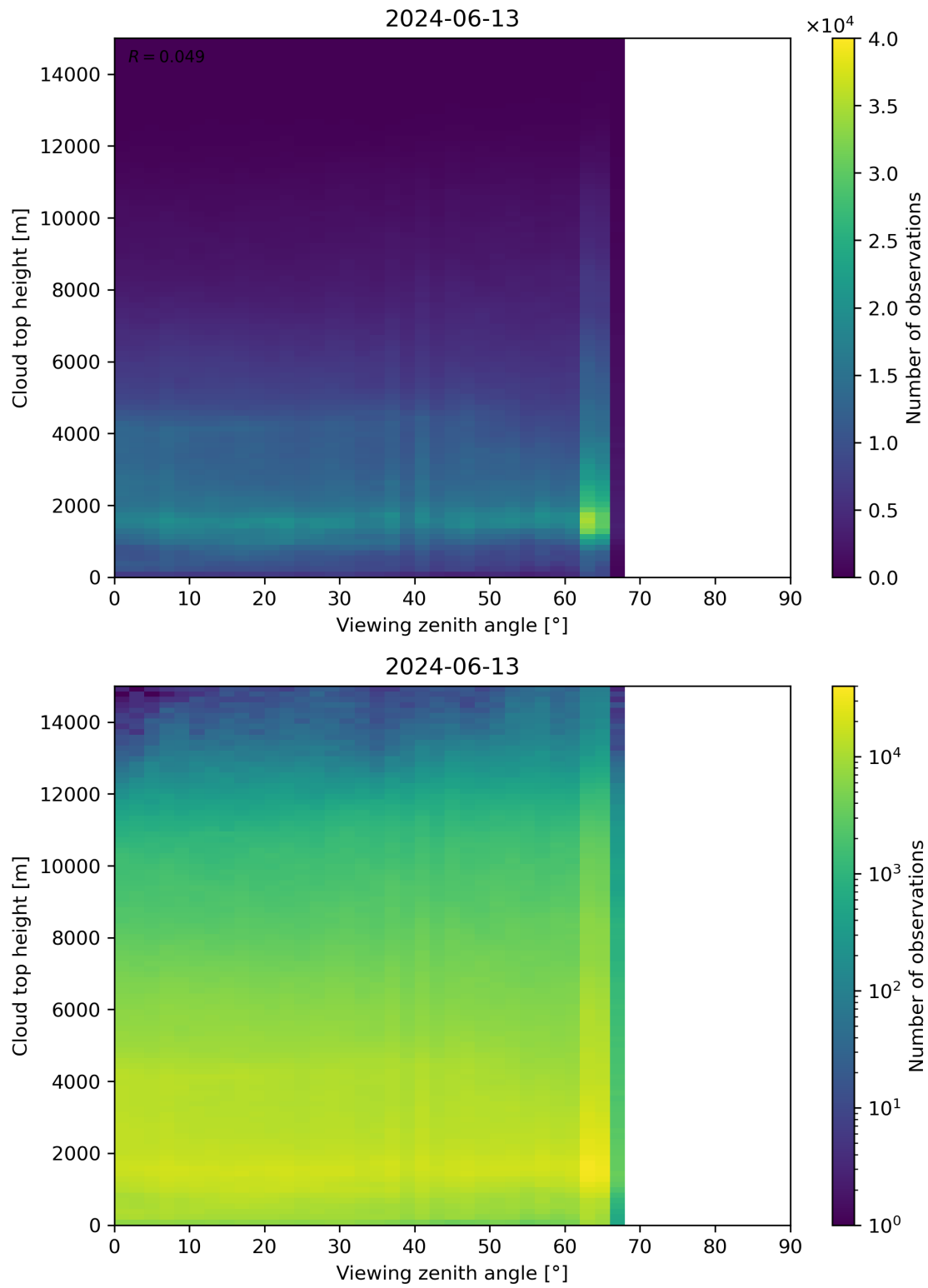
Figure 112: Scatter density plot of “Viewing zenith angle” against “Cloud top height” for 2024-06-13 to 2024-06-14.
