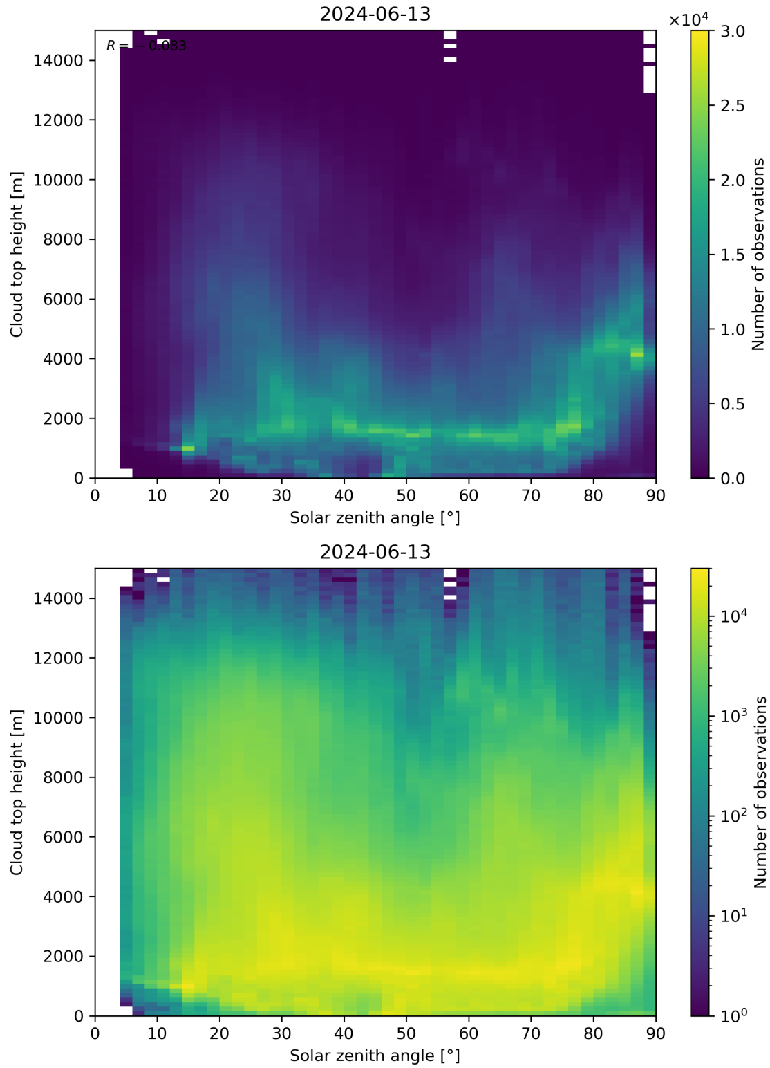
Figure 104: Scatter density plot of “Solar zenith angle” against “Cloud top height” for 2024-06-13 to 2024-06-14.
