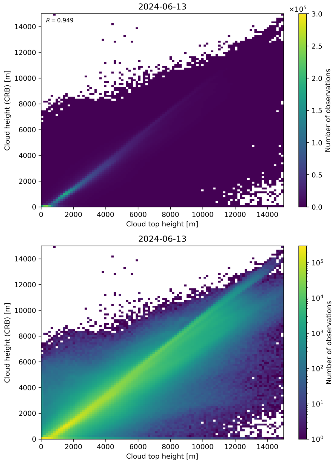
Figure 89: Scatter density plot of “Cloud top height” against “Cloud height (CRB)” for 2024-06-13 to 2024-06-14.
