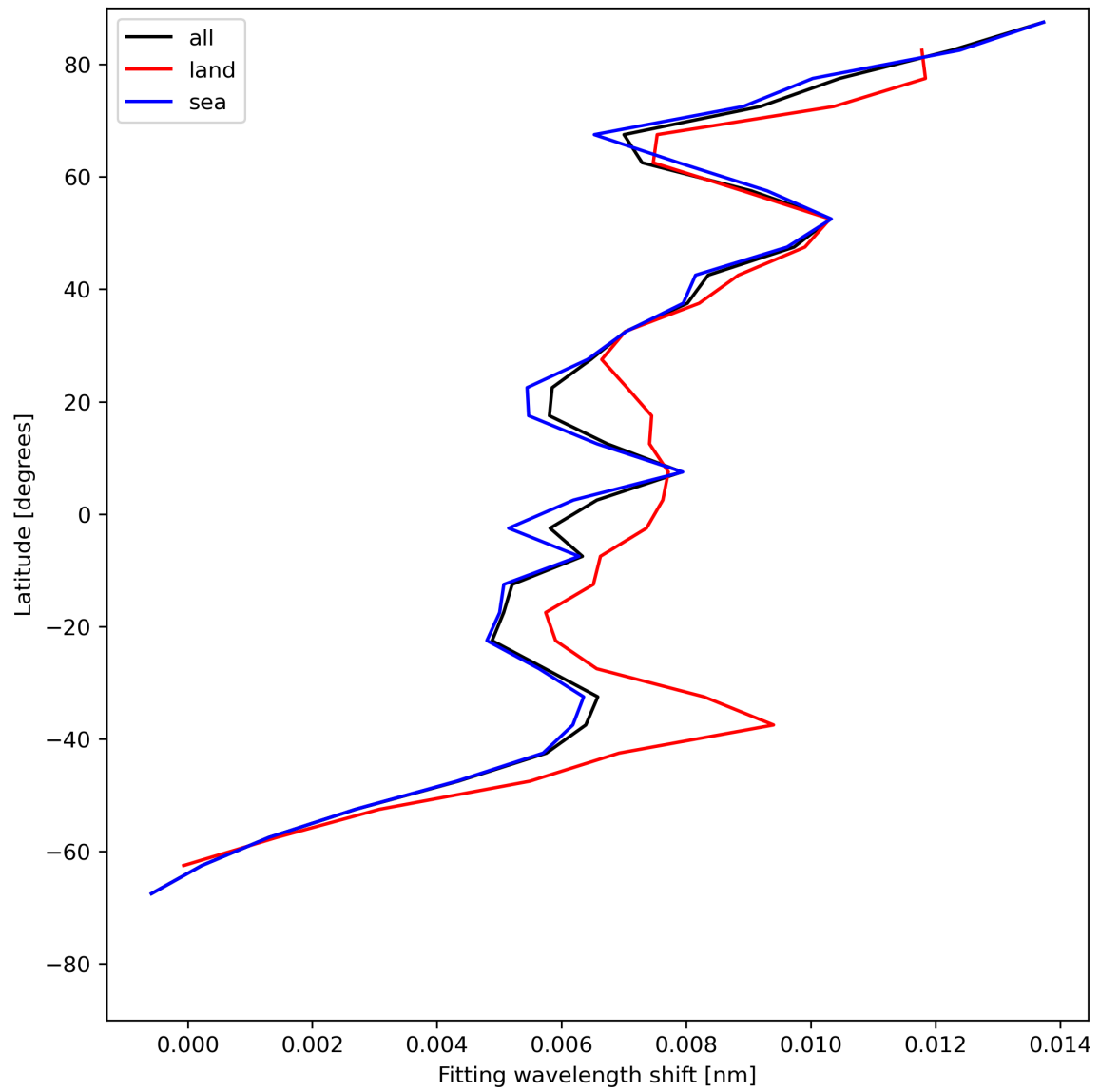
Figure 33: Zonal average of “Fitting wavelength shift” for 2024-06-13 to 2024-06-14.
