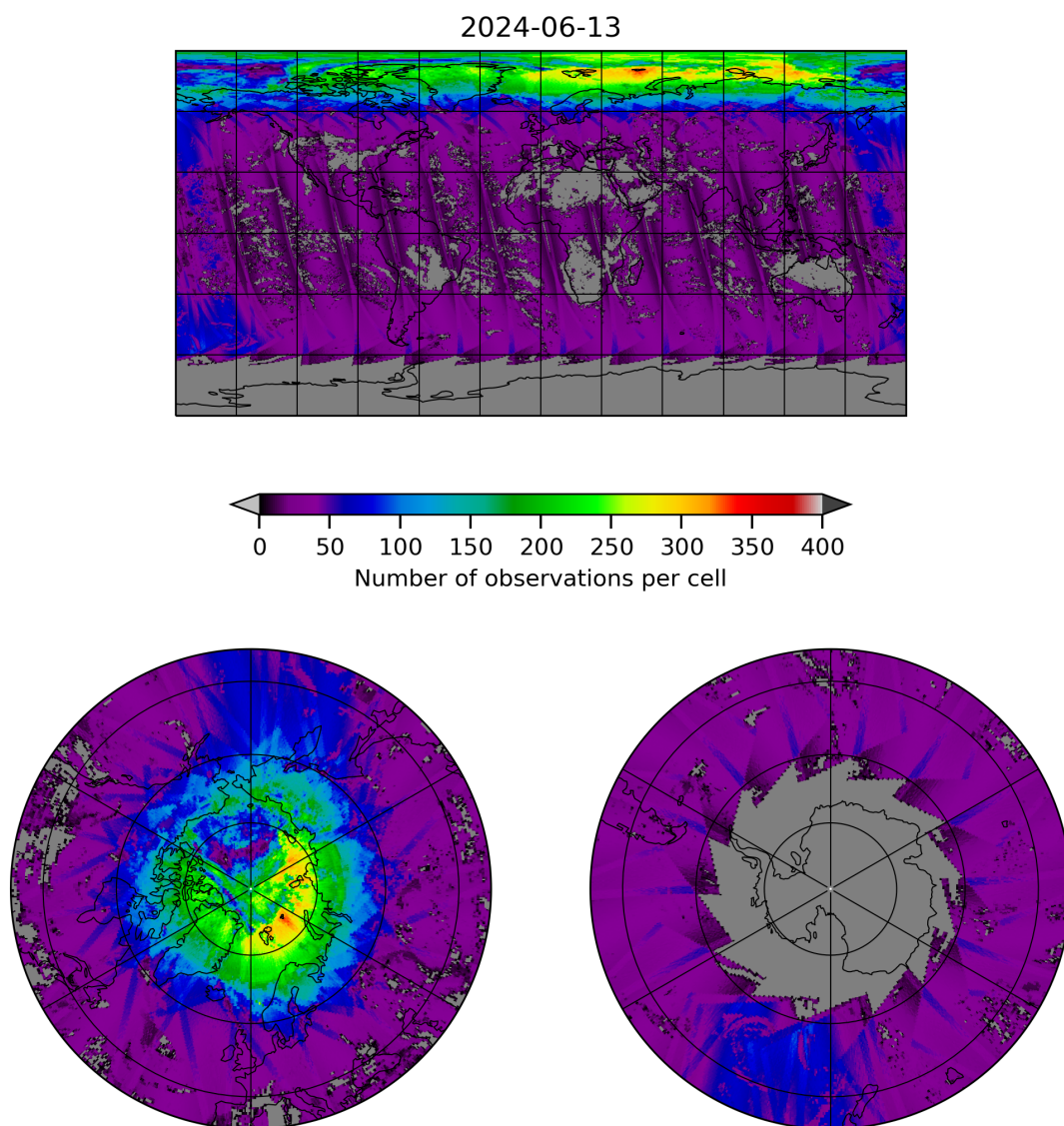
Figure 21: Map of the number of observations for 2024-06-13 to 2024-06-14
