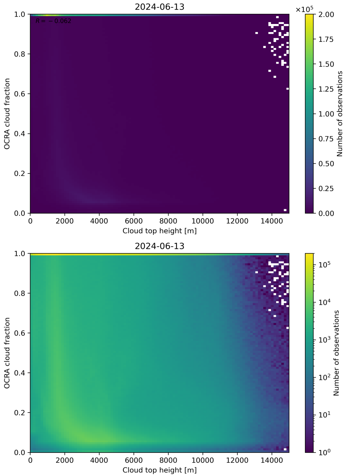
Figure 87: Scatter density plot of “Cloud top height” against “OCRA cloud fraction” for 2024-06-13 to 2024-06-14.
