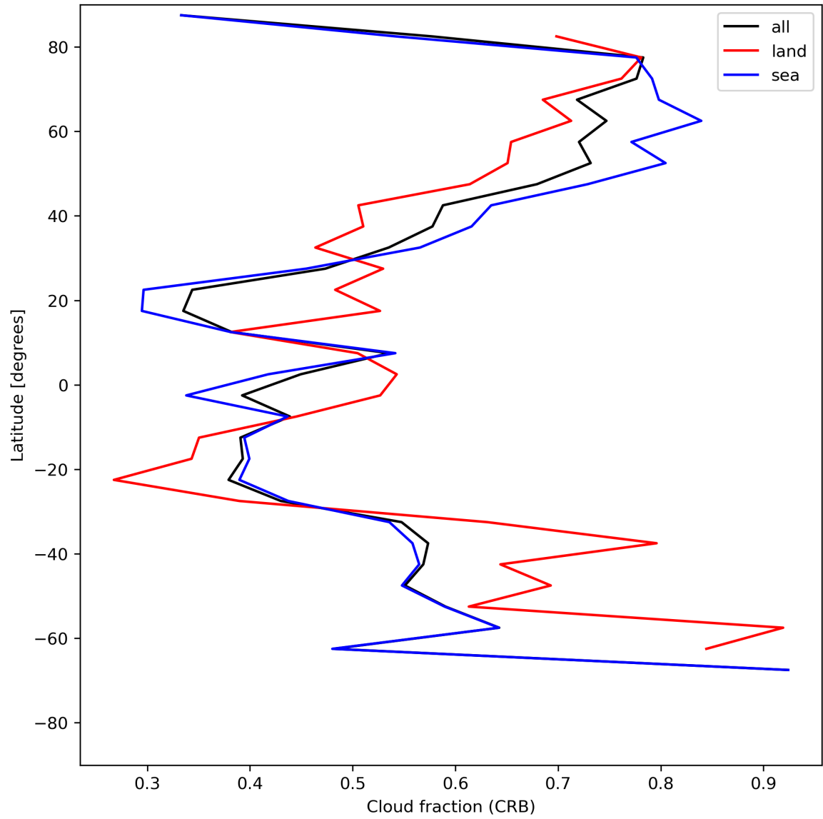
Figure 26: Zonal average of “Cloud fraction (CRB)” for 2024-06-13 to 2024-06-14.
