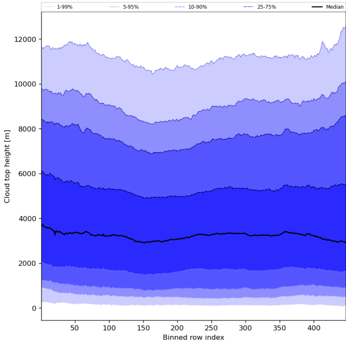
Figure 56: Along track statistics of “Cloud top height” for 2024-06-13 to 2024-06-14
