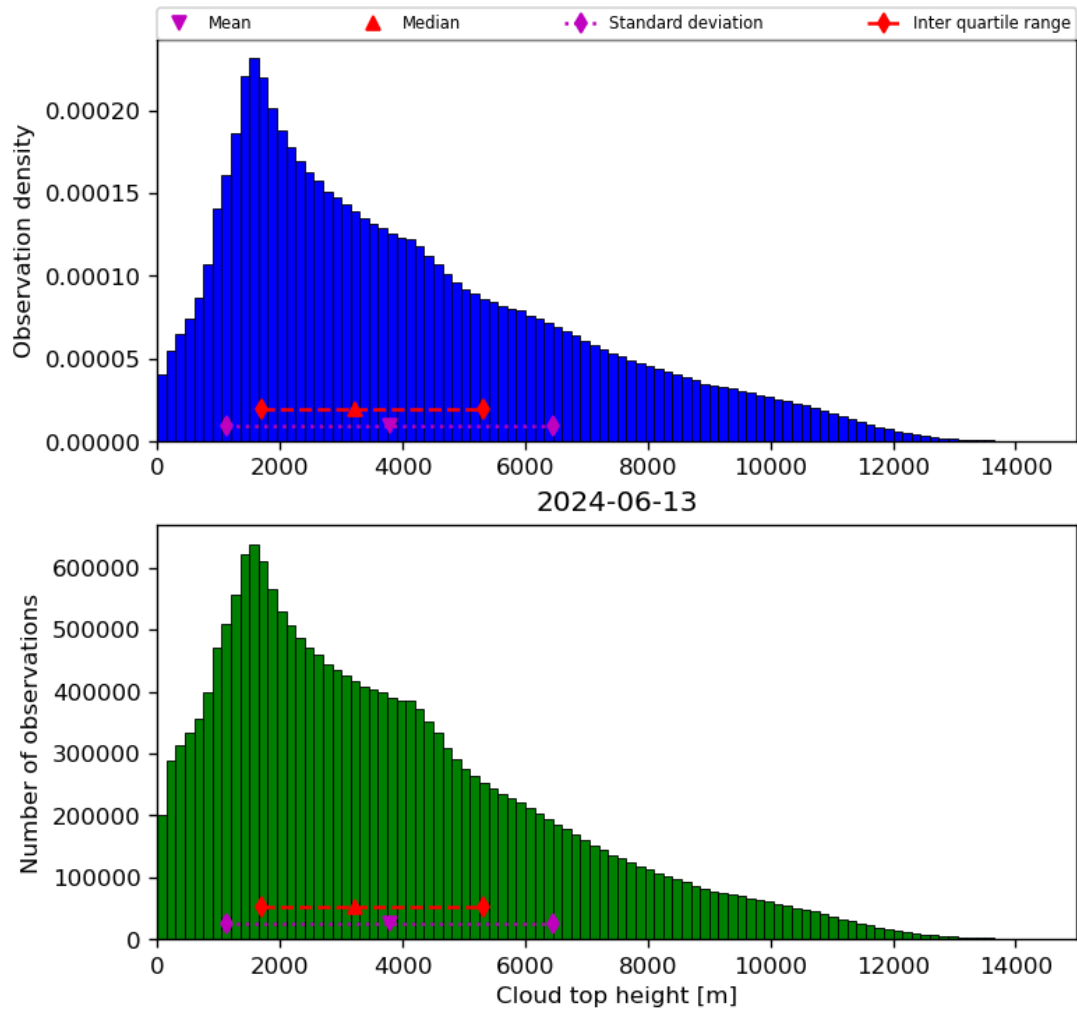
Figure 40: Histogram of “Cloud top height” for 2024-06-13 to 2024-06-14
