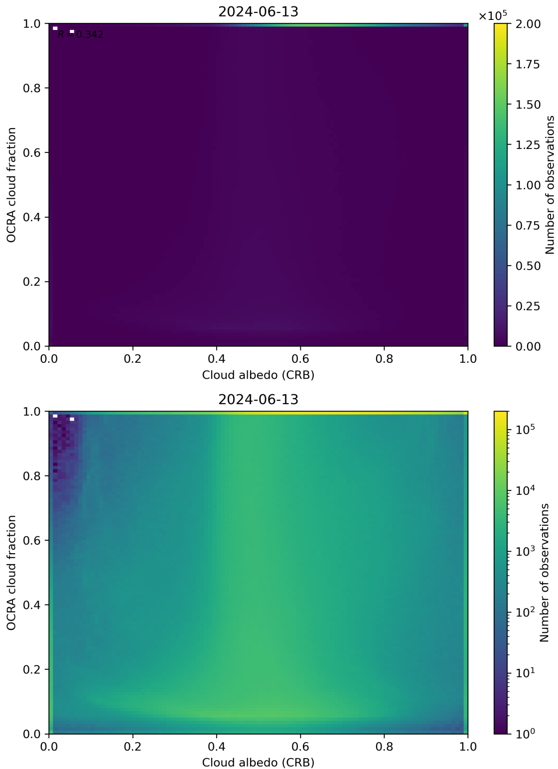
Figure 70: Scatter density plot of “Cloud albedo (CRB)” against “OCRA cloud fraction” for 2024-06-13 to 2024-06-14.
