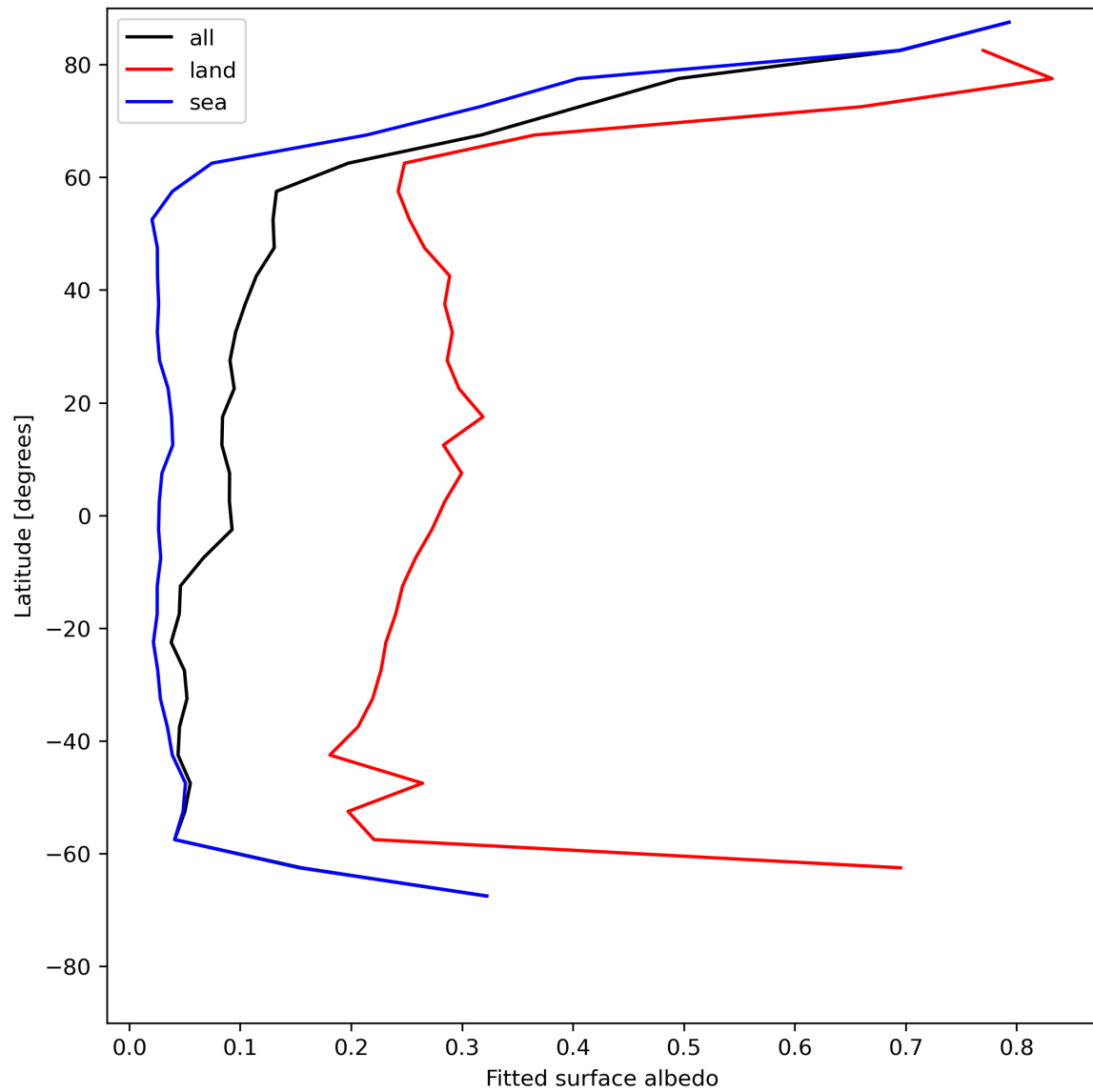
Figure 29: Zonal average of “Fitted surface albedo” for 2024-06-13 to 2024-06-14.
