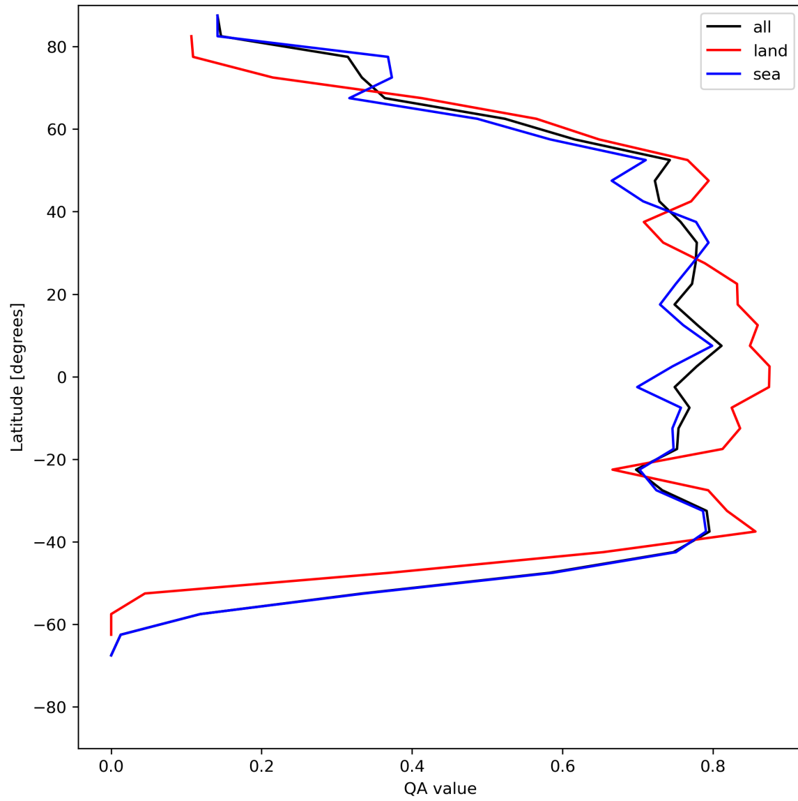
Figure 22: Zonal average of “QA value” for 2024-06-13 to 2024-06-14.
