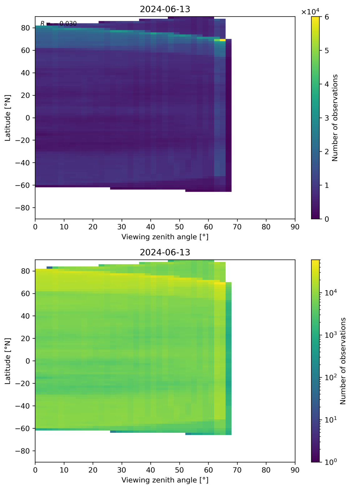
Figure 113: Scatter density plot of “Viewing zenith angle” against “Latitude” for 2024-06-13 to 2024-06-14.
