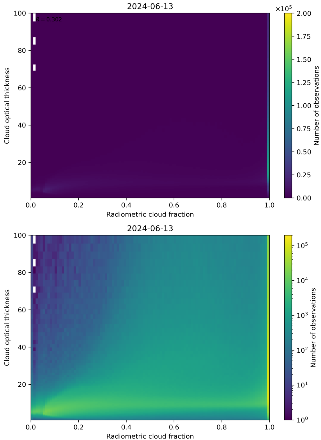
Figure 75: Scatter density plot of “Radiometric cloud fraction” against “Cloud optical thickness” for 2024-06-13 to 2024-06-14.
