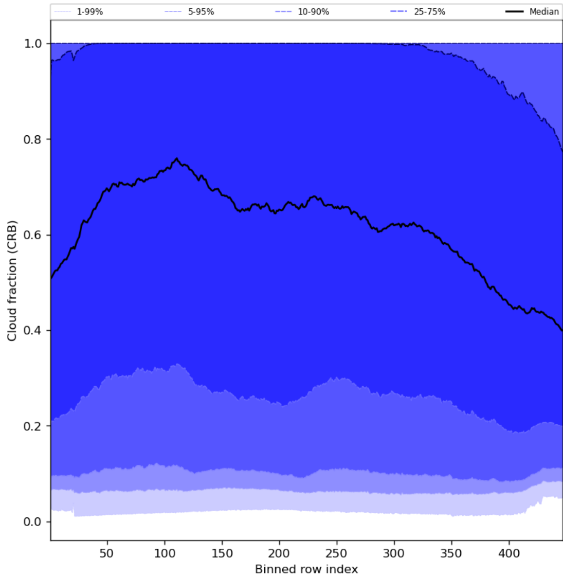
Figure 58: Along track statistics of “Cloud fraction (CRB)” for 2024-06-13 to 2024-06-14
