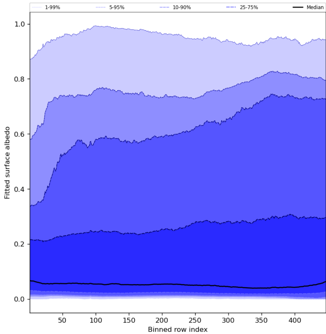
Figure 61: Along track statistics of “Fitted surface albedo” for 2024-06-13 to 2024-06-14
