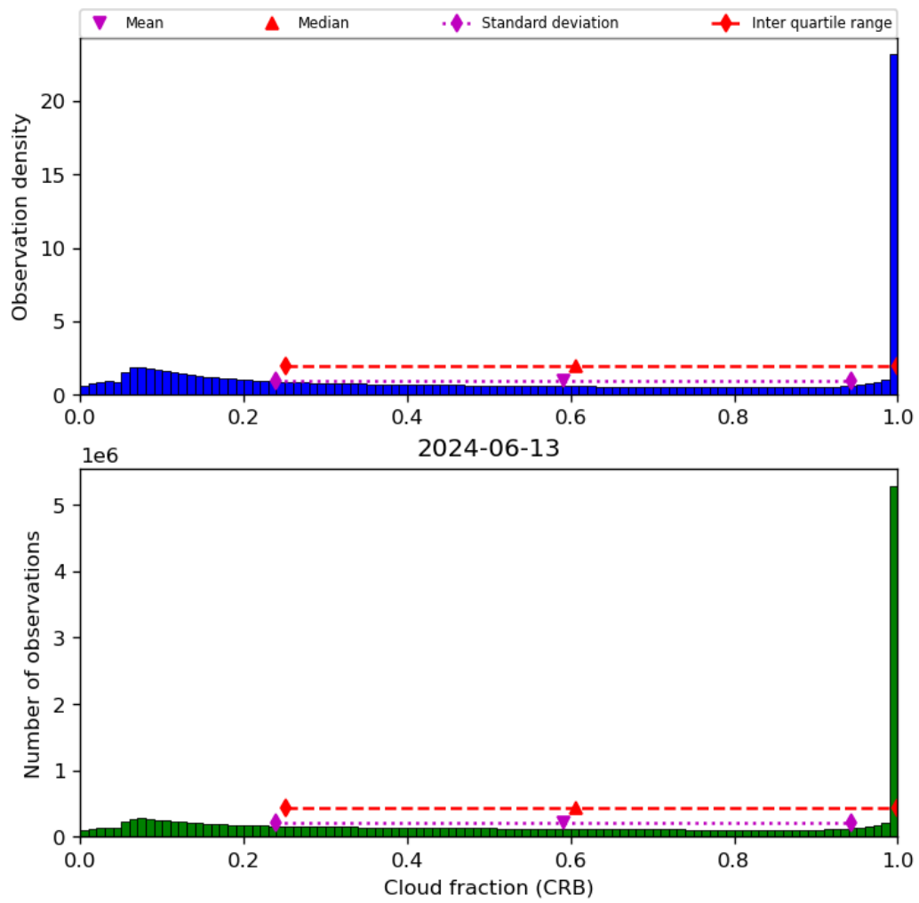
Figure 42: Histogram of “Cloud fraction (CRB)” for 2024-06-13 to 2024-06-14
