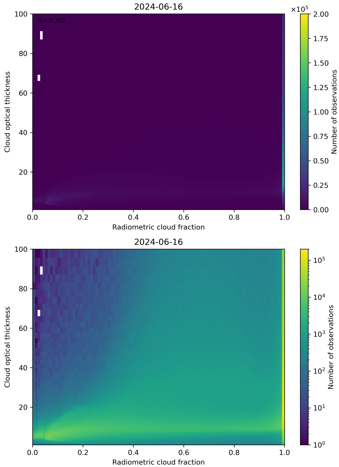
Figure 75: Scatter density plot of “Radiometric cloud fraction” against “Cloud optical thickness” for 2024-06-15 to 2024-06-17.
