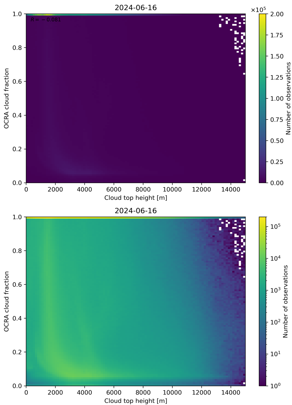
Figure 87: Scatter density plot of “Cloud top height” against “OCRA cloud fraction” for 2024-06-15 to 2024-06-17.
