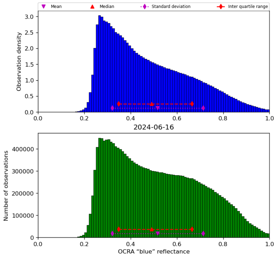
Figure 51: Histogram of “OCRA “blue” reflectance” for 2024-06-15 to 2024-06-17
