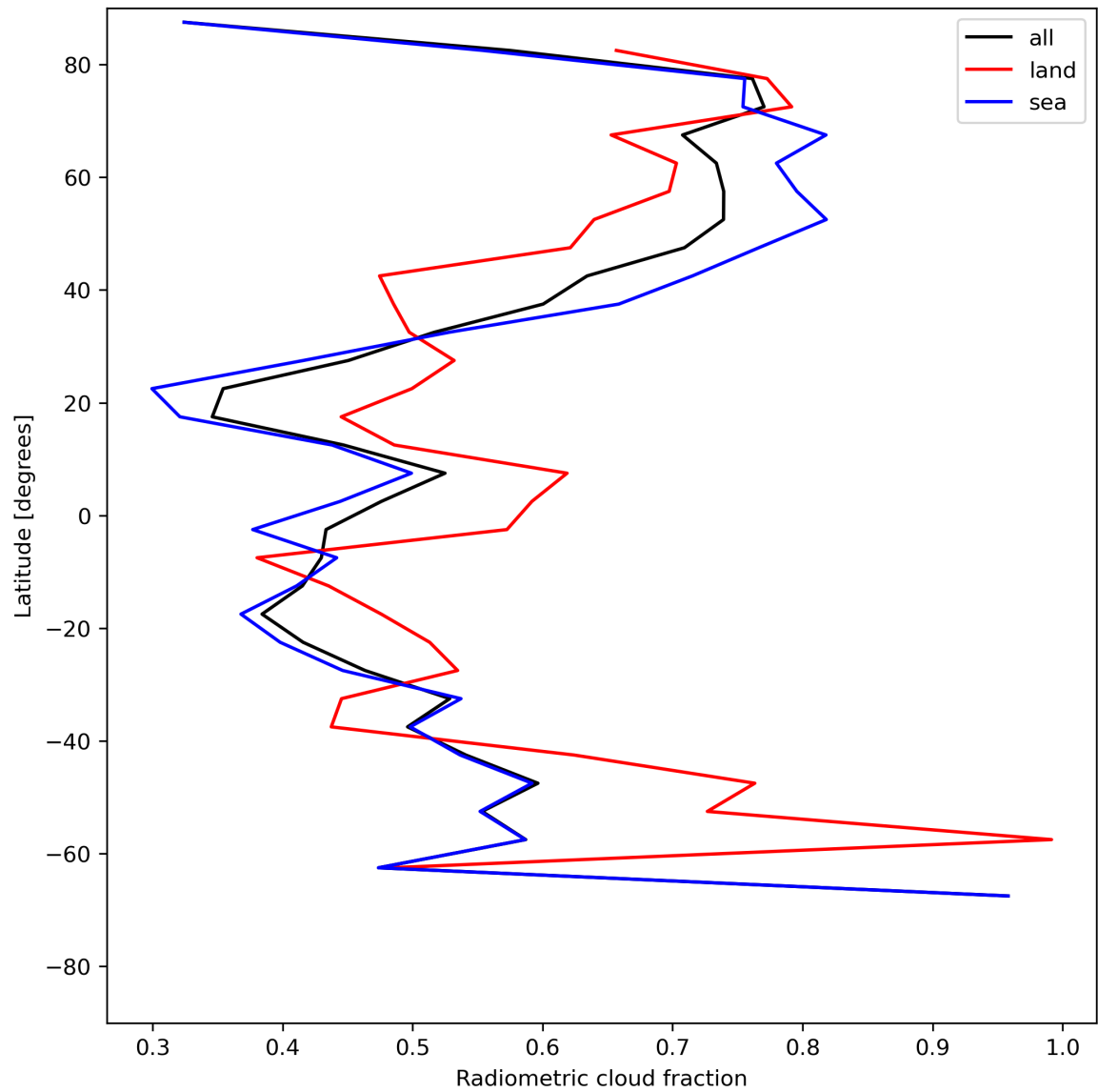
Figure 23: Zonal average of “Radiometric cloud fraction” for 2024-06-15 to 2024-06-17.
