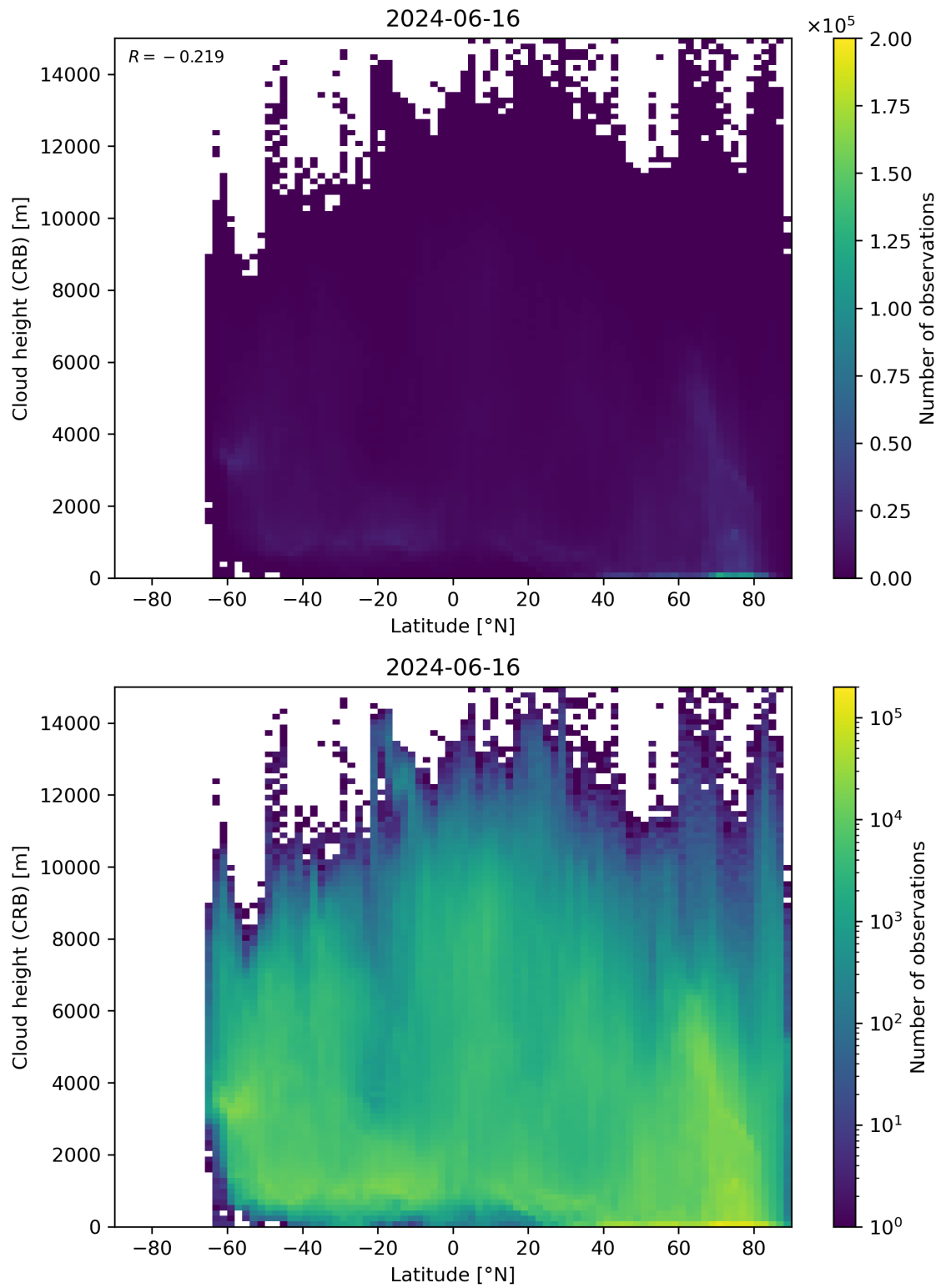
Figure 95: Scatter density plot of “Latitude” against “Cloud height (CRB)” for 2024-06-15 to 2024-06-17.
