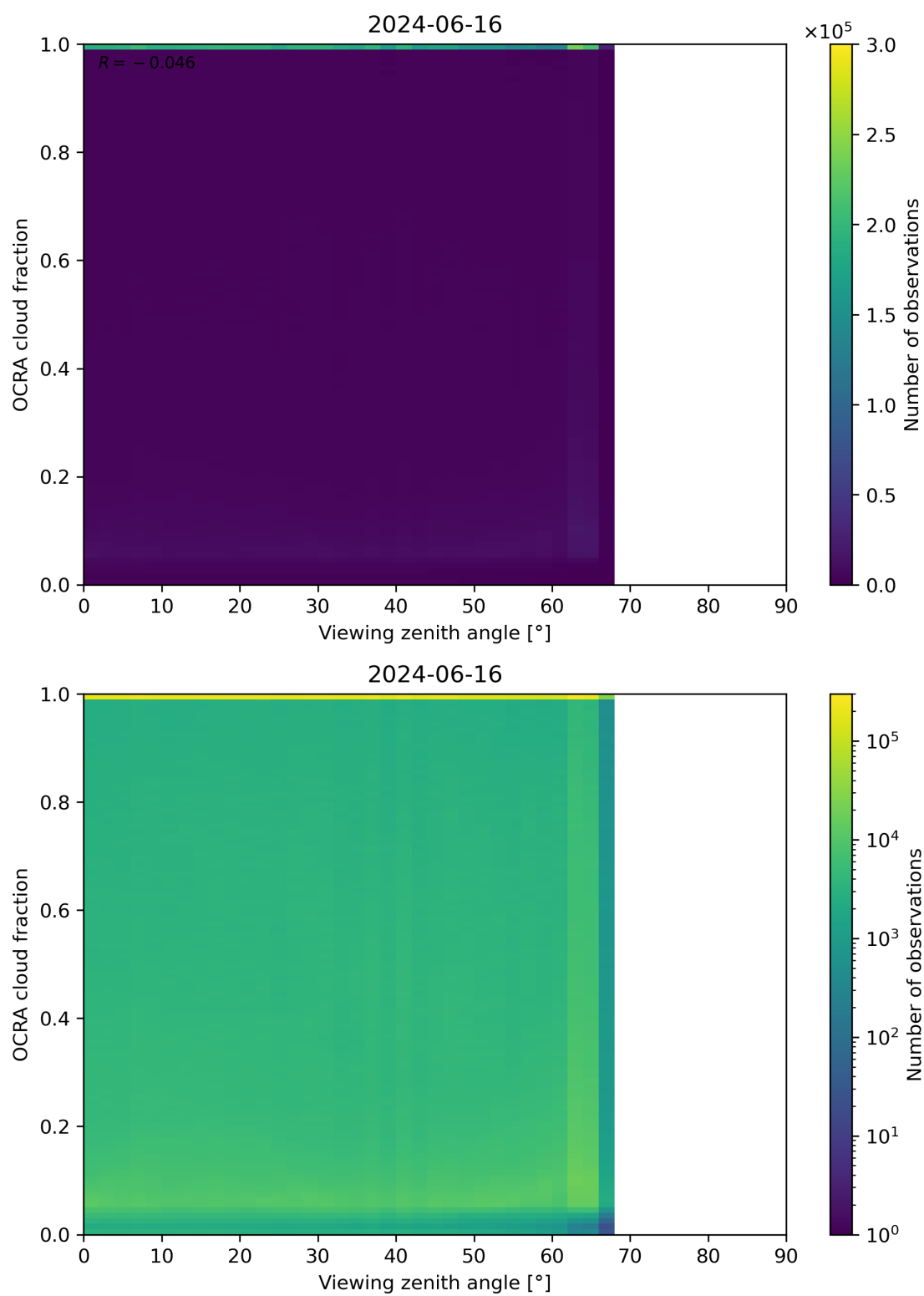
Figure 108: Scatter density plot of “Viewing zenith angle” against “OCRA cloud fraction” for 2024-06-15 to 2024-06-17.
