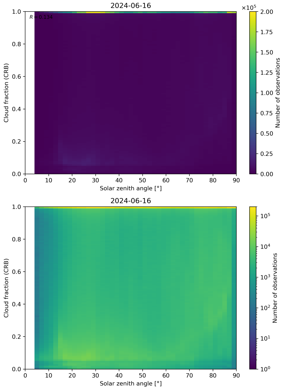
Figure 101: Scatter density plot of “Solar zenith angle” against “Cloud fraction (CRB)” for 2024-06-15 to 2024-06-17.
