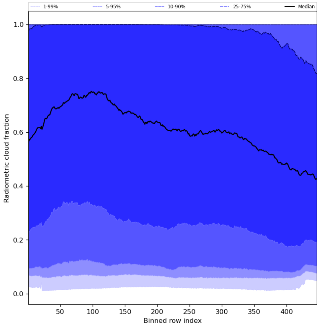
Figure 55: Along track statistics of “Radiometric cloud fraction” for 2024-06-15 to 2024-06-17
