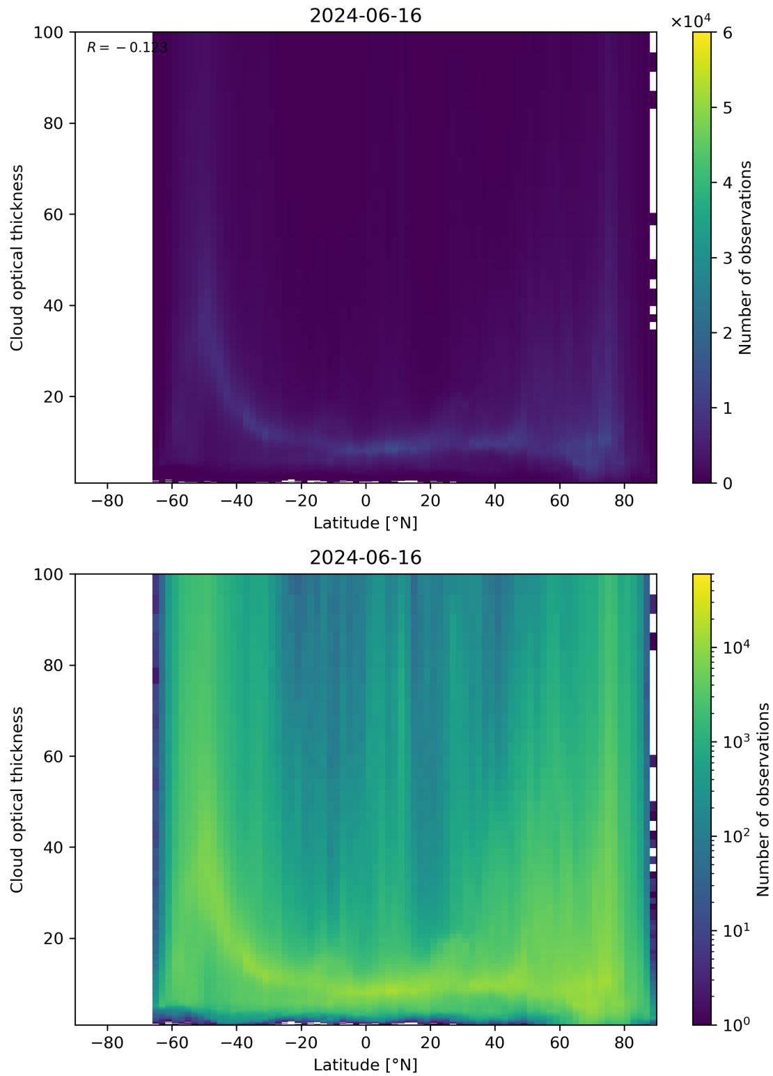
Figure 96: Scatter density plot of “Latitude” against “Cloud optical thickness” for 2024-06-15 to 2024-06-17.
