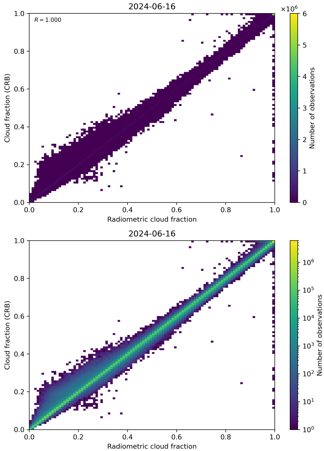
Figure 73: Scatter density plot of “Radiometric cloud fraction” against “Cloud fraction (CRB)” for 2024-06-15 to 2024-06-17.
