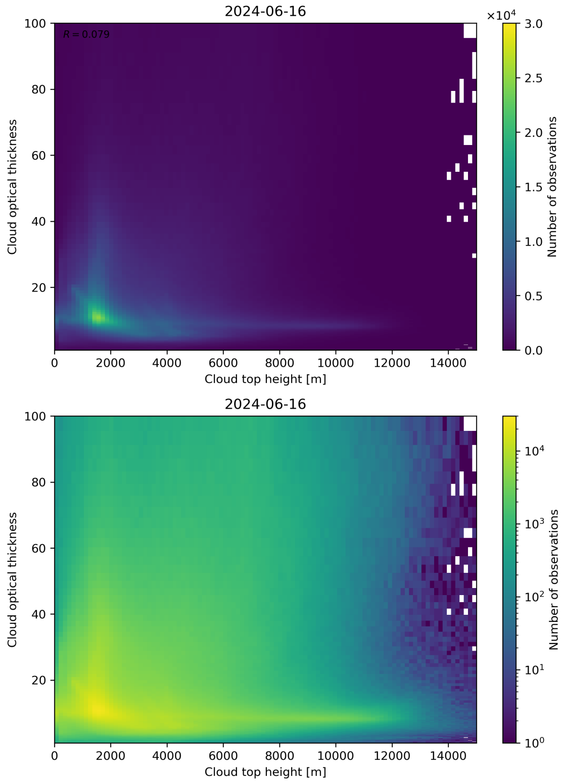
Figure 90: Scatter density plot of “Cloud top height” against “Cloud optical thickness” for 2024-06-15 to 2024-06-17.
