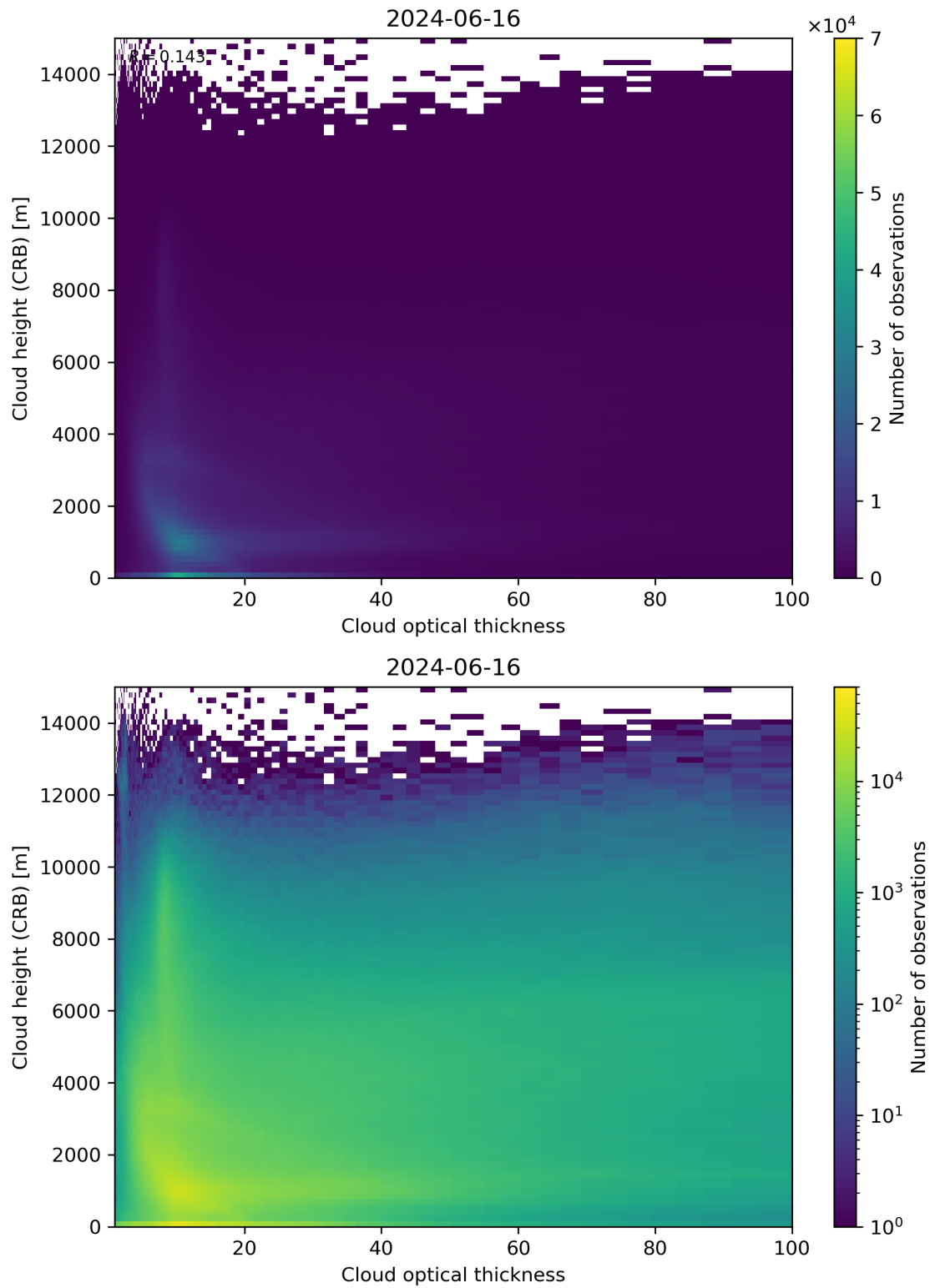
Figure 85: Scatter density plot of “Cloud optical thickness” against “Cloud height (CRB)” for 2024-06-15 to 2024-06-17.
