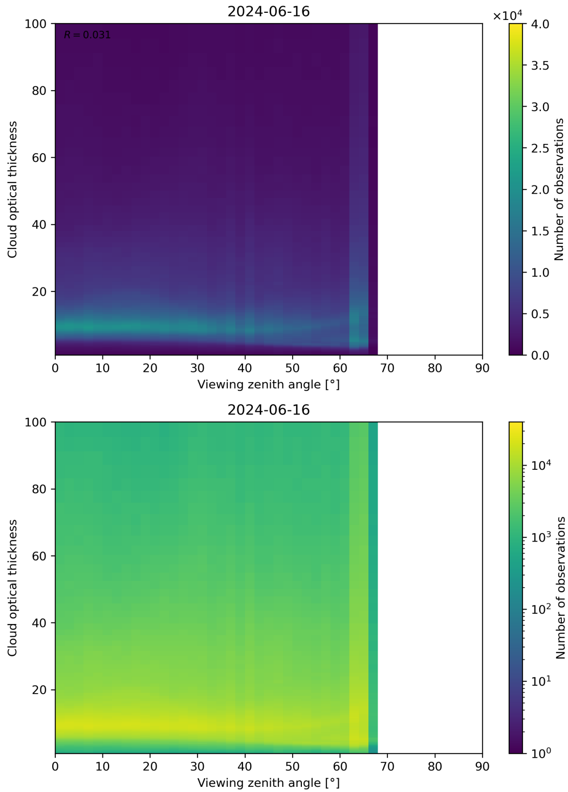
Figure 111: Scatter density plot of “Viewing zenith angle” against “Cloud optical thickness” for 2024-06-15 to 2024-06-17.
