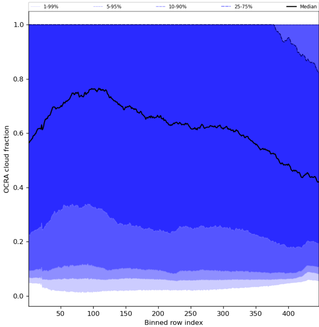
Figure 66: Along track statistics of “OCRA cloud fraction” for 2024-06-15 to 2024-06-17
