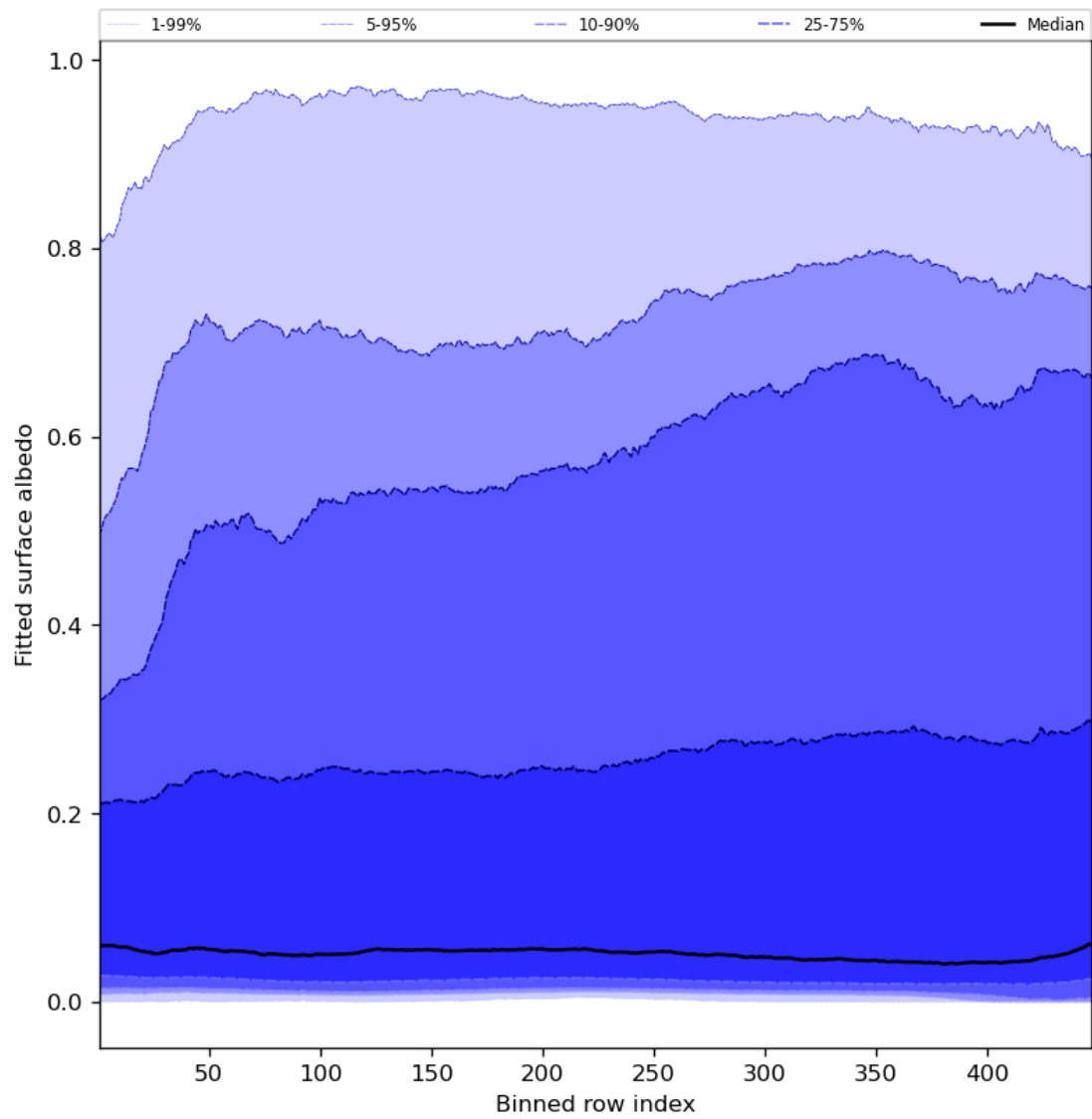
Figure 61: Along track statistics of “Fitted surface albedo” for 2024-06-15 to 2024-06-17
