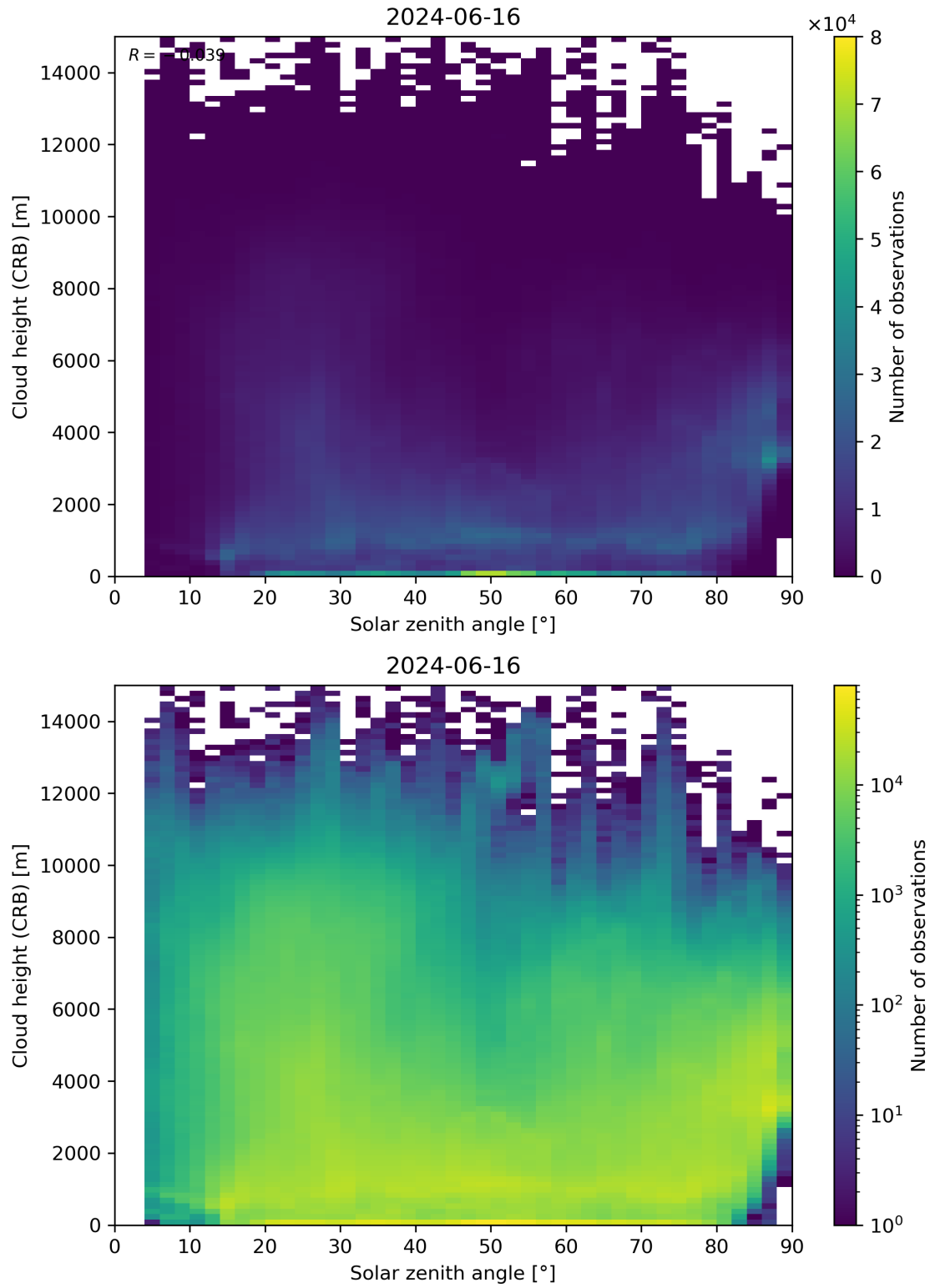
Figure 102: Scatter density plot of “Solar zenith angle” against “Cloud height (CRB)” for 2024-06-15 to 2024-06-17.
