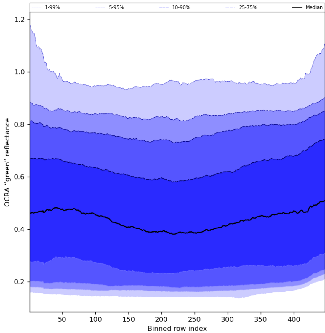
Figure 68: Along track statistics of "OCRA "green" reflectance" for 2024-06-15 to 2024-06-17
