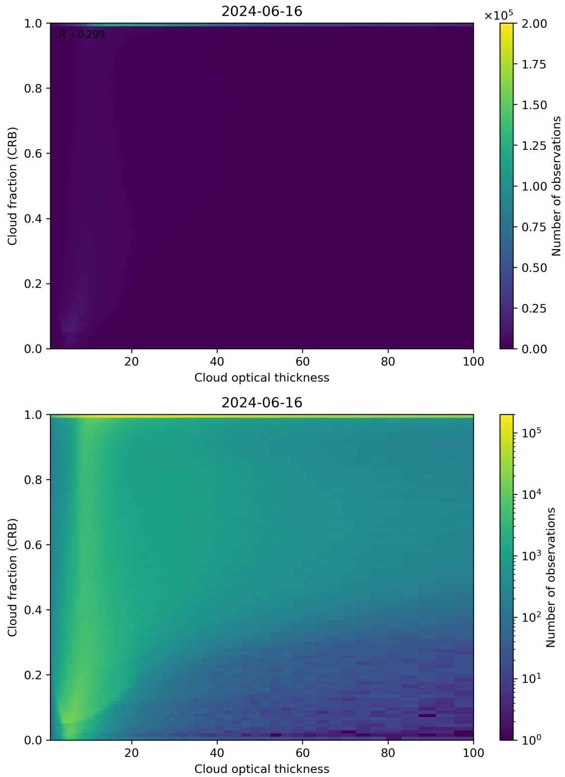
Figure 84: Scatter density plot of “Cloud optical thickness” against “Cloud fraction (CRB)” for 2024-06-15 to 2024-06-17.
