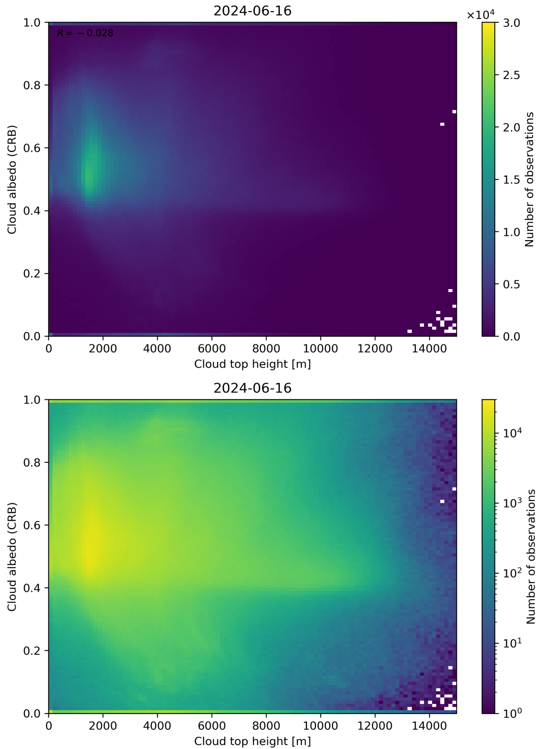
Figure 86: Scatter density plot of “Cloud top height” against “Cloud albedo (CRB)” for 2024-06-15 to 2024-06-17.
