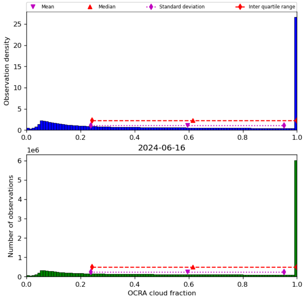
Figure 50: Histogram of “OCRA cloud fraction” for 2024-06-15 to 2024-06-17
