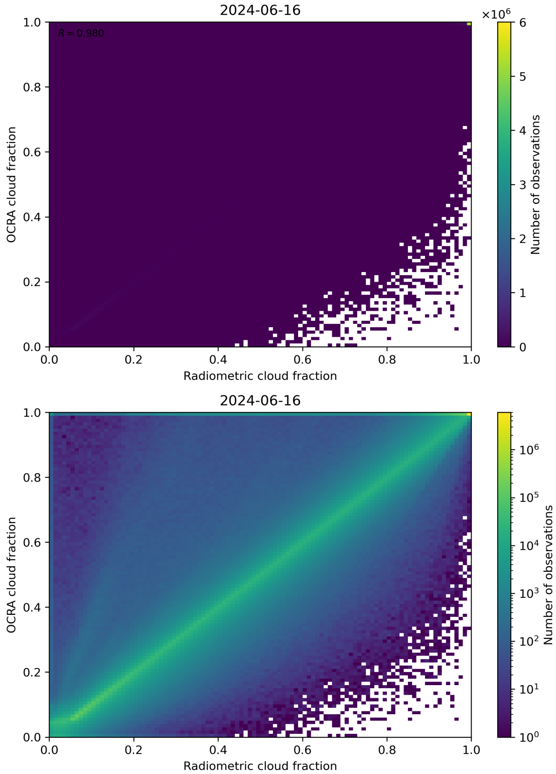
Figure 72: Scatter density plot of “Radiometric cloud fraction” against “OCRA cloud fraction” for 2024-06-15 to 2024-06-17.
