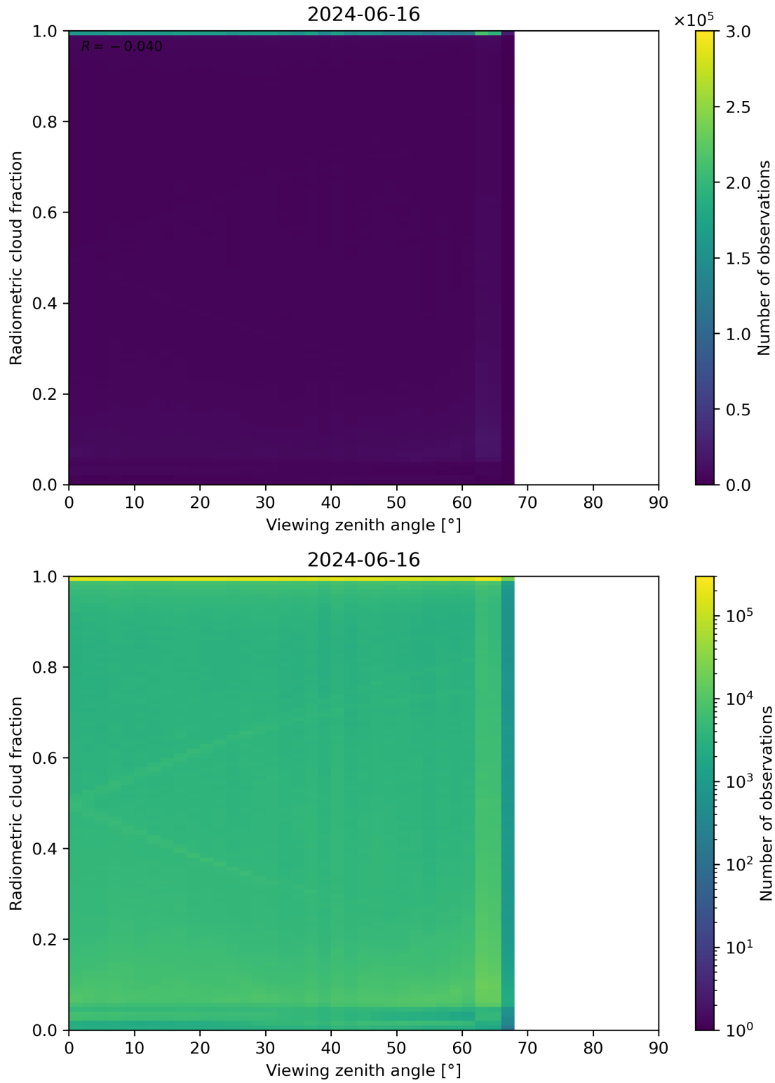
Figure 107: Scatter density plot of “Viewing zenith angle” against “Radiometric cloud fraction” for 2024-06-15 to 2024-06-17.
