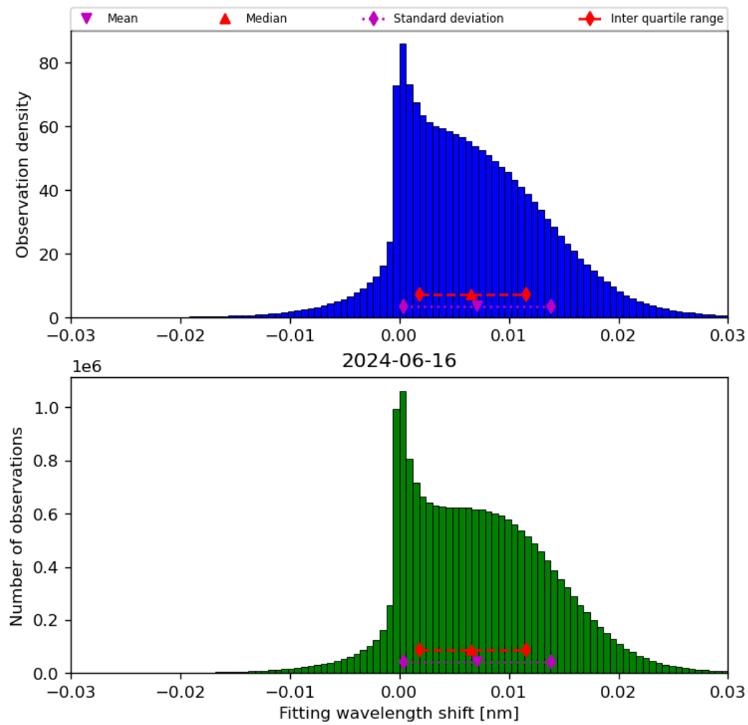
Figure 49: Histogram of “Fitting wavelength shift” for 2024-06-15 to 2024-06-17
