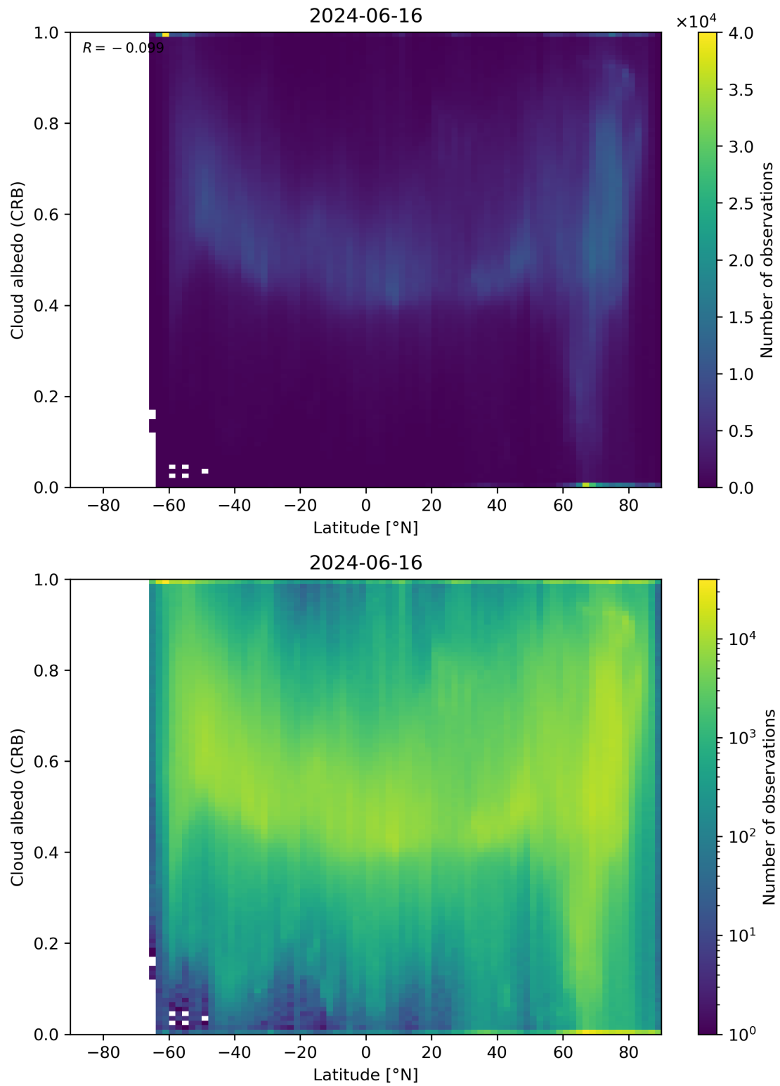
Figure 91: Scatter density plot of “Latitude” against “Cloud albedo (CRB)” for 2024-06-15 to 2024-06-17.
