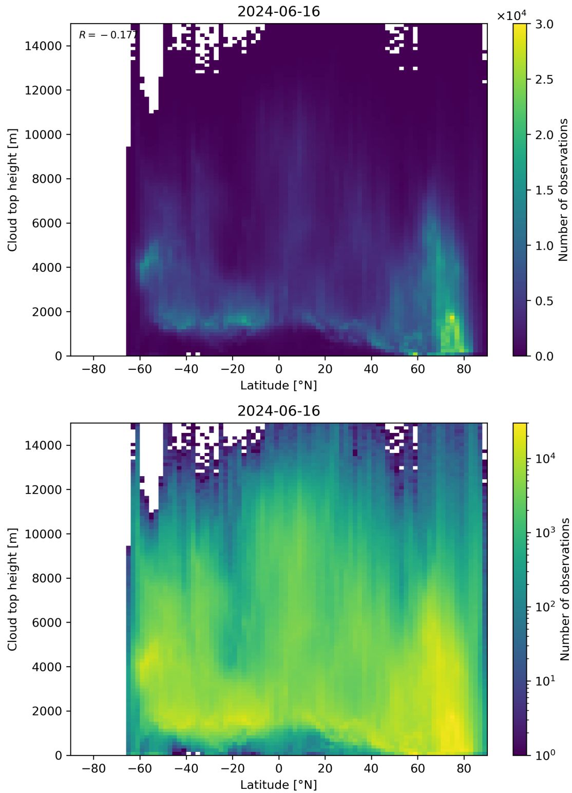
Figure 97: Scatter density plot of “Latitude” against “Cloud top height” for 2024-06-15 to 2024-06-17.
