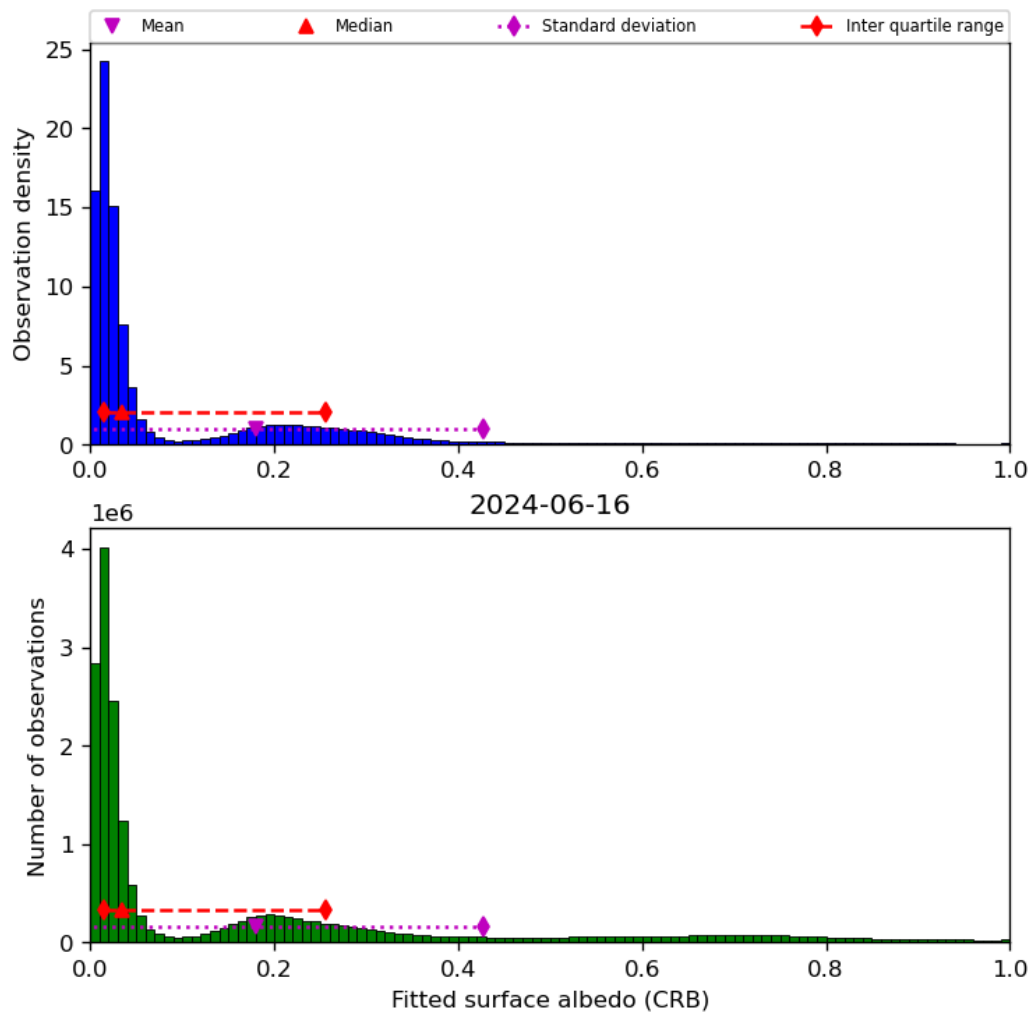
Figure 46: Histogram of “Fitted surface albedo (CRB)” for 2024-06-15 to 2024-06-17
