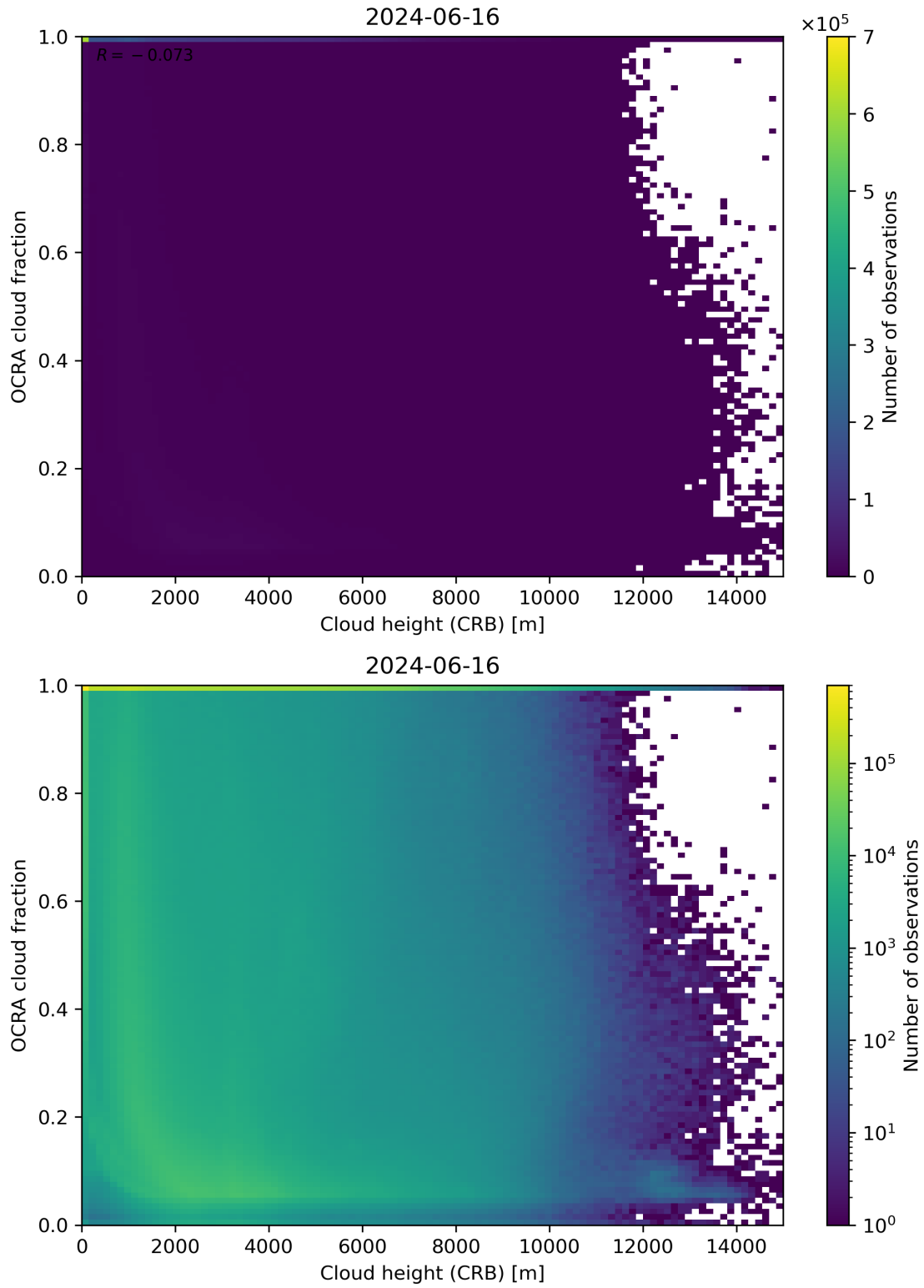
Figure 81: Scatter density plot of “Cloud height (CRB)” against “OCRA cloud fraction” for 2024-06-15 to 2024-06-17.
