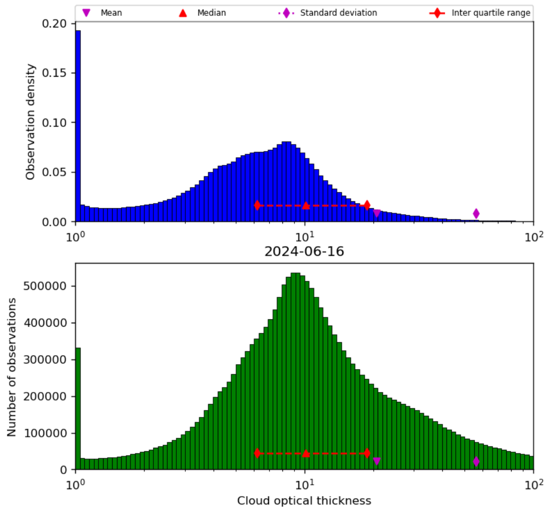
Figure 41: Histogram of “Cloud optical thickness” for 2024-06-15 to 2024-06-17
