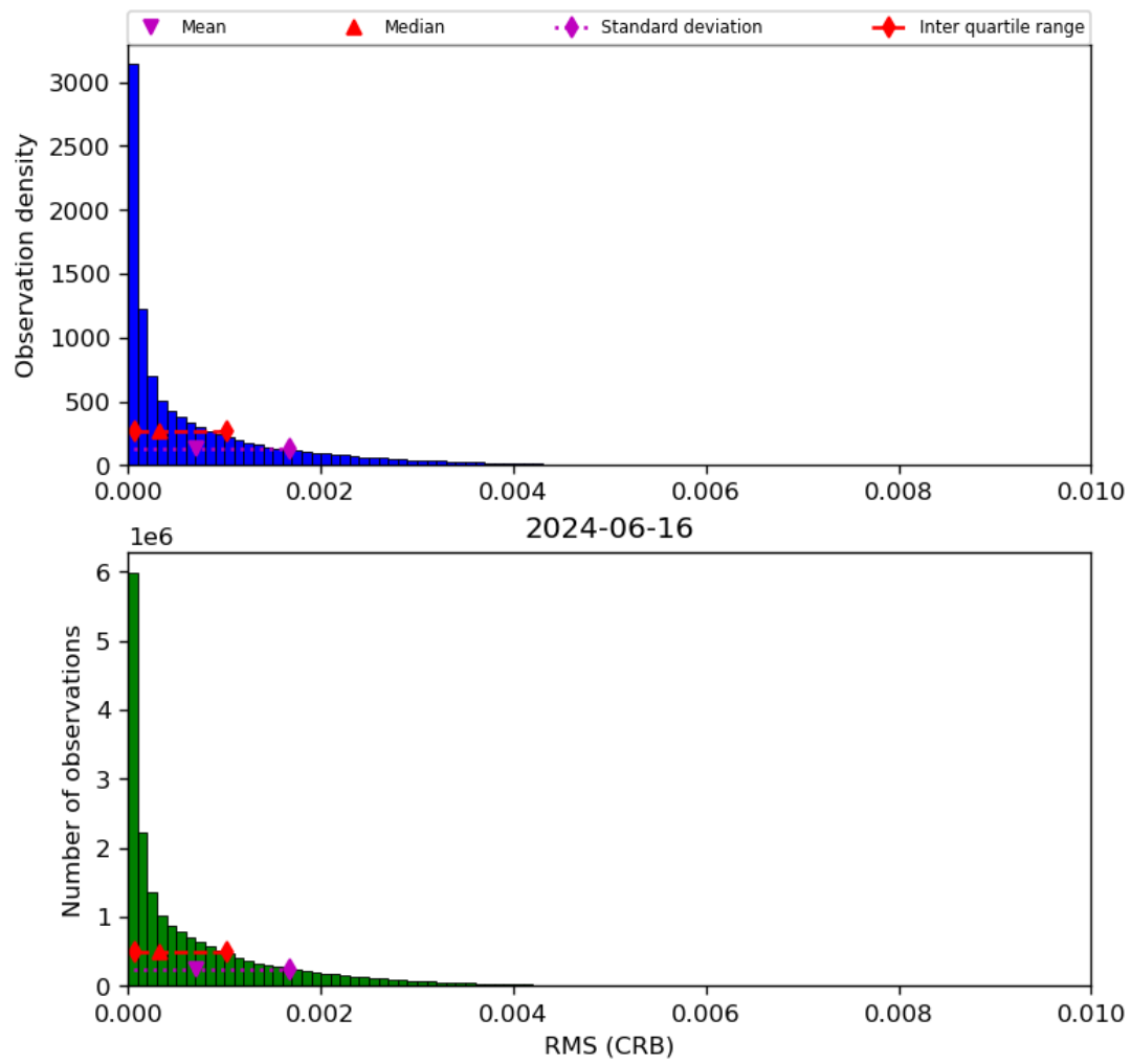
Figure 48: Histogram of “RMS (CRB)” for 2024-06-15 to 2024-06-17
