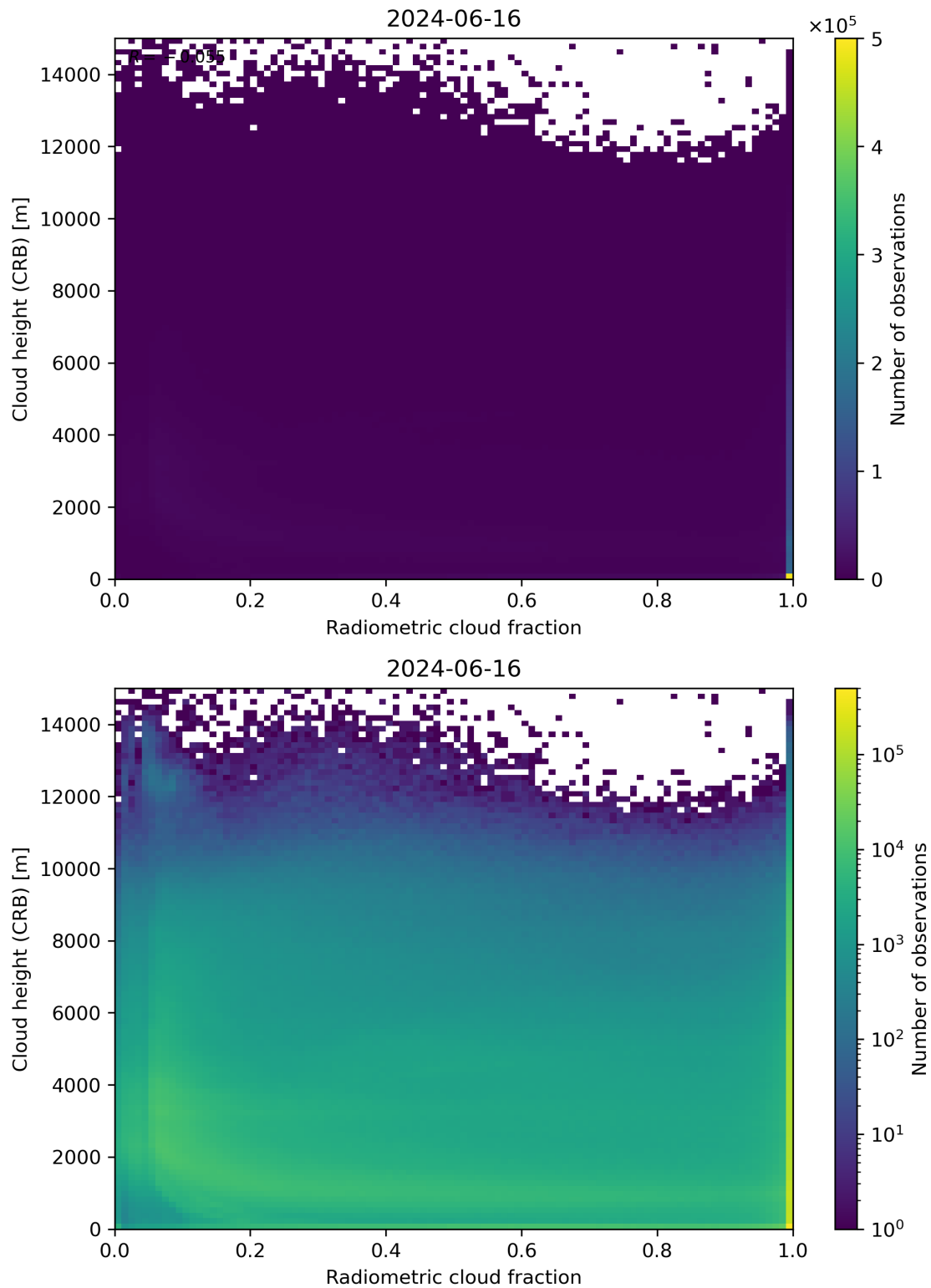
Figure 74: Scatter density plot of “Radiometric cloud fraction” against “Cloud height (CRB)” for 2024-06-15 to 2024-06-17.
