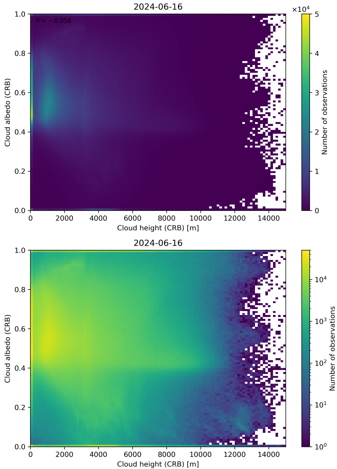
Figure 80: Scatter density plot of “Cloud height (CRB)” against “Cloud albedo (CRB)” for 2024-06-15 to 2024-06-17.
