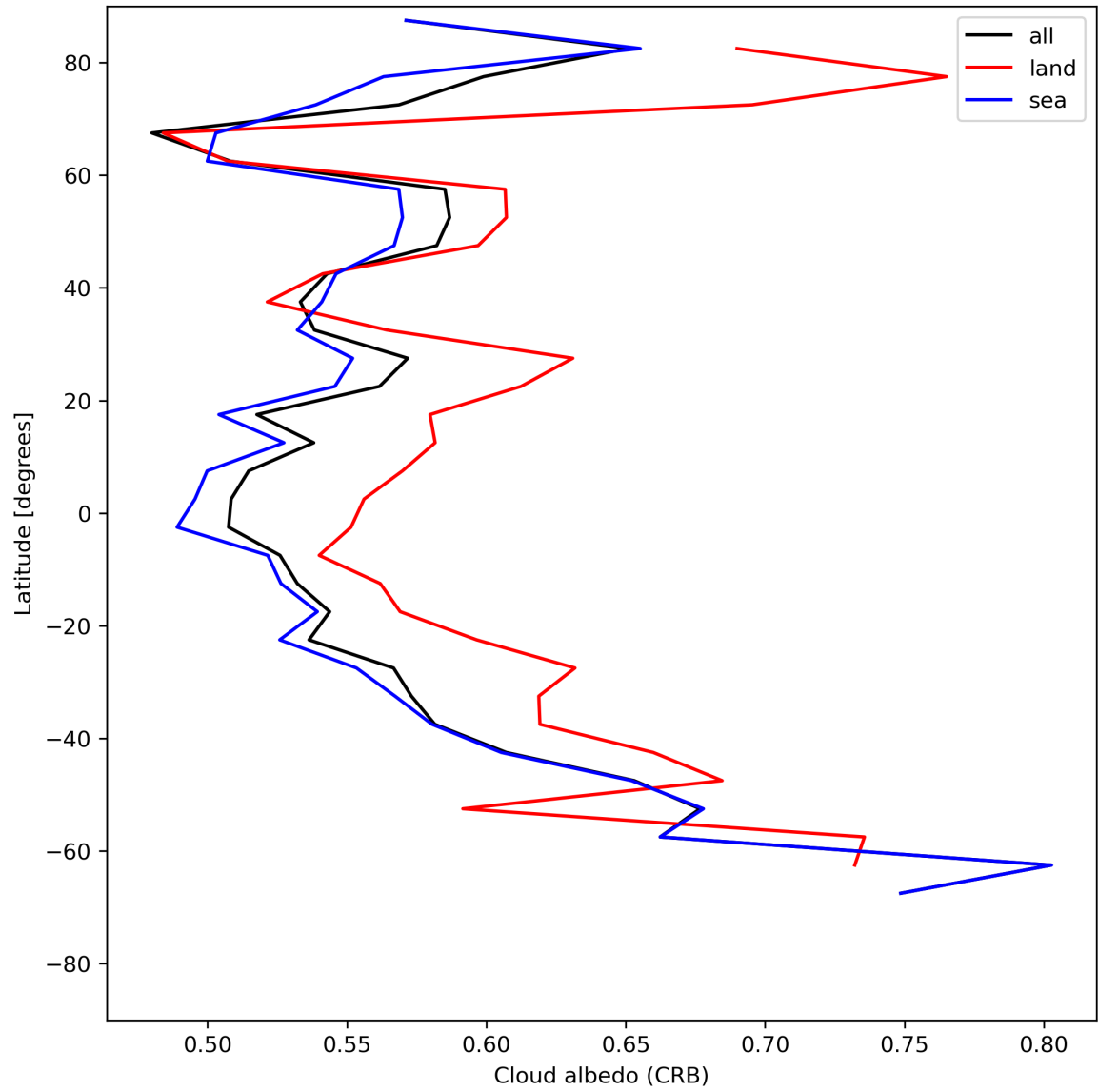
Figure 28: Zonal average of “Cloud albedo (CRB)” for 2024-06-15 to 2024-06-17.
