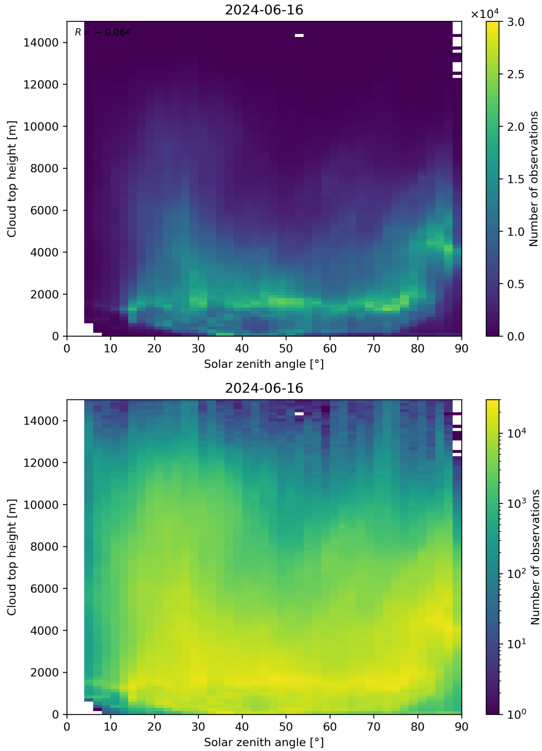
Figure 104: Scatter density plot of “Solar zenith angle” against “Cloud top height” for 2024-06-15 to 2024-06-17.
