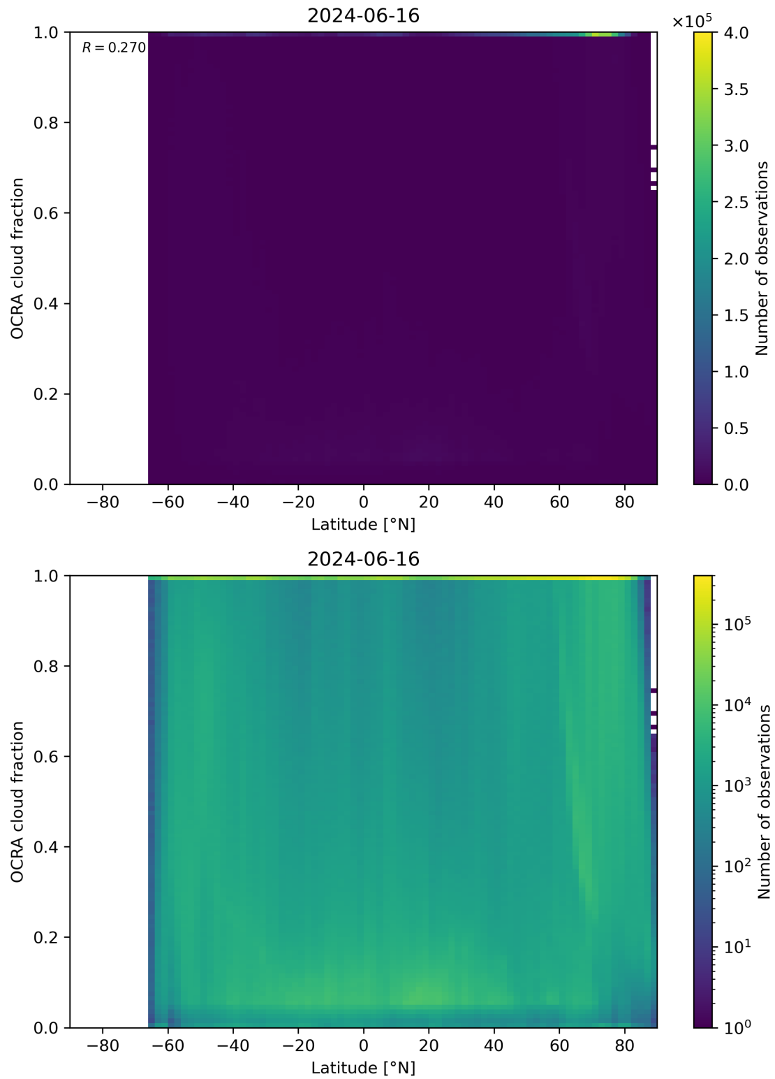
Figure 93: Scatter density plot of “Latitude” against “OCRA cloud fraction” for 2024-06-15 to 2024-06-17.
