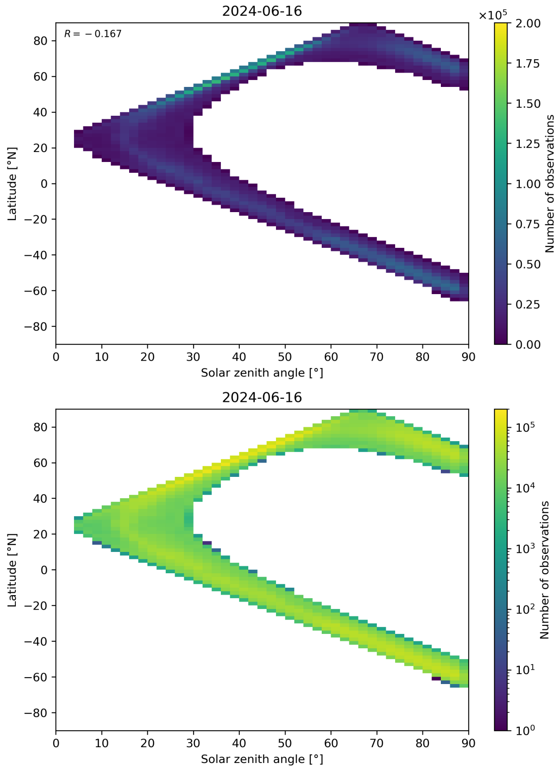
Figure 105: Scatter density plot of “Solar zenith angle” against “Latitude” for 2024-06-15 to 2024-06-17.
