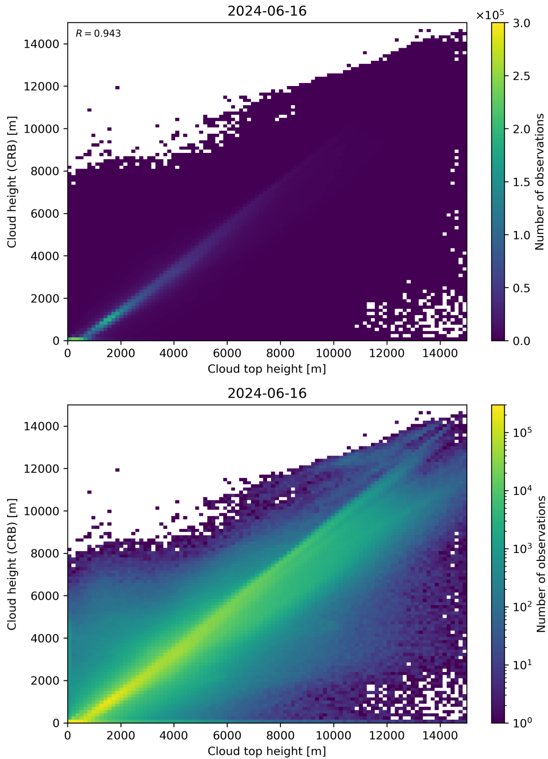
Figure 89: Scatter density plot of “Cloud top height” against “Cloud height (CRB)” for 2024-06-15 to 2024-06-17.
