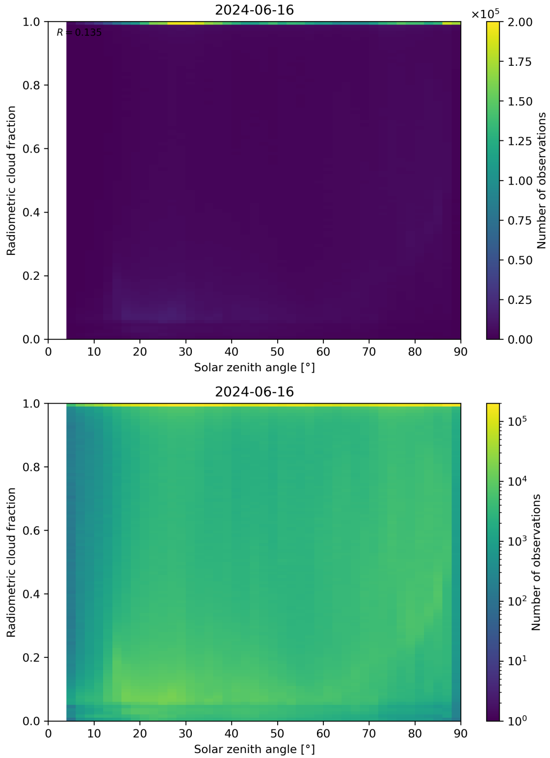
Figure 99: Scatter density plot of “Solar zenith angle” against “Radiometric cloud fraction” for 2024-06-15 to 2024-06-17.
