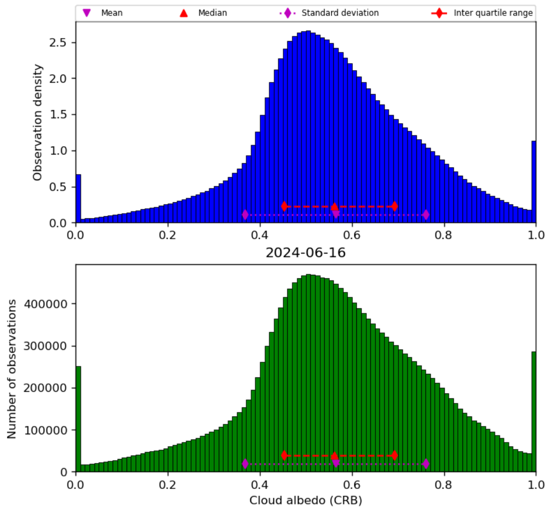
Figure 44: Histogram of “Cloud albedo (CRB)” for 2024-06-15 to 2024-06-17
