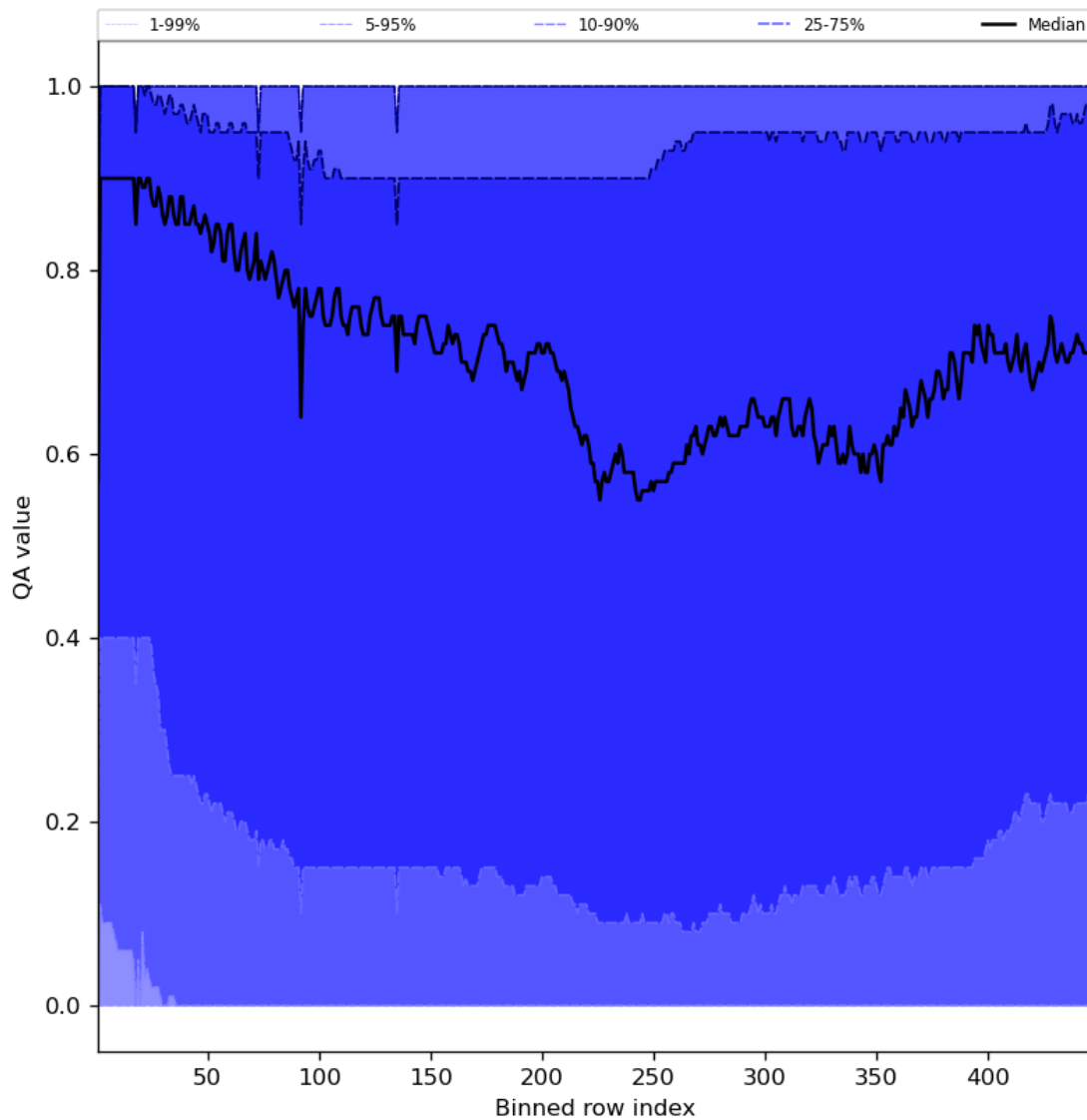
Figure 54: Along track statistics of "QA value" for 2024-06-15 to 2024-06-17
