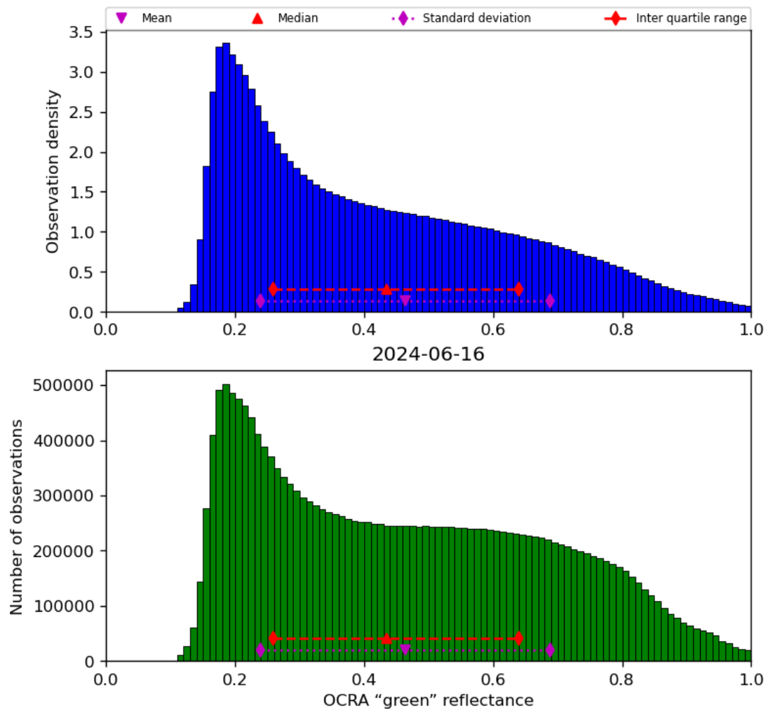
Figure 52: Histogram of “OCRA “green” reflectance” for 2024-06-15 to 2024-06-17
