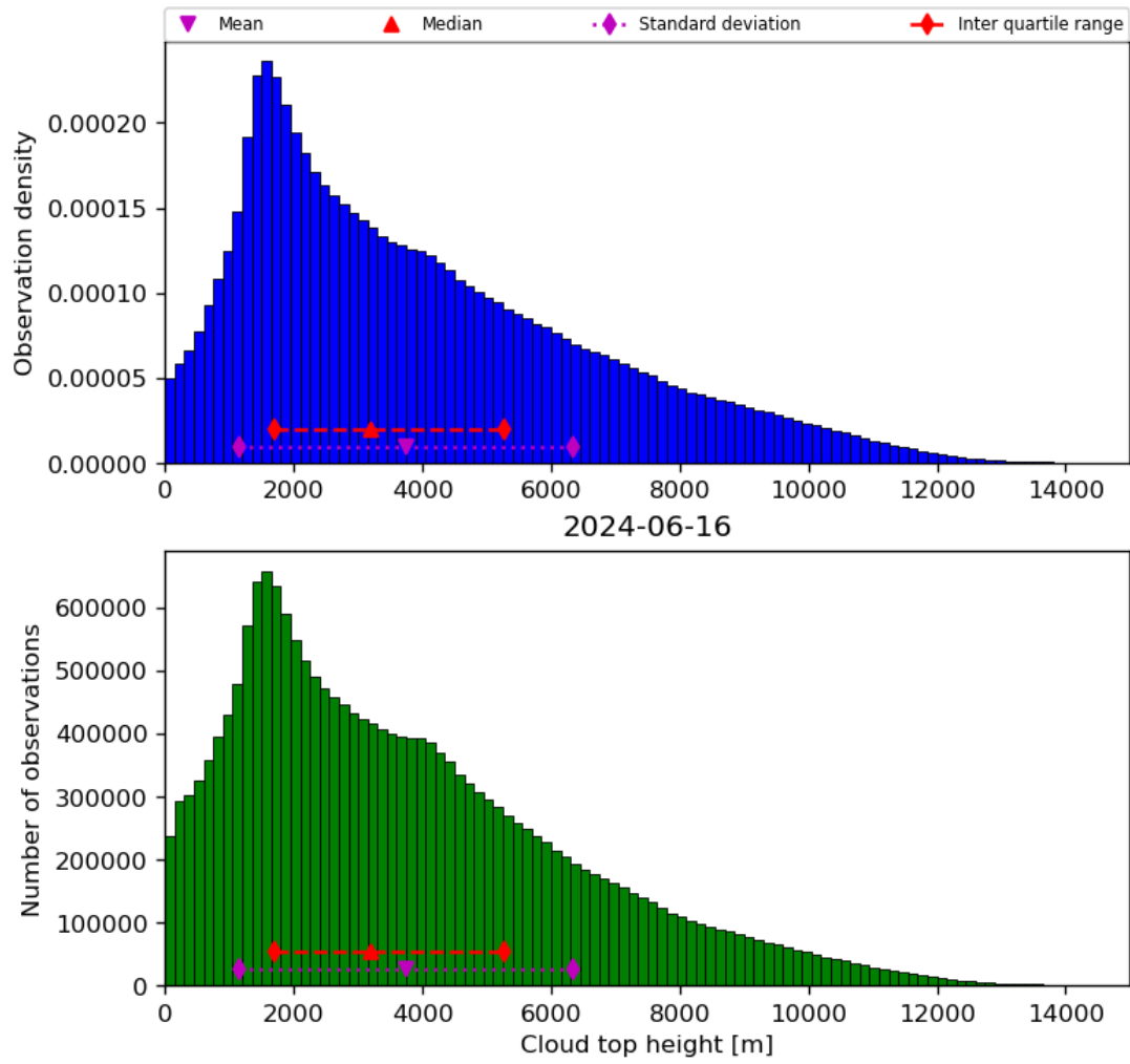
Figure 40: Histogram of “Cloud top height” for 2024-06-15 to 2024-06-17
