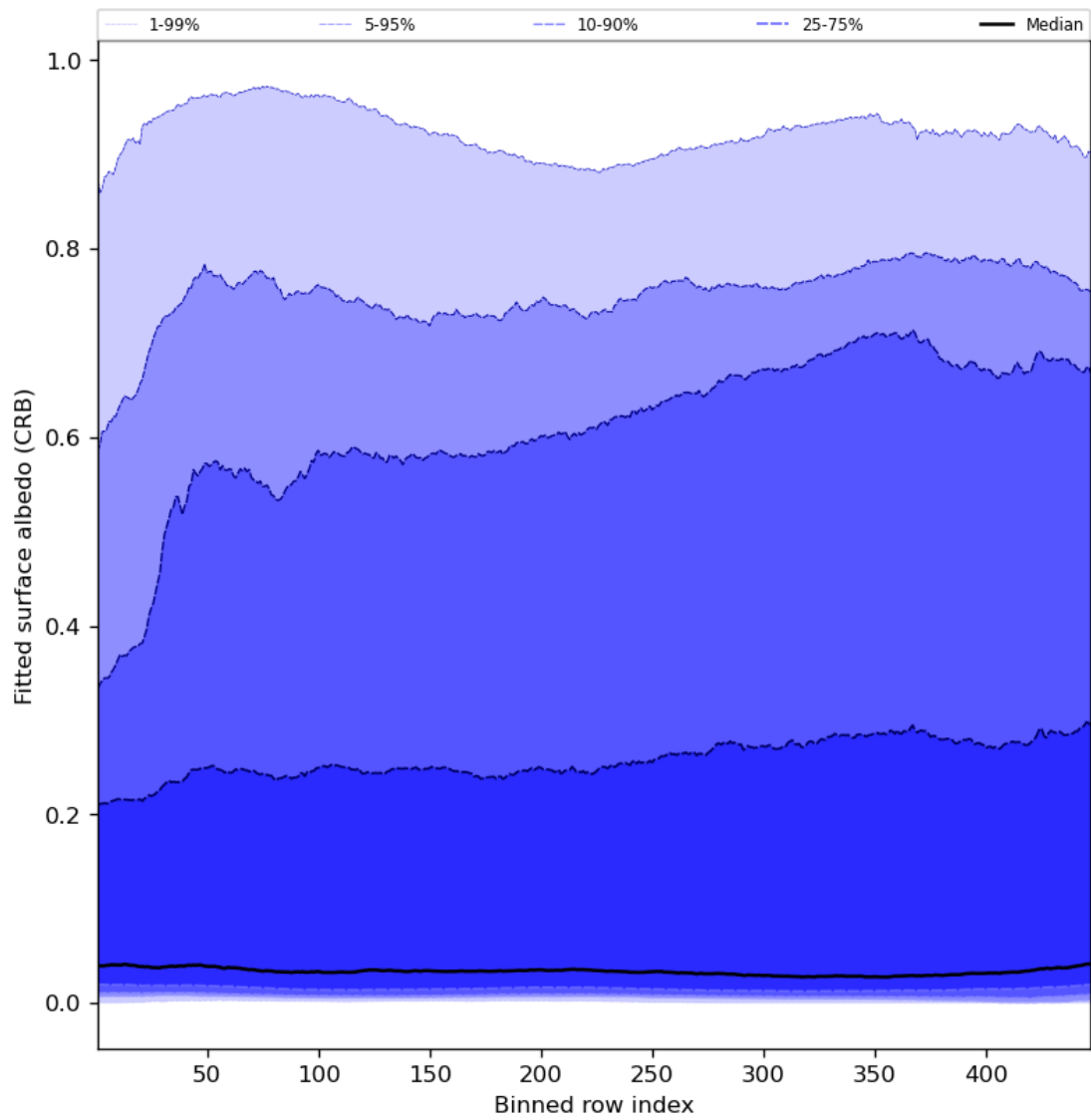
Figure 62: Along track statistics of “Fitted surface albedo (CRB)” for 2024-06-15 to 2024-06-17
