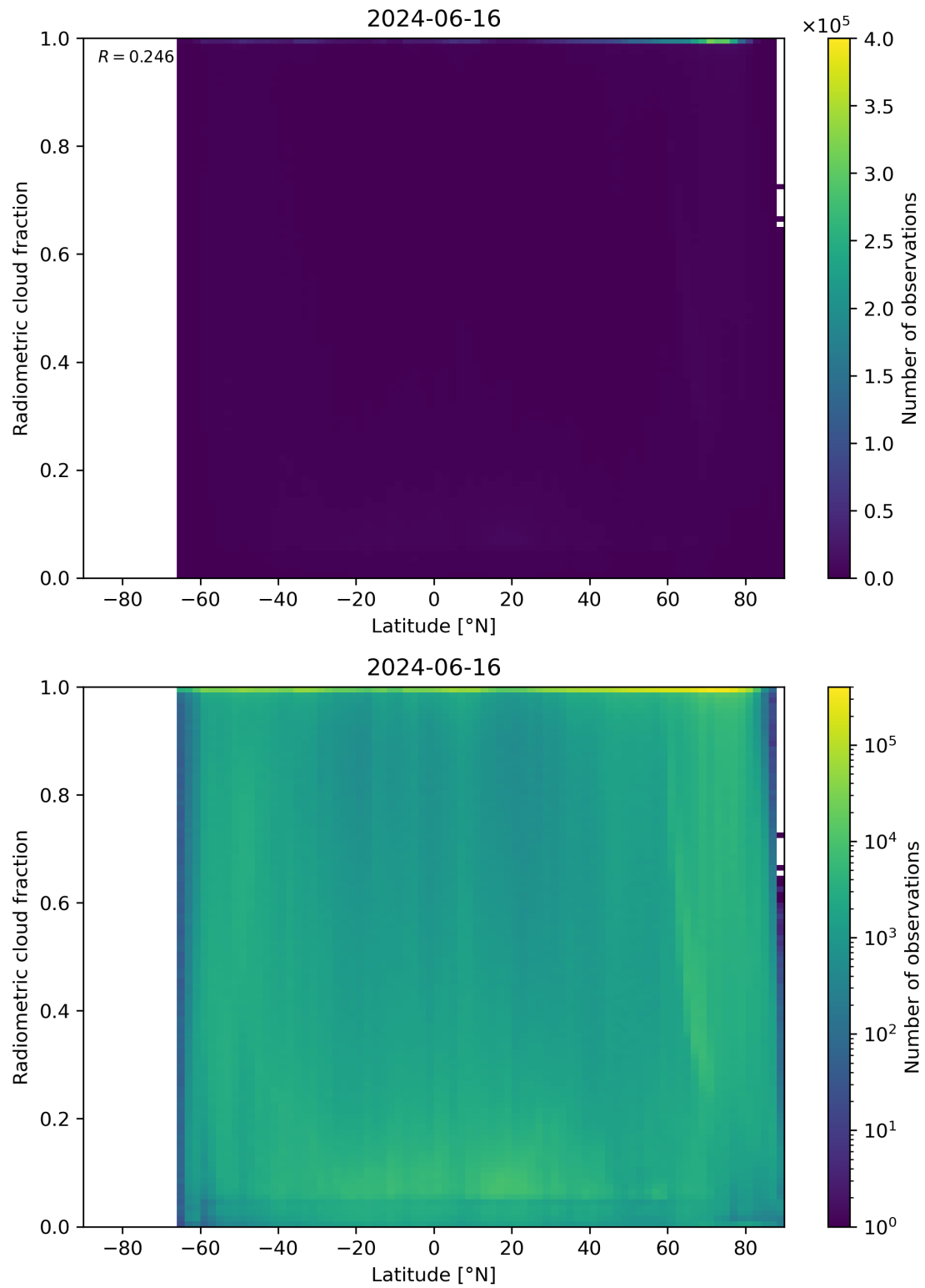
Figure 92: Scatter density plot of “Latitude” against “Radiometric cloud fraction” for 2024-06-15 to 2024-06-17.
