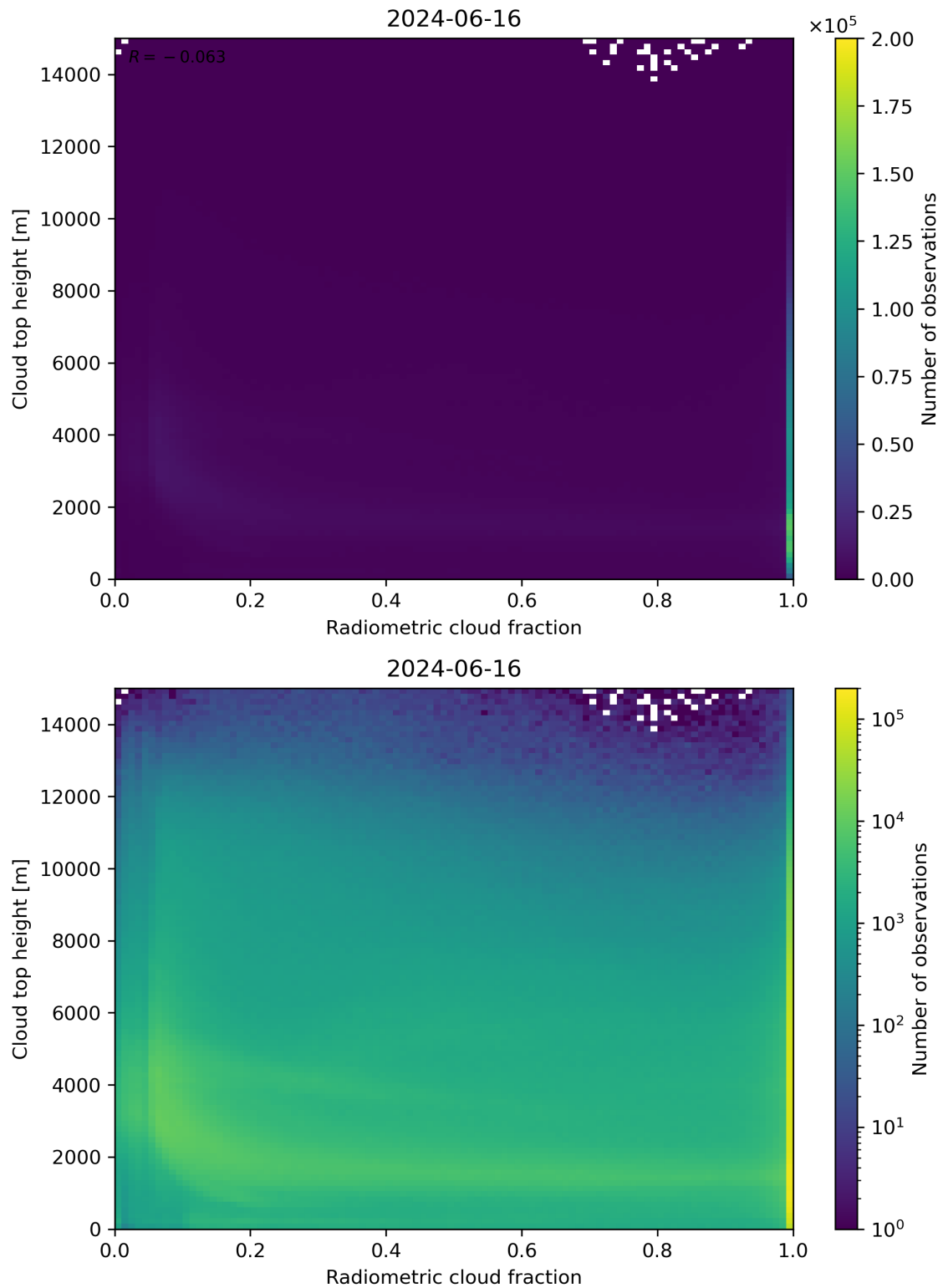
Figure 76: Scatter density plot of “Radiometric cloud fraction” against “Cloud top height” for 2024-06-15 to 2024-06-17.
