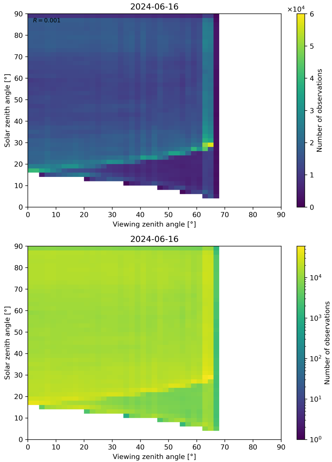
Figure 114: Scatter density plot of “Viewing zenith angle” against “Solar zenith angle” for 2024-06-15 to 2024-06-17.
