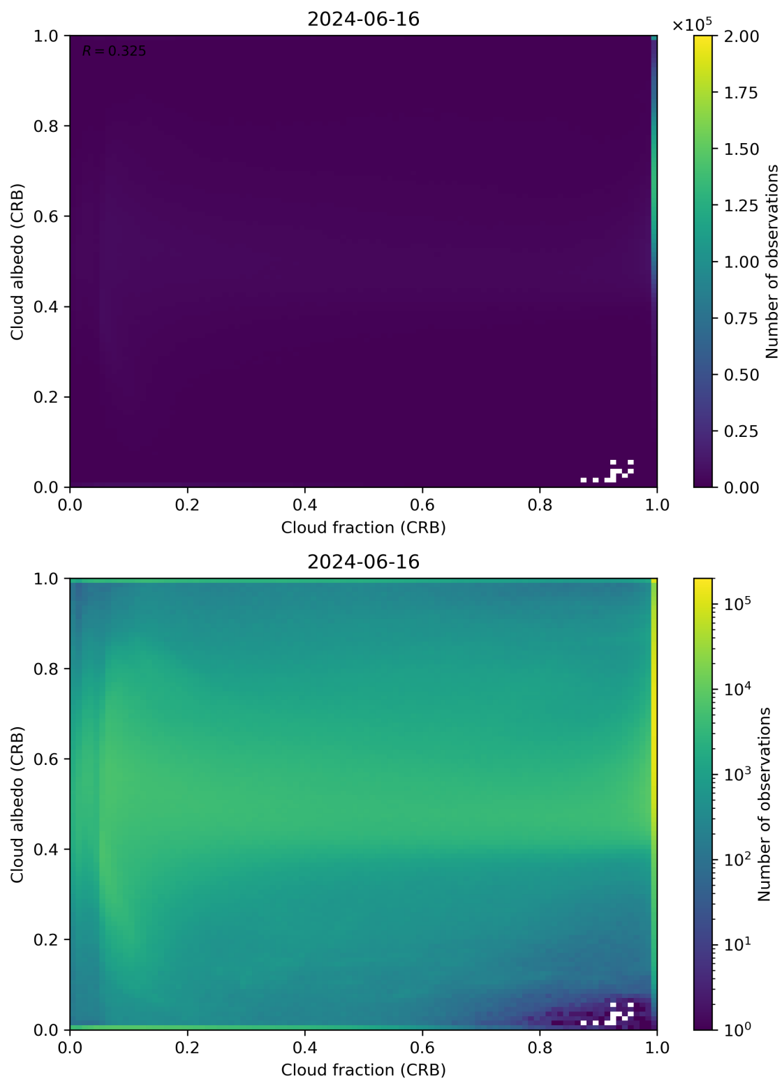
Figure 77: Scatter density plot of “Cloud fraction (CRB)” against “Cloud albedo (CRB)” for 2024-06-15 to 2024-06-17.
