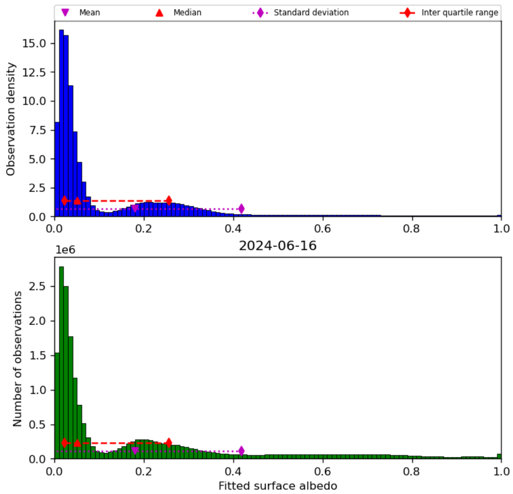
Figure 45: Histogram of “Fitted surface albedo” for 2024-06-15 to 2024-06-17
