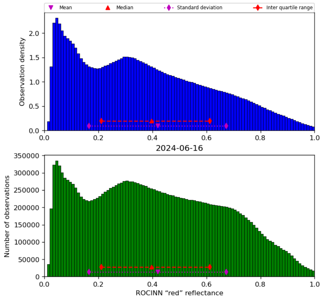
Figure 53: Histogram of “ROCINN “red” reflectance” for 2024-06-15 to 2024-06-17
