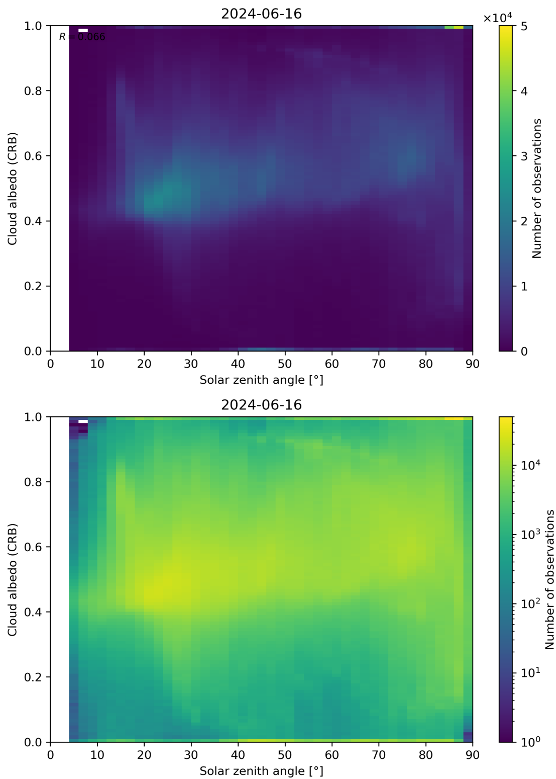
Figure 98: Scatter density plot of “Solar zenith angle” against “Cloud albedo (CRB)” for 2024-06-15 to 2024-06-17.
