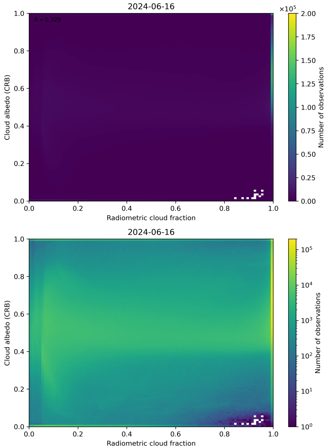
Figure 71: Scatter density plot of “Radiometric cloud fraction” against “Cloud albedo (CRB)” for 2024-06-15 to 2024-06-17.
