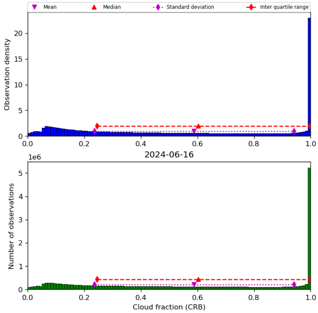
Figure 42: Histogram of “Cloud fraction (CRB)” for 2024-06-15 to 2024-06-17
