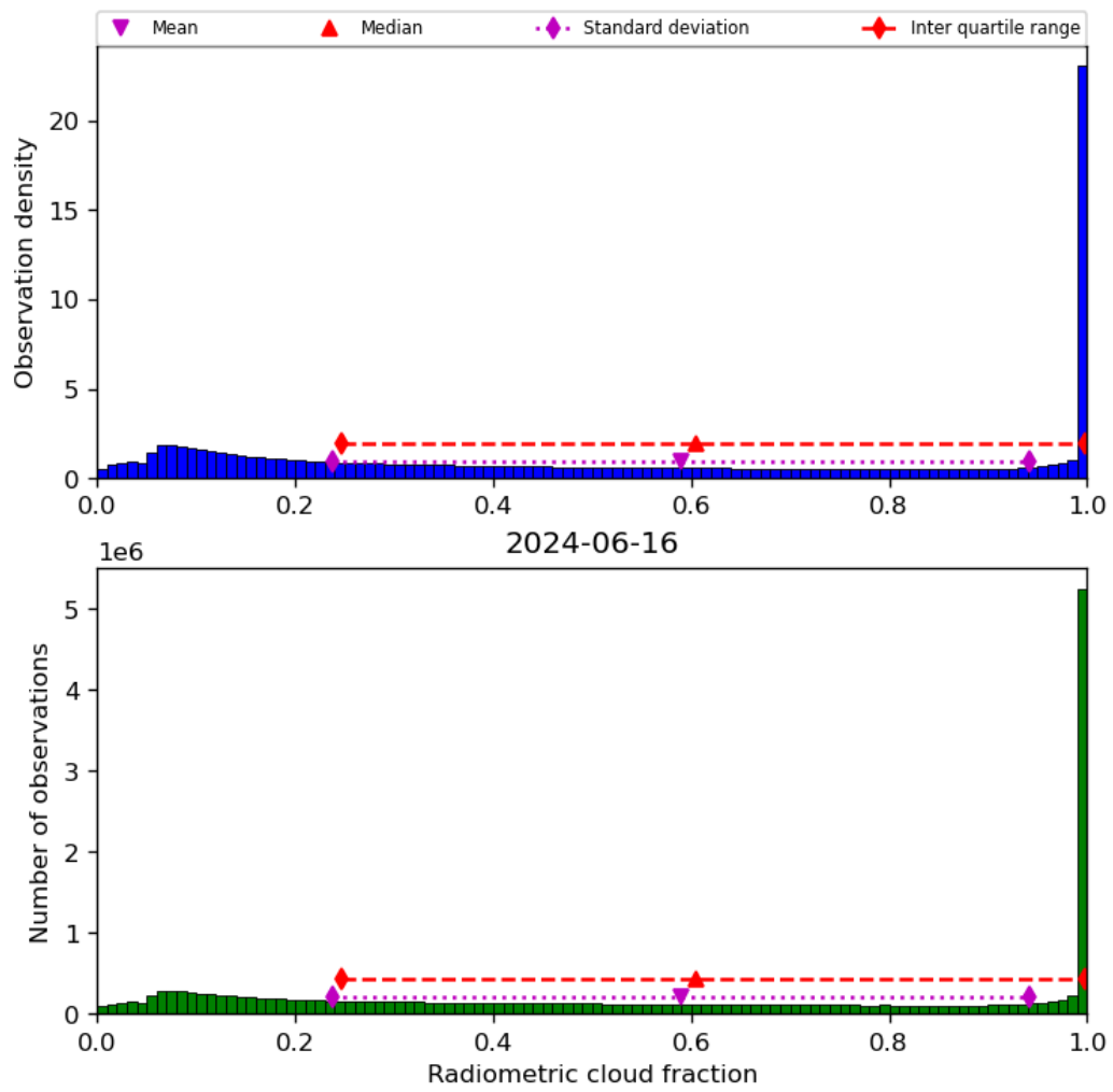
Figure 39: Histogram of “Radiometric cloud fraction” for 2024-06-15 to 2024-06-17
