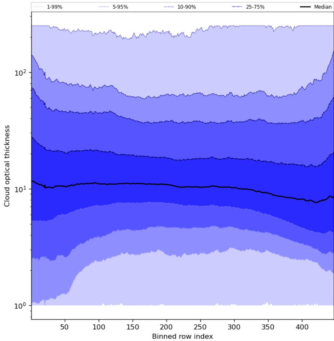
Figure 57: Along track statistics of “Cloud optical thickness” for 2024-06-15 to 2024-06-17
