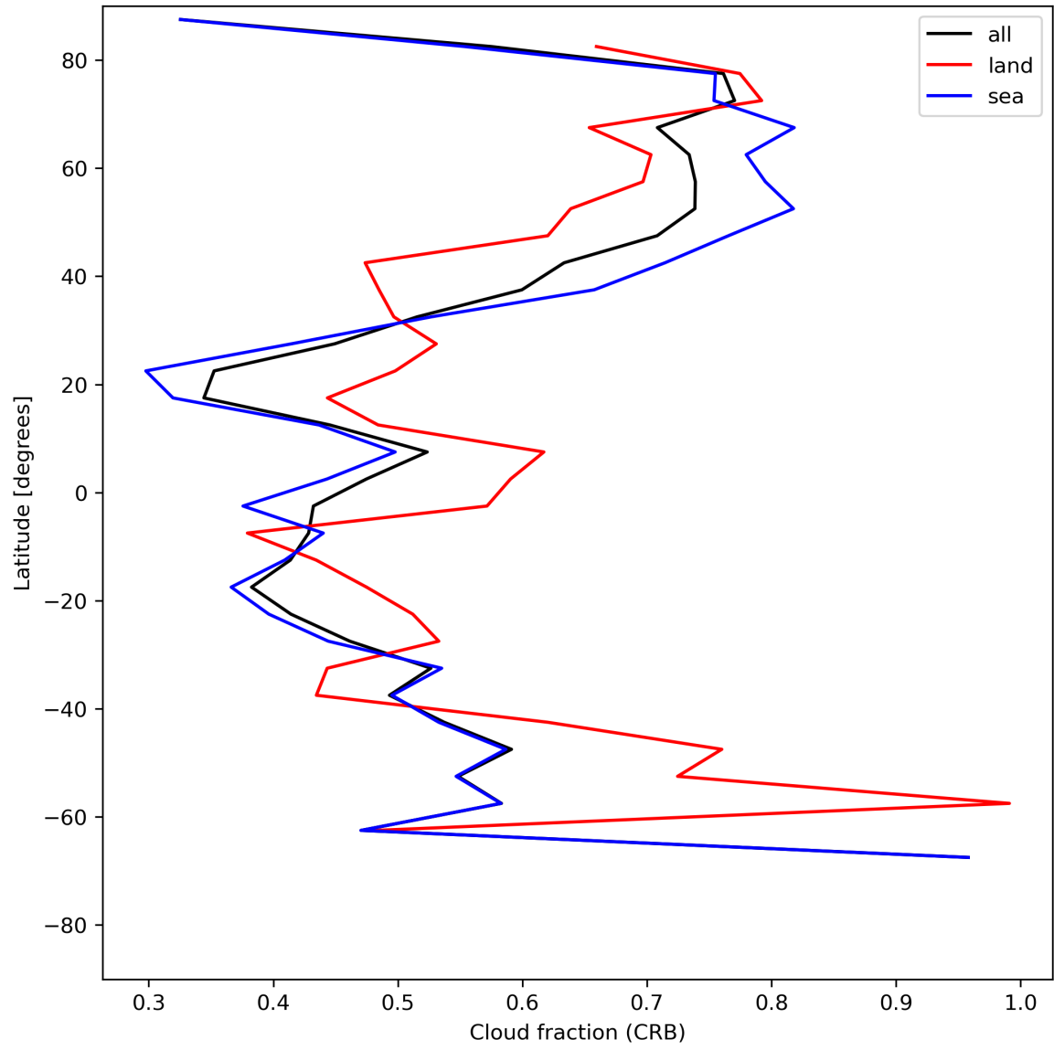
Figure 26: Zonal average of “Cloud fraction (CRB)” for 2024-06-15 to 2024-06-17.
