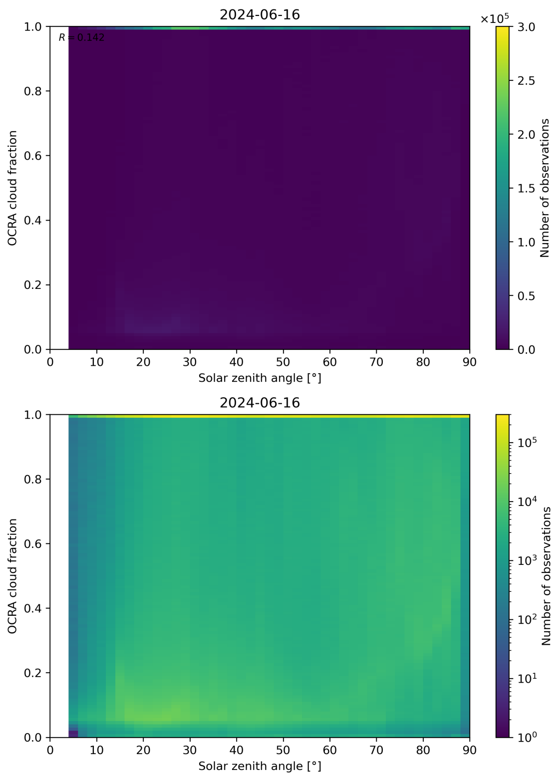
Figure 100: Scatter density plot of “Solar zenith angle” against “OCRA cloud fraction” for 2024-06-15 to 2024-06-17.
