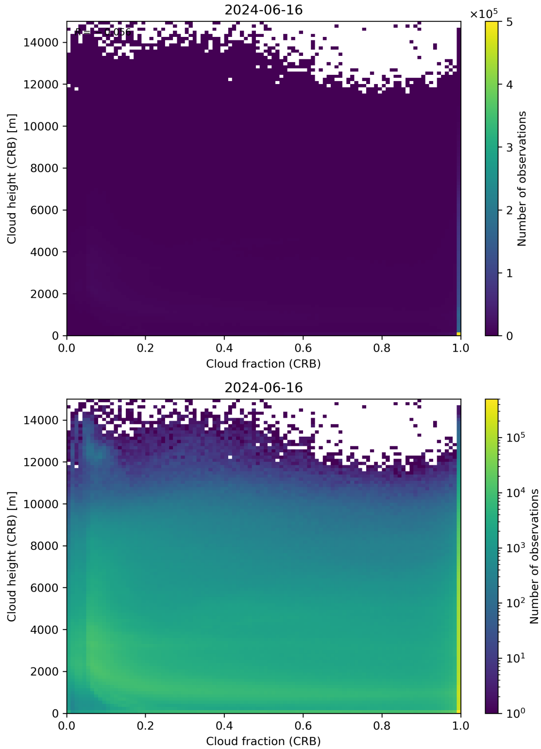
Figure 79: Scatter density plot of “Cloud fraction (CRB)” against “Cloud height (CRB)” for 2024-06-15 to 2024-06-17.
