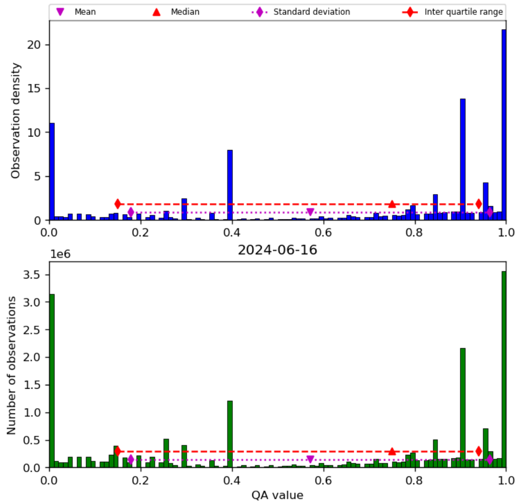
Figure 38: Histogram of “QA value” for 2024-06-15 to 2024-06-17
