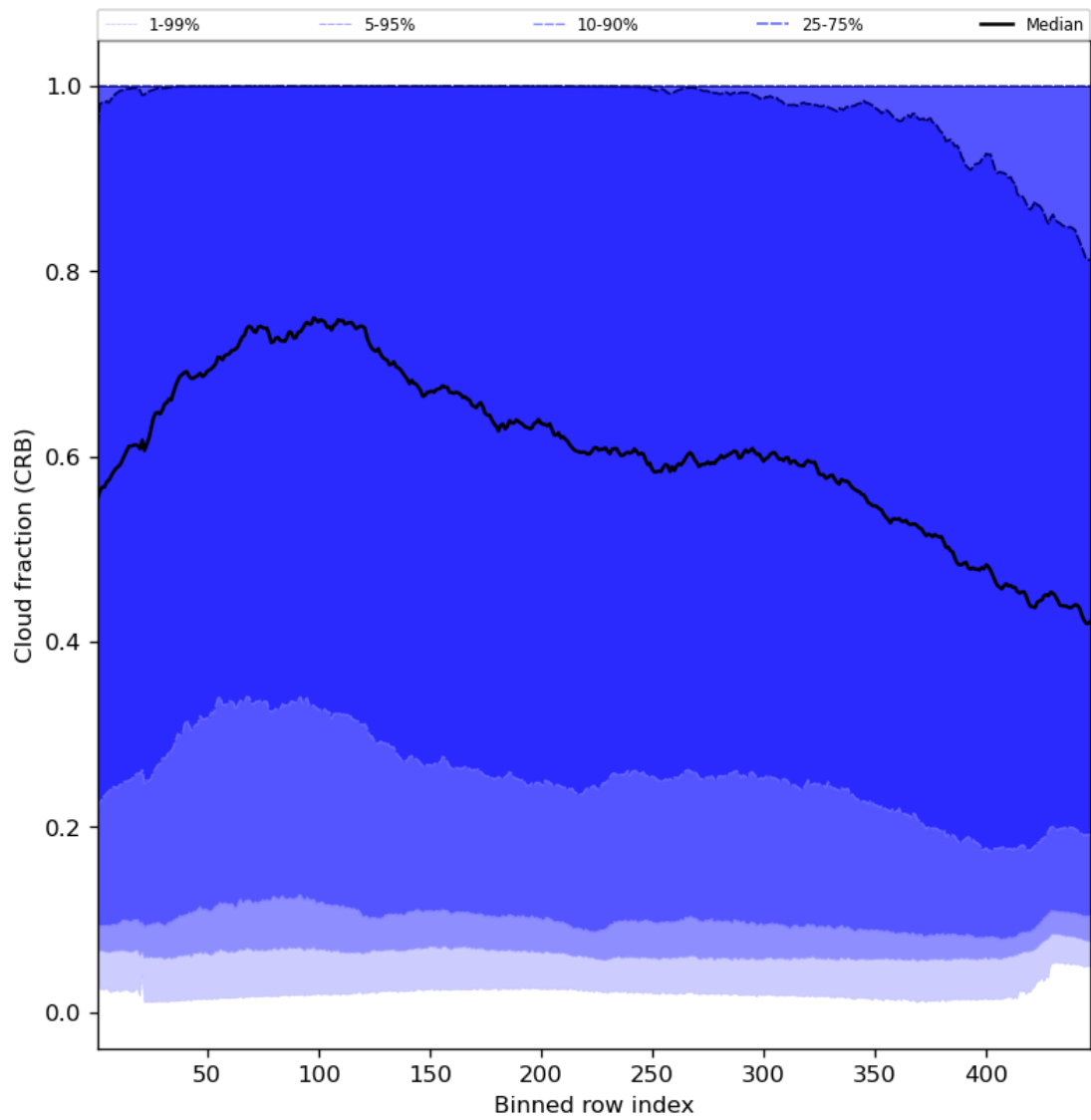
Figure 58: Along track statistics of “Cloud fraction (CRB)” for 2024-06-15 to 2024-06-17
