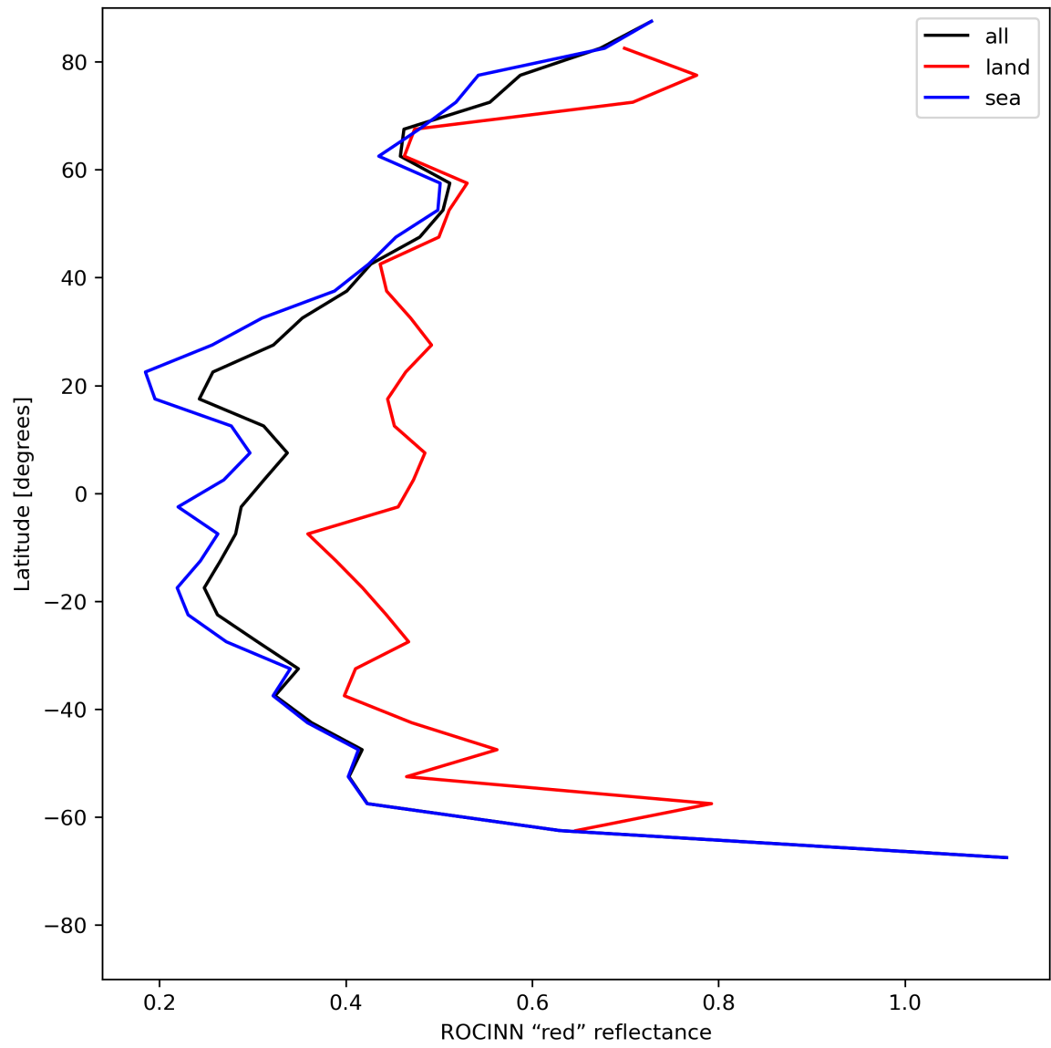
Figure 37: Zonal average of “ROCINN “red” reflectance” for 2024-06-15 to 2024-06-17.
