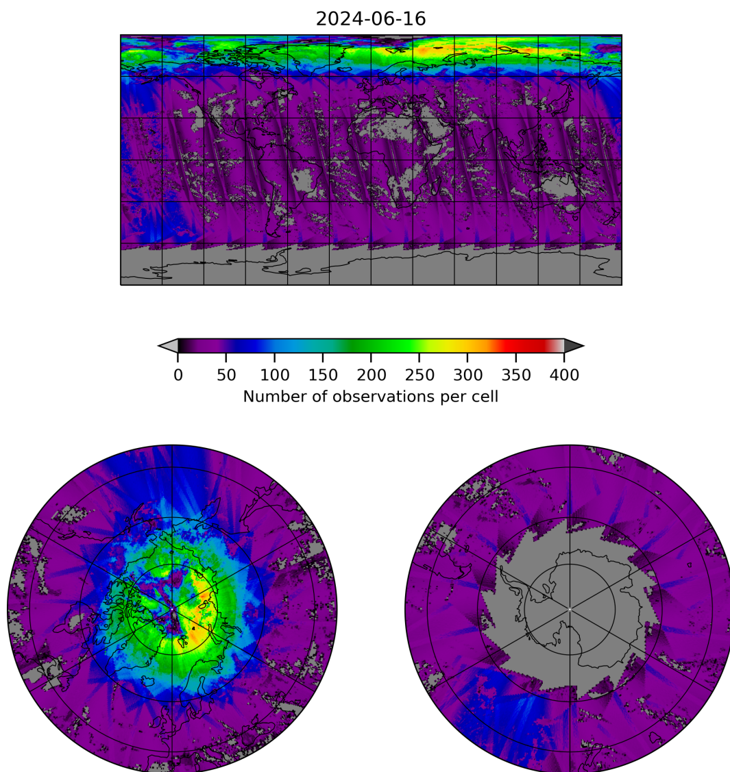
Figure 21: Map of the number of observations for 2024-06-15 to 2024-06-17
