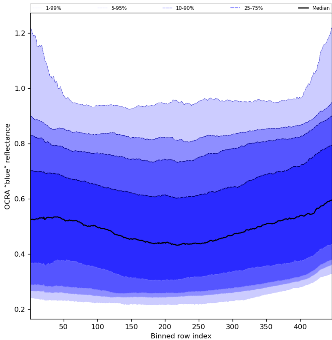
Figure 67: Along track statistics of “OCRA “blue” reflectance” for 2024-06-15 to 2024-06-17
