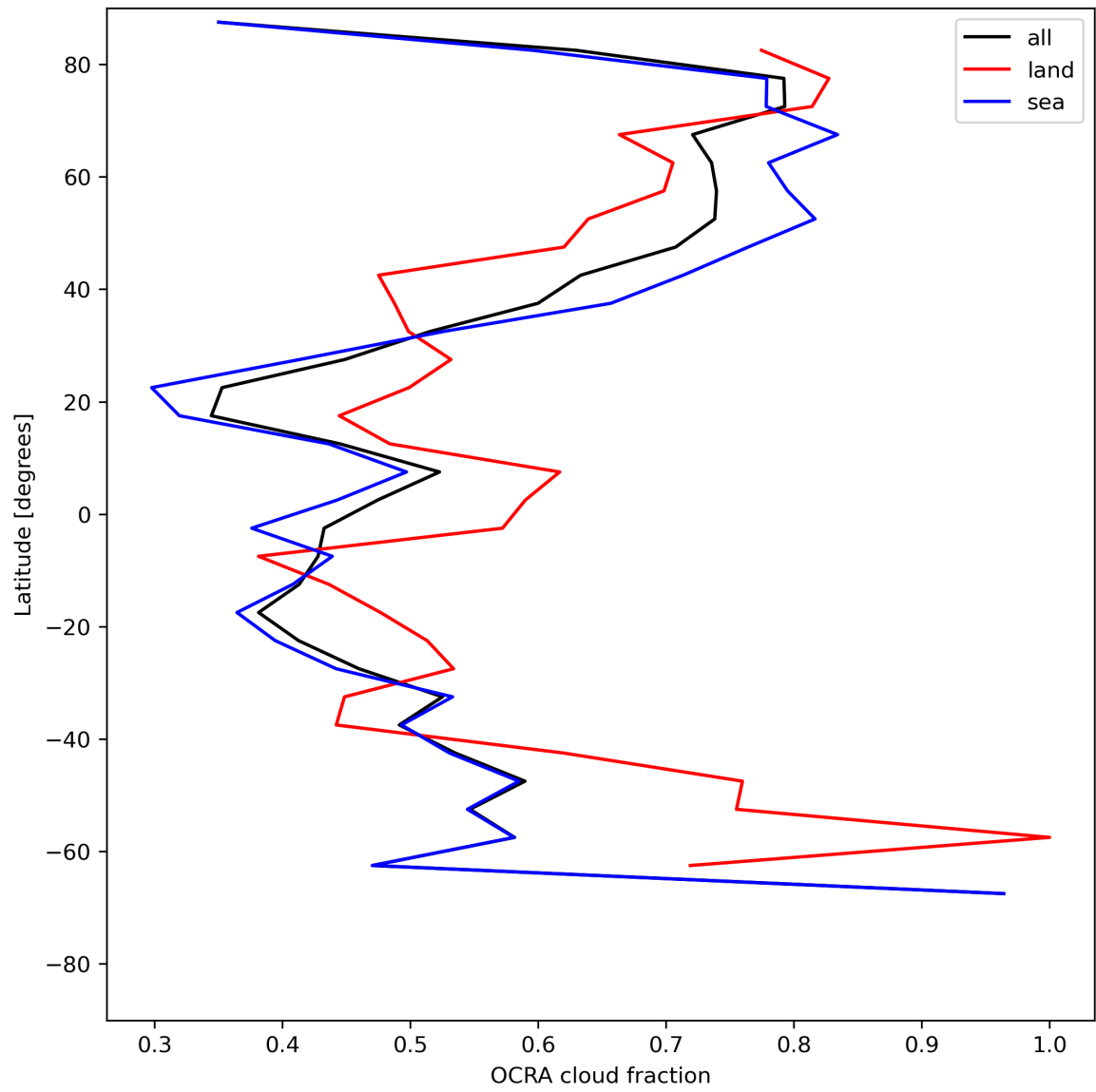
Figure 34: Zonal average of “OCRA cloud fraction” for 2024-06-15 to 2024-06-17.
