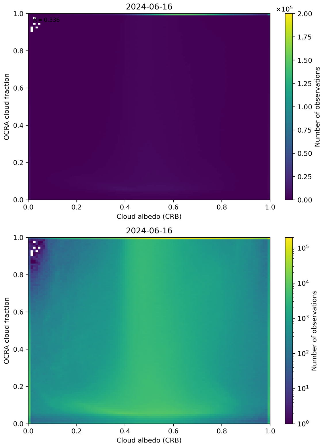
Figure 70: Scatter density plot of “Cloud albedo (CRB)” against “OCRA cloud fraction” for 2024-06-15 to 2024-06-17.
