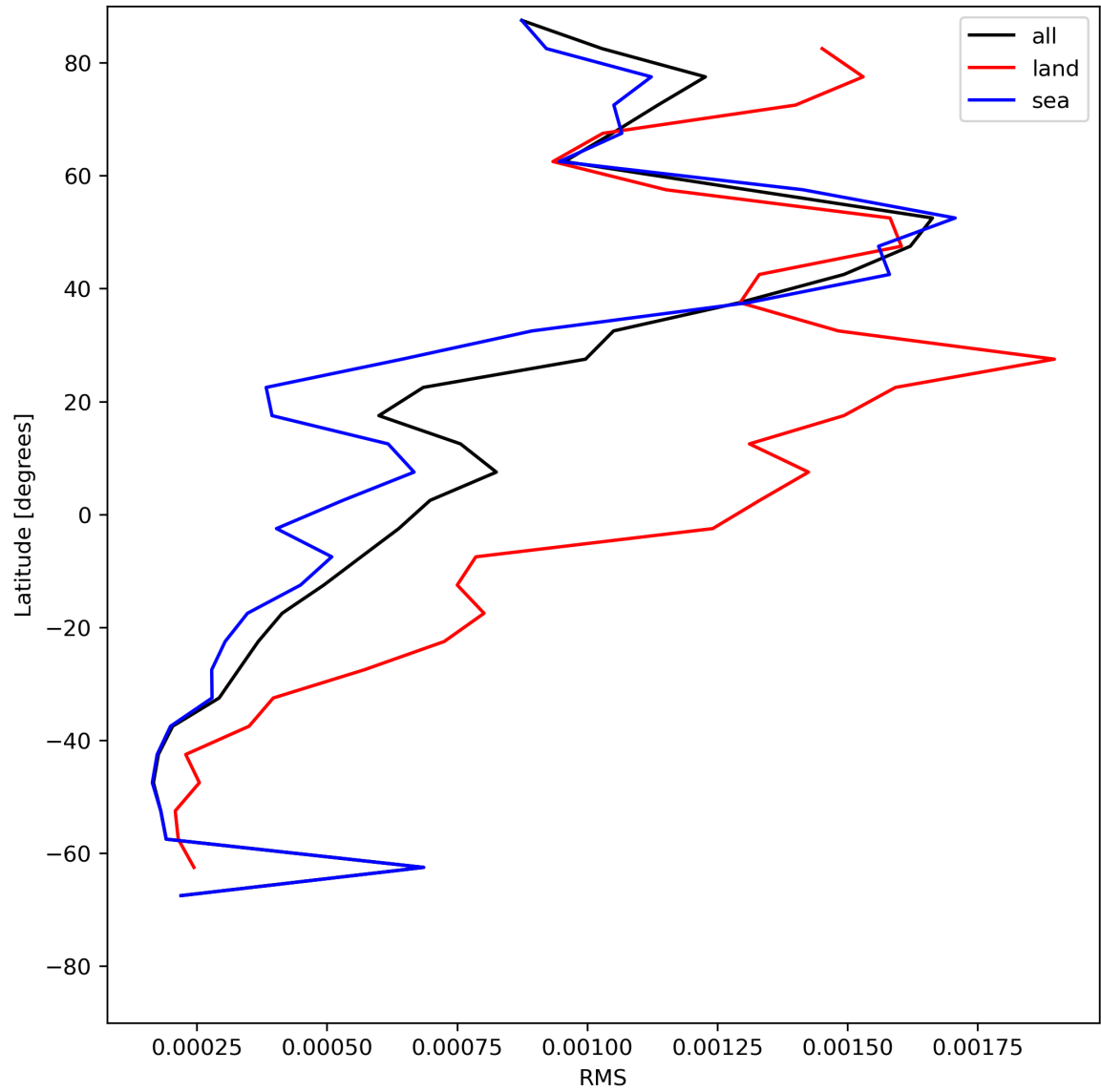
Figure 31: Zonal average of “RMS” for 2024-06-15 to 2024-06-17.
