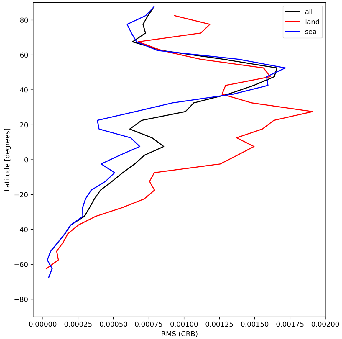
Figure 32: Zonal average of “RMS (CRB)” for 2024-06-15 to 2024-06-17.
