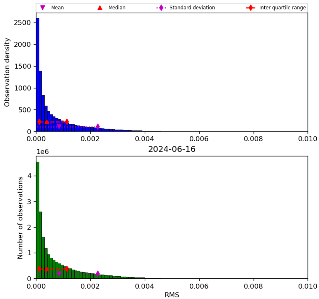
Figure 47: Histogram of “RMS” for 2024-06-15 to 2024-06-17
