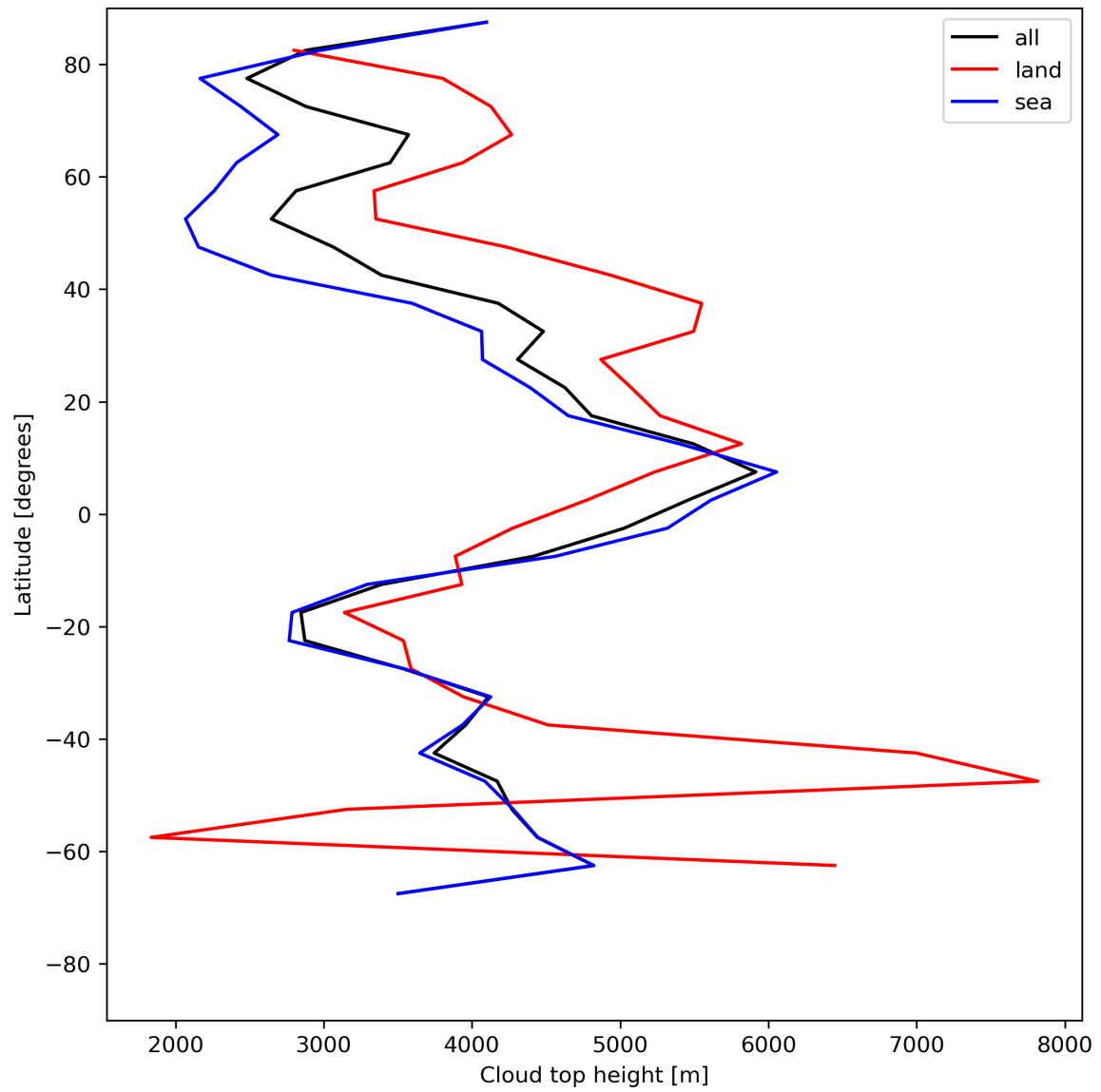
Figure 24: Zonal average of “Cloud top height” for 2024-06-15 to 2024-06-17.
