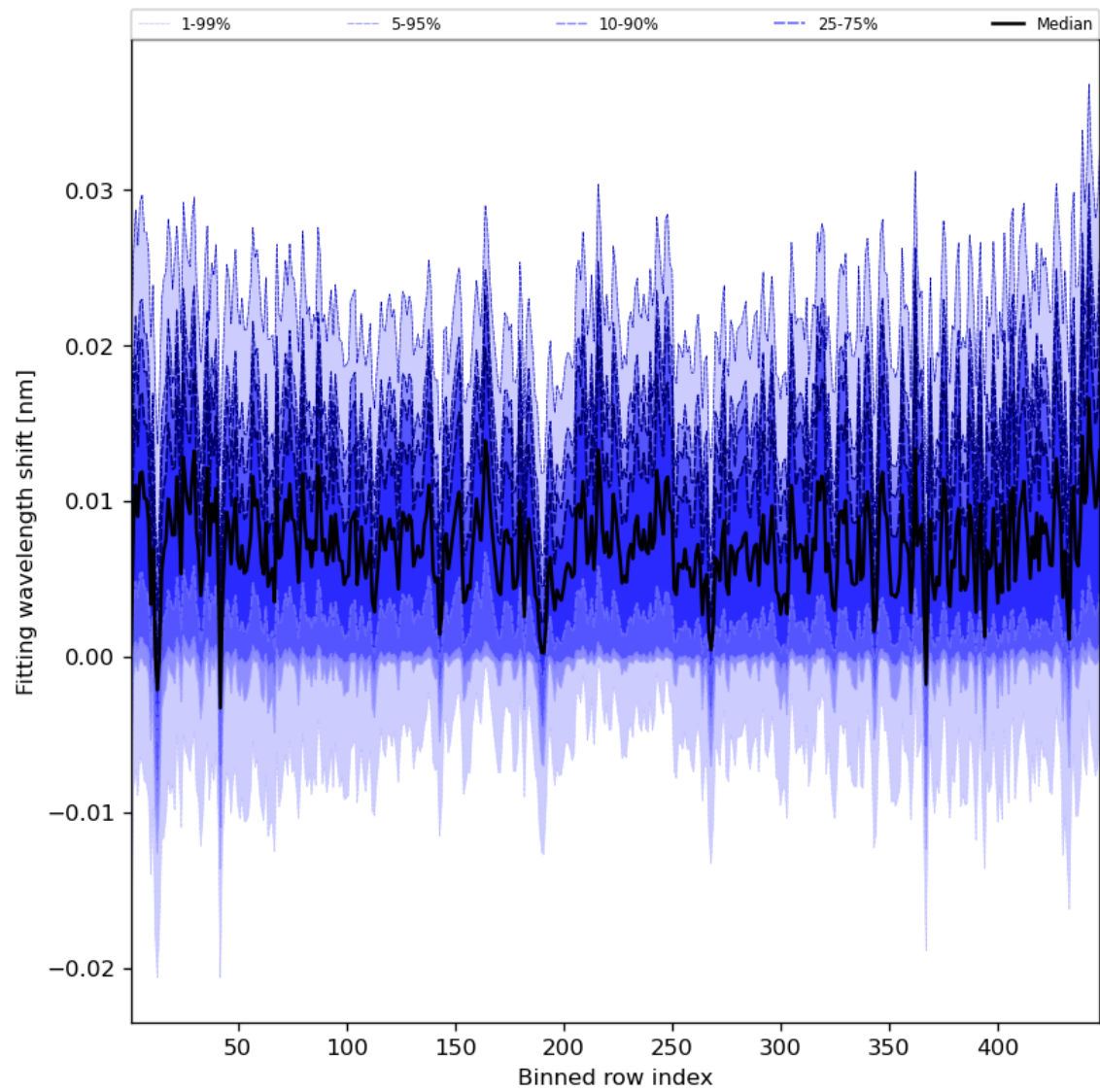
Figure 65: Along track statistics of “Fitting wavelength shift” for 2024-06-15 to 2024-06-17
