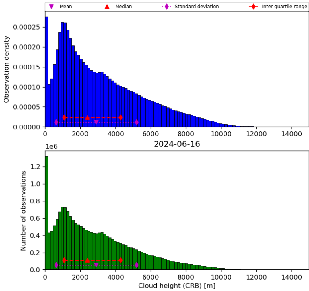
Figure 43: Histogram of “Cloud height (CRB)” for 2024-06-15 to 2024-06-17
