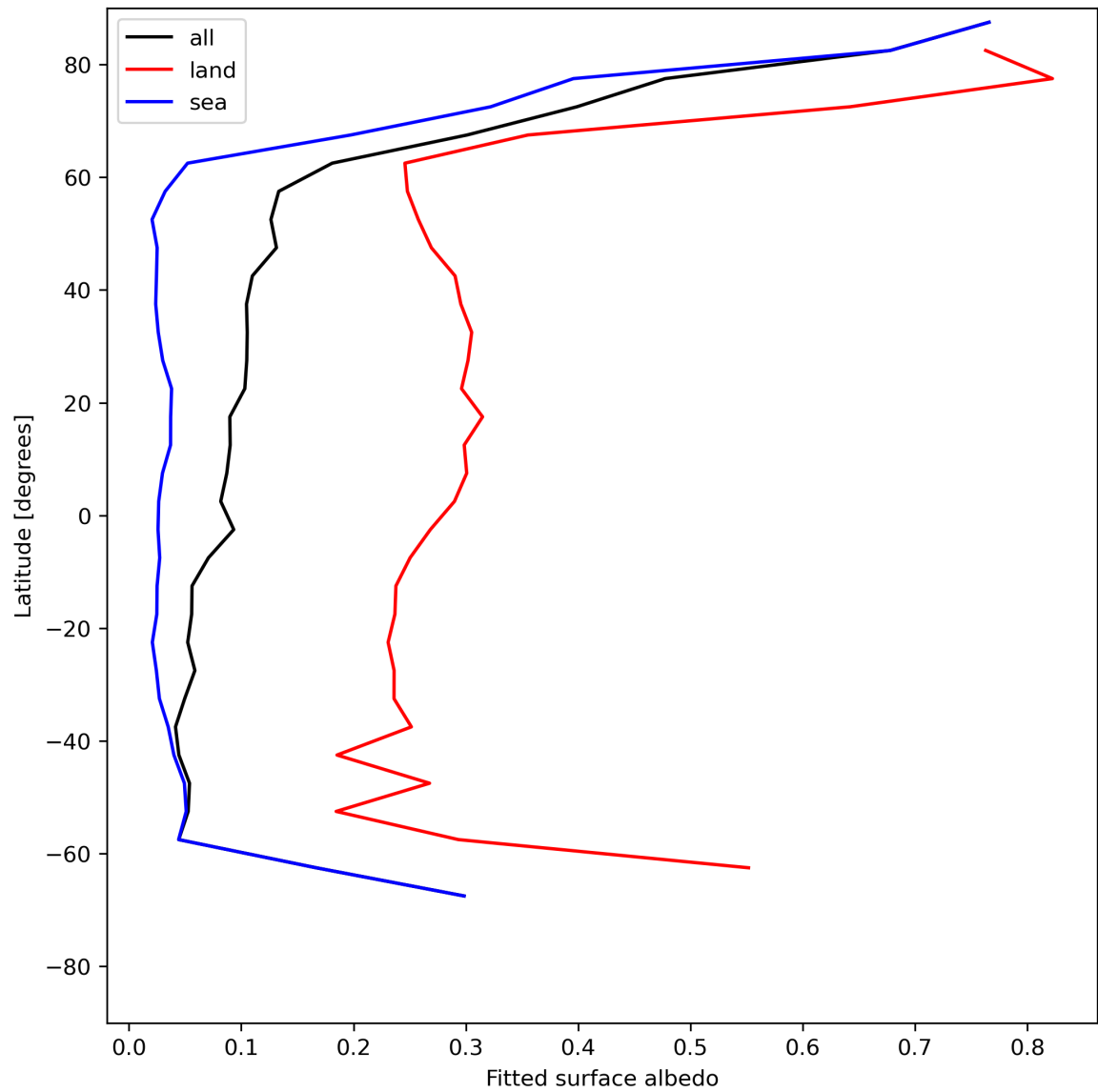
Figure 29: Zonal average of “Fitted surface albedo” for 2024-06-15 to 2024-06-17.
