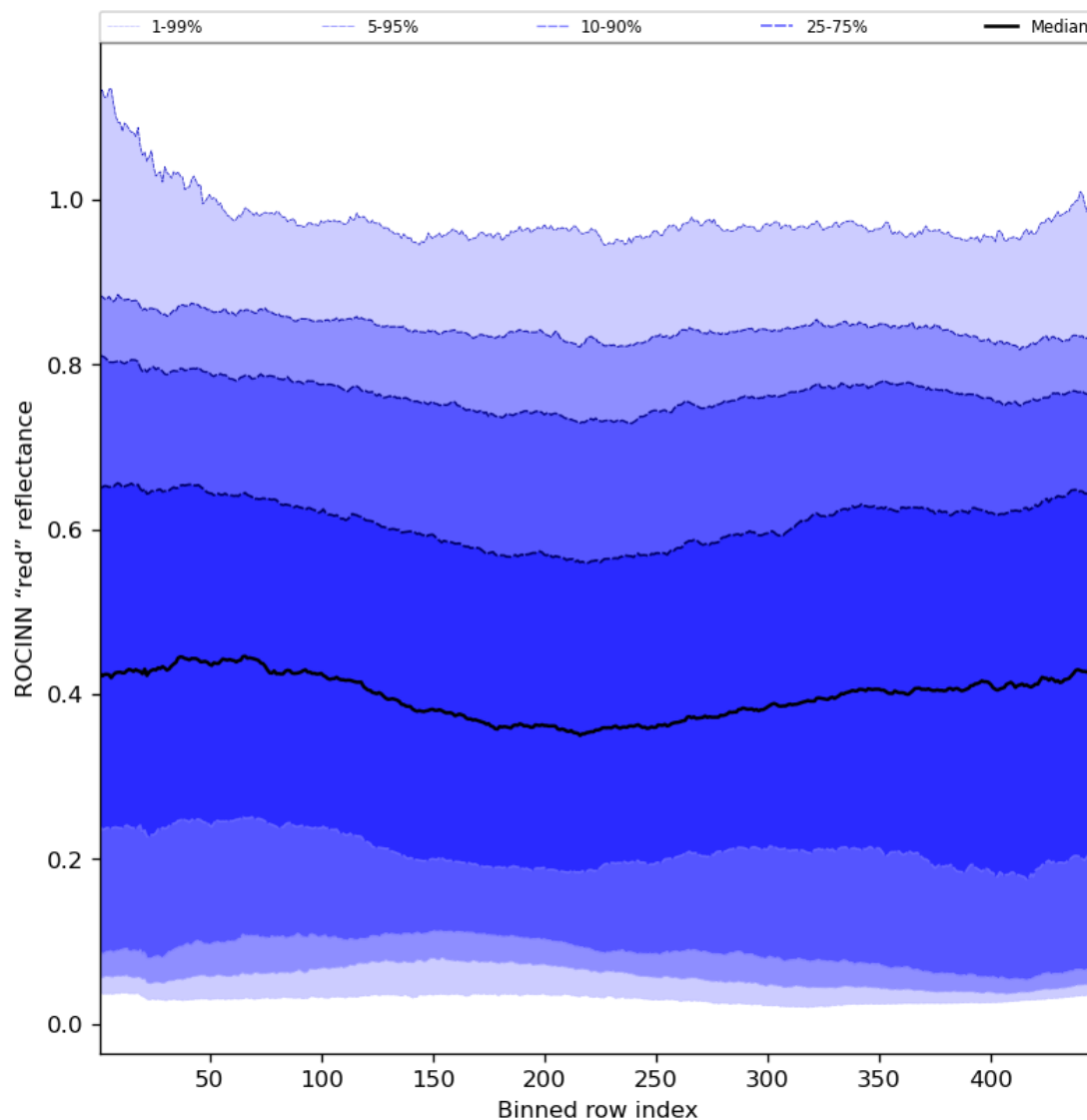
Figure 69: Along track statistics of “ROCINN “red” reflectance” for 2024-06-15 to 2024-06-17
