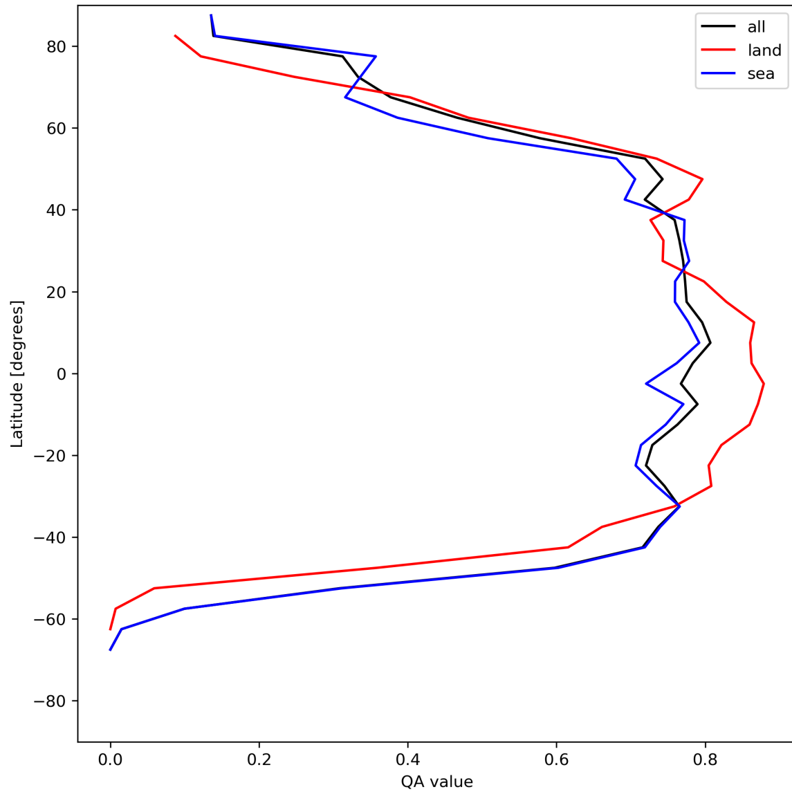
Figure 22: Zonal average of “QA value” for 2024-06-15 to 2024-06-17.
