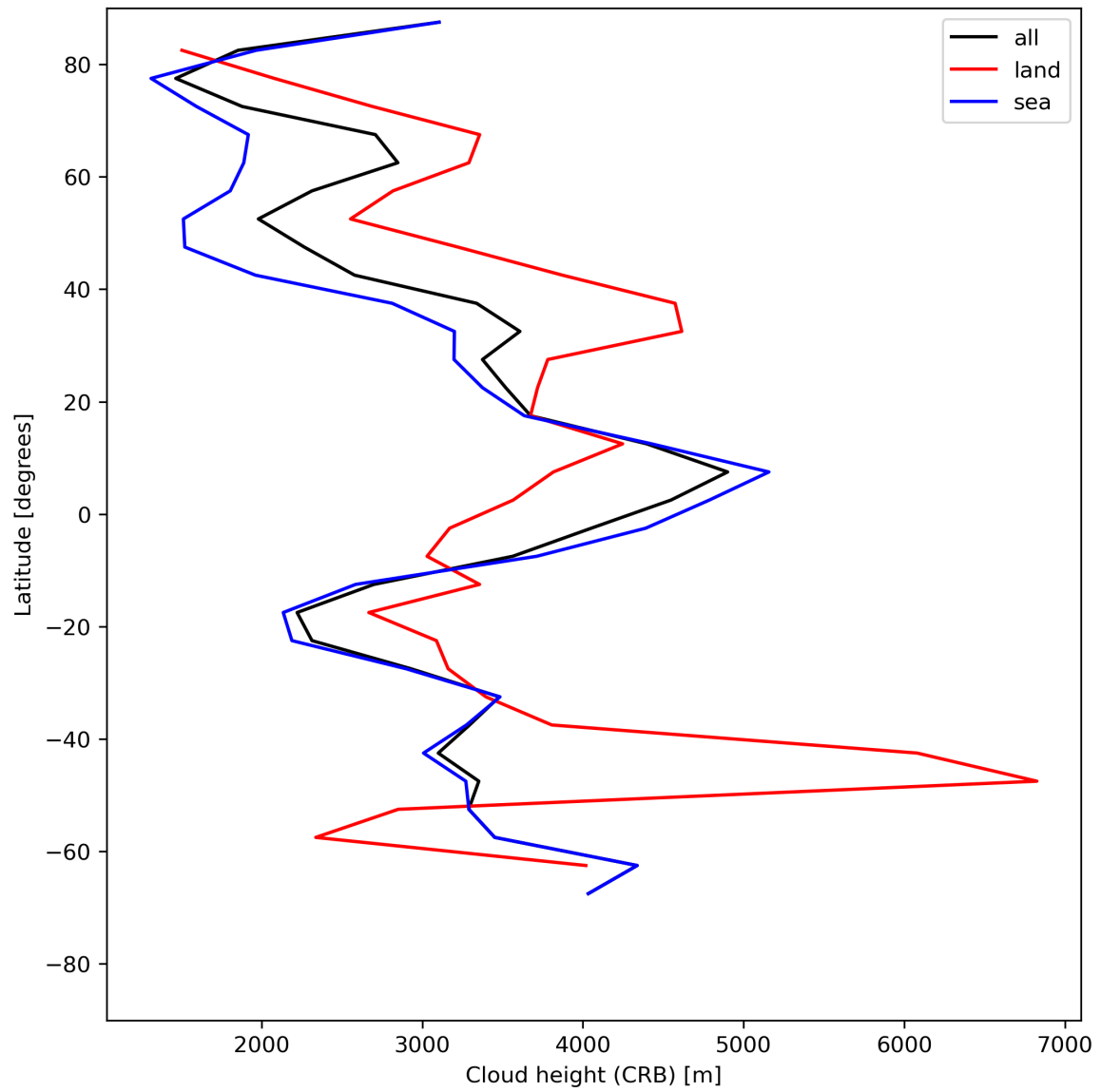
Figure 27: Zonal average of “Cloud height (CRB)” for 2024-06-15 to 2024-06-17.
