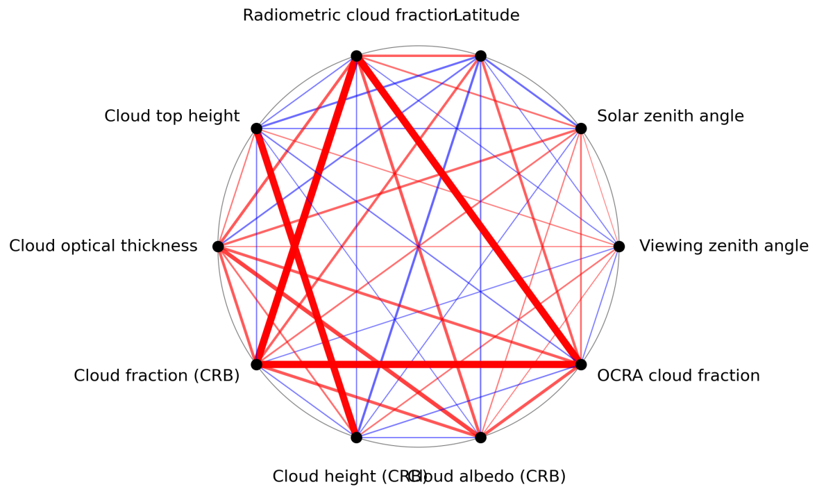
Figure 1: Map of correlation graph for 2024-06-15 to 2024-06-17.
