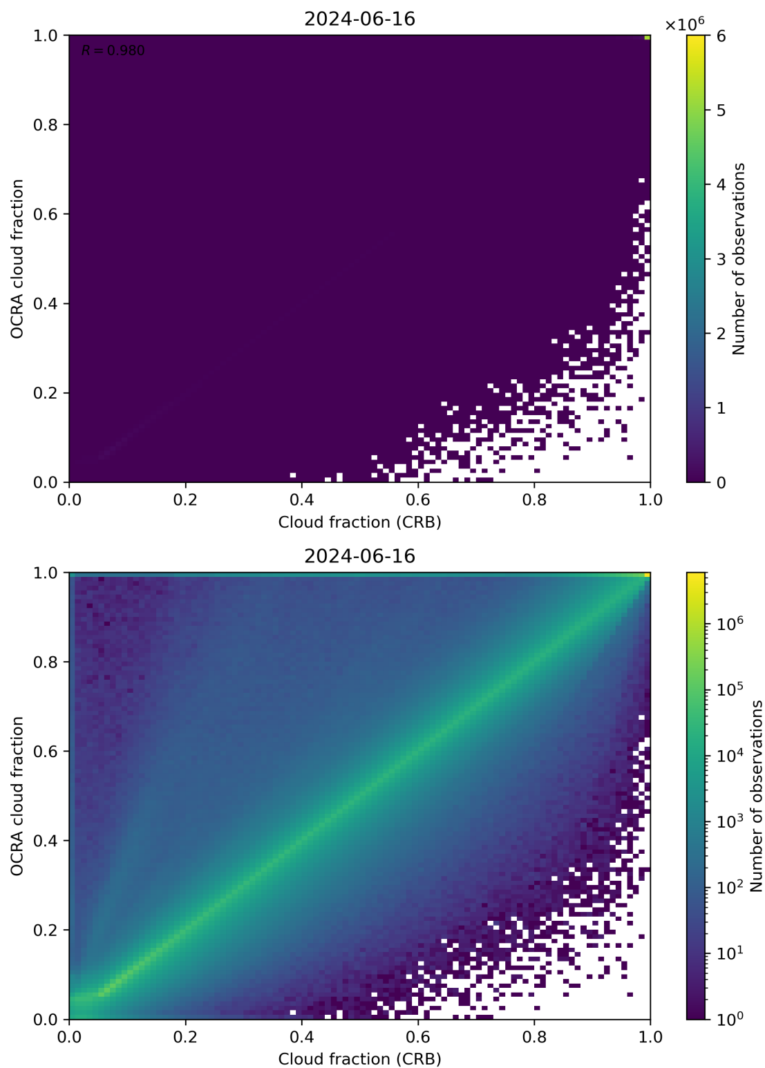
Figure 78: Scatter density plot of “Cloud fraction (CRB)” against “OCRA cloud fraction” for 2024-06-15 to 2024-06-17.
