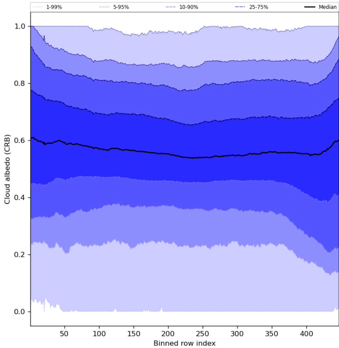
Figure 60: Along track statistics of “Cloud albedo (CRB)” for 2024-06-15 to 2024-06-17
