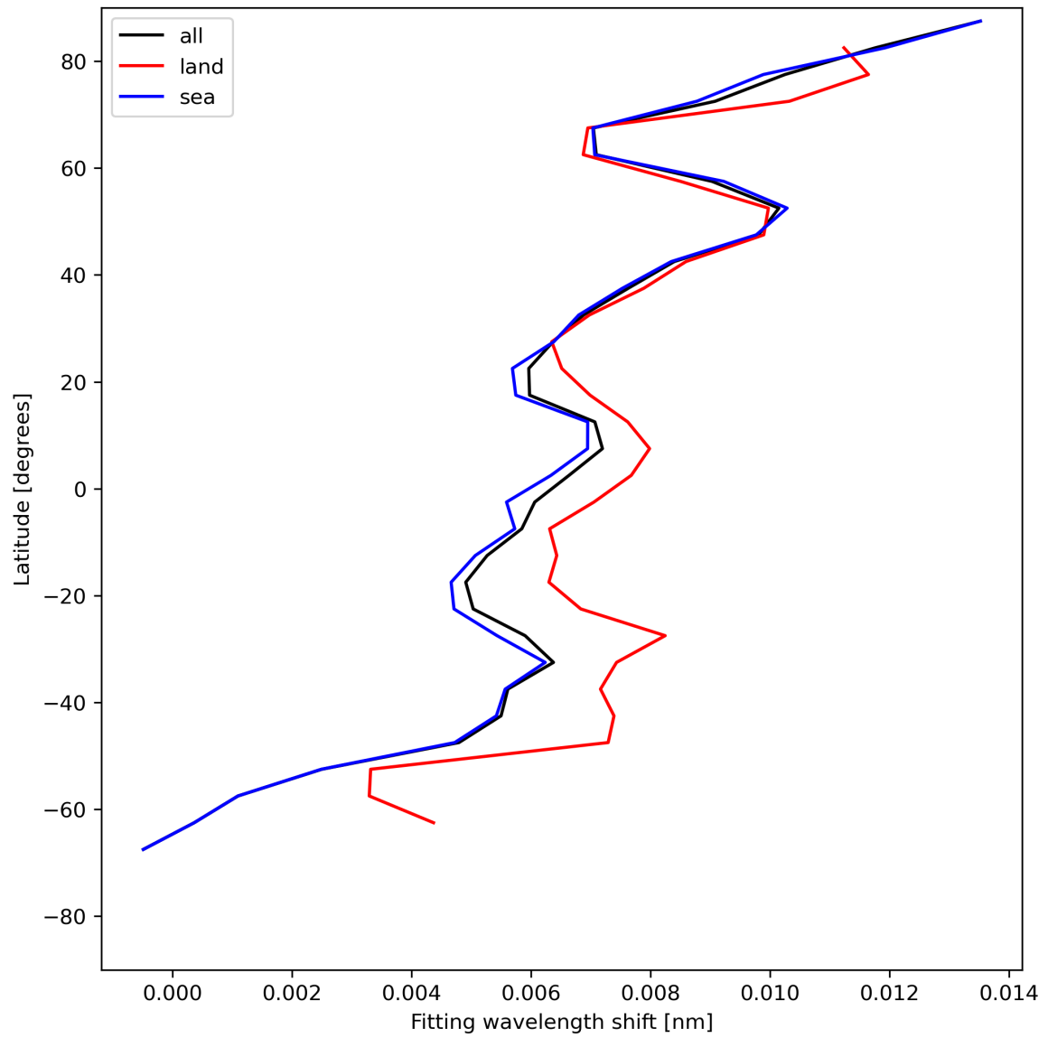
Figure 33: Zonal average of “Fitting wavelength shift” for 2024-06-15 to 2024-06-17.
