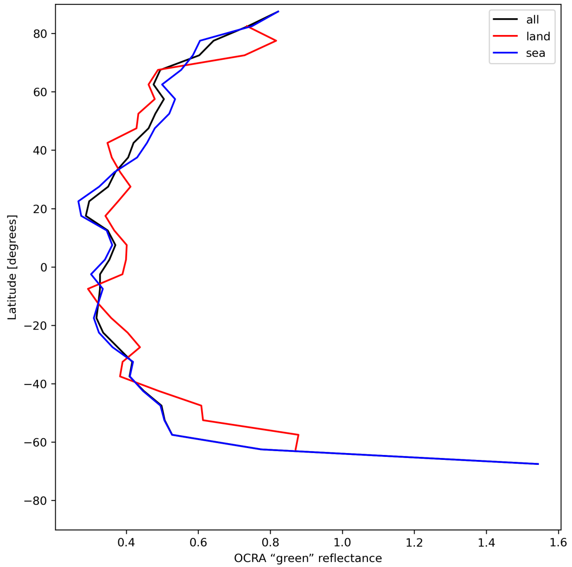
Figure 36: Zonal average of “OCRA “green” reflectance” for 2024-06-15 to 2024-06-17.
