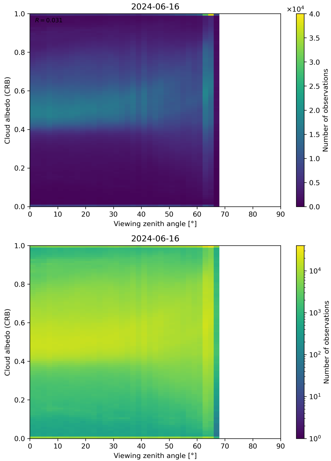
Figure 106: Scatter density plot of “Viewing zenith angle” against “Cloud albedo (CRB)” for 2024-06-15 to 2024-06-17.
