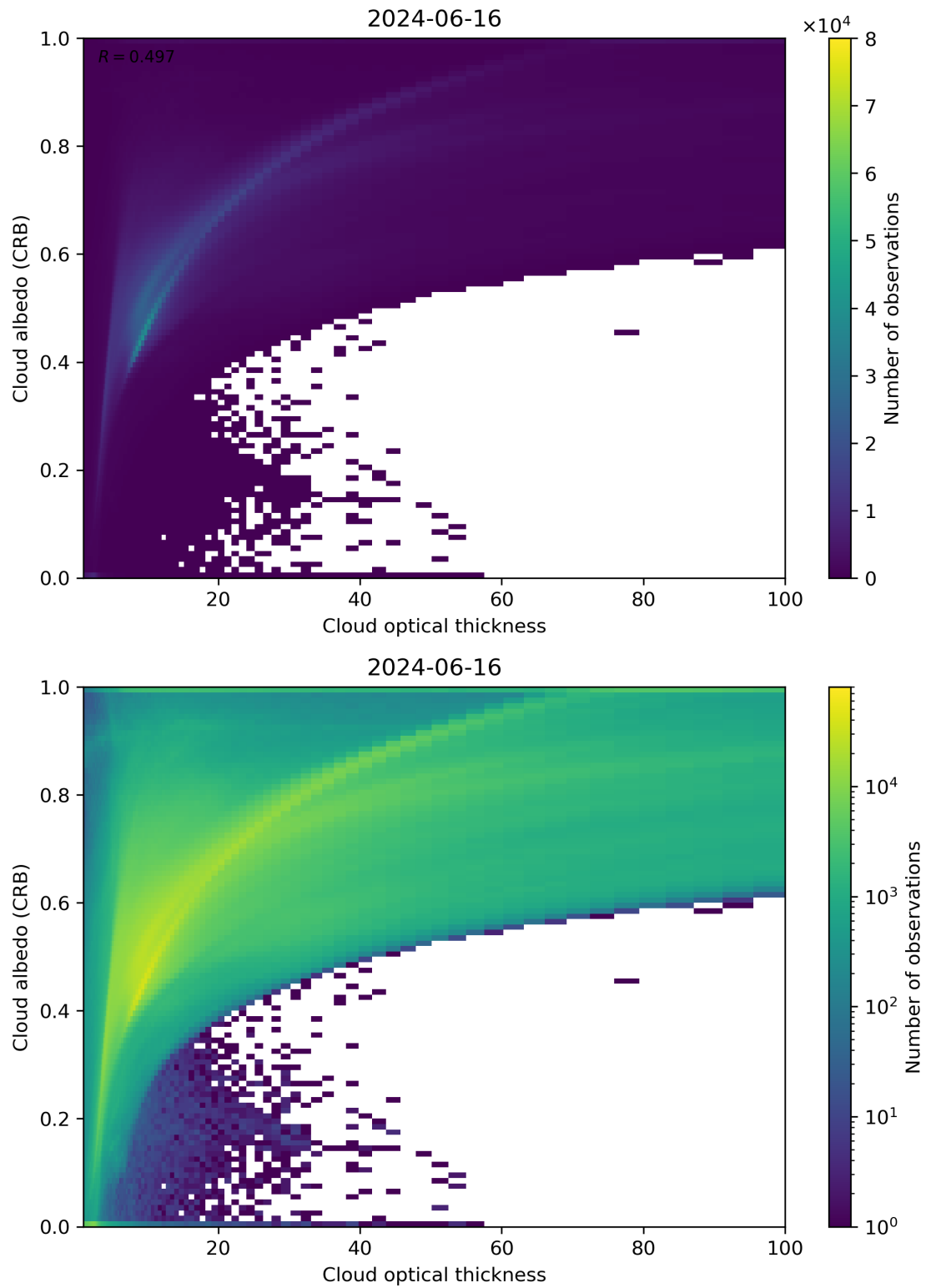
Figure 82: Scatter density plot of “Cloud optical thickness” against “Cloud albedo (CRB)” for 2024-06-15 to 2024-06-17.
