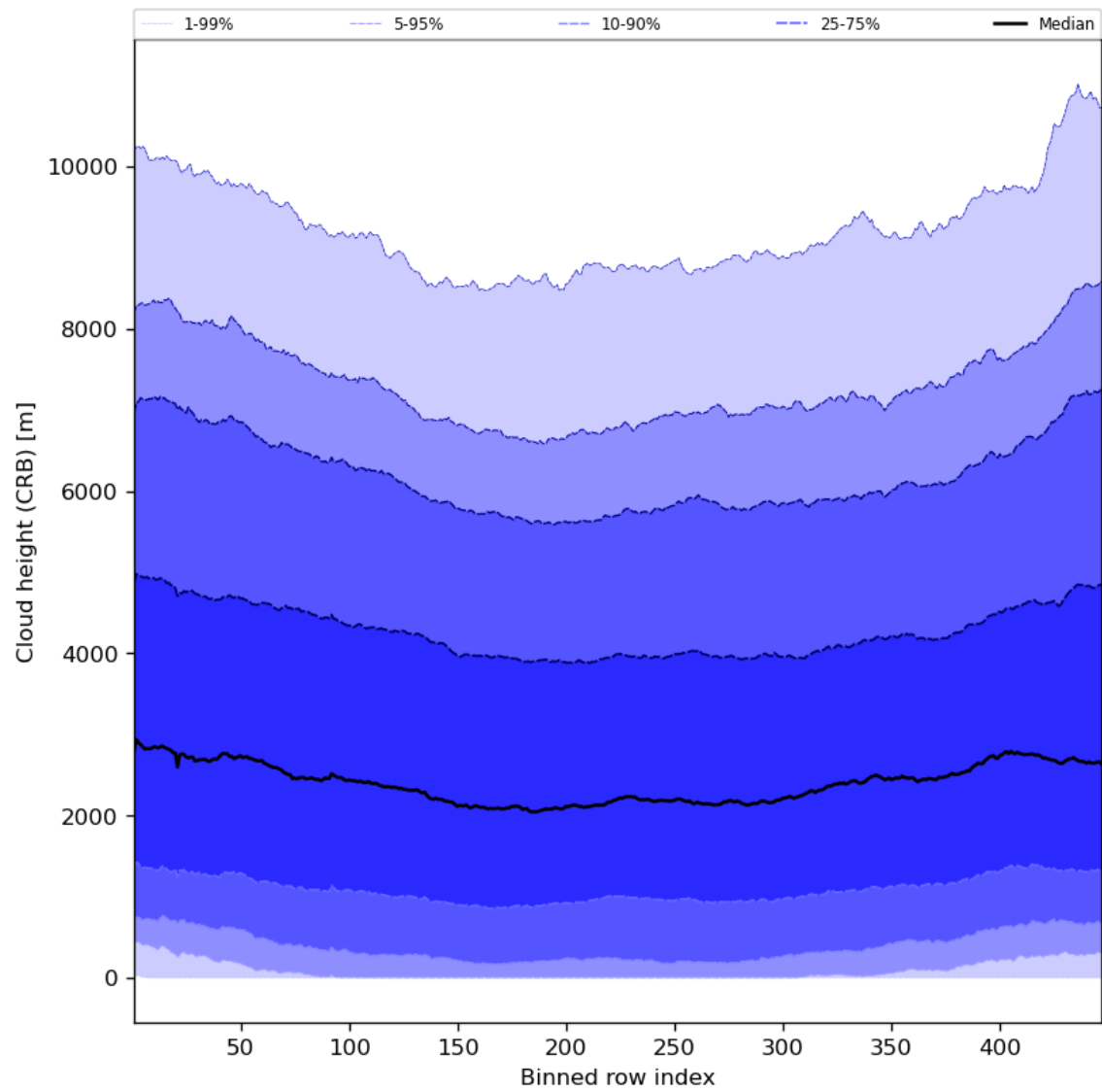
Figure 59: Along track statistics of “Cloud height (CRB)” for 2024-06-15 to 2024-06-17
