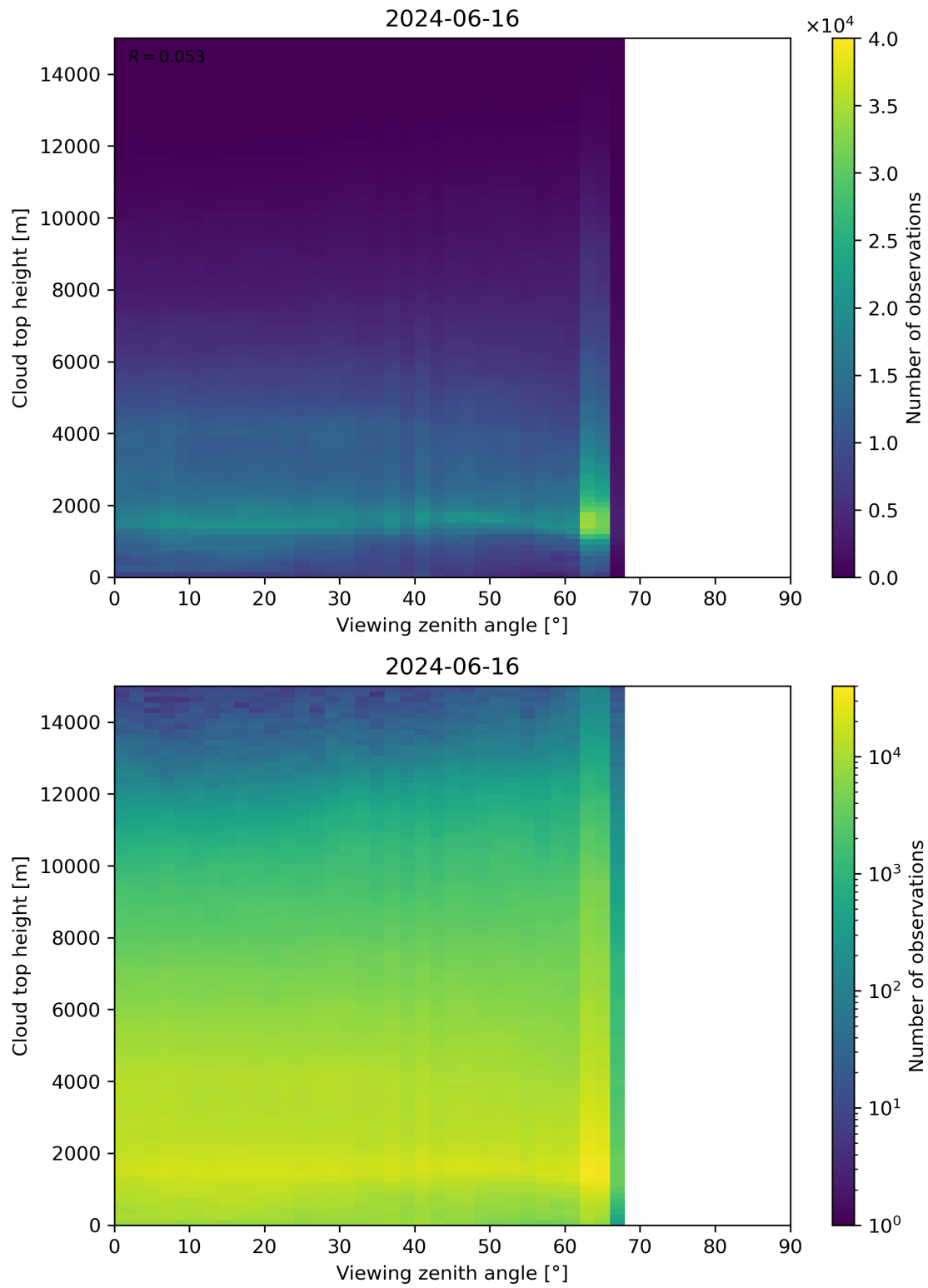
Figure 112: Scatter density plot of “Viewing zenith angle” against “Cloud top height” for 2024-06-15 to 2024-06-17.
