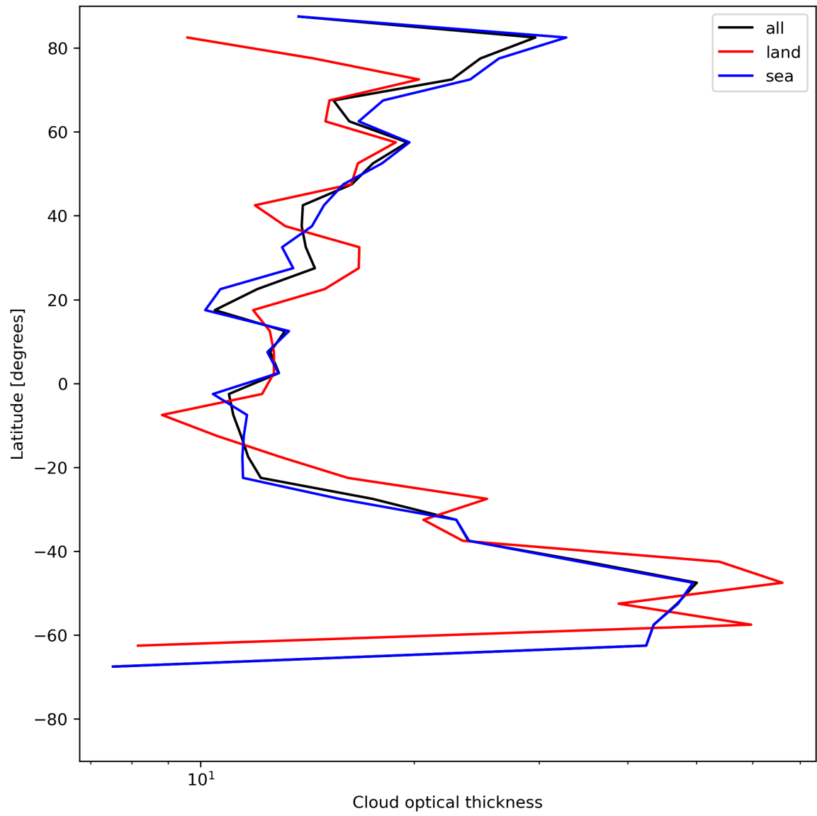
Figure 25: Zonal average of “Cloud optical thickness” for 2024-06-15 to 2024-06-17.
