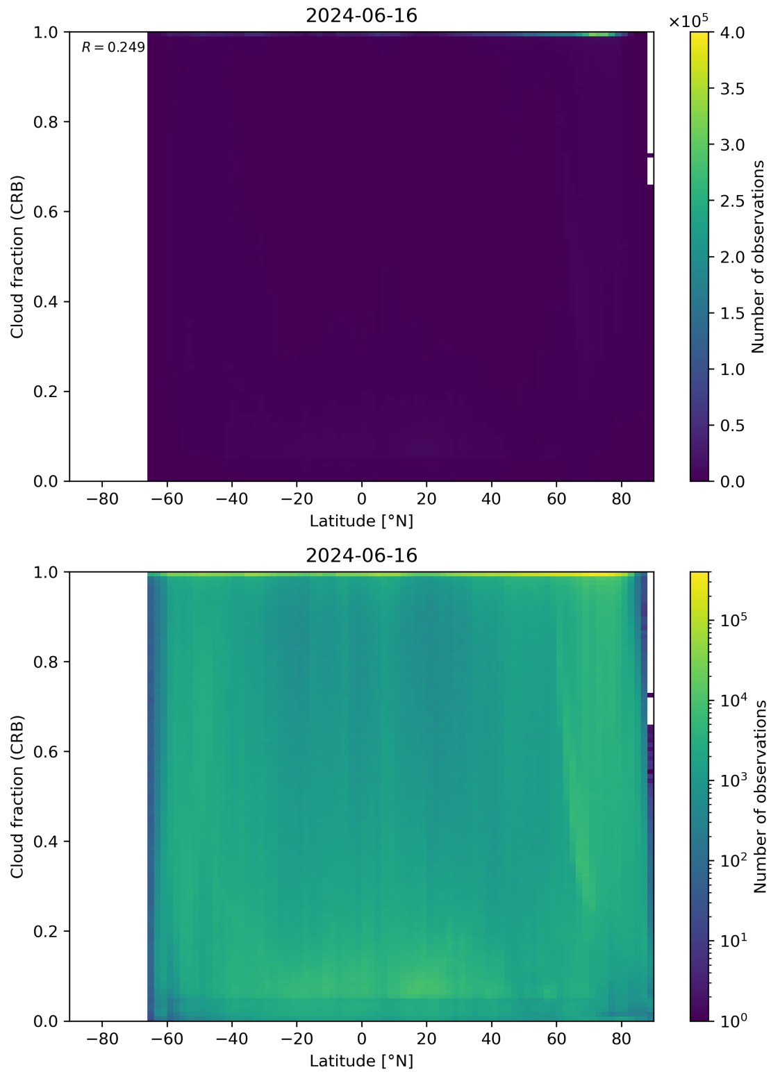
Figure 94: Scatter density plot of “Latitude” against “Cloud fraction (CRB)” for 2024-06-15 to 2024-06-17.
