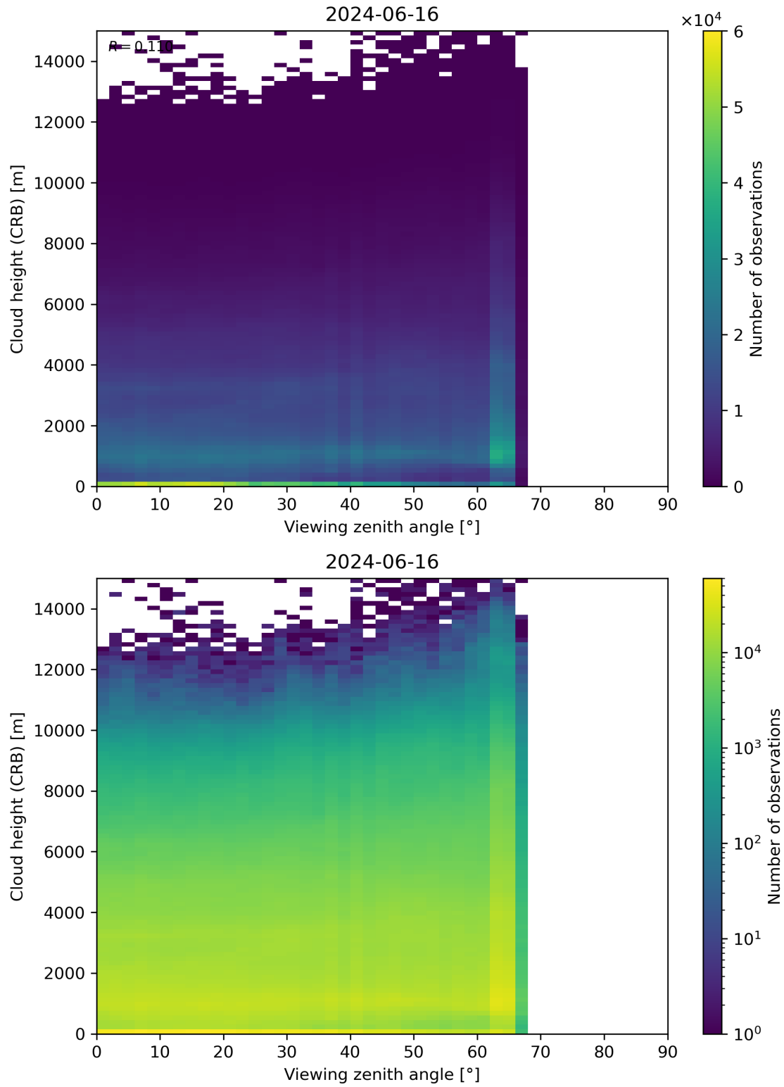
Figure 110: Scatter density plot of “Viewing zenith angle” against “Cloud height (CRB)” for 2024-06-15 to 2024-06-17.
