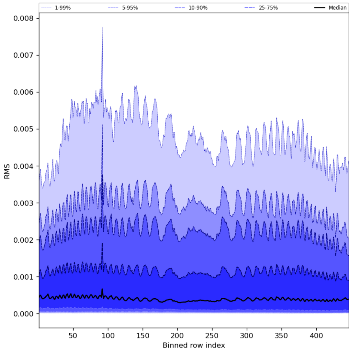
Figure 63: Along track statistics of “RMS” for 2024-06-15 to 2024-06-17
