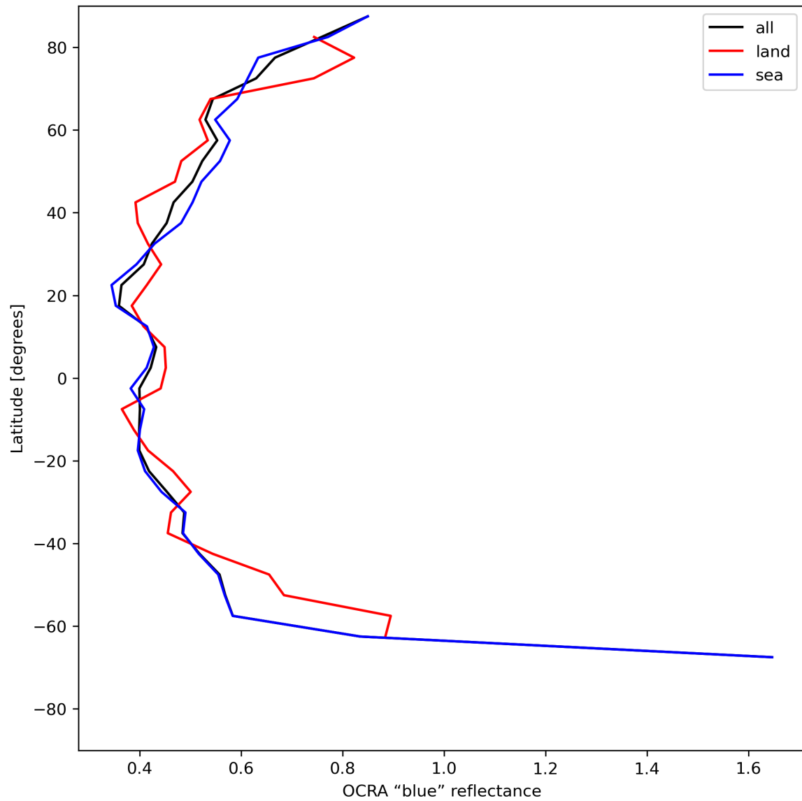
Figure 35: Zonal average of “OCRA “blue” reflectance” for 2024-06-15 to 2024-06-17.
