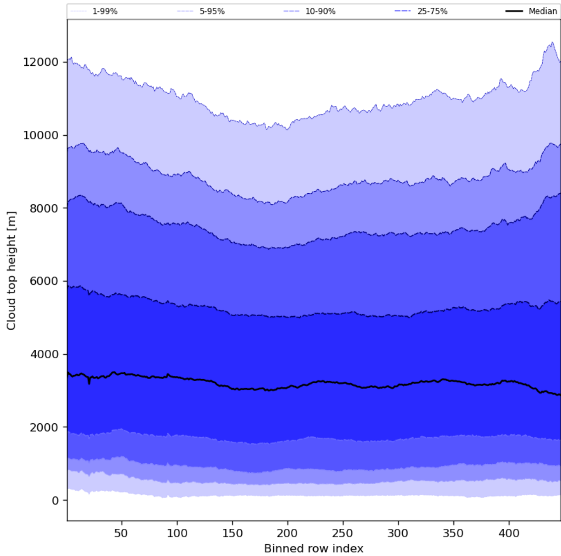
Figure 56: Along track statistics of “Cloud top height” for 2024-06-15 to 2024-06-17
