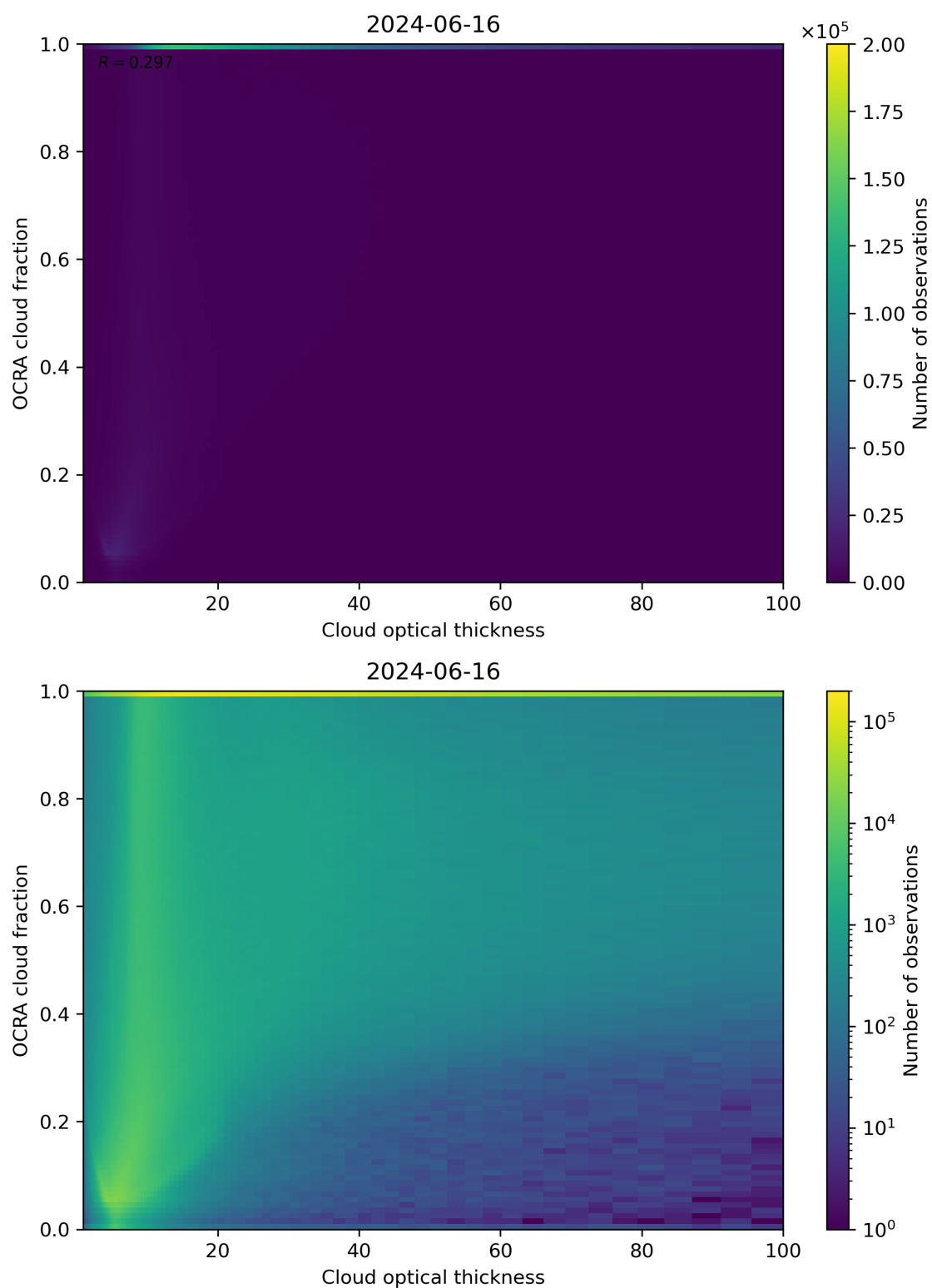
Figure 83: Scatter density plot of “Cloud optical thickness” against “OCRA cloud fraction” for 2024-06-15 to 2024-06-17.
