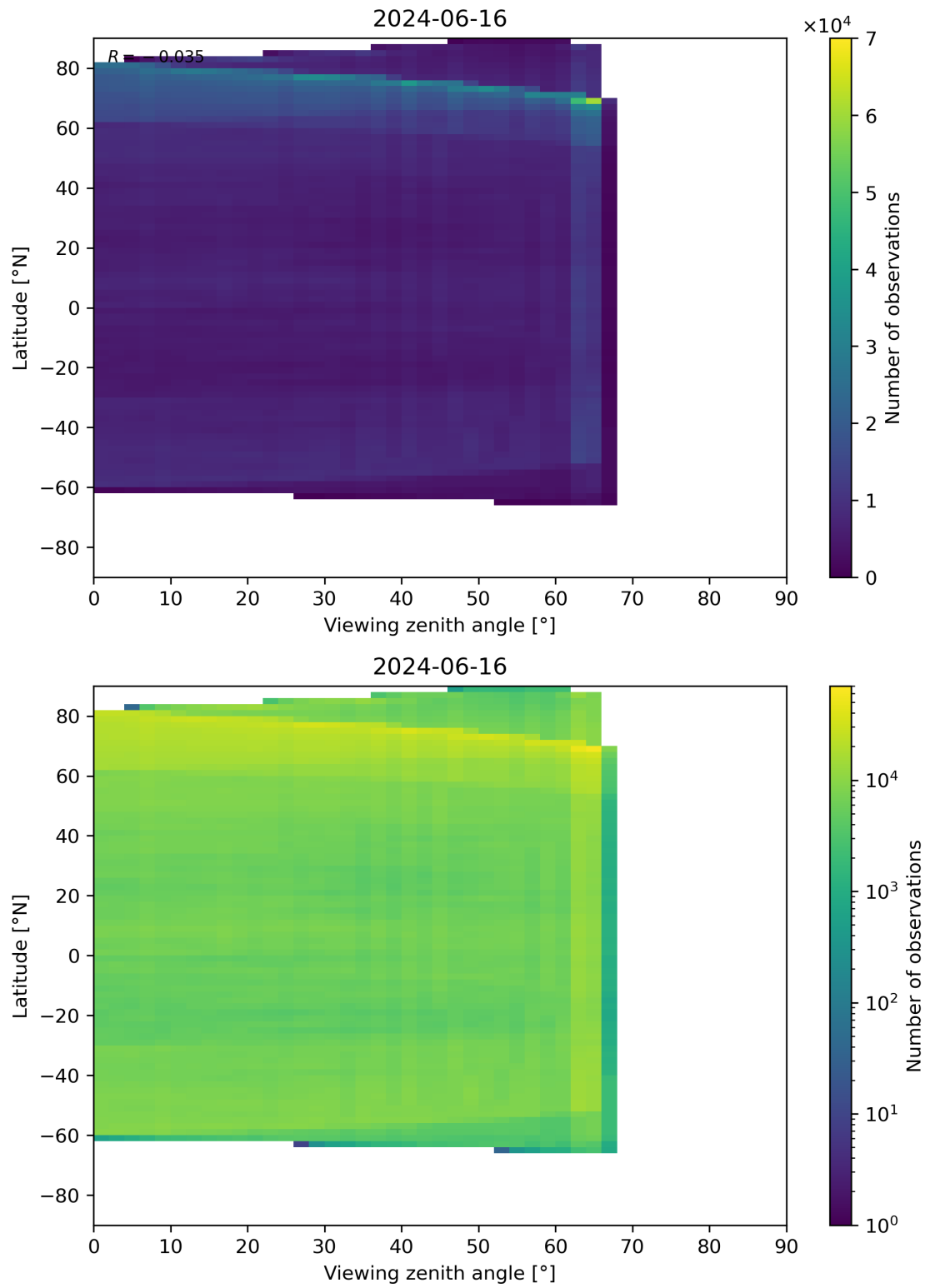
Figure 113: Scatter density plot of “Viewing zenith angle” against “Latitude” for 2024-06-15 to 2024-06-17.
