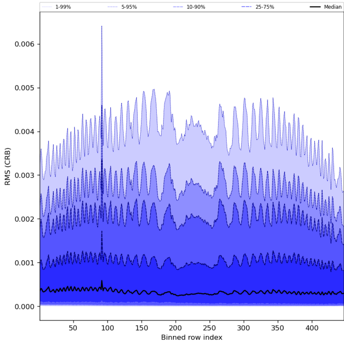
Figure 64: Along track statistics of "RMS (CRB)" for 2024-06-15 to 2024-06-17
