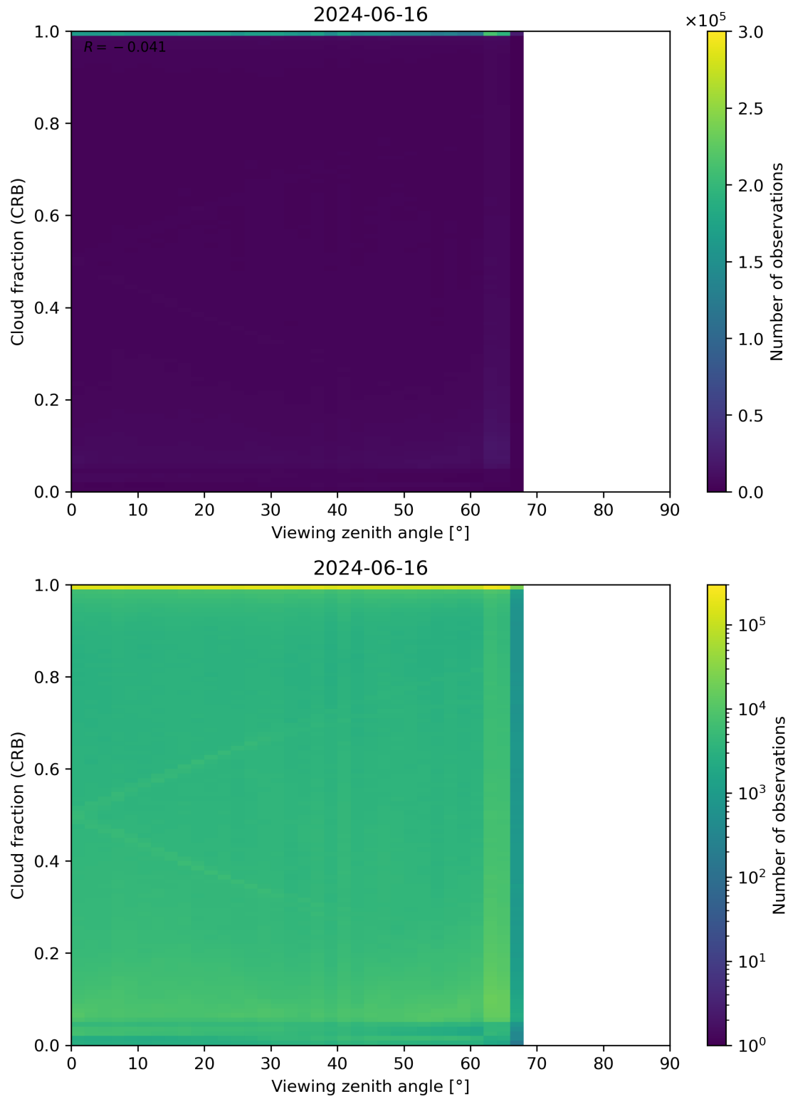
Figure 109: Scatter density plot of “Viewing zenith angle” against “Cloud fraction (CRB)” for 2024-06-15 to 2024-06-17.
