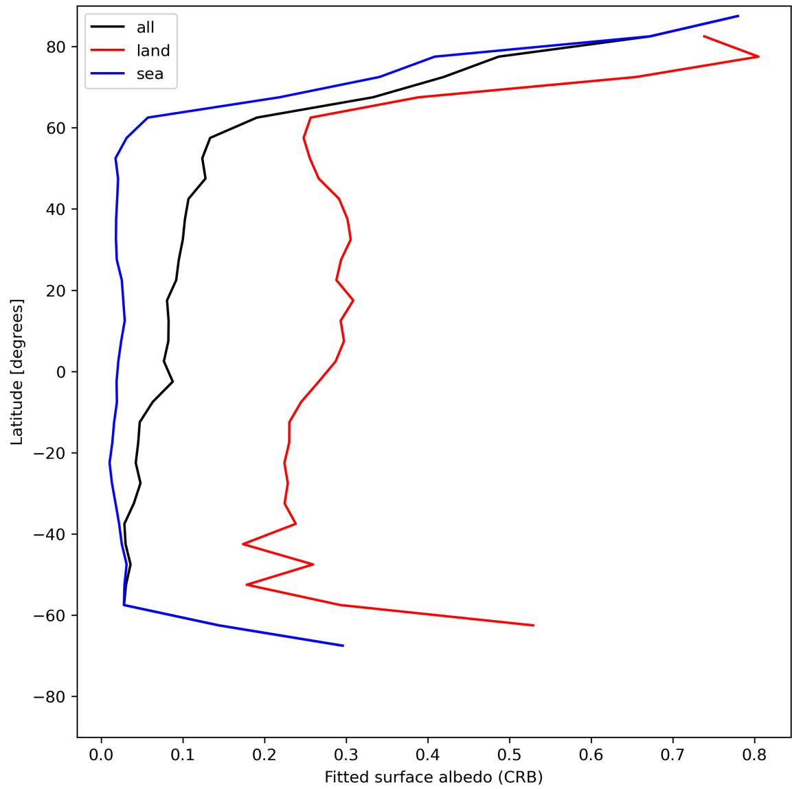
Figure 30: Zonal average of “Fitted surface albedo (CRB)” for 2024-06-15 to 2024-06-17.
