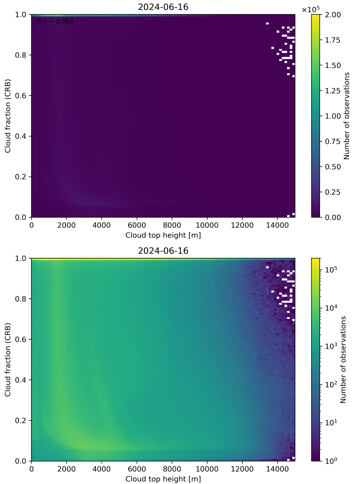
Figure 88: Scatter density plot of “Cloud top height” against “Cloud fraction (CRB)” for 2024-06-15 to 2024-06-17.
