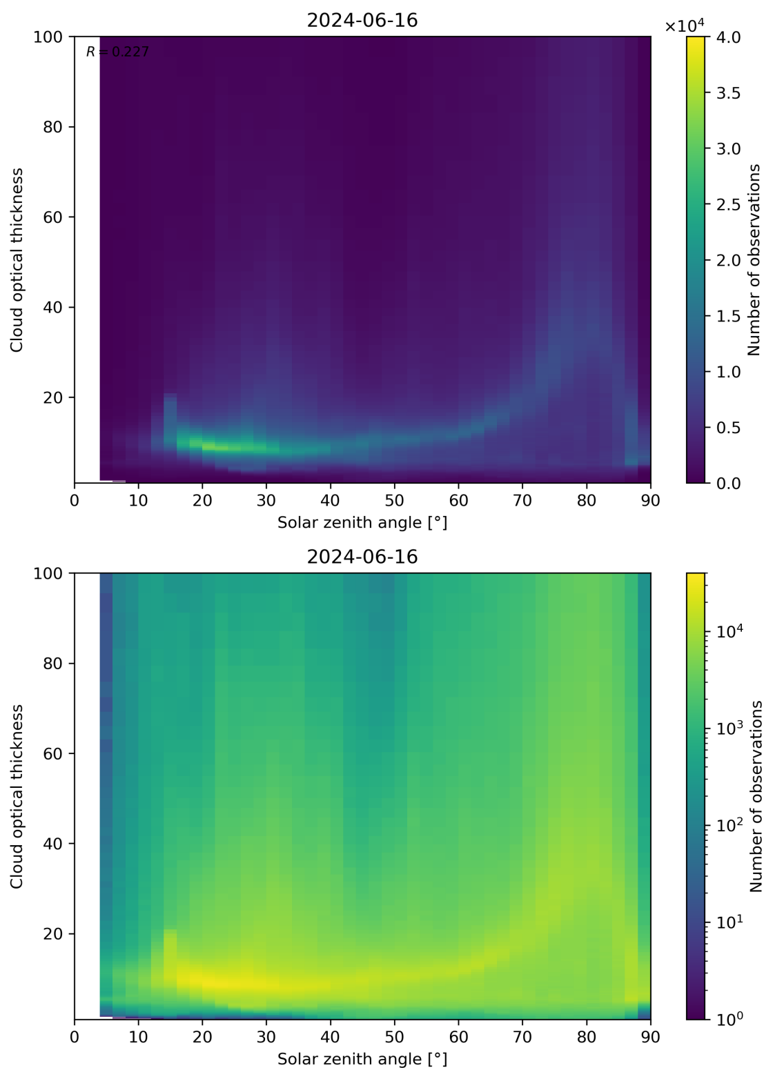
Figure 103: Scatter density plot of “Solar zenith angle” against “Cloud optical thickness” for 2024-06-15 to 2024-06-17.
