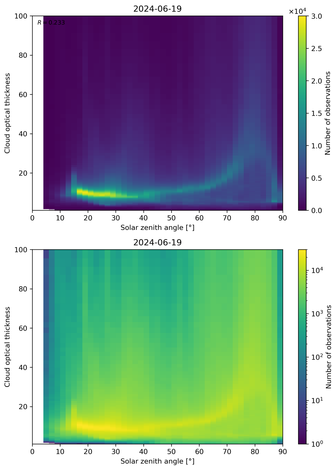
Figure 103: Scatter density plot of “Solar zenith angle” against “Cloud optical thickness” for 2024-06-19 to 2024-06-20.
