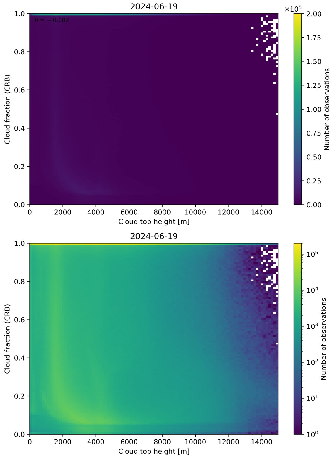
Figure 88: Scatter density plot of “Cloud top height” against “Cloud fraction (CRB)” for 2024-06-19 to 2024-06-20.
