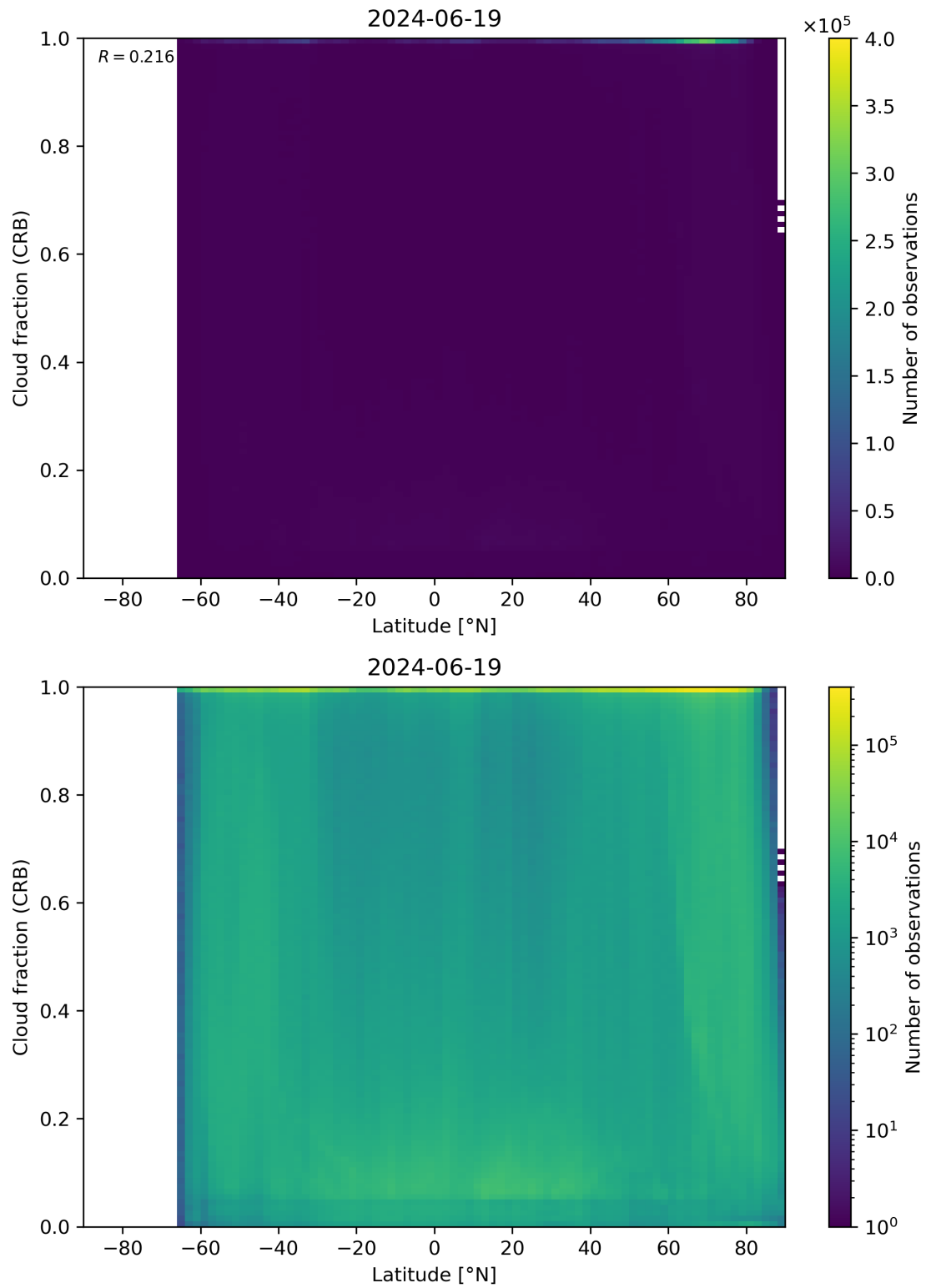
Figure 94: Scatter density plot of “Latitude” against “Cloud fraction (CRB)” for 2024-06-19 to 2024-06-20.
