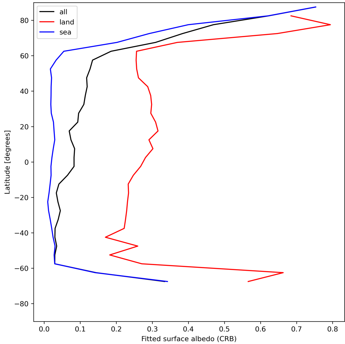
Figure 30: Zonal average of "Fitted surface albedo (CRB)" for 2024-06-19 to 2024-06-20.
