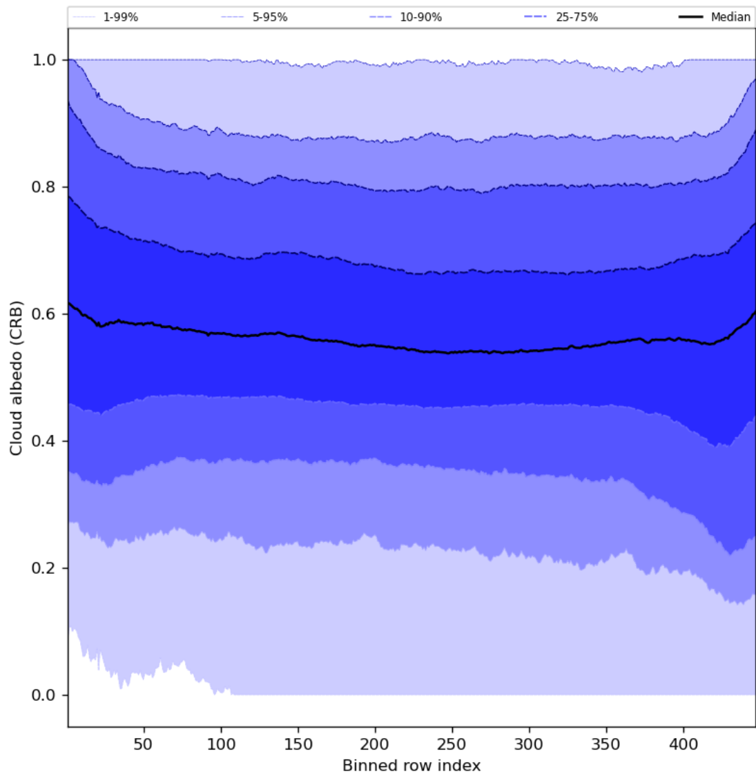
Figure 60: Along track statistics of “Cloud albedo (CRB)” for 2024-06-19 to 2024-06-20
