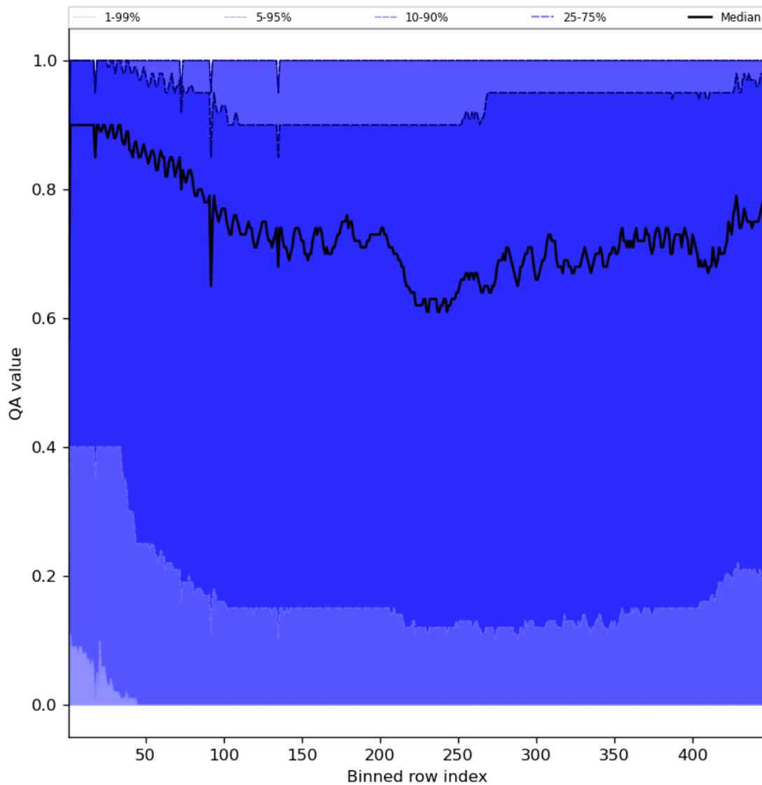
Figure 54: Along track statistics of “QA value” for 2024-06-19 to 2024-06-20
