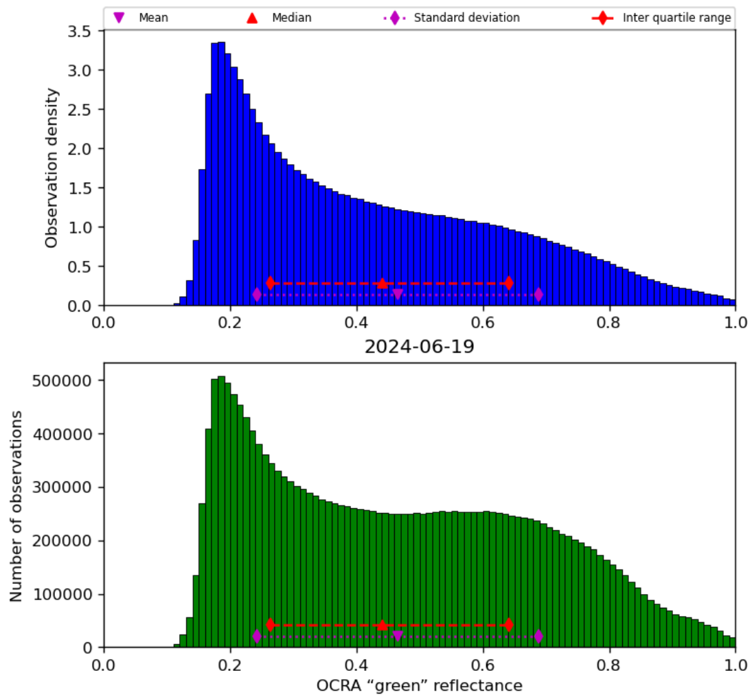
Figure 52: Histogram of “OCRA “green” reflectance” for 2024-06-19 to 2024-06-20
