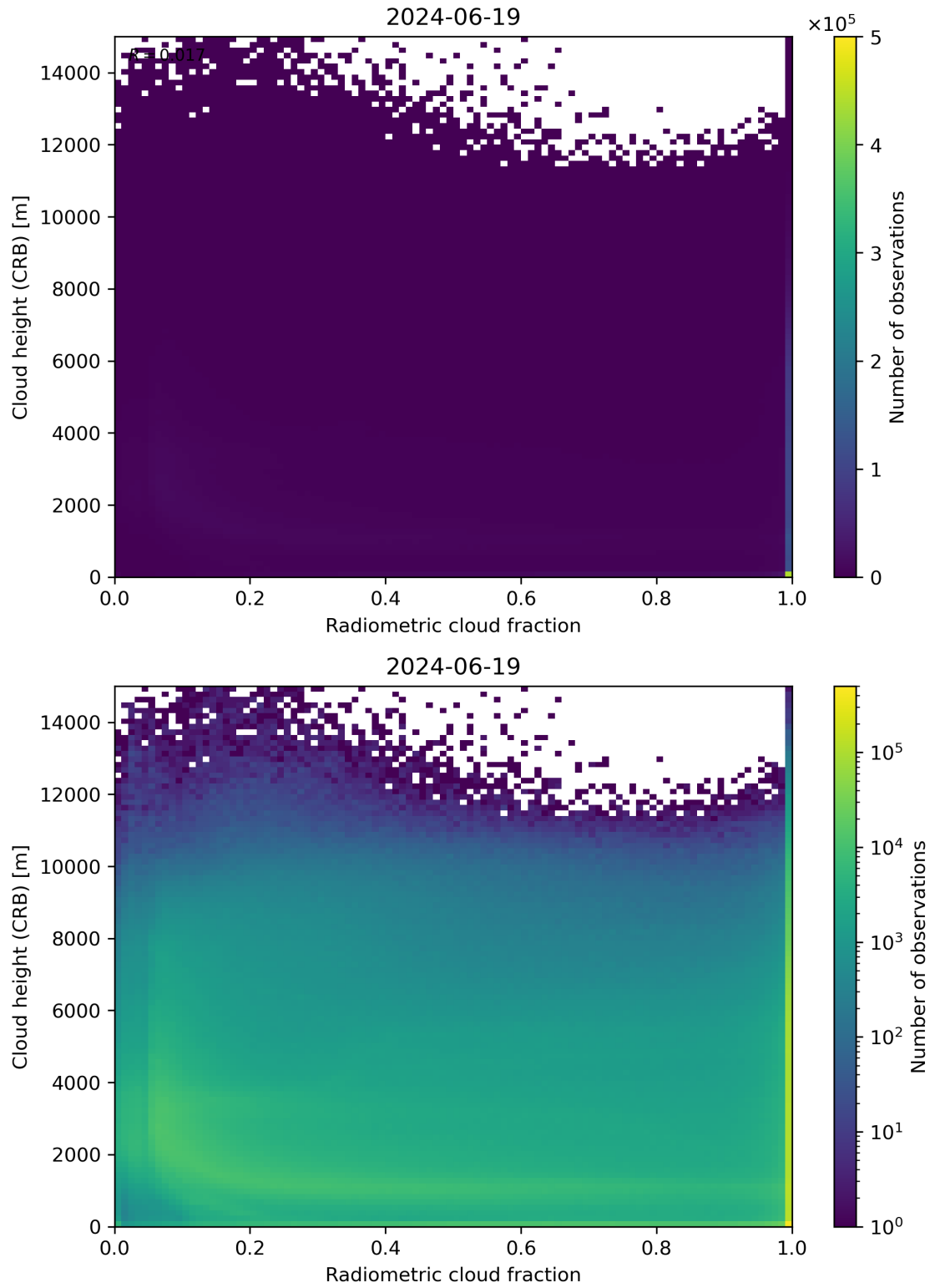
Figure 74: Scatter density plot of “Radiometric cloud fraction” against “Cloud height (CRB)” for 2024-06-19 to 2024-06-20.
