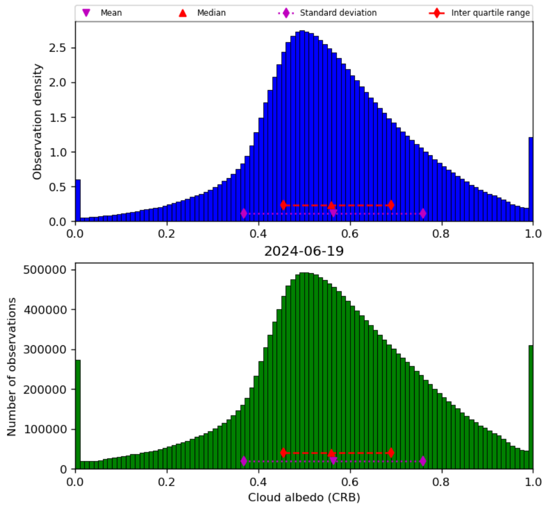
Figure 44: Histogram of “Cloud albedo (CRB)” for 2024-06-19 to 2024-06-20
