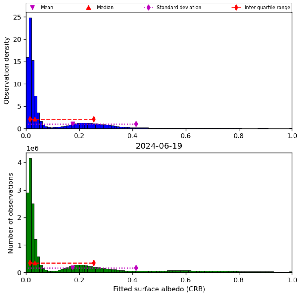
Figure 46: Histogram of “Fitted surface albedo (CRB)” for 2024-06-19 to 2024-06-20
