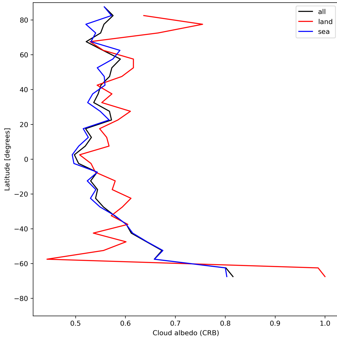
Figure 28: Zonal average of “Cloud albedo (CRB)” for 2024-06-19 to 2024-06-20.
