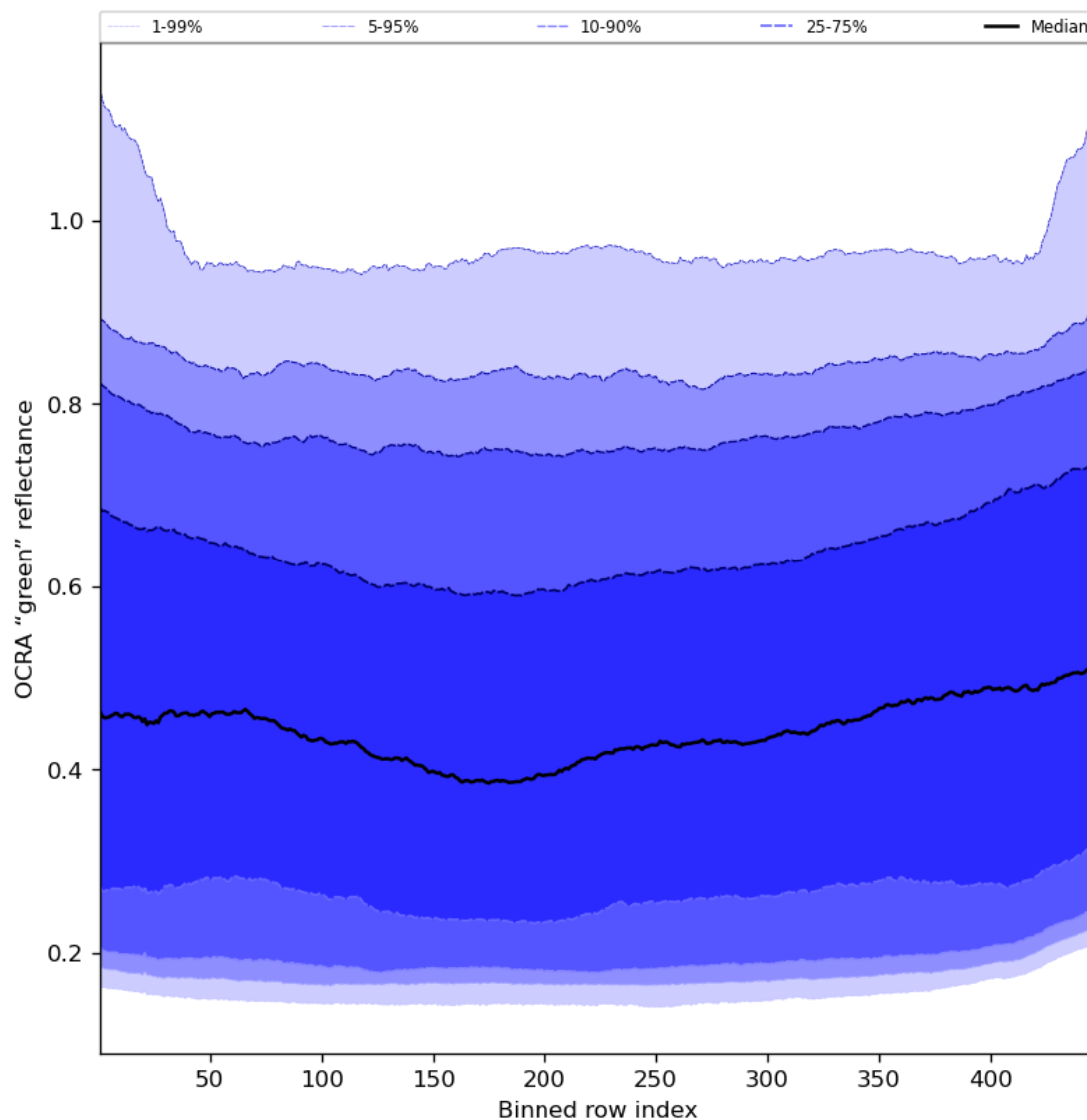
Figure 68: Along track statistics of “OCRA “green” reflectance” for 2024-06-19 to 2024-06-20
