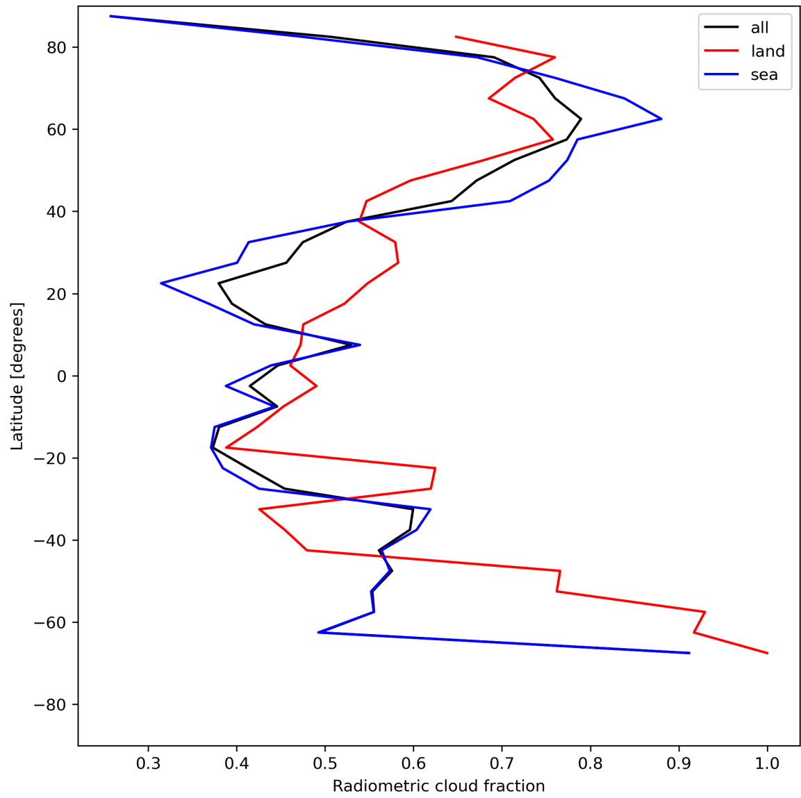
Figure 23: Zonal average of “Radiometric cloud fraction” for 2024-06-19 to 2024-06-20.
