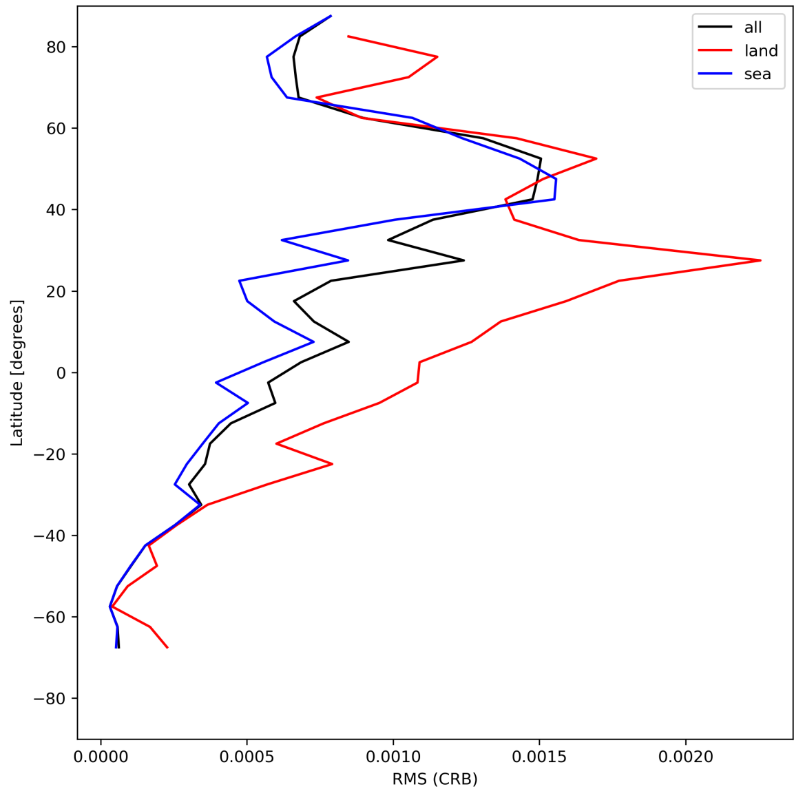
Figure 32: Zonal average of “RMS (CRB)” for 2024-06-19 to 2024-06-20.
