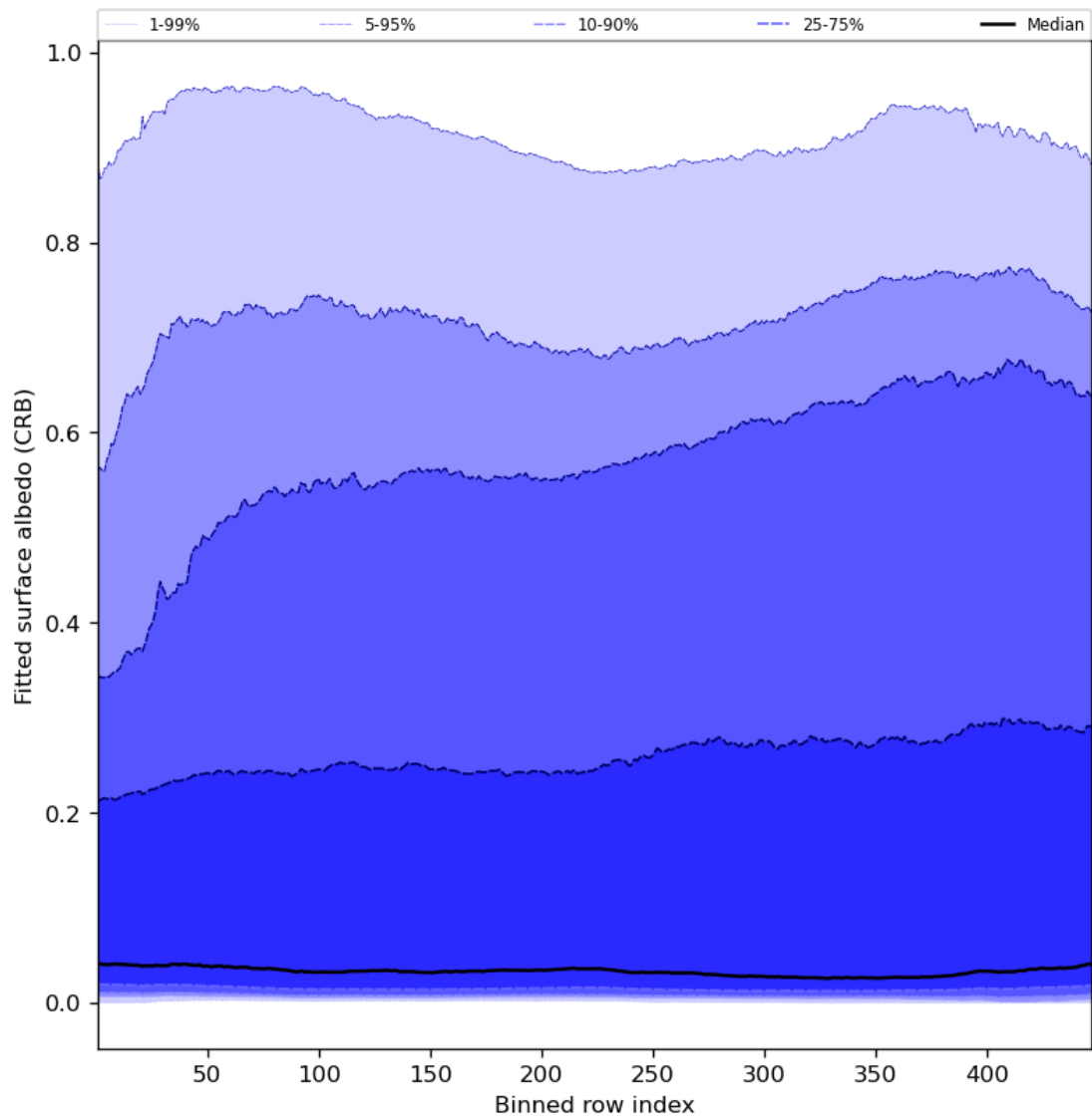
Figure 62: Along track statistics of “Fitted surface albedo (CRB)” for 2024-06-19 to 2024-06-20
