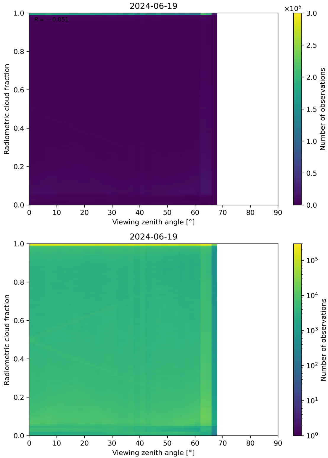
Figure 107: Scatter density plot of “Viewing zenith angle” against “Radiometric cloud fraction” for 2024-06-19 to 2024-06-20.
