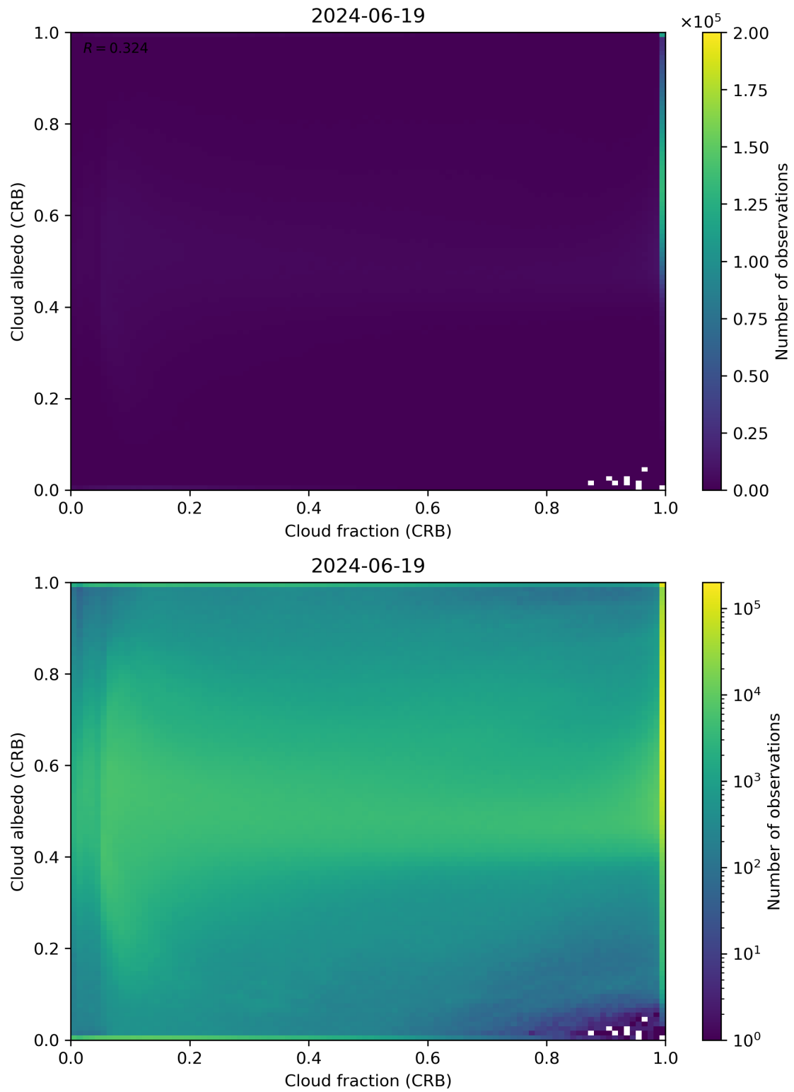
Figure 77: Scatter density plot of “Cloud fraction (CRB)” against “Cloud albedo (CRB)” for 2024-06-19 to 2024-06-20.
