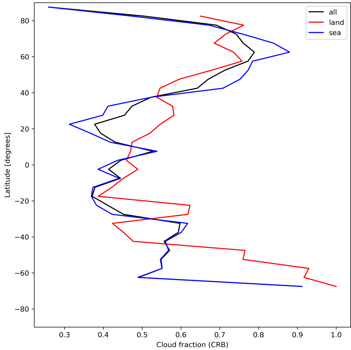
Figure 26: Zonal average of “Cloud fraction (CRB)” for 2024-06-19 to 2024-06-20.
