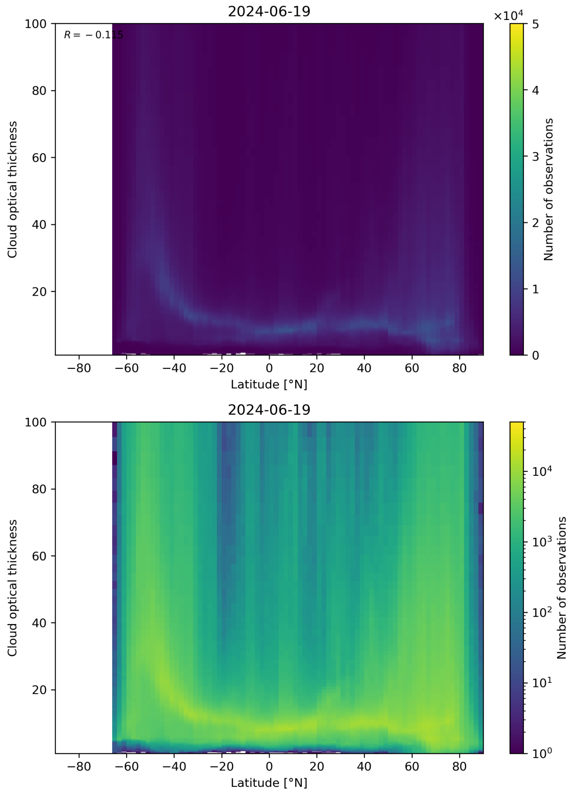
Figure 96: Scatter density plot of “Latitude” against “Cloud optical thickness” for 2024-06-19 to 2024-06-20.
