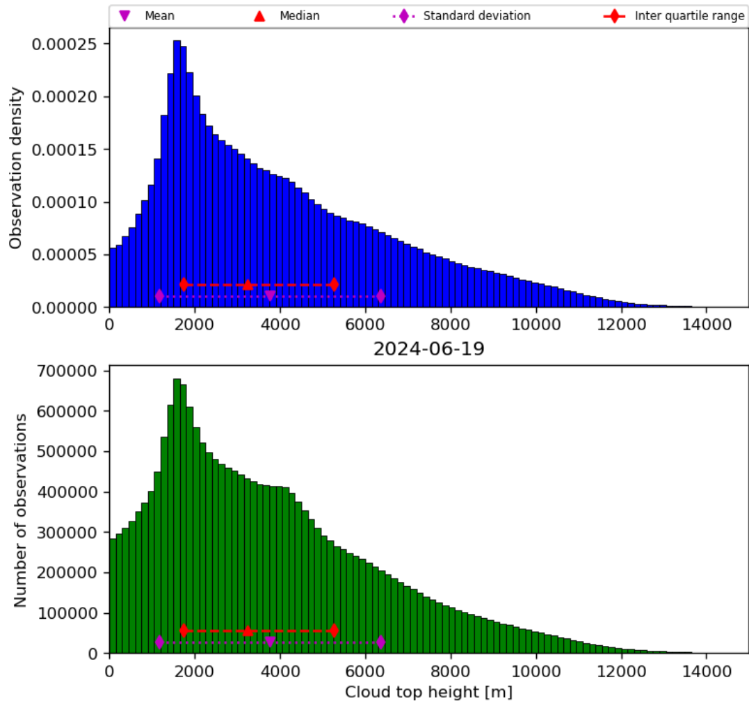
Figure 40: Histogram of “Cloud top height” for 2024-06-19 to 2024-06-20
