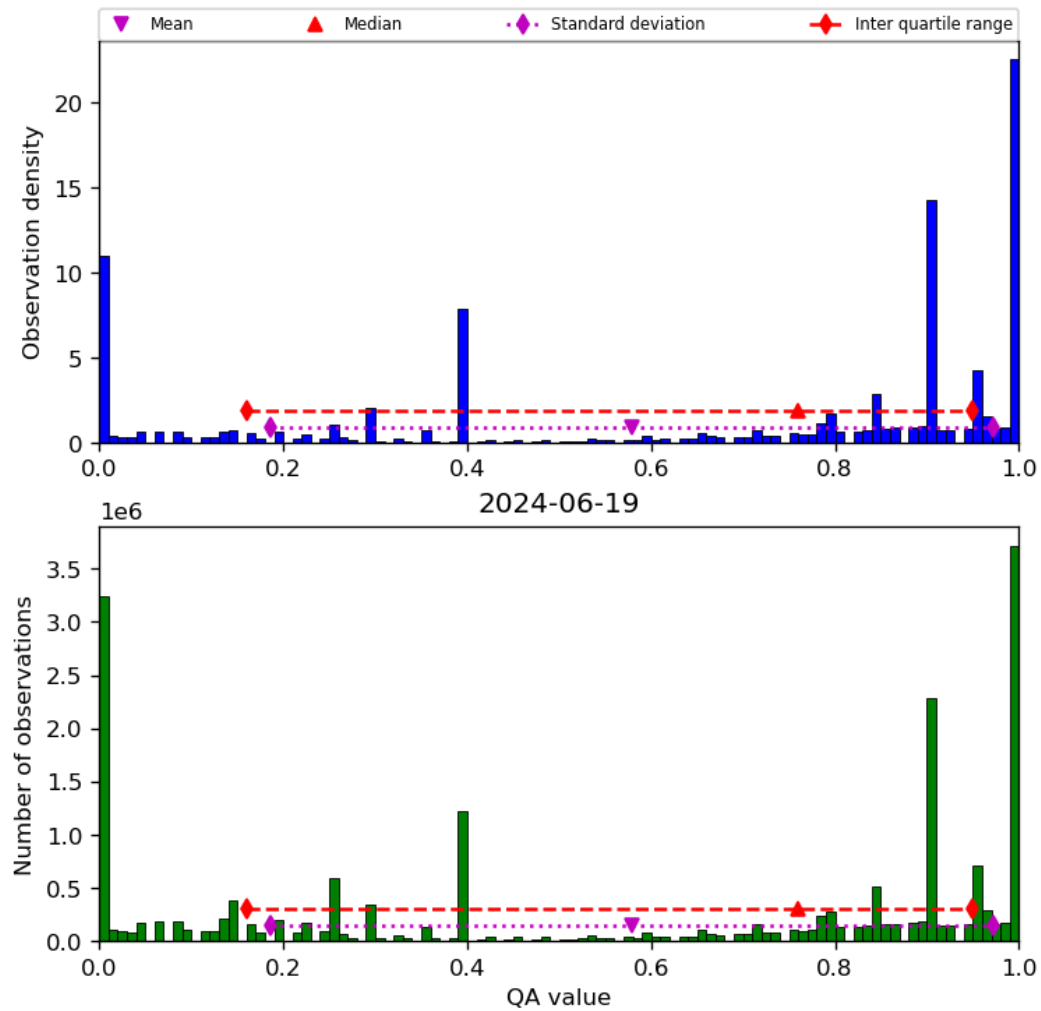
Figure 38: Histogram of “QA value” for 2024-06-19 to 2024-06-20
