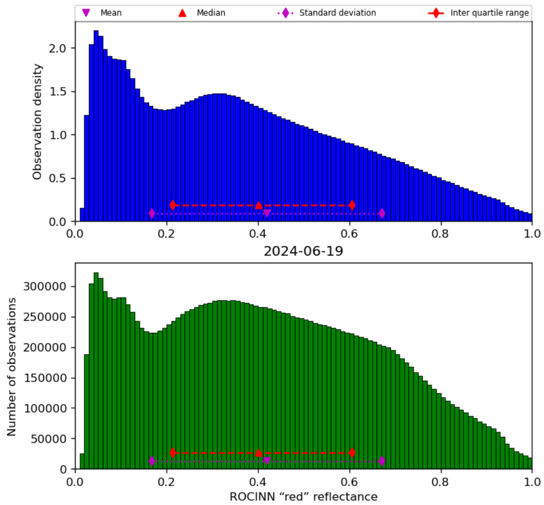
Figure 53: Histogram of “ROCINN “red” reflectance” for 2024-06-19 to 2024-06-20
