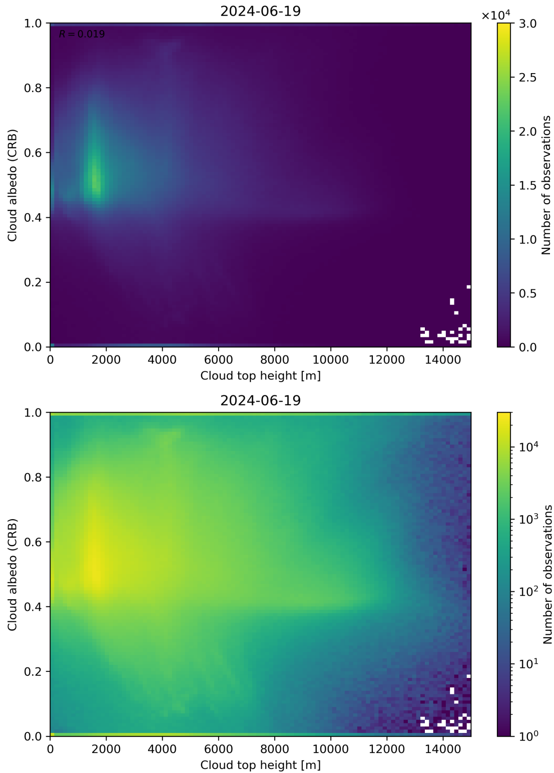
Figure 86: Scatter density plot of “Cloud top height” against “Cloud albedo (CRB)” for 2024-06-19 to 2024-06-20.
