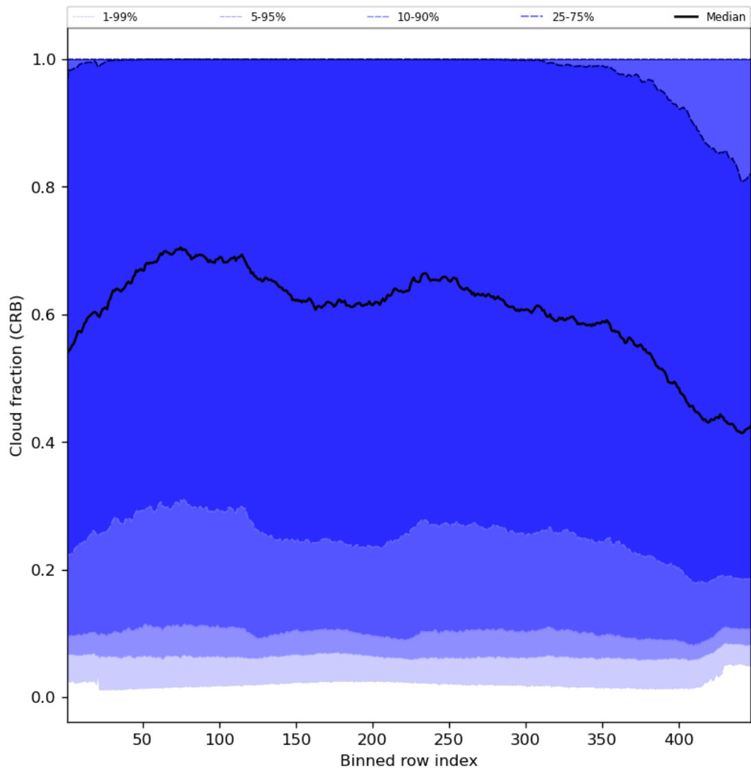
Figure 58: Along track statistics of “Cloud fraction (CRB)” for 2024-06-19 to 2024-06-20
