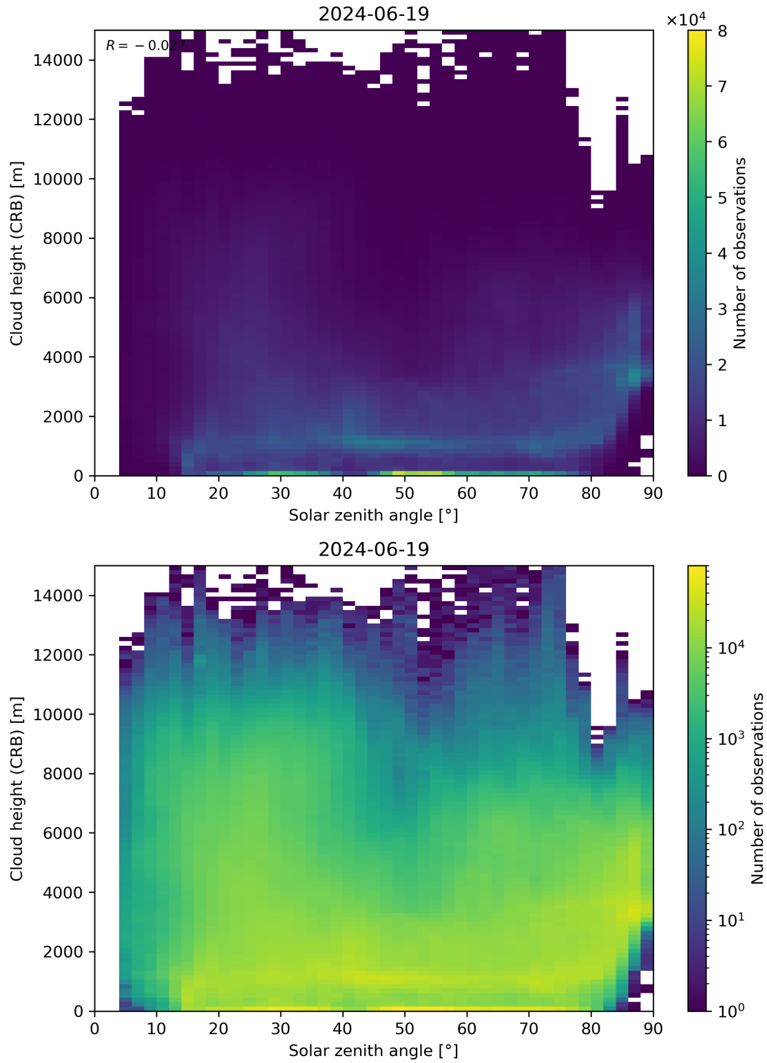
Figure 102: Scatter density plot of “Solar zenith angle” against “Cloud height (CRB)” for 2024-06-19 to 2024-06-20.
