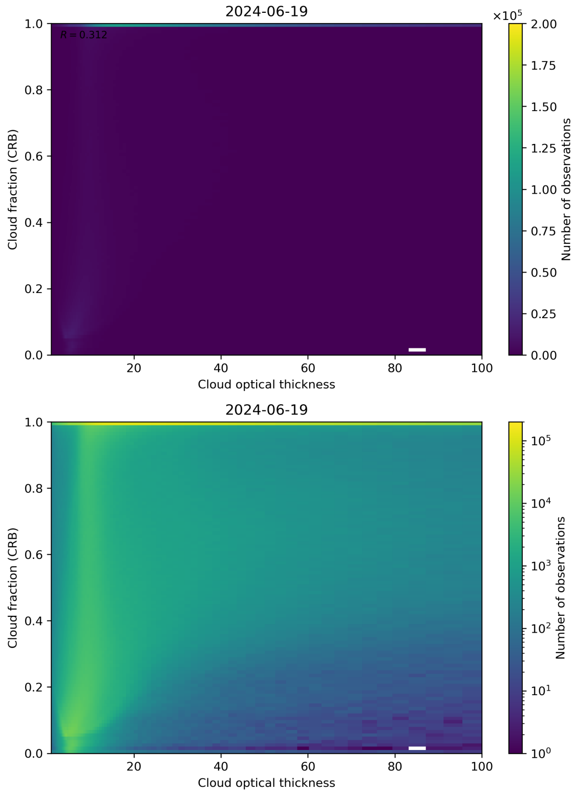
Figure 84: Scatter density plot of “Cloud optical thickness” against “Cloud fraction (CRB)” for 2024-06-19 to 2024-06-20.
