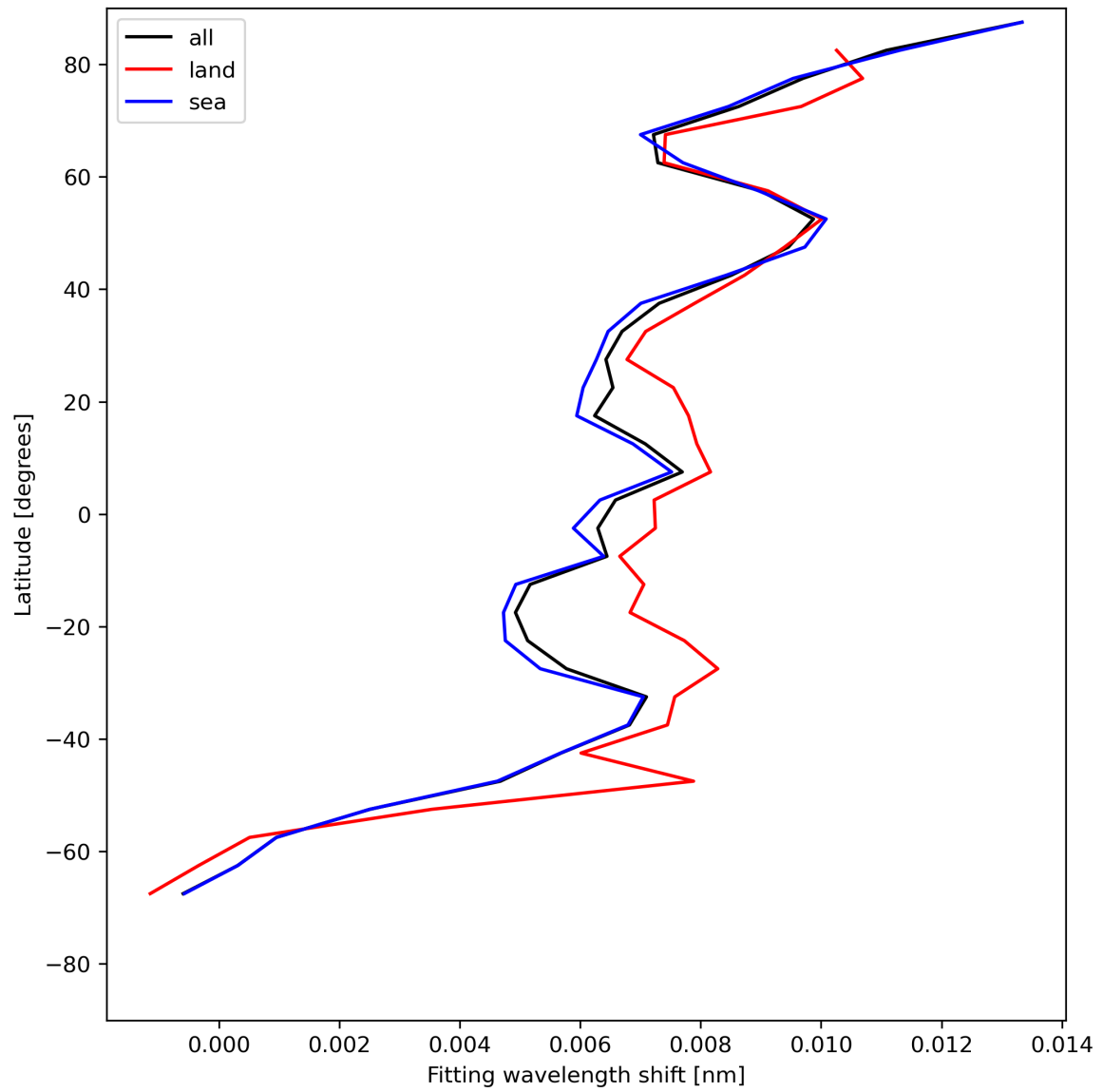
Figure 33: Zonal average of “Fitting wavelength shift” for 2024-06-19 to 2024-06-20.
