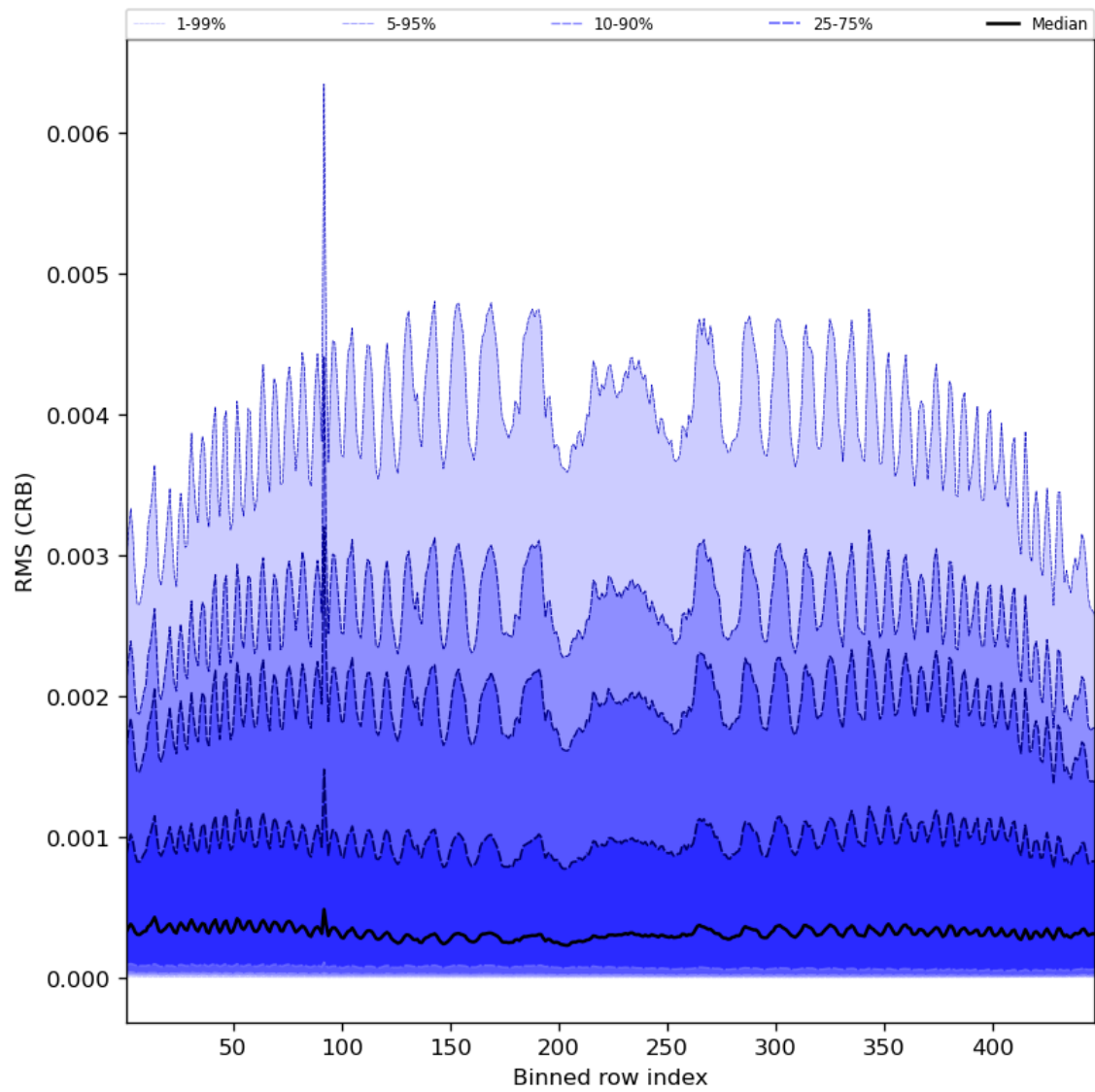
Figure 64: Along track statistics of “RMS (CRB)” for 2024-06-19 to 2024-06-20
