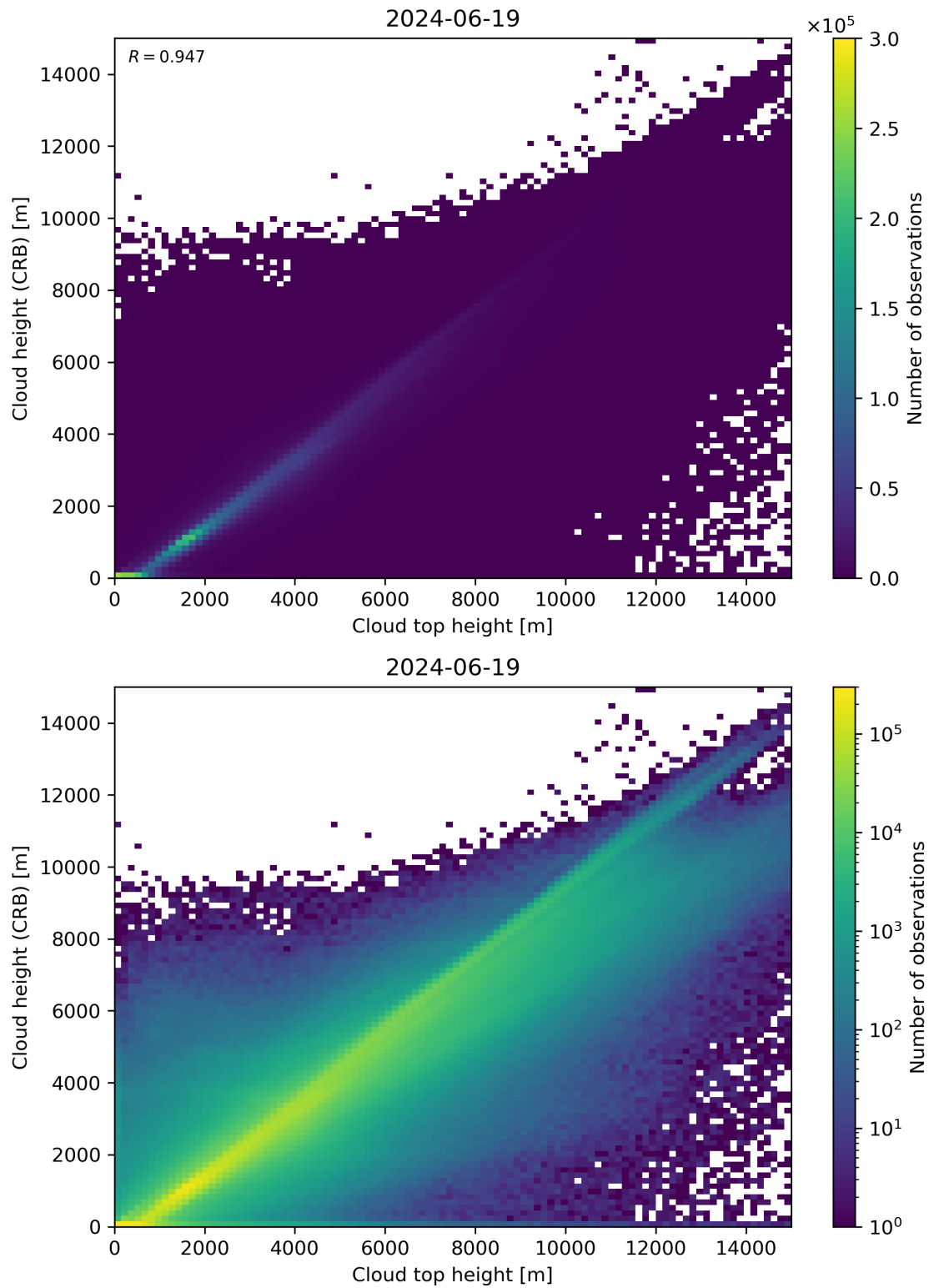
Figure 89: Scatter density plot of “Cloud top height” against “Cloud height (CRB)” for 2024-06-19 to 2024-06-20.
