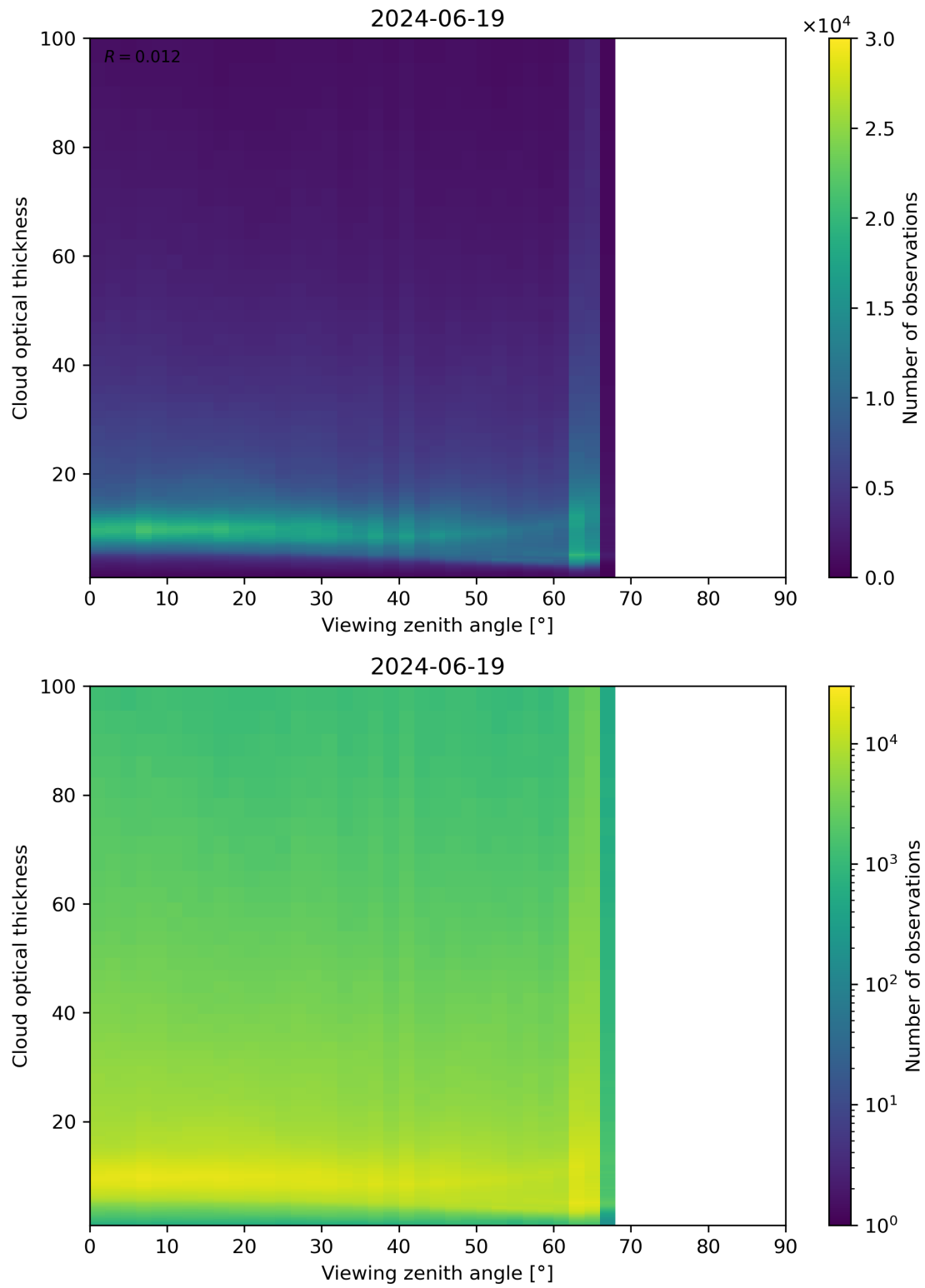
Figure 111: Scatter density plot of “Viewing zenith angle” against “Cloud optical thickness” for 2024-06-19 to 2024-06-20.
