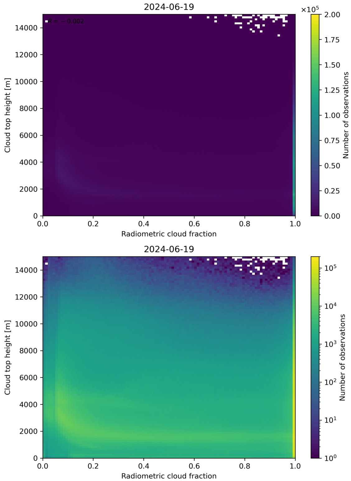
Figure 76: Scatter density plot of “Radiometric cloud fraction” against “Cloud top height” for 2024-06-19 to 2024-06-20.
