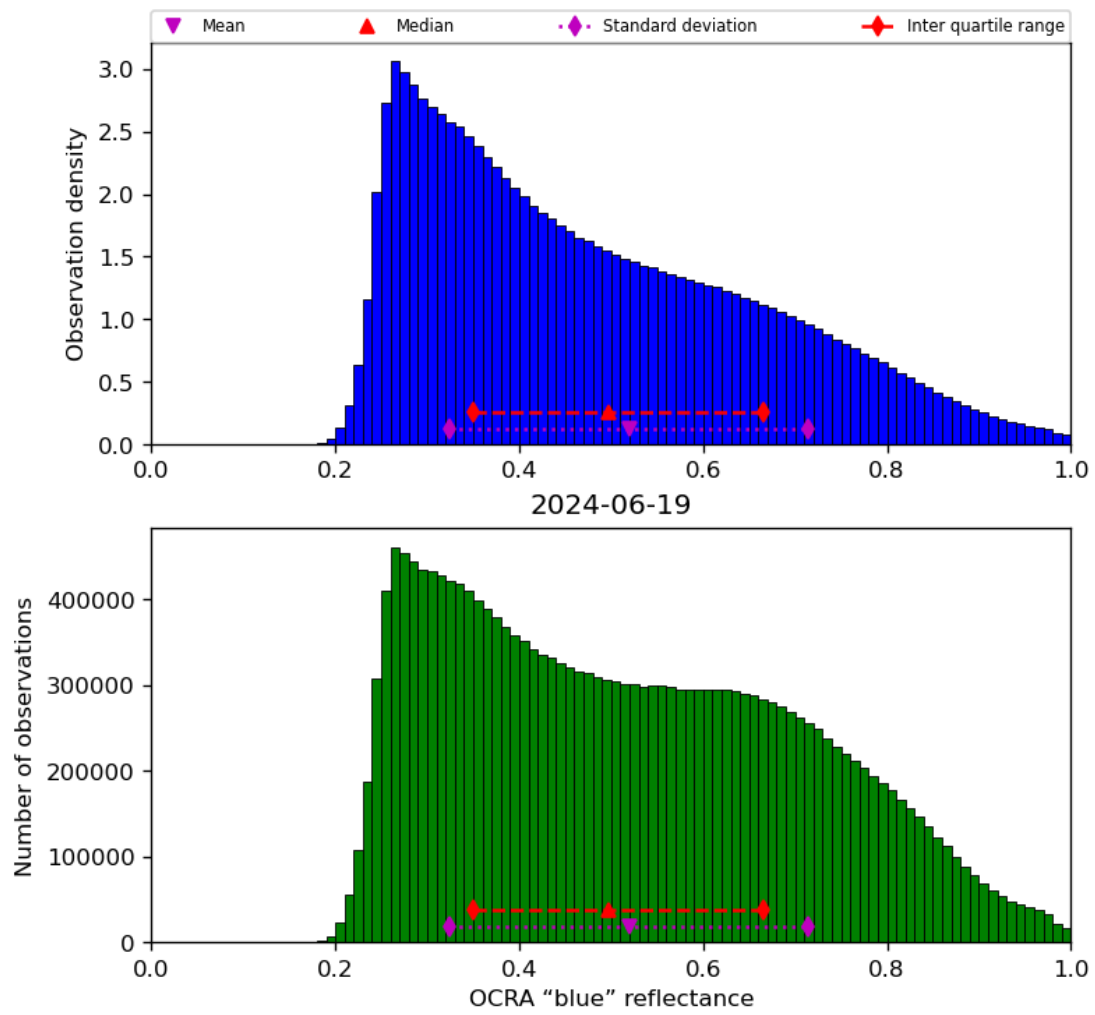
Figure 51: Histogram of “OCRA “blue” reflectance” for 2024-06-19 to 2024-06-20
