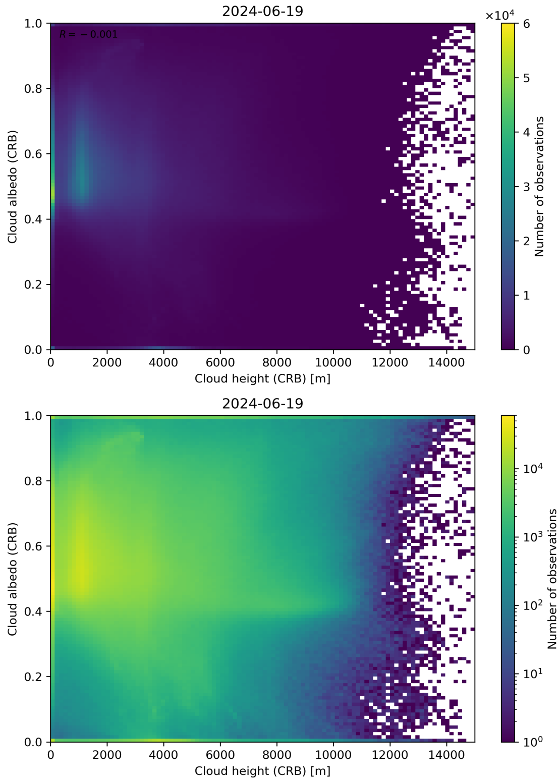
Figure 80: Scatter density plot of “Cloud height (CRB)” against “Cloud albedo (CRB)” for 2024-06-19 to 2024-06-20.
