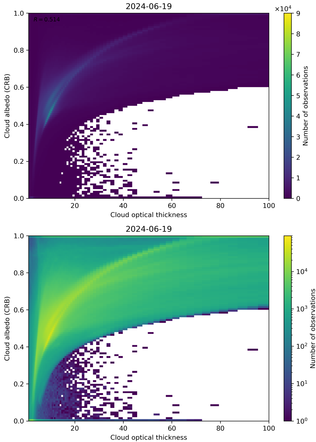
Figure 82: Scatter density plot of “Cloud optical thickness” against “Cloud albedo (CRB)” for 2024-06-19 to 2024-06-20.
