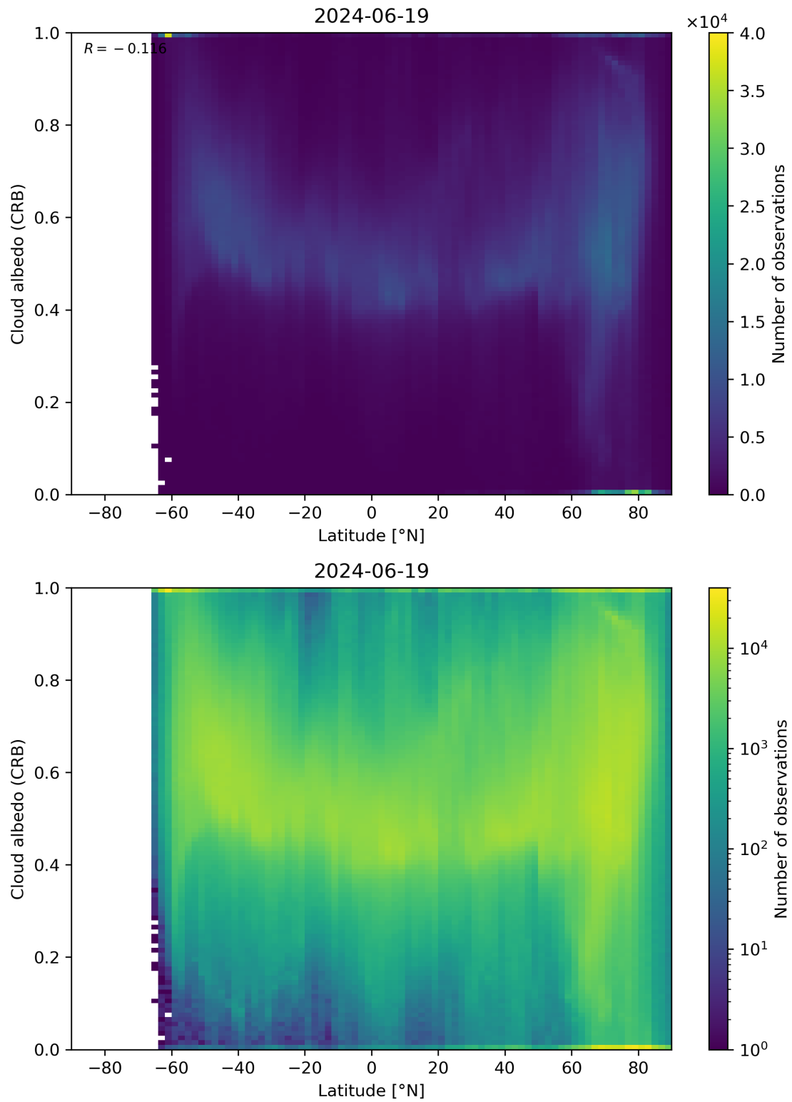
Figure 91: Scatter density plot of “Latitude” against “Cloud albedo (CRB)” for 2024-06-19 to 2024-06-20.
