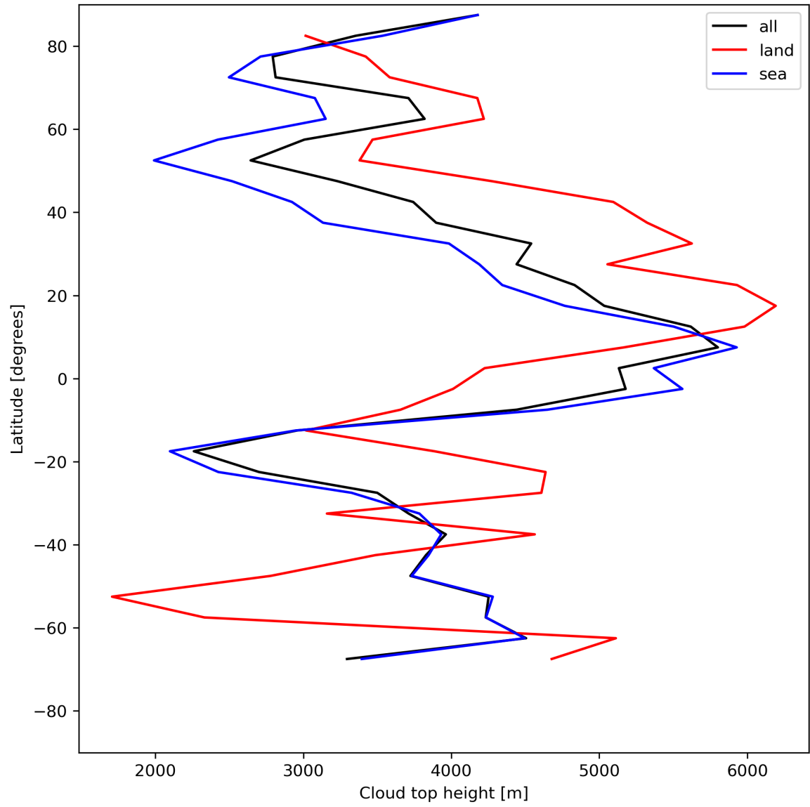
Figure 24: Zonal average of “Cloud top height” for 2024-06-19 to 2024-06-20.
