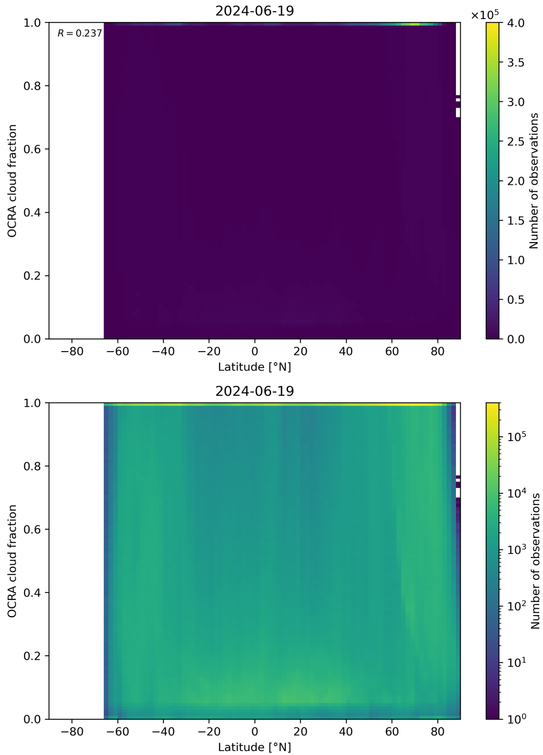
Figure 93: Scatter density plot of “Latitude” against “OCRA cloud fraction” for 2024-06-19 to 2024-06-20.
