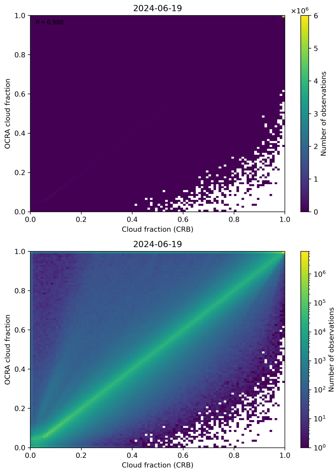
Figure 78: Scatter density plot of “Cloud fraction (CRB)” against “OCRA cloud fraction” for 2024-06-19 to 2024-06-20.
