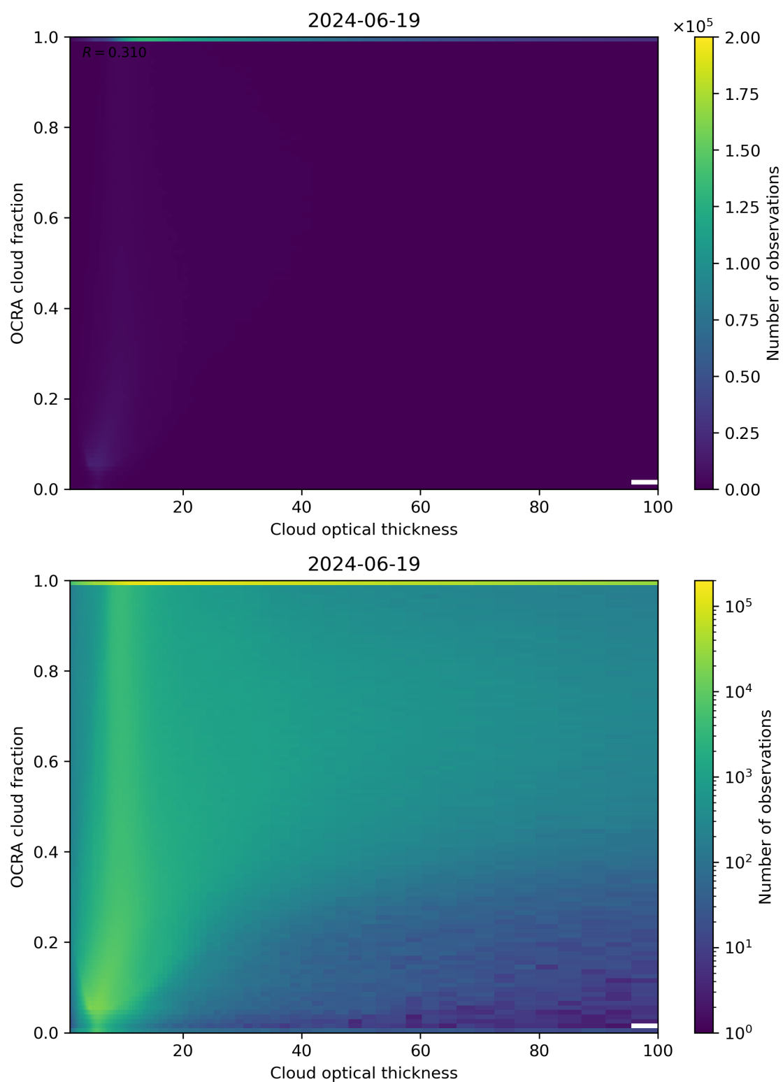
Figure 83: Scatter density plot of “Cloud optical thickness” against “OCRA cloud fraction” for 2024-06-19 to 2024-06-20.
