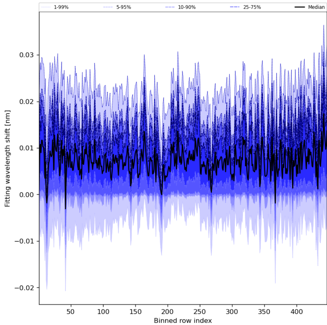
Figure 65: Along track statistics of “Fitting wavelength shift” for 2024-06-19 to 2024-06-20
