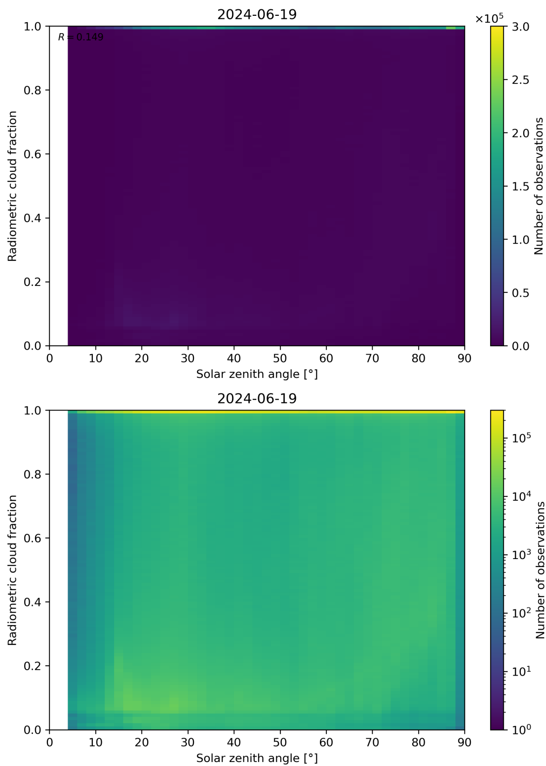
Figure 99: Scatter density plot of “Solar zenith angle” against “Radiometric cloud fraction” for 2024-06-19 to 2024-06-20.
