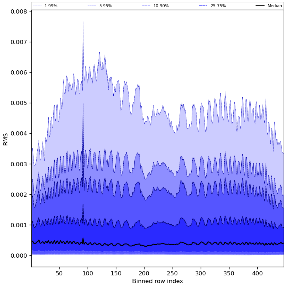
Figure 63: Along track statistics of “RMS” for 2024-06-19 to 2024-06-20
