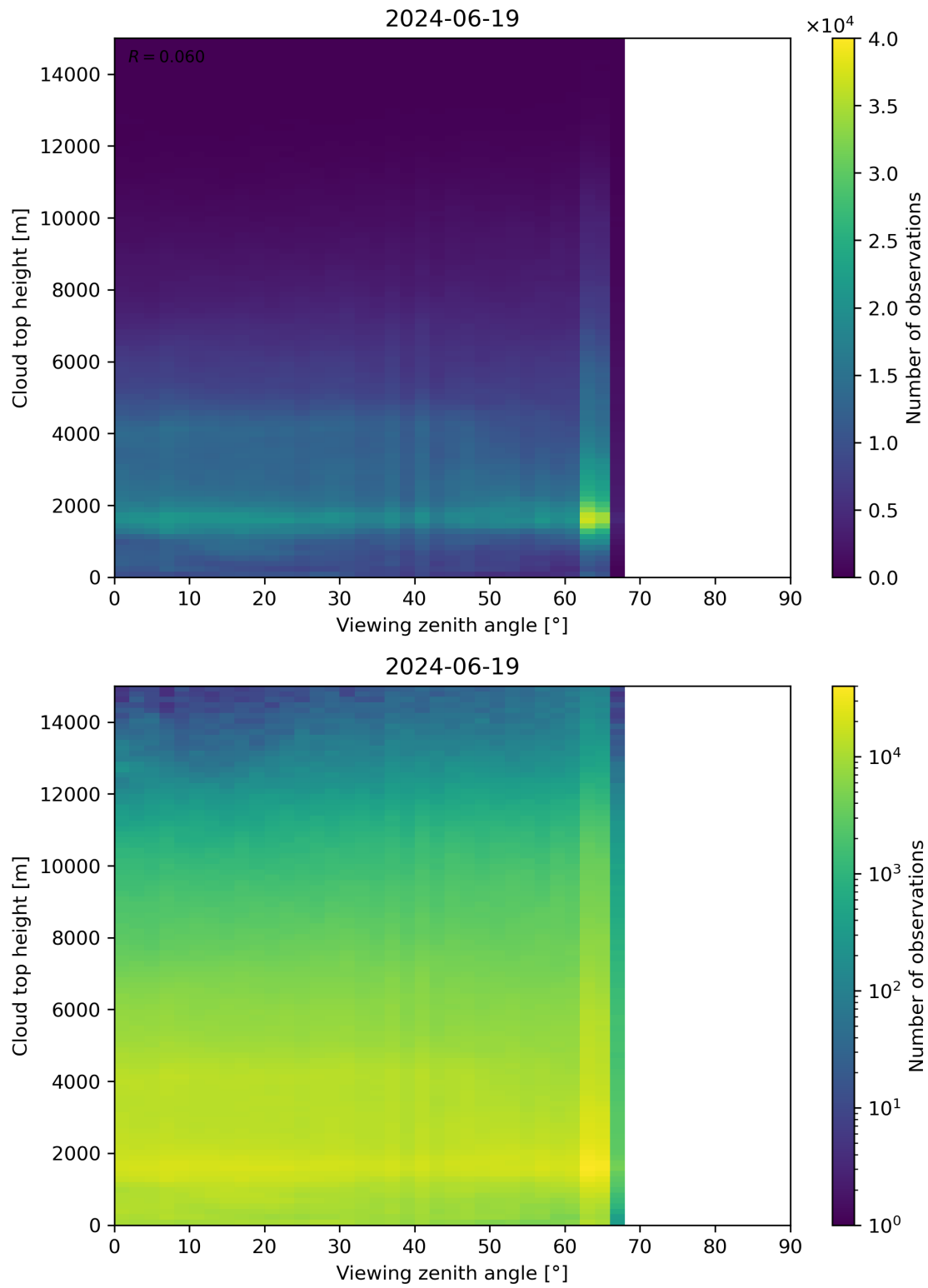
Figure 112: Scatter density plot of “Viewing zenith angle” against “Cloud top height” for 2024-06-19 to 2024-06-20.
