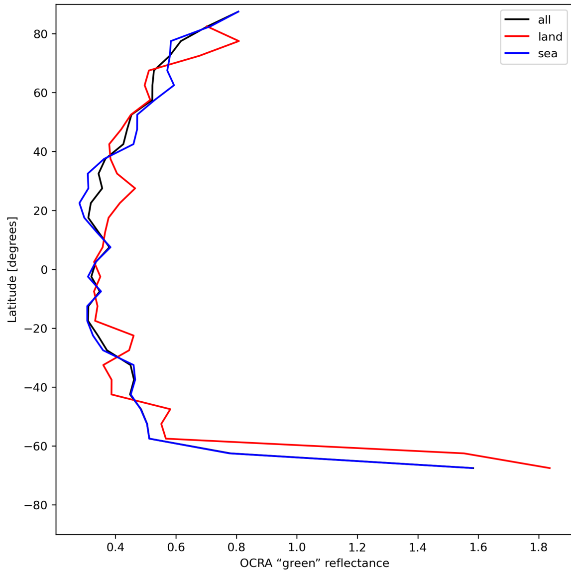
Figure 36: Zonal average of “OCRA “green” reflectance” for 2024-06-19 to 2024-06-20.
