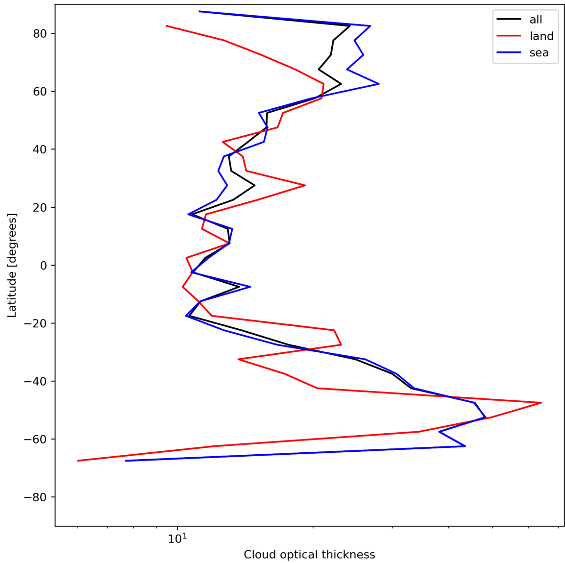
Figure 25: Zonal average of “Cloud optical thickness” for 2024-06-19 to 2024-06-20.
