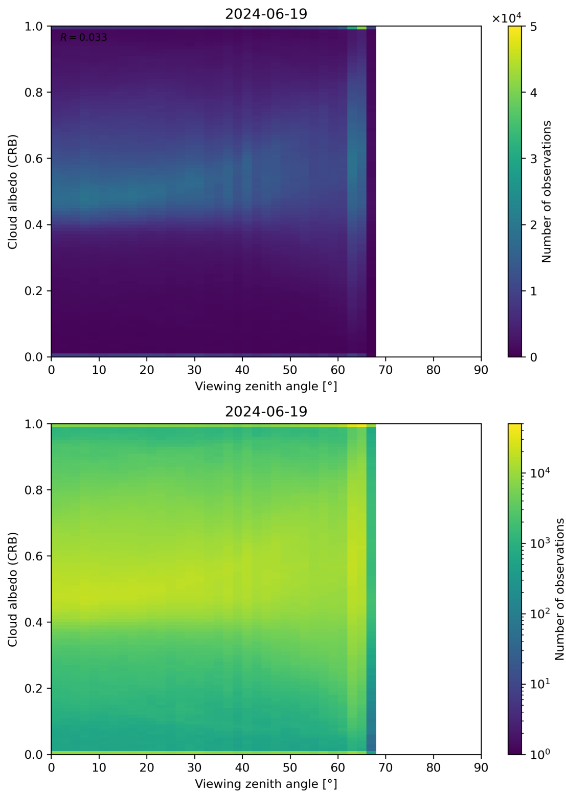
Figure 106: Scatter density plot of “Viewing zenith angle” against “Cloud albedo (CRB)” for 2024-06-19 to 2024-06-20.
