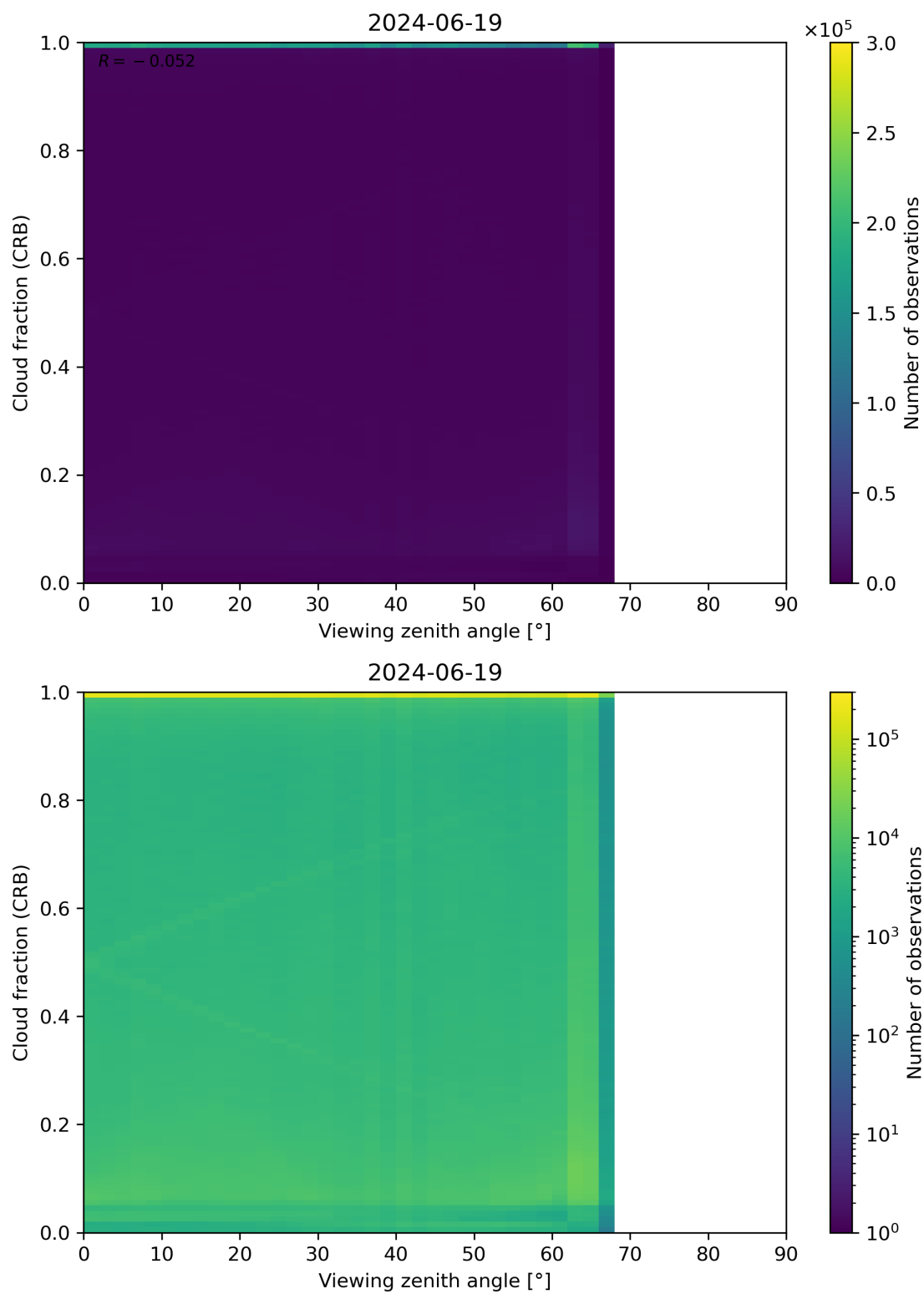
Figure 109: Scatter density plot of “Viewing zenith angle” against “Cloud fraction (CRB)” for 2024-06-19 to 2024-06-20.
