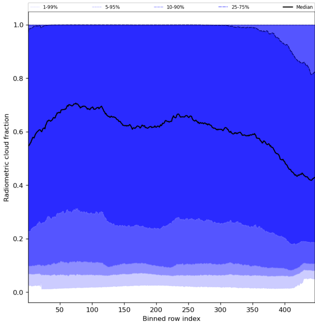
Figure 55: Along track statistics of “Radiometric cloud fraction” for 2024-06-19 to 2024-06-20
