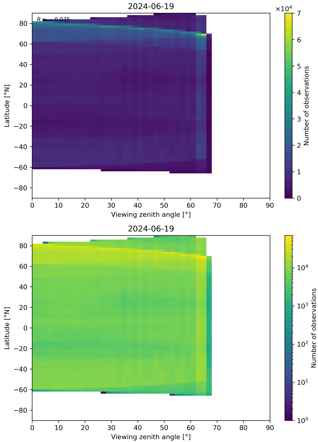
Figure 113: Scatter density plot of “Viewing zenith angle” against “Latitude” for 2024-06-19 to 2024-06-20.
