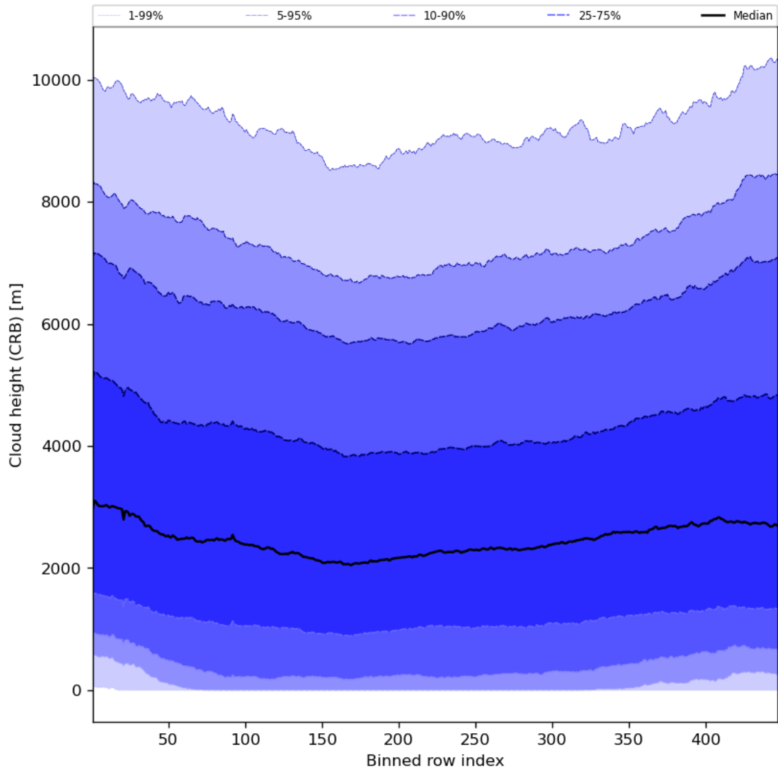
Figure 59: Along track statistics of “Cloud height (CRB)” for 2024-06-19 to 2024-06-20
