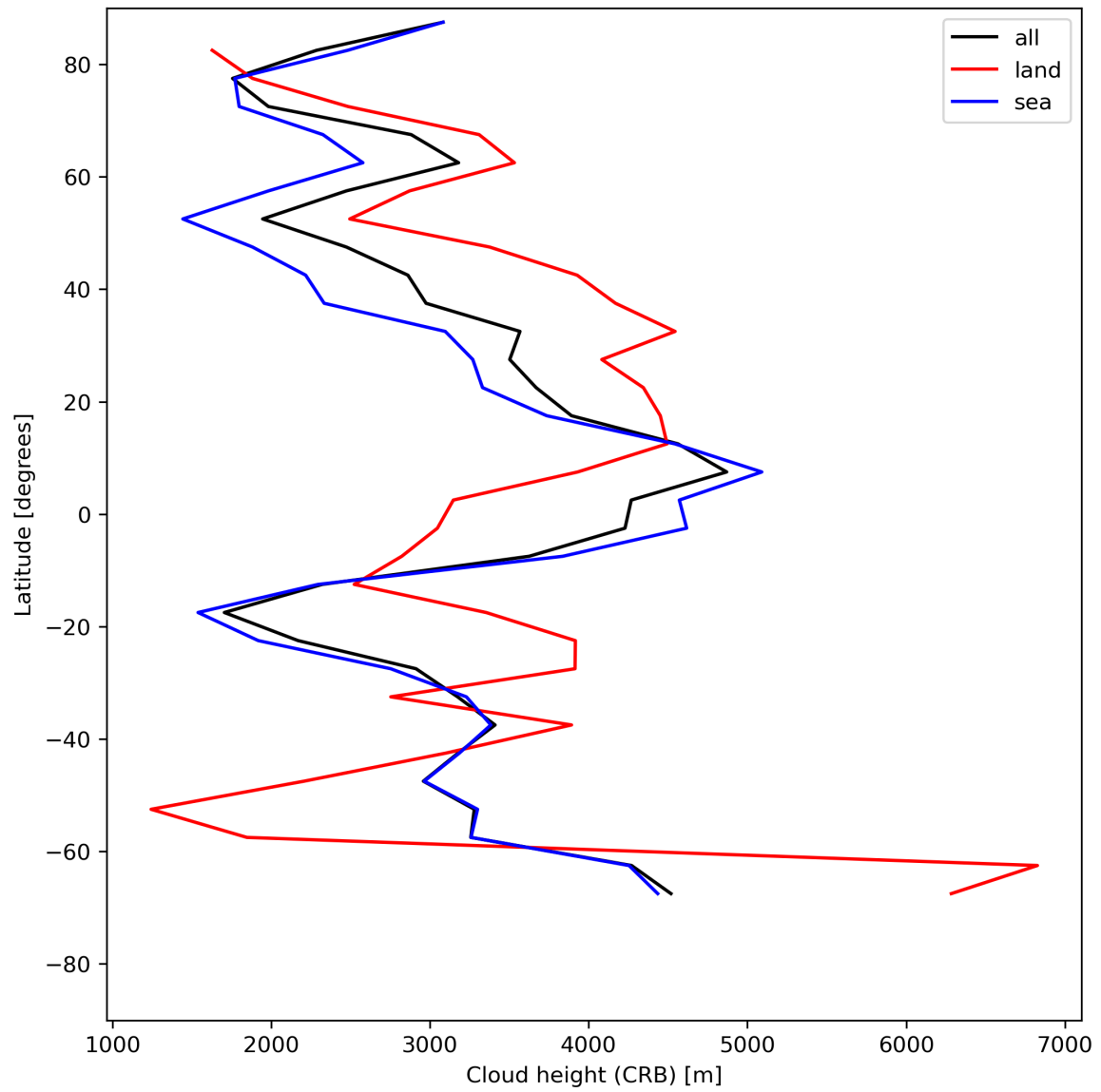
Figure 27: Zonal average of “Cloud height (CRB)” for 2024-06-19 to 2024-06-20.
