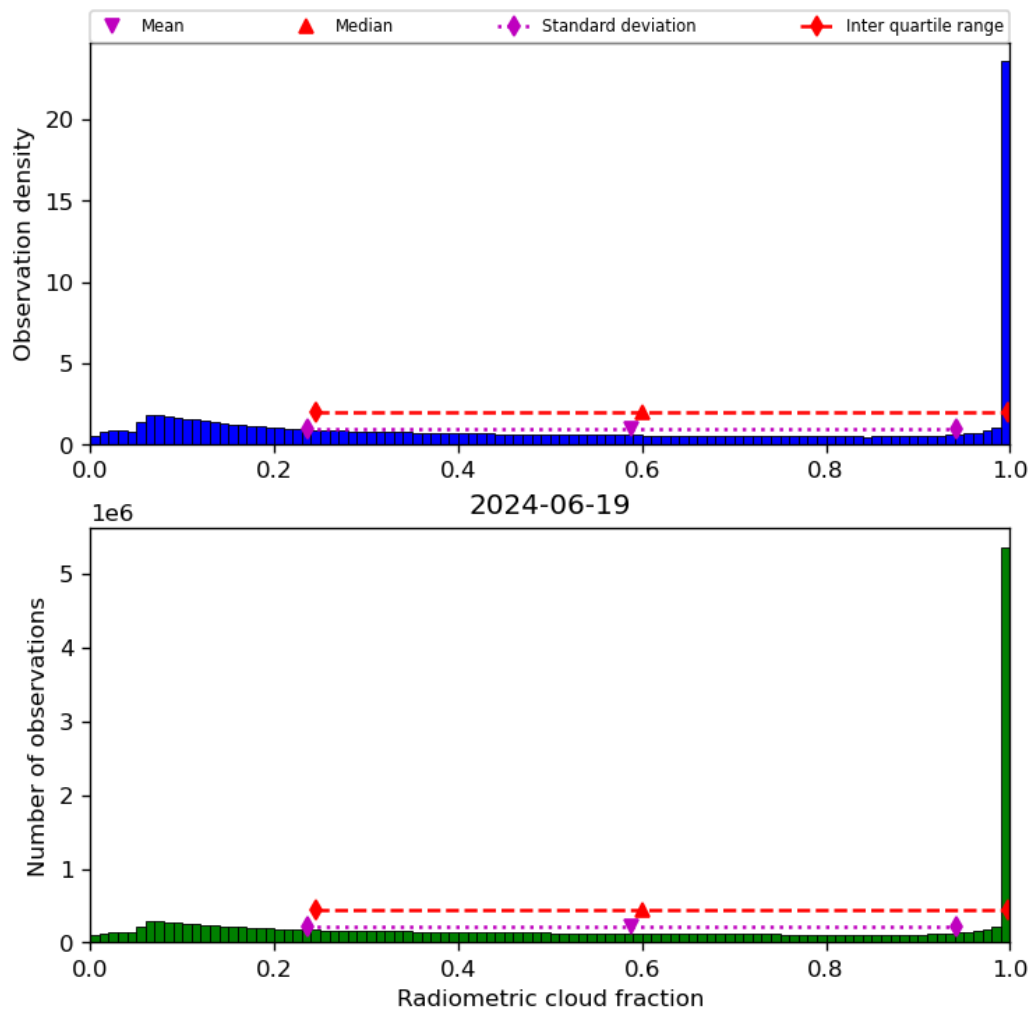
Figure 39: Histogram of “Radiometric cloud fraction” for 2024-06-19 to 2024-06-20
