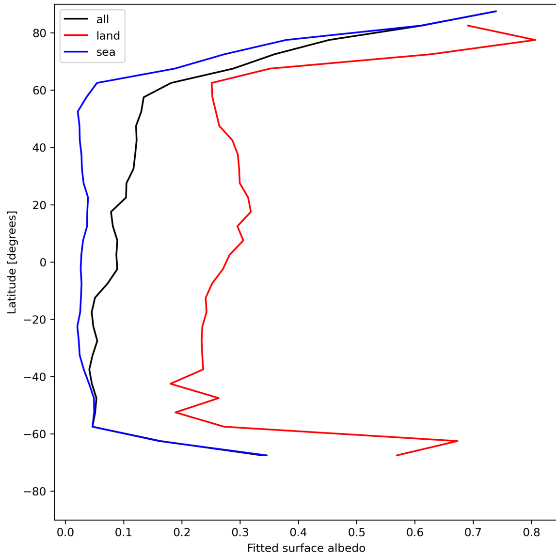
Figure 29: Zonal average of “Fitted surface albedo” for 2024-06-19 to 2024-06-20.
