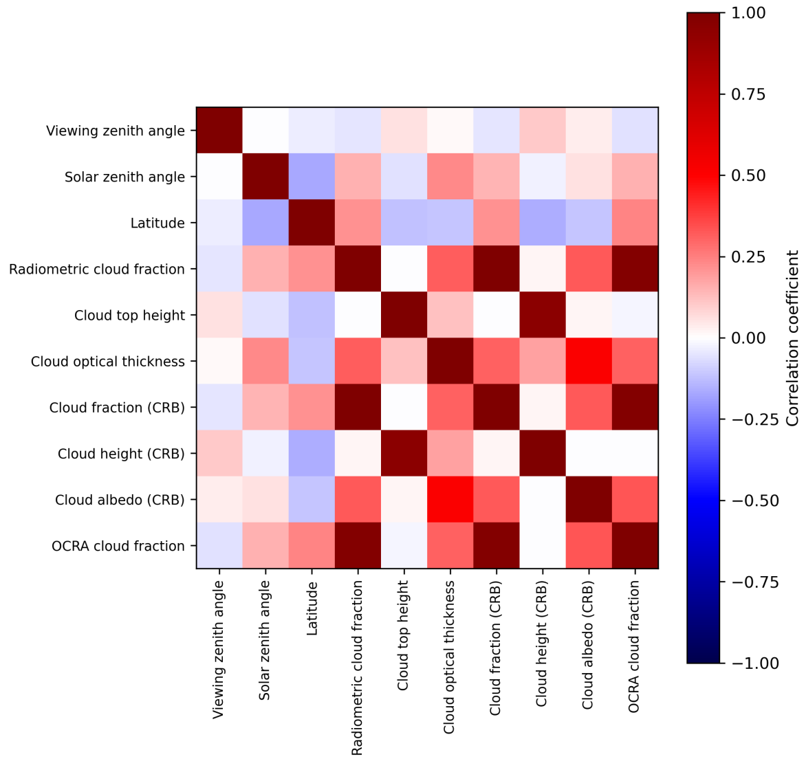
Figure 2: Map of correlation matrix for 2024-06-19 to 2024-06-20.
