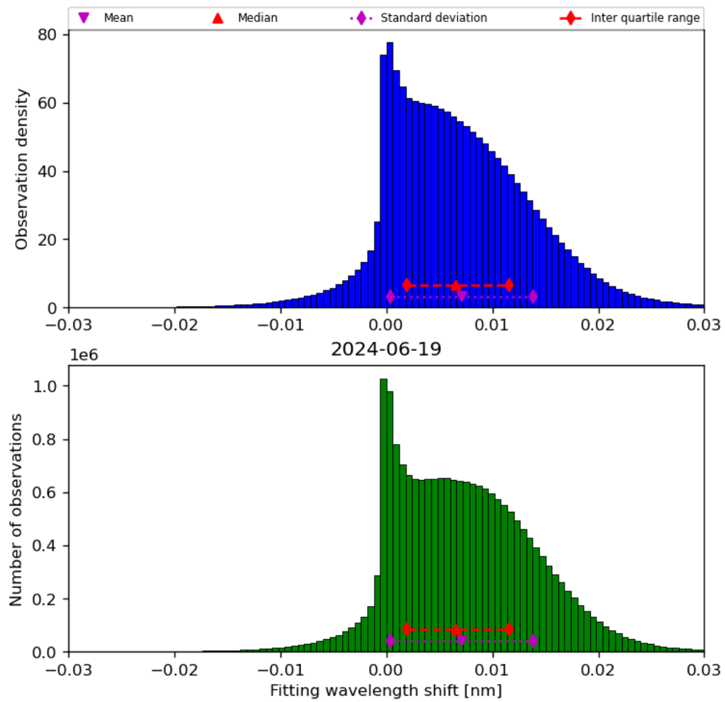
Figure 49: Histogram of “Fitting wavelength shift” for 2024-06-19 to 2024-06-20
