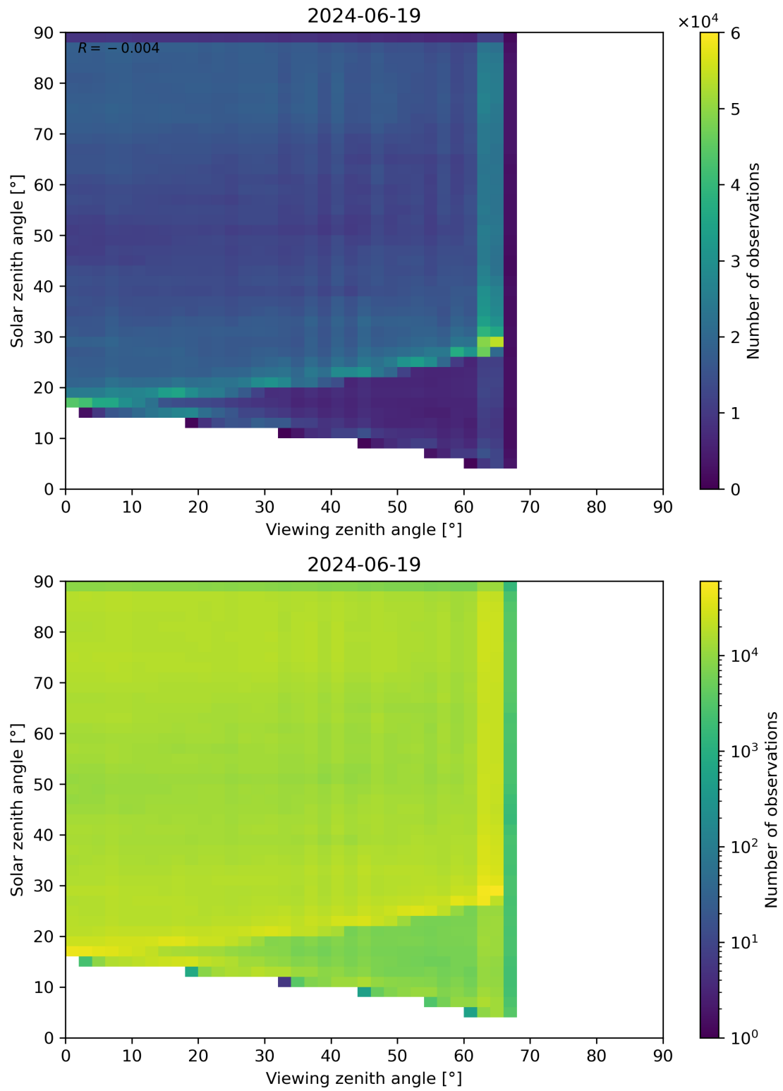
Figure 114: Scatter density plot of “Viewing zenith angle” against “Solar zenith angle” for 2024-06-19 to 2024-06-20.
