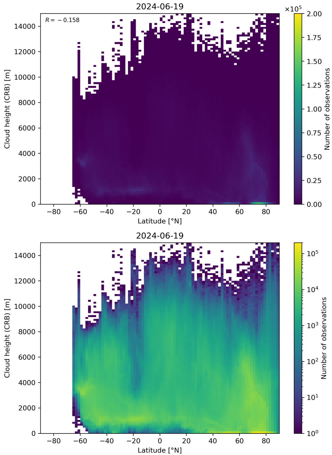
Figure 95: Scatter density plot of “Latitude” against “Cloud height (CRB)” for 2024-06-19 to 2024-06-20.
