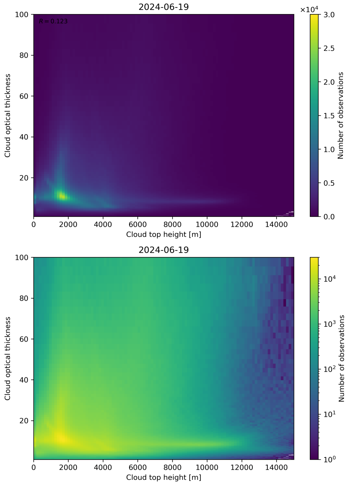
Figure 90: Scatter density plot of “Cloud top height” against “Cloud optical thickness” for 2024-06-19 to 2024-06-20.
