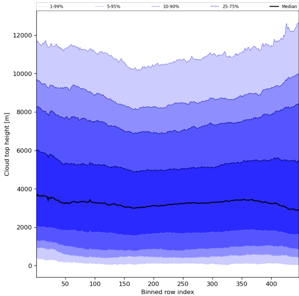
Figure 56: Along track statistics of “Cloud top height” for 2024-06-19 to 2024-06-20
