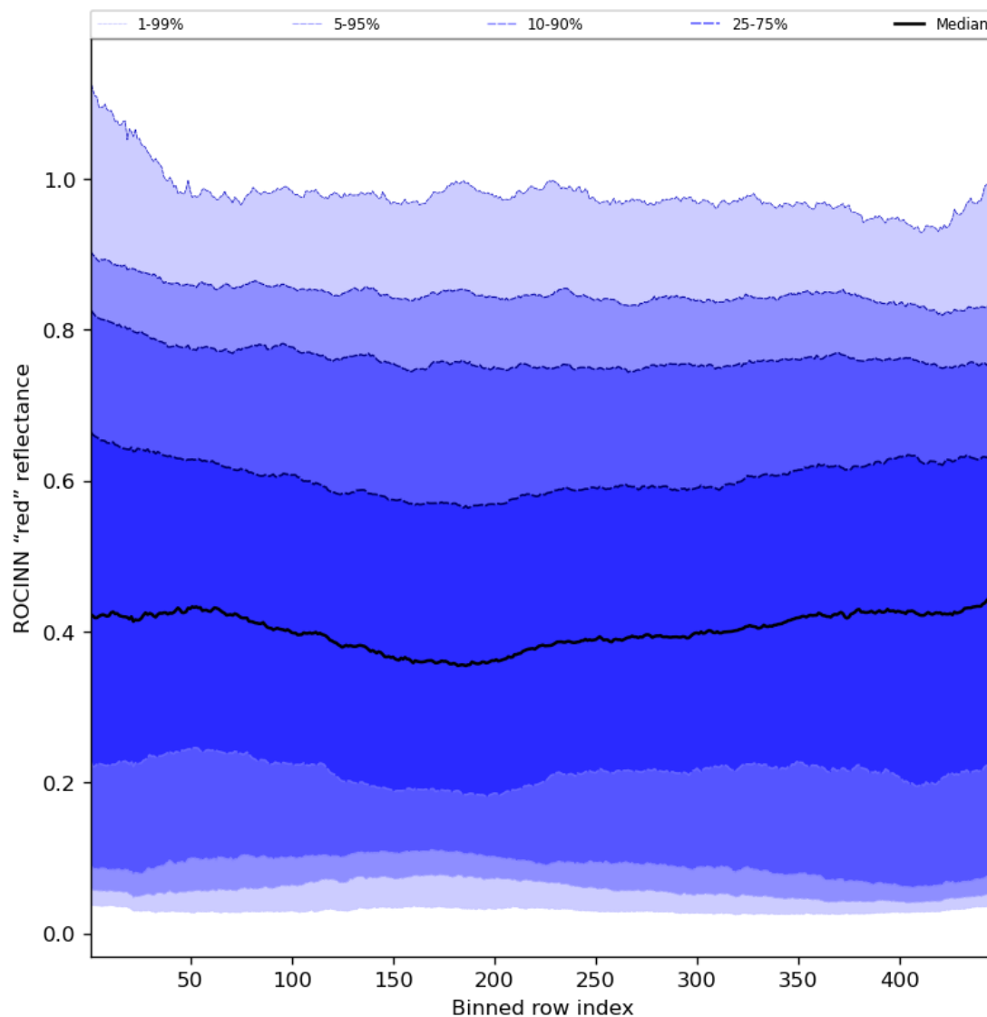
Figure 69: Along track statistics of “ROCINN “red” reflectance” for 2024-06-19 to 2024-06-20
