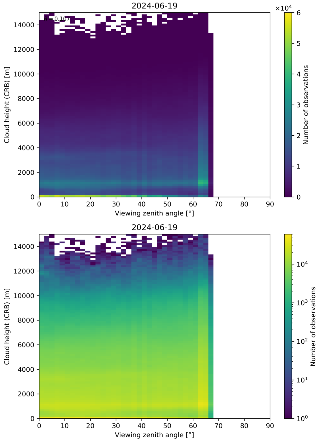
Figure 110: Scatter density plot of “Viewing zenith angle” against “Cloud height (CRB)” for 2024-06-19 to 2024-06-20.
