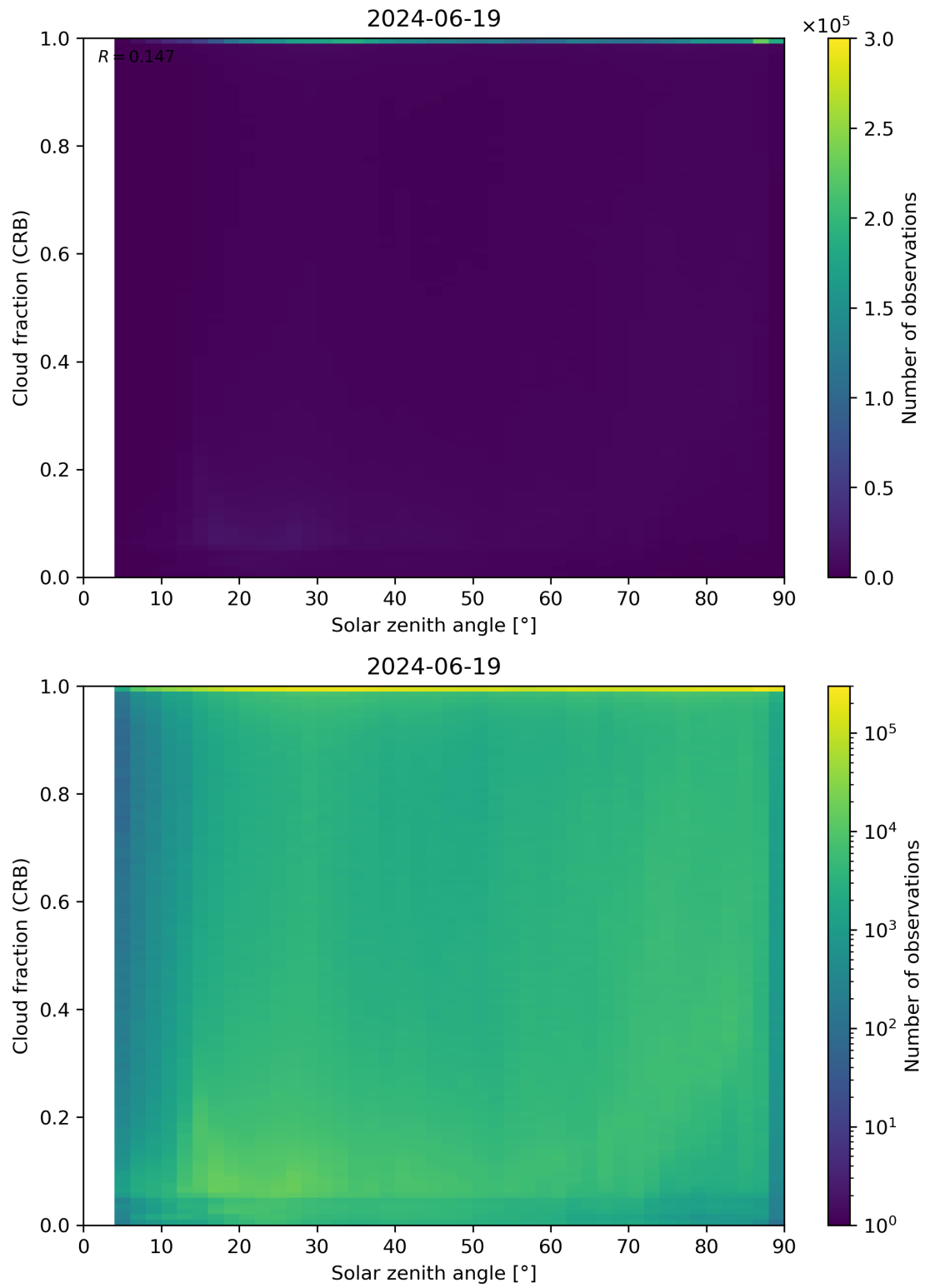
Figure 101: Scatter density plot of “Solar zenith angle” against “Cloud fraction (CRB)” for 2024-06-19 to 2024-06-20.
