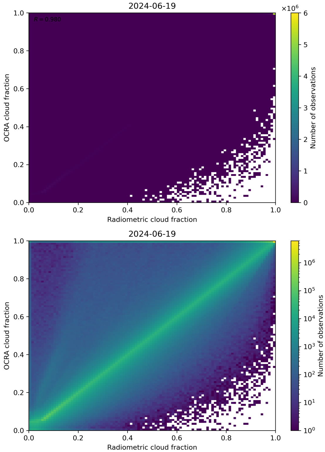
Figure 72: Scatter density plot of “Radiometric cloud fraction” against “OCRA cloud fraction” for 2024-06-19 to 2024-06-20.
