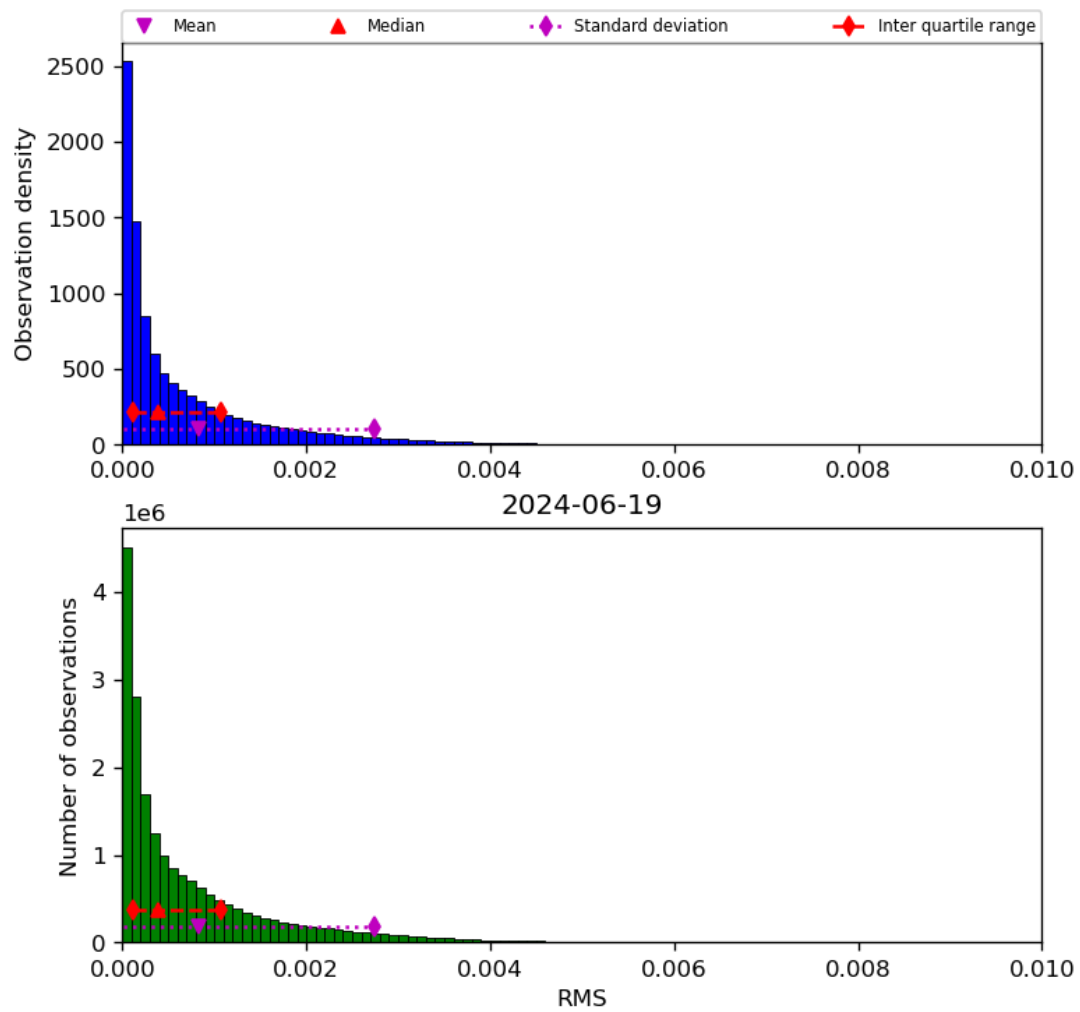
Figure 47: Histogram of “RMS” for 2024-06-19 to 2024-06-20
