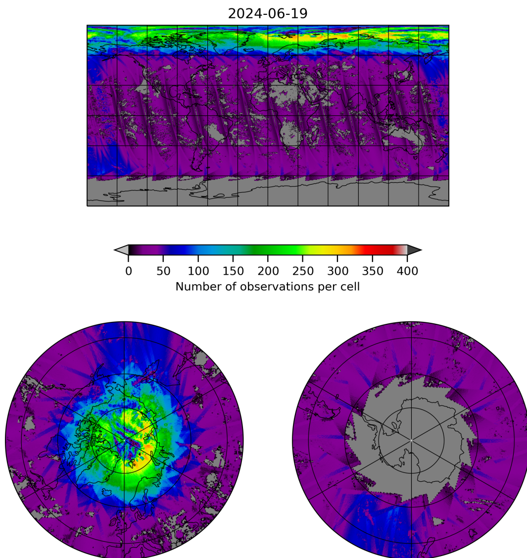
Figure 21: Map of the number of observations for 2024-06-19 to 2024-06-20
