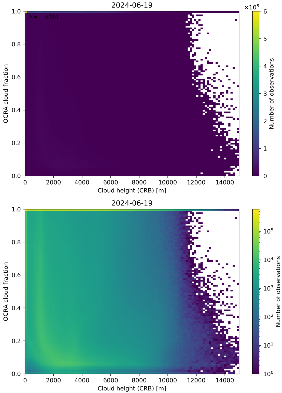
Figure 81: Scatter density plot of “Cloud height (CRB)” against “OCRA cloud fraction” for 2024-06-19 to 2024-06-20.
