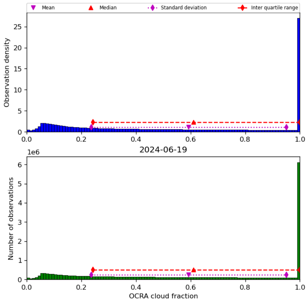
Figure 50: Histogram of “OCRA cloud fraction” for 2024-06-19 to 2024-06-20
