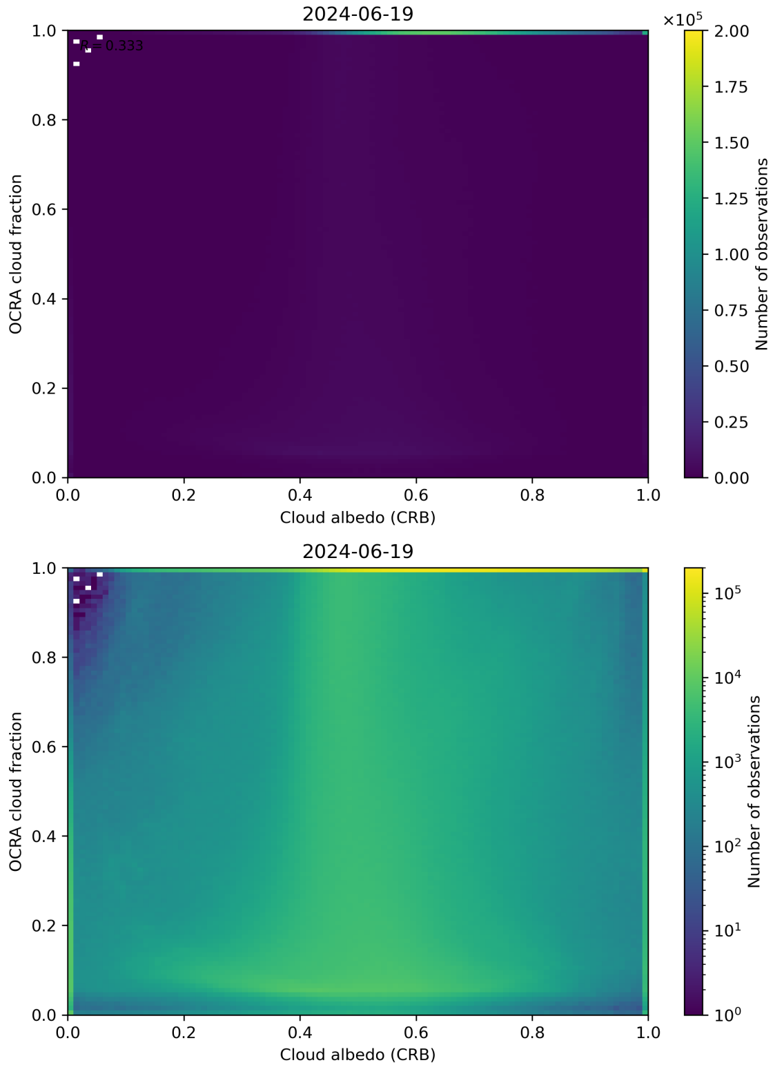
Figure 70: Scatter density plot of “Cloud albedo (CRB)” against “OCRA cloud fraction” for 2024-06-19 to 2024-06-20.
