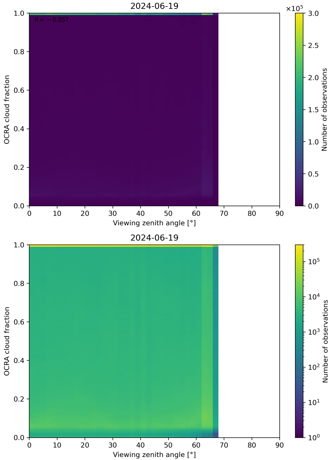
Figure 108: Scatter density plot of “Viewing zenith angle” against “OCRA cloud fraction” for 2024-06-19 to 2024-06-20.
