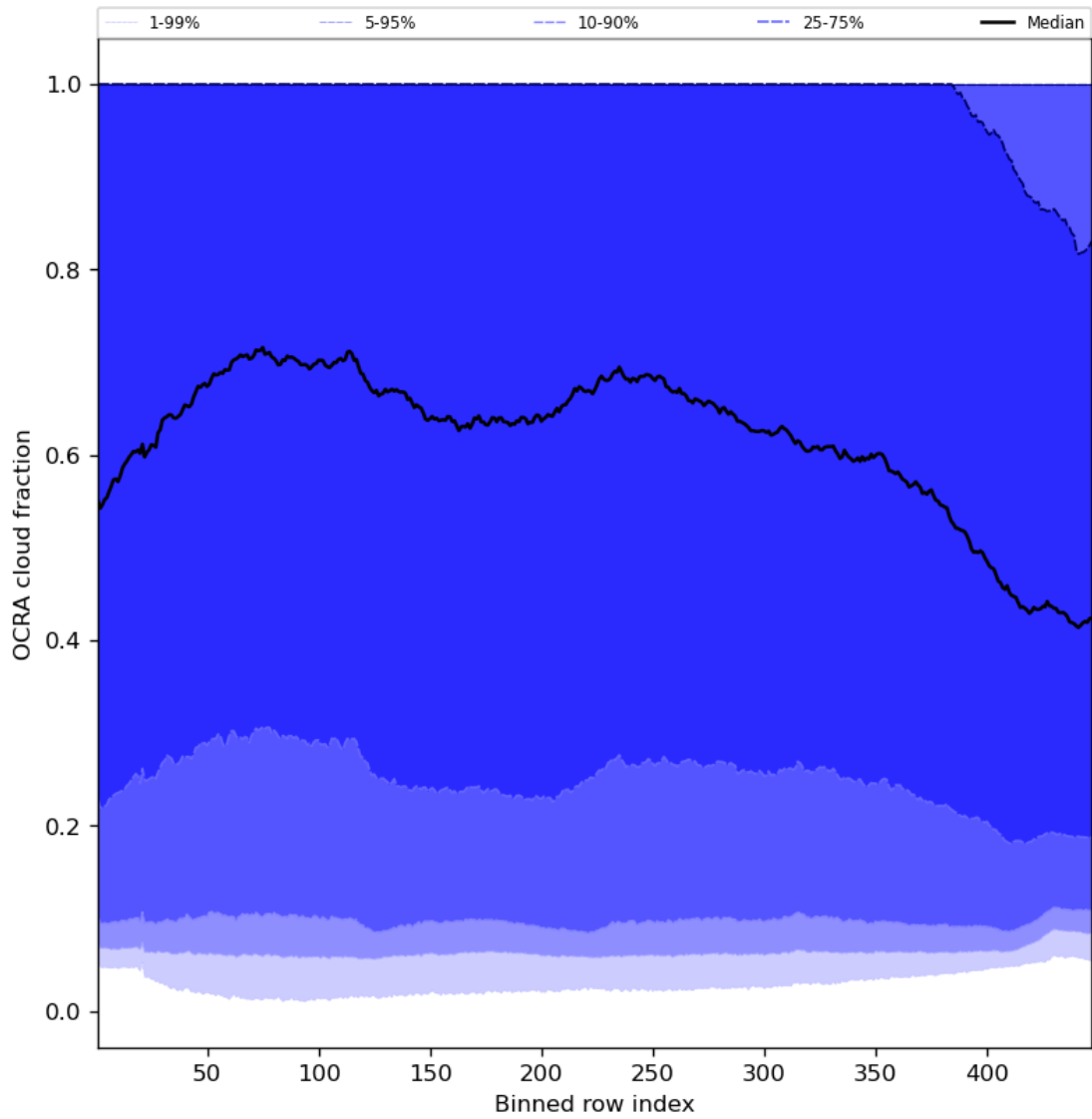
Figure 66: Along track statistics of “OCRA cloud fraction” for 2024-06-19 to 2024-06-20
