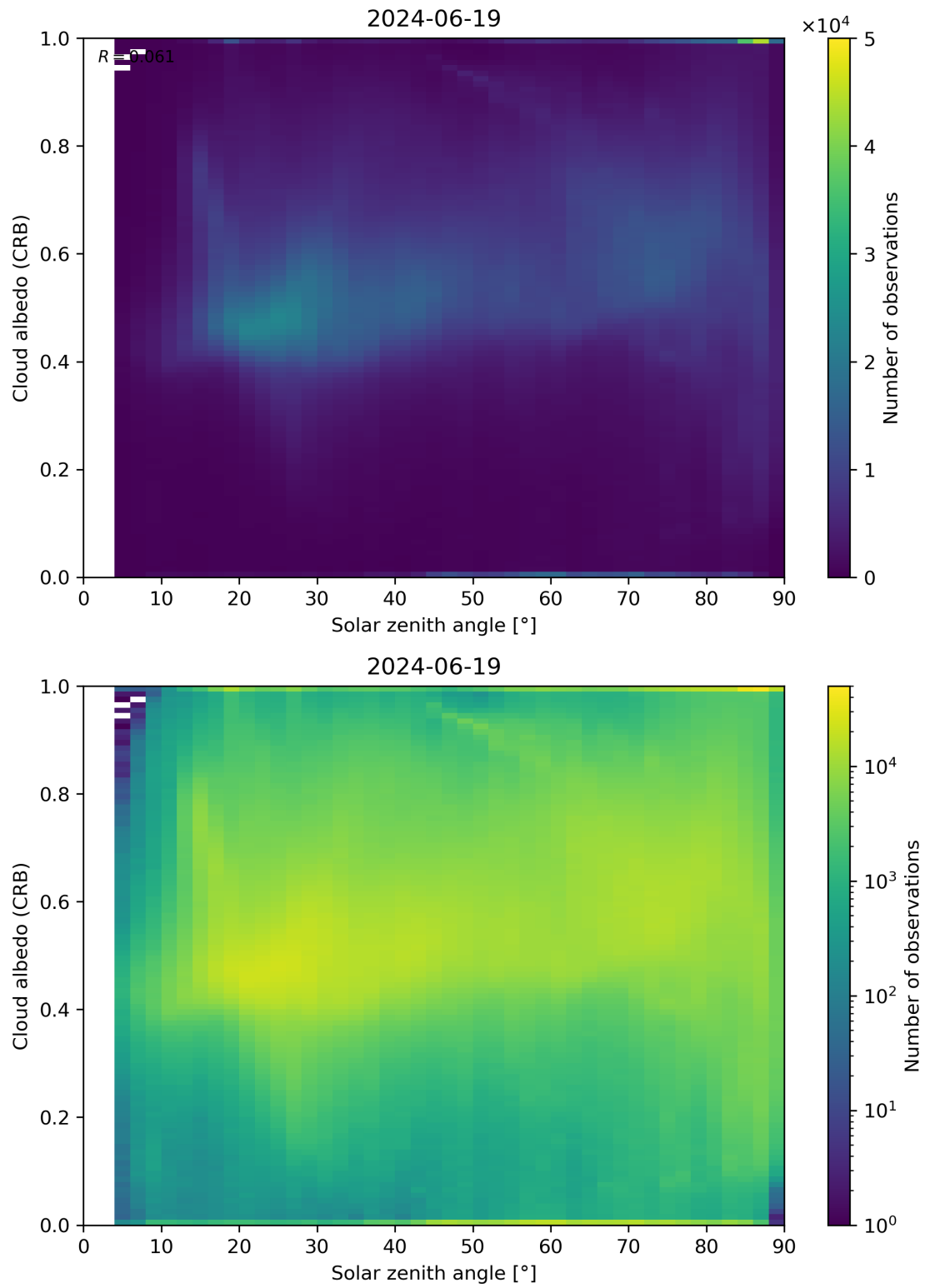
Figure 98: Scatter density plot of “Solar zenith angle” against “Cloud albedo (CRB)” for 2024-06-19 to 2024-06-20.
