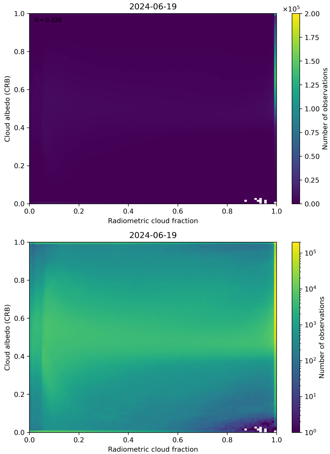
Figure 71: Scatter density plot of “Radiometric cloud fraction” against “Cloud albedo (CRB)” for 2024-06-19 to 2024-06-20.
