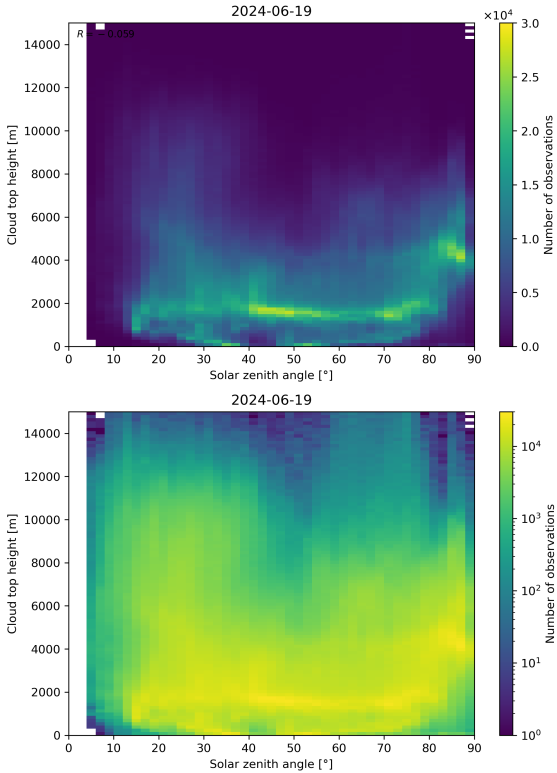
Figure 104: Scatter density plot of “Solar zenith angle” against “Cloud top height” for 2024-06-19 to 2024-06-20.
