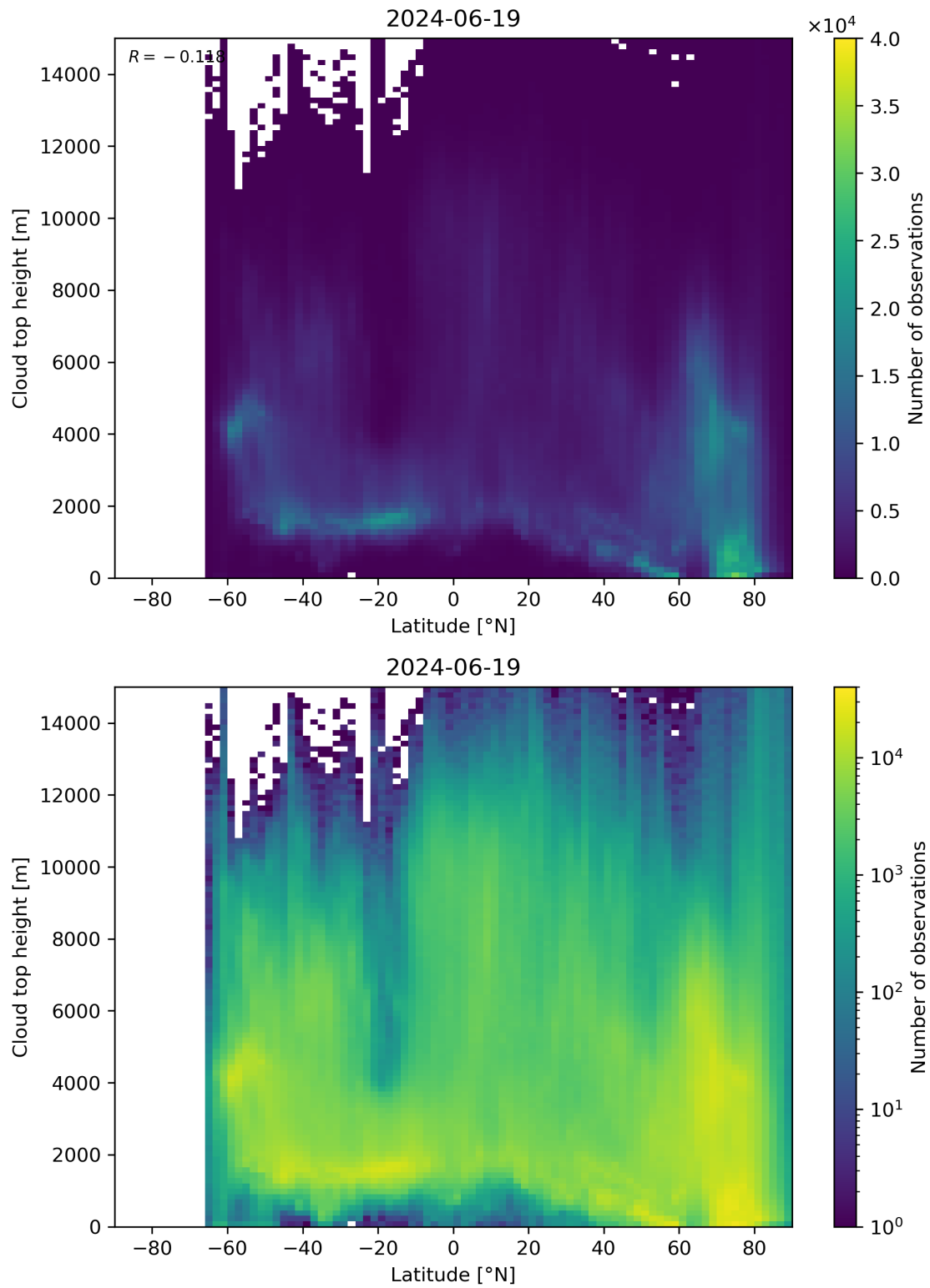
Figure 97: Scatter density plot of “Latitude” against “Cloud top height” for 2024-06-19 to 2024-06-20.
