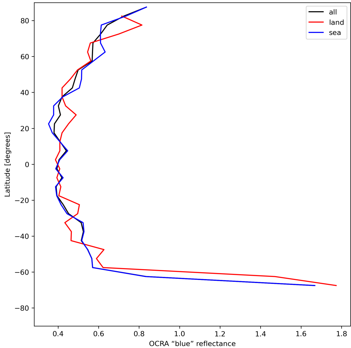
Figure 35: Zonal average of “OCRA “blue” reflectance” for 2024-06-19 to 2024-06-20.
