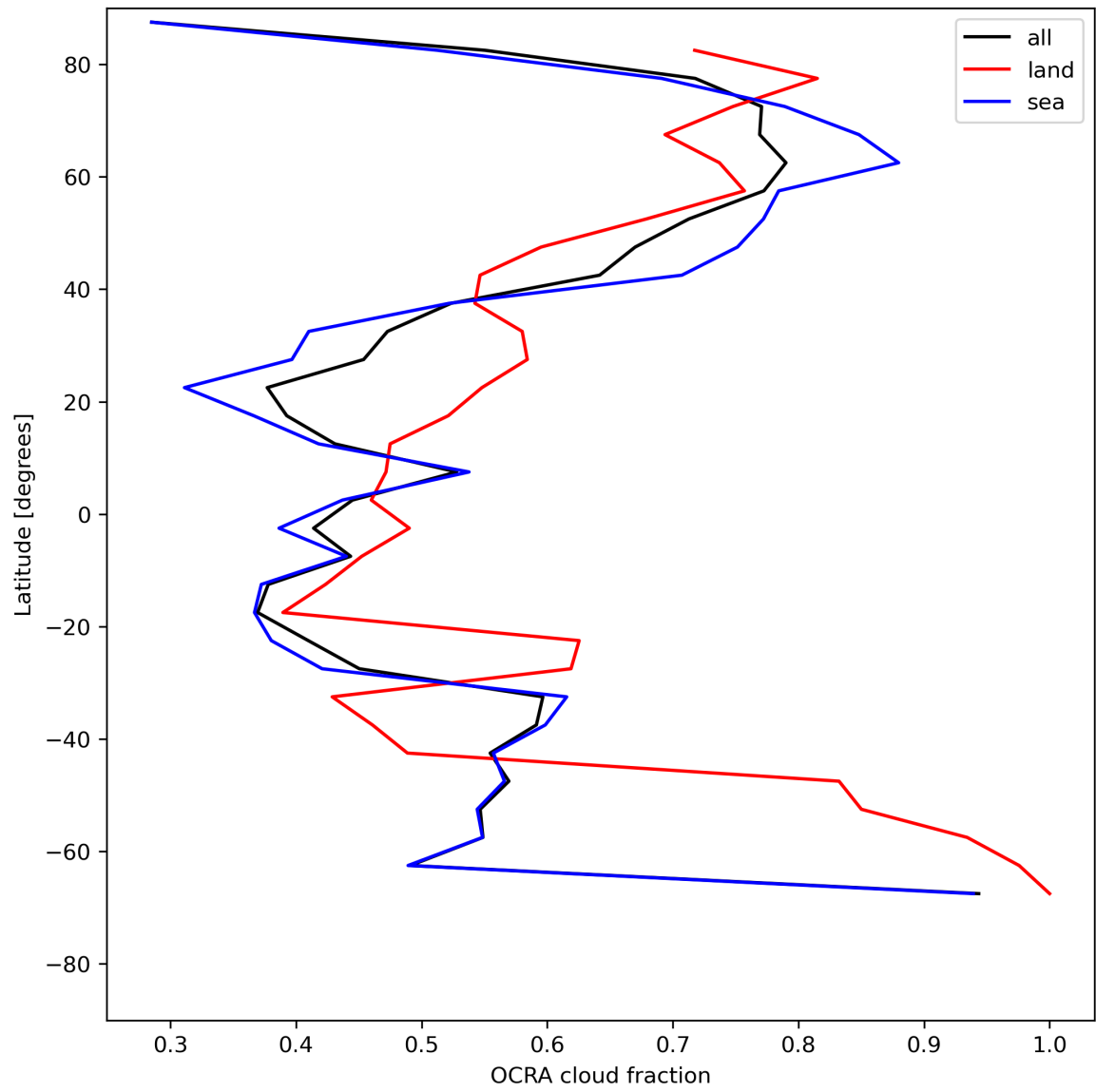
Figure 34: Zonal average of “OCRA cloud fraction” for 2024-06-19 to 2024-06-20.
