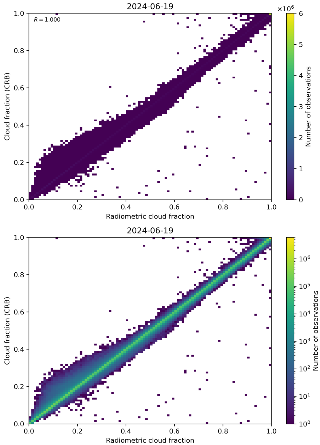
Figure 73: Scatter density plot of “Radiometric cloud fraction” against “Cloud fraction (CRB)” for 2024-06-19 to 2024-06-20.
