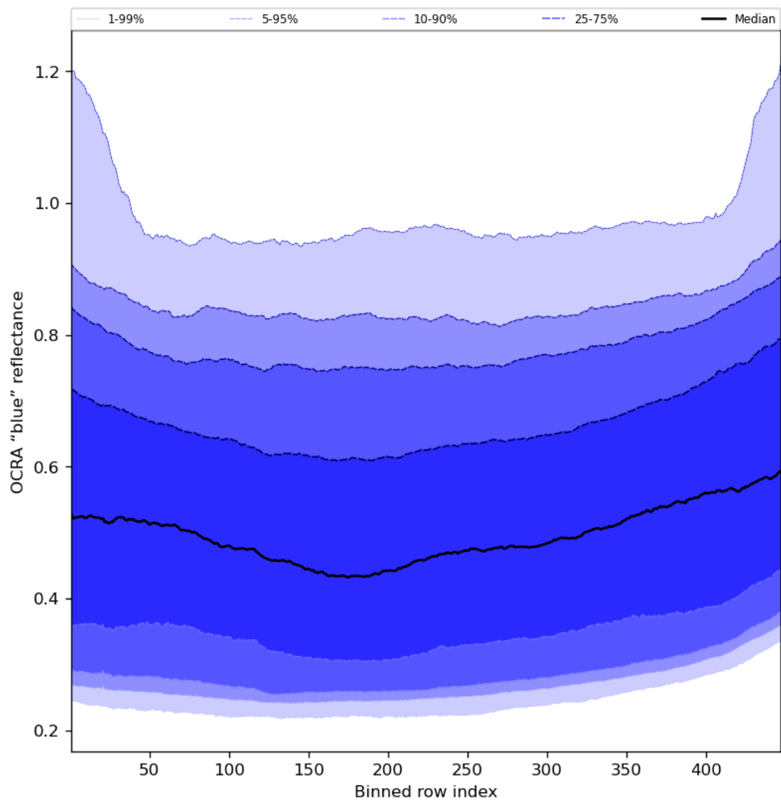
Figure 67: Along track statistics of “OCRA “blue” reflectance” for 2024-06-19 to 2024-06-20
