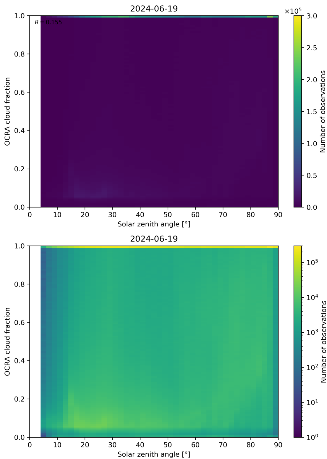
Figure 100: Scatter density plot of “Solar zenith angle” against “OCRA cloud fraction” for 2024-06-19 to 2024-06-20.
