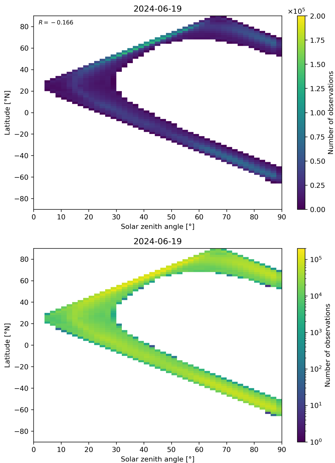
Figure 105: Scatter density plot of “Solar zenith angle” against “Latitude” for 2024-06-19 to 2024-06-20.
