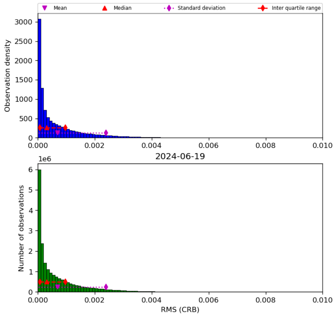
Figure 48: Histogram of "RMS (CRB)" for 2024-06-19 to 2024-06-20
