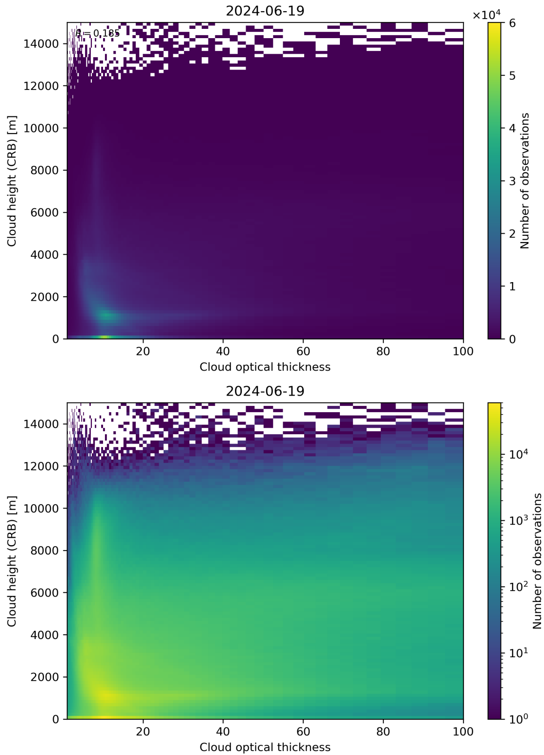
Figure 85: Scatter density plot of “Cloud optical thickness” against “Cloud height (CRB)” for 2024-06-19 to 2024-06-20.
