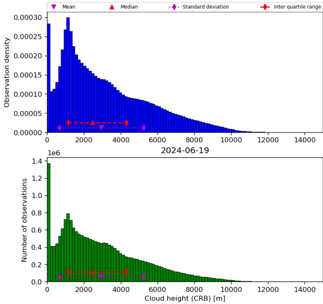
Figure 43: Histogram of “Cloud height (CRB)” for 2024-06-19 to 2024-06-20
