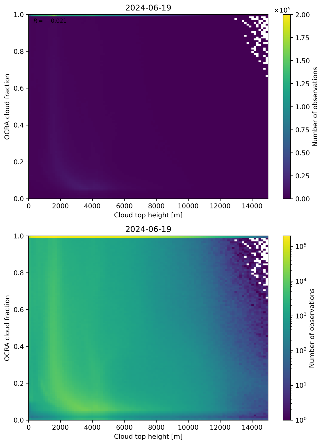
Figure 87: Scatter density plot of “Cloud top height” against “OCRA cloud fraction” for 2024-06-19 to 2024-06-20.
