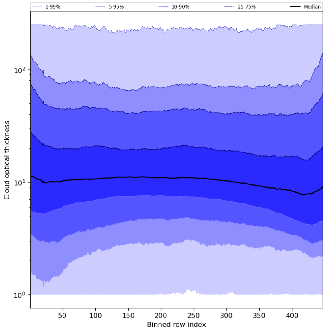
Figure 57: Along track statistics of “Cloud optical thickness” for 2024-06-19 to 2024-06-20
