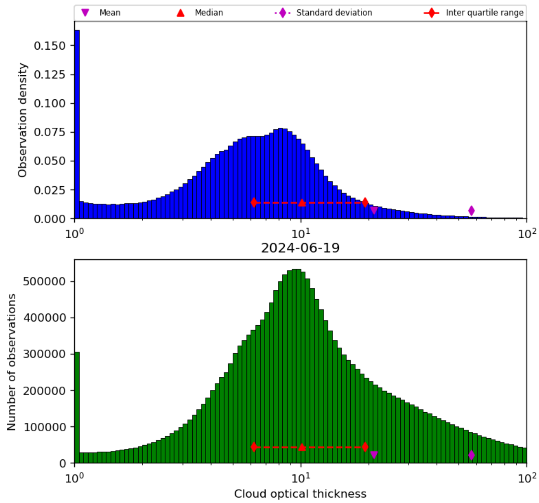
Figure 41: Histogram of “Cloud optical thickness” for 2024-06-19 to 2024-06-20
