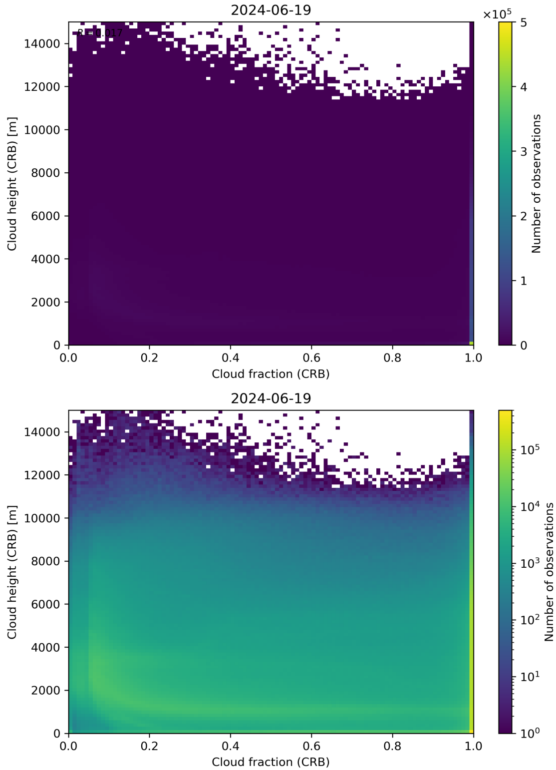
Figure 79: Scatter density plot of “Cloud fraction (CRB)” against “Cloud height (CRB)” for 2024-06-19 to 2024-06-20.
