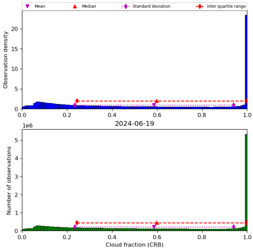
Figure 42: Histogram of “Cloud fraction (CRB)” for 2024-06-19 to 2024-06-20
