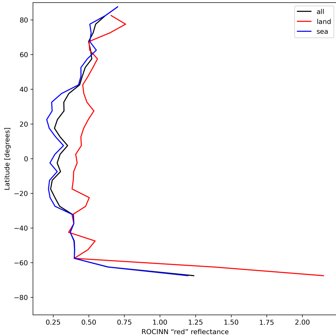
Figure 37: Zonal average of “ROCINN “red” reflectance” for 2024-06-19 to 2024-06-20.
