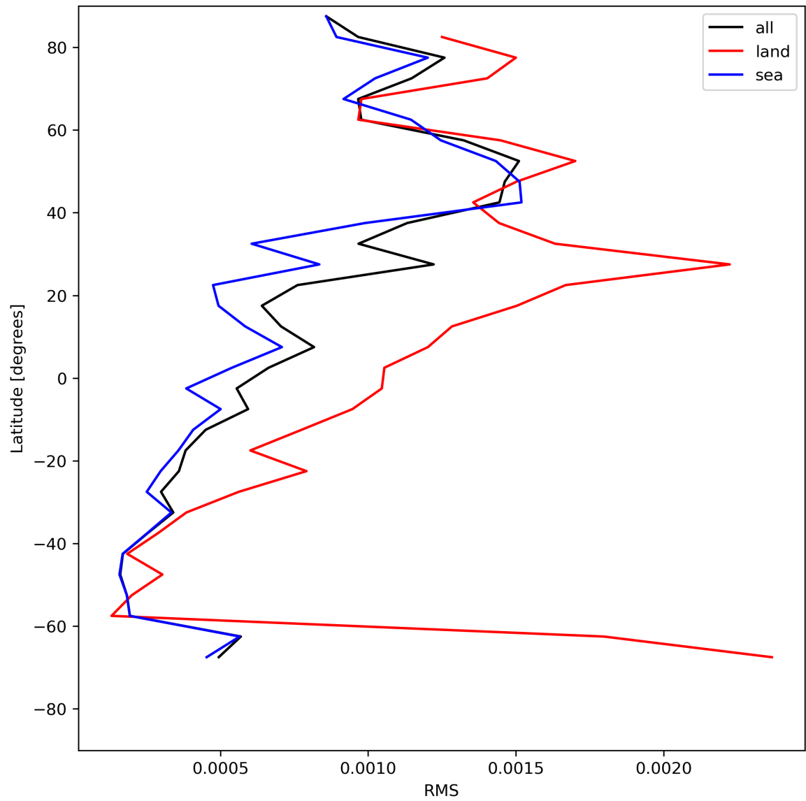
Figure 31: Zonal average of “RMS” for 2024-06-19 to 2024-06-20.
