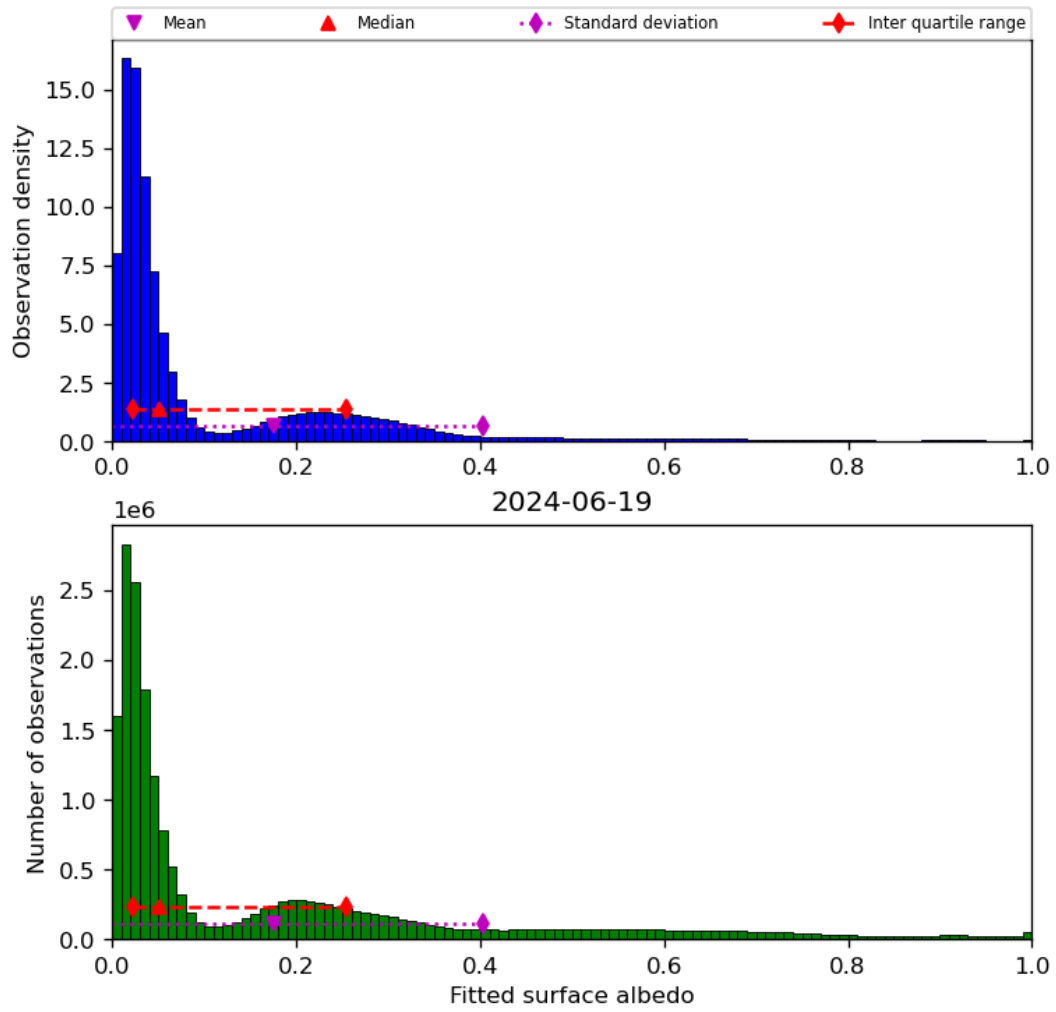
Figure 45: Histogram of “Fitted surface albedo” for 2024-06-19 to 2024-06-20
