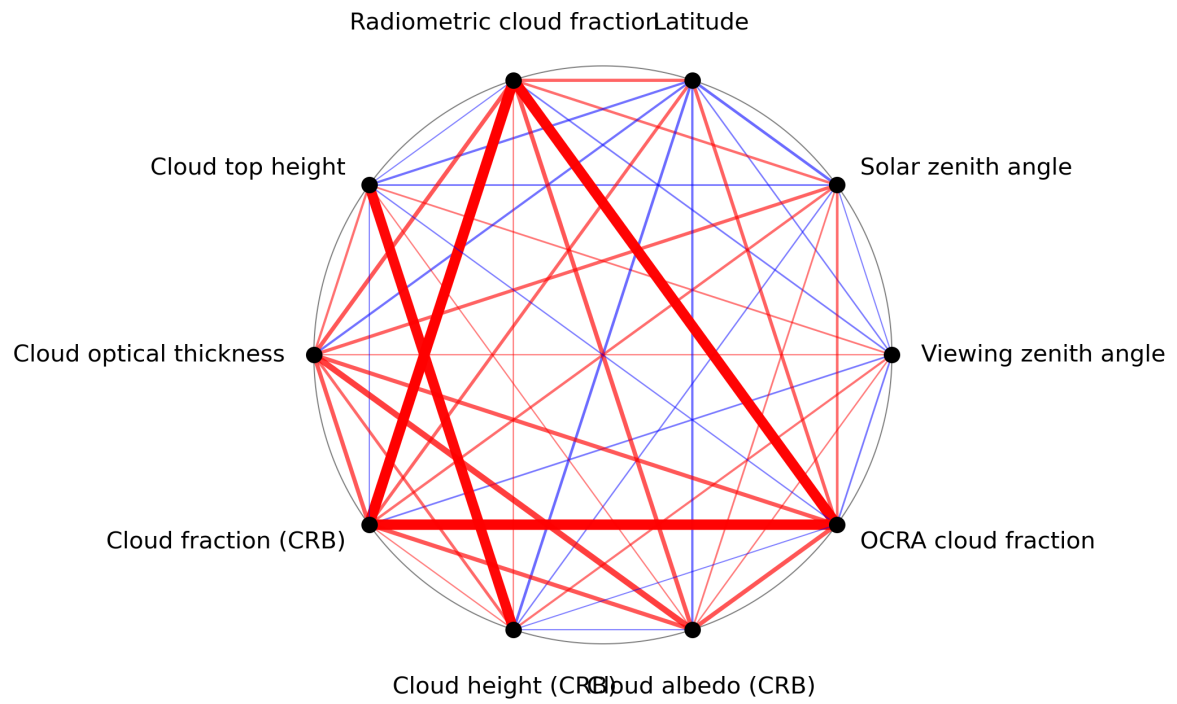
Figure 1: Map of correlation graph for 2024-06-19 to 2024-06-20.
