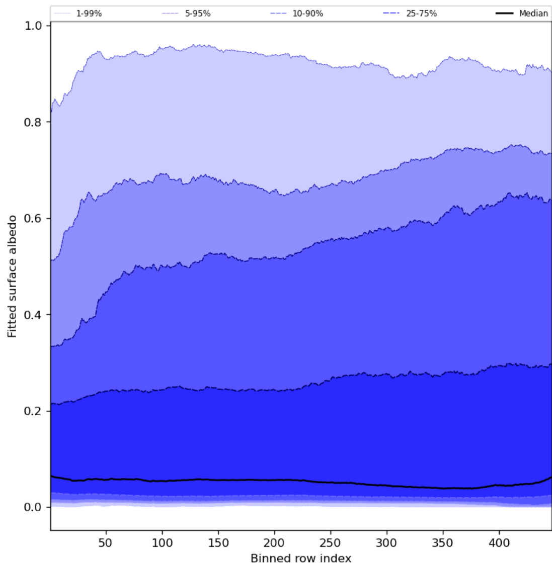
Figure 61: Along track statistics of “Fitted surface albedo” for 2024-06-19 to 2024-06-20
