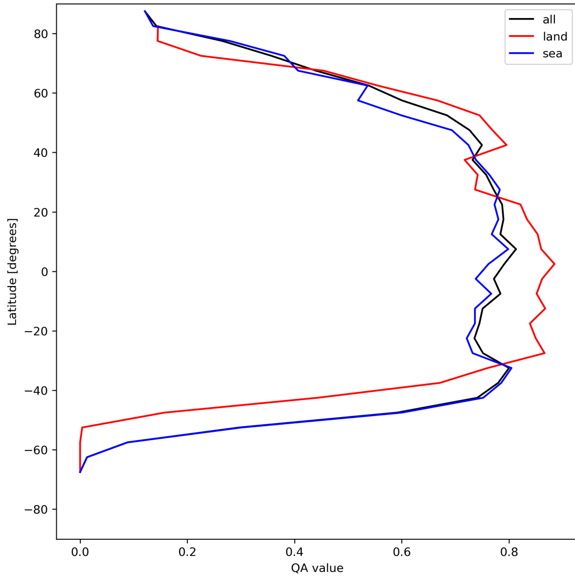
Figure 22: Zonal average of “QA value” for 2024-06-19 to 2024-06-20.
