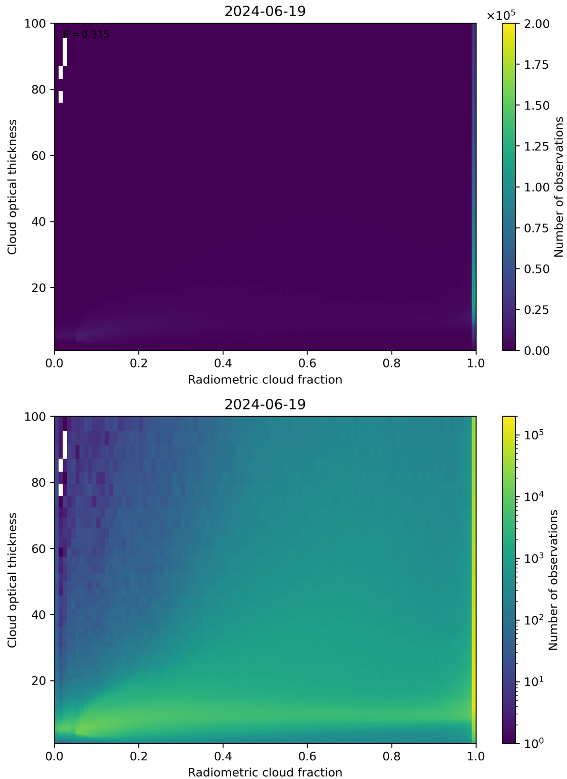
Figure 75: Scatter density plot of “Radiometric cloud fraction” against “Cloud optical thickness” for 2024-06-19 to 2024-06-20.
