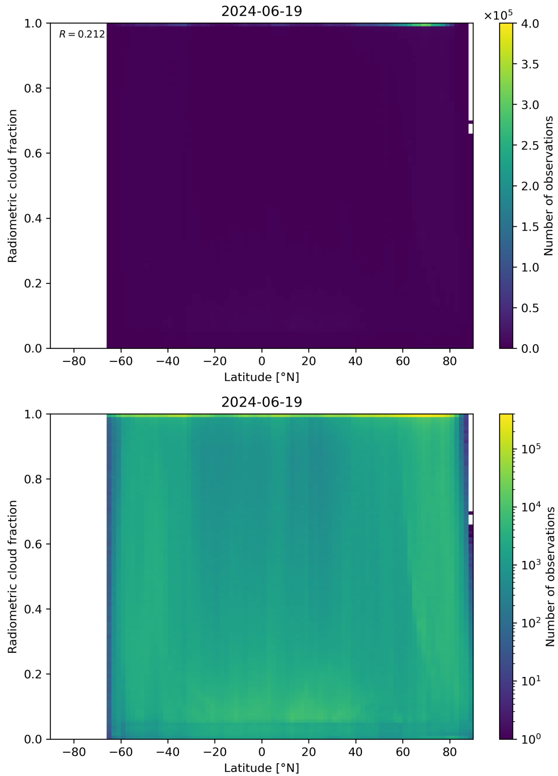
Figure 92: Scatter density plot of “Latitude” against “Radiometric cloud fraction” for 2024-06-19 to 2024-06-20.
