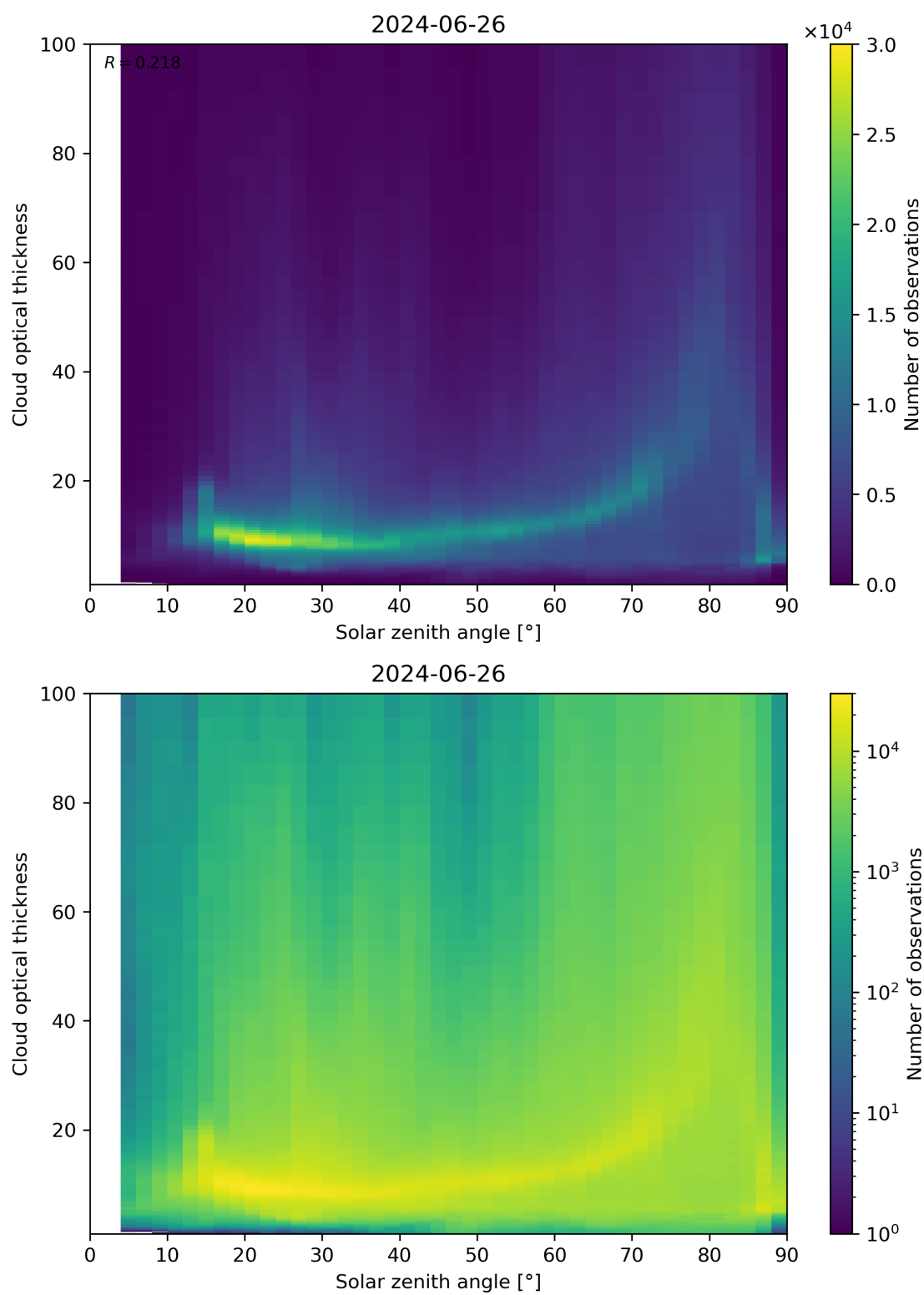
Figure 103: Scatter density plot of “Solar zenith angle” against “Cloud optical thickness” for 2024-06-25 to 2024-06-27.
