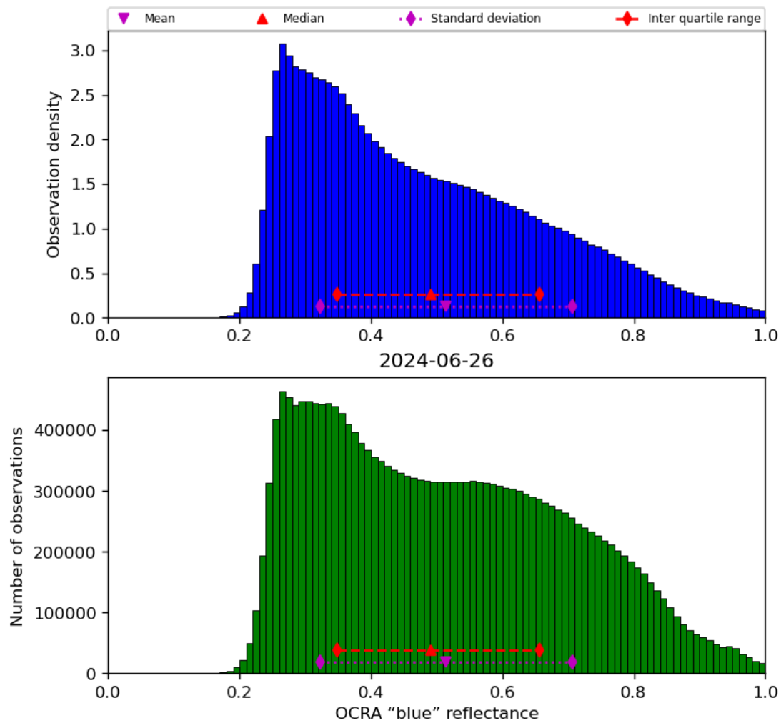
Figure 51: Histogram of “OCRA “blue” reflectance” for 2024-06-25 to 2024-06-27
