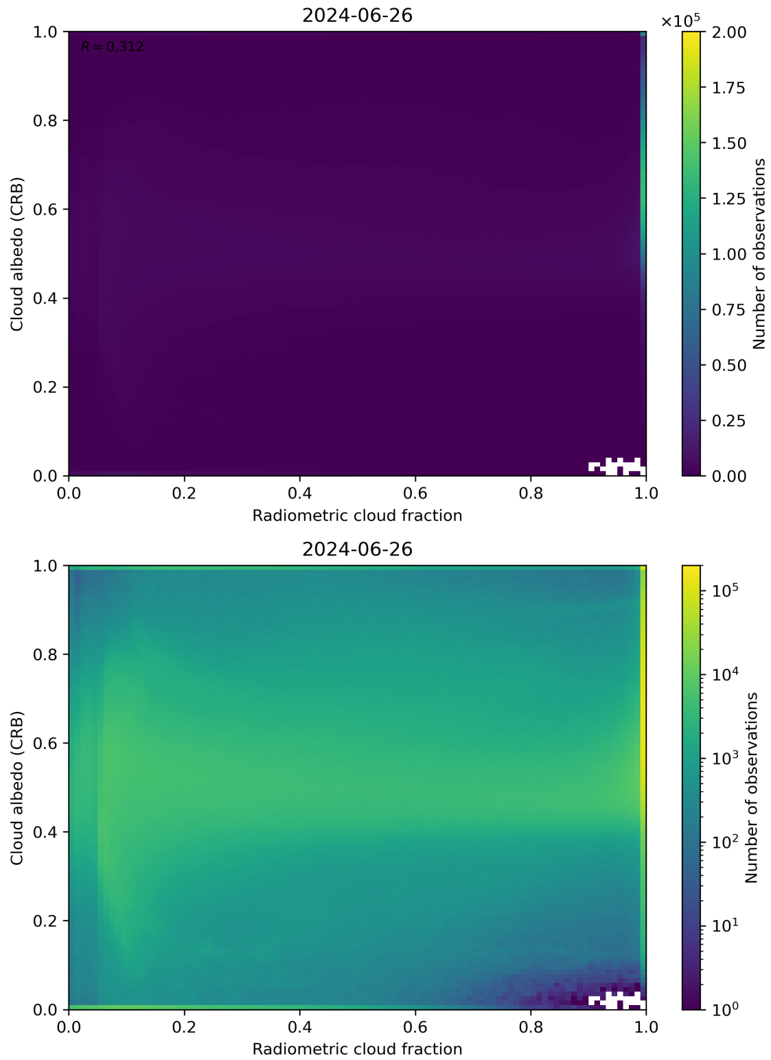
Figure 71: Scatter density plot of “Radiometric cloud fraction” against “Cloud albedo (CRB)” for 2024-06-25 to 2024-06-27.
