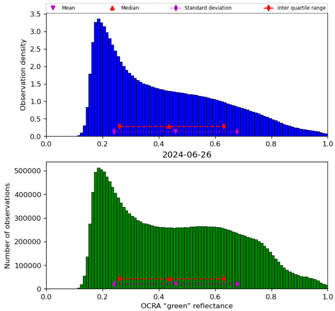
Figure 52: Histogram of “OCRA “green” reflectance” for 2024-06-25 to 2024-06-27
