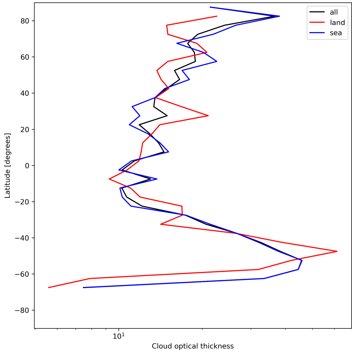
Figure 25: Zonal average of “Cloud optical thickness” for 2024-06-25 to 2024-06-27.
