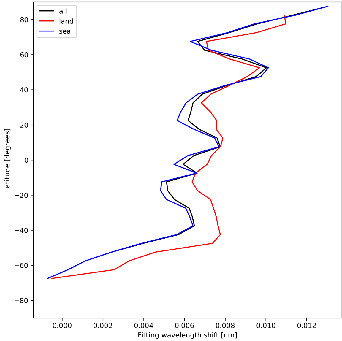
Figure 33: Zonal average of “Fitting wavelength shift” for 2024-06-25 to 2024-06-27.
