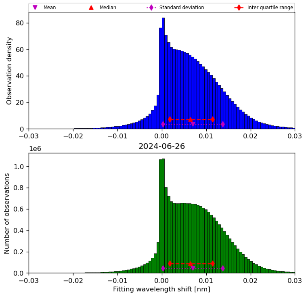
Figure 49: Histogram of “Fitting wavelength shift” for 2024-06-25 to 2024-06-27
