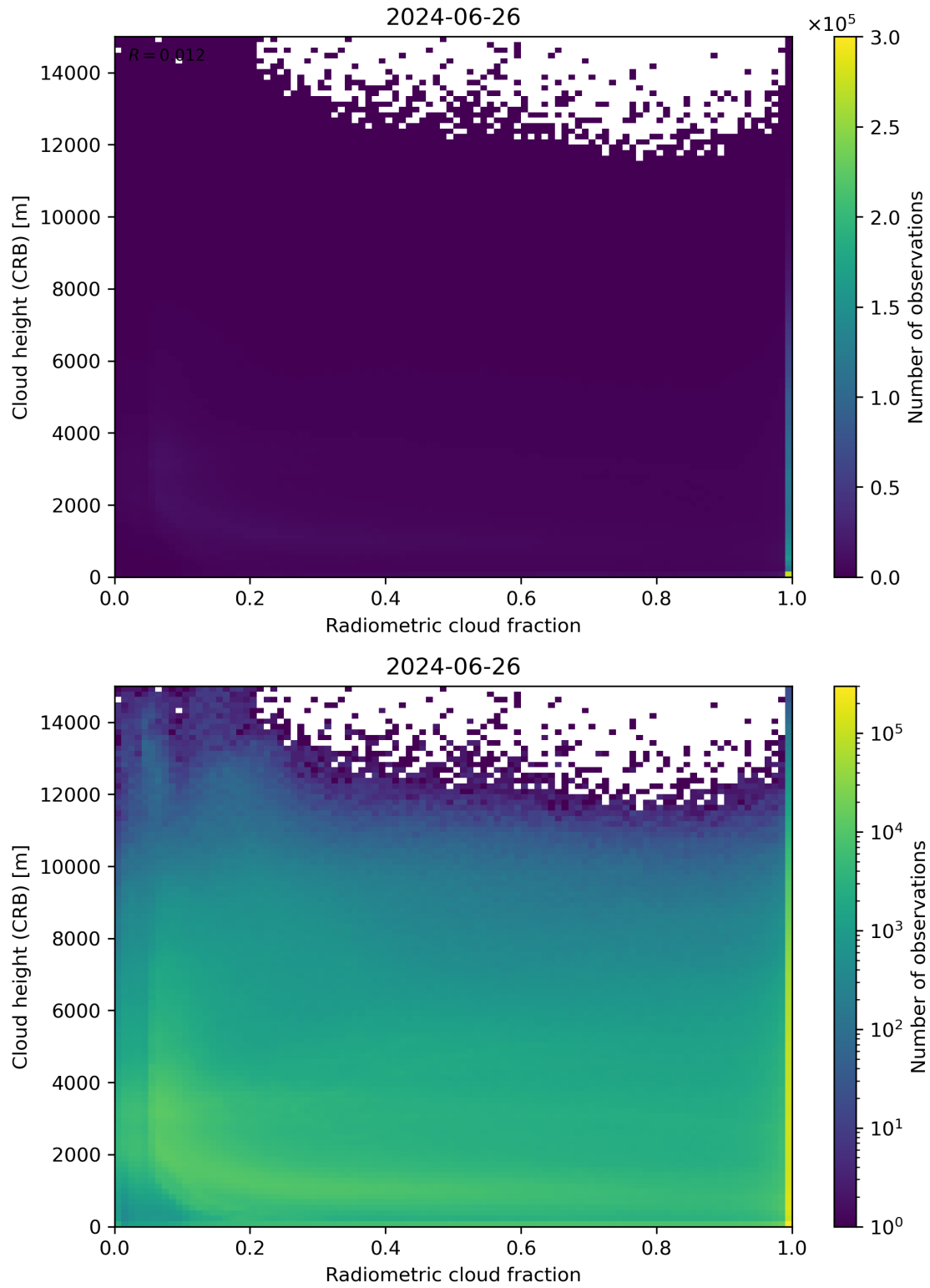
Figure 74: Scatter density plot of “Radiometric cloud fraction” against “Cloud height (CRB)” for 2024-06-25 to 2024-06-27.
