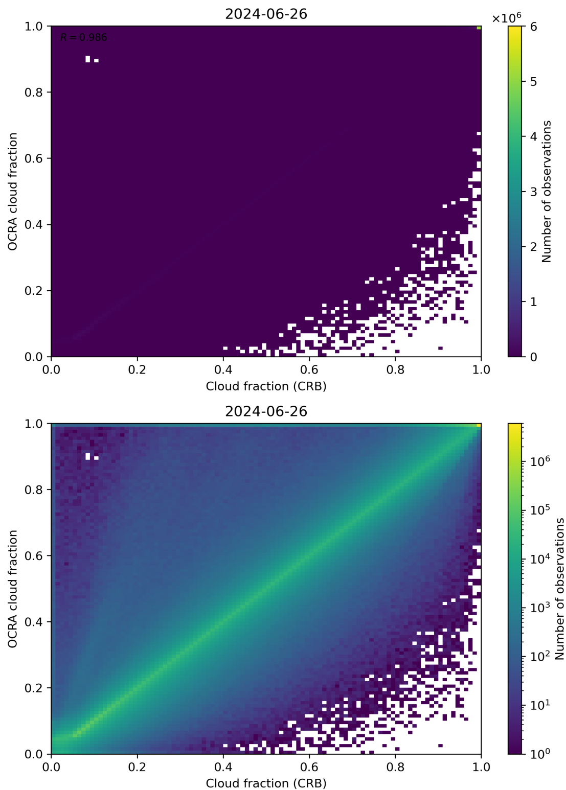
Figure 78: Scatter density plot of “Cloud fraction (CRB)” against “OCRA cloud fraction” for 2024-06-25 to 2024-06-27.
