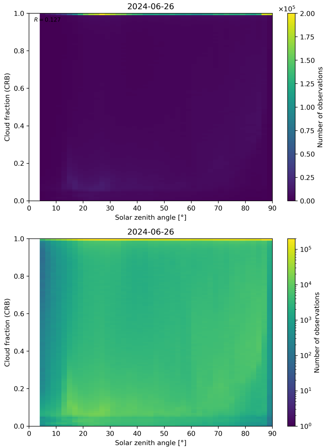
Figure 101: Scatter density plot of “Solar zenith angle” against “Cloud fraction (CRB)” for 2024-06-25 to 2024-06-27.
