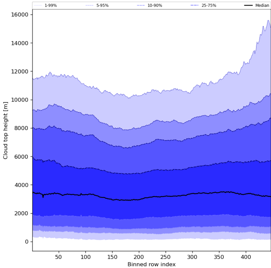
Figure 56: Along track statistics of “Cloud top height” for 2024-06-25 to 2024-06-27
