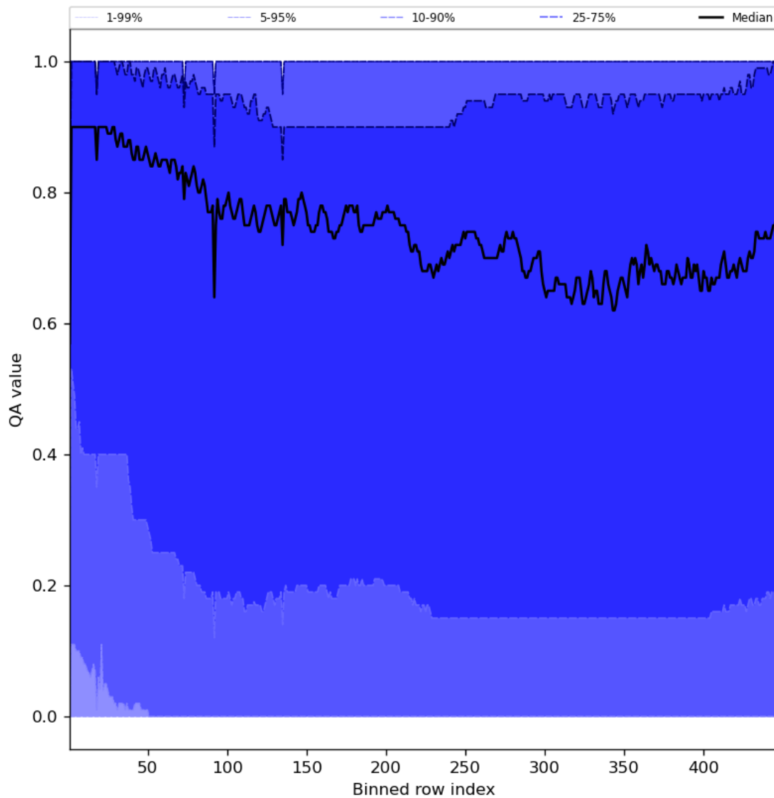
Figure 54: Along track statistics of “QA value” for 2024-06-25 to 2024-06-27
