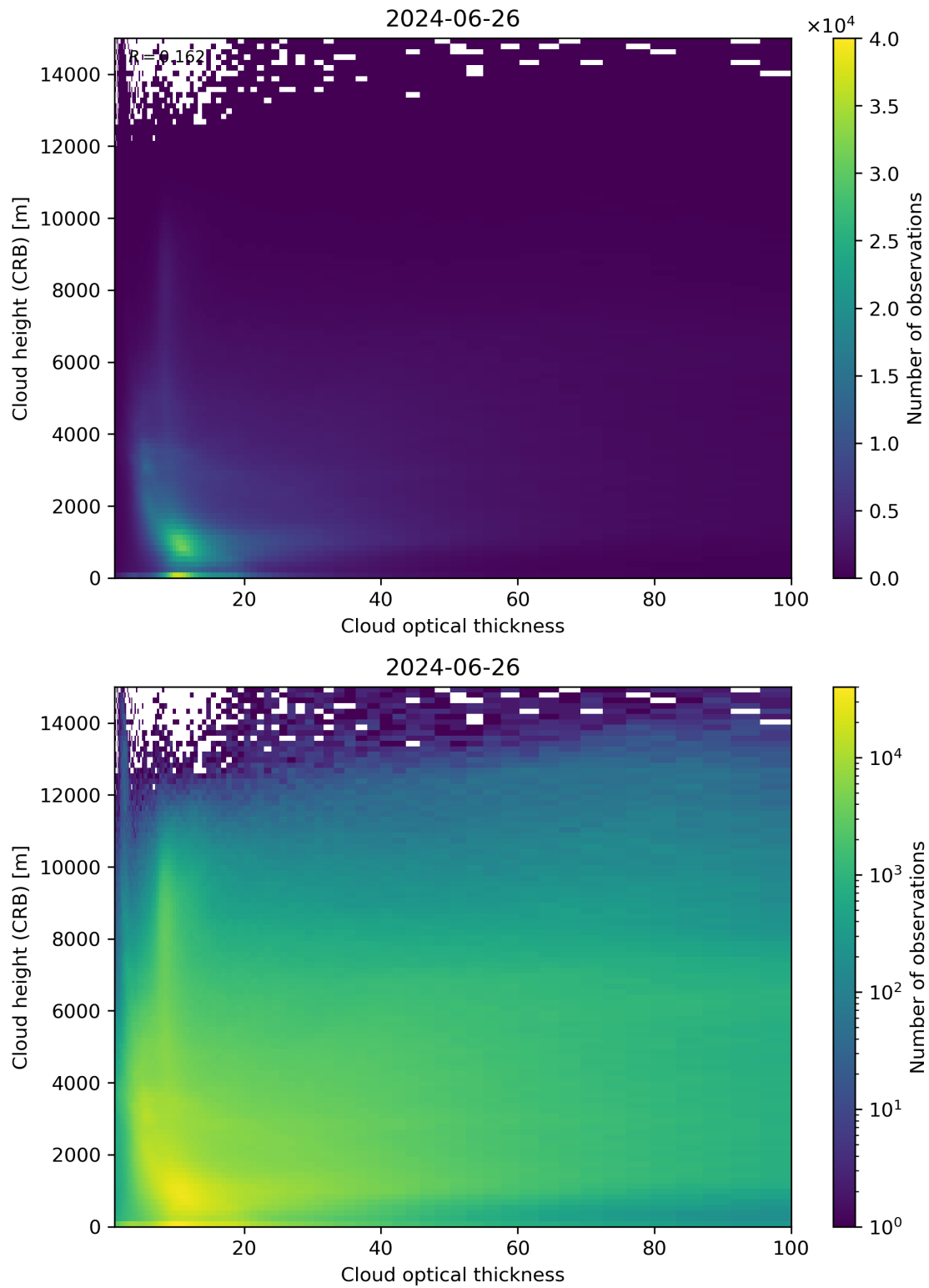
Figure 85: Scatter density plot of “Cloud optical thickness” against “Cloud height (CRB)” for 2024-06-25 to 2024-06-27.
