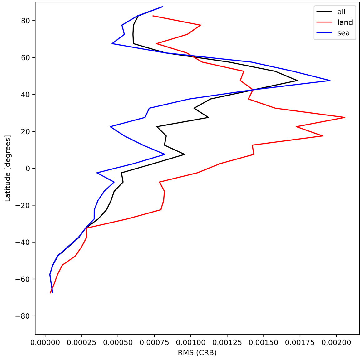
Figure 32: Zonal average of “RMS (CRB)” for 2024-06-25 to 2024-06-27.
