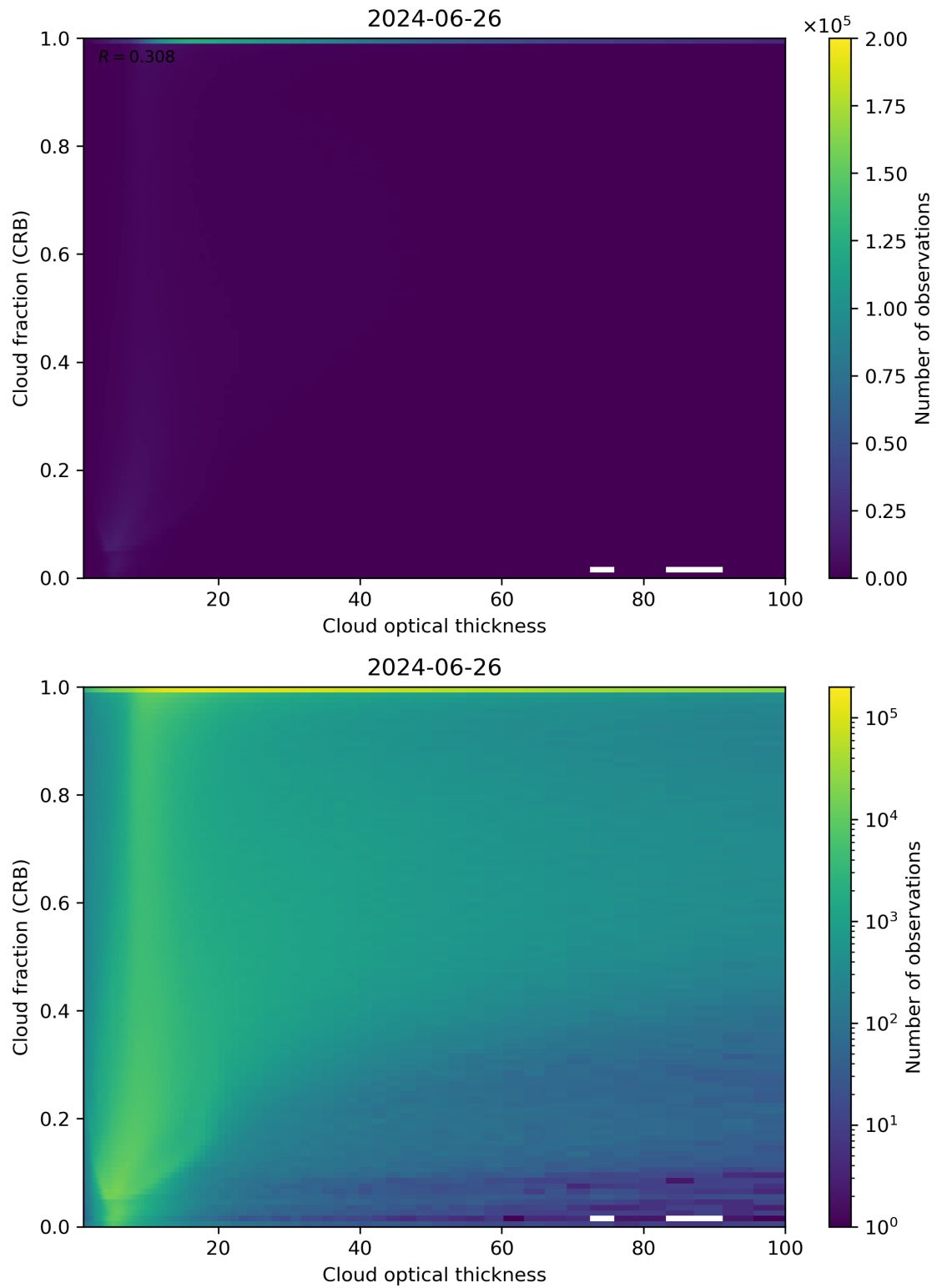
Figure 84: Scatter density plot of “Cloud optical thickness” against “Cloud fraction (CRB)” for 2024-06-25 to 2024-06-27.
