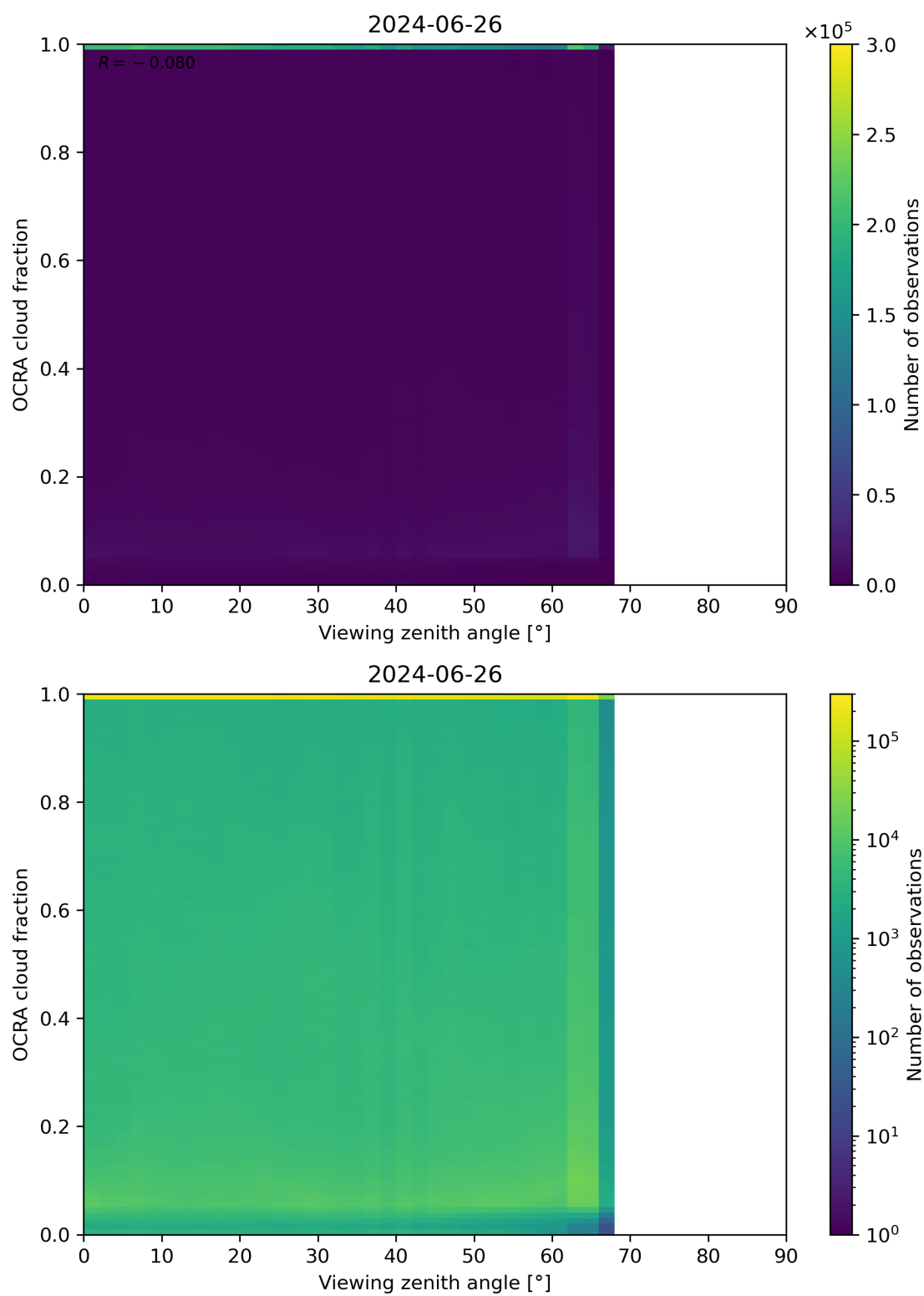
Figure 108: Scatter density plot of “Viewing zenith angle” against “OCRA cloud fraction” for 2024-06-25 to 2024-06-27.
