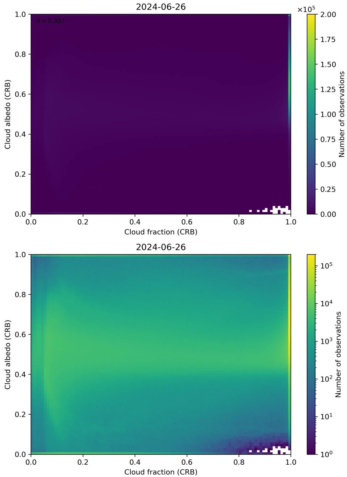
Figure 77: Scatter density plot of “Cloud fraction (CRB)” against “Cloud albedo (CRB)” for 2024-06-25 to 2024-06-27.
