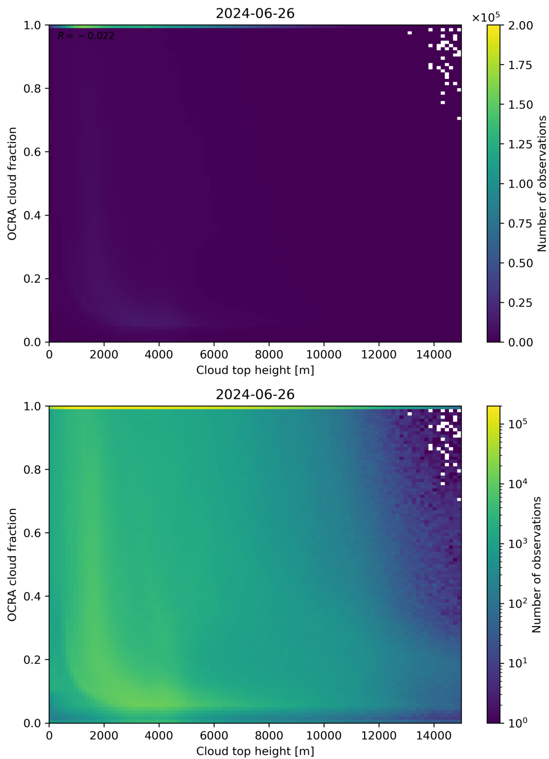
Figure 87: Scatter density plot of “Cloud top height” against “OCRA cloud fraction” for 2024-06-25 to 2024-06-27.
