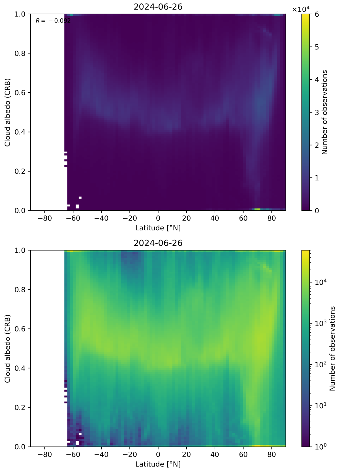
Figure 91: Scatter density plot of “Latitude” against “Cloud albedo (CRB)” for 2024-06-25 to 2024-06-27.
