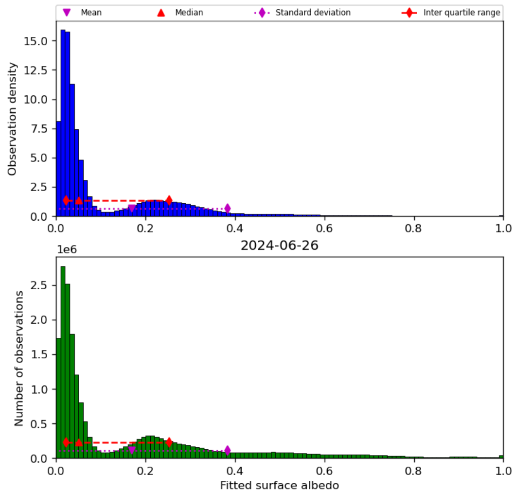
Figure 45: Histogram of “Fitted surface albedo” for 2024-06-25 to 2024-06-27
