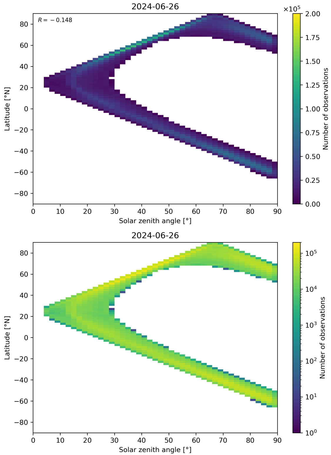
Figure 105: Scatter density plot of “Solar zenith angle” against “Latitude” for 2024-06-25 to 2024-06-27.
