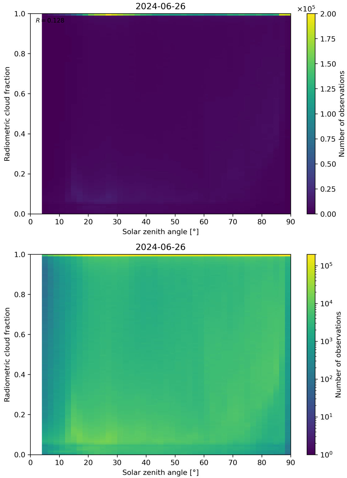
Figure 99: Scatter density plot of “Solar zenith angle” against “Radiometric cloud fraction” for 2024-06-25 to 2024-06-27.
