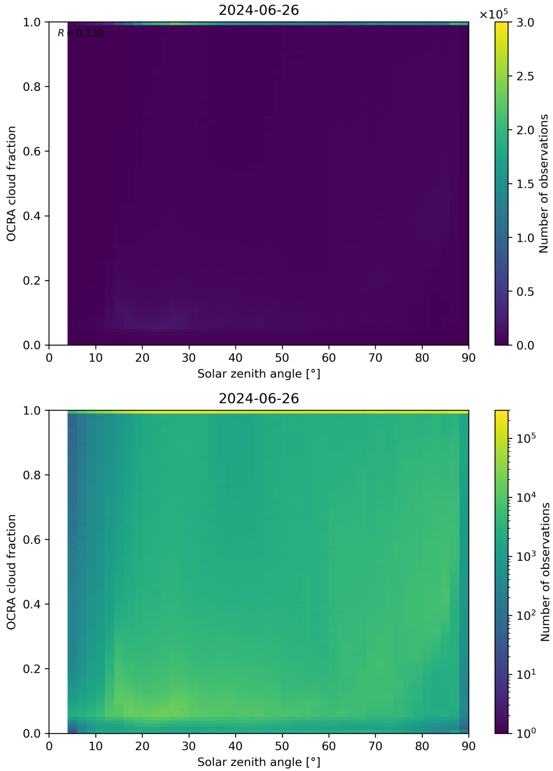
Figure 100: Scatter density plot of “Solar zenith angle” against “OCRA cloud fraction” for 2024-06-25 to 2024-06-27.
