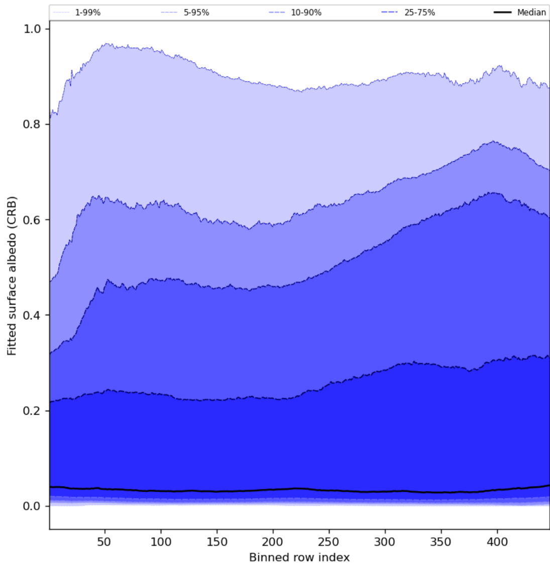
Figure 62: Along track statistics of “Fitted surface albedo (CRB)” for 2024-06-25 to 2024-06-27
