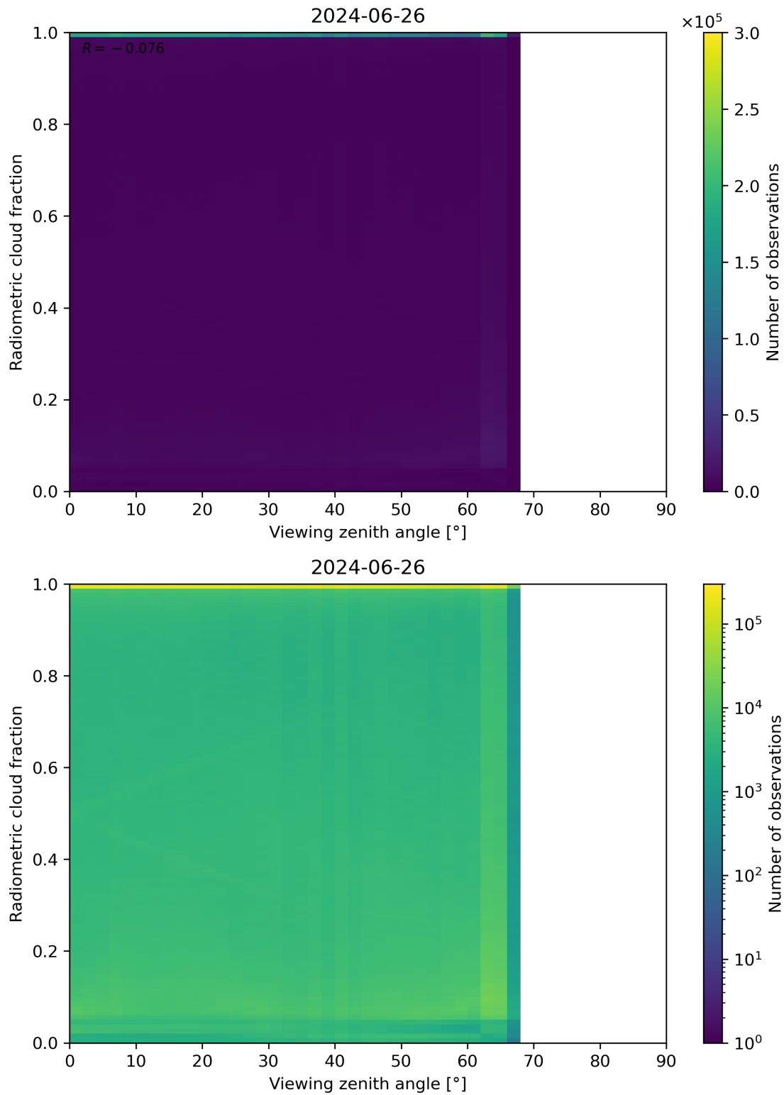
Figure 107: Scatter density plot of “Viewing zenith angle” against “Radiometric cloud fraction” for 2024-06-25 to 2024-06-27.
