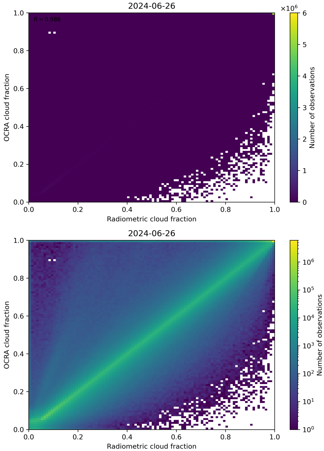
Figure 72: Scatter density plot of “Radiometric cloud fraction” against “OCRA cloud fraction” for 2024-06-25 to 2024-06-27.
