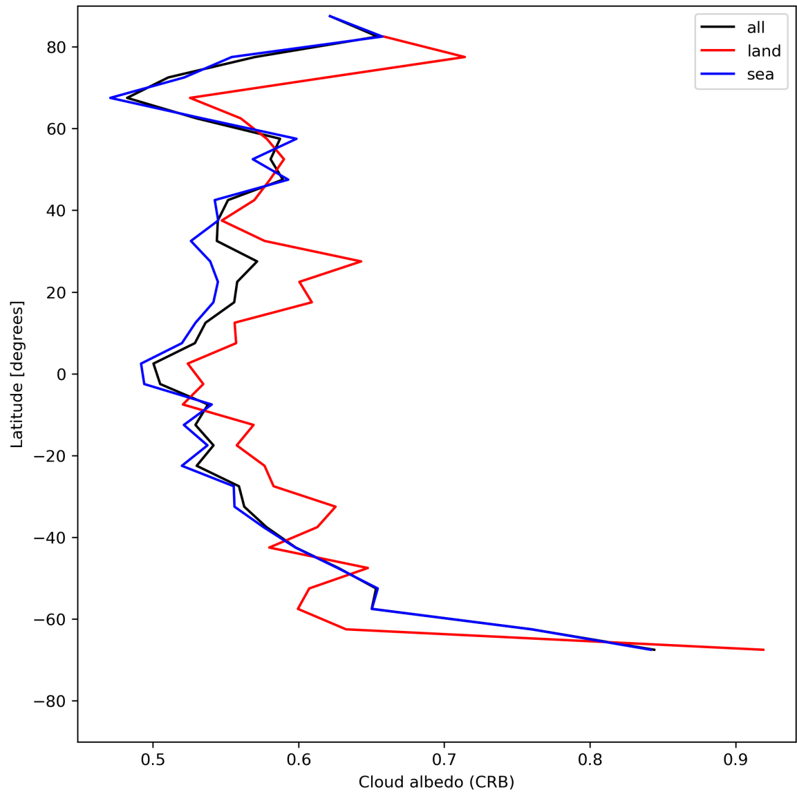
Figure 28: Zonal average of “Cloud albedo (CRB)” for 2024-06-25 to 2024-06-27.
