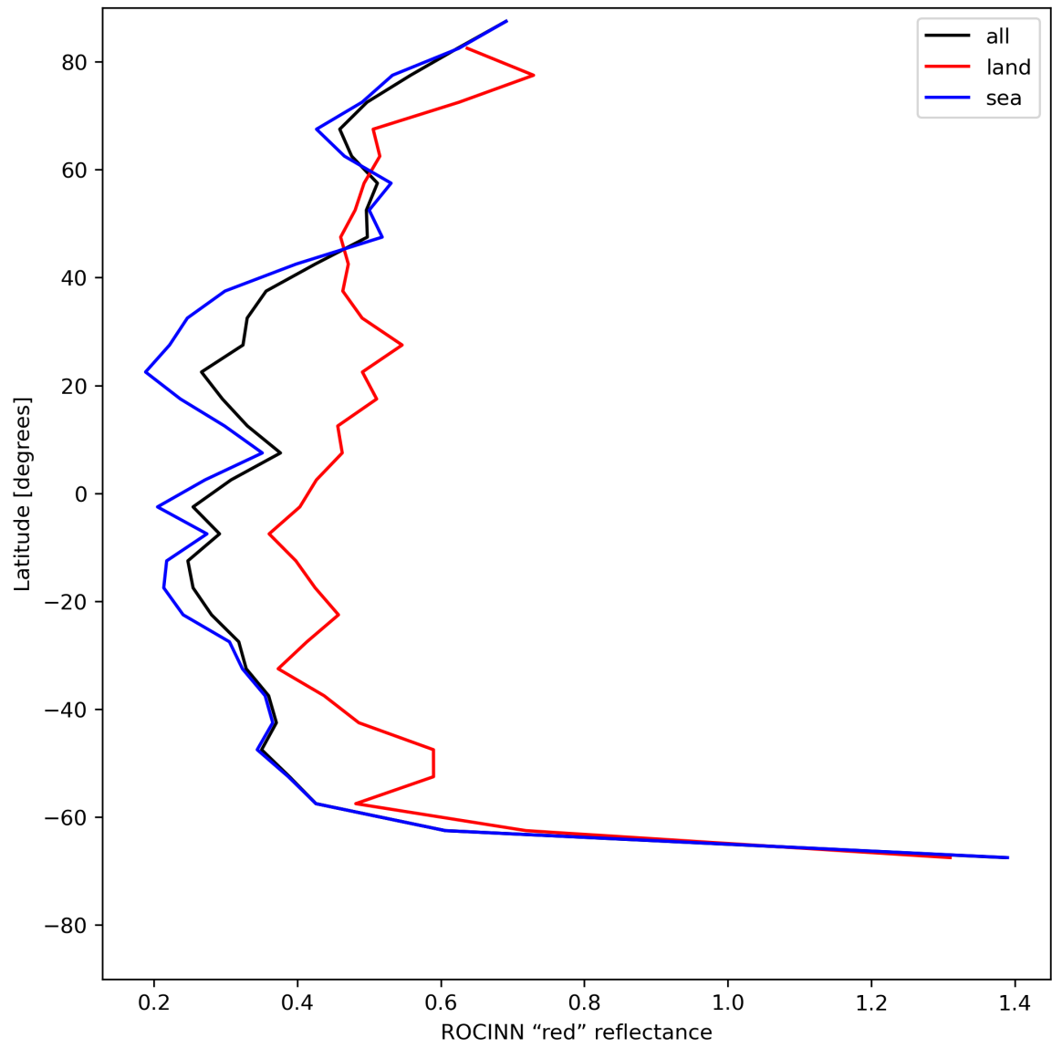
Figure 37: Zonal average of “ROCINN “red” reflectance” for 2024-06-25 to 2024-06-27.
