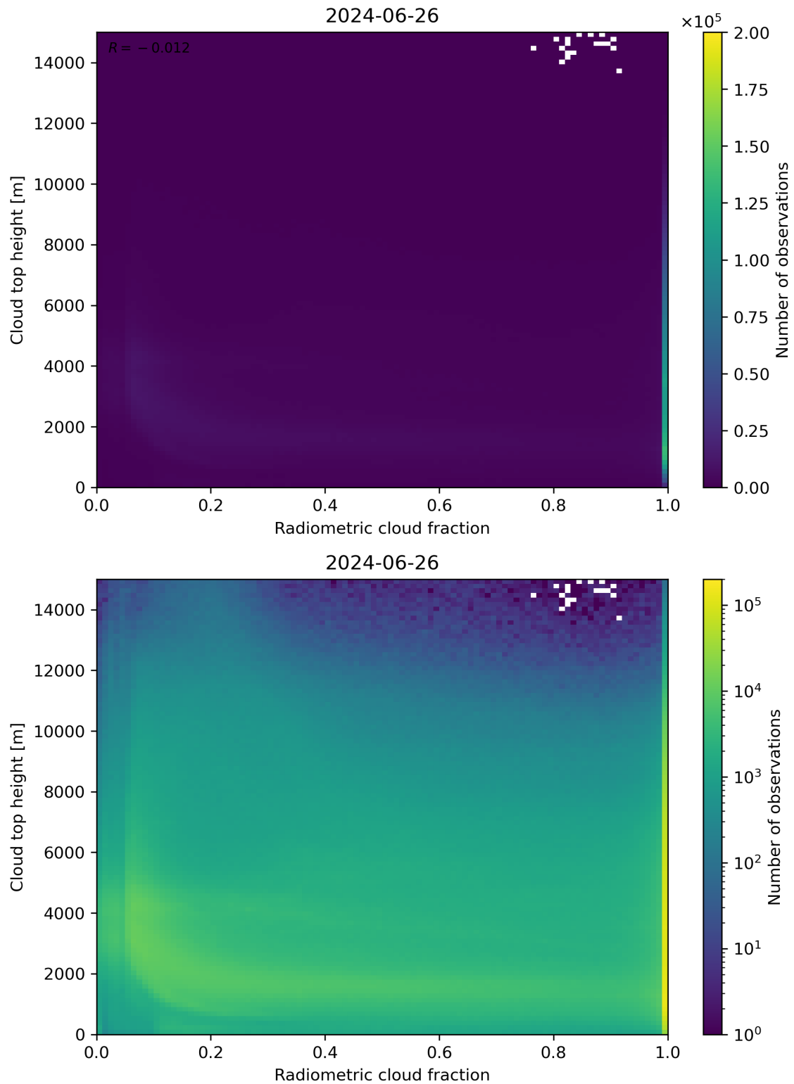
Figure 76: Scatter density plot of “Radiometric cloud fraction” against “Cloud top height” for 2024-06-25 to 2024-06-27.
