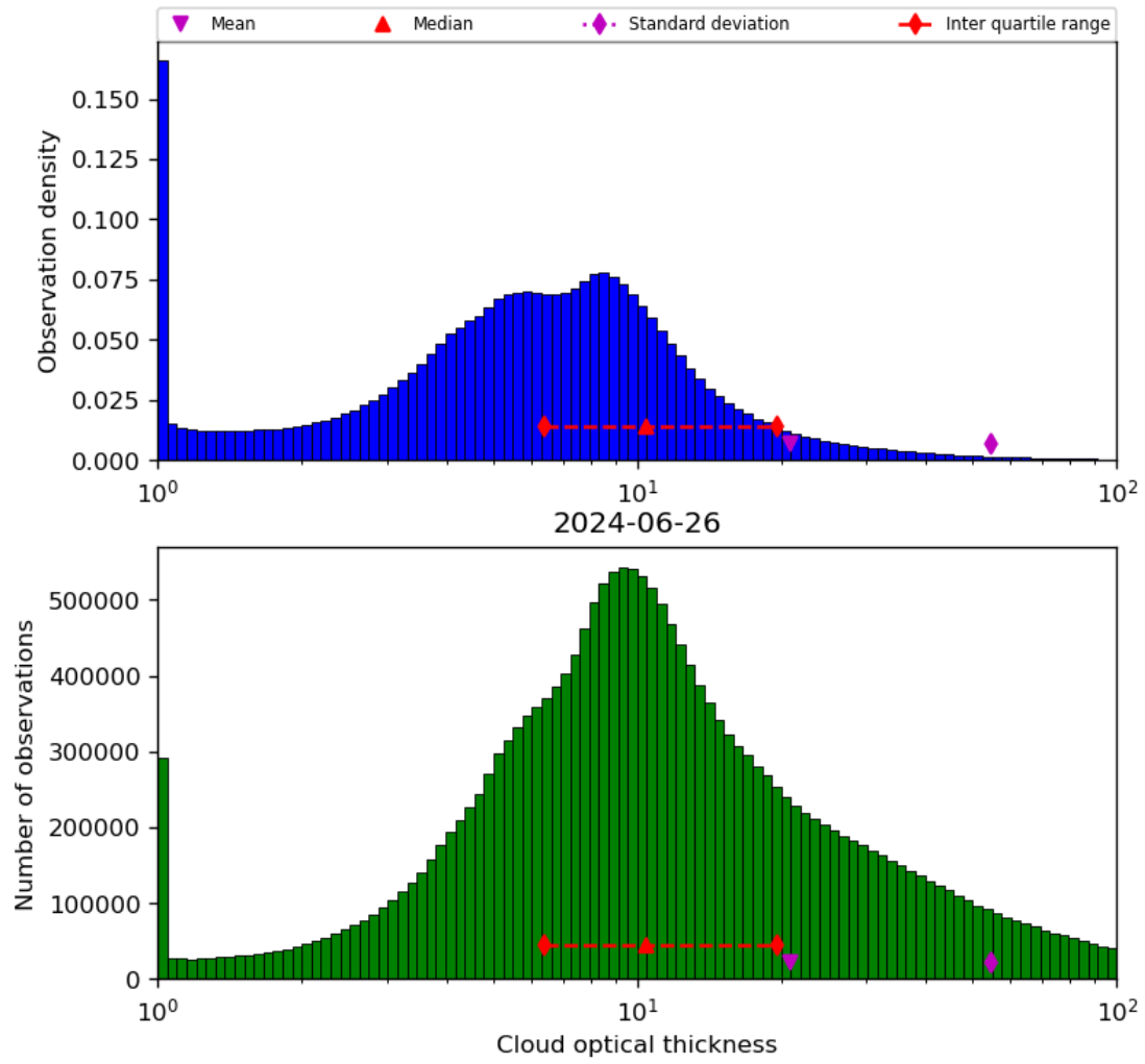
Figure 41: Histogram of “Cloud optical thickness” for 2024-06-25 to 2024-06-27
