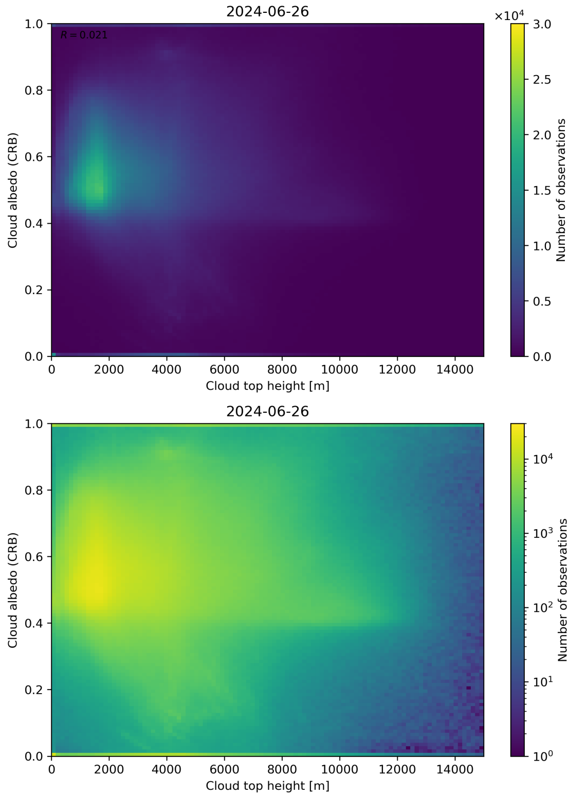
Figure 86: Scatter density plot of “Cloud top height” against “Cloud albedo (CRB)” for 2024-06-25 to 2024-06-27.
