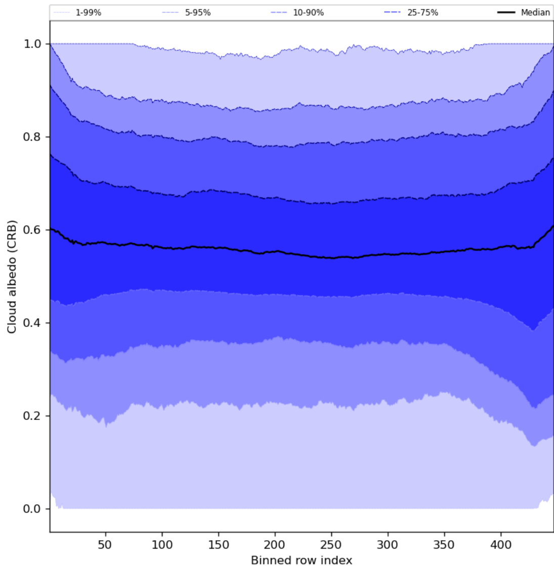
Figure 60: Along track statistics of “Cloud albedo (CRB)” for 2024-06-25 to 2024-06-27
