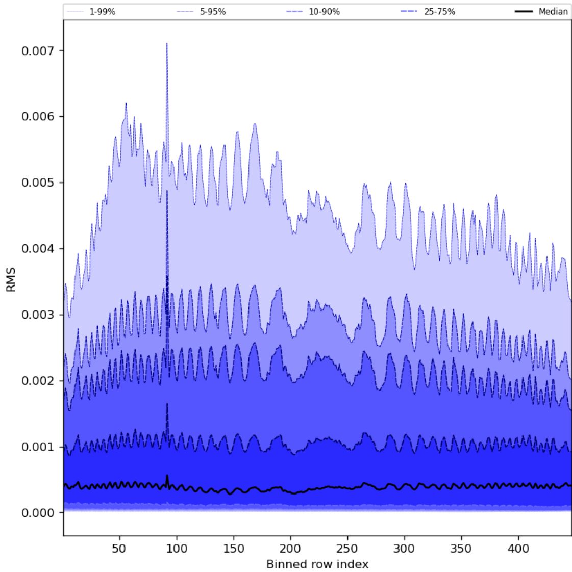
Figure 63: Along track statistics of “RMS” for 2024-06-25 to 2024-06-27
