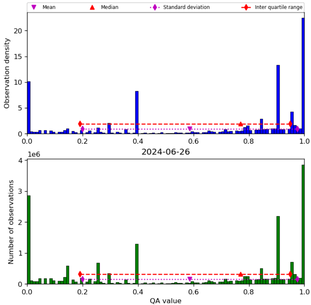
Figure 38: Histogram of “QA value” for 2024-06-25 to 2024-06-27
