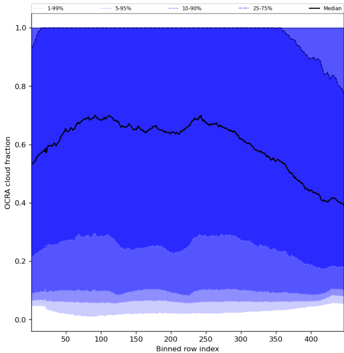
Figure 66: Along track statistics of “OCRA cloud fraction” for 2024-06-25 to 2024-06-27
