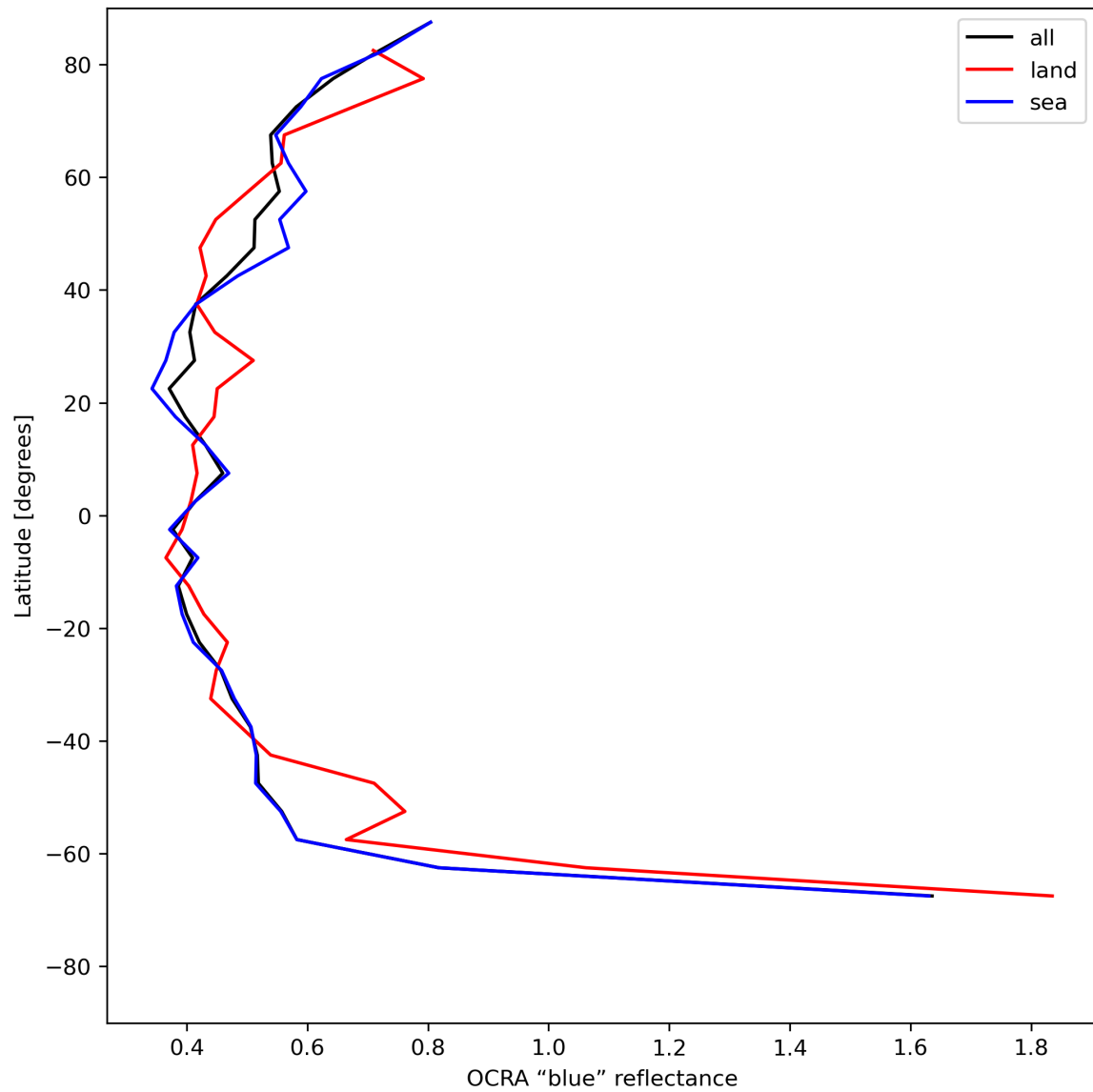
Figure 35: Zonal average of “OCRA “blue” reflectance” for 2024-06-25 to 2024-06-27.
