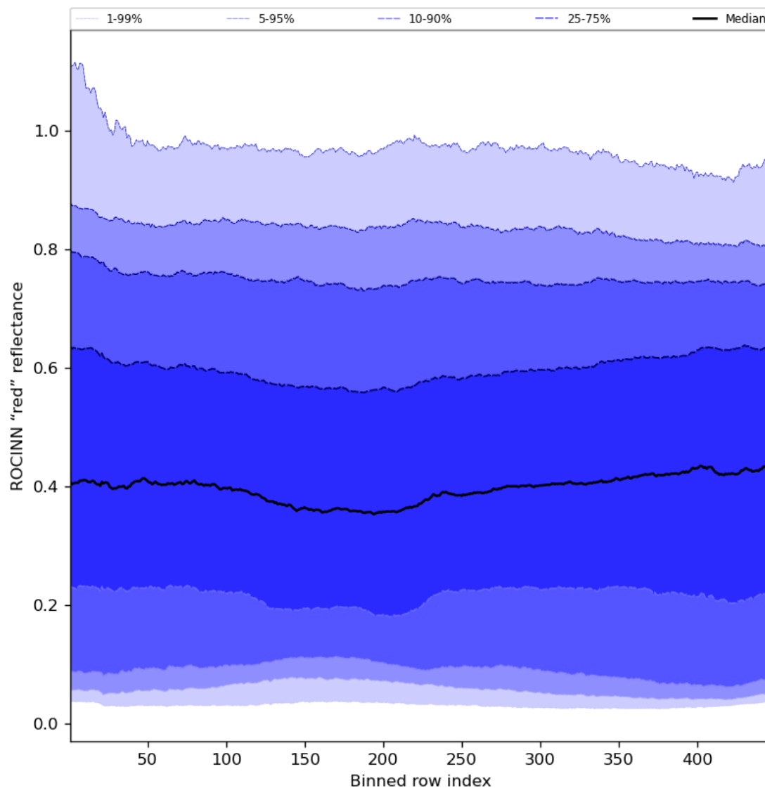
Figure 69: Along track statistics of “ROCINN “red” reflectance” for 2024-06-25 to 2024-06-27
