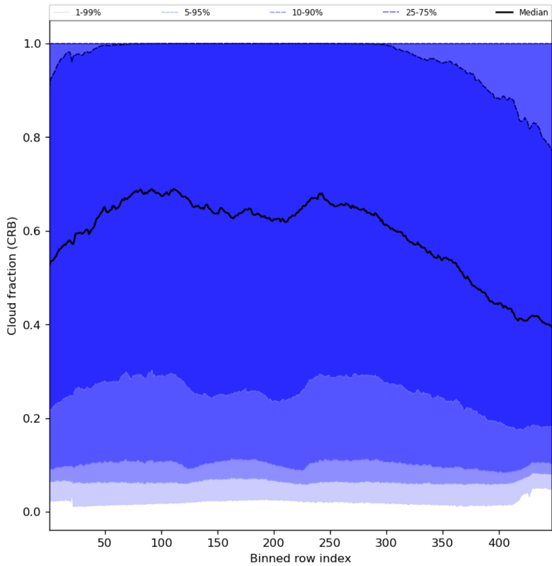
Figure 58: Along track statistics of “Cloud fraction (CRB)” for 2024-06-25 to 2024-06-27
