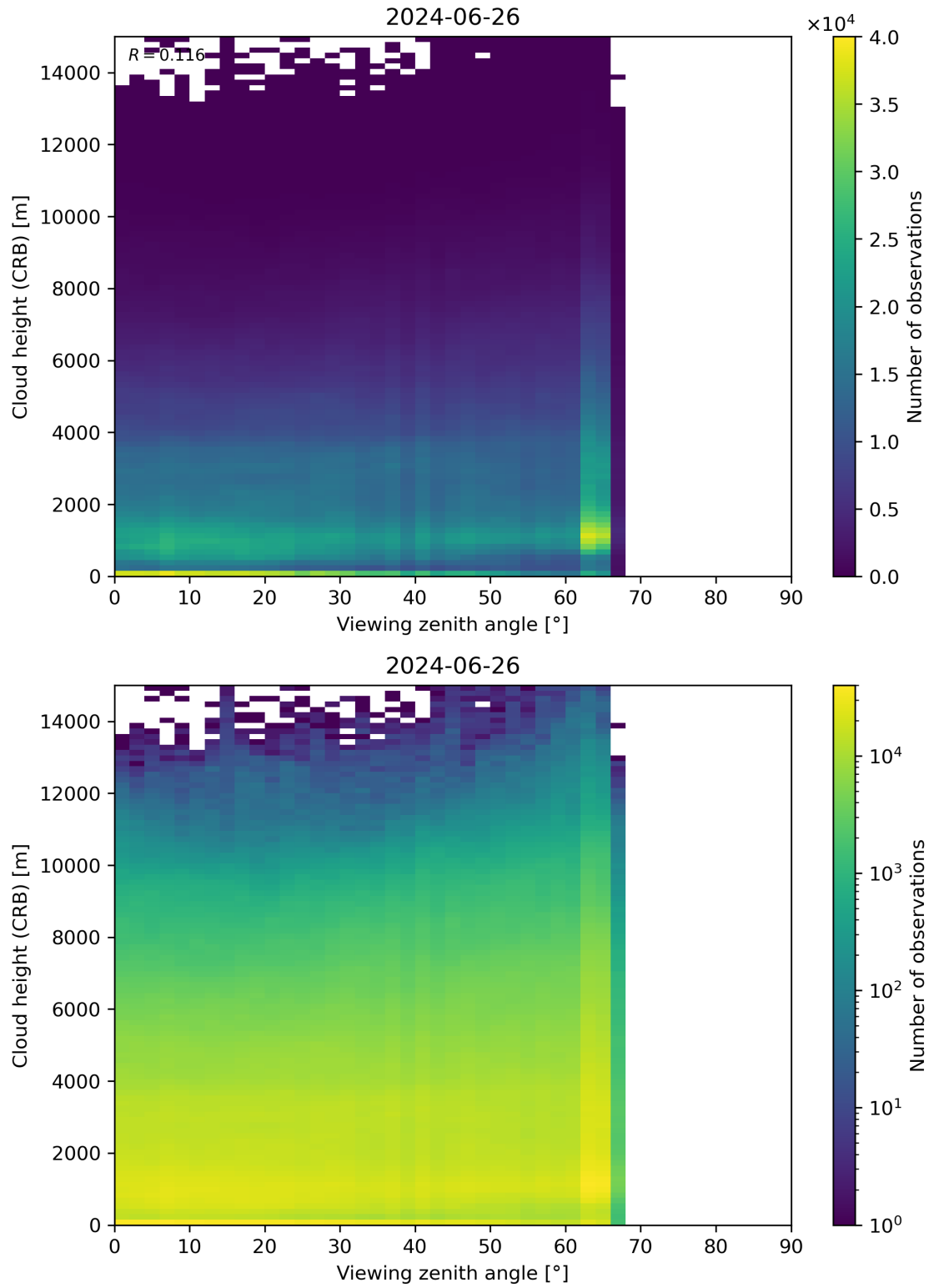
Figure 110: Scatter density plot of “Viewing zenith angle” against “Cloud height (CRB)” for 2024-06-25 to 2024-06-27.
