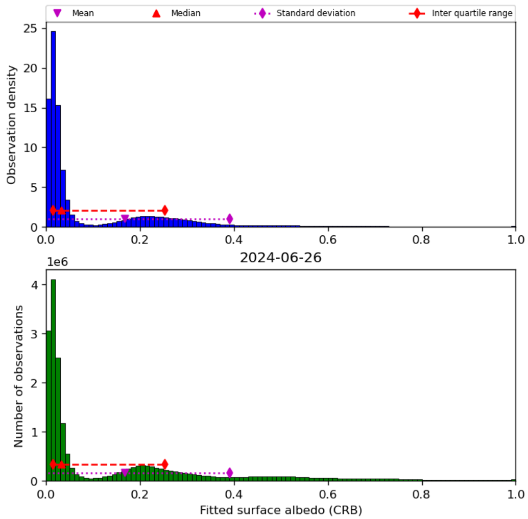
Figure 46: Histogram of “Fitted surface albedo (CRB)” for 2024-06-25 to 2024-06-27
