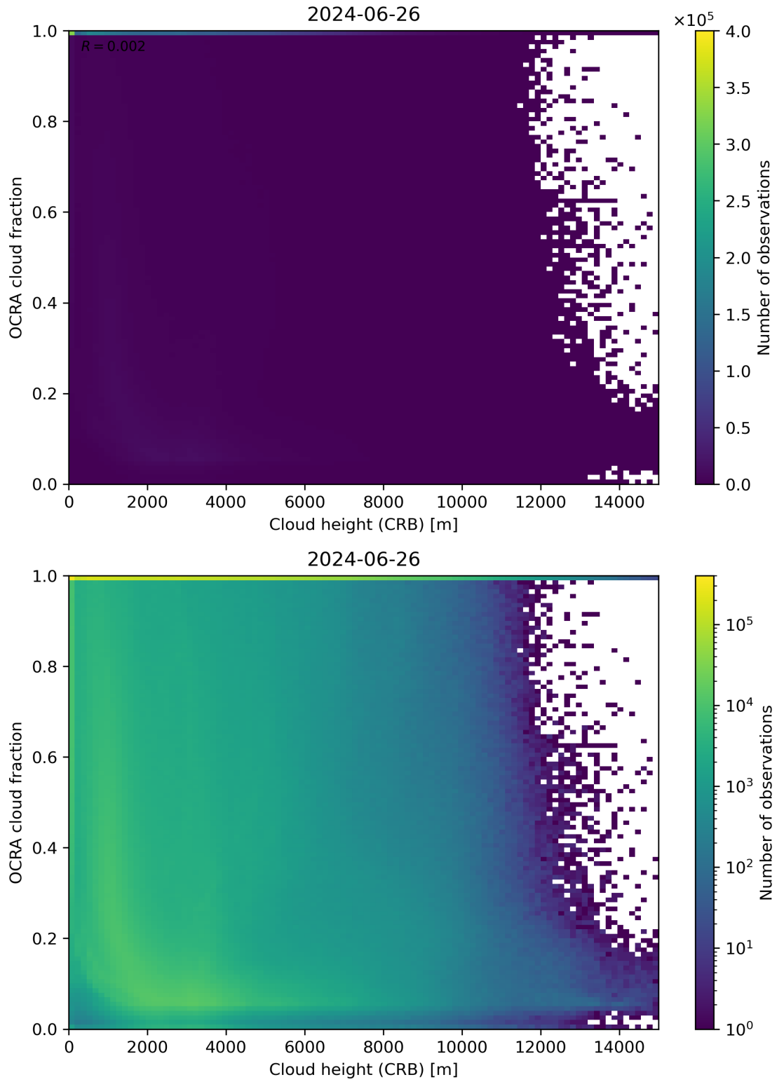
Figure 81: Scatter density plot of “Cloud height (CRB)” against “OCRA cloud fraction” for 2024-06-25 to 2024-06-27.
