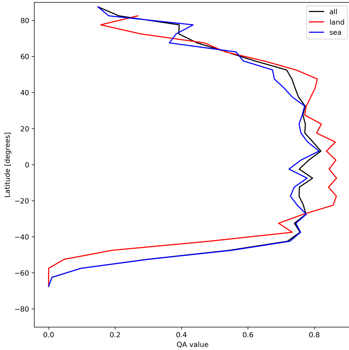
Figure 22: Zonal average of “QA value” for 2024-06-25 to 2024-06-27.
