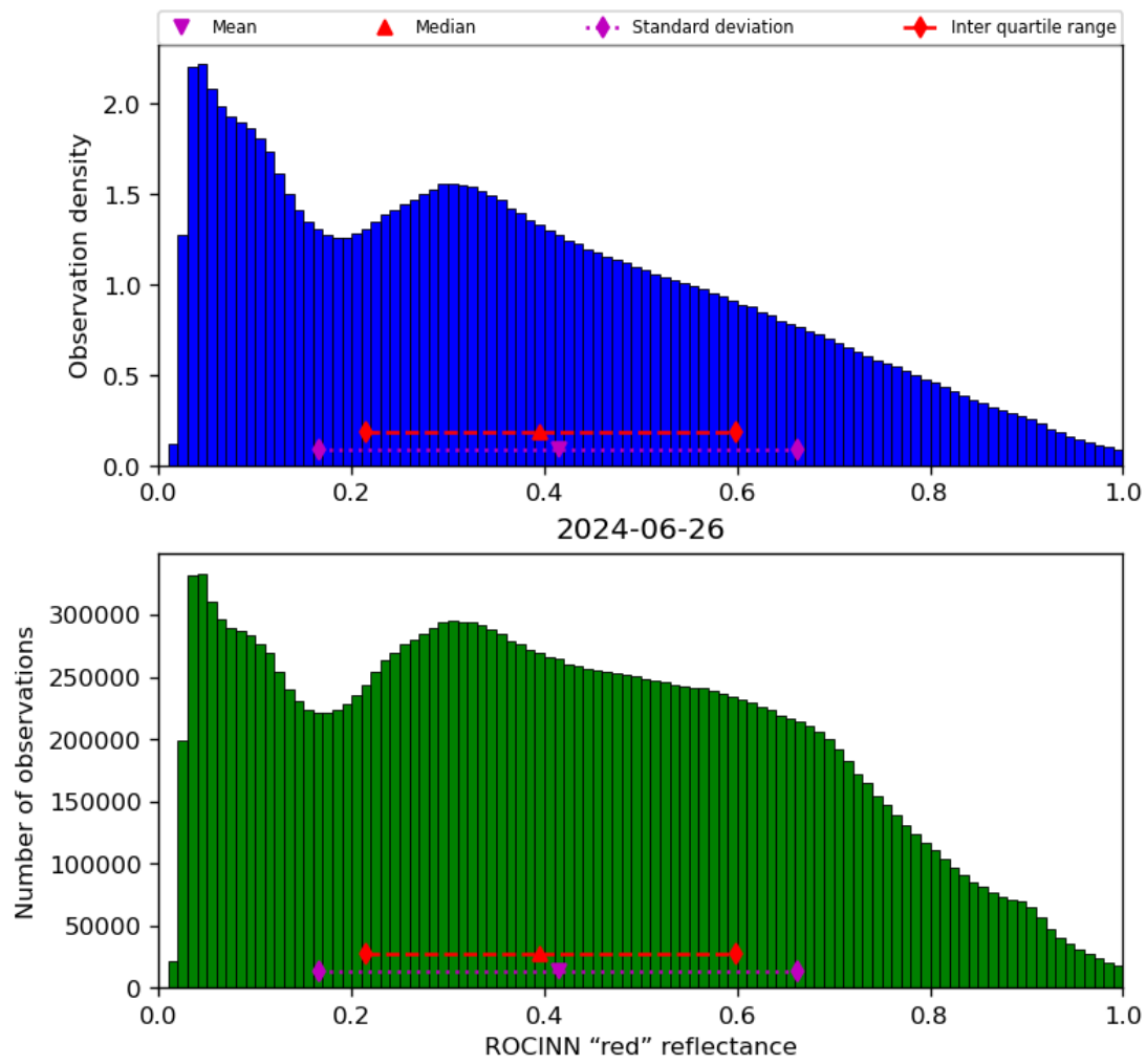
Figure 53: Histogram of “ROCINN “red” reflectance” for 2024-06-25 to 2024-06-27
