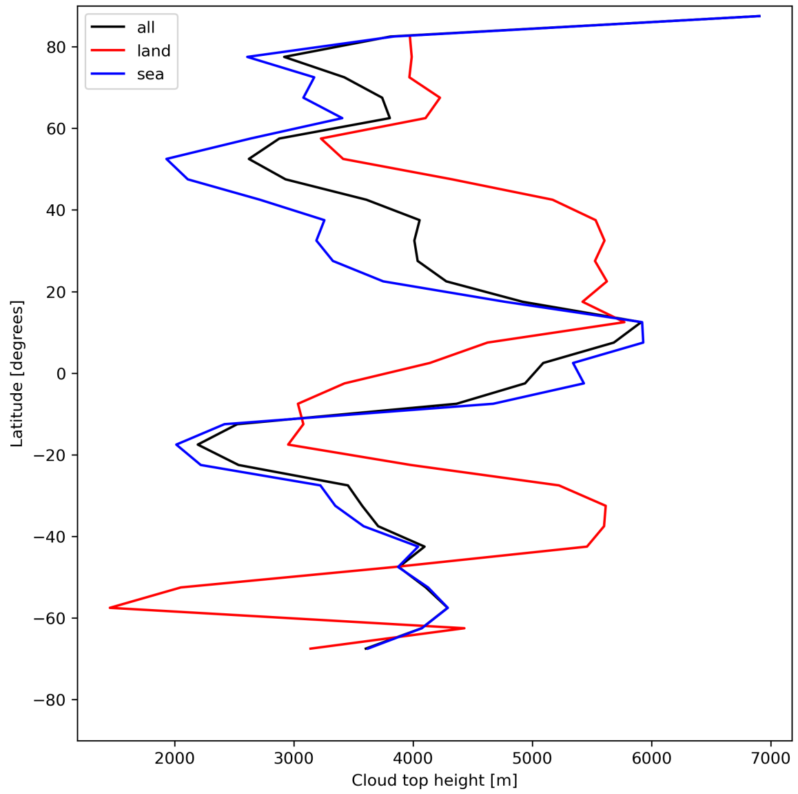
Figure 24: Zonal average of “Cloud top height” for 2024-06-25 to 2024-06-27.
