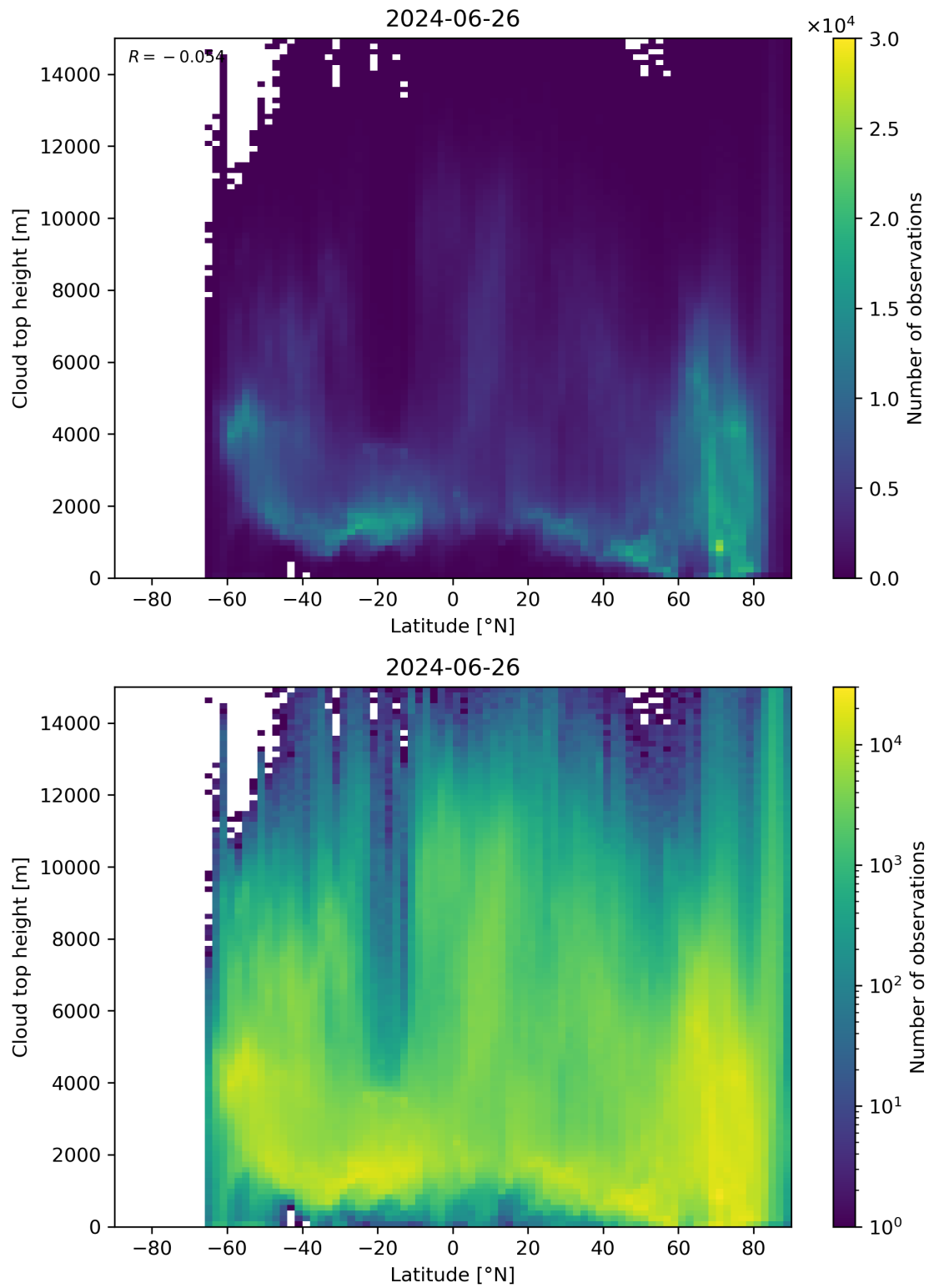
Figure 97: Scatter density plot of “Latitude” against “Cloud top height” for 2024-06-25 to 2024-06-27.
