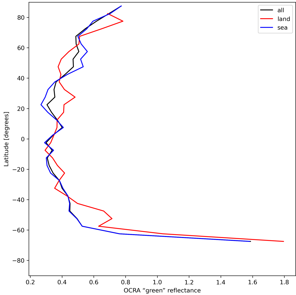
Figure 36: Zonal average of “OCRA “green” reflectance” for 2024-06-25 to 2024-06-27.
