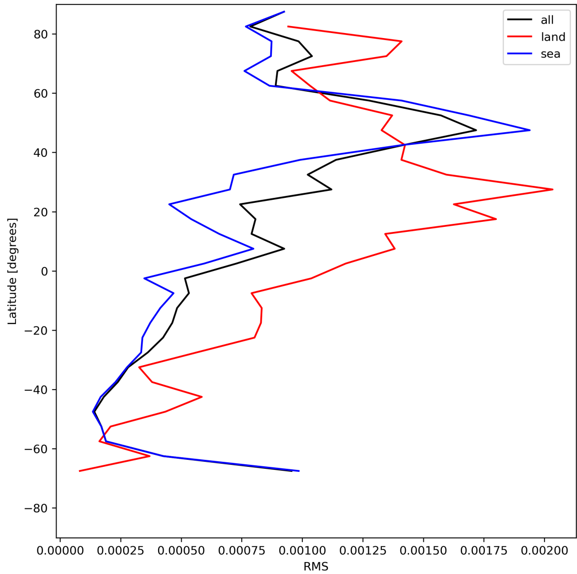
Figure 31: Zonal average of “RMS” for 2024-06-25 to 2024-06-27.
