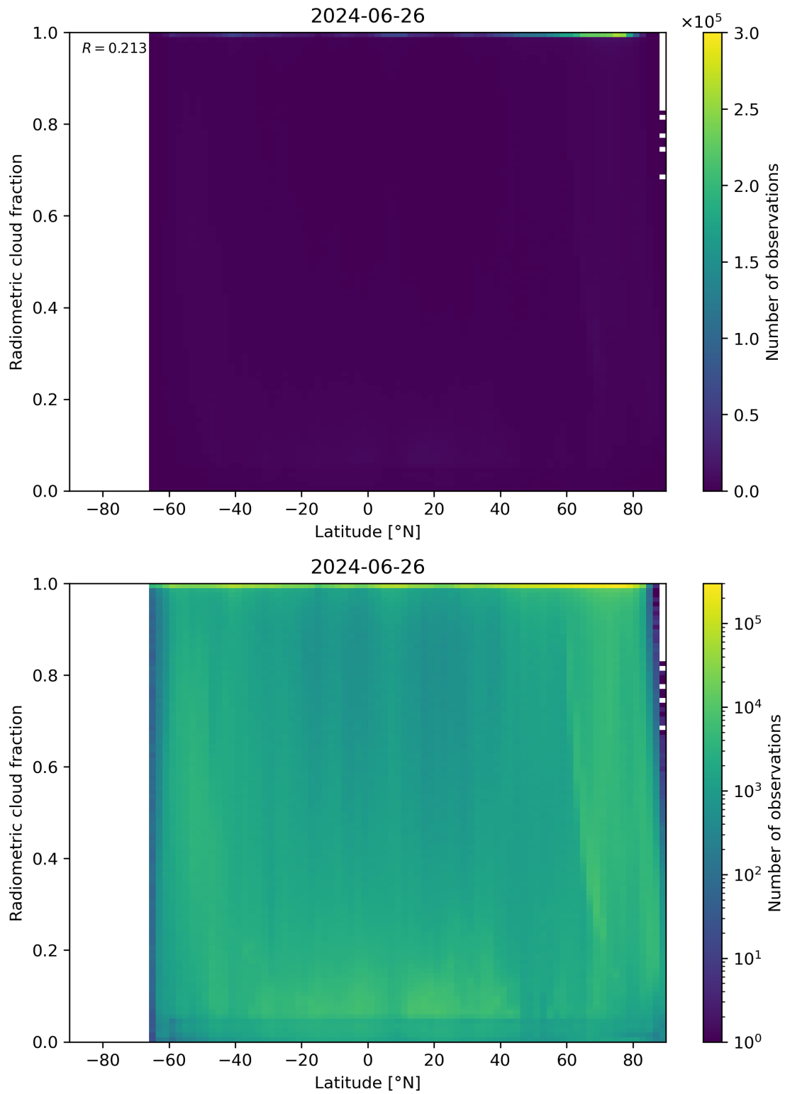
Figure 92: Scatter density plot of “Latitude” against “Radiometric cloud fraction” for 2024-06-25 to 2024-06-27.
