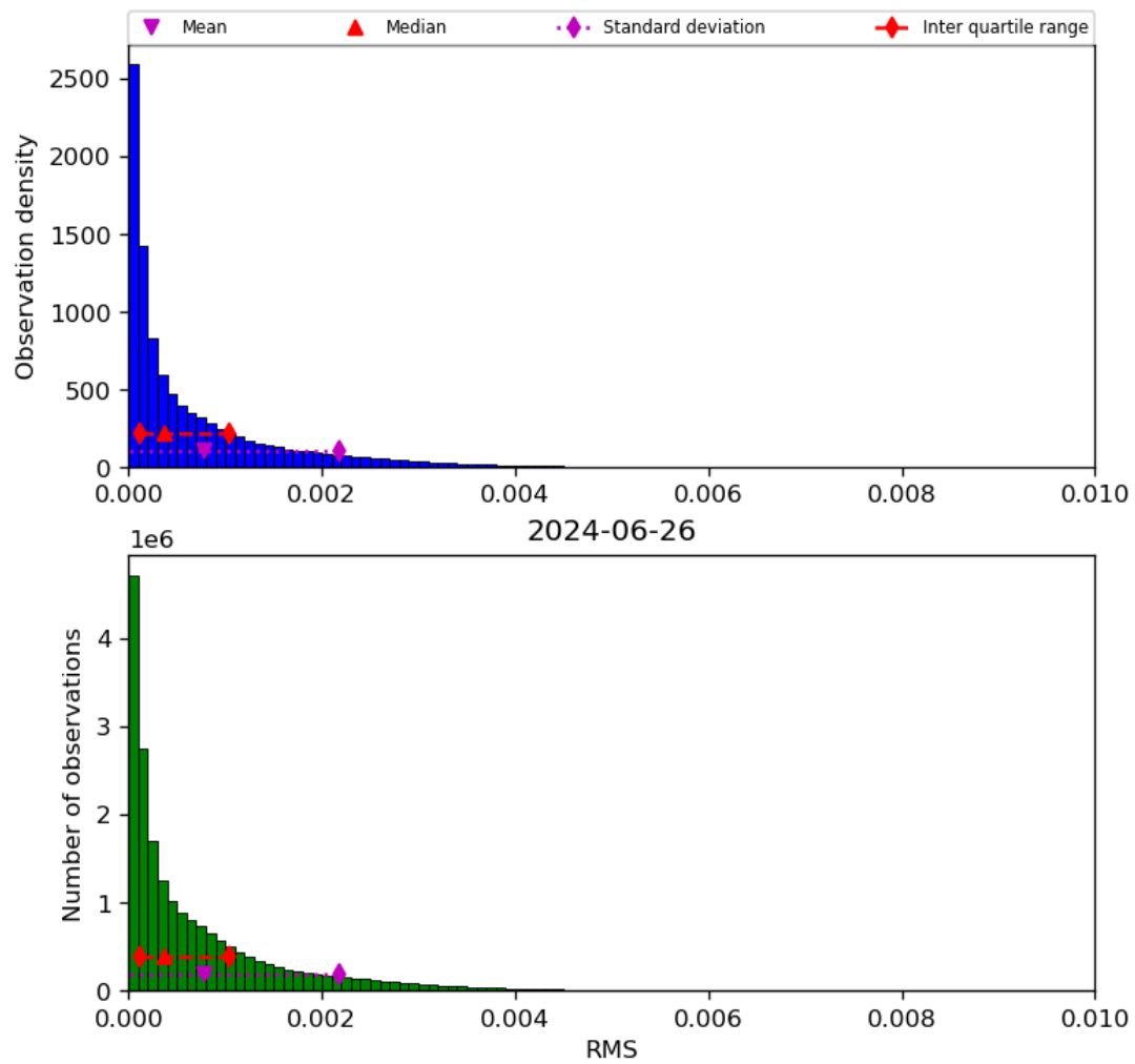
Figure 47: Histogram of “RMS” for 2024-06-25 to 2024-06-27
