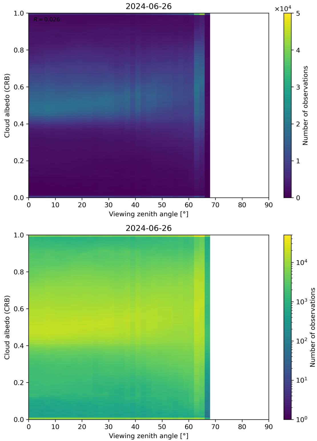
Figure 106: Scatter density plot of “Viewing zenith angle” against “Cloud albedo (CRB)” for 2024-06-25 to 2024-06-27.
