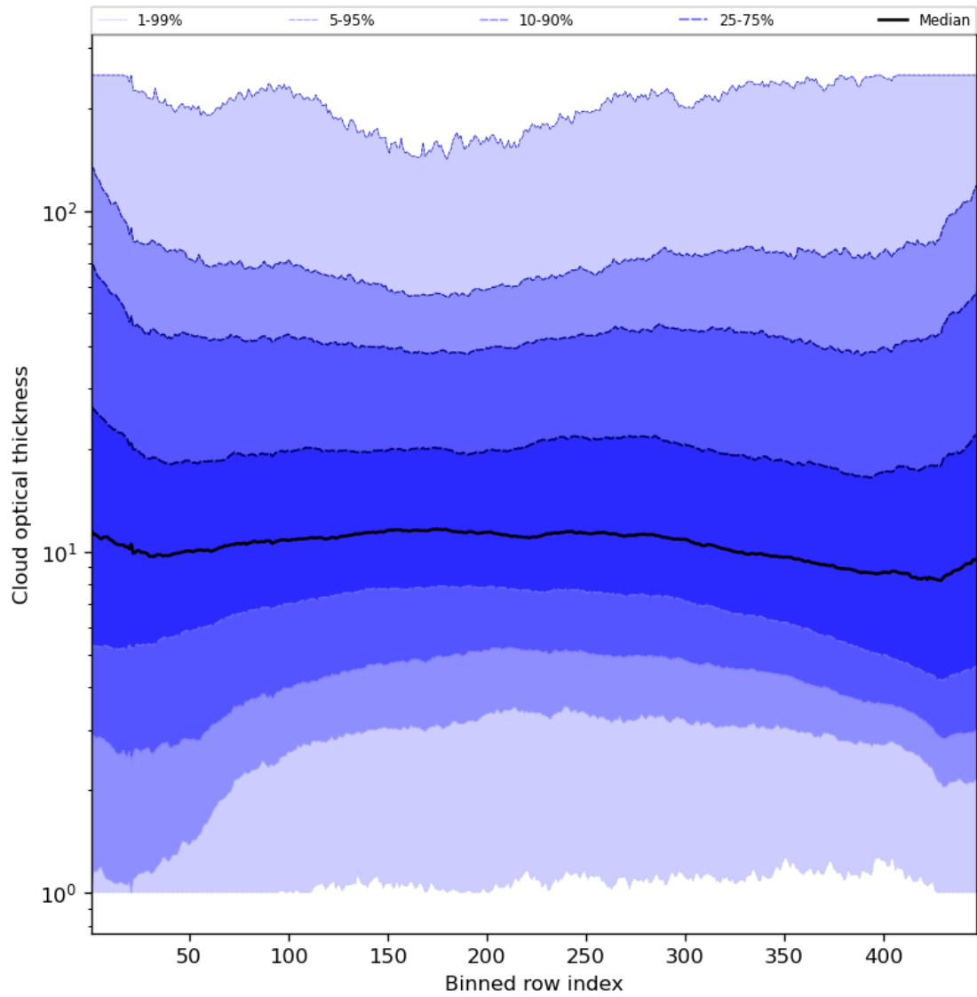
Figure 57: Along track statistics of “Cloud optical thickness” for 2024-06-25 to 2024-06-27
