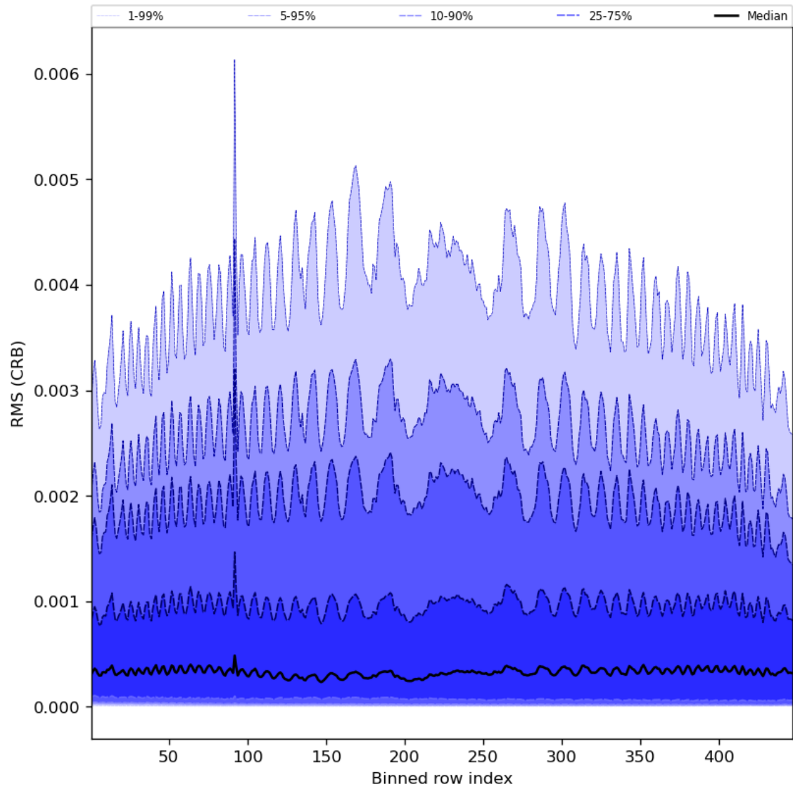
Figure 64: Along track statistics of “RMS (CRB)” for 2024-06-25 to 2024-06-27
