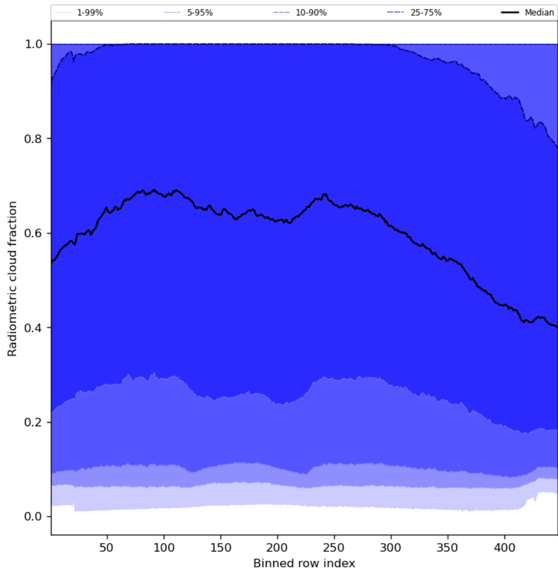
Figure 55: Along track statistics of “Radiometric cloud fraction” for 2024-06-25 to 2024-06-27
