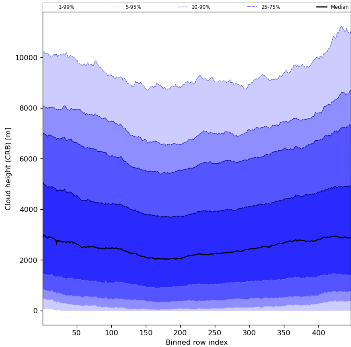
Figure 59: Along track statistics of “Cloud height (CRB)” for 2024-06-25 to 2024-06-27
