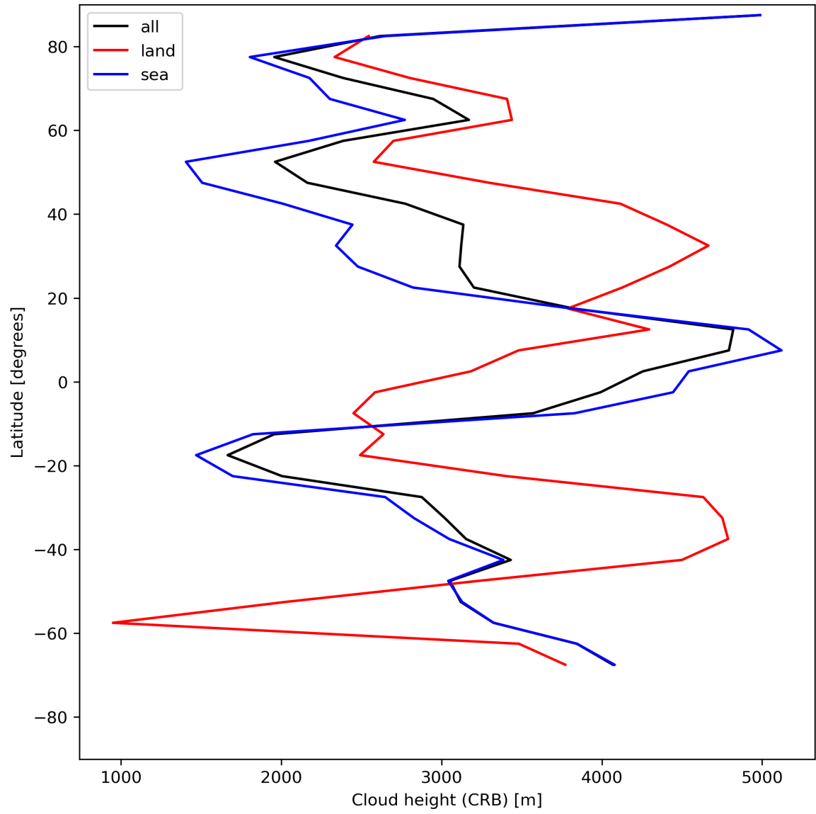
Figure 27: Zonal average of “Cloud height (CRB)” for 2024-06-25 to 2024-06-27.
