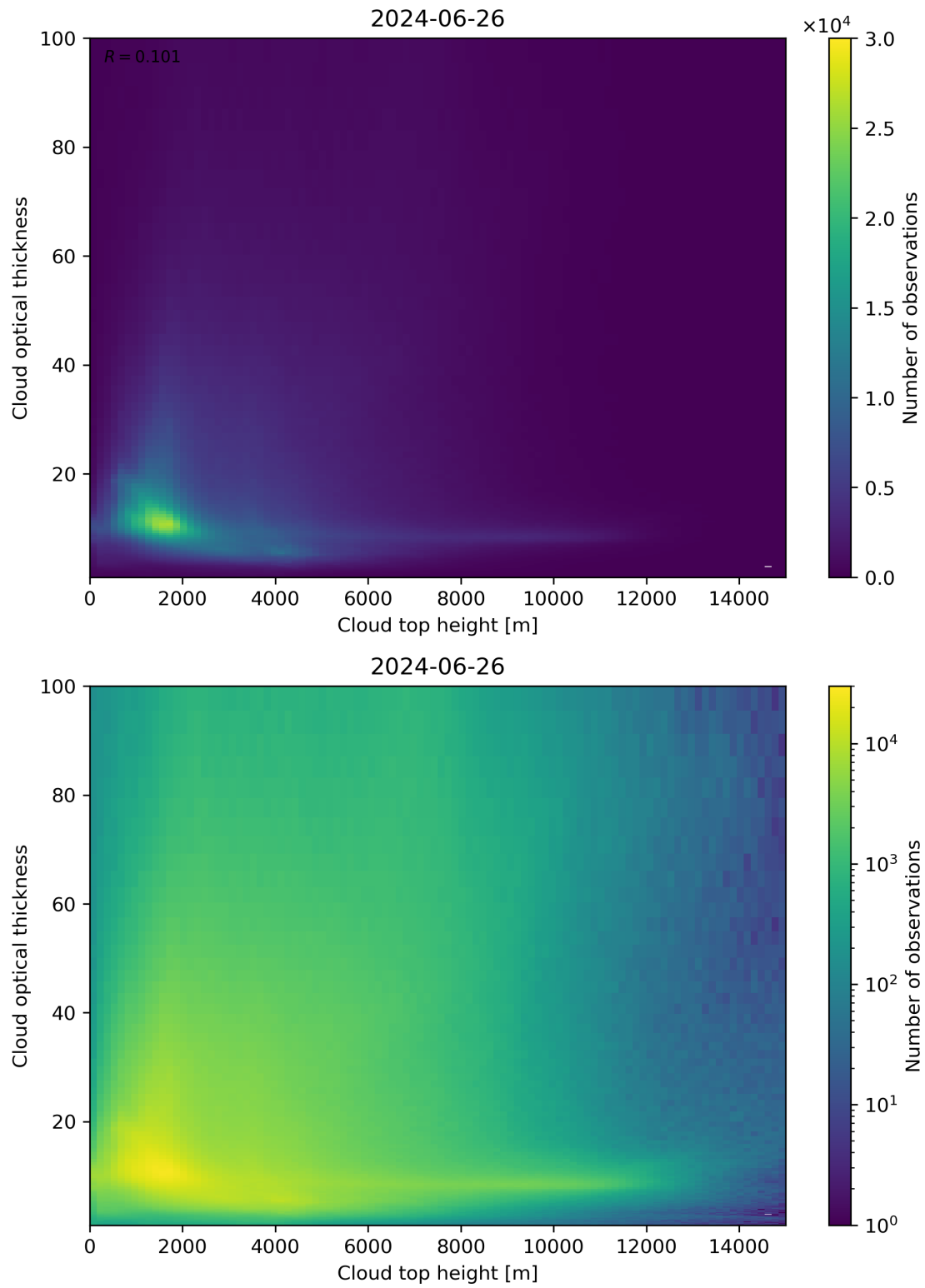
Figure 90: Scatter density plot of “Cloud top height” against “Cloud optical thickness” for 2024-06-25 to 2024-06-27.
