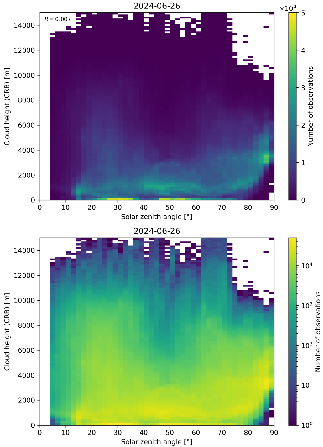
Figure 102: Scatter density plot of “Solar zenith angle” against “Cloud height (CRB)” for 2024-06-25 to 2024-06-27.
