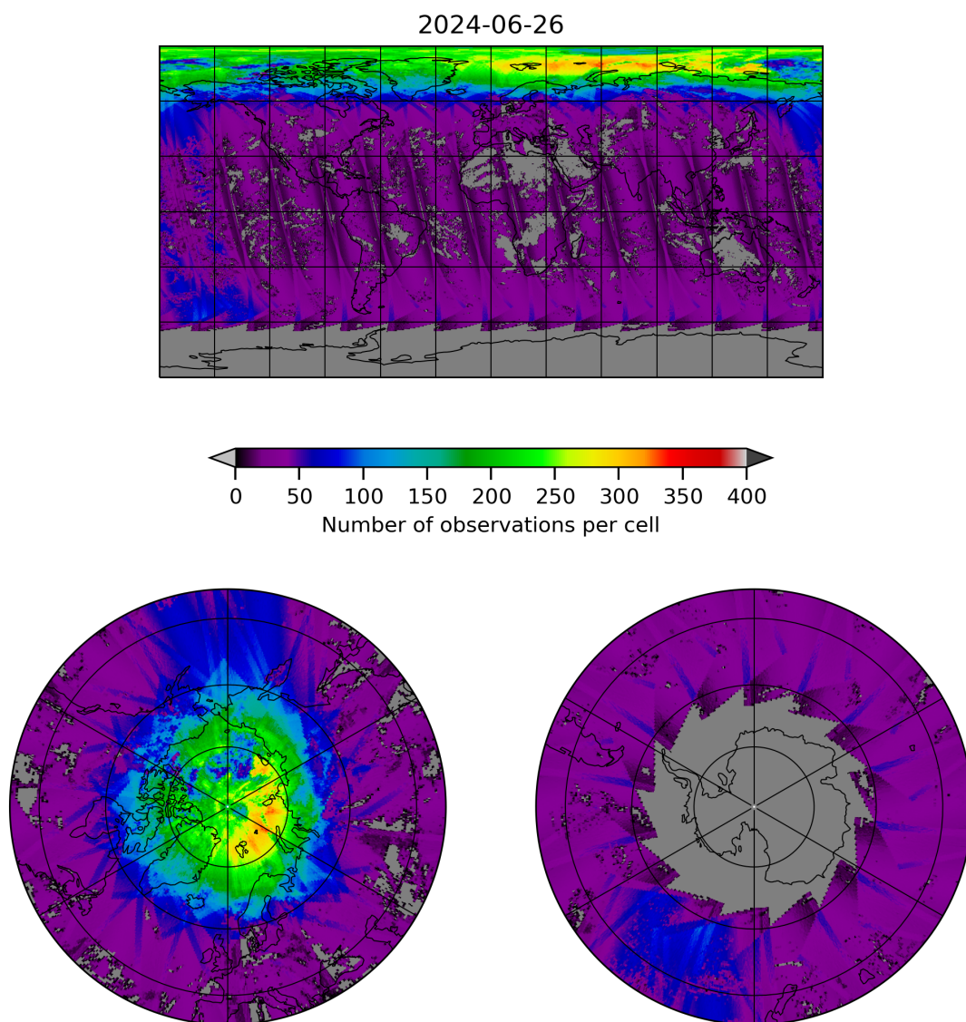
Figure 21: Map of the number of observations for 2024-06-25 to 2024-06-27
