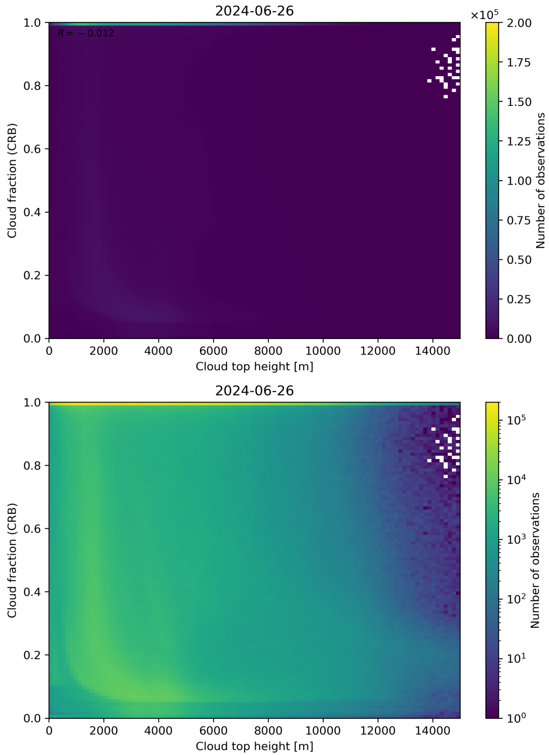
Figure 88: Scatter density plot of “Cloud top height” against “Cloud fraction (CRB)” for 2024-06-25 to 2024-06-27.
