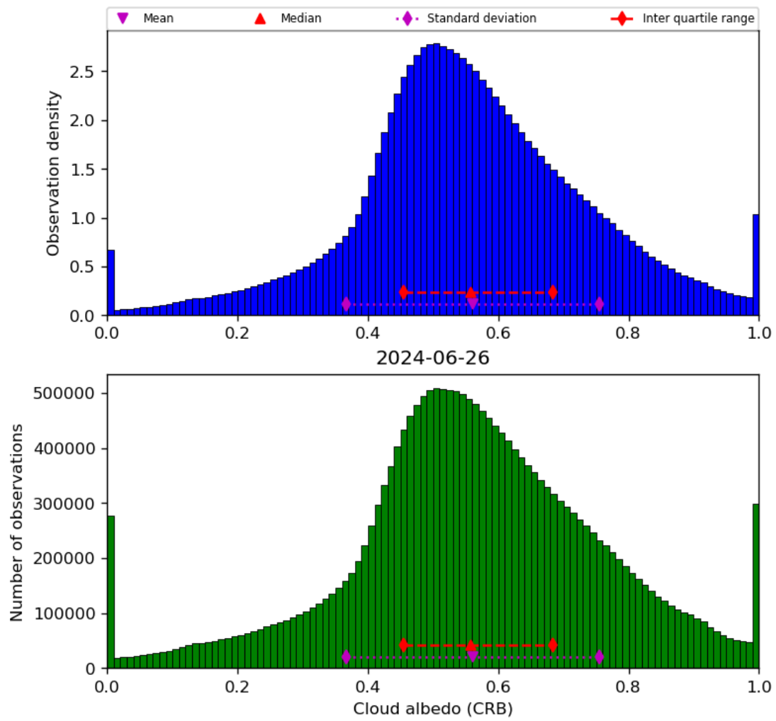
Figure 44: Histogram of “Cloud albedo (CRB)” for 2024-06-25 to 2024-06-27
