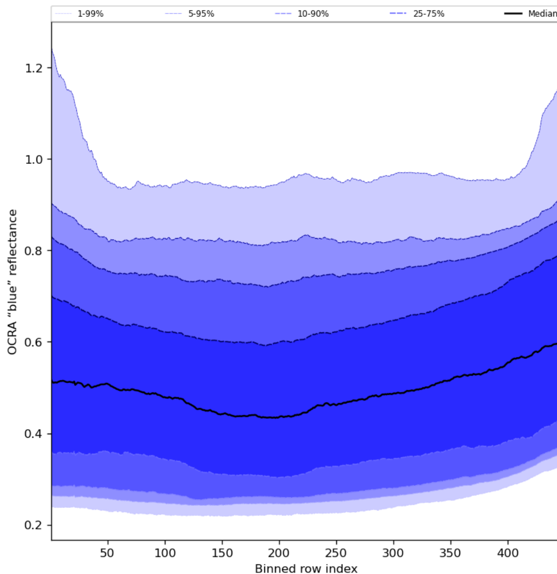
Figure 67: Along track statistics of “OCRA “blue” reflectance” for 2024-06-25 to 2024-06-27
