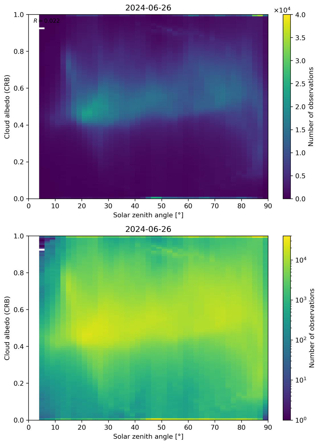
Figure 98: Scatter density plot of “Solar zenith angle” against “Cloud albedo (CRB)” for 2024-06-25 to 2024-06-27.
