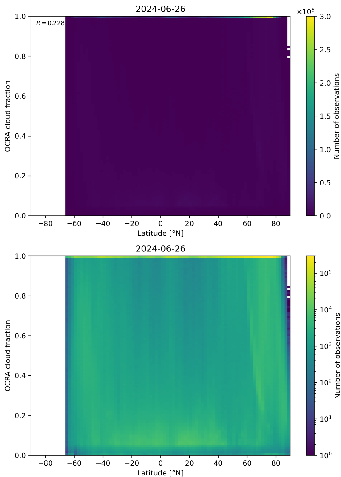
Figure 93: Scatter density plot of “Latitude” against “OCRA cloud fraction” for 2024-06-25 to 2024-06-27.
