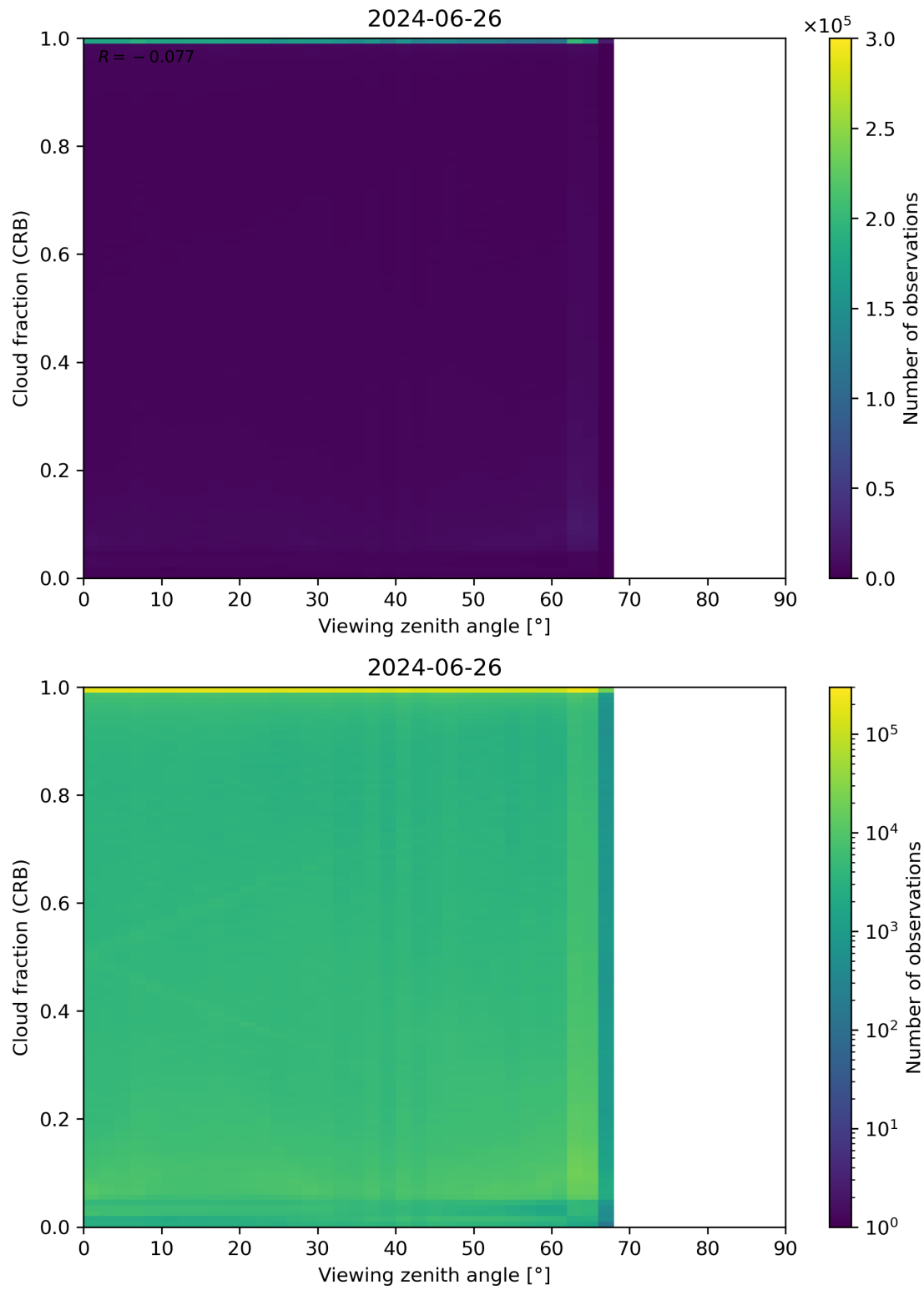
Figure 109: Scatter density plot of “Viewing zenith angle” against “Cloud fraction (CRB)” for 2024-06-25 to 2024-06-27.
