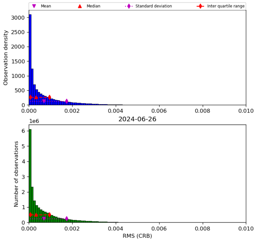
Figure 48: Histogram of “RMS (CRB)” for 2024-06-25 to 2024-06-27
