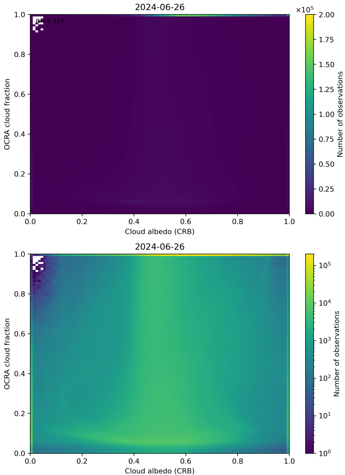
Figure 70: Scatter density plot of “Cloud albedo (CRB)” against “OCRA cloud fraction” for 2024-06-25 to 2024-06-27.
