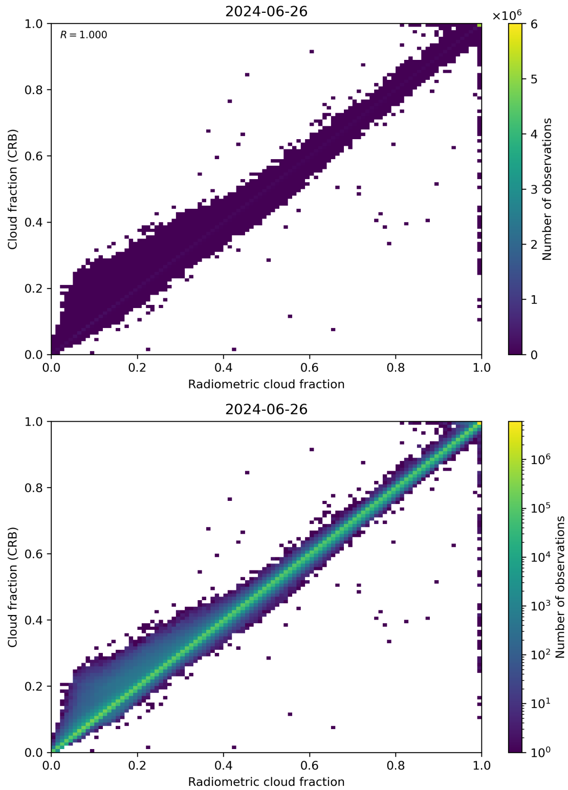
Figure 73: Scatter density plot of “Radiometric cloud fraction” against “Cloud fraction (CRB)” for 2024-06-25 to 2024-06-27.
