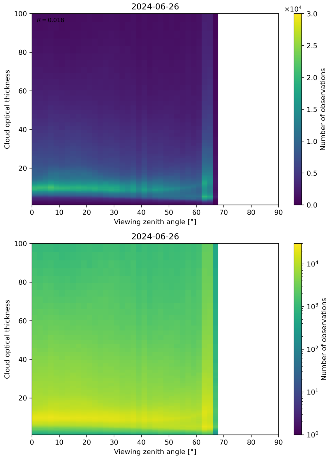
Figure 111: Scatter density plot of “Viewing zenith angle” against “Cloud optical thickness” for 2024-06-25 to 2024-06-27.
