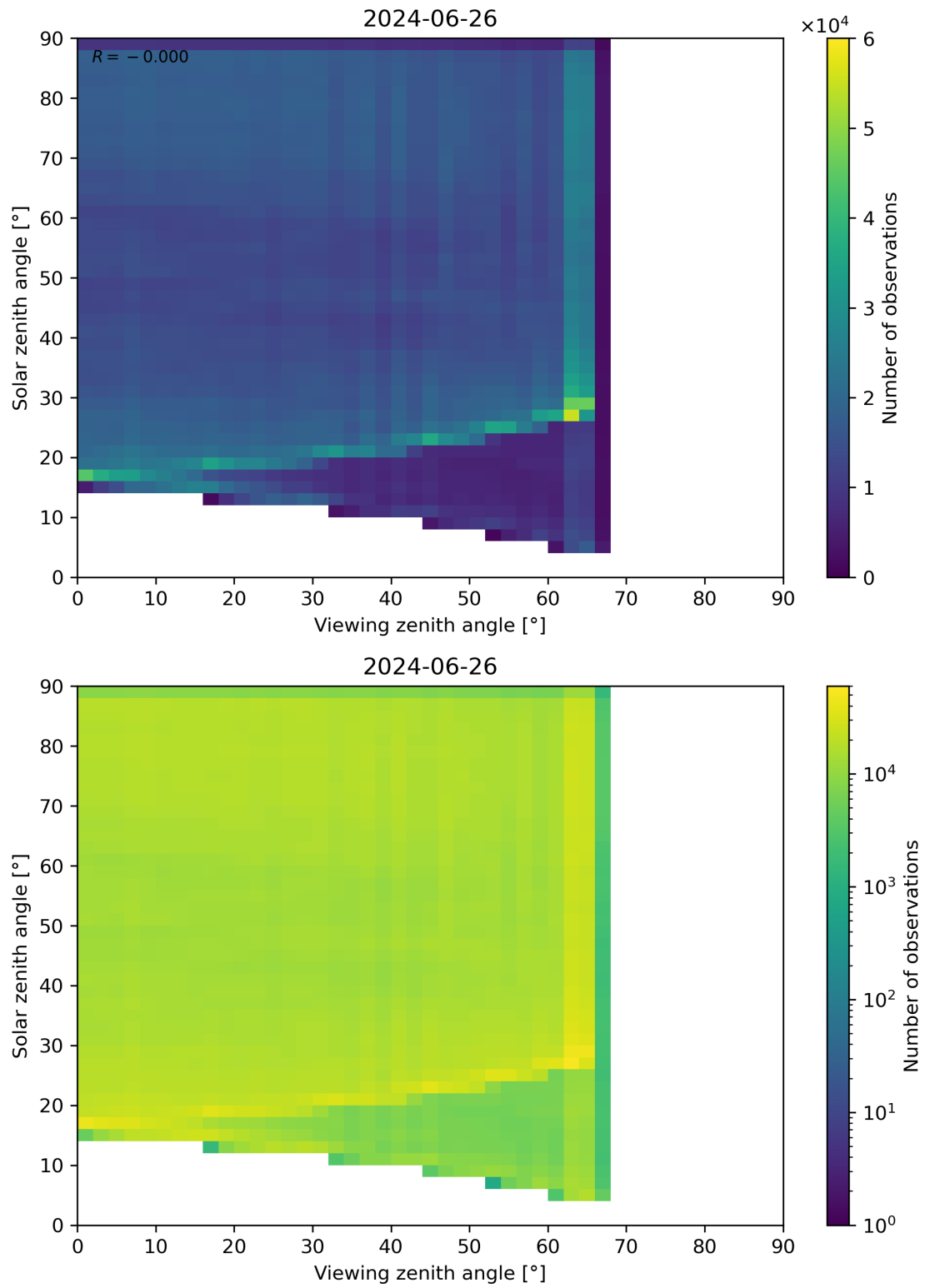
Figure 114: Scatter density plot of “Viewing zenith angle” against “Solar zenith angle” for 2024-06-25 to 2024-06-27.
