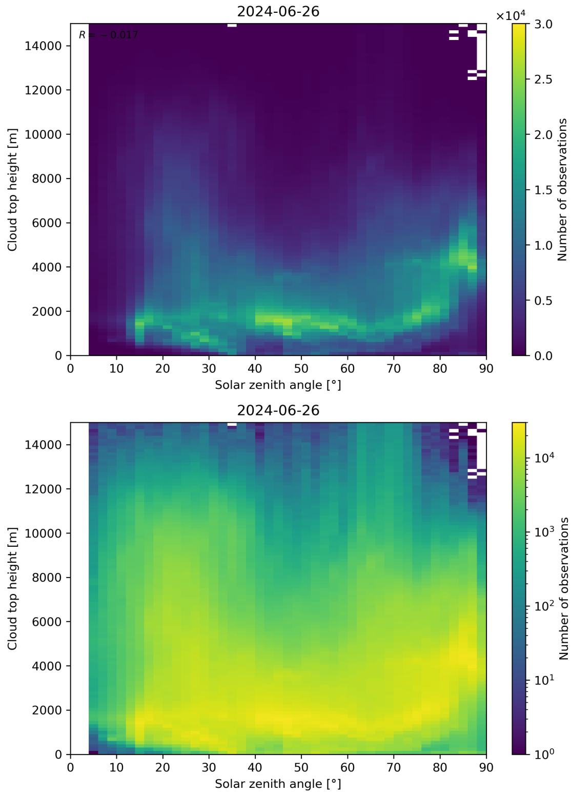
Figure 104: Scatter density plot of “Solar zenith angle” against “Cloud top height” for 2024-06-25 to 2024-06-27.
