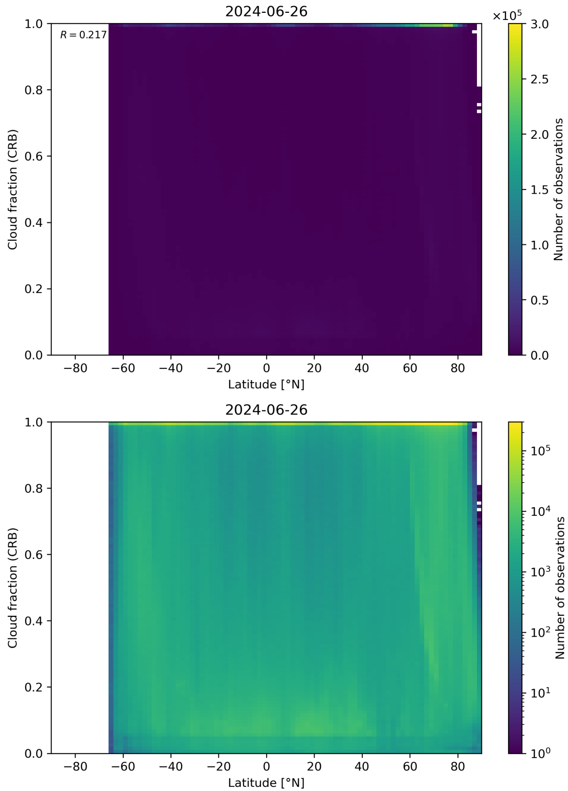
Figure 94: Scatter density plot of “Latitude” against “Cloud fraction (CRB)” for 2024-06-25 to 2024-06-27.
