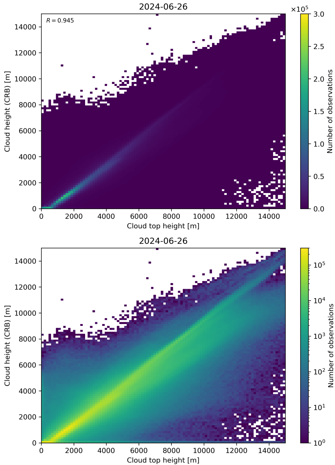
Figure 89: Scatter density plot of “Cloud top height” against “Cloud height (CRB)” for 2024-06-25 to 2024-06-27.
