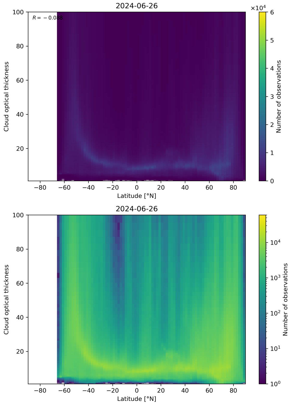
Figure 96: Scatter density plot of “Latitude” against “Cloud optical thickness” for 2024-06-25 to 2024-06-27.
