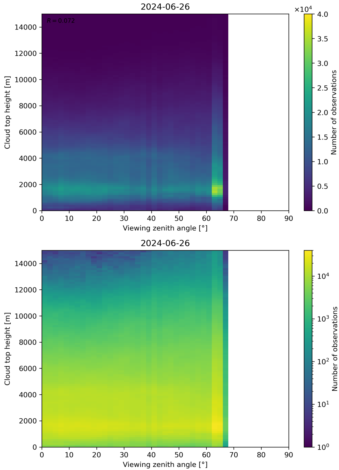
Figure 112: Scatter density plot of “Viewing zenith angle” against “Cloud top height” for 2024-06-25 to 2024-06-27.
