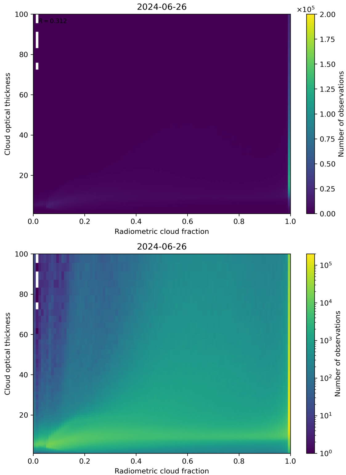
Figure 75: Scatter density plot of “Radiometric cloud fraction” against “Cloud optical thickness” for 2024-06-25 to 2024-06-27.
