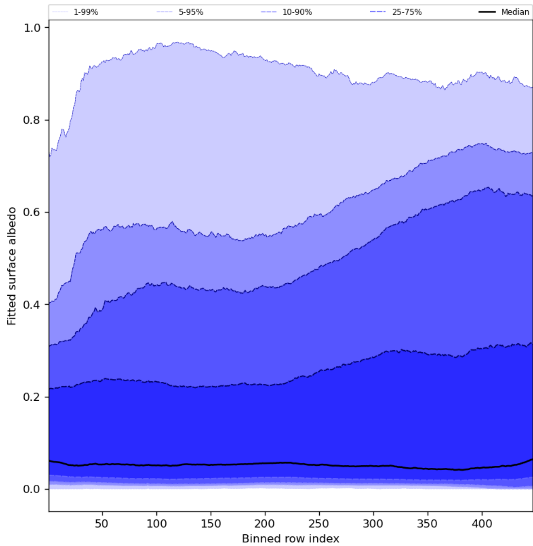
Figure 61: Along track statistics of “Fitted surface albedo” for 2024-06-25 to 2024-06-27
