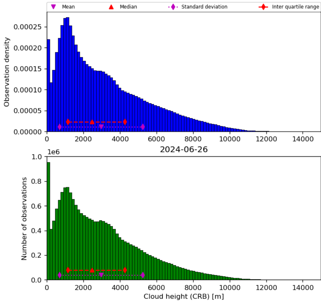
Figure 43: Histogram of “Cloud height (CRB)” for 2024-06-25 to 2024-06-27
