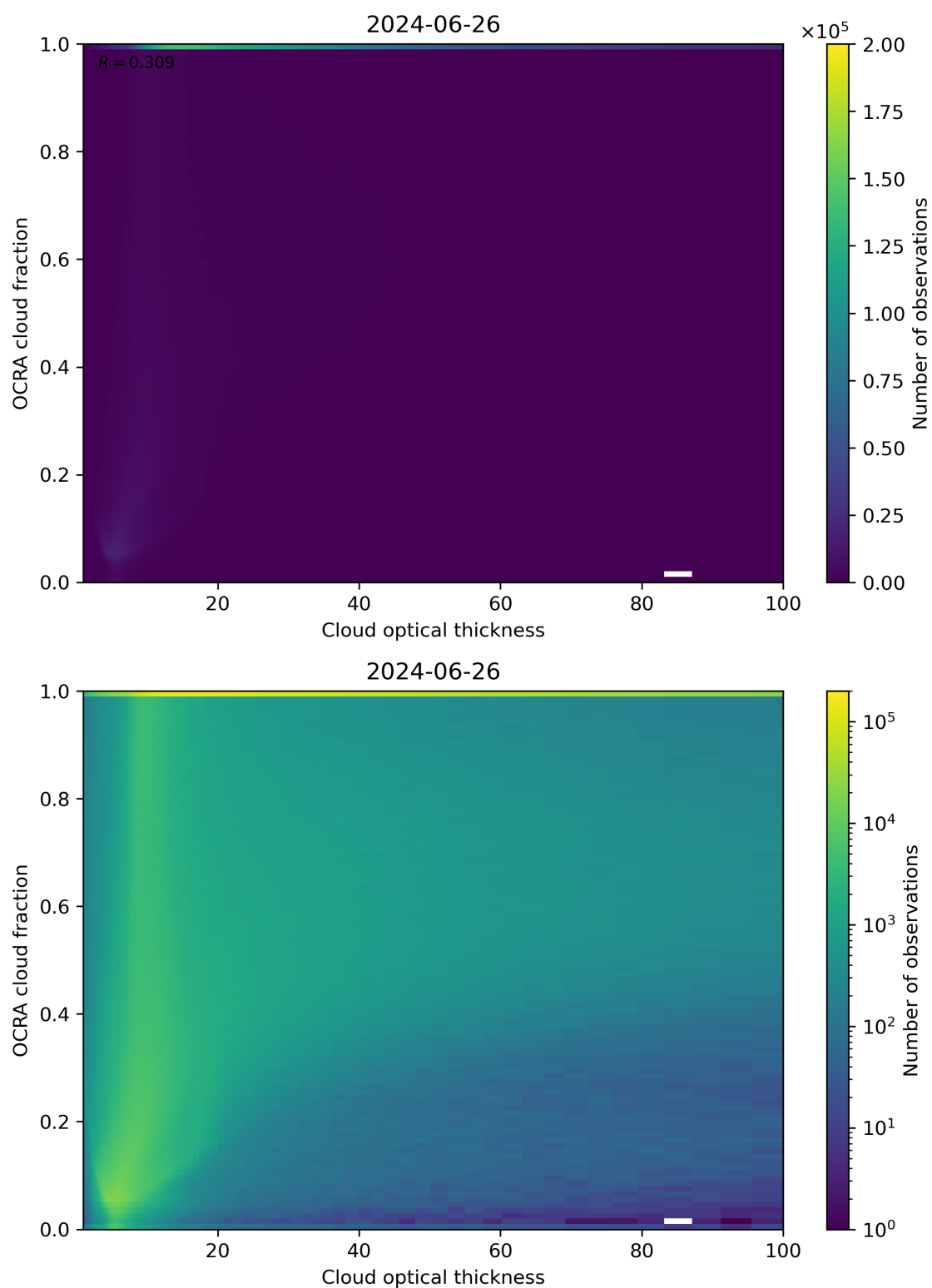
Figure 83: Scatter density plot of “Cloud optical thickness” against “OCRA cloud fraction” for 2024-06-25 to 2024-06-27.
