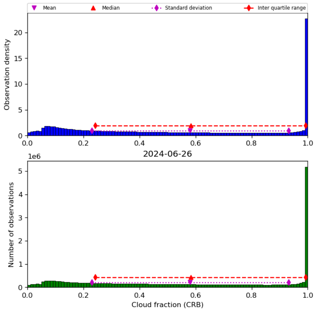
Figure 42: Histogram of “Cloud fraction (CRB)” for 2024-06-25 to 2024-06-27
