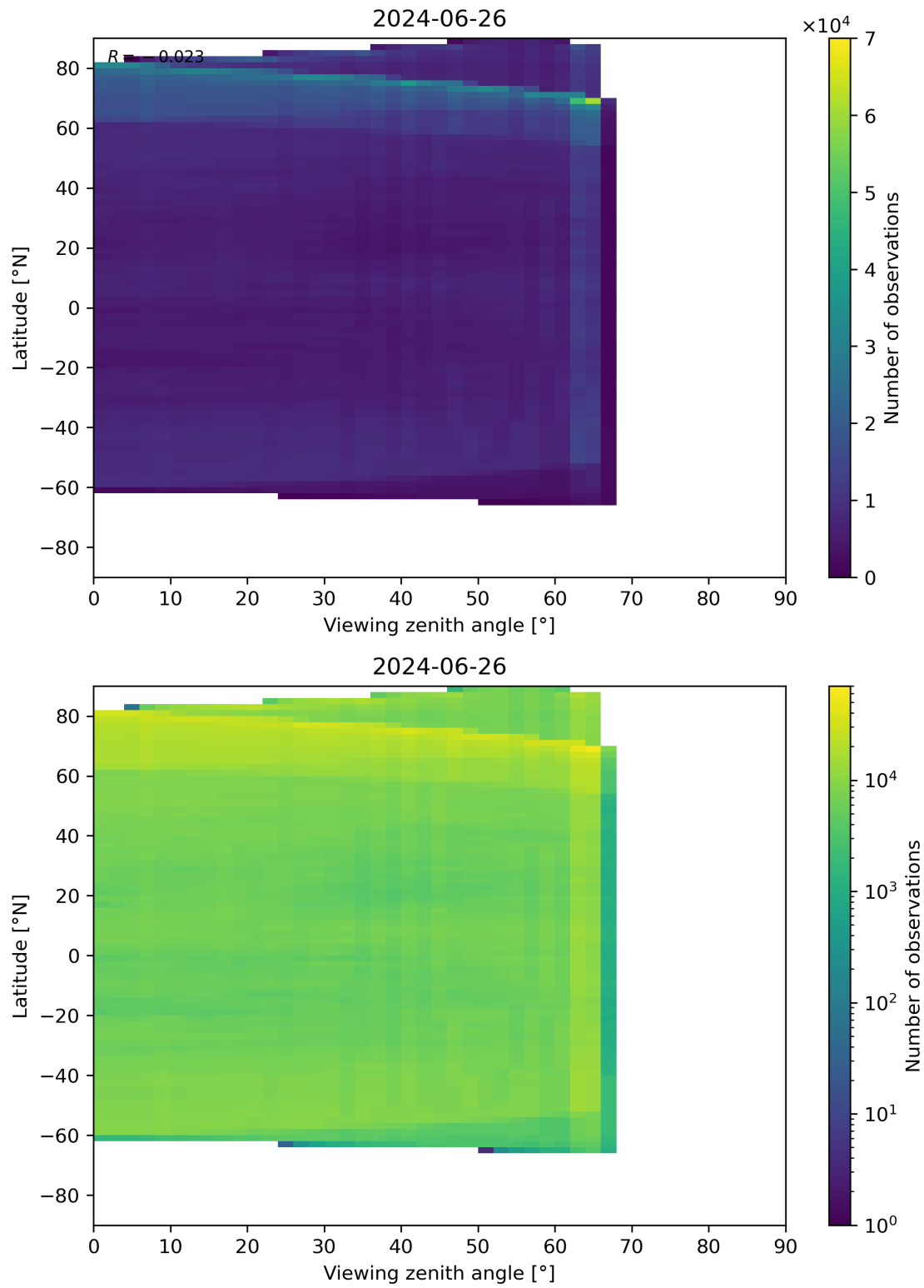
Figure 113: Scatter density plot of “Viewing zenith angle” against “Latitude” for 2024-06-25 to 2024-06-27.
