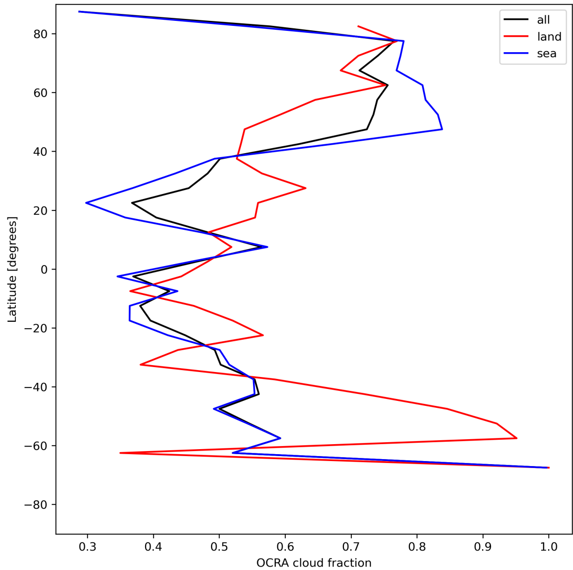
Figure 34: Zonal average of “OCRA cloud fraction” for 2024-06-25 to 2024-06-27.
