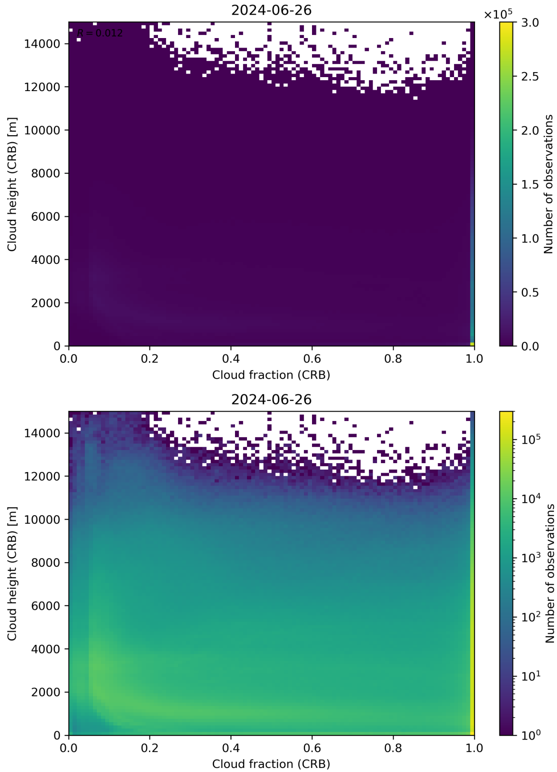
Figure 79: Scatter density plot of “Cloud fraction (CRB)” against “Cloud height (CRB)” for 2024-06-25 to 2024-06-27.
