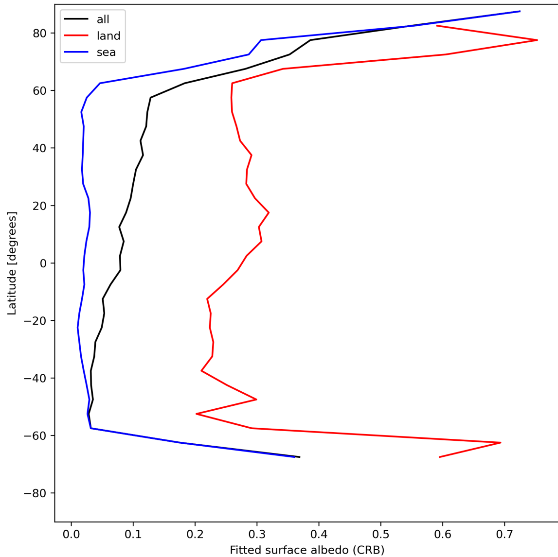
Figure 30: Zonal average of “Fitted surface albedo (CRB)” for 2024-06-25 to 2024-06-27.
