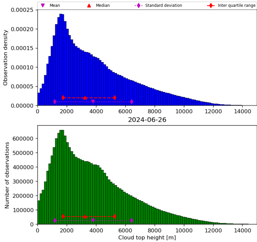
Figure 40: Histogram of “Cloud top height” for 2024-06-25 to 2024-06-27
