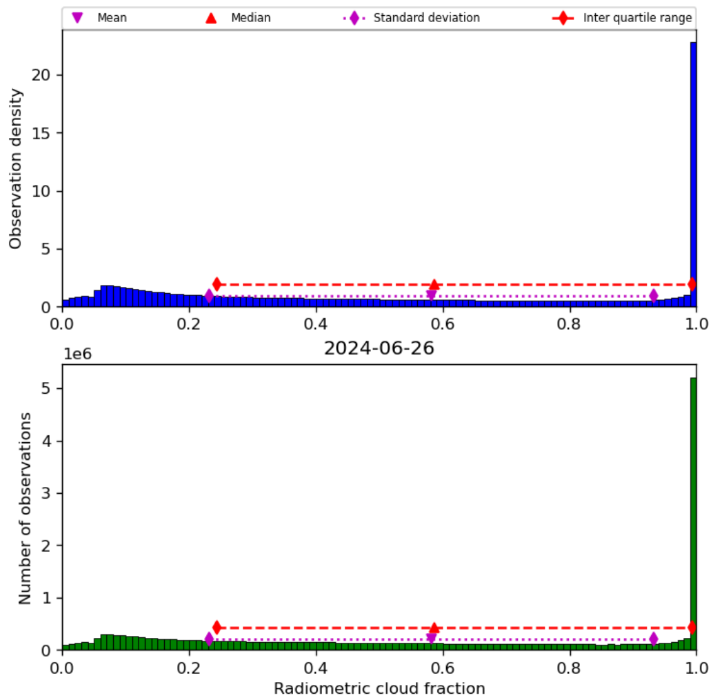
Figure 39: Histogram of “Radiometric cloud fraction” for 2024-06-25 to 2024-06-27
