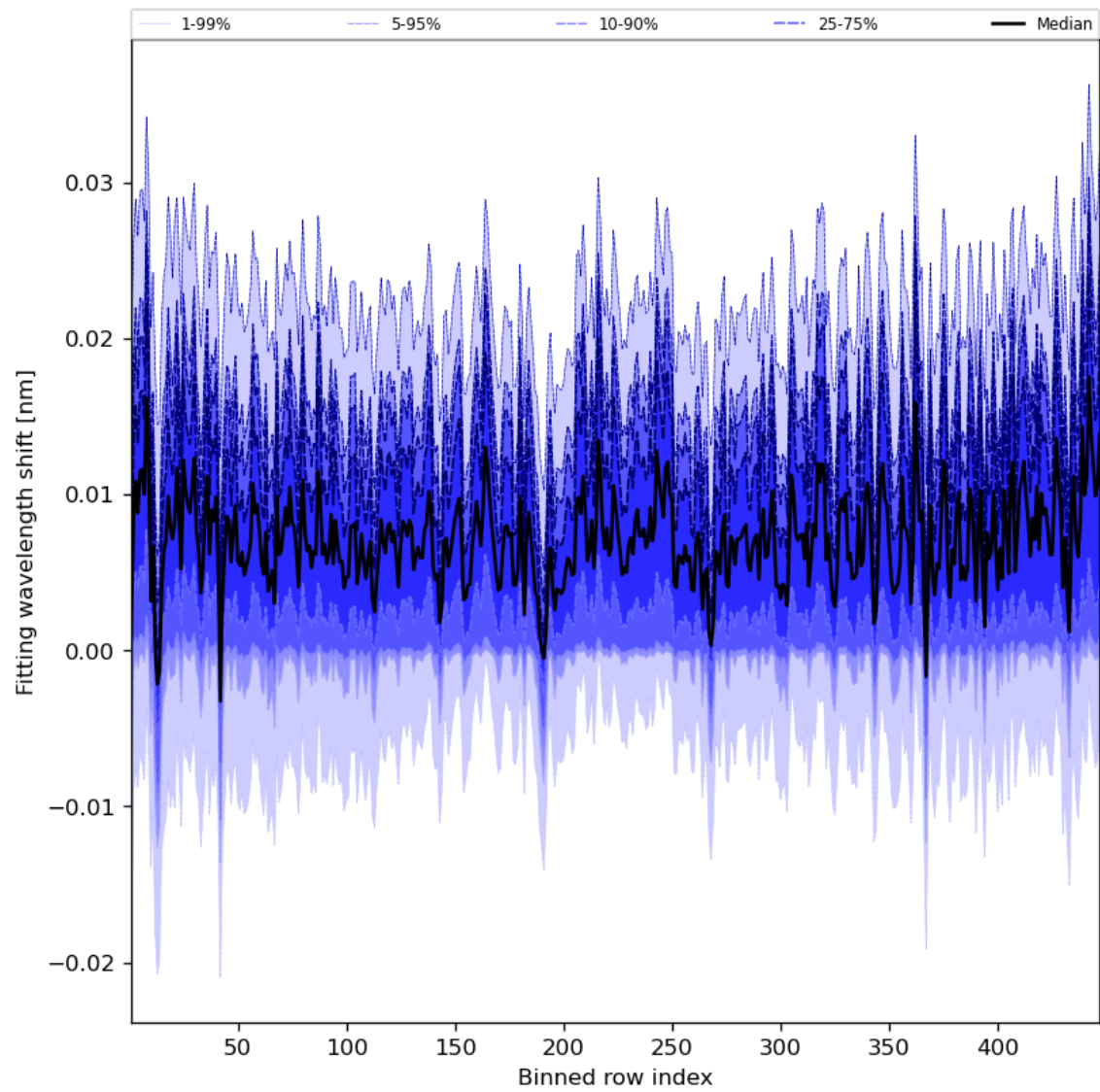
Figure 65: Along track statistics of “Fitting wavelength shift” for 2024-06-25 to 2024-06-27
