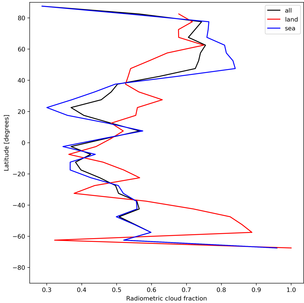
Figure 23: Zonal average of “Radiometric cloud fraction” for 2024-06-25 to 2024-06-27.
