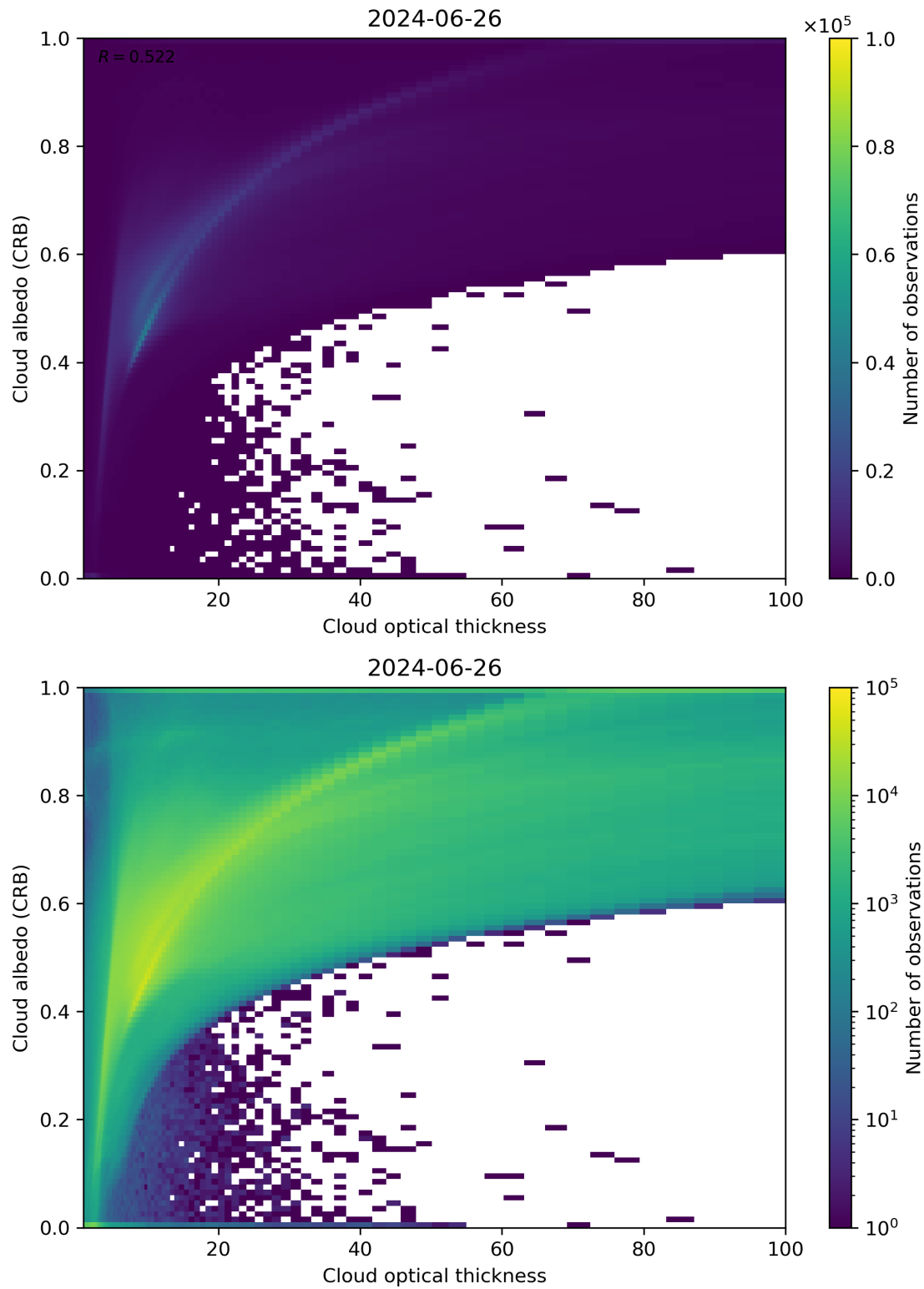
Figure 82: Scatter density plot of “Cloud optical thickness” against “Cloud albedo (CRB)” for 2024-06-25 to 2024-06-27.
