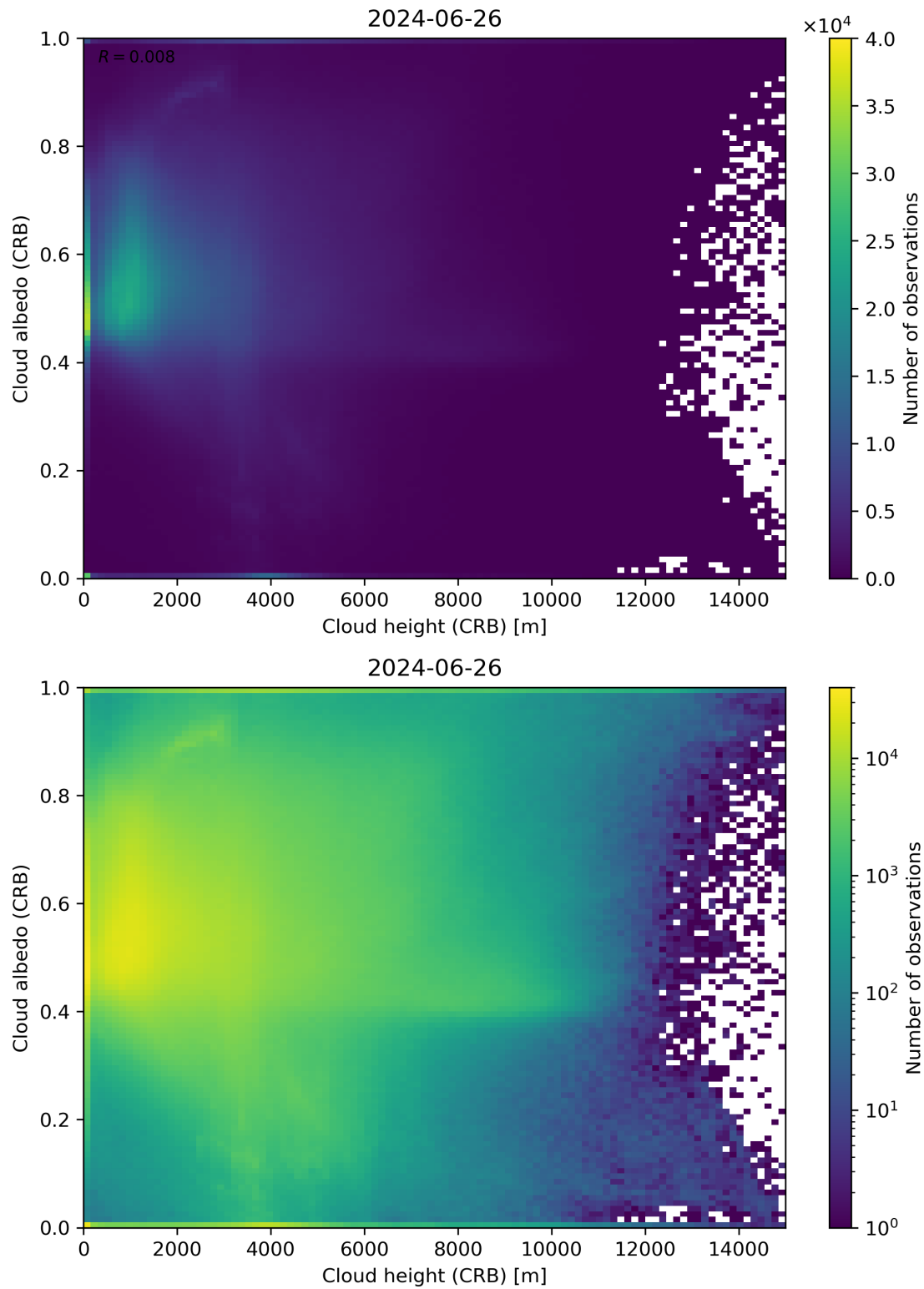
Figure 80: Scatter density plot of “Cloud height (CRB)” against “Cloud albedo (CRB)” for 2024-06-25 to 2024-06-27.
