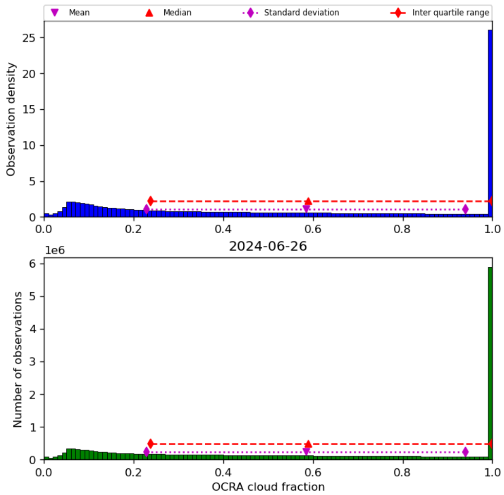
Figure 50: Histogram of “OCRA cloud fraction” for 2024-06-25 to 2024-06-27
