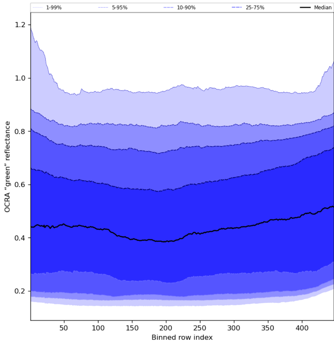
Figure 68: Along track statistics of “OCRA “green” reflectance” for 2024-06-25 to 2024-06-27
