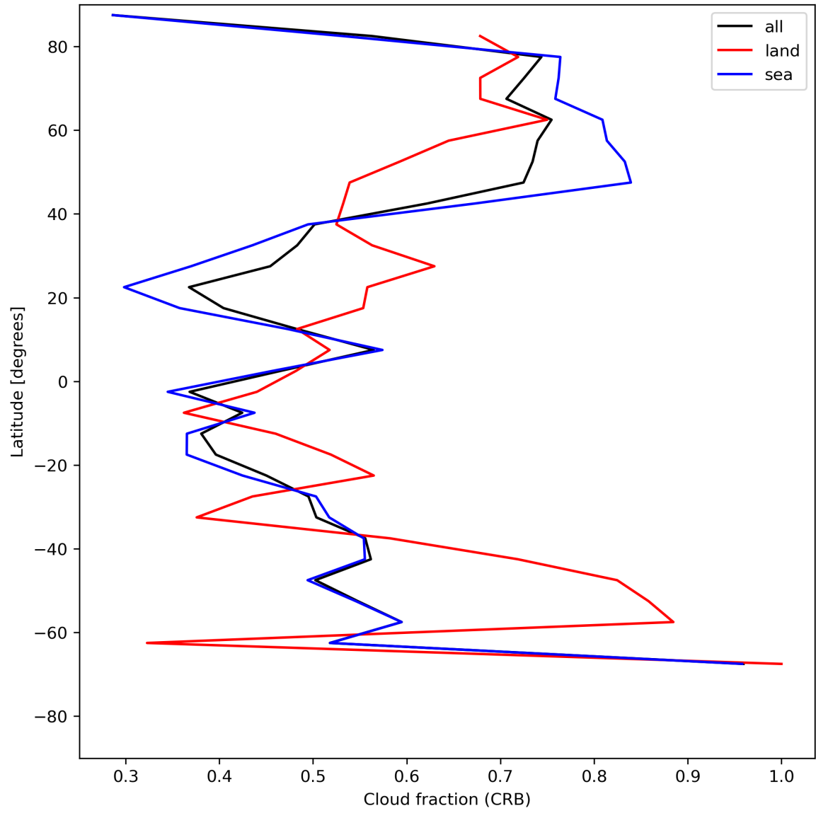
Figure 26: Zonal average of “Cloud fraction (CRB)” for 2024-06-25 to 2024-06-27.
