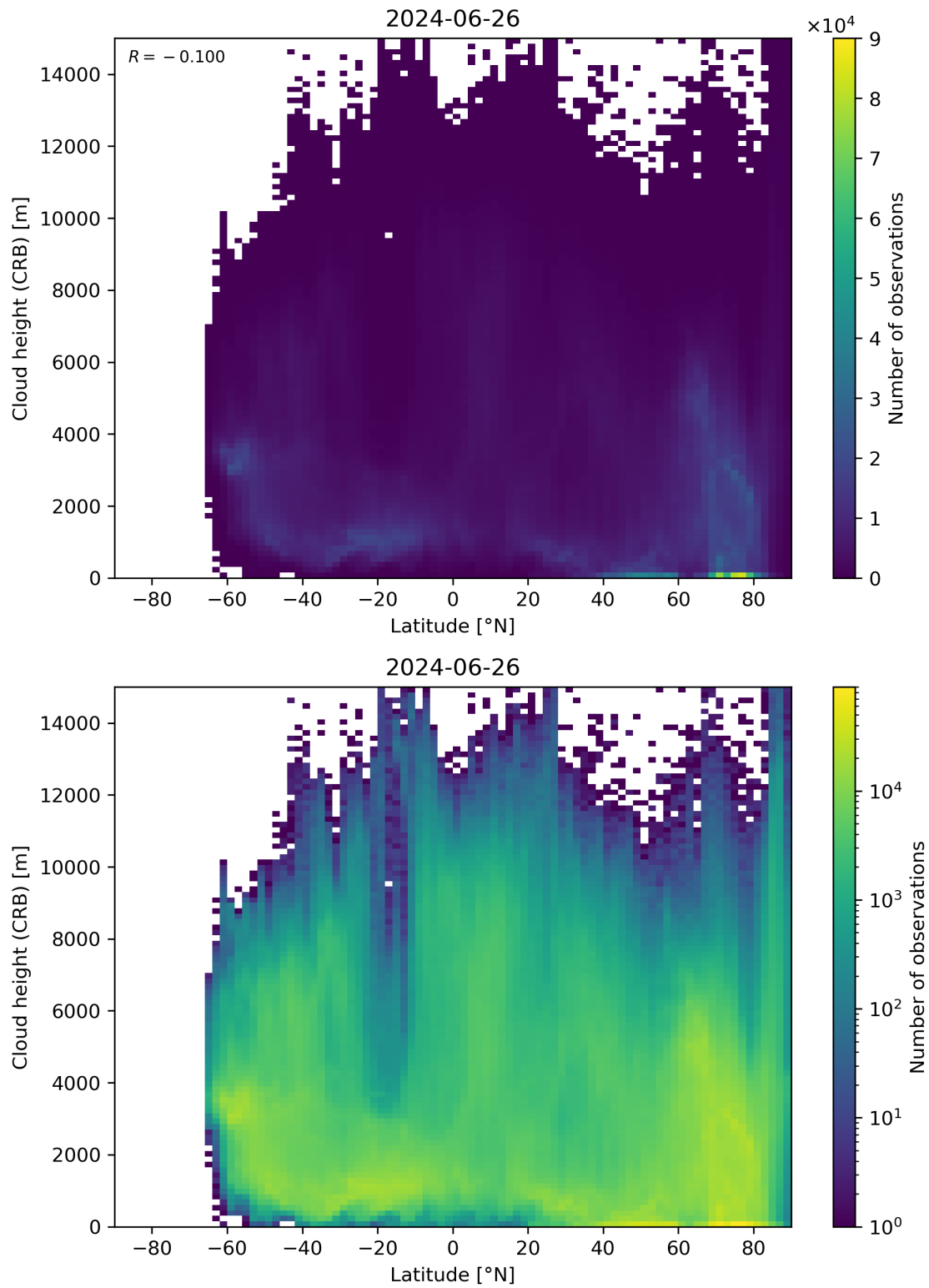
Figure 95: Scatter density plot of “Latitude” against “Cloud height (CRB)” for 2024-06-25 to 2024-06-27.
