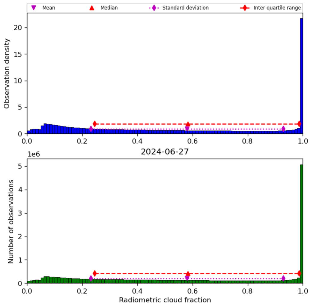
Figure 39: Histogram of “Radiometric cloud fraction” for 2024-06-26 to 2024-06-28
