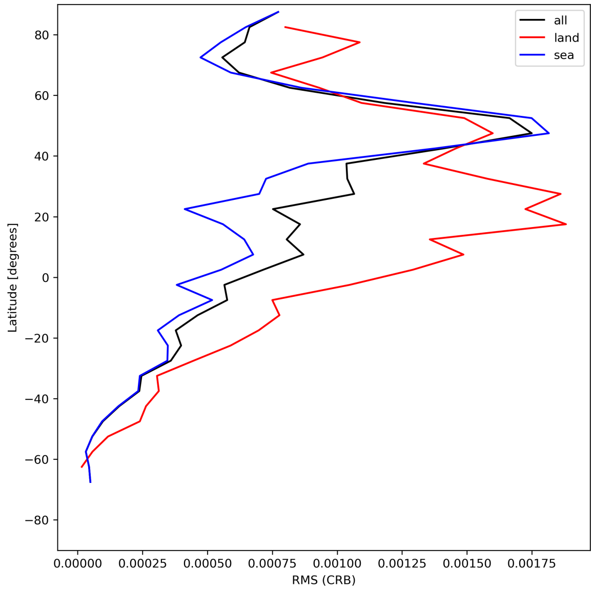
Figure 32: Zonal average of “RMS (CRB)” for 2024-06-26 to 2024-06-28.
