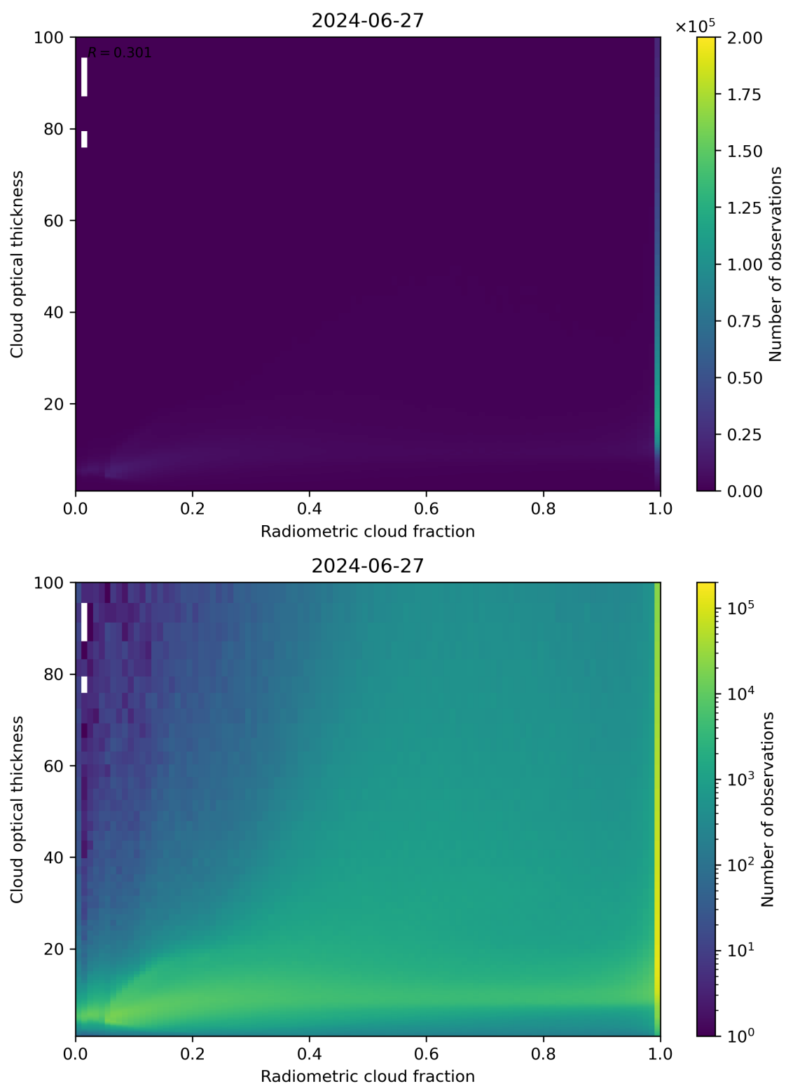
Figure 75: Scatter density plot of “Radiometric cloud fraction” against “Cloud optical thickness” for 2024-06-26 to 2024-06-28.
