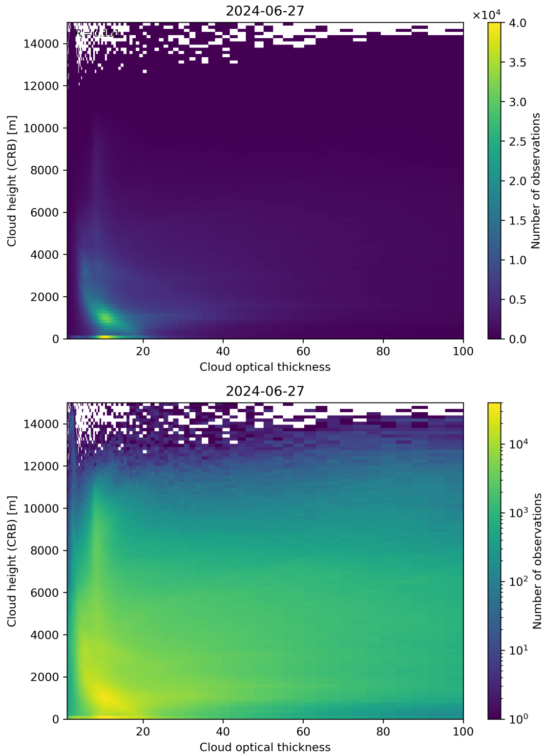
Figure 85: Scatter density plot of “Cloud optical thickness” against “Cloud height (CRB)” for 2024-06-26 to 2024-06-28.
