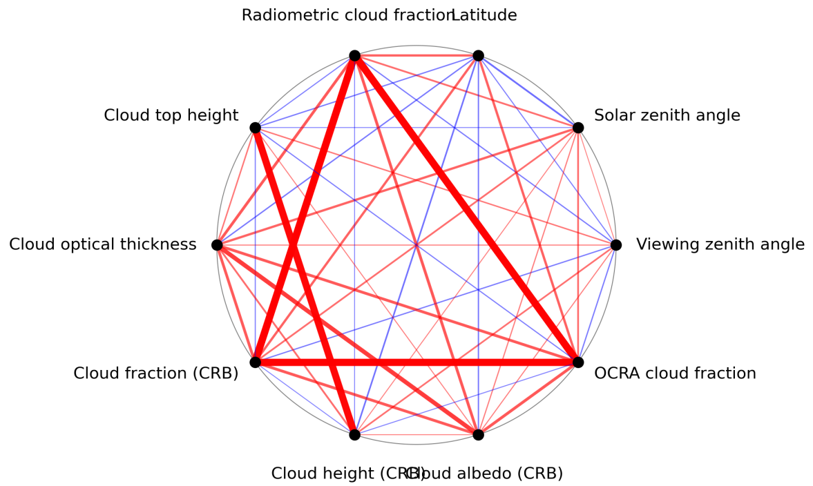
Figure 1: Map of correlation graph for 2024-06-26 to 2024-06-28.
