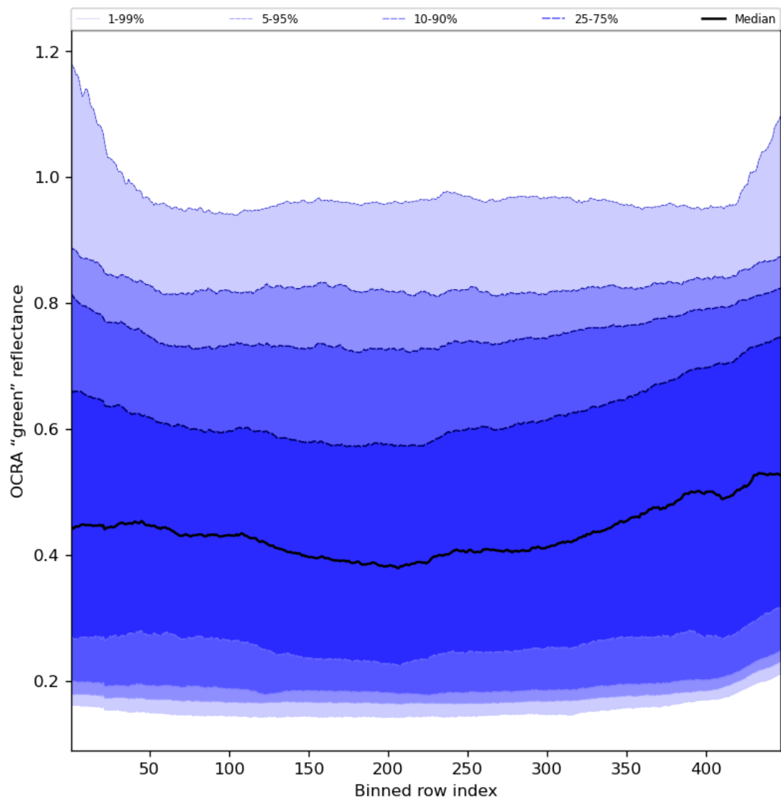
Figure 68: Along track statistics of “OCRA “green” reflectance” for 2024-06-26 to 2024-06-28
