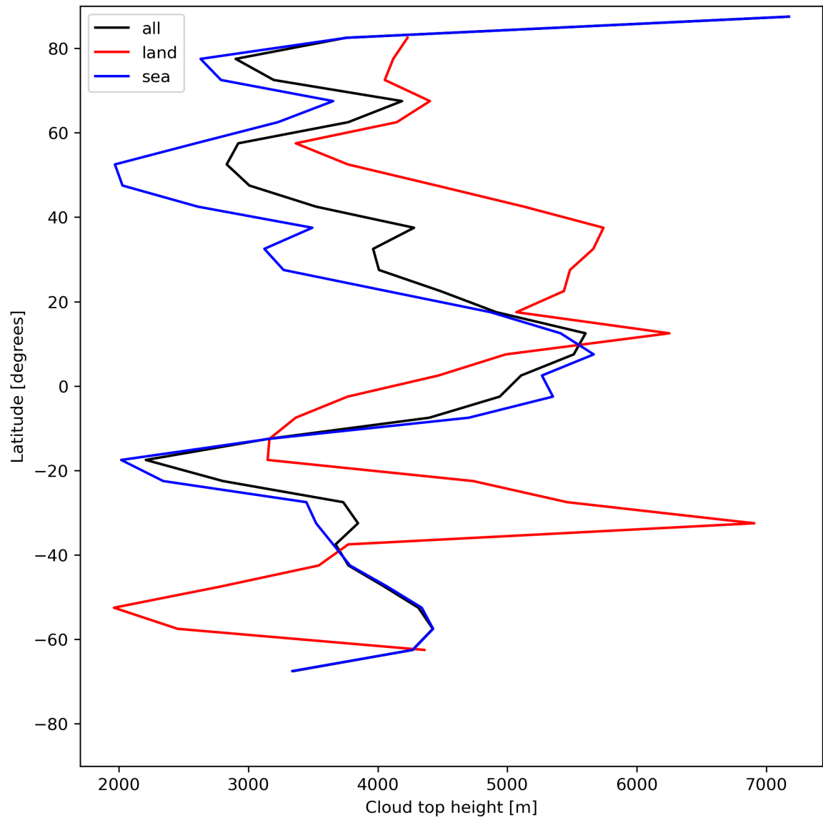
Figure 24: Zonal average of “Cloud top height” for 2024-06-26 to 2024-06-28.
