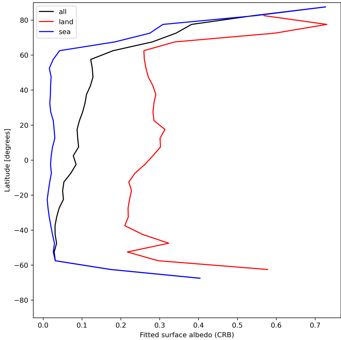
Figure 30: Zonal average of “Fitted surface albedo (CRB)” for 2024-06-26 to 2024-06-28.
