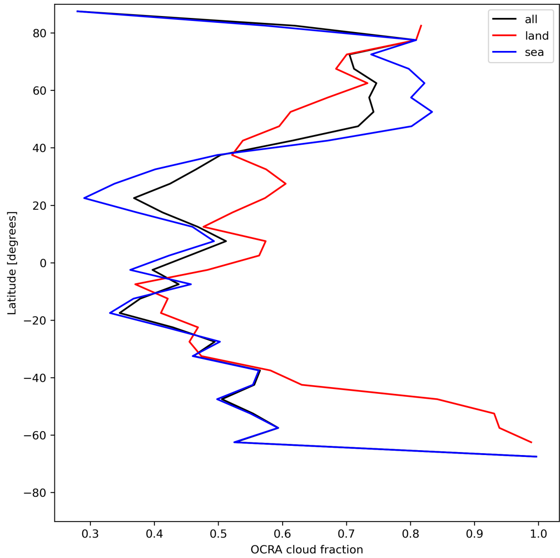
Figure 34: Zonal average of “OCRA cloud fraction” for 2024-06-26 to 2024-06-28.
