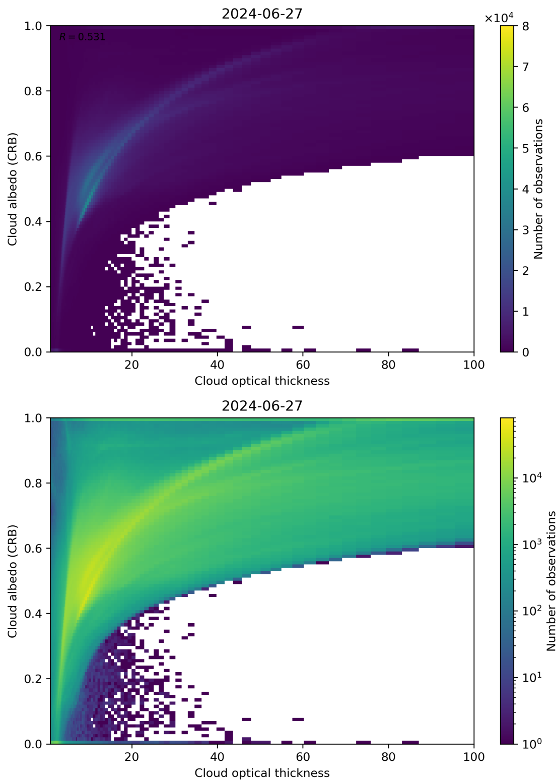
Figure 82: Scatter density plot of “Cloud optical thickness” against “Cloud albedo (CRB)” for 2024-06-26 to 2024-06-28.
