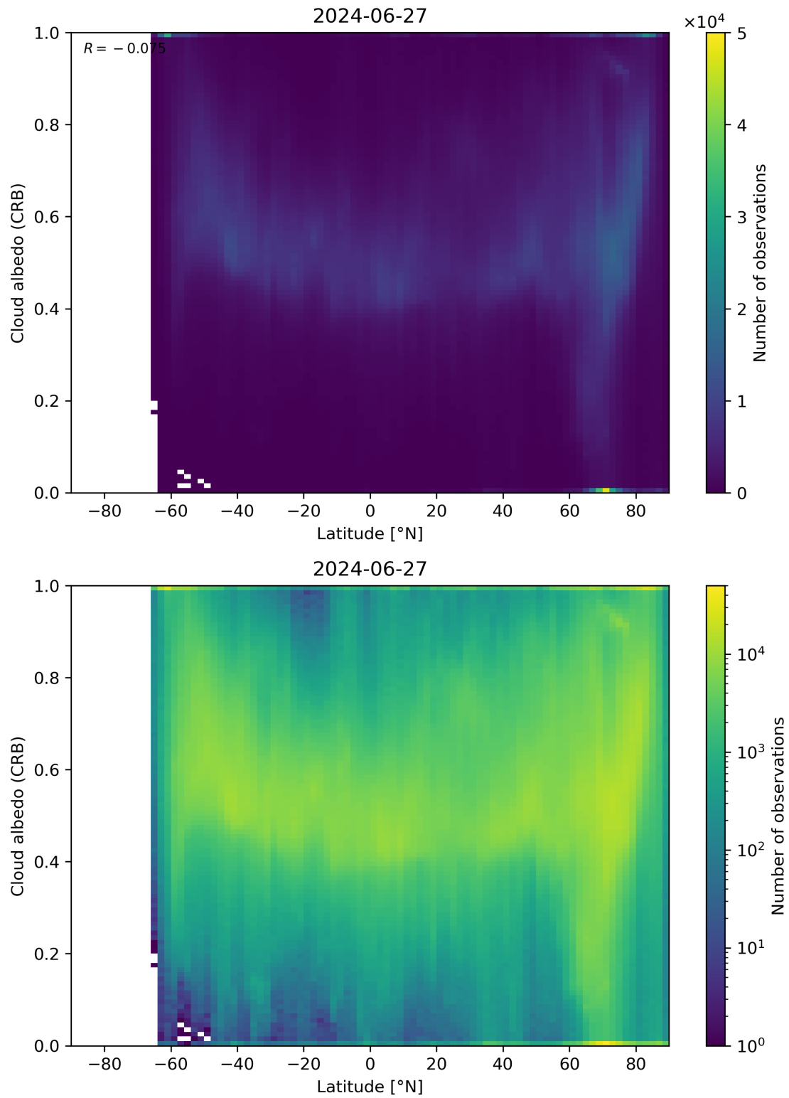
Figure 91: Scatter density plot of “Latitude” against “Cloud albedo (CRB)” for 2024-06-26 to 2024-06-28.
