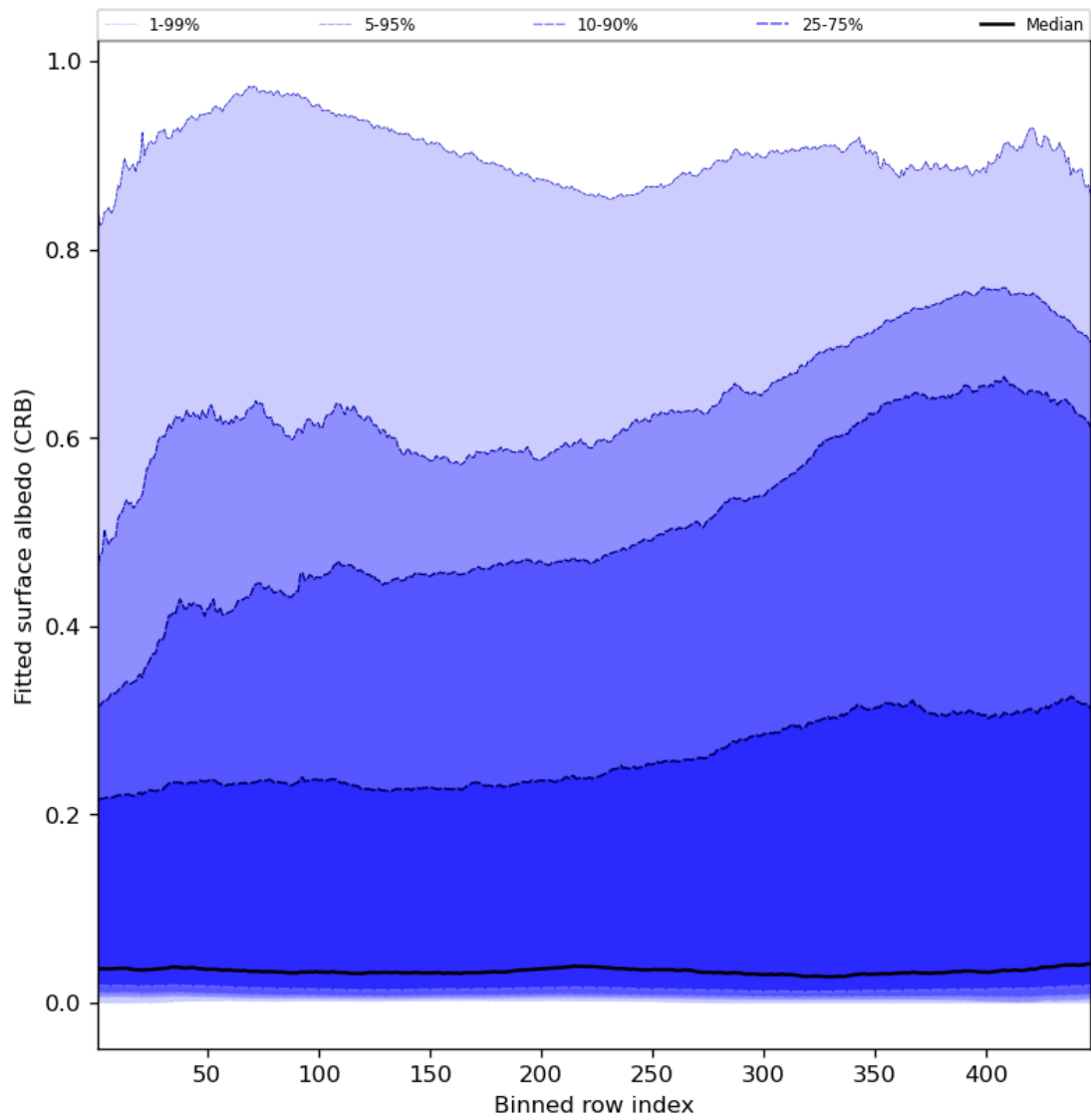
Figure 62: Along track statistics of “Fitted surface albedo (CRB)” for 2024-06-26 to 2024-06-28
