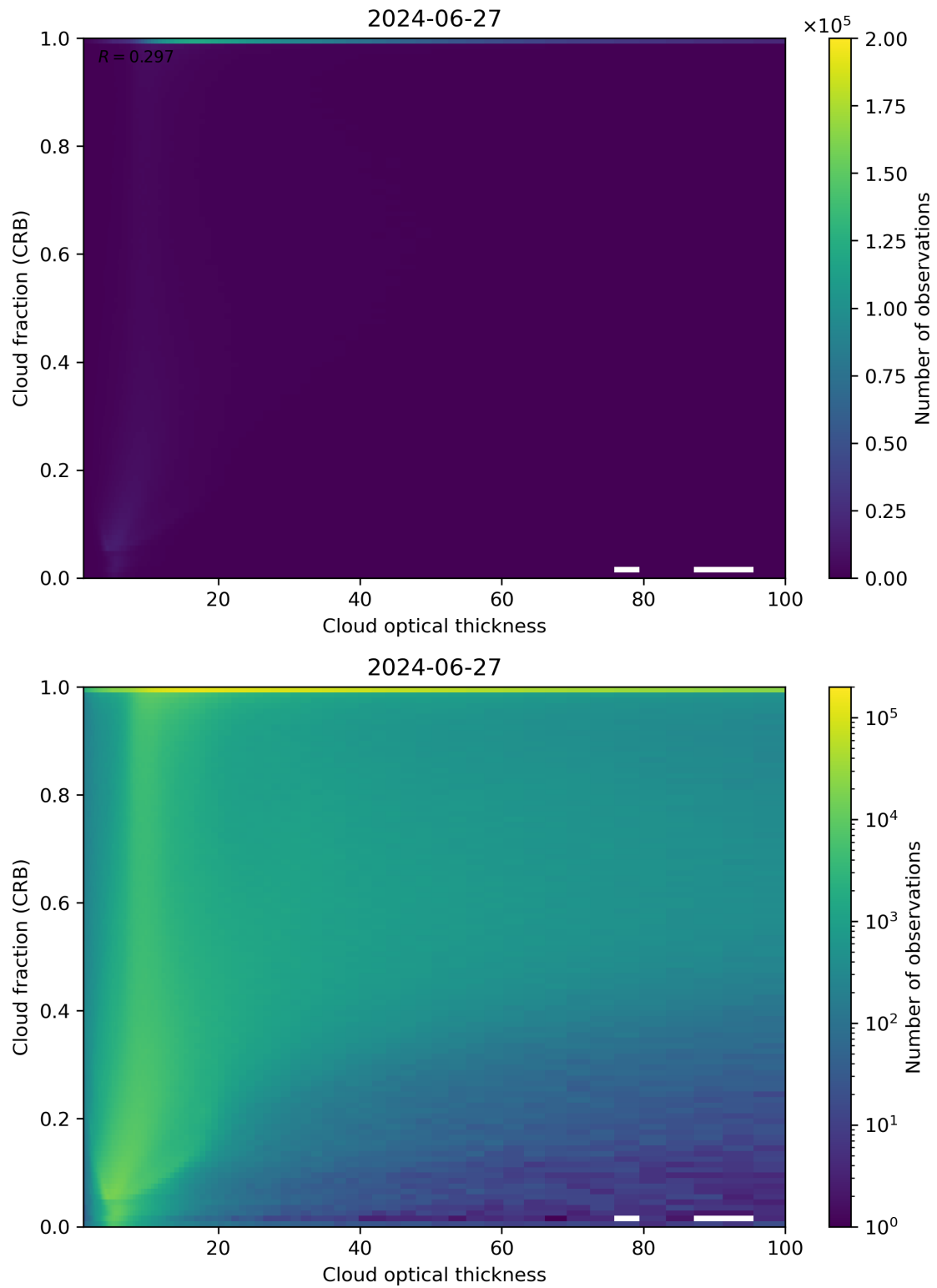
Figure 84: Scatter density plot of “Cloud optical thickness” against “Cloud fraction (CRB)” for 2024-06-26 to 2024-06-28.
