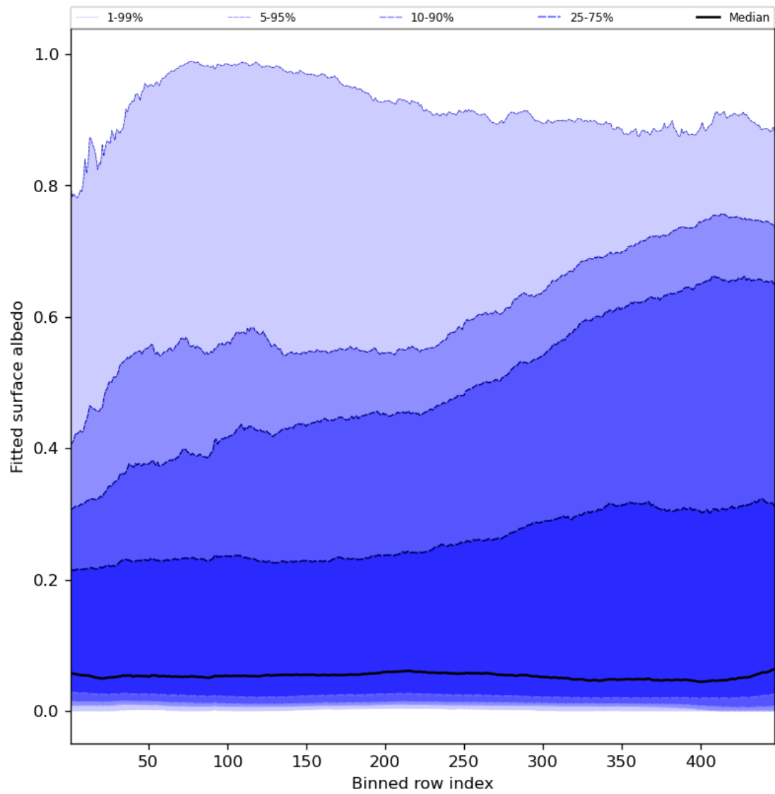
Figure 61: Along track statistics of “Fitted surface albedo” for 2024-06-26 to 2024-06-28
