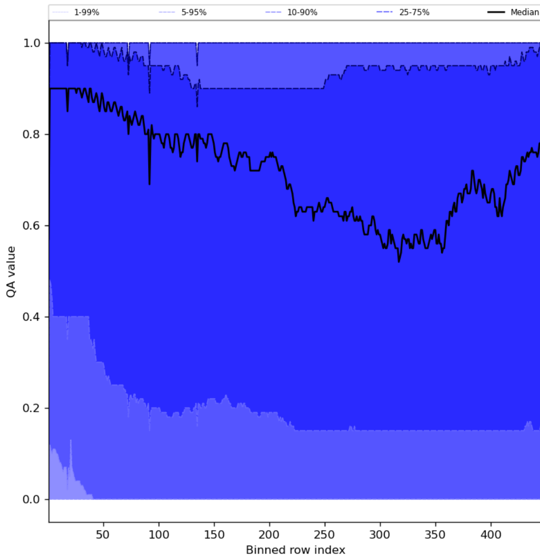
Figure 54: Along track statistics of “QA value” for 2024-06-26 to 2024-06-28
