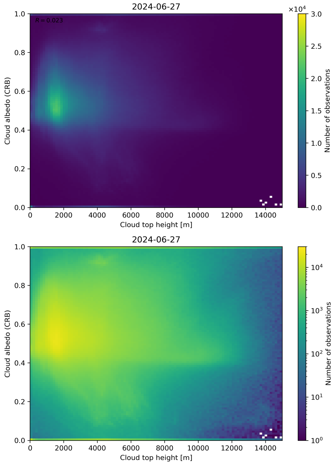
Figure 86: Scatter density plot of “Cloud top height” against “Cloud albedo (CRB)” for 2024-06-26 to 2024-06-28.
