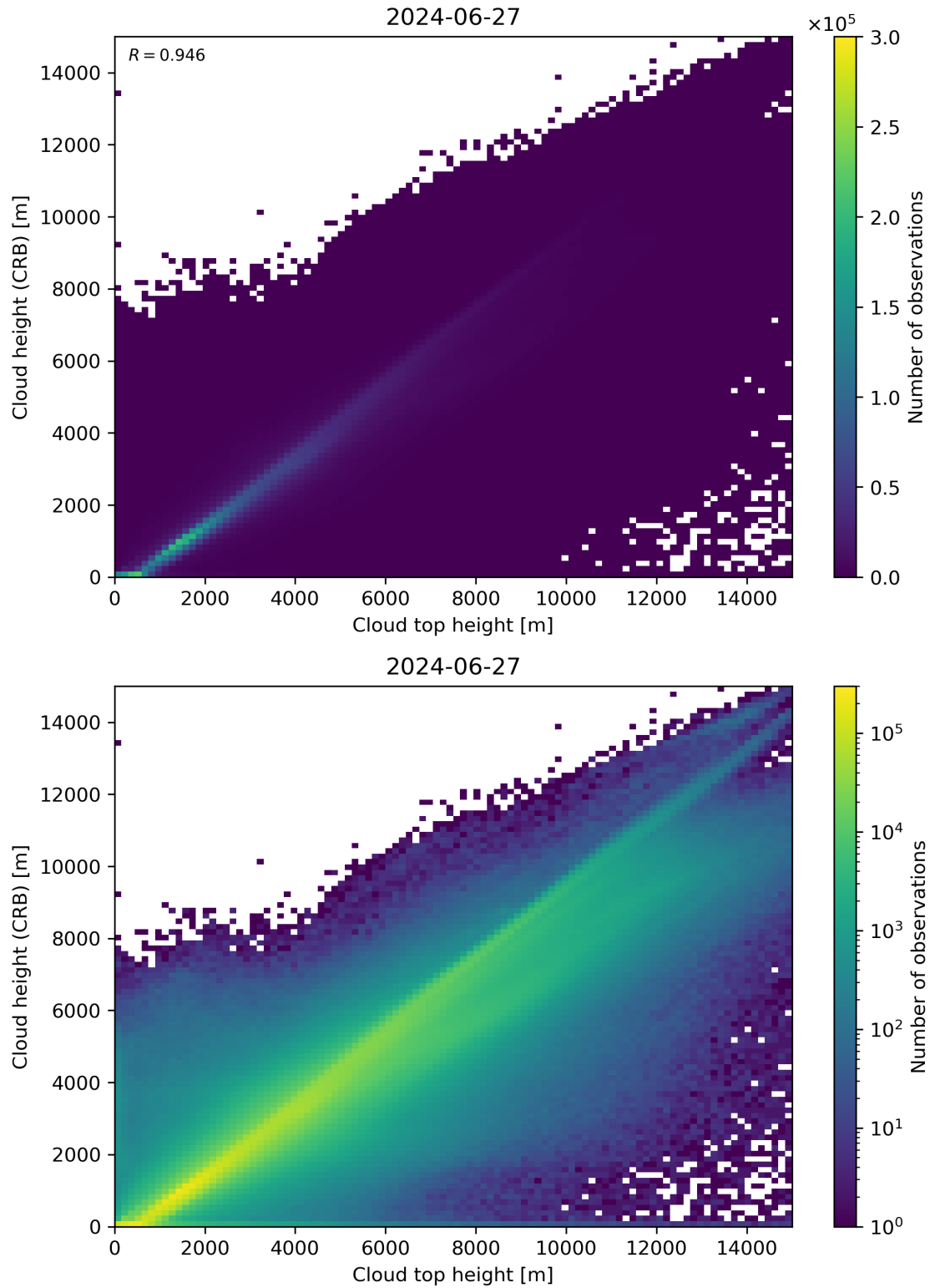
Figure 89: Scatter density plot of “Cloud top height” against “Cloud height (CRB)” for 2024-06-26 to 2024-06-28.
