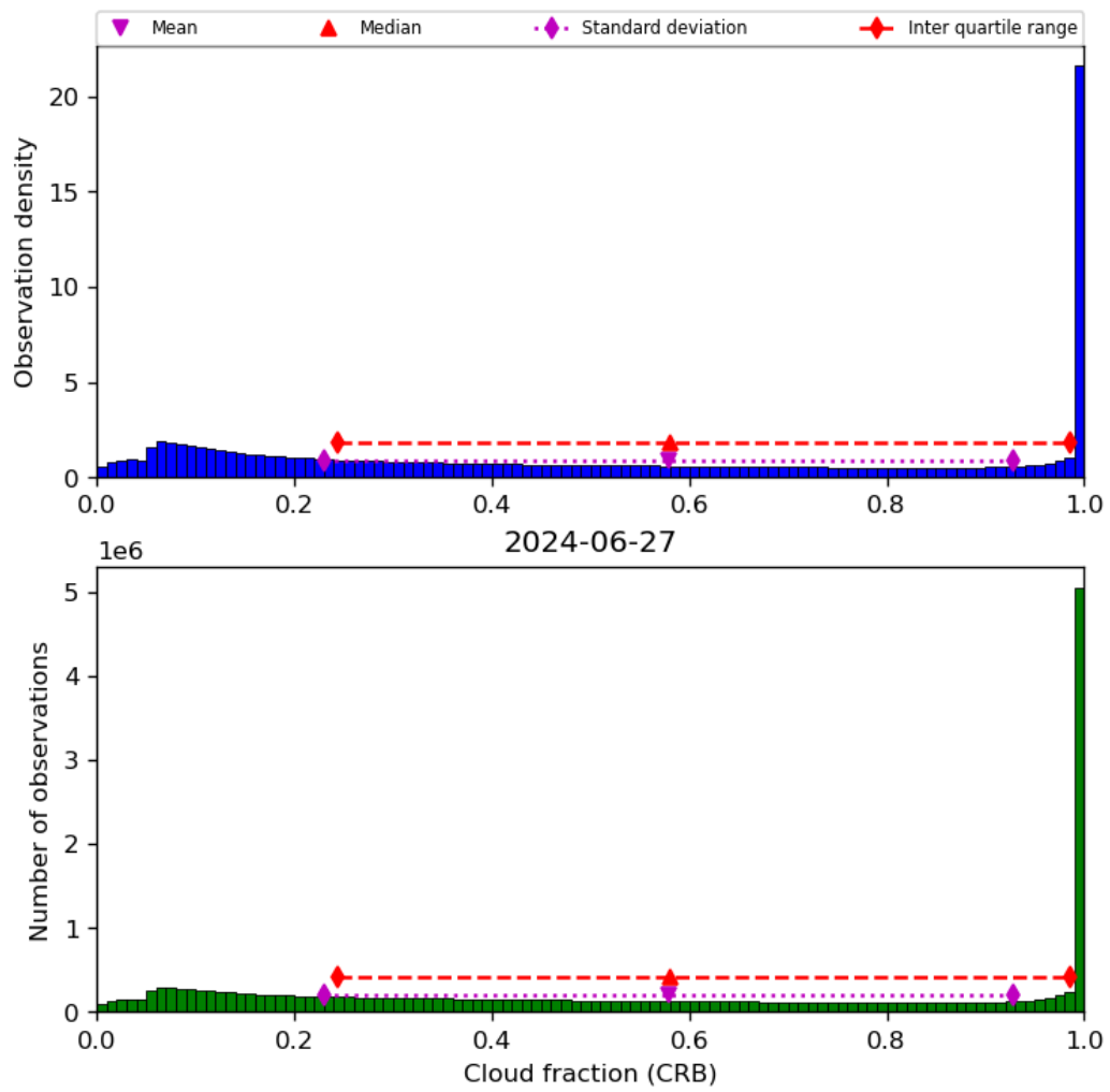
Figure 42: Histogram of “Cloud fraction (CRB)” for 2024-06-26 to 2024-06-28
