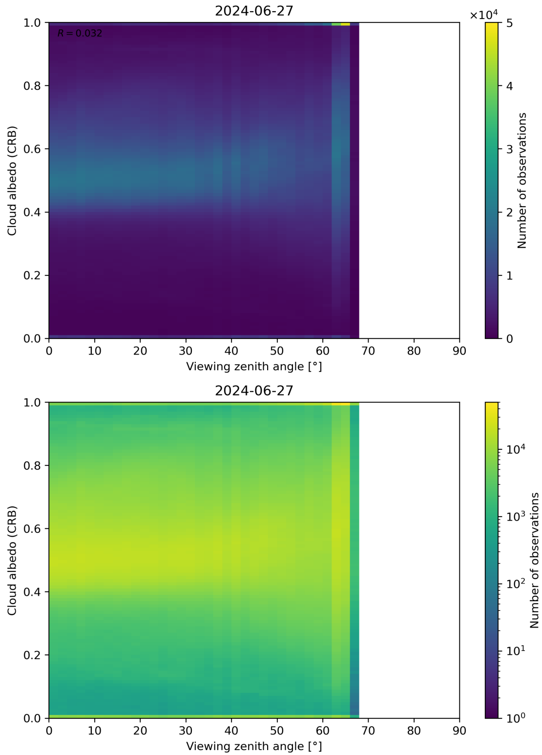
Figure 106: Scatter density plot of “Viewing zenith angle” against “Cloud albedo (CRB)” for 2024-06-26 to 2024-06-28.
