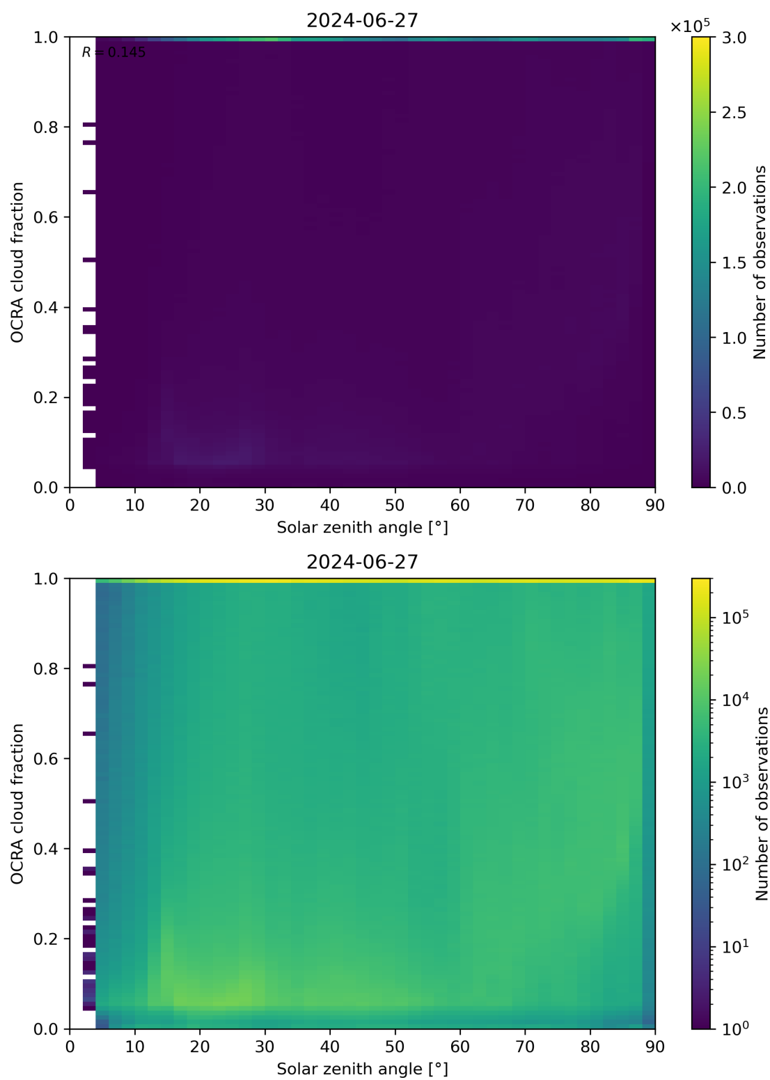
Figure 100: Scatter density plot of “Solar zenith angle” against “OCRA cloud fraction” for 2024-06-26 to 2024-06-28.
