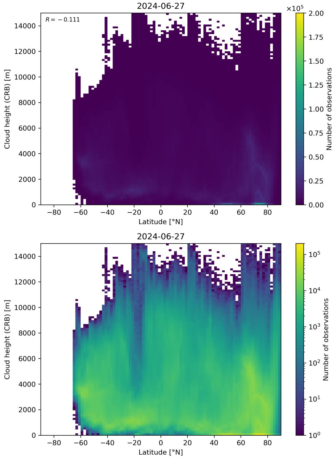
Figure 95: Scatter density plot of “Latitude” against “Cloud height (CRB)” for 2024-06-26 to 2024-06-28.
