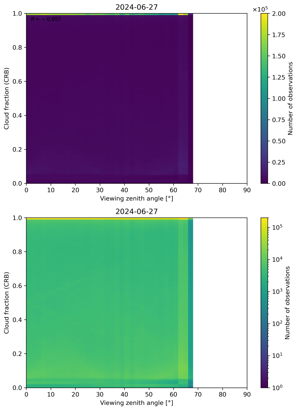
Figure 109: Scatter density plot of “Viewing zenith angle” against “Cloud fraction (CRB)” for 2024-06-26 to 2024-06-28.
