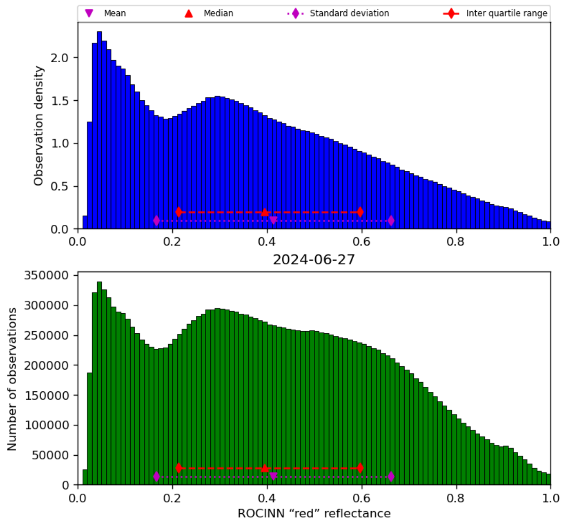
Figure 53: Histogram of “ROCINN “red” reflectance” for 2024-06-26 to 2024-06-28
