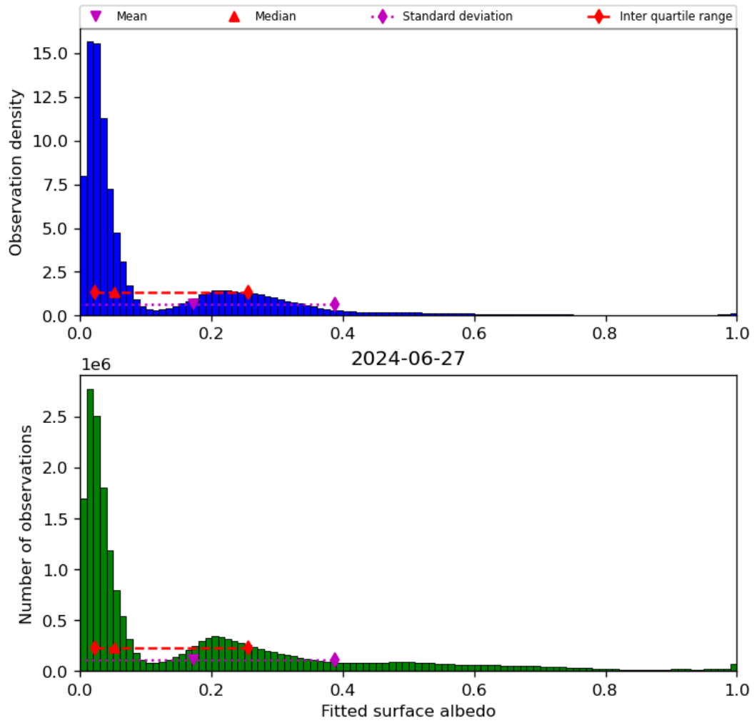
Figure 45: Histogram of “Fitted surface albedo” for 2024-06-26 to 2024-06-28
