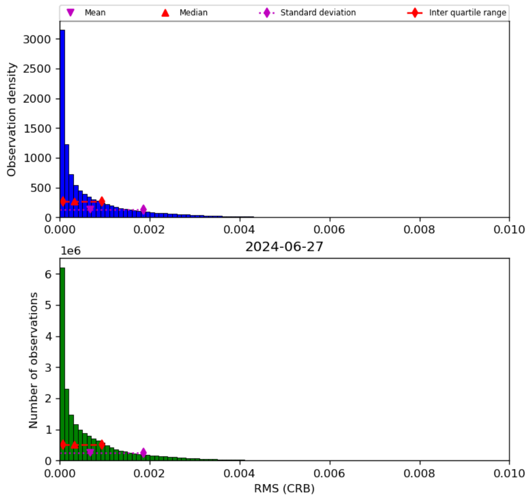
Figure 48: Histogram of “RMS (CRB)” for 2024-06-26 to 2024-06-28
