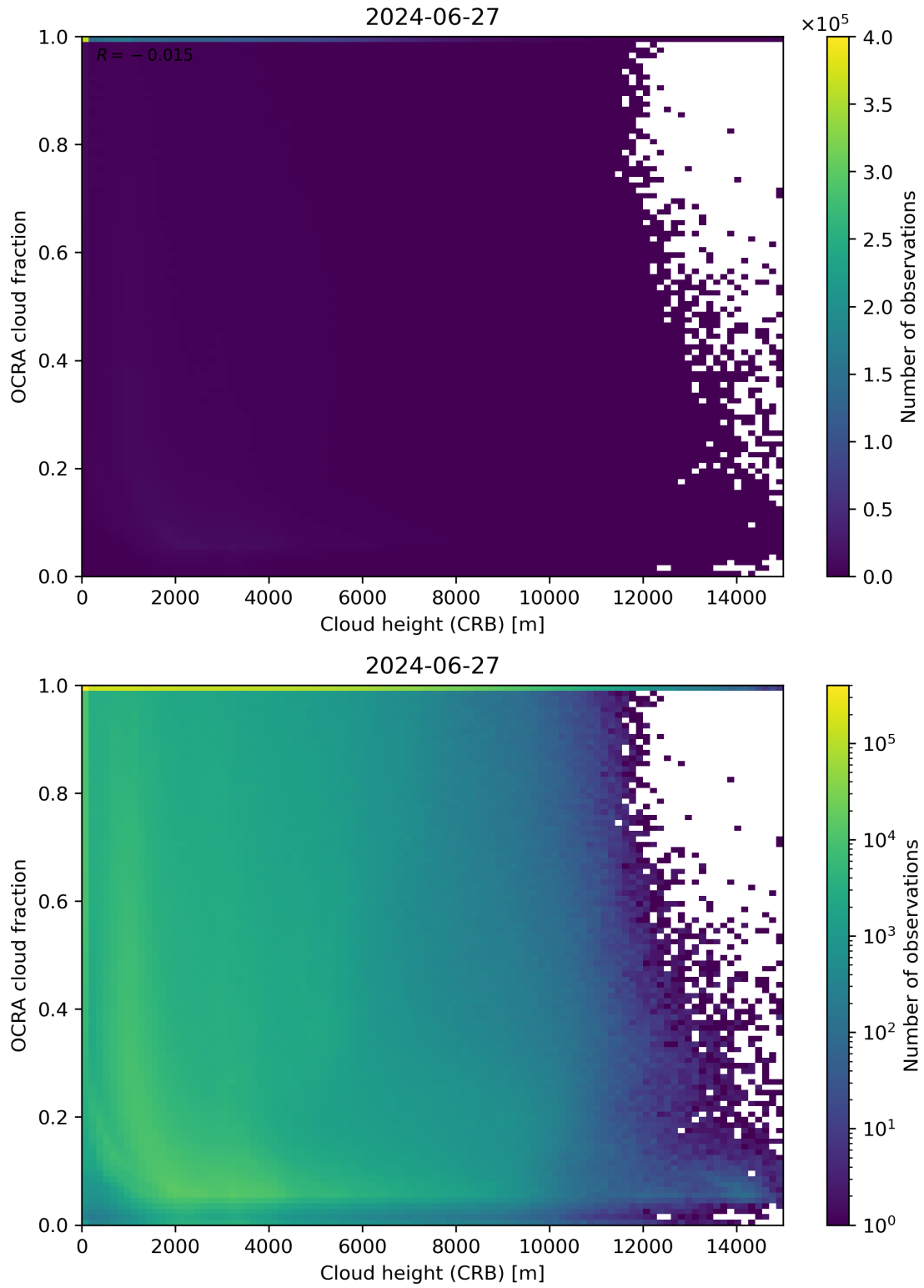
Figure 81: Scatter density plot of “Cloud height (CRB)” against “OCRA cloud fraction” for 2024-06-26 to 2024-06-28.
