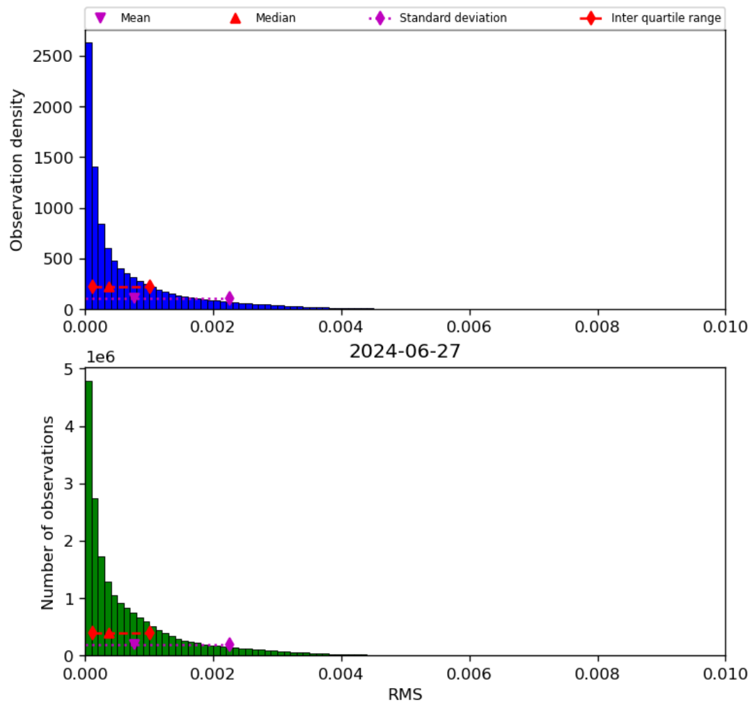
Figure 47: Histogram of “RMS” for 2024-06-26 to 2024-06-28
