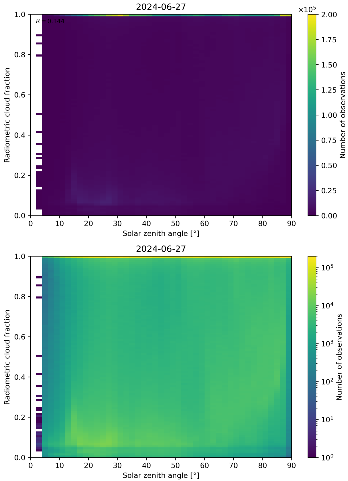
Figure 99: Scatter density plot of “Solar zenith angle” against “Radiometric cloud fraction” for 2024-06-26 to 2024-06-28.
