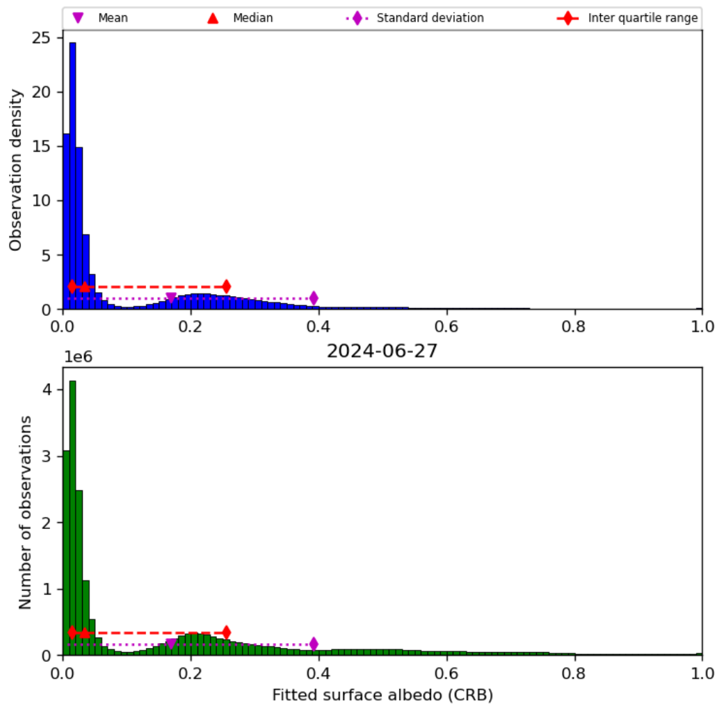
Figure 46: Histogram of “Fitted surface albedo (CRB)” for 2024-06-26 to 2024-06-28
