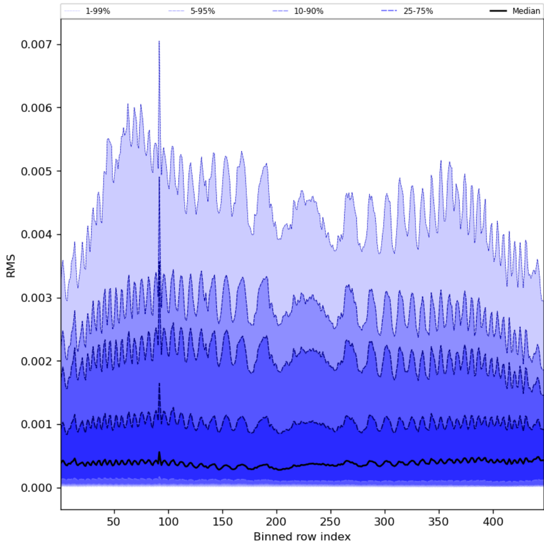
Figure 63: Along track statistics of “RMS” for 2024-06-26 to 2024-06-28
