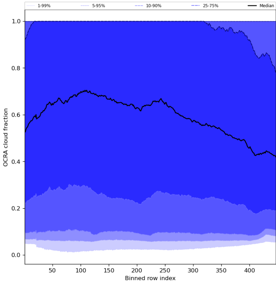
Figure 66: Along track statistics of “OCRA cloud fraction” for 2024-06-26 to 2024-06-28
