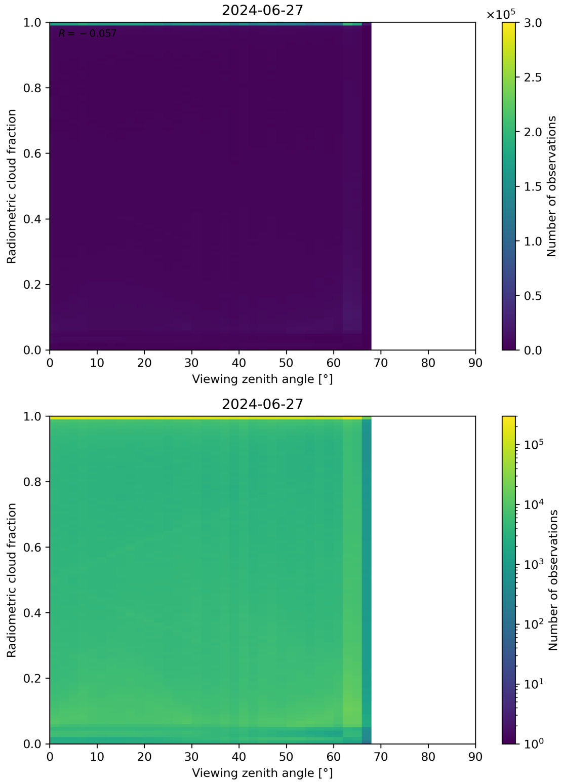
Figure 107: Scatter density plot of “Viewing zenith angle” against “Radiometric cloud fraction” for 2024-06-26 to 2024-06-28.
