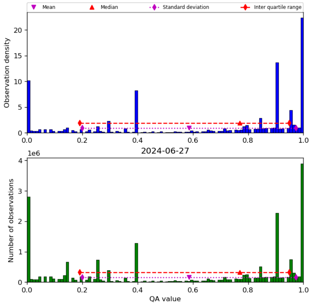
Figure 38: Histogram of “QA value” for 2024-06-26 to 2024-06-28
