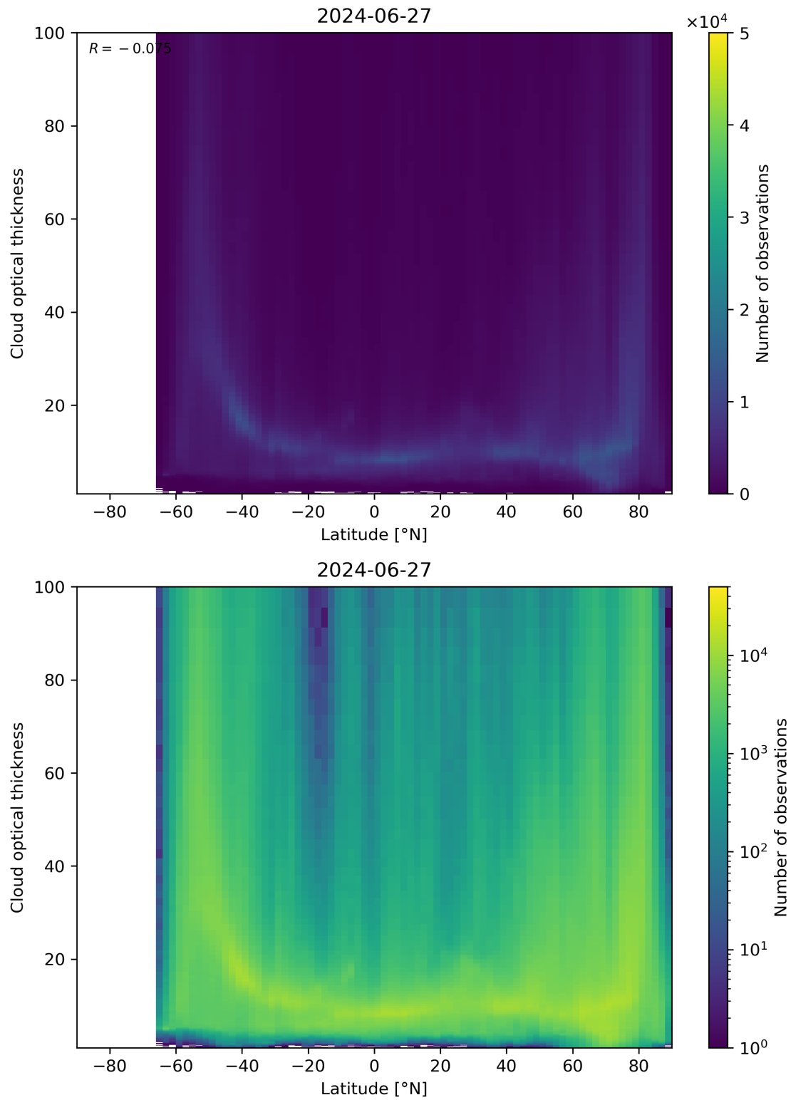
Figure 96: Scatter density plot of “Latitude” against “Cloud optical thickness” for 2024-06-26 to 2024-06-28.
