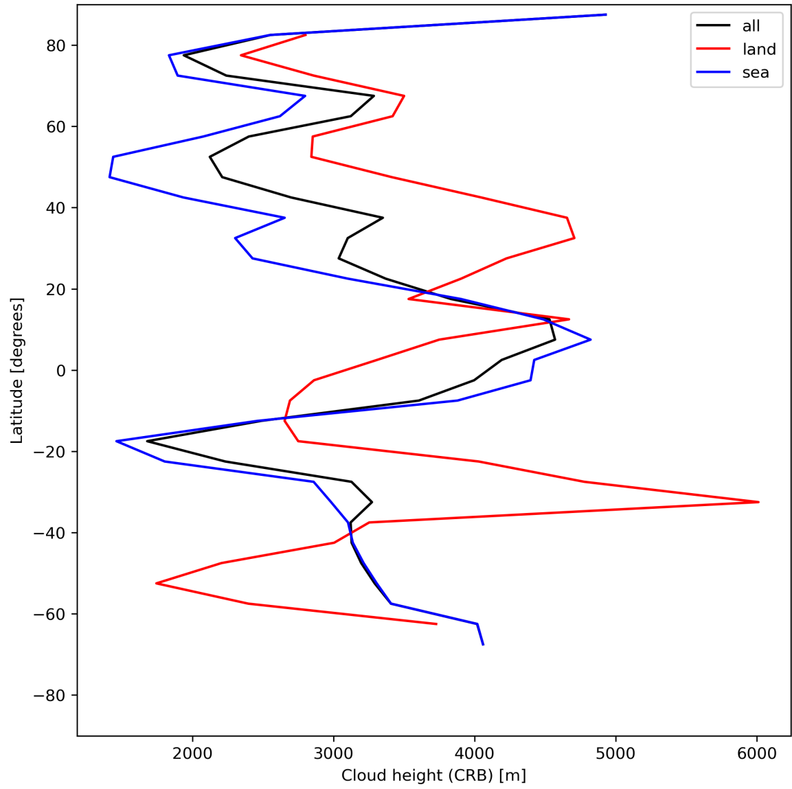
Figure 27: Zonal average of “Cloud height (CRB)” for 2024-06-26 to 2024-06-28.
