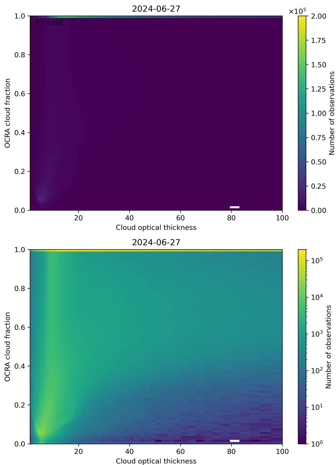
Figure 83: Scatter density plot of “Cloud optical thickness” against “OCRA cloud fraction” for 2024-06-26 to 2024-06-28.
