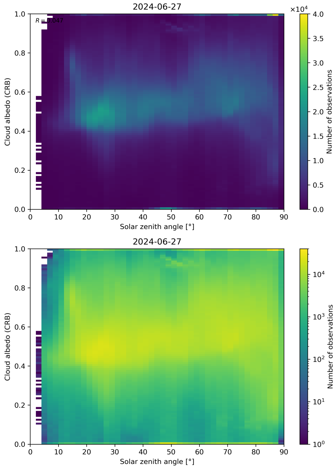
Figure 98: Scatter density plot of “Solar zenith angle” against “Cloud albedo (CRB)” for 2024-06-26 to 2024-06-28.
