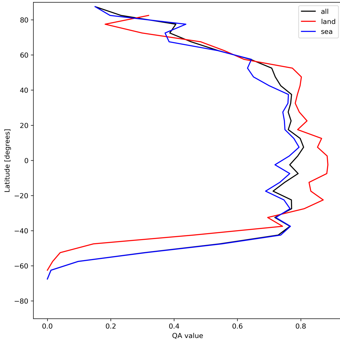
Figure 22: Zonal average of “QA value” for 2024-06-26 to 2024-06-28.
