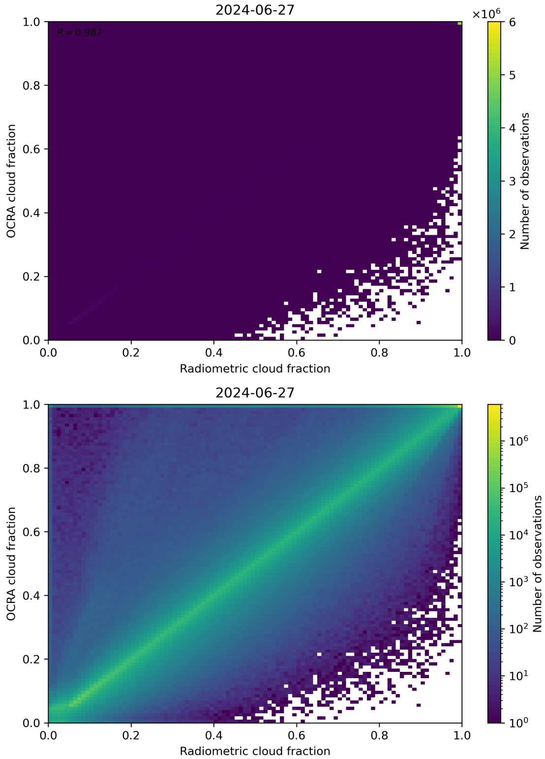
Figure 72: Scatter density plot of “Radiometric cloud fraction” against “OCRA cloud fraction” for 2024-06-26 to 2024-06-28.
