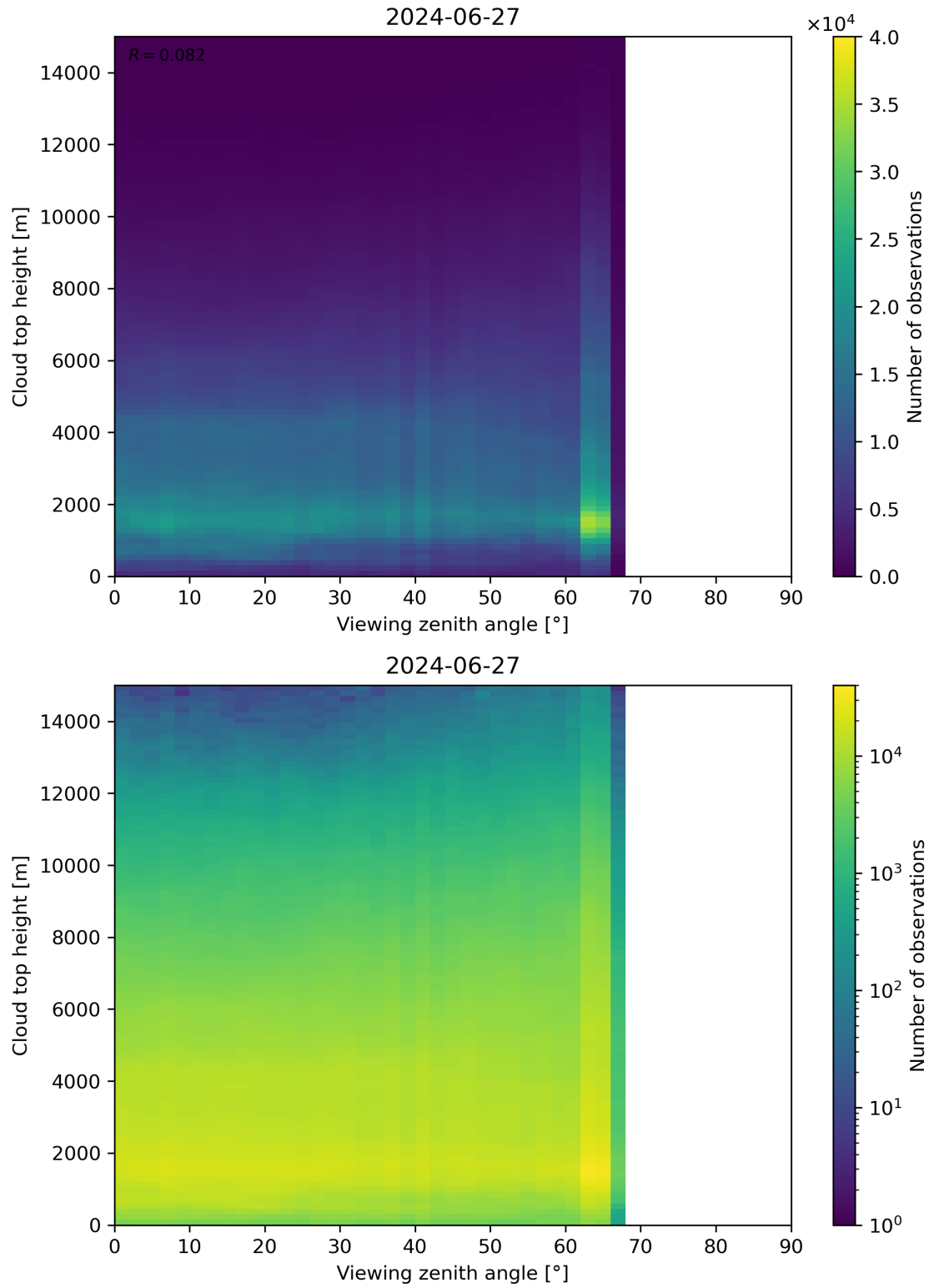
Figure 112: Scatter density plot of “Viewing zenith angle” against “Cloud top height” for 2024-06-26 to 2024-06-28.
