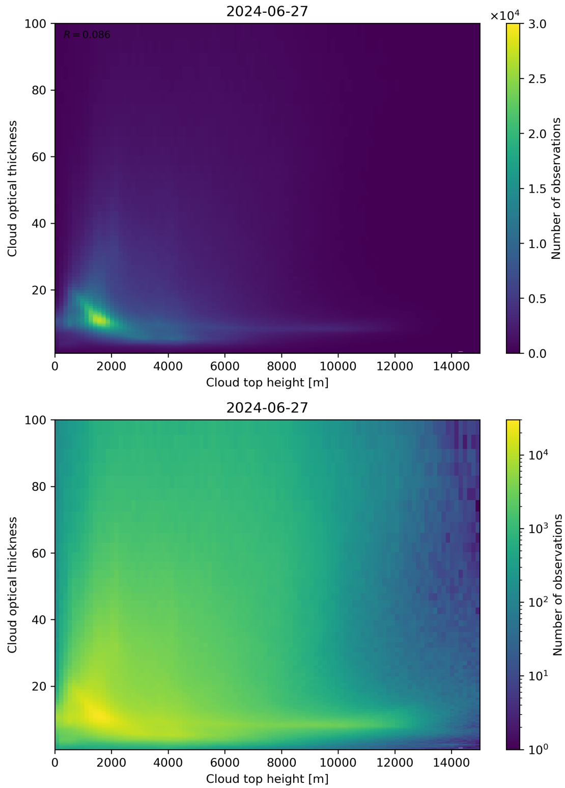
Figure 90: Scatter density plot of “Cloud top height” against “Cloud optical thickness” for 2024-06-26 to 2024-06-28.
