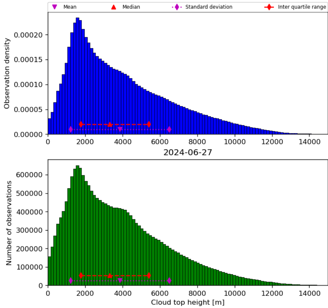
Figure 40: Histogram of “Cloud top height” for 2024-06-26 to 2024-06-28
