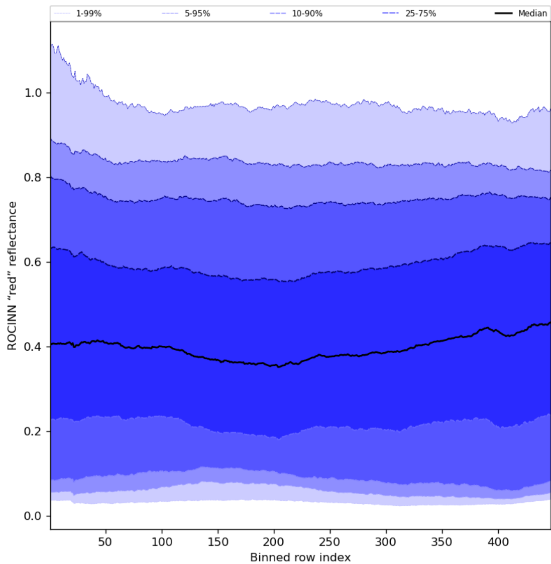
Figure 69: Along track statistics of “ROCINN “red” reflectance” for 2024-06-26 to 2024-06-28
