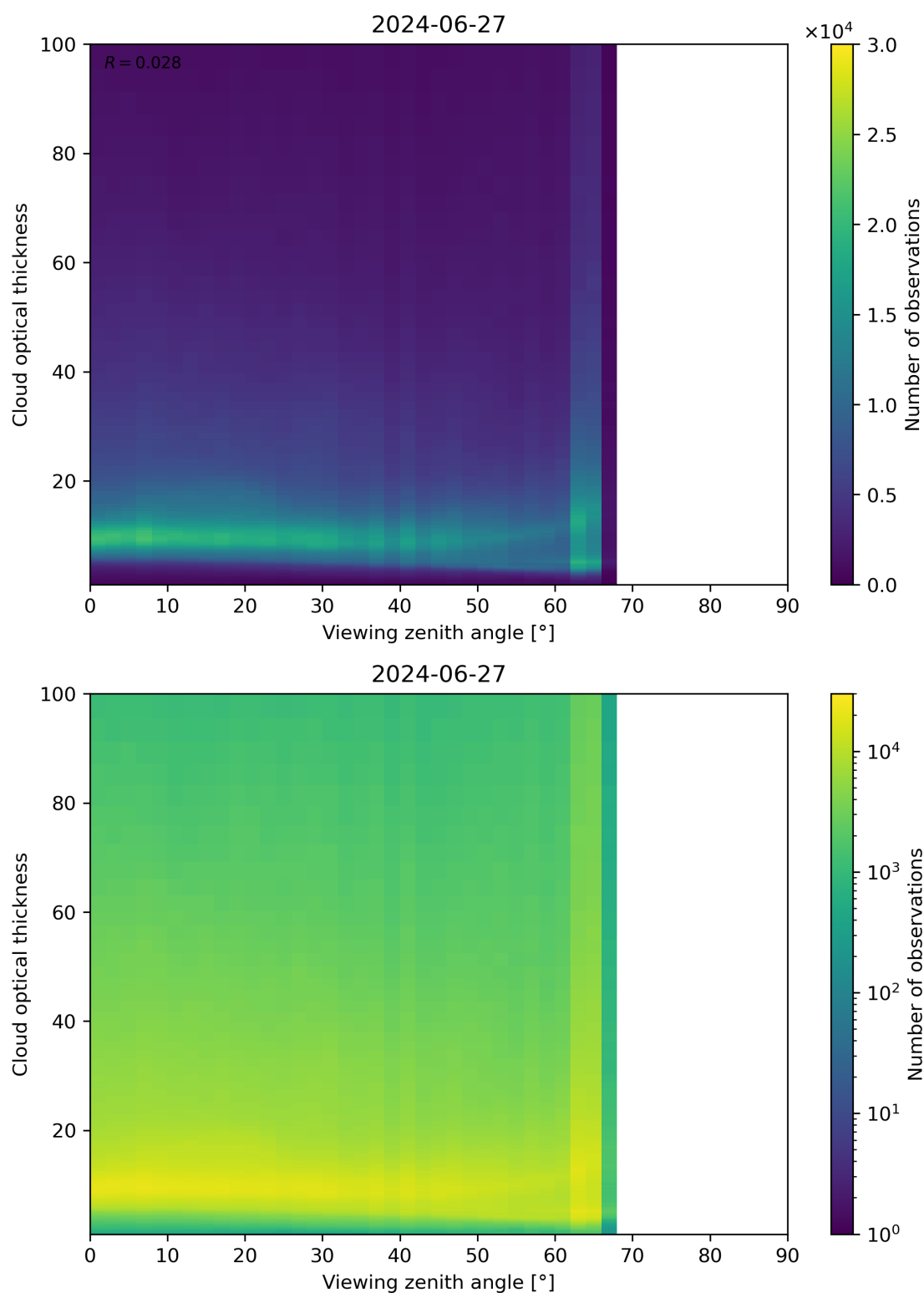
Figure 111: Scatter density plot of “Viewing zenith angle” against “Cloud optical thickness” for 2024-06-26 to 2024-06-28.
