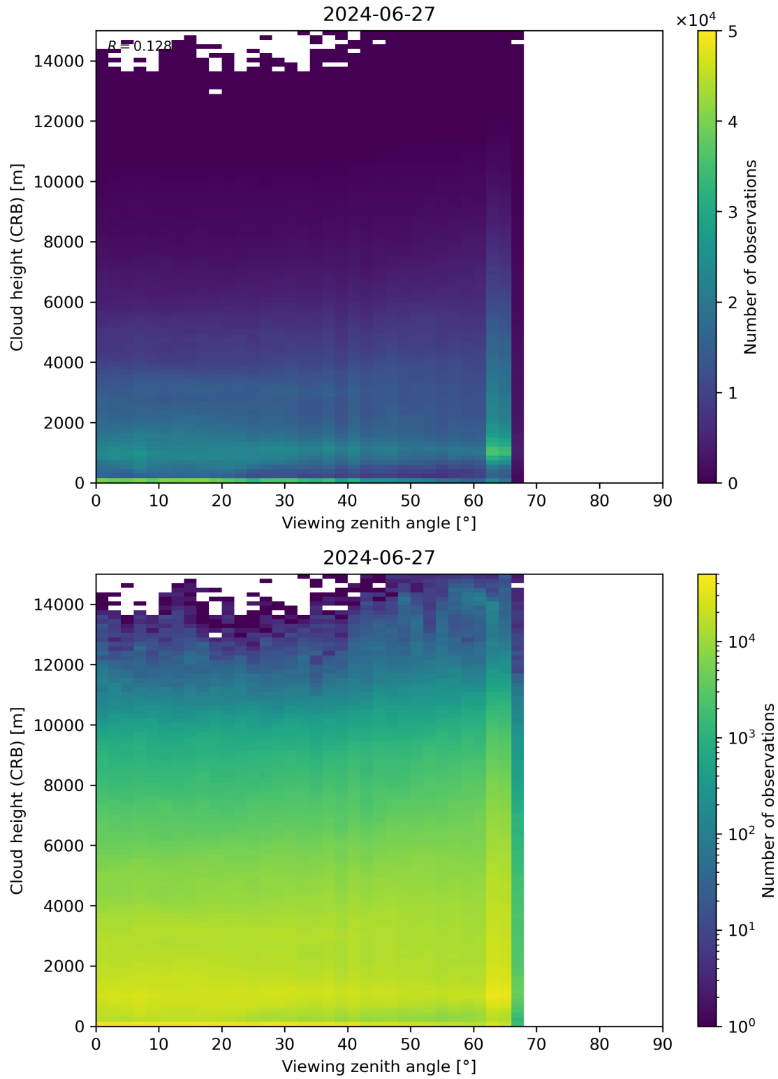
Figure 110: Scatter density plot of “Viewing zenith angle” against “Cloud height (CRB)” for 2024-06-26 to 2024-06-28.
