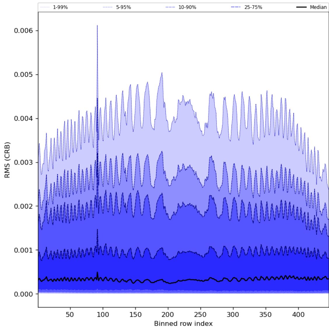
Figure 64: Along track statistics of “RMS (CRB)” for 2024-06-26 to 2024-06-28
