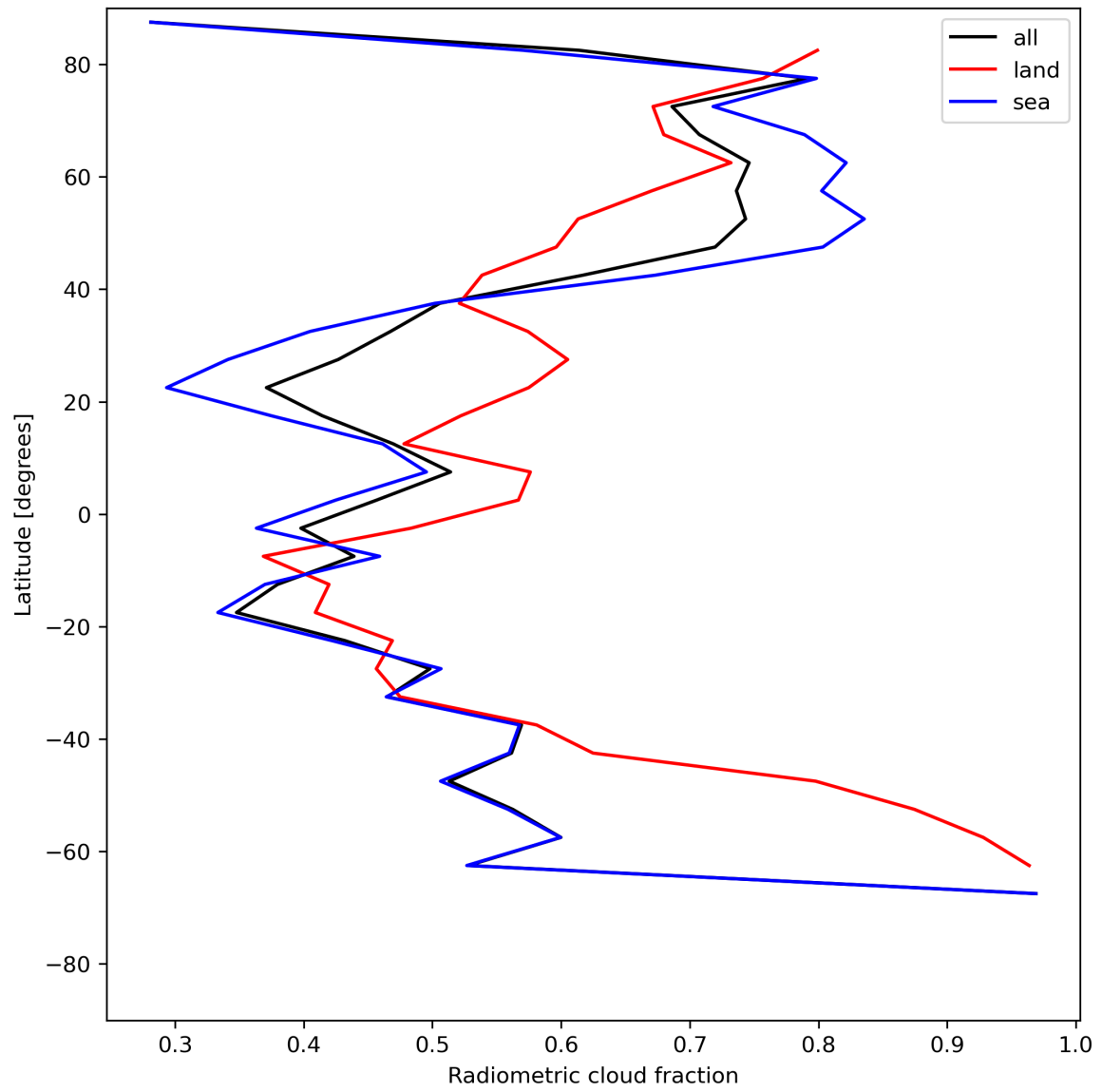
Figure 23: Zonal average of “Radiometric cloud fraction” for 2024-06-26 to 2024-06-28.
