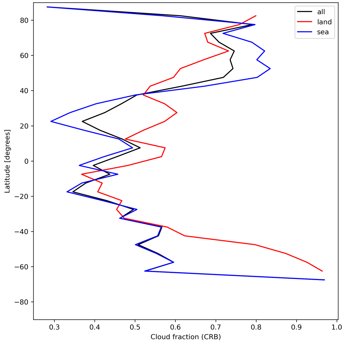
Figure 26: Zonal average of “Cloud fraction (CRB)” for 2024-06-26 to 2024-06-28.
