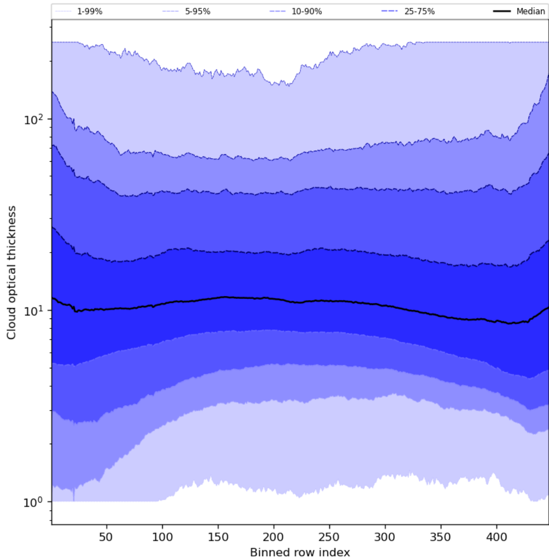
Figure 57: Along track statistics of “Cloud optical thickness” for 2024-06-26 to 2024-06-28
