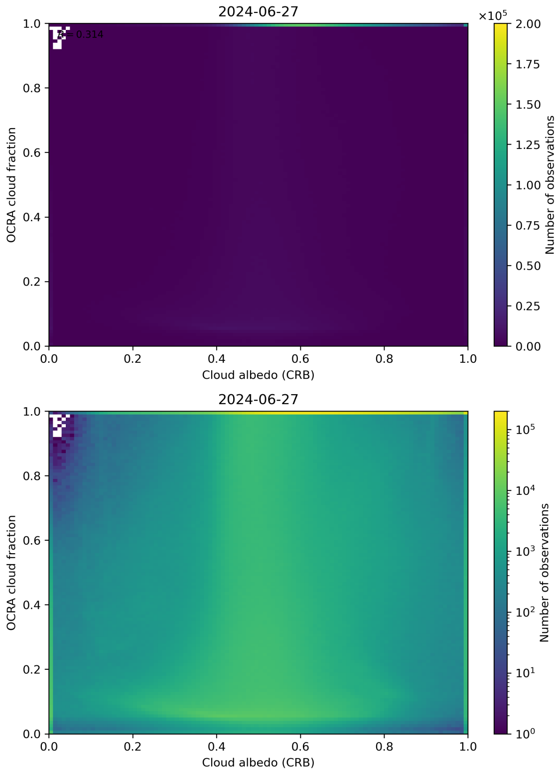
Figure 70: Scatter density plot of “Cloud albedo (CRB)” against “OCRA cloud fraction” for 2024-06-26 to 2024-06-28.
