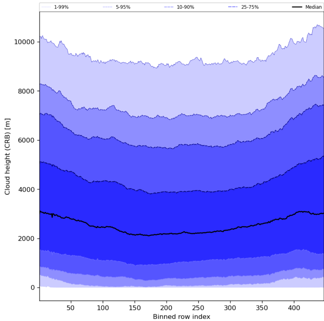
Figure 59: Along track statistics of “Cloud height (CRB)” for 2024-06-26 to 2024-06-28
