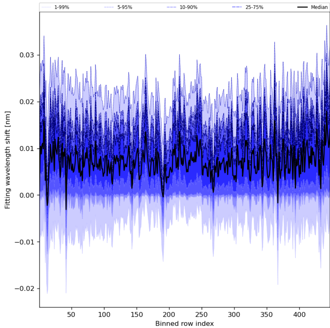
Figure 65: Along track statistics of “Fitting wavelength shift” for 2024-06-26 to 2024-06-28
