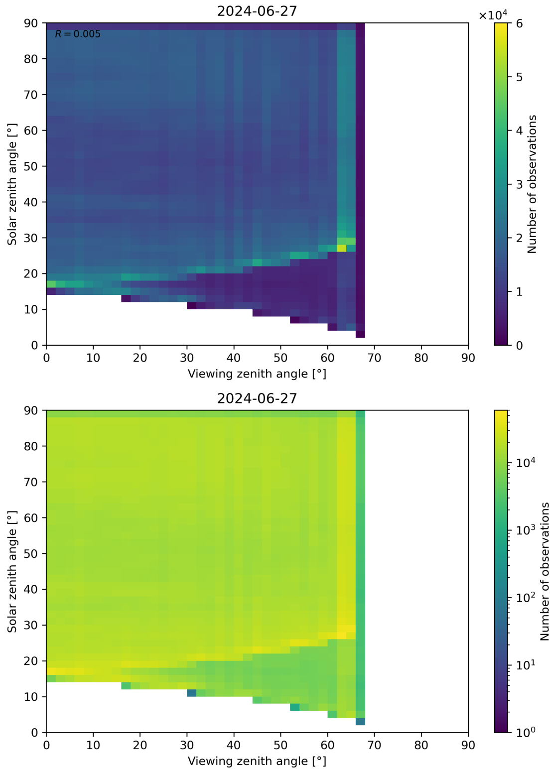
Figure 114: Scatter density plot of “Viewing zenith angle” against “Solar zenith angle” for 2024-06-26 to 2024-06-28.
