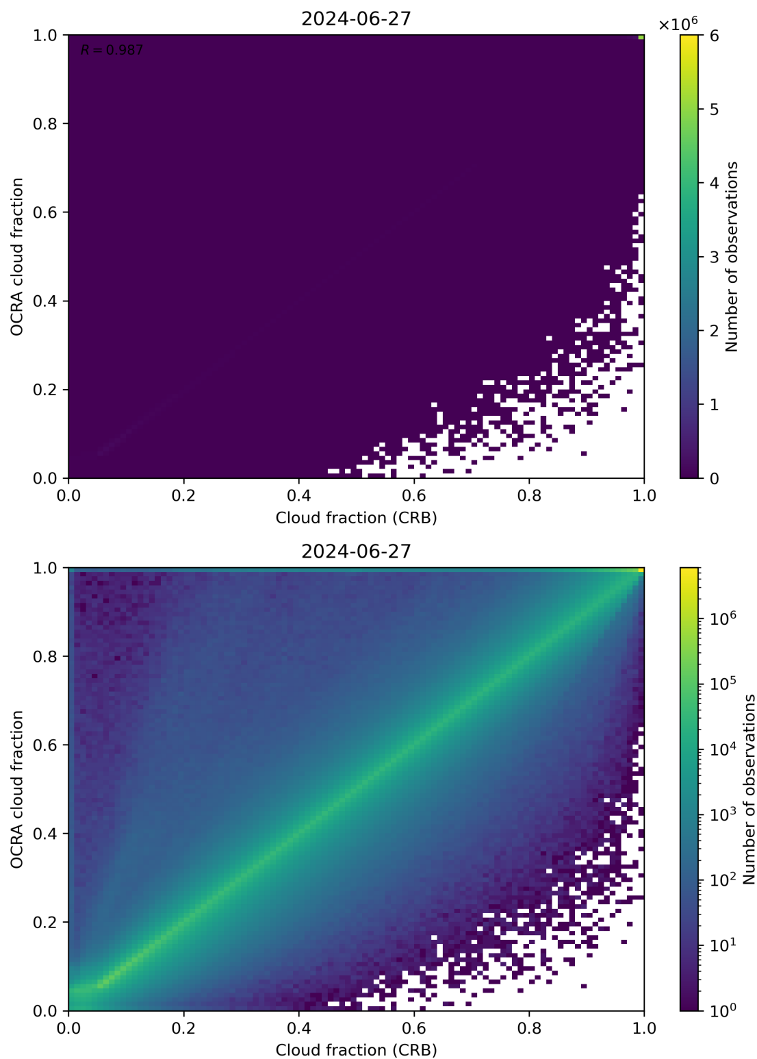
Figure 78: Scatter density plot of “Cloud fraction (CRB)” against “OCRA cloud fraction” for 2024-06-26 to 2024-06-28.
