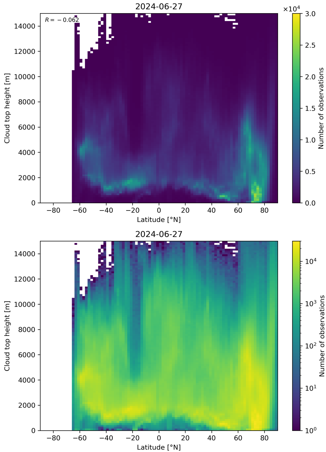
Figure 97: Scatter density plot of “Latitude” against “Cloud top height” for 2024-06-26 to 2024-06-28.
