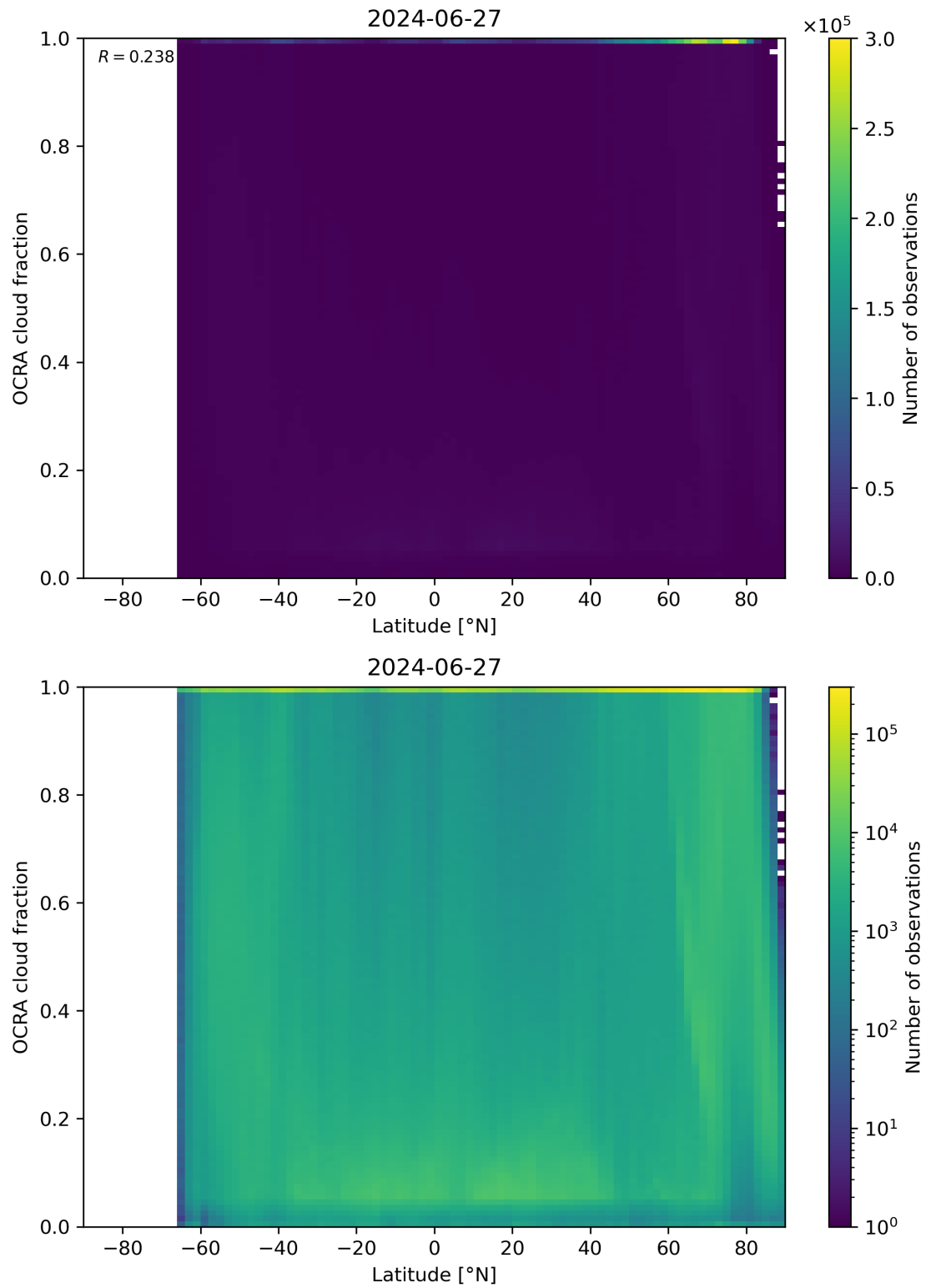
Figure 93: Scatter density plot of “Latitude” against “OCRA cloud fraction” for 2024-06-26 to 2024-06-28.
