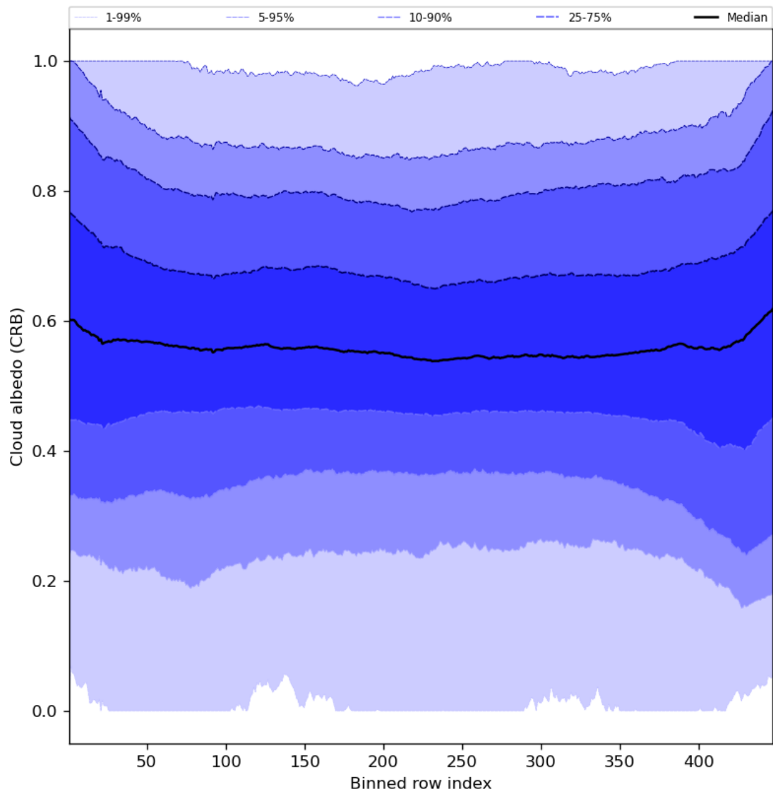
Figure 60: Along track statistics of “Cloud albedo (CRB)” for 2024-06-26 to 2024-06-28
