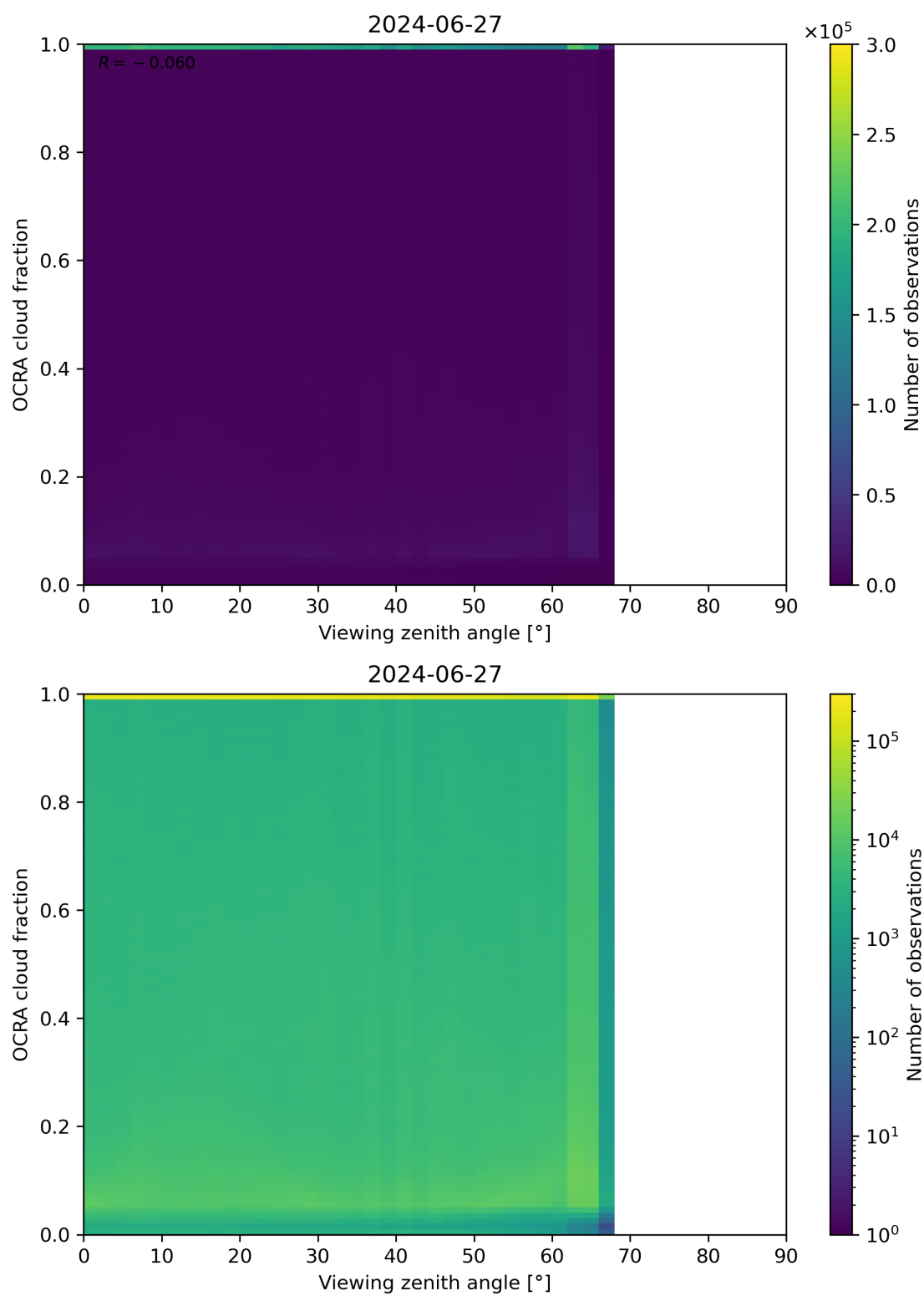
Figure 108: Scatter density plot of “Viewing zenith angle” against “OCRA cloud fraction” for 2024-06-26 to 2024-06-28.
