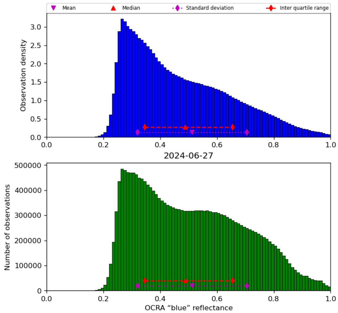
Figure 51: Histogram of “OCRA “blue” reflectance” for 2024-06-26 to 2024-06-28
