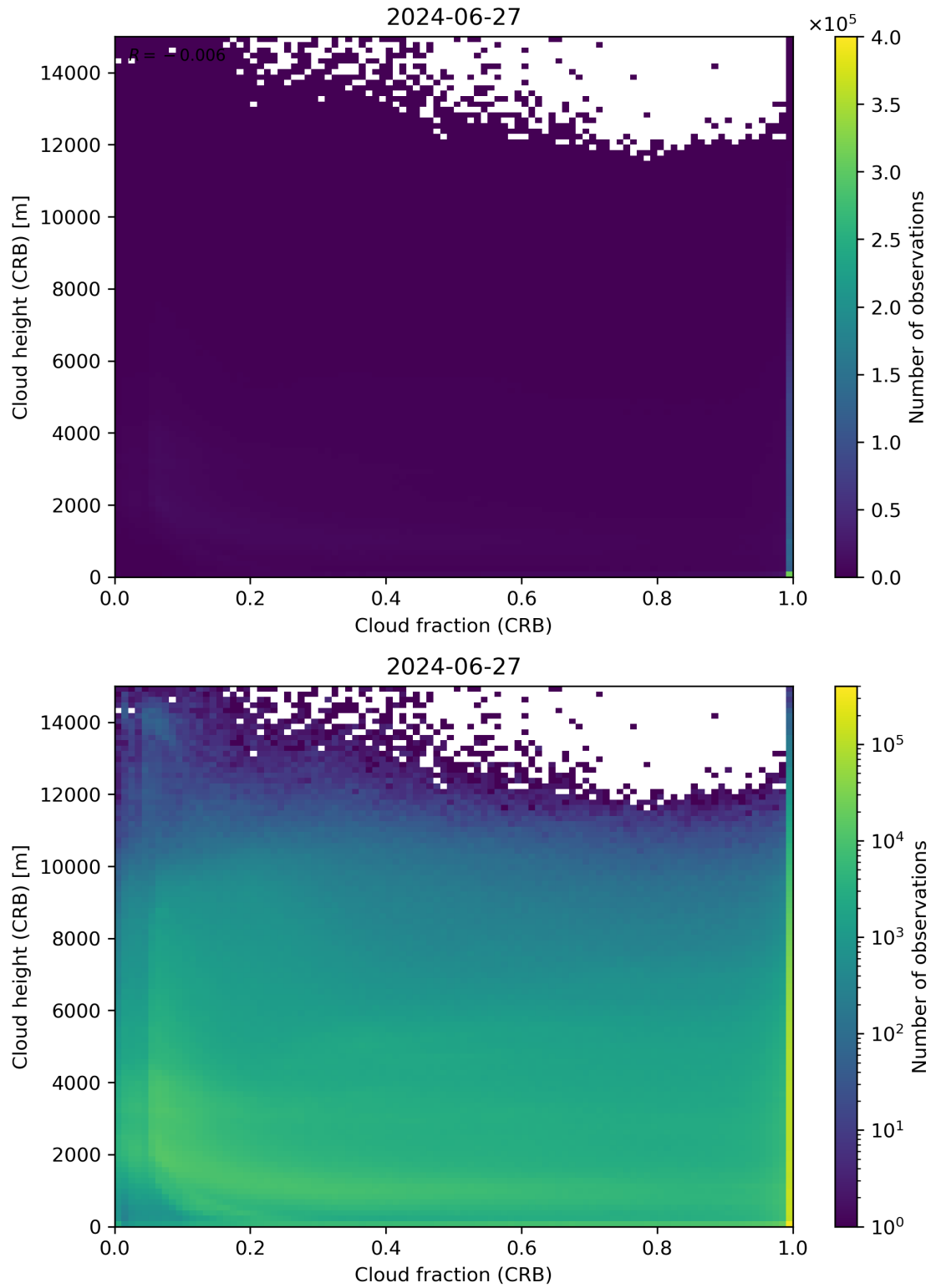
Figure 79: Scatter density plot of “Cloud fraction (CRB)” against “Cloud height (CRB)” for 2024-06-26 to 2024-06-28.
