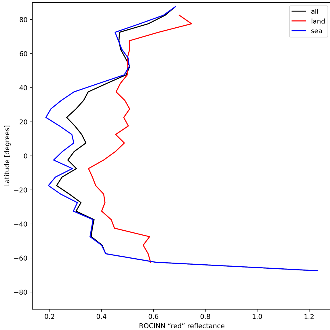
Figure 37: Zonal average of “ROCINN “red” reflectance” for 2024-06-26 to 2024-06-28.
