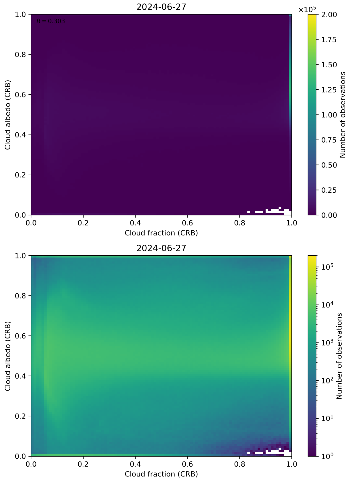
Figure 77: Scatter density plot of “Cloud fraction (CRB)” against “Cloud albedo (CRB)” for 2024-06-26 to 2024-06-28.
