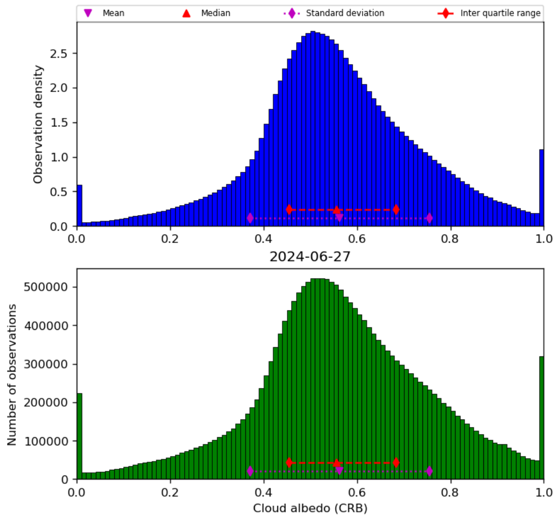
Figure 44: Histogram of “Cloud albedo (CRB)” for 2024-06-26 to 2024-06-28
