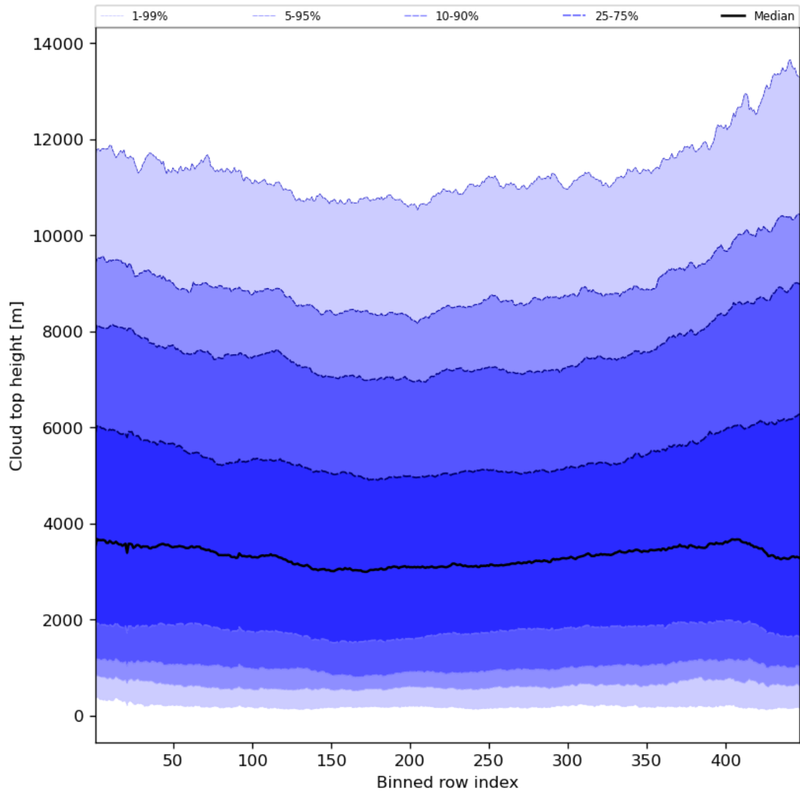
Figure 56: Along track statistics of “Cloud top height” for 2024-06-26 to 2024-06-28
