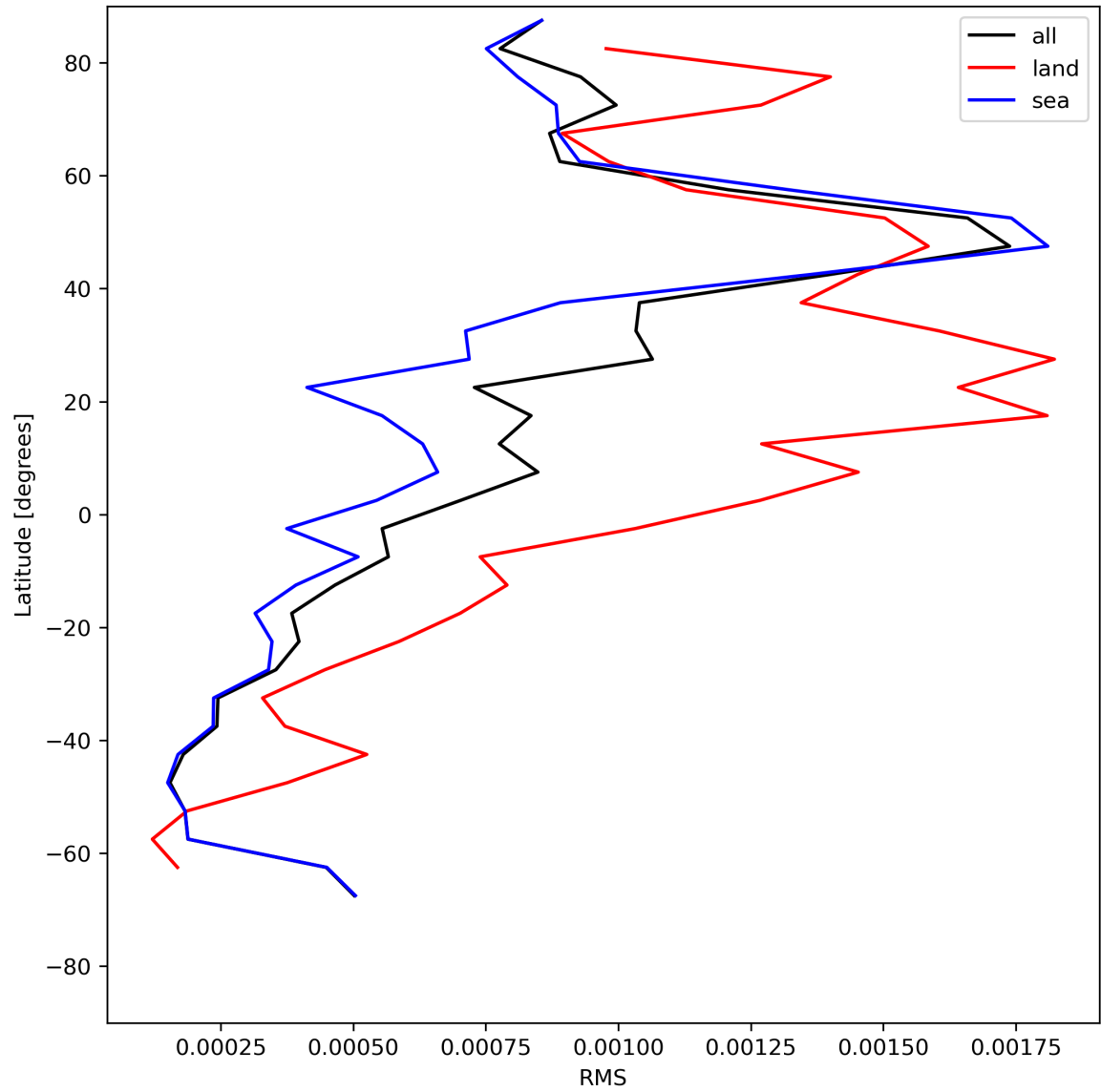
Figure 31: Zonal average of “RMS” for 2024-06-26 to 2024-06-28.
