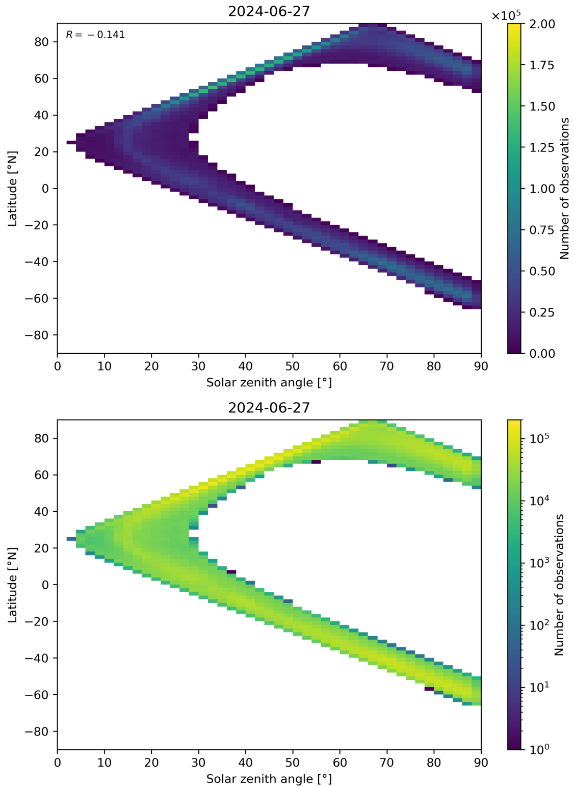
Figure 105: Scatter density plot of “Solar zenith angle” against “Latitude” for 2024-06-26 to 2024-06-28.
