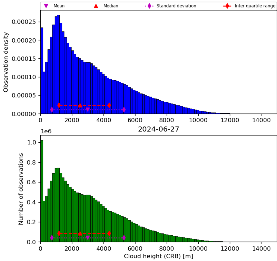
Figure 43: Histogram of “Cloud height (CRB)” for 2024-06-26 to 2024-06-28
