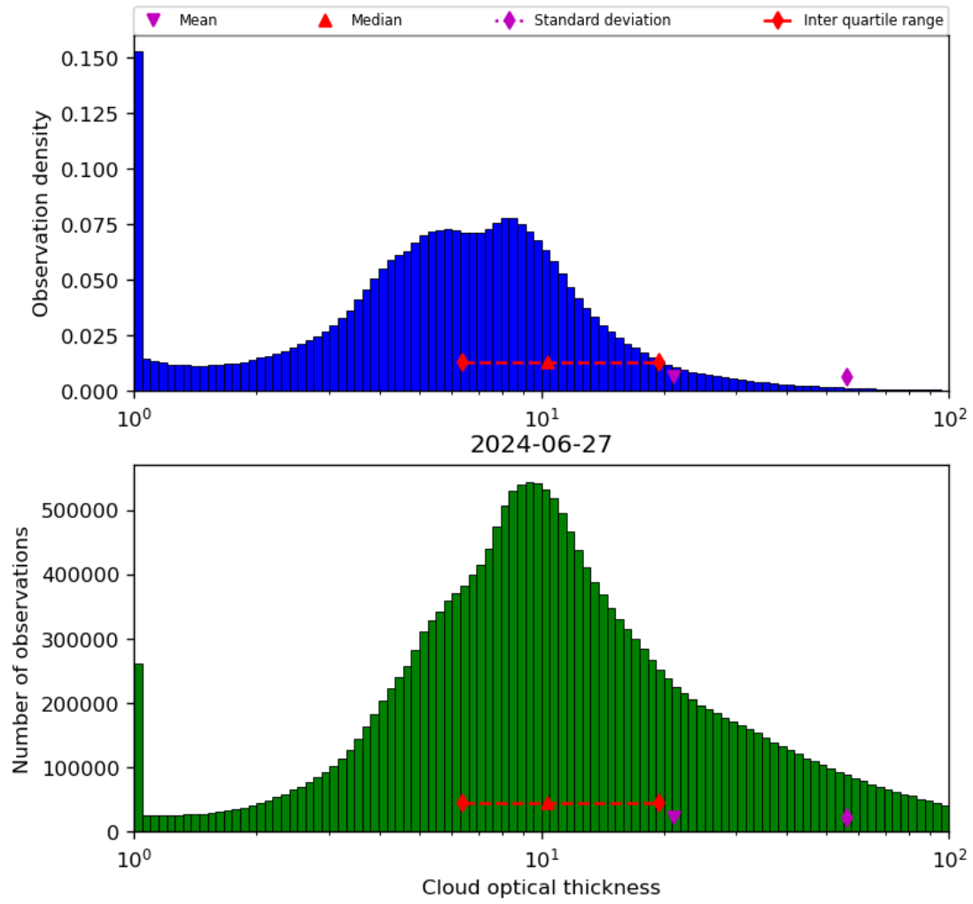
Figure 41: Histogram of “Cloud optical thickness” for 2024-06-26 to 2024-06-28
