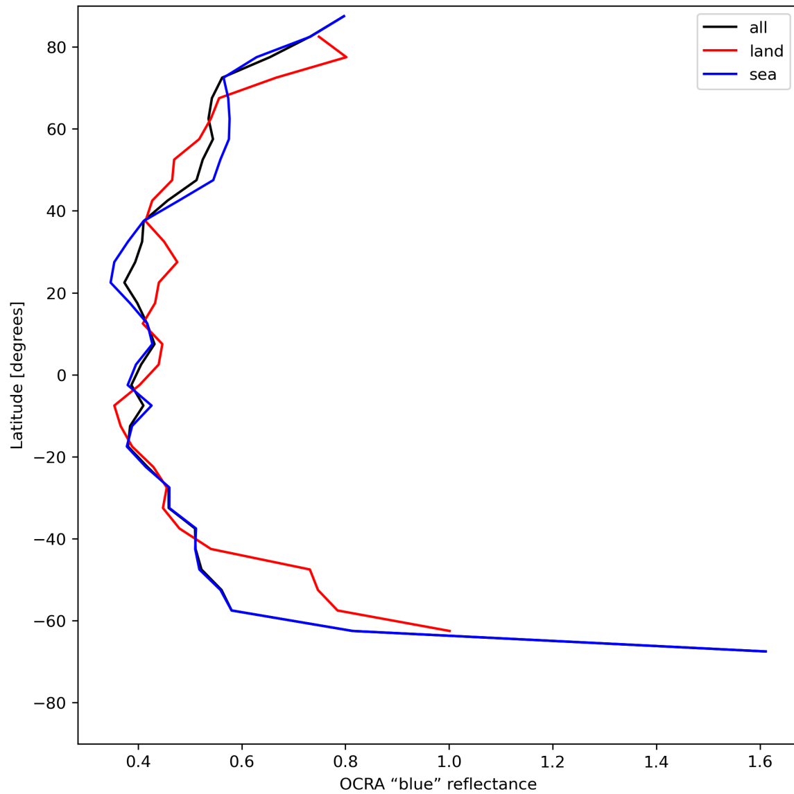
Figure 35: Zonal average of “OCRA “blue” reflectance” for 2024-06-26 to 2024-06-28.
