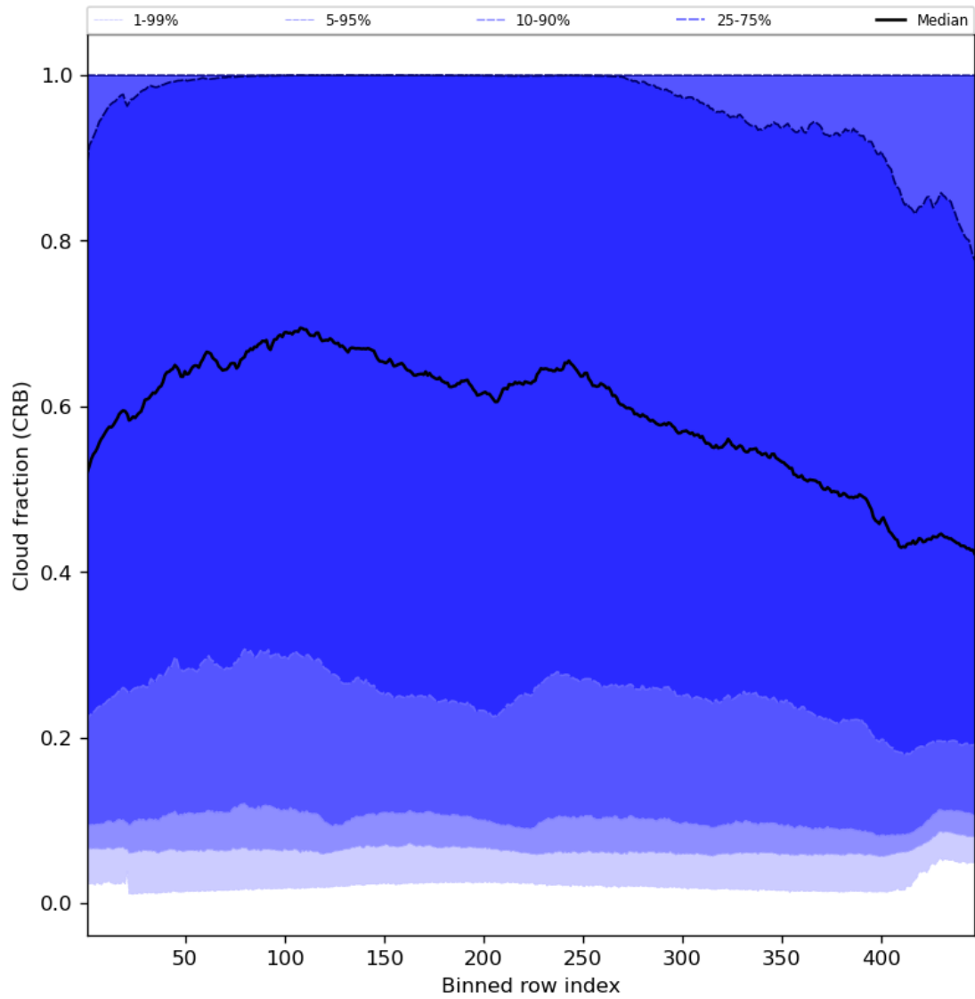
Figure 58: Along track statistics of “Cloud fraction (CRB)” for 2024-06-26 to 2024-06-28
