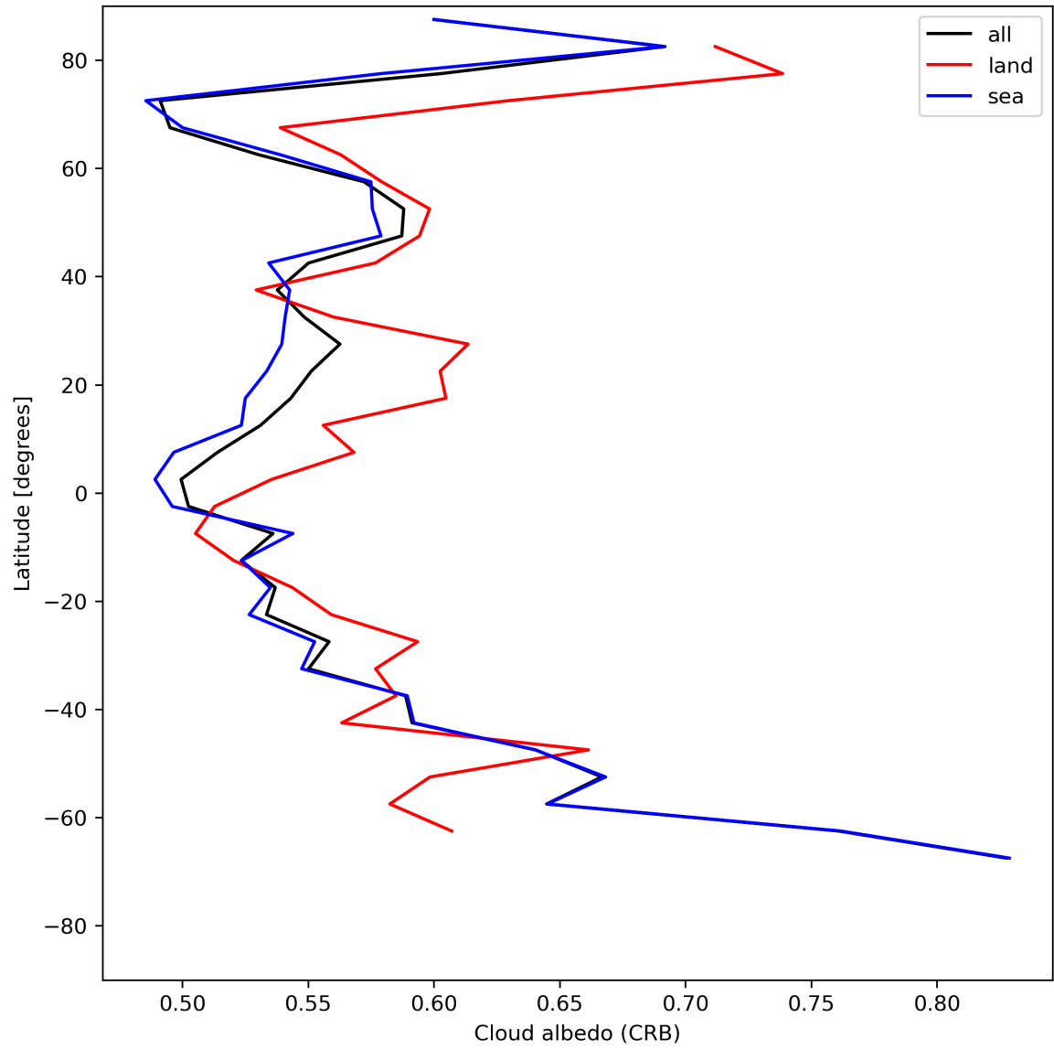
Figure 28: Zonal average of “Cloud albedo (CRB)” for 2024-06-26 to 2024-06-28.
