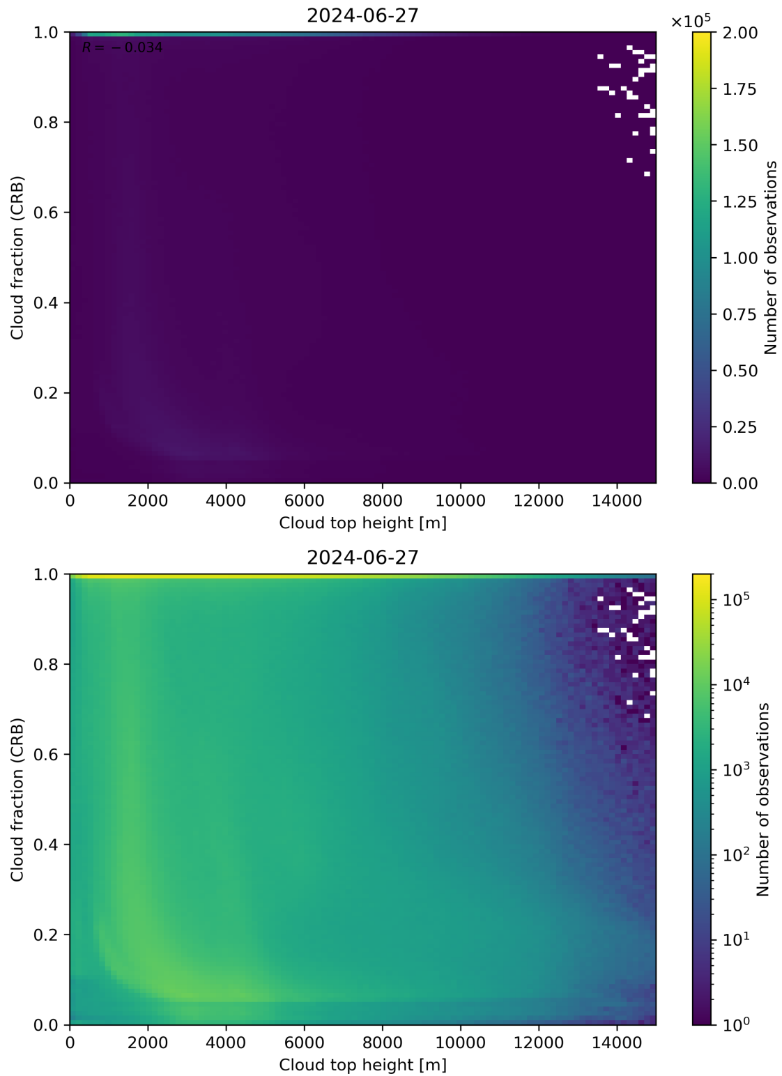
Figure 88: Scatter density plot of “Cloud top height” against “Cloud fraction (CRB)” for 2024-06-26 to 2024-06-28.
