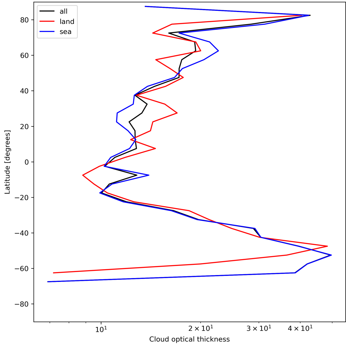
Figure 25: Zonal average of “Cloud optical thickness” for 2024-06-26 to 2024-06-28.
