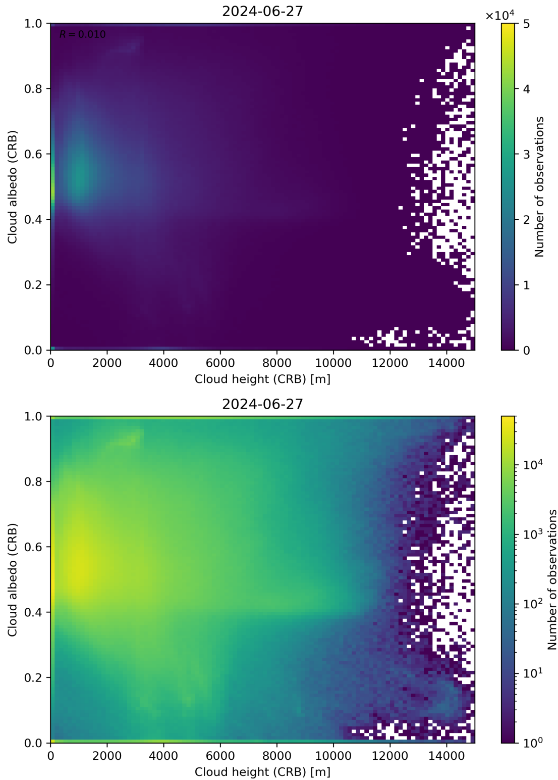
Figure 80: Scatter density plot of “Cloud height (CRB)” against “Cloud albedo (CRB)” for 2024-06-26 to 2024-06-28.
