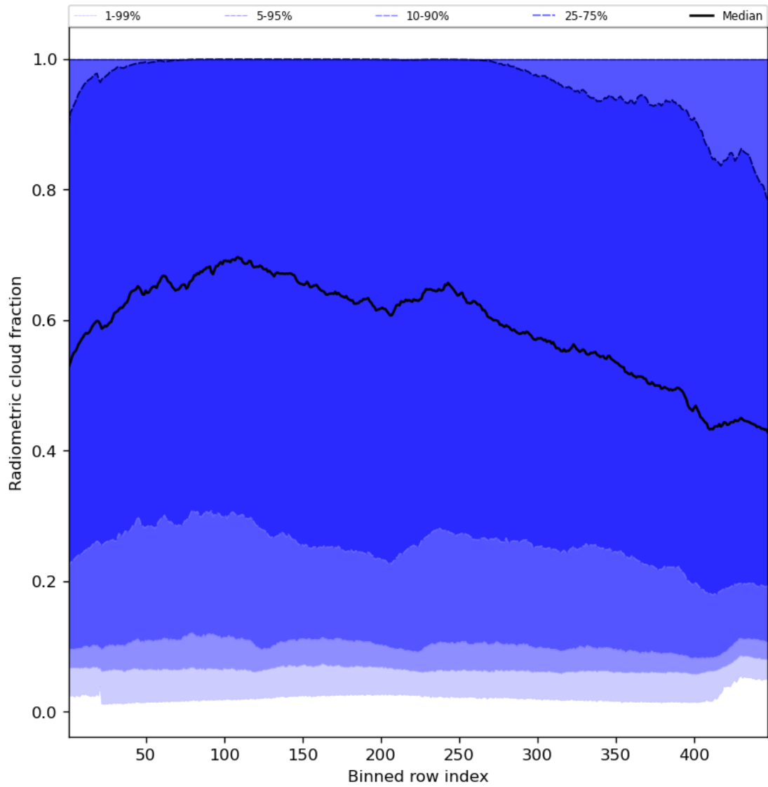
Figure 55: Along track statistics of “Radiometric cloud fraction” for 2024-06-26 to 2024-06-28
