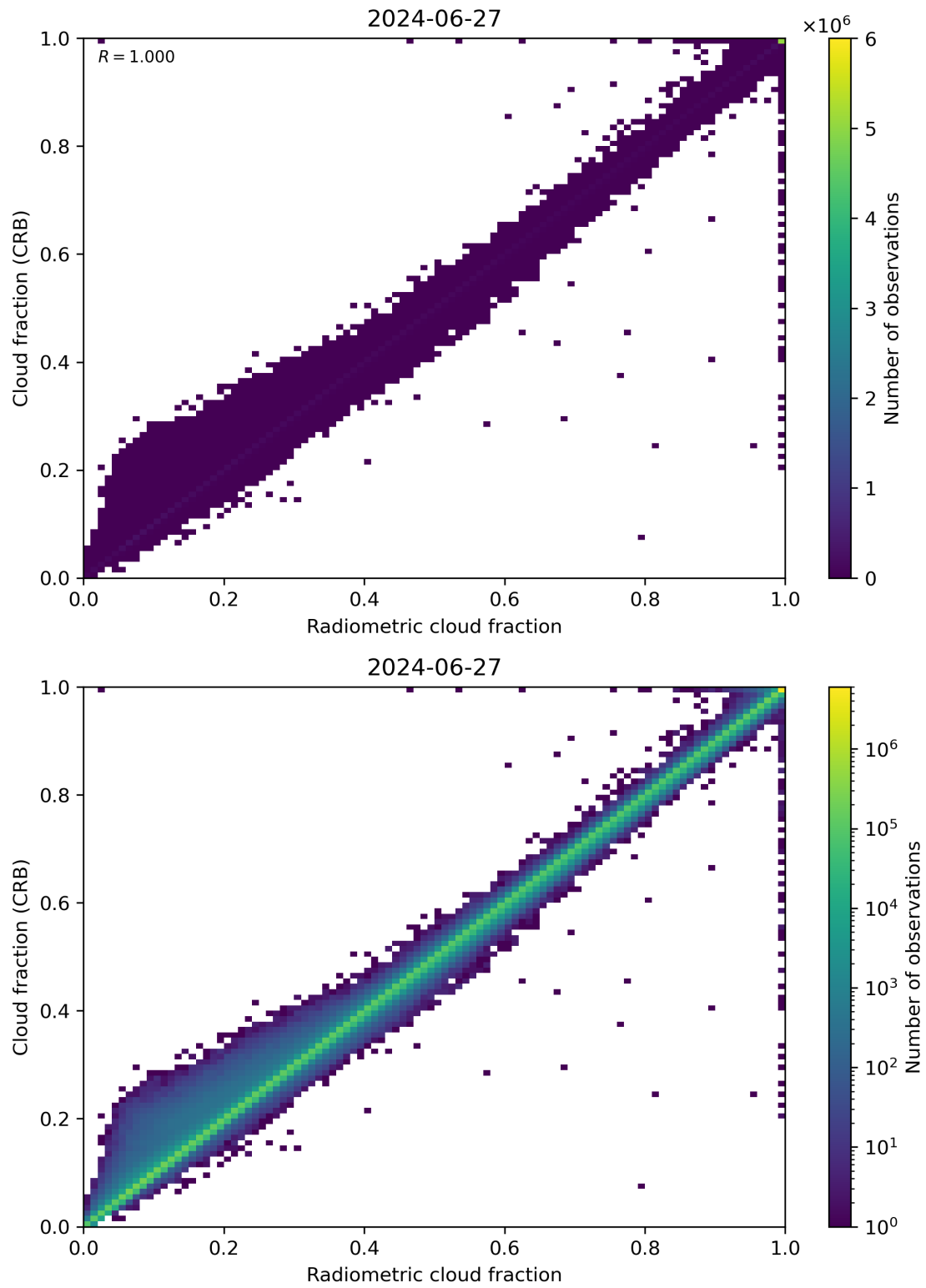
Figure 73: Scatter density plot of “Radiometric cloud fraction” against “Cloud fraction (CRB)” for 2024-06-26 to 2024-06-28.
