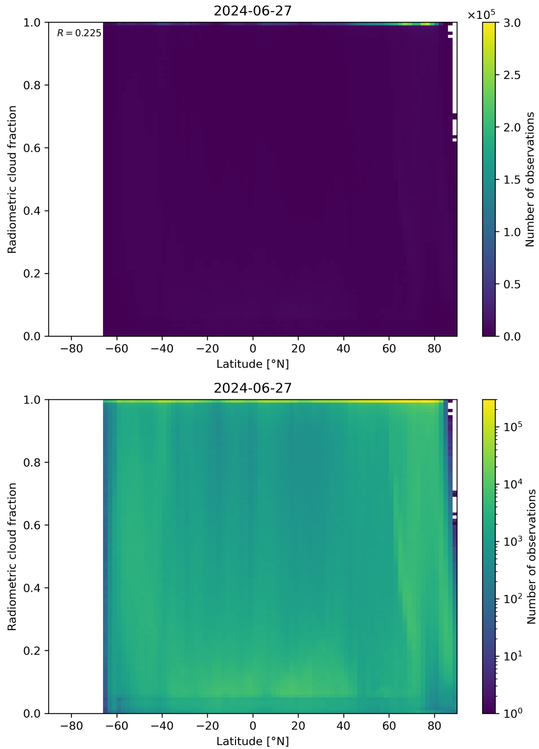
Figure 92: Scatter density plot of “Latitude” against “Radiometric cloud fraction” for 2024-06-26 to 2024-06-28.
