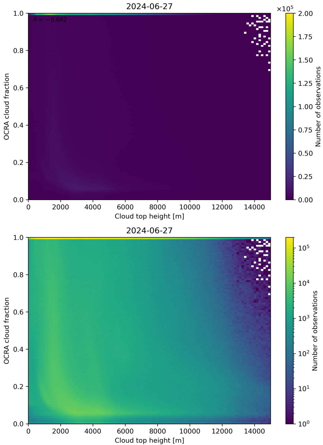
Figure 87: Scatter density plot of “Cloud top height” against “OCRA cloud fraction” for 2024-06-26 to 2024-06-28.
