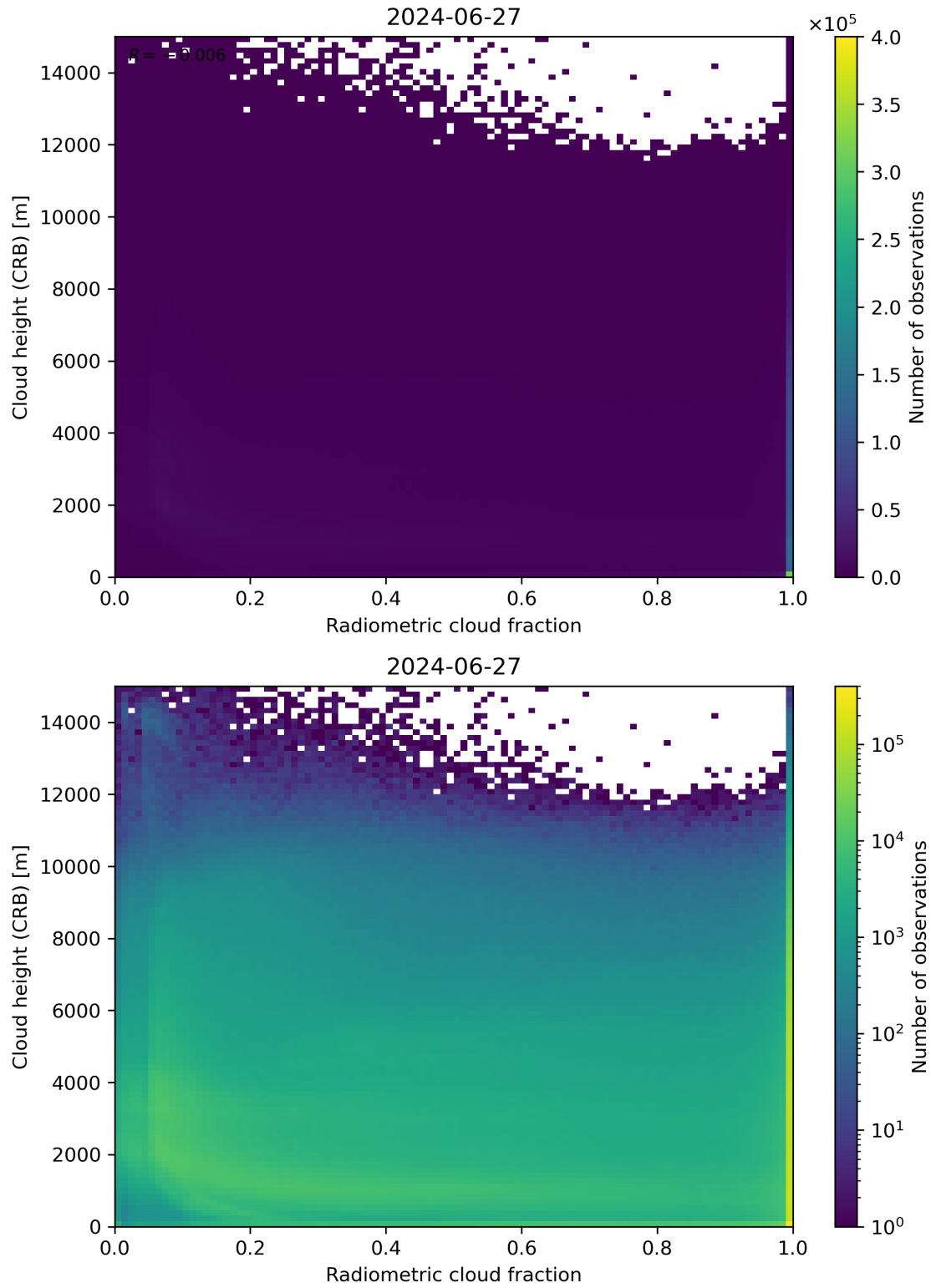
Figure 74: Scatter density plot of “Radiometric cloud fraction” against “Cloud height (CRB)” for 2024-06-26 to 2024-06-28.
