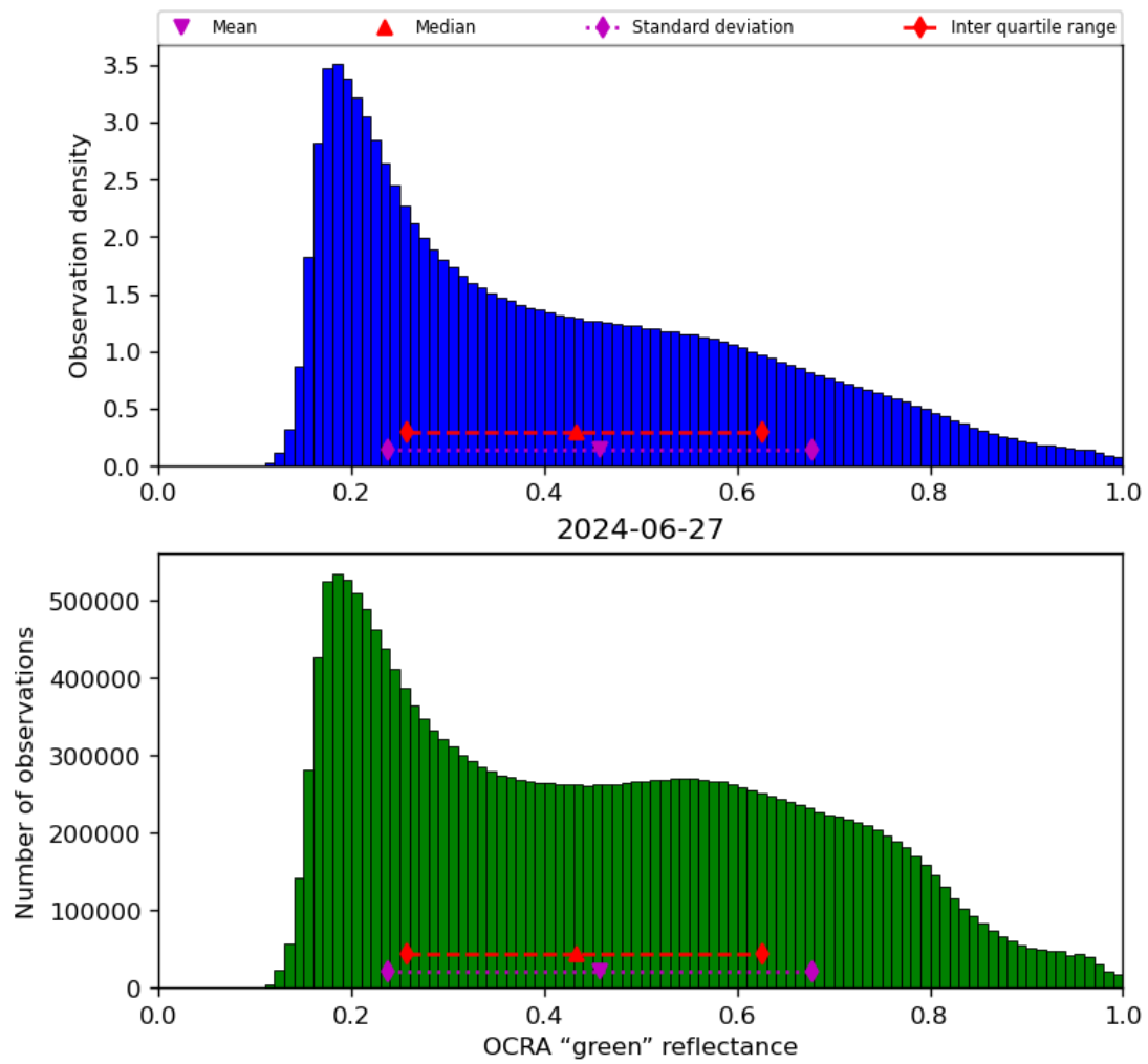
Figure 52: Histogram of “OCRA “green” reflectance” for 2024-06-26 to 2024-06-28
