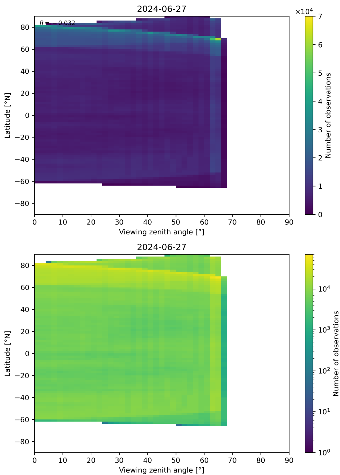
Figure 113: Scatter density plot of “Viewing zenith angle” against “Latitude” for 2024-06-26 to 2024-06-28.
