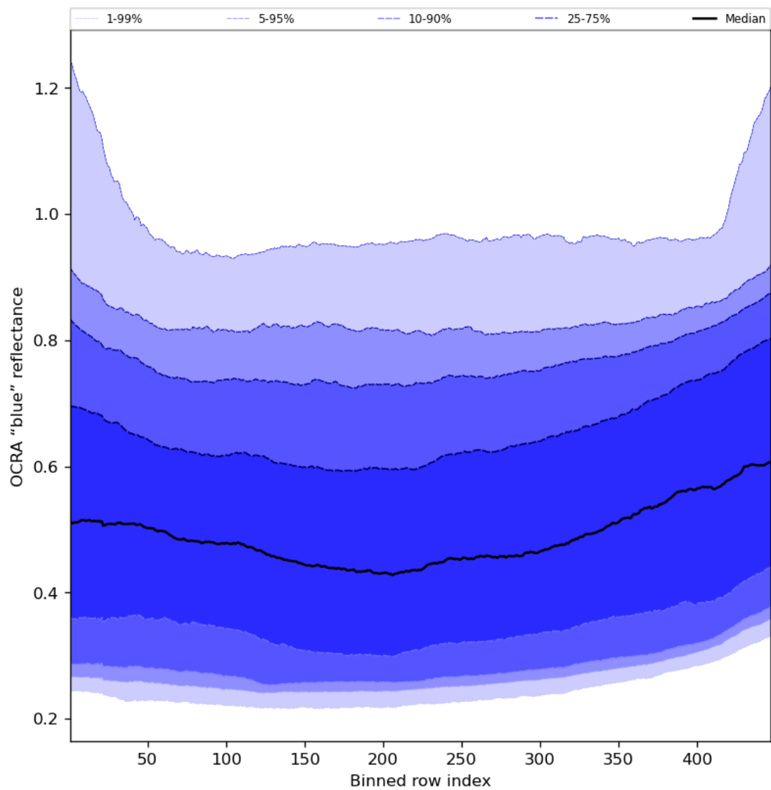
Figure 67: Along track statistics of “OCRA “blue” reflectance” for 2024-06-26 to 2024-06-28
