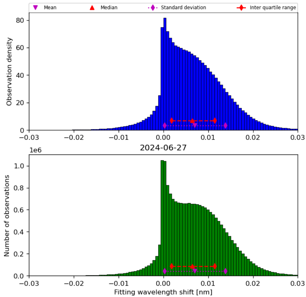
Figure 49: Histogram of “Fitting wavelength shift” for 2024-06-26 to 2024-06-28
