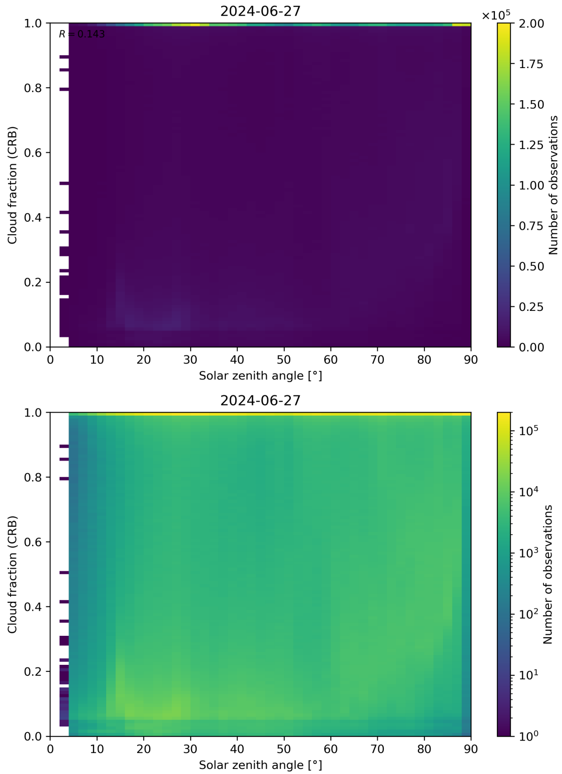
Figure 101: Scatter density plot of “Solar zenith angle” against “Cloud fraction (CRB)” for 2024-06-26 to 2024-06-28.
