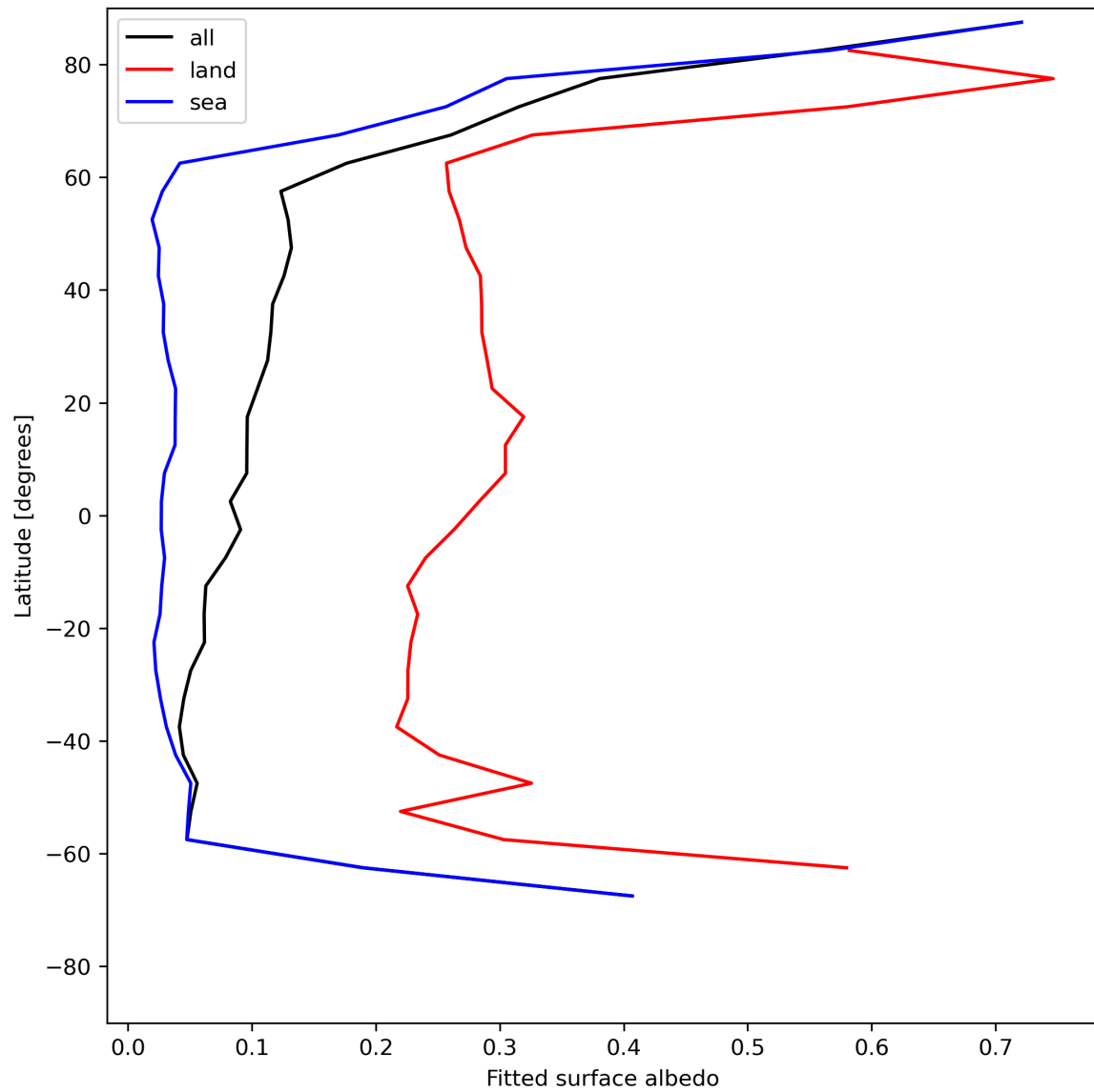
Figure 29: Zonal average of “Fitted surface albedo” for 2024-06-26 to 2024-06-28.
