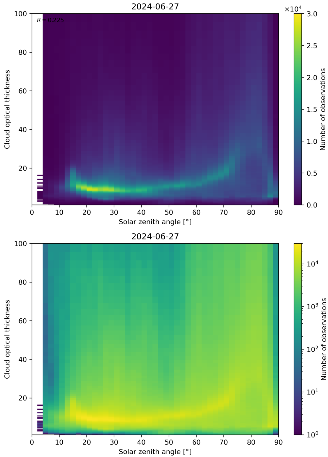
Figure 103: Scatter density plot of “Solar zenith angle” against “Cloud optical thickness” for 2024-06-26 to 2024-06-28.
