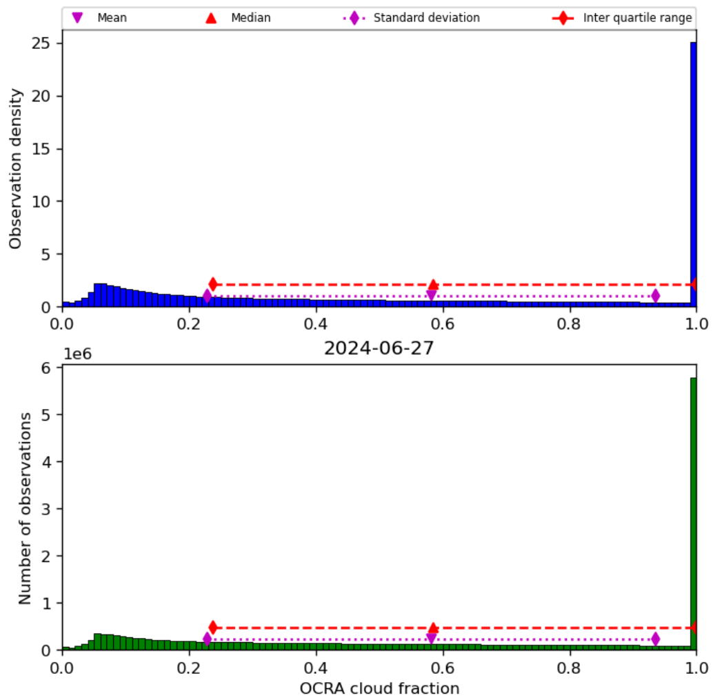
Figure 50: Histogram of “OCRA cloud fraction” for 2024-06-26 to 2024-06-28
