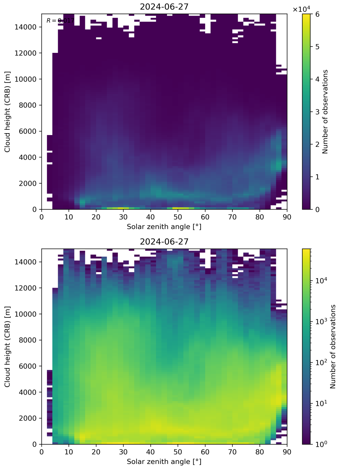
Figure 102: Scatter density plot of “Solar zenith angle” against “Cloud height (CRB)” for 2024-06-26 to 2024-06-28.
