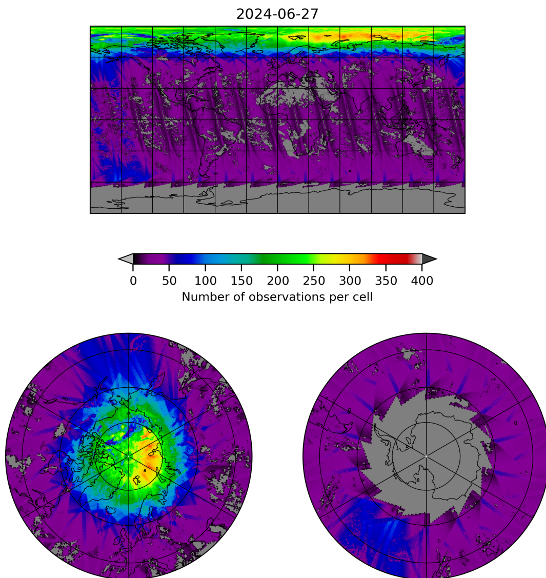
Figure 21: Map of the number of observations for 2024-06-26 to 2024-06-28
