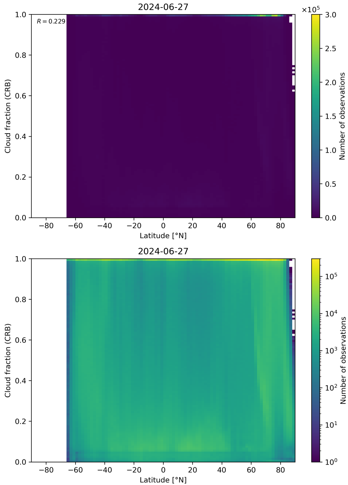
Figure 94: Scatter density plot of “Latitude” against “Cloud fraction (CRB)” for 2024-06-26 to 2024-06-28.
