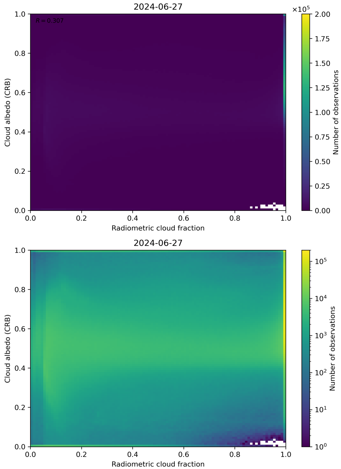
Figure 71: Scatter density plot of “Radiometric cloud fraction” against “Cloud albedo (CRB)” for 2024-06-26 to 2024-06-28.
