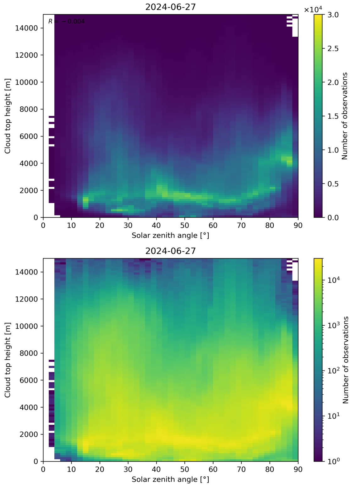
Figure 104: Scatter density plot of “Solar zenith angle” against “Cloud top height” for 2024-06-26 to 2024-06-28.
