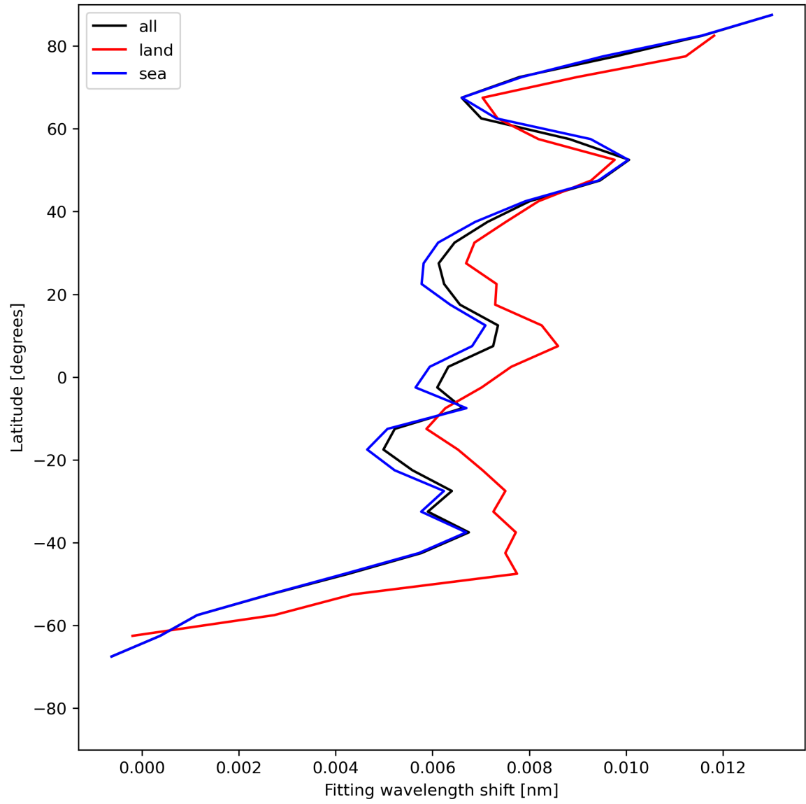
Figure 33: Zonal average of “Fitting wavelength shift” for 2024-06-26 to 2024-06-28.
