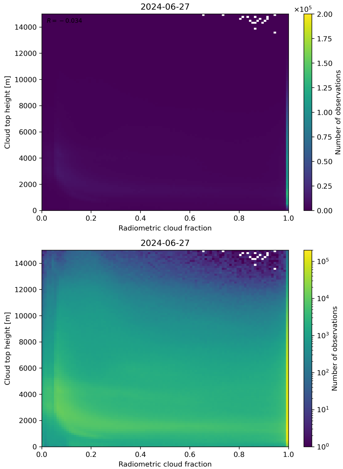
Figure 76: Scatter density plot of “Radiometric cloud fraction” against “Cloud top height” for 2024-06-26 to 2024-06-28.
