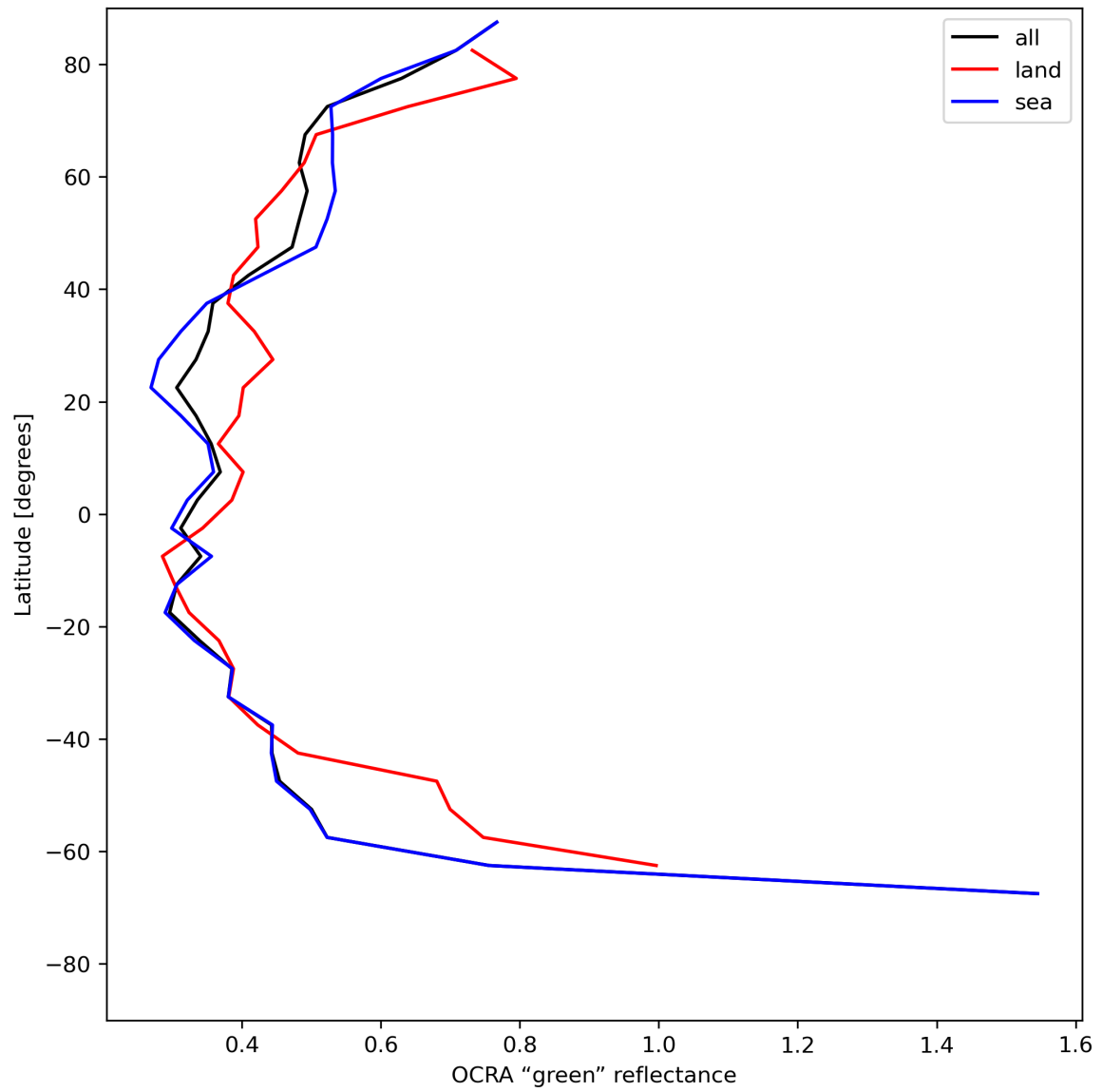
Figure 36: Zonal average of “OCRA “green” reflectance” for 2024-06-26 to 2024-06-28.
