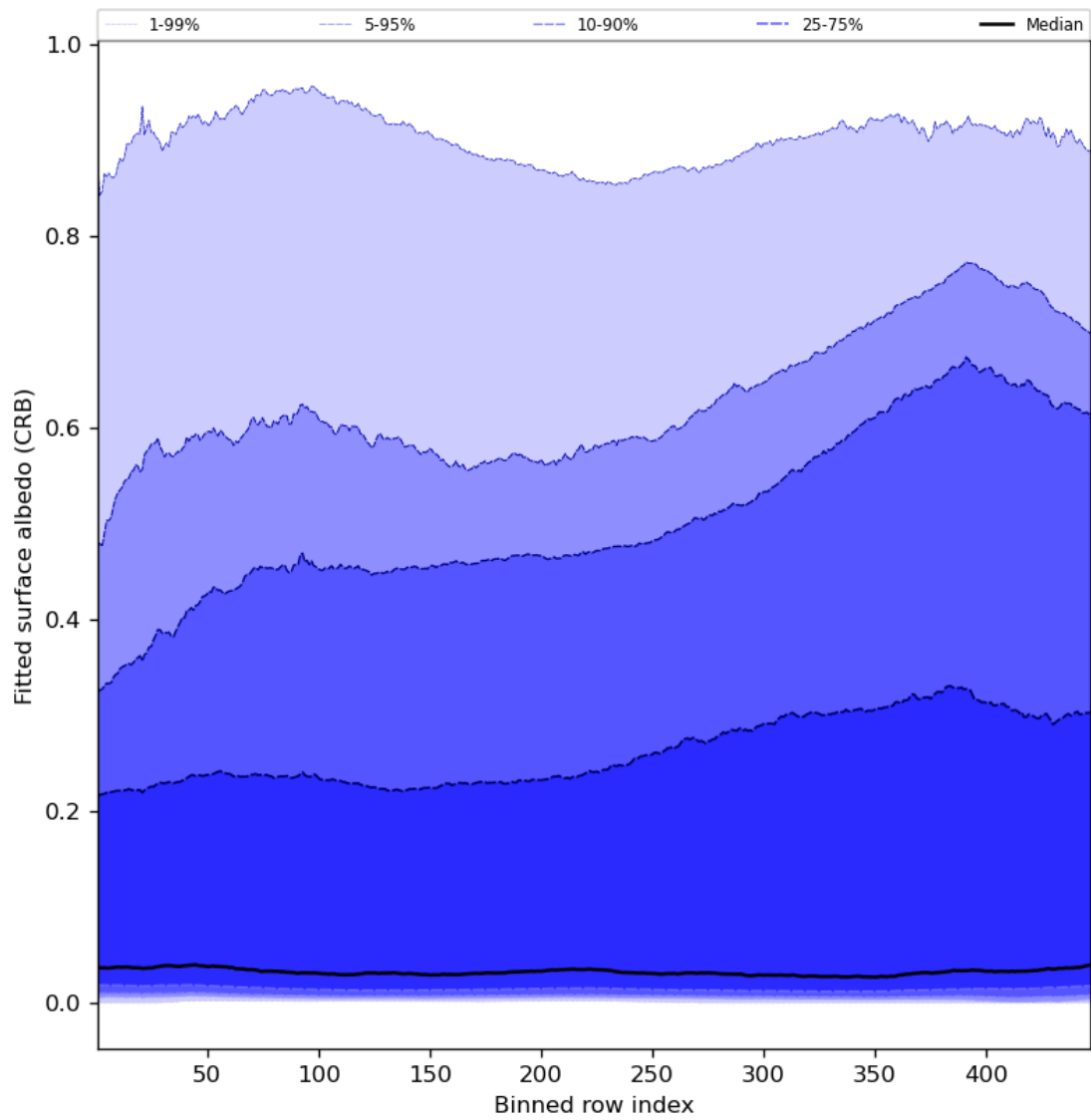
Figure 62: Along track statistics of “Fitted surface albedo (CRB)” for 2024-06-27 to 2024-06-29
