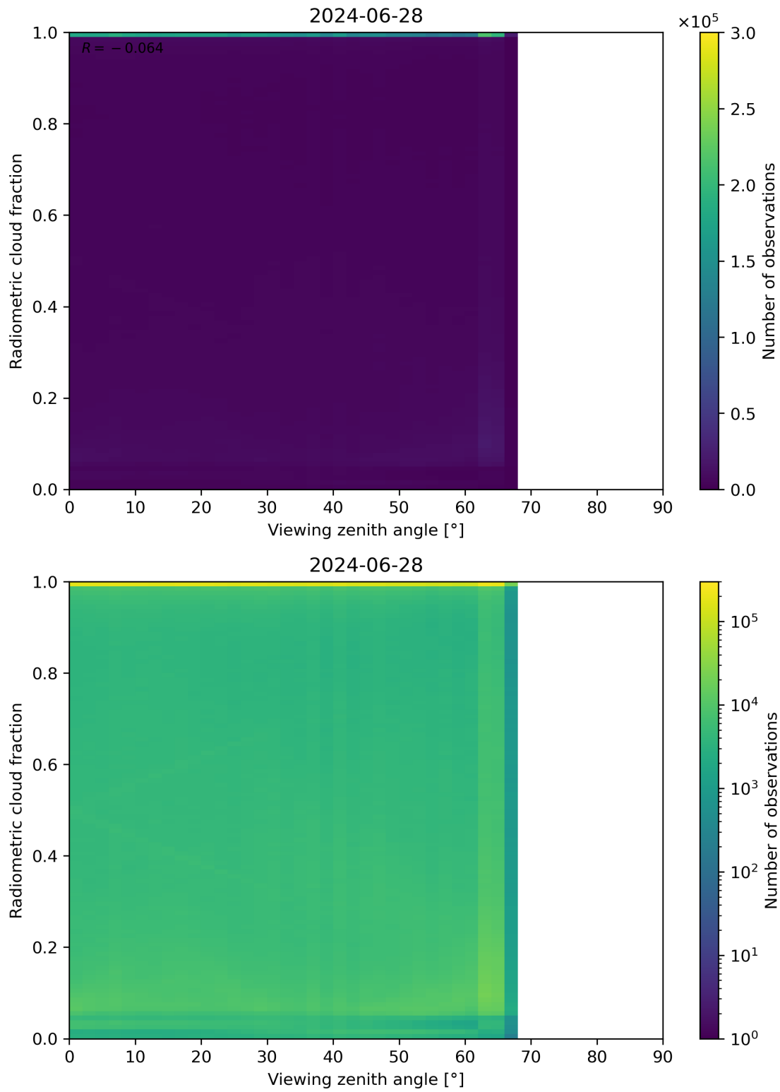
Figure 107: Scatter density plot of “Viewing zenith angle” against “Radiometric cloud fraction” for 2024-06-27 to 2024-06-29.
