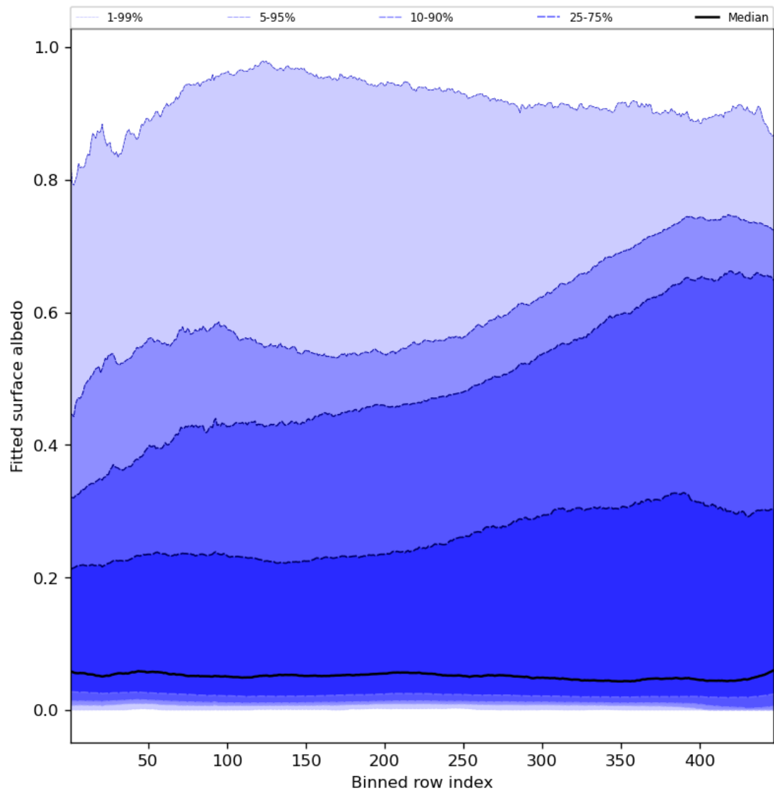
Figure 61: Along track statistics of “Fitted surface albedo” for 2024-06-27 to 2024-06-29
