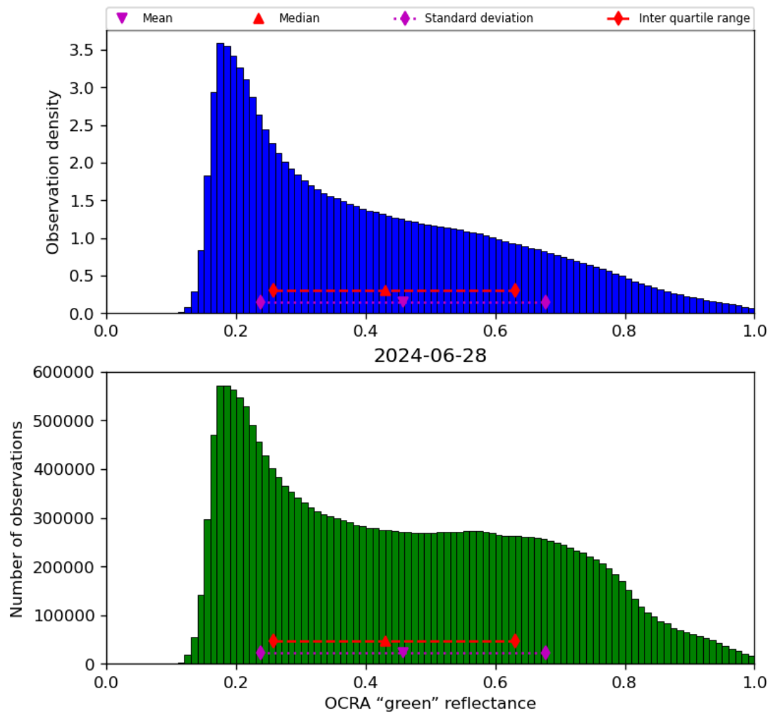
Figure 52: Histogram of “OCRA “green” reflectance” for 2024-06-27 to 2024-06-29
