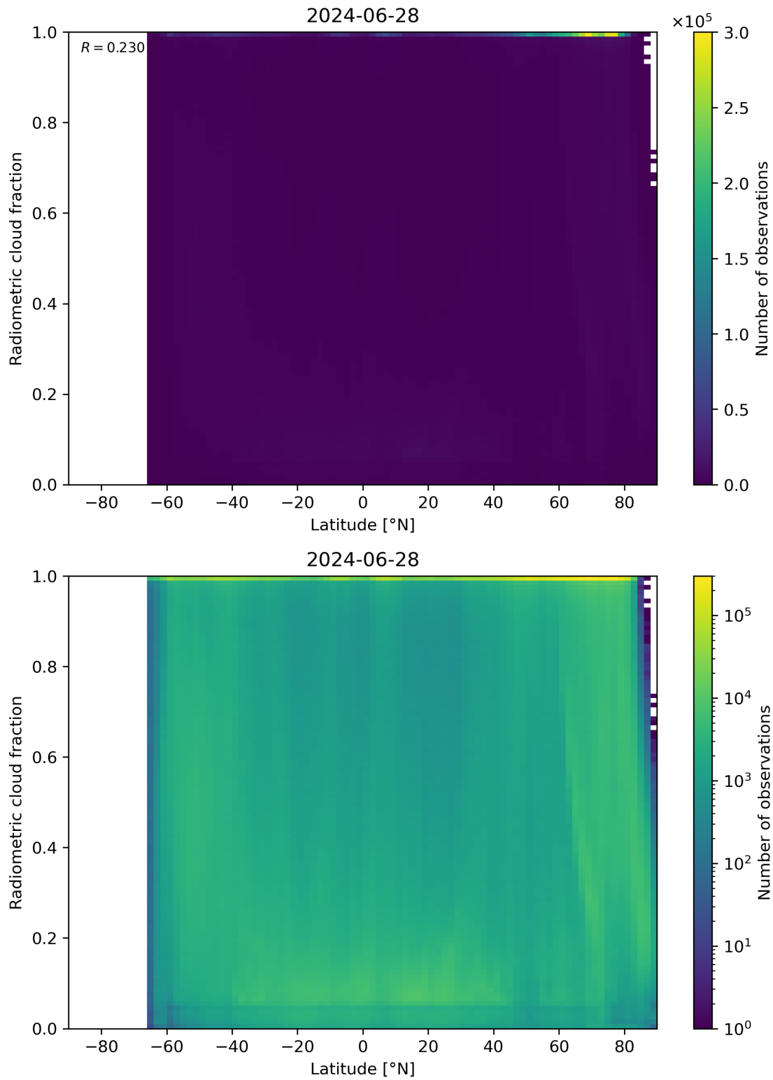
Figure 92: Scatter density plot of “Latitude” against “Radiometric cloud fraction” for 2024-06-27 to 2024-06-29.
