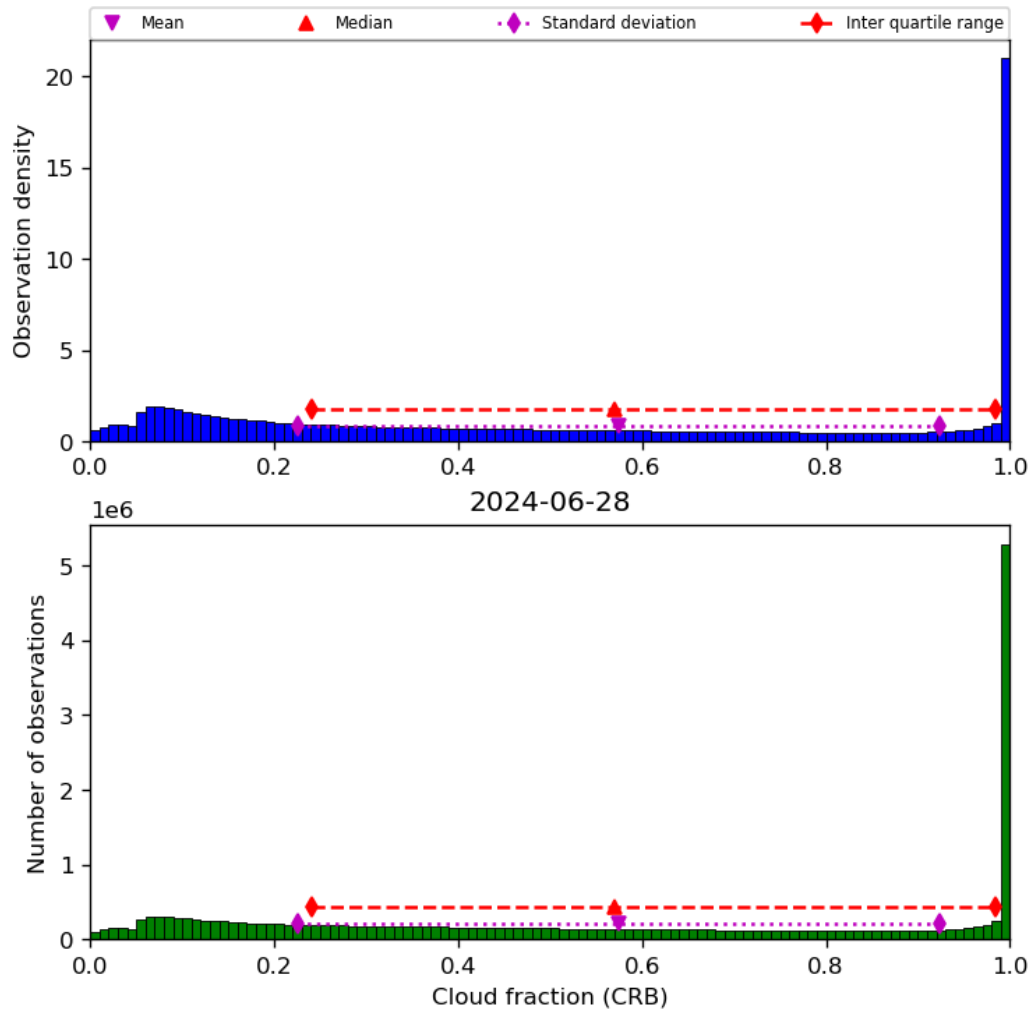
Figure 42: Histogram of “Cloud fraction (CRB)” for 2024-06-27 to 2024-06-29
