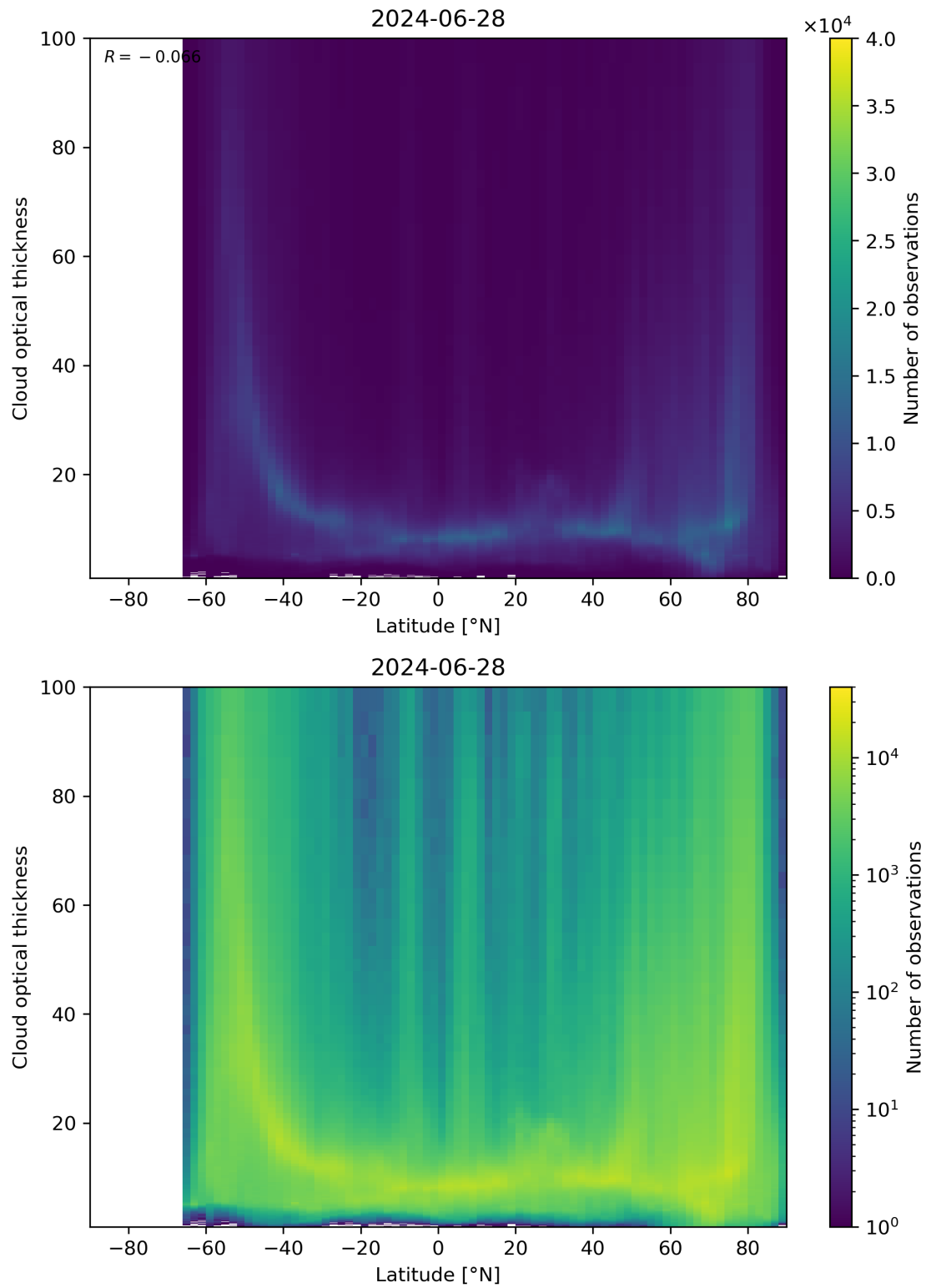
Figure 96: Scatter density plot of “Latitude” against “Cloud optical thickness” for 2024-06-27 to 2024-06-29.
