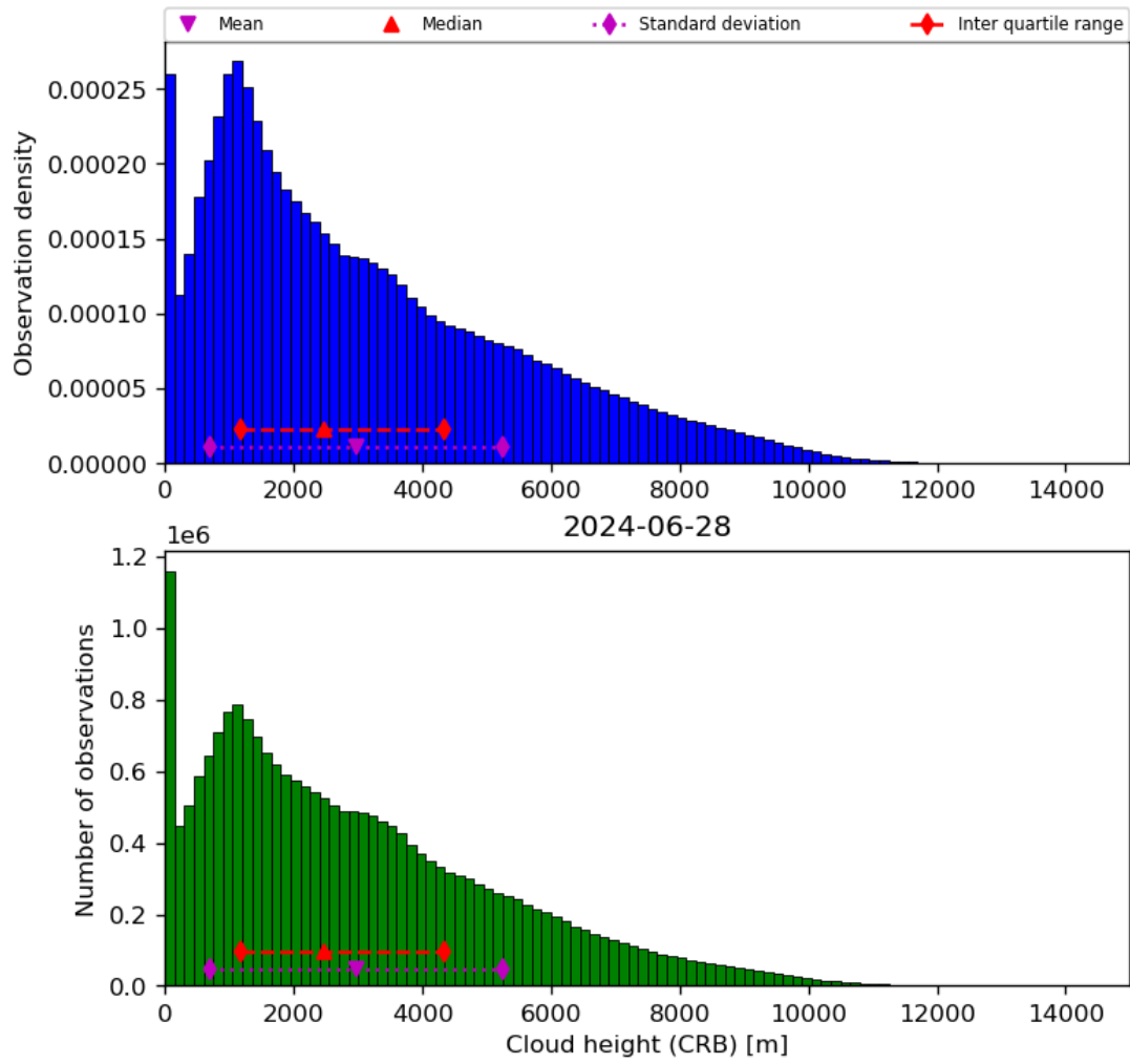
Figure 43: Histogram of “Cloud height (CRB)” for 2024-06-27 to 2024-06-29
