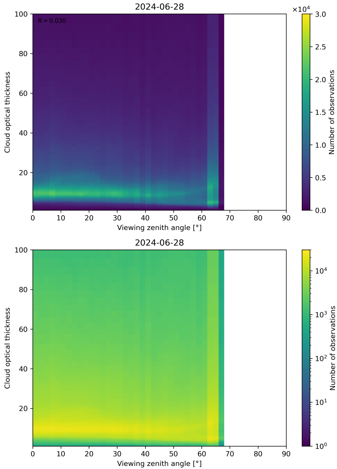
Figure 111: Scatter density plot of “Viewing zenith angle” against “Cloud optical thickness” for 2024-06-27 to 2024-06-29.
