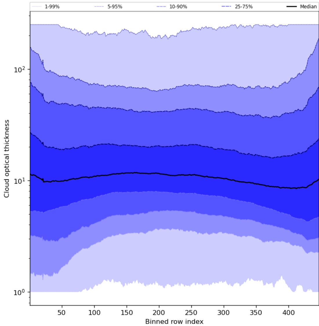
Figure 57: Along track statistics of “Cloud optical thickness” for 2024-06-27 to 2024-06-29
