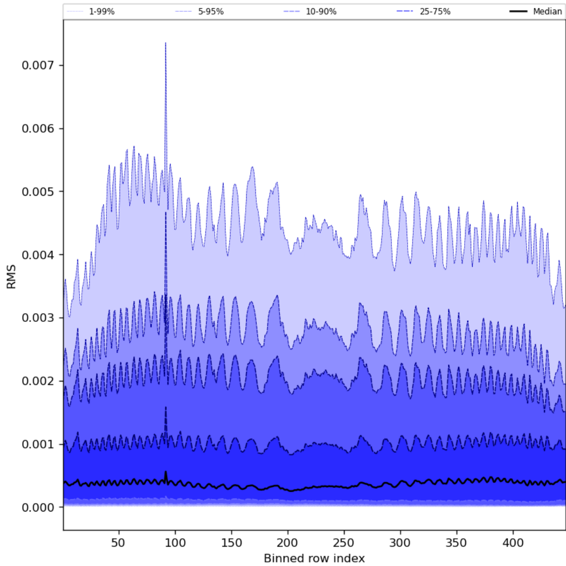
Figure 63: Along track statistics of “RMS” for 2024-06-27 to 2024-06-29
