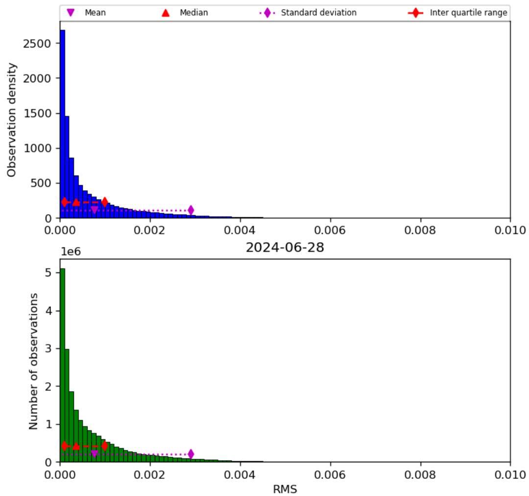
Figure 47: Histogram of “RMS” for 2024-06-27 to 2024-06-29
