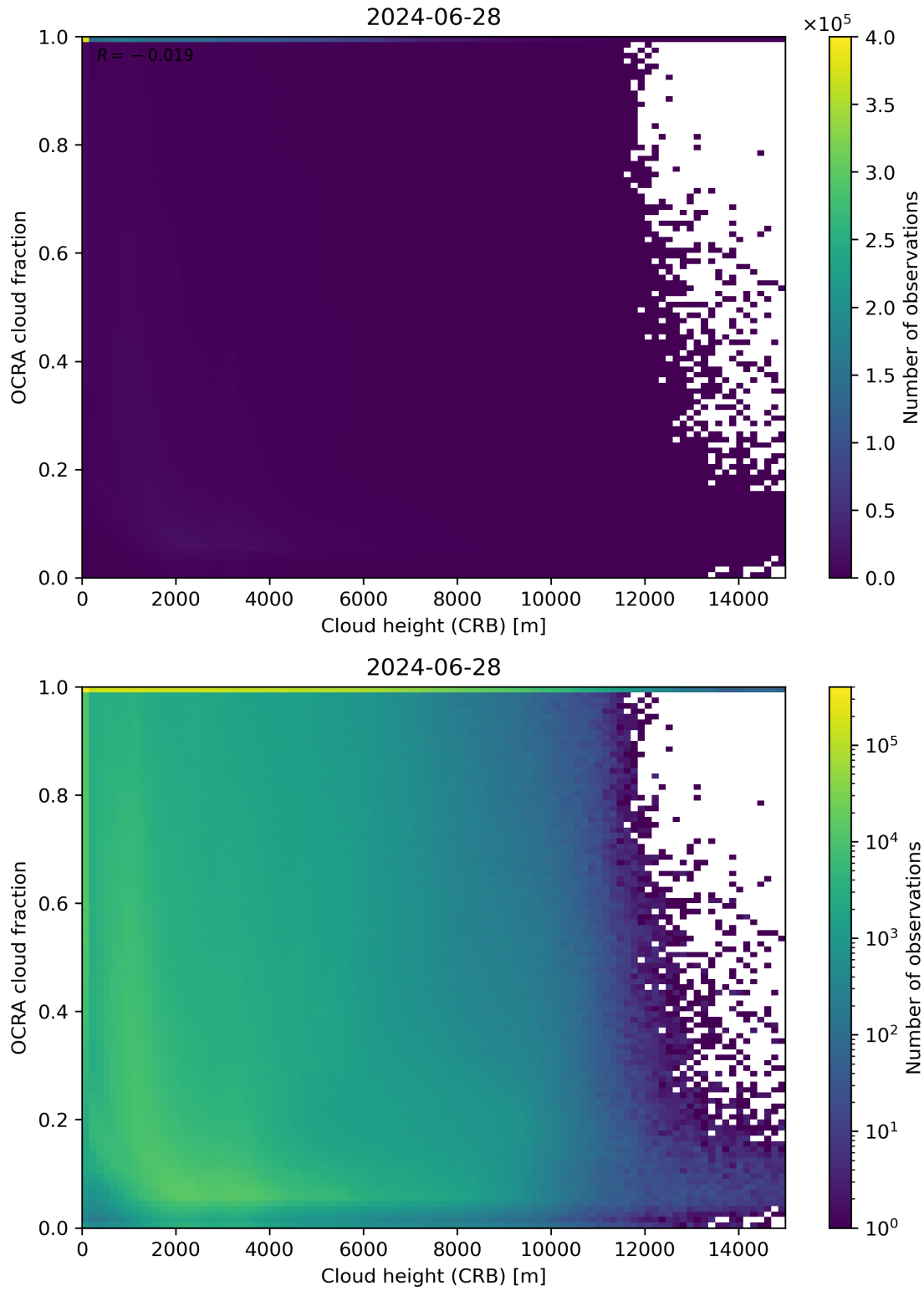
Figure 81: Scatter density plot of “Cloud height (CRB)” against “OCRA cloud fraction” for 2024-06-27 to 2024-06-29.
