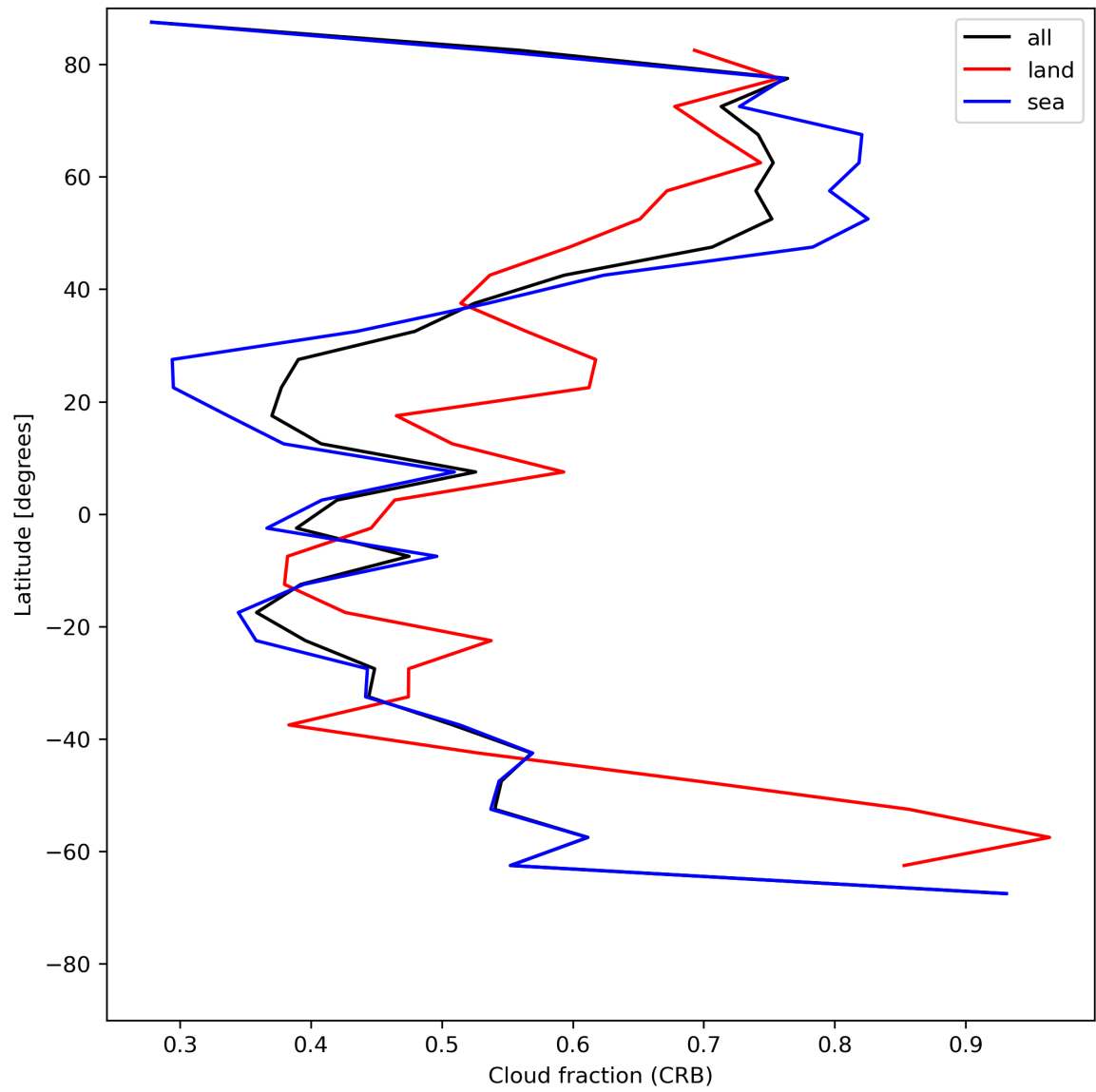
Figure 26: Zonal average of “Cloud fraction (CRB)” for 2024-06-27 to 2024-06-29.
