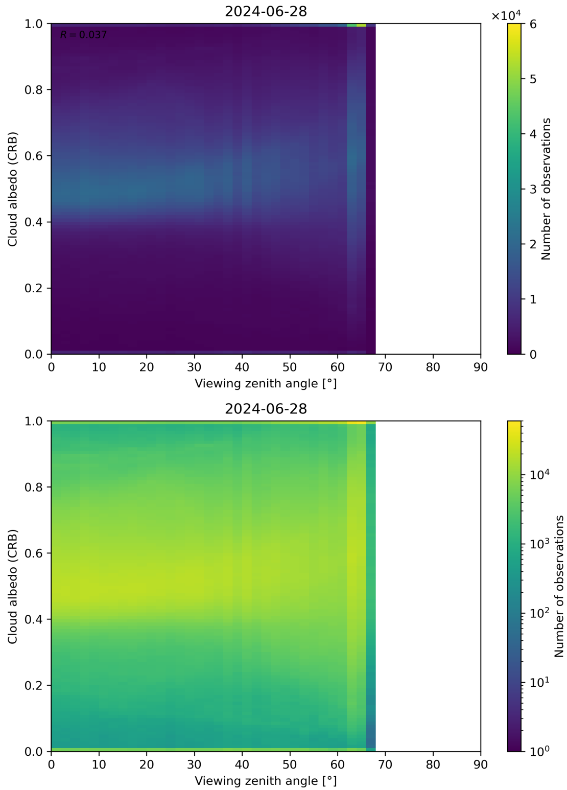
Figure 106: Scatter density plot of “Viewing zenith angle” against “Cloud albedo (CRB)” for 2024-06-27 to 2024-06-29.
