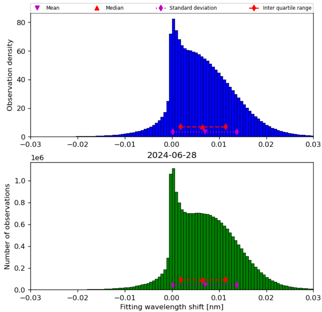
Figure 49: Histogram of “Fitting wavelength shift” for 2024-06-27 to 2024-06-29
