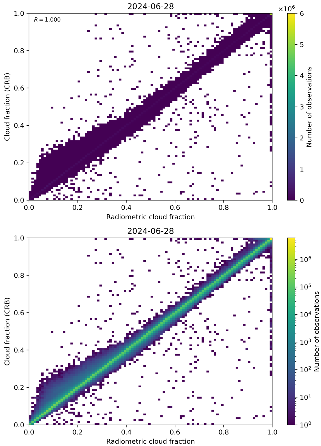
Figure 73: Scatter density plot of “Radiometric cloud fraction” against “Cloud fraction (CRB)” for 2024-06-27 to 2024-06-29.
