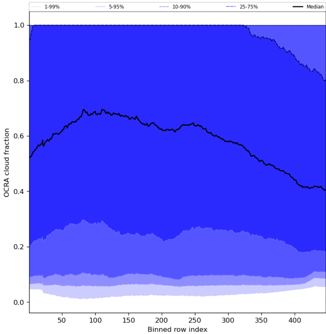
Figure 66: Along track statistics of “OCRA cloud fraction” for 2024-06-27 to 2024-06-29
