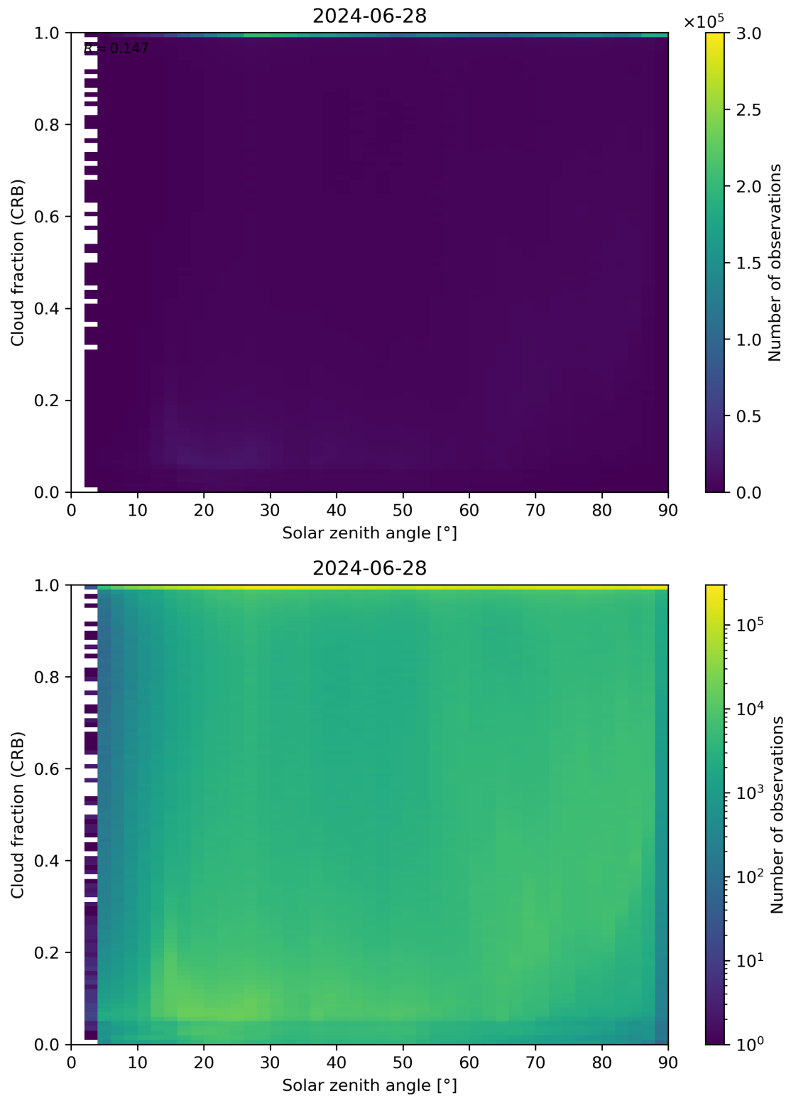
Figure 101: Scatter density plot of “Solar zenith angle” against “Cloud fraction (CRB)” for 2024-06-27 to 2024-06-29.
