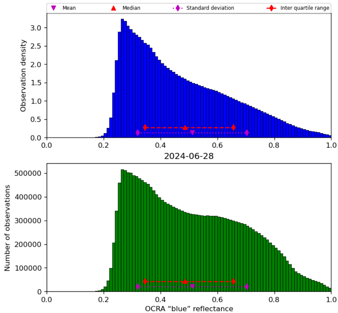
Figure 51: Histogram of “OCRA “blue” reflectance” for 2024-06-27 to 2024-06-29
