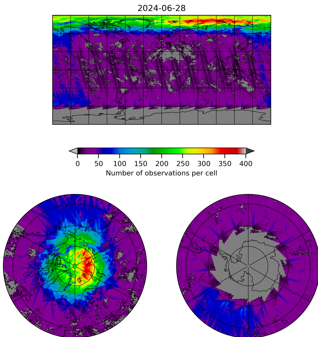
Figure 21: Map of the number of observations for 2024-06-27 to 2024-06-29
