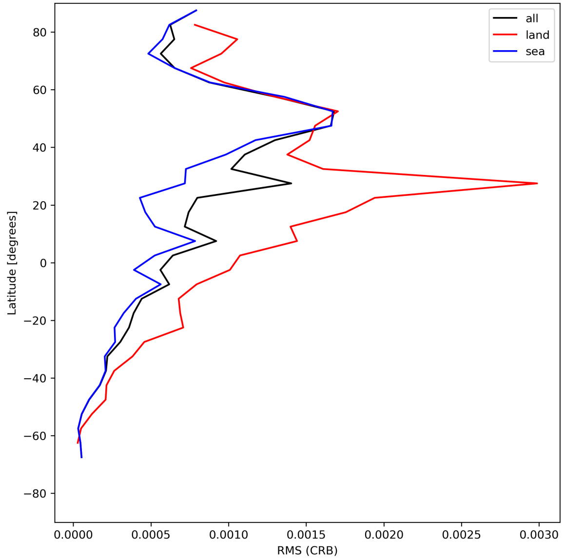
Figure 32: Zonal average of “RMS (CRB)” for 2024-06-27 to 2024-06-29.
