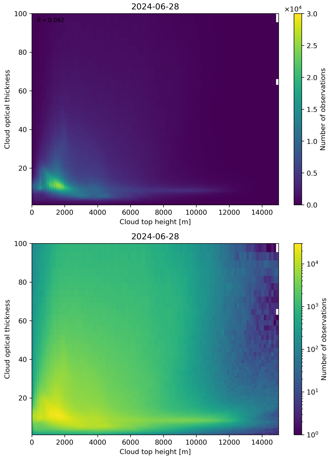
Figure 90: Scatter density plot of “Cloud top height” against “Cloud optical thickness” for 2024-06-27 to 2024-06-29.
