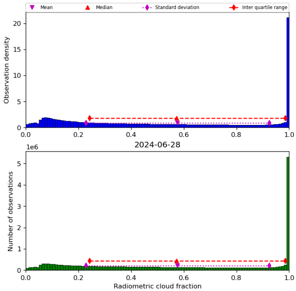
Figure 39: Histogram of “Radiometric cloud fraction” for 2024-06-27 to 2024-06-29
