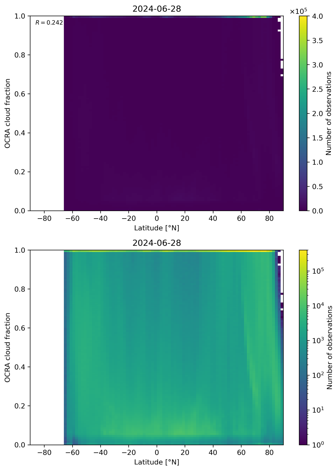
Figure 93: Scatter density plot of “Latitude” against “OCRA cloud fraction” for 2024-06-27 to 2024-06-29.
