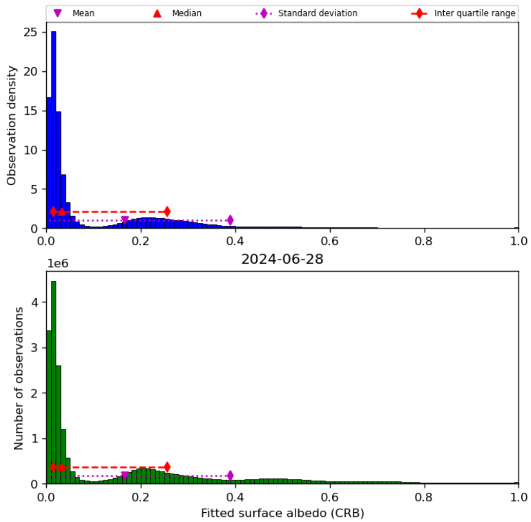
Figure 46: Histogram of “Fitted surface albedo (CRB)” for 2024-06-27 to 2024-06-29
