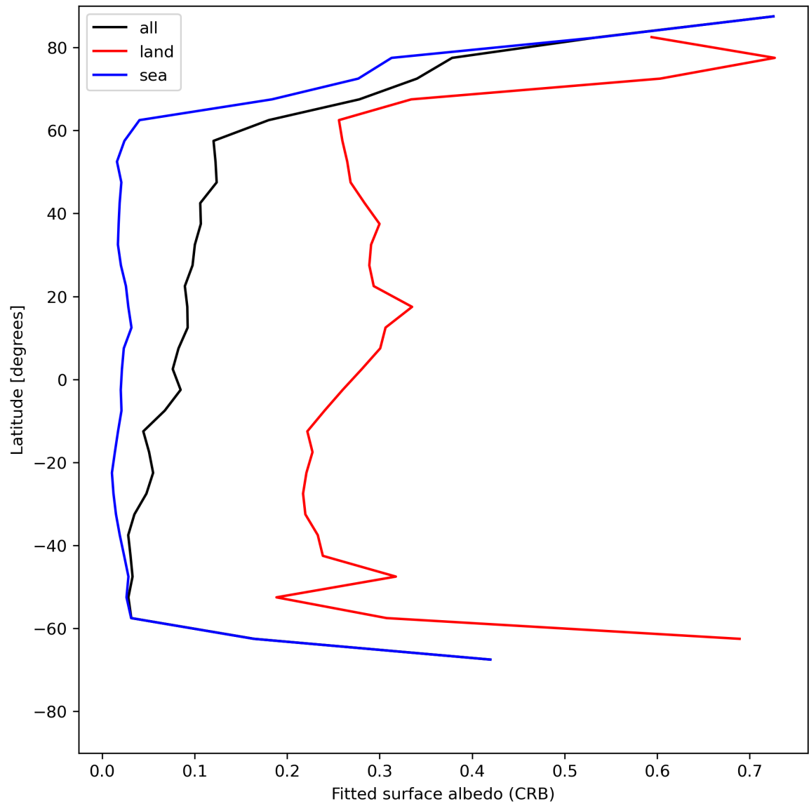
Figure 30: Zonal average of “Fitted surface albedo (CRB)” for 2024-06-27 to 2024-06-29.
