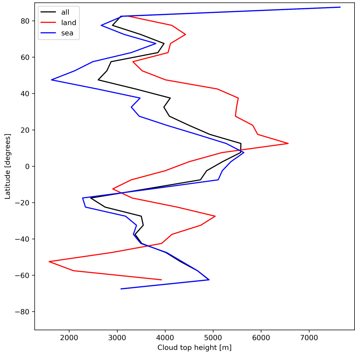
Figure 24: Zonal average of “Cloud top height” for 2024-06-27 to 2024-06-29.
