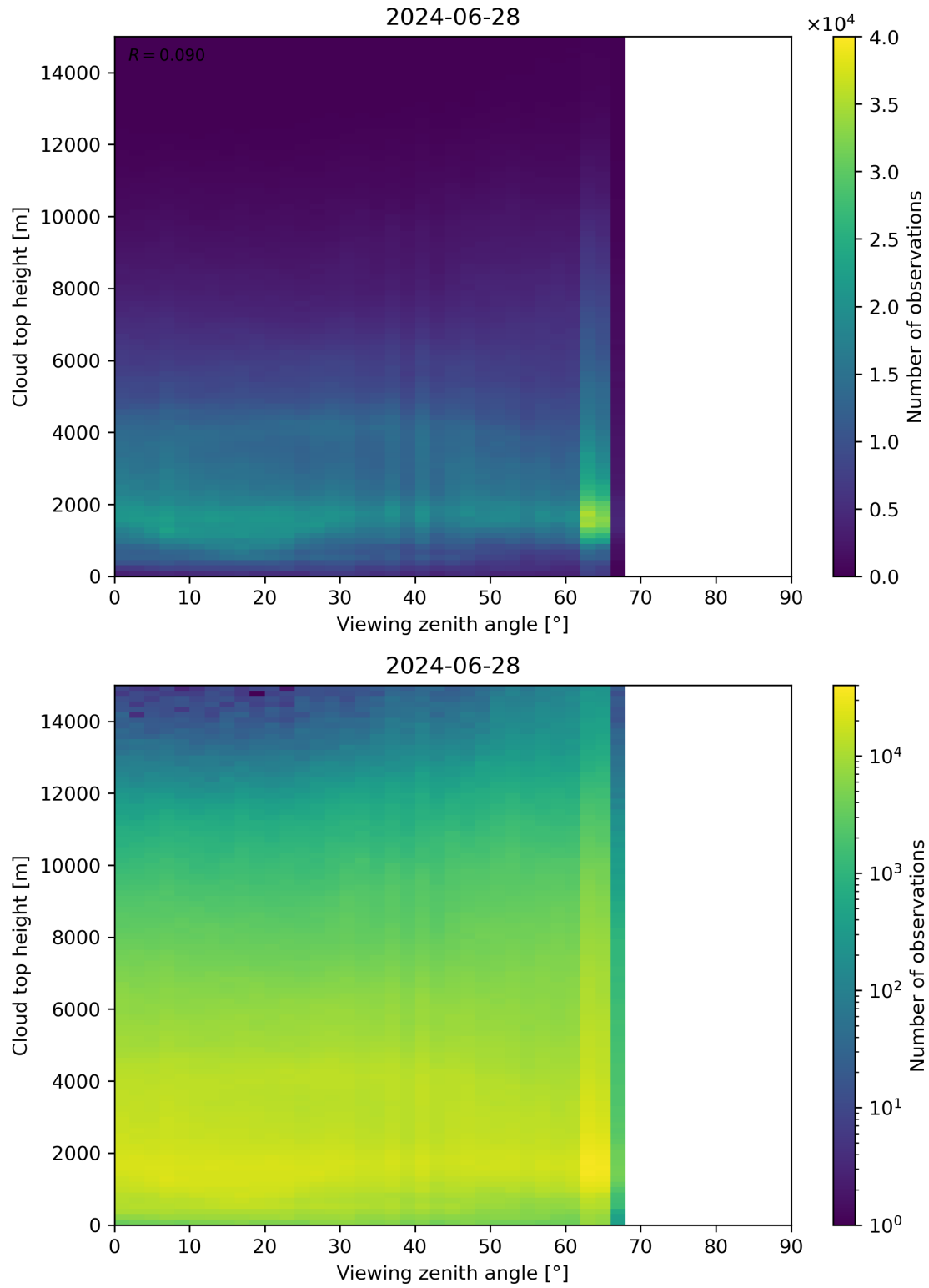
Figure 112: Scatter density plot of “Viewing zenith angle” against “Cloud top height” for 2024-06-27 to 2024-06-29.
