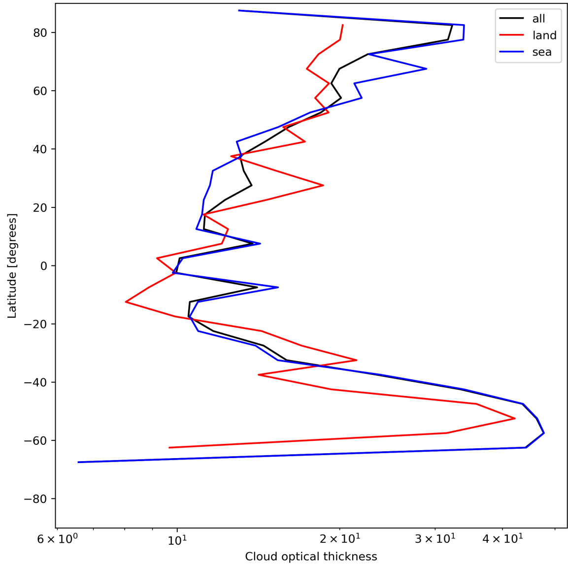
Figure 25: Zonal average of “Cloud optical thickness” for 2024-06-27 to 2024-06-29.
