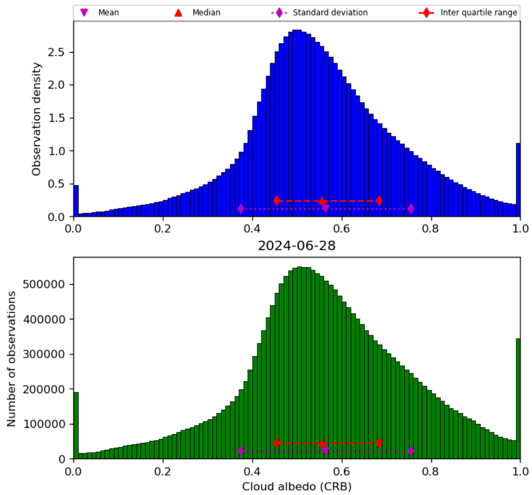
Figure 44: Histogram of “Cloud albedo (CRB)” for 2024-06-27 to 2024-06-29
