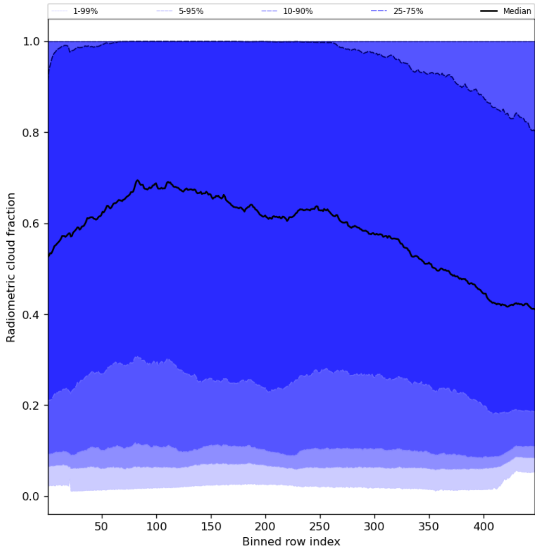
Figure 55: Along track statistics of “Radiometric cloud fraction” for 2024-06-27 to 2024-06-29
