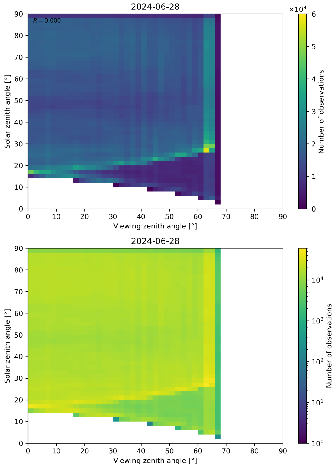
Figure 114: Scatter density plot of “Viewing zenith angle” against “Solar zenith angle” for 2024-06-27 to 2024-06-29.
