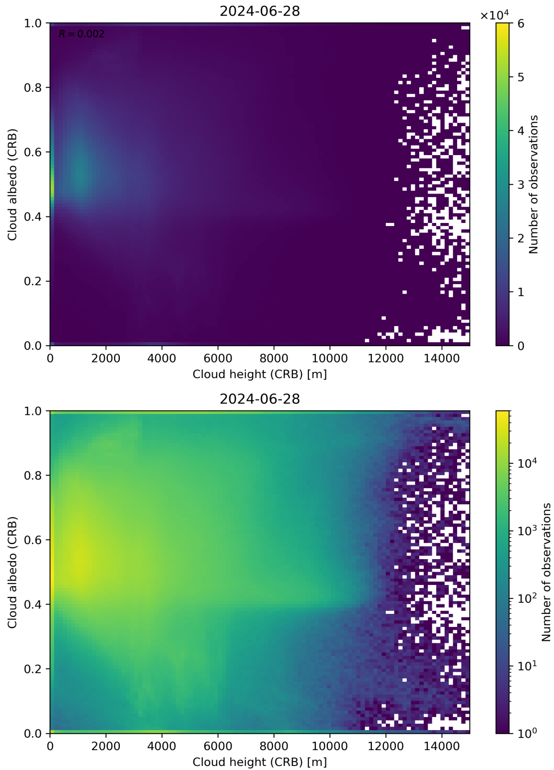
Figure 80: Scatter density plot of “Cloud height (CRB)” against “Cloud albedo (CRB)” for 2024-06-27 to 2024-06-29.
