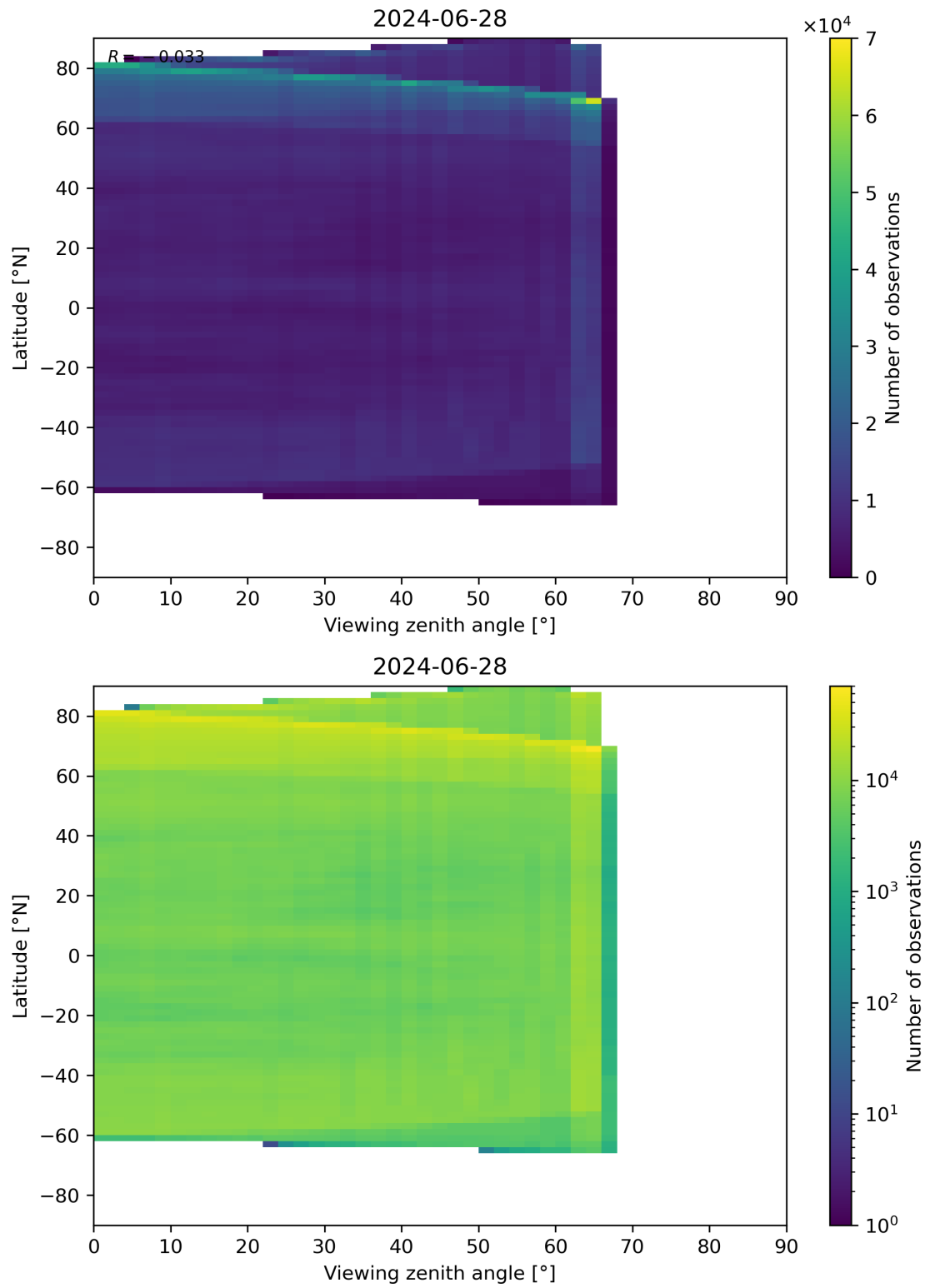
Figure 113: Scatter density plot of “Viewing zenith angle” against “Latitude” for 2024-06-27 to 2024-06-29.
