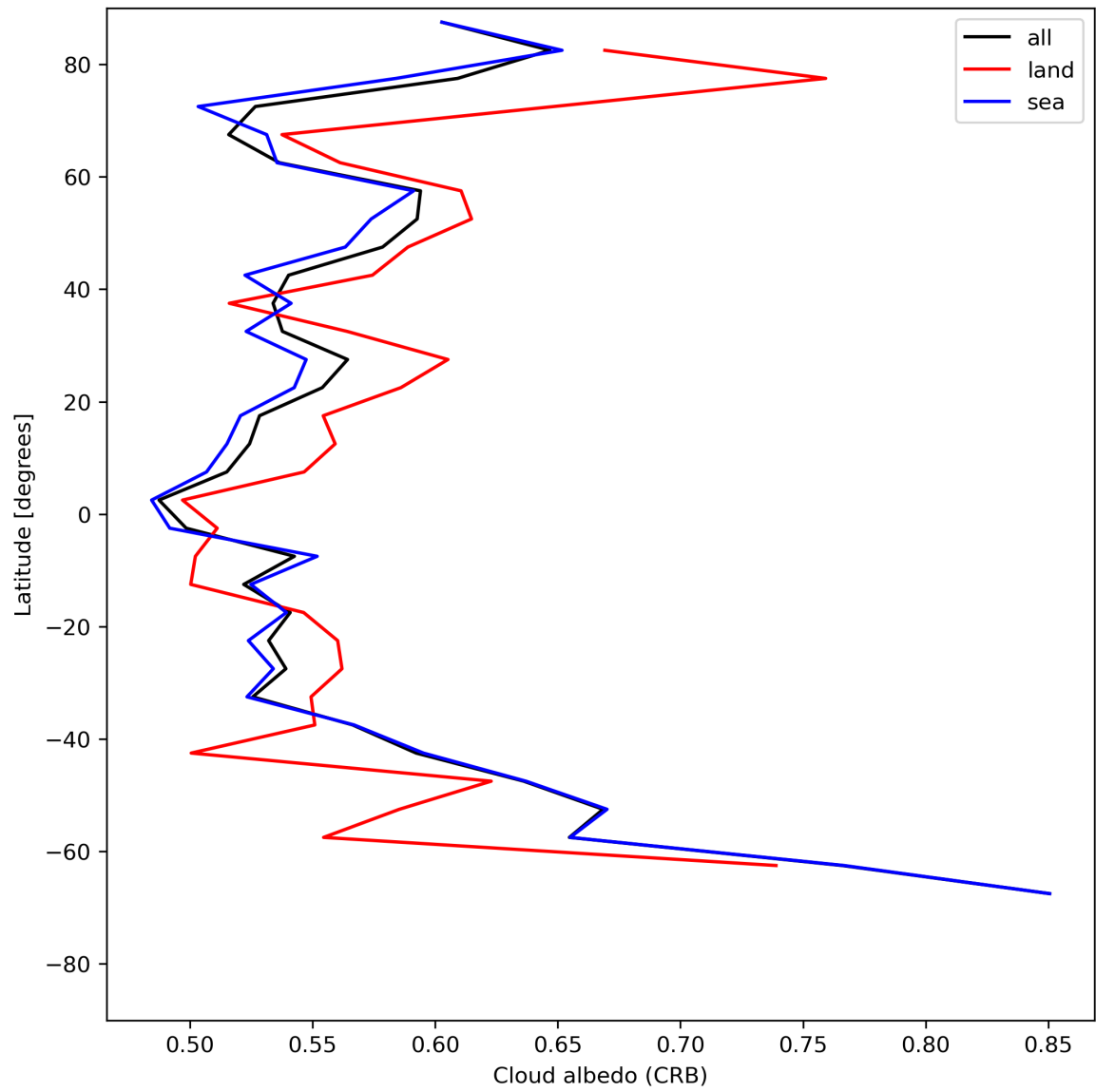
Figure 28: Zonal average of “Cloud albedo (CRB)” for 2024-06-27 to 2024-06-29.
