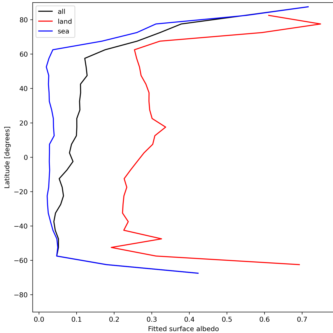
Figure 29: Zonal average of “Fitted surface albedo” for 2024-06-27 to 2024-06-29.
