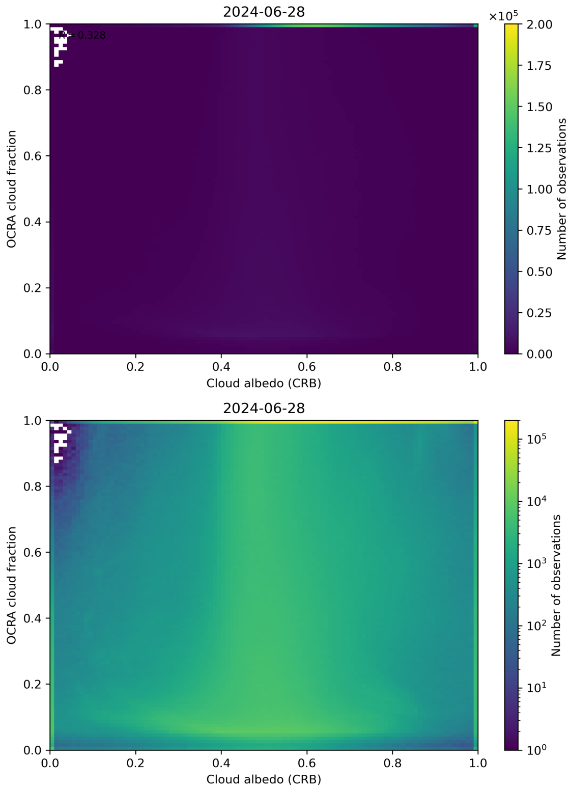
Figure 70: Scatter density plot of “Cloud albedo (CRB)” against “OCRA cloud fraction” for 2024-06-27 to 2024-06-29.
