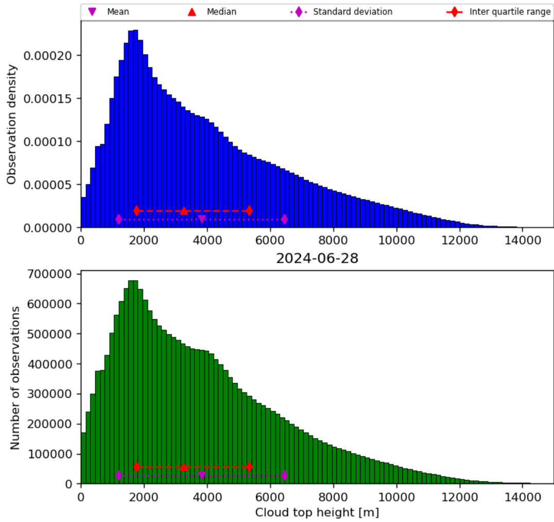
Figure 40: Histogram of “Cloud top height” for 2024-06-27 to 2024-06-29
