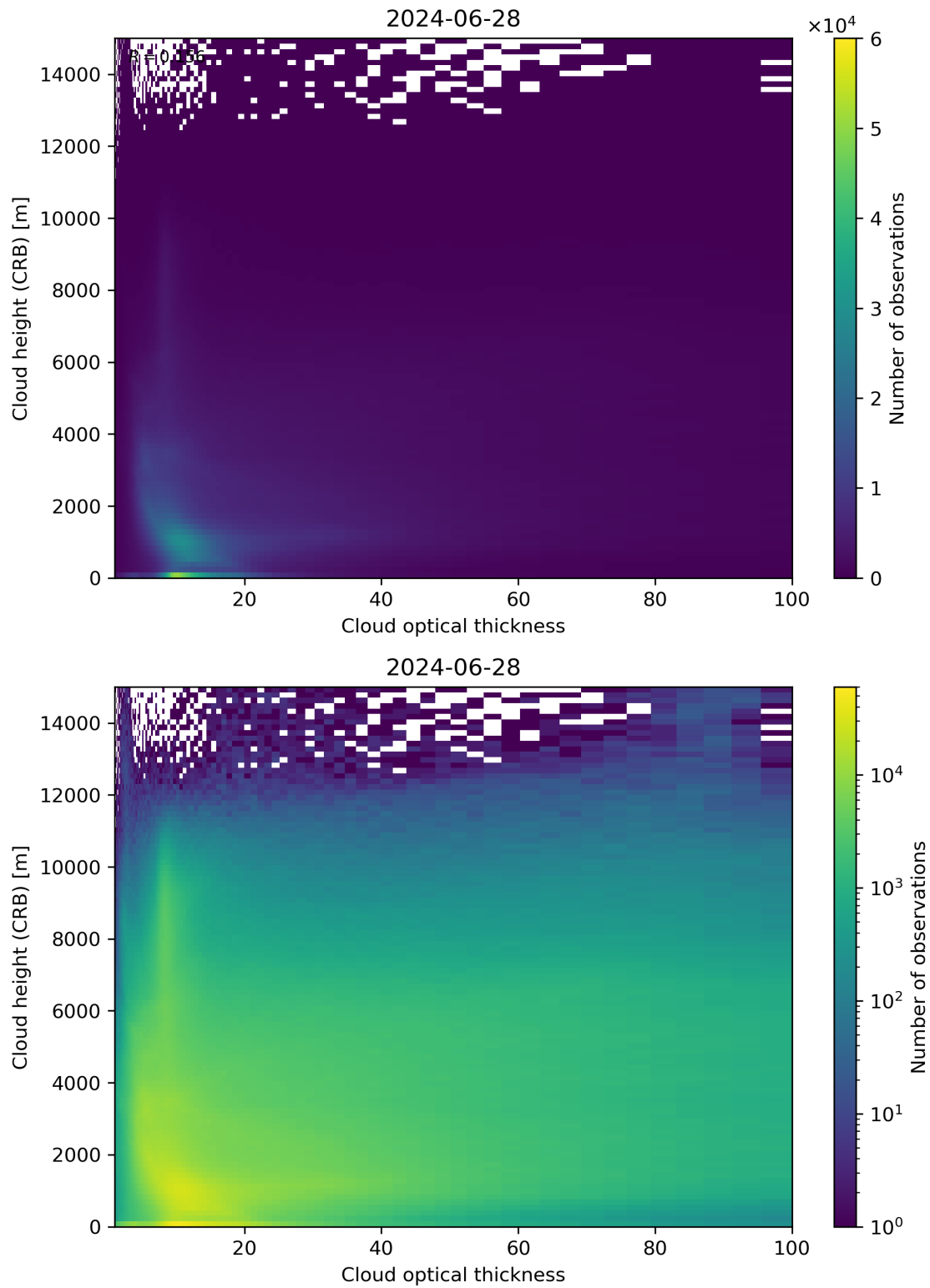
Figure 85: Scatter density plot of “Cloud optical thickness” against “Cloud height (CRB)” for 2024-06-27 to 2024-06-29.
