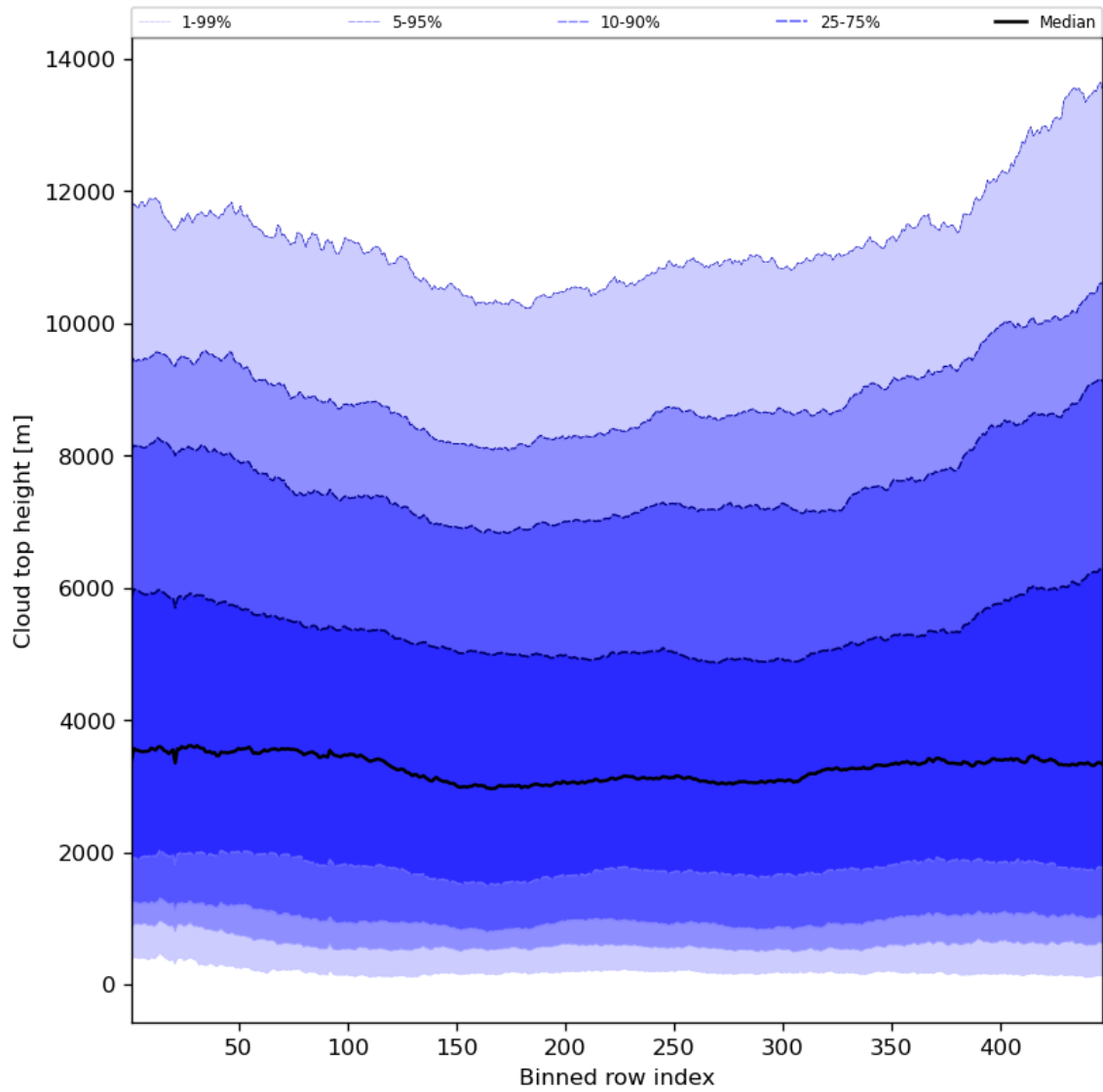
Figure 56: Along track statistics of “Cloud top height” for 2024-06-27 to 2024-06-29
