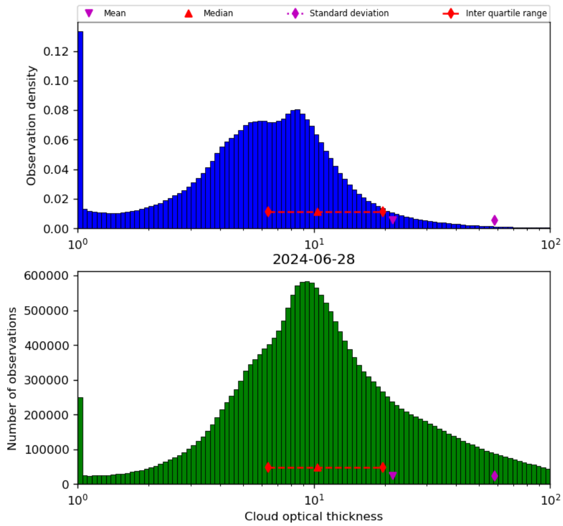
Figure 41: Histogram of “Cloud optical thickness” for 2024-06-27 to 2024-06-29
