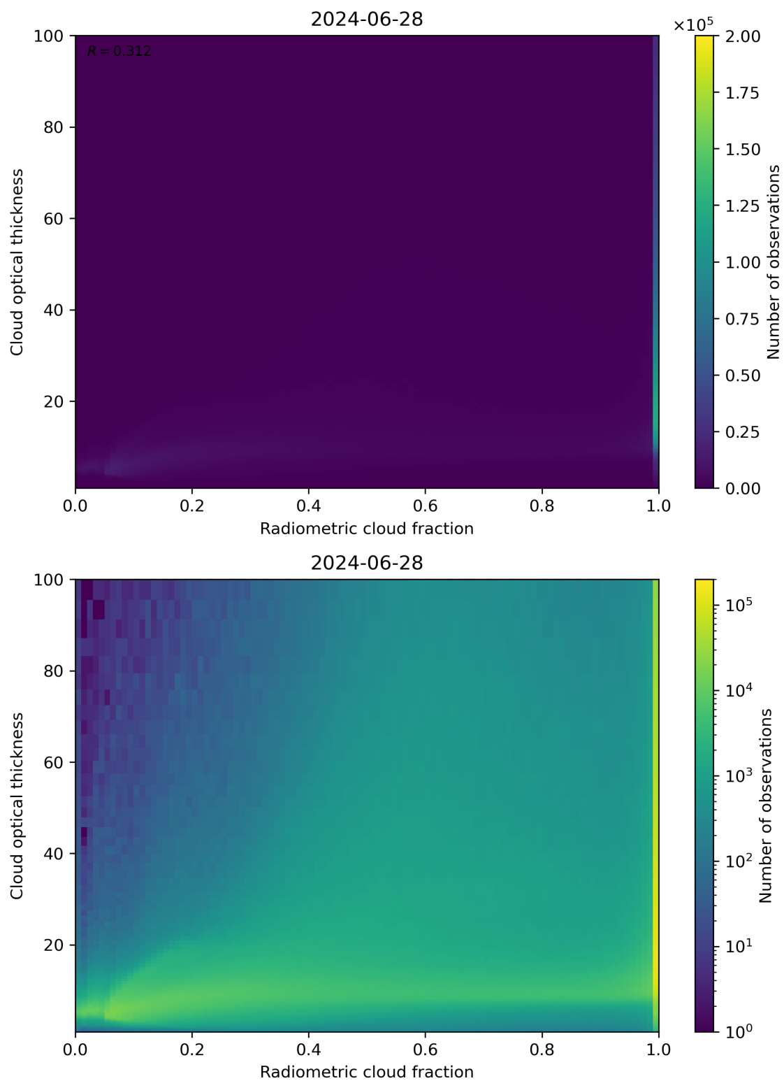
Figure 75: Scatter density plot of “Radiometric cloud fraction” against “Cloud optical thickness” for 2024-06-27 to 2024-06-29.
