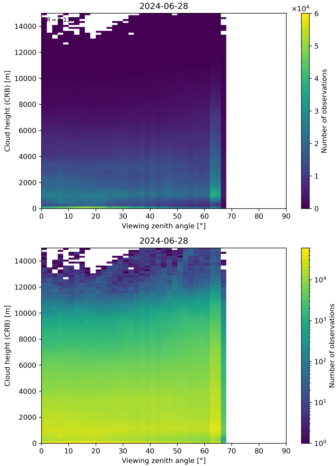
Figure 110: Scatter density plot of “Viewing zenith angle” against “Cloud height (CRB)” for 2024-06-27 to 2024-06-29.
