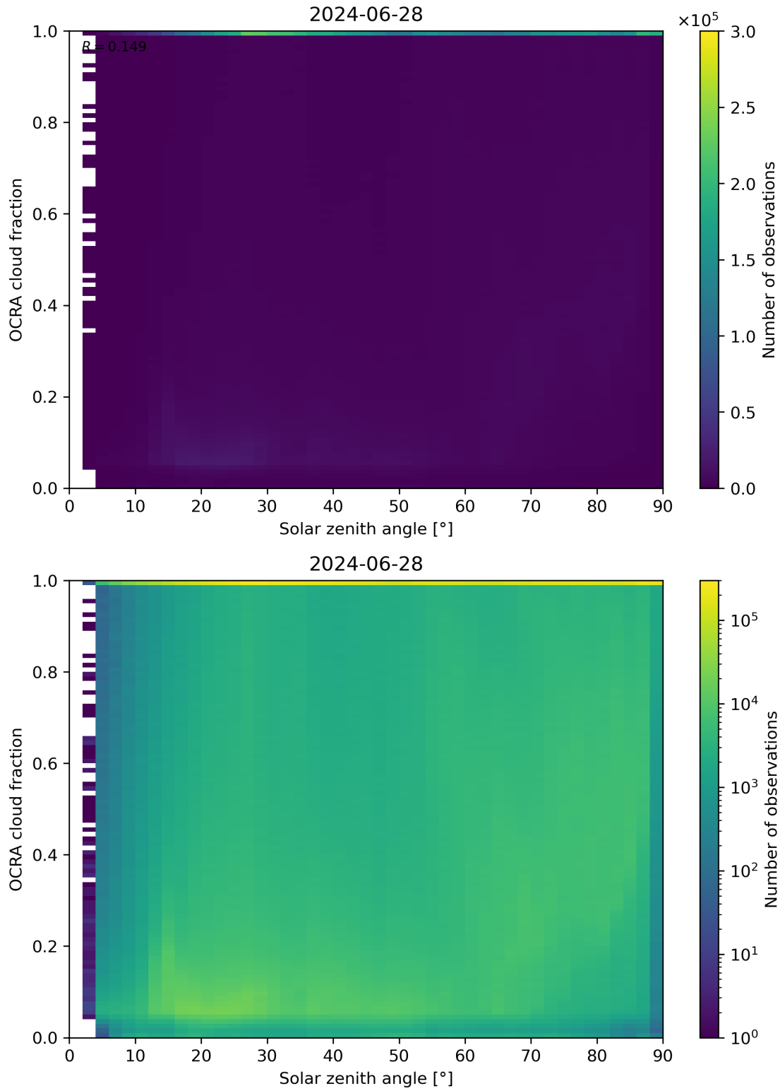
Figure 100: Scatter density plot of “Solar zenith angle” against “OCRA cloud fraction” for 2024-06-27 to 2024-06-29.
