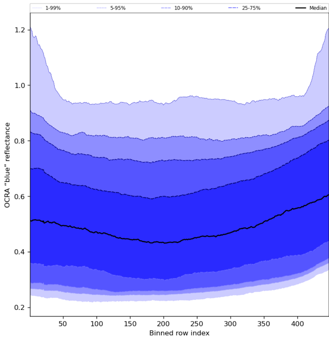
Figure 67: Along track statistics of “OCRA “blue” reflectance” for 2024-06-27 to 2024-06-29
