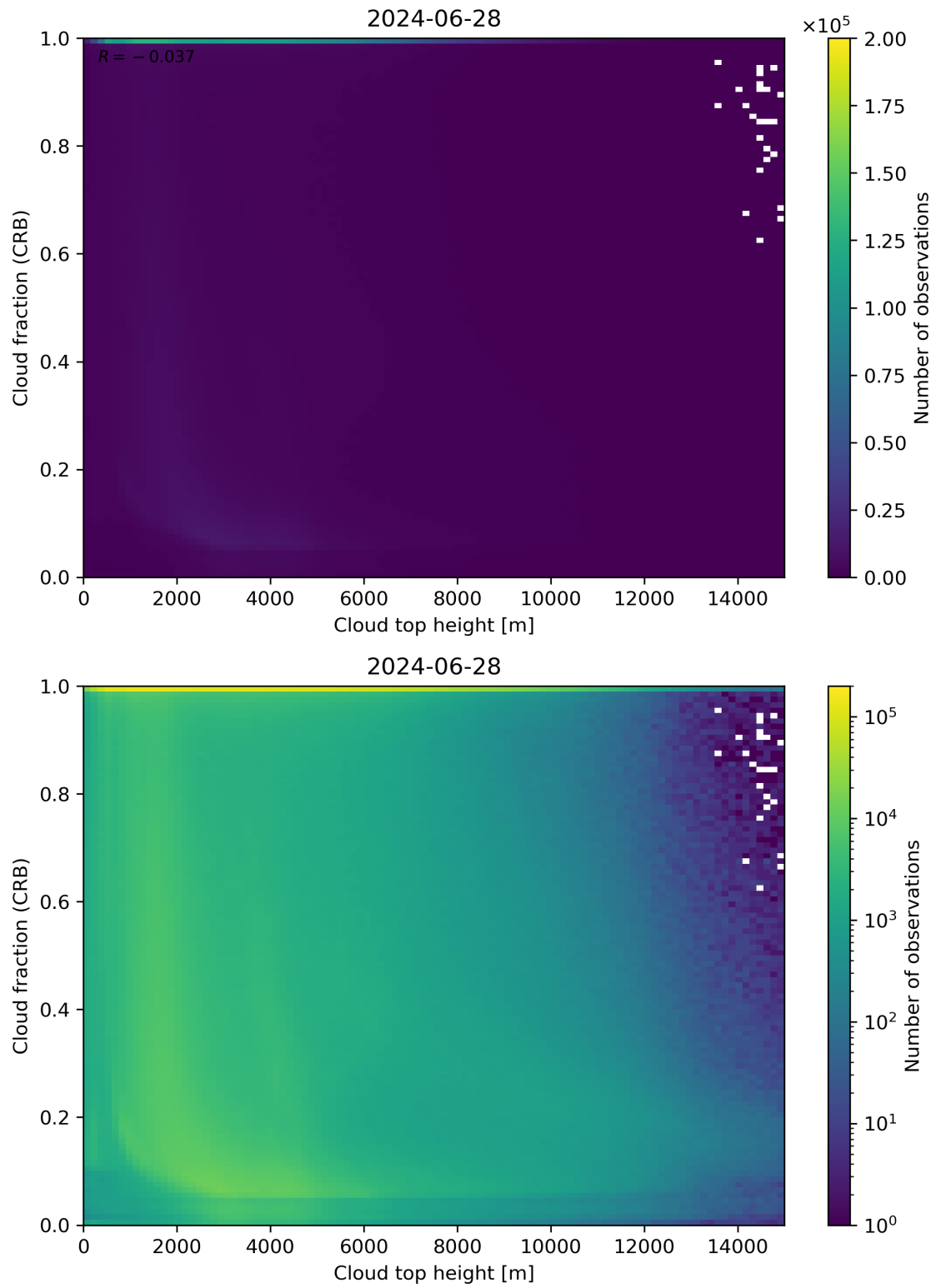
Figure 88: Scatter density plot of “Cloud top height” against “Cloud fraction (CRB)” for 2024-06-27 to 2024-06-29.
