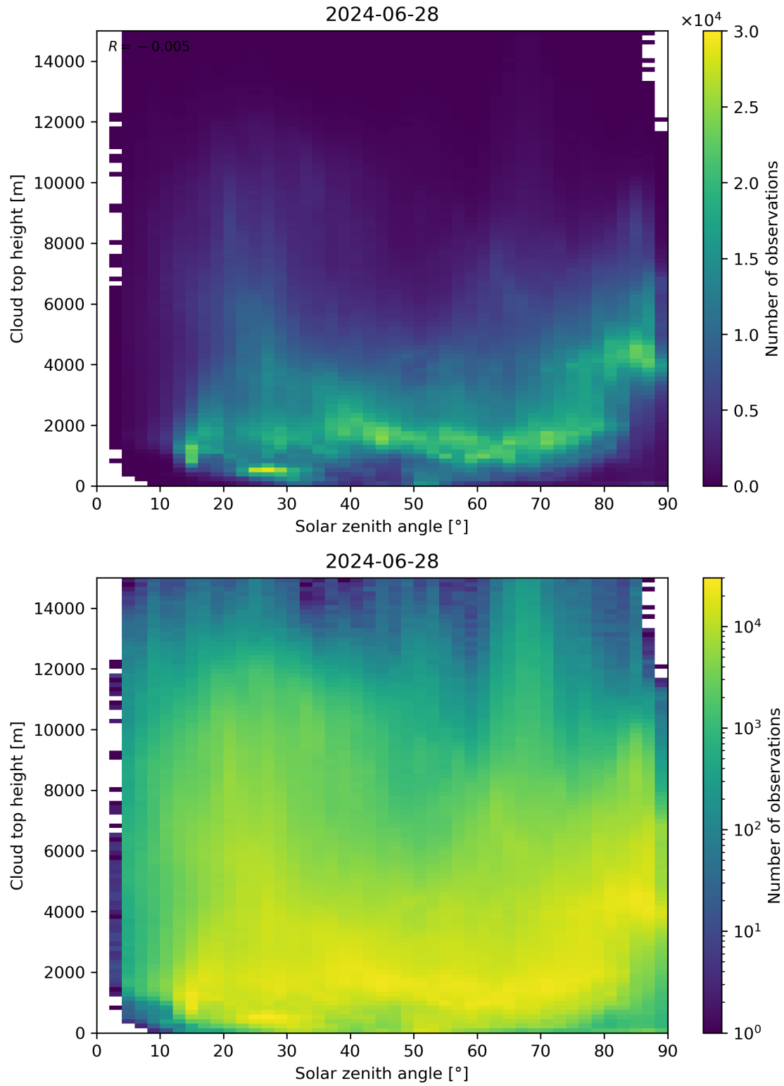
Figure 104: Scatter density plot of “Solar zenith angle” against “Cloud top height” for 2024-06-27 to 2024-06-29.
