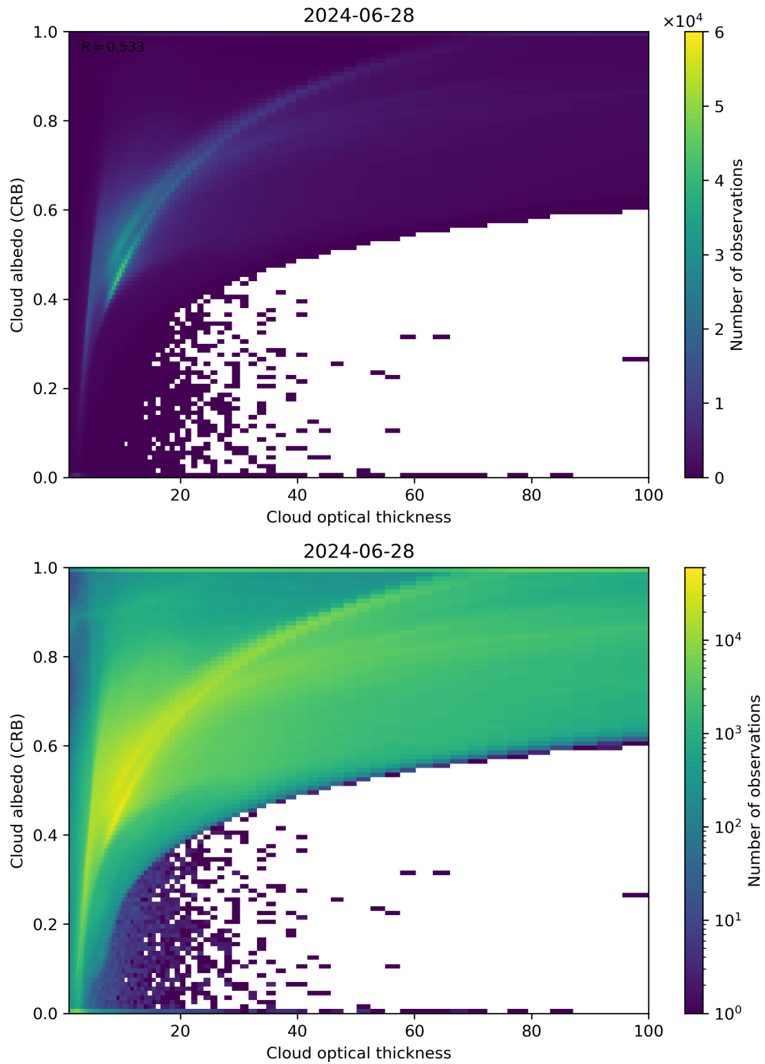
Figure 82: Scatter density plot of “Cloud optical thickness” against “Cloud albedo (CRB)” for 2024-06-27 to 2024-06-29.
