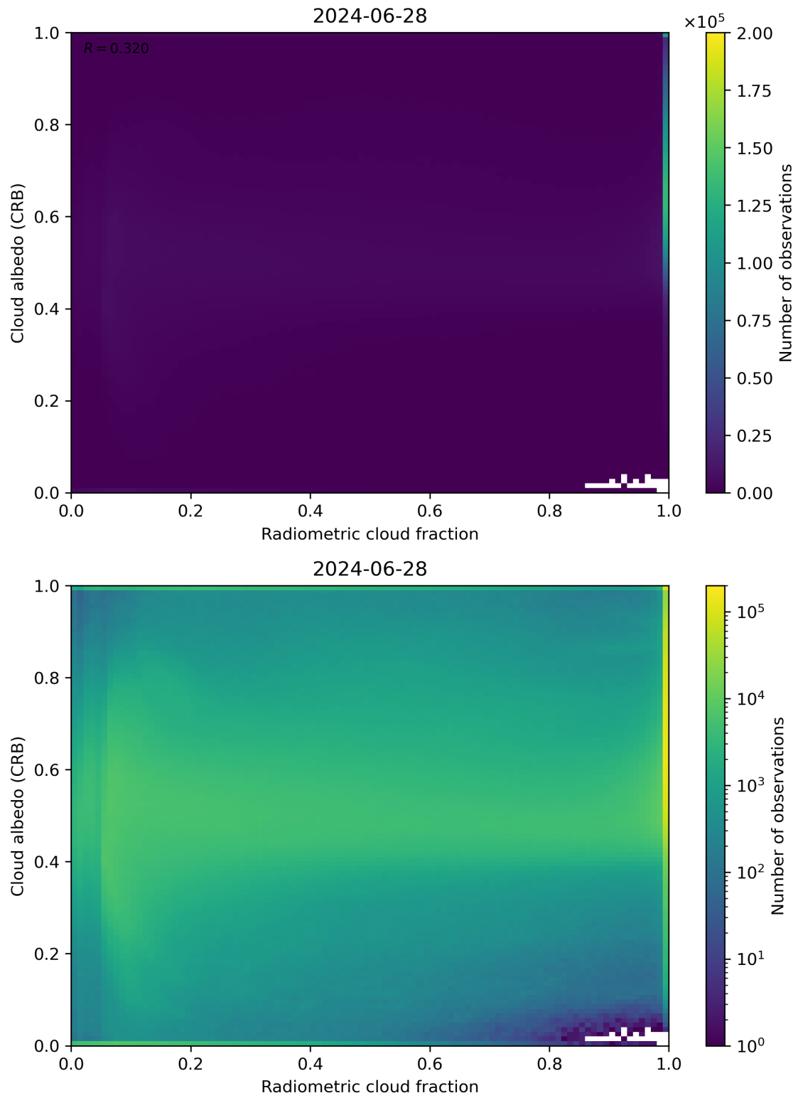
Figure 71: Scatter density plot of “Radiometric cloud fraction” against “Cloud albedo (CRB)” for 2024-06-27 to 2024-06-29.
