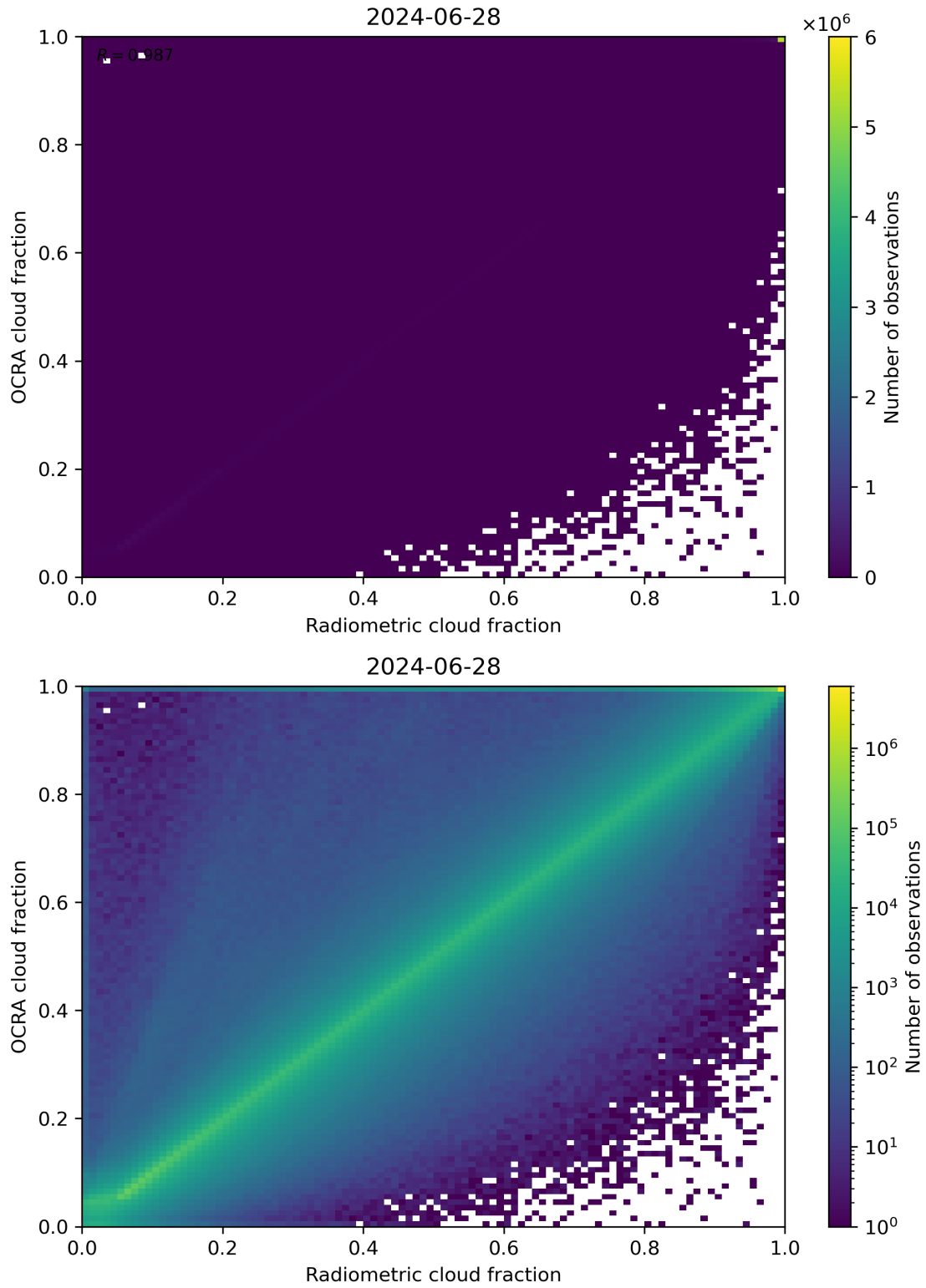
Figure 72: Scatter density plot of “Radiometric cloud fraction” against “OCRA cloud fraction” for 2024-06-27 to 2024-06-29.
