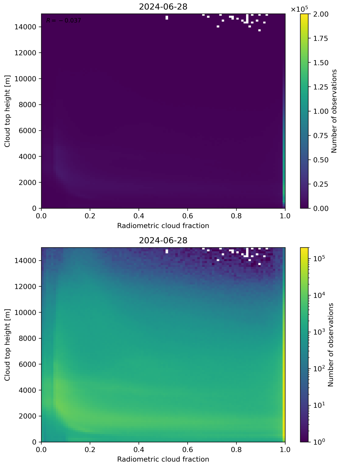
Figure 76: Scatter density plot of “Radiometric cloud fraction” against “Cloud top height” for 2024-06-27 to 2024-06-29.
