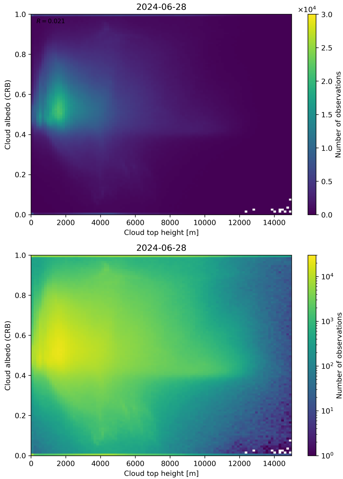
Figure 86: Scatter density plot of “Cloud top height” against “Cloud albedo (CRB)” for 2024-06-27 to 2024-06-29.
