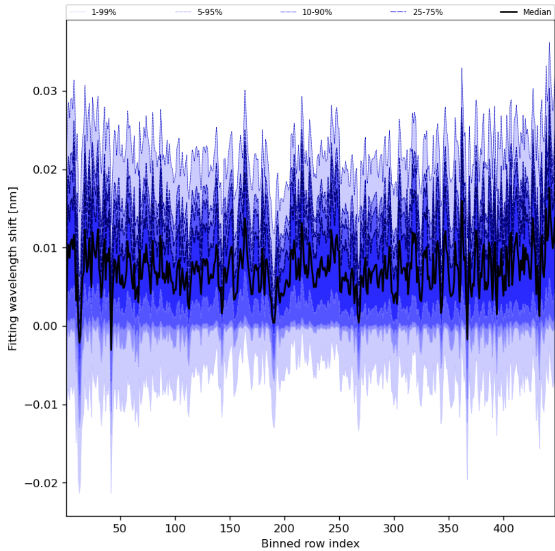
Figure 65: Along track statistics of “Fitting wavelength shift” for 2024-06-27 to 2024-06-29
