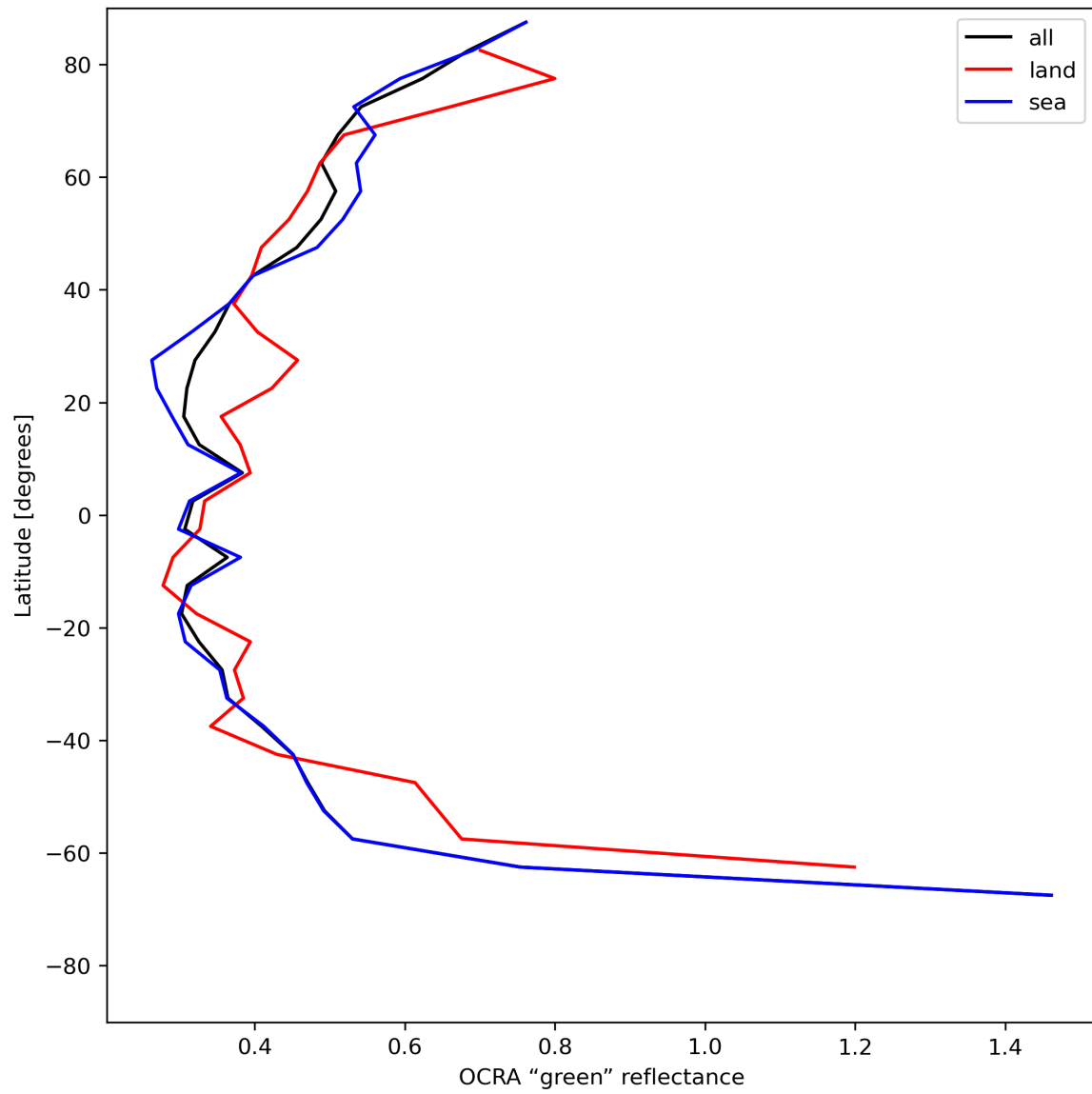
Figure 36: Zonal average of “OCRA “green” reflectance” for 2024-06-27 to 2024-06-29.
