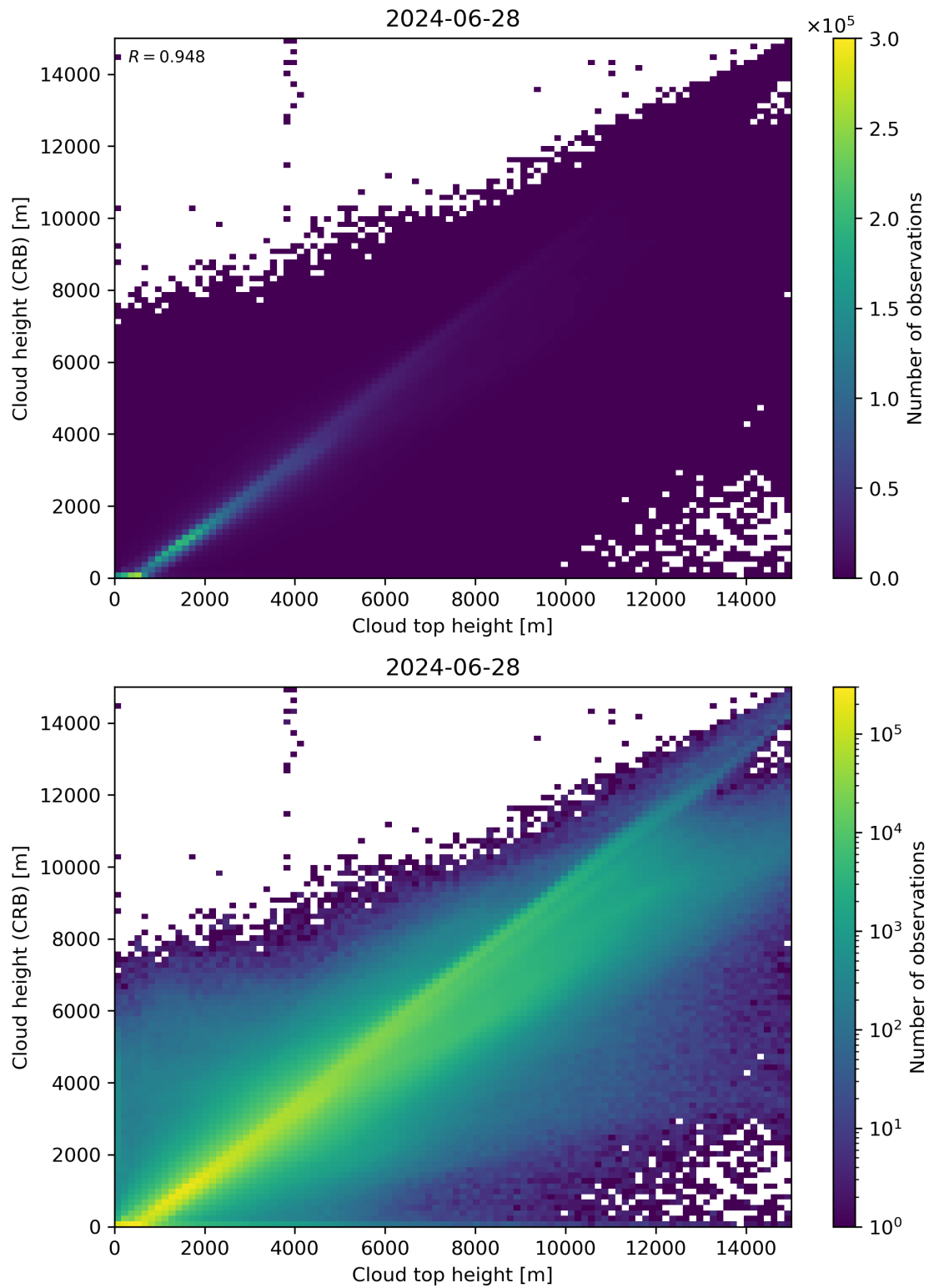
Figure 89: Scatter density plot of “Cloud top height” against “Cloud height (CRB)” for 2024-06-27 to 2024-06-29.
