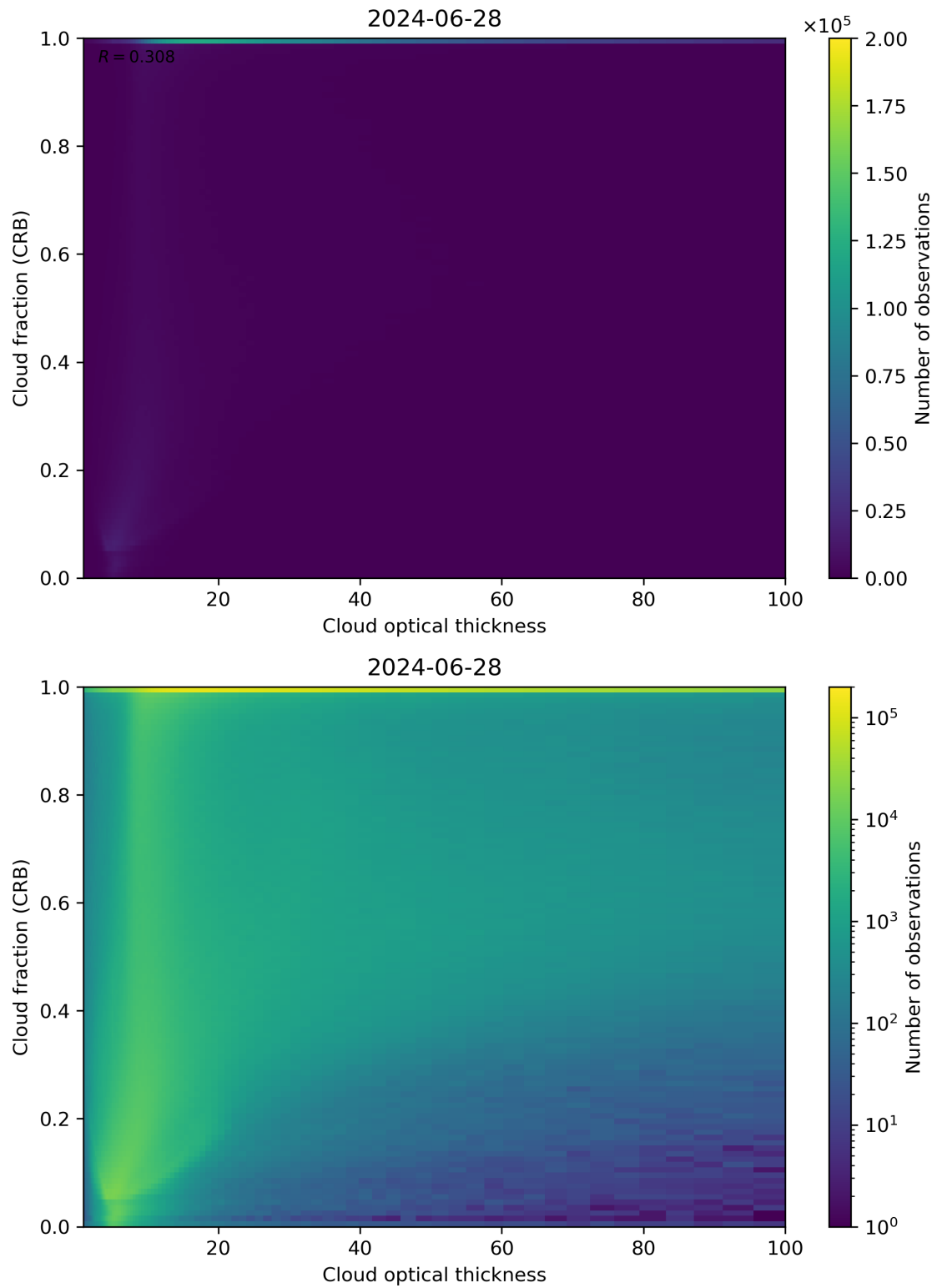
Figure 84: Scatter density plot of “Cloud optical thickness” against “Cloud fraction (CRB)” for 2024-06-27 to 2024-06-29.
