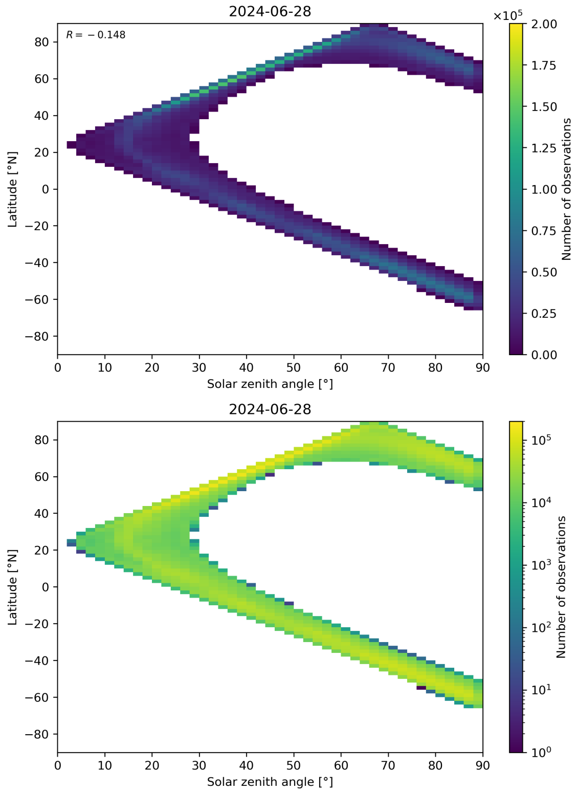
Figure 105: Scatter density plot of “Solar zenith angle” against “Latitude” for 2024-06-27 to 2024-06-29.
