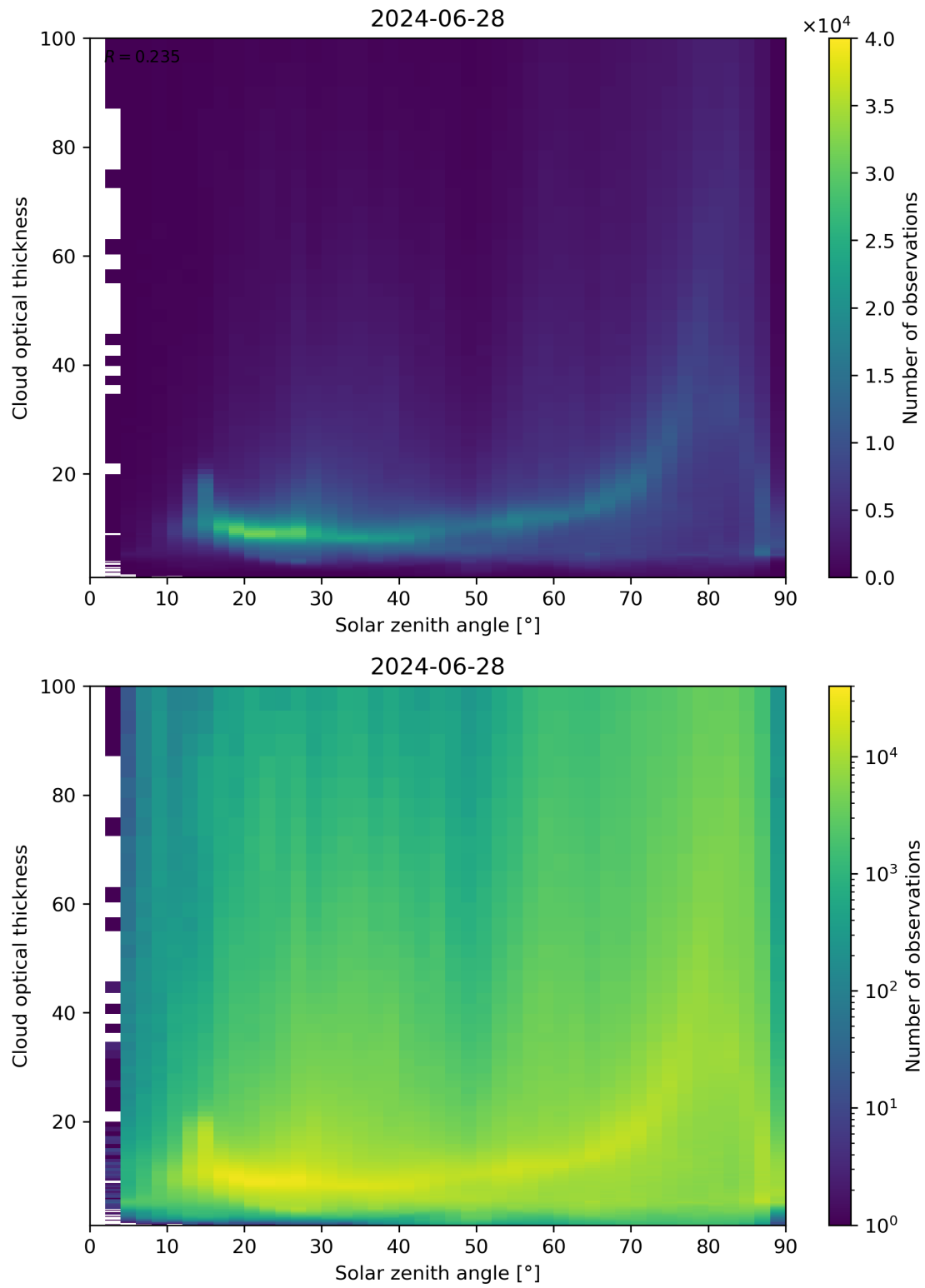
Figure 103: Scatter density plot of “Solar zenith angle” against “Cloud optical thickness” for 2024-06-27 to 2024-06-29.
