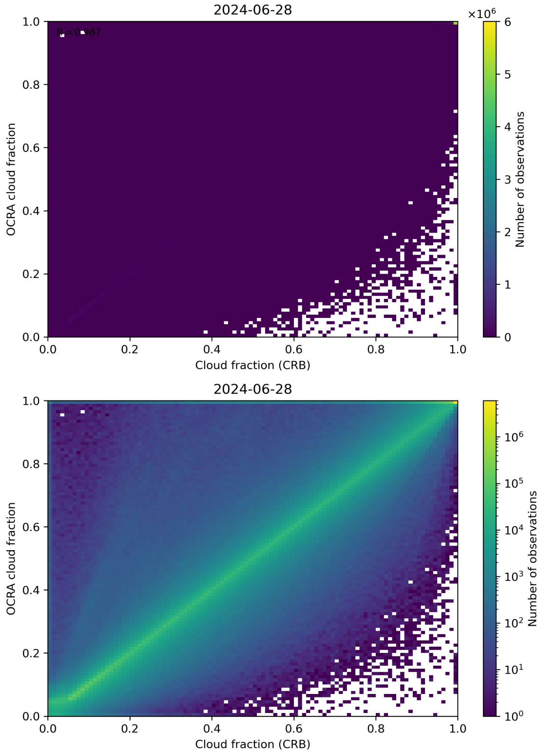
Figure 78: Scatter density plot of “Cloud fraction (CRB)” against “OCRA cloud fraction” for 2024-06-27 to 2024-06-29.
