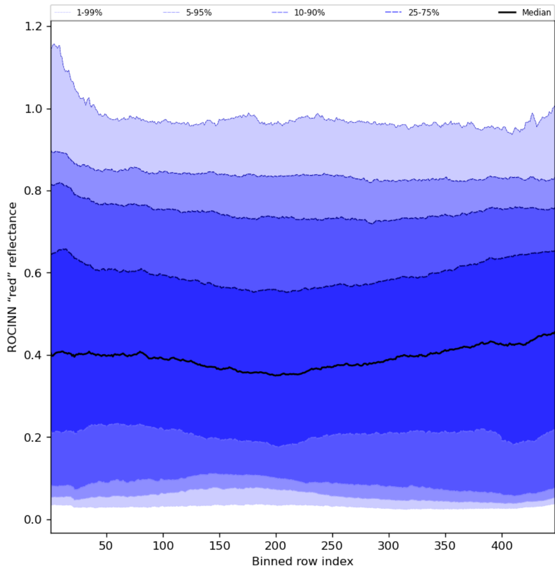
Figure 69: Along track statistics of “ROCINN “red” reflectance” for 2024-06-27 to 2024-06-29
