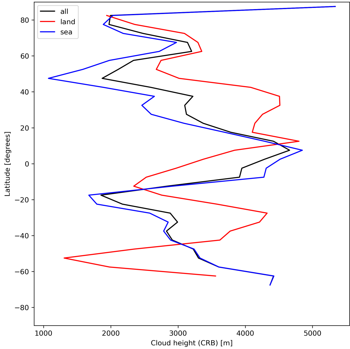
Figure 27: Zonal average of “Cloud height (CRB)” for 2024-06-27 to 2024-06-29.
