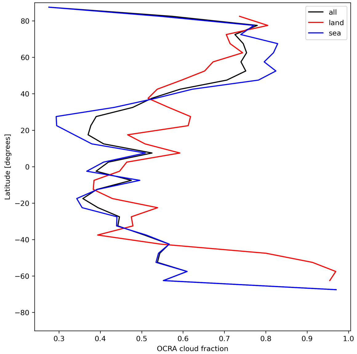
Figure 34: Zonal average of “OCRA cloud fraction” for 2024-06-27 to 2024-06-29.
