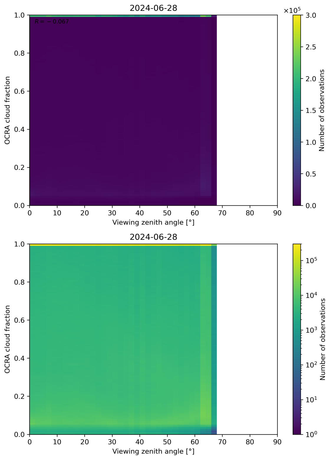
Figure 108: Scatter density plot of “Viewing zenith angle” against “OCRA cloud fraction” for 2024-06-27 to 2024-06-29.
