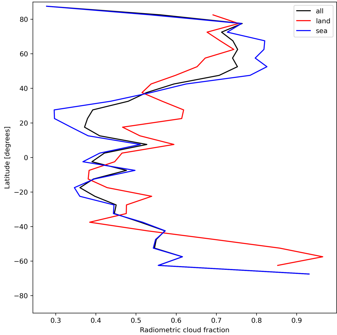
Figure 23: Zonal average of “Radiometric cloud fraction” for 2024-06-27 to 2024-06-29.
