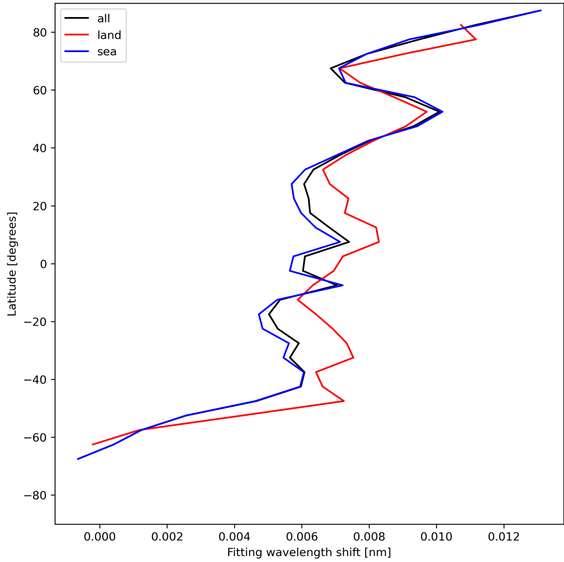
Figure 33: Zonal average of “Fitting wavelength shift” for 2024-06-27 to 2024-06-29.
