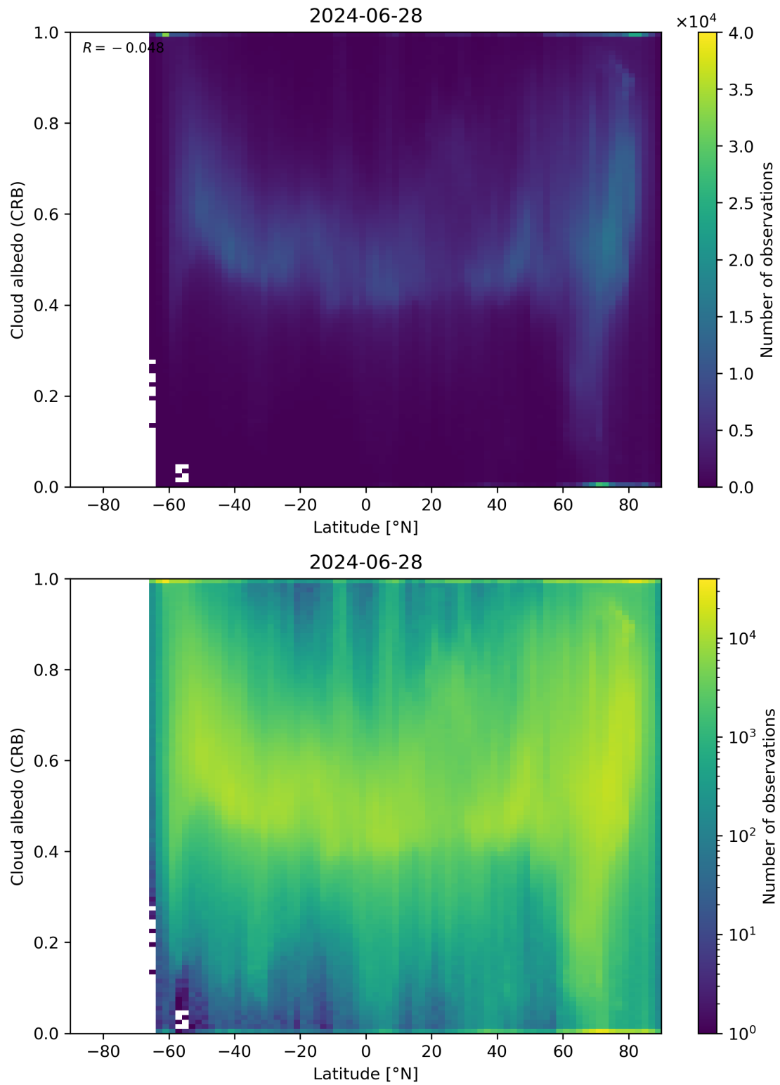
Figure 91: Scatter density plot of “Latitude” against “Cloud albedo (CRB)” for 2024-06-27 to 2024-06-29.
