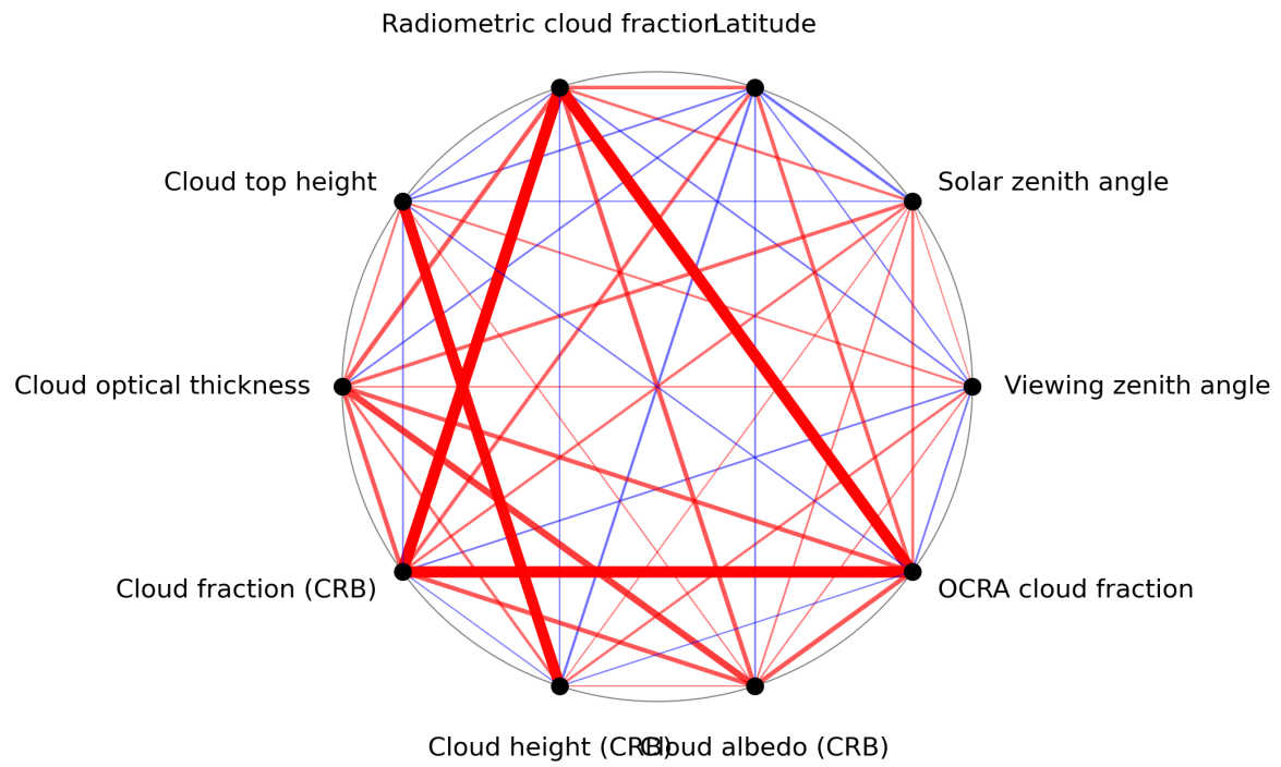
Figure 1: Map of correlation graph for 2024-06-27 to 2024-06-29.
