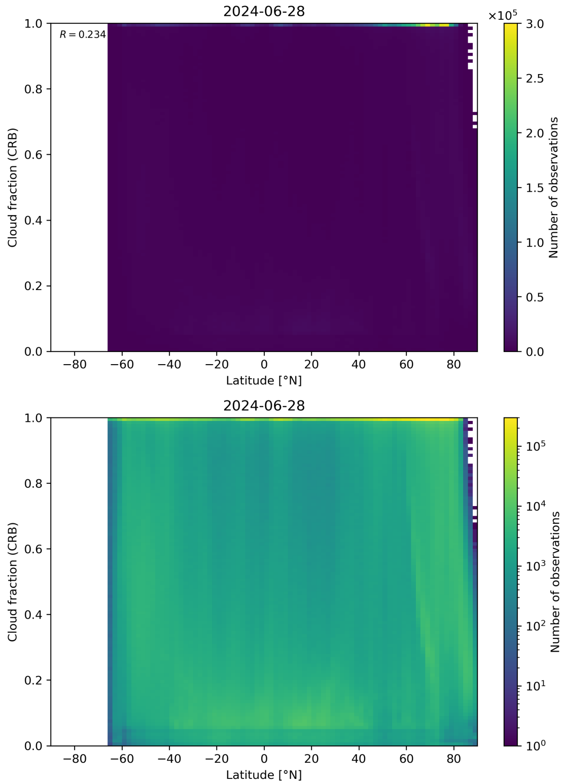
Figure 94: Scatter density plot of “Latitude” against “Cloud fraction (CRB)” for 2024-06-27 to 2024-06-29.
