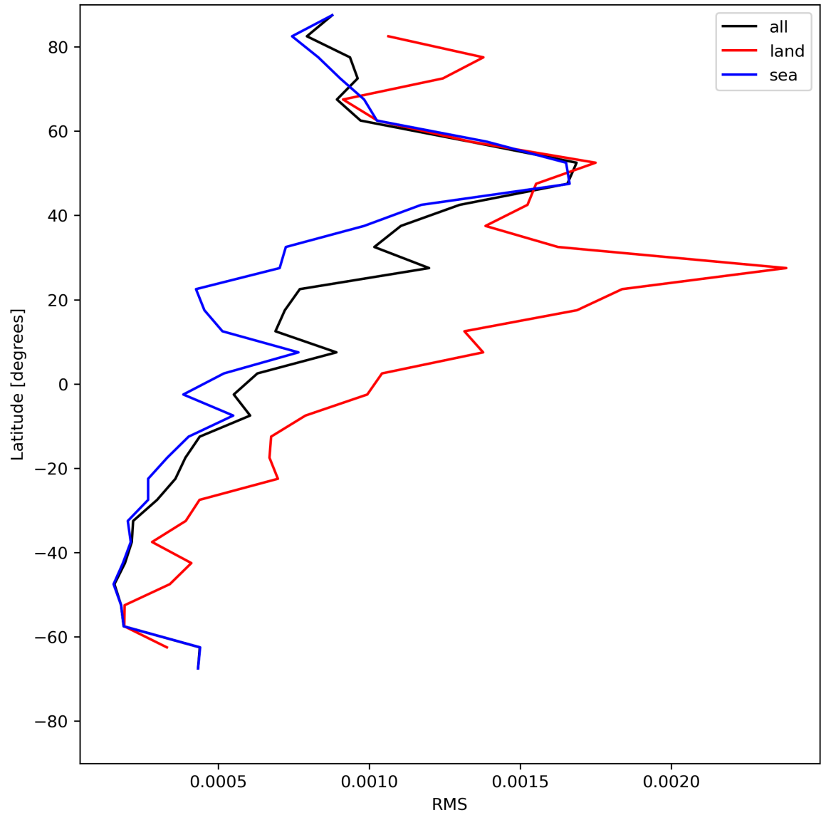
Figure 31: Zonal average of “RMS” for 2024-06-27 to 2024-06-29.
