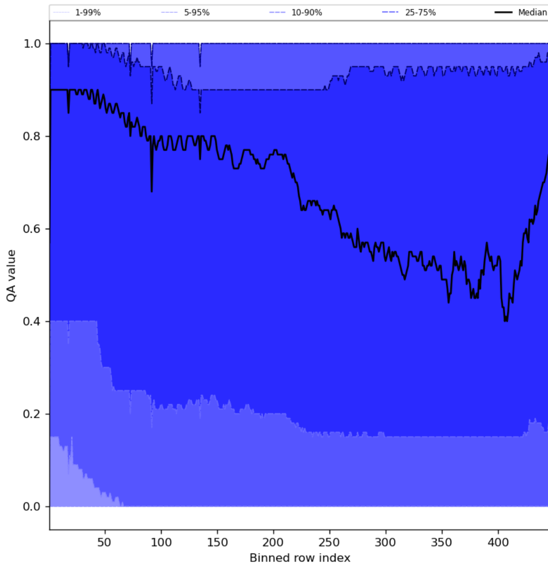
Figure 54: Along track statistics of “QA value” for 2024-06-27 to 2024-06-29
