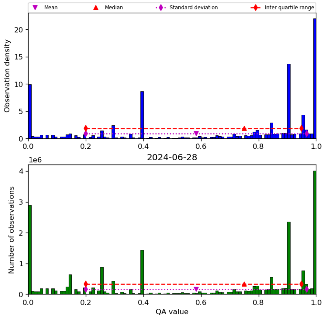
Figure 38: Histogram of “QA value” for 2024-06-27 to 2024-06-29
