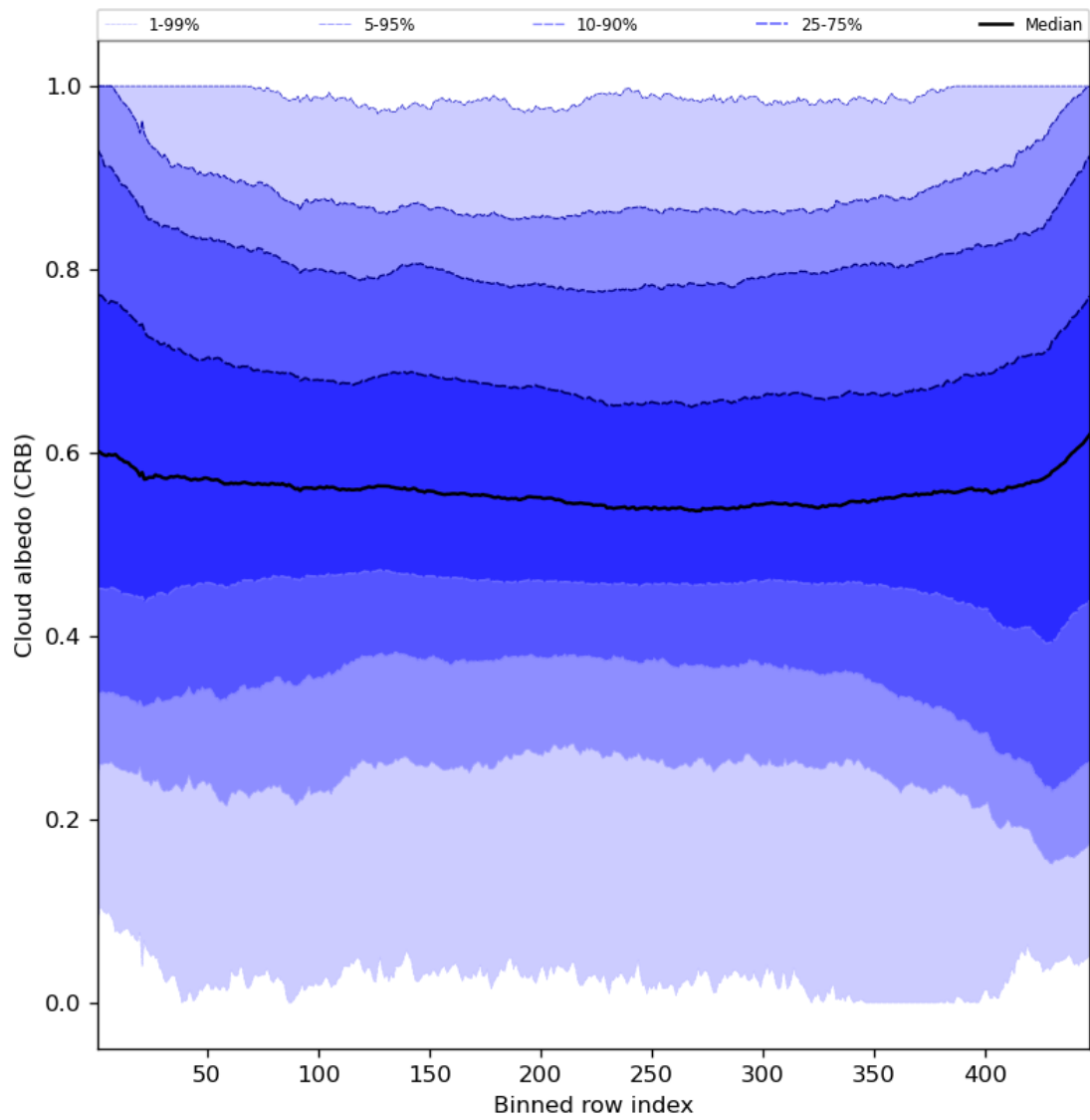
Figure 60: Along track statistics of “Cloud albedo (CRB)” for 2024-06-27 to 2024-06-29
