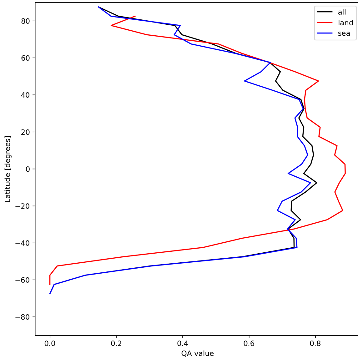
Figure 22: Zonal average of “QA value” for 2024-06-27 to 2024-06-29.
