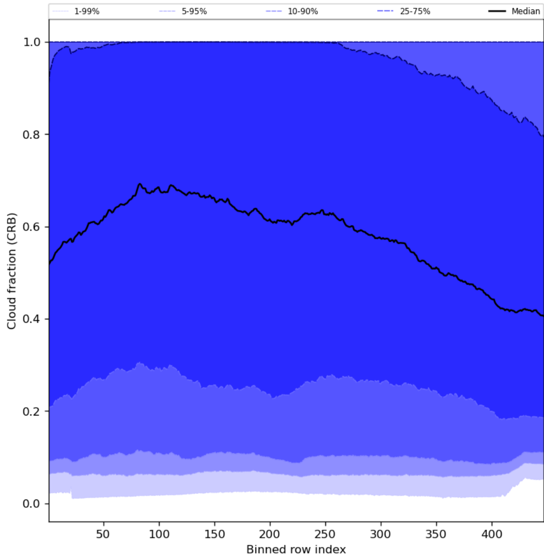
Figure 58: Along track statistics of “Cloud fraction (CRB)” for 2024-06-27 to 2024-06-29
