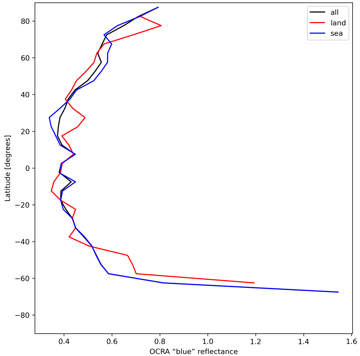
Figure 35: Zonal average of “OCRA “blue” reflectance” for 2024-06-27 to 2024-06-29.
