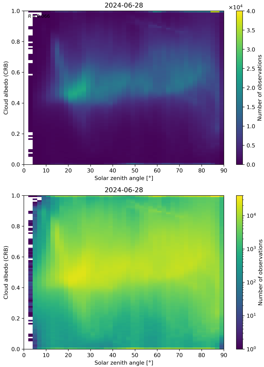
Figure 98: Scatter density plot of “Solar zenith angle” against “Cloud albedo (CRB)” for 2024-06-27 to 2024-06-29.
