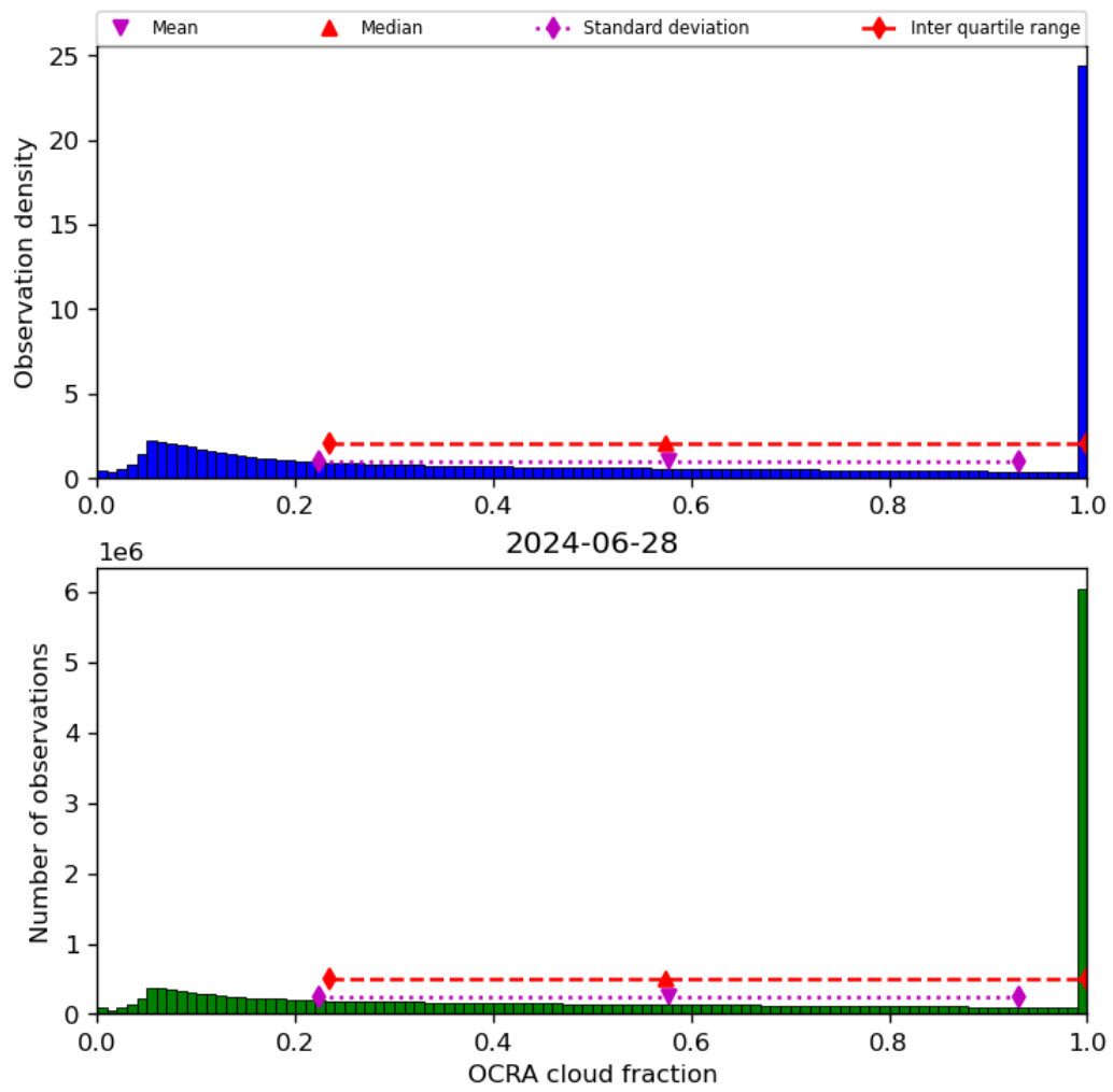
Figure 50: Histogram of “OCRA cloud fraction” for 2024-06-27 to 2024-06-29
