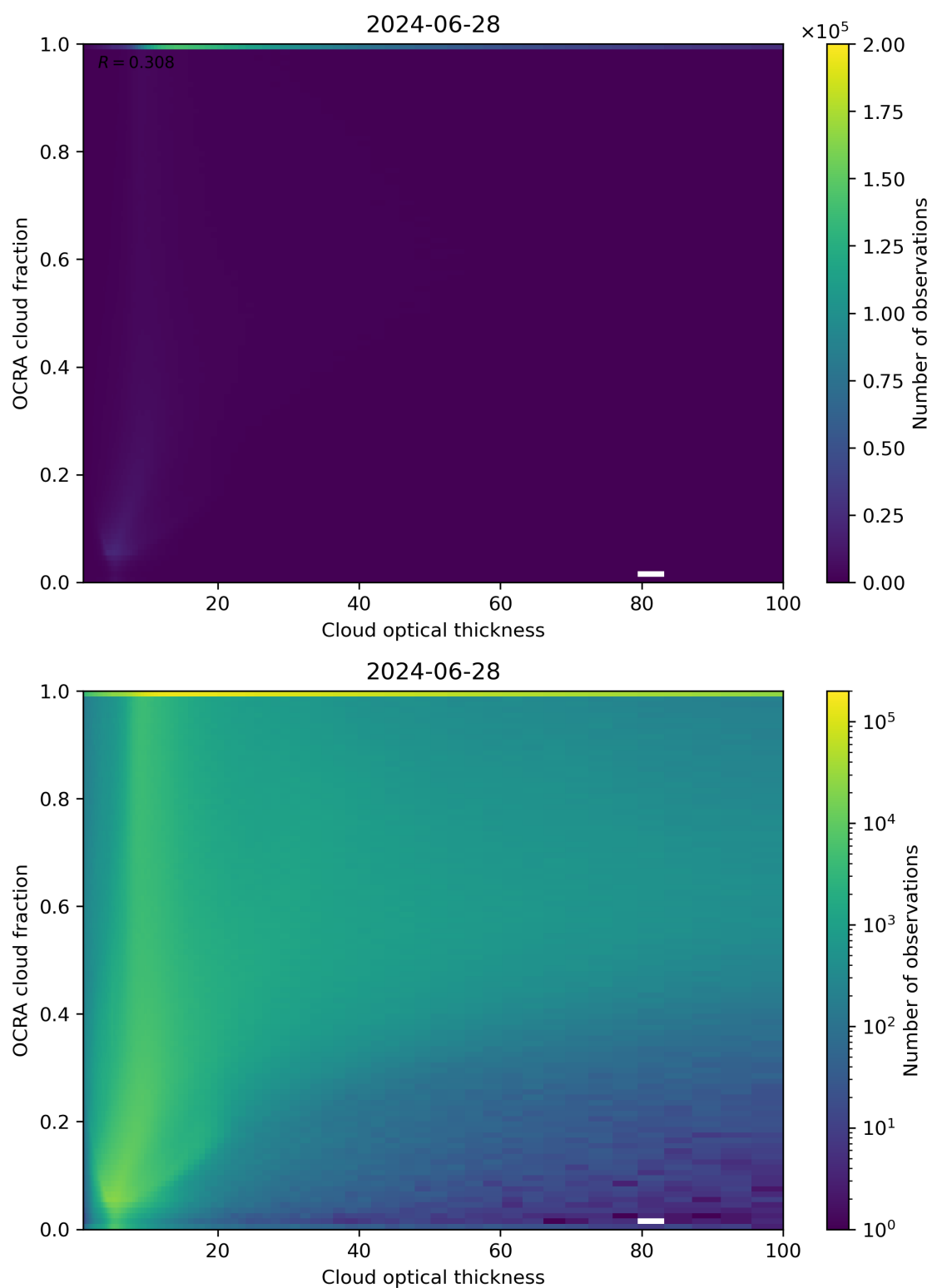
Figure 83: Scatter density plot of “Cloud optical thickness” against “OCRA cloud fraction” for 2024-06-27 to 2024-06-29.
