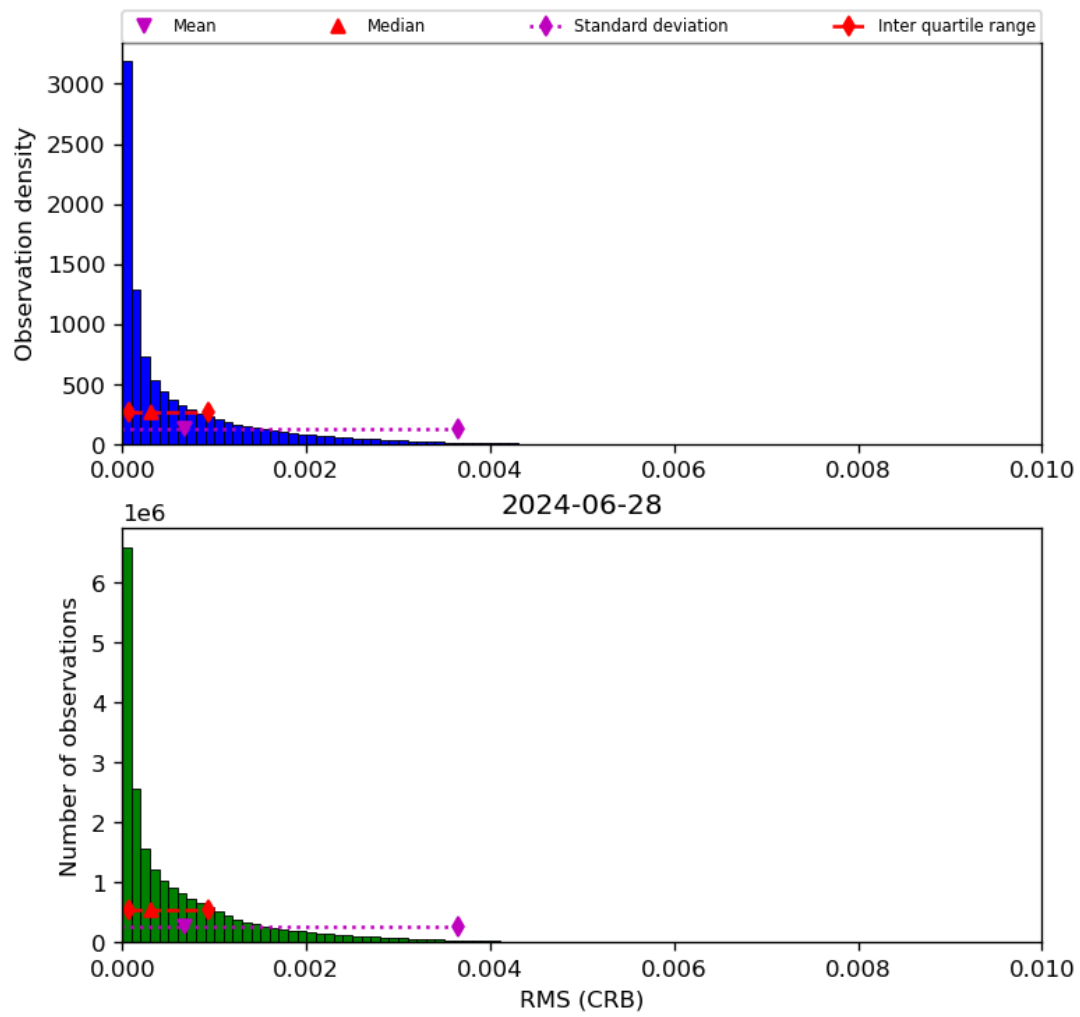
Figure 48: Histogram of “RMS (CRB)” for 2024-06-27 to 2024-06-29
