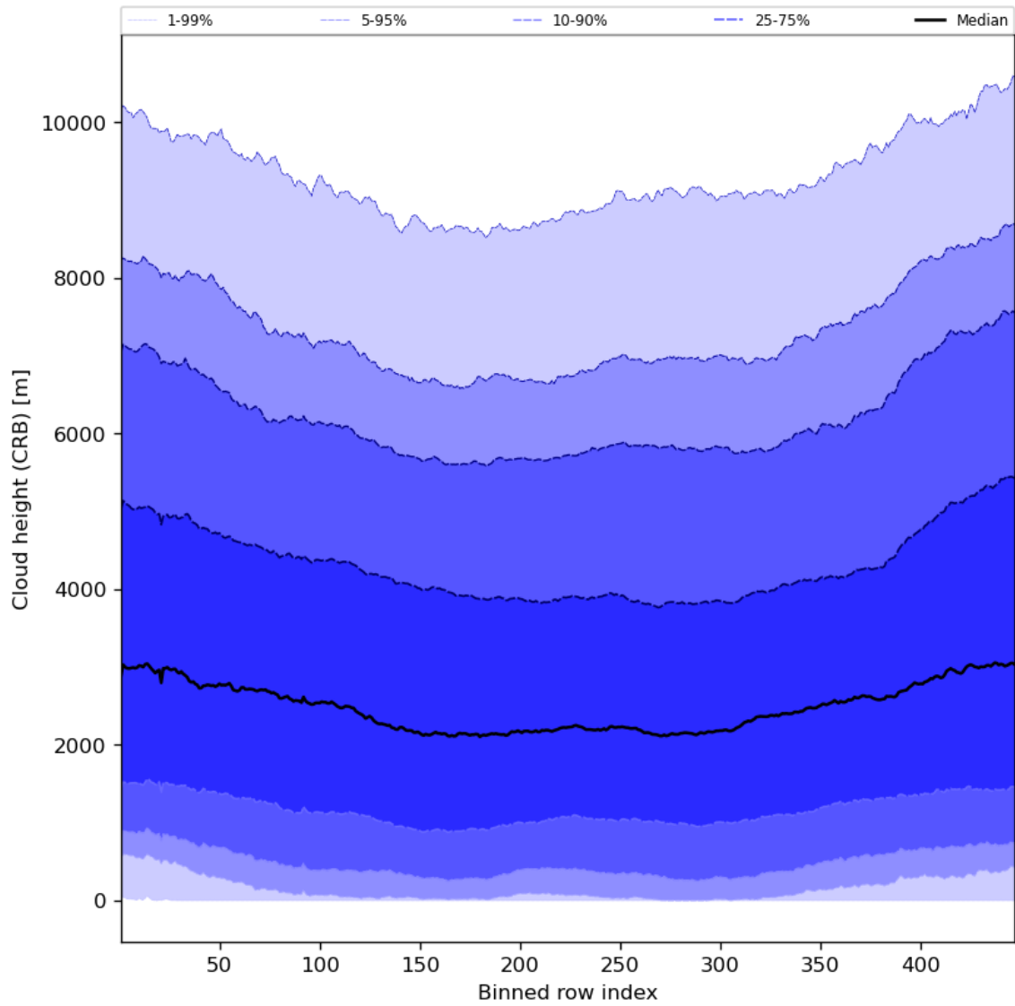
Figure 59: Along track statistics of “Cloud height (CRB)” for 2024-06-27 to 2024-06-29
