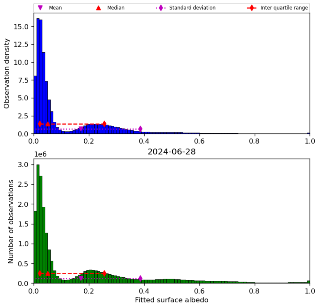
Figure 45: Histogram of “Fitted surface albedo” for 2024-06-27 to 2024-06-29
