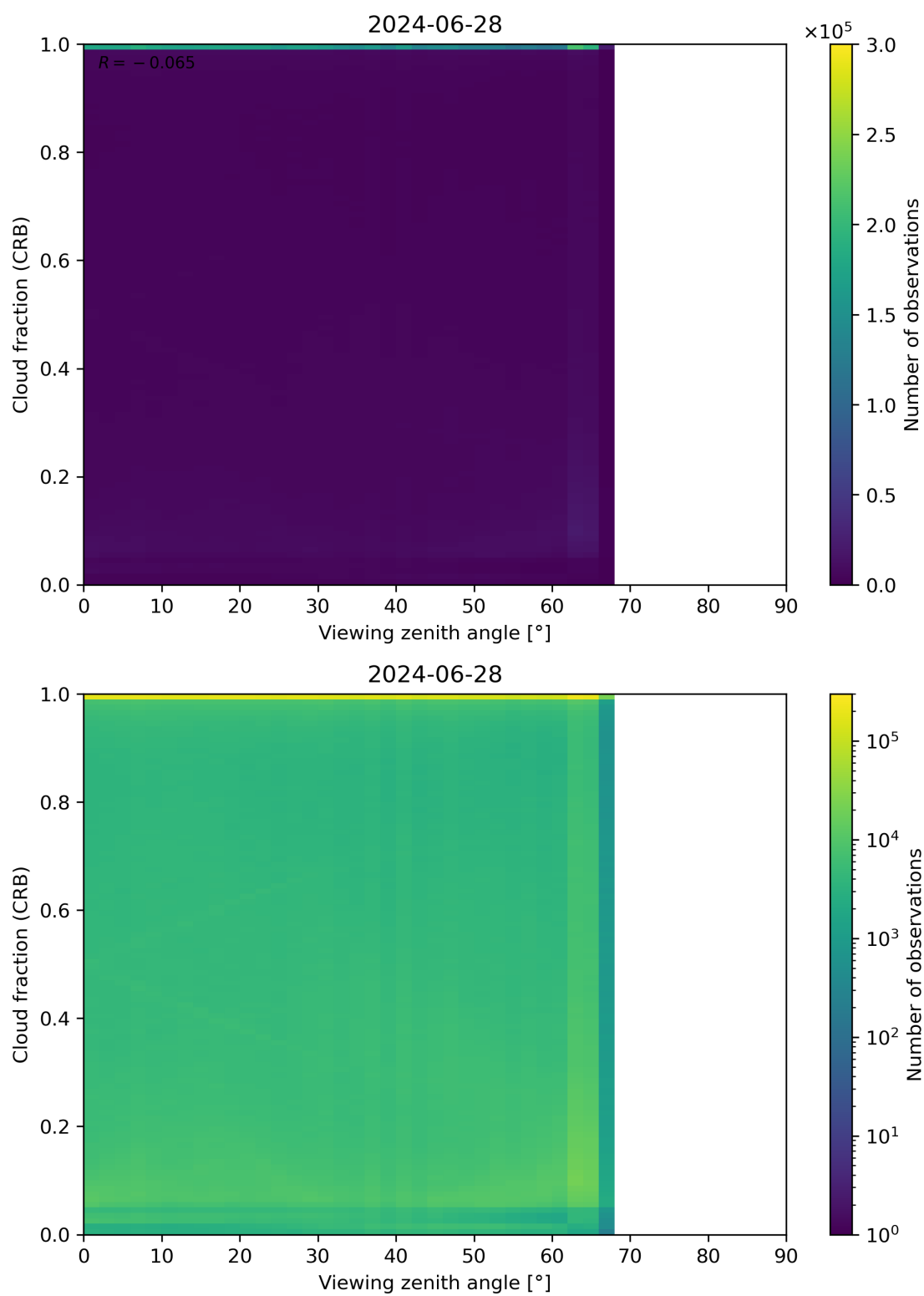
Figure 109: Scatter density plot of “Viewing zenith angle” against “Cloud fraction (CRB)” for 2024-06-27 to 2024-06-29.
