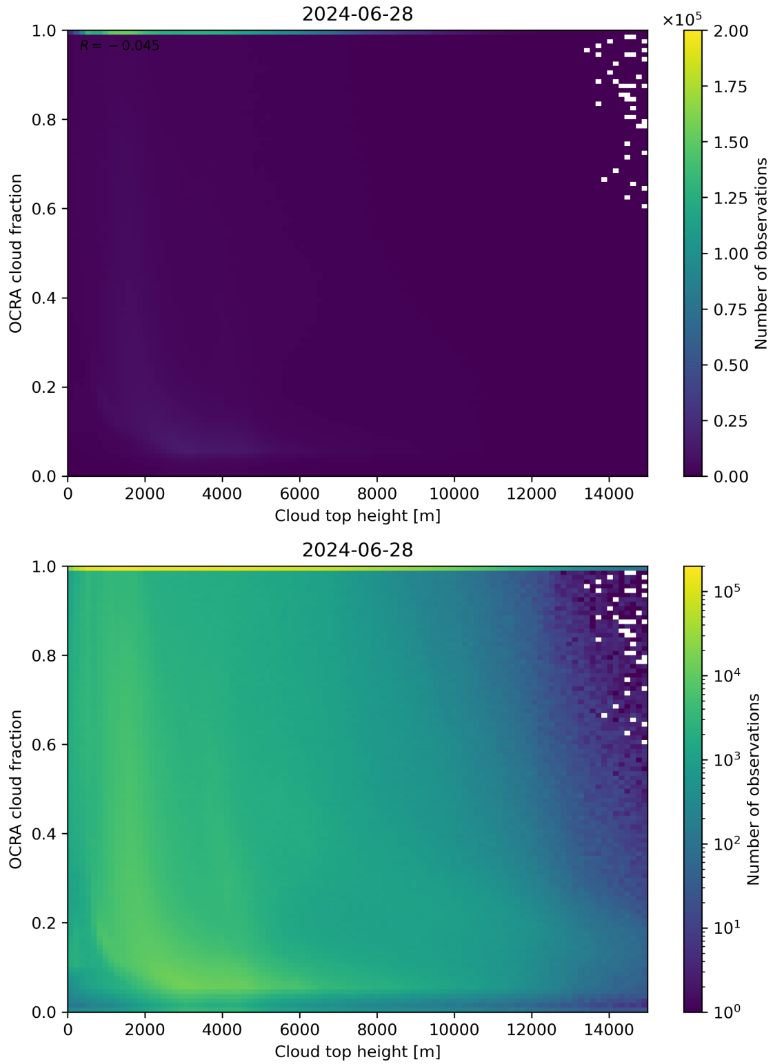
Figure 87: Scatter density plot of “Cloud top height” against “OCRA cloud fraction” for 2024-06-27 to 2024-06-29.
