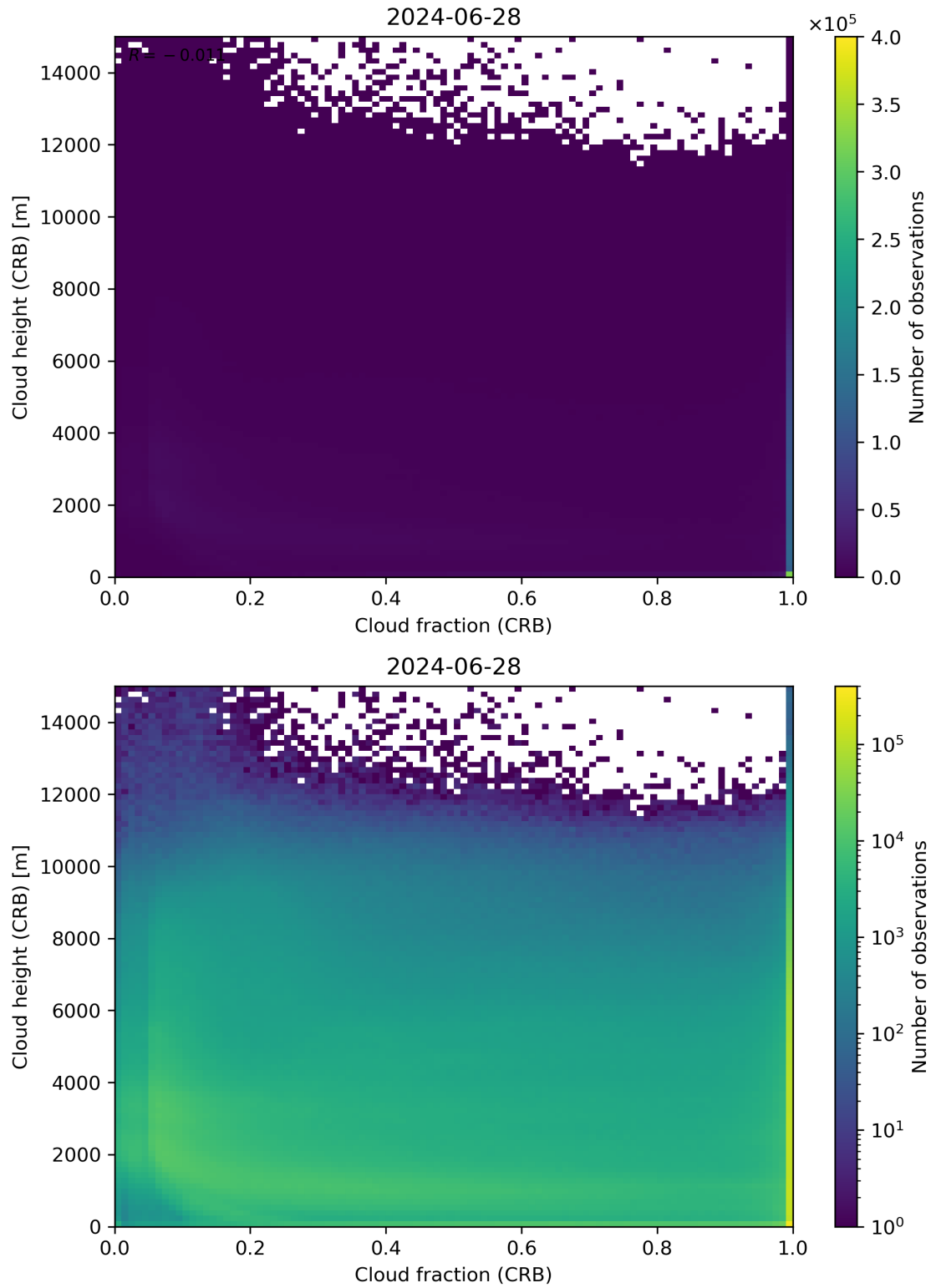
Figure 79: Scatter density plot of “Cloud fraction (CRB)” against “Cloud height (CRB)” for 2024-06-27 to 2024-06-29.
