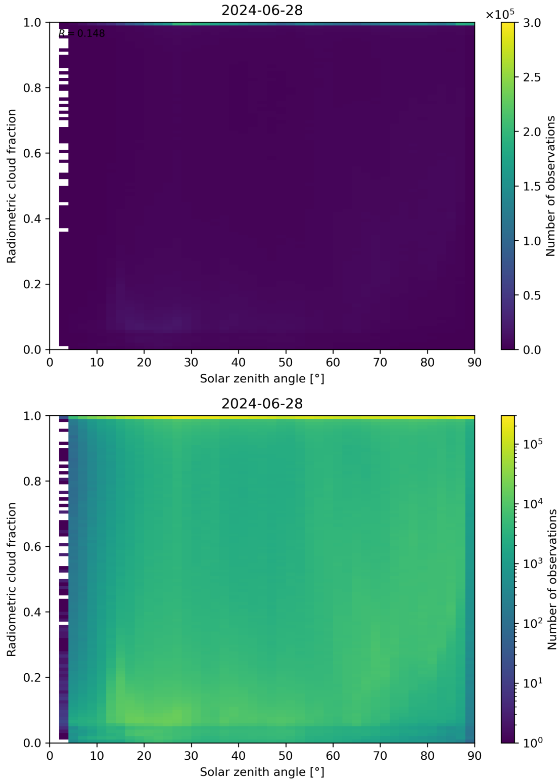
Figure 99: Scatter density plot of “Solar zenith angle” against “Radiometric cloud fraction” for 2024-06-27 to 2024-06-29.
