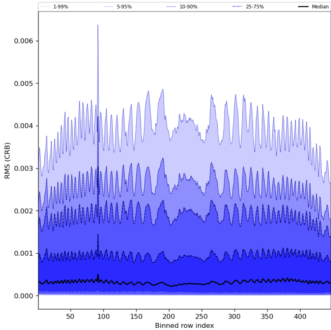
Figure 64: Along track statistics of “RMS (CRB)” for 2024-06-27 to 2024-06-29
