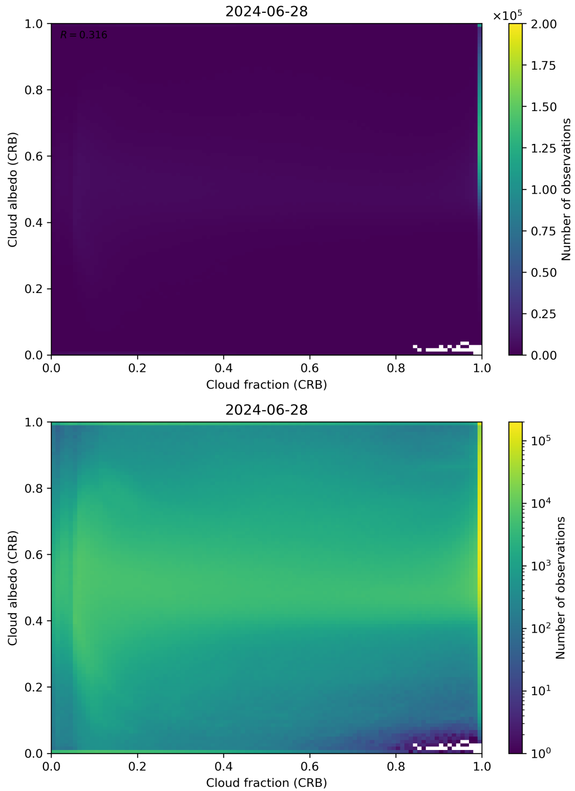
Figure 77: Scatter density plot of “Cloud fraction (CRB)” against “Cloud albedo (CRB)” for 2024-06-27 to 2024-06-29.
