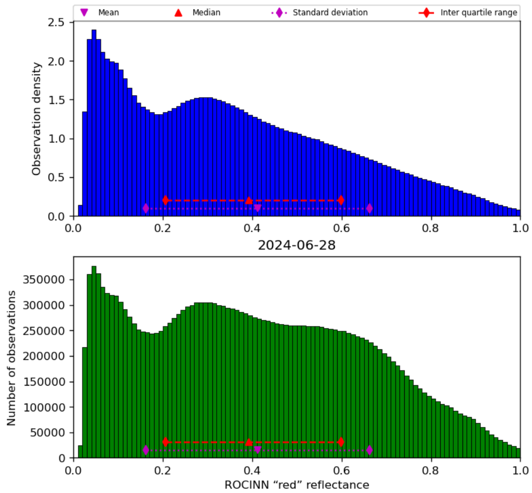
Figure 53: Histogram of “ROCINN “red” reflectance” for 2024-06-27 to 2024-06-29
