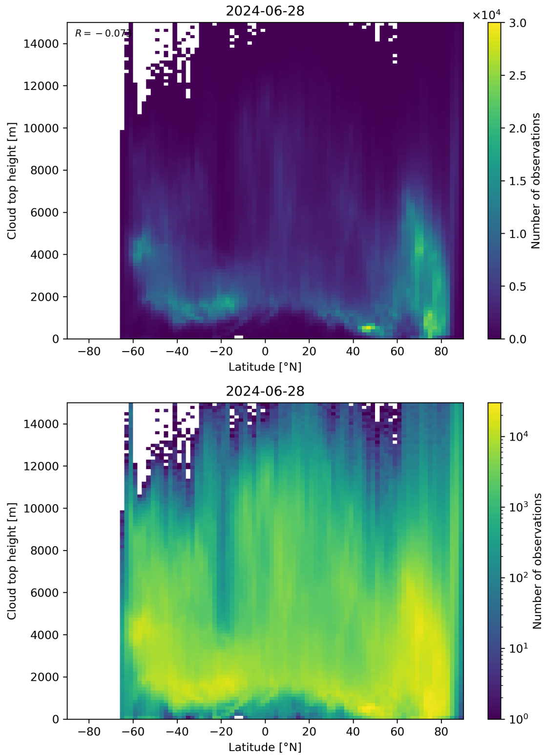
Figure 97: Scatter density plot of “Latitude” against “Cloud top height” for 2024-06-27 to 2024-06-29.
