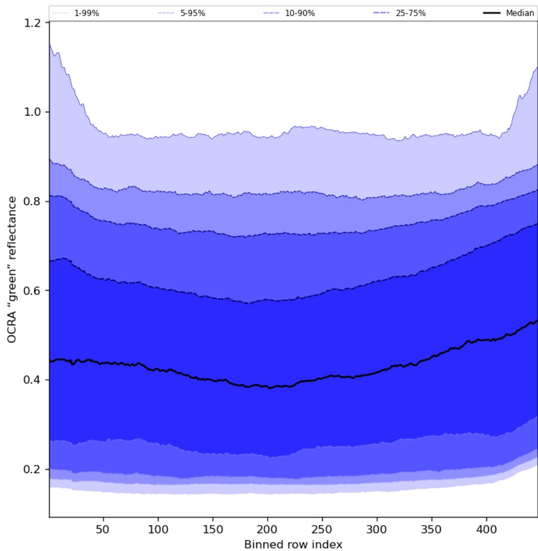
Figure 68: Along track statistics of “OCRA “green” reflectance” for 2024-06-27 to 2024-06-29
