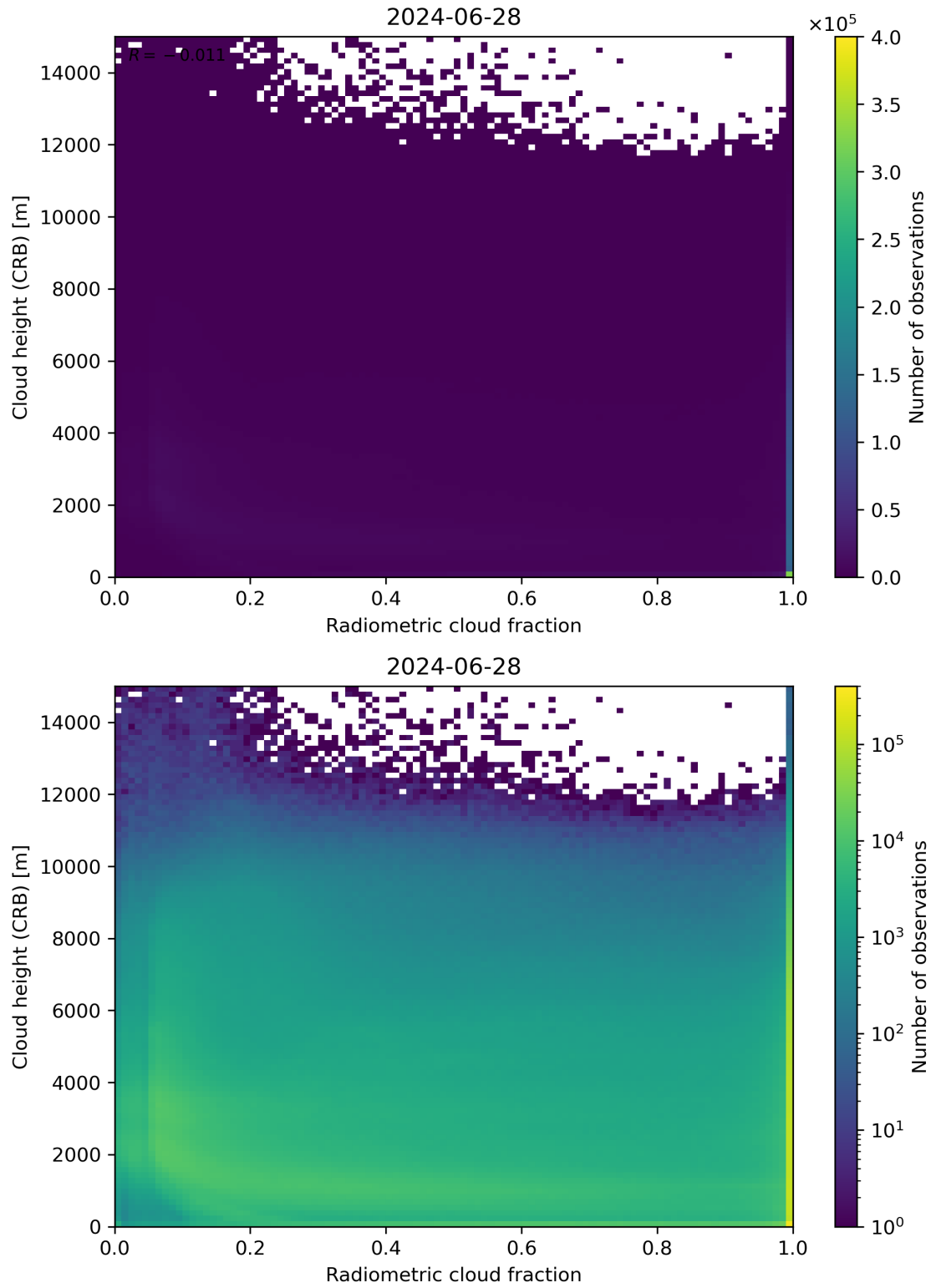
Figure 74: Scatter density plot of “Radiometric cloud fraction” against “Cloud height (CRB)” for 2024-06-27 to 2024-06-29.
