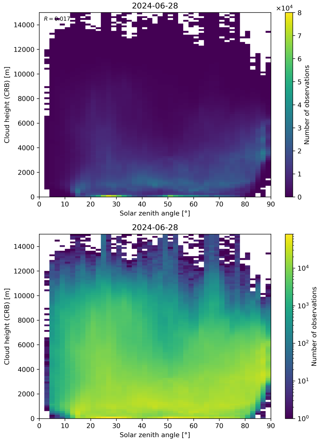
Figure 102: Scatter density plot of “Solar zenith angle” against “Cloud height (CRB)” for 2024-06-27 to 2024-06-29.
