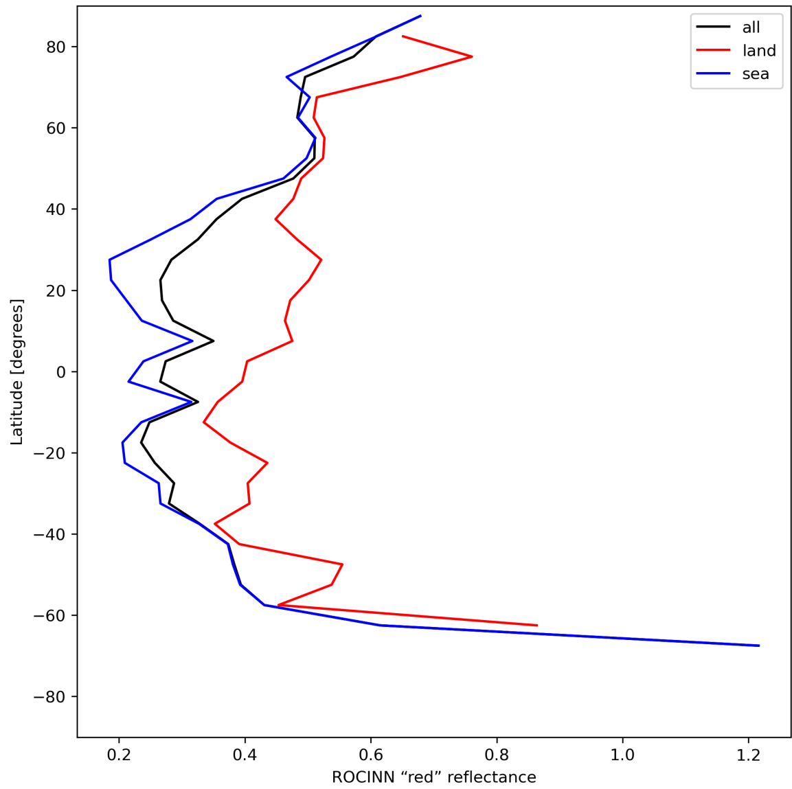
Figure 37: Zonal average of “ROCINN “red” reflectance” for 2024-06-27 to 2024-06-29.
