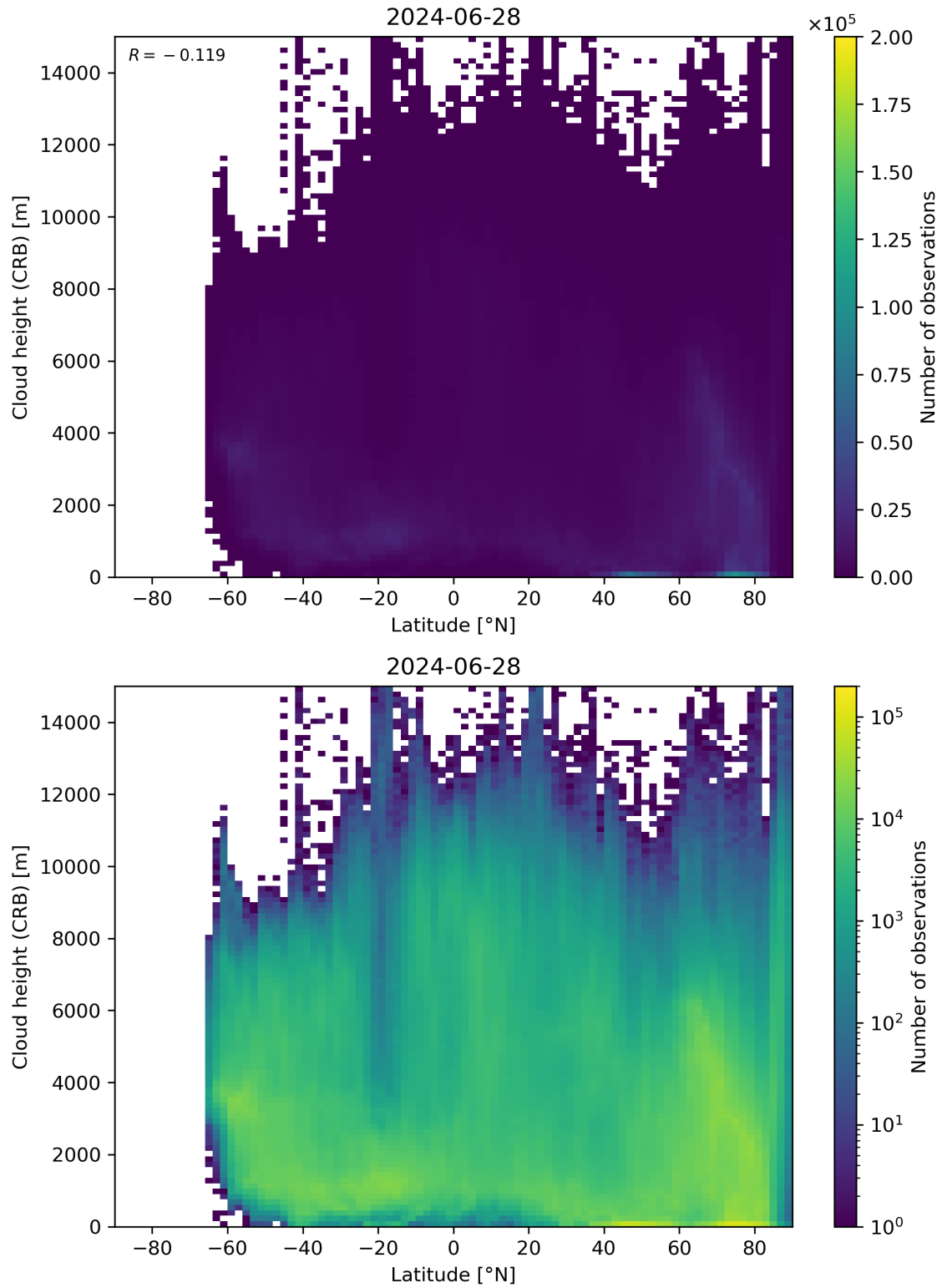
Figure 95: Scatter density plot of “Latitude” against “Cloud height (CRB)” for 2024-06-27 to 2024-06-29.
