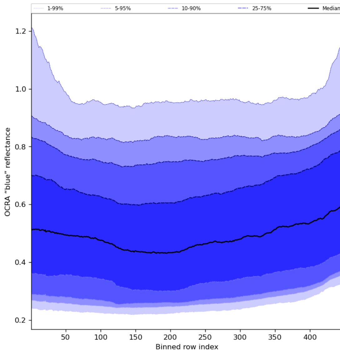
Figure 67: Along track statistics of “OCRA “blue” reflectance” for 2024-06-29 to 2024-06-30
