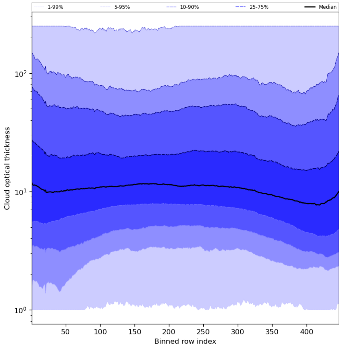
Figure 57: Along track statistics of “Cloud optical thickness” for 2024-06-29 to 2024-06-30
