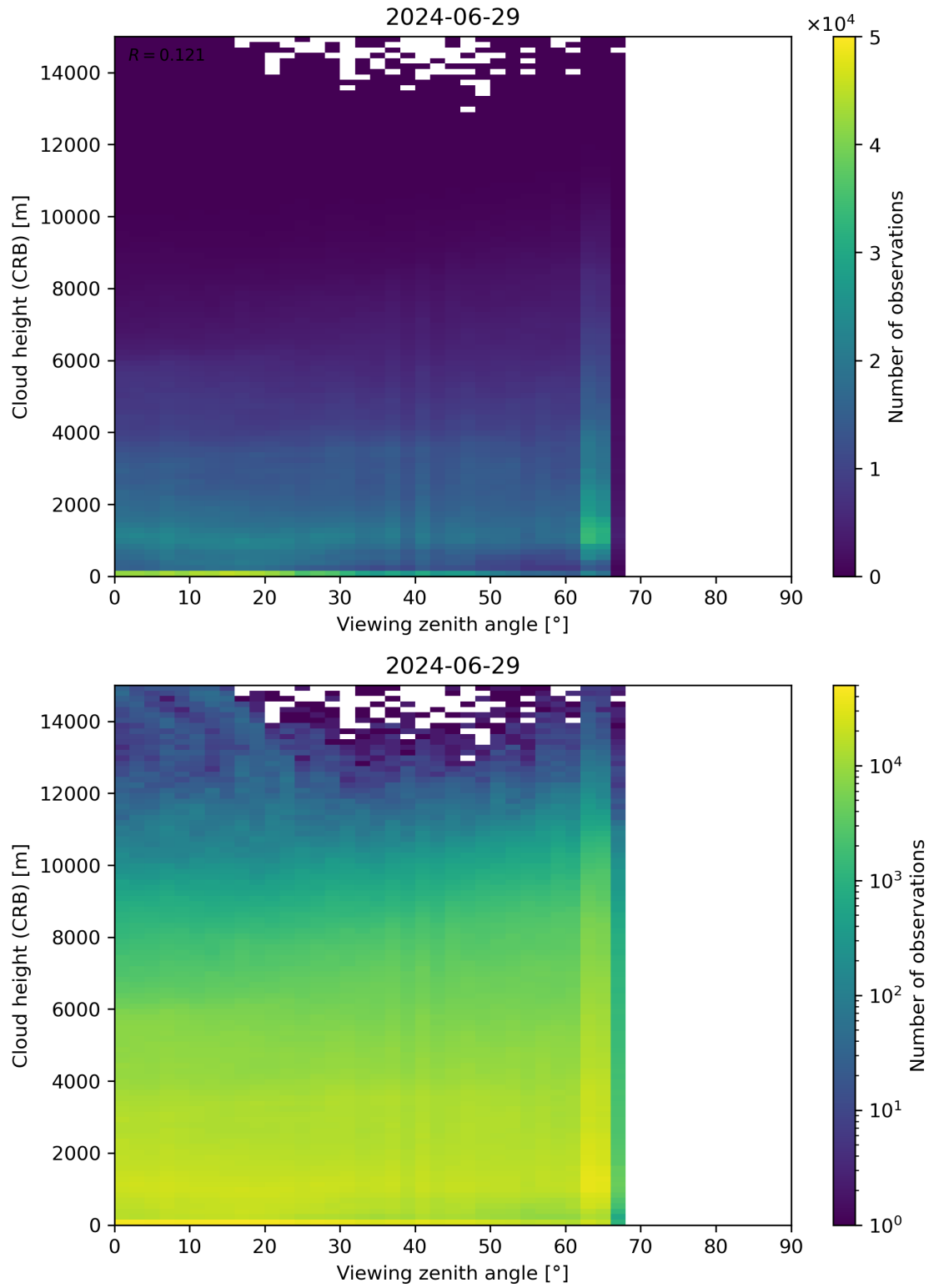
Figure 110: Scatter density plot of “Viewing zenith angle” against “Cloud height (CRB)” for 2024-06-29 to 2024-06-30.
