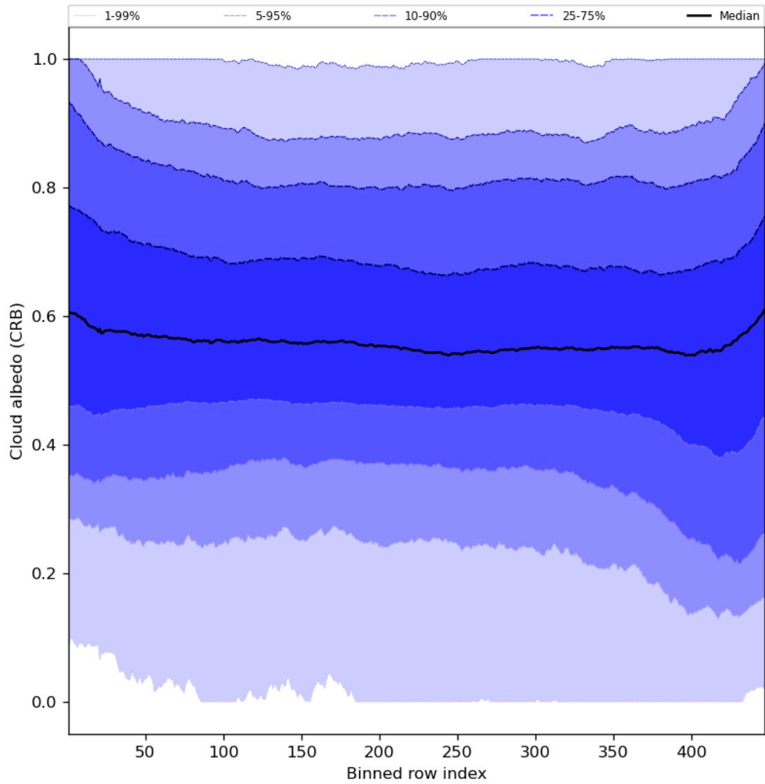
Figure 60: Along track statistics of “Cloud albedo (CRB)” for 2024-06-29 to 2024-06-30
