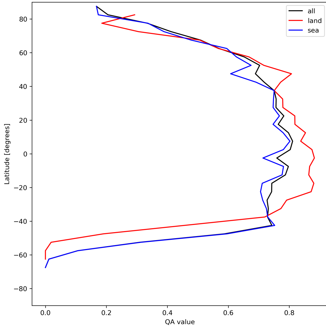
Figure 22: Zonal average of “QA value” for 2024-06-29 to 2024-06-30.
