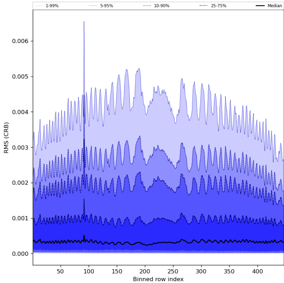
Figure 64: Along track statistics of “RMS (CRB)” for 2024-06-29 to 2024-06-30
