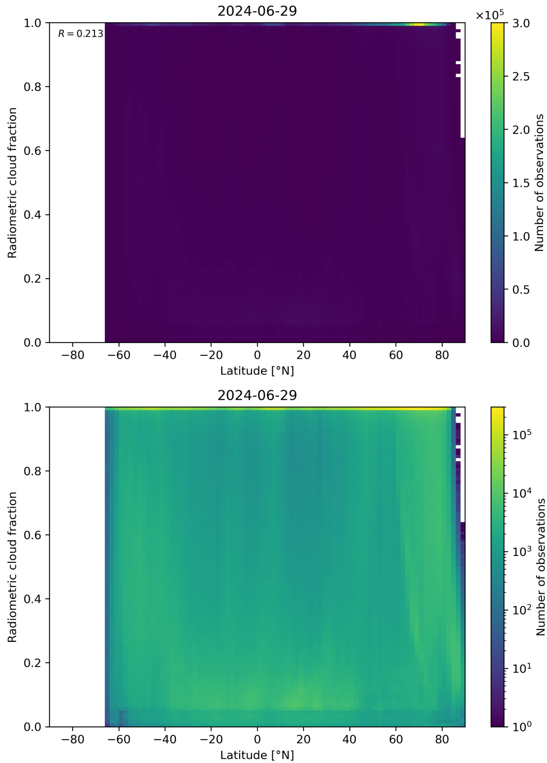
Figure 92: Scatter density plot of “Latitude” against “Radiometric cloud fraction” for 2024-06-29 to 2024-06-30.
