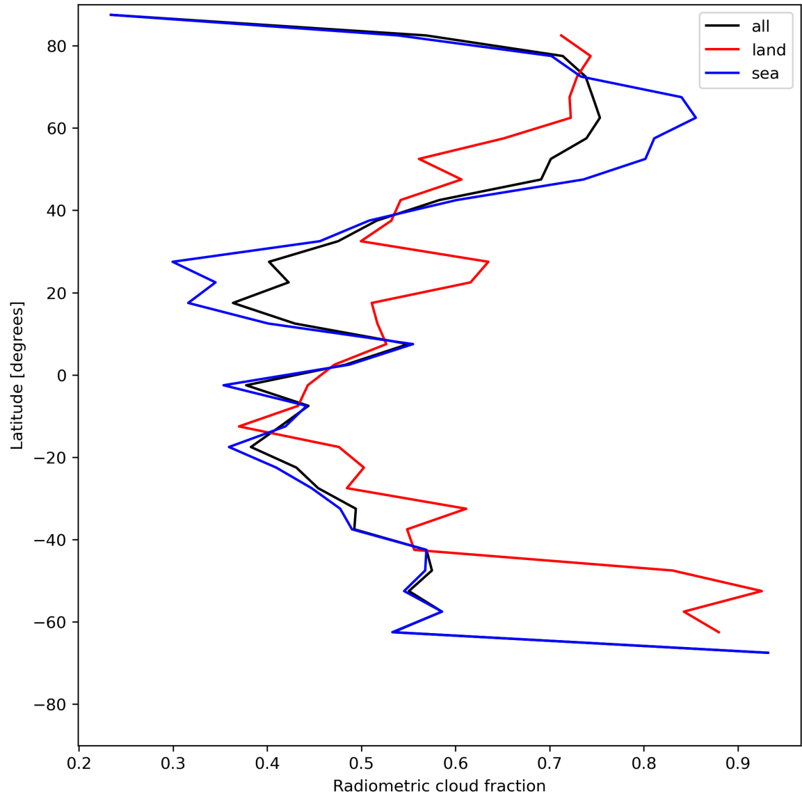
Figure 23: Zonal average of “Radiometric cloud fraction” for 2024-06-29 to 2024-06-30.
