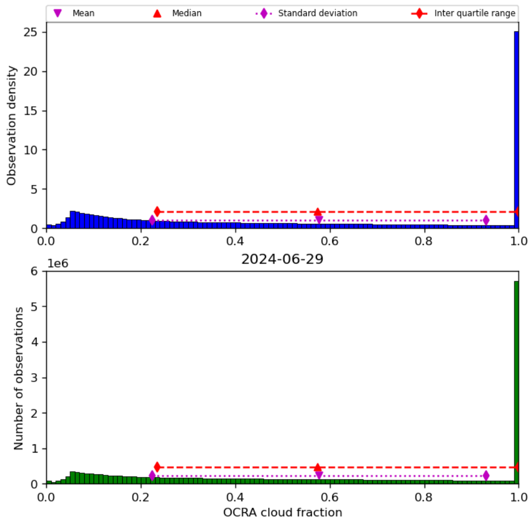
Figure 50: Histogram of “OCRA cloud fraction” for 2024-06-29 to 2024-06-30
