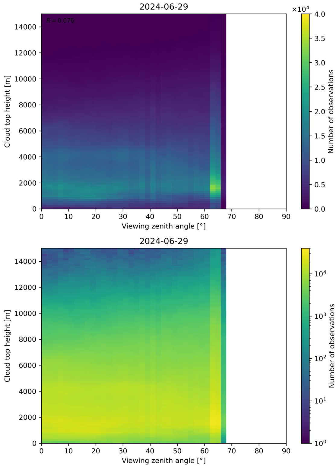
Figure 112: Scatter density plot of “Viewing zenith angle” against “Cloud top height” for 2024-06-29 to 2024-06-30.
