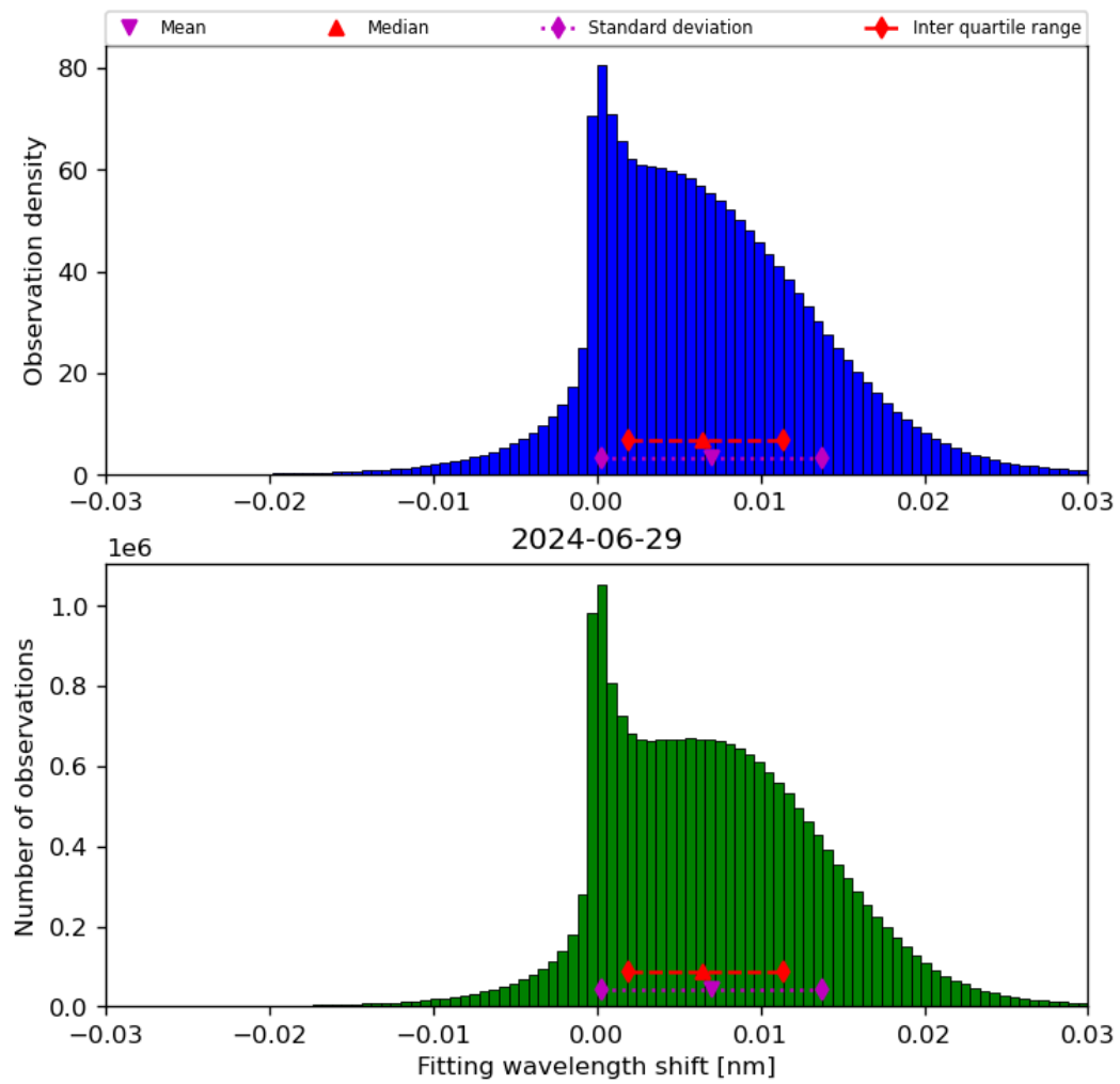
Figure 49: Histogram of “Fitting wavelength shift” for 2024-06-29 to 2024-06-30
