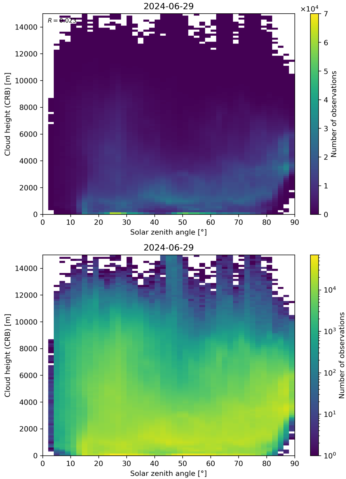
Figure 102: Scatter density plot of “Solar zenith angle” against “Cloud height (CRB)” for 2024-06-29 to 2024-06-30.
