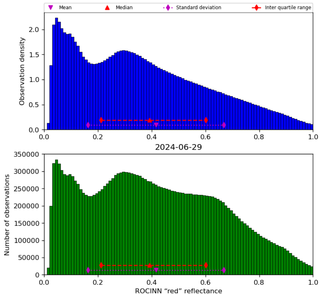
Figure 53: Histogram of “ROCINN “red” reflectance” for 2024-06-29 to 2024-06-30
