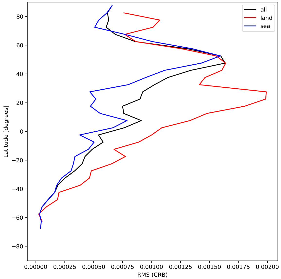
Figure 32: Zonal average of “RMS (CRB)” for 2024-06-29 to 2024-06-30.
