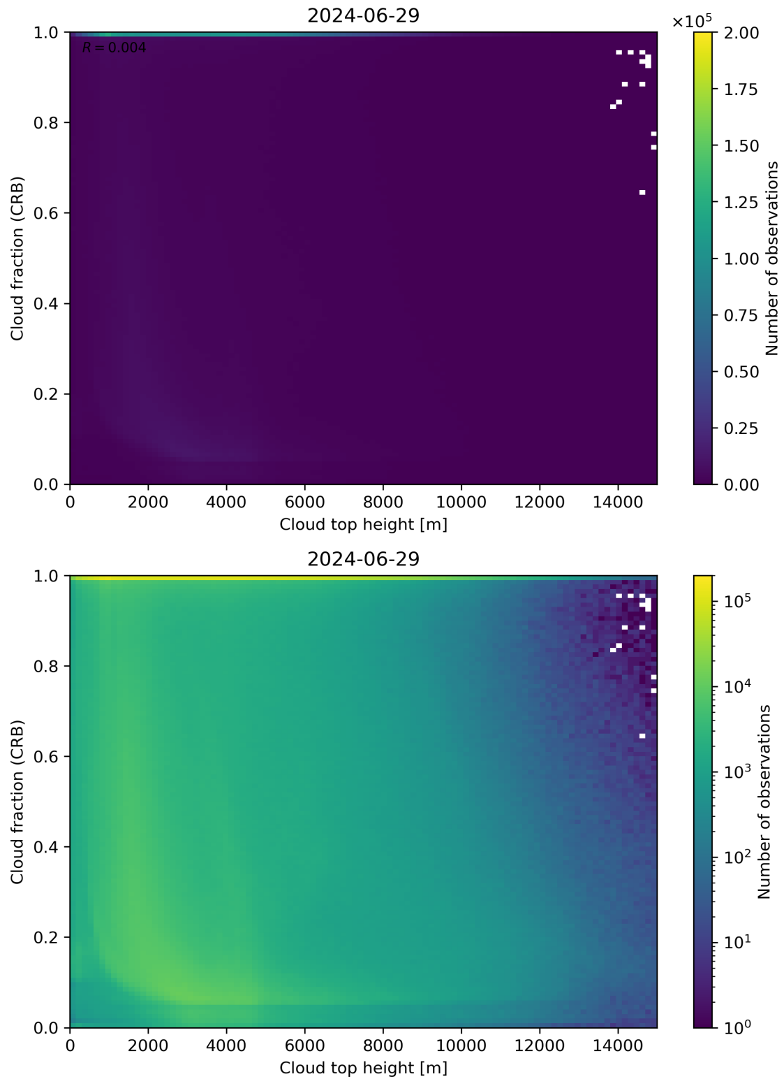
Figure 88: Scatter density plot of “Cloud top height” against “Cloud fraction (CRB)” for 2024-06-29 to 2024-06-30.
