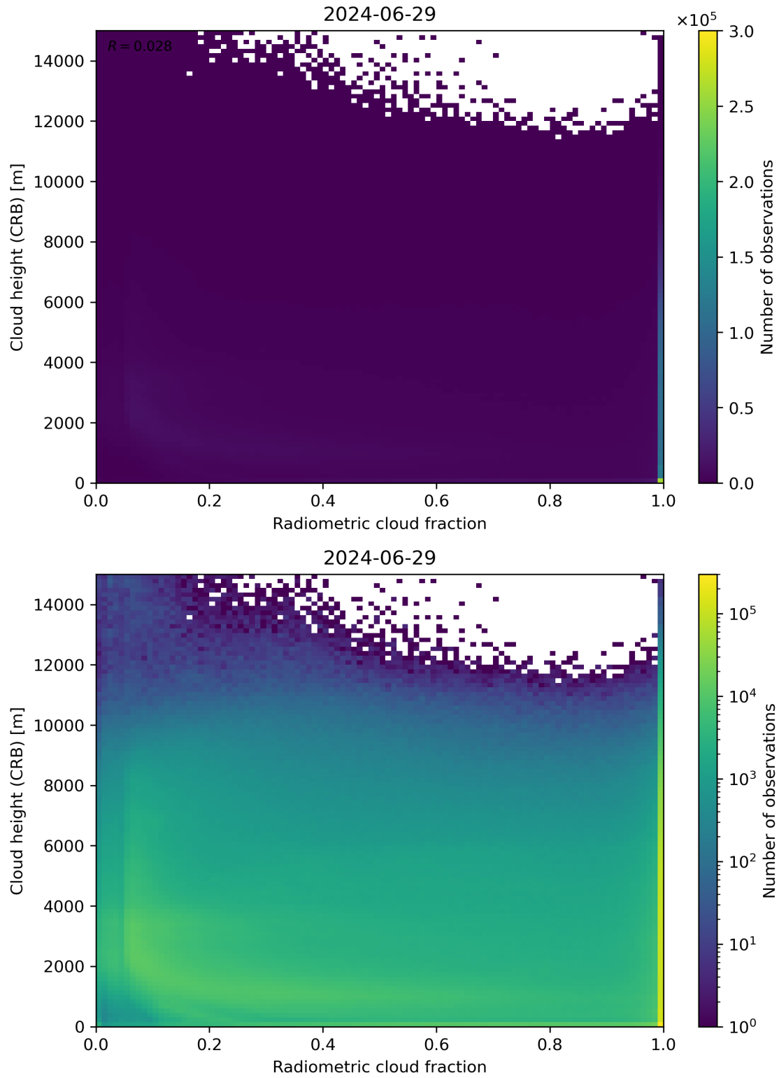
Figure 74: Scatter density plot of “Radiometric cloud fraction” against “Cloud height (CRB)” for 2024-06-29 to 2024-06-30.
