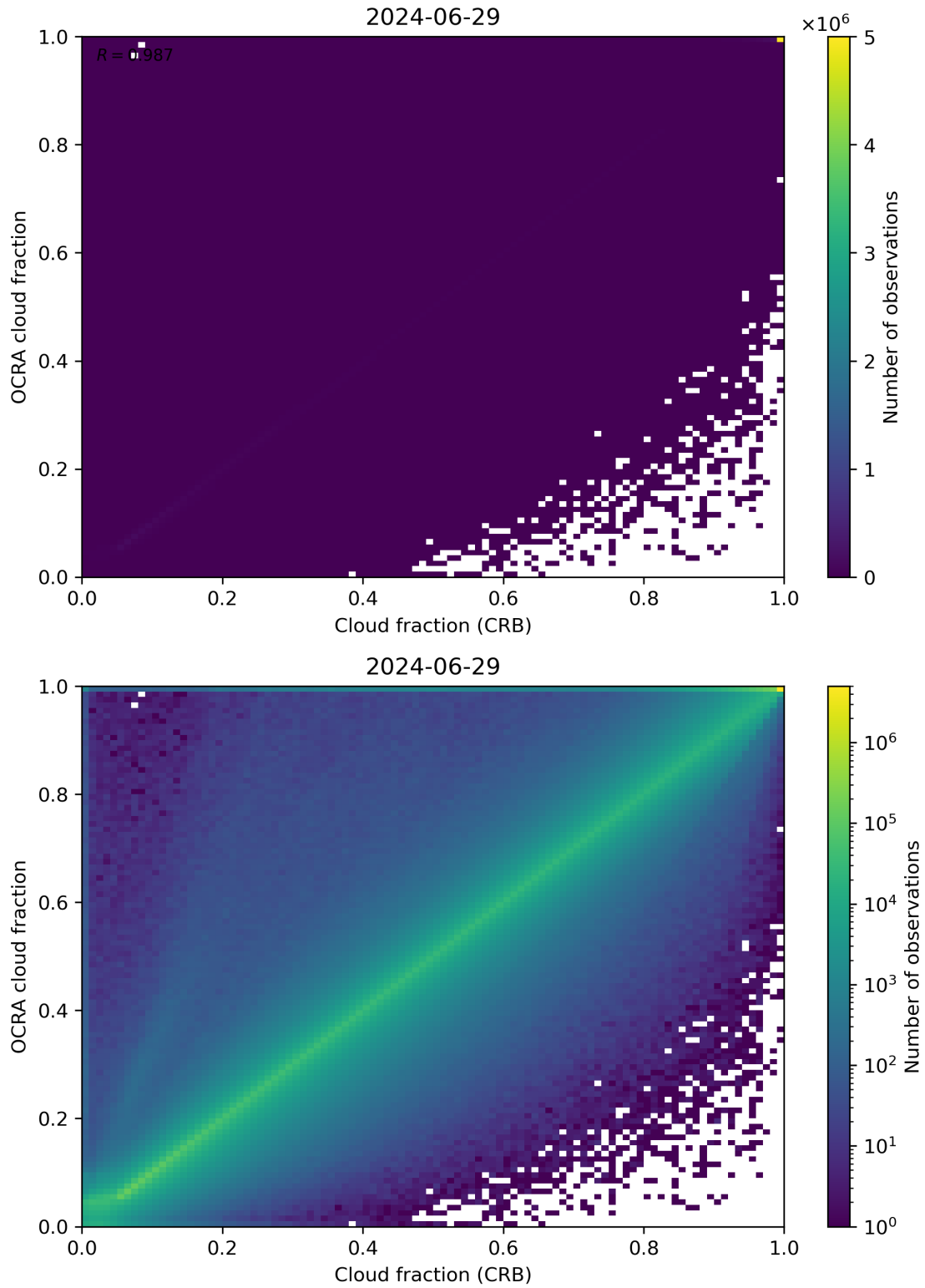
Figure 78: Scatter density plot of “Cloud fraction (CRB)” against “OCRA cloud fraction” for 2024-06-29 to 2024-06-30.
