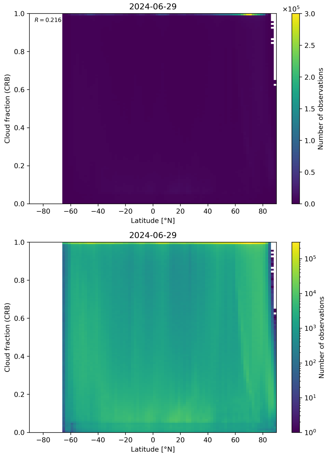
Figure 94: Scatter density plot of “Latitude” against “Cloud fraction (CRB)” for 2024-06-29 to 2024-06-30.
