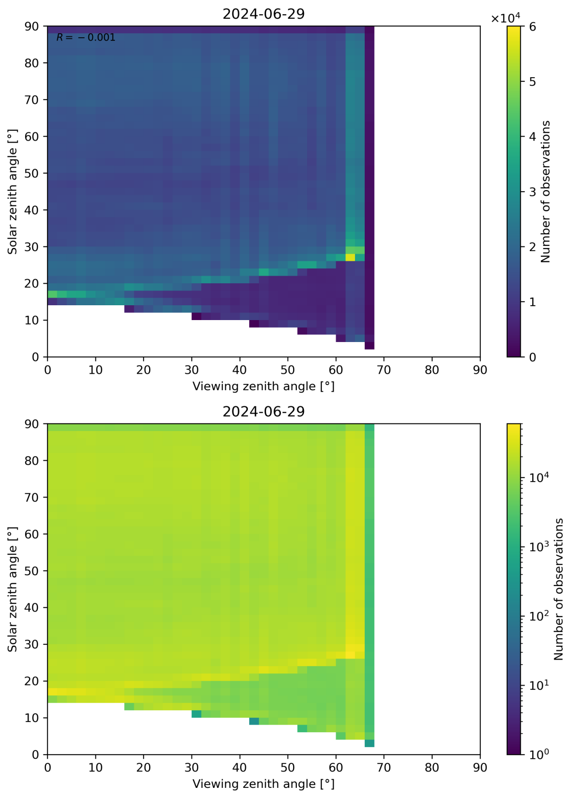
Figure 114: Scatter density plot of “Viewing zenith angle” against “Solar zenith angle” for 2024-06-29 to 2024-06-30.
