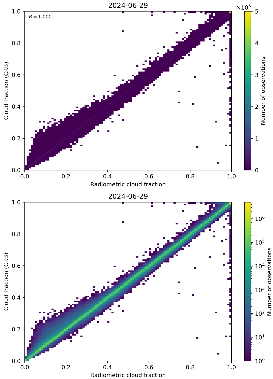
Figure 73: Scatter density plot of “Radiometric cloud fraction” against “Cloud fraction (CRB)” for 2024-06-29 to 2024-06-30.
