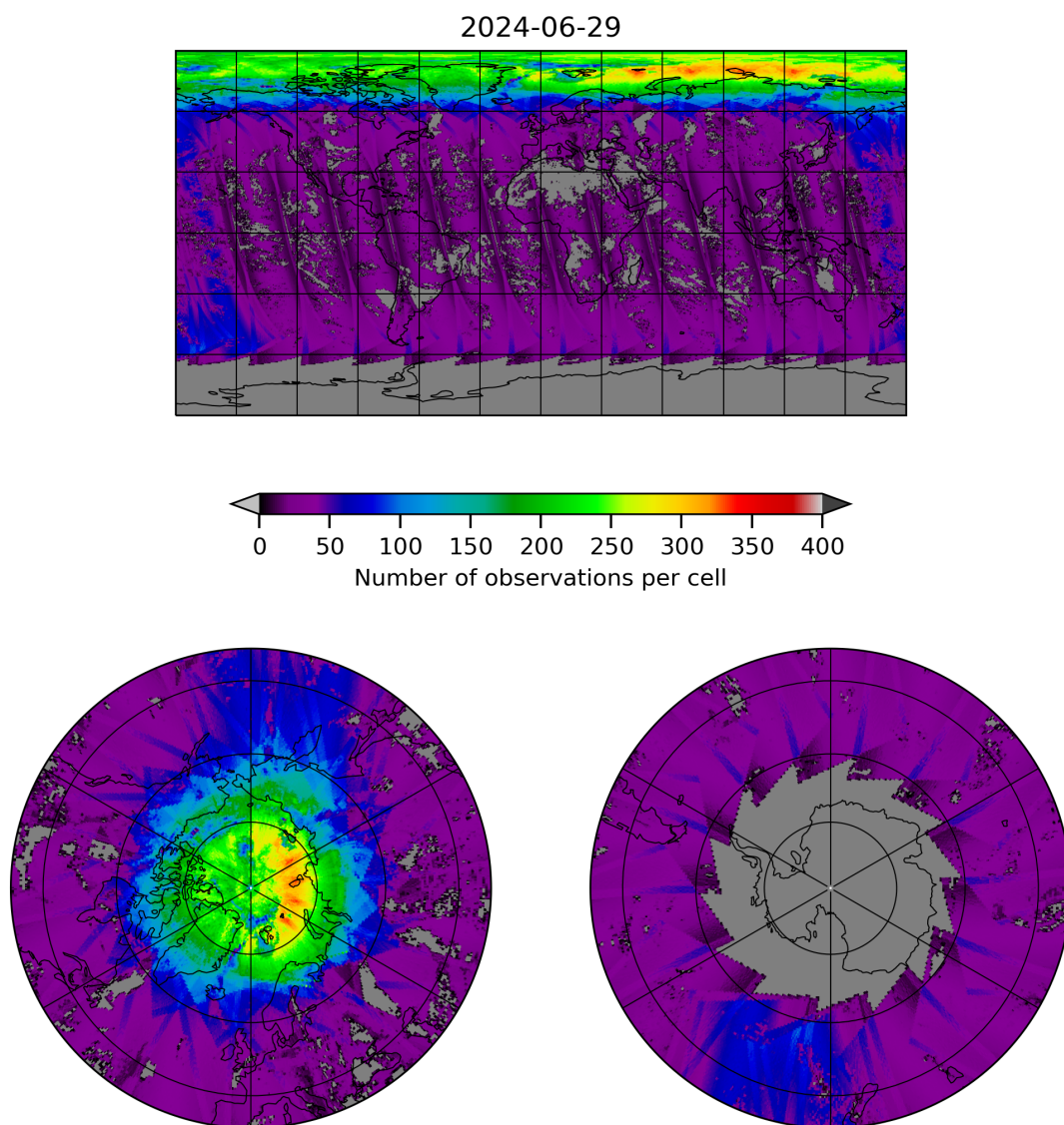
Figure 21: Map of the number of observations for 2024-06-29 to 2024-06-30
