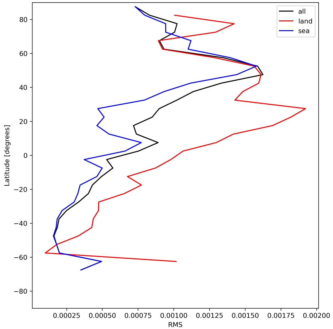
Figure 31: Zonal average of “RMS” for 2024-06-29 to 2024-06-30.
