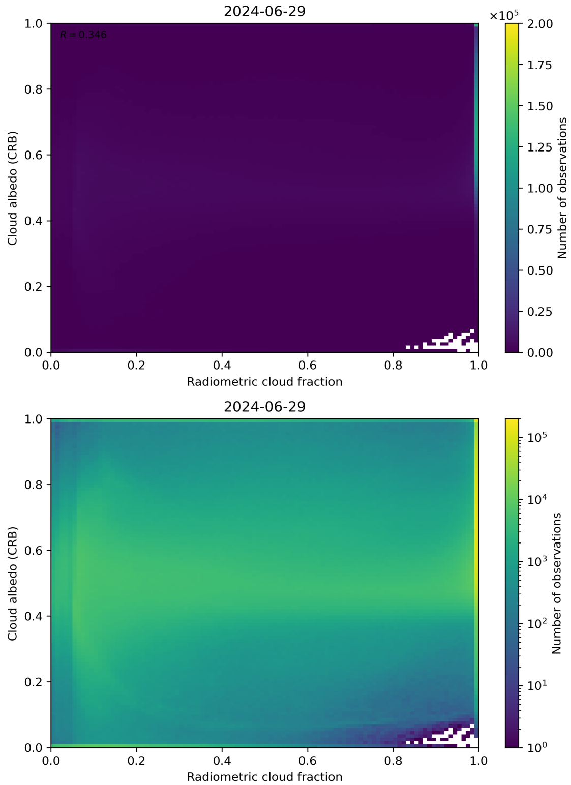
Figure 71: Scatter density plot of “Radiometric cloud fraction” against “Cloud albedo (CRB)” for 2024-06-29 to 2024-06-30.
