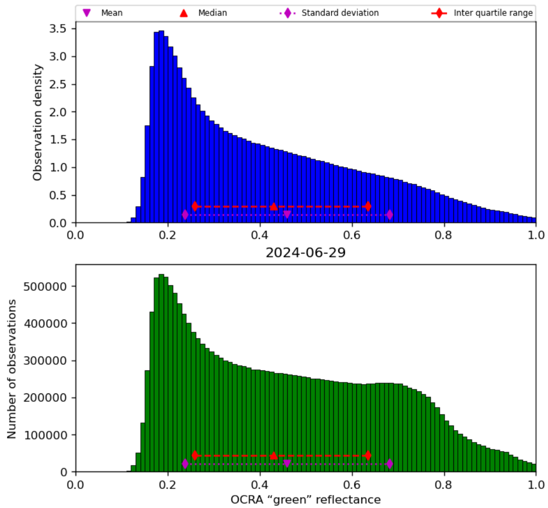
Figure 52: Histogram of “OCRA “green” reflectance” for 2024-06-29 to 2024-06-30
