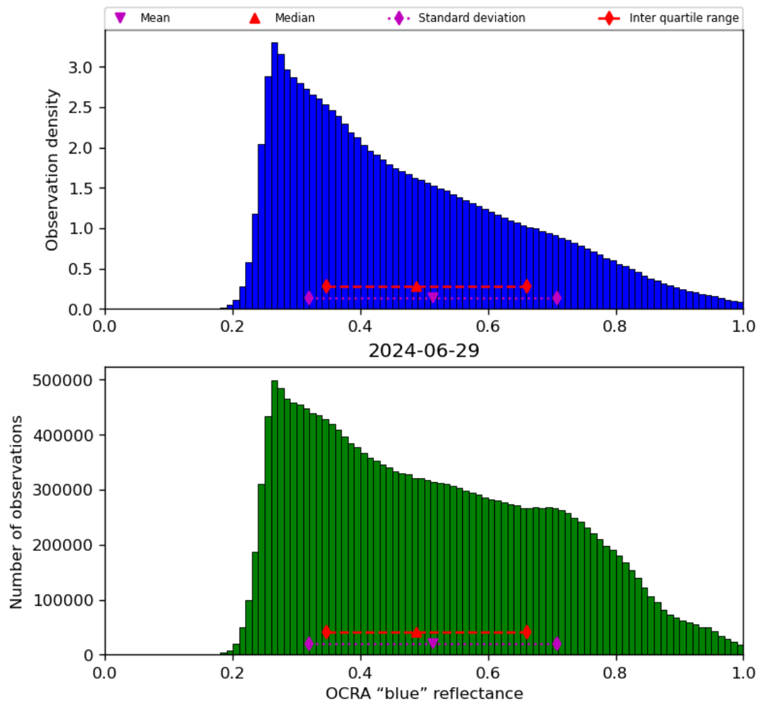
Figure 51: Histogram of “OCRA “blue” reflectance” for 2024-06-29 to 2024-06-30
