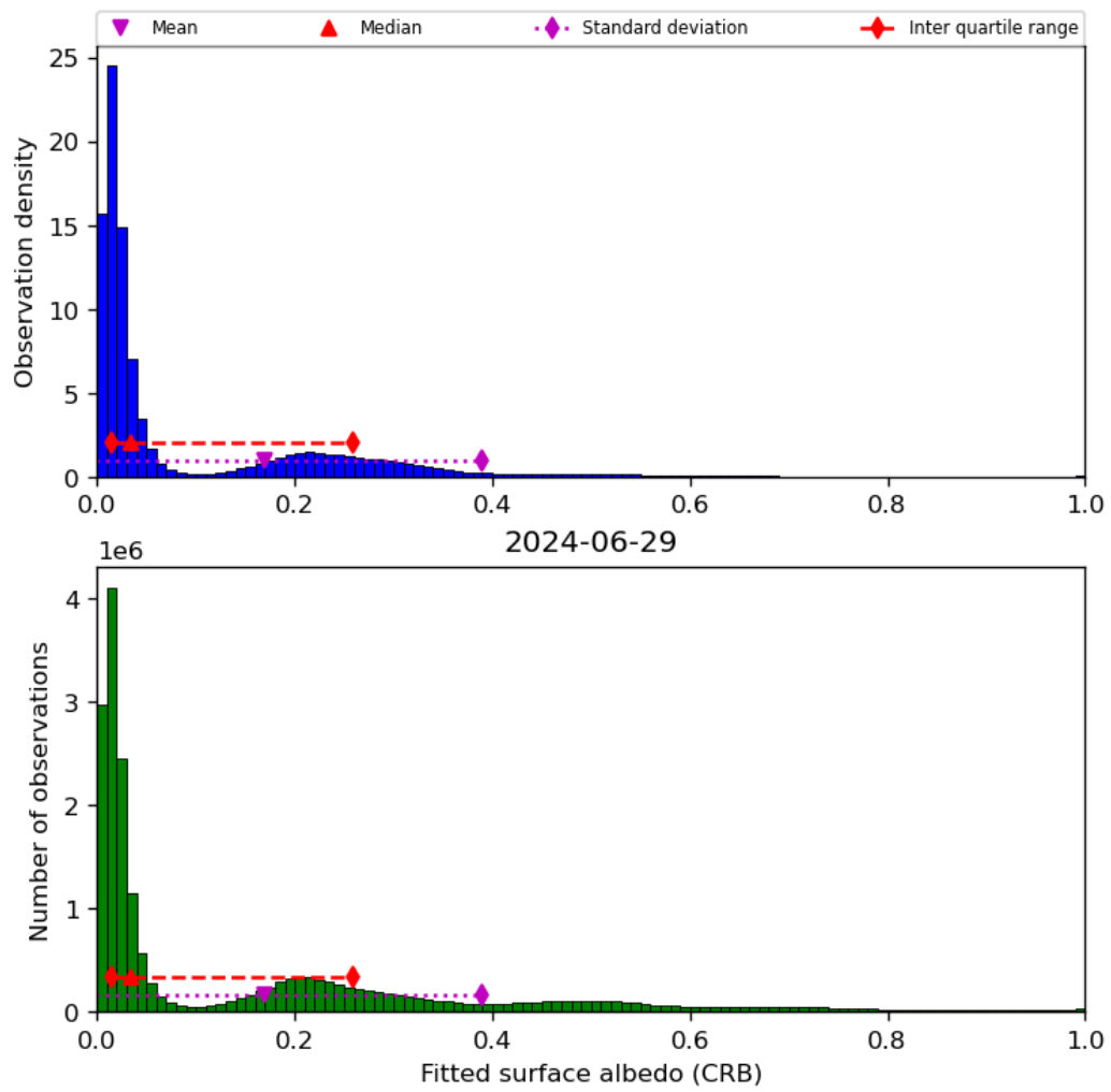
Figure 46: Histogram of “Fitted surface albedo (CRB)” for 2024-06-29 to 2024-06-30
