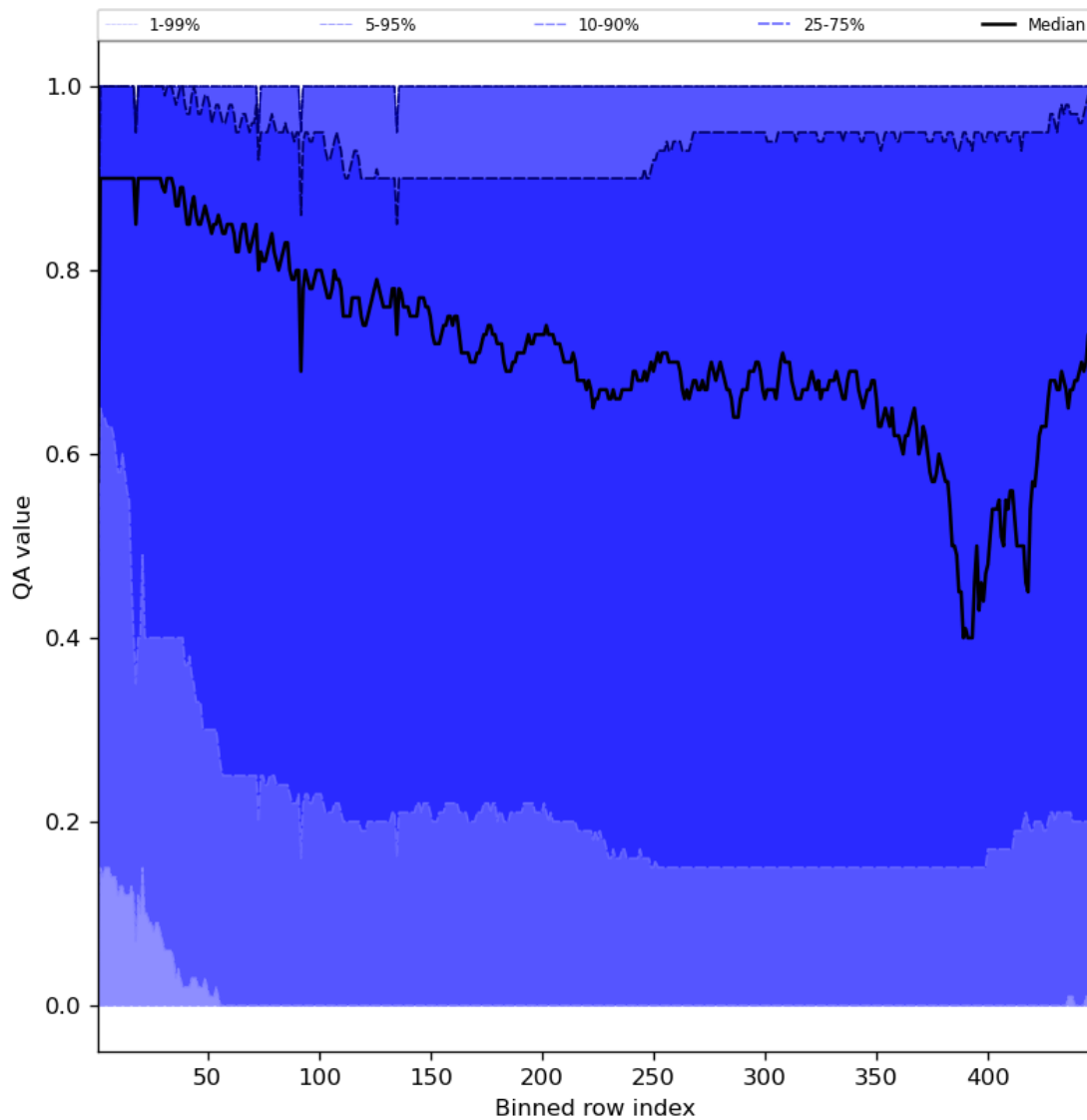
Figure 54: Along track statistics of “QA value” for 2024-06-29 to 2024-06-30
