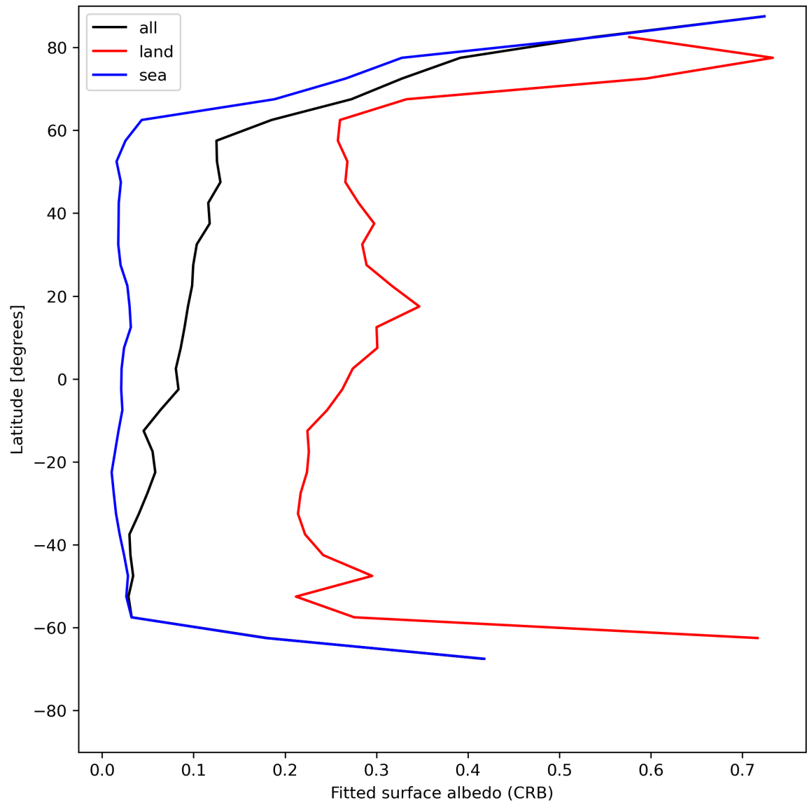
Figure 30: Zonal average of “Fitted surface albedo (CRB)” for 2024-06-29 to 2024-06-30.
