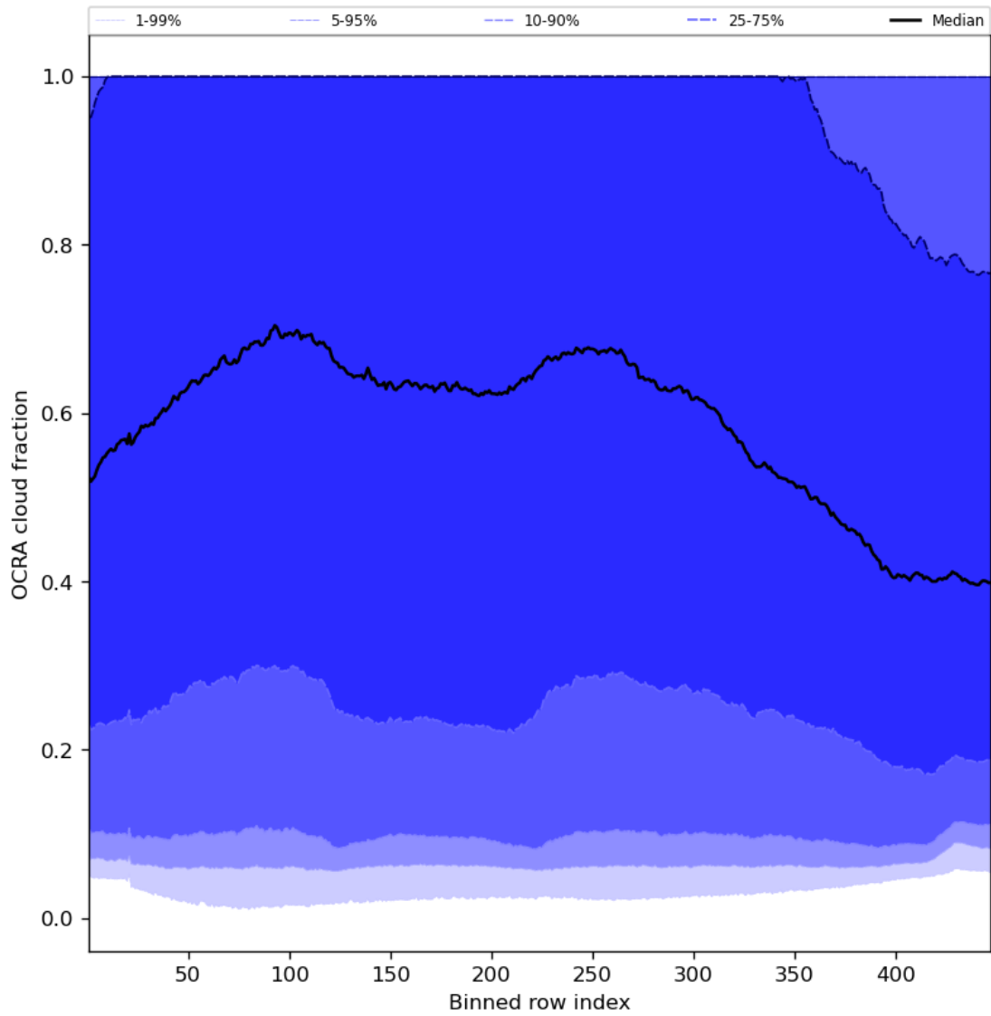
Figure 66: Along track statistics of “OCRA cloud fraction” for 2024-06-29 to 2024-06-30
