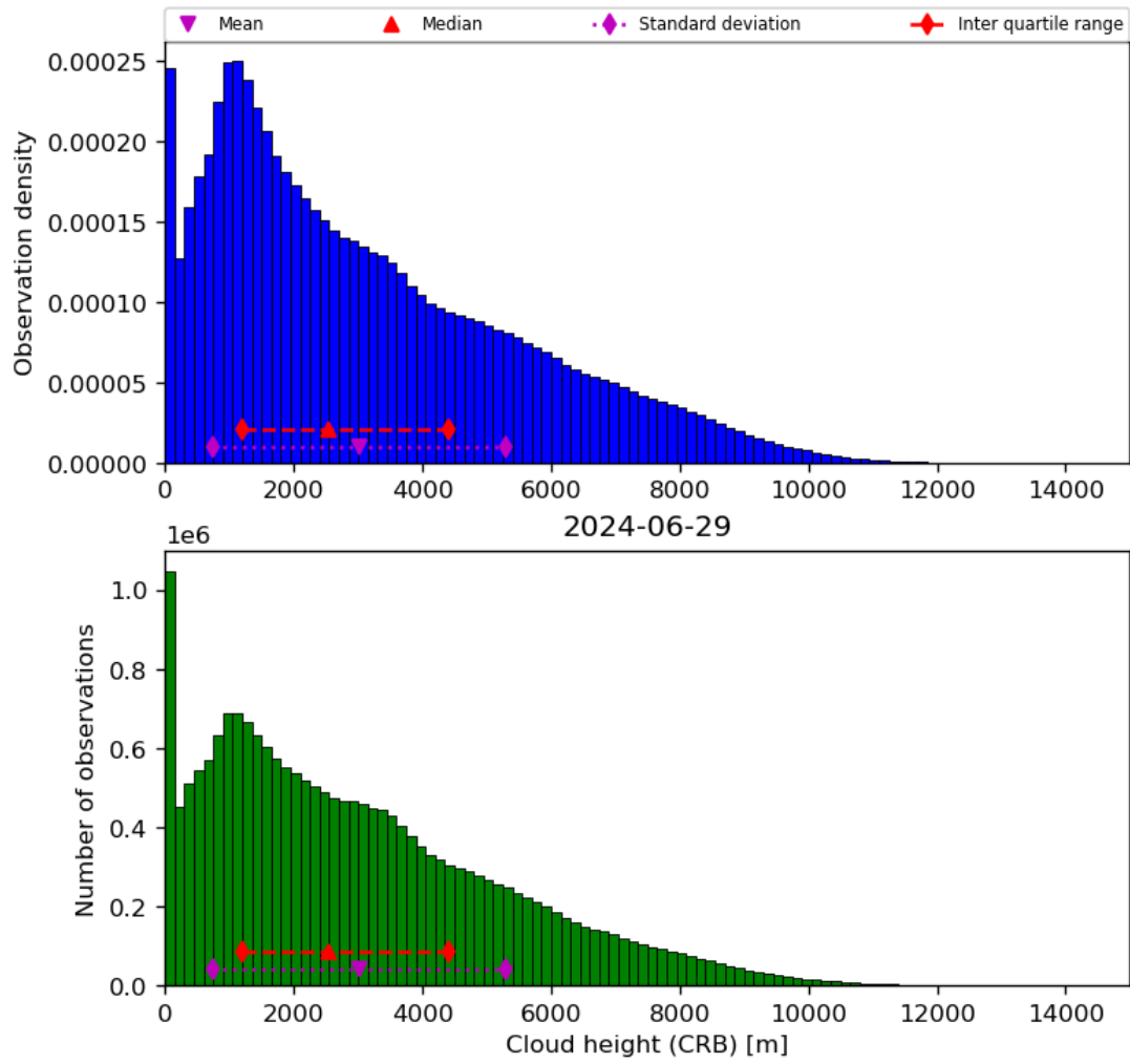
Figure 43: Histogram of “Cloud height (CRB)” for 2024-06-29 to 2024-06-30
