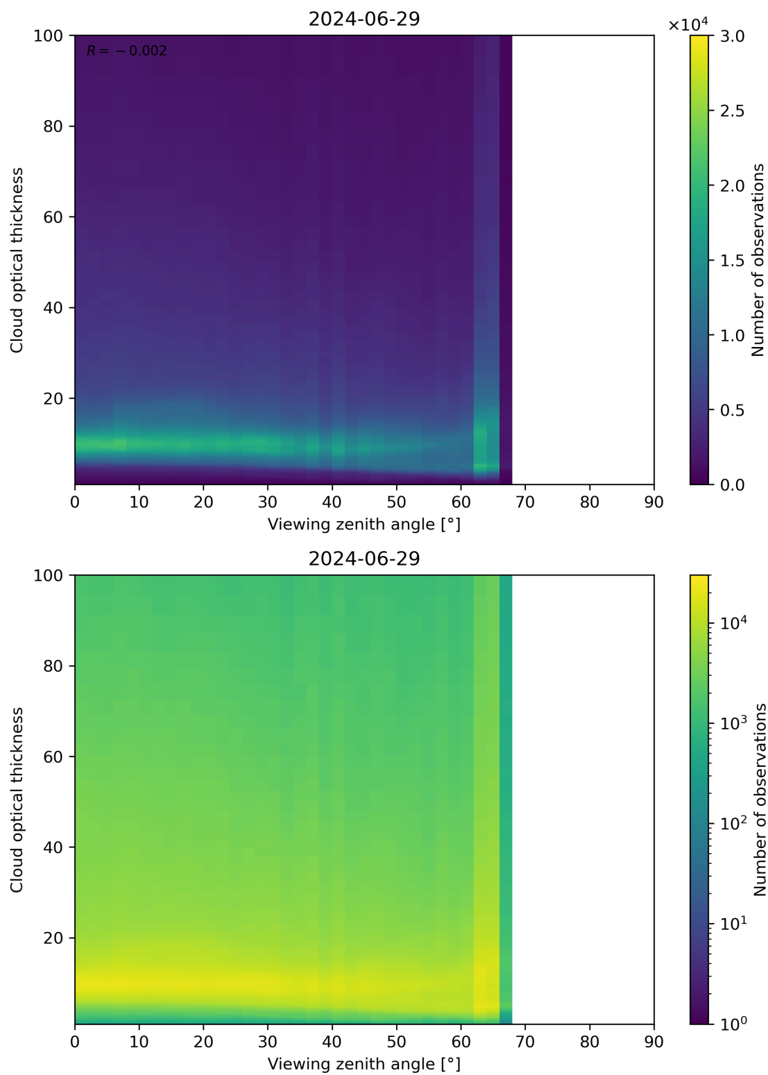
Figure 111: Scatter density plot of “Viewing zenith angle” against “Cloud optical thickness” for 2024-06-29 to 2024-06-30.
