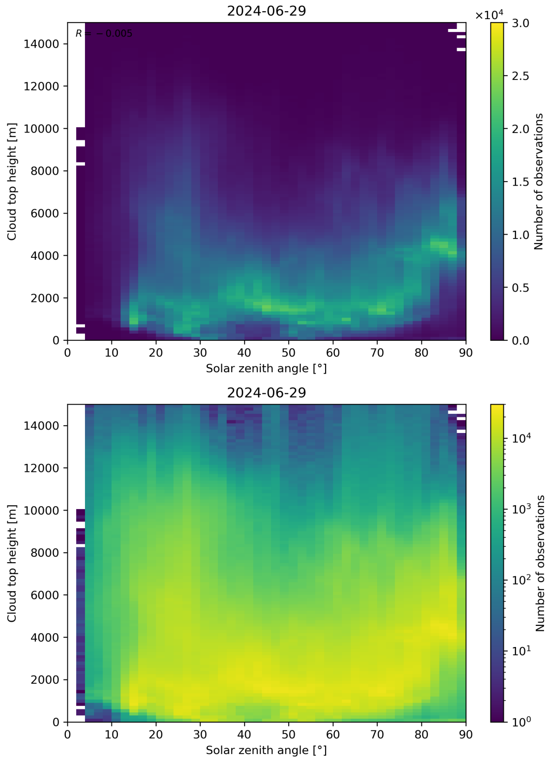
Figure 104: Scatter density plot of “Solar zenith angle” against “Cloud top height” for 2024-06-29 to 2024-06-30.
