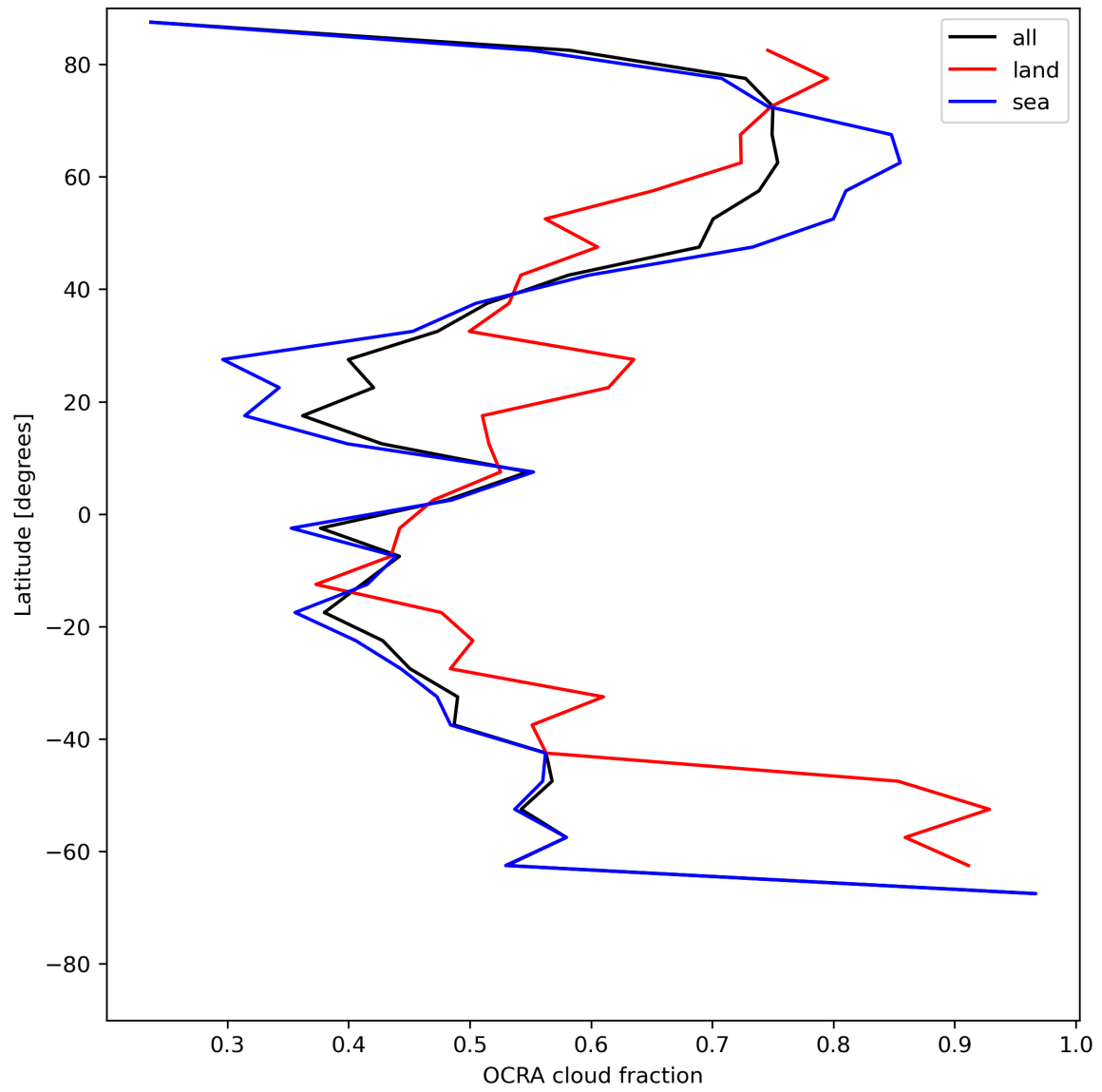
Figure 34: Zonal average of “OCRA cloud fraction” for 2024-06-29 to 2024-06-30.
