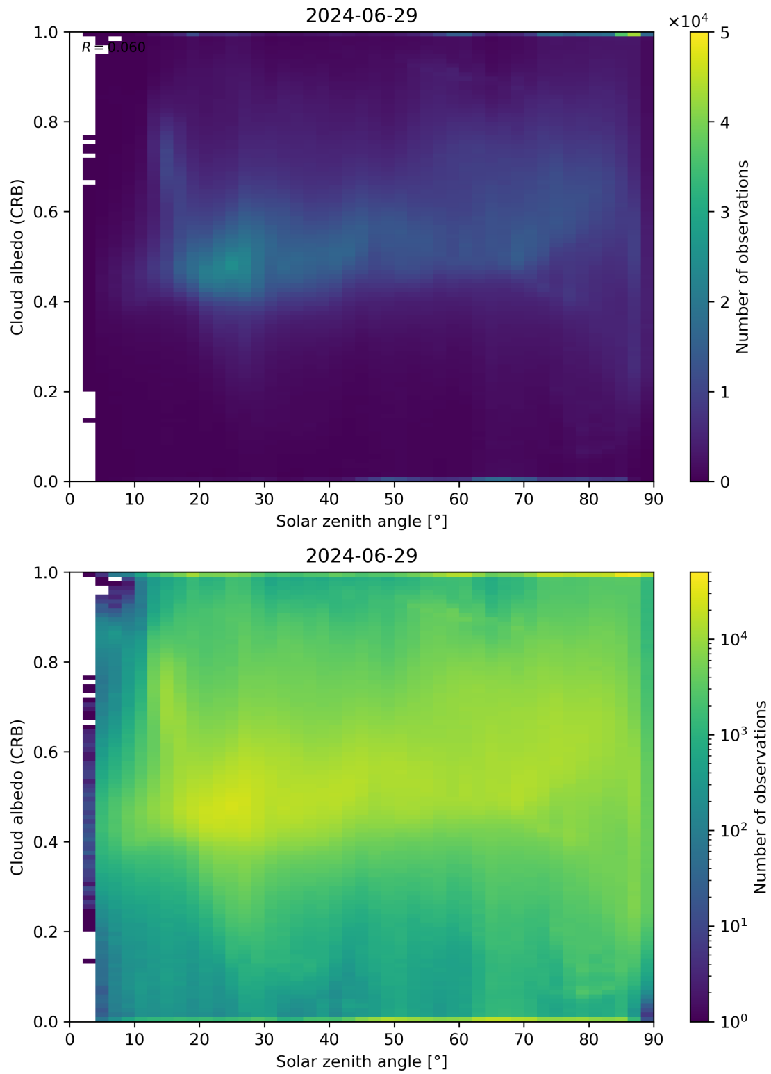
Figure 98: Scatter density plot of “Solar zenith angle” against “Cloud albedo (CRB)” for 2024-06-29 to 2024-06-30.
