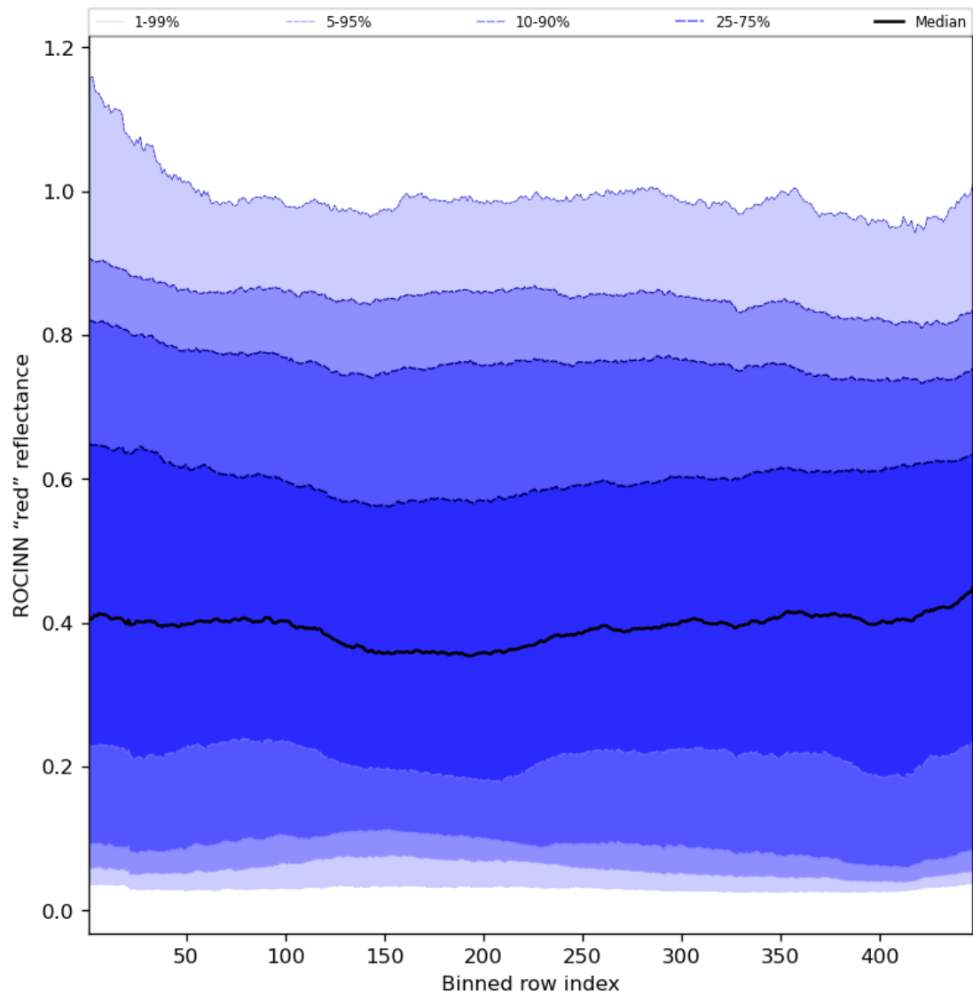
Figure 69: Along track statistics of “ROCINN “red” reflectance” for 2024-06-29 to 2024-06-30
