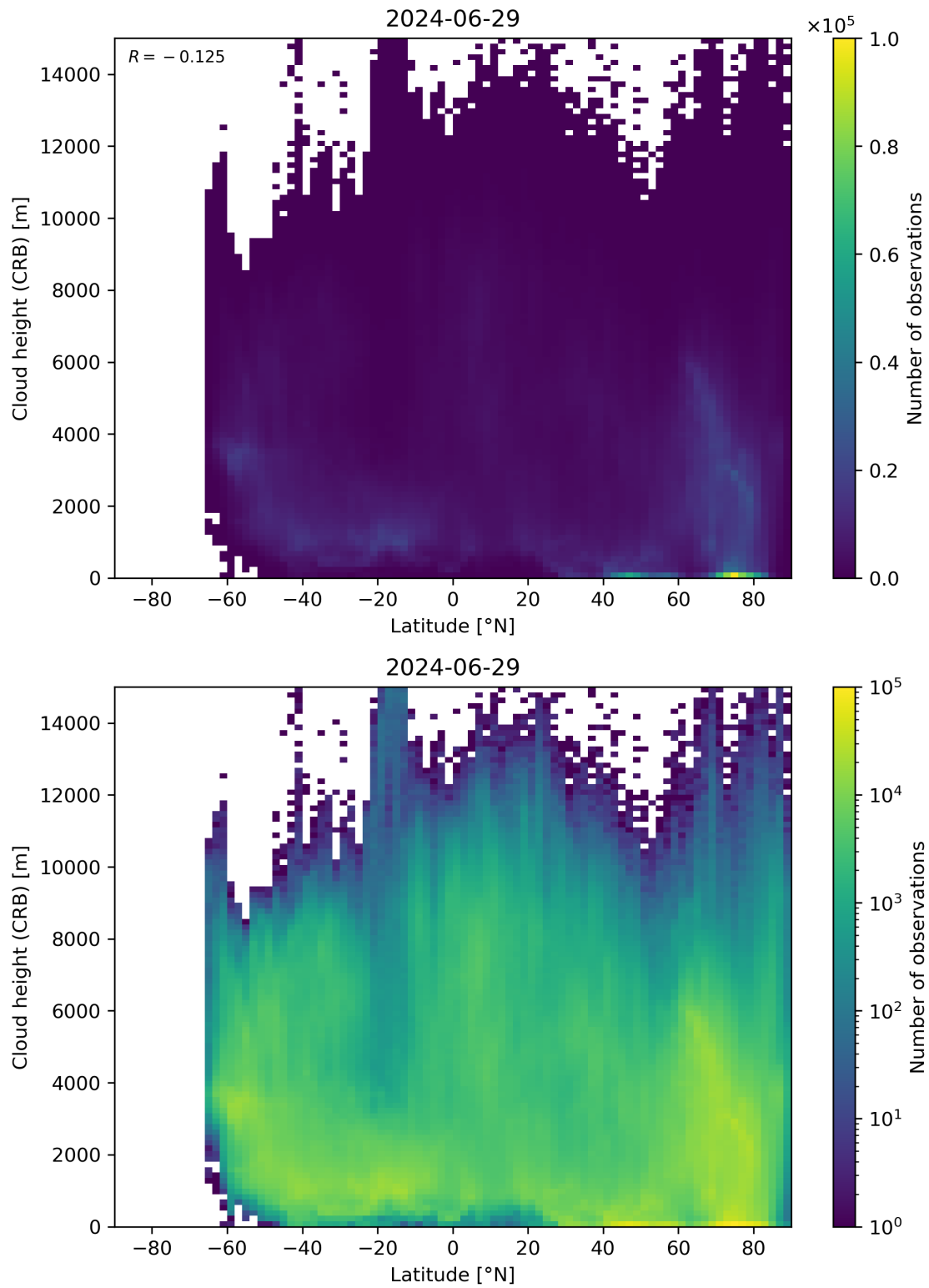
Figure 95: Scatter density plot of “Latitude” against “Cloud height (CRB)” for 2024-06-29 to 2024-06-30.
