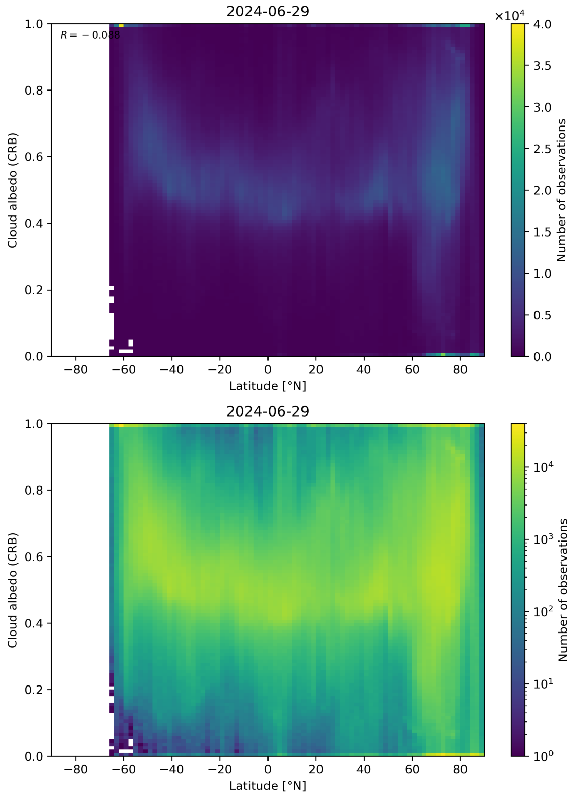
Figure 91: Scatter density plot of “Latitude” against “Cloud albedo (CRB)” for 2024-06-29 to 2024-06-30.
