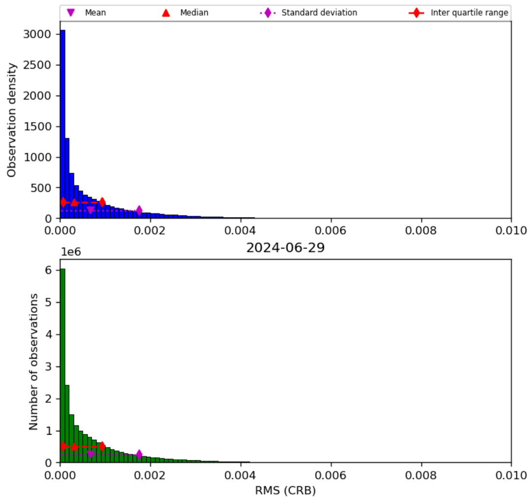
Figure 48: Histogram of “RMS (CRB)” for 2024-06-29 to 2024-06-30
