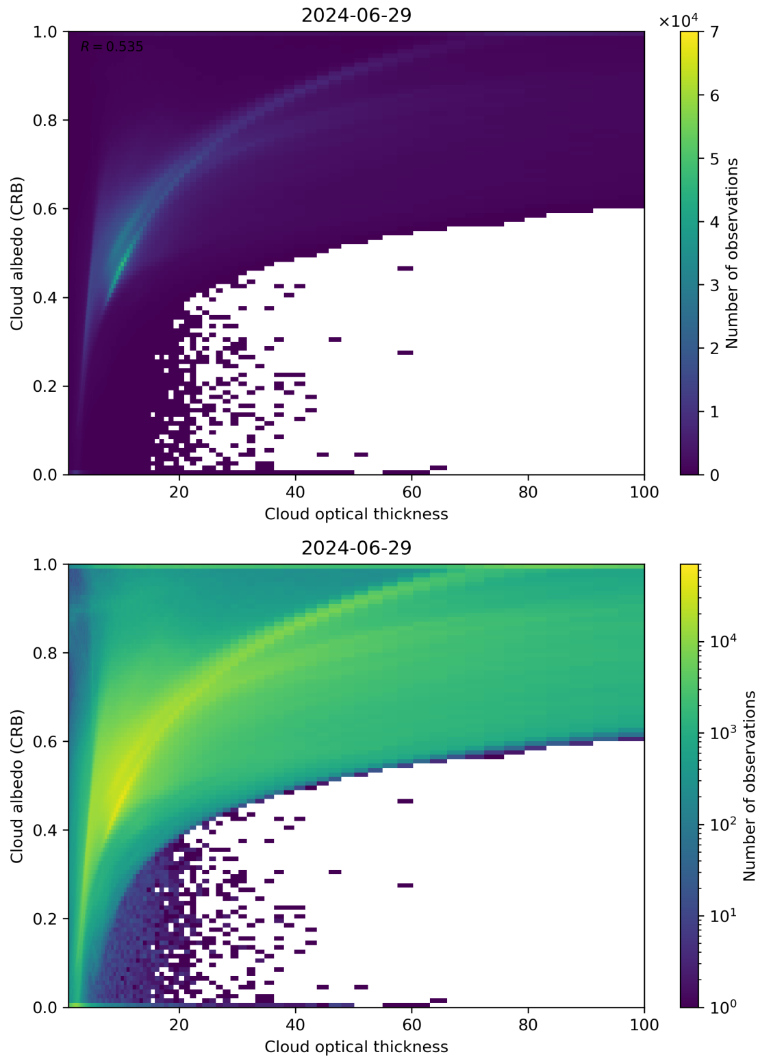
Figure 82: Scatter density plot of “Cloud optical thickness” against “Cloud albedo (CRB)” for 2024-06-29 to 2024-06-30.
