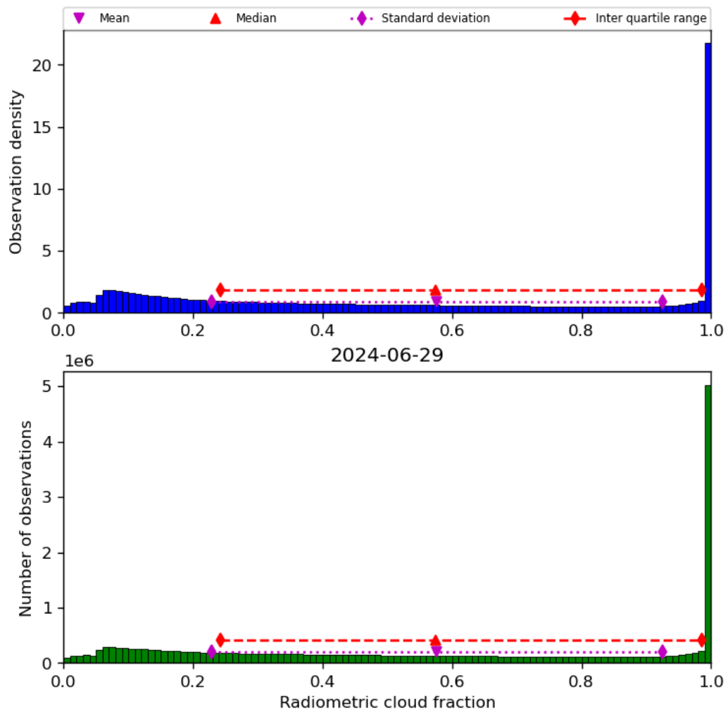
Figure 39: Histogram of “Radiometric cloud fraction” for 2024-06-29 to 2024-06-30
