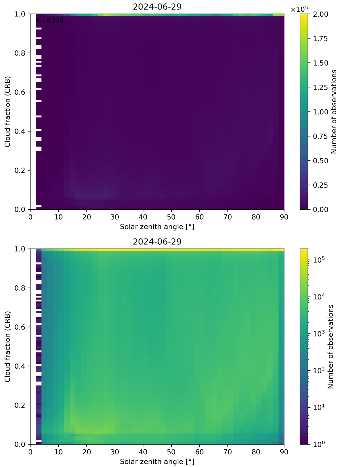
Figure 101: Scatter density plot of “Solar zenith angle” against “Cloud fraction (CRB)” for 2024-06-29 to 2024-06-30.
