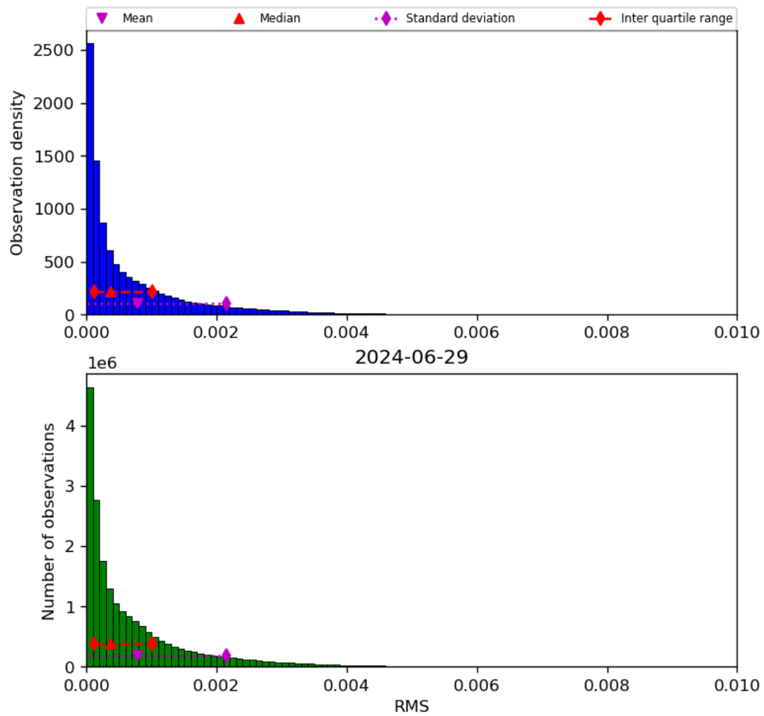
Figure 47: Histogram of “RMS” for 2024-06-29 to 2024-06-30
