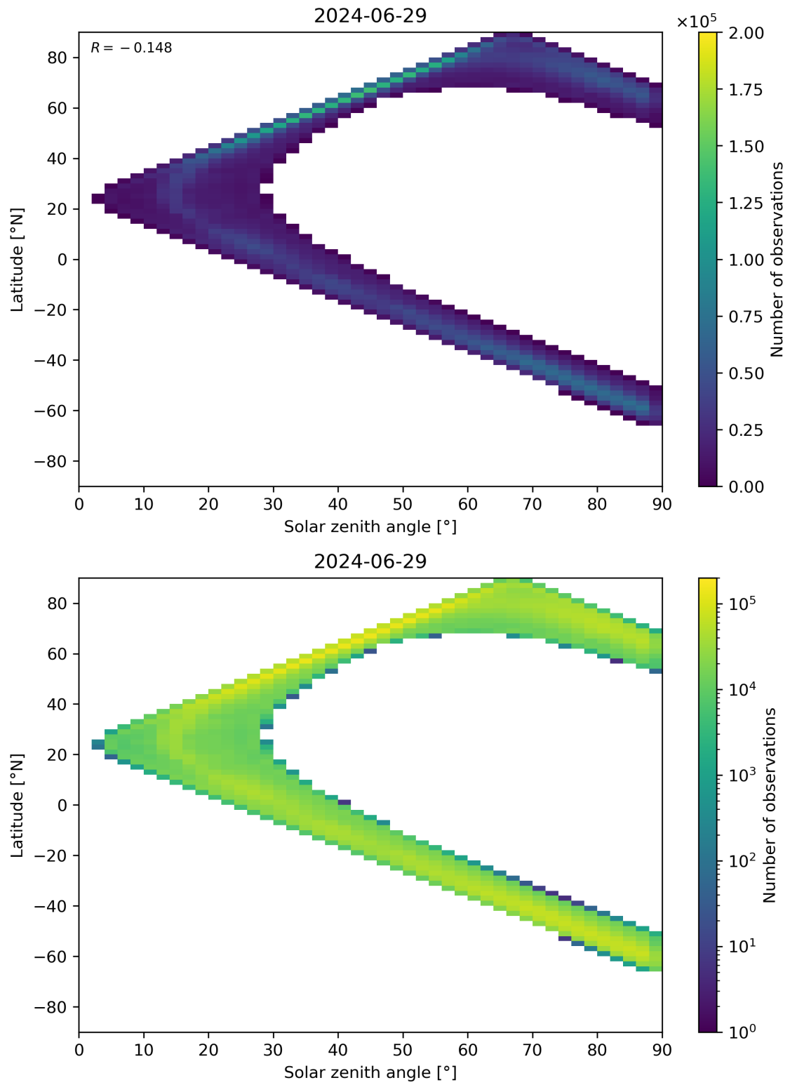
Figure 105: Scatter density plot of “Solar zenith angle” against “Latitude” for 2024-06-29 to 2024-06-30.
