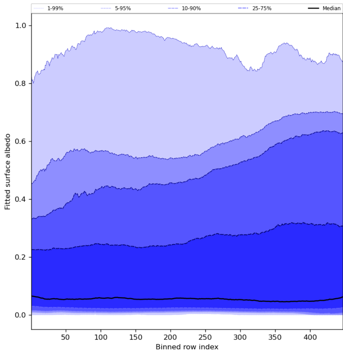
Figure 61: Along track statistics of “Fitted surface albedo” for 2024-06-29 to 2024-06-30
