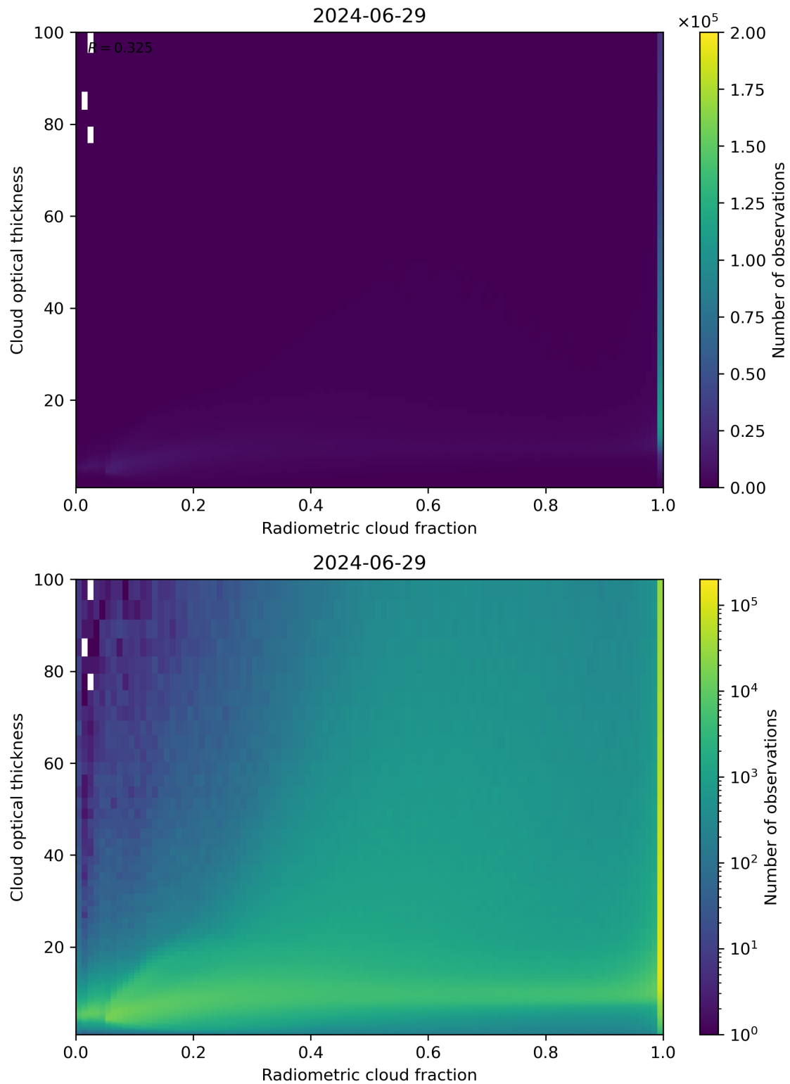
Figure 75: Scatter density plot of “Radiometric cloud fraction” against “Cloud optical thickness” for 2024-06-29 to 2024-06-30.
