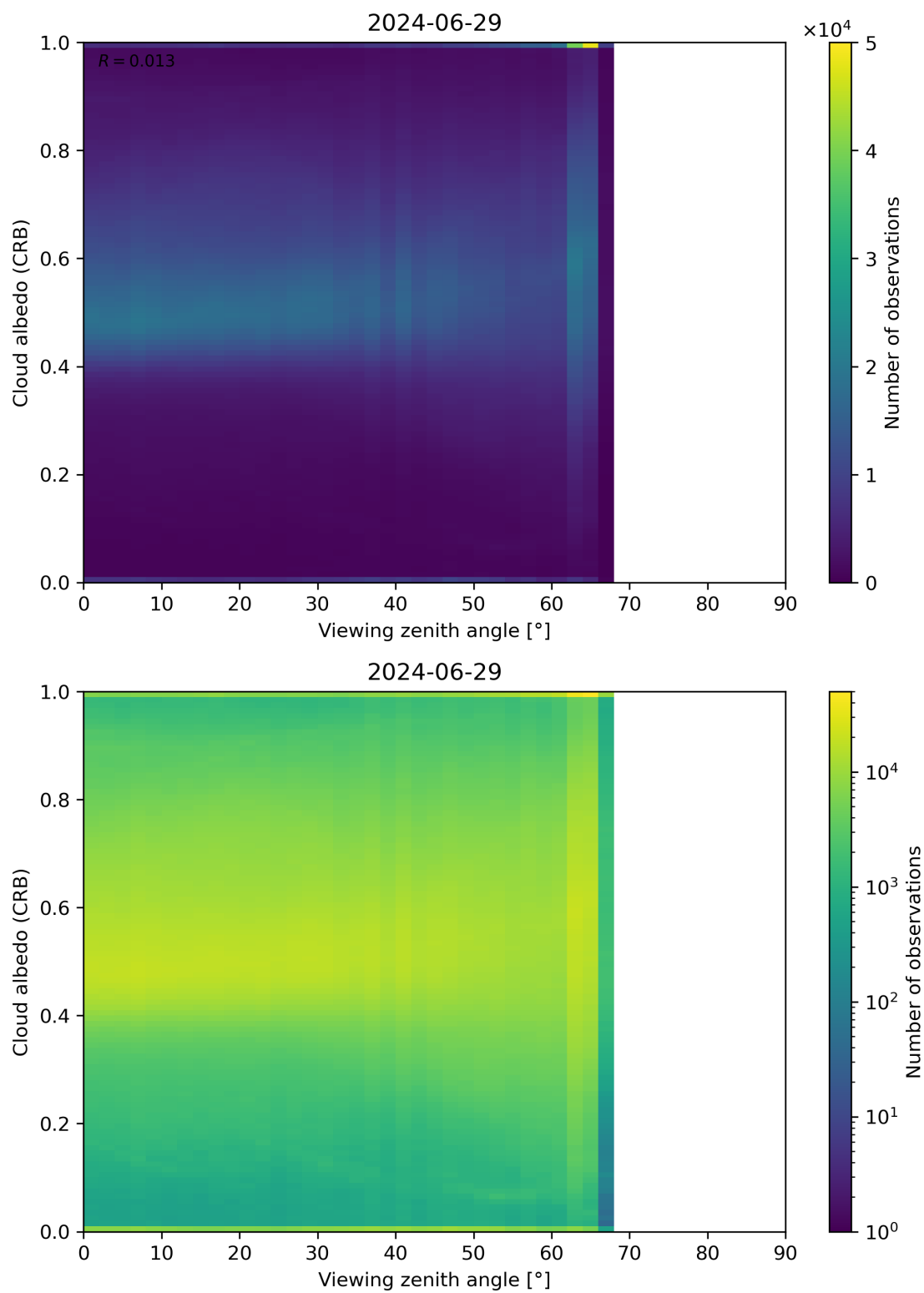
Figure 106: Scatter density plot of “Viewing zenith angle” against “Cloud albedo (CRB)” for 2024-06-29 to 2024-06-30.
