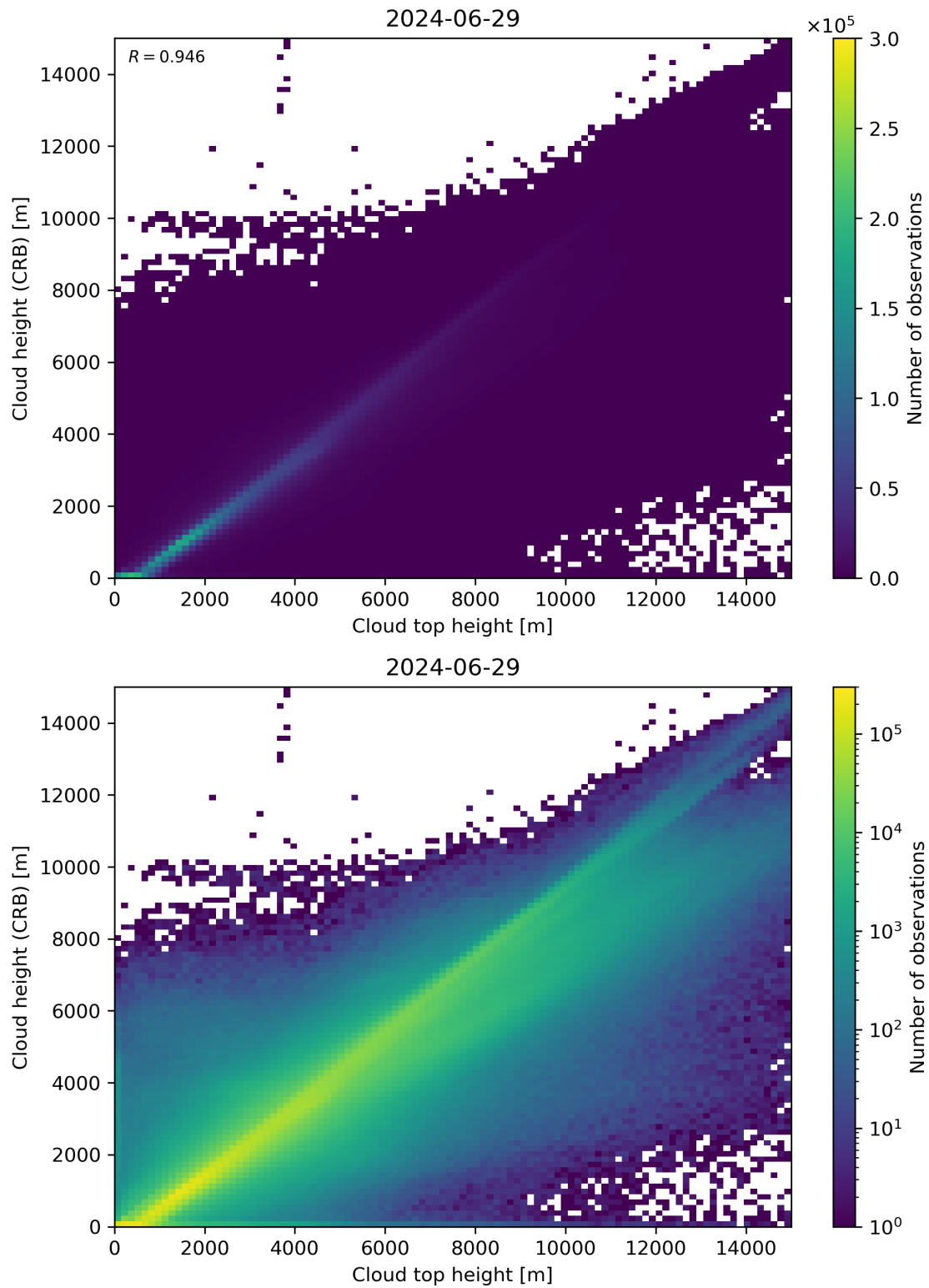
Figure 89: Scatter density plot of “Cloud top height” against “Cloud height (CRB)” for 2024-06-29 to 2024-06-30.
