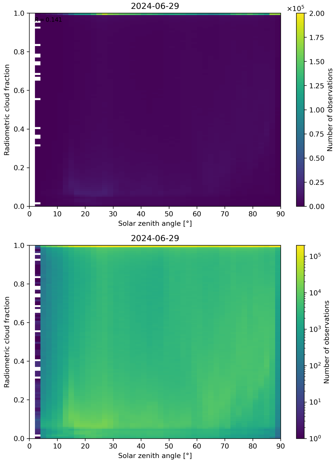
Figure 99: Scatter density plot of “Solar zenith angle” against “Radiometric cloud fraction” for 2024-06-29 to 2024-06-30.
