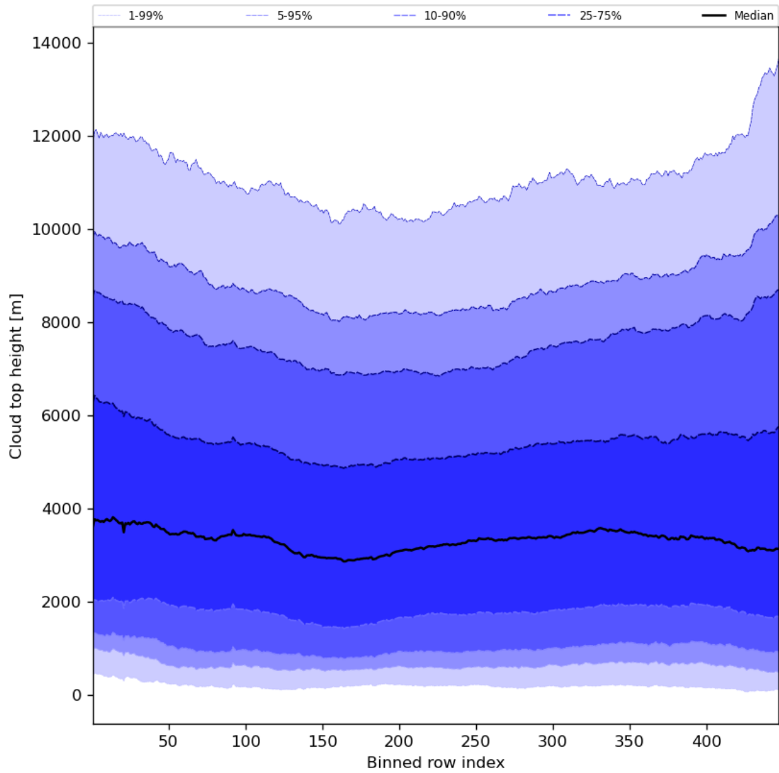
Figure 56: Along track statistics of “Cloud top height” for 2024-06-29 to 2024-06-30
