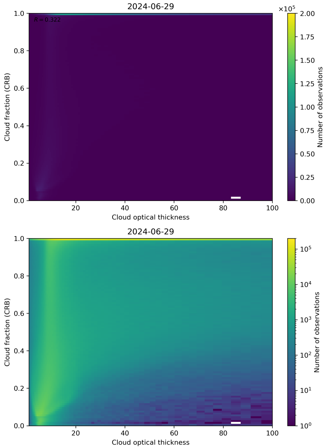
Figure 84: Scatter density plot of “Cloud optical thickness” against “Cloud fraction (CRB)” for 2024-06-29 to 2024-06-30.
