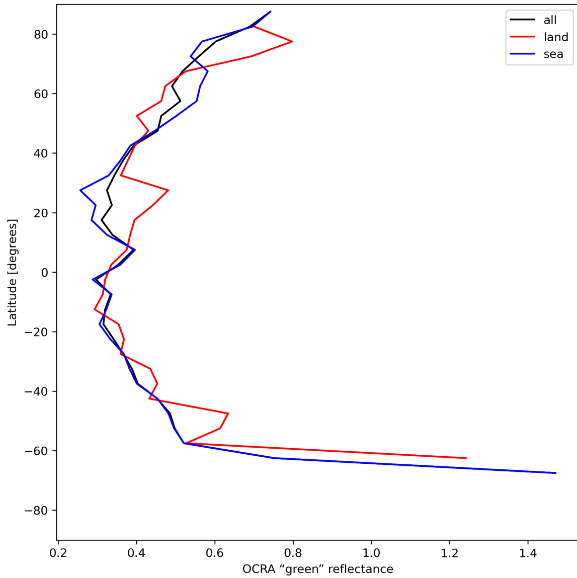
Figure 36: Zonal average of “OCRA “green” reflectance” for 2024-06-29 to 2024-06-30.
