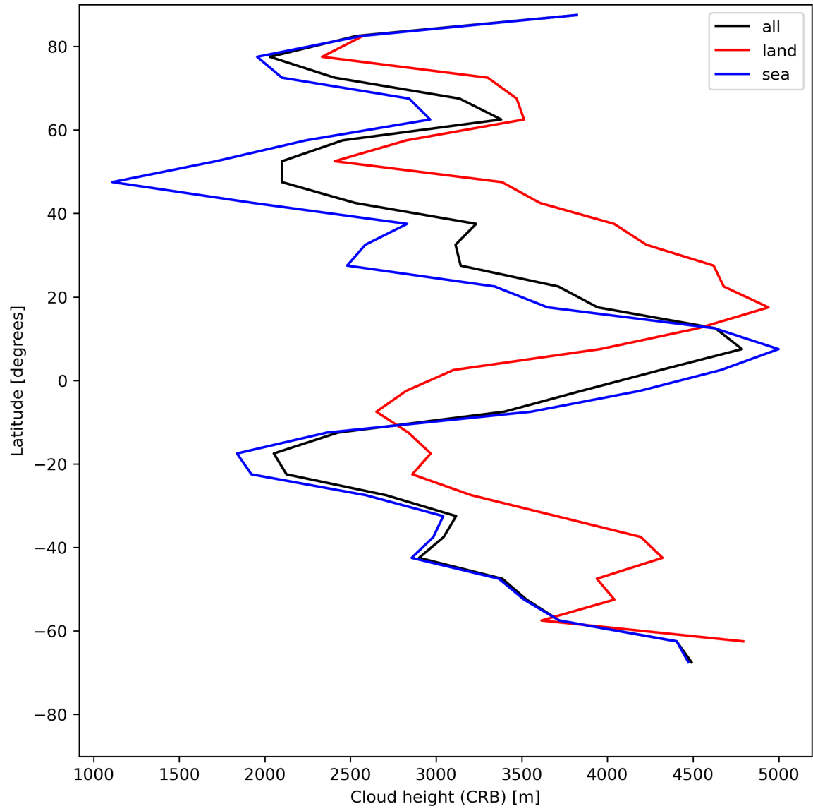
Figure 27: Zonal average of “Cloud height (CRB)” for 2024-06-29 to 2024-06-30.
