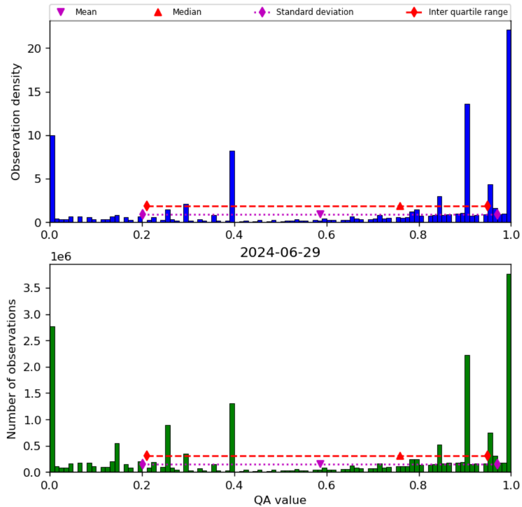
Figure 38: Histogram of “QA value” for 2024-06-29 to 2024-06-30
