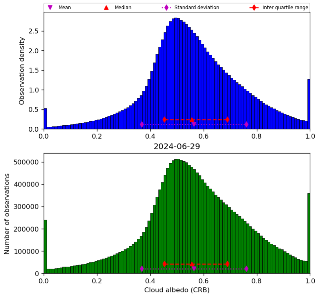
Figure 44: Histogram of “Cloud albedo (CRB)” for 2024-06-29 to 2024-06-30
