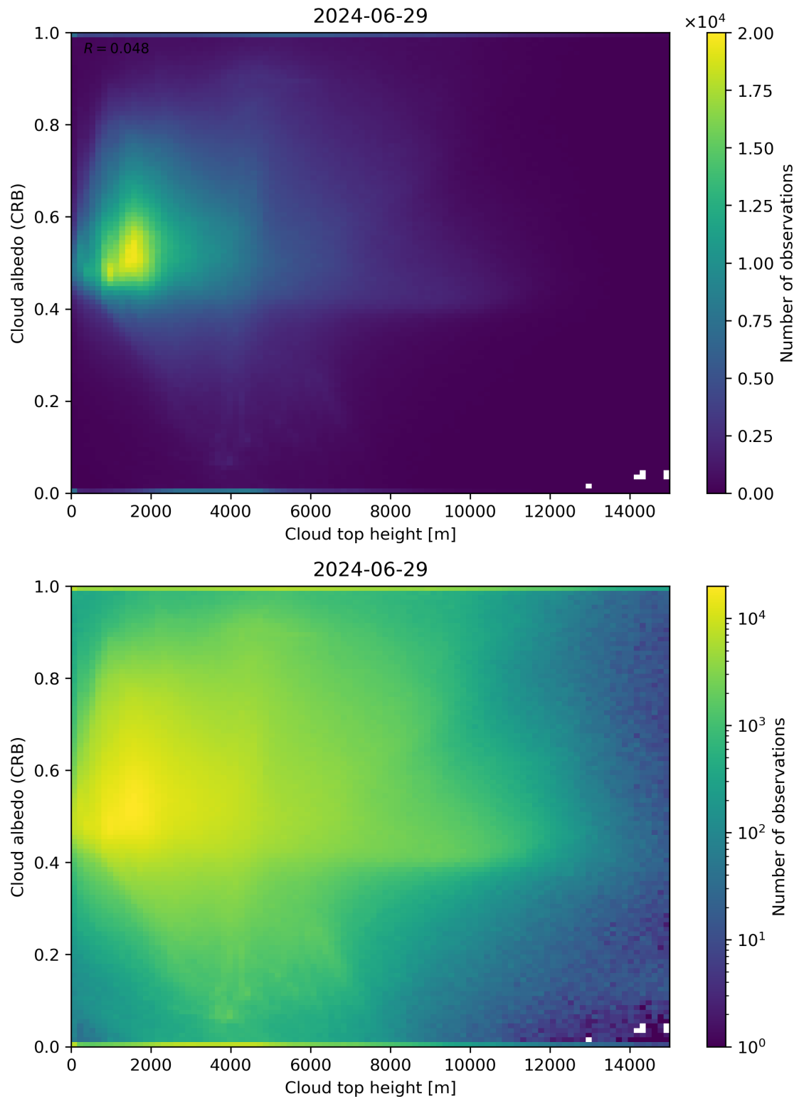
Figure 86: Scatter density plot of “Cloud top height” against “Cloud albedo (CRB)” for 2024-06-29 to 2024-06-30.
