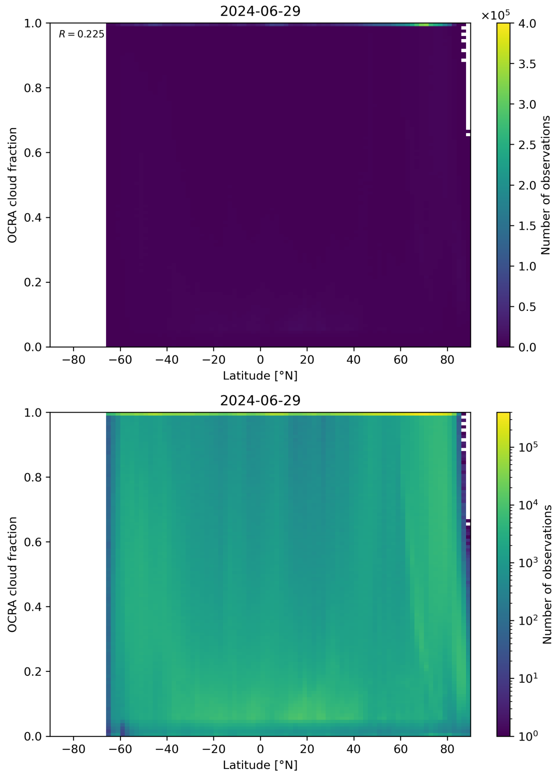
Figure 93: Scatter density plot of “Latitude” against “OCRA cloud fraction” for 2024-06-29 to 2024-06-30.
