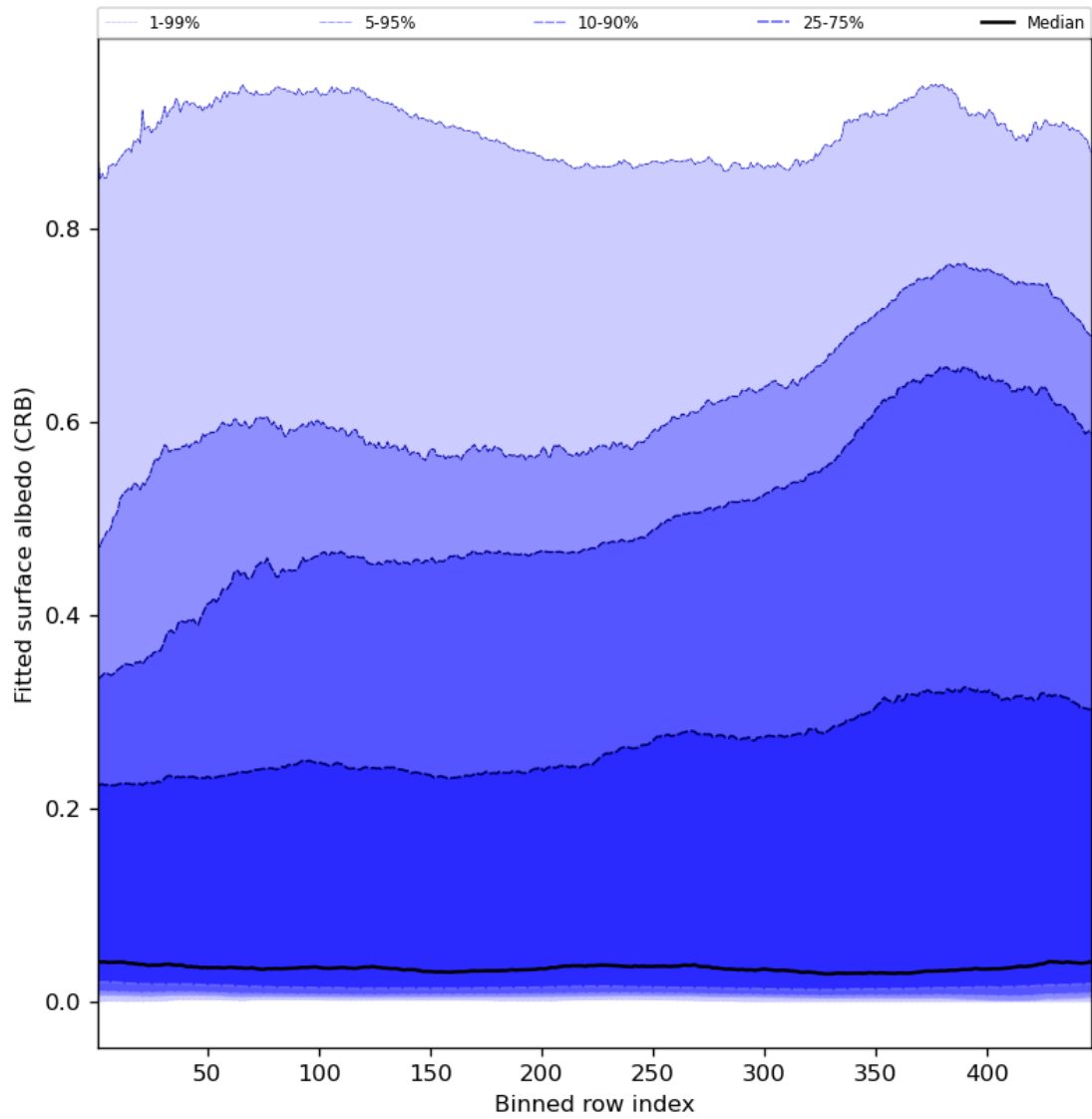
Figure 62: Along track statistics of “Fitted surface albedo (CRB)” for 2024-06-29 to 2024-06-30
