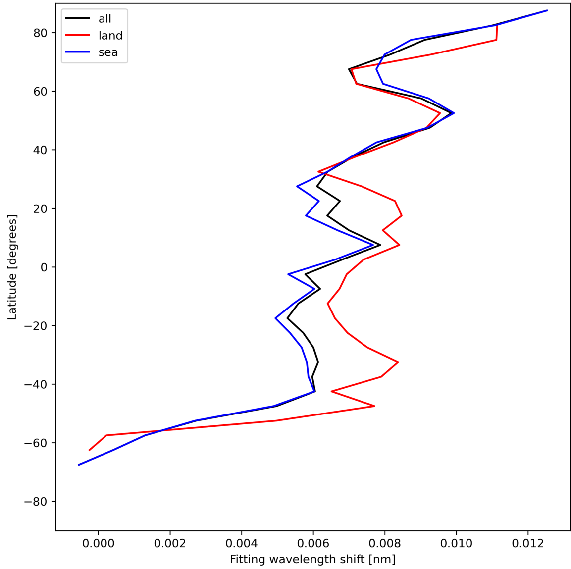
Figure 33: Zonal average of “Fitting wavelength shift” for 2024-06-29 to 2024-06-30.
