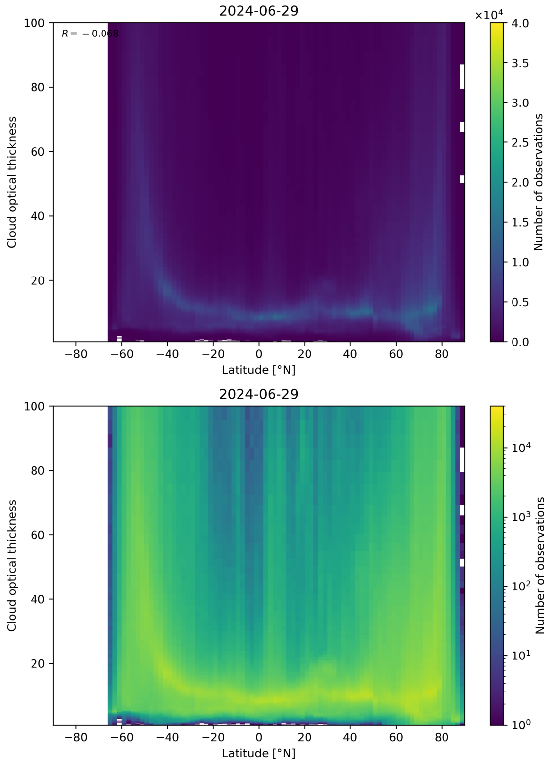
Figure 96: Scatter density plot of “Latitude” against “Cloud optical thickness” for 2024-06-29 to 2024-06-30.
