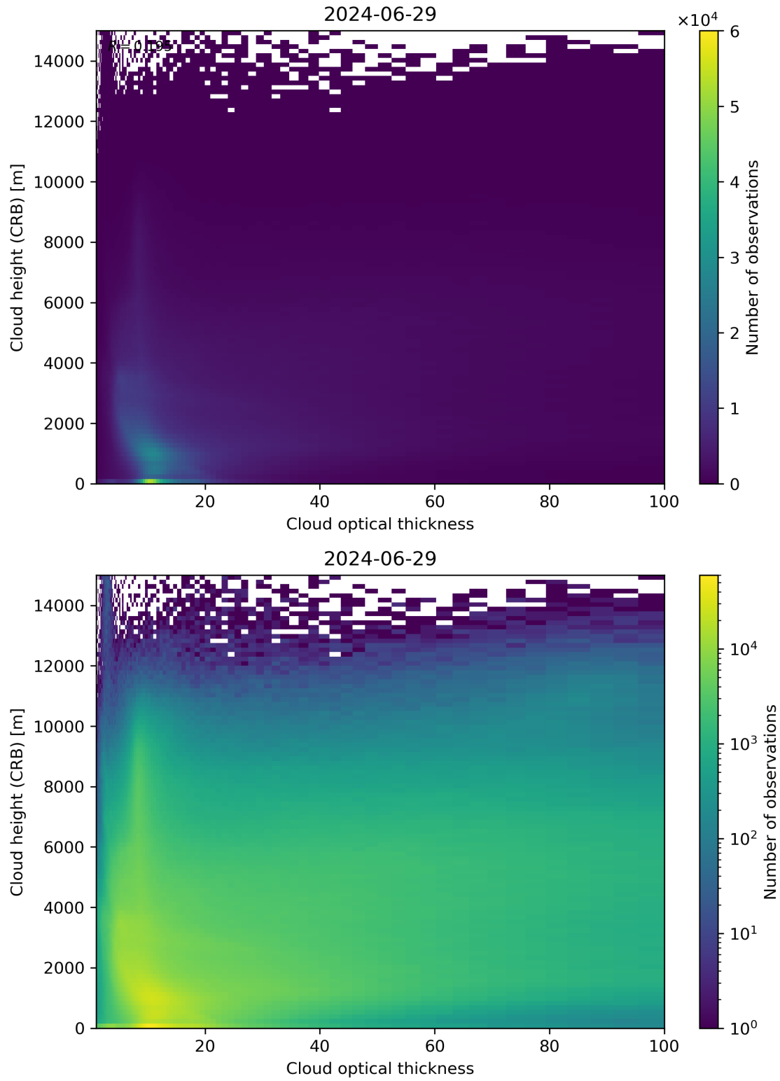
Figure 85: Scatter density plot of “Cloud optical thickness” against “Cloud height (CRB)” for 2024-06-29 to 2024-06-30.
