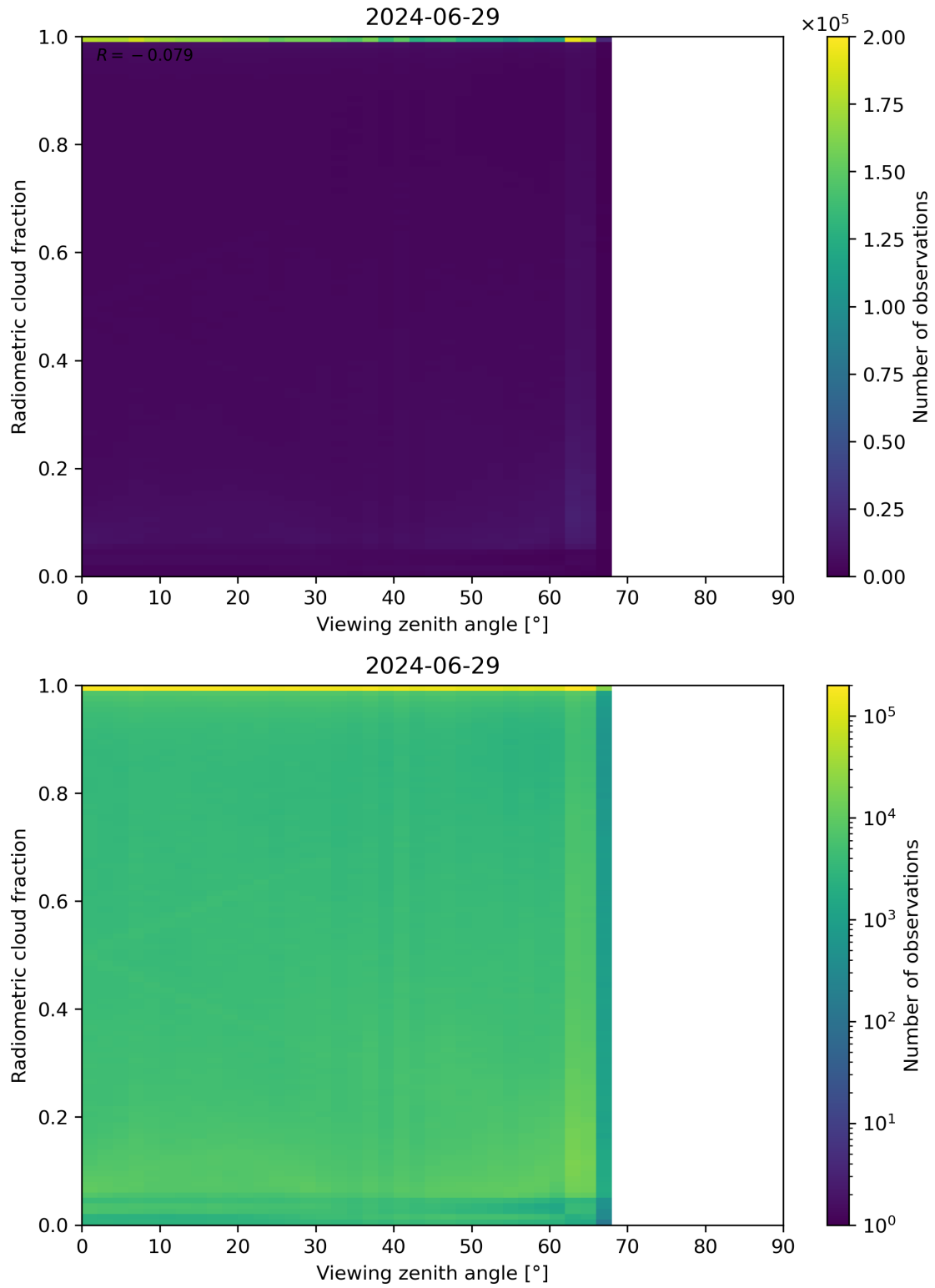
Figure 107: Scatter density plot of “Viewing zenith angle” against “Radiometric cloud fraction” for 2024-06-29 to 2024-06-30.
