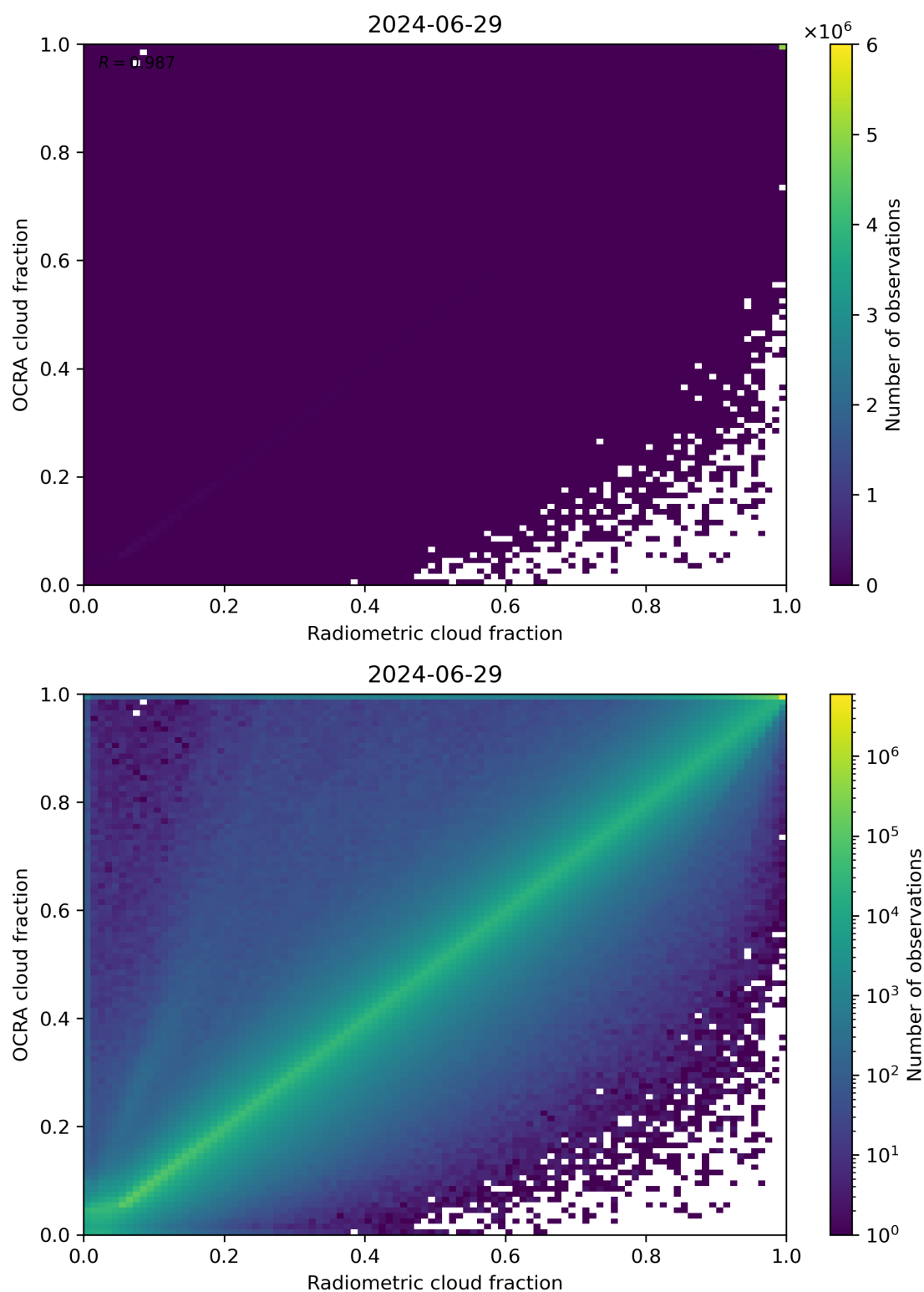
Figure 72: Scatter density plot of “Radiometric cloud fraction” against “OCRA cloud fraction” for 2024-06-29 to 2024-06-30.
