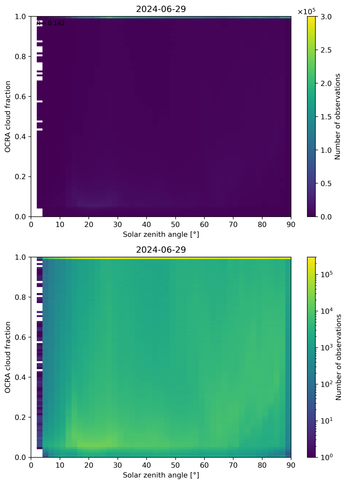
Figure 100: Scatter density plot of “Solar zenith angle” against “OCRA cloud fraction” for 2024-06-29 to 2024-06-30.
