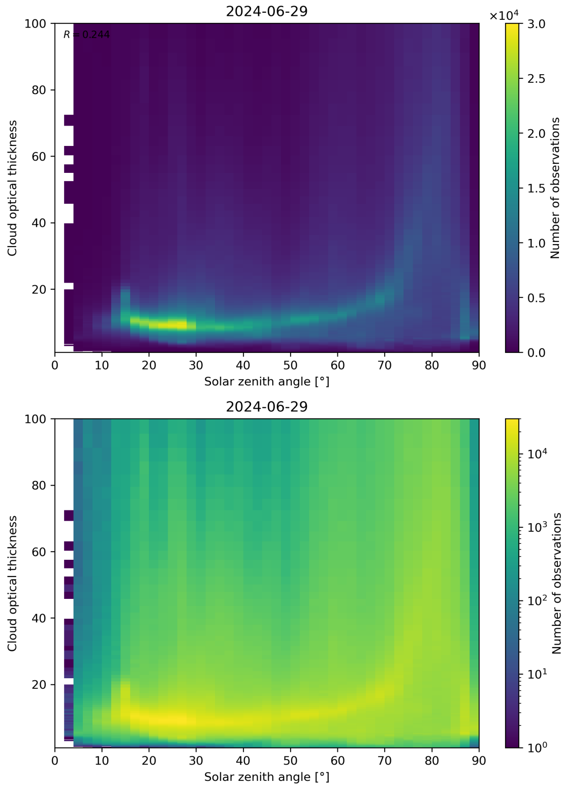
Figure 103: Scatter density plot of “Solar zenith angle” against “Cloud optical thickness” for 2024-06-29 to 2024-06-30.
