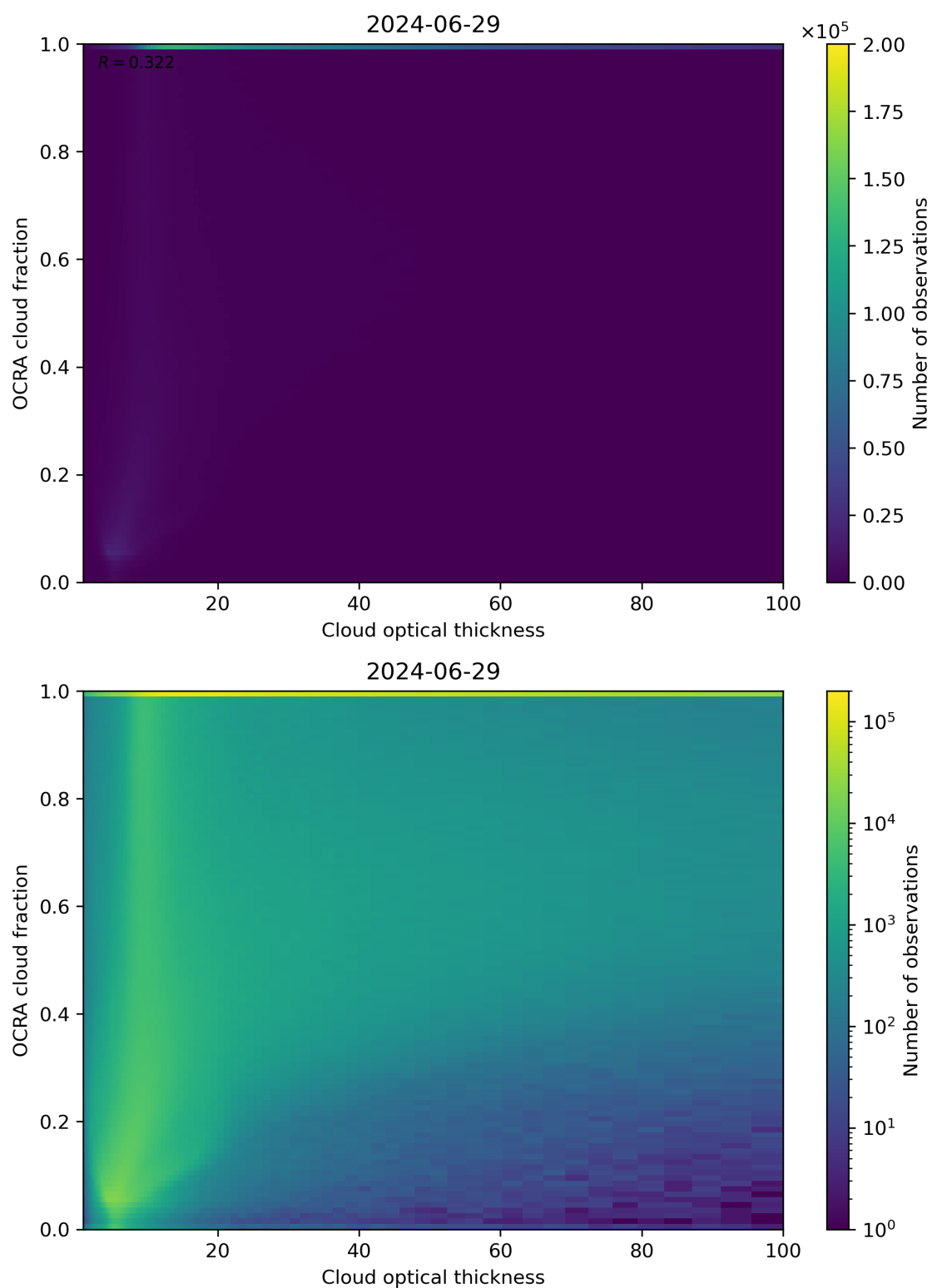
Figure 83: Scatter density plot of “Cloud optical thickness” against “OCRA cloud fraction” for 2024-06-29 to 2024-06-30.
