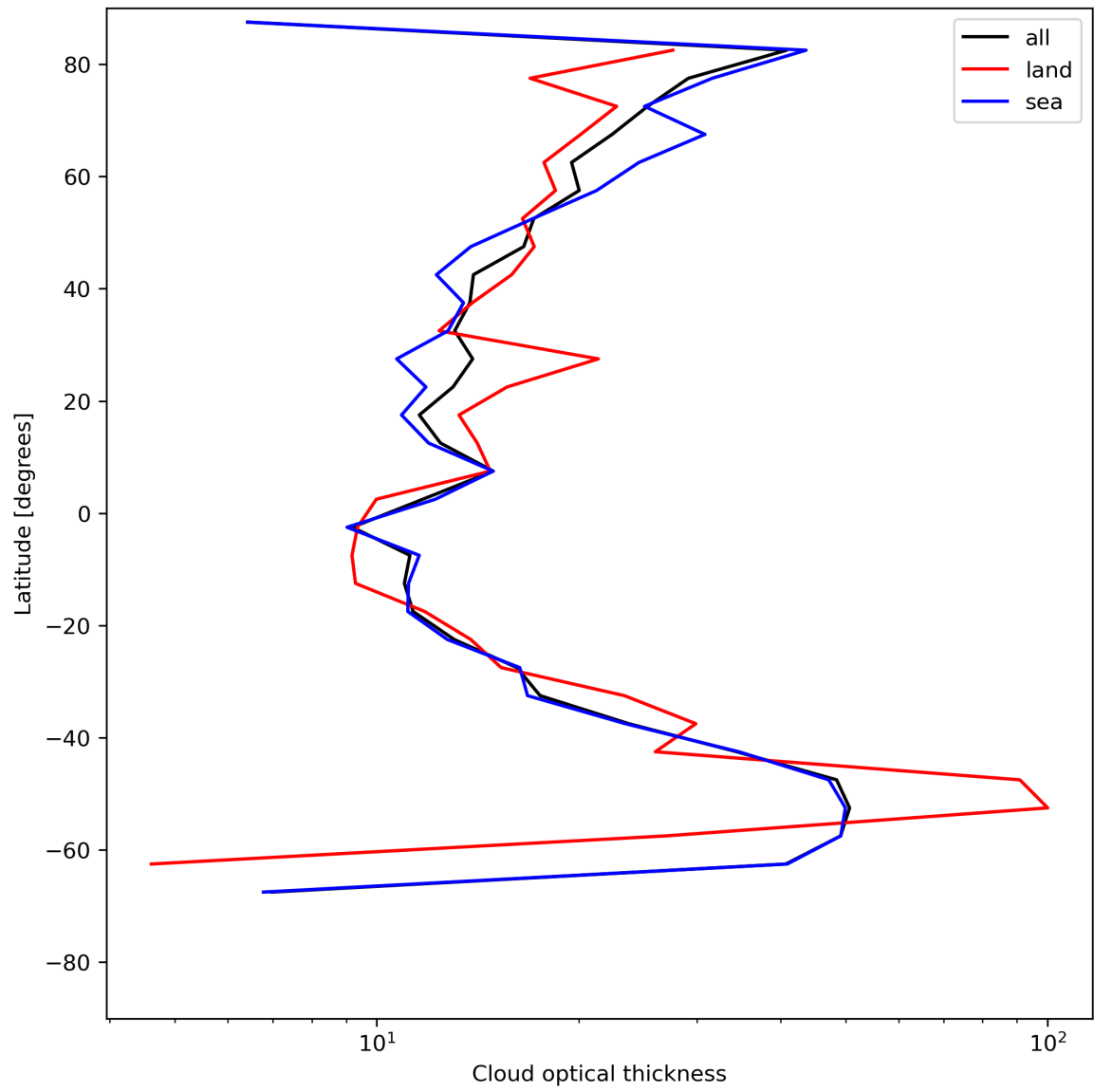
Figure 25: Zonal average of “Cloud optical thickness” for 2024-06-29 to 2024-06-30.
