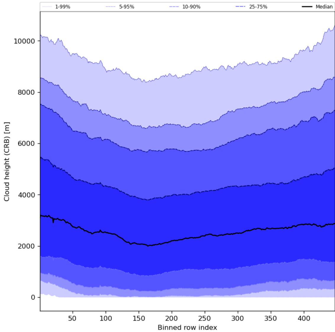
Figure 59: Along track statistics of “Cloud height (CRB)” for 2024-06-29 to 2024-06-30
