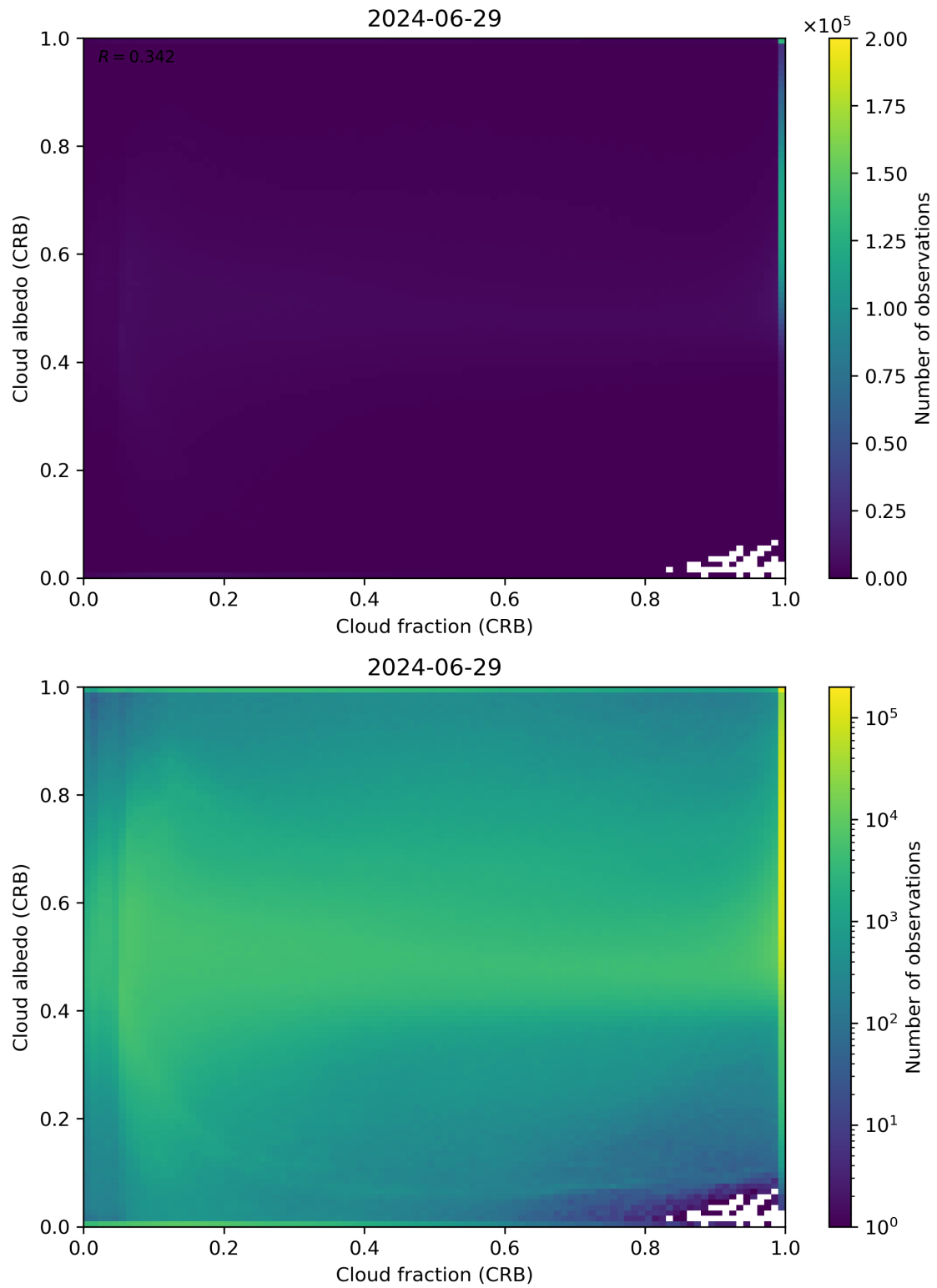
Figure 77: Scatter density plot of “Cloud fraction (CRB)” against “Cloud albedo (CRB)” for 2024-06-29 to 2024-06-30.
