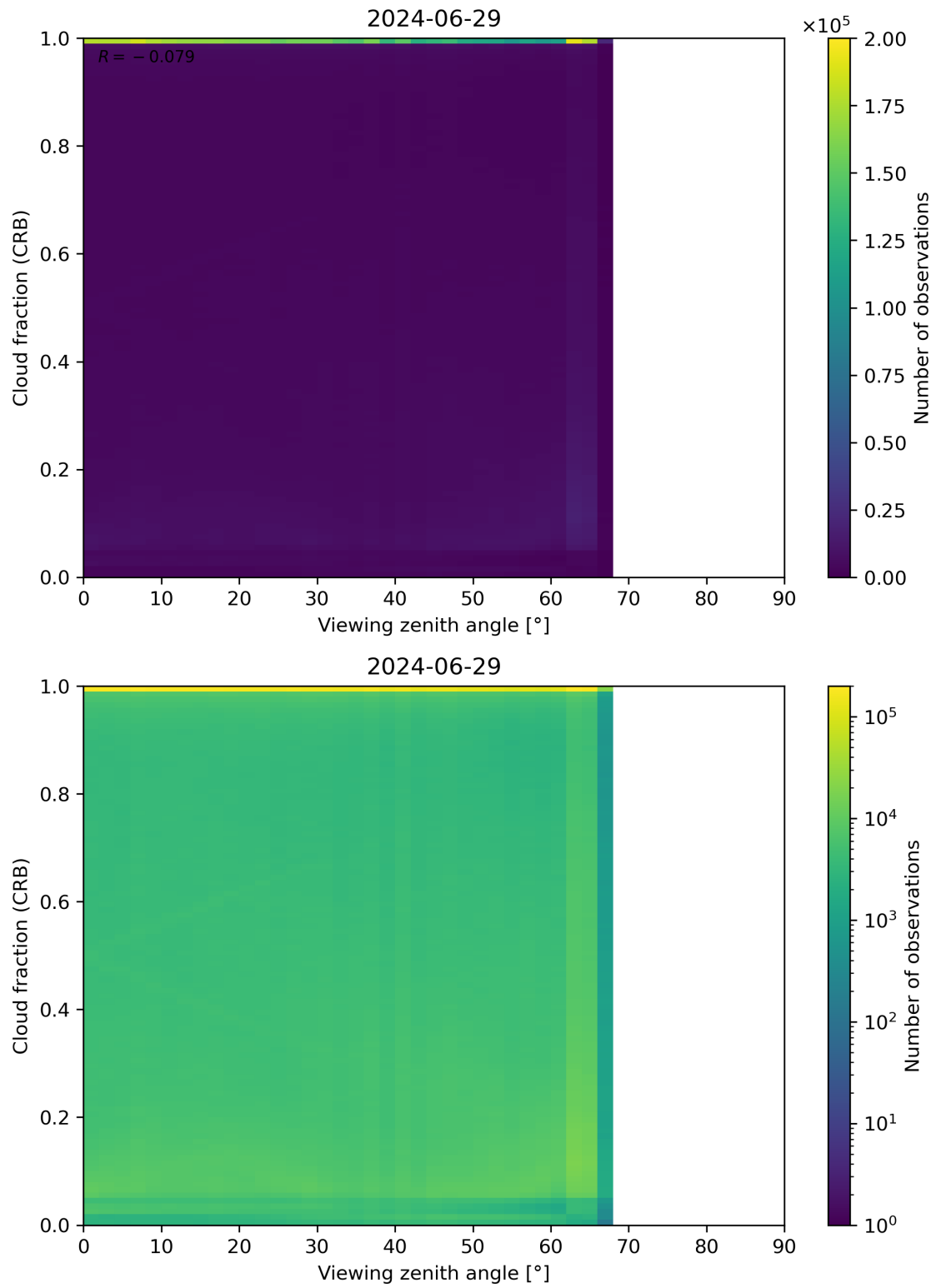
Figure 109: Scatter density plot of “Viewing zenith angle” against “Cloud fraction (CRB)” for 2024-06-29 to 2024-06-30.
