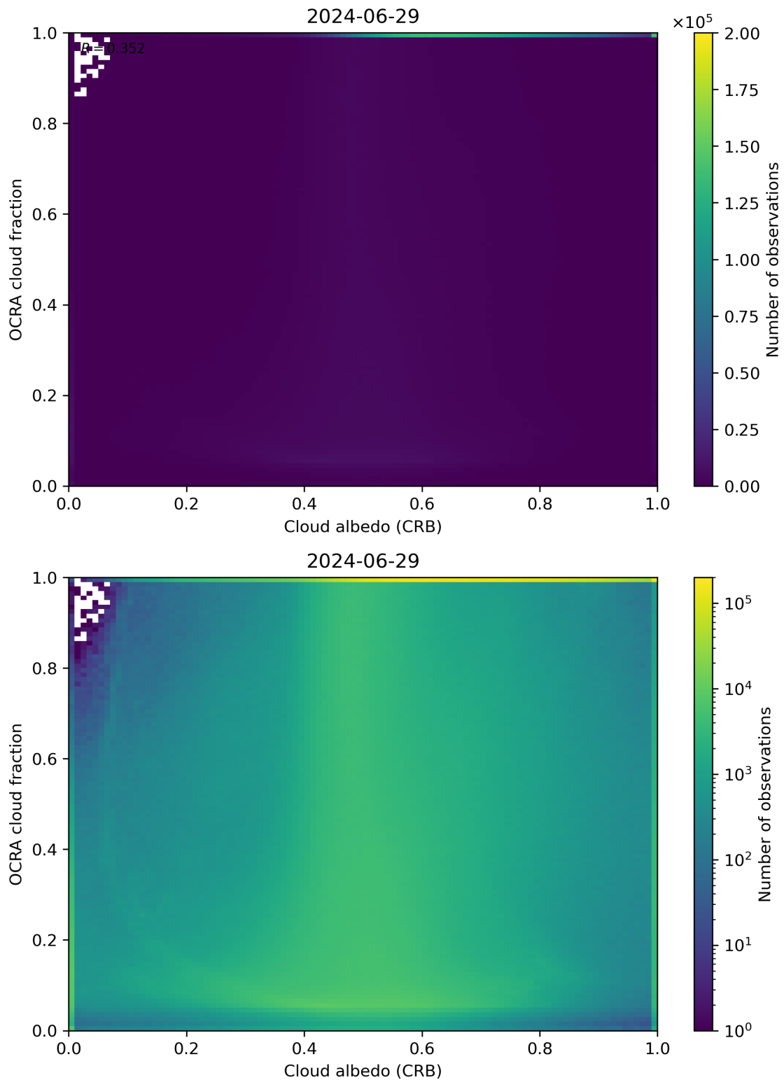
Figure 70: Scatter density plot of “Cloud albedo (CRB)” against “OCRA cloud fraction” for 2024-06-29 to 2024-06-30.
