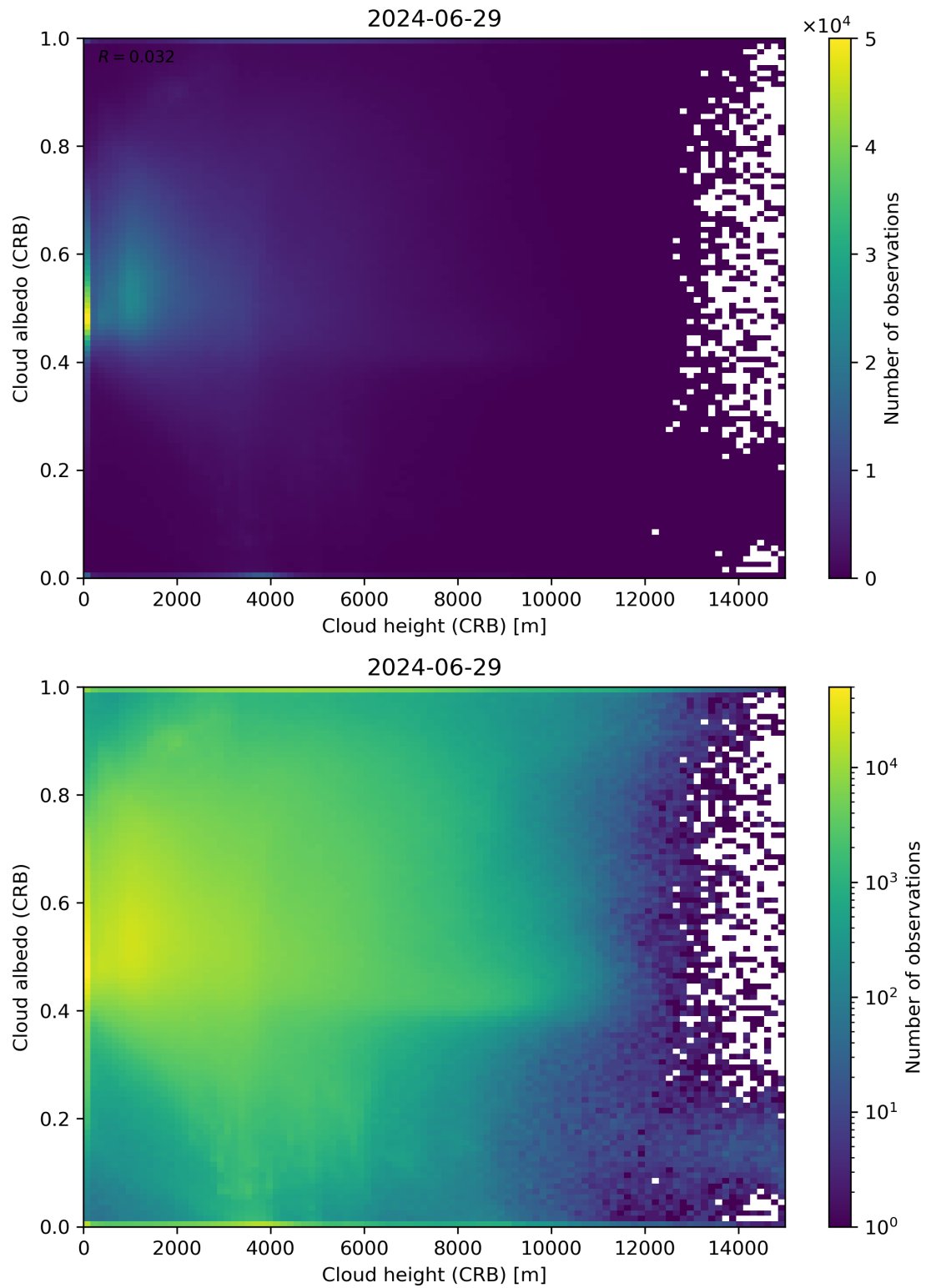
Figure 80: Scatter density plot of “Cloud height (CRB)” against “Cloud albedo (CRB)” for 2024-06-29 to 2024-06-30.
