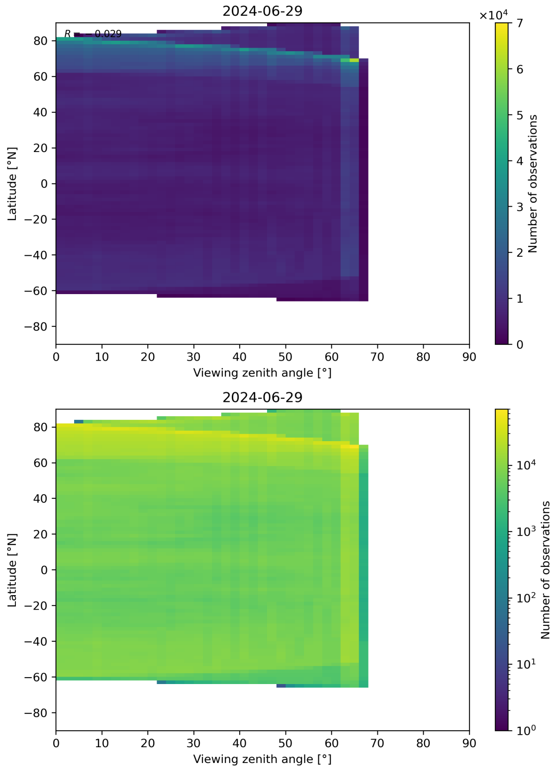
Figure 113: Scatter density plot of “Viewing zenith angle” against “Latitude” for 2024-06-29 to 2024-06-30.
