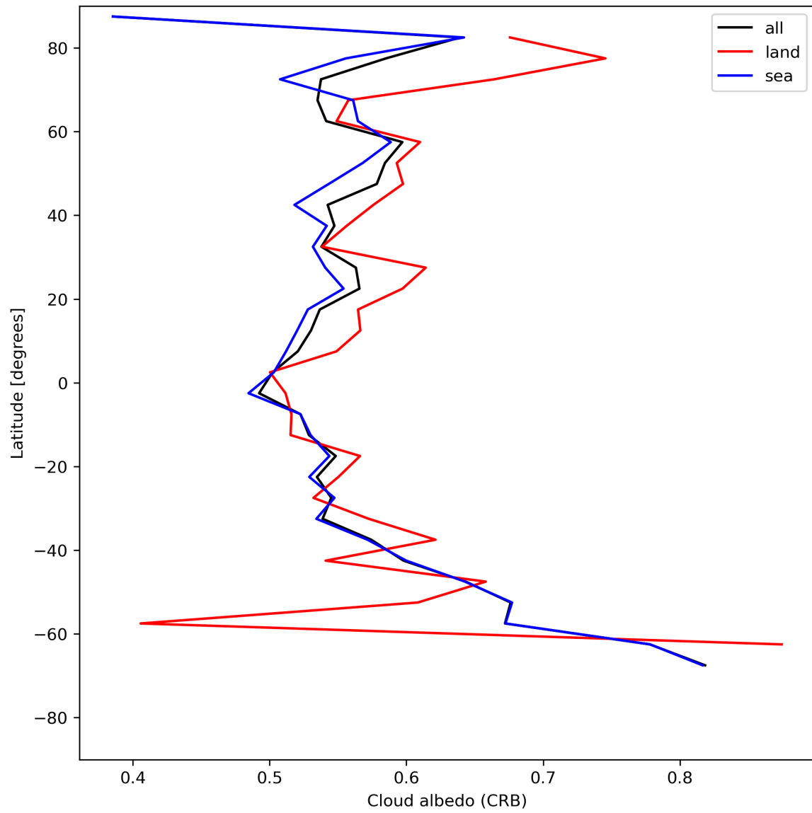
Figure 28: Zonal average of “Cloud albedo (CRB)” for 2024-06-29 to 2024-06-30.
