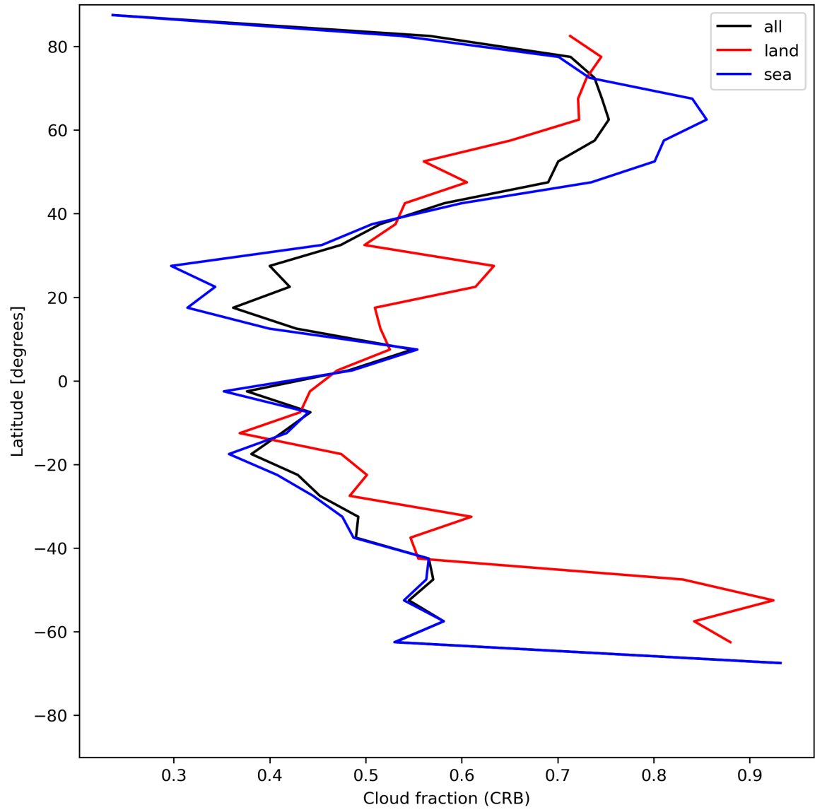
Figure 26: Zonal average of “Cloud fraction (CRB)” for 2024-06-29 to 2024-06-30.
