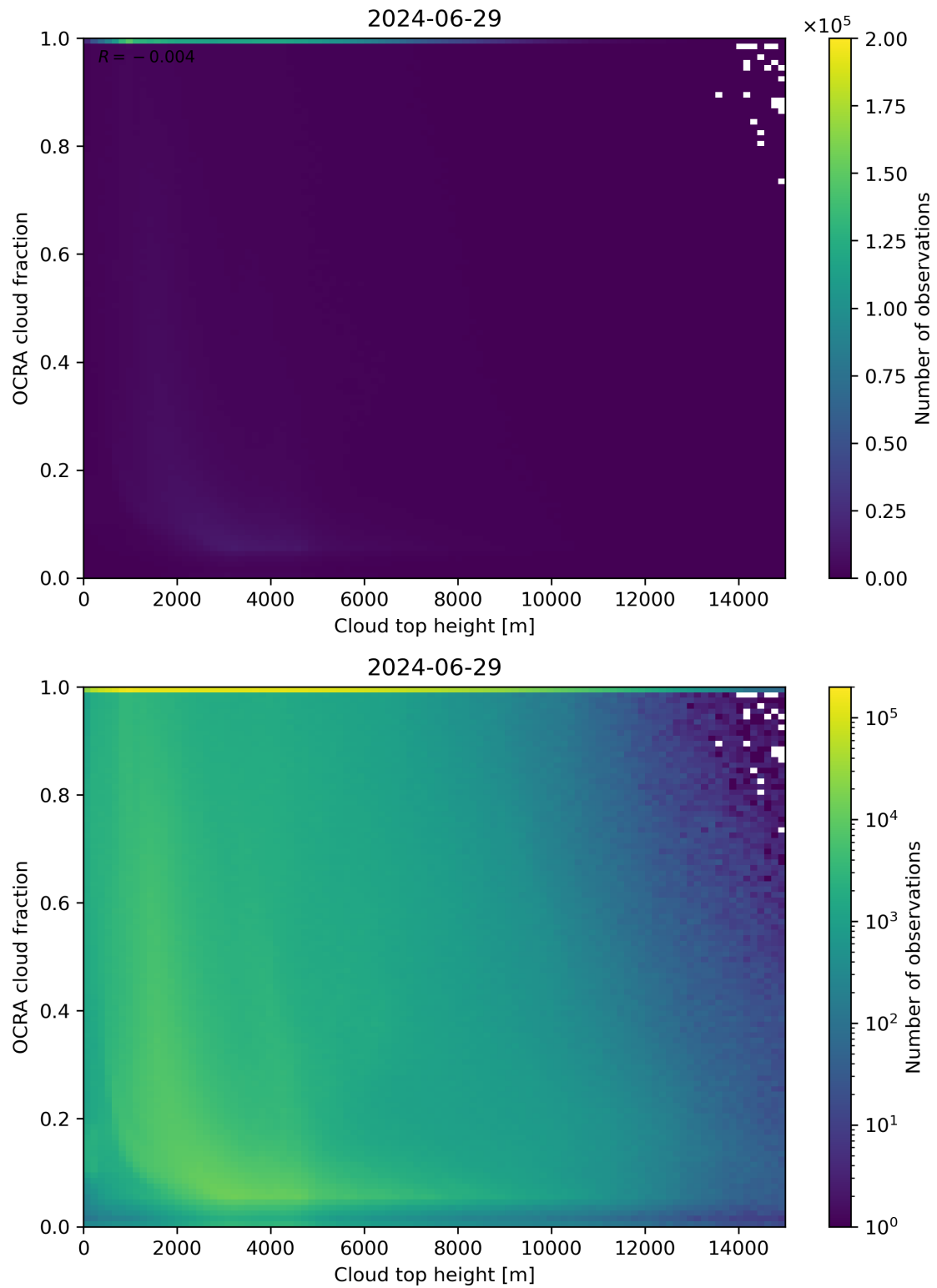
Figure 87: Scatter density plot of “Cloud top height” against “OCRA cloud fraction” for 2024-06-29 to 2024-06-30.
