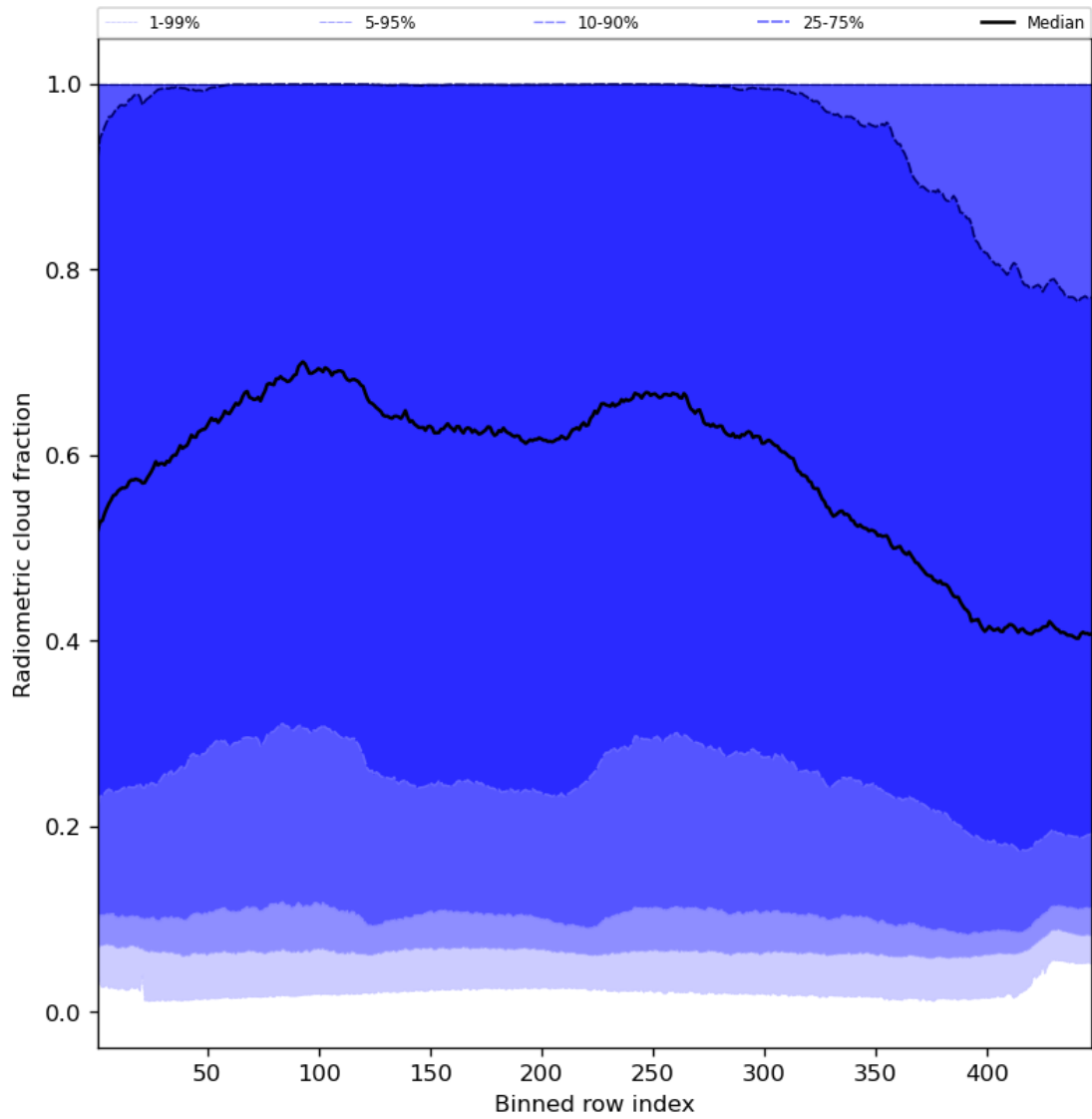
Figure 55: Along track statistics of “Radiometric cloud fraction” for 2024-06-29 to 2024-06-30
