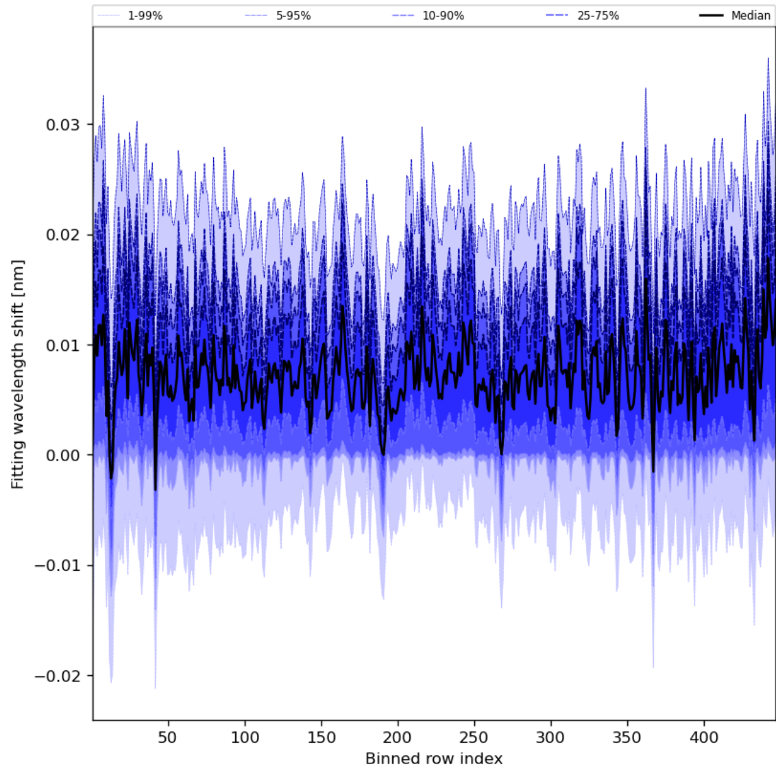
Figure 65: Along track statistics of “Fitting wavelength shift” for 2024-06-29 to 2024-06-30
