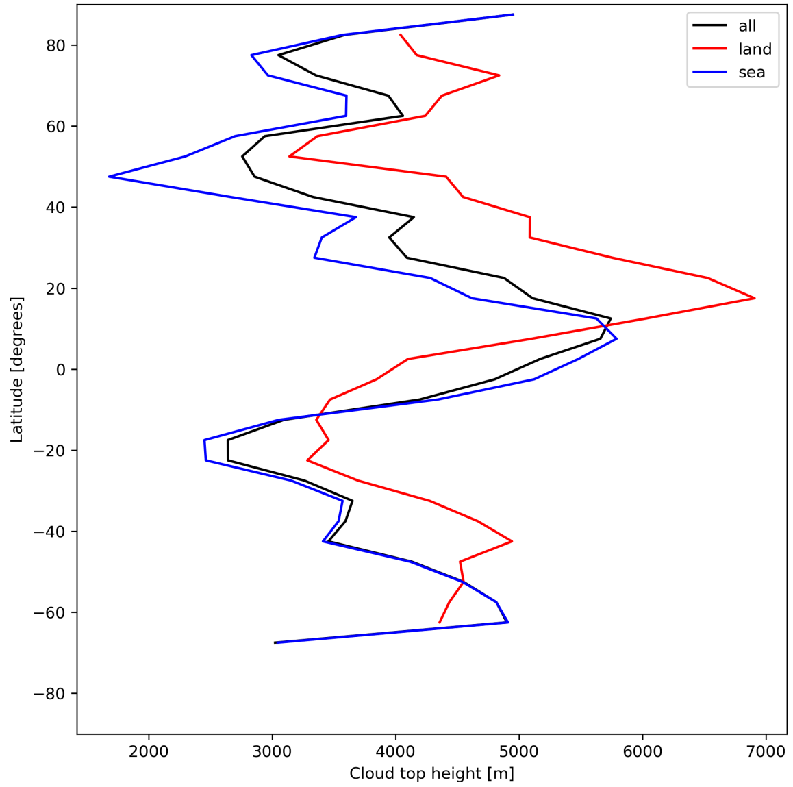
Figure 24: Zonal average of “Cloud top height” for 2024-06-29 to 2024-06-30.
