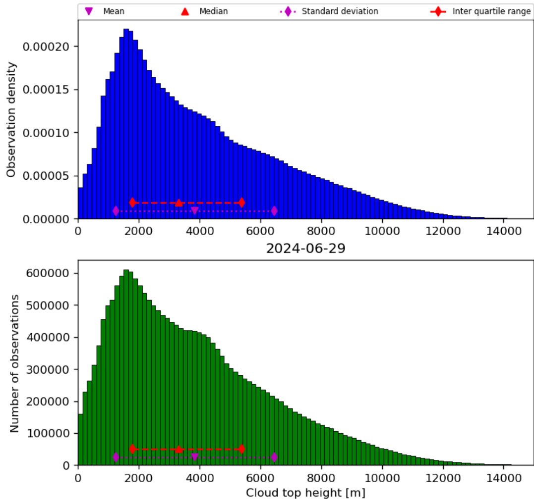
Figure 40: Histogram of “Cloud top height” for 2024-06-29 to 2024-06-30
