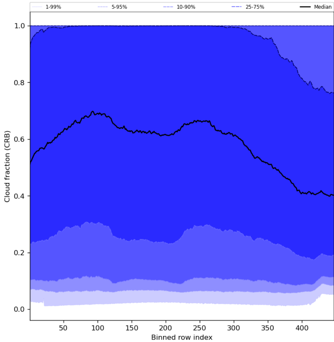
Figure 58: Along track statistics of “Cloud fraction (CRB)” for 2024-06-29 to 2024-06-30
