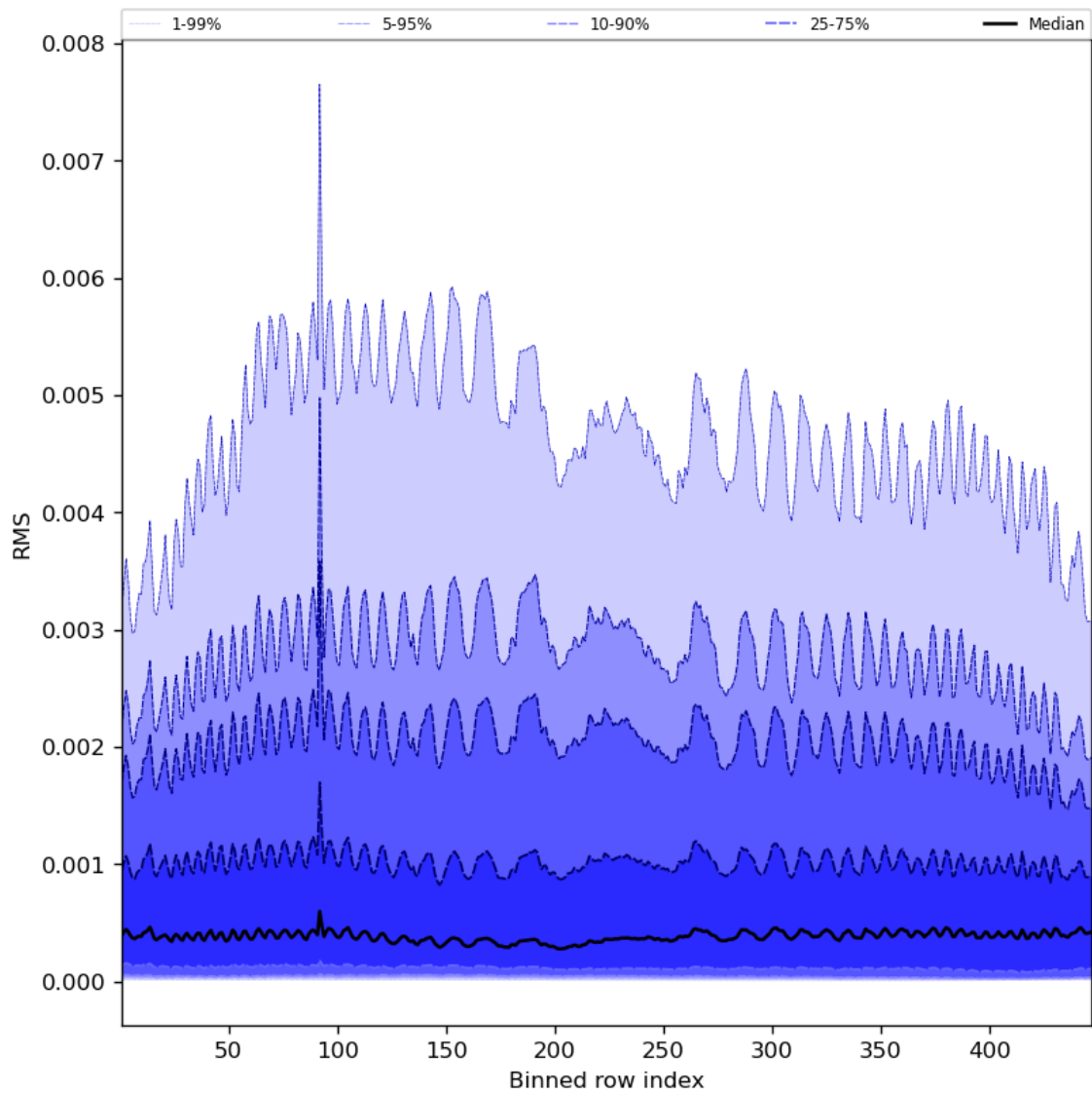
Figure 63: Along track statistics of “RMS” for 2024-06-29 to 2024-06-30
