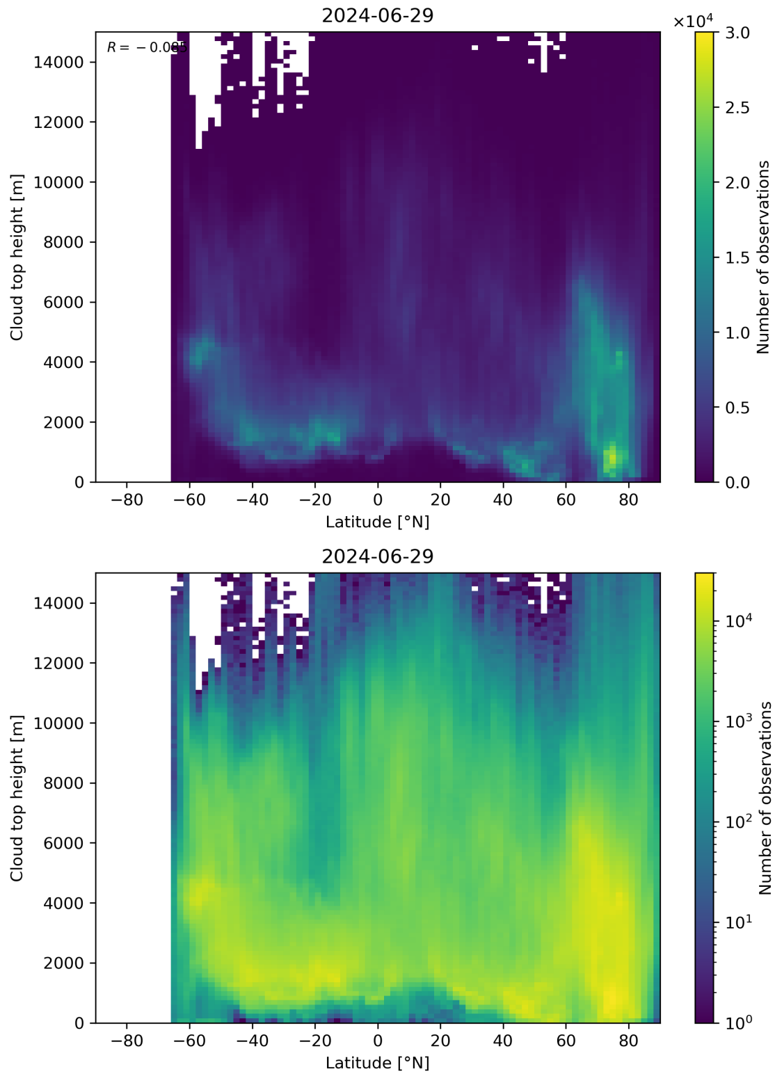
Figure 97: Scatter density plot of “Latitude” against “Cloud top height” for 2024-06-29 to 2024-06-30.
