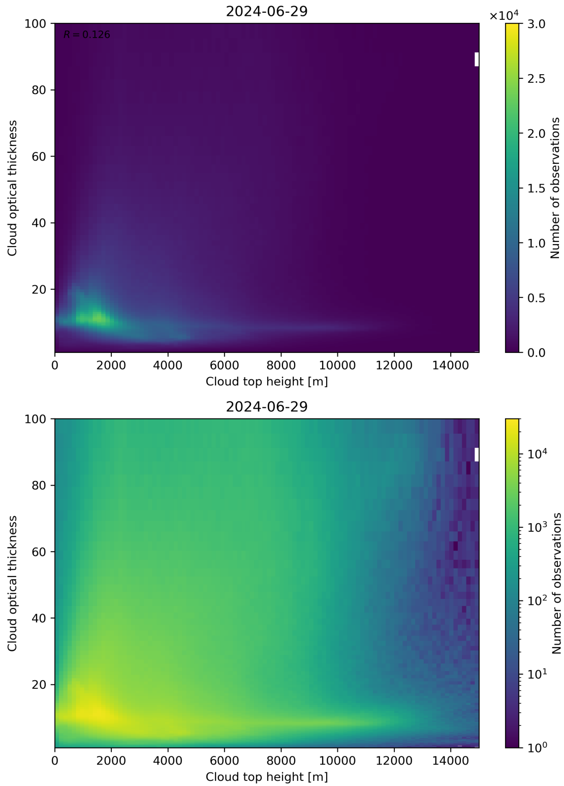
Figure 90: Scatter density plot of “Cloud top height” against “Cloud optical thickness” for 2024-06-29 to 2024-06-30.
