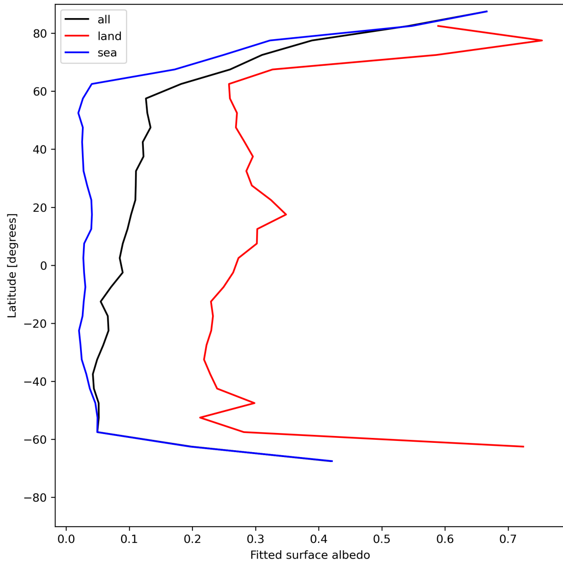
Figure 29: Zonal average of “Fitted surface albedo” for 2024-06-29 to 2024-06-30.
