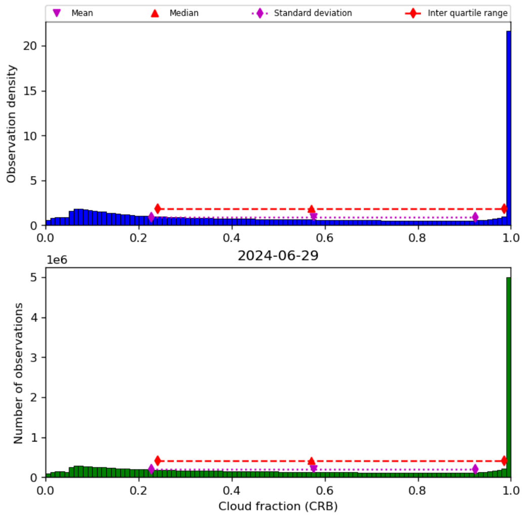
Figure 42: Histogram of “Cloud fraction (CRB)” for 2024-06-29 to 2024-06-30
