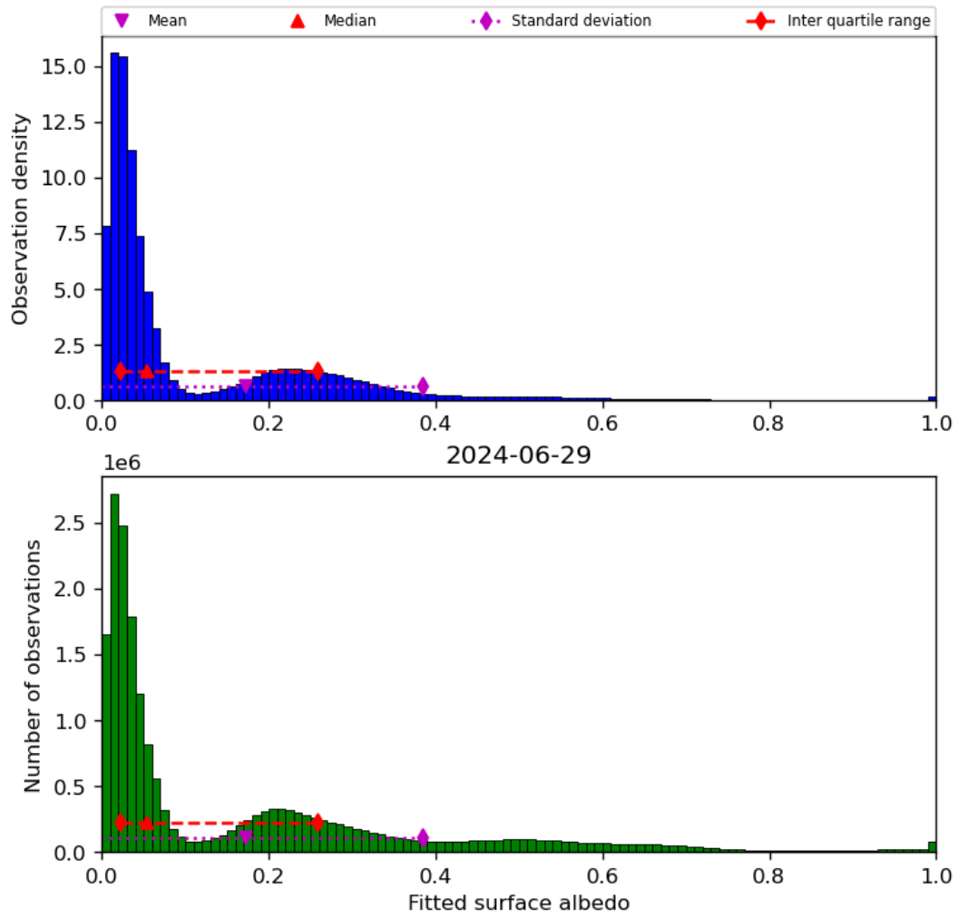
Figure 45: Histogram of “Fitted surface albedo” for 2024-06-29 to 2024-06-30
