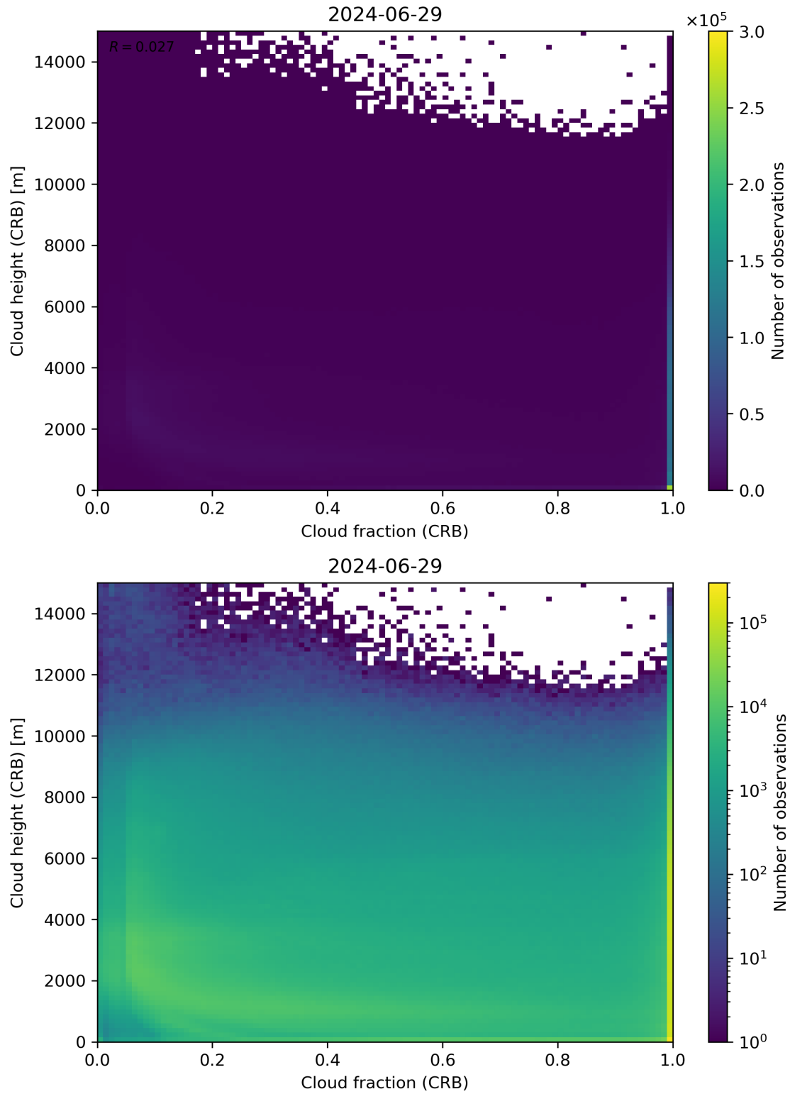
Figure 79: Scatter density plot of “Cloud fraction (CRB)” against “Cloud height (CRB)” for 2024-06-29 to 2024-06-30.
