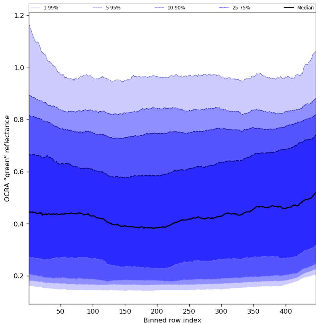
Figure 68: Along track statistics of “OCRA “green” reflectance” for 2024-06-29 to 2024-06-30
