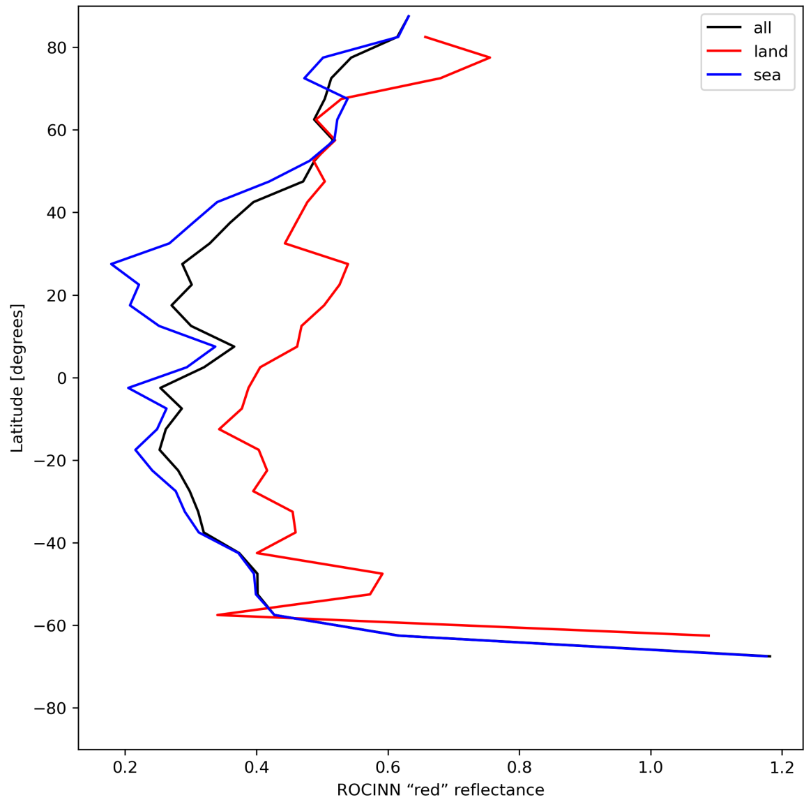
Figure 37: Zonal average of “ROCINN “red” reflectance” for 2024-06-29 to 2024-06-30.
