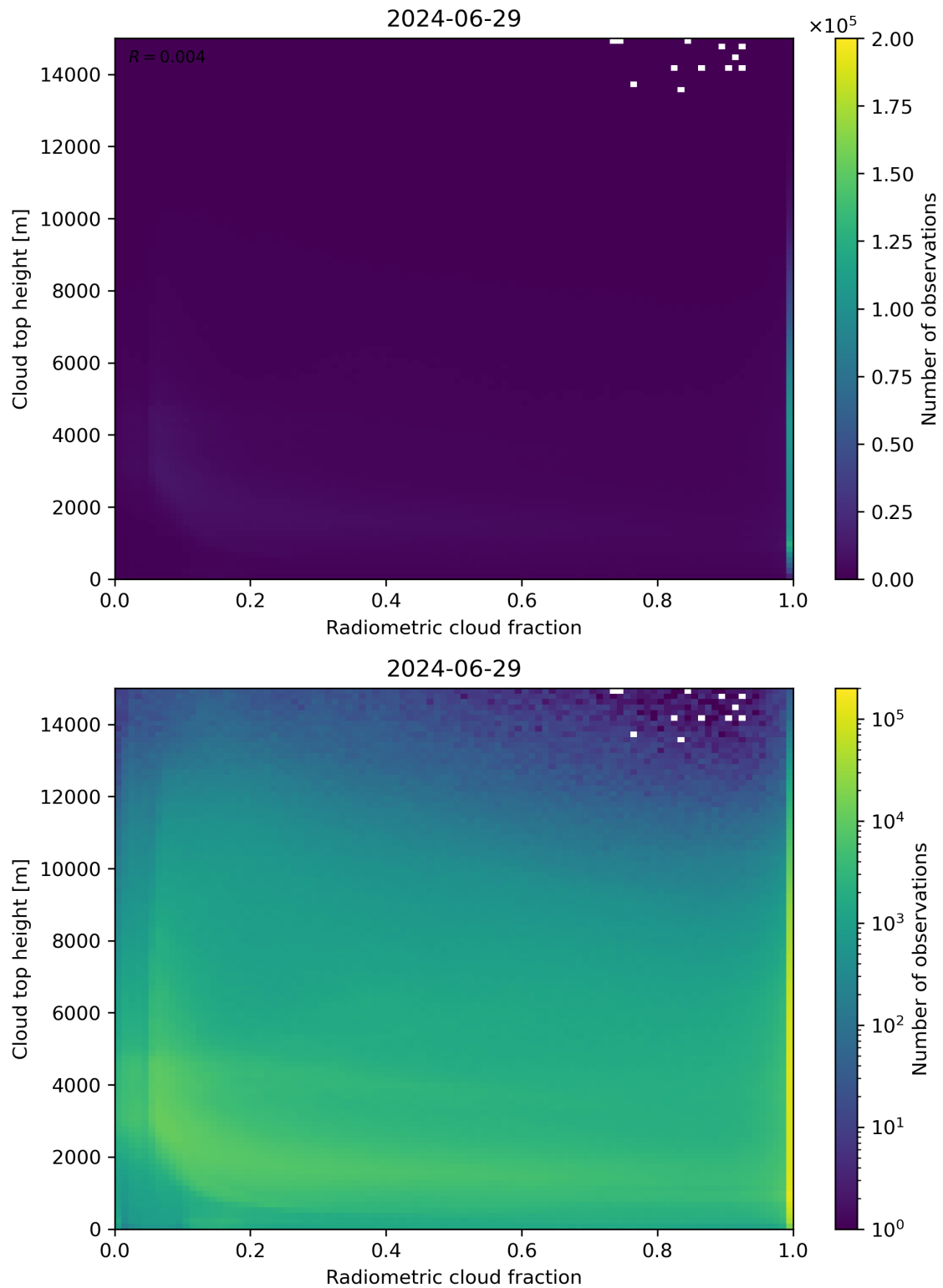
Figure 76: Scatter density plot of “Radiometric cloud fraction” against “Cloud top height” for 2024-06-29 to 2024-06-30.
