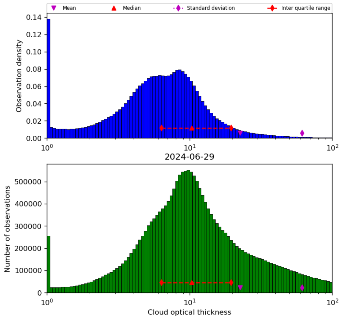
Figure 41: Histogram of “Cloud optical thickness” for 2024-06-29 to 2024-06-30
