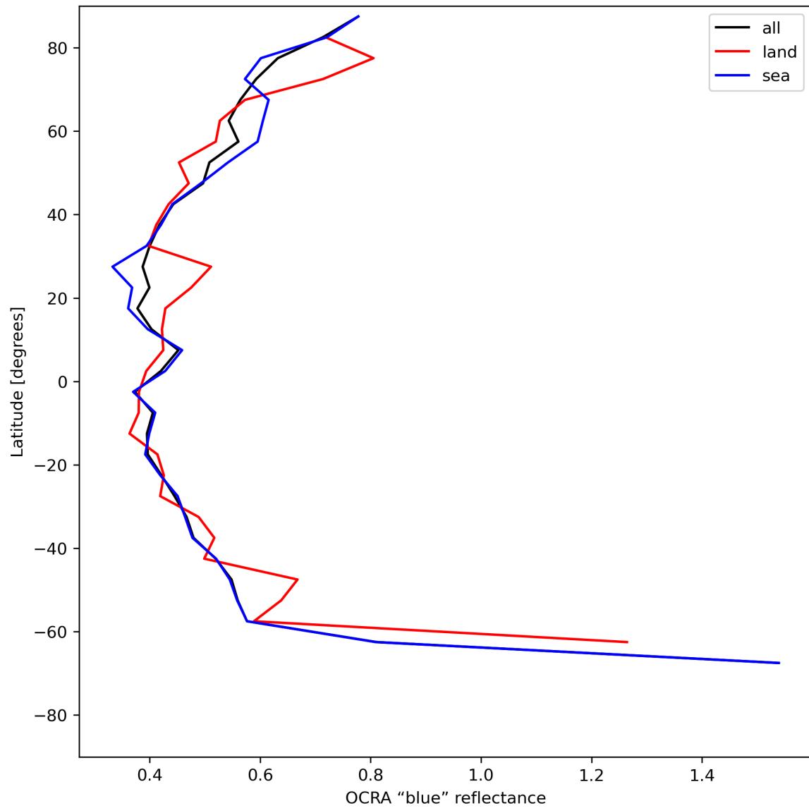
Figure 35: Zonal average of "OCRA "blue" reflectance" for 2024-06-29 to 2024-06-30.
