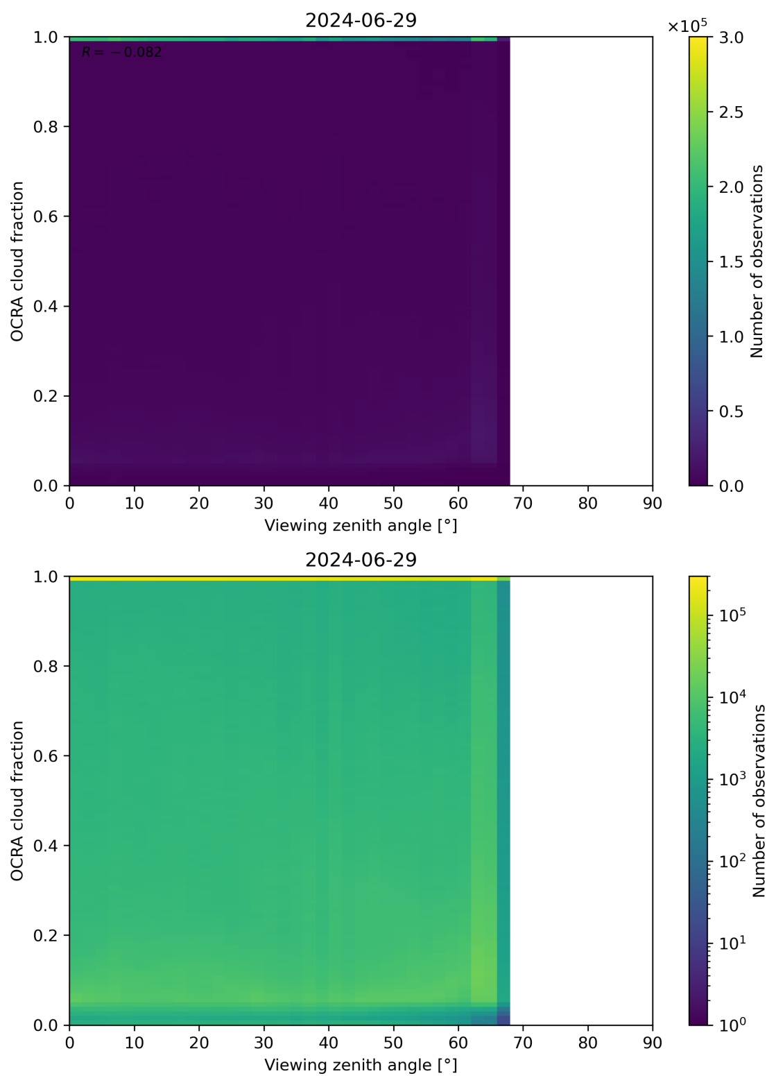
Figure 108: Scatter density plot of “Viewing zenith angle” against “OCRA cloud fraction” for 2024-06-29 to 2024-06-30.
