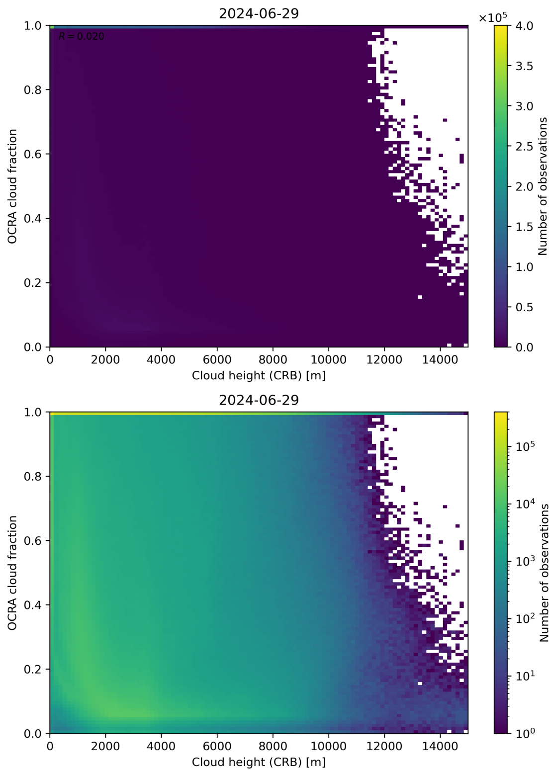
Figure 81: Scatter density plot of “Cloud height (CRB)” against “OCRA cloud fraction” for 2024-06-29 to 2024-06-30.
