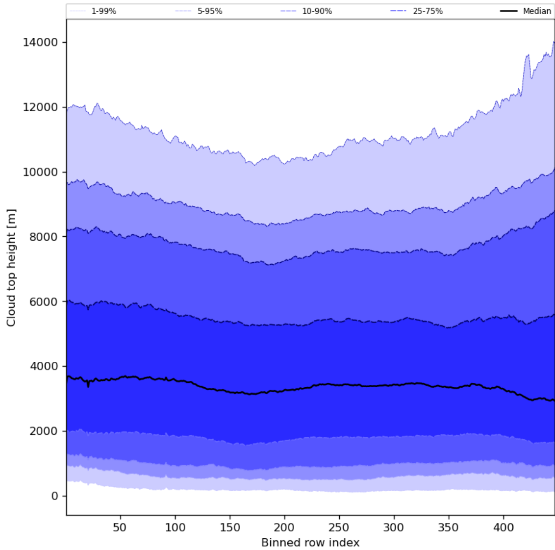
Figure 56: Along track statistics of “Cloud top height” for 2024-06-30 to 2024-07-02
