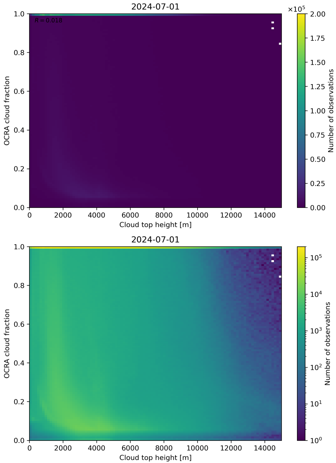
Figure 87: Scatter density plot of “Cloud top height” against “OCRA cloud fraction” for 2024-06-30 to 2024-07-02.
