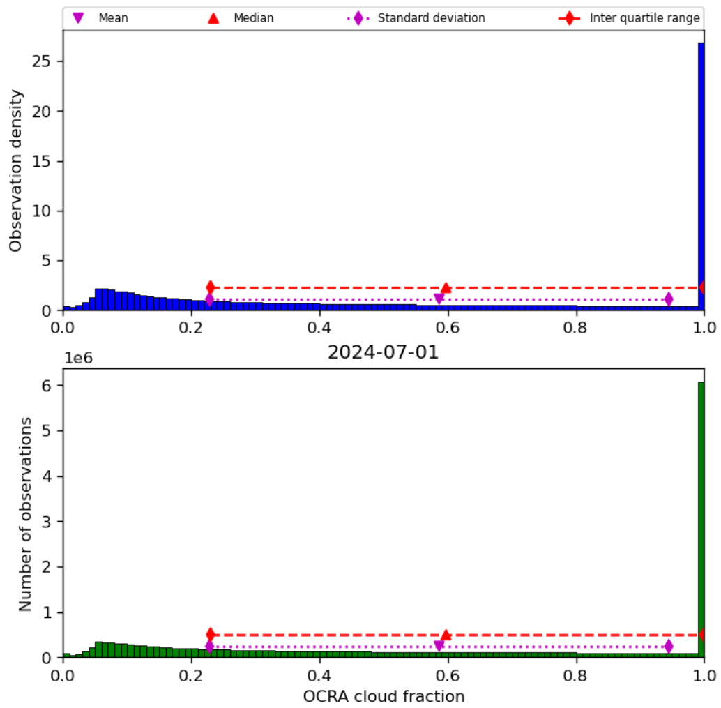
Figure 50: Histogram of “OCRA cloud fraction” for 2024-06-30 to 2024-07-02
