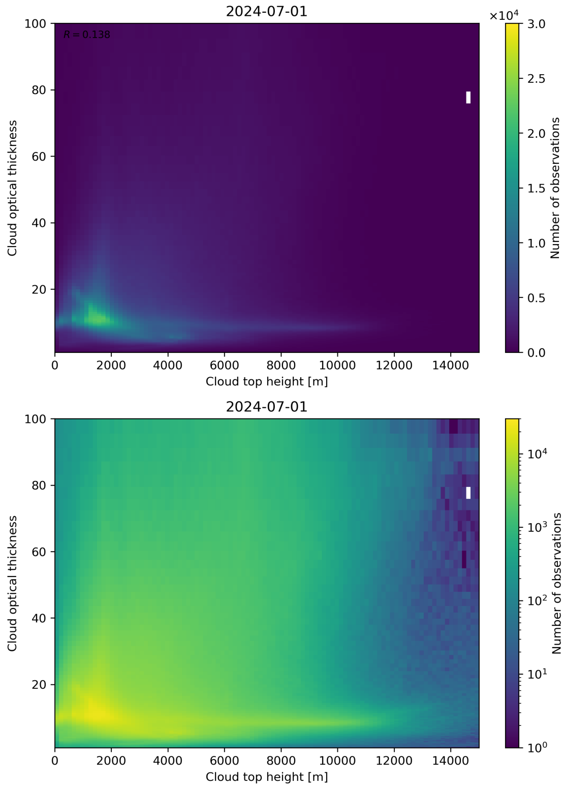
Figure 90: Scatter density plot of “Cloud top height” against “Cloud optical thickness” for 2024-06-30 to 2024-07-02.
