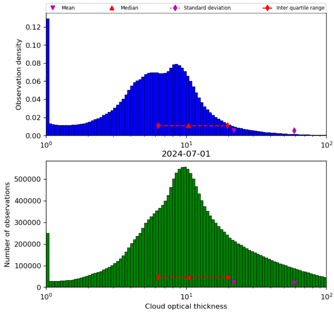
Figure 41: Histogram of “Cloud optical thickness” for 2024-06-30 to 2024-07-02
