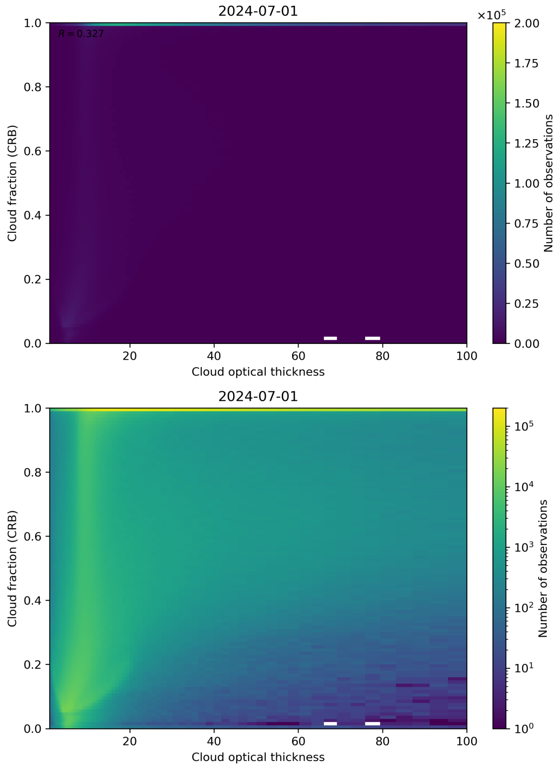
Figure 84: Scatter density plot of “Cloud optical thickness” against “Cloud fraction (CRB)” for 2024-06-30 to 2024-07-02.
