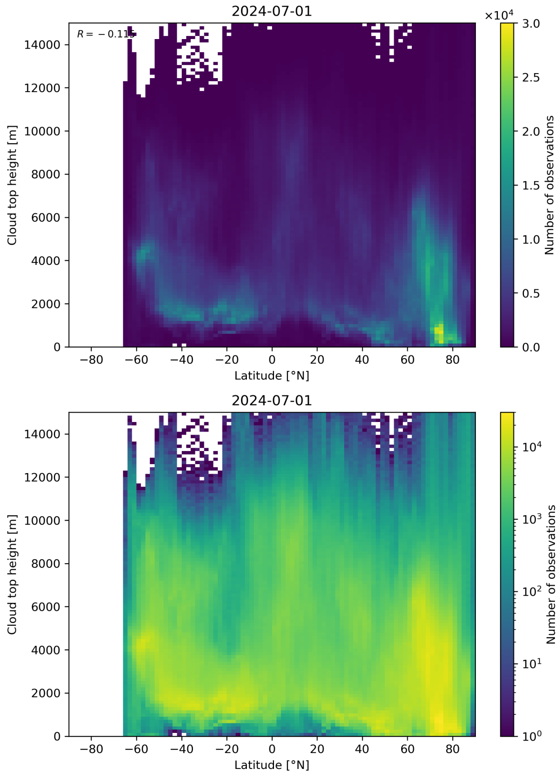
Figure 97: Scatter density plot of “Latitude” against “Cloud top height” for 2024-06-30 to 2024-07-02.
