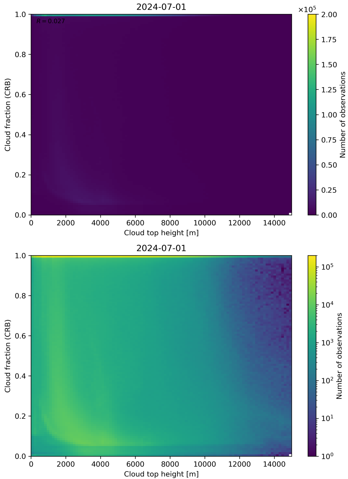
Figure 88: Scatter density plot of “Cloud top height” against “Cloud fraction (CRB)” for 2024-06-30 to 2024-07-02.
