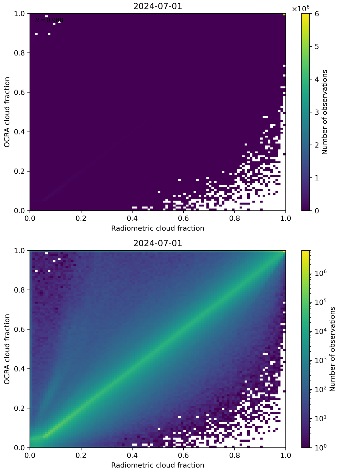
Figure 72: Scatter density plot of “Radiometric cloud fraction” against “OCRA cloud fraction” for 2024-06-30 to 2024-07-02.
