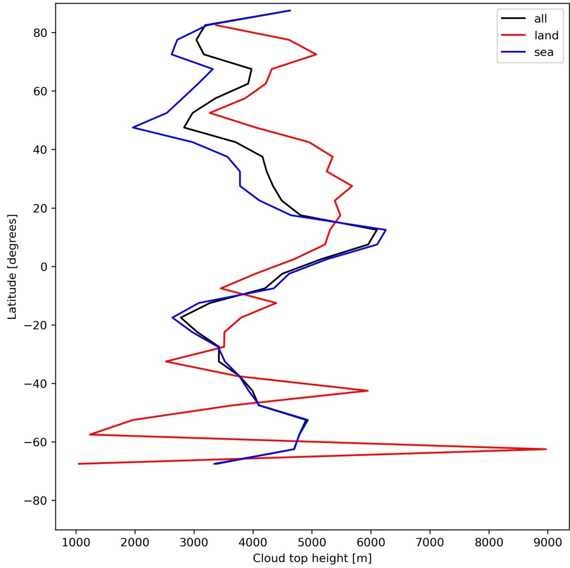
Figure 24: Zonal average of “Cloud top height” for 2024-06-30 to 2024-07-02.
