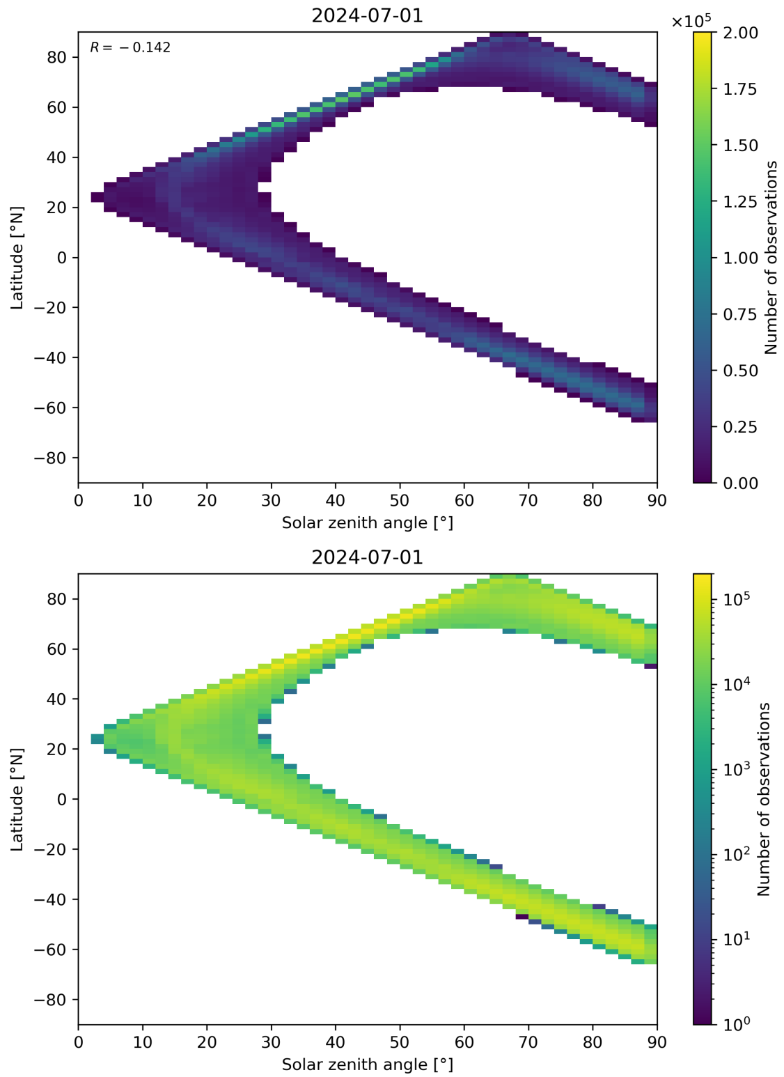
Figure 105: Scatter density plot of “Solar zenith angle” against “Latitude” for 2024-06-30 to 2024-07-02.
