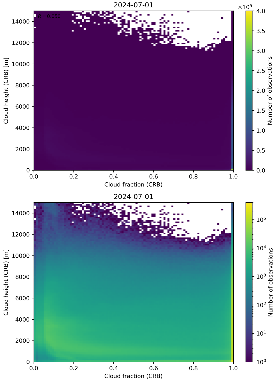
Figure 79: Scatter density plot of “Cloud fraction (CRB)” against “Cloud height (CRB)” for 2024-06-30 to 2024-07-02.
