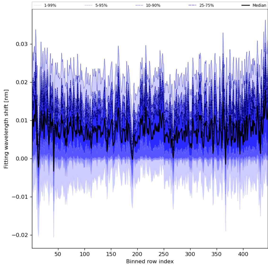
Figure 65: Along track statistics of “Fitting wavelength shift” for 2024-06-30 to 2024-07-02
