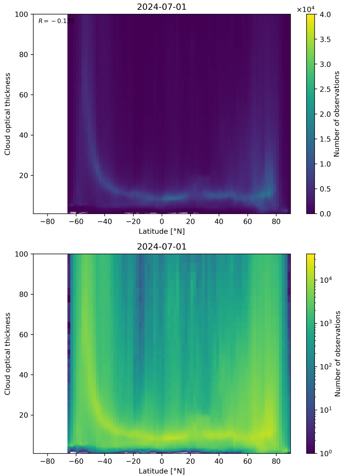
Figure 96: Scatter density plot of “Latitude” against “Cloud optical thickness” for 2024-06-30 to 2024-07-02.
