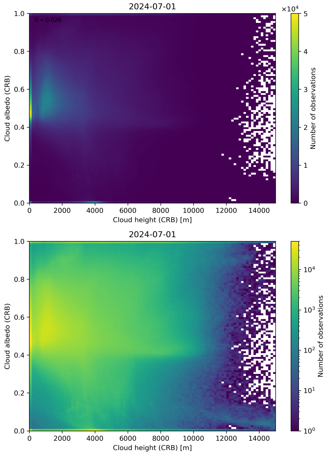
Figure 80: Scatter density plot of “Cloud height (CRB)” against “Cloud albedo (CRB)” for 2024-06-30 to 2024-07-02.
