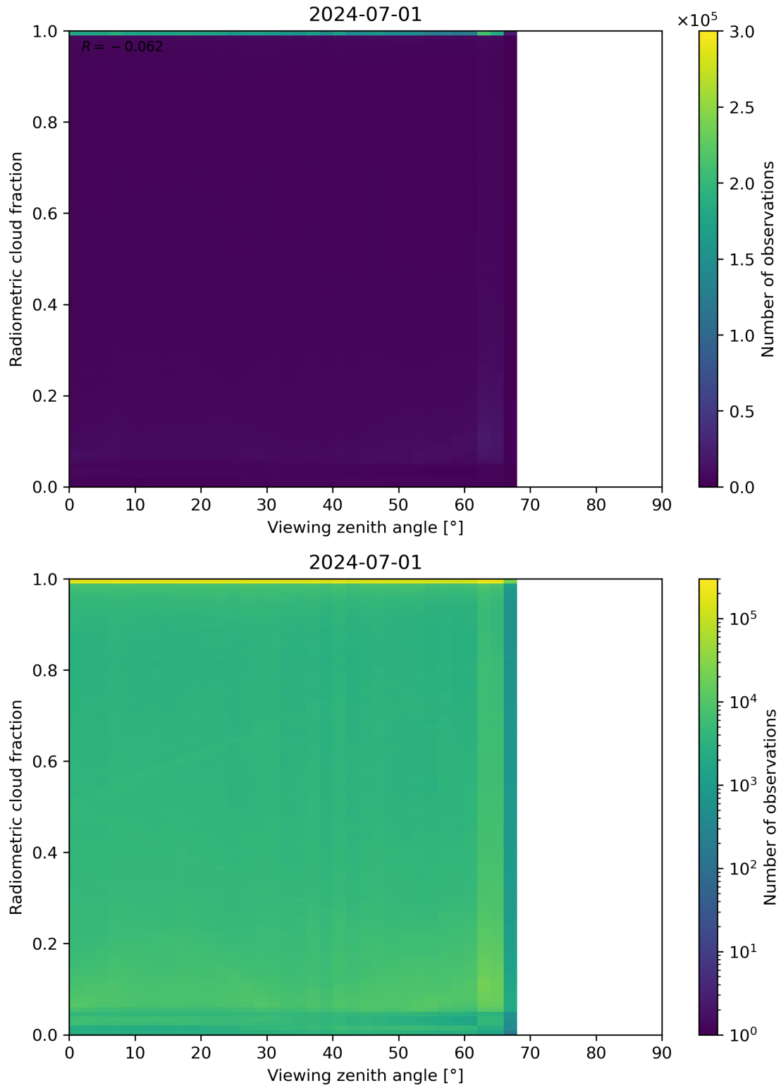
Figure 107: Scatter density plot of “Viewing zenith angle” against “Radiometric cloud fraction” for 2024-06-30 to 2024-07-02.
