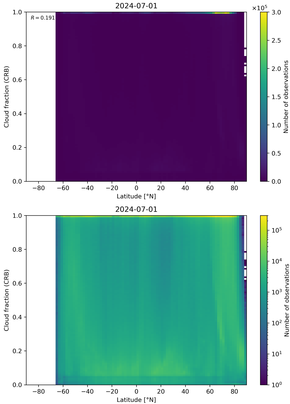
Figure 94: Scatter density plot of “Latitude” against “Cloud fraction (CRB)” for 2024-06-30 to 2024-07-02.
