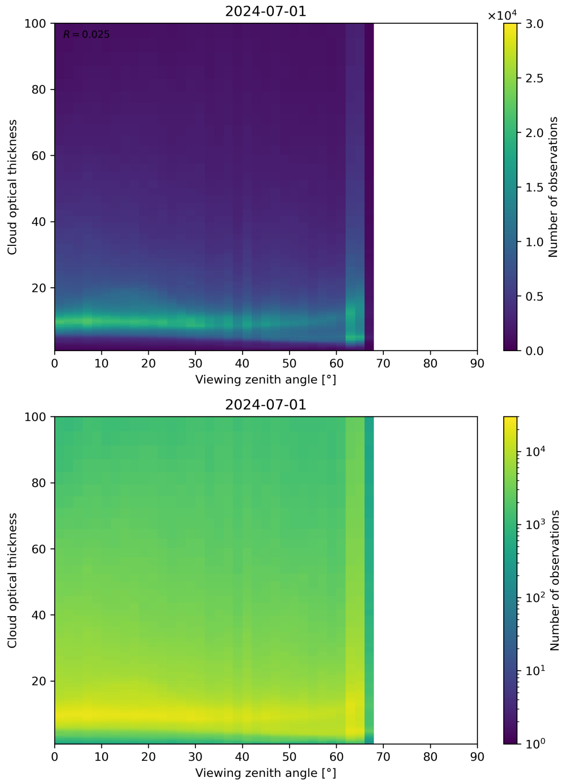
Figure 111: Scatter density plot of “Viewing zenith angle” against “Cloud optical thickness” for 2024-06-30 to 2024-07-02.
