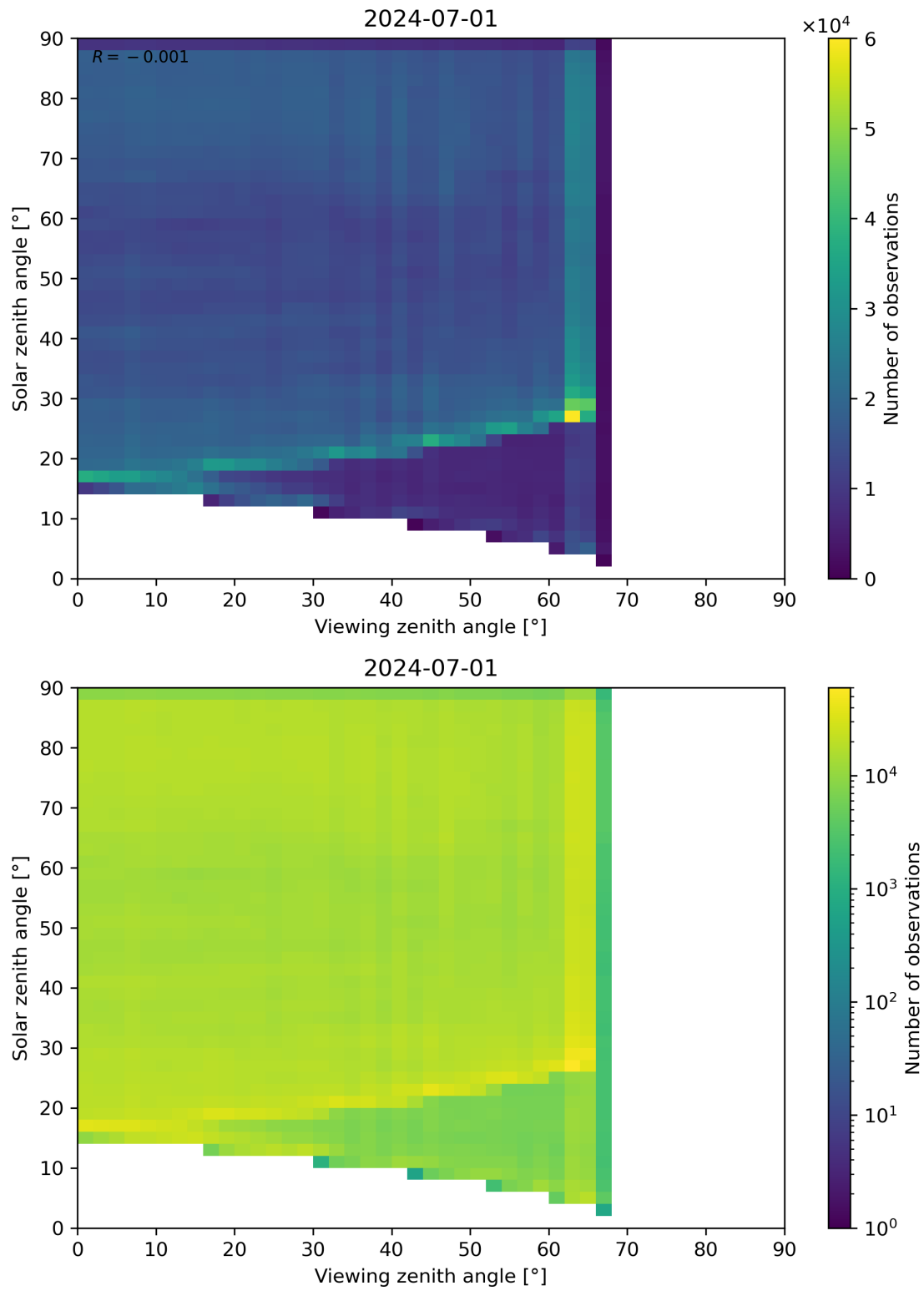
Figure 114: Scatter density plot of “Viewing zenith angle” against “Solar zenith angle” for 2024-06-30 to 2024-07-02.
