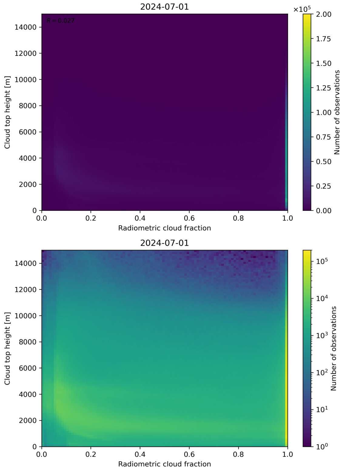
Figure 76: Scatter density plot of “Radiometric cloud fraction” against “Cloud top height” for 2024-06-30 to 2024-07-02.
