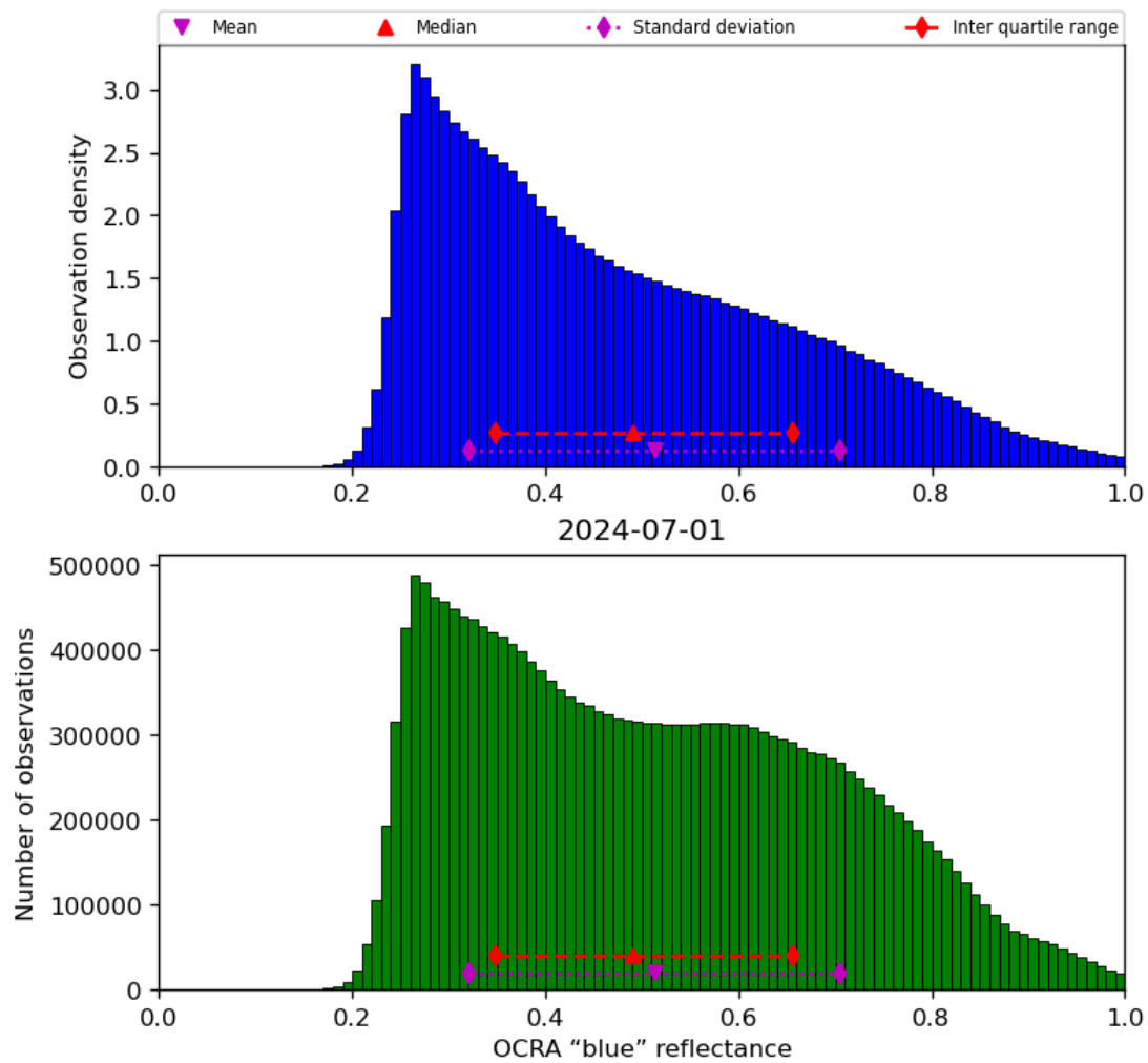
Figure 51: Histogram of “OCRA “blue” reflectance” for 2024-06-30 to 2024-07-02
