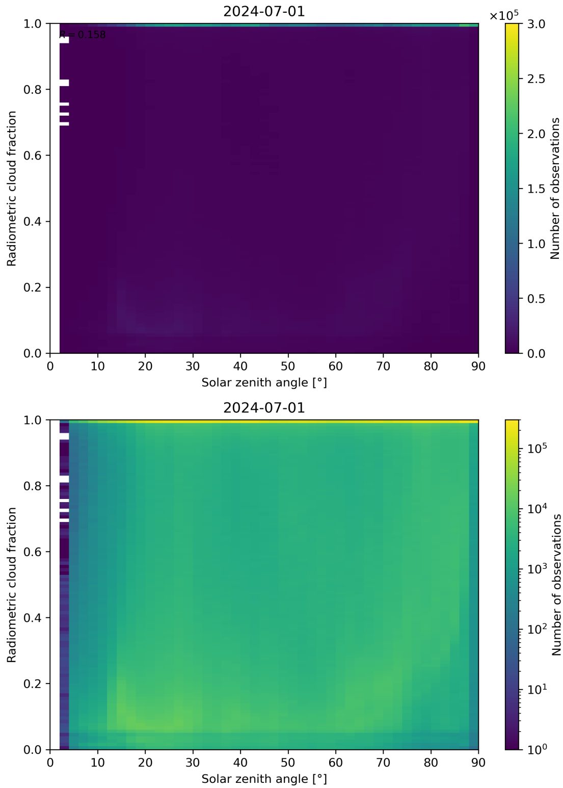
Figure 99: Scatter density plot of “Solar zenith angle” against “Radiometric cloud fraction” for 2024-06-30 to 2024-07-02.
