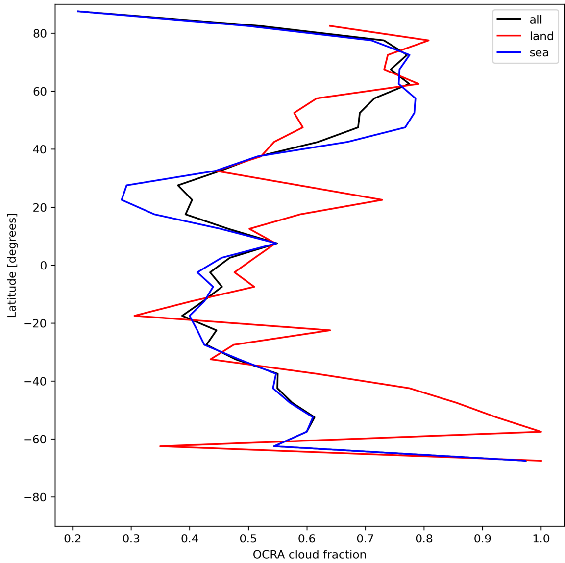
Figure 34: Zonal average of “OCRA cloud fraction” for 2024-06-30 to 2024-07-02.
