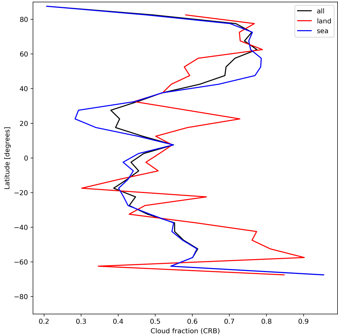
Figure 26: Zonal average of “Cloud fraction (CRB)” for 2024-06-30 to 2024-07-02.
