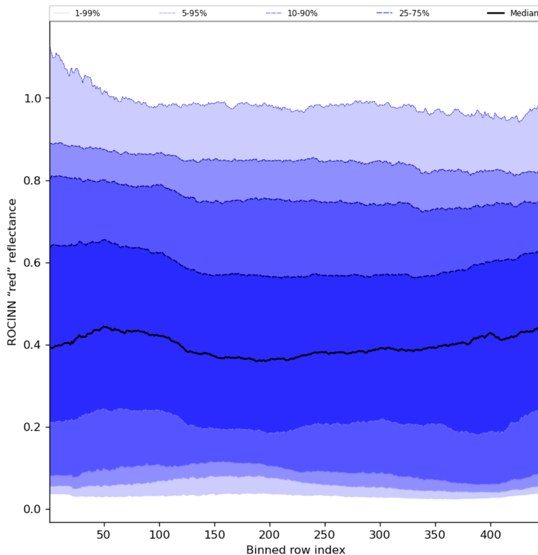
Figure 69: Along track statistics of "ROCINN "red" reflectance" for 2024-06-30 to 2024-07-02
