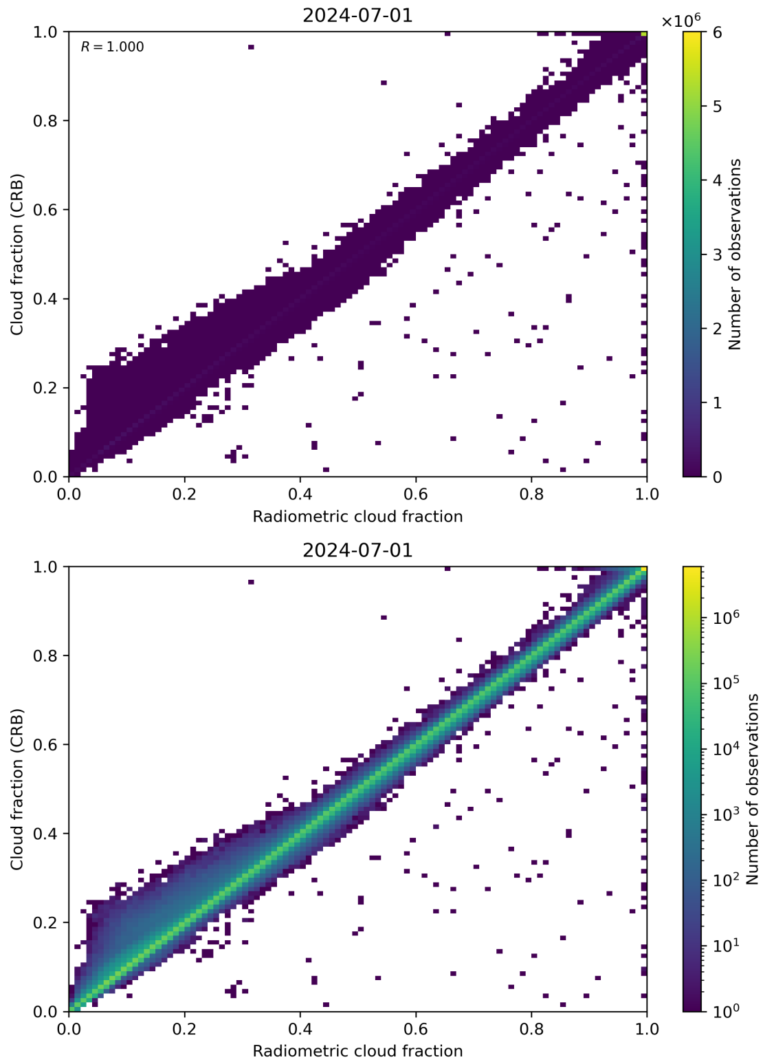
Figure 73: Scatter density plot of “Radiometric cloud fraction” against “Cloud fraction (CRB)” for 2024-06-30 to 2024-07-02.
