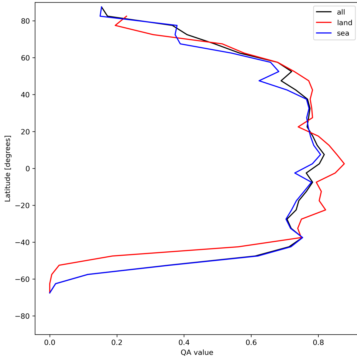
Figure 22: Zonal average of “QA value” for 2024-06-30 to 2024-07-02.
