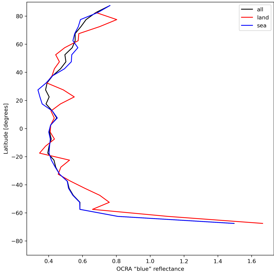
Figure 35: Zonal average of “OCRA “blue” reflectance” for 2024-06-30 to 2024-07-02.
