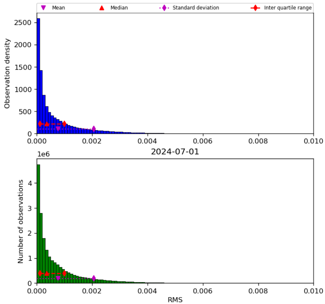
Figure 47: Histogram of “RMS” for 2024-06-30 to 2024-07-02
