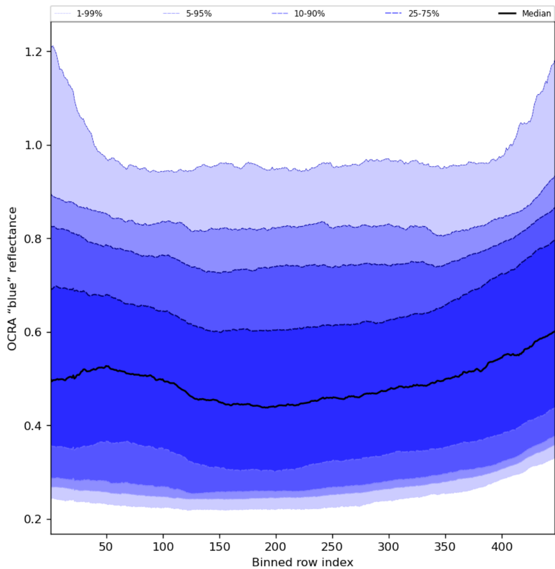
Figure 67: Along track statistics of “OCRA “blue” reflectance” for 2024-06-30 to 2024-07-02
