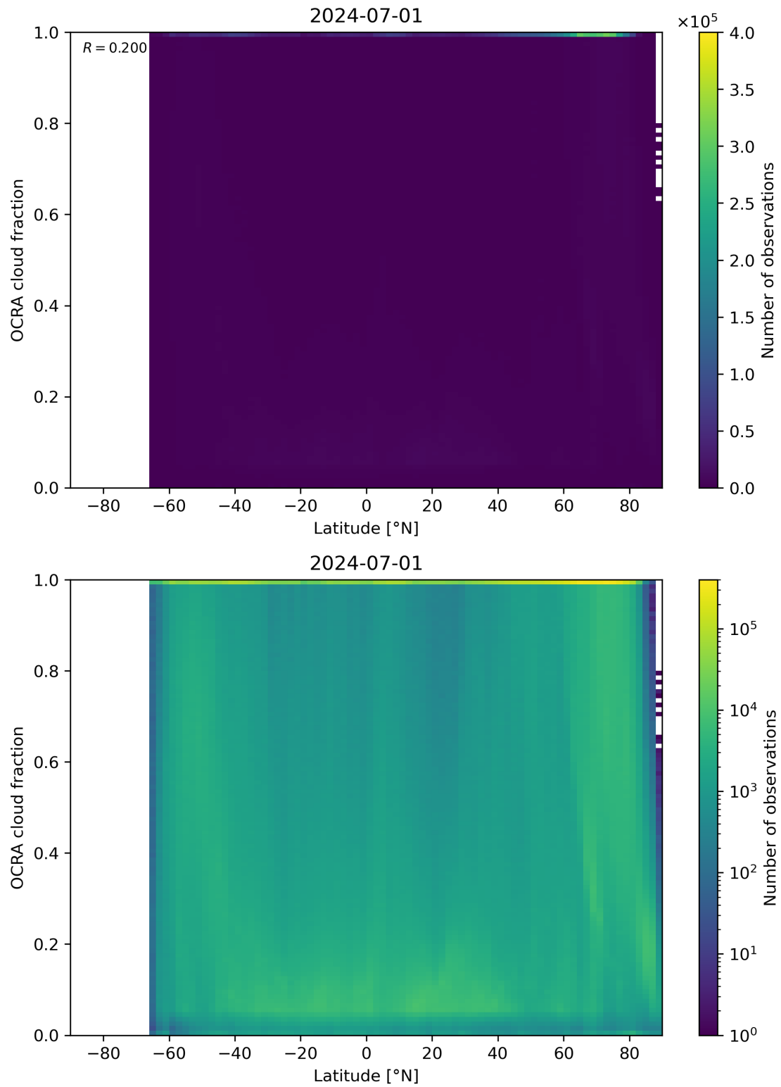
Figure 93: Scatter density plot of “Latitude” against “OCRA cloud fraction” for 2024-06-30 to 2024-07-02.
