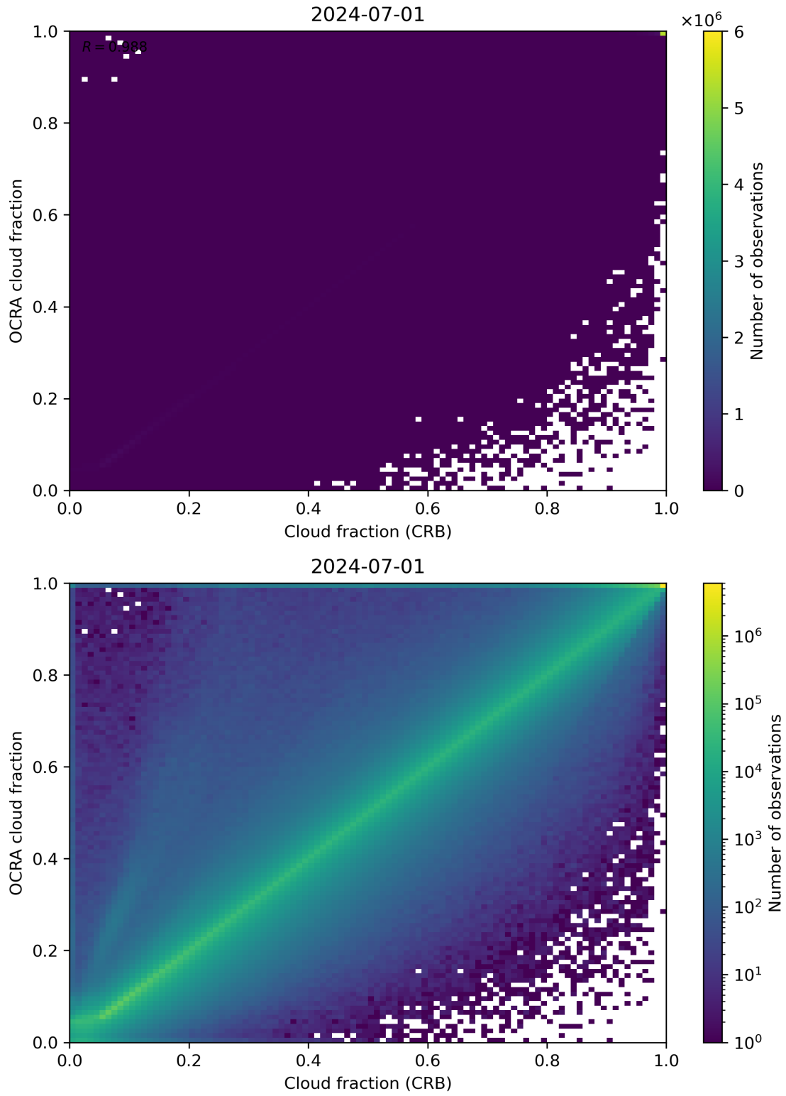
Figure 78: Scatter density plot of “Cloud fraction (CRB)” against “OCRA cloud fraction” for 2024-06-30 to 2024-07-02.
