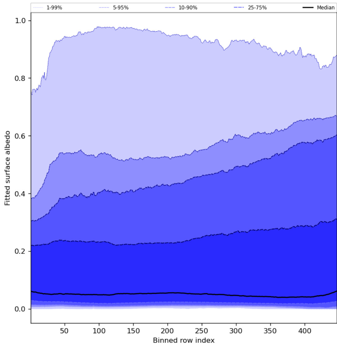
Figure 61: Along track statistics of “Fitted surface albedo” for 2024-06-30 to 2024-07-02
