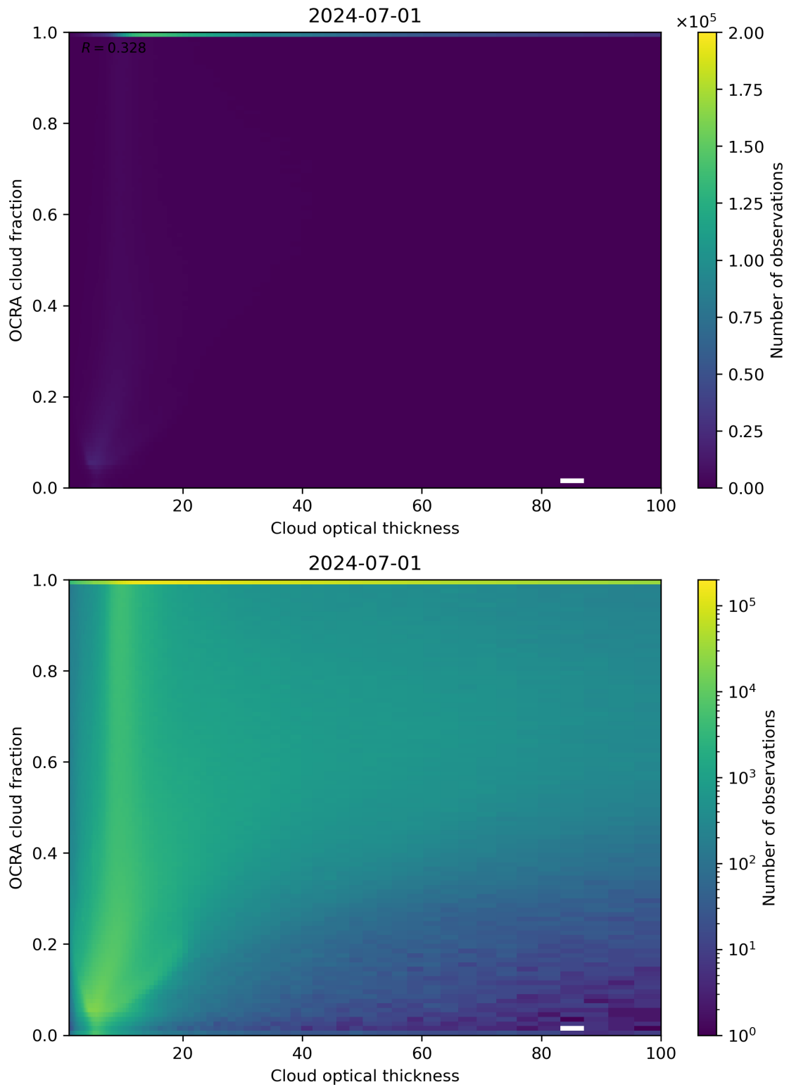
Figure 83: Scatter density plot of “Cloud optical thickness” against “OCRA cloud fraction” for 2024-06-30 to 2024-07-02.
