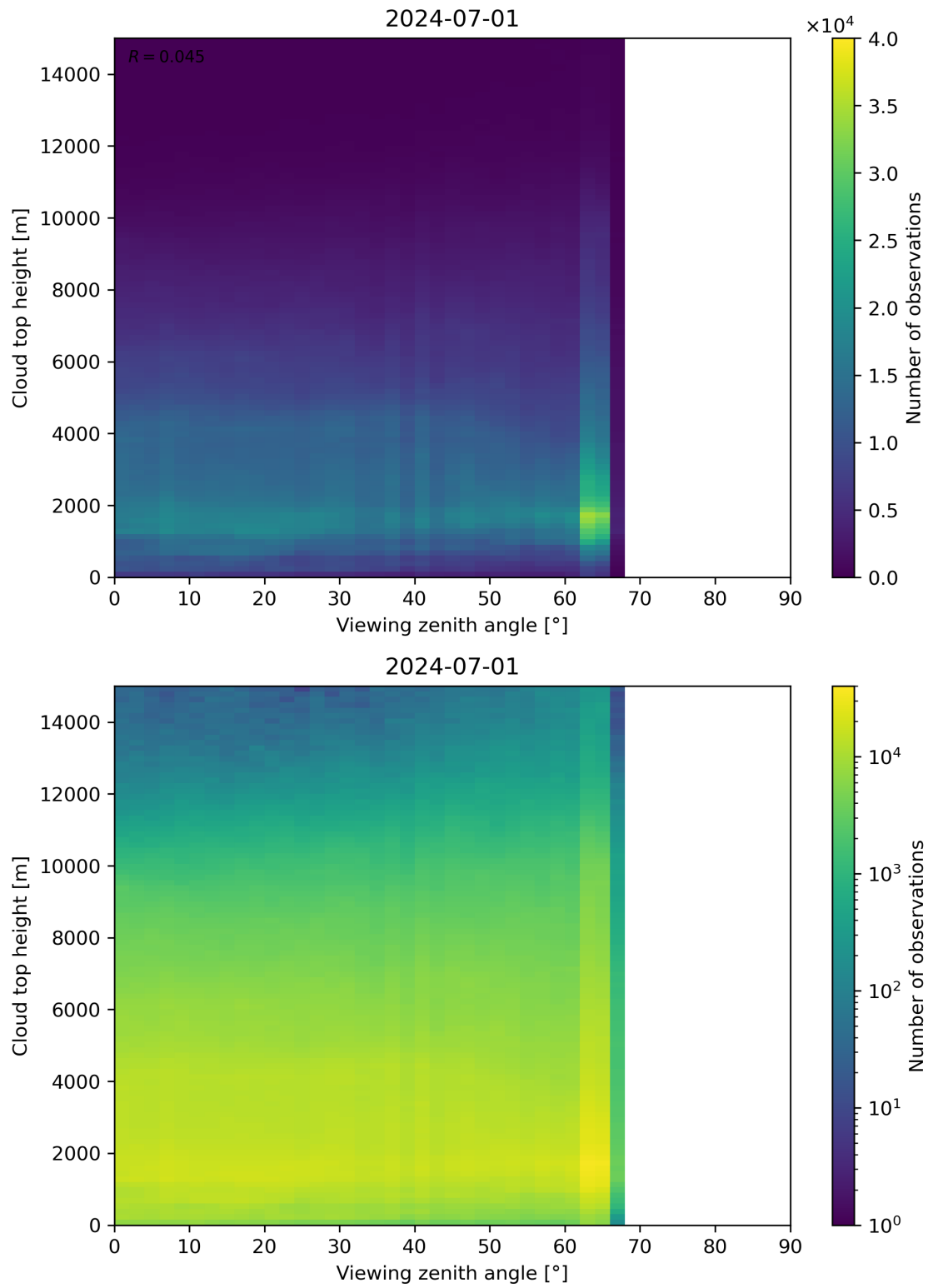
Figure 112: Scatter density plot of “Viewing zenith angle” against “Cloud top height” for 2024-06-30 to 2024-07-02.
