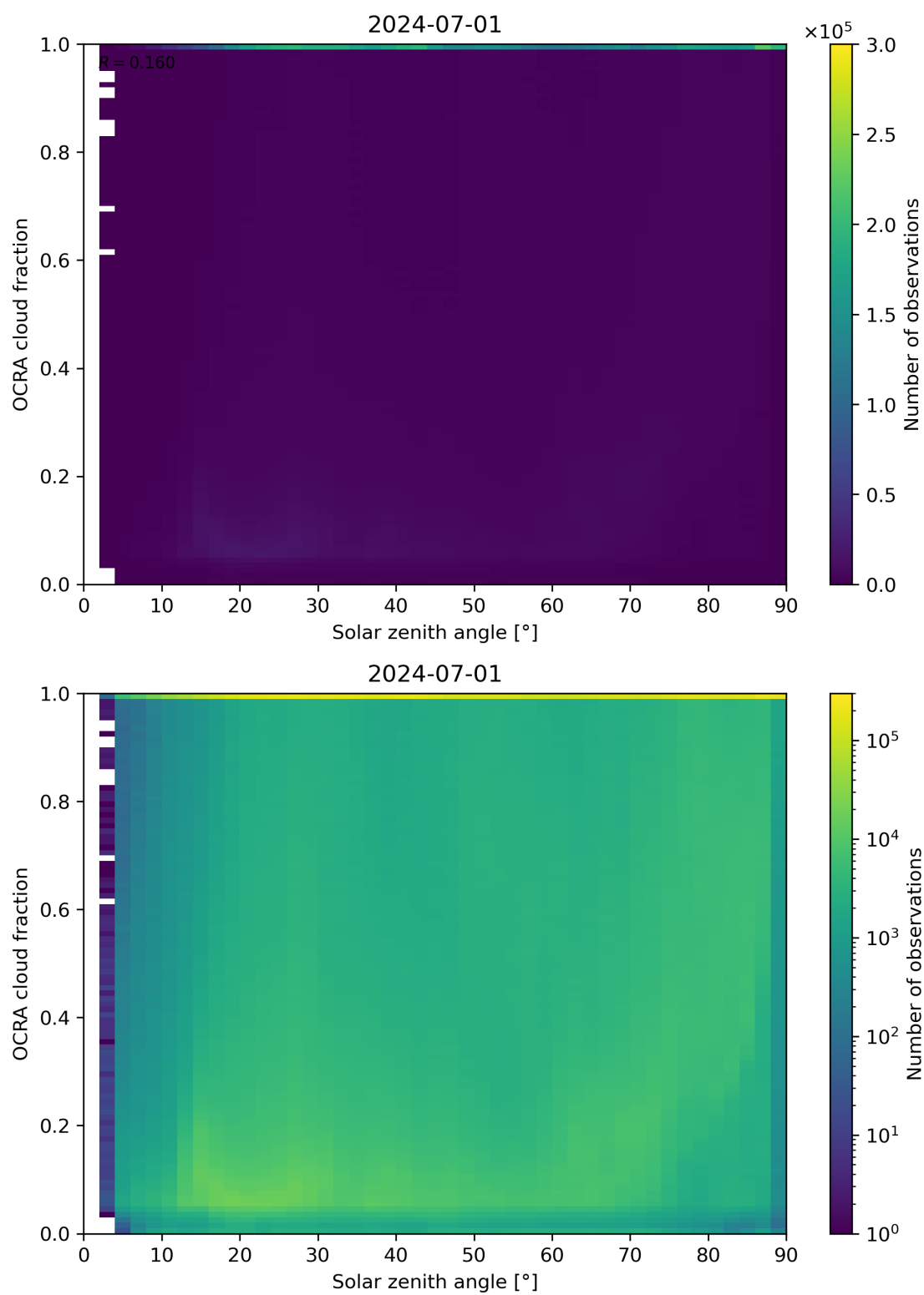
Figure 100: Scatter density plot of “Solar zenith angle” against “OCRA cloud fraction” for 2024-06-30 to 2024-07-02.
