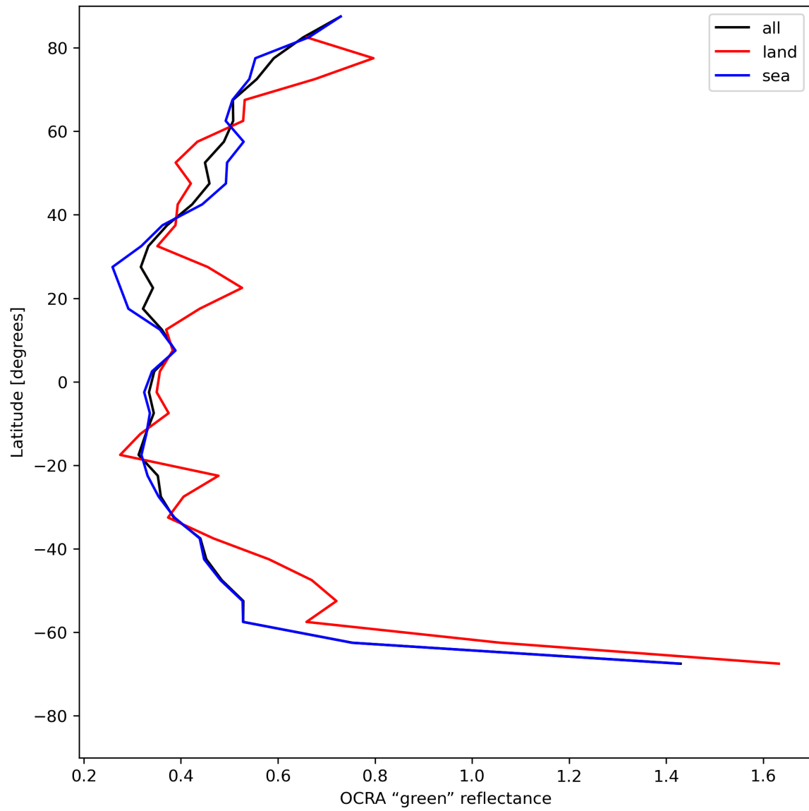
Figure 36: Zonal average of “OCRA “green” reflectance” for 2024-06-30 to 2024-07-02.
