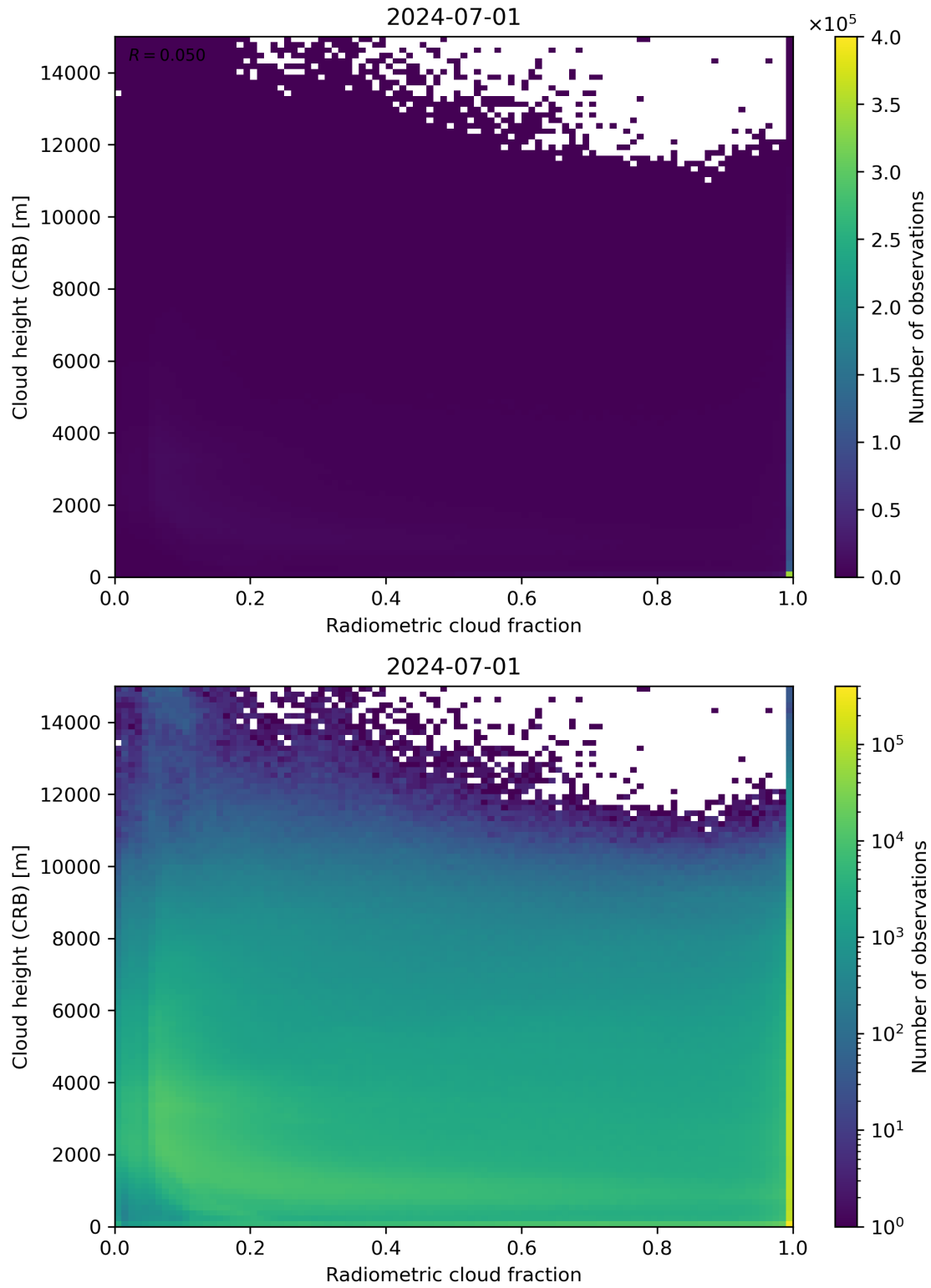
Figure 74: Scatter density plot of “Radiometric cloud fraction” against “Cloud height (CRB)” for 2024-06-30 to 2024-07-02.
