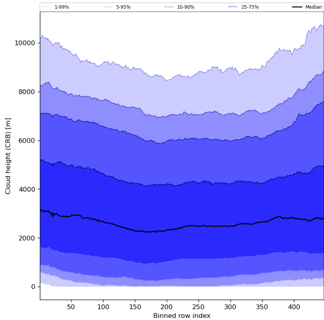
Figure 59: Along track statistics of “Cloud height (CRB)” for 2024-06-30 to 2024-07-02
