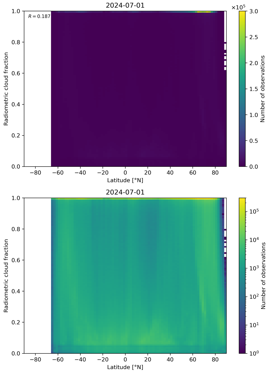
Figure 92: Scatter density plot of “Latitude” against “Radiometric cloud fraction” for 2024-06-30 to 2024-07-02.
