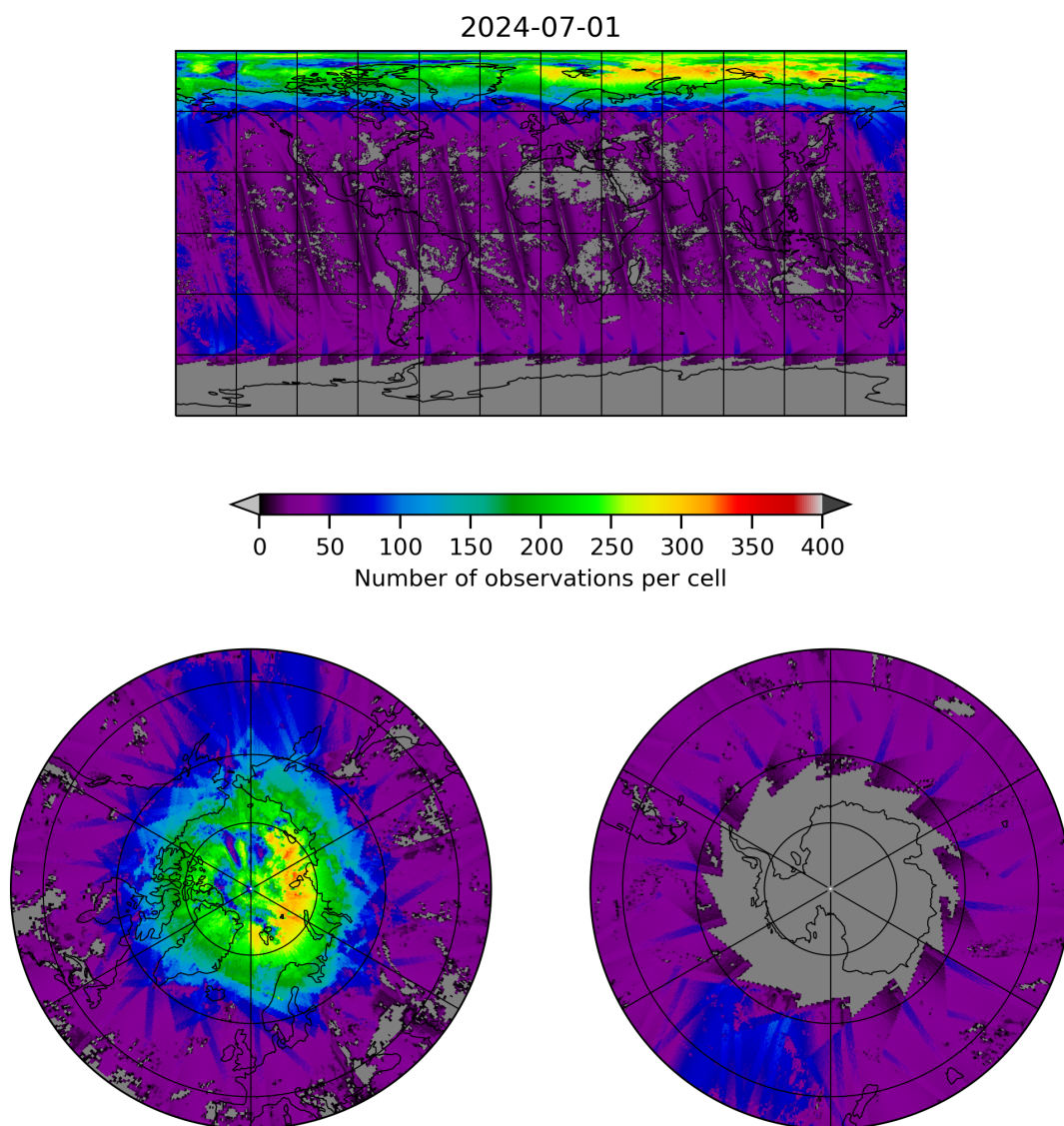
Figure 21: Map of the number of observations for 2024-06-30 to 2024-07-02
