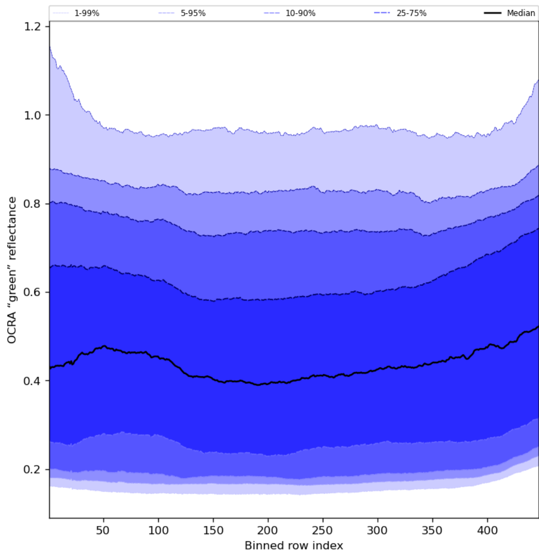
Figure 68: Along track statistics of “OCRA “green” reflectance” for 2024-06-30 to 2024-07-02
