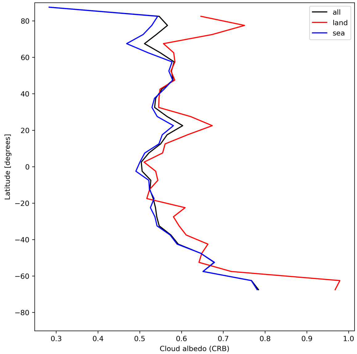
Figure 28: Zonal average of “Cloud albedo (CRB)” for 2024-06-30 to 2024-07-02.
