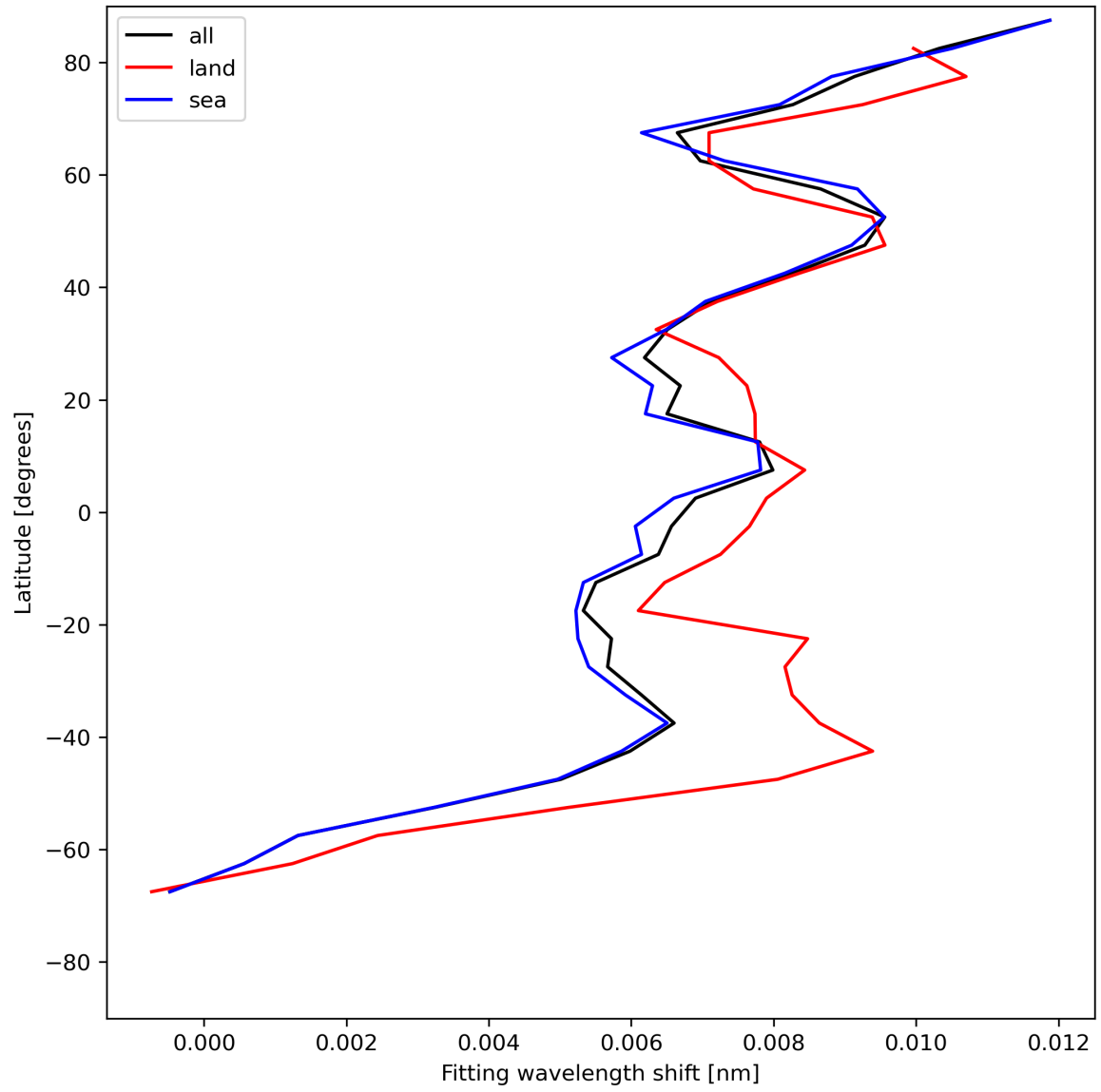
Figure 33: Zonal average of “Fitting wavelength shift” for 2024-06-30 to 2024-07-02.
