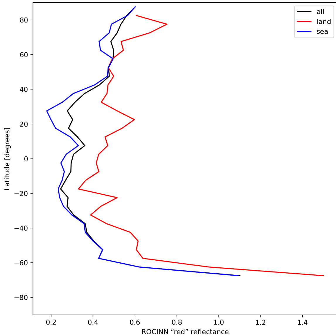
Figure 37: Zonal average of “ROCINN “red” reflectance” for 2024-06-30 to 2024-07-02.
