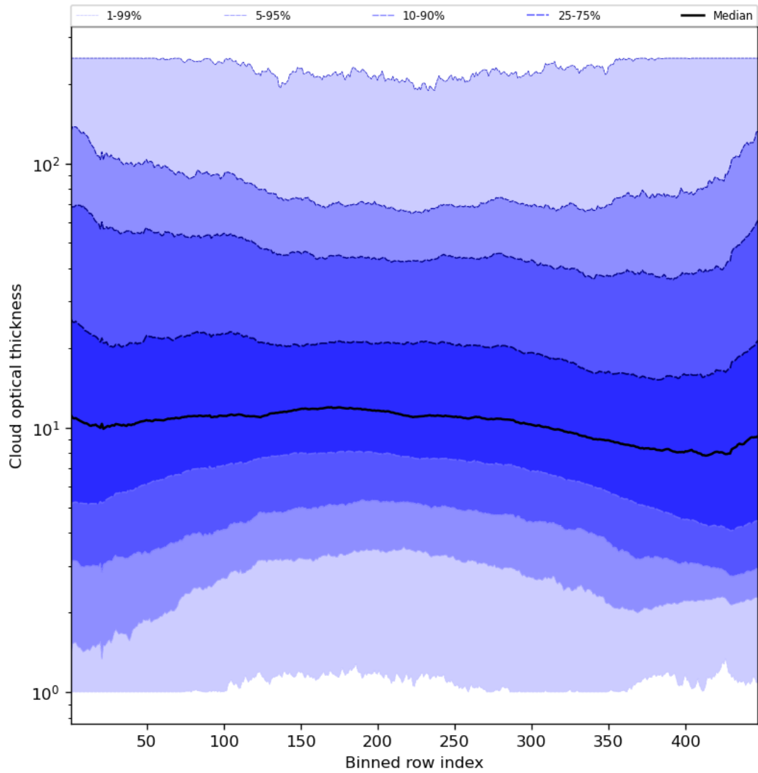
Figure 57: Along track statistics of “Cloud optical thickness” for 2024-06-30 to 2024-07-02
