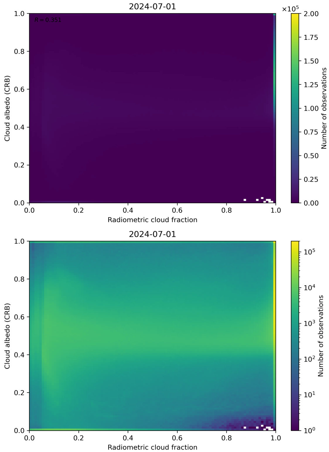
Figure 71: Scatter density plot of “Radiometric cloud fraction” against “Cloud albedo (CRB)” for 2024-06-30 to 2024-07-02.
