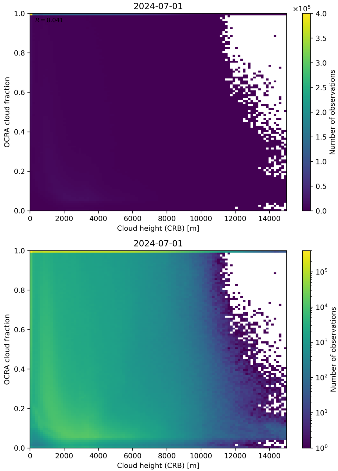
Figure 81: Scatter density plot of “Cloud height (CRB)” against “OCRA cloud fraction” for 2024-06-30 to 2024-07-02.
