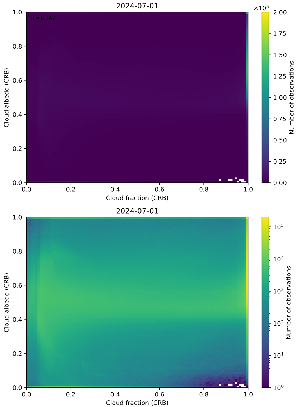
Figure 77: Scatter density plot of “Cloud fraction (CRB)” against “Cloud albedo (CRB)” for 2024-06-30 to 2024-07-02.
