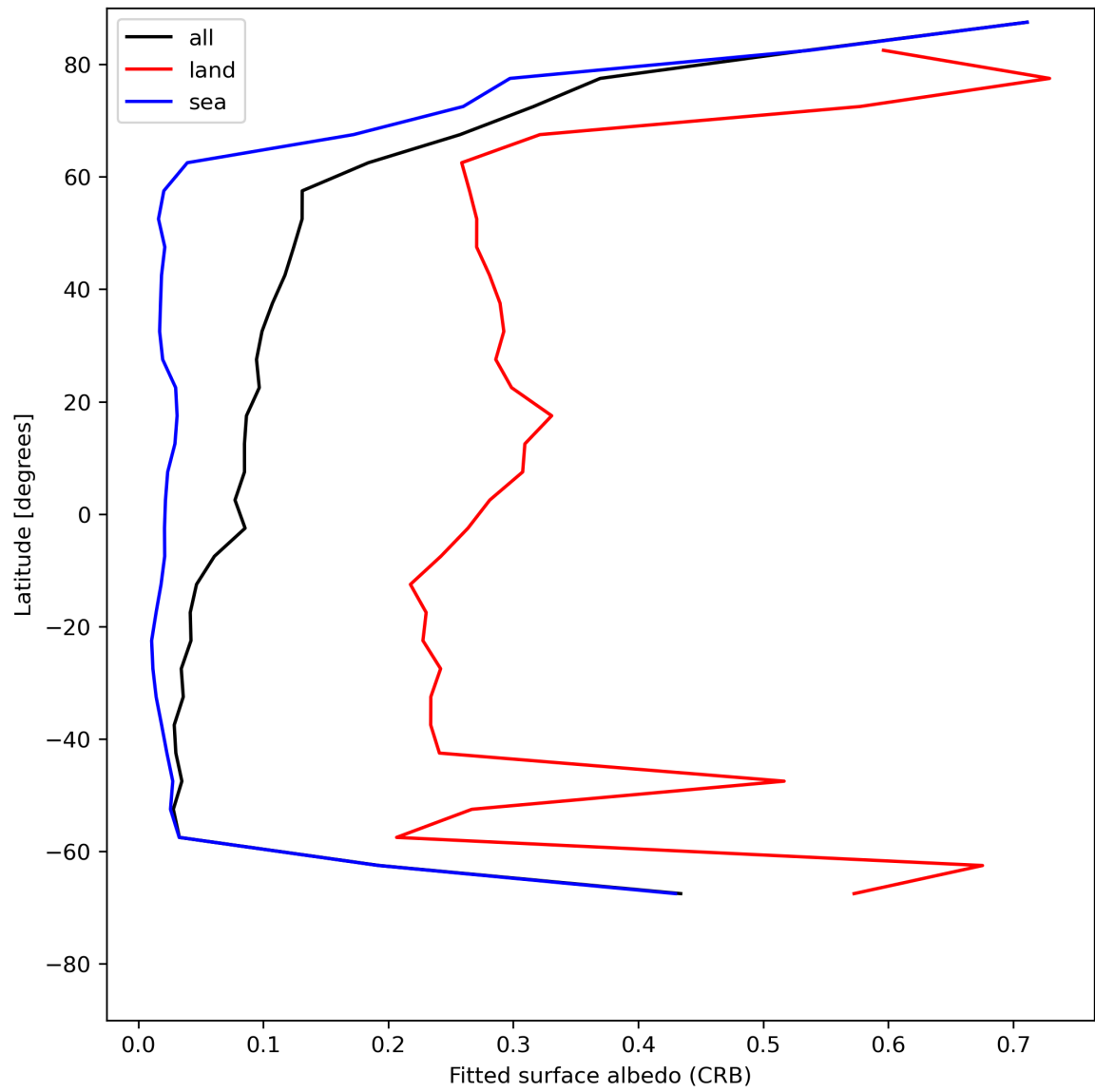
Figure 30: Zonal average of “Fitted surface albedo (CRB)” for 2024-06-30 to 2024-07-02.
