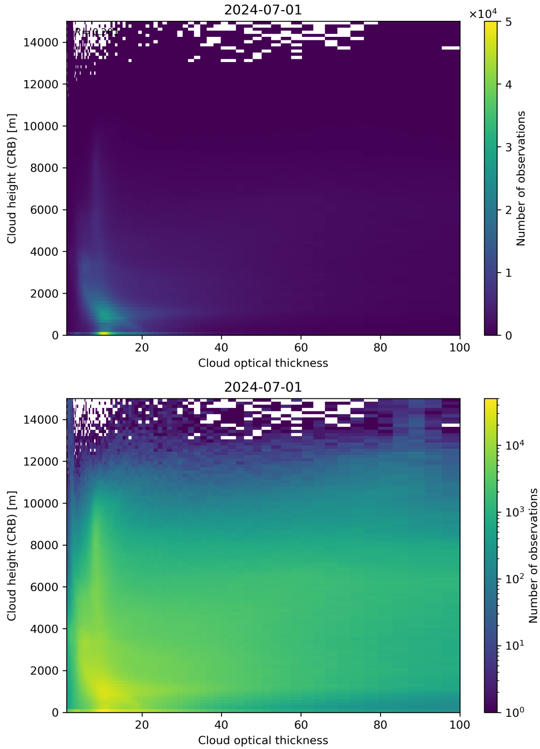
Figure 85: Scatter density plot of “Cloud optical thickness” against “Cloud height (CRB)” for 2024-06-30 to 2024-07-02.
