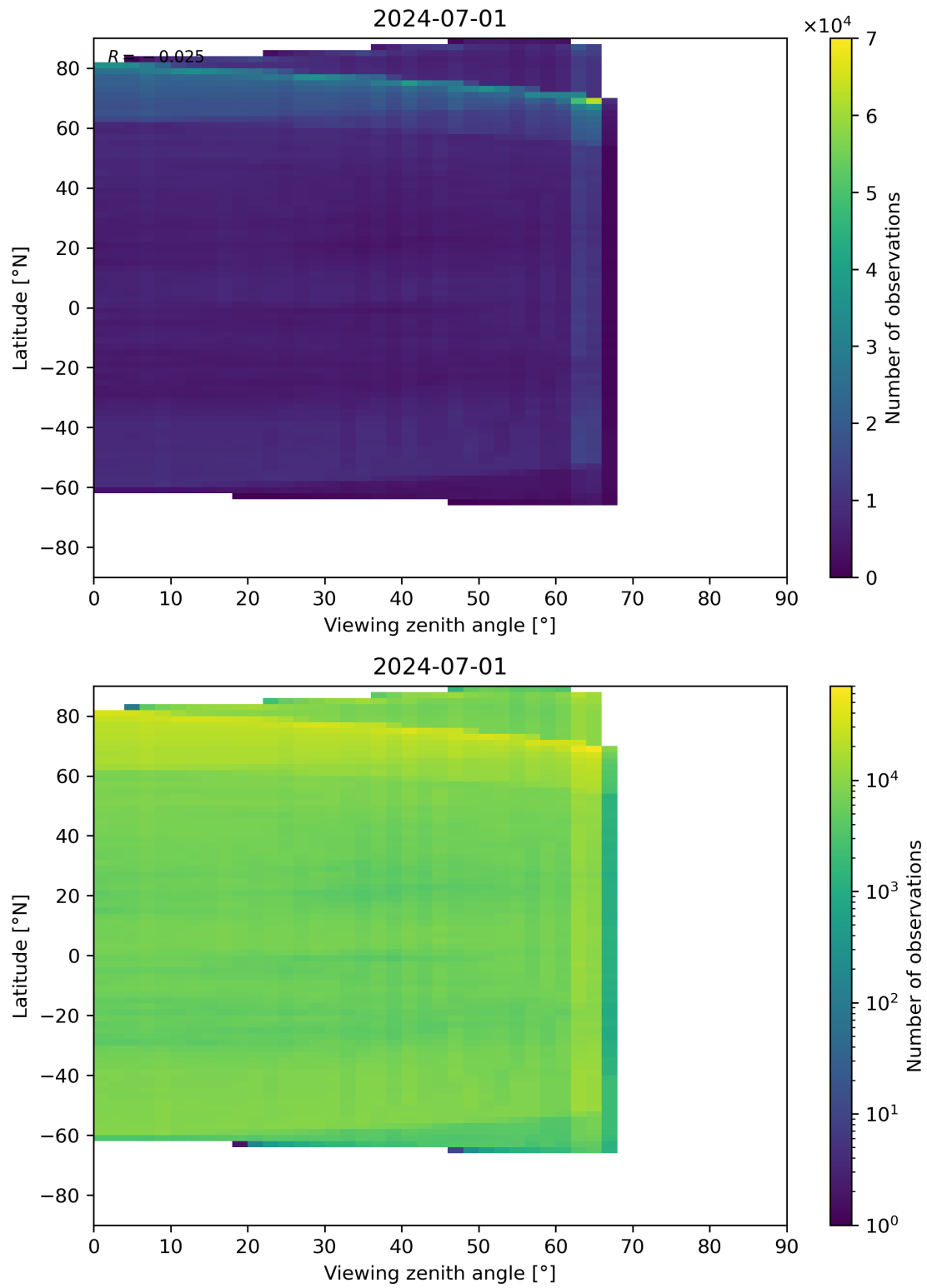
Figure 113: Scatter density plot of “Viewing zenith angle” against “Latitude” for 2024-06-30 to 2024-07-02.
