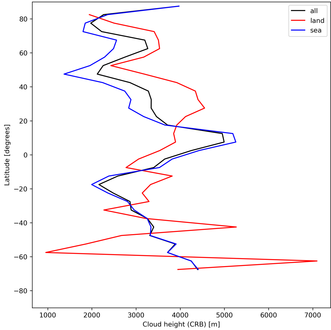
Figure 27: Zonal average of “Cloud height (CRB)” for 2024-06-30 to 2024-07-02.
