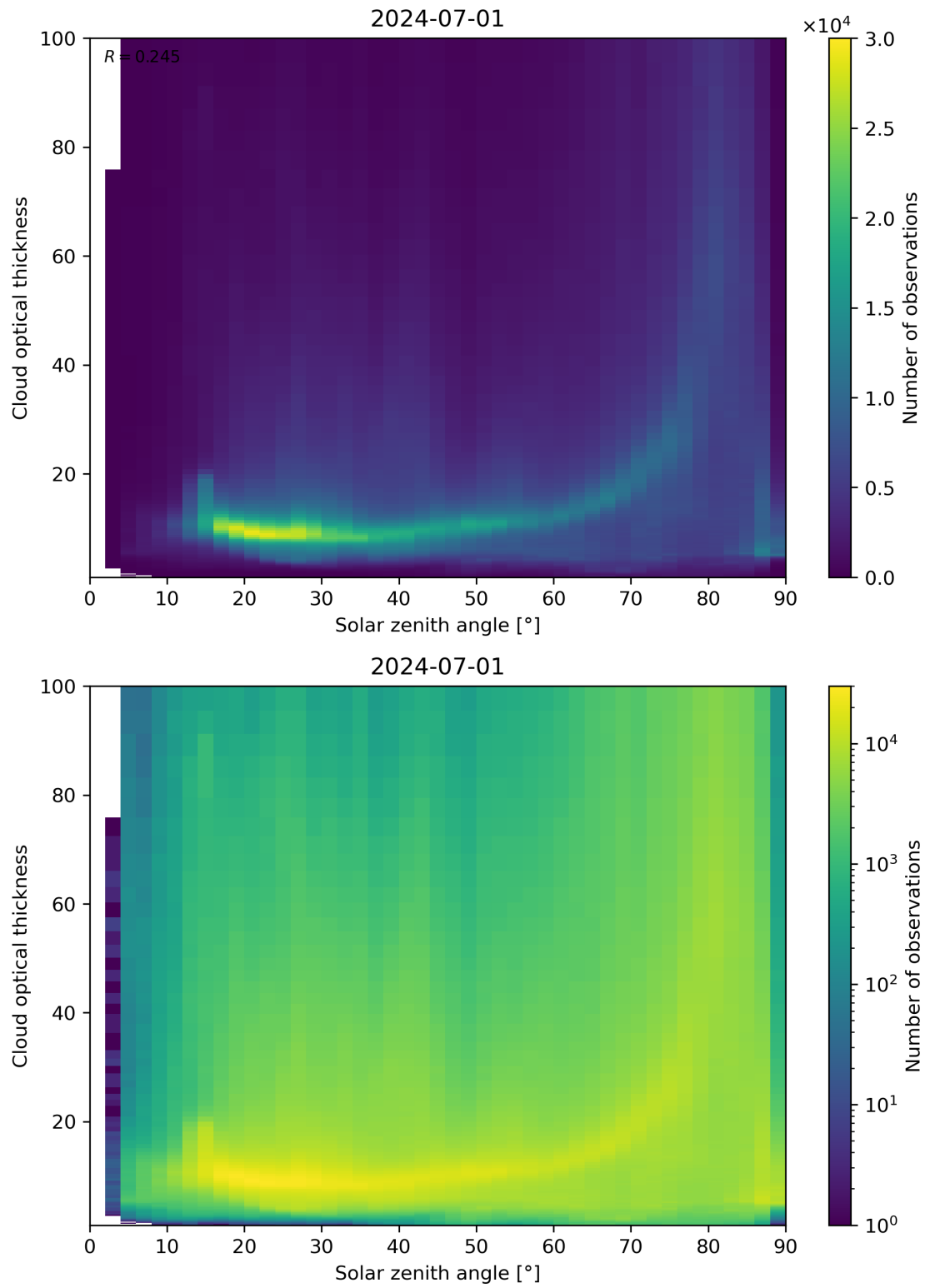
Figure 103: Scatter density plot of “Solar zenith angle” against “Cloud optical thickness” for 2024-06-30 to 2024-07-02.
