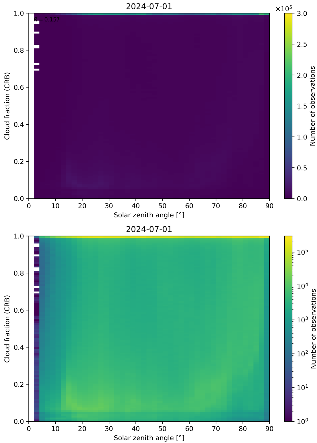
Figure 101: Scatter density plot of “Solar zenith angle” against “Cloud fraction (CRB)” for 2024-06-30 to 2024-07-02.
