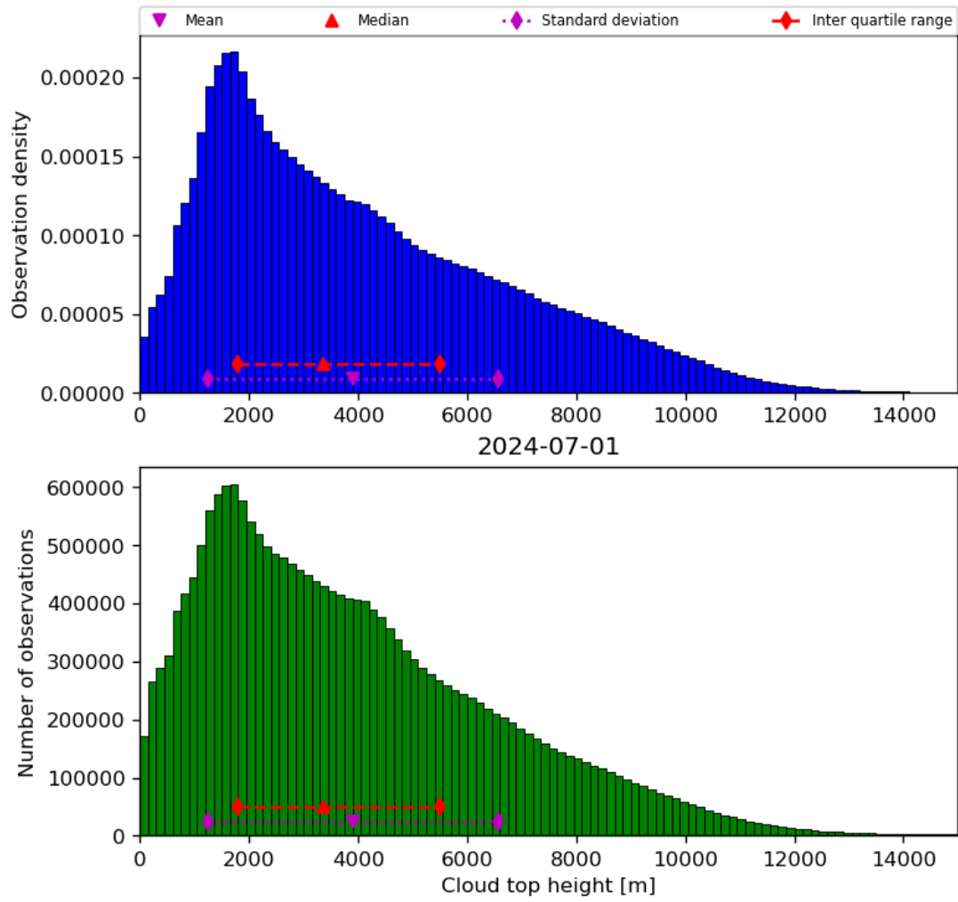
Figure 40: Histogram of “Cloud top height” for 2024-06-30 to 2024-07-02
