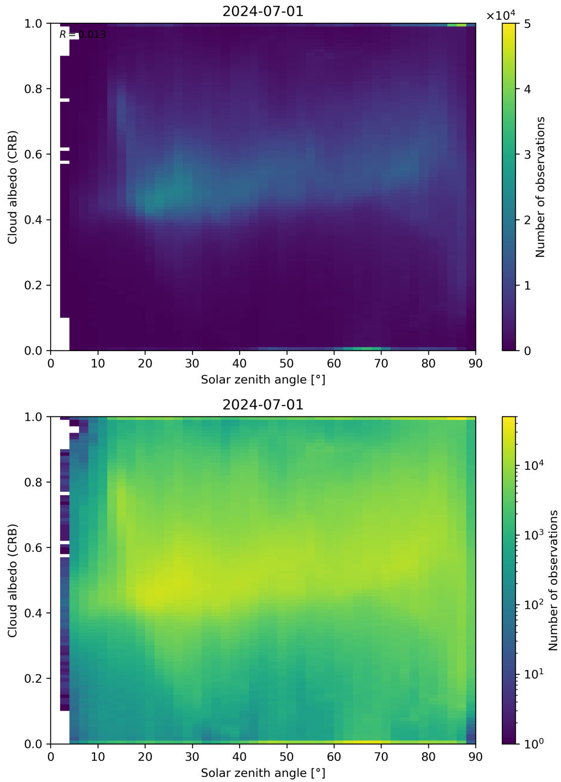
Figure 98: Scatter density plot of “Solar zenith angle” against “Cloud albedo (CRB)” for 2024-06-30 to 2024-07-02.
