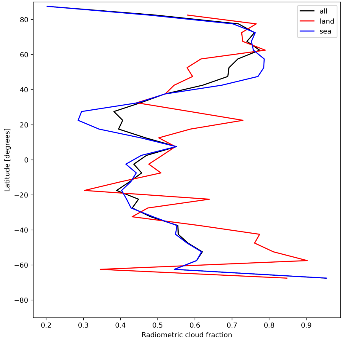
Figure 23: Zonal average of “Radiometric cloud fraction” for 2024-06-30 to 2024-07-02.
