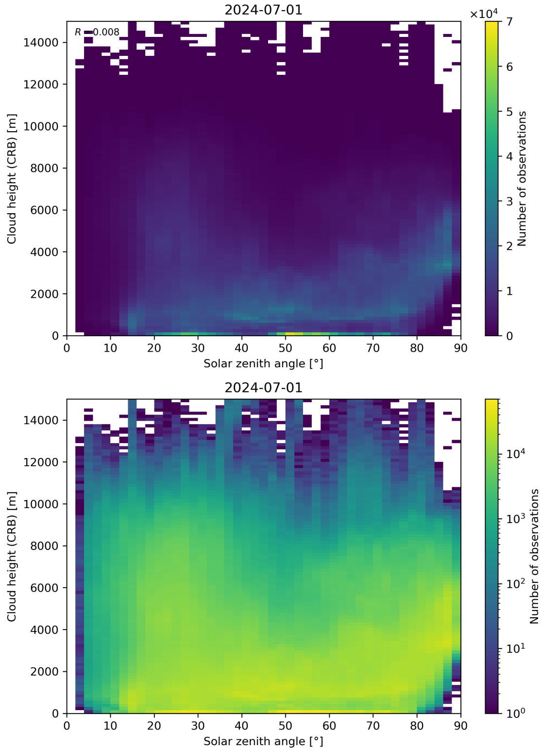
Figure 102: Scatter density plot of “Solar zenith angle” against “Cloud height (CRB)” for 2024-06-30 to 2024-07-02.
