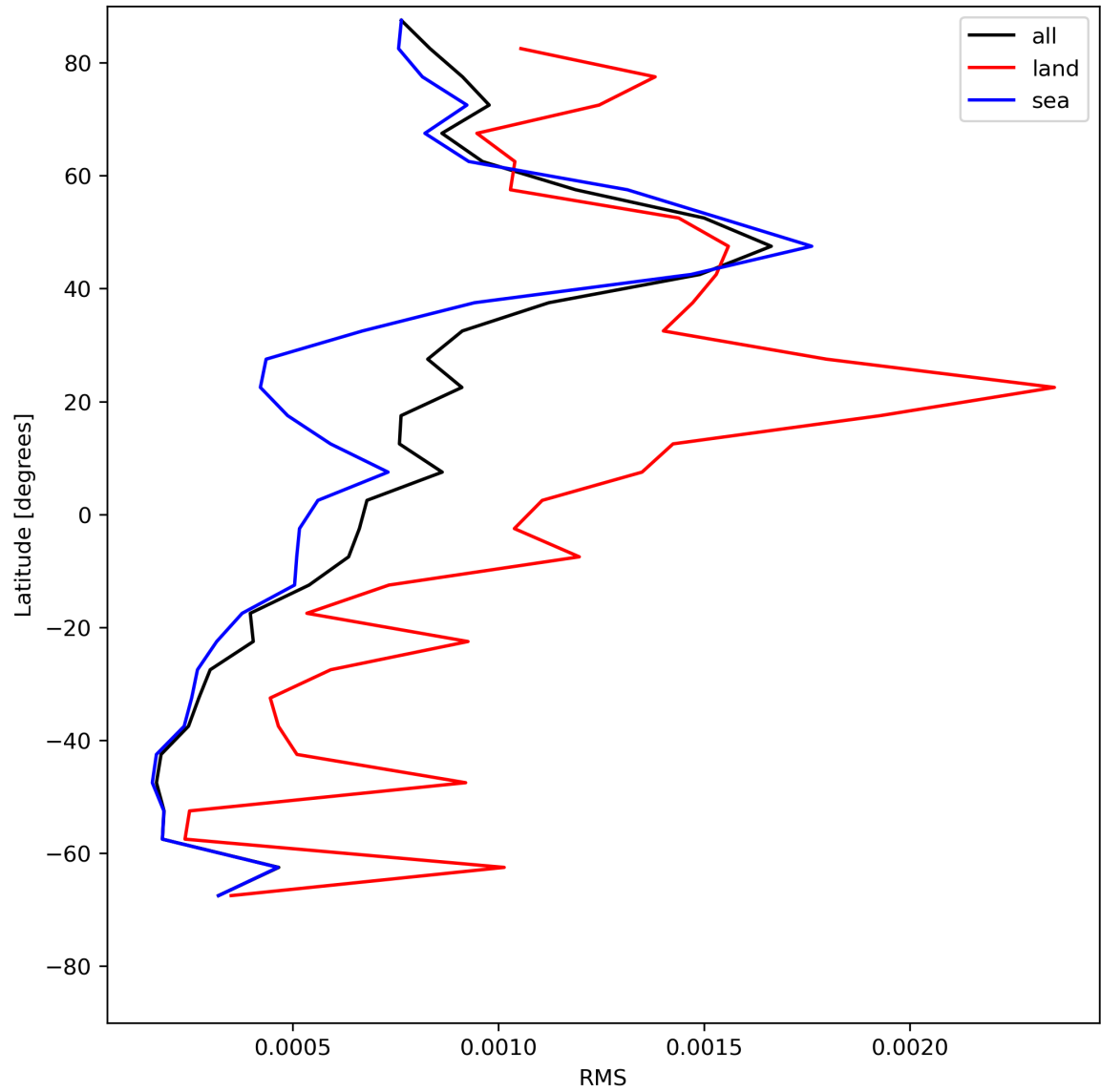
Figure 31: Zonal average of “RMS” for 2024-06-30 to 2024-07-02.
