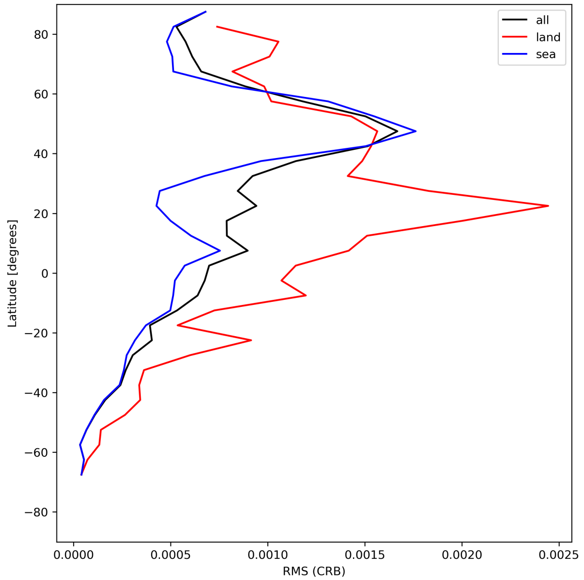
Figure 32: Zonal average of “RMS (CRB)” for 2024-06-30 to 2024-07-02.
