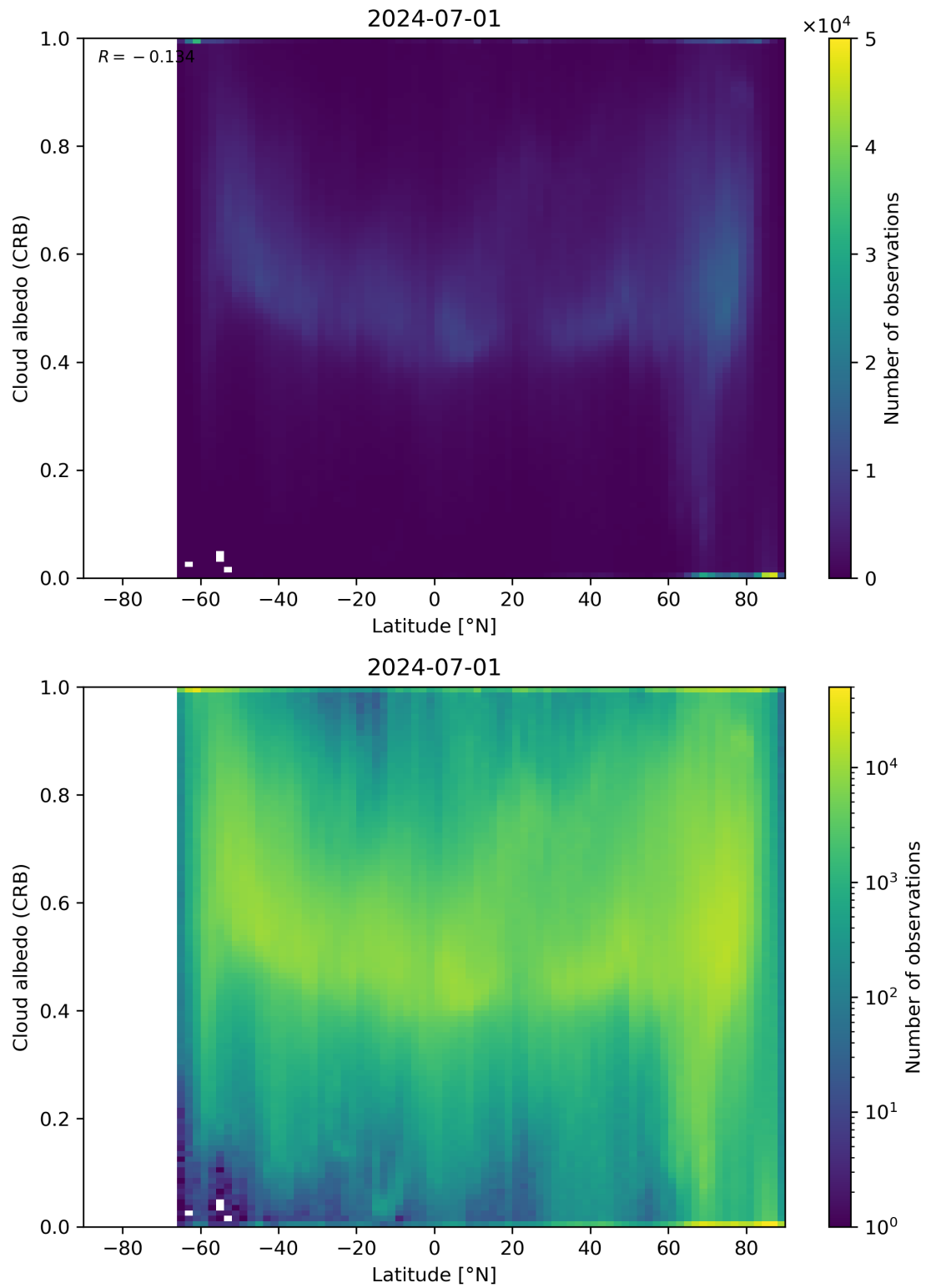
Figure 91: Scatter density plot of “Latitude” against “Cloud albedo (CRB)” for 2024-06-30 to 2024-07-02.
