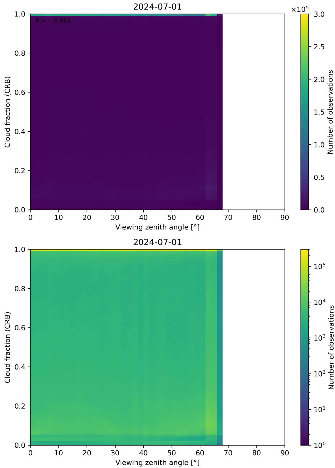
Figure 109: Scatter density plot of “Viewing zenith angle” against “Cloud fraction (CRB)” for 2024-06-30 to 2024-07-02.
