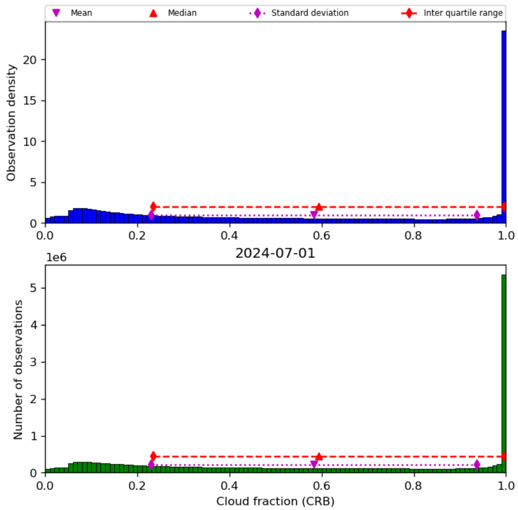
Figure 42: Histogram of “Cloud fraction (CRB)” for 2024-06-30 to 2024-07-02
