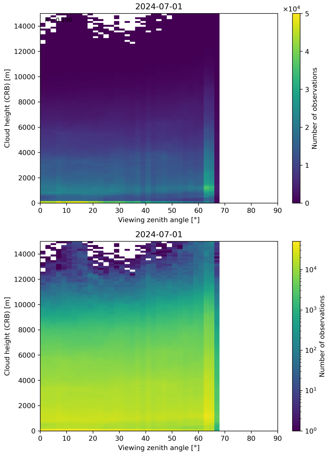
Figure 110: Scatter density plot of “Viewing zenith angle” against “Cloud height (CRB)” for 2024-06-30 to 2024-07-02.
