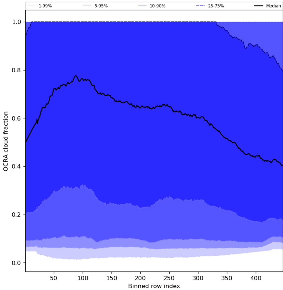
Figure 66: Along track statistics of “OCRA cloud fraction” for 2024-06-30 to 2024-07-02
