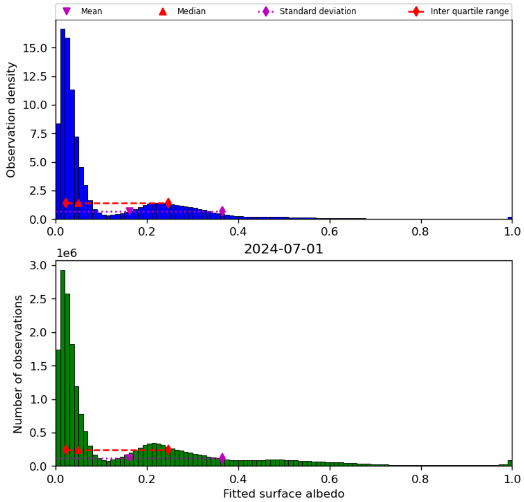
Figure 45: Histogram of “Fitted surface albedo” for 2024-06-30 to 2024-07-02
