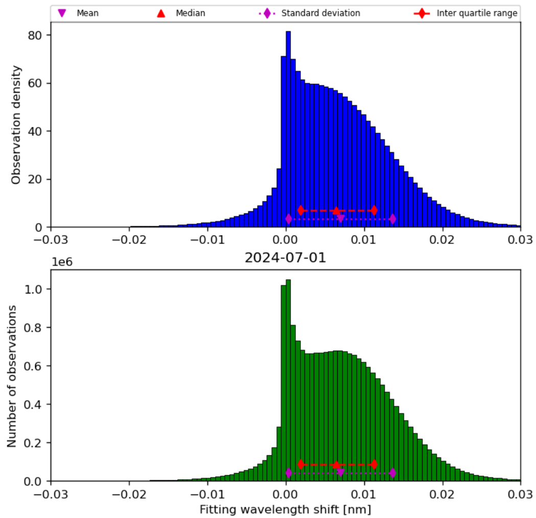
Figure 49: Histogram of “Fitting wavelength shift” for 2024-06-30 to 2024-07-02
