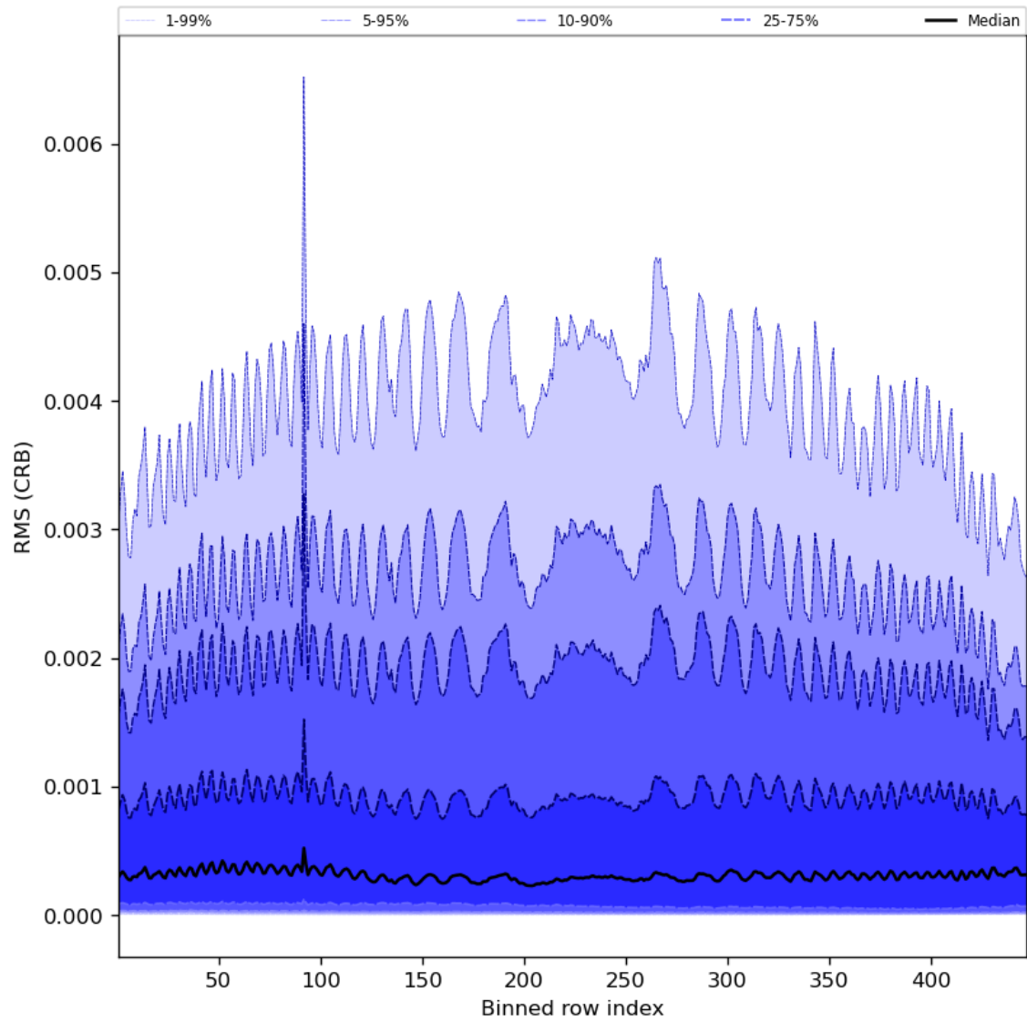
Figure 64: Along track statistics of “RMS (CRB)” for 2024-06-30 to 2024-07-02
