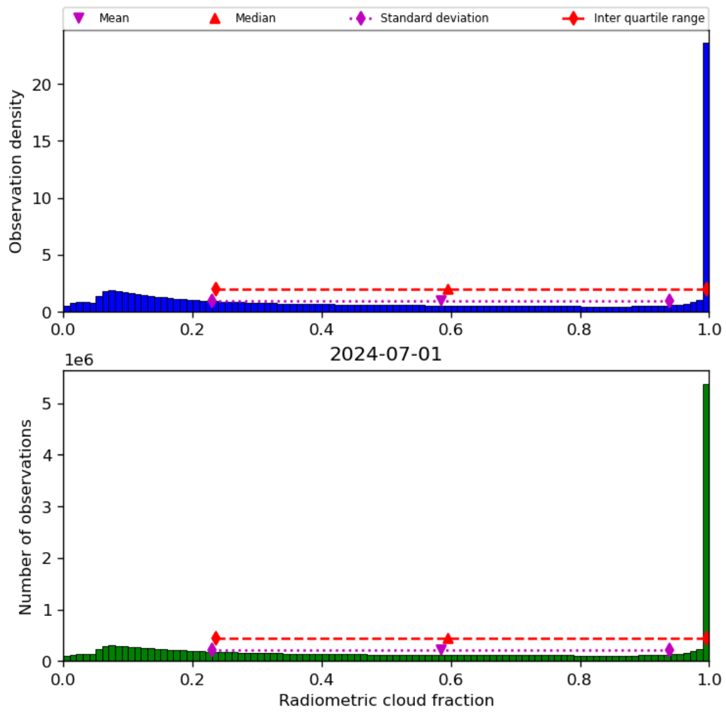
Figure 39: Histogram of “Radiometric cloud fraction” for 2024-06-30 to 2024-07-02
