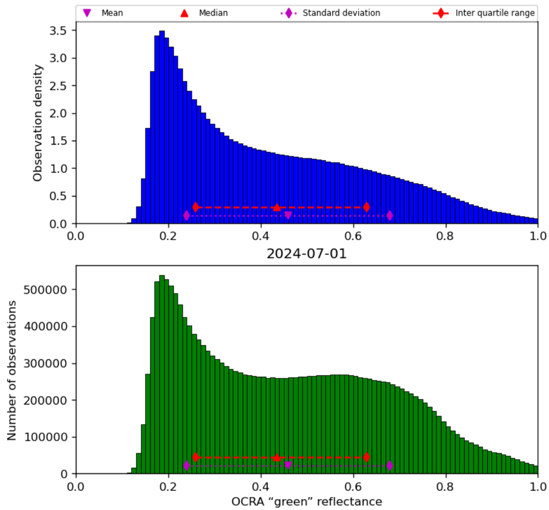
Figure 52: Histogram of “OCRA “green” reflectance” for 2024-06-30 to 2024-07-02
