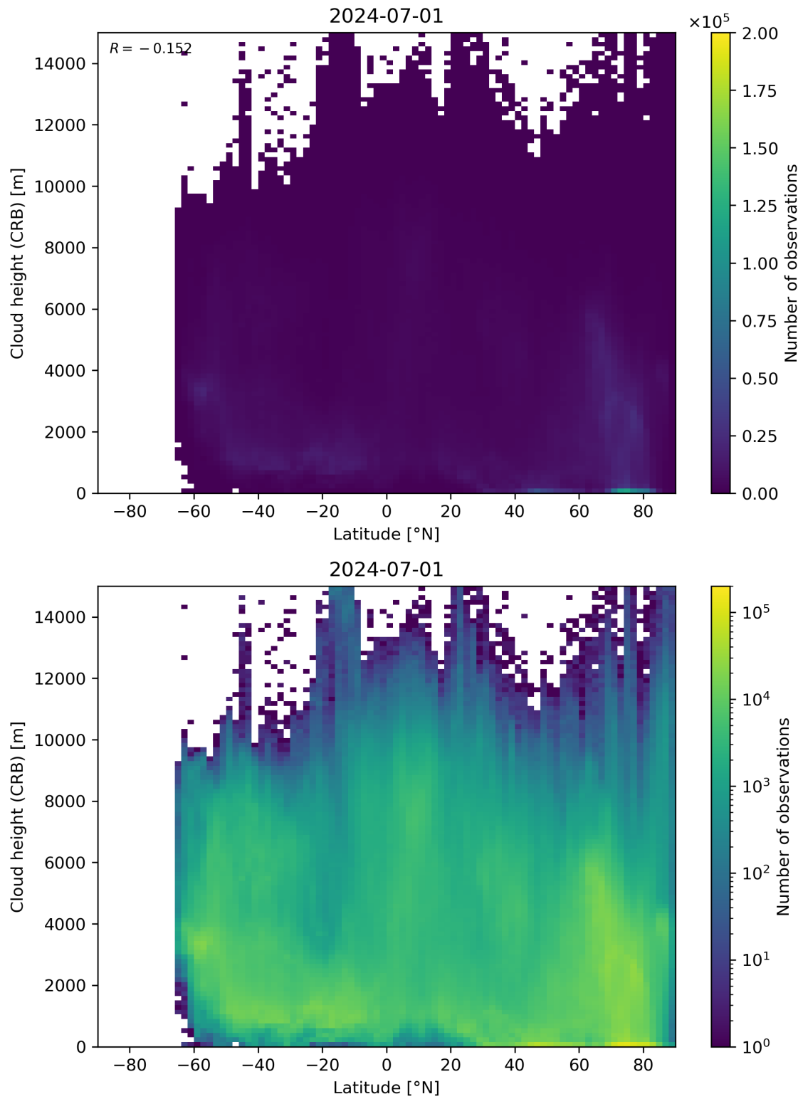
Figure 95: Scatter density plot of “Latitude” against “Cloud height (CRB)” for 2024-06-30 to 2024-07-02.
