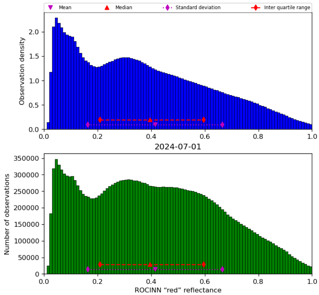
Figure 53: Histogram of “ROCINN “red” reflectance” for 2024-06-30 to 2024-07-02
