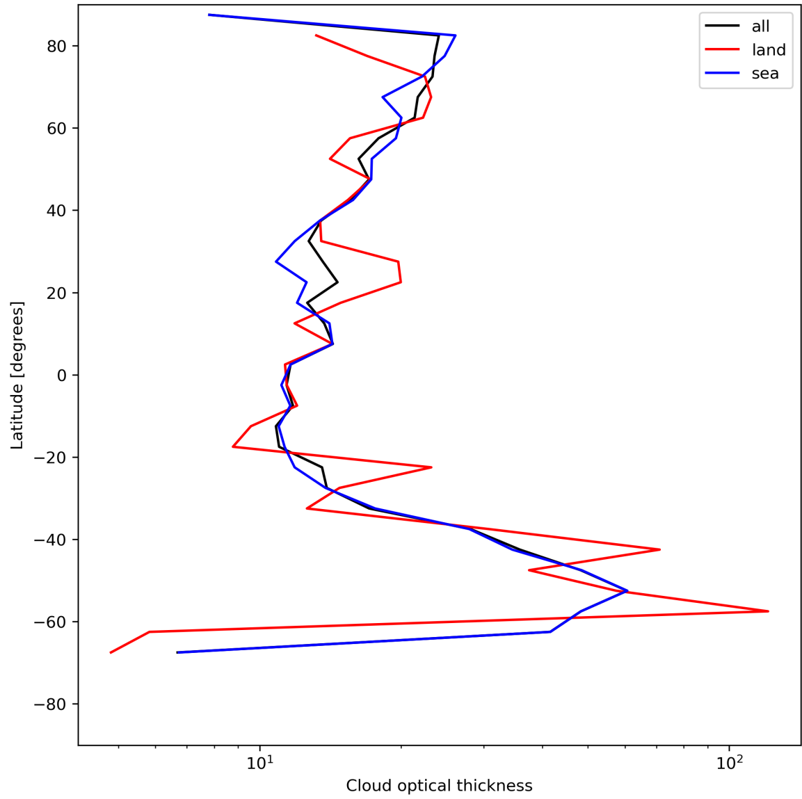
Figure 25: Zonal average of “Cloud optical thickness” for 2024-06-30 to 2024-07-02.
