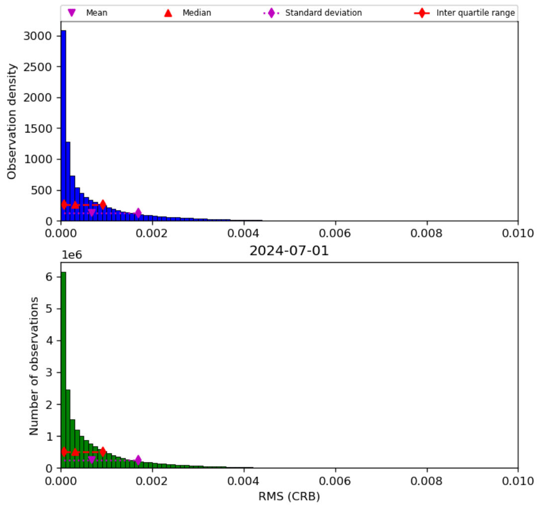
Figure 48: Histogram of “RMS (CRB)” for 2024-06-30 to 2024-07-02
