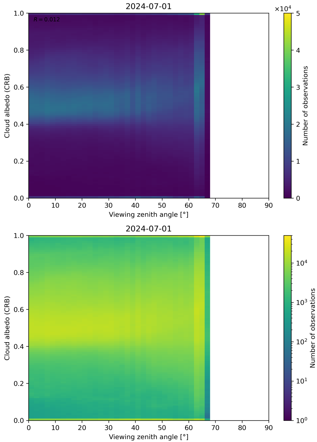
Figure 106: Scatter density plot of “Viewing zenith angle” against “Cloud albedo (CRB)” for 2024-06-30 to 2024-07-02.
