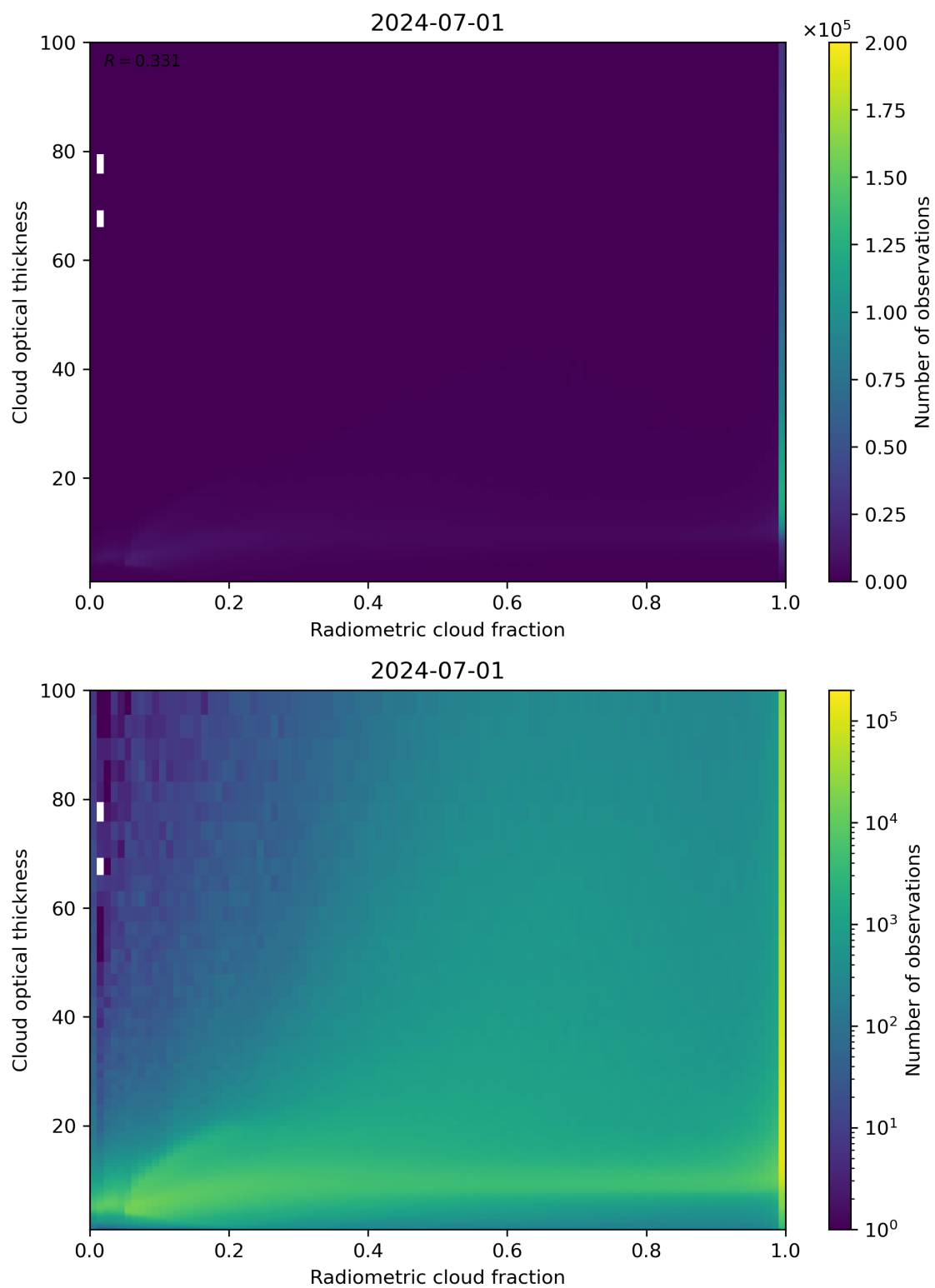
Figure 75: Scatter density plot of “Radiometric cloud fraction” against “Cloud optical thickness” for 2024-06-30 to 2024-07-02.
