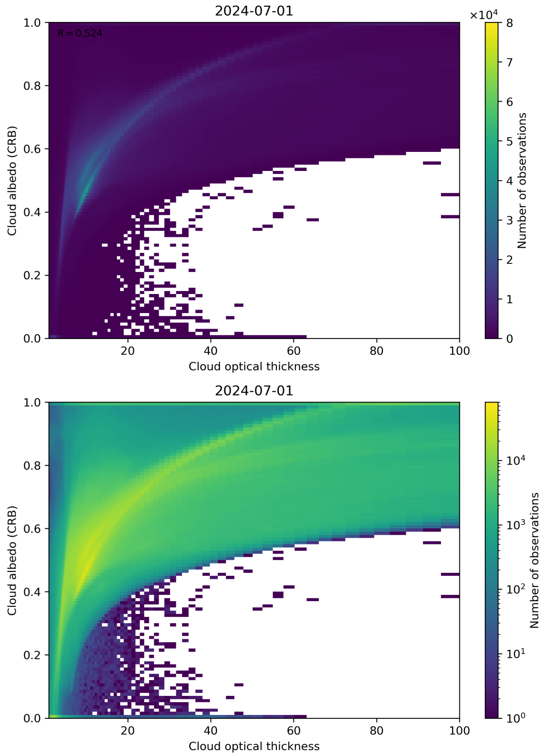
Figure 82: Scatter density plot of “Cloud optical thickness” against “Cloud albedo (CRB)” for 2024-06-30 to 2024-07-02.
