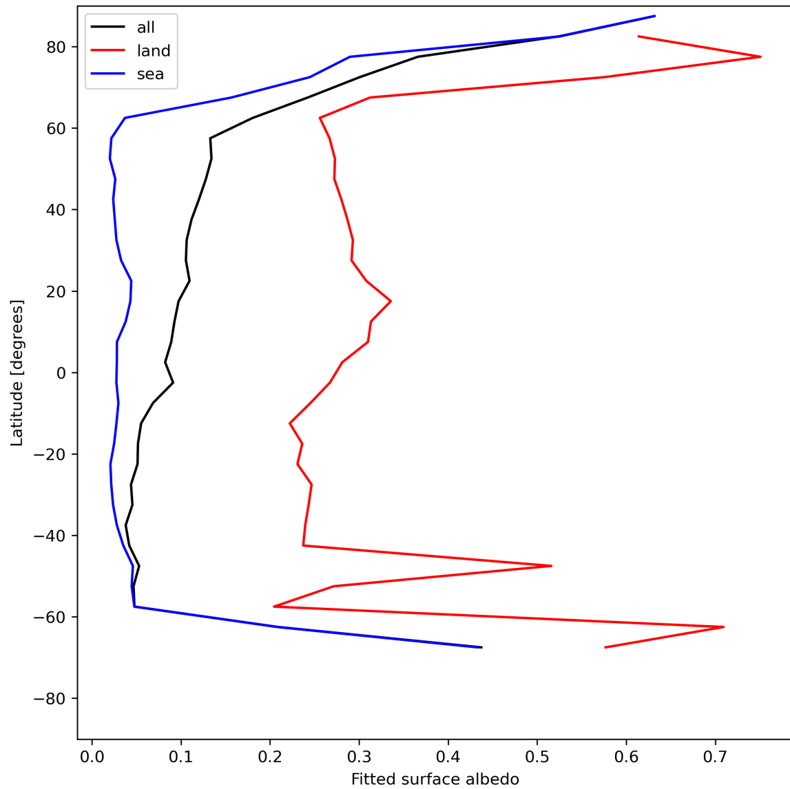
Figure 29: Zonal average of “Fitted surface albedo” for 2024-06-30 to 2024-07-02.
