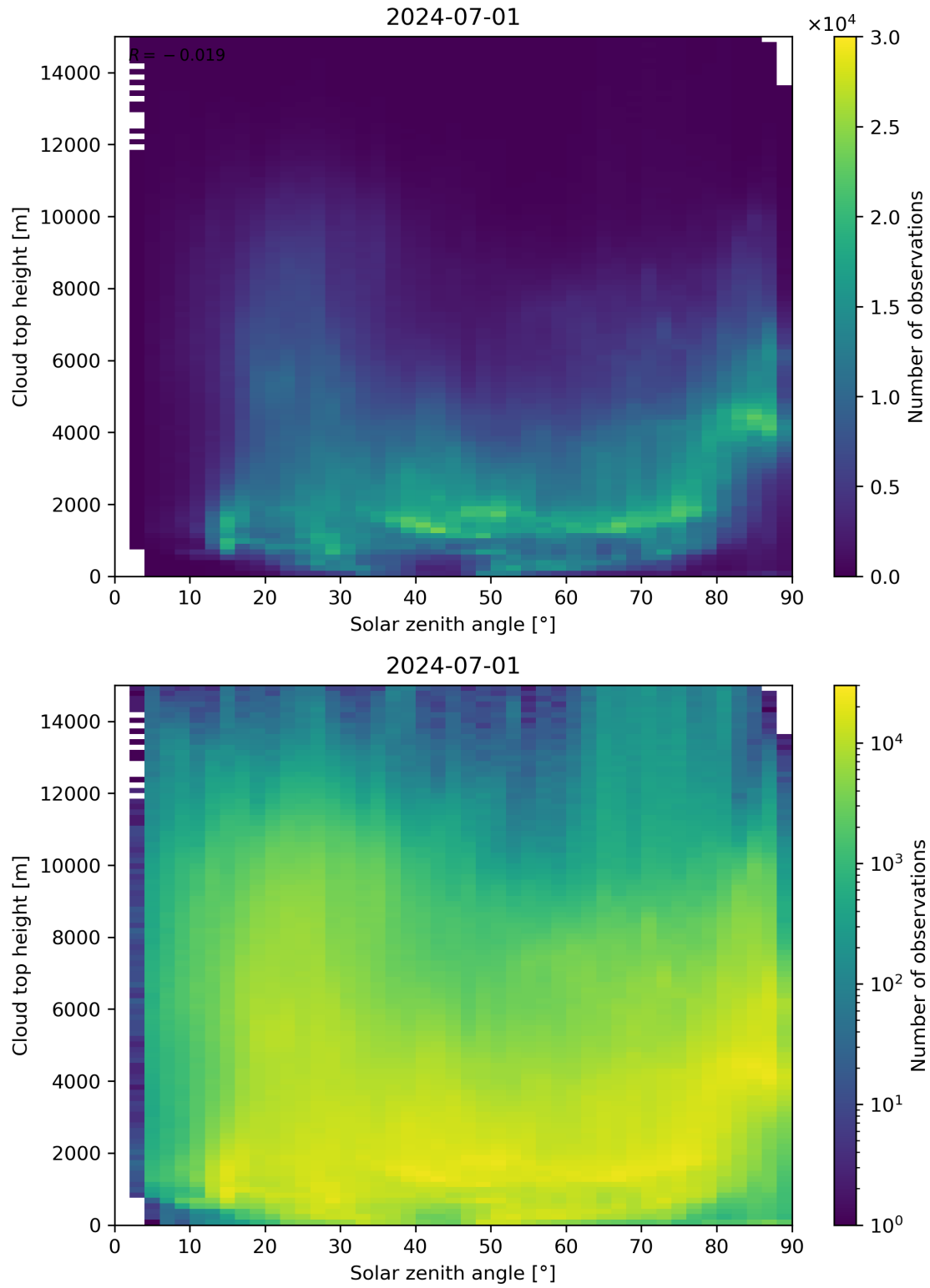
Figure 104: Scatter density plot of “Solar zenith angle” against “Cloud top height” for 2024-06-30 to 2024-07-02.
