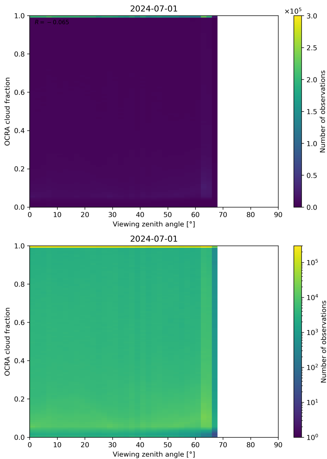
Figure 108: Scatter density plot of “Viewing zenith angle” against “OCRA cloud fraction” for 2024-06-30 to 2024-07-02.
