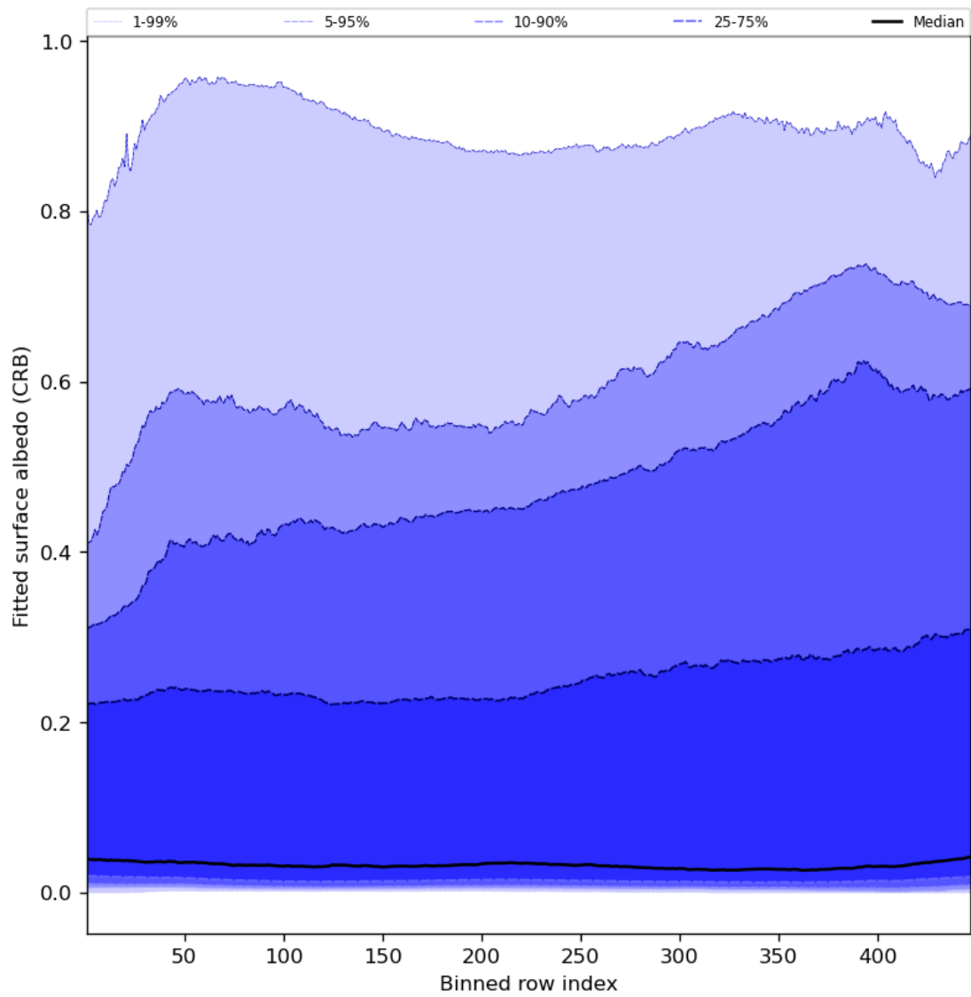
Figure 62: Along track statistics of “Fitted surface albedo (CRB)” for 2024-06-30 to 2024-07-02
