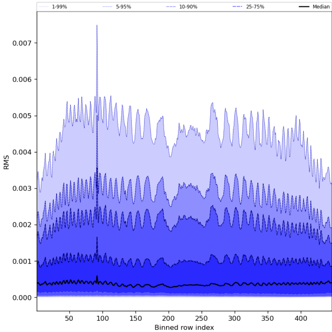
Figure 63: Along track statistics of “RMS” for 2024-06-30 to 2024-07-02
