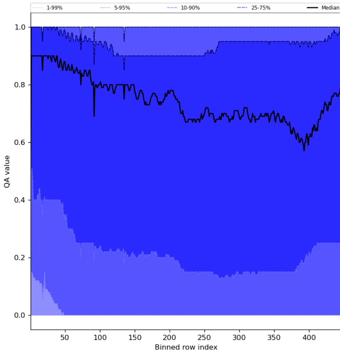
Figure 54: Along track statistics of “QA value” for 2024-06-30 to 2024-07-02
