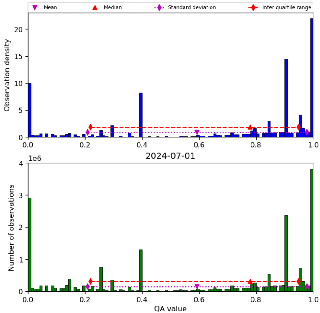
Figure 38: Histogram of “QA value” for 2024-06-30 to 2024-07-02
