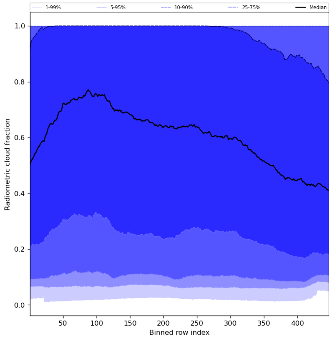
Figure 55: Along track statistics of “Radiometric cloud fraction” for 2024-06-30 to 2024-07-02
