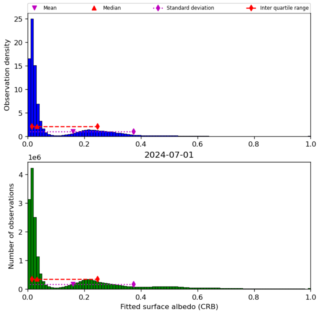
Figure 46: Histogram of “Fitted surface albedo (CRB)” for 2024-06-30 to 2024-07-02
