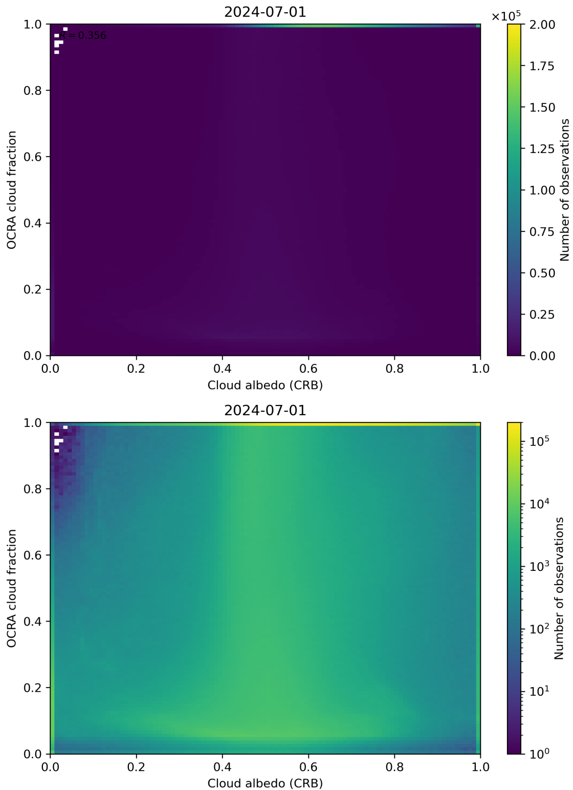
Figure 70: Scatter density plot of “Cloud albedo (CRB)” against “OCRA cloud fraction” for 2024-06-30 to 2024-07-02.
