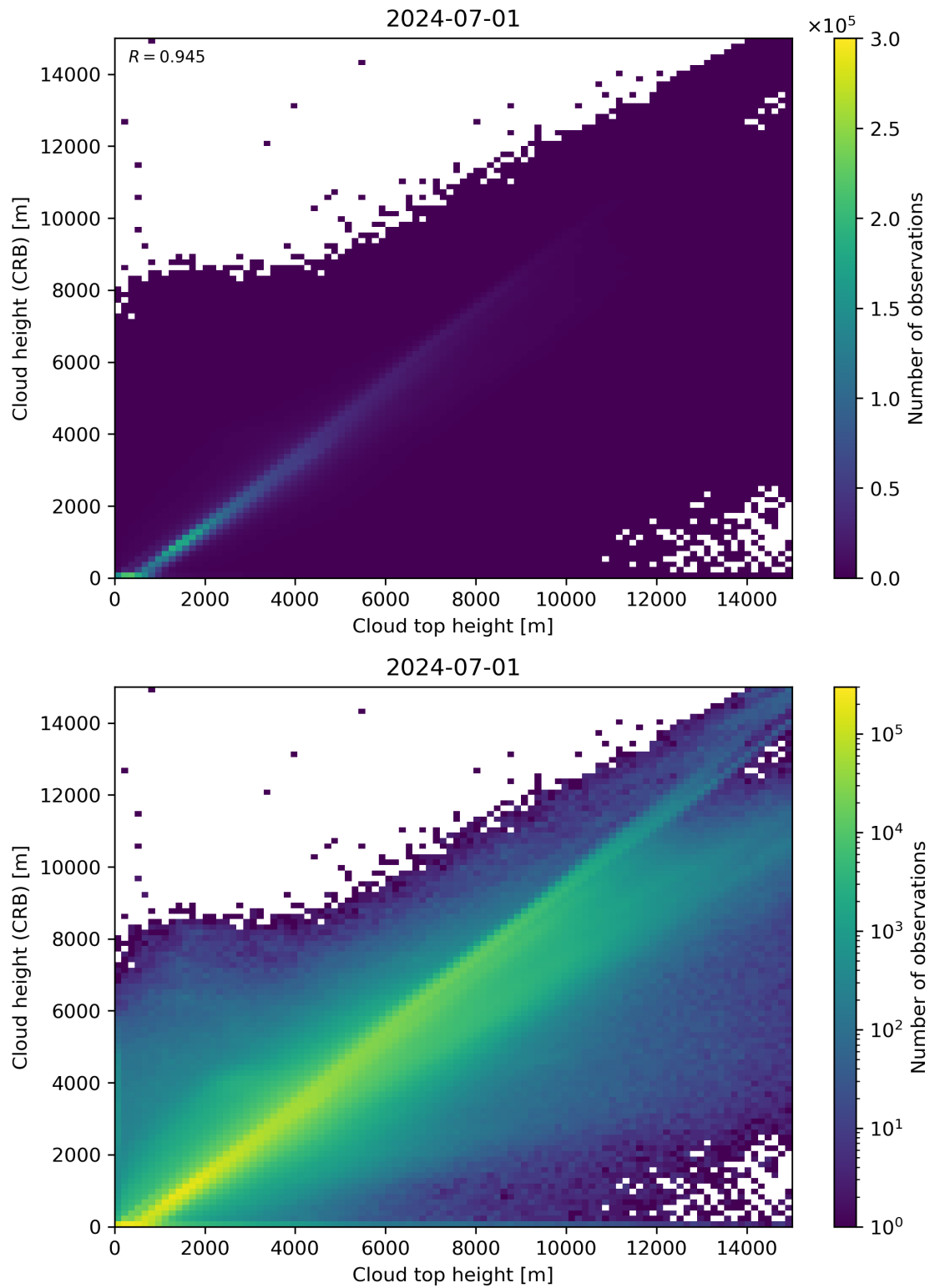
Figure 89: Scatter density plot of “Cloud top height” against “Cloud height (CRB)” for 2024-06-30 to 2024-07-02.
