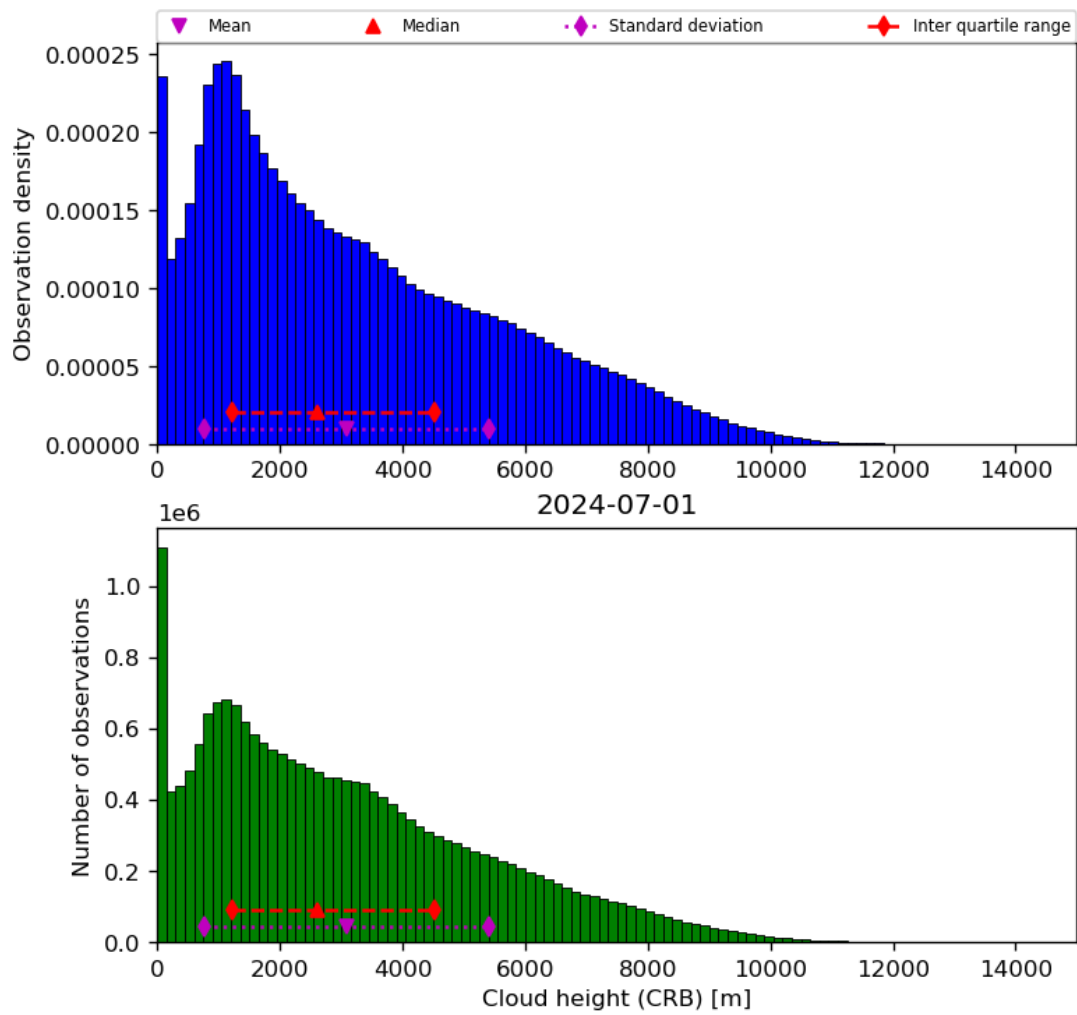
Figure 43: Histogram of “Cloud height (CRB)” for 2024-06-30 to 2024-07-02
