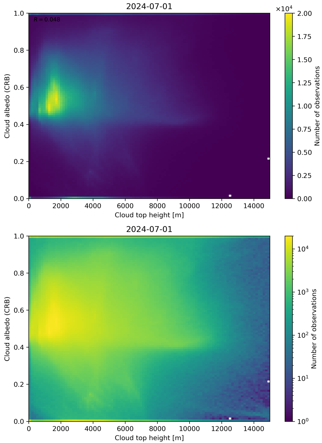
Figure 86: Scatter density plot of “Cloud top height” against “Cloud albedo (CRB)” for 2024-06-30 to 2024-07-02.
