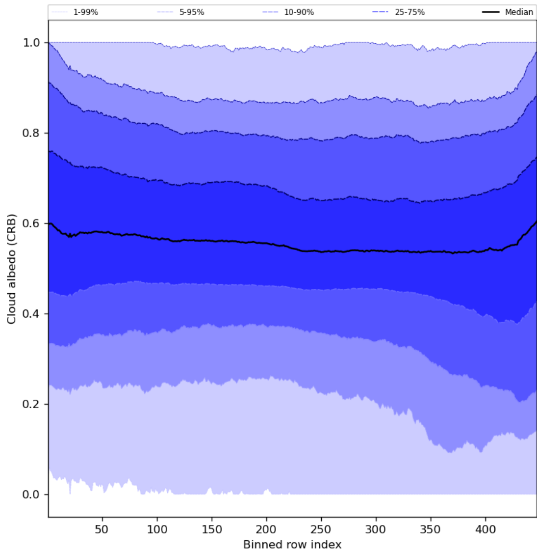
Figure 60: Along track statistics of “Cloud albedo (CRB)” for 2024-06-30 to 2024-07-02
