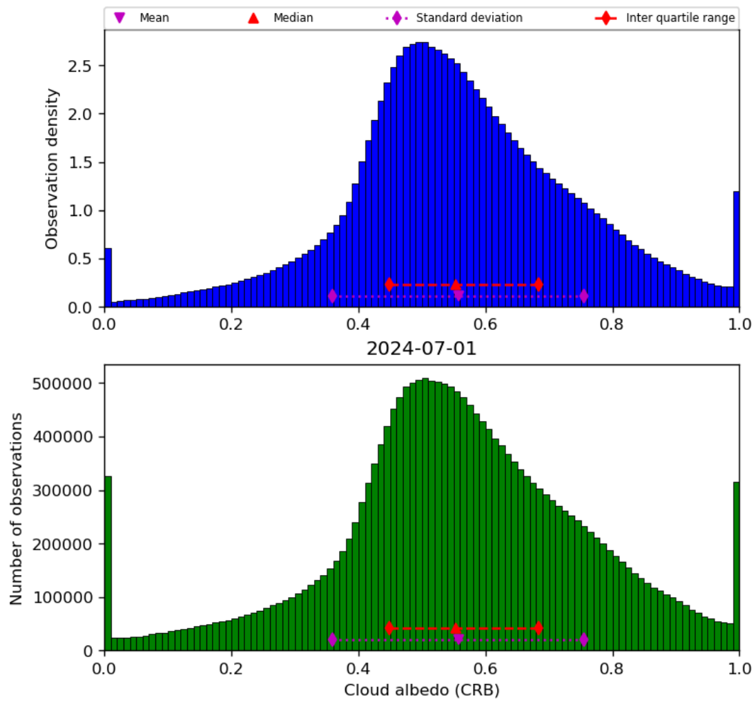
Figure 44: Histogram of “Cloud albedo (CRB)” for 2024-06-30 to 2024-07-02
