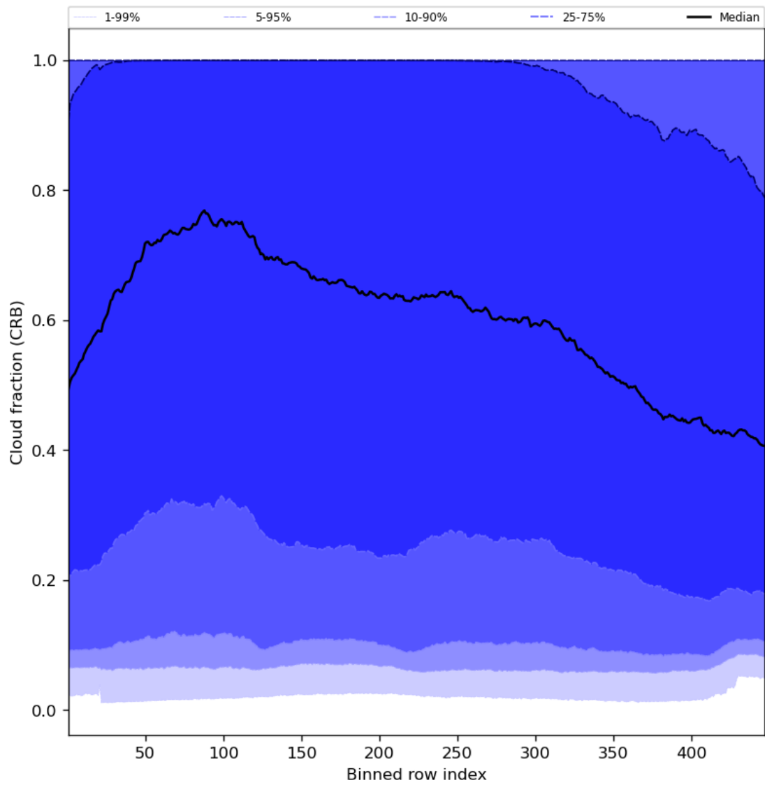
Figure 58: Along track statistics of “Cloud fraction (CRB)” for 2024-06-30 to 2024-07-02
