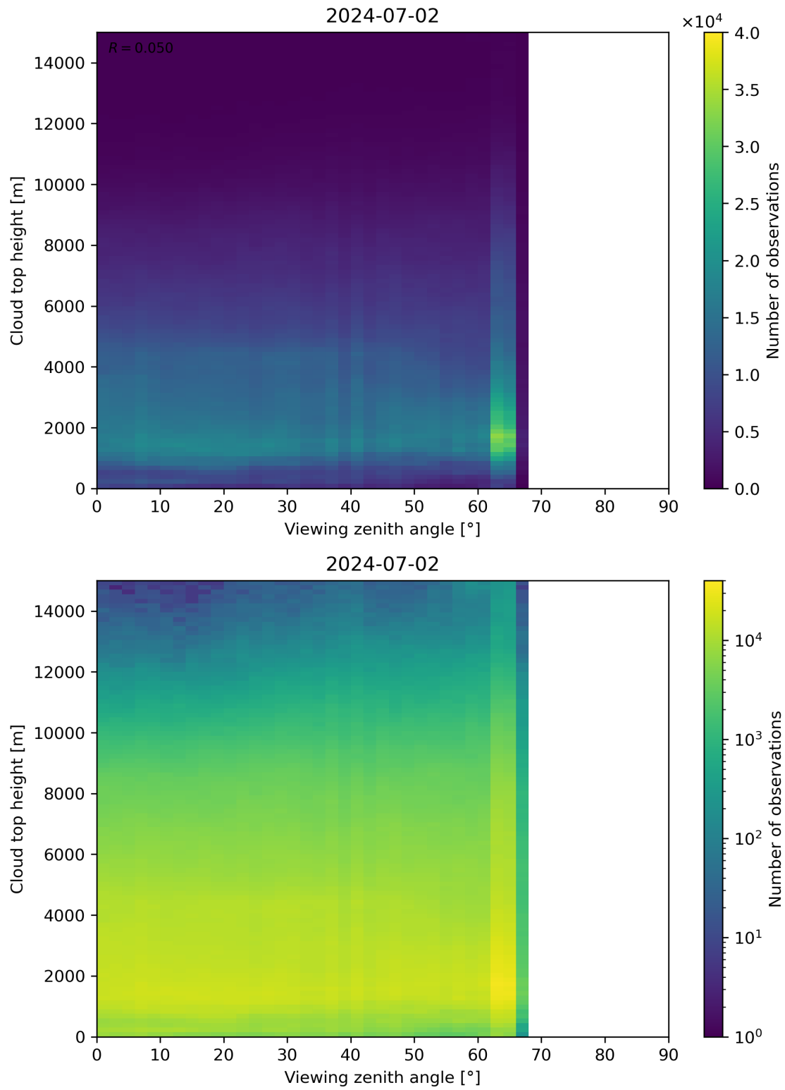
Figure 112: Scatter density plot of “Viewing zenith angle” against “Cloud top height” for 2024-07-01 to 2024-07-03.
