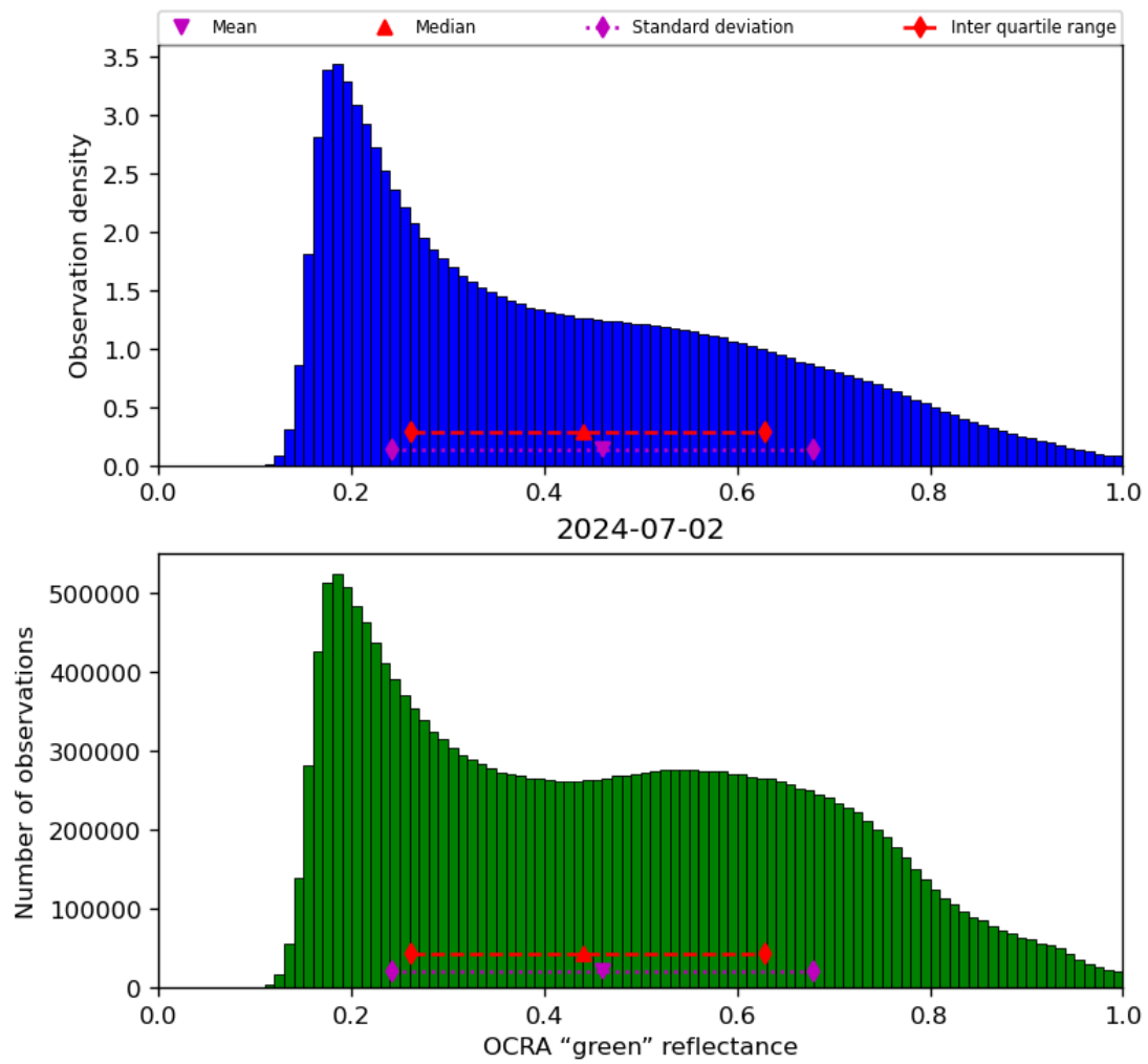
Figure 52: Histogram of “OCRA “green” reflectance” for 2024-07-01 to 2024-07-03
