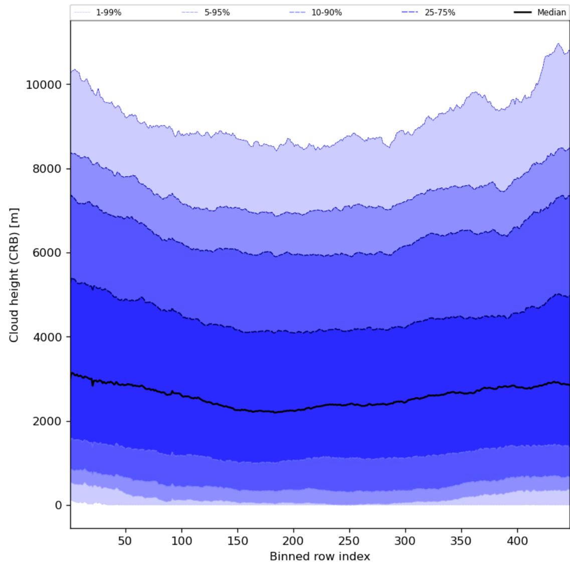
Figure 59: Along track statistics of “Cloud height (CRB)” for 2024-07-01 to 2024-07-03
