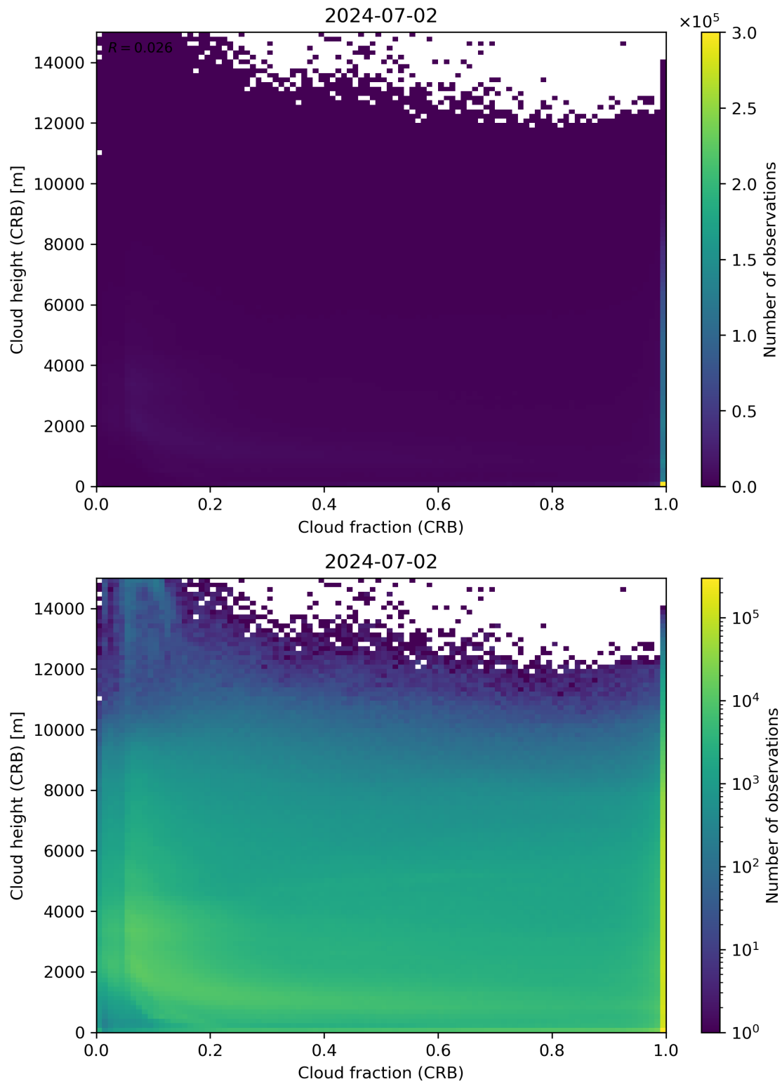
Figure 79: Scatter density plot of “Cloud fraction (CRB)” against “Cloud height (CRB)” for 2024-07-01 to 2024-07-03.
