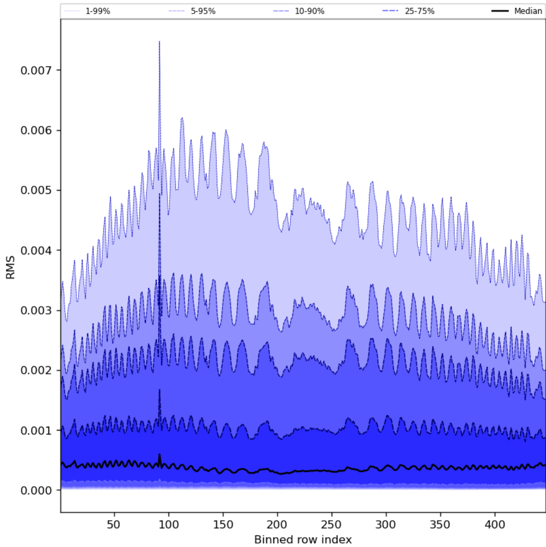
Figure 63: Along track statistics of “RMS” for 2024-07-01 to 2024-07-03
