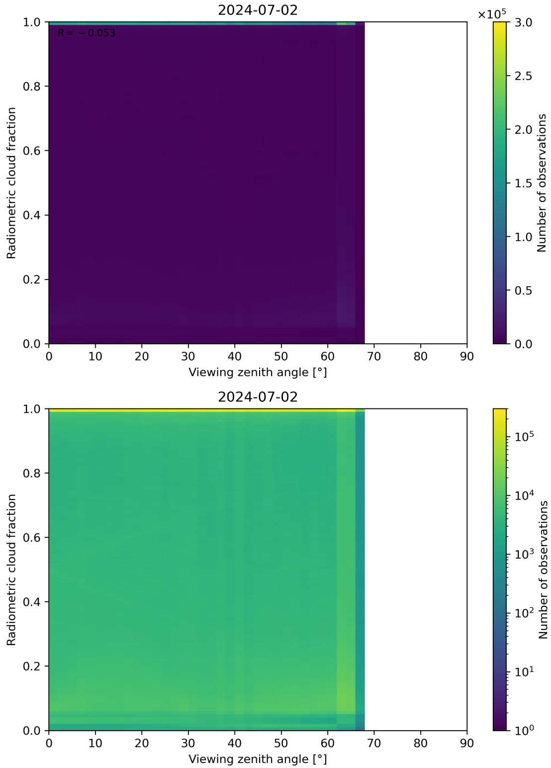
Figure 107: Scatter density plot of “Viewing zenith angle” against “Radiometric cloud fraction” for 2024-07-01 to 2024-07-03.
