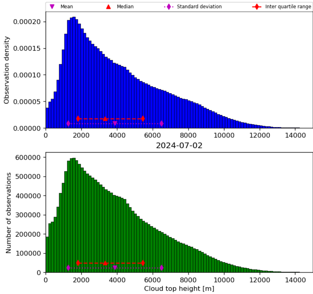
Figure 40: Histogram of “Cloud top height” for 2024-07-01 to 2024-07-03
