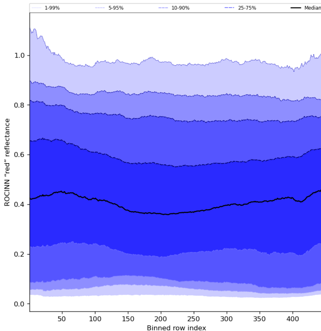
Figure 69: Along track statistics of “ROCINN “red” reflectance” for 2024-07-01 to 2024-07-03
