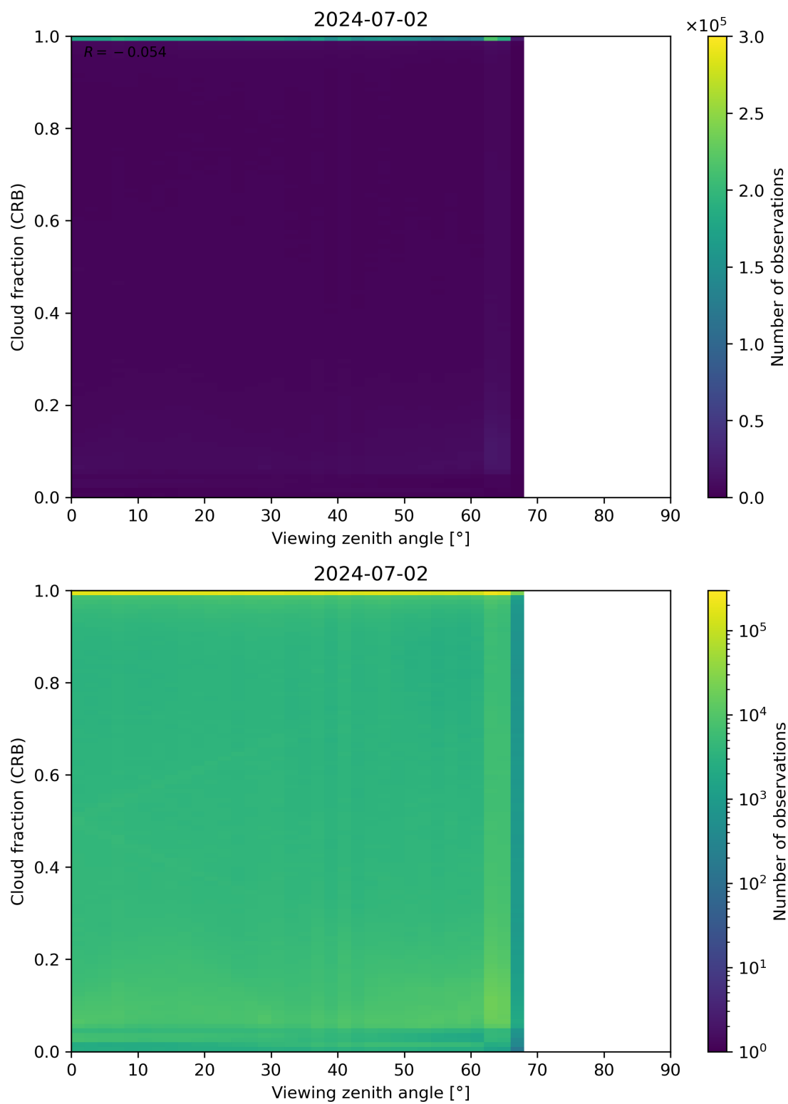
Figure 109: Scatter density plot of “Viewing zenith angle” against “Cloud fraction (CRB)” for 2024-07-01 to 2024-07-03.
