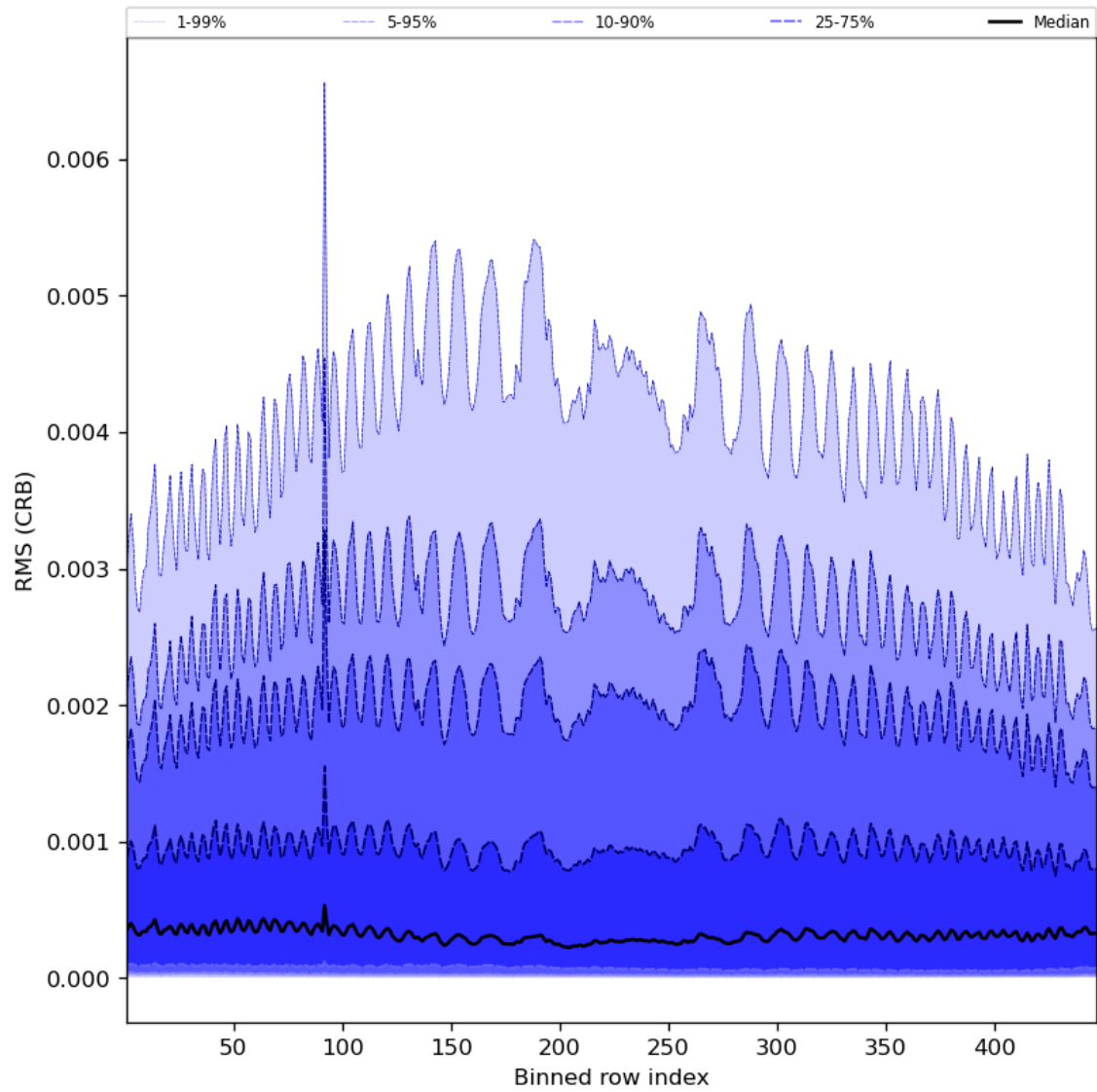
Figure 64: Along track statistics of “RMS (CRB)” for 2024-07-01 to 2024-07-03
