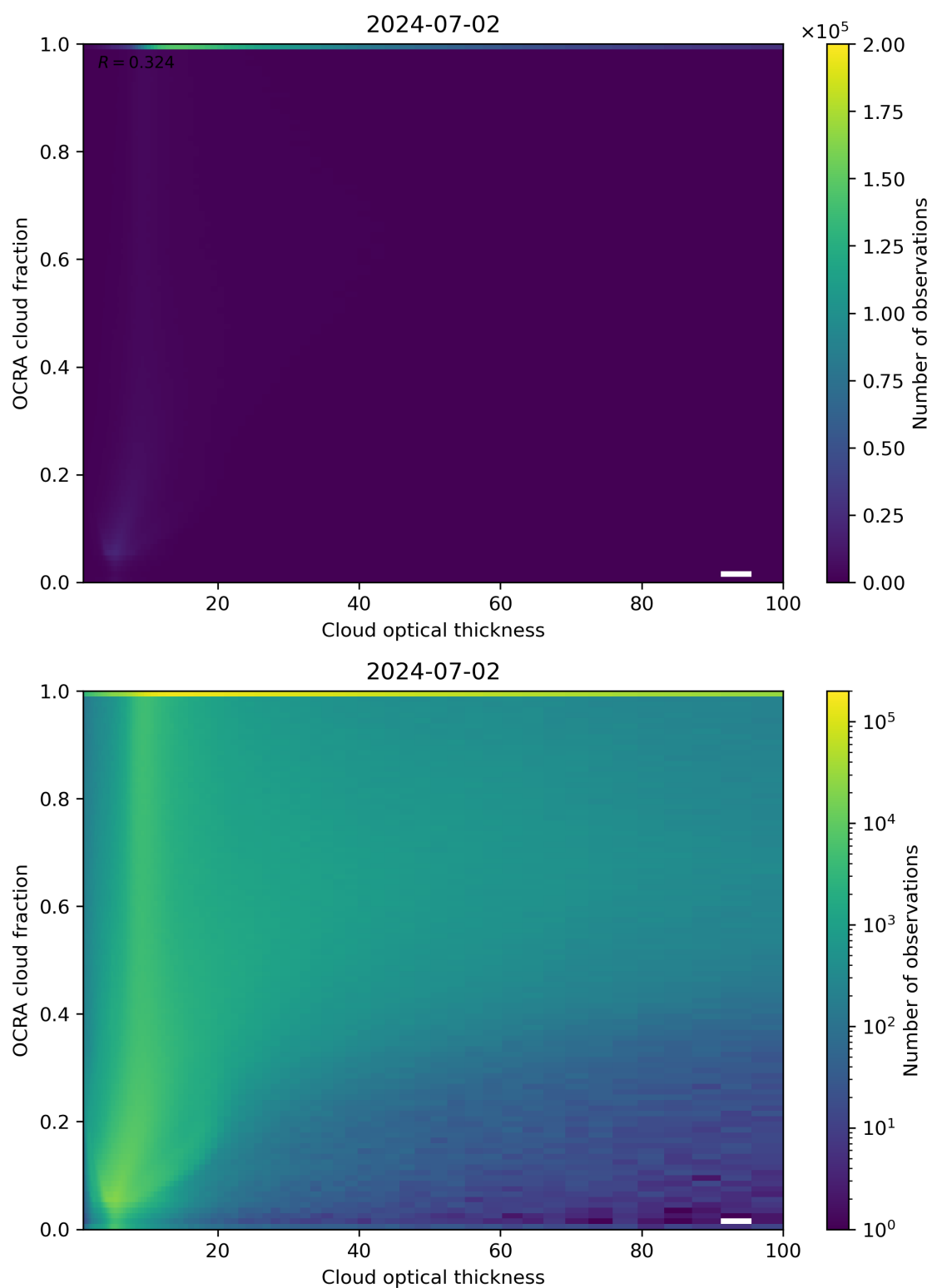
Figure 83: Scatter density plot of “Cloud optical thickness” against “OCRA cloud fraction” for 2024-07-01 to 2024-07-03.
