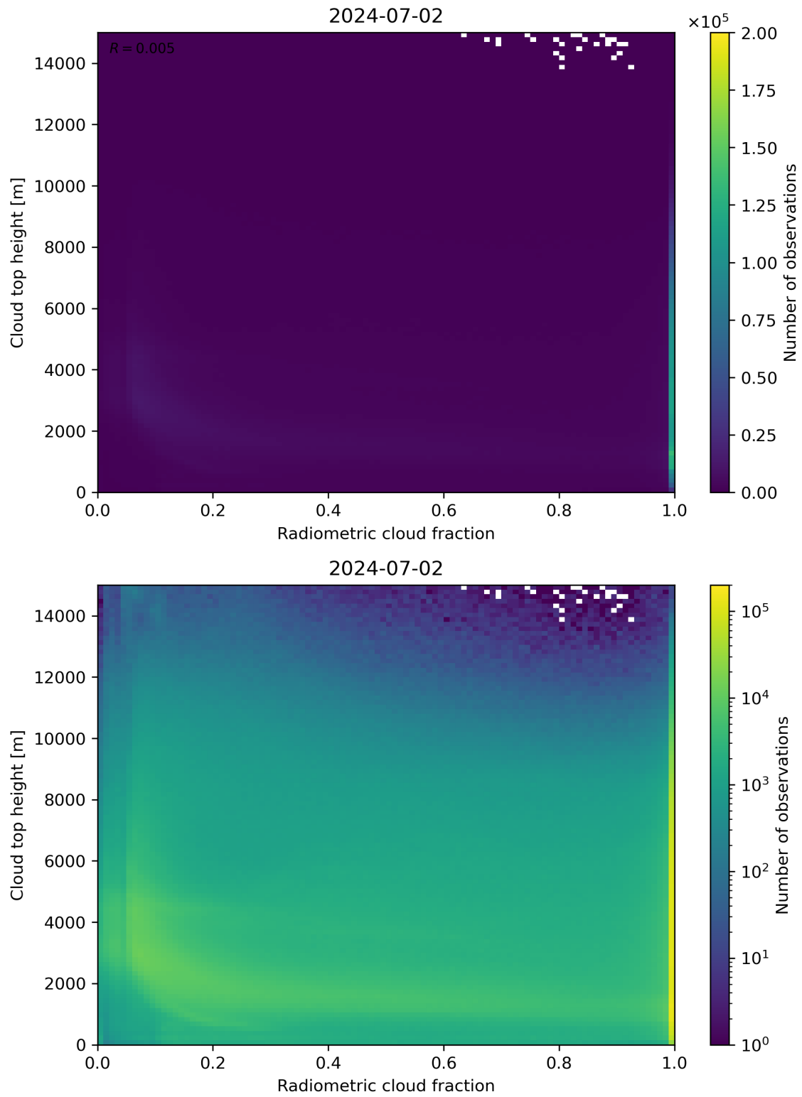
Figure 76: Scatter density plot of “Radiometric cloud fraction” against “Cloud top height” for 2024-07-01 to 2024-07-03.
