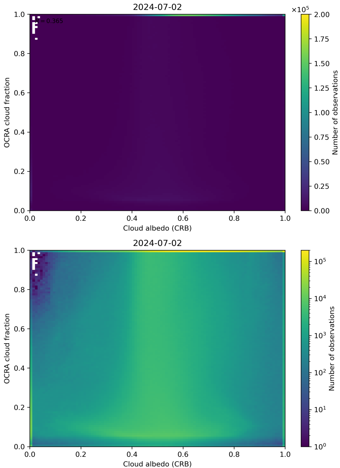
Figure 70: Scatter density plot of “Cloud albedo (CRB)” against “OCRA cloud fraction” for 2024-07-01 to 2024-07-03.
