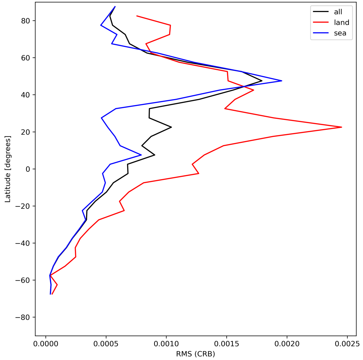
Figure 32: Zonal average of “RMS (CRB)” for 2024-07-01 to 2024-07-03.
