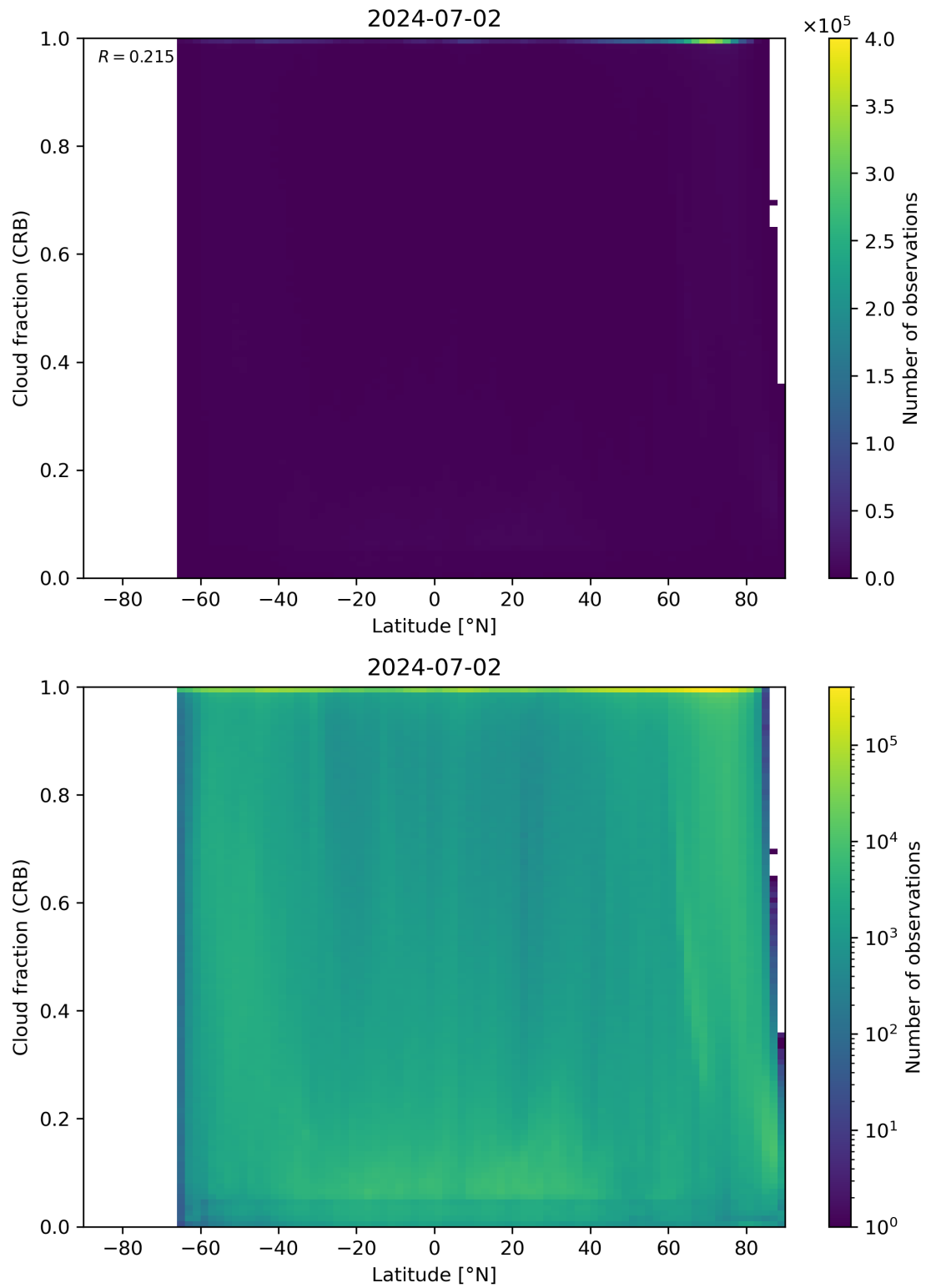
Figure 94: Scatter density plot of “Latitude” against “Cloud fraction (CRB)” for 2024-07-01 to 2024-07-03.
