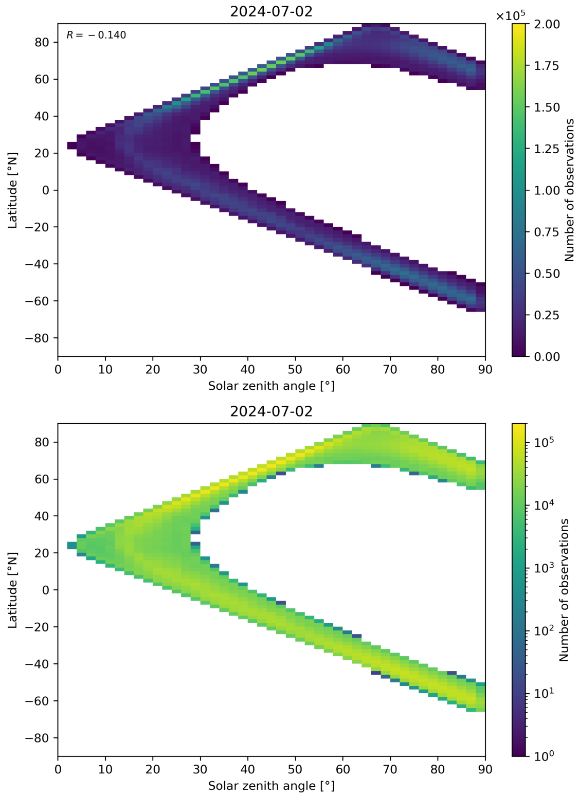
Figure 105: Scatter density plot of “Solar zenith angle” against “Latitude” for 2024-07-01 to 2024-07-03.
