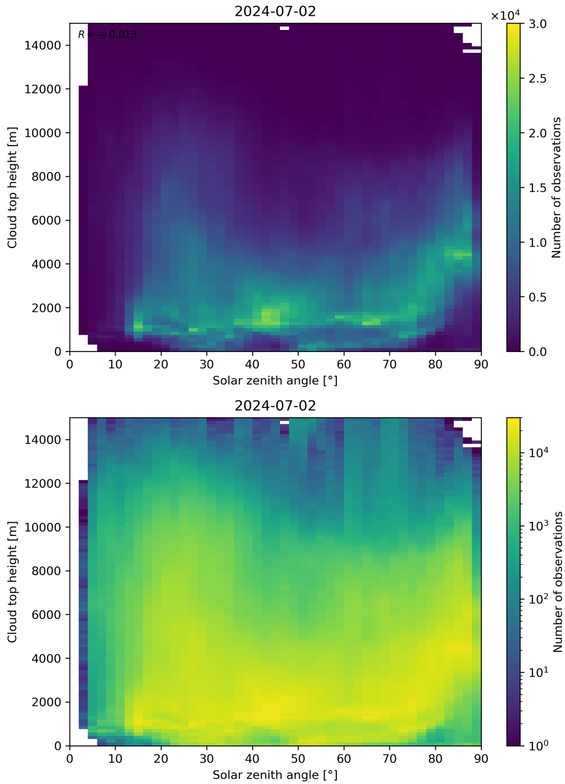
Figure 104: Scatter density plot of “Solar zenith angle” against “Cloud top height” for 2024-07-01 to 2024-07-03.
