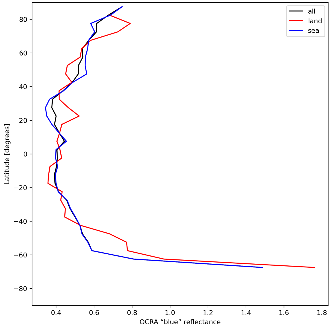
Figure 35: Zonal average of “OCRA “blue” reflectance” for 2024-07-01 to 2024-07-03.
