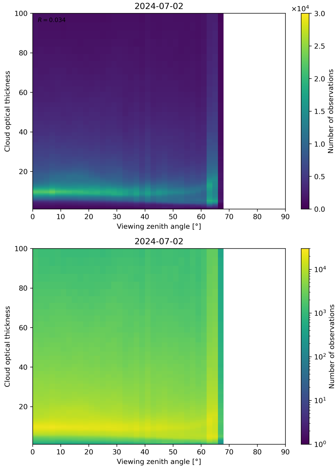
Figure 111: Scatter density plot of “Viewing zenith angle” against “Cloud optical thickness” for 2024-07-01 to 2024-07-03.
