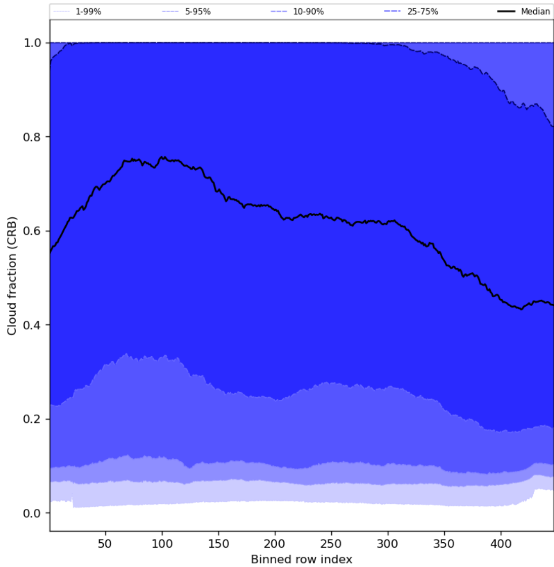
Figure 58: Along track statistics of “Cloud fraction (CRB)” for 2024-07-01 to 2024-07-03
