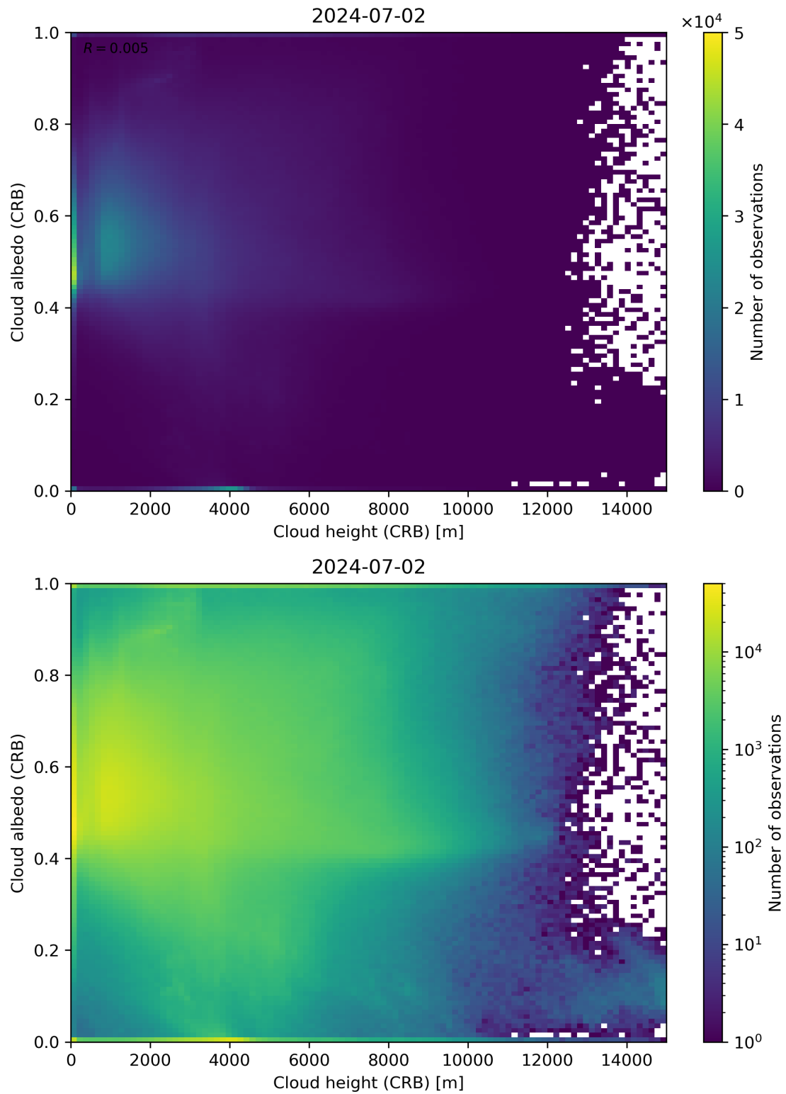
Figure 80: Scatter density plot of “Cloud height (CRB)” against “Cloud albedo (CRB)” for 2024-07-01 to 2024-07-03.
