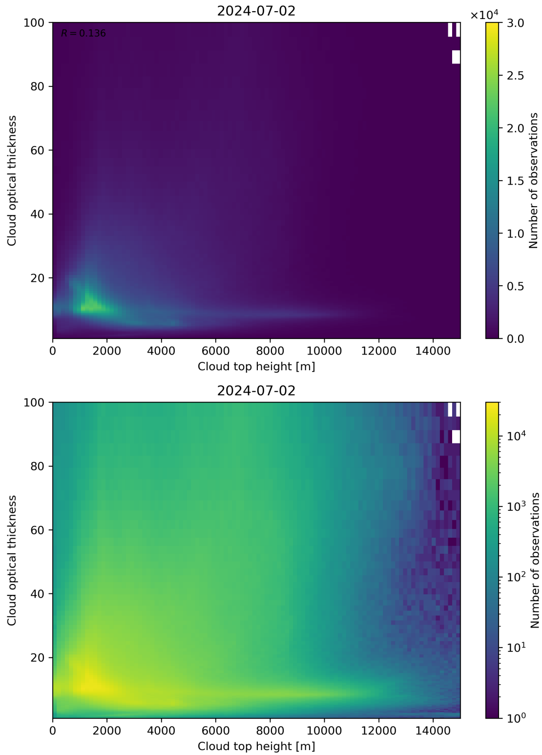
Figure 90: Scatter density plot of “Cloud top height” against “Cloud optical thickness” for 2024-07-01 to 2024-07-03.
