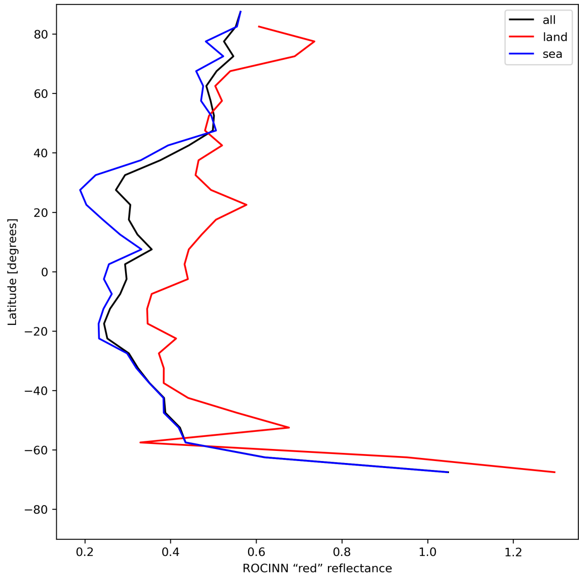
Figure 37: Zonal average of “ROCINN “red” reflectance” for 2024-07-01 to 2024-07-03.
