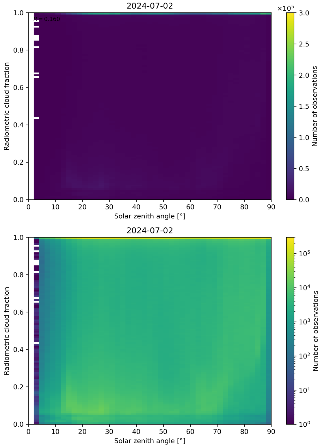
Figure 99: Scatter density plot of “Solar zenith angle” against “Radiometric cloud fraction” for 2024-07-01 to 2024-07-03.
