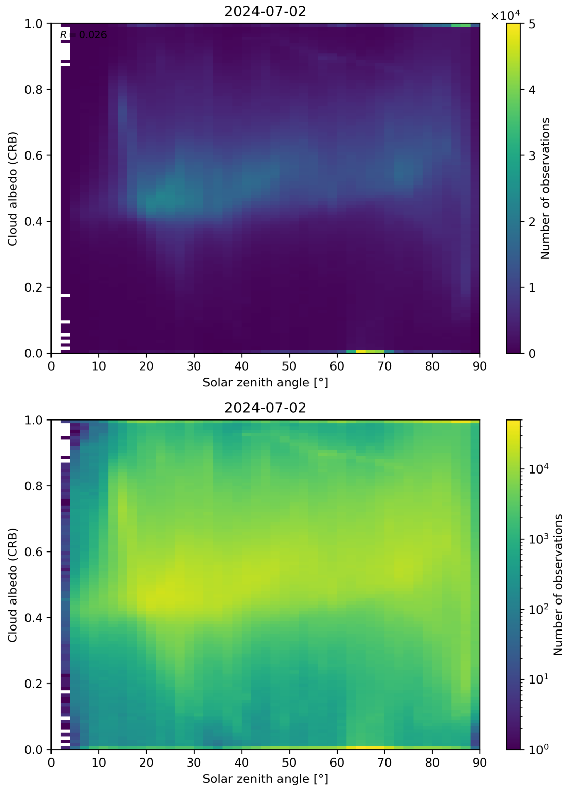
Figure 98: Scatter density plot of “Solar zenith angle” against “Cloud albedo (CRB)” for 2024-07-01 to 2024-07-03.
