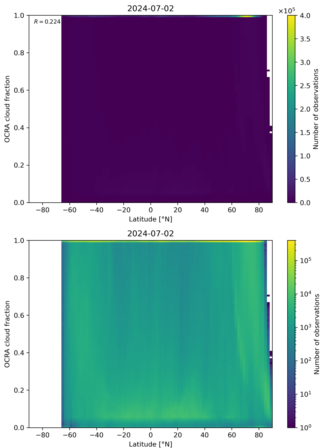
Figure 93: Scatter density plot of “Latitude” against “OCRA cloud fraction” for 2024-07-01 to 2024-07-03.
