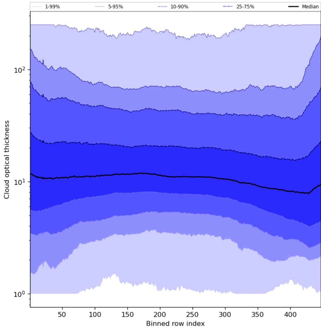
Figure 57: Along track statistics of “Cloud optical thickness” for 2024-07-01 to 2024-07-03
