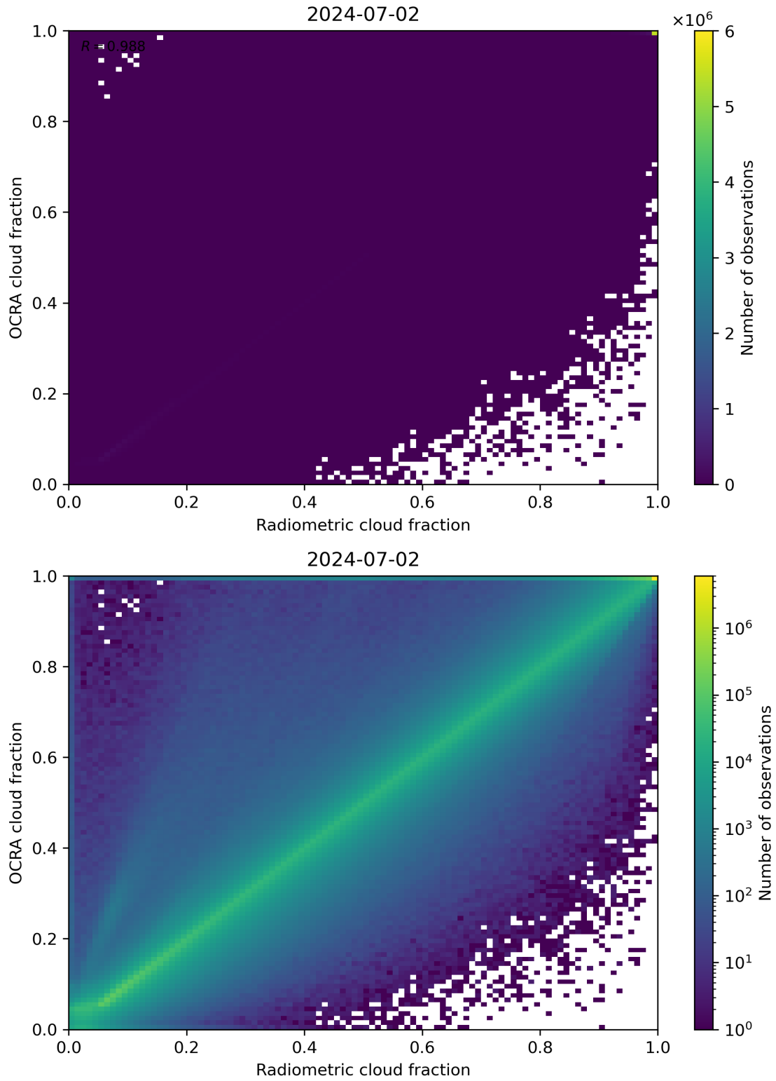
Figure 72: Scatter density plot of “Radiometric cloud fraction” against “OCRA cloud fraction” for 2024-07-01 to 2024-07-03.
