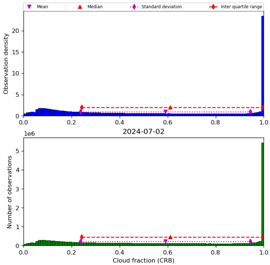
Figure 42: Histogram of “Cloud fraction (CRB)” for 2024-07-01 to 2024-07-03
