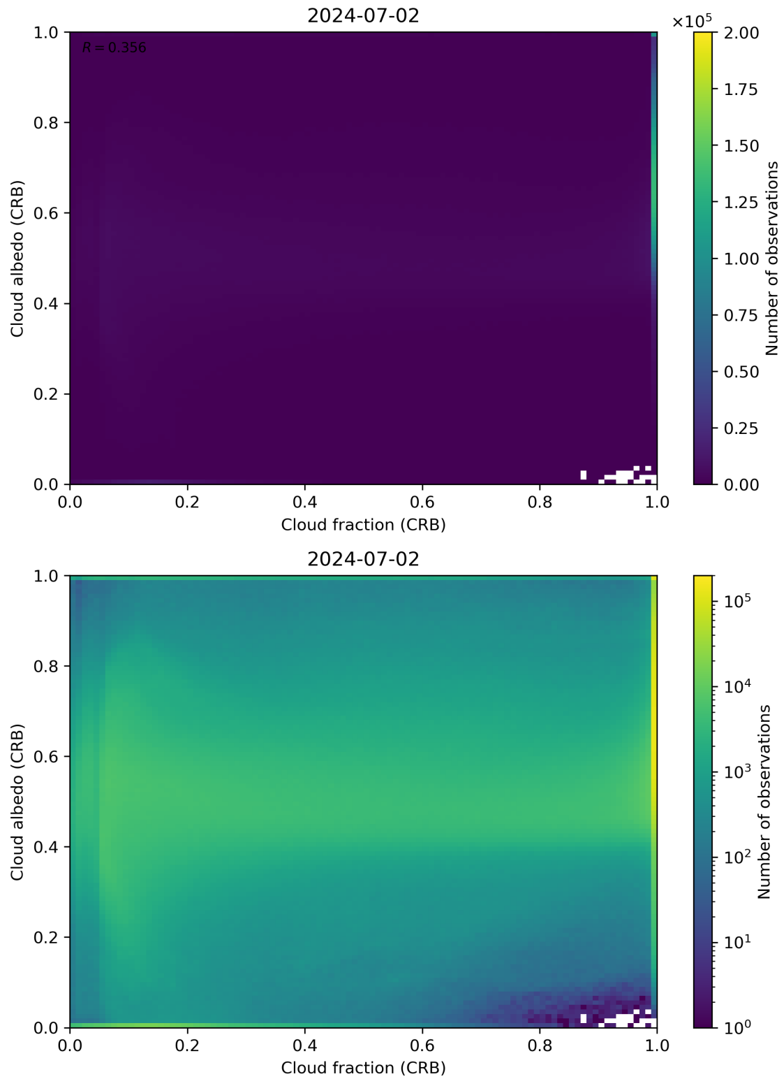
Figure 77: Scatter density plot of “Cloud fraction (CRB)” against “Cloud albedo (CRB)” for 2024-07-01 to 2024-07-03.
