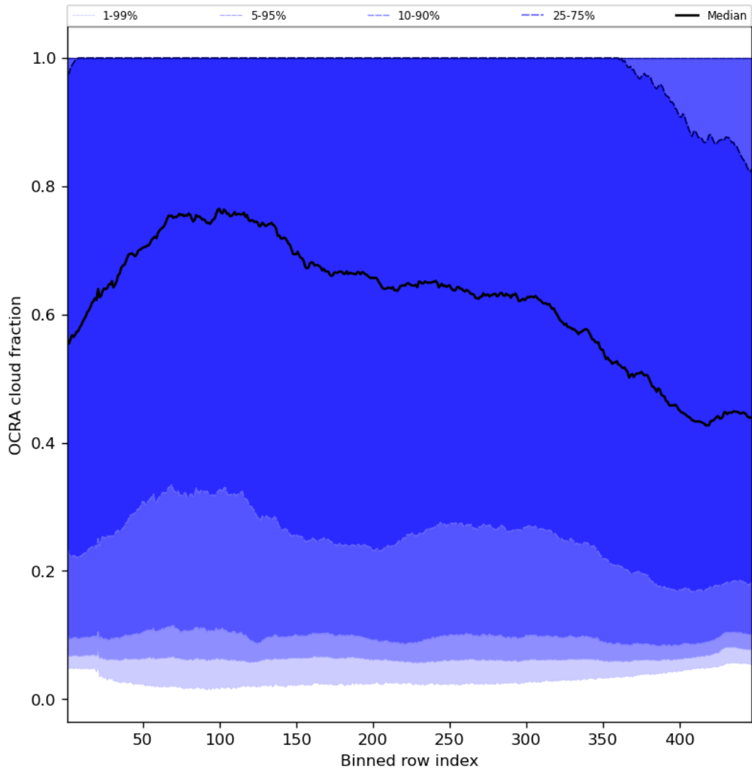
Figure 66: Along track statistics of “OCRA cloud fraction” for 2024-07-01 to 2024-07-03
