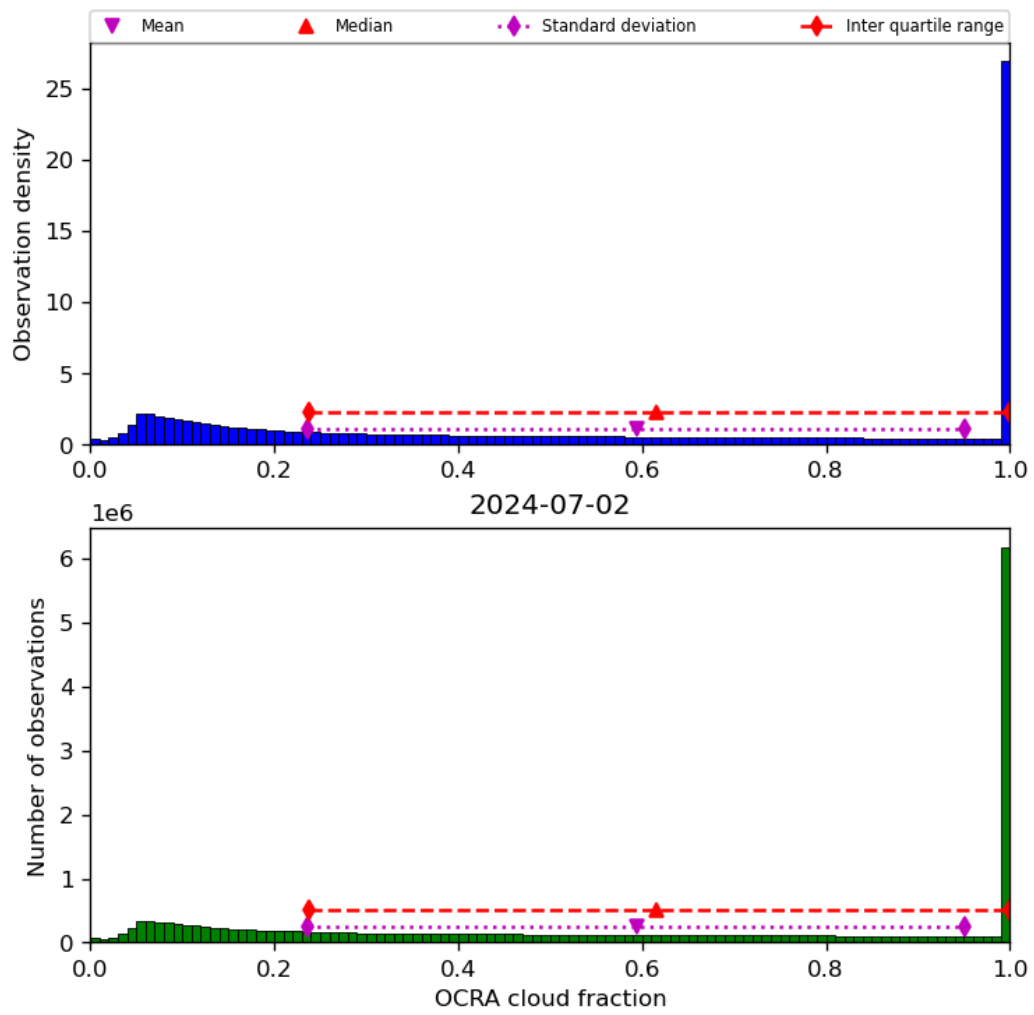
Figure 50: Histogram of “OCRA cloud fraction” for 2024-07-01 to 2024-07-03
