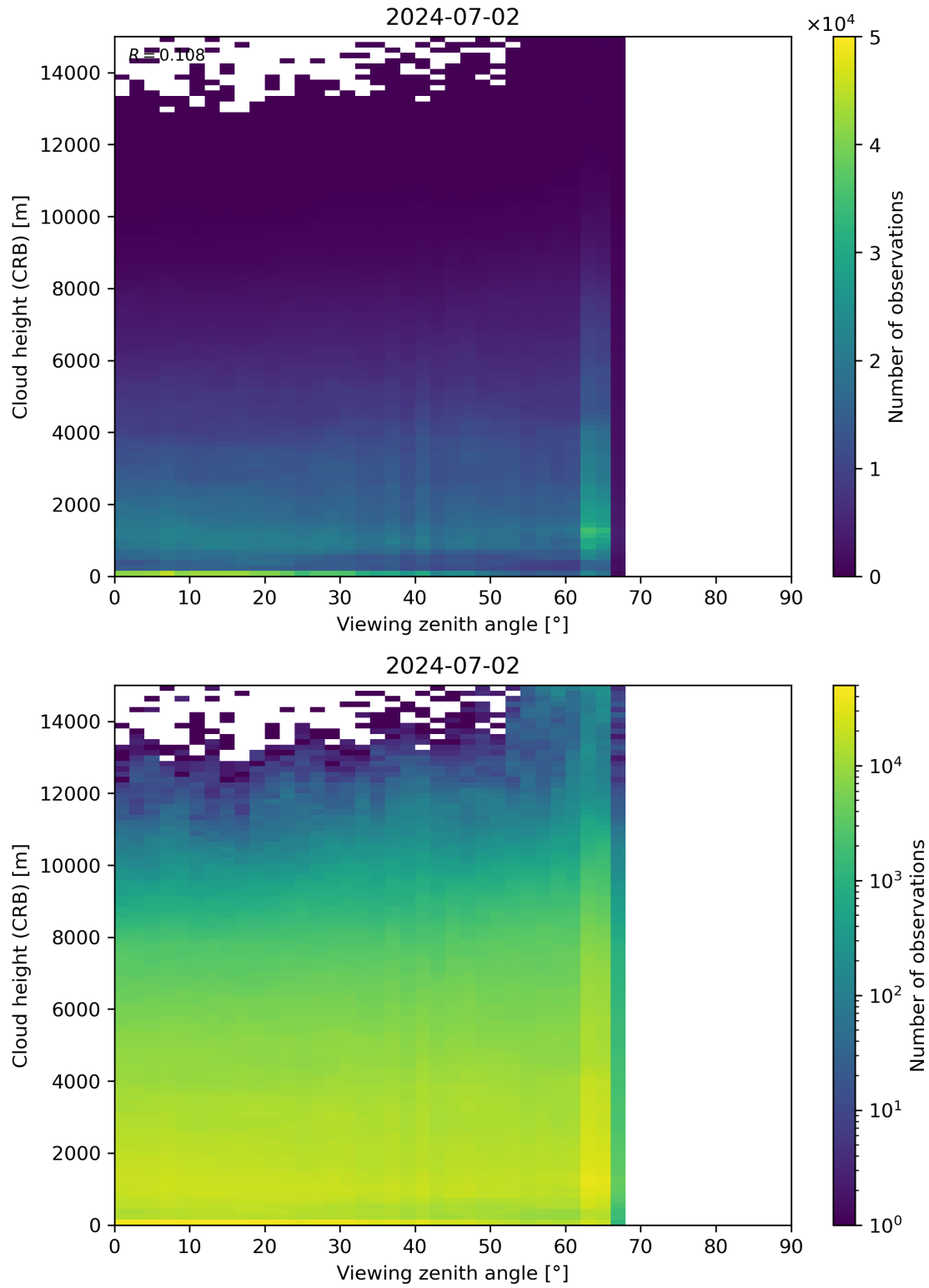
Figure 110: Scatter density plot of “Viewing zenith angle” against “Cloud height (CRB)” for 2024-07-01 to 2024-07-03.
