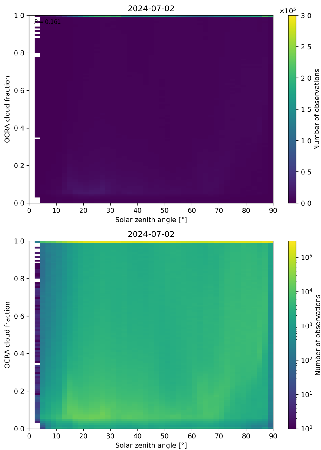
Figure 100: Scatter density plot of “Solar zenith angle” against “OCRA cloud fraction” for 2024-07-01 to 2024-07-03.
