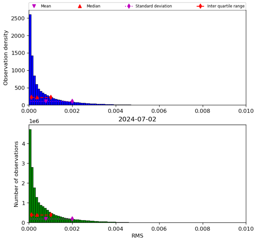
Figure 47: Histogram of “RMS” for 2024-07-01 to 2024-07-03
