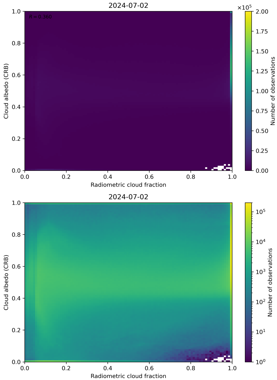
Figure 71: Scatter density plot of “Radiometric cloud fraction” against “Cloud albedo (CRB)” for 2024-07-01 to 2024-07-03.
