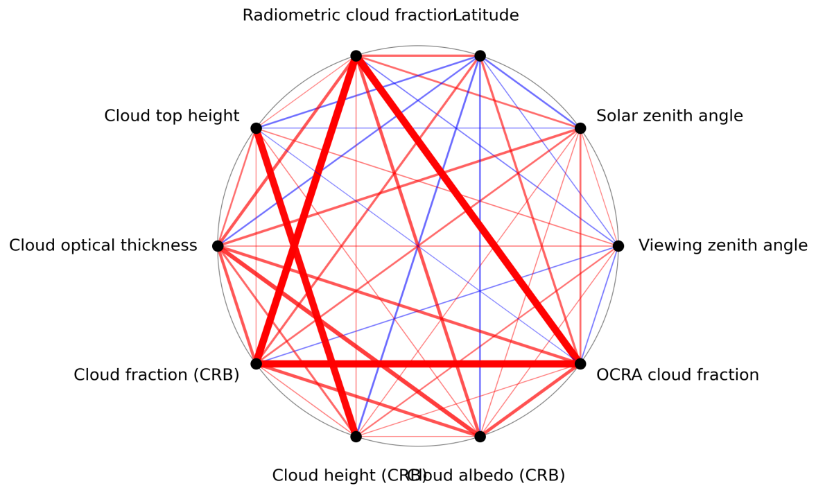
Figure 1: Map of correlation graph for 2024-07-01 to 2024-07-03.
