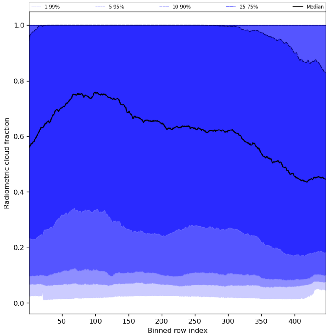
Figure 55: Along track statistics of “Radiometric cloud fraction” for 2024-07-01 to 2024-07-03
