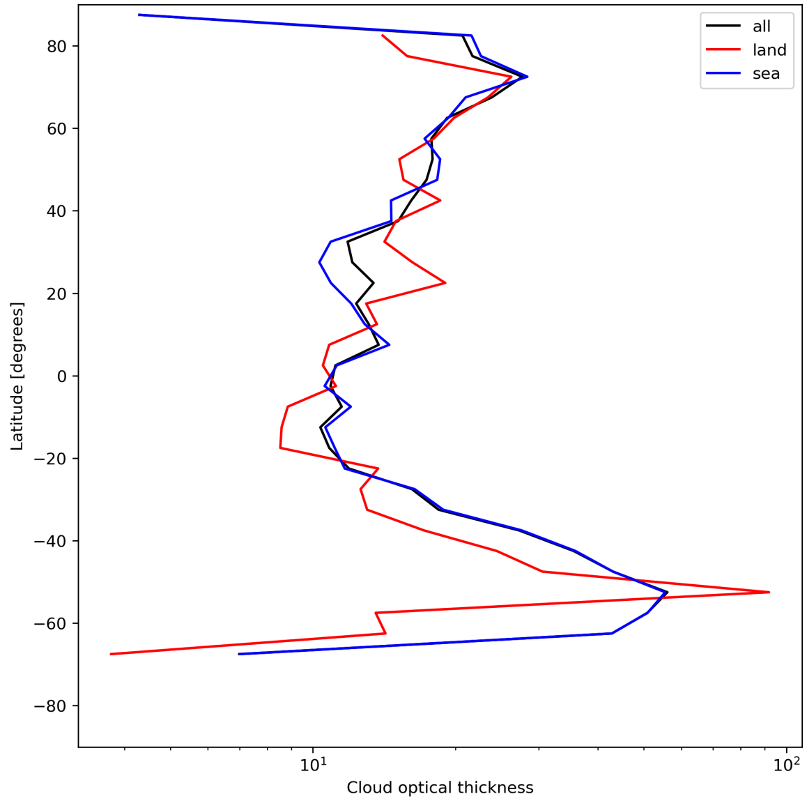
Figure 25: Zonal average of “Cloud optical thickness” for 2024-07-01 to 2024-07-03.
