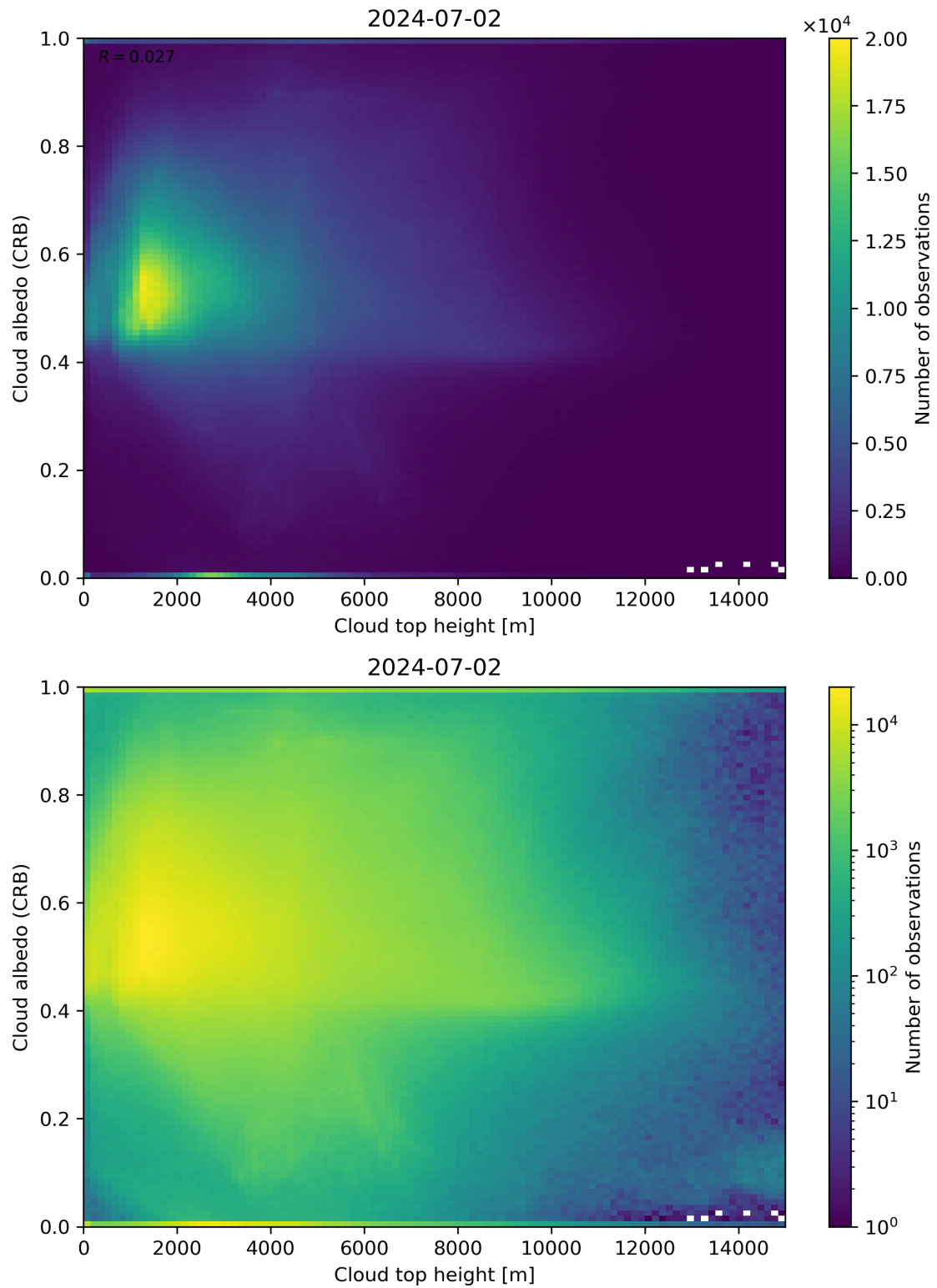
Figure 86: Scatter density plot of “Cloud top height” against “Cloud albedo (CRB)” for 2024-07-01 to 2024-07-03.
