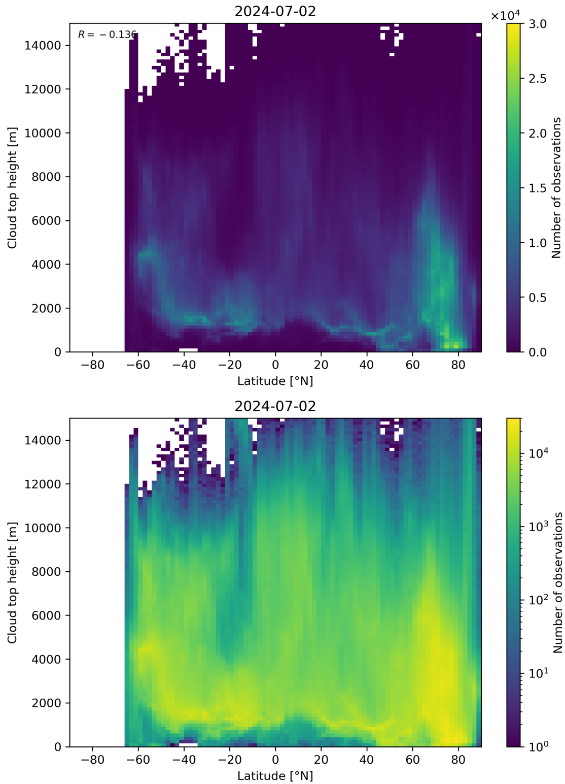
Figure 97: Scatter density plot of “Latitude” against “Cloud top height” for 2024-07-01 to 2024-07-03.
