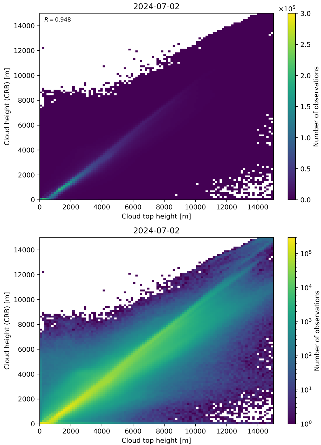
Figure 89: Scatter density plot of “Cloud top height” against “Cloud height (CRB)” for 2024-07-01 to 2024-07-03.
