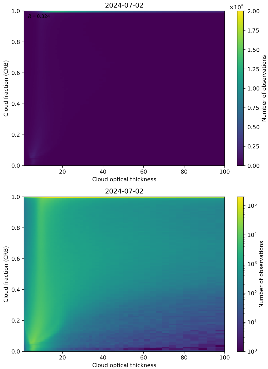
Figure 84: Scatter density plot of “Cloud optical thickness” against “Cloud fraction (CRB)” for 2024-07-01 to 2024-07-03.
