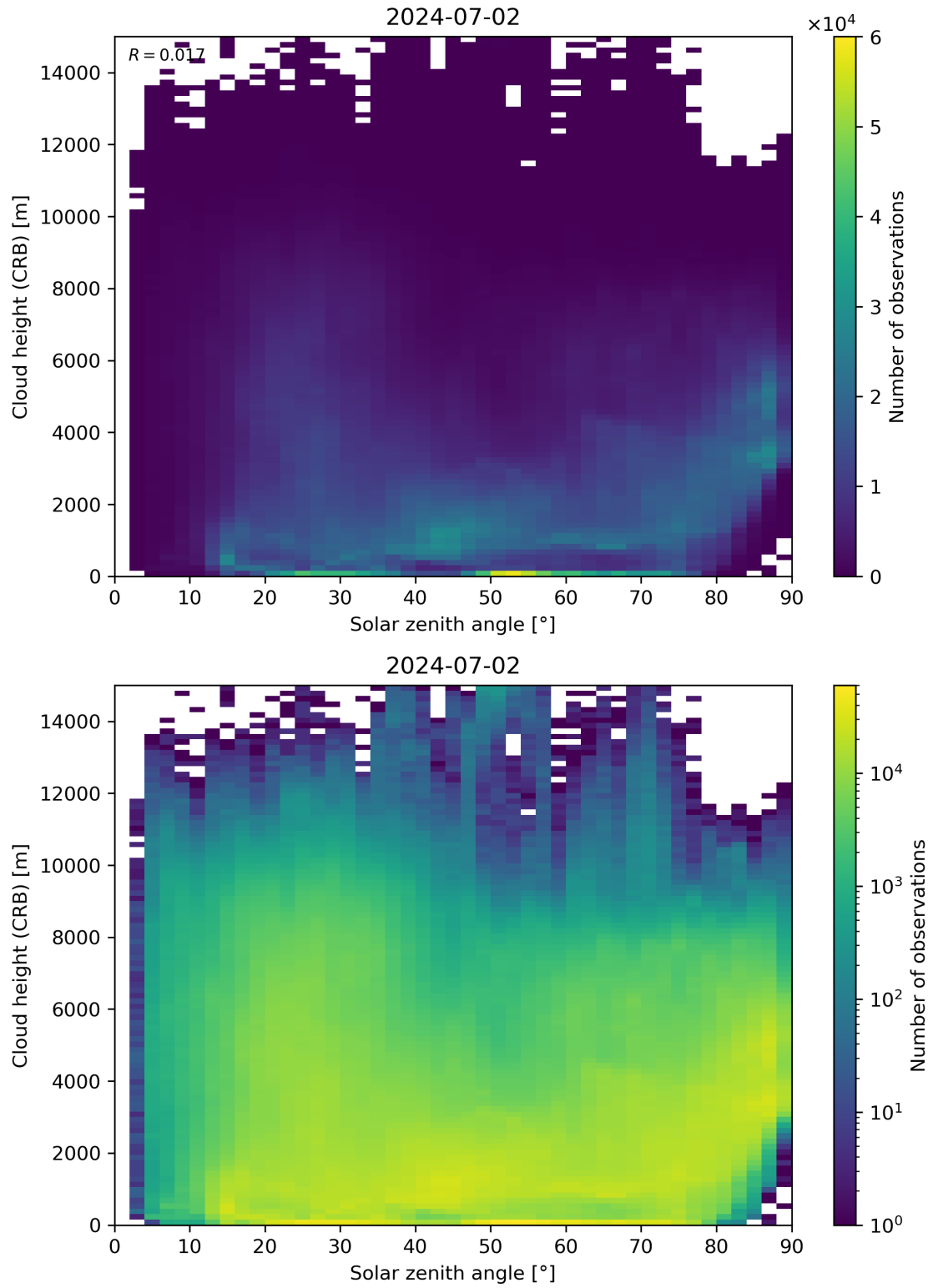
Figure 102: Scatter density plot of “Solar zenith angle” against “Cloud height (CRB)” for 2024-07-01 to 2024-07-03.
