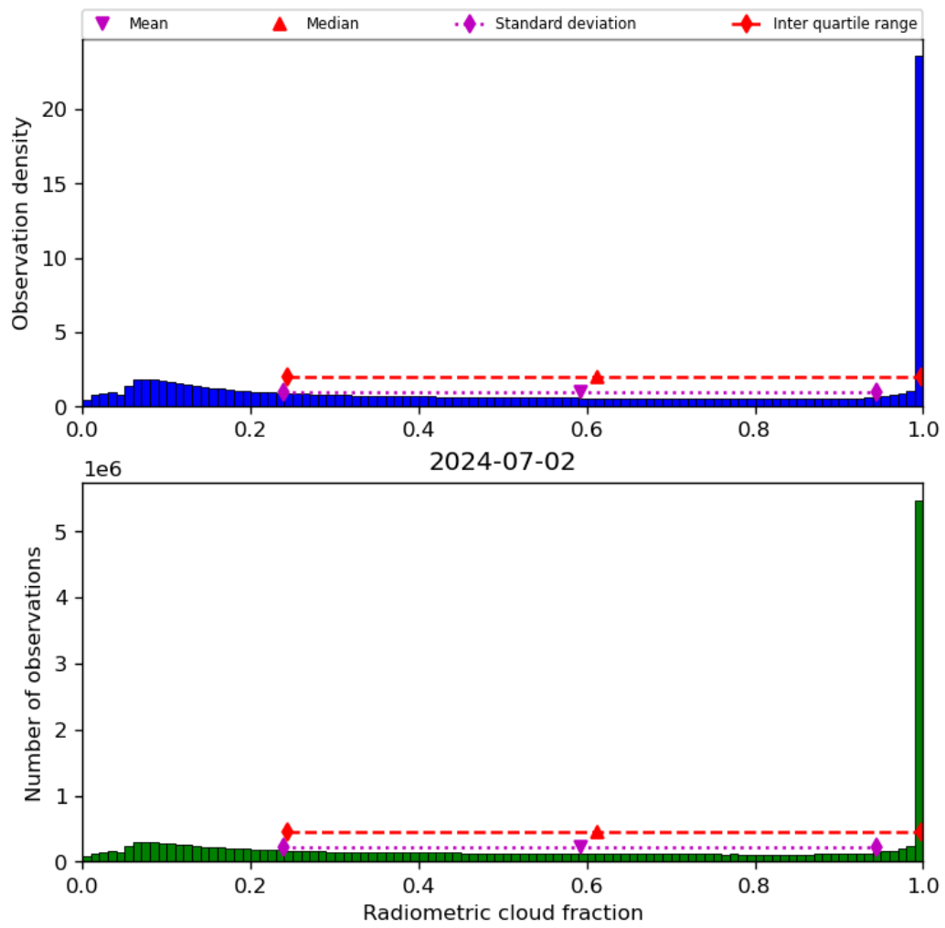
Figure 39: Histogram of “Radiometric cloud fraction” for 2024-07-01 to 2024-07-03
