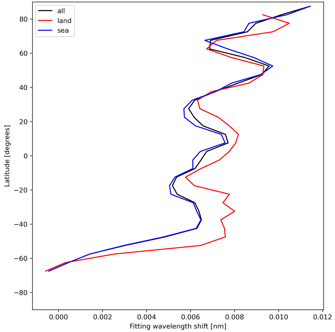
Figure 33: Zonal average of “Fitting wavelength shift” for 2024-07-01 to 2024-07-03.
