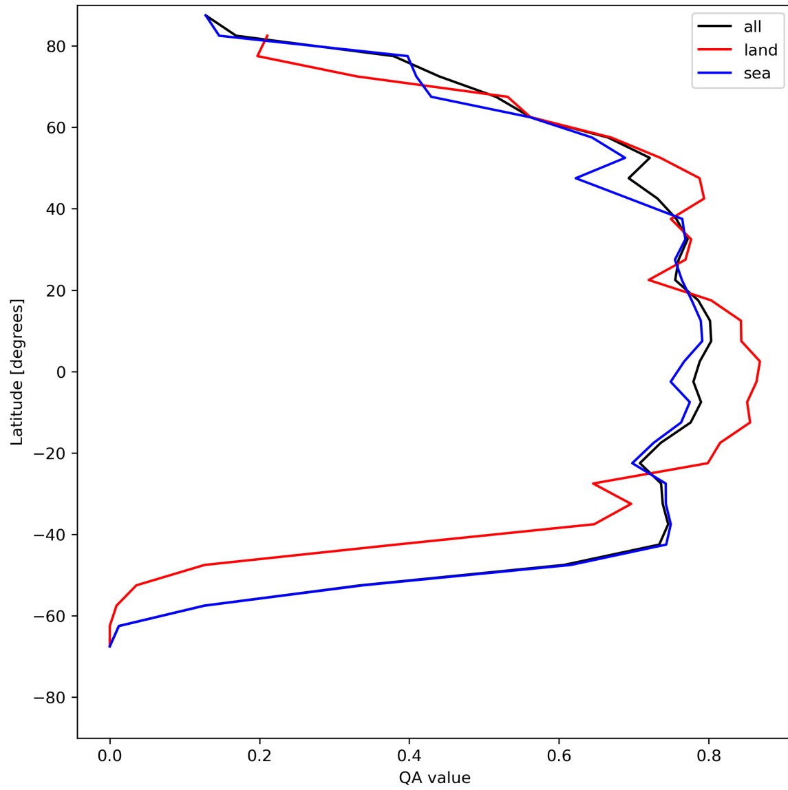
Figure 22: Zonal average of “QA value” for 2024-07-01 to 2024-07-03.
