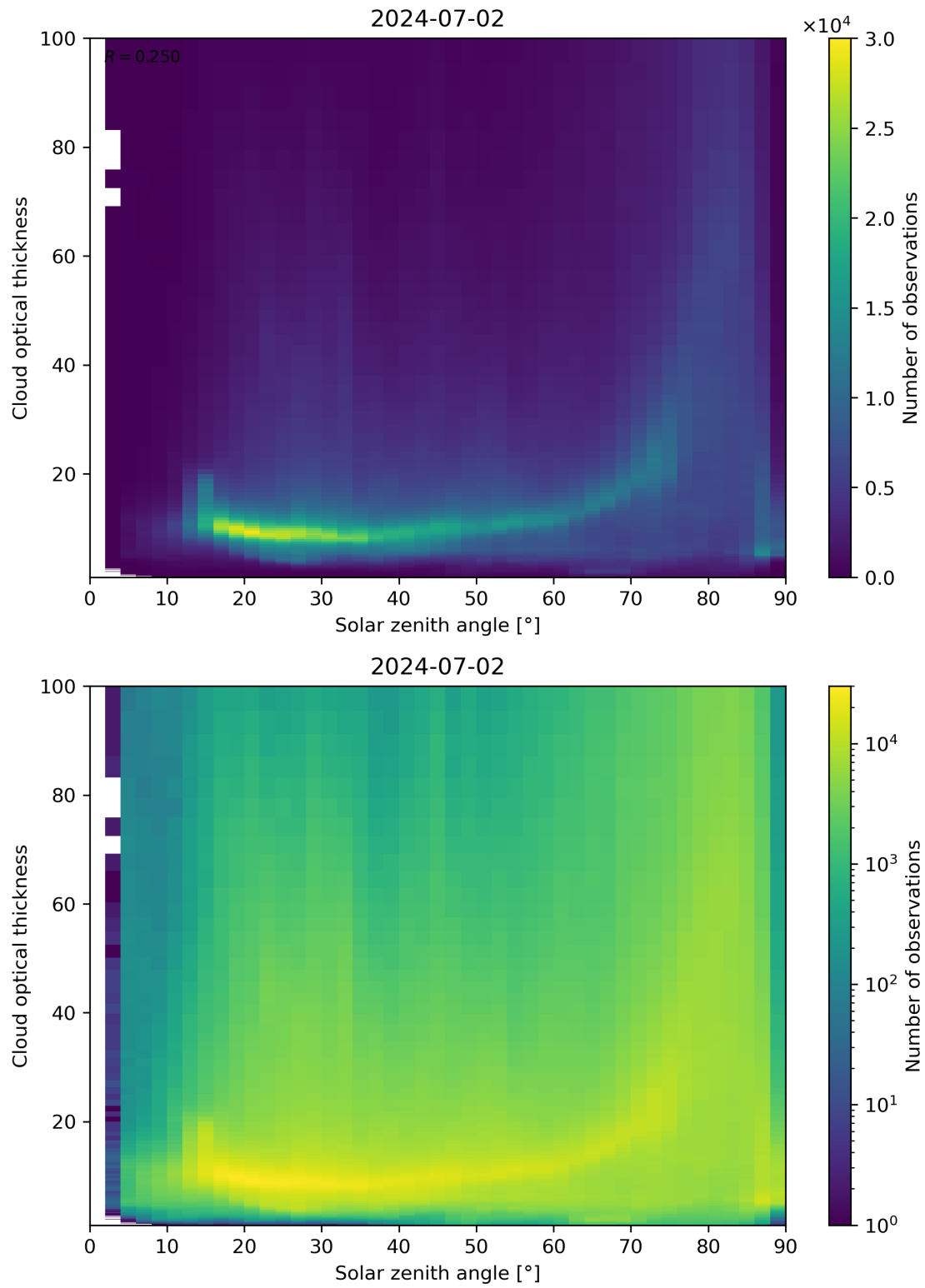
Figure 103: Scatter density plot of “Solar zenith angle” against “Cloud optical thickness” for 2024-07-01 to 2024-07-03.
