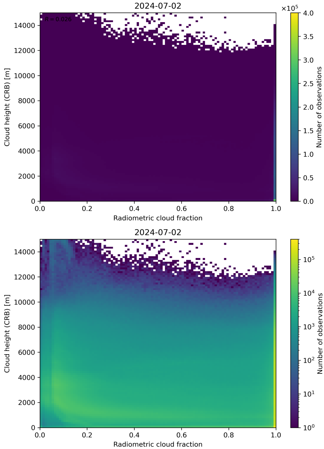
Figure 74: Scatter density plot of “Radiometric cloud fraction” against “Cloud height (CRB)” for 2024-07-01 to 2024-07-03.
