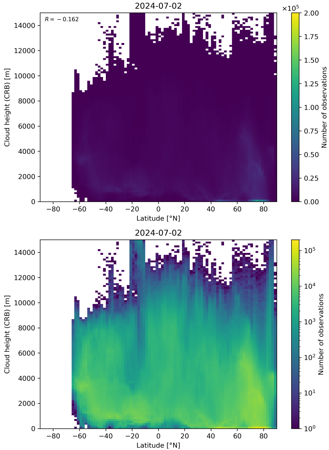
Figure 95: Scatter density plot of “Latitude” against “Cloud height (CRB)” for 2024-07-01 to 2024-07-03.
