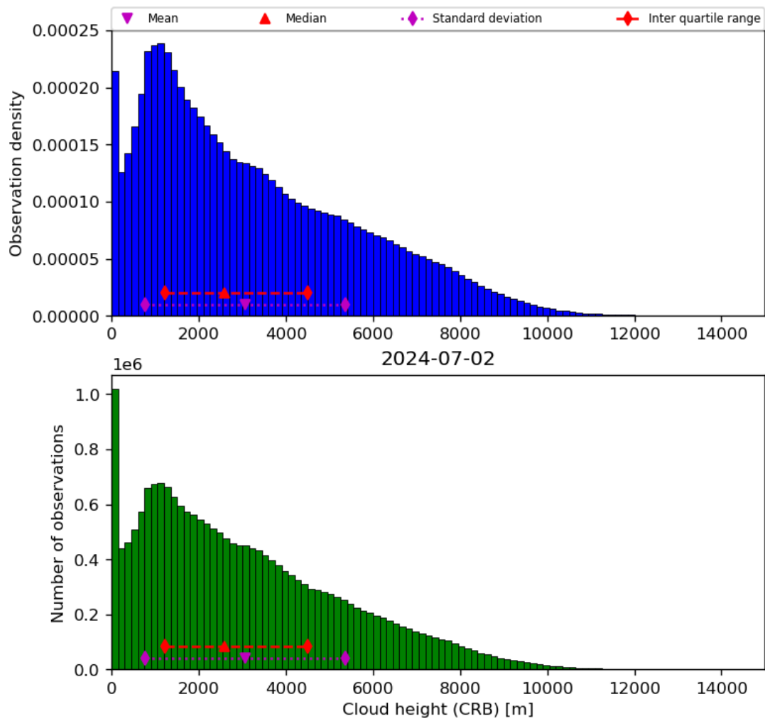
Figure 43: Histogram of “Cloud height (CRB)” for 2024-07-01 to 2024-07-03
