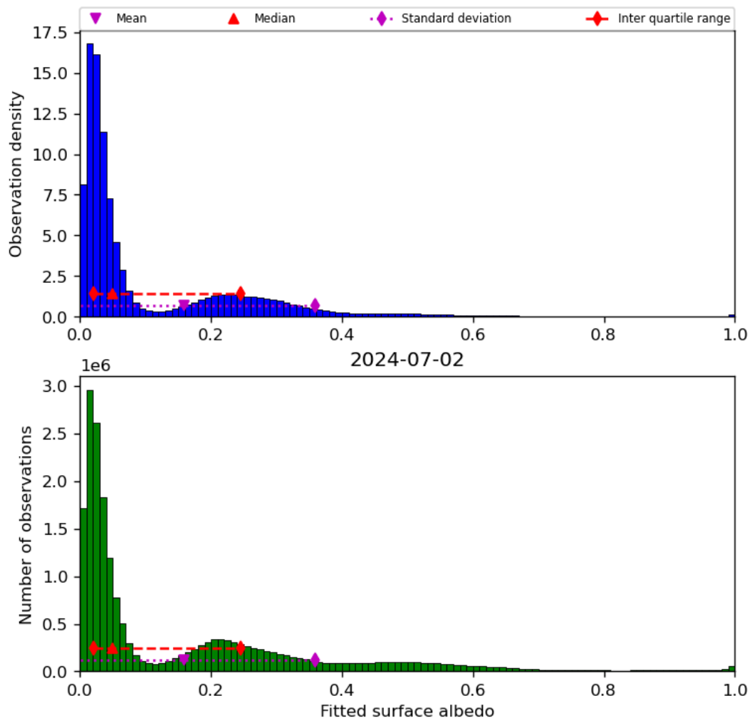
Figure 45: Histogram of “Fitted surface albedo” for 2024-07-01 to 2024-07-03
