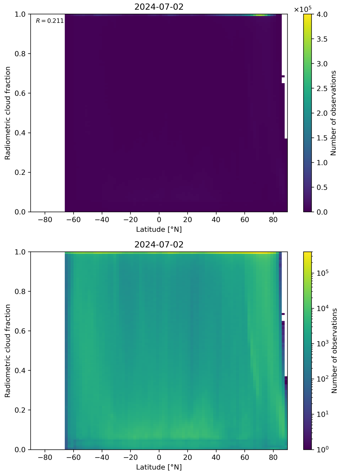
Figure 92: Scatter density plot of “Latitude” against “Radiometric cloud fraction” for 2024-07-01 to 2024-07-03.
