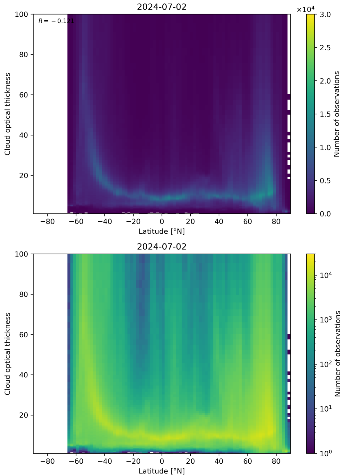
Figure 96: Scatter density plot of “Latitude” against “Cloud optical thickness” for 2024-07-01 to 2024-07-03.
