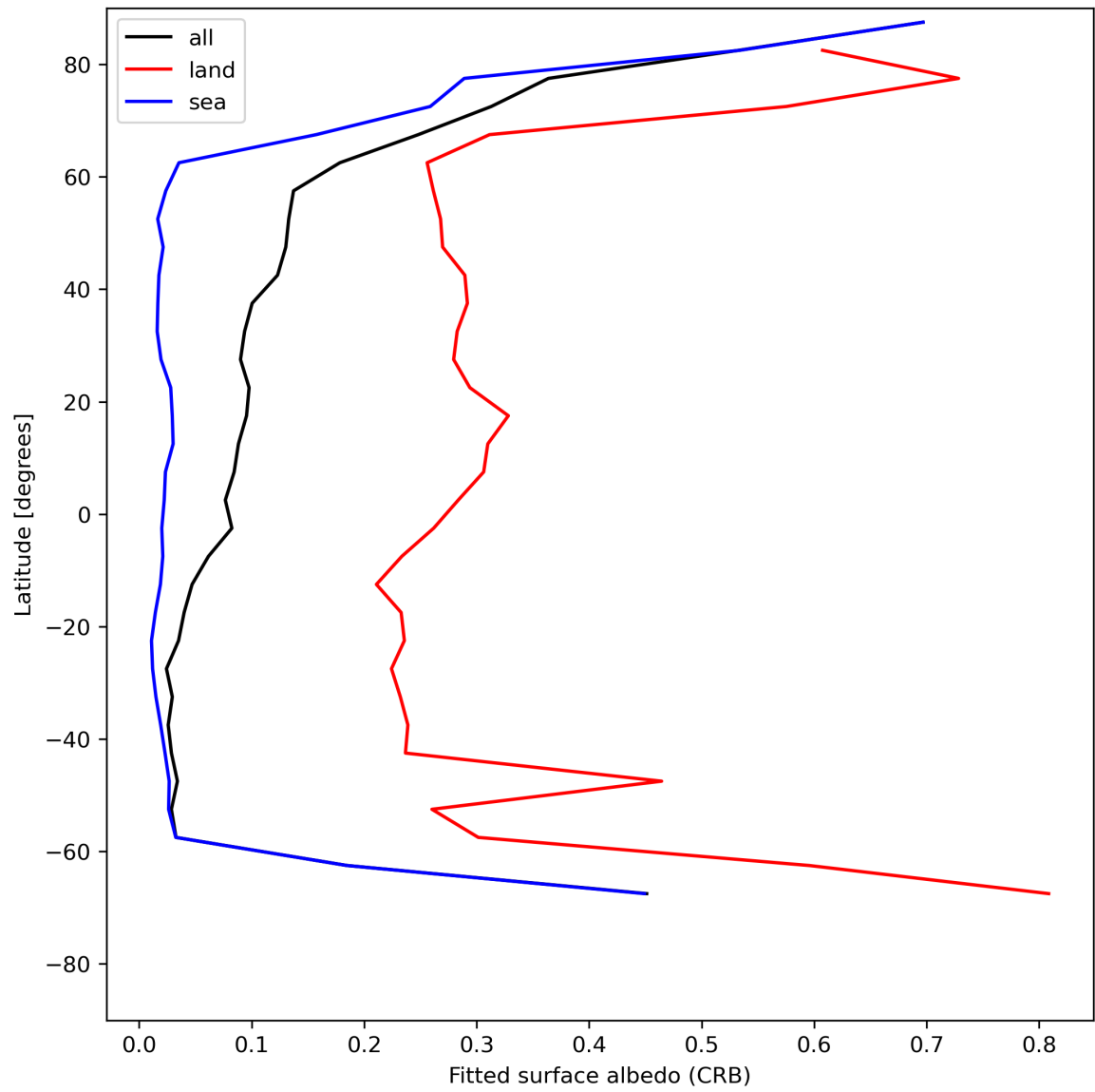
Figure 30: Zonal average of “Fitted surface albedo (CRB)” for 2024-07-01 to 2024-07-03.
