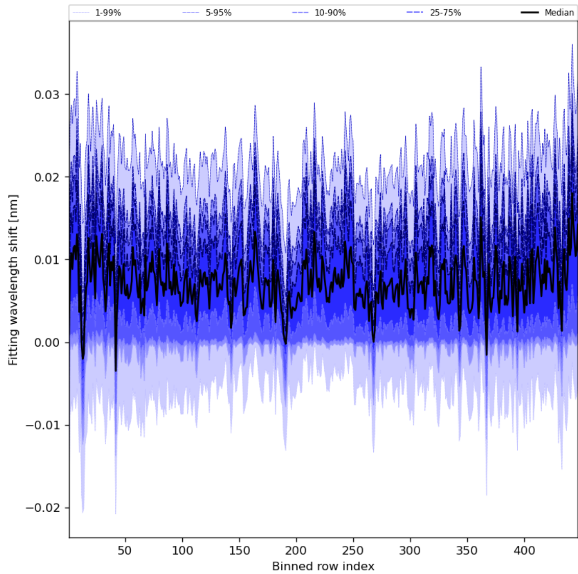
Figure 65: Along track statistics of “Fitting wavelength shift” for 2024-07-01 to 2024-07-03
