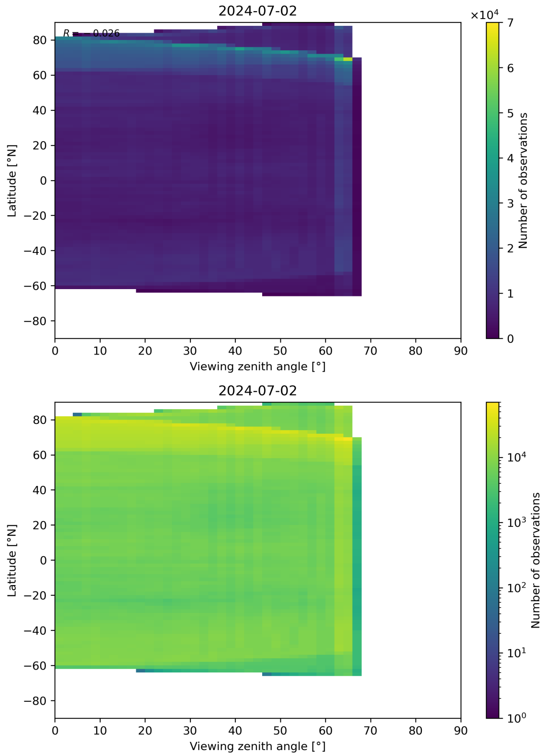
Figure 113: Scatter density plot of “Viewing zenith angle” against “Latitude” for 2024-07-01 to 2024-07-03.
