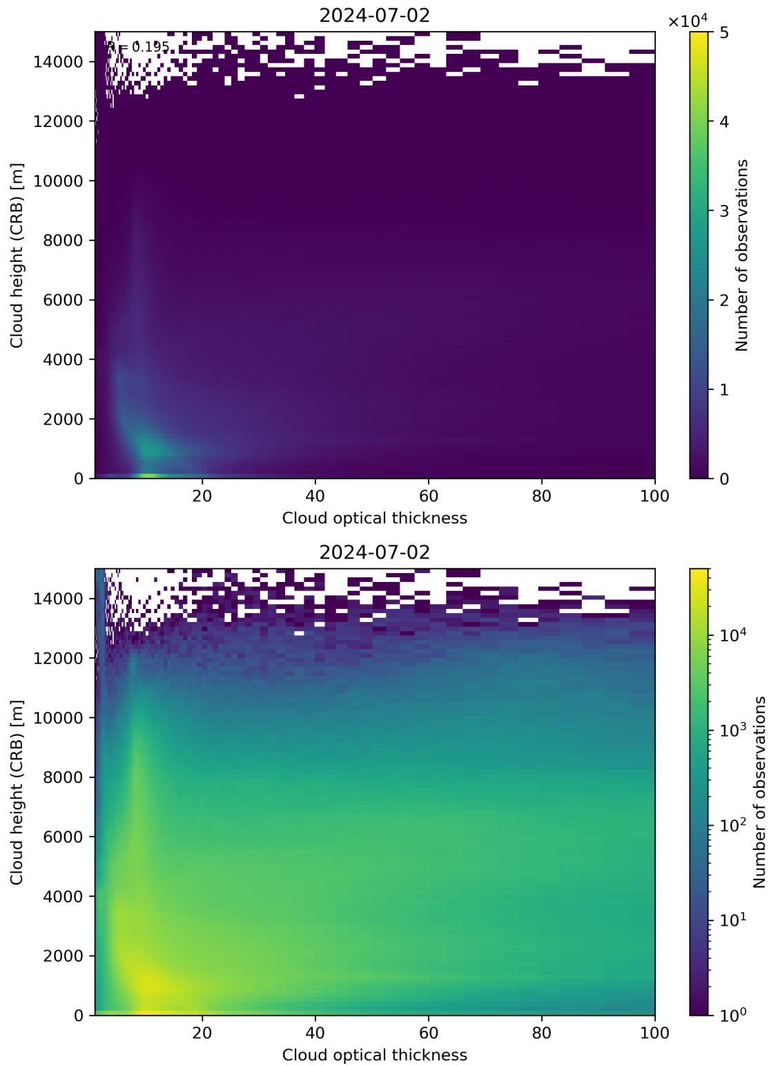
Figure 85: Scatter density plot of “Cloud optical thickness” against “Cloud height (CRB)” for 2024-07-01 to 2024-07-03.
