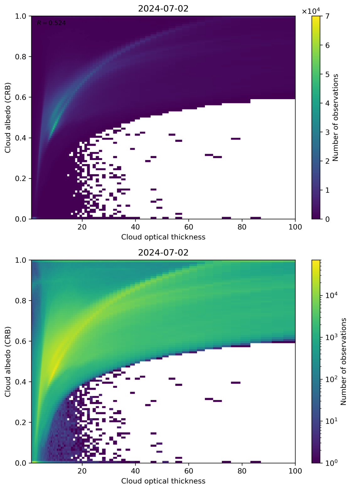
Figure 82: Scatter density plot of “Cloud optical thickness” against “Cloud albedo (CRB)” for 2024-07-01 to 2024-07-03.
