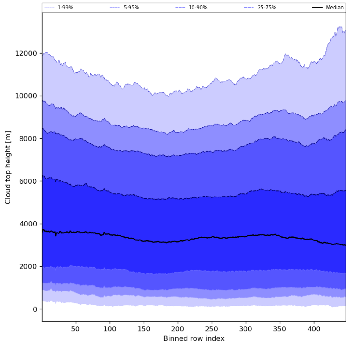
Figure 56: Along track statistics of “Cloud top height” for 2024-07-01 to 2024-07-03
