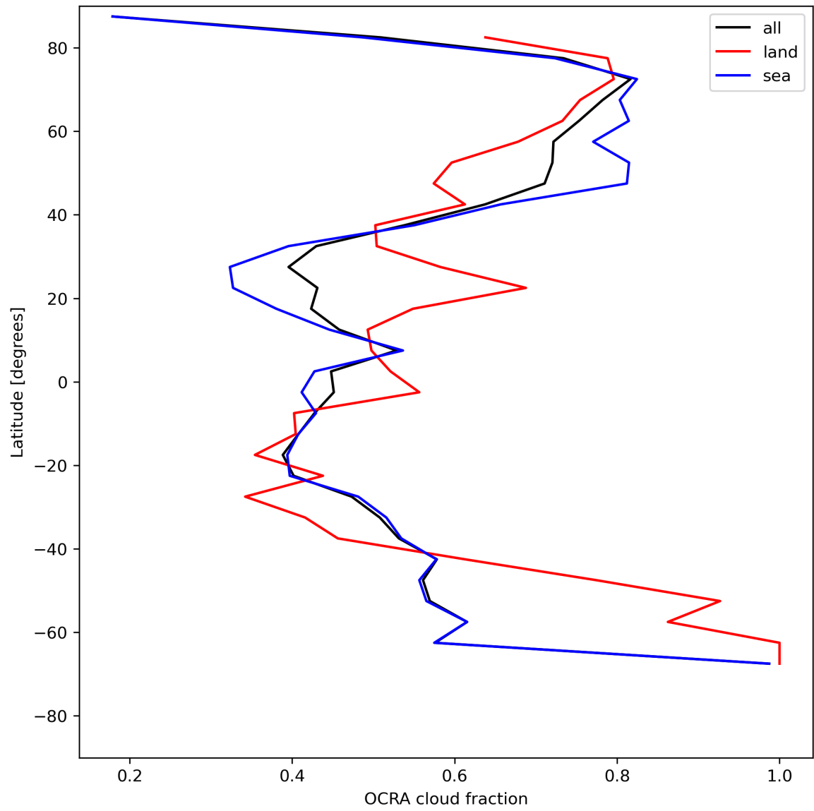
Figure 34: Zonal average of “OCRA cloud fraction” for 2024-07-01 to 2024-07-03.
