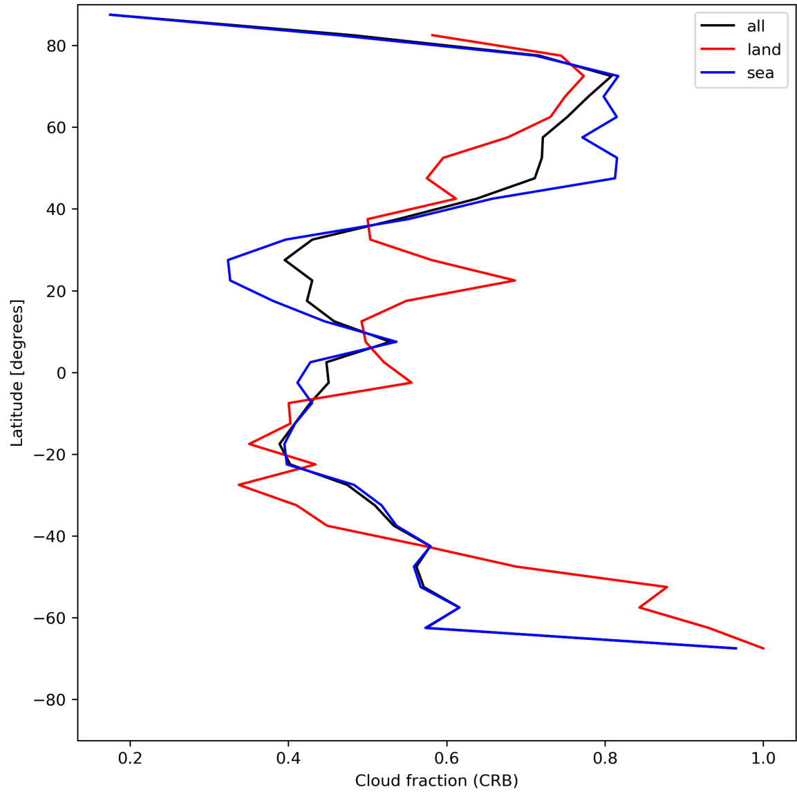
Figure 26: Zonal average of “Cloud fraction (CRB)” for 2024-07-01 to 2024-07-03.
