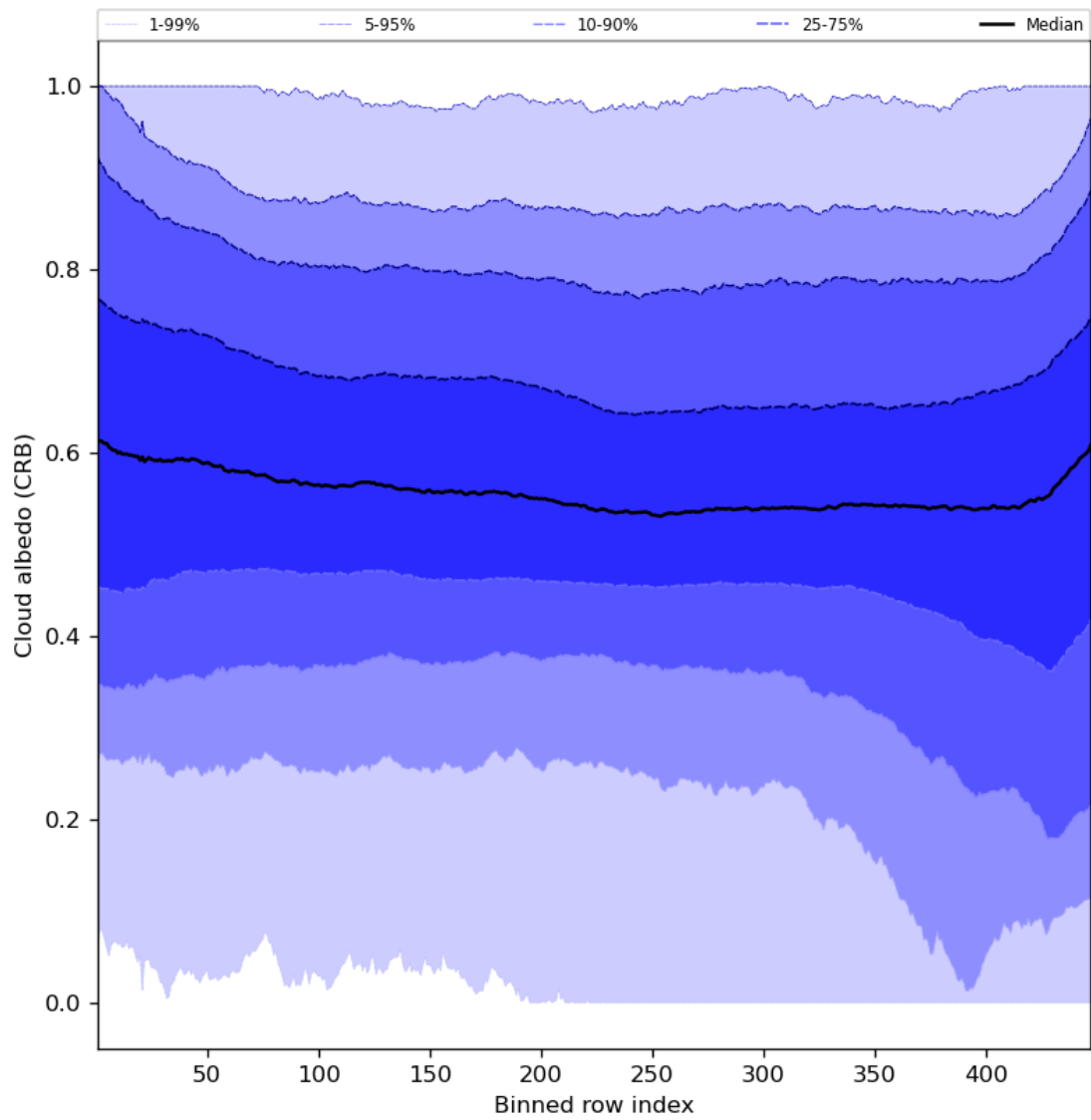
Figure 60: Along track statistics of “Cloud albedo (CRB)” for 2024-07-01 to 2024-07-03
