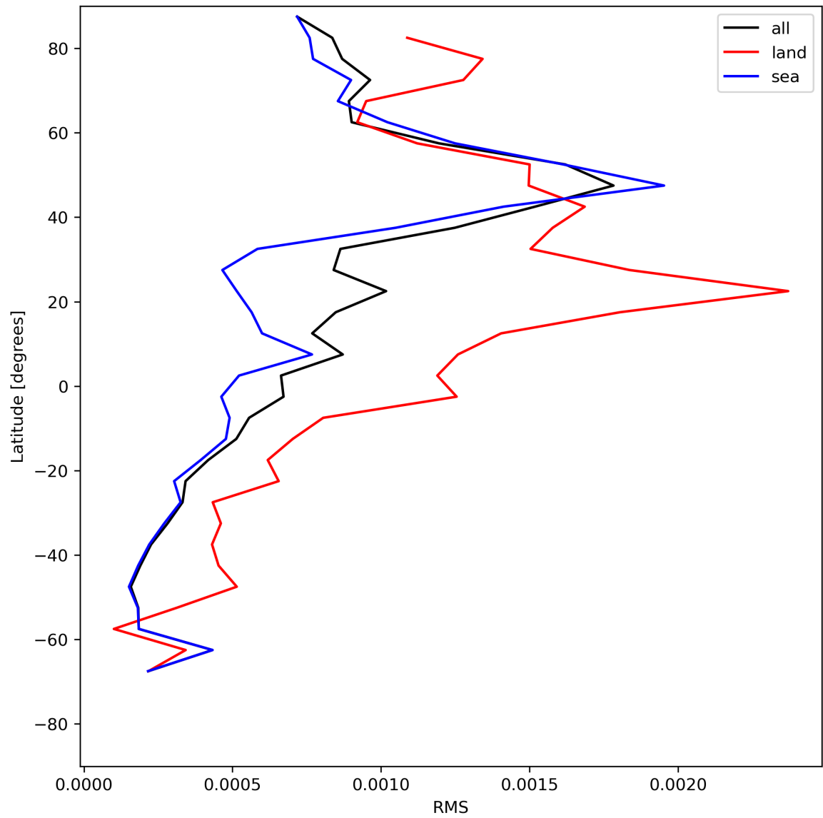
Figure 31: Zonal average of “RMS” for 2024-07-01 to 2024-07-03.
