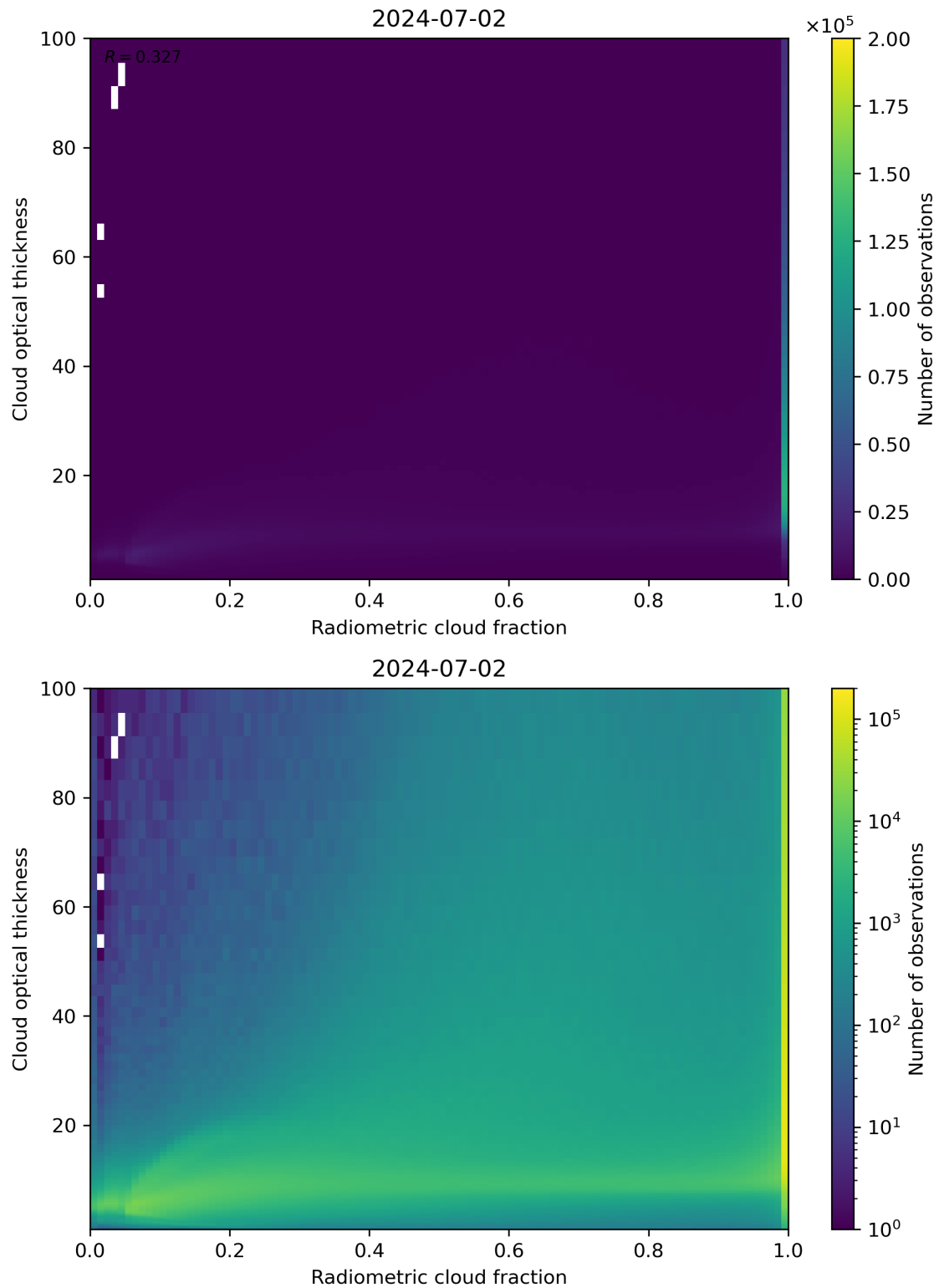
Figure 75: Scatter density plot of “Radiometric cloud fraction” against “Cloud optical thickness” for 2024-07-01 to 2024-07-03.
