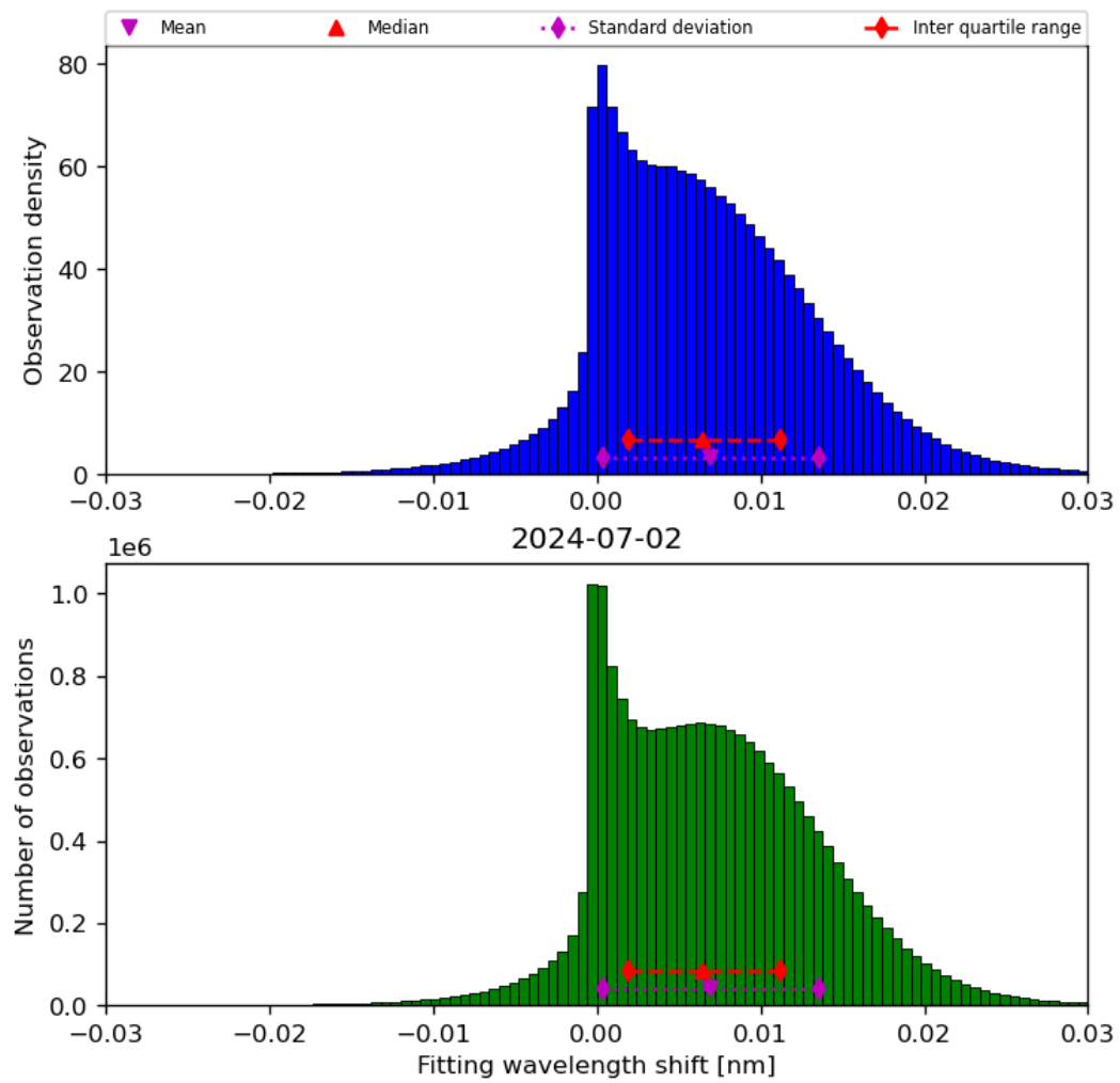
Figure 49: Histogram of “Fitting wavelength shift” for 2024-07-01 to 2024-07-03
