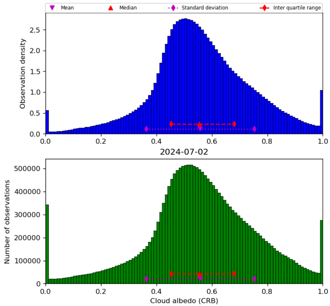
Figure 44: Histogram of “Cloud albedo (CRB)” for 2024-07-01 to 2024-07-03
