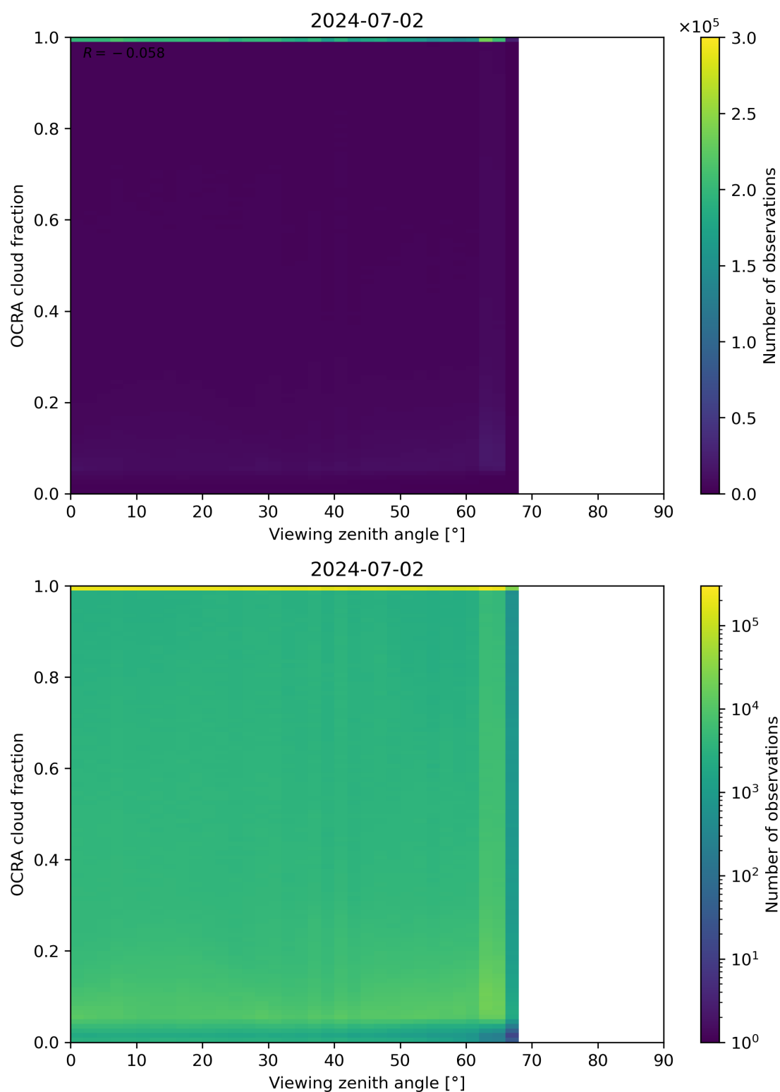
Figure 108: Scatter density plot of “Viewing zenith angle” against “OCRA cloud fraction” for 2024-07-01 to 2024-07-03.
