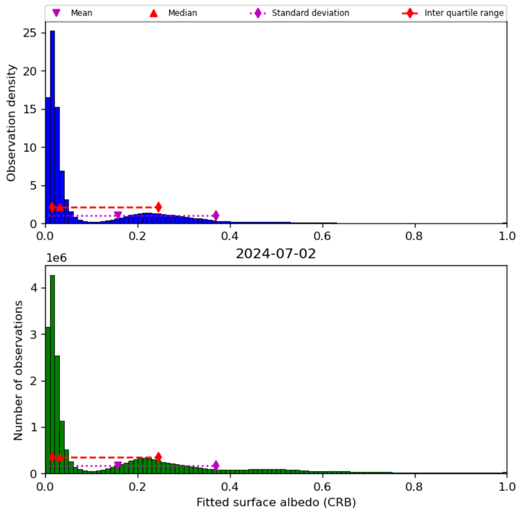
Figure 46: Histogram of “Fitted surface albedo (CRB)” for 2024-07-01 to 2024-07-03
