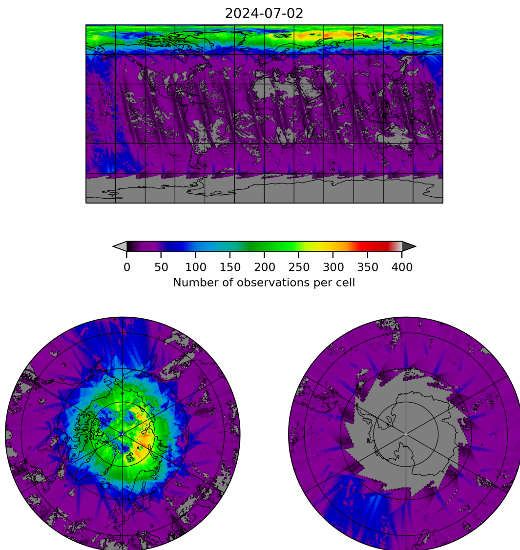
Figure 21: Map of the number of observations for 2024-07-01 to 2024-07-03
