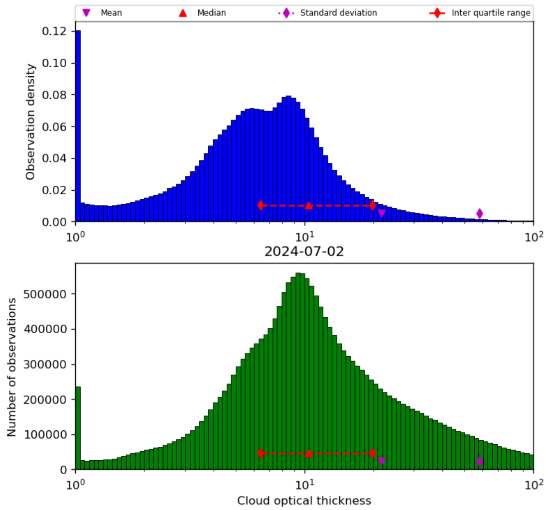
Figure 41: Histogram of “Cloud optical thickness” for 2024-07-01 to 2024-07-03
