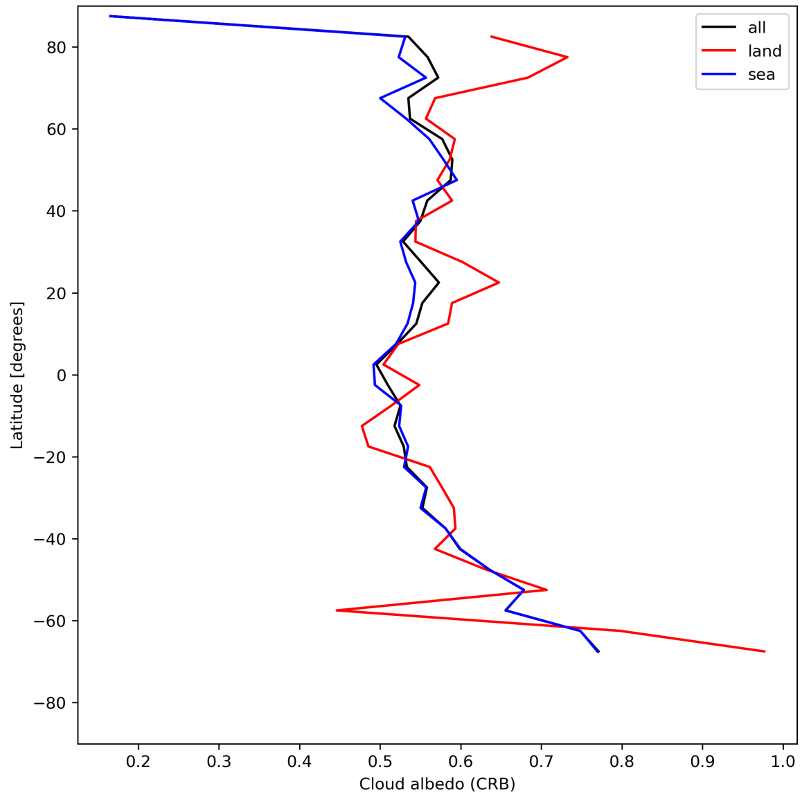
Figure 28: Zonal average of “Cloud albedo (CRB)” for 2024-07-01 to 2024-07-03.
