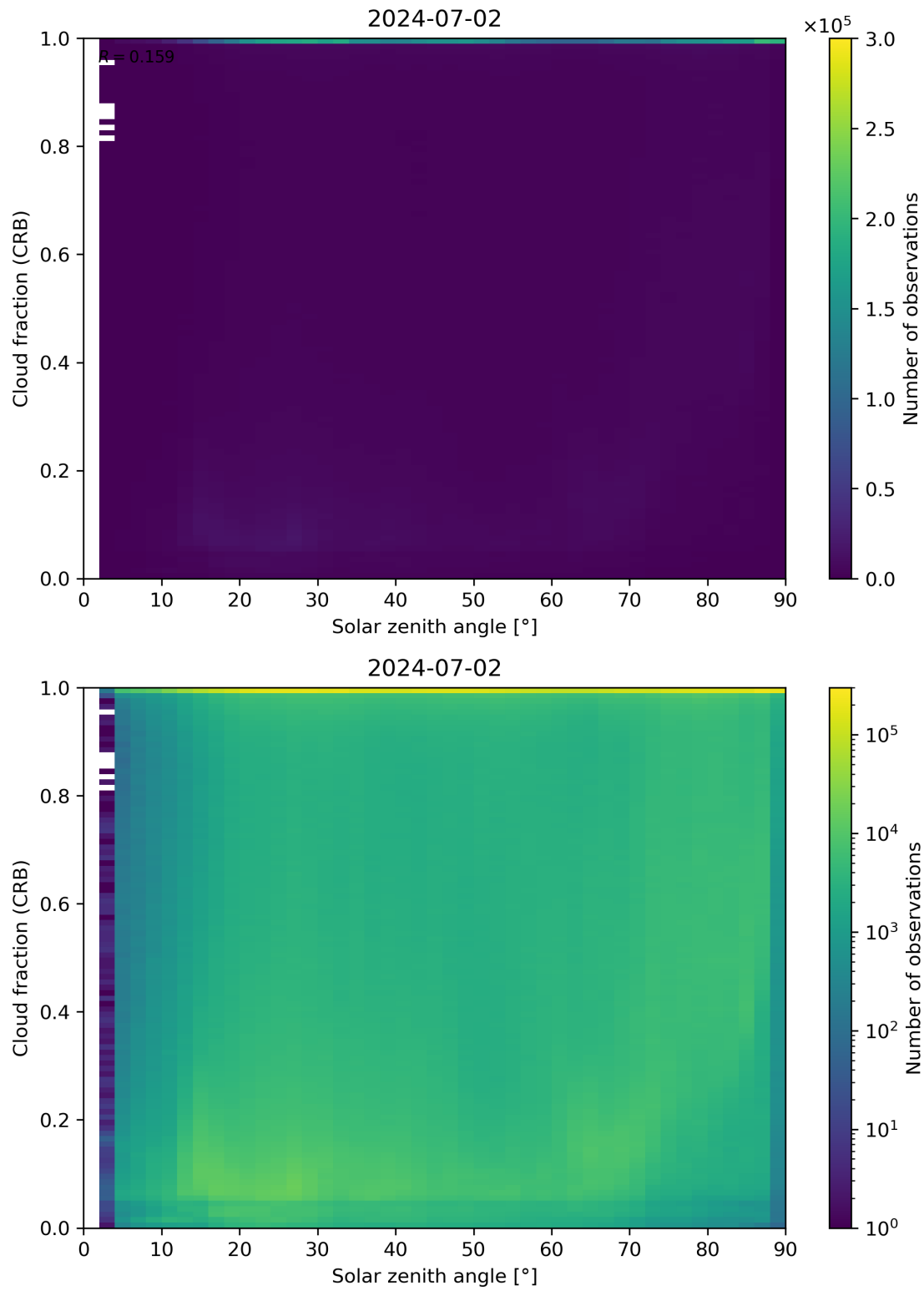
Figure 101: Scatter density plot of “Solar zenith angle” against “Cloud fraction (CRB)” for 2024-07-01 to 2024-07-03.
