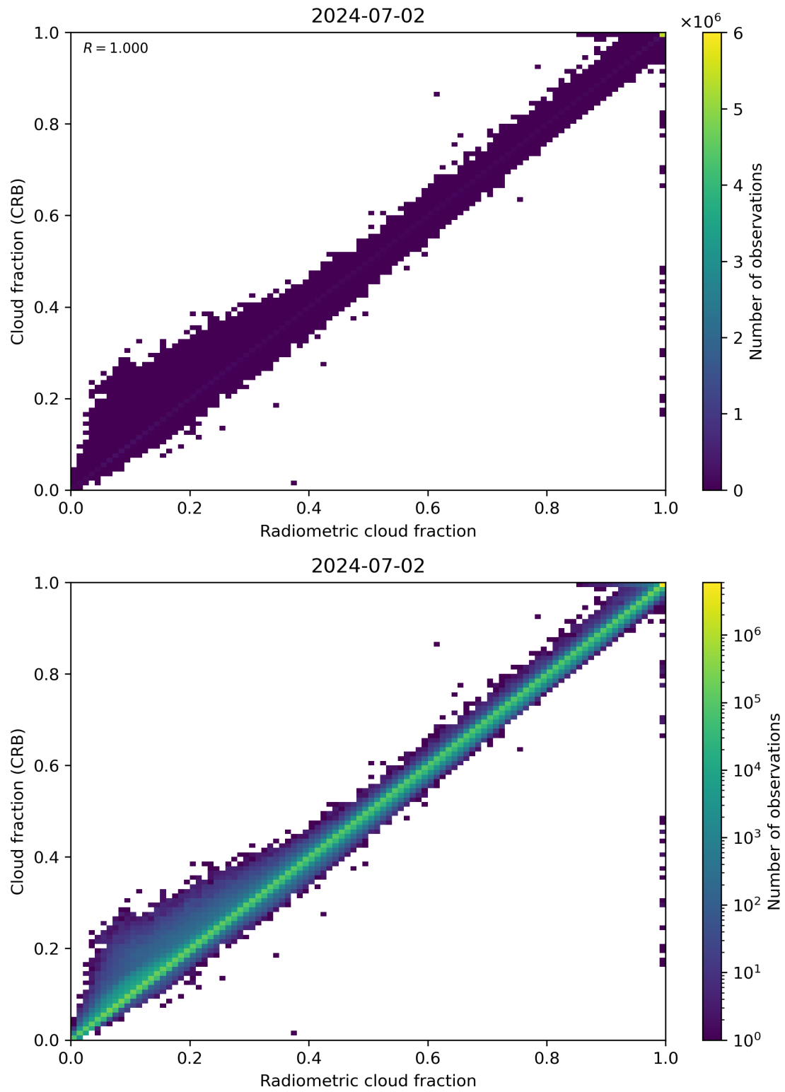
Figure 73: Scatter density plot of “Radiometric cloud fraction” against “Cloud fraction (CRB)” for 2024-07-01 to 2024-07-03.
