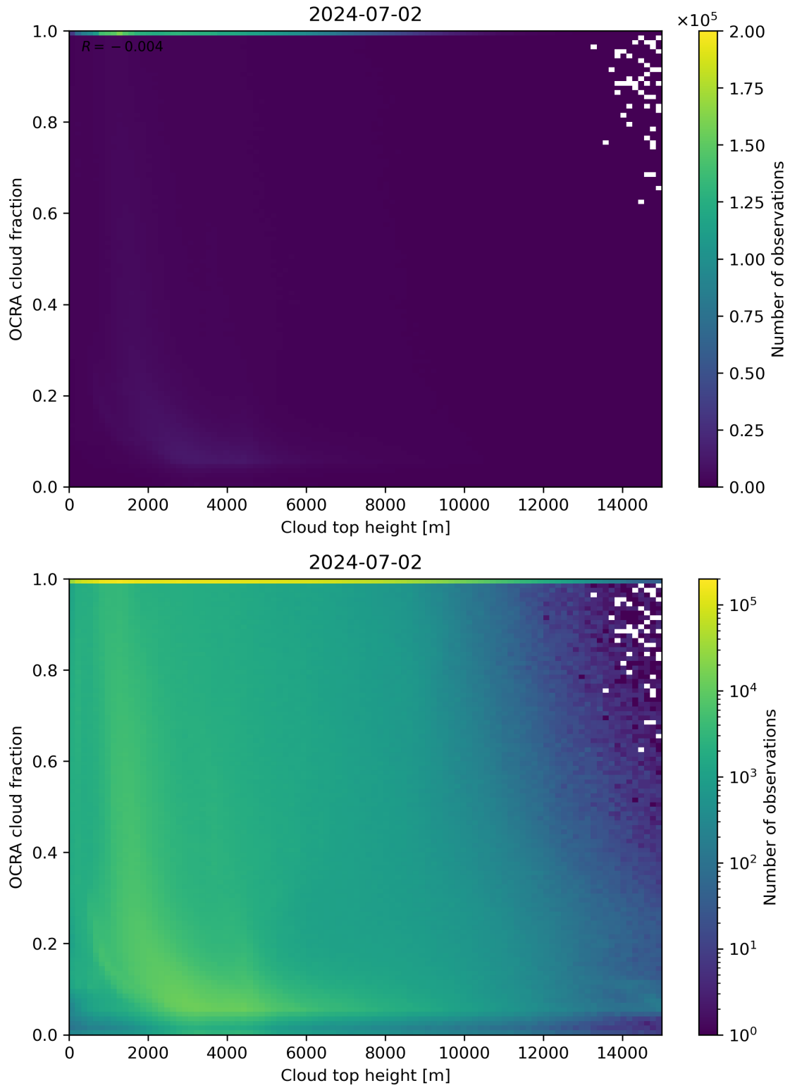
Figure 87: Scatter density plot of “Cloud top height” against “OCRA cloud fraction” for 2024-07-01 to 2024-07-03.
