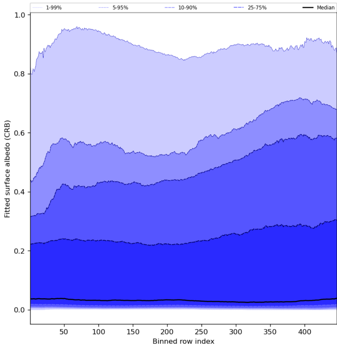
Figure 62: Along track statistics of “Fitted surface albedo (CRB)” for 2024-07-01 to 2024-07-03
