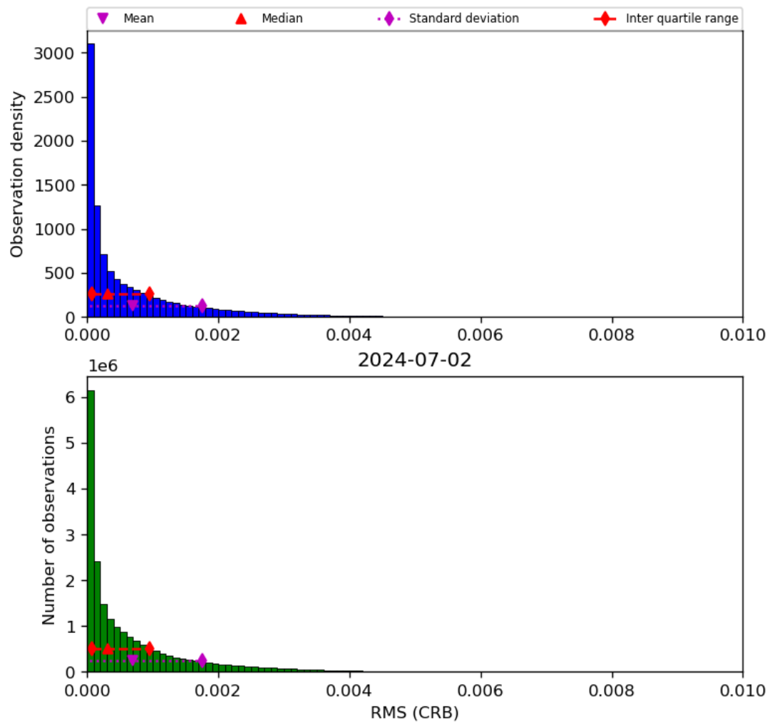
Figure 48: Histogram of “RMS (CRB)” for 2024-07-01 to 2024-07-03
