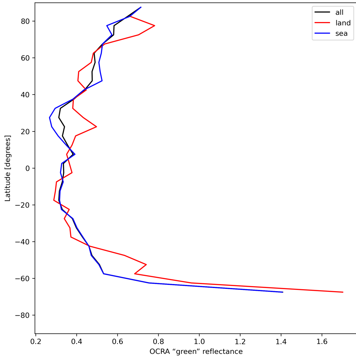
Figure 36: Zonal average of “OCRA “green” reflectance” for 2024-07-01 to 2024-07-03.
