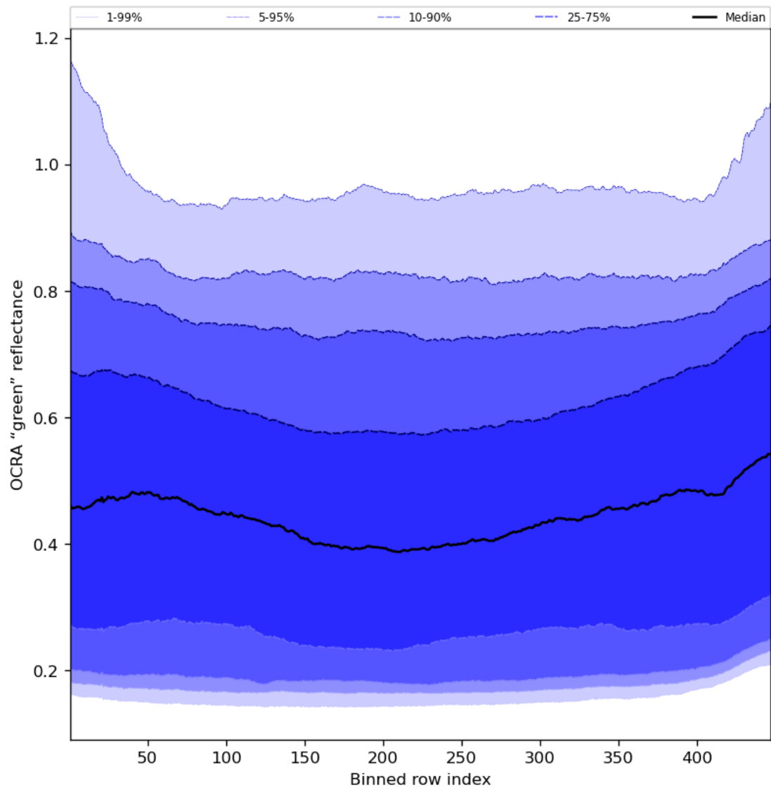
Figure 68: Along track statistics of “OCRA “green” reflectance” for 2024-07-01 to 2024-07-03
