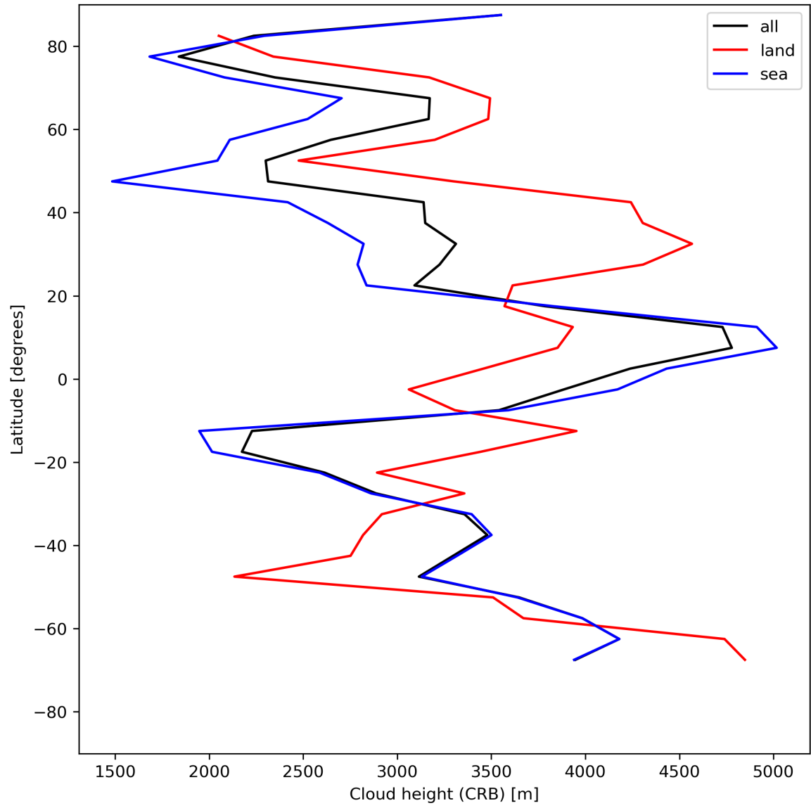
Figure 27: Zonal average of “Cloud height (CRB)” for 2024-07-01 to 2024-07-03.
