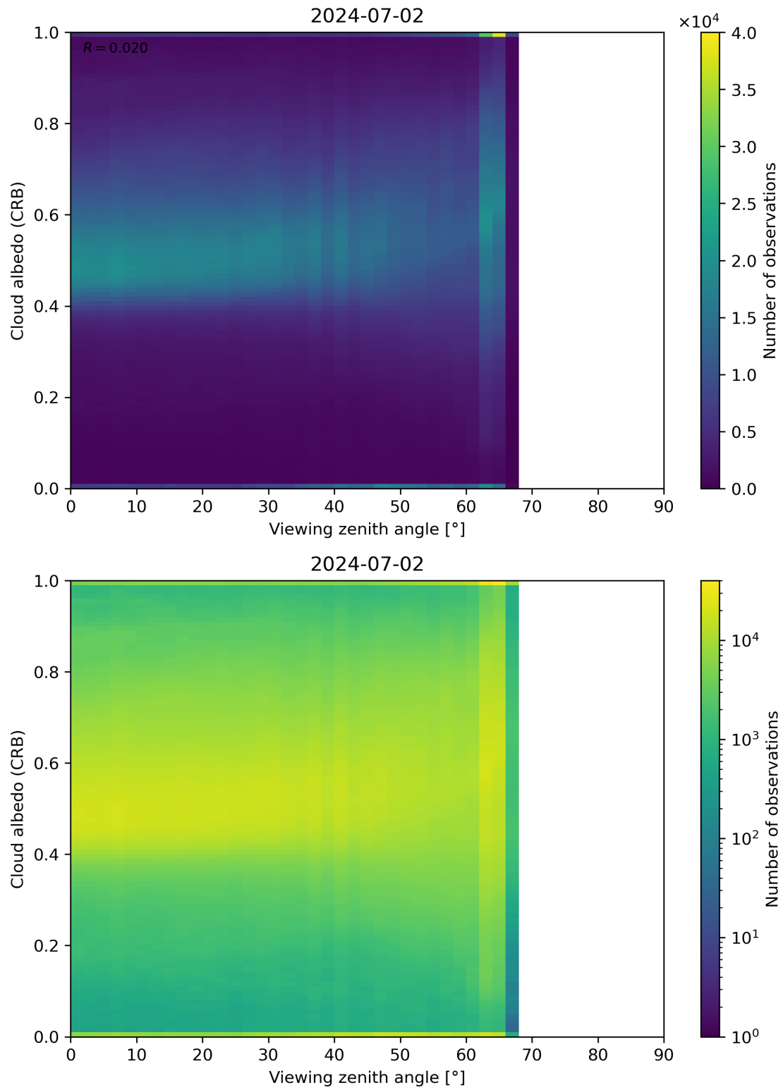
Figure 106: Scatter density plot of “Viewing zenith angle” against “Cloud albedo (CRB)” for 2024-07-01 to 2024-07-03.
