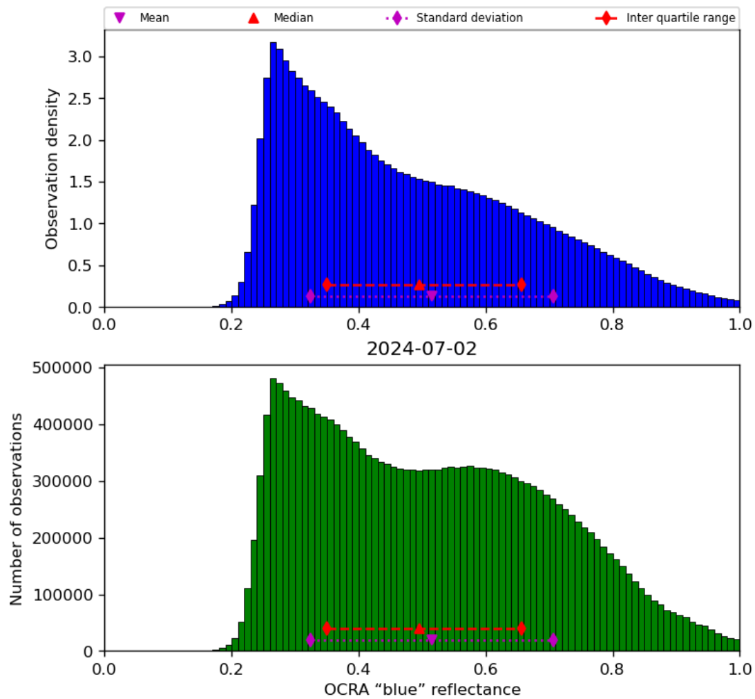
Figure 51: Histogram of “OCRA “blue” reflectance” for 2024-07-01 to 2024-07-03
