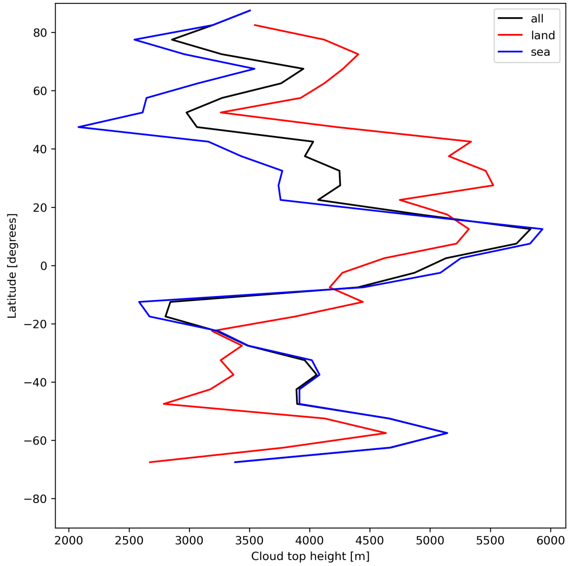
Figure 24: Zonal average of “Cloud top height” for 2024-07-01 to 2024-07-03.
