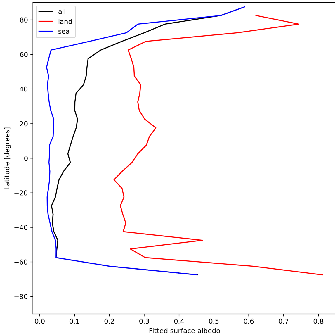
Figure 29: Zonal average of “Fitted surface albedo” for 2024-07-01 to 2024-07-03.
