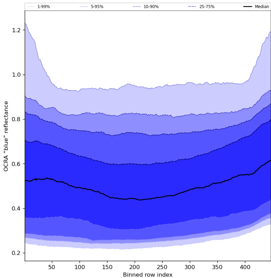
Figure 67: Along track statistics of “OCRA “blue” reflectance” for 2024-07-01 to 2024-07-03
