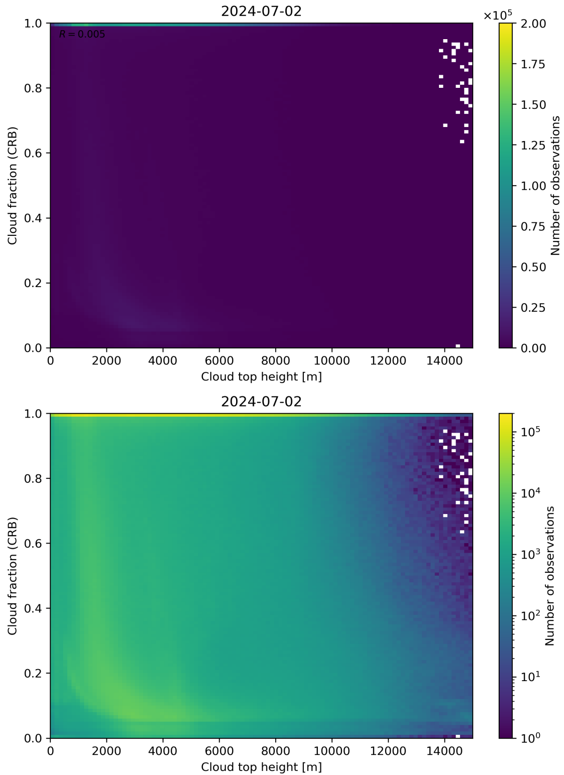
Figure 88: Scatter density plot of “Cloud top height” against “Cloud fraction (CRB)” for 2024-07-01 to 2024-07-03.
