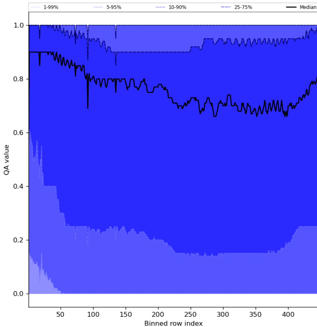
Figure 54: Along track statistics of “QA value” for 2024-07-01 to 2024-07-03
