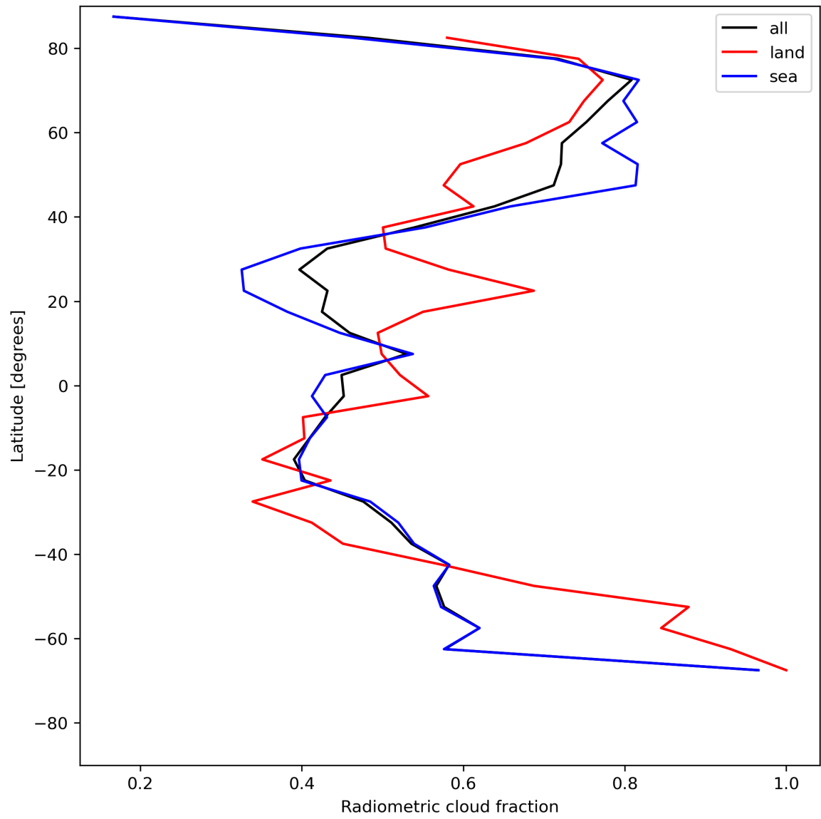
Figure 23: Zonal average of “Radiometric cloud fraction” for 2024-07-01 to 2024-07-03.
