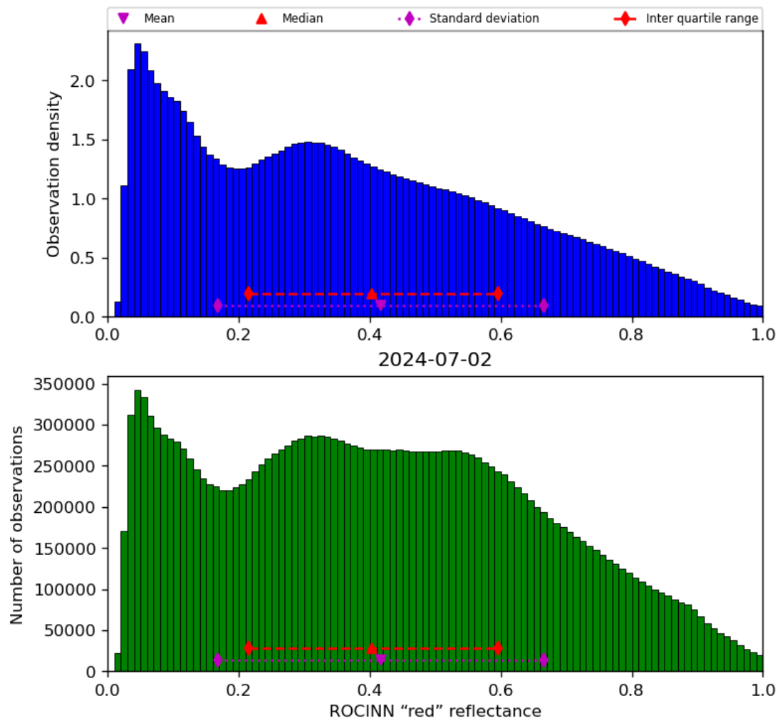
Figure 53: Histogram of “ROCINN “red” reflectance” for 2024-07-01 to 2024-07-03
