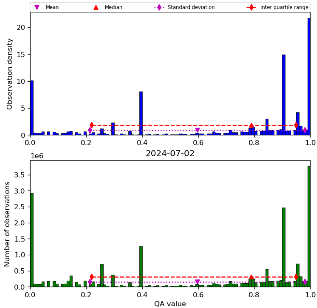
Figure 38: Histogram of “QA value” for 2024-07-01 to 2024-07-03
