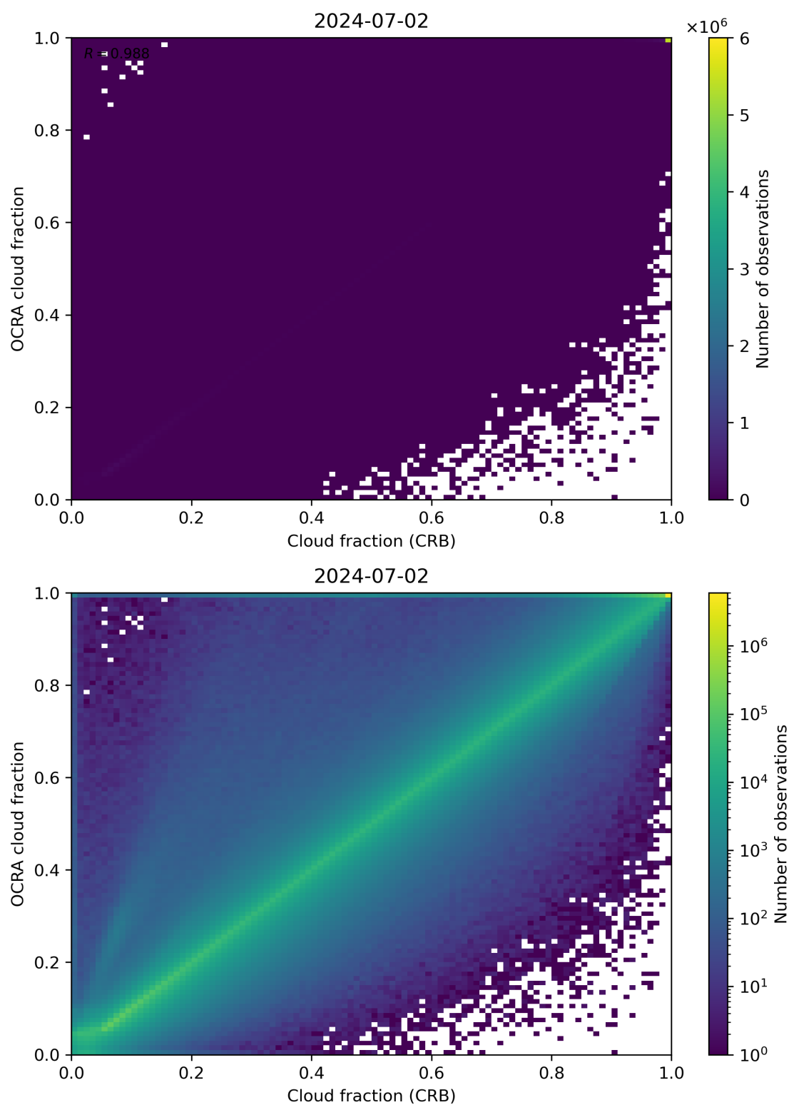
Figure 78: Scatter density plot of “Cloud fraction (CRB)” against “OCRA cloud fraction” for 2024-07-01 to 2024-07-03.
