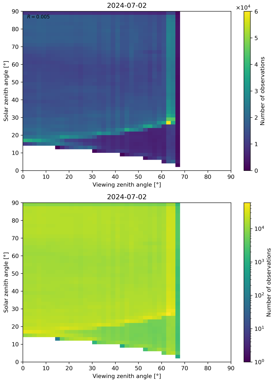
Figure 114: Scatter density plot of “Viewing zenith angle” against “Solar zenith angle” for 2024-07-01 to 2024-07-03.
