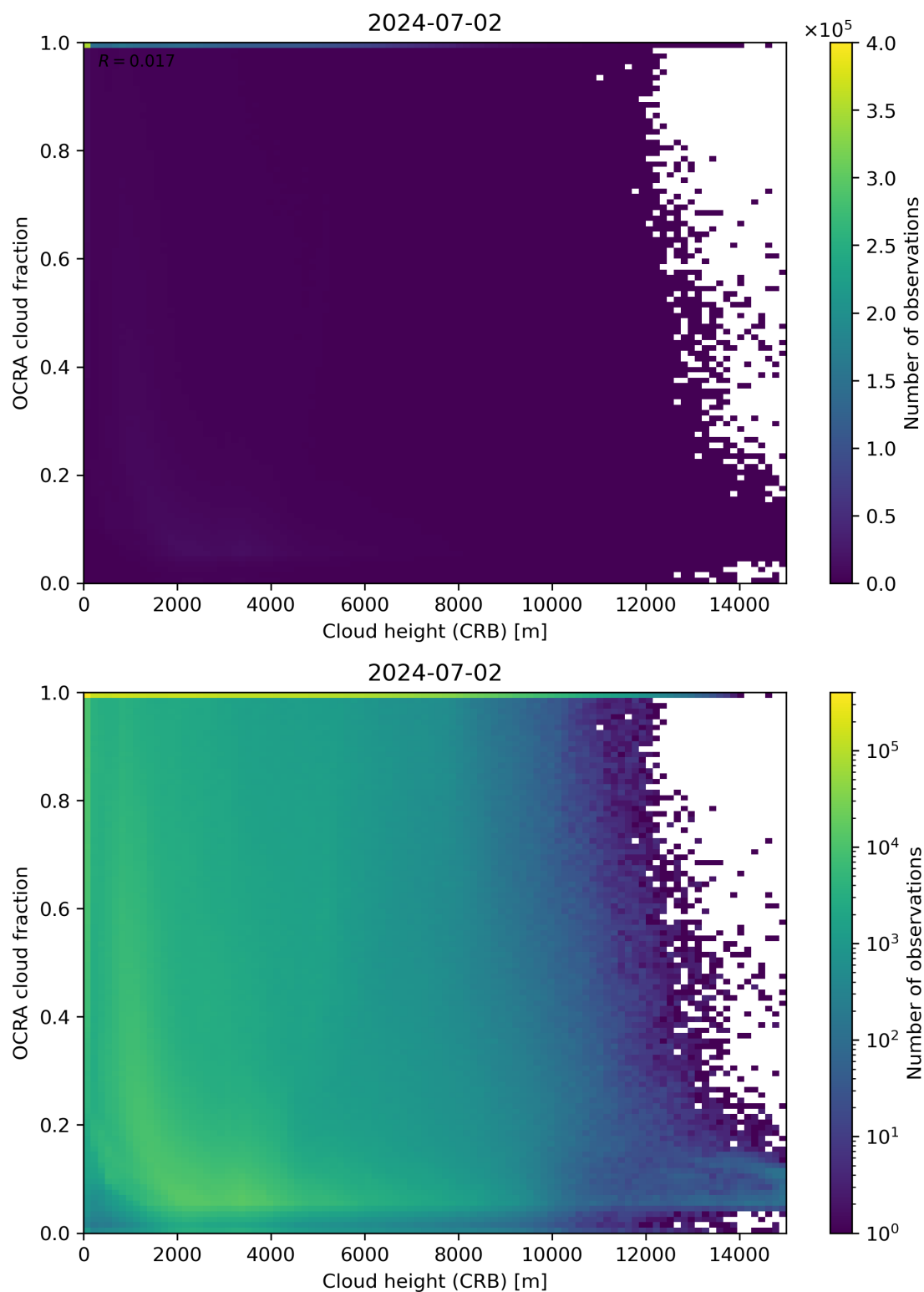
Figure 81: Scatter density plot of “Cloud height (CRB)” against “OCRA cloud fraction” for 2024-07-01 to 2024-07-03.
