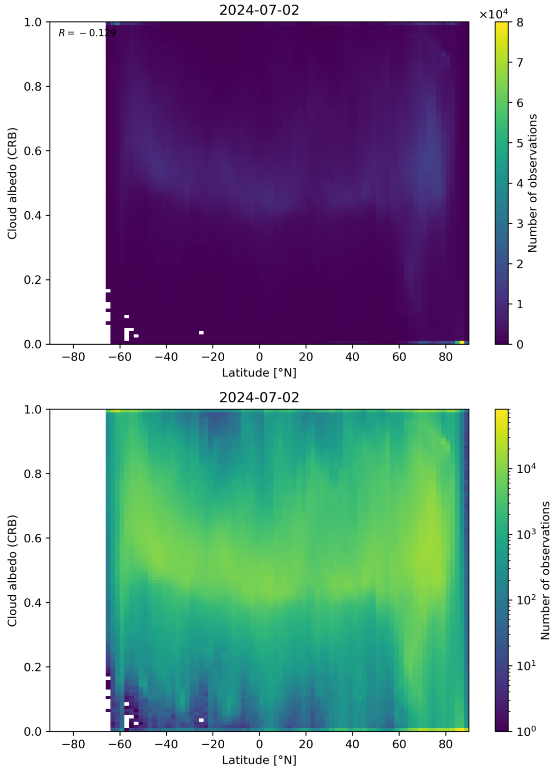
Figure 91: Scatter density plot of “Latitude” against “Cloud albedo (CRB)” for 2024-07-01 to 2024-07-03.
