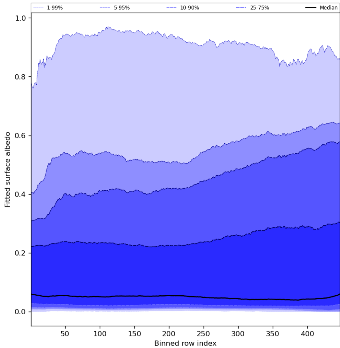
Figure 61: Along track statistics of “Fitted surface albedo” for 2024-07-01 to 2024-07-03
