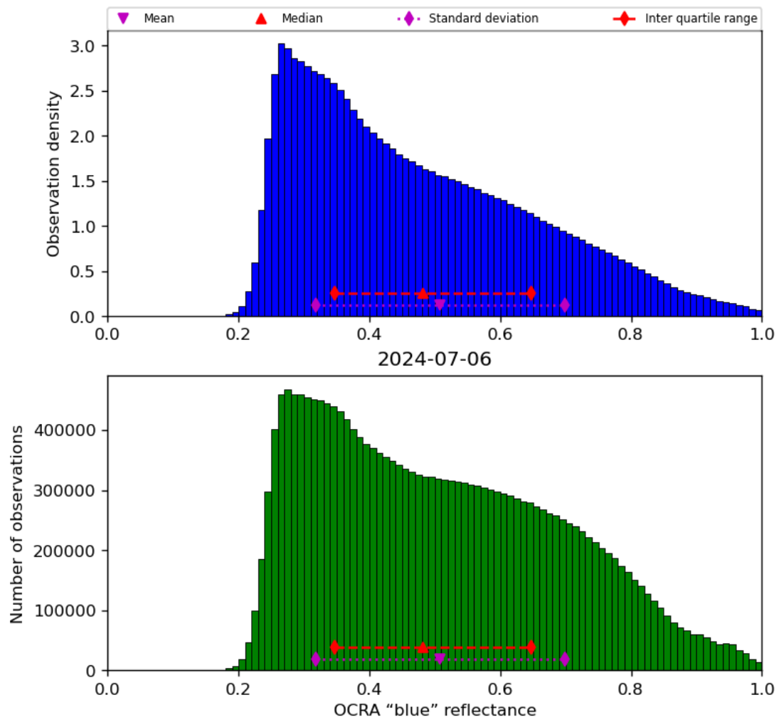
Figure 51: Histogram of “OCRA “blue” reflectance” for 2024-07-05 to 2024-07-07
