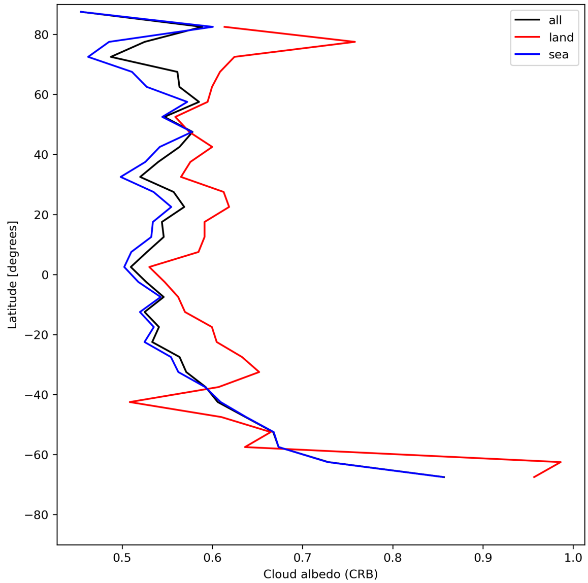
Figure 28: Zonal average of “Cloud albedo (CRB)” for 2024-07-05 to 2024-07-07.
