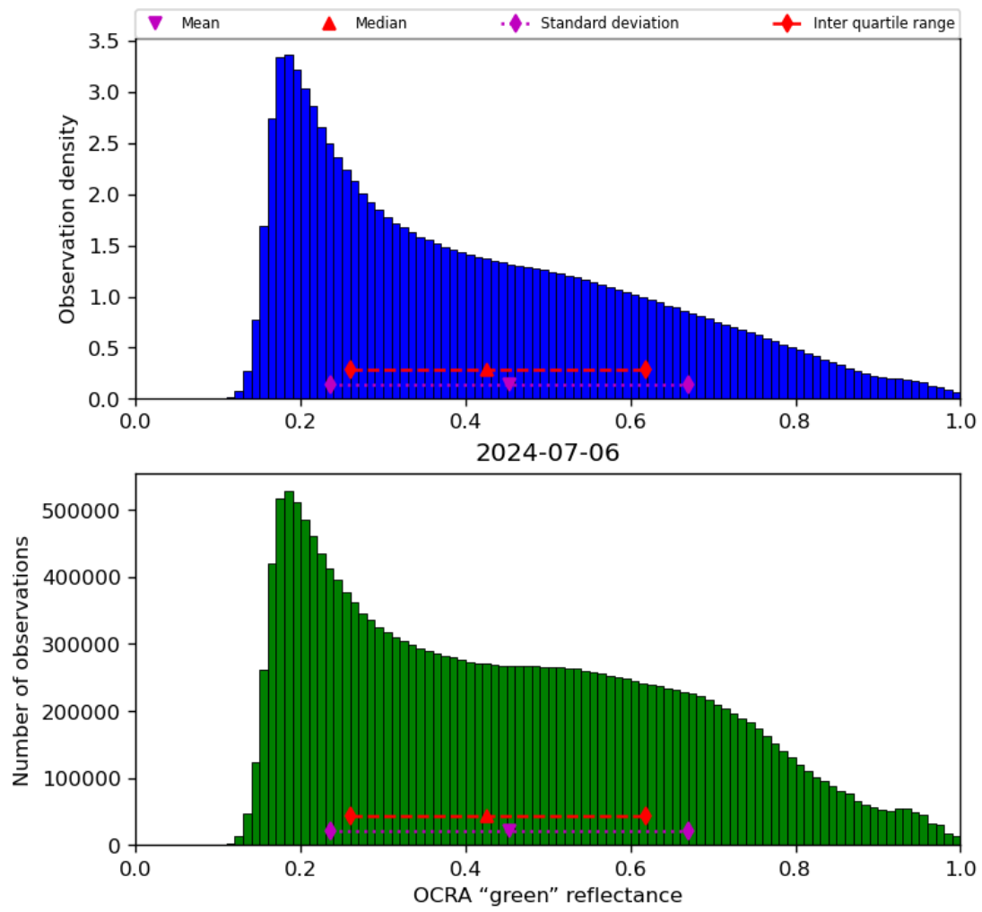
Figure 52: Histogram of “OCRA “green” reflectance” for 2024-07-05 to 2024-07-07
