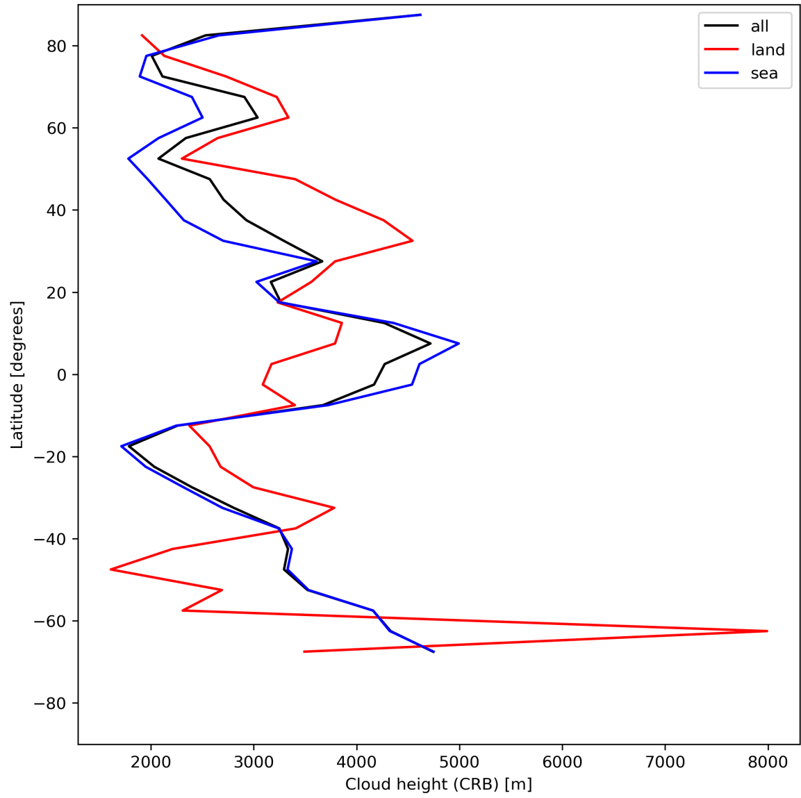
Figure 27: Zonal average of “Cloud height (CRB)” for 2024-07-05 to 2024-07-07.
