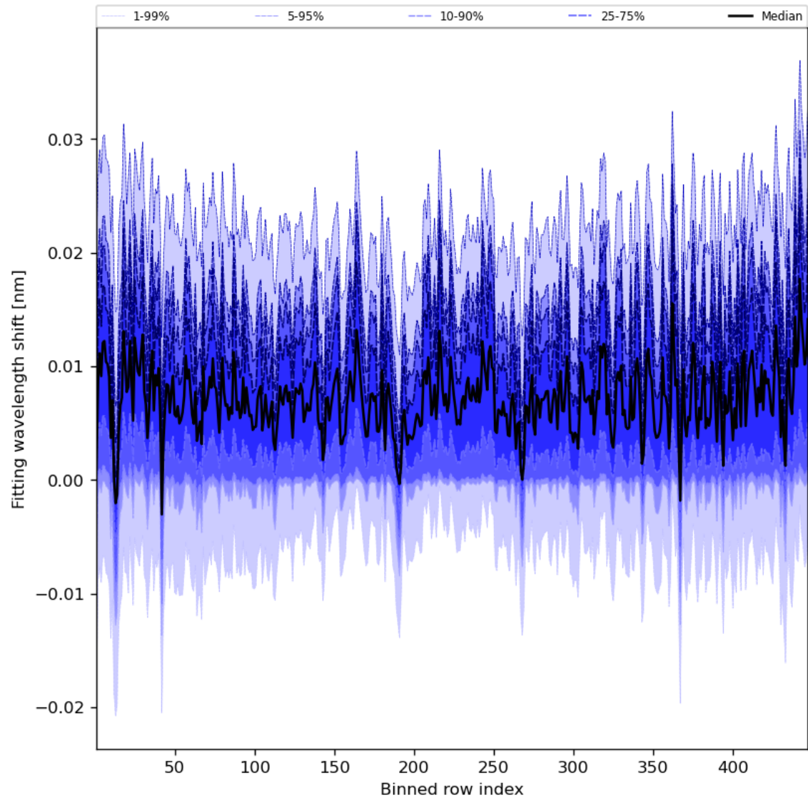
Figure 65: Along track statistics of “Fitting wavelength shift” for 2024-07-05 to 2024-07-07
