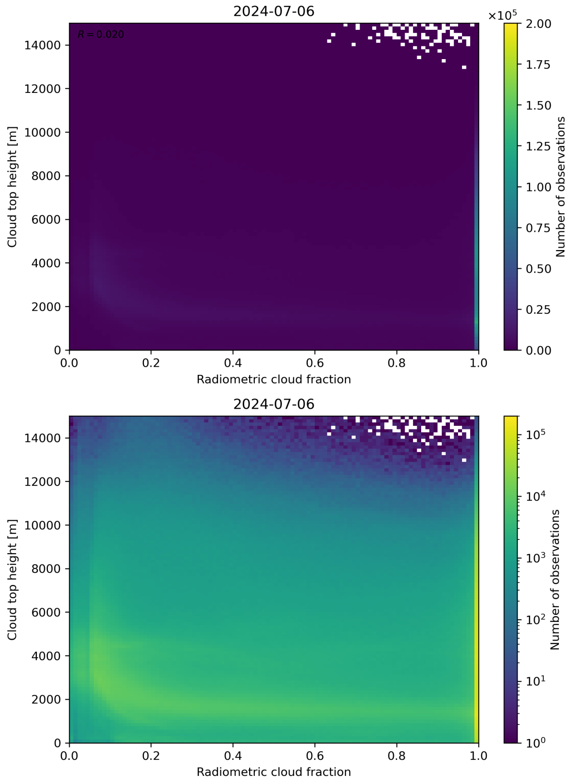
Figure 76: Scatter density plot of “Radiometric cloud fraction” against “Cloud top height” for 2024-07-05 to 2024-07-07.
