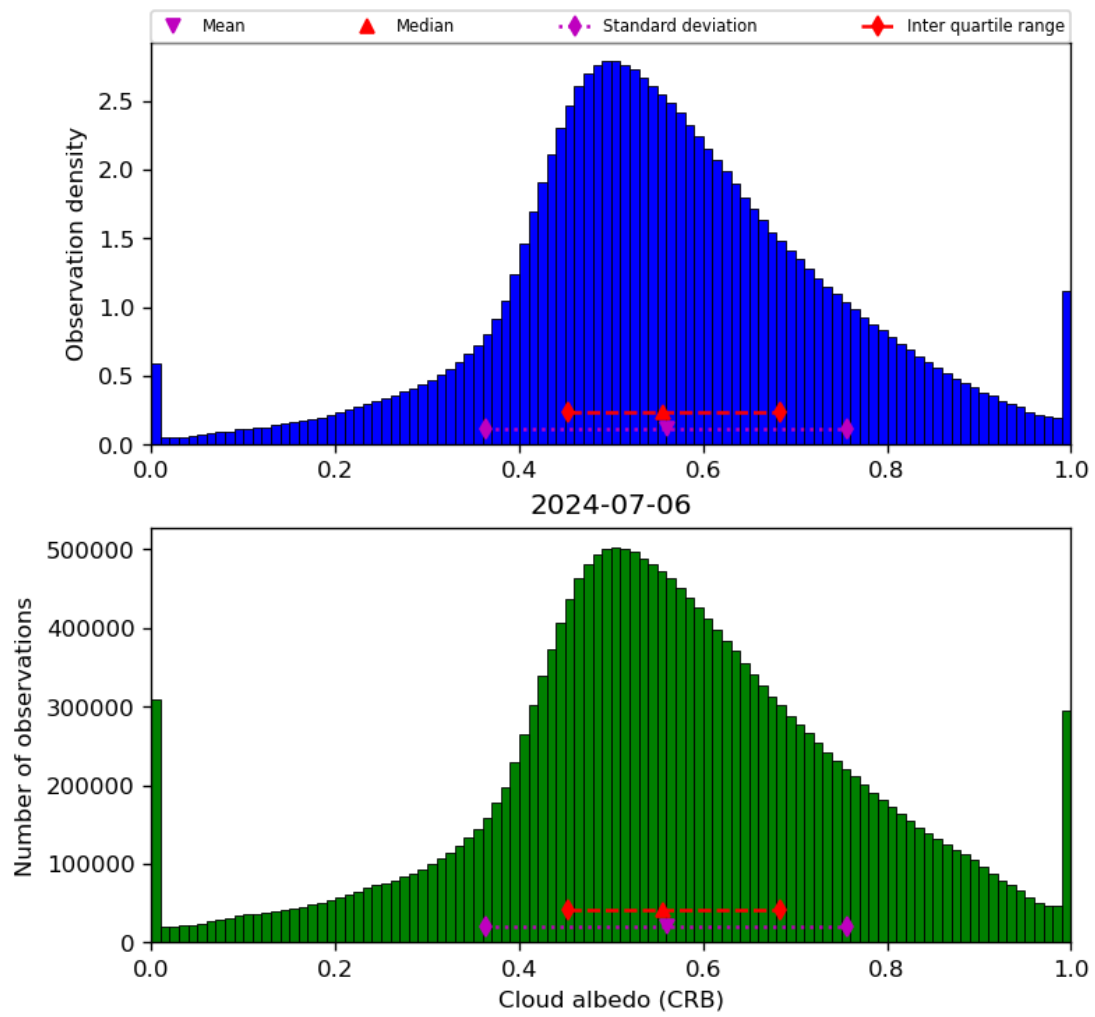
Figure 44: Histogram of “Cloud albedo (CRB)” for 2024-07-05 to 2024-07-07
