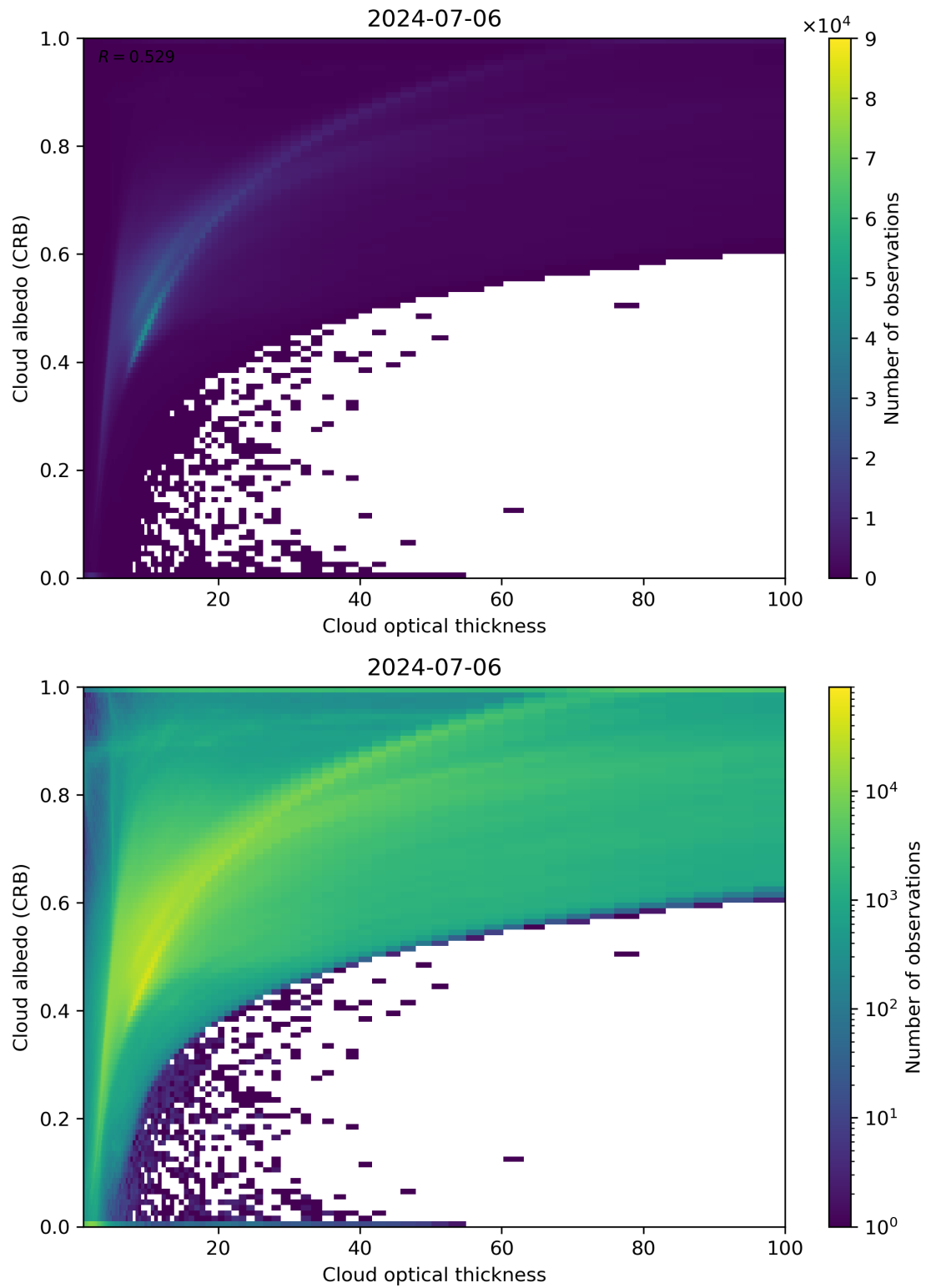
Figure 82: Scatter density plot of “Cloud optical thickness” against “Cloud albedo (CRB)” for 2024-07-05 to 2024-07-07.
