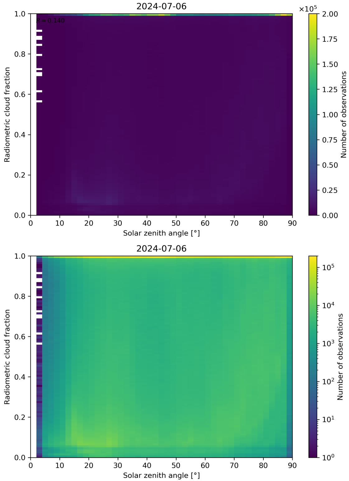
Figure 99: Scatter density plot of “Solar zenith angle” against “Radiometric cloud fraction” for 2024-07-05 to 2024-07-07.
