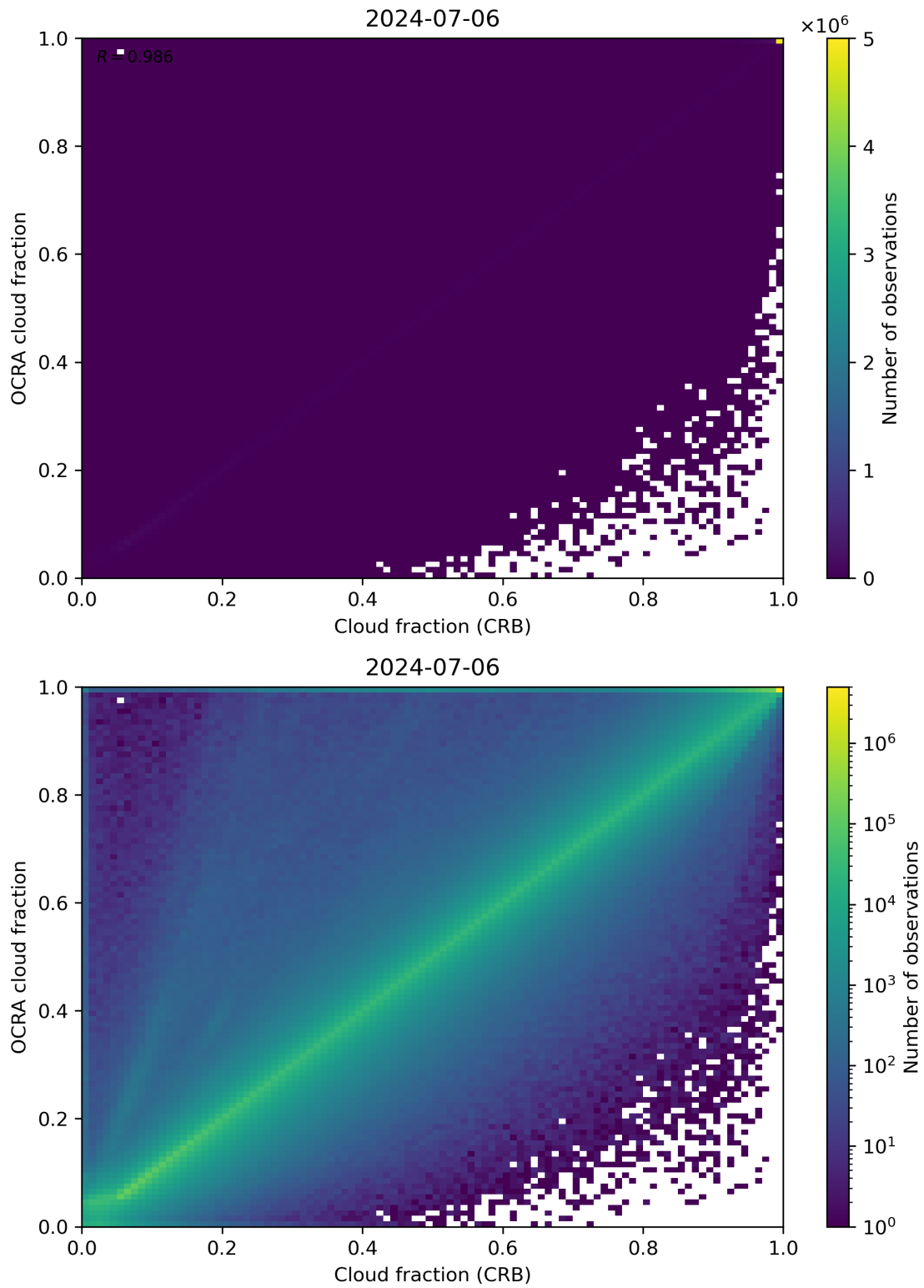
Figure 78: Scatter density plot of “Cloud fraction (CRB)” against “OCRA cloud fraction” for 2024-07-05 to 2024-07-07.
