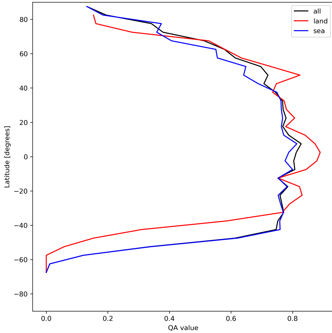
Figure 22: Zonal average of “QA value” for 2024-07-05 to 2024-07-07.
