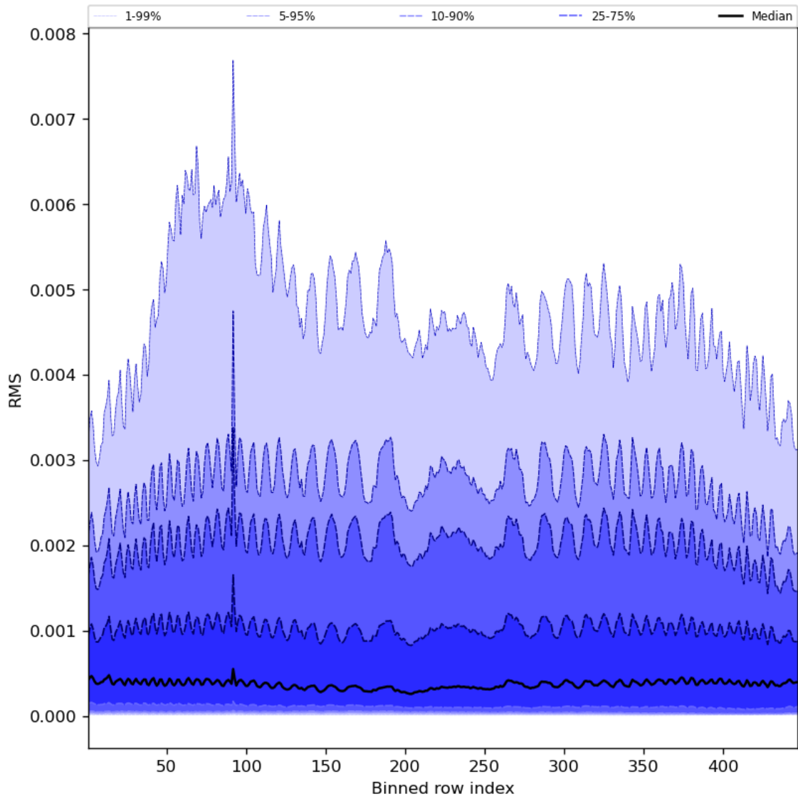
Figure 63: Along track statistics of “RMS” for 2024-07-05 to 2024-07-07
