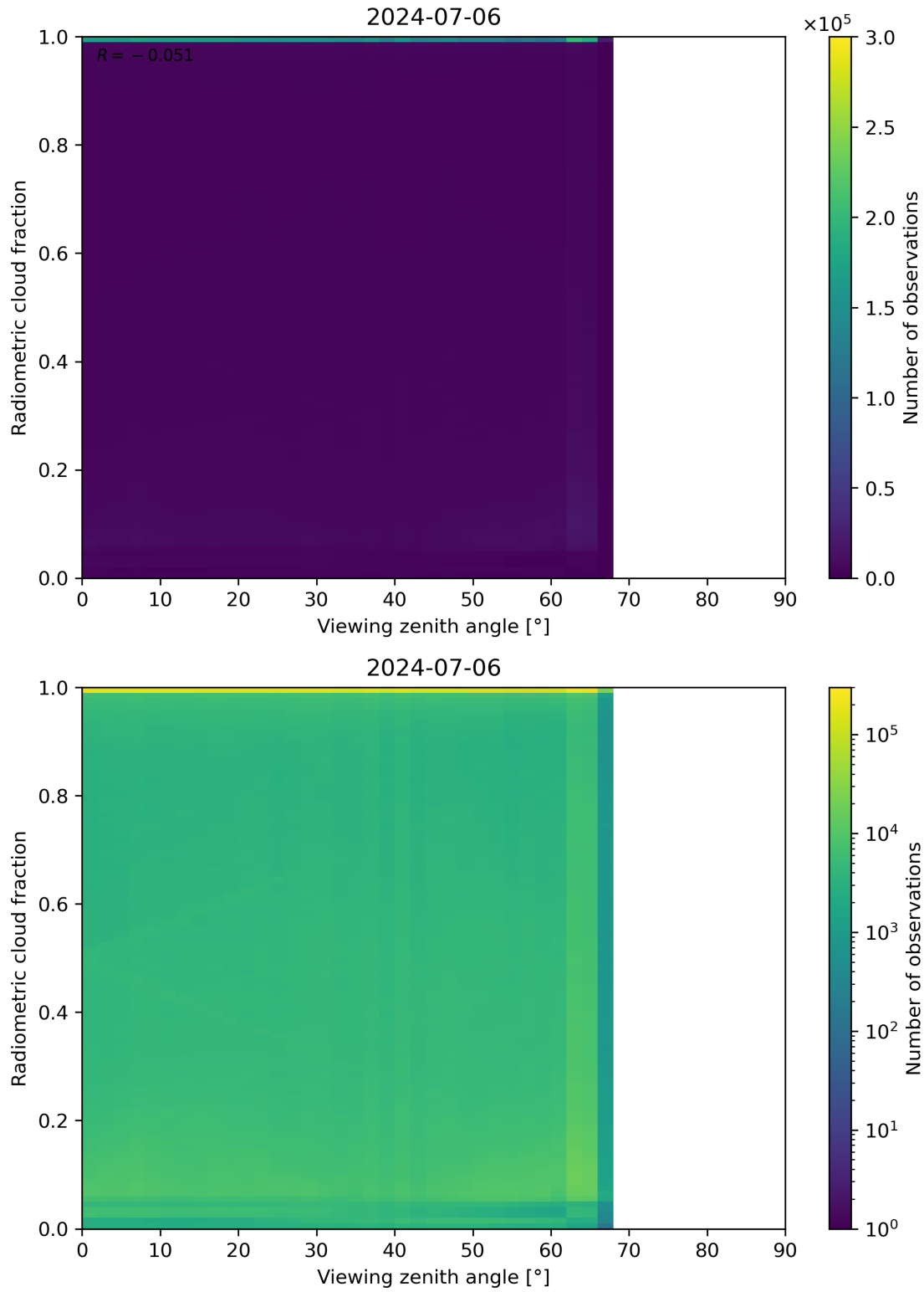
Figure 107: Scatter density plot of “Viewing zenith angle” against “Radiometric cloud fraction” for 2024-07-05 to 2024-07-07.
