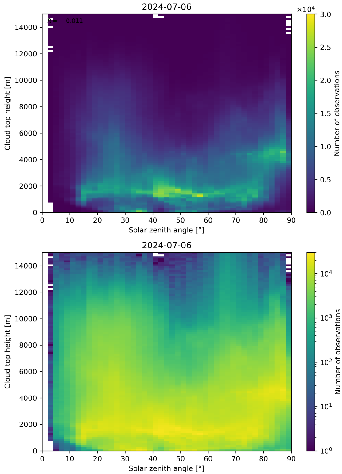
Figure 104: Scatter density plot of “Solar zenith angle” against “Cloud top height” for 2024-07-05 to 2024-07-07.
