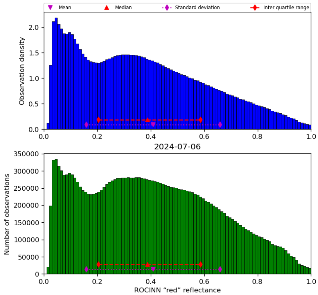
Figure 53: Histogram of “ROCINN “red” reflectance” for 2024-07-05 to 2024-07-07
