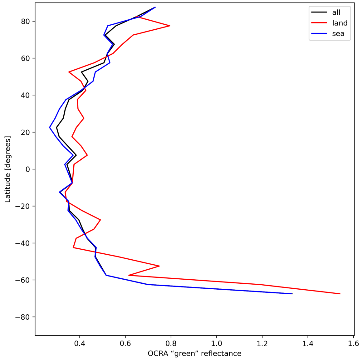
Figure 36: Zonal average of “OCRA “green” reflectance” for 2024-07-05 to 2024-07-07.
