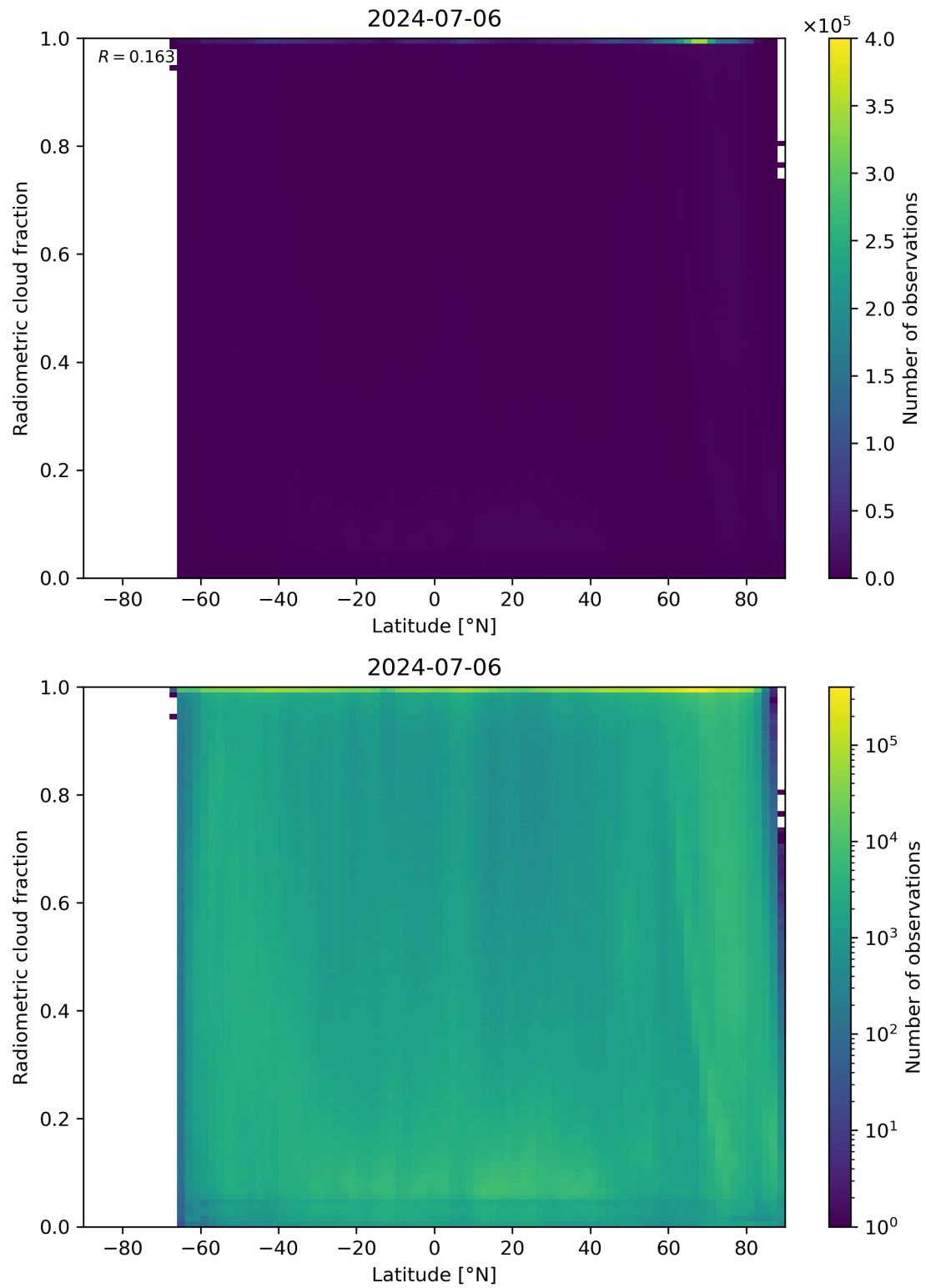
Figure 92: Scatter density plot of “Latitude” against “Radiometric cloud fraction” for 2024-07-05 to 2024-07-07.
