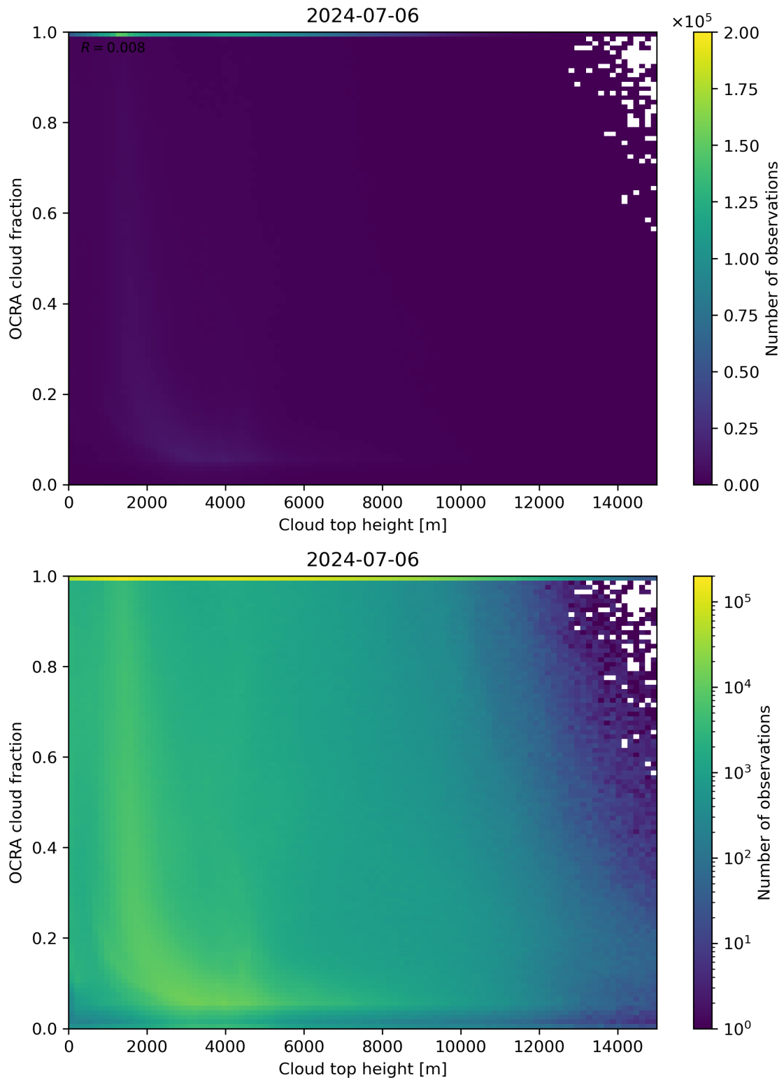
Figure 87: Scatter density plot of “Cloud top height” against “OCRA cloud fraction” for 2024-07-05 to 2024-07-07.
