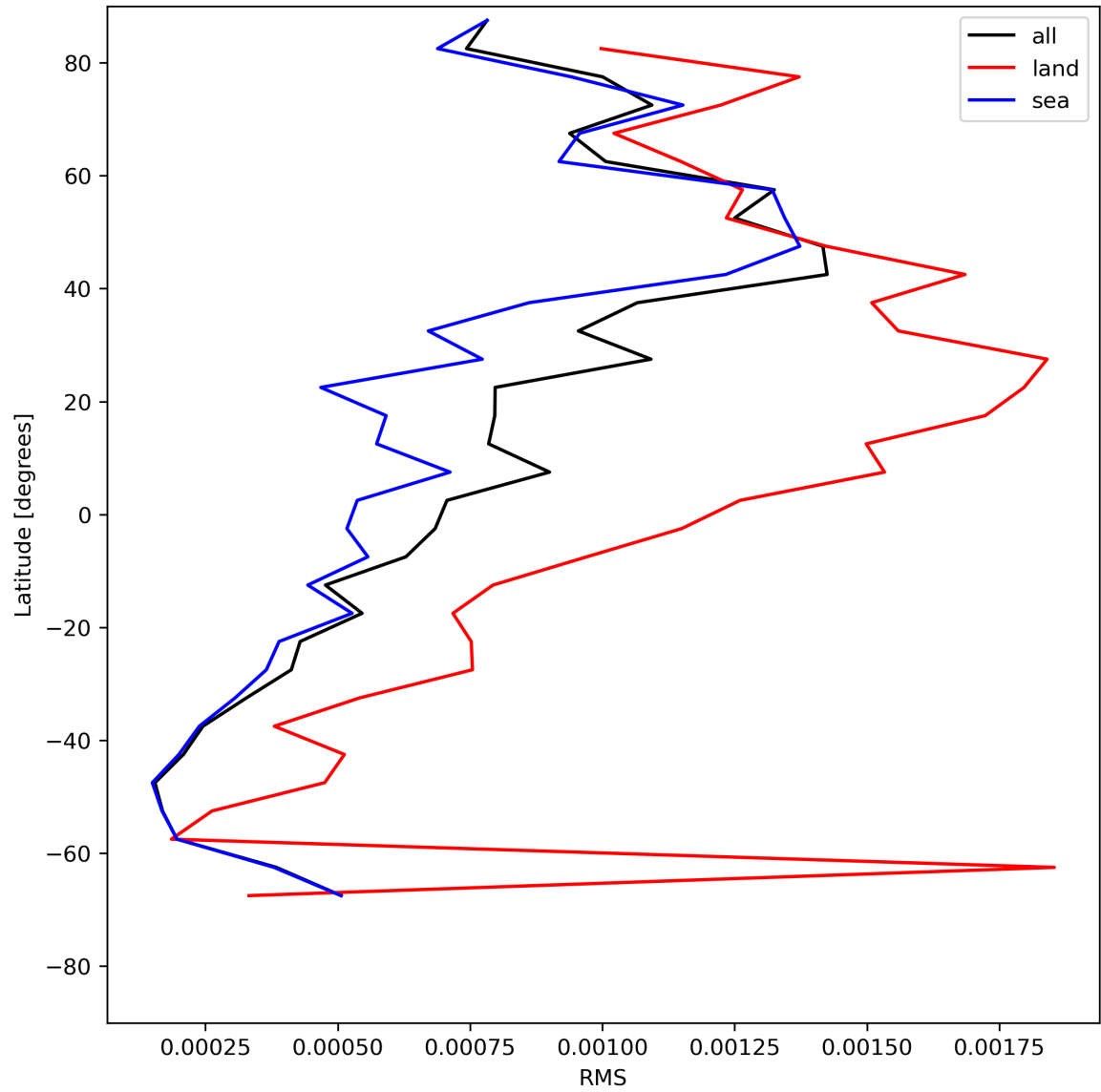
Figure 31: Zonal average of “RMS” for 2024-07-05 to 2024-07-07.
