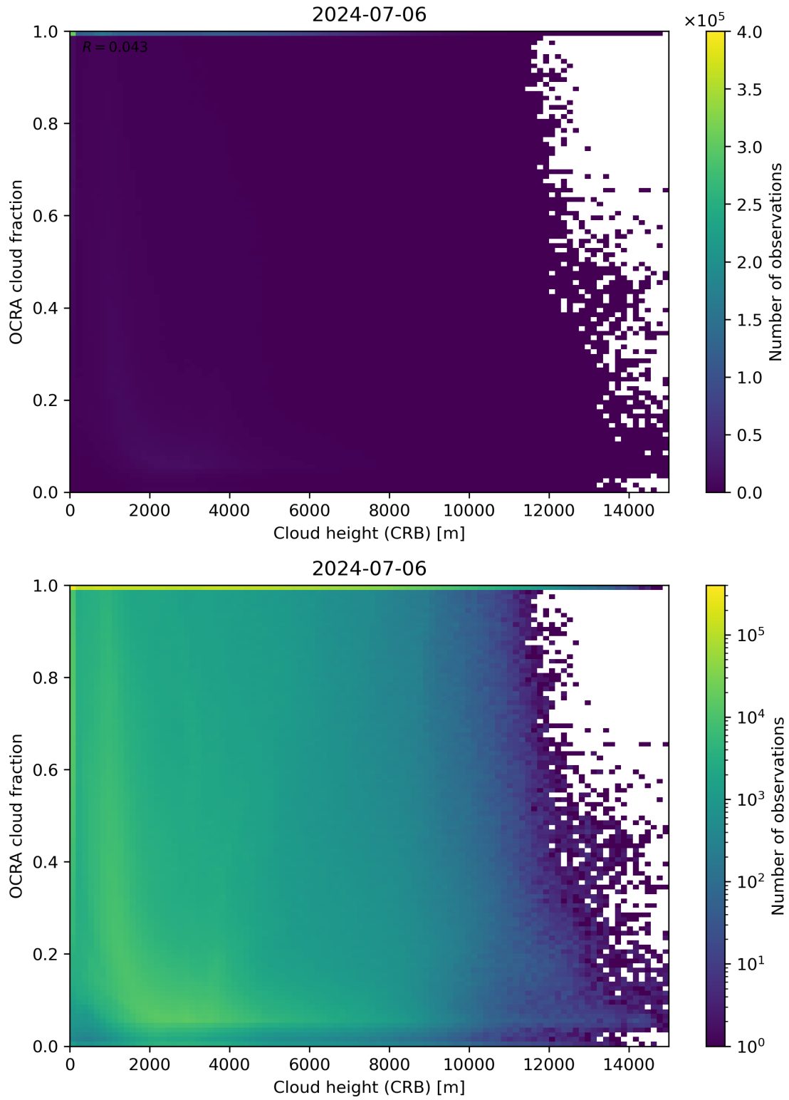
Figure 81: Scatter density plot of “Cloud height (CRB)” against “OCRA cloud fraction” for 2024-07-05 to 2024-07-07.
