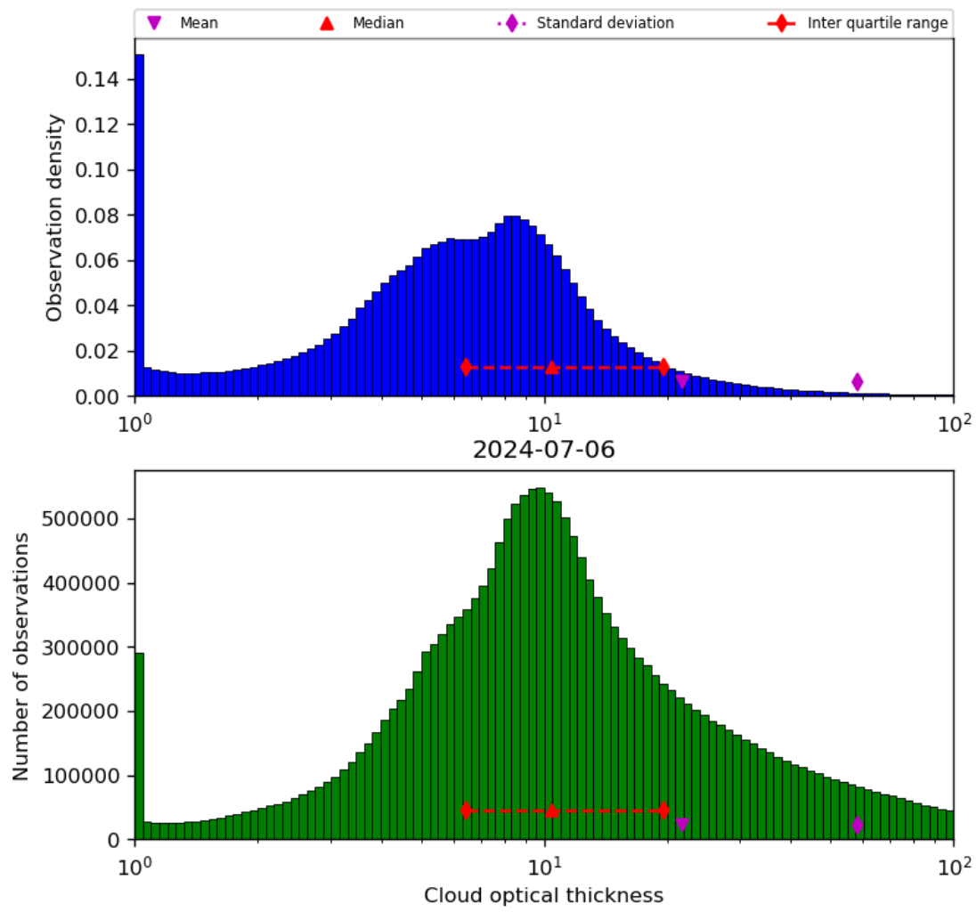
Figure 41: Histogram of “Cloud optical thickness” for 2024-07-05 to 2024-07-07
