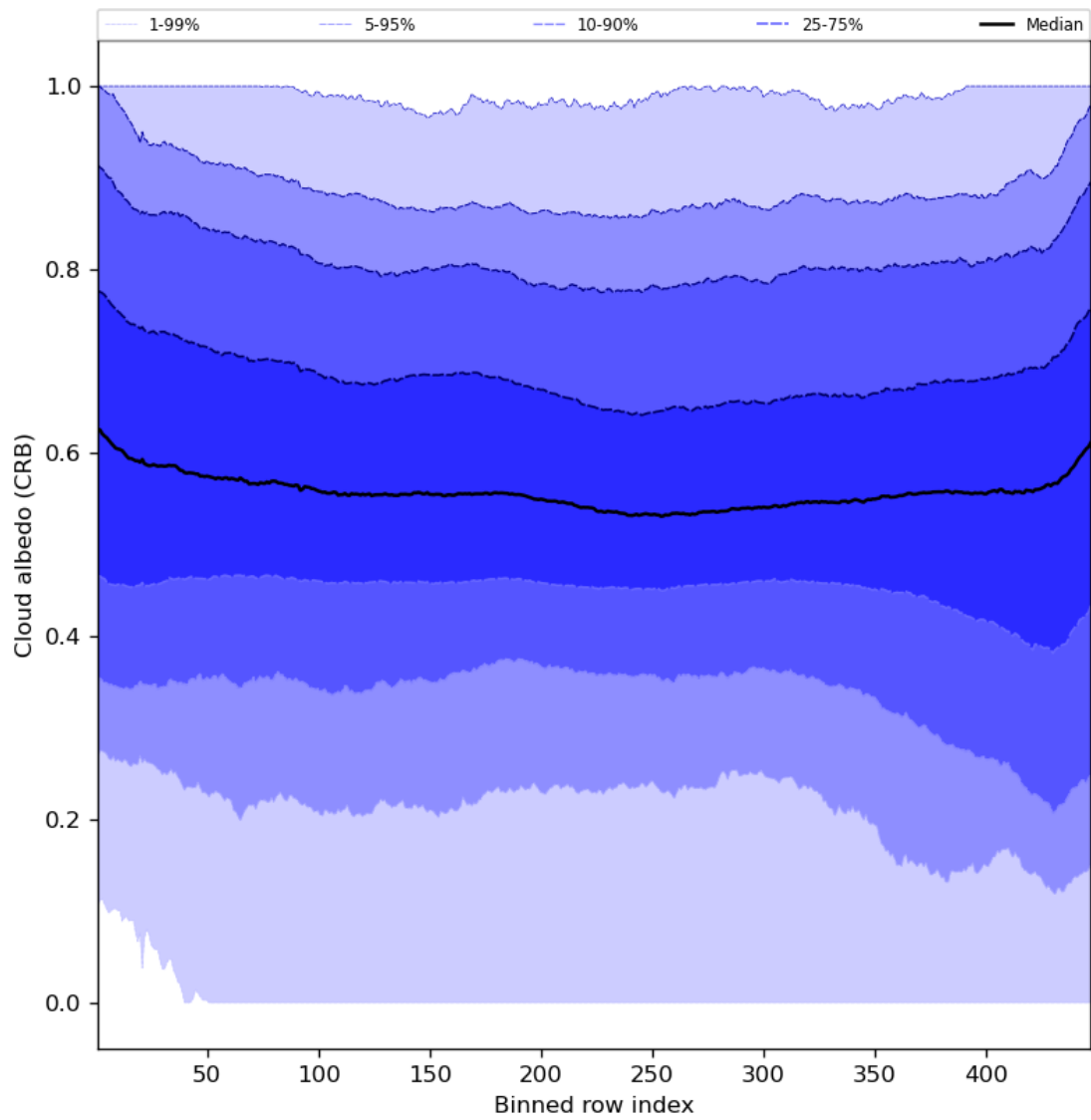
Figure 60: Along track statistics of “Cloud albedo (CRB)” for 2024-07-05 to 2024-07-07
