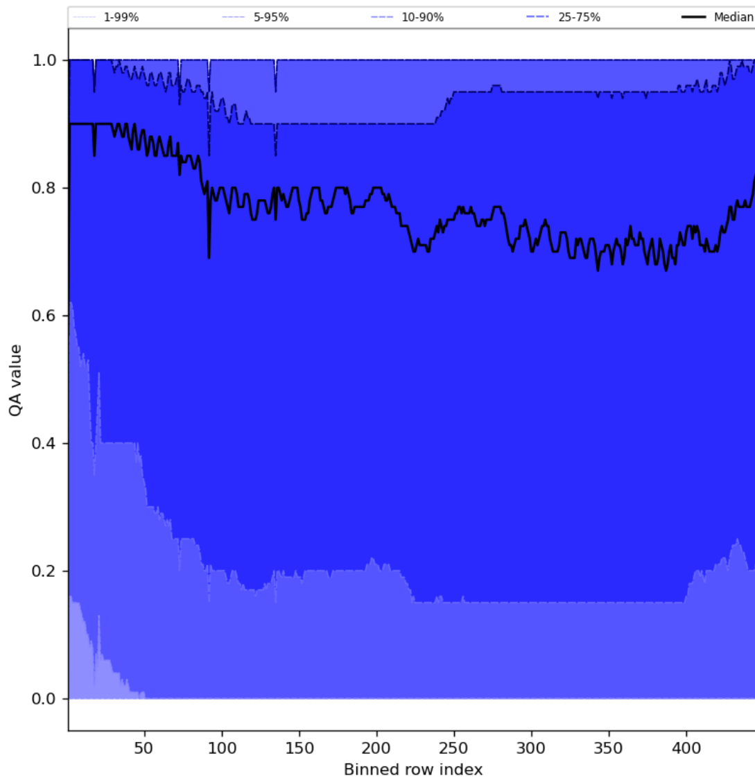
Figure 54: Along track statistics of “QA value” for 2024-07-05 to 2024-07-07
