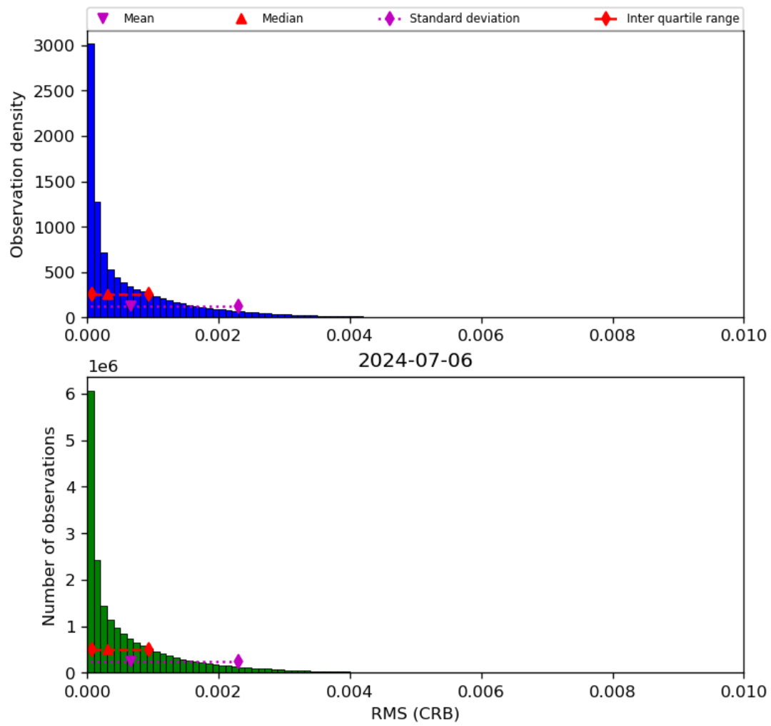
Figure 48: Histogram of “RMS (CRB)” for 2024-07-05 to 2024-07-07
