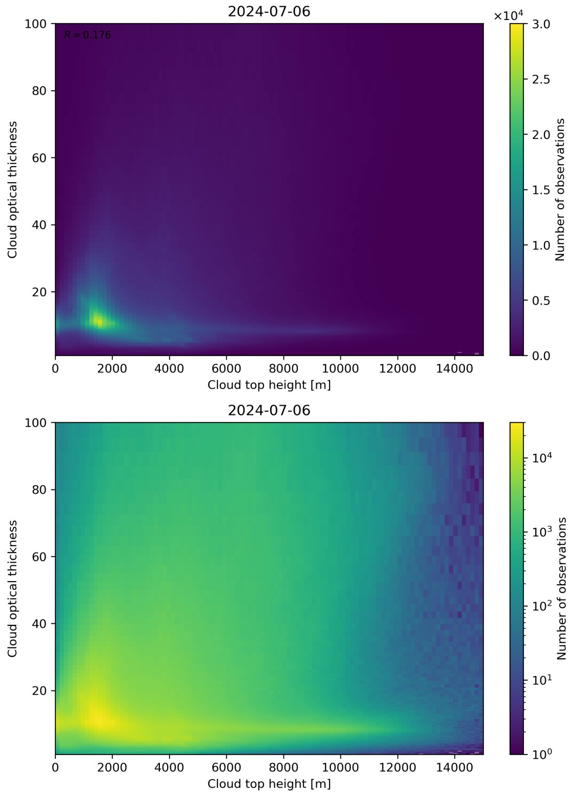
Figure 90: Scatter density plot of “Cloud top height” against “Cloud optical thickness” for 2024-07-05 to 2024-07-07.
