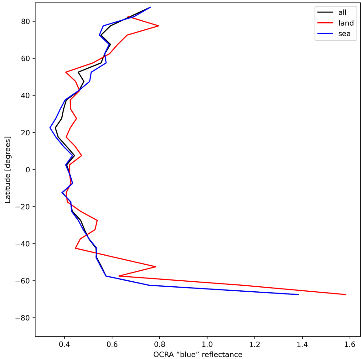
Figure 35: Zonal average of “OCRA “blue” reflectance” for 2024-07-05 to 2024-07-07.
