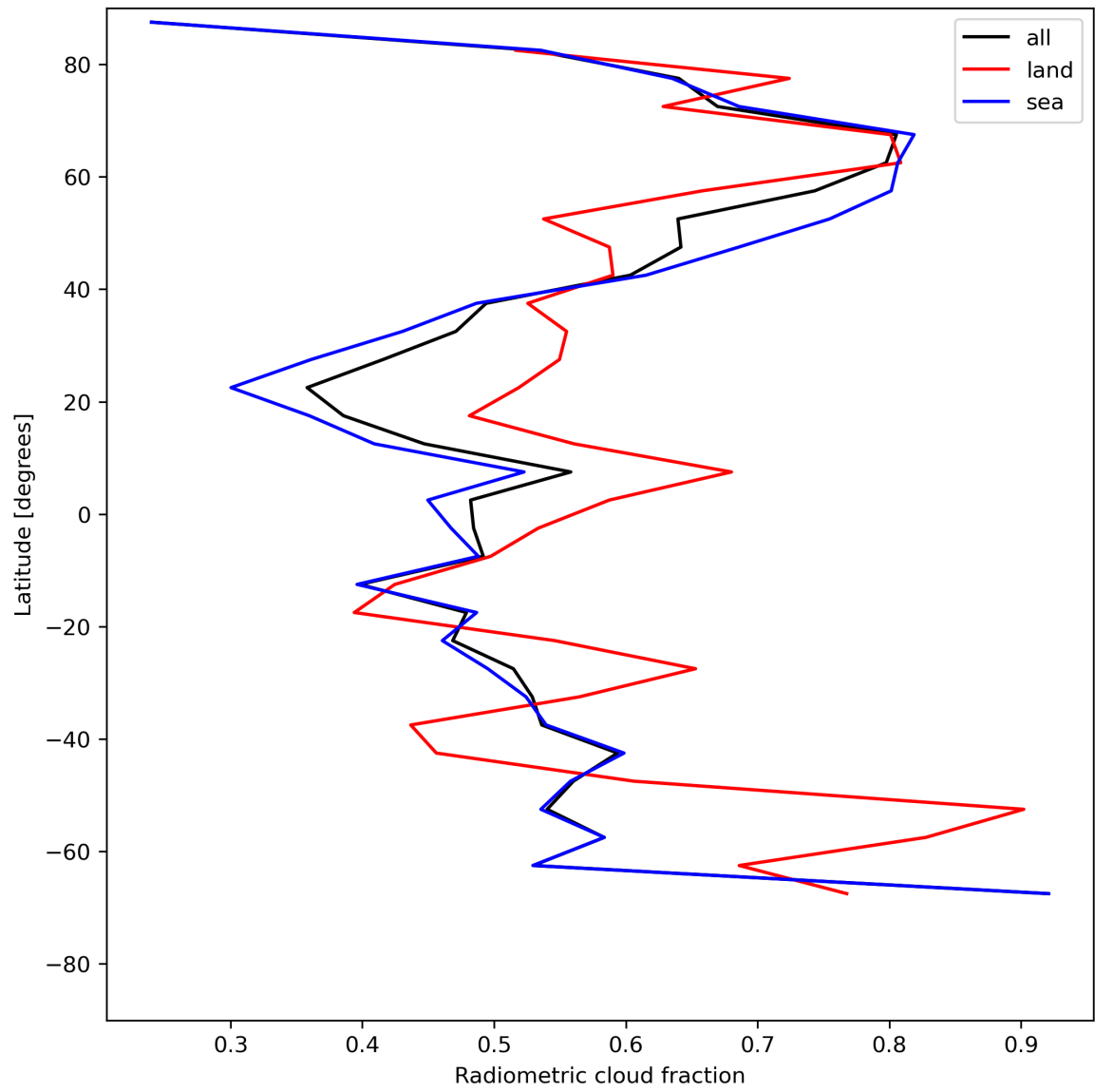
Figure 23: Zonal average of “Radiometric cloud fraction” for 2024-07-05 to 2024-07-07.
