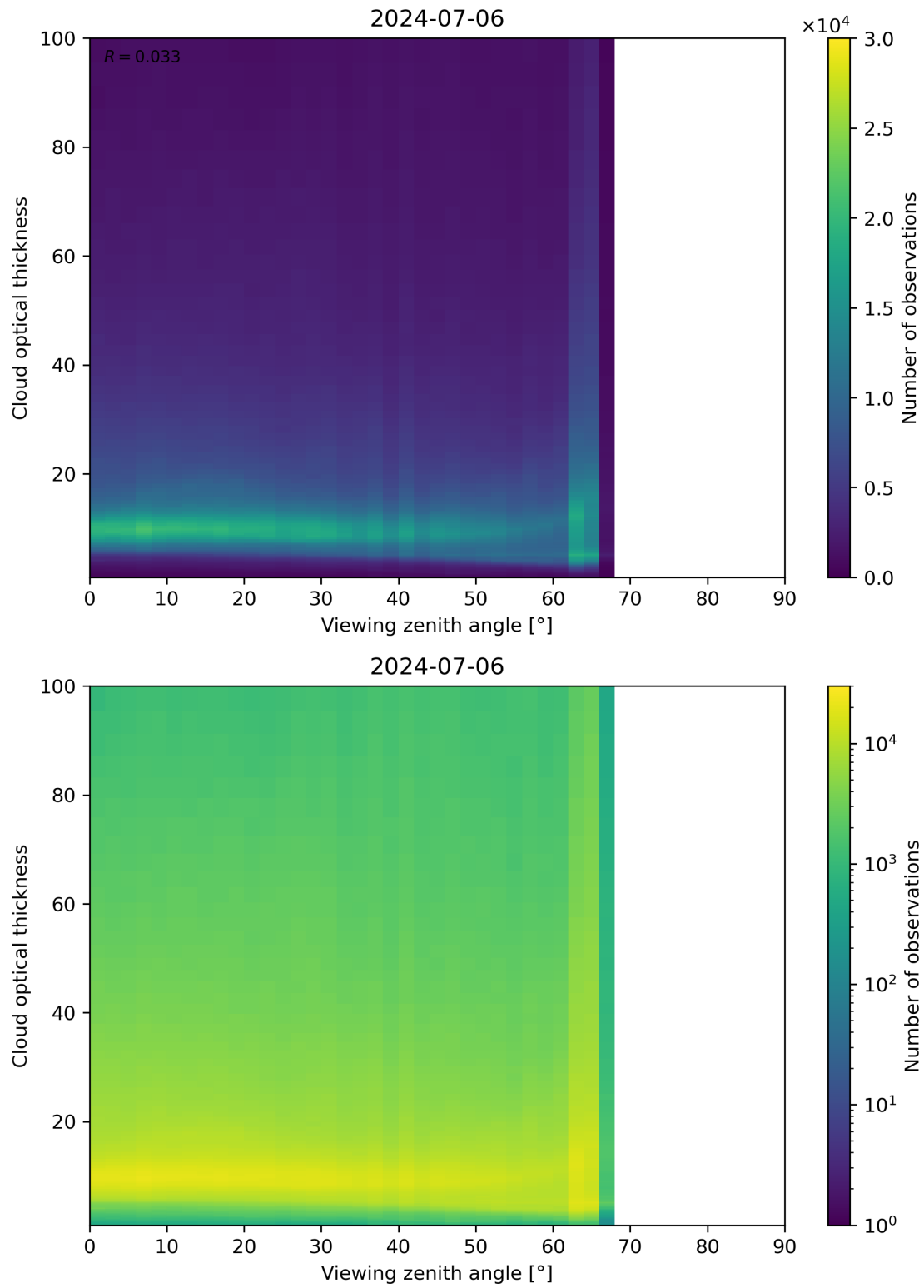
Figure 111: Scatter density plot of “Viewing zenith angle” against “Cloud optical thickness” for 2024-07-05 to 2024-07-07.
