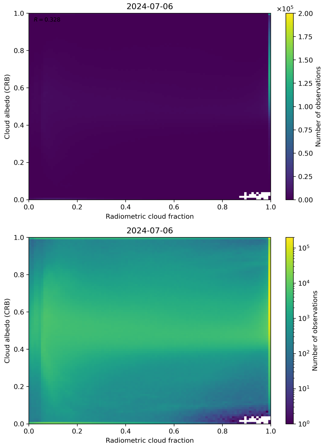
Figure 71: Scatter density plot of “Radiometric cloud fraction” against “Cloud albedo (CRB)” for 2024-07-05 to 2024-07-07.
