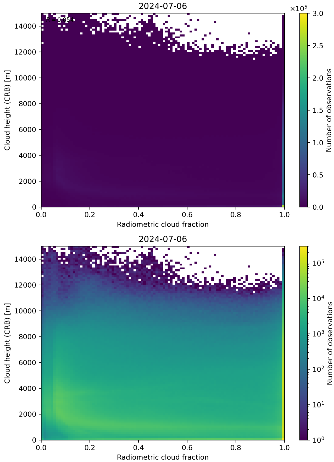
Figure 74: Scatter density plot of “Radiometric cloud fraction” against “Cloud height (CRB)” for 2024-07-05 to 2024-07-07.
