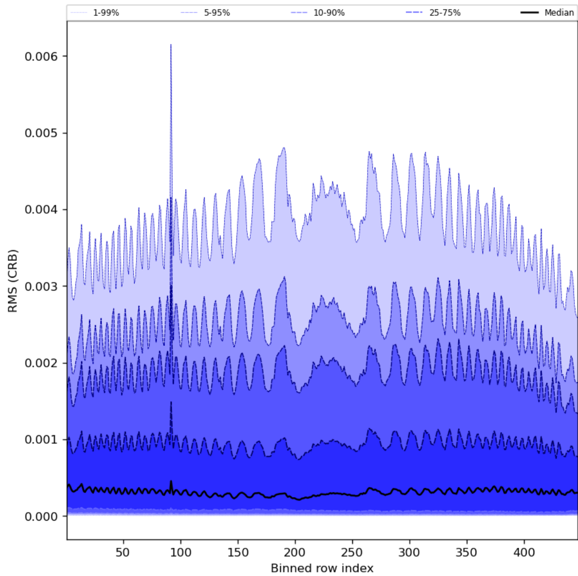
Figure 64: Along track statistics of "RMS (CRB)" for 2024-07-05 to 2024-07-07
