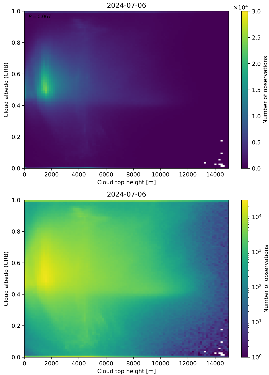
Figure 86: Scatter density plot of “Cloud top height” against “Cloud albedo (CRB)” for 2024-07-05 to 2024-07-07.
