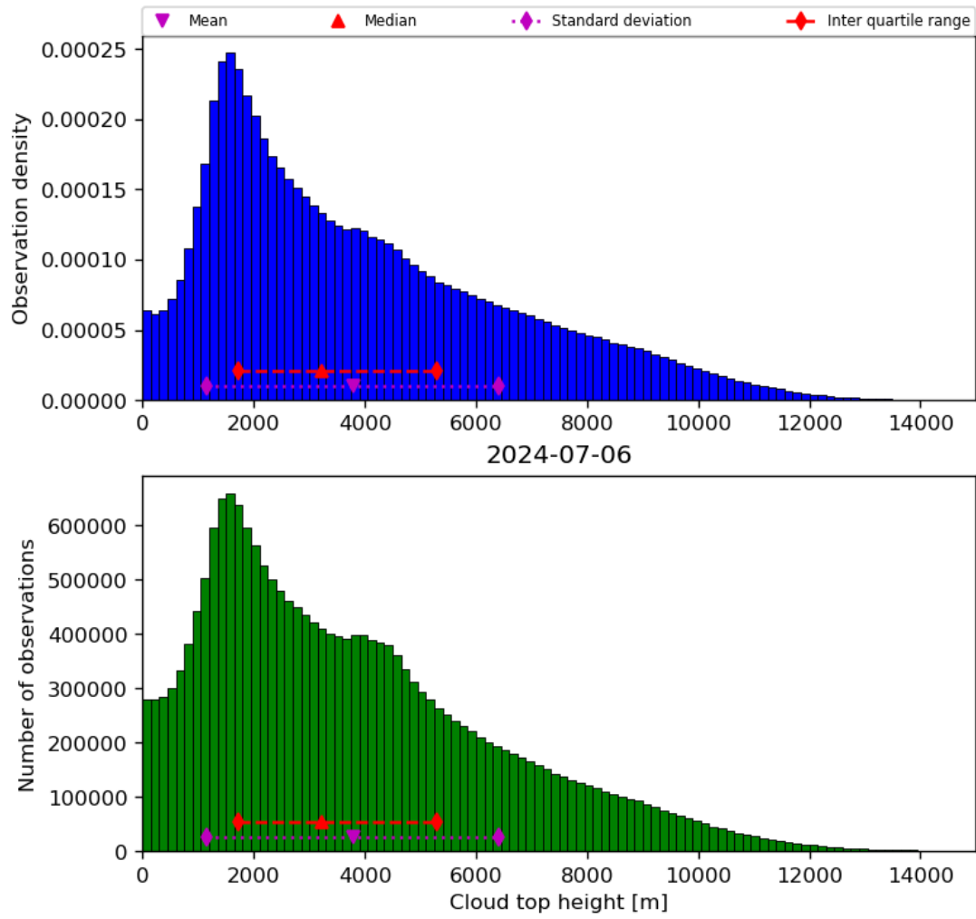
Figure 40: Histogram of “Cloud top height” for 2024-07-05 to 2024-07-07
