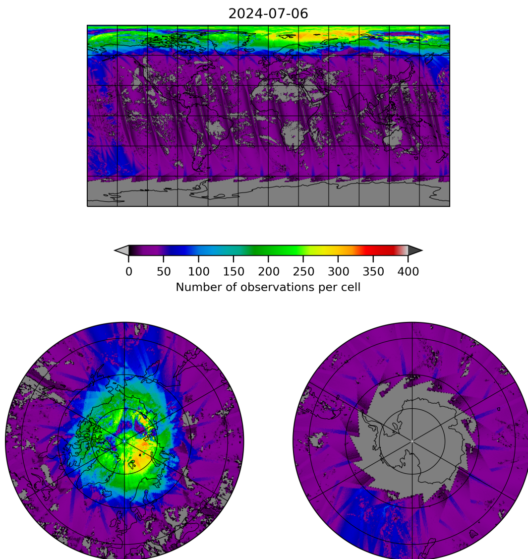
Figure 21: Map of the number of observations for 2024-07-05 to 2024-07-07
