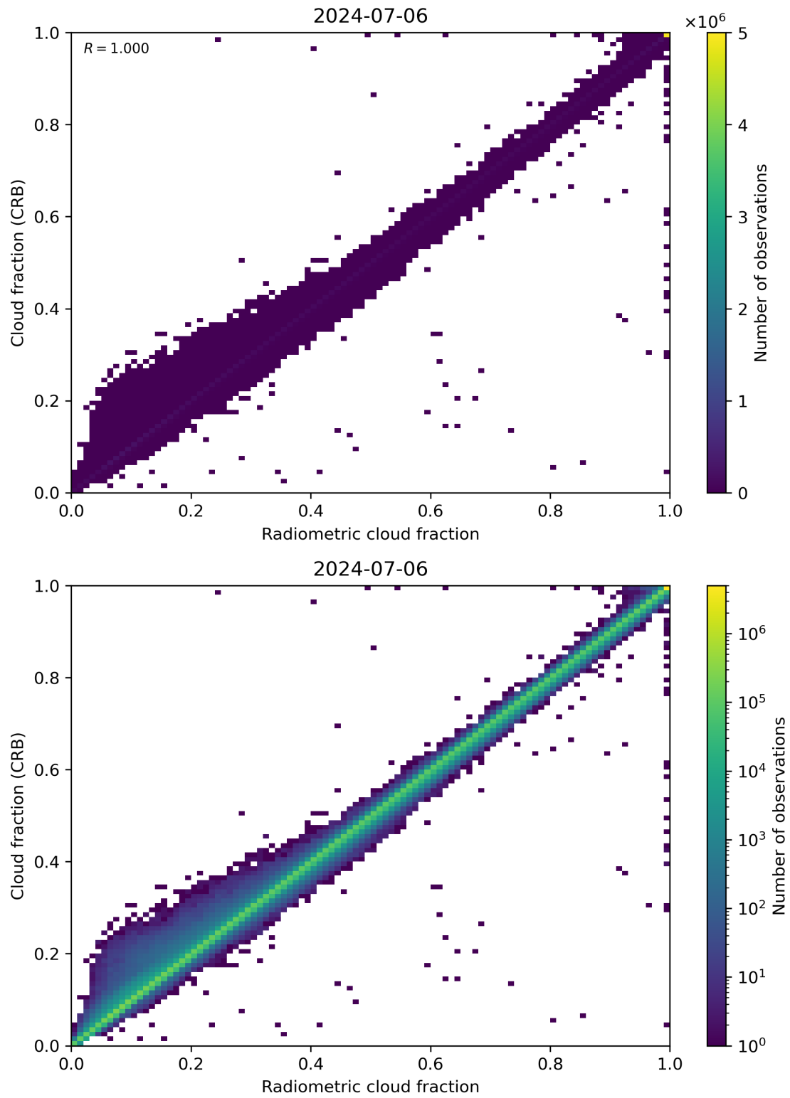
Figure 73: Scatter density plot of “Radiometric cloud fraction” against “Cloud fraction (CRB)” for 2024-07-05 to 2024-07-07.
