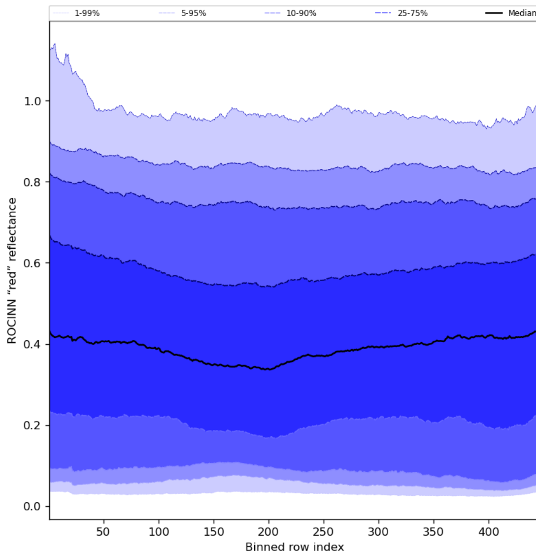
Figure 69: Along track statistics of “ROCINN “red” reflectance” for 2024-07-05 to 2024-07-07
