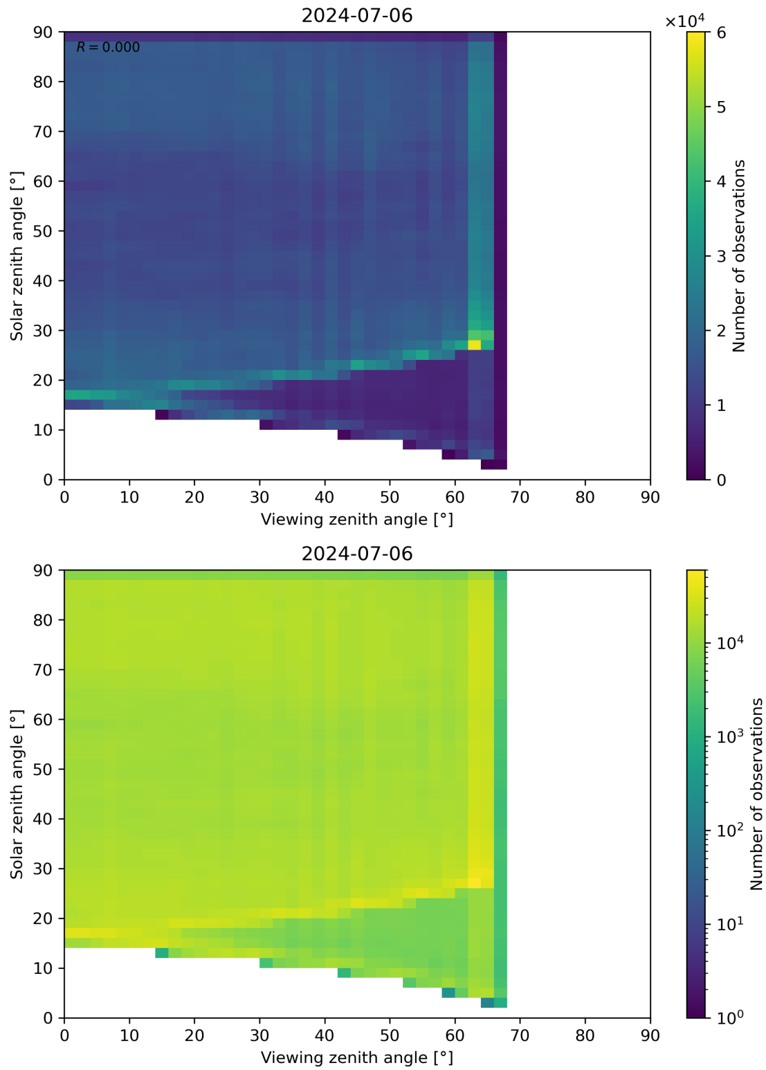
Figure 114: Scatter density plot of “Viewing zenith angle” against “Solar zenith angle” for 2024-07-05 to 2024-07-07.
