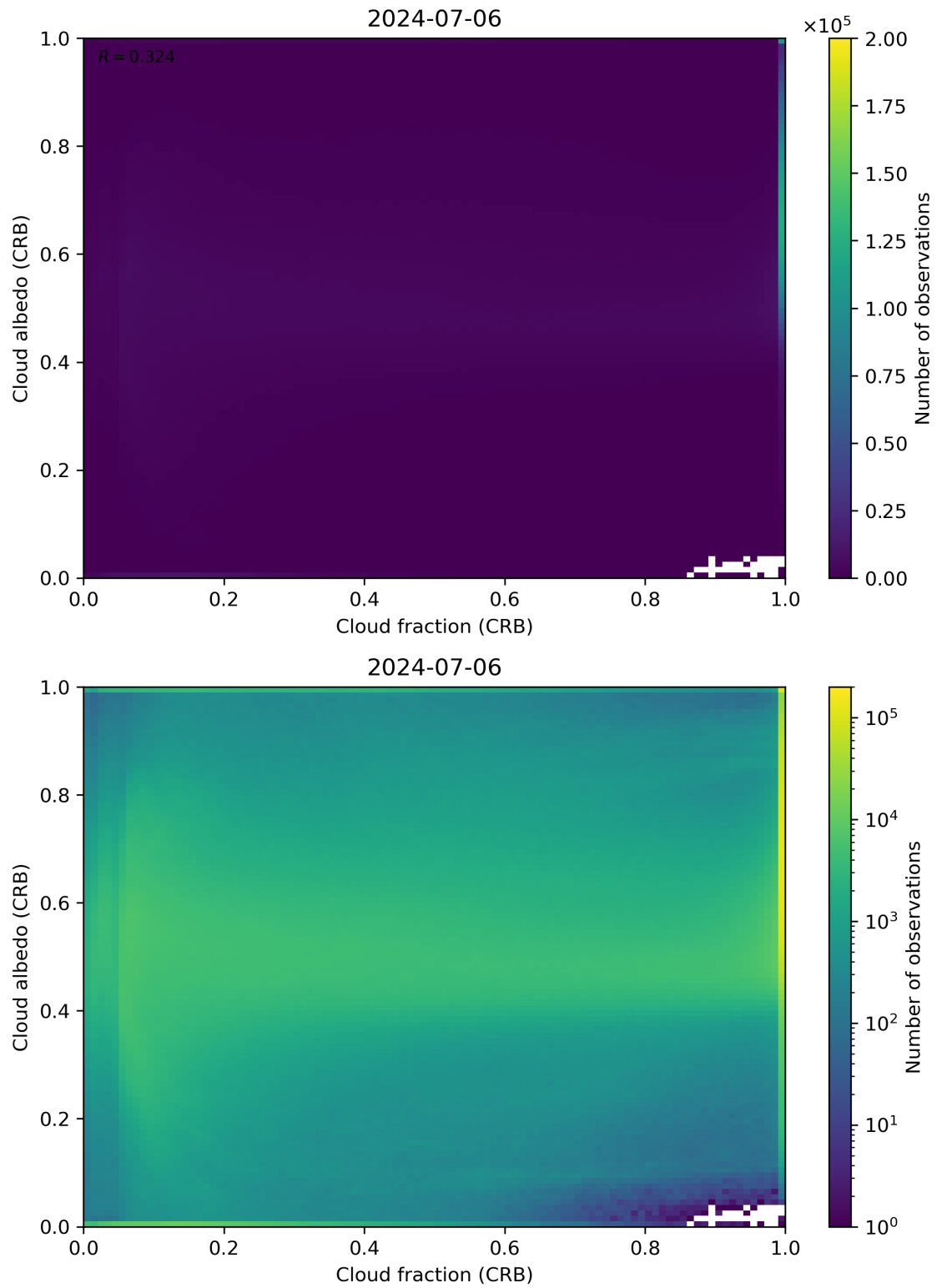
Figure 77: Scatter density plot of “Cloud fraction (CRB)” against “Cloud albedo (CRB)” for 2024-07-05 to 2024-07-07.
