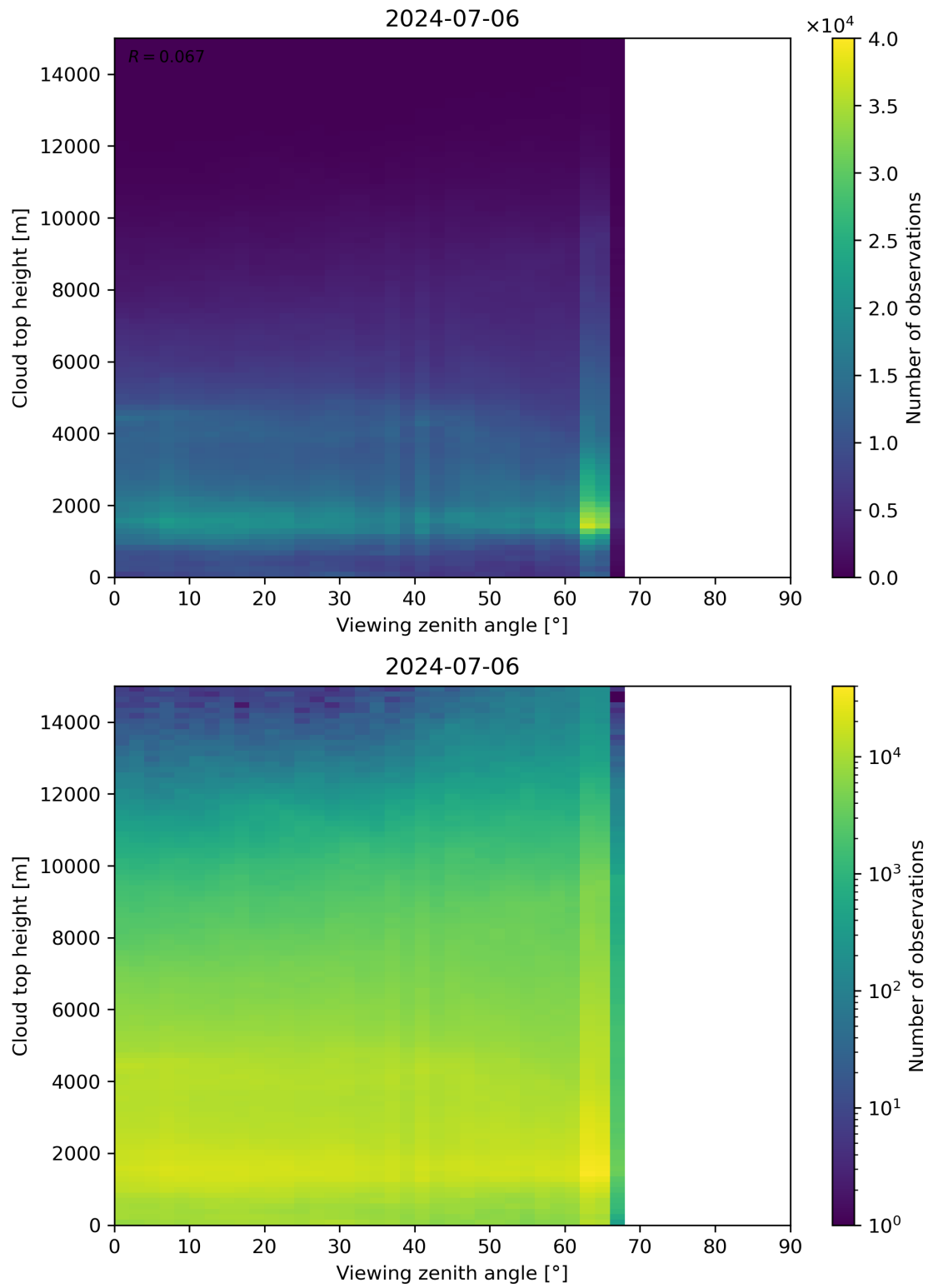
Figure 112: Scatter density plot of “Viewing zenith angle” against “Cloud top height” for 2024-07-05 to 2024-07-07.
