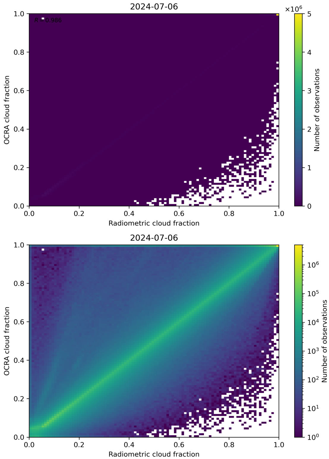
Figure 72: Scatter density plot of “Radiometric cloud fraction” against “OCRA cloud fraction” for 2024-07-05 to 2024-07-07.
