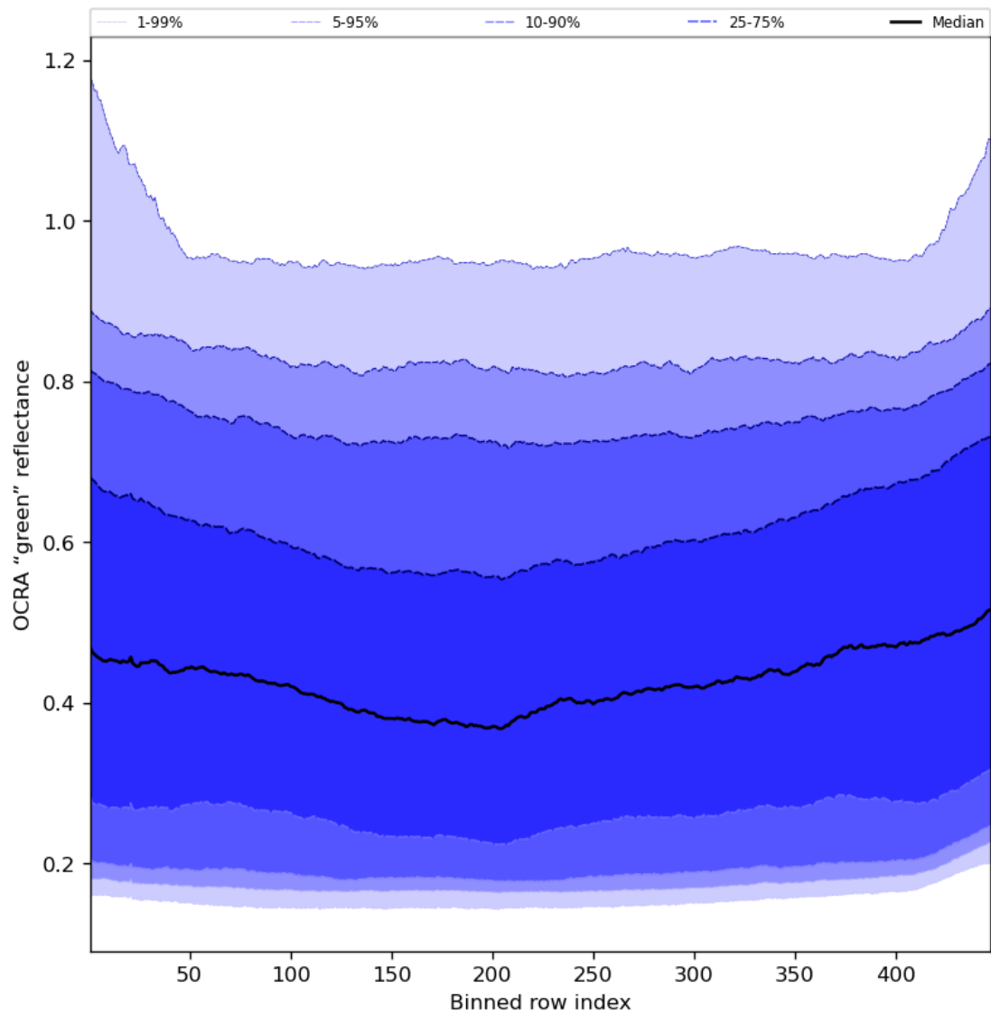
Figure 68: Along track statistics of “OCRA “green” reflectance” for 2024-07-05 to 2024-07-07
