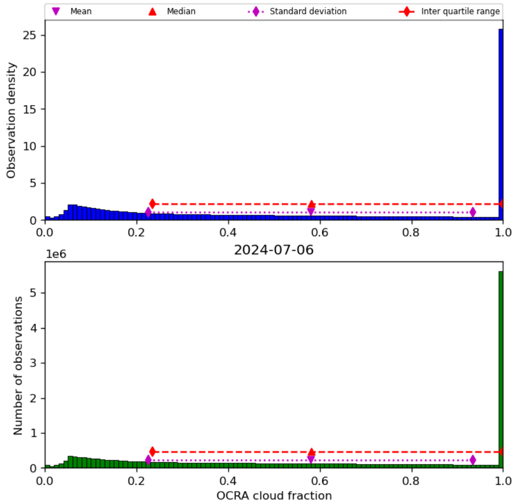
Figure 50: Histogram of “OCRA cloud fraction” for 2024-07-05 to 2024-07-07
