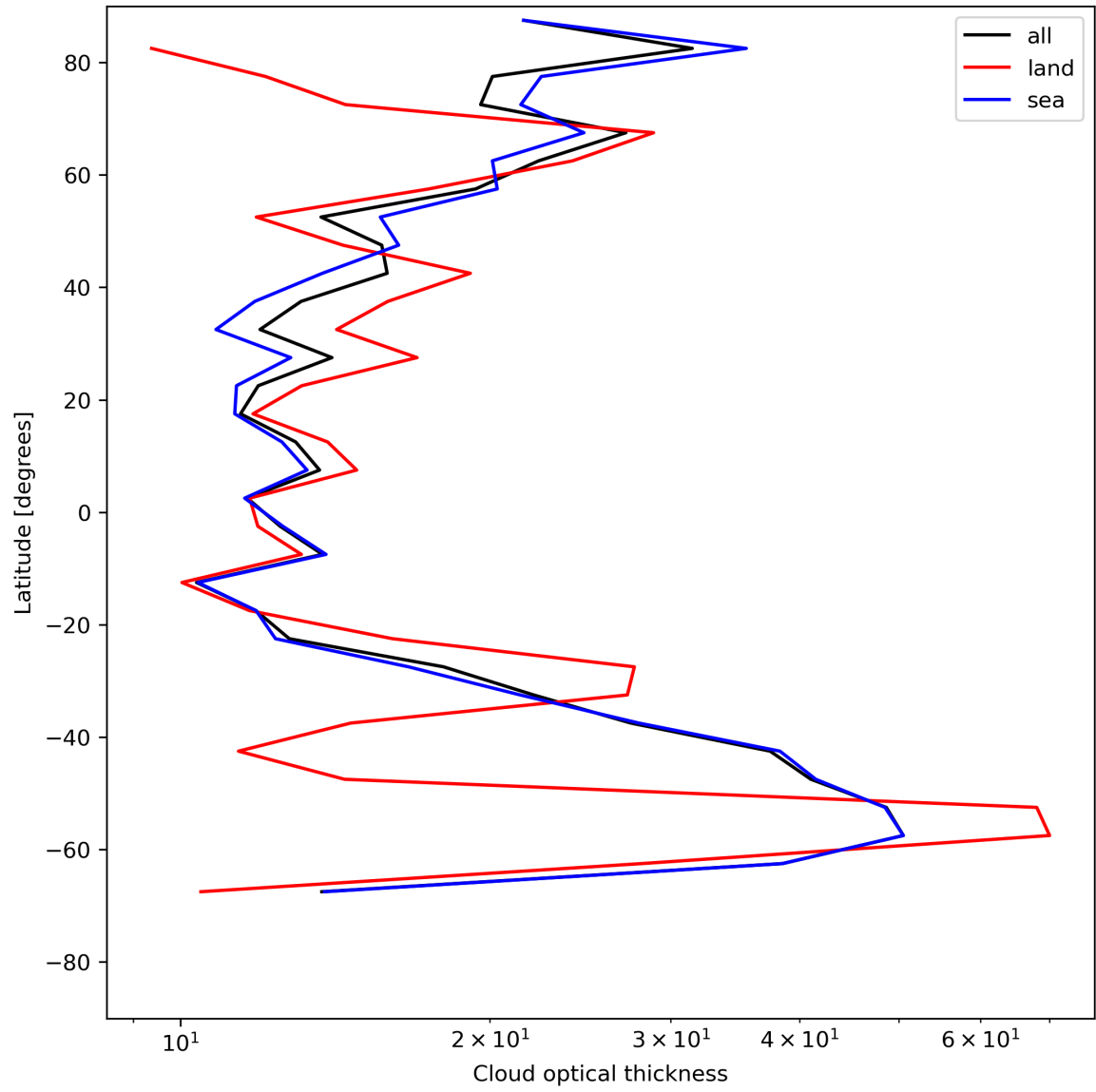
Figure 25: Zonal average of “Cloud optical thickness” for 2024-07-05 to 2024-07-07.
