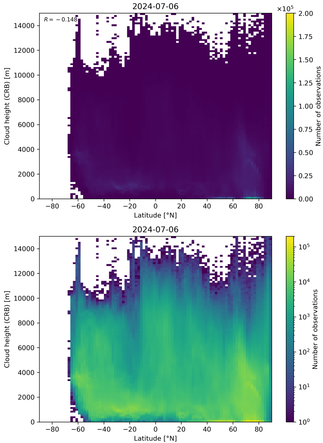
Figure 95: Scatter density plot of “Latitude” against “Cloud height (CRB)” for 2024-07-05 to 2024-07-07.
