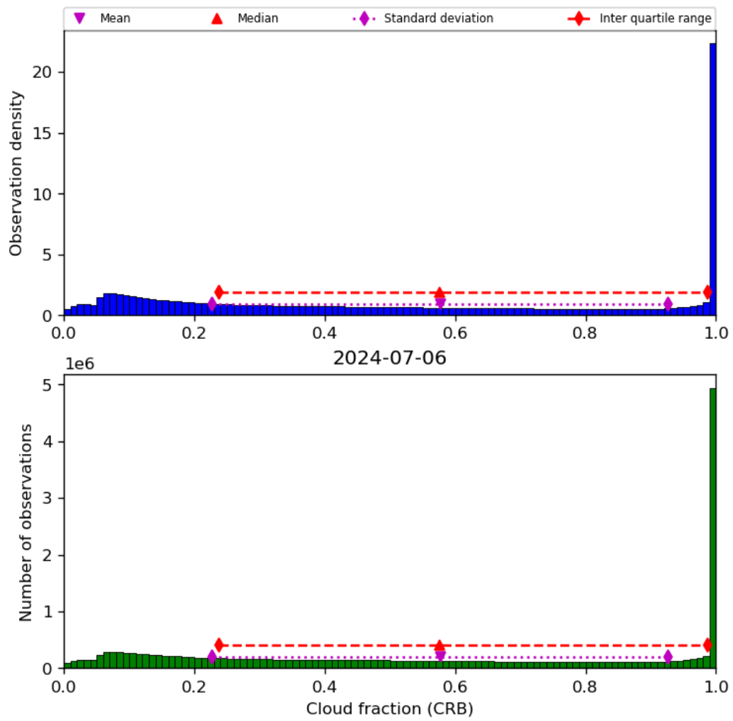
Figure 42: Histogram of “Cloud fraction (CRB)” for 2024-07-05 to 2024-07-07
