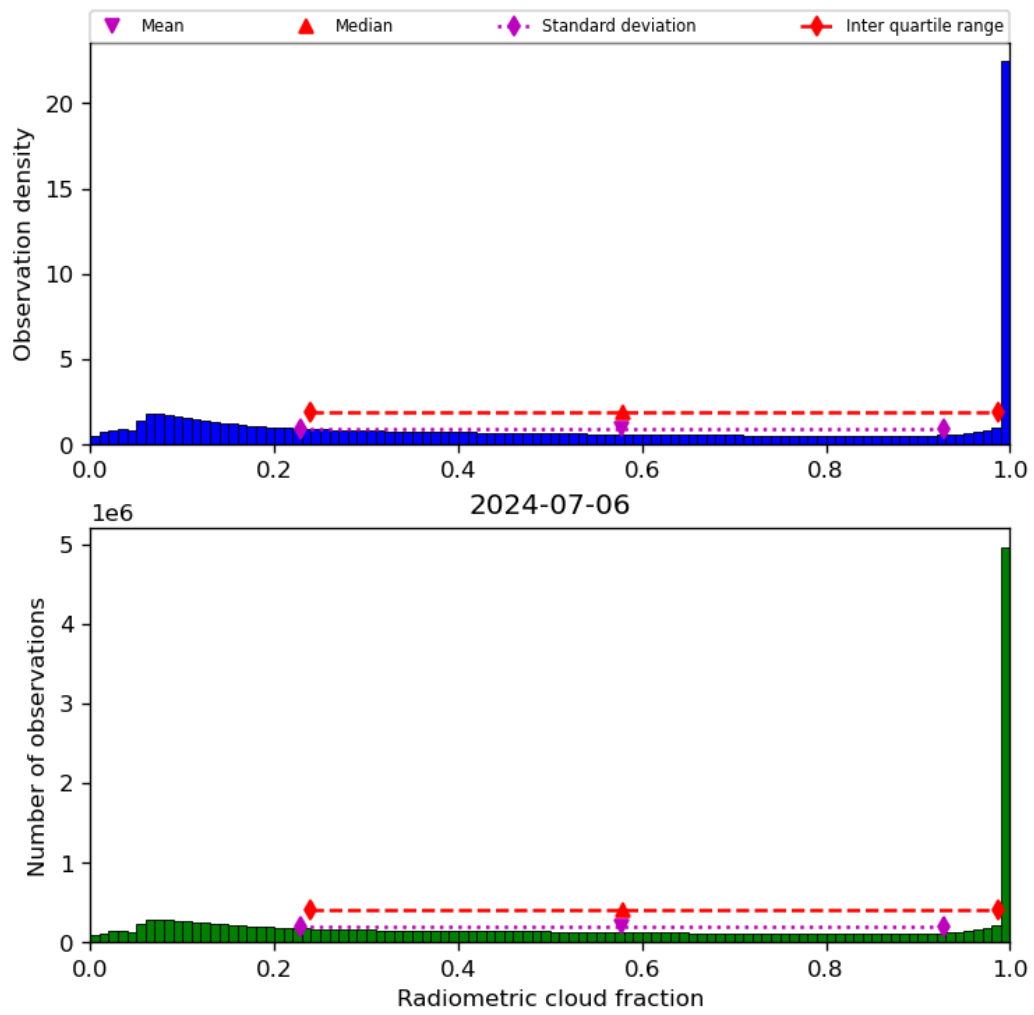
Figure 39: Histogram of “Radiometric cloud fraction” for 2024-07-05 to 2024-07-07
