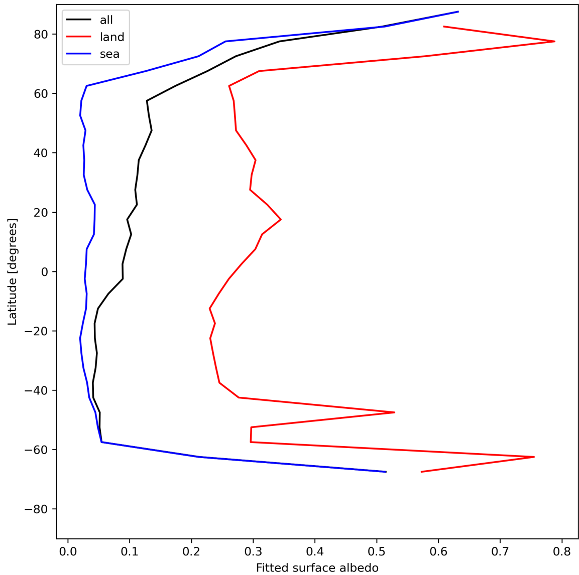
Figure 29: Zonal average of “Fitted surface albedo” for 2024-07-05 to 2024-07-07.
