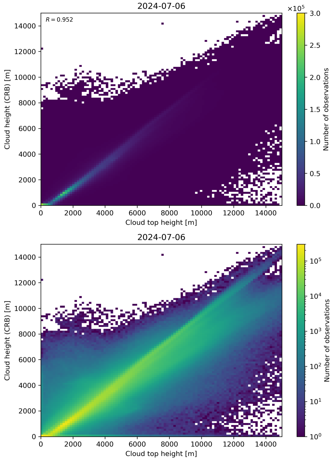
Figure 89: Scatter density plot of “Cloud top height” against “Cloud height (CRB)” for 2024-07-05 to 2024-07-07.
