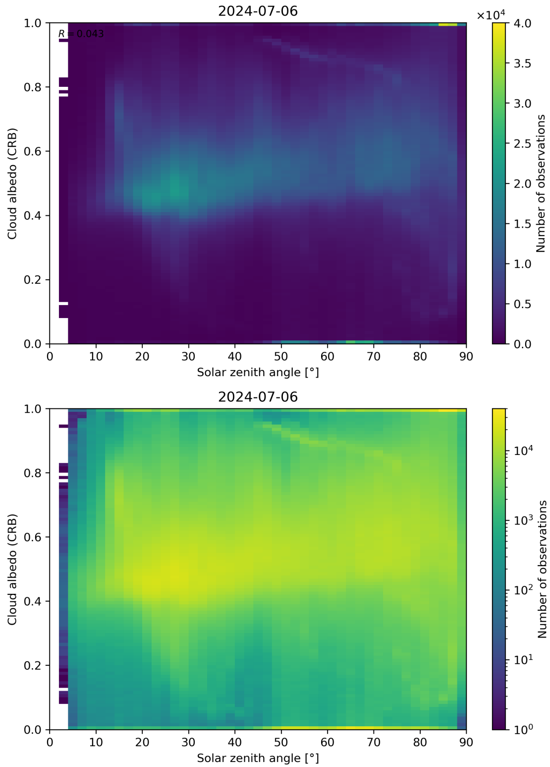
Figure 98: Scatter density plot of “Solar zenith angle” against “Cloud albedo (CRB)” for 2024-07-05 to 2024-07-07.
