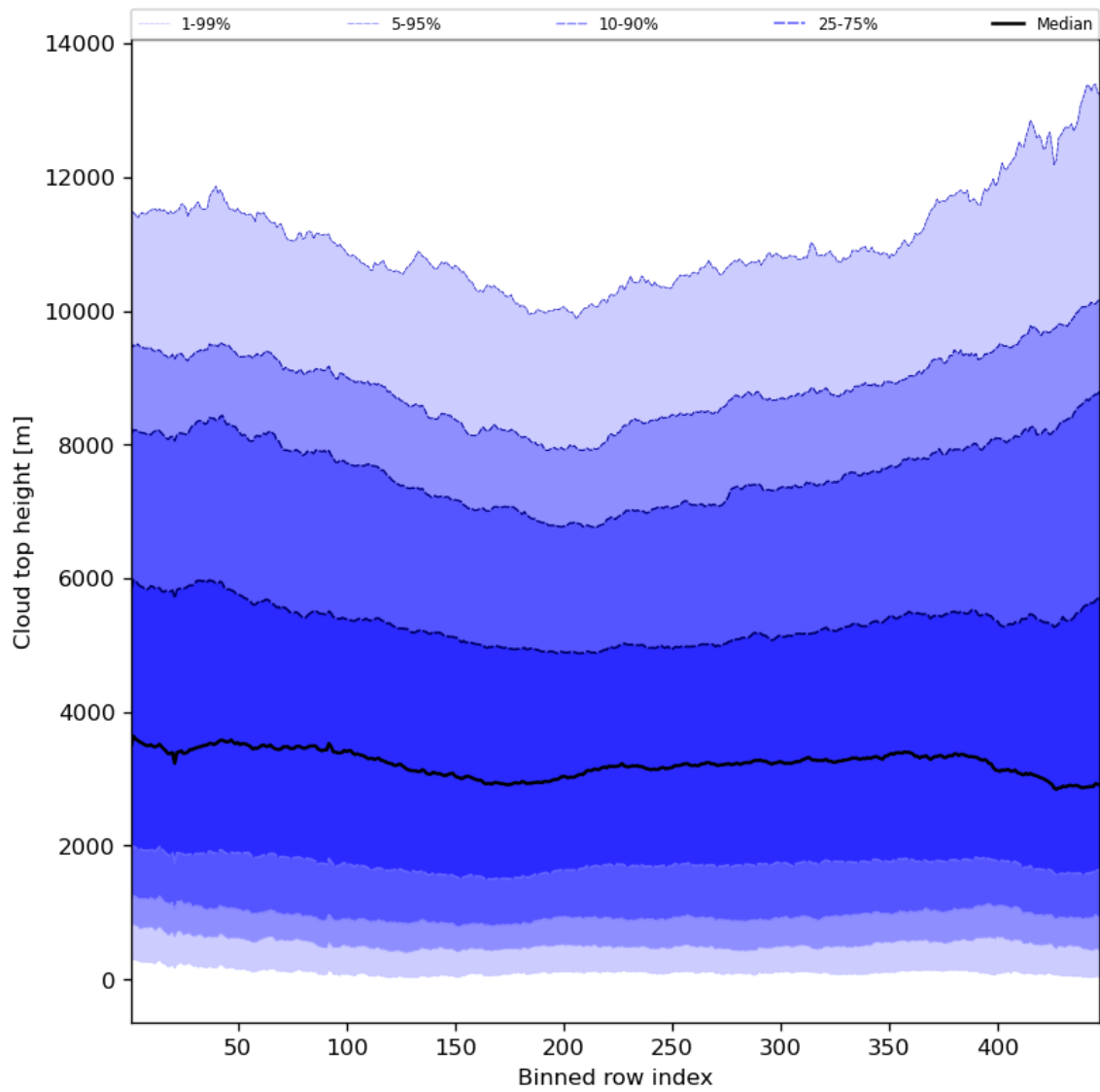
Figure 56: Along track statistics of “Cloud top height” for 2024-07-05 to 2024-07-07
