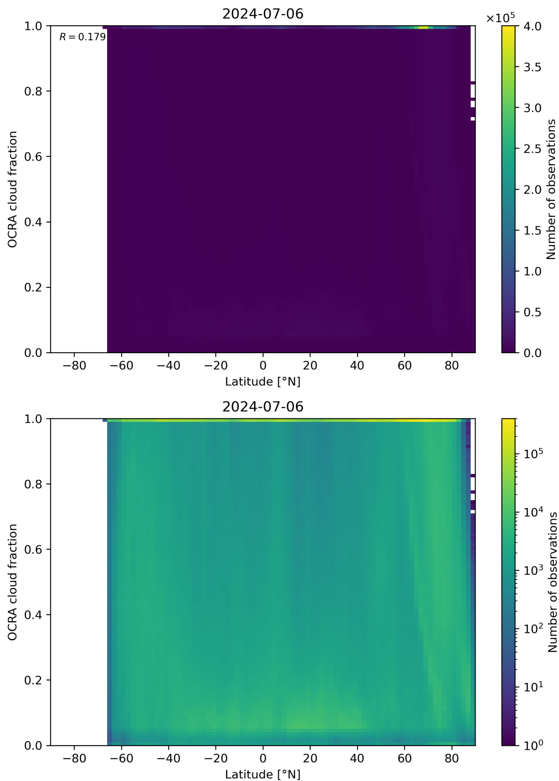
Figure 93: Scatter density plot of “Latitude” against “OCRA cloud fraction” for 2024-07-05 to 2024-07-07.
