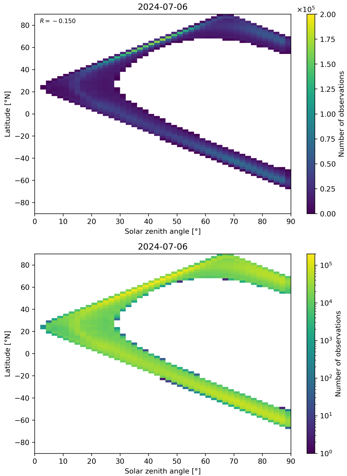
Figure 105: Scatter density plot of “Solar zenith angle” against “Latitude” for 2024-07-05 to 2024-07-07.
