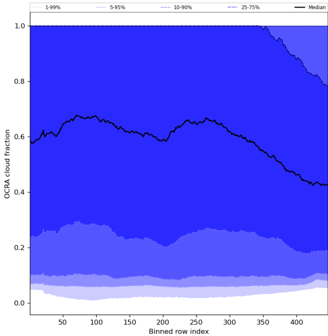
Figure 66: Along track statistics of “OCRA cloud fraction” for 2024-07-05 to 2024-07-07
