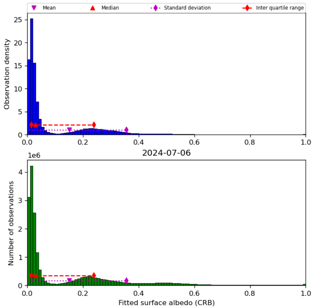
Figure 46: Histogram of “Fitted surface albedo (CRB)” for 2024-07-05 to 2024-07-07
