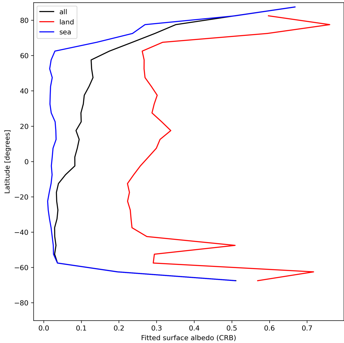
Figure 30: Zonal average of “Fitted surface albedo (CRB)” for 2024-07-05 to 2024-07-07.
