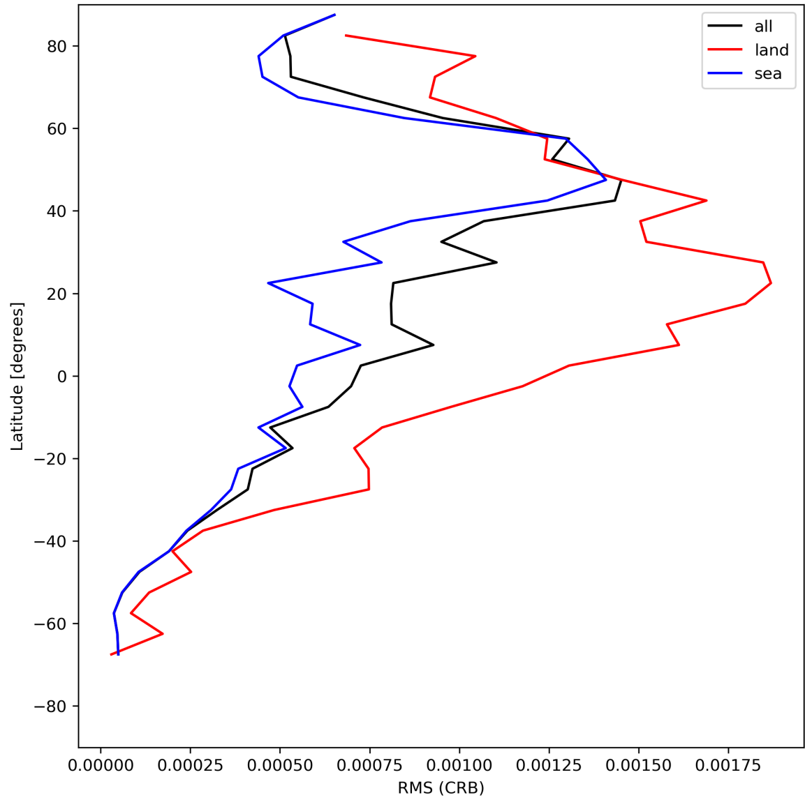
Figure 32: Zonal average of “RMS (CRB)” for 2024-07-05 to 2024-07-07.
