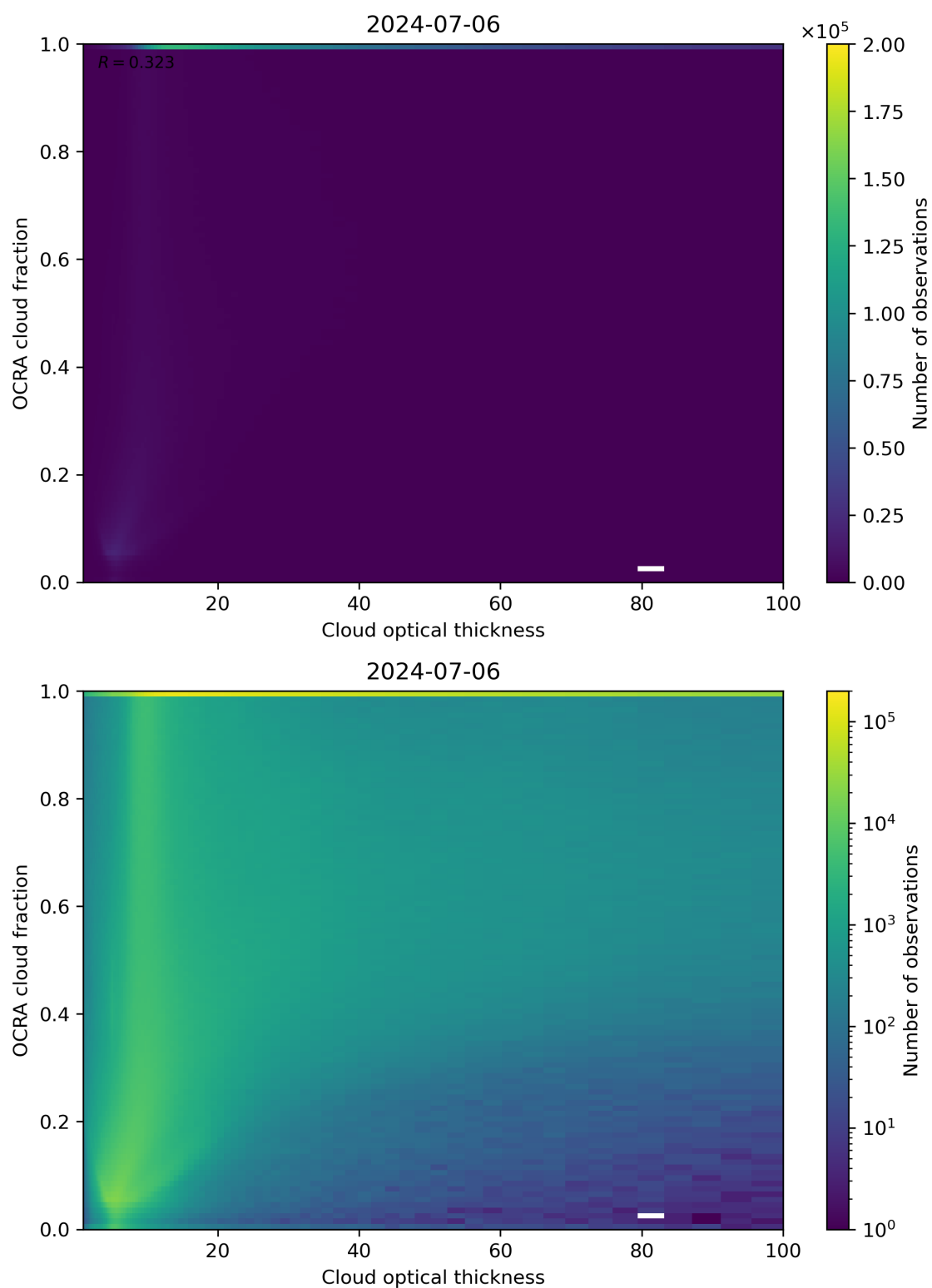
Figure 83: Scatter density plot of “Cloud optical thickness” against “OCRA cloud fraction” for 2024-07-05 to 2024-07-07.
