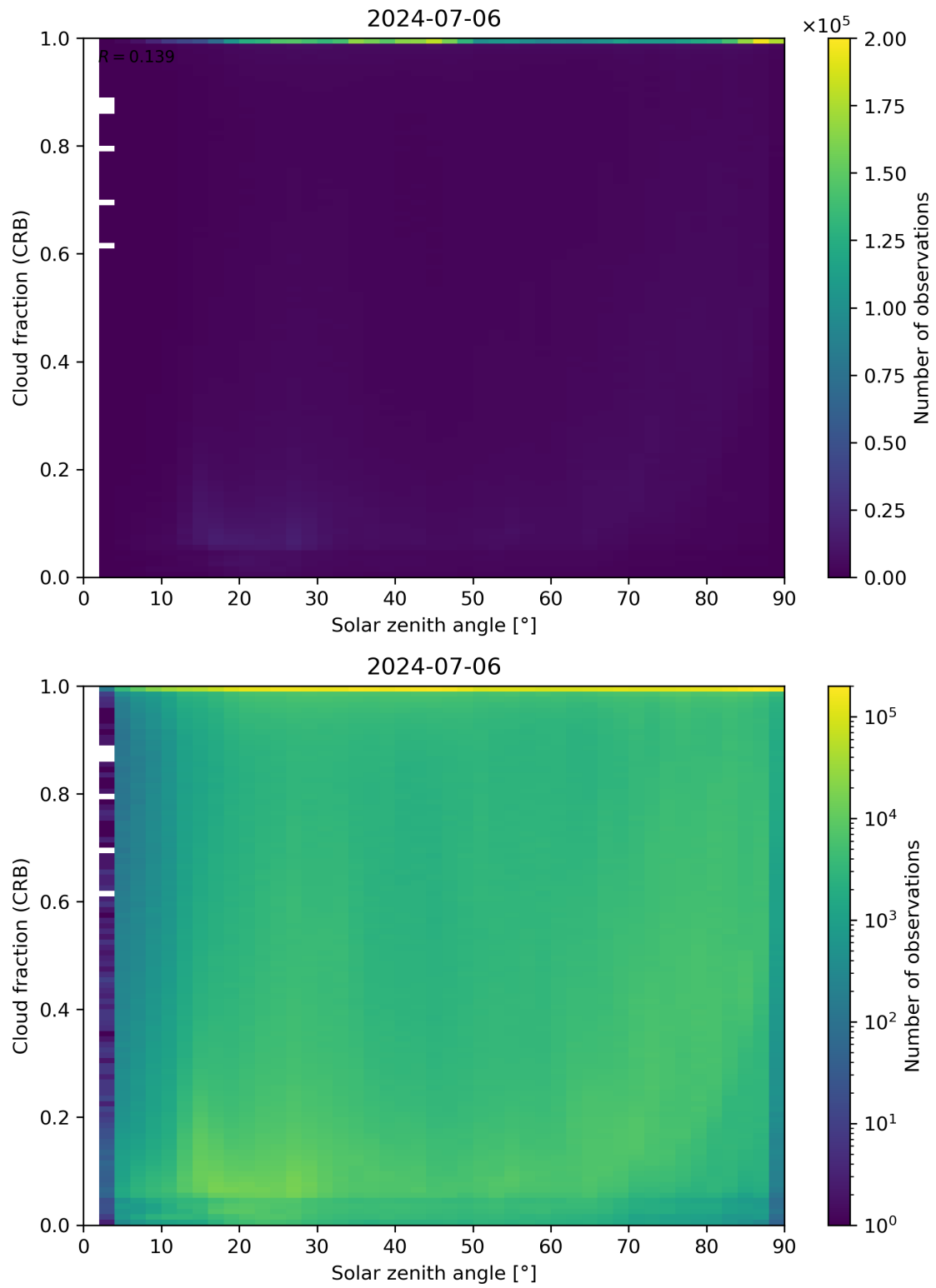
Figure 101: Scatter density plot of “Solar zenith angle” against “Cloud fraction (CRB)” for 2024-07-05 to 2024-07-07.
