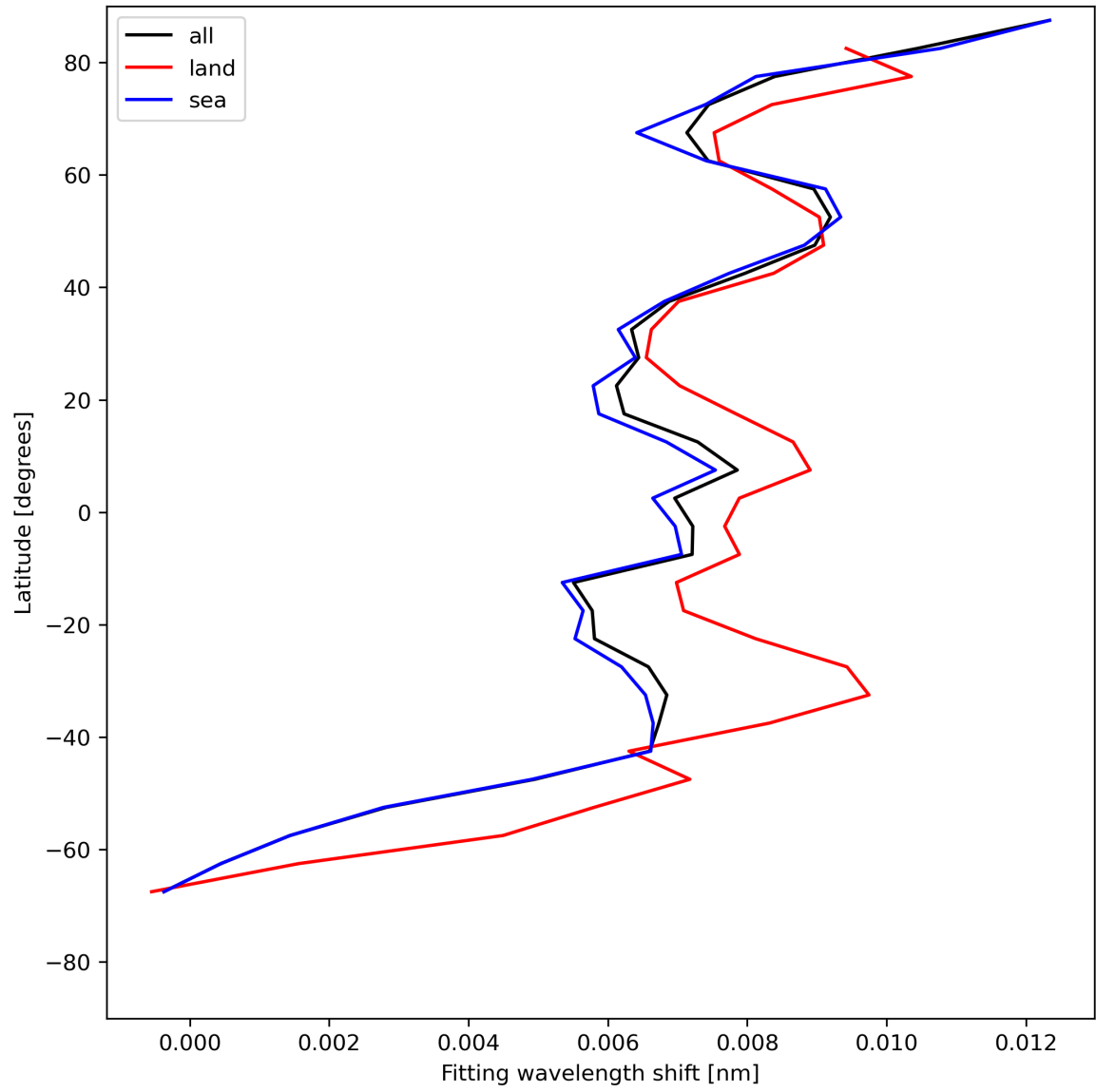
Figure 33: Zonal average of “Fitting wavelength shift” for 2024-07-05 to 2024-07-07.
