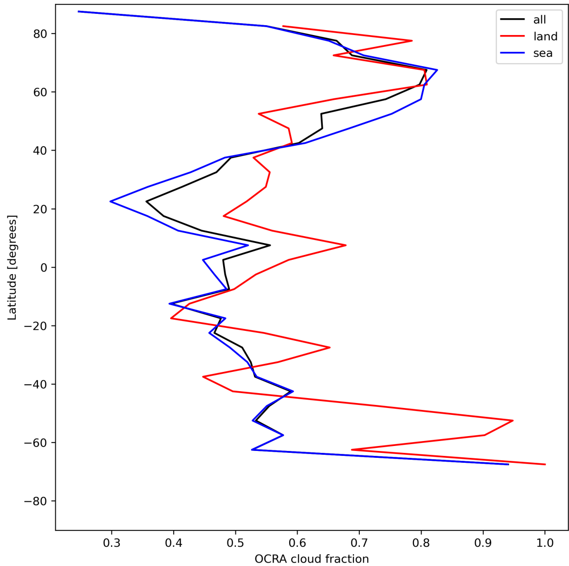
Figure 34: Zonal average of “OCRA cloud fraction” for 2024-07-05 to 2024-07-07.
