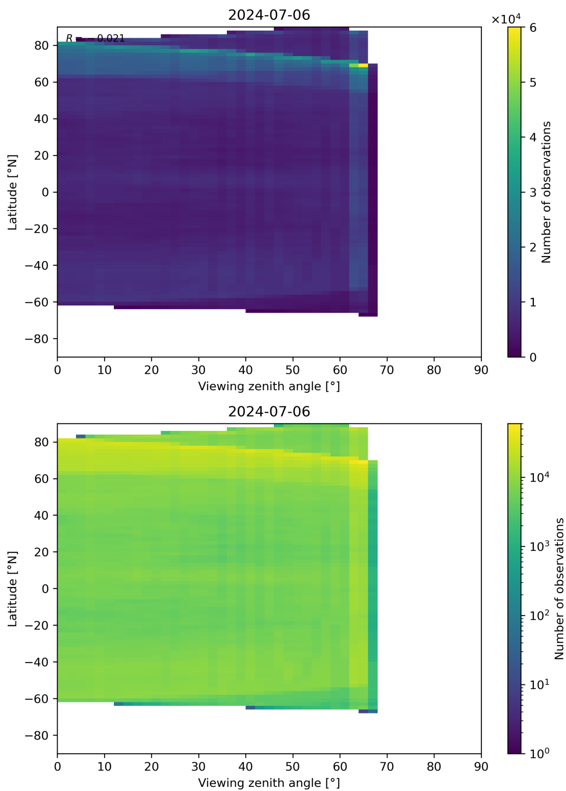
Figure 113: Scatter density plot of “Viewing zenith angle” against “Latitude” for 2024-07-05 to 2024-07-07.
