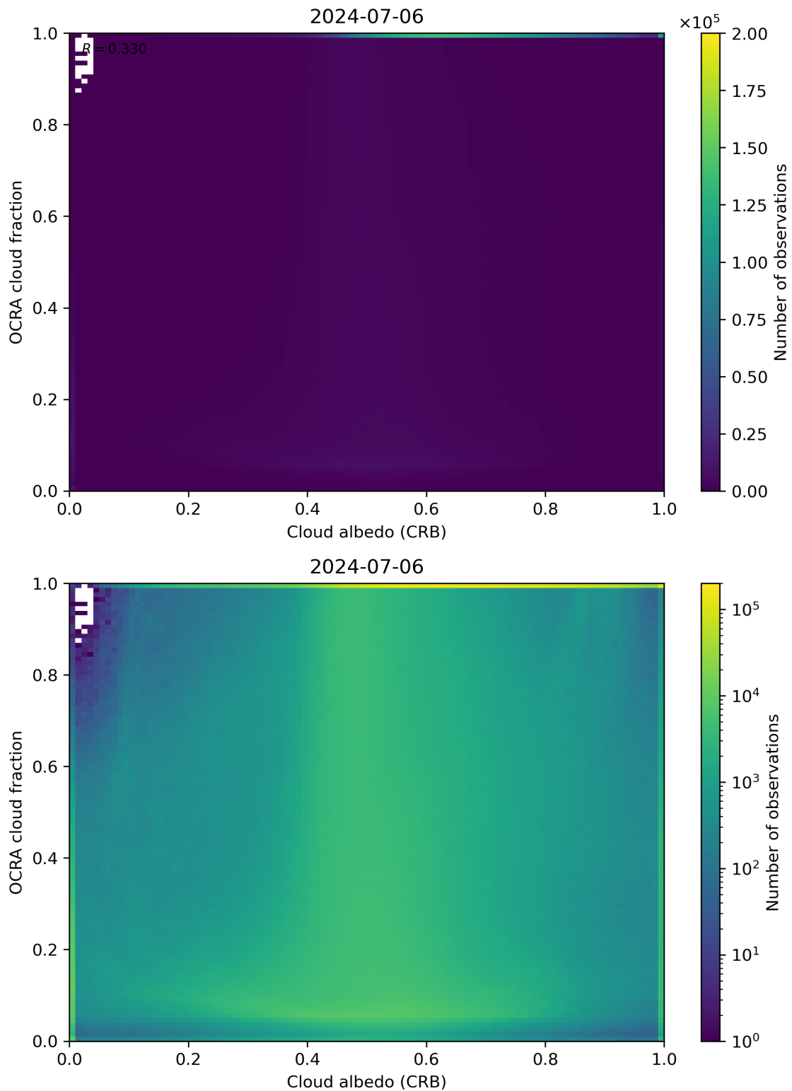
Figure 70: Scatter density plot of “Cloud albedo (CRB)” against “OCRA cloud fraction” for 2024-07-05 to 2024-07-07.
