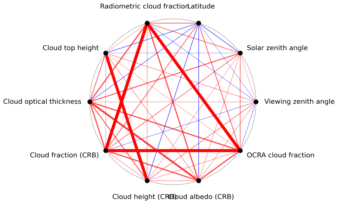
Figure 1: Map of correlation graph for 2024-07-05 to 2024-07-07.
