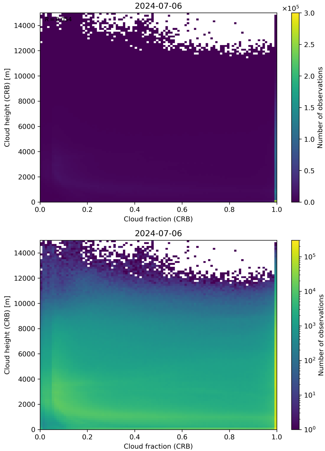
Figure 79: Scatter density plot of “Cloud fraction (CRB)” against “Cloud height (CRB)” for 2024-07-05 to 2024-07-07.
