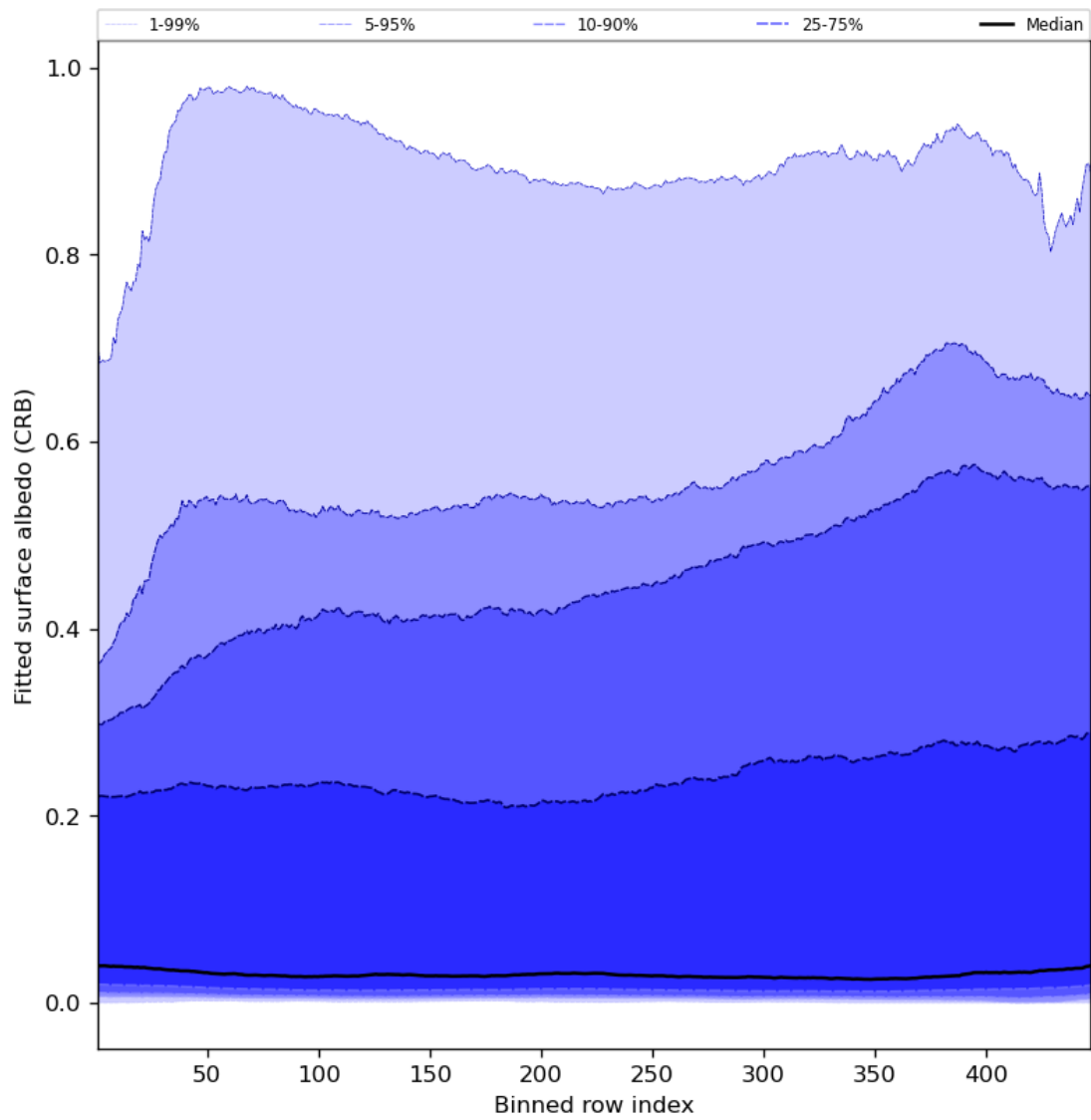
Figure 62: Along track statistics of “Fitted surface albedo (CRB)” for 2024-07-05 to 2024-07-07
