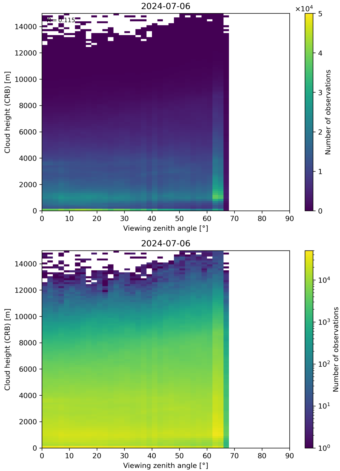
Figure 110: Scatter density plot of “Viewing zenith angle” against “Cloud height (CRB)” for 2024-07-05 to 2024-07-07.
