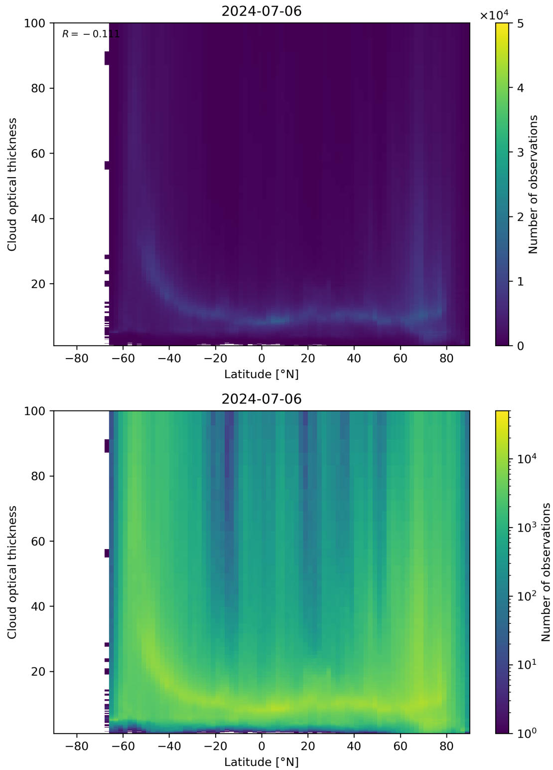
Figure 96: Scatter density plot of “Latitude” against “Cloud optical thickness” for 2024-07-05 to 2024-07-07.
