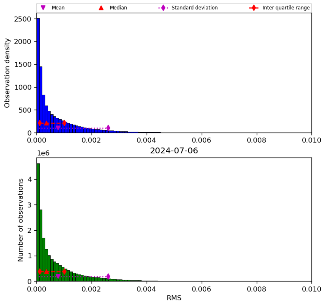
Figure 47: Histogram of “RMS” for 2024-07-05 to 2024-07-07
