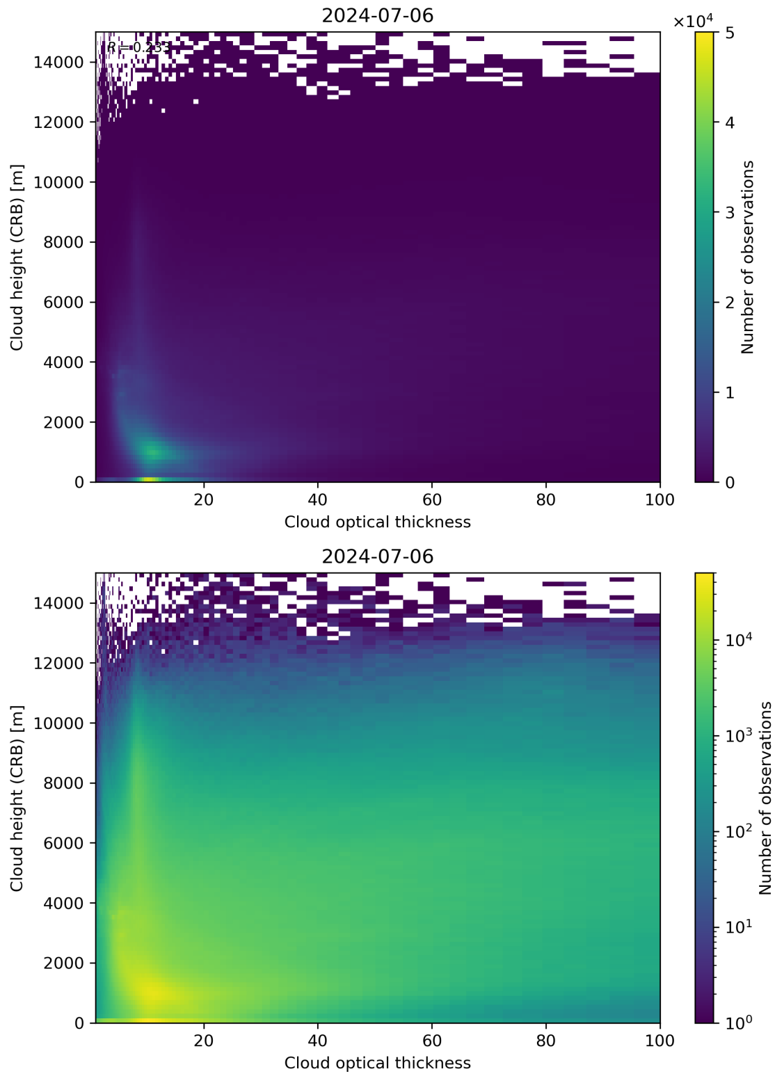
Figure 85: Scatter density plot of “Cloud optical thickness” against “Cloud height (CRB)” for 2024-07-05 to 2024-07-07.
