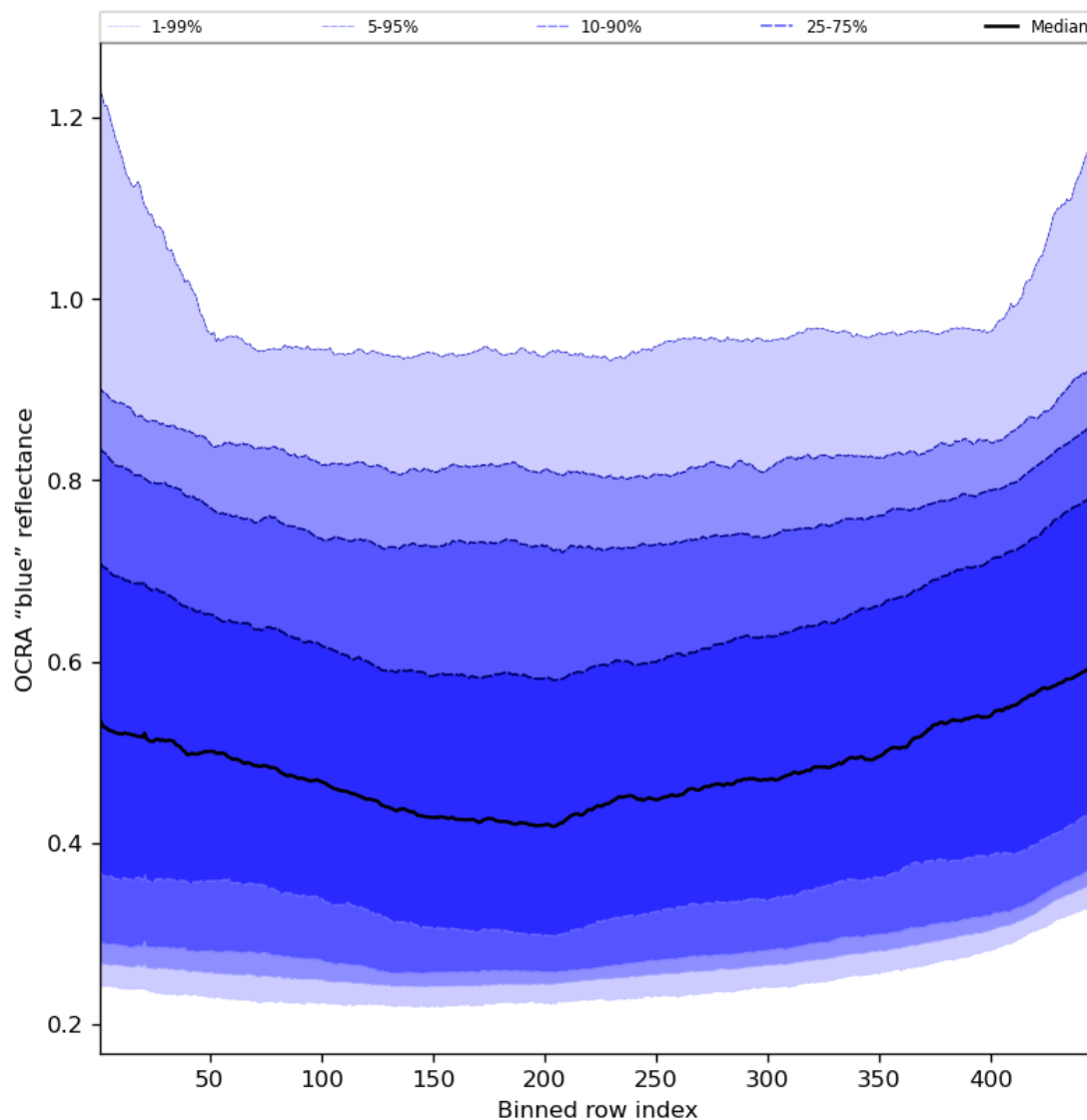
Figure 67: Along track statistics of “OCRA “blue” reflectance” for 2024-07-05 to 2024-07-07
