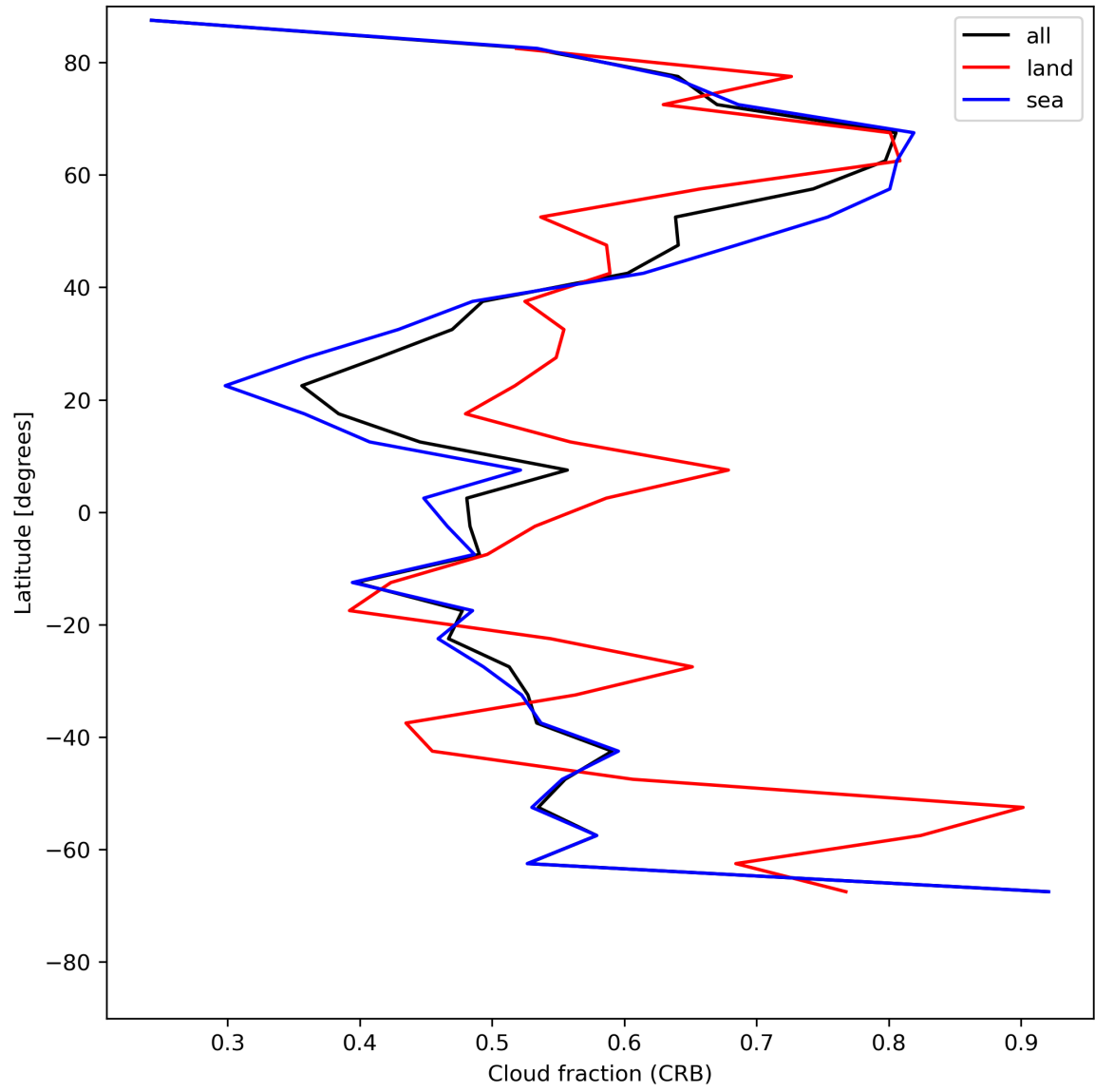
Figure 26: Zonal average of “Cloud fraction (CRB)” for 2024-07-05 to 2024-07-07.
