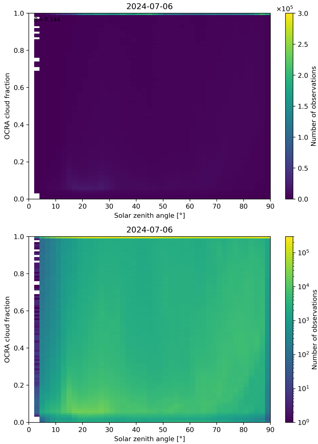
Figure 100: Scatter density plot of “Solar zenith angle” against “OCRA cloud fraction” for 2024-07-05 to 2024-07-07.
