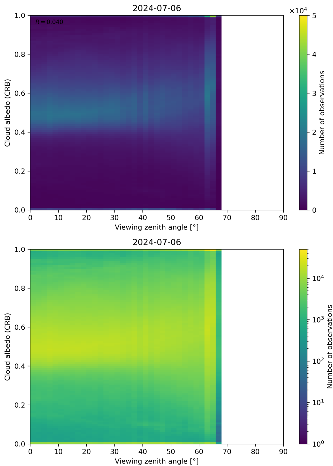
Figure 106: Scatter density plot of “Viewing zenith angle” against “Cloud albedo (CRB)” for 2024-07-05 to 2024-07-07.
