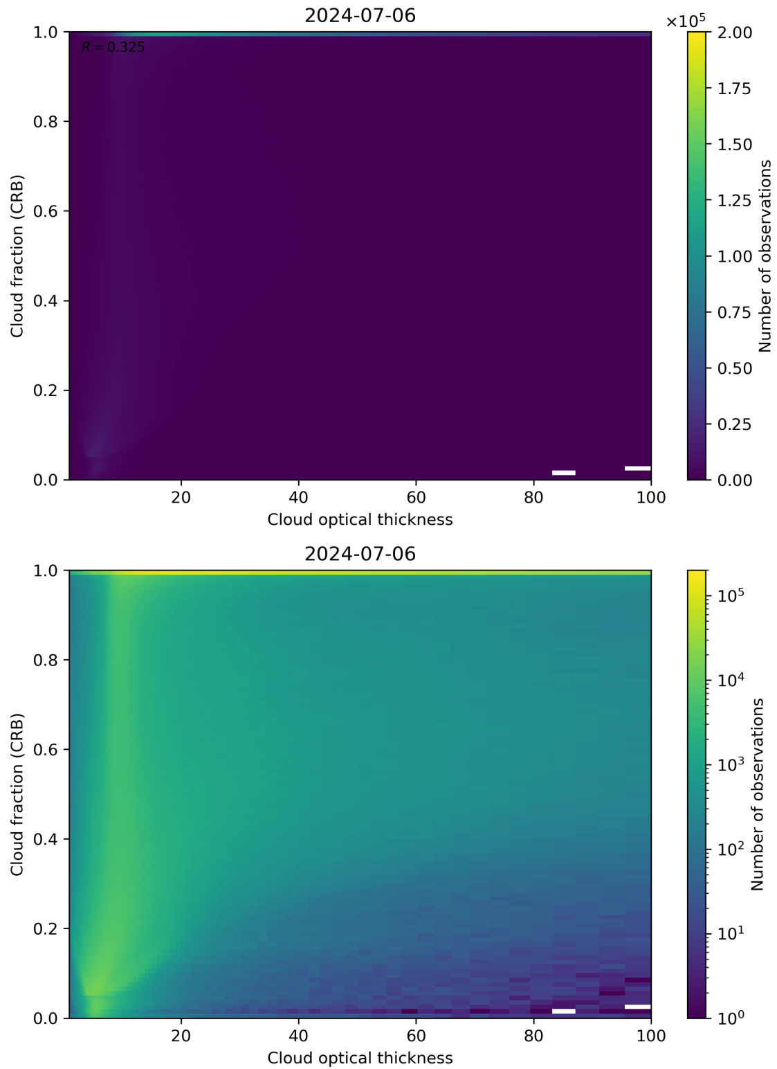
Figure 84: Scatter density plot of “Cloud optical thickness” against “Cloud fraction (CRB)” for 2024-07-05 to 2024-07-07.
