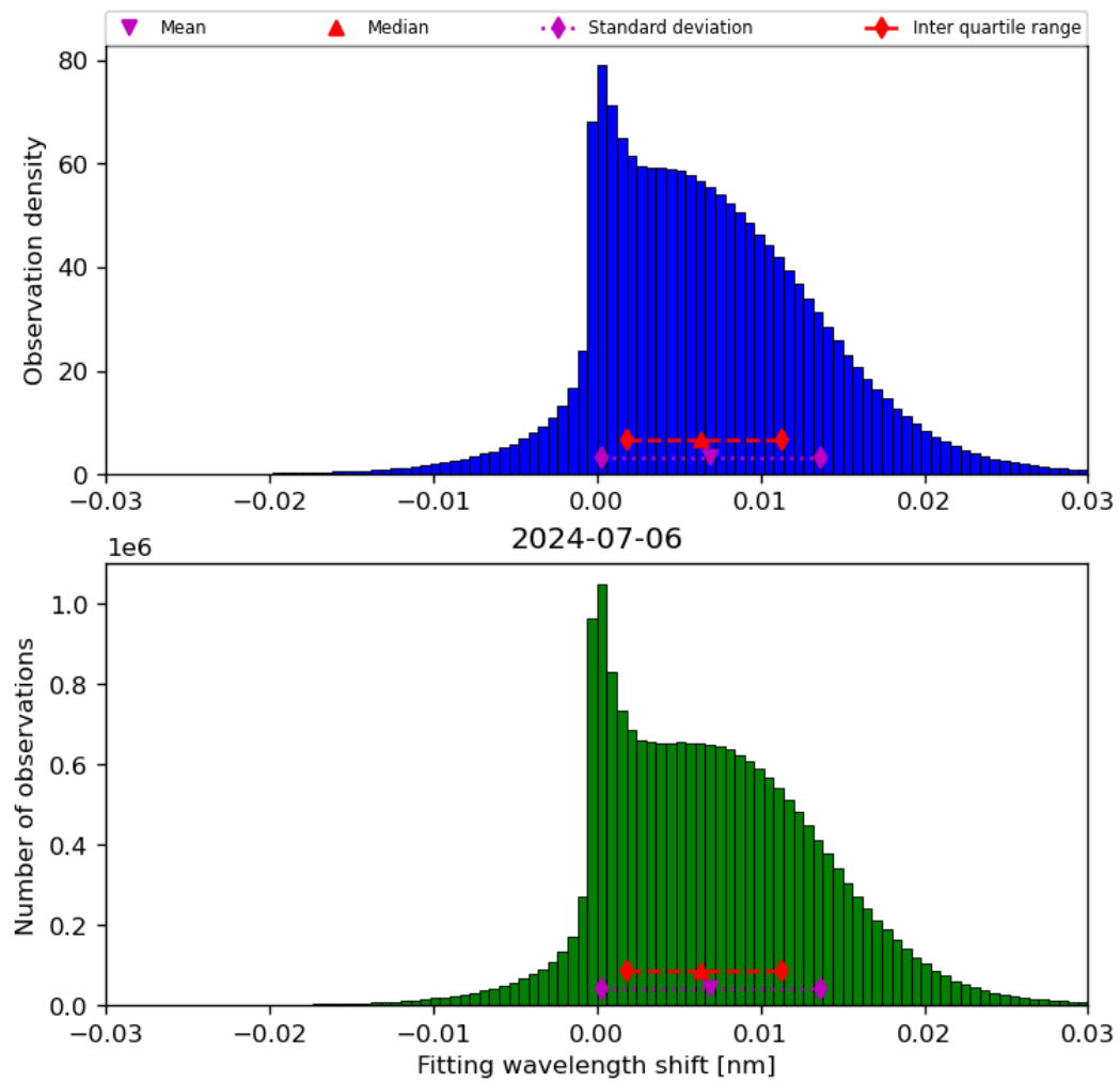
Figure 49: Histogram of “Fitting wavelength shift” for 2024-07-05 to 2024-07-07
