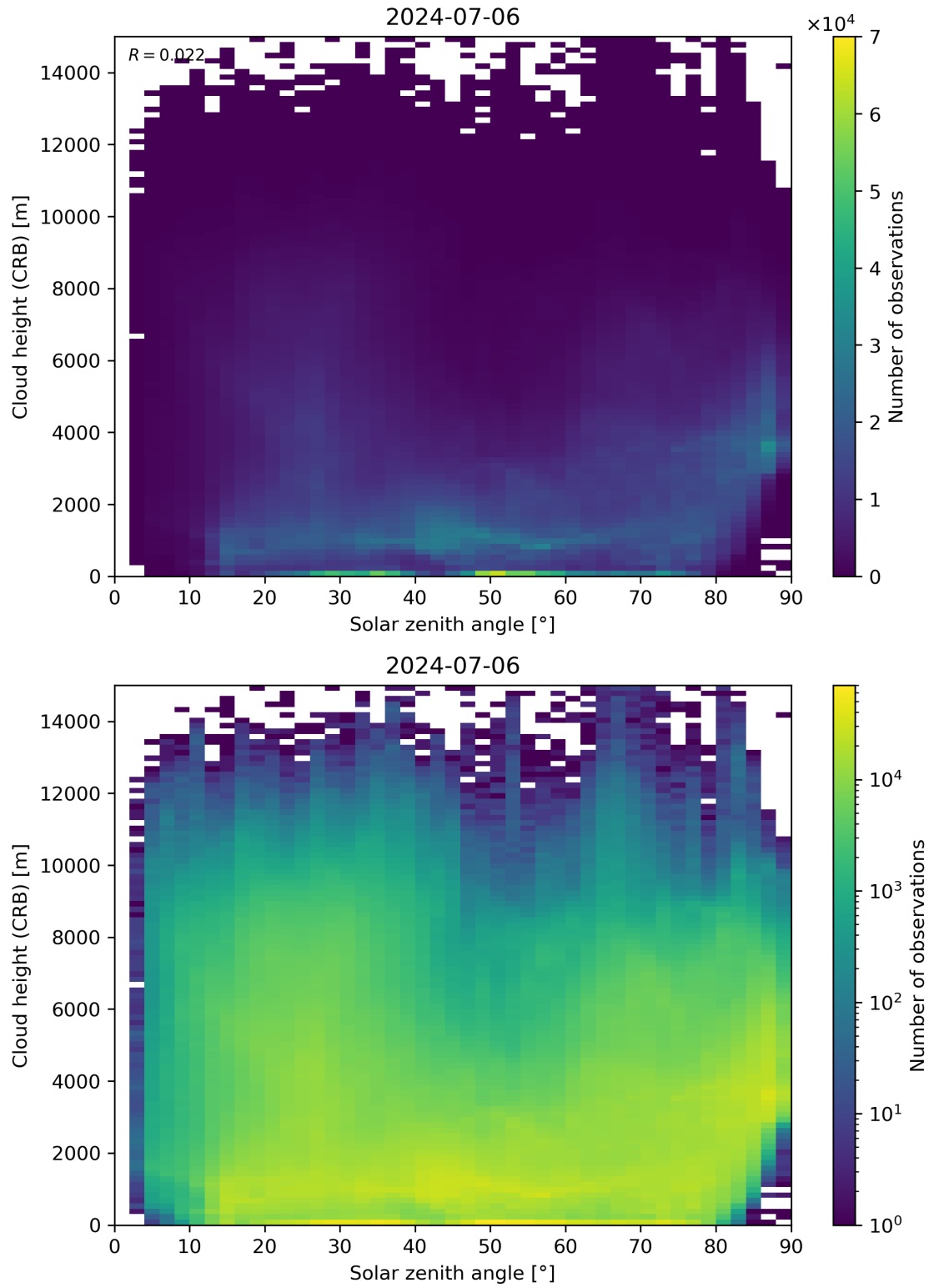
Figure 102: Scatter density plot of “Solar zenith angle” against “Cloud height (CRB)” for 2024-07-05 to 2024-07-07.
