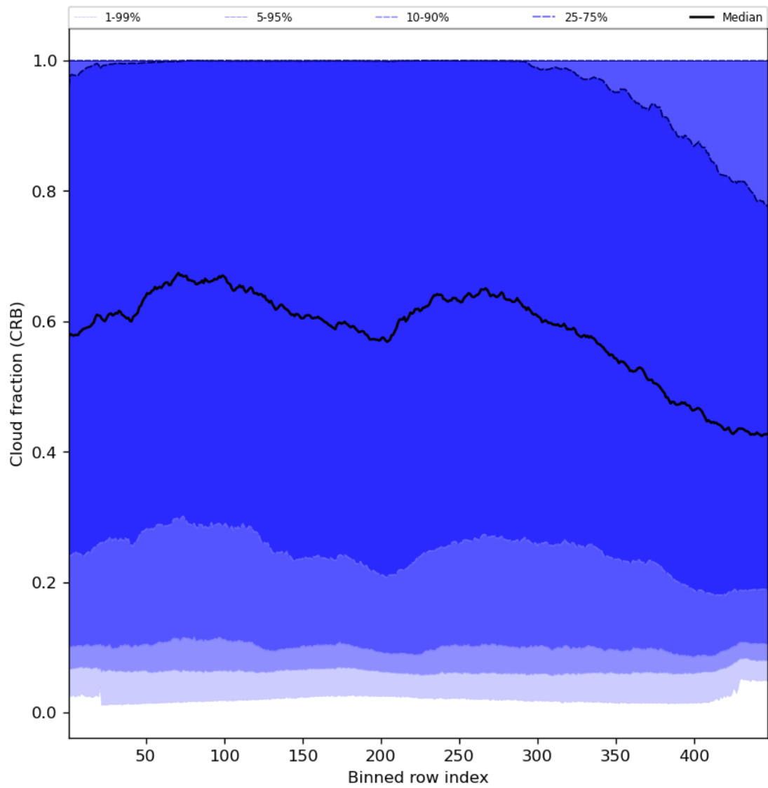
Figure 58: Along track statistics of “Cloud fraction (CRB)” for 2024-07-05 to 2024-07-07
