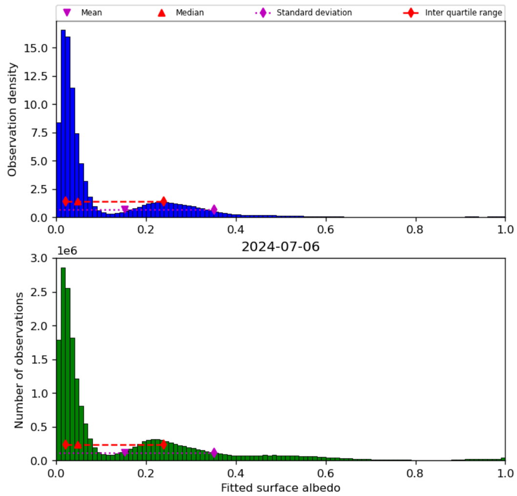
Figure 45: Histogram of “Fitted surface albedo” for 2024-07-05 to 2024-07-07
