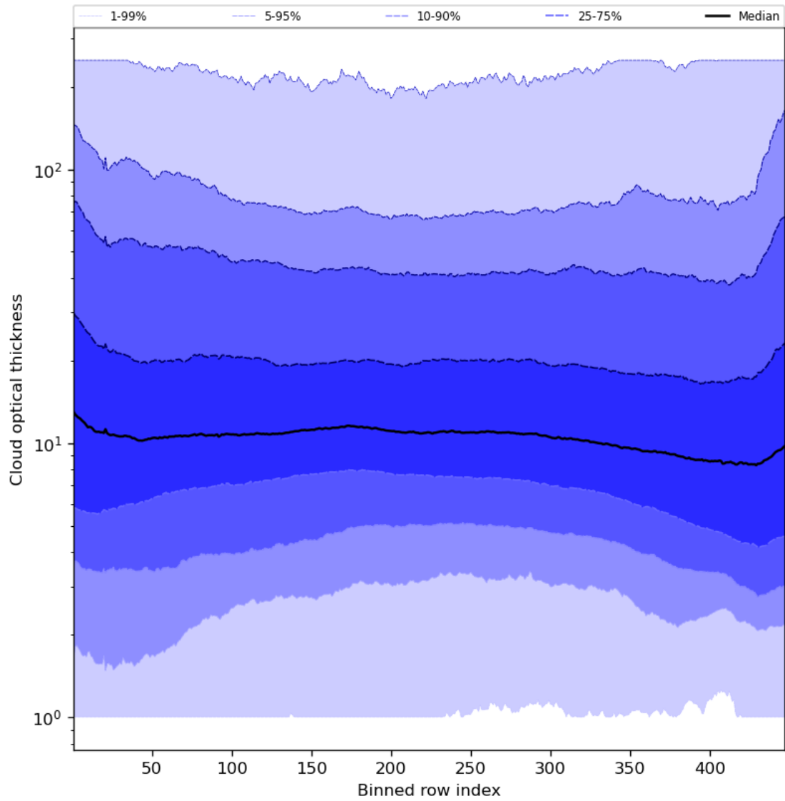
Figure 57: Along track statistics of “Cloud optical thickness” for 2024-07-05 to 2024-07-07
