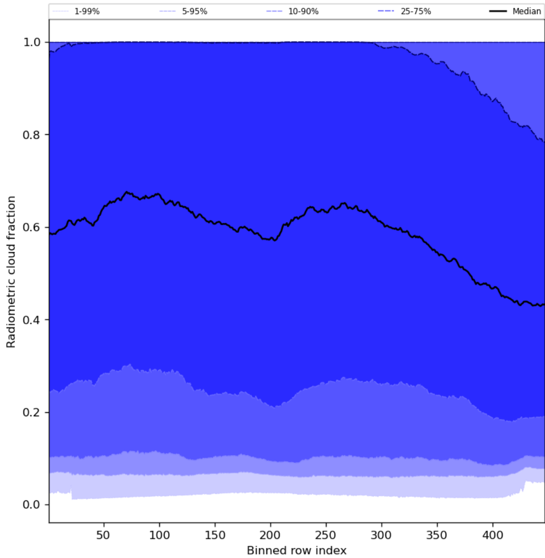
Figure 55: Along track statistics of “Radiometric cloud fraction” for 2024-07-05 to 2024-07-07
