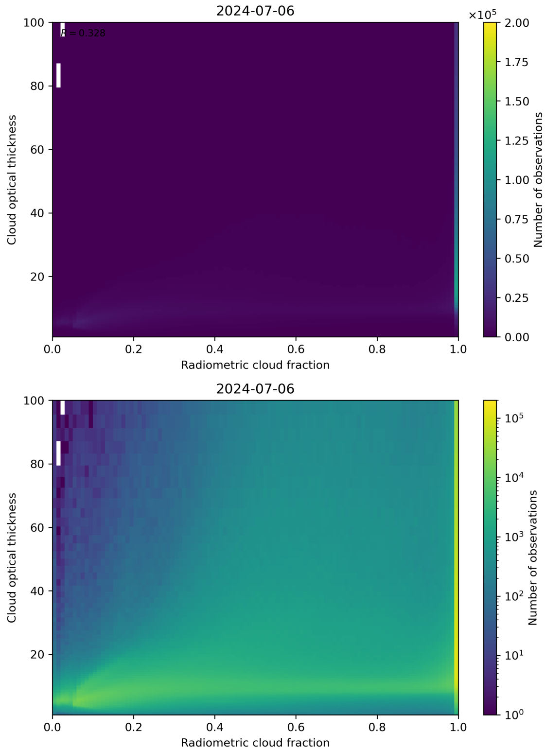
Figure 75: Scatter density plot of “Radiometric cloud fraction” against “Cloud optical thickness” for 2024-07-05 to 2024-07-07.
