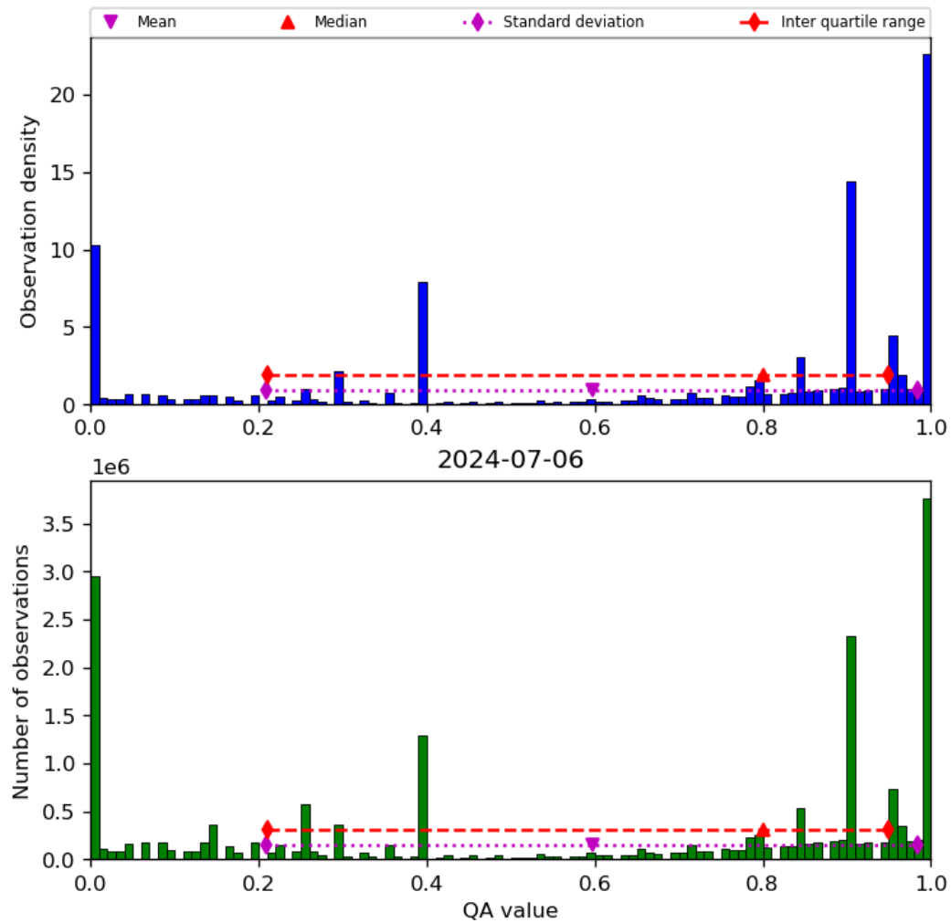
Figure 38: Histogram of “QA value” for 2024-07-05 to 2024-07-07
