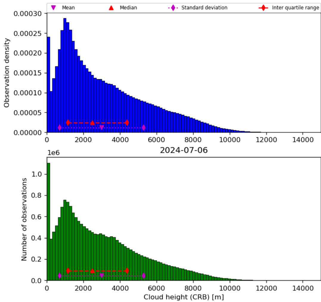
Figure 43: Histogram of “Cloud height (CRB)” for 2024-07-05 to 2024-07-07
