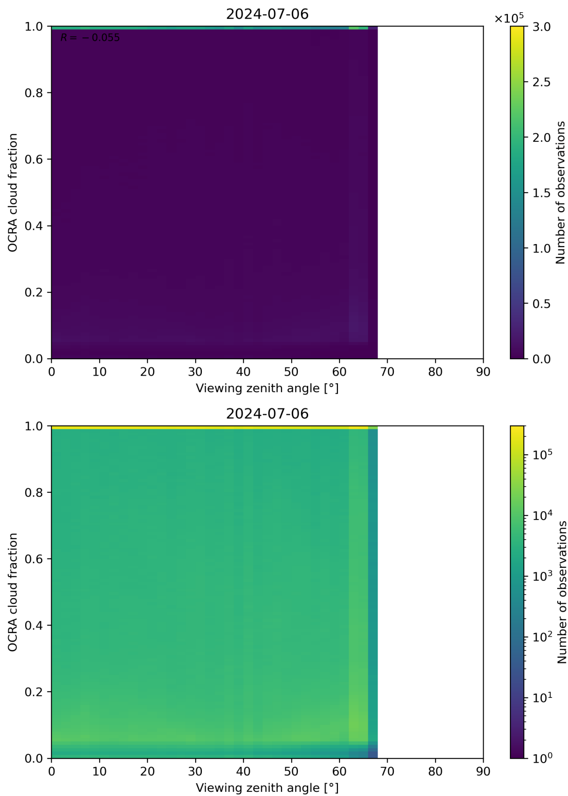
Figure 108: Scatter density plot of “Viewing zenith angle” against “OCRA cloud fraction” for 2024-07-05 to 2024-07-07.
