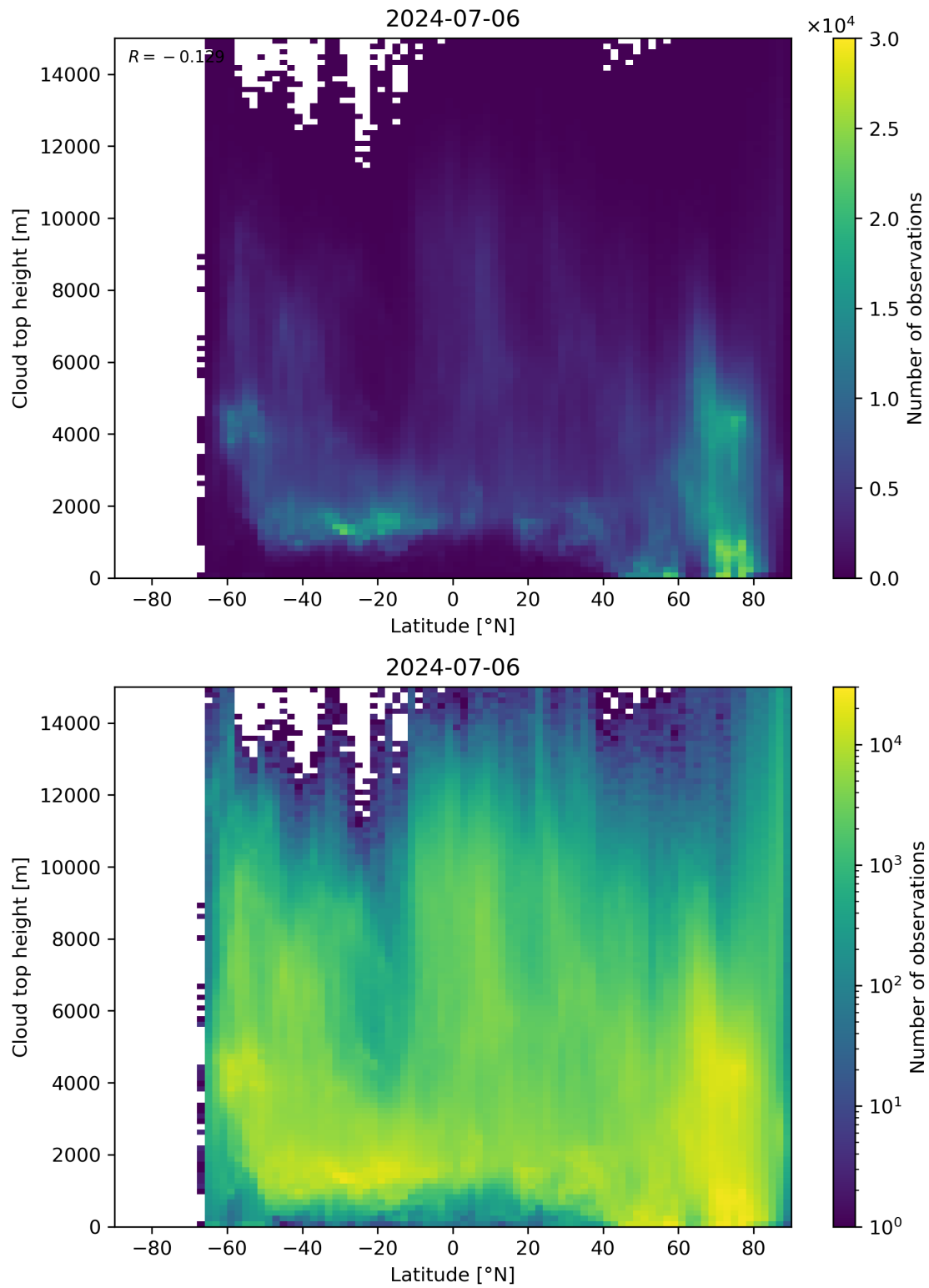
Figure 97: Scatter density plot of “Latitude” against “Cloud top height” for 2024-07-05 to 2024-07-07.
