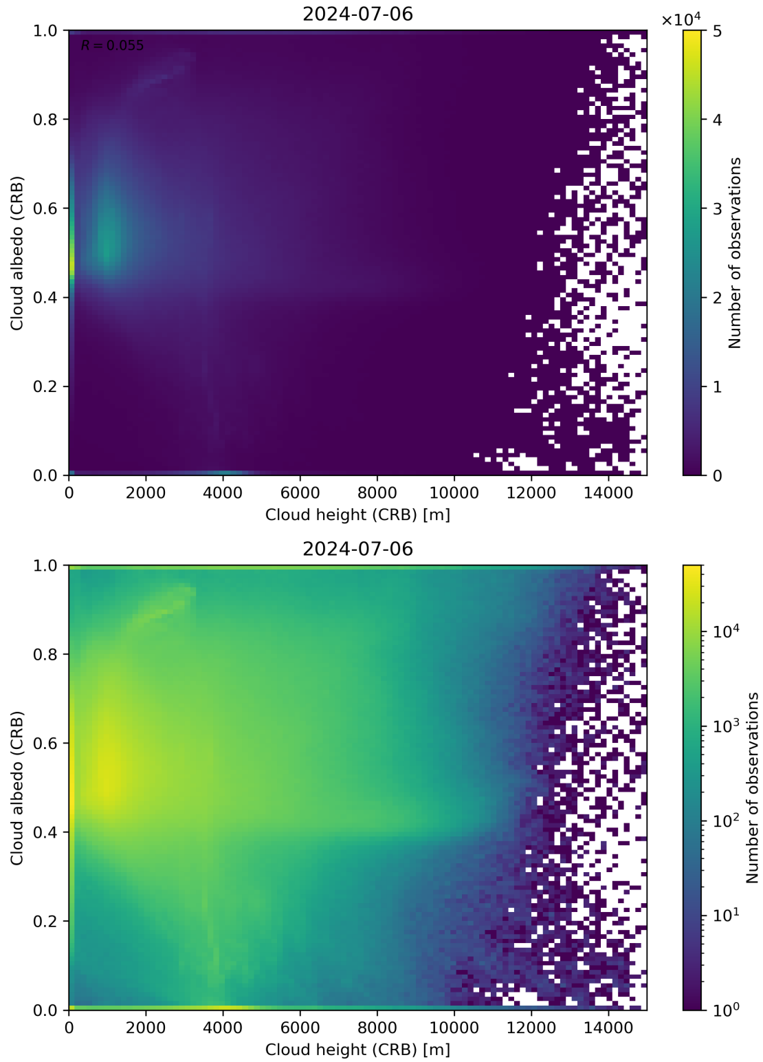
Figure 80: Scatter density plot of “Cloud height (CRB)” against “Cloud albedo (CRB)” for 2024-07-05 to 2024-07-07.
