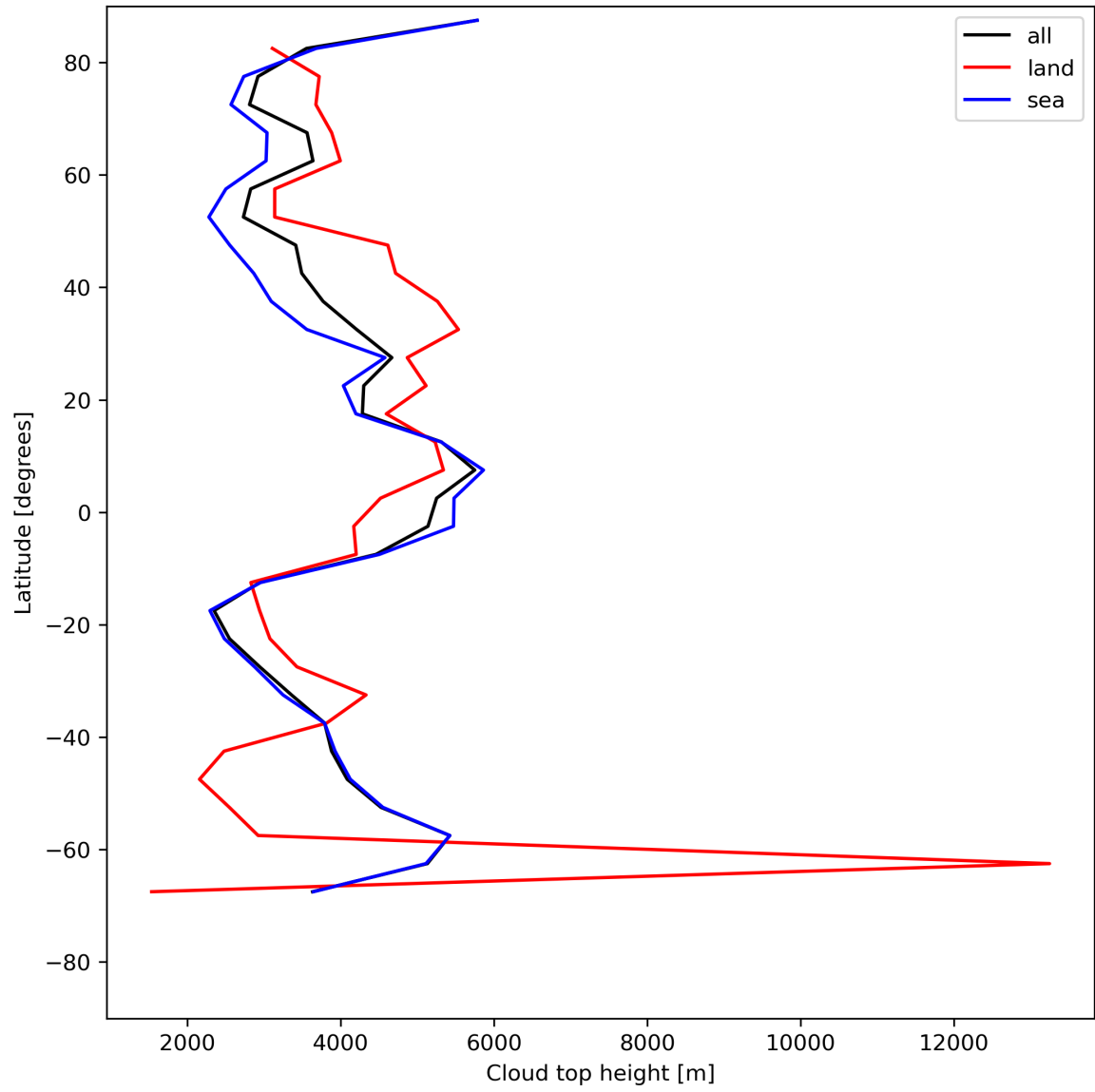
Figure 24: Zonal average of “Cloud top height” for 2024-07-05 to 2024-07-07.
