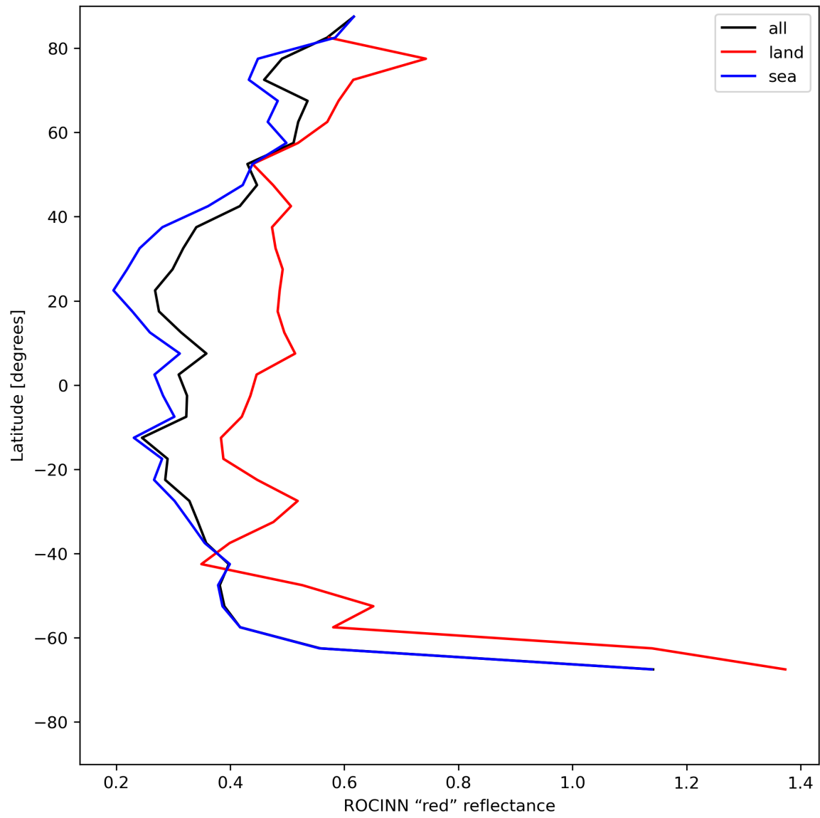
Figure 37: Zonal average of “ROCINN “red” reflectance” for 2024-07-05 to 2024-07-07.
