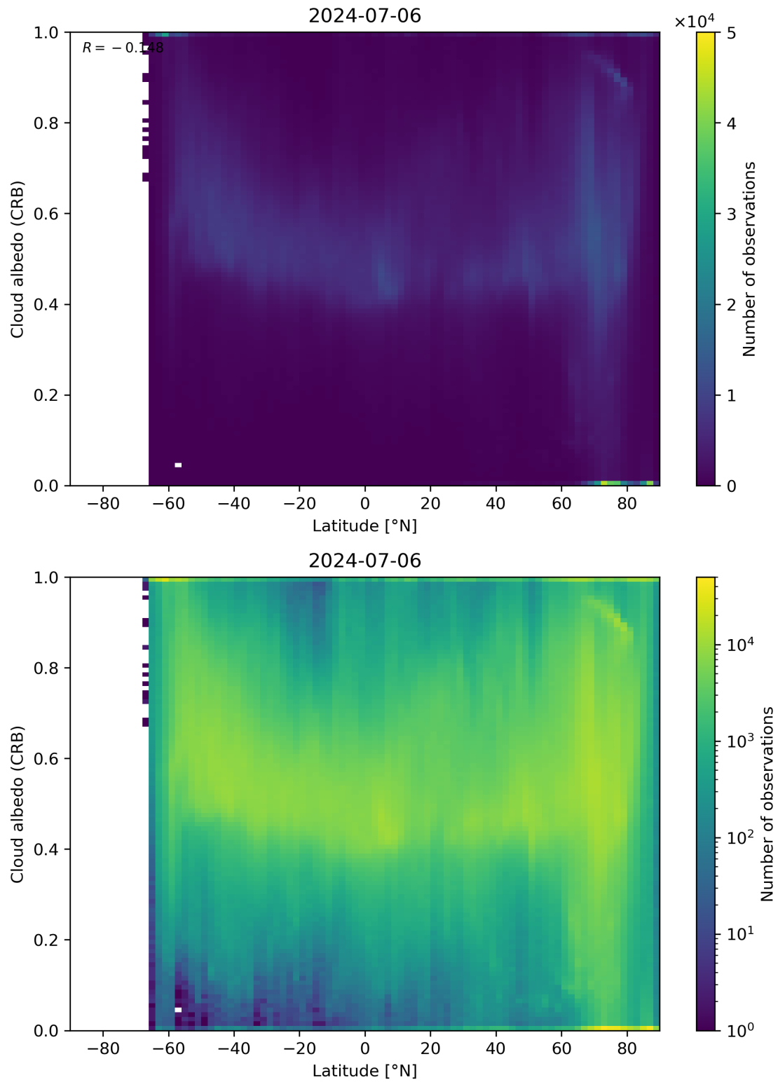
Figure 91: Scatter density plot of “Latitude” against “Cloud albedo (CRB)” for 2024-07-05 to 2024-07-07.
