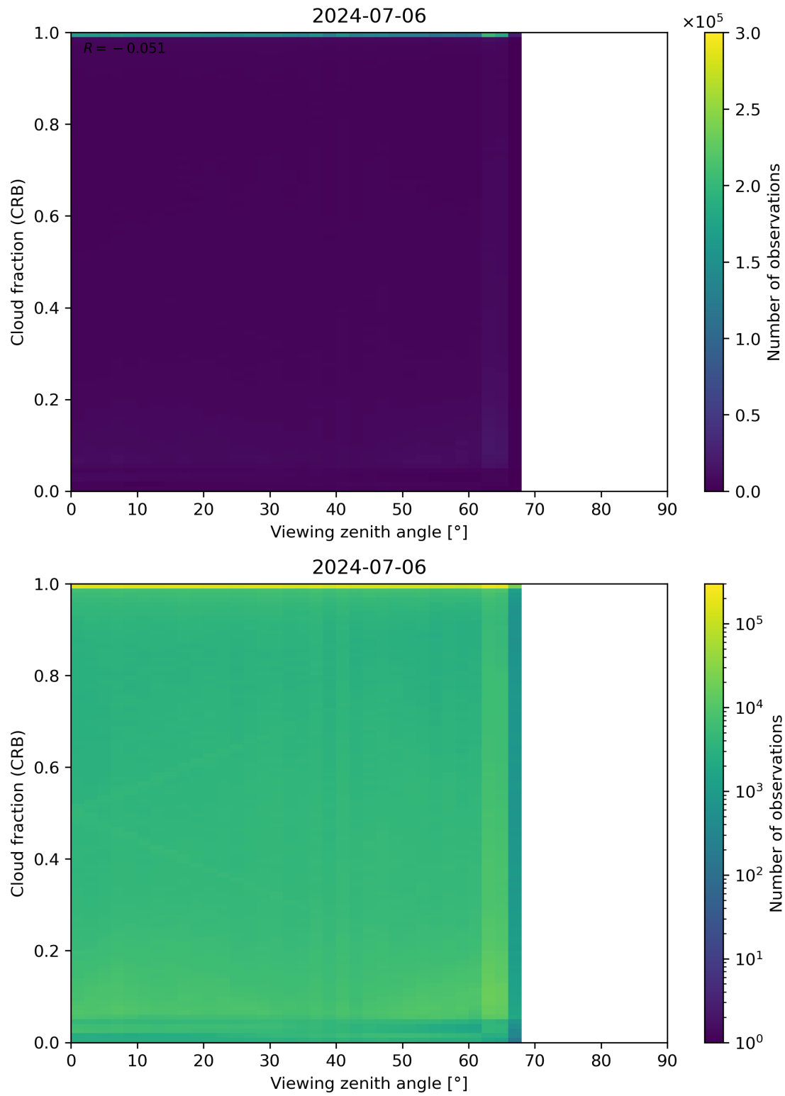
Figure 109: Scatter density plot of “Viewing zenith angle” against “Cloud fraction (CRB)” for 2024-07-05 to 2024-07-07.
