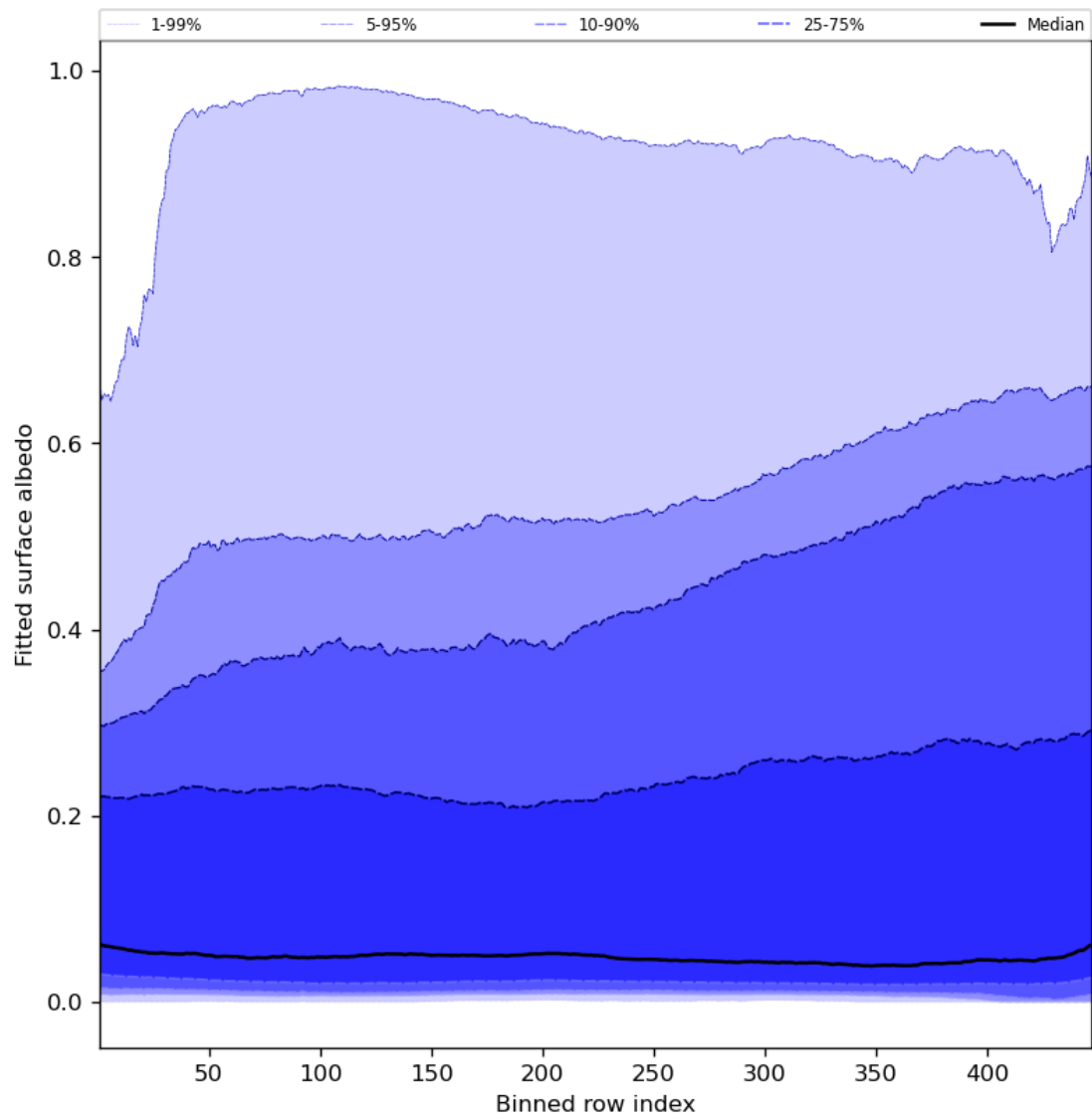
Figure 61: Along track statistics of “Fitted surface albedo” for 2024-07-05 to 2024-07-07
