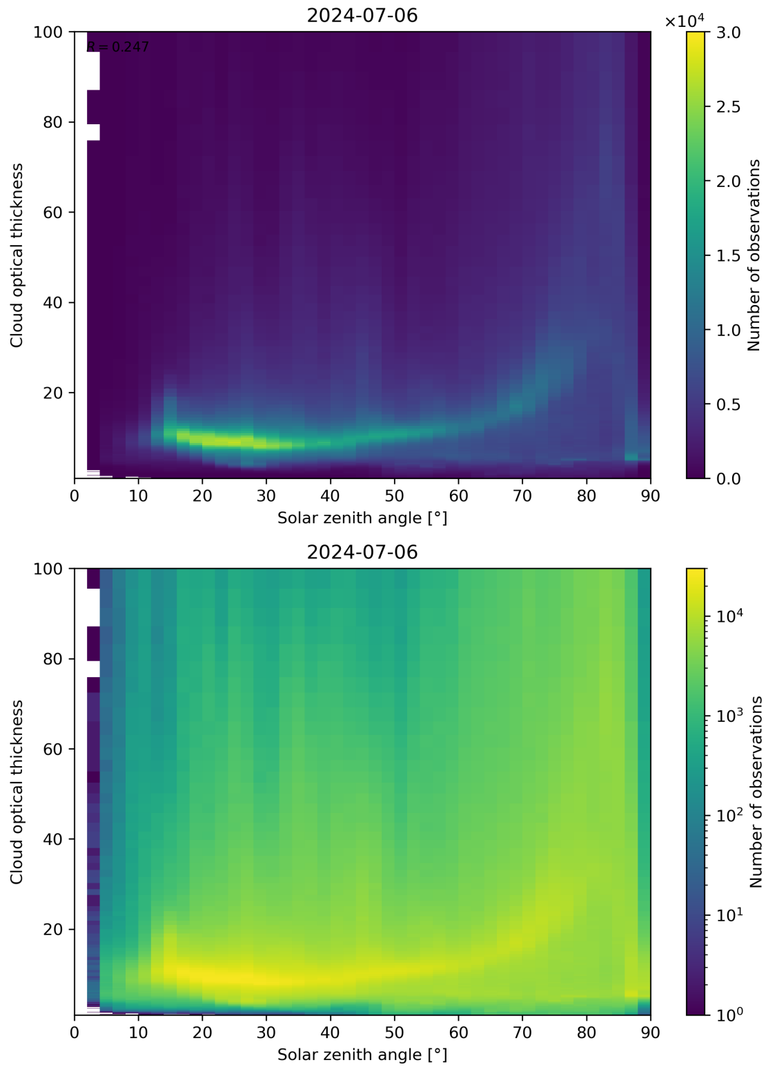
Figure 103: Scatter density plot of “Solar zenith angle” against “Cloud optical thickness” for 2024-07-05 to 2024-07-07.
