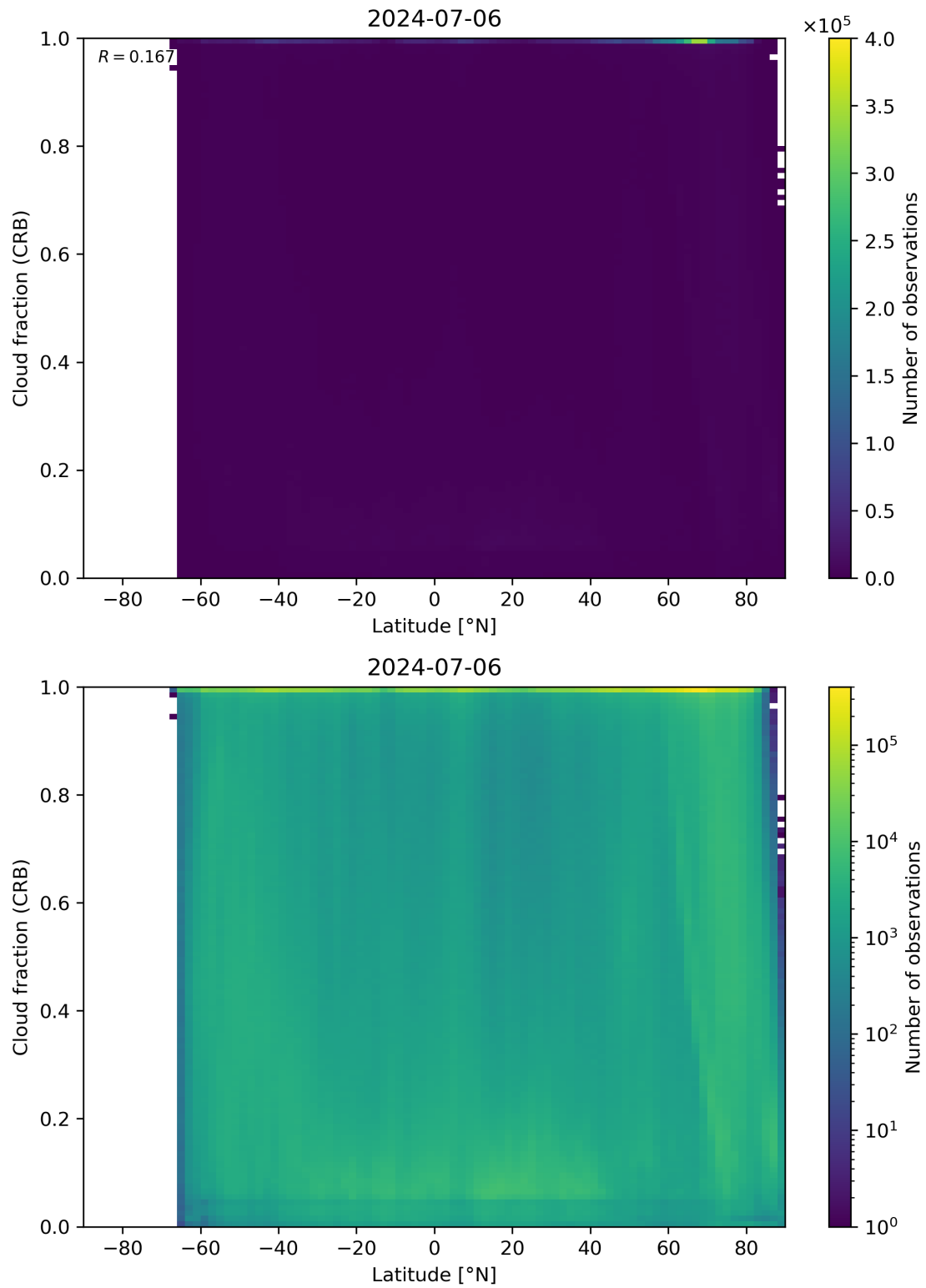
Figure 94: Scatter density plot of “Latitude” against “Cloud fraction (CRB)” for 2024-07-05 to 2024-07-07.
