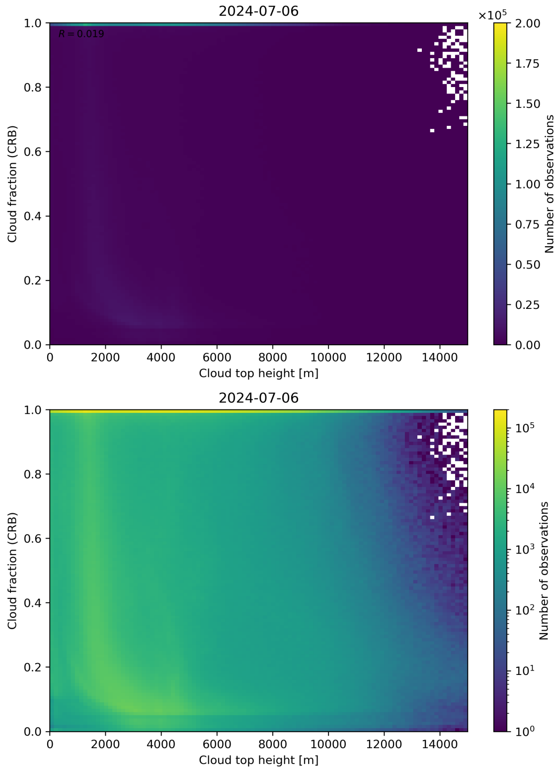
Figure 88: Scatter density plot of “Cloud top height” against “Cloud fraction (CRB)” for 2024-07-05 to 2024-07-07.
