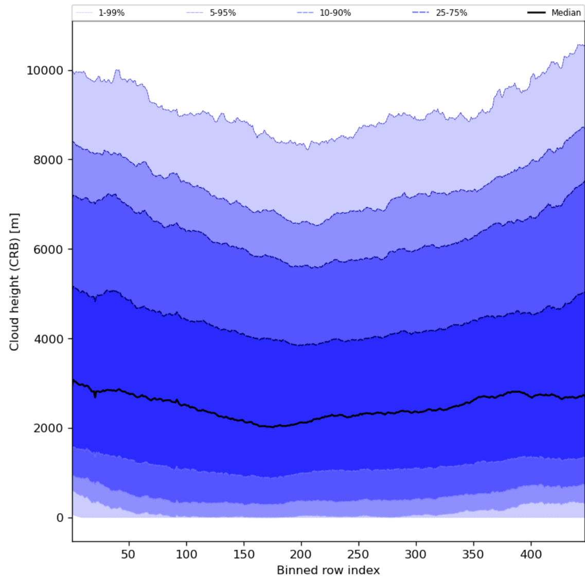
Figure 59: Along track statistics of “Cloud height (CRB)” for 2024-07-05 to 2024-07-07
