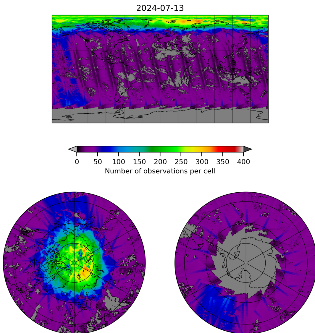
Figure 21: Map of the number of observations for 2024-07-12 to 2024-07-14
