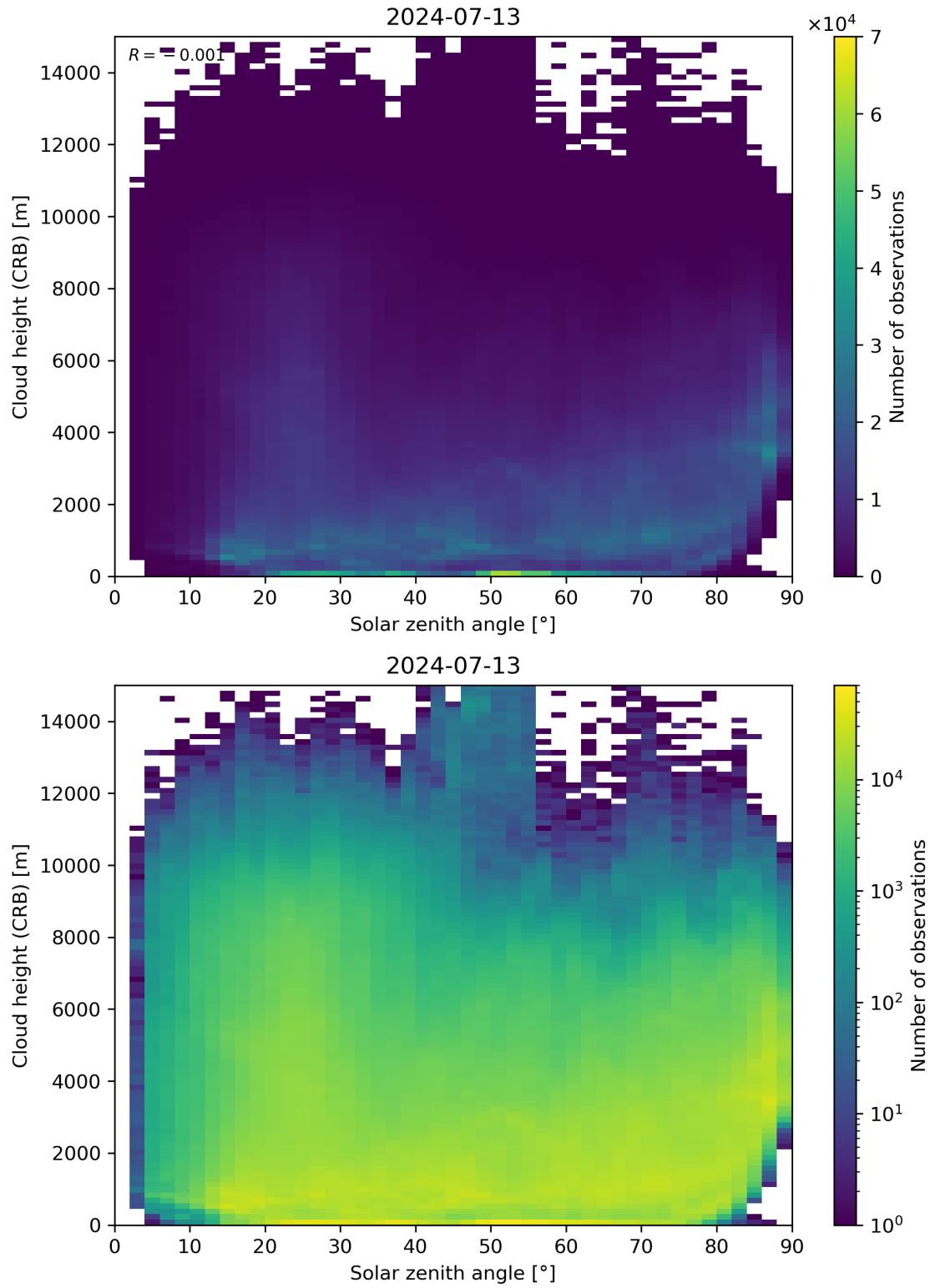
Figure 102: Scatter density plot of “Solar zenith angle” against “Cloud height (CRB)” for 2024-07-12 to 2024-07-14.
