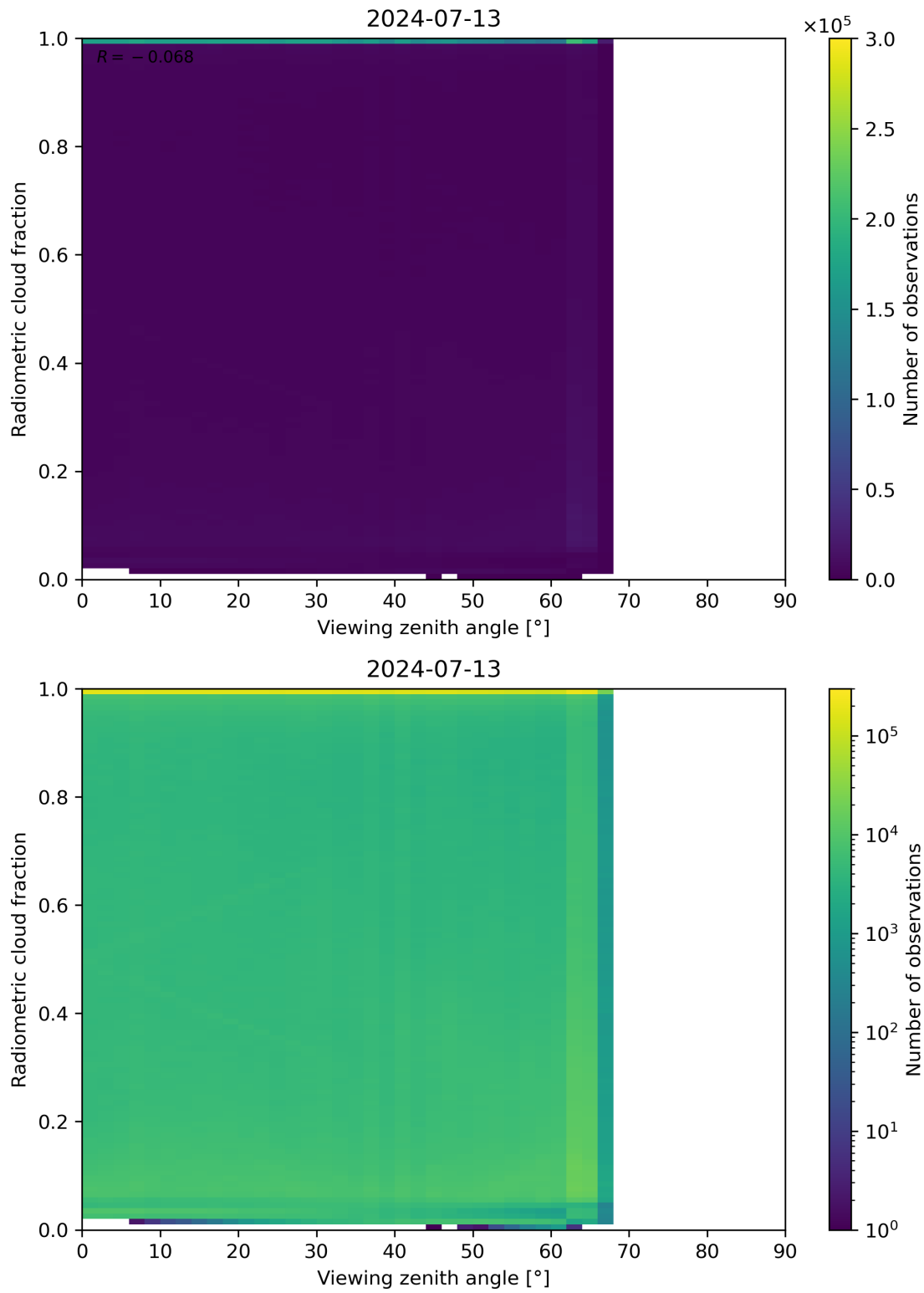
Figure 107: Scatter density plot of “Viewing zenith angle” against “Radiometric cloud fraction” for 2024-07-12 to 2024-07-14.
