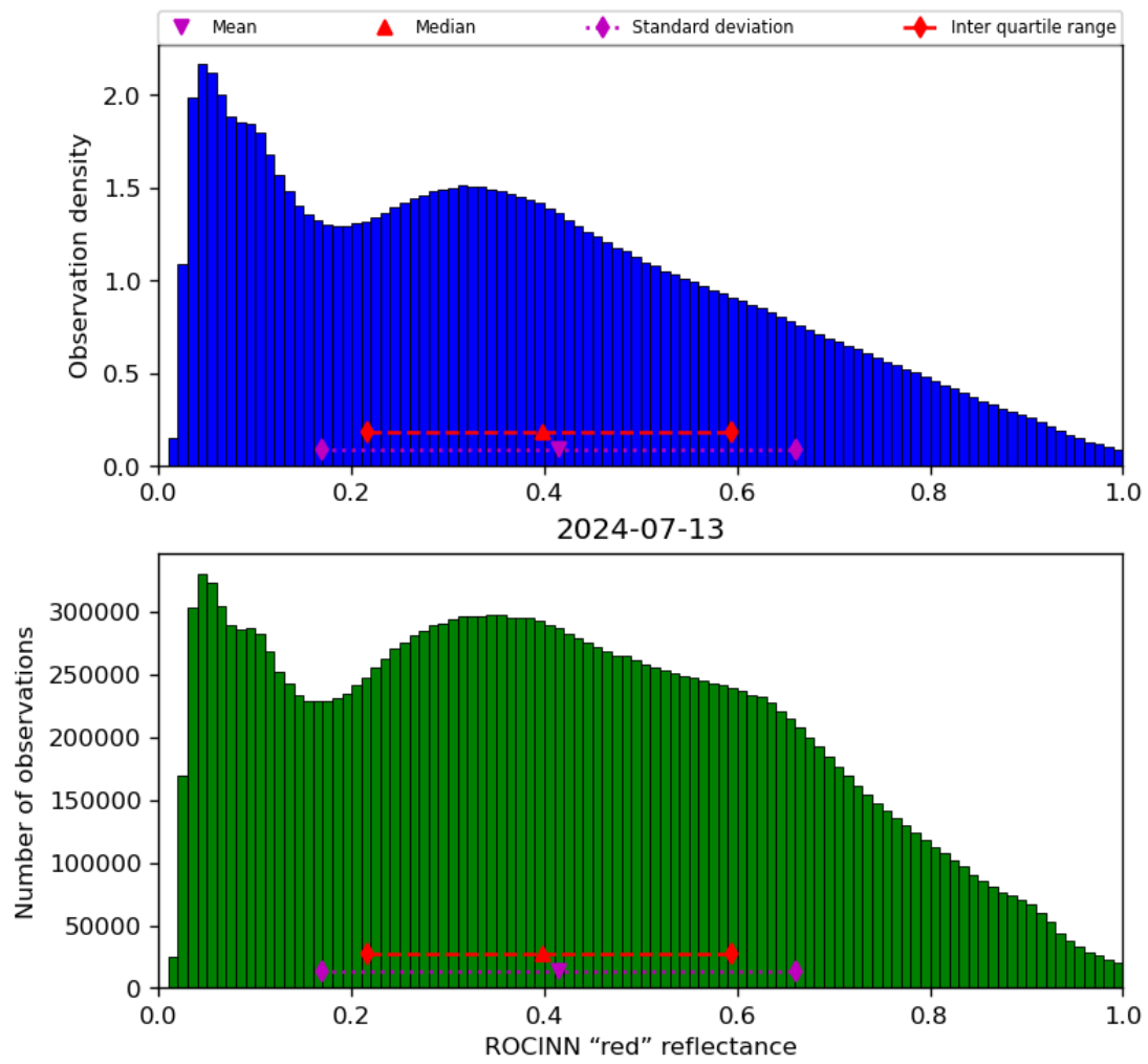
Figure 53: Histogram of “ROCINN “red” reflectance” for 2024-07-12 to 2024-07-14
