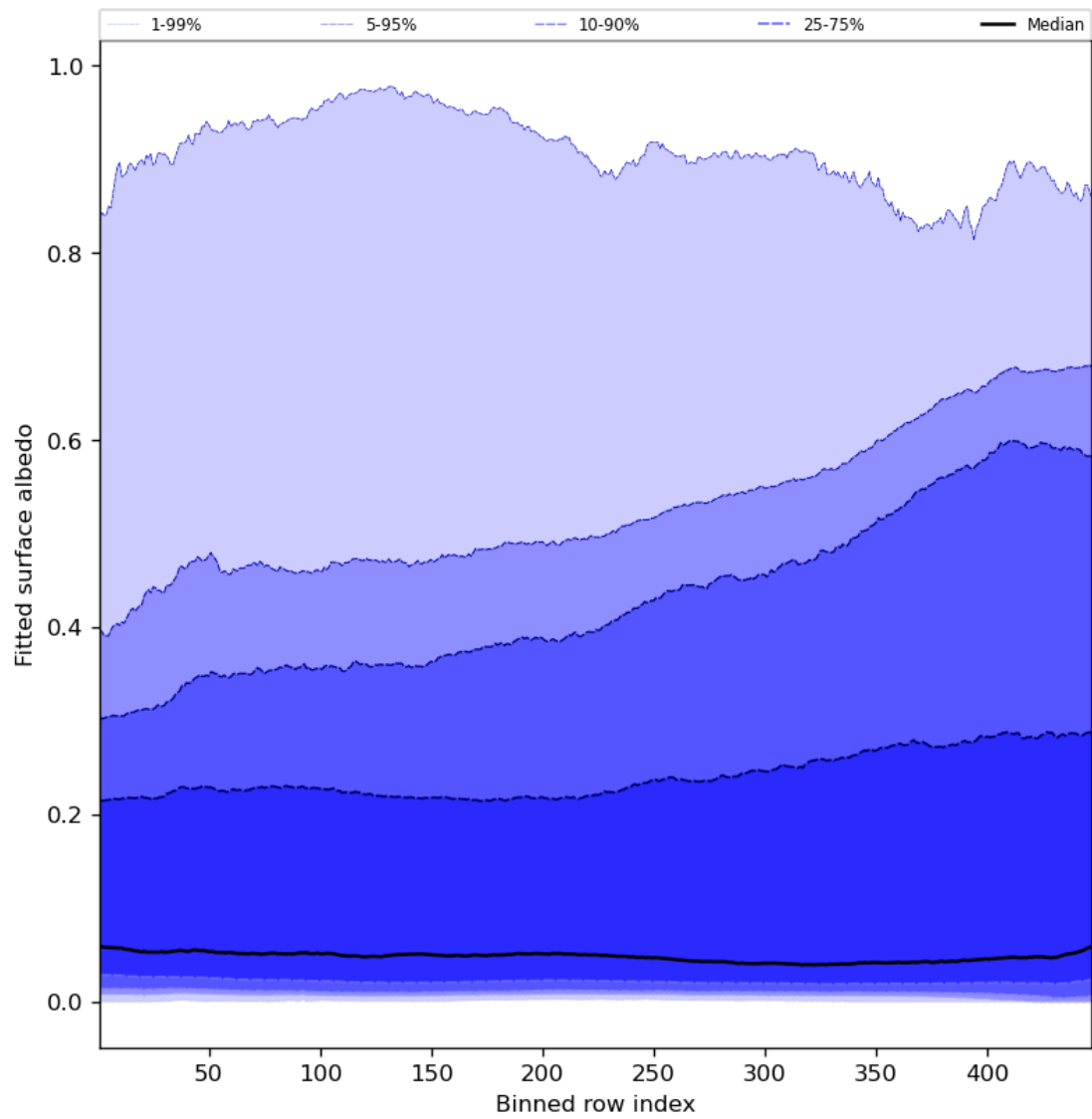
Figure 61: Along track statistics of “Fitted surface albedo” for 2024-07-12 to 2024-07-14
