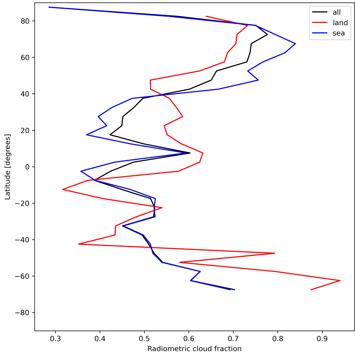
Figure 23: Zonal average of “Radiometric cloud fraction” for 2024-07-12 to 2024-07-14.
