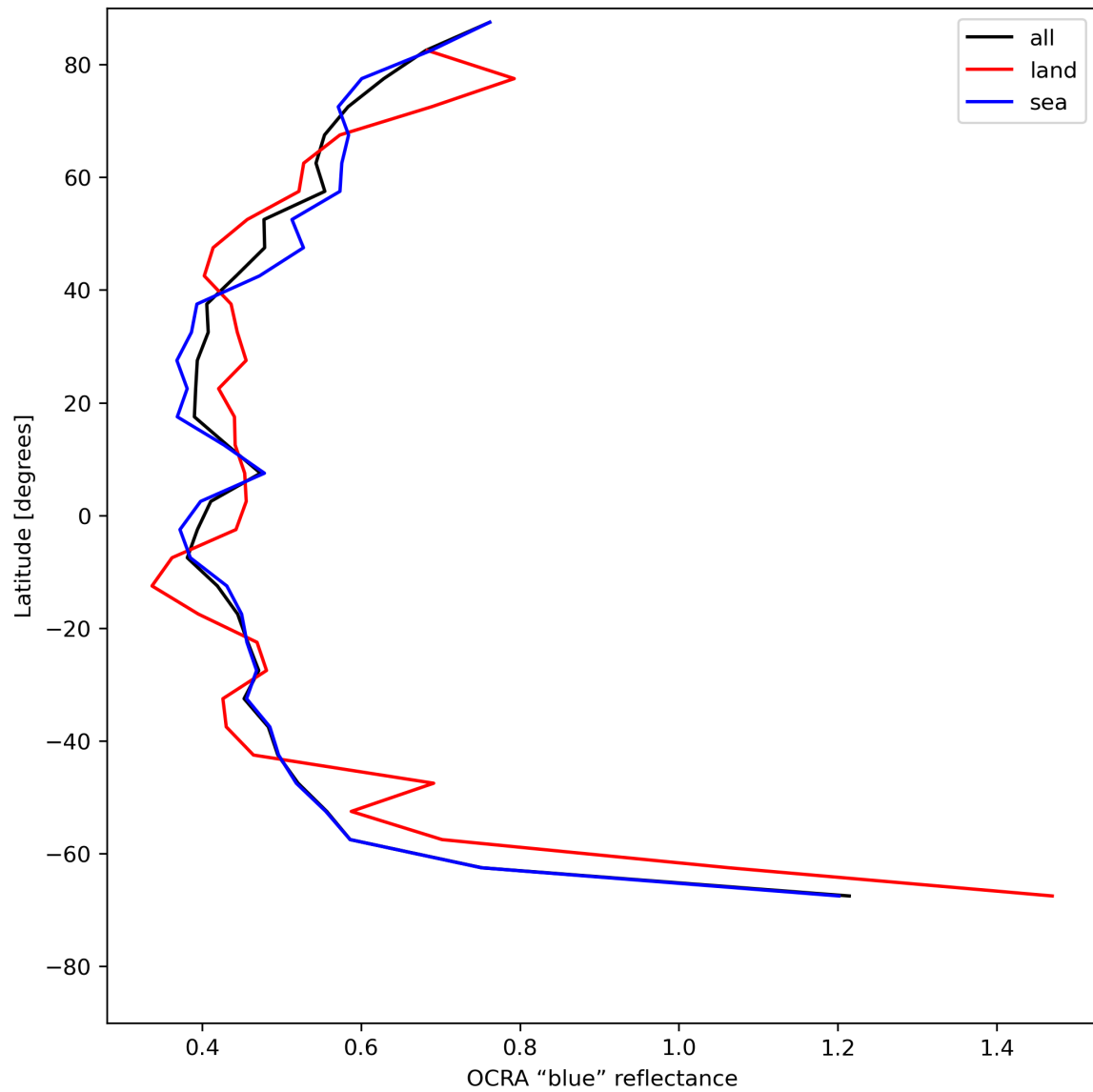
Figure 35: Zonal average of “OCRA “blue” reflectance” for 2024-07-12 to 2024-07-14.
