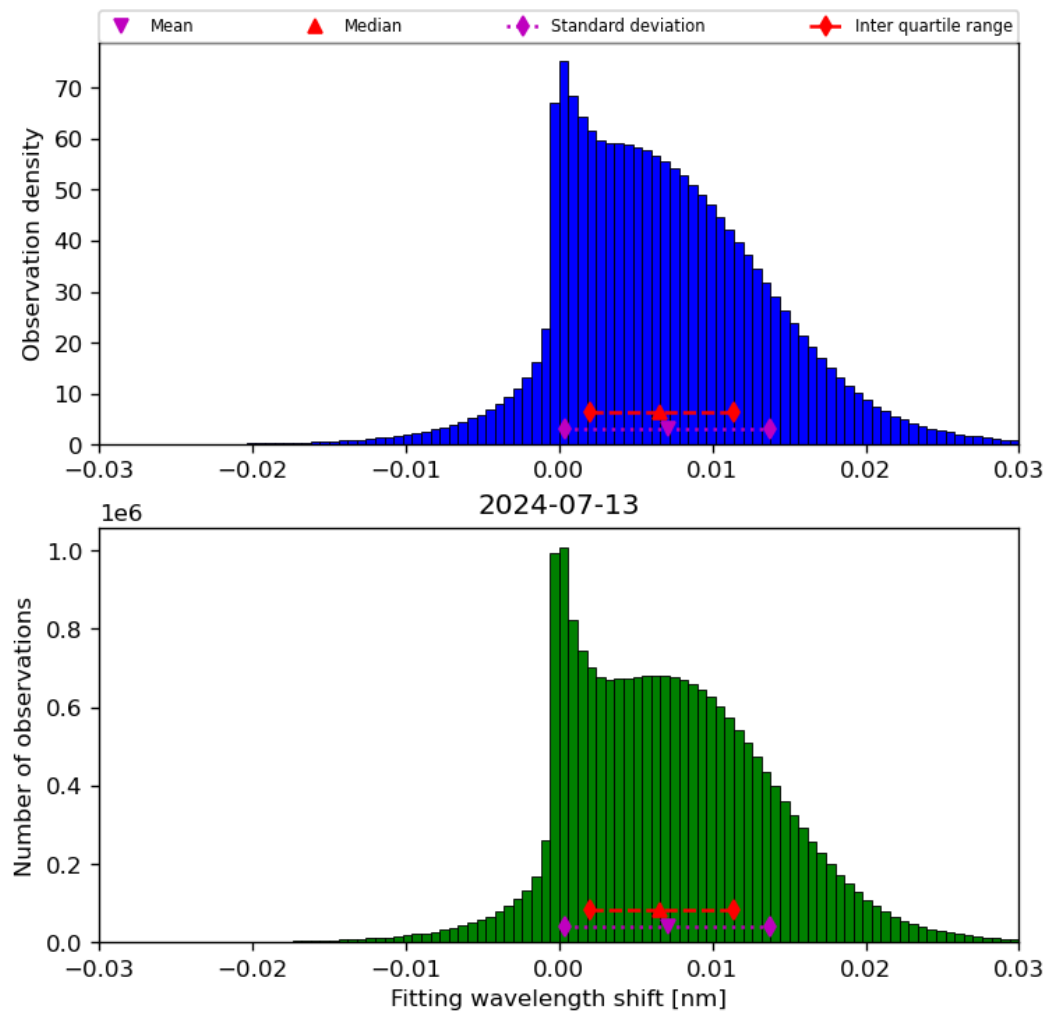
Figure 49: Histogram of “Fitting wavelength shift” for 2024-07-12 to 2024-07-14
