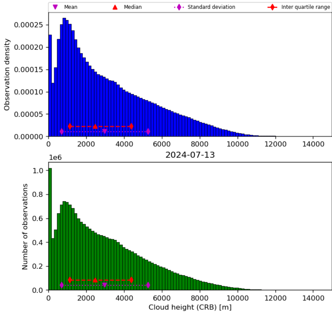
Figure 43: Histogram of “Cloud height (CRB)” for 2024-07-12 to 2024-07-14
