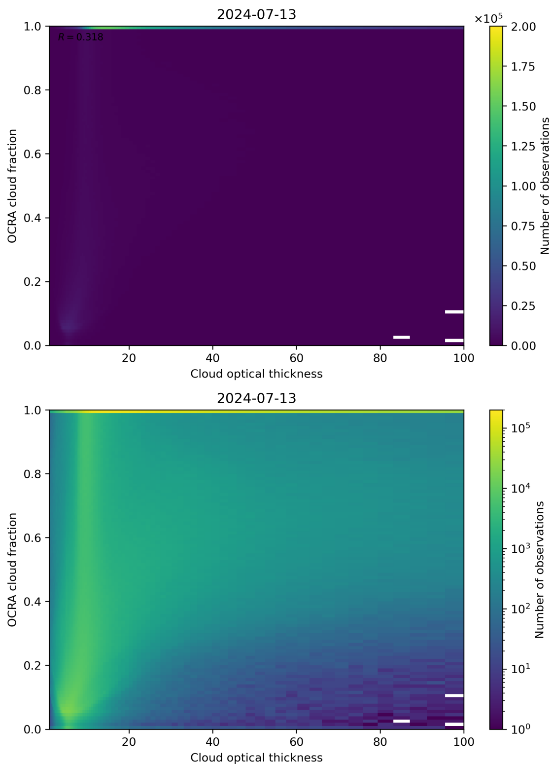
Figure 83: Scatter density plot of “Cloud optical thickness” against “OCRA cloud fraction” for 2024-07-12 to 2024-07-14.
