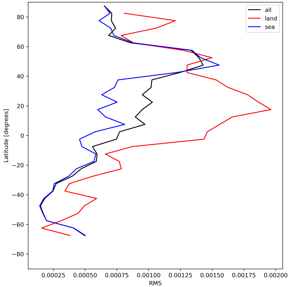
Figure 31: Zonal average of “RMS” for 2024-07-12 to 2024-07-14.
