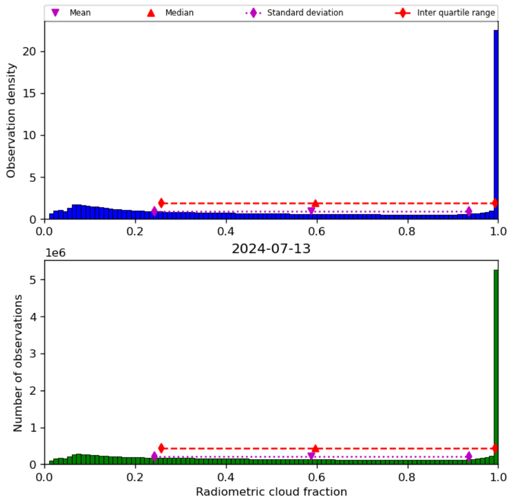
Figure 39: Histogram of “Radiometric cloud fraction” for 2024-07-12 to 2024-07-14
