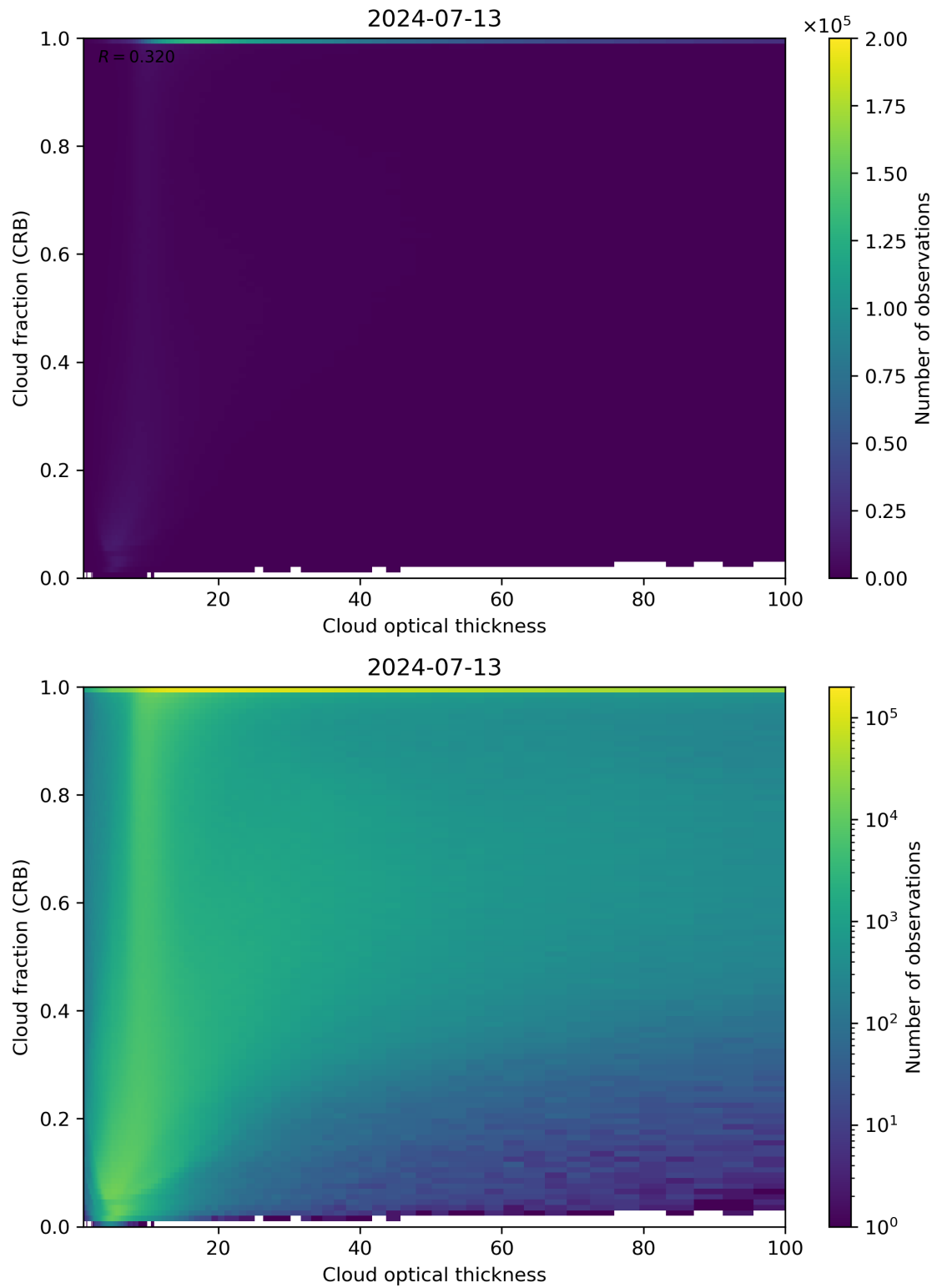
Figure 84: Scatter density plot of “Cloud optical thickness” against “Cloud fraction (CRB)” for 2024-07-12 to 2024-07-14.
