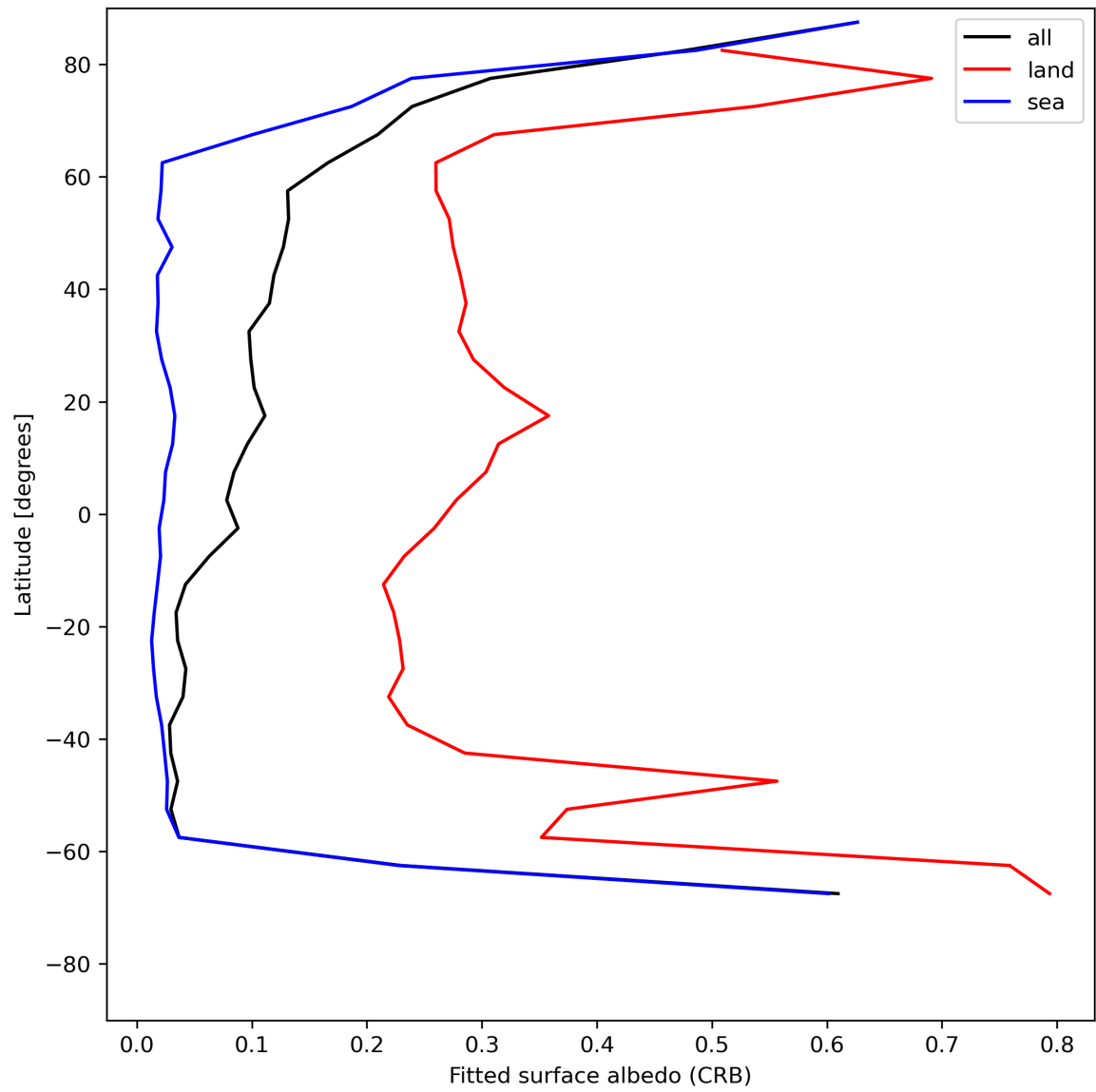
Figure 30: Zonal average of “Fitted surface albedo (CRB)” for 2024-07-12 to 2024-07-14.
