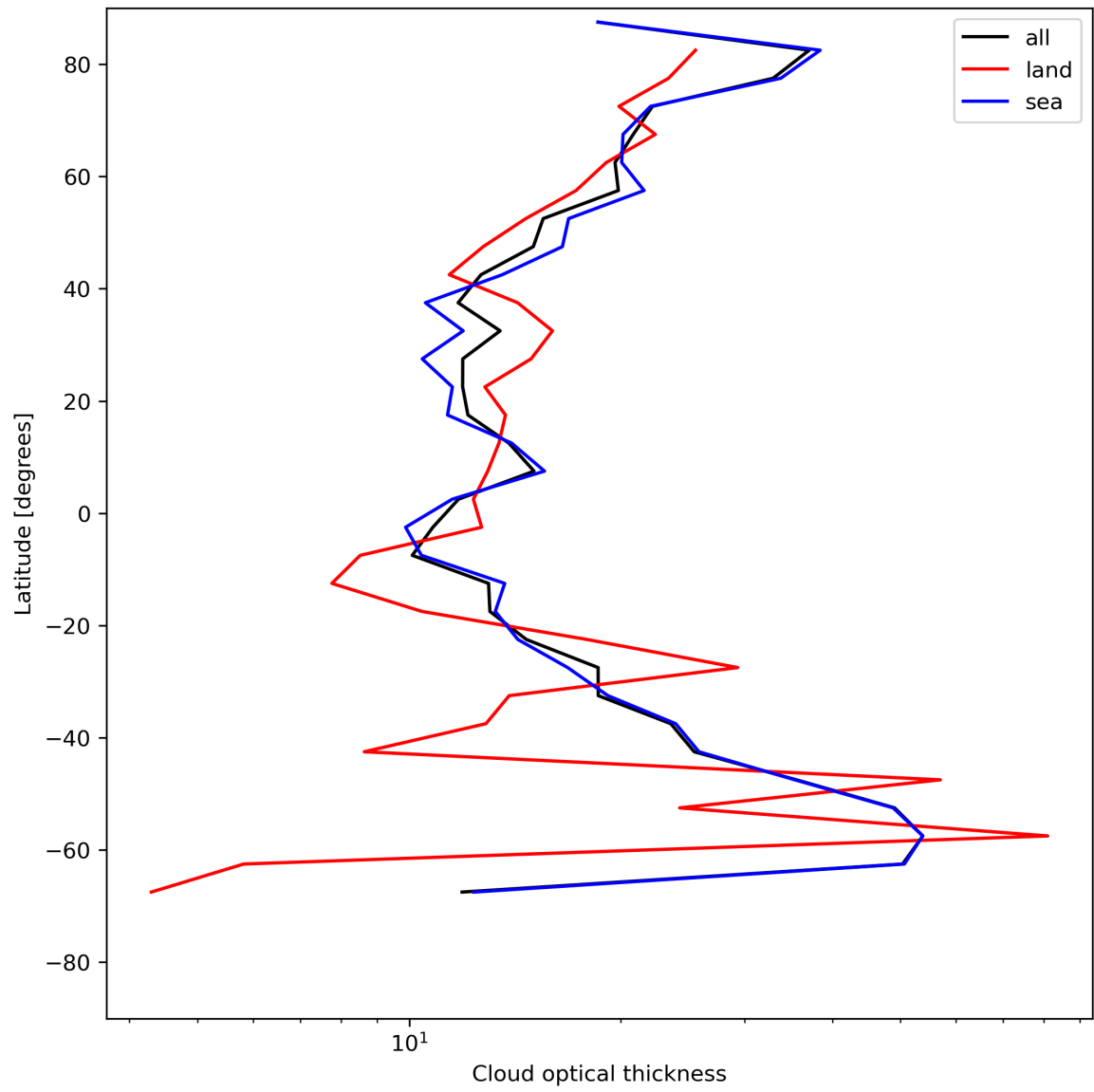
Figure 25: Zonal average of “Cloud optical thickness” for 2024-07-12 to 2024-07-14.
