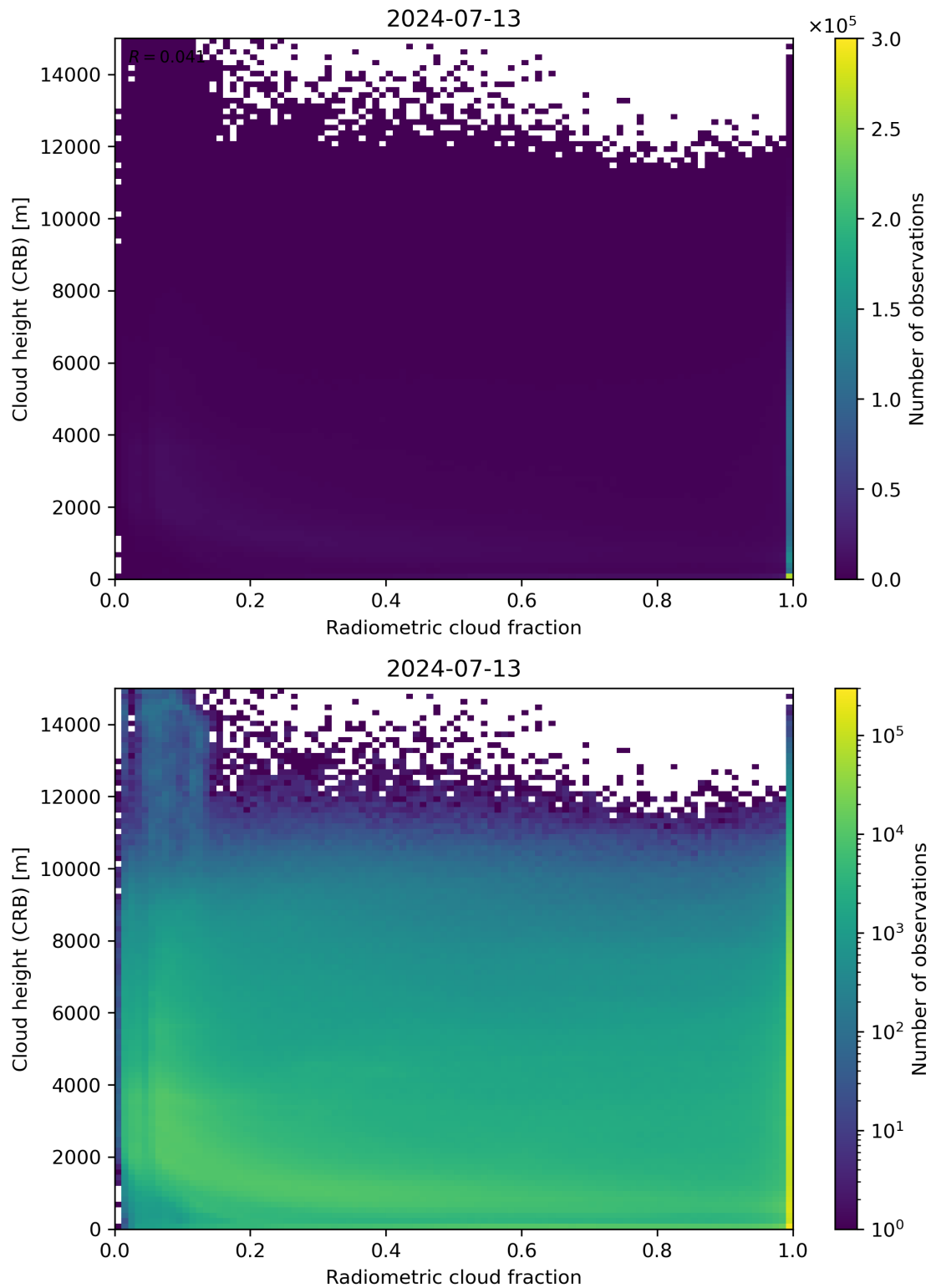
Figure 74: Scatter density plot of “Radiometric cloud fraction” against “Cloud height (CRB)” for 2024-07-12 to 2024-07-14.
