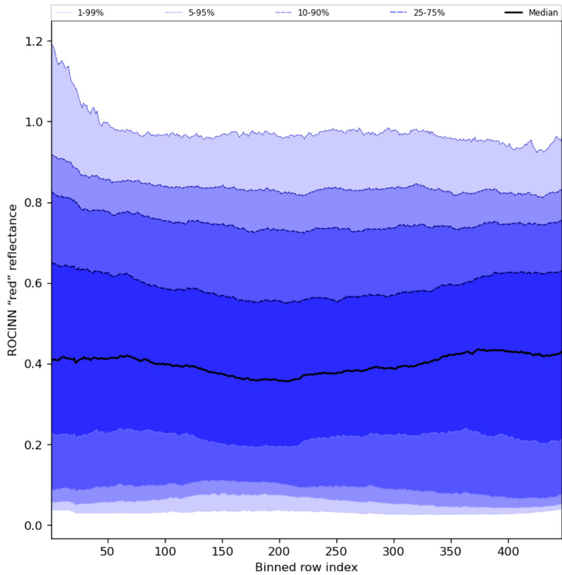
Figure 69: Along track statistics of “ROCINN “red” reflectance” for 2024-07-12 to 2024-07-14
