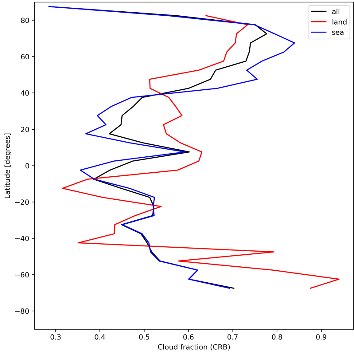
Figure 26: Zonal average of “Cloud fraction (CRB)” for 2024-07-12 to 2024-07-14.
