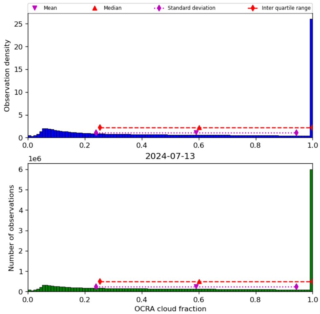
Figure 50: Histogram of “OCRA cloud fraction” for 2024-07-12 to 2024-07-14
