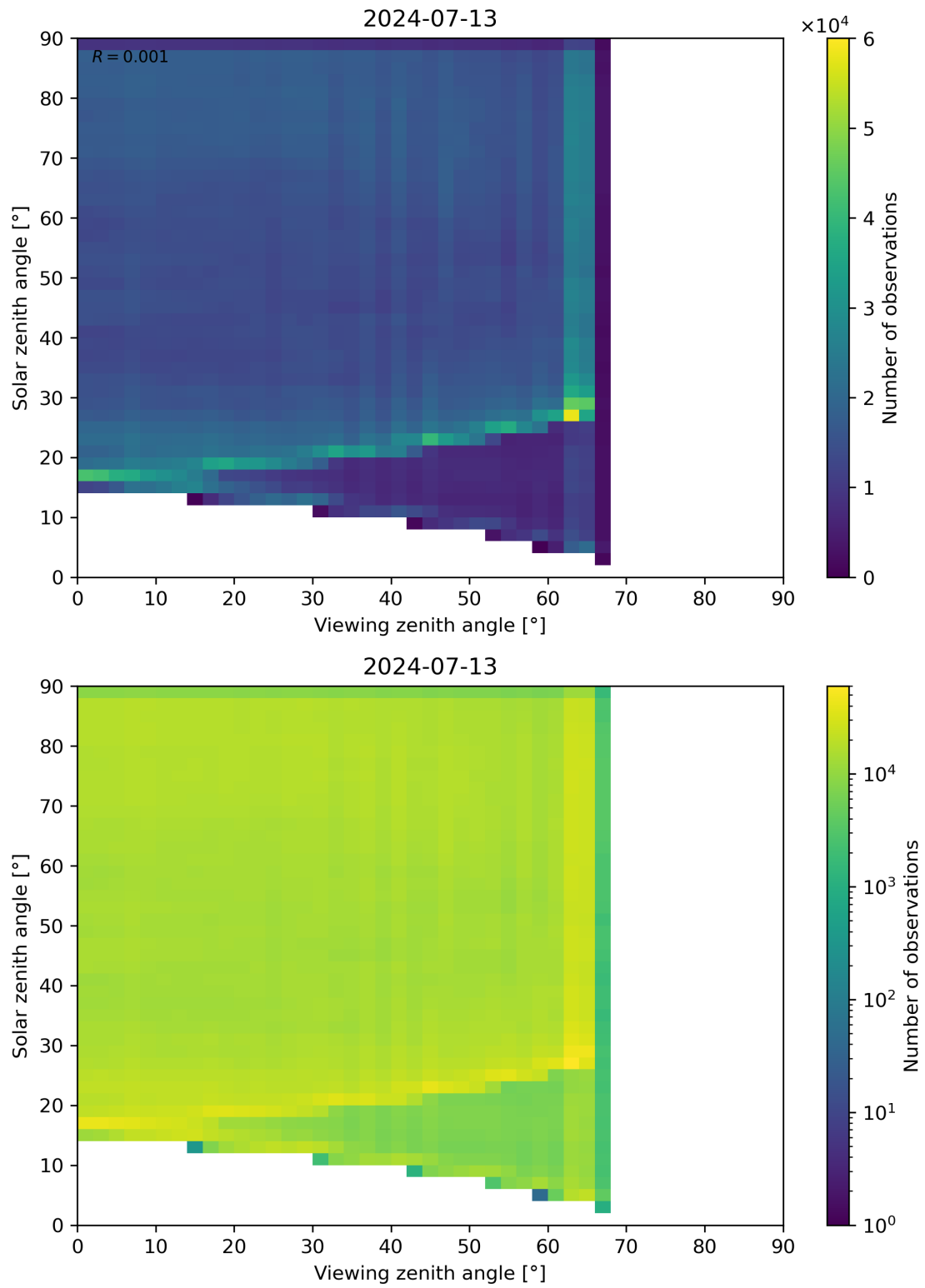
Figure 114: Scatter density plot of “Viewing zenith angle” against “Solar zenith angle” for 2024-07-12 to 2024-07-14.
