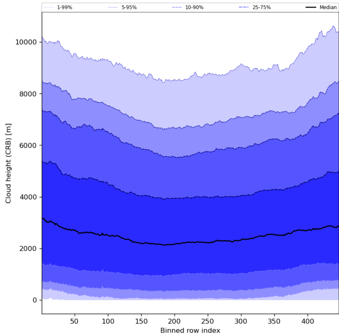
Figure 59: Along track statistics of “Cloud height (CRB)” for 2024-07-12 to 2024-07-14
