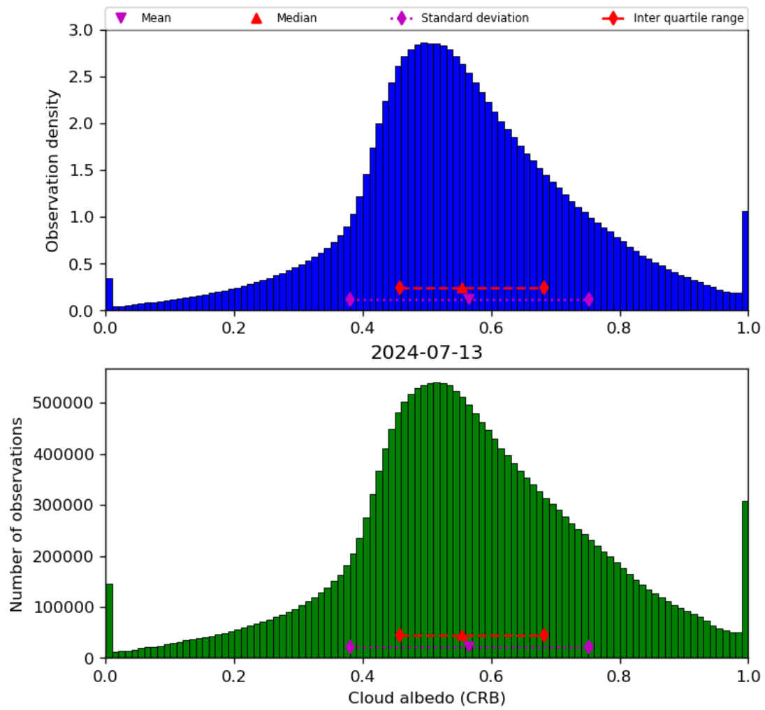
Figure 44: Histogram of “Cloud albedo (CRB)” for 2024-07-12 to 2024-07-14
