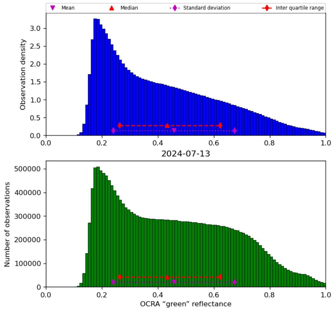
Figure 52: Histogram of “OCRA “green” reflectance” for 2024-07-12 to 2024-07-14
