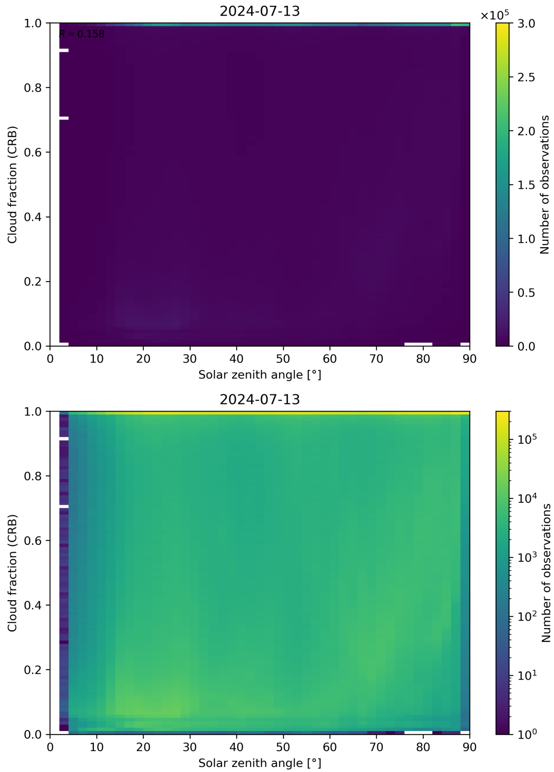
Figure 101: Scatter density plot of “Solar zenith angle” against “Cloud fraction (CRB)” for 2024-07-12 to 2024-07-14.
