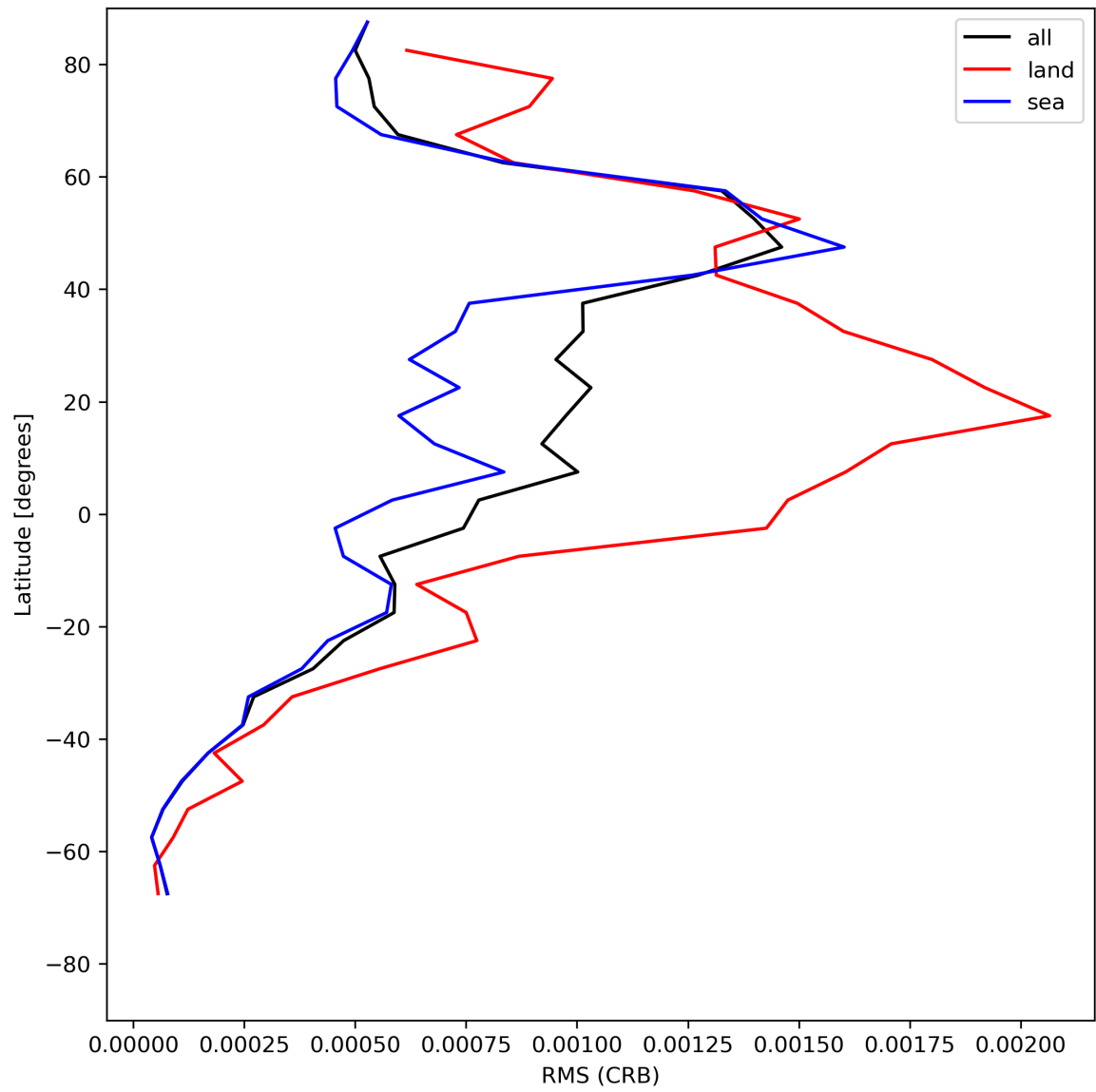
Figure 32: Zonal average of “RMS (CRB)” for 2024-07-12 to 2024-07-14.
