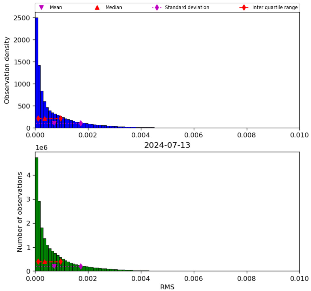
Figure 47: Histogram of “RMS” for 2024-07-12 to 2024-07-14
