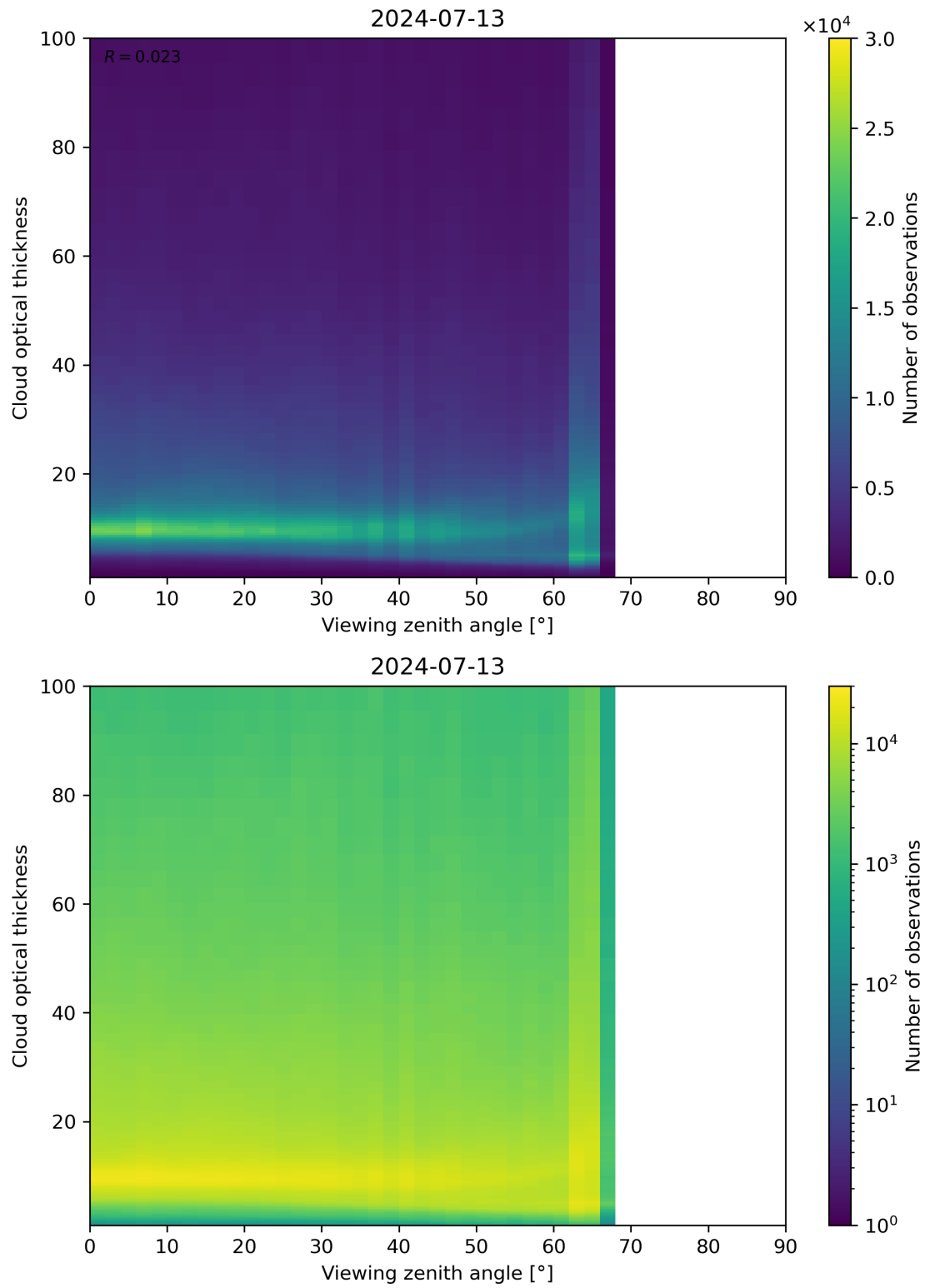
Figure 111: Scatter density plot of “Viewing zenith angle” against “Cloud optical thickness” for 2024-07-12 to 2024-07-14.
