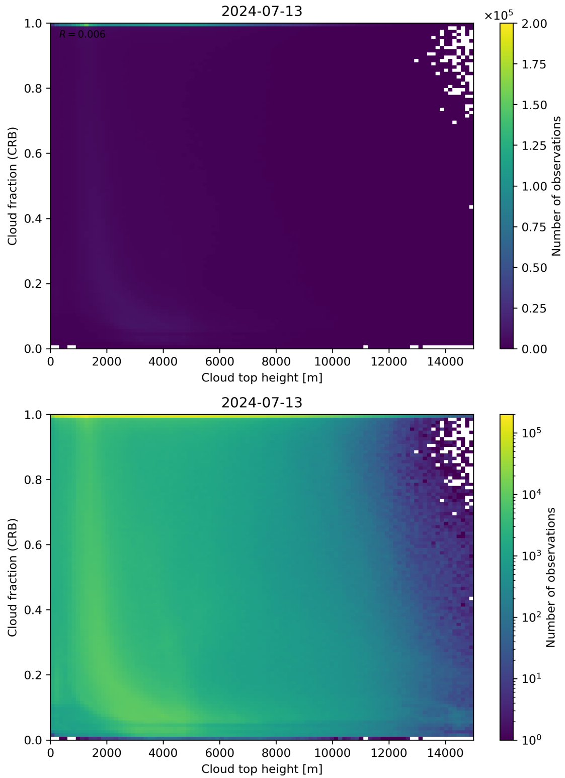
Figure 88: Scatter density plot of “Cloud top height” against “Cloud fraction (CRB)” for 2024-07-12 to 2024-07-14.
