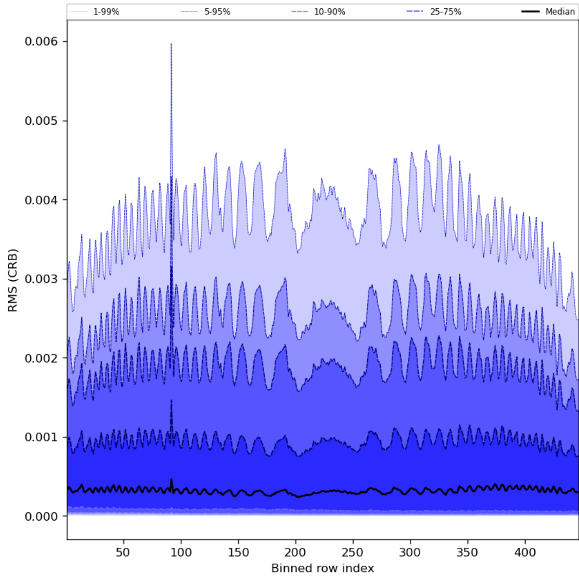
Figure 64: Along track statistics of “RMS (CRB)” for 2024-07-12 to 2024-07-14
