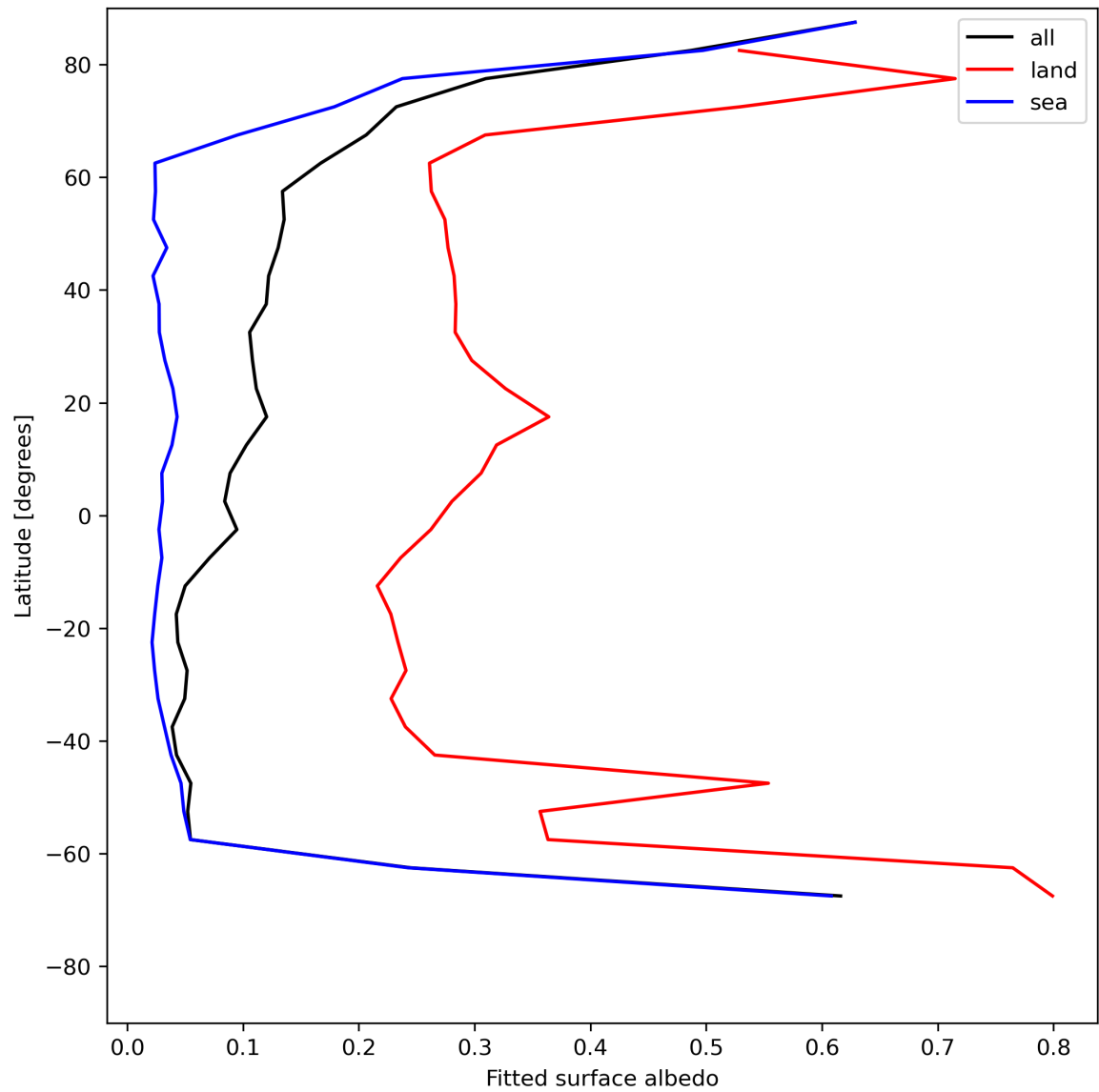
Figure 29: Zonal average of “Fitted surface albedo” for 2024-07-12 to 2024-07-14.
