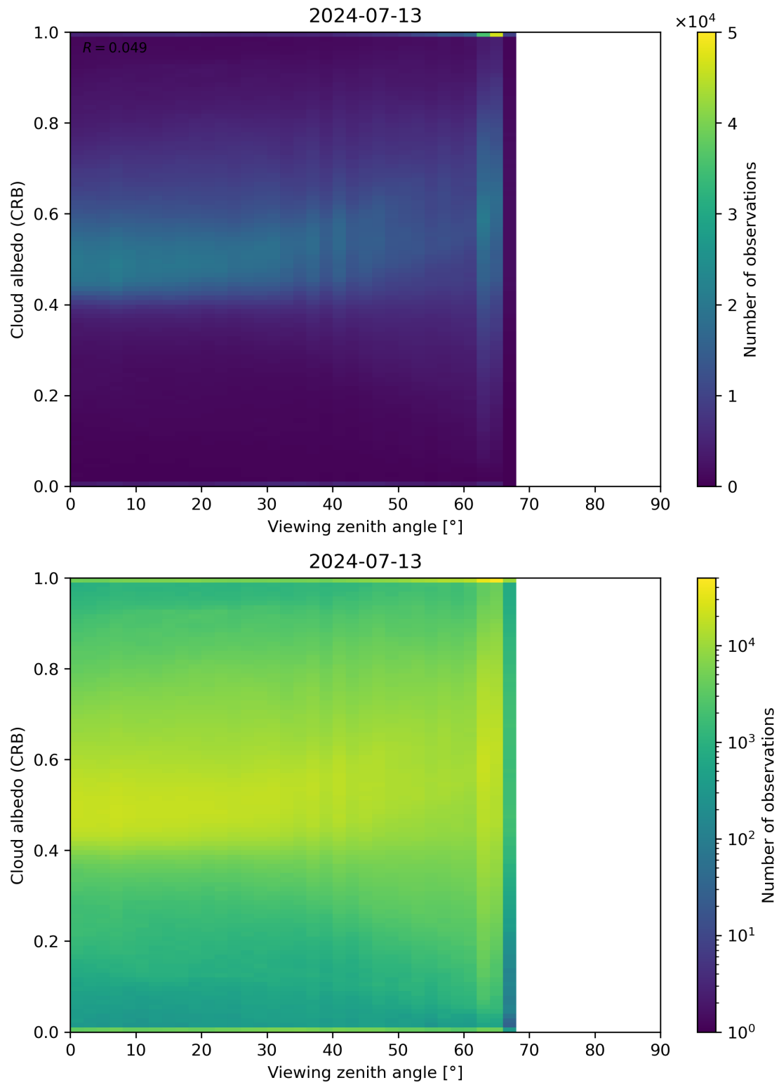
Figure 106: Scatter density plot of “Viewing zenith angle” against “Cloud albedo (CRB)” for 2024-07-12 to 2024-07-14.
