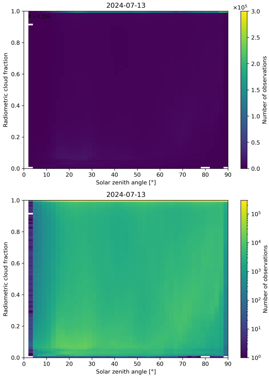
Figure 99: Scatter density plot of “Solar zenith angle” against “Radiometric cloud fraction” for 2024-07-12 to 2024-07-14.
