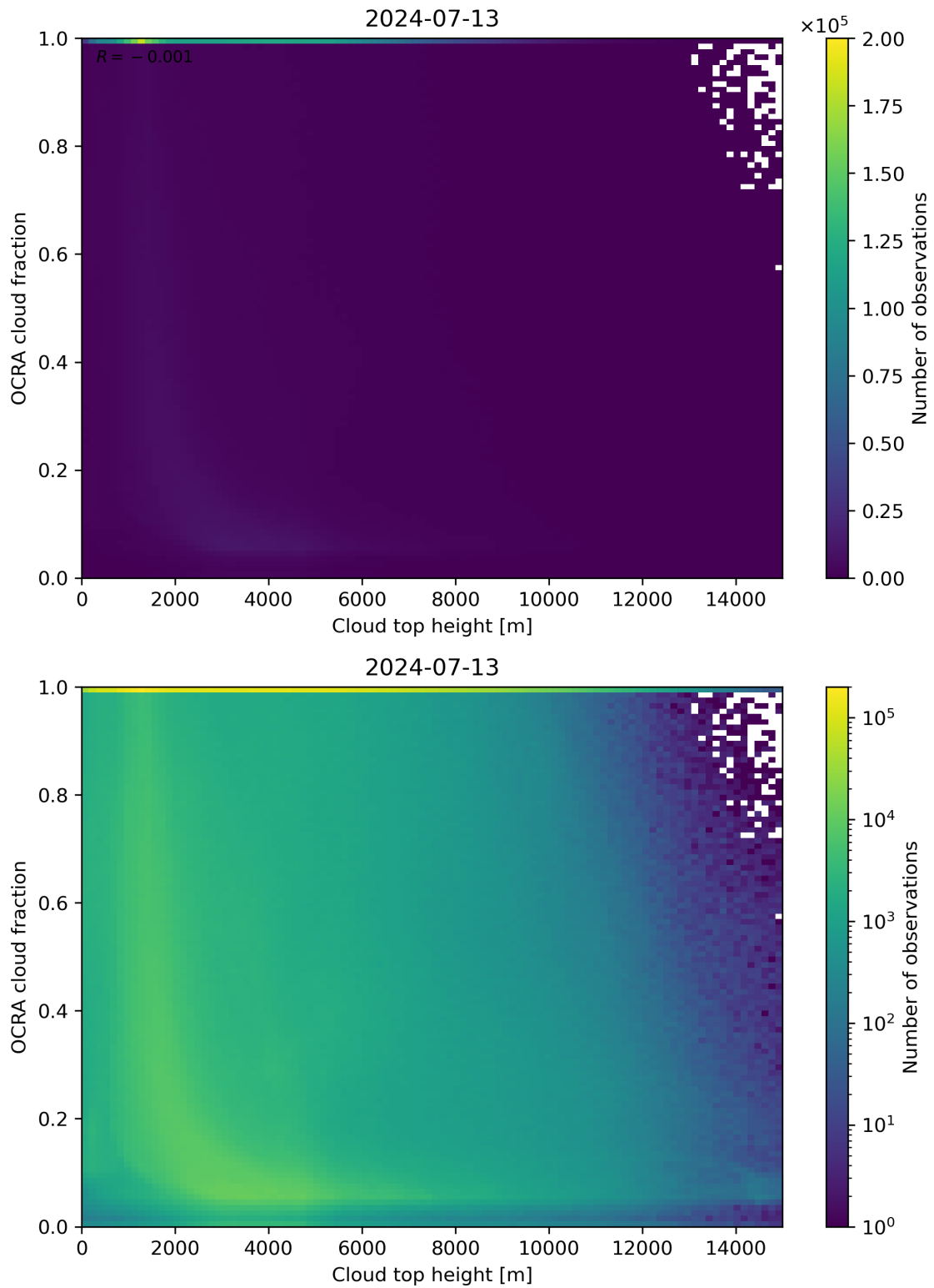
Figure 87: Scatter density plot of “Cloud top height” against “OCRA cloud fraction” for 2024-07-12 to 2024-07-14.
