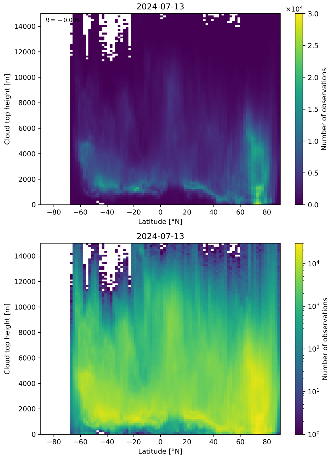
Figure 97: Scatter density plot of “Latitude” against “Cloud top height” for 2024-07-12 to 2024-07-14.
