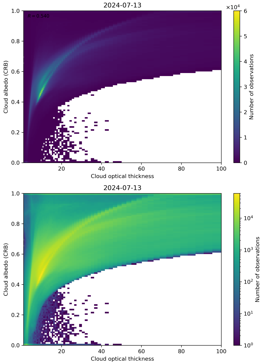
Figure 82: Scatter density plot of “Cloud optical thickness” against “Cloud albedo (CRB)” for 2024-07-12 to 2024-07-14.
