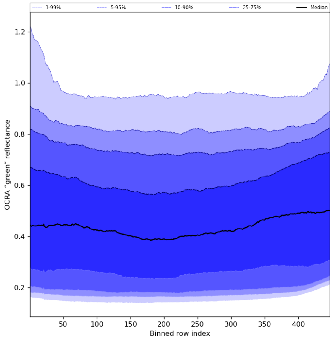
Figure 68: Along track statistics of "OCRA "green" reflectance" for 2024-07-12 to 2024-07-14
