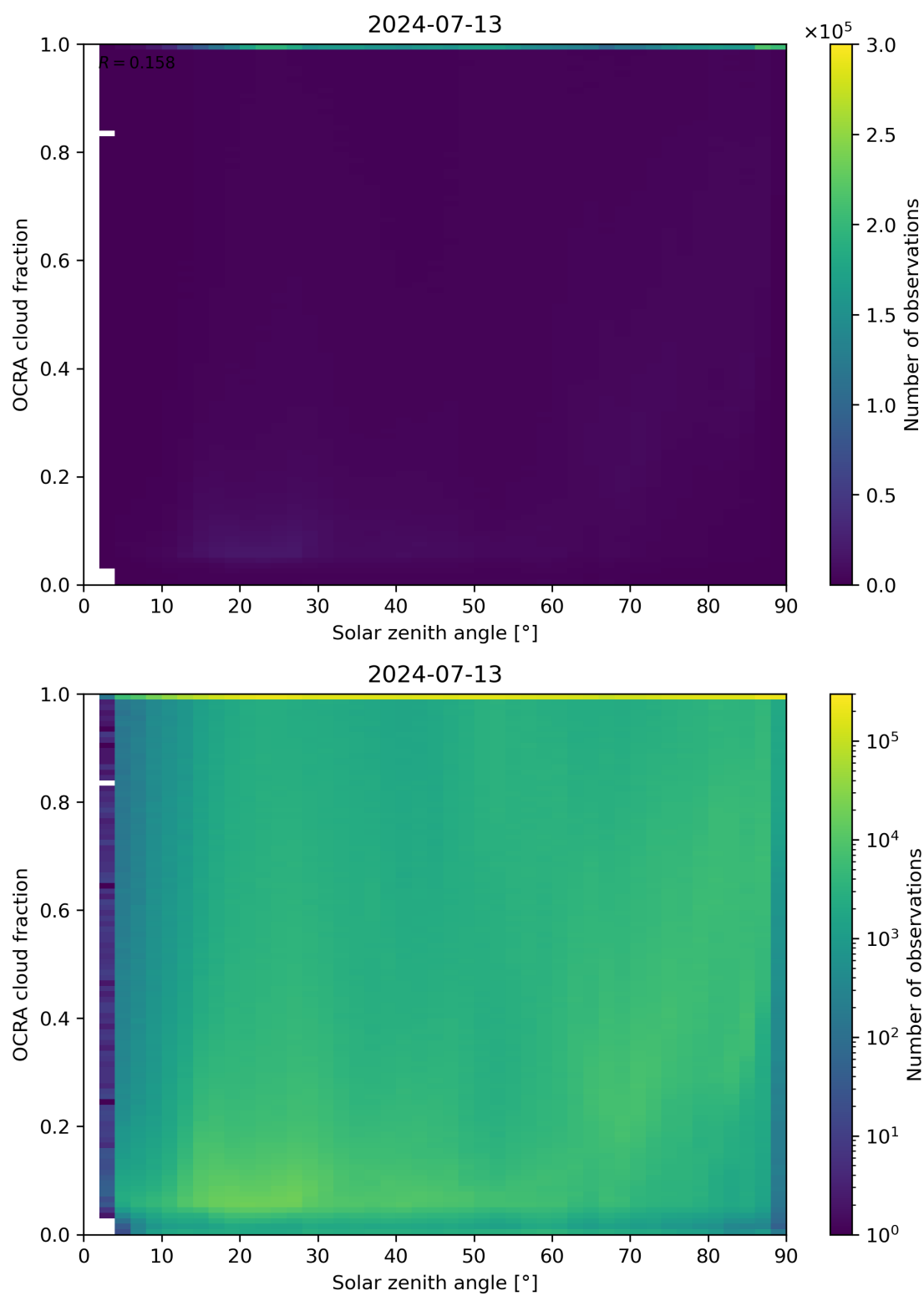
Figure 100: Scatter density plot of “Solar zenith angle” against “OCRA cloud fraction” for 2024-07-12 to 2024-07-14.
