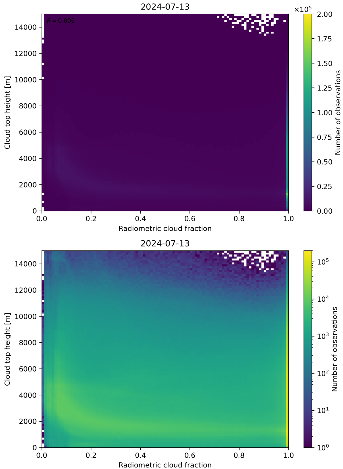
Figure 76: Scatter density plot of “Radiometric cloud fraction” against “Cloud top height” for 2024-07-12 to 2024-07-14.
