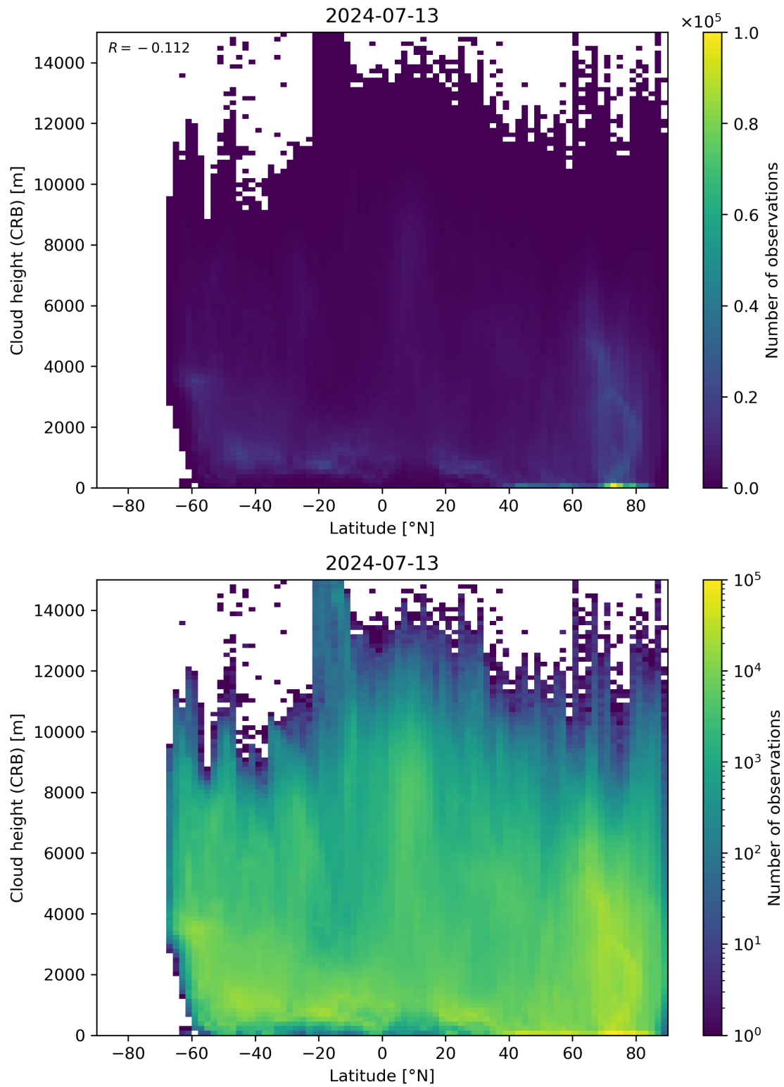
Figure 95: Scatter density plot of “Latitude” against “Cloud height (CRB)” for 2024-07-12 to 2024-07-14.
