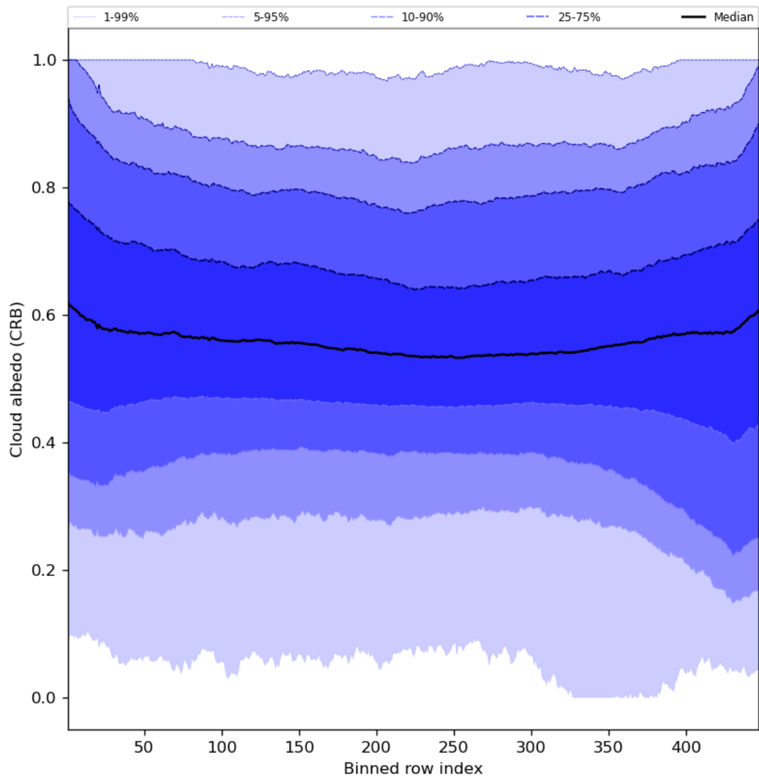
Figure 60: Along track statistics of “Cloud albedo (CRB)” for 2024-07-12 to 2024-07-14
