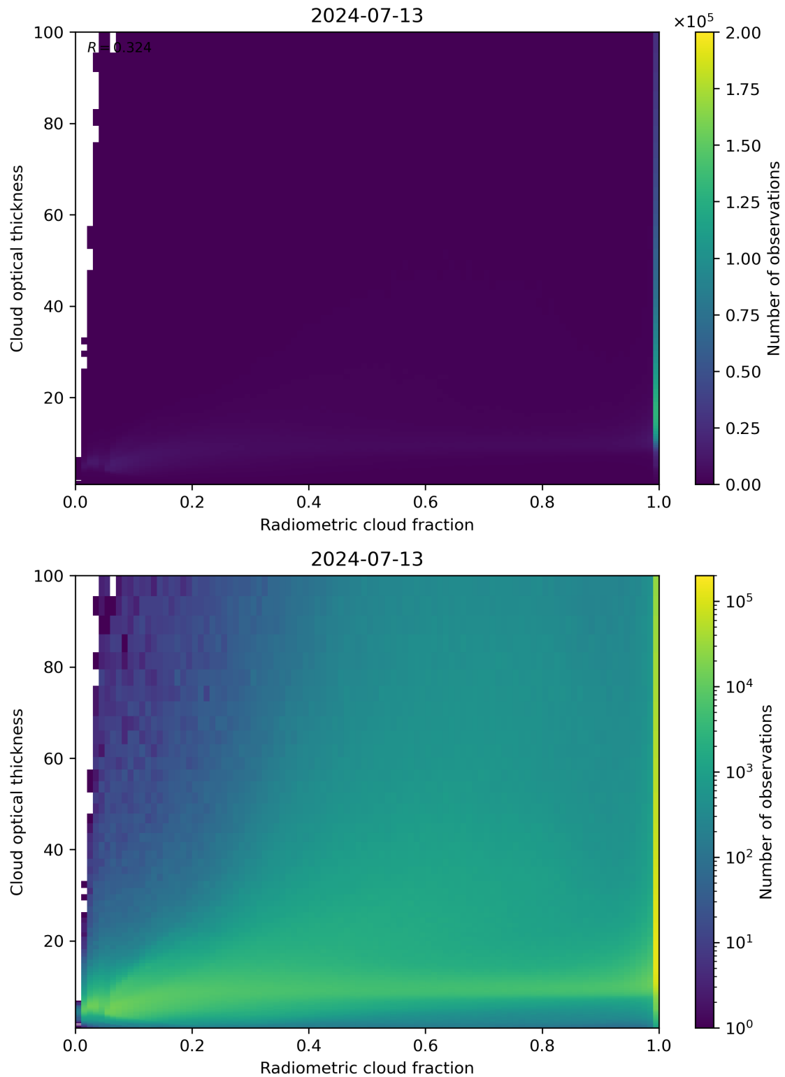
Figure 75: Scatter density plot of “Radiometric cloud fraction” against “Cloud optical thickness” for 2024-07-12 to 2024-07-14.
