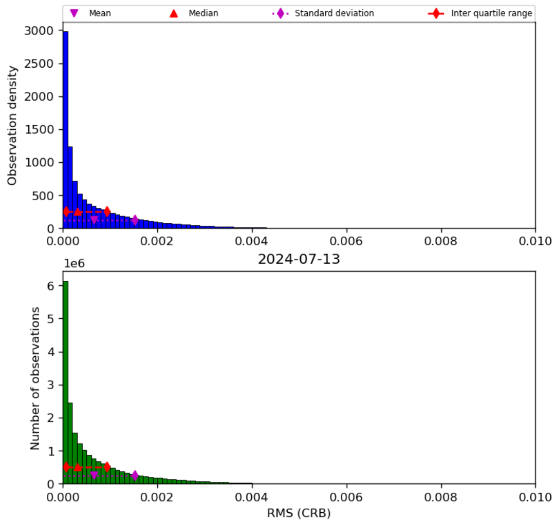
Figure 48: Histogram of “RMS (CRB)” for 2024-07-12 to 2024-07-14
