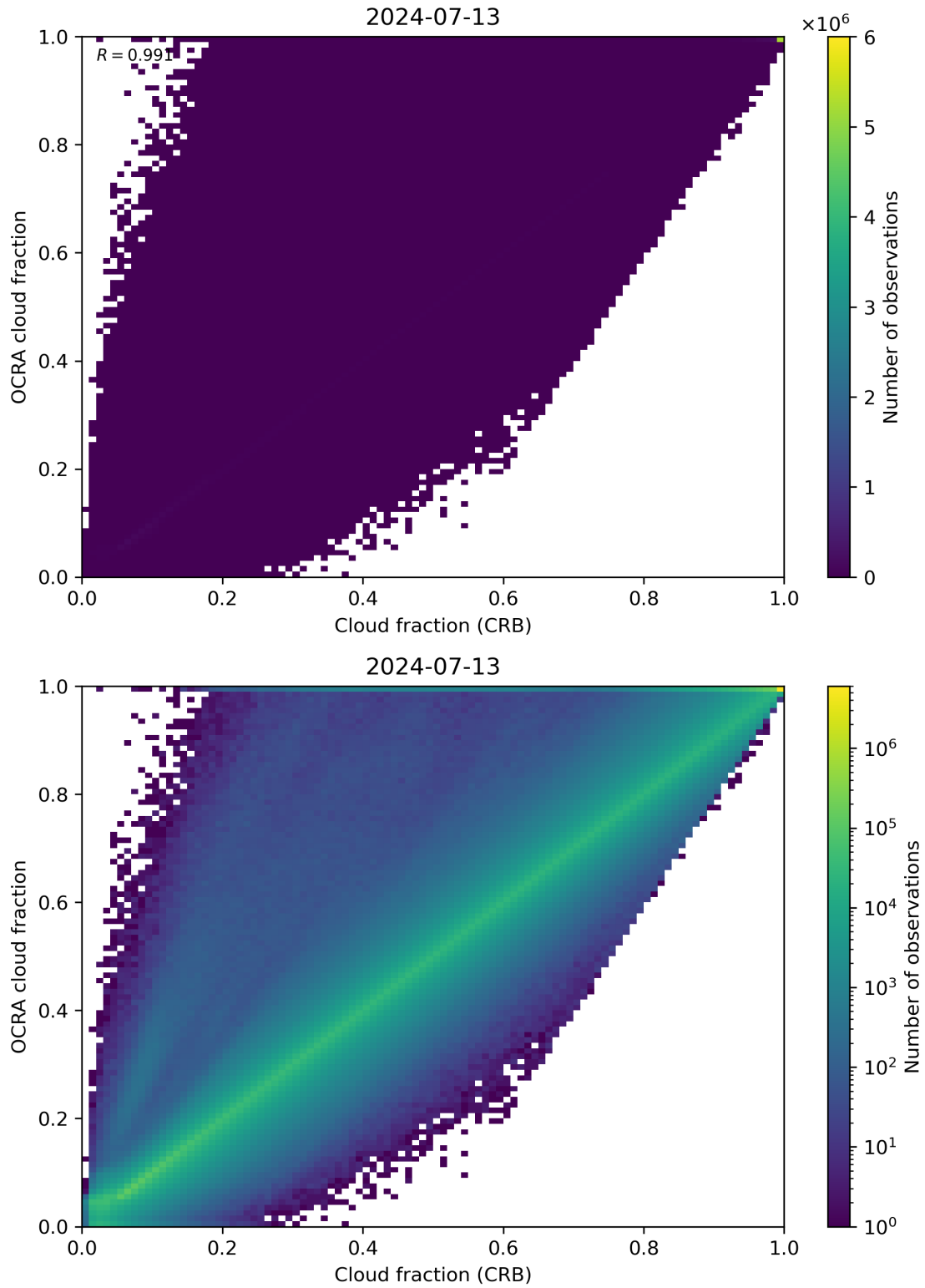
Figure 78: Scatter density plot of “Cloud fraction (CRB)” against “OCRA cloud fraction” for 2024-07-12 to 2024-07-14.
