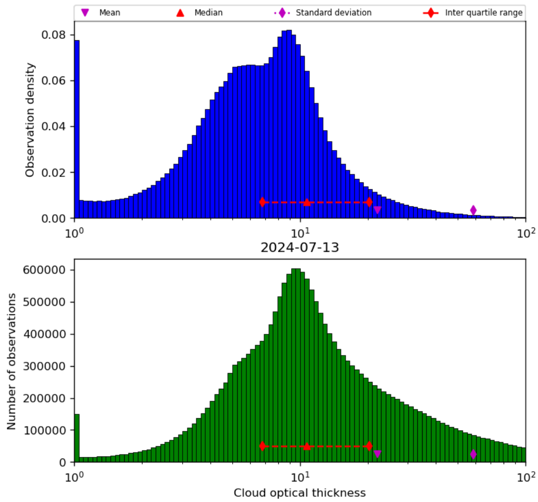
Figure 41: Histogram of “Cloud optical thickness” for 2024-07-12 to 2024-07-14
