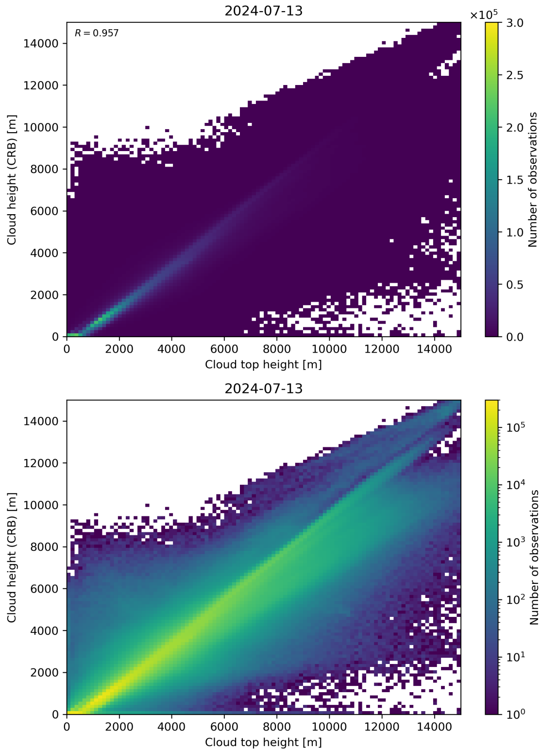
Figure 89: Scatter density plot of “Cloud top height” against “Cloud height (CRB)” for 2024-07-12 to 2024-07-14.
