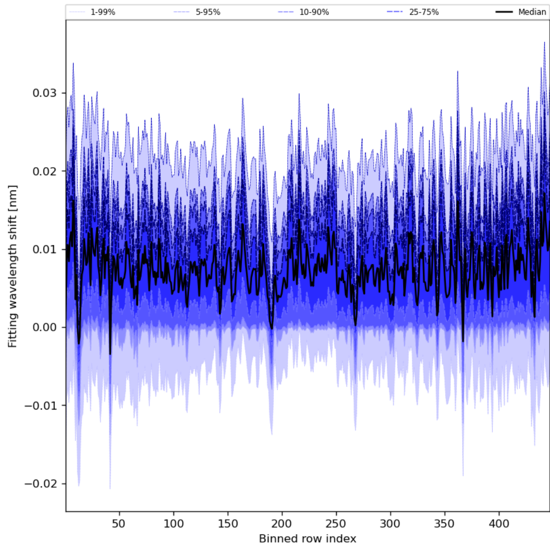
Figure 65: Along track statistics of “Fitting wavelength shift” for 2024-07-12 to 2024-07-14
