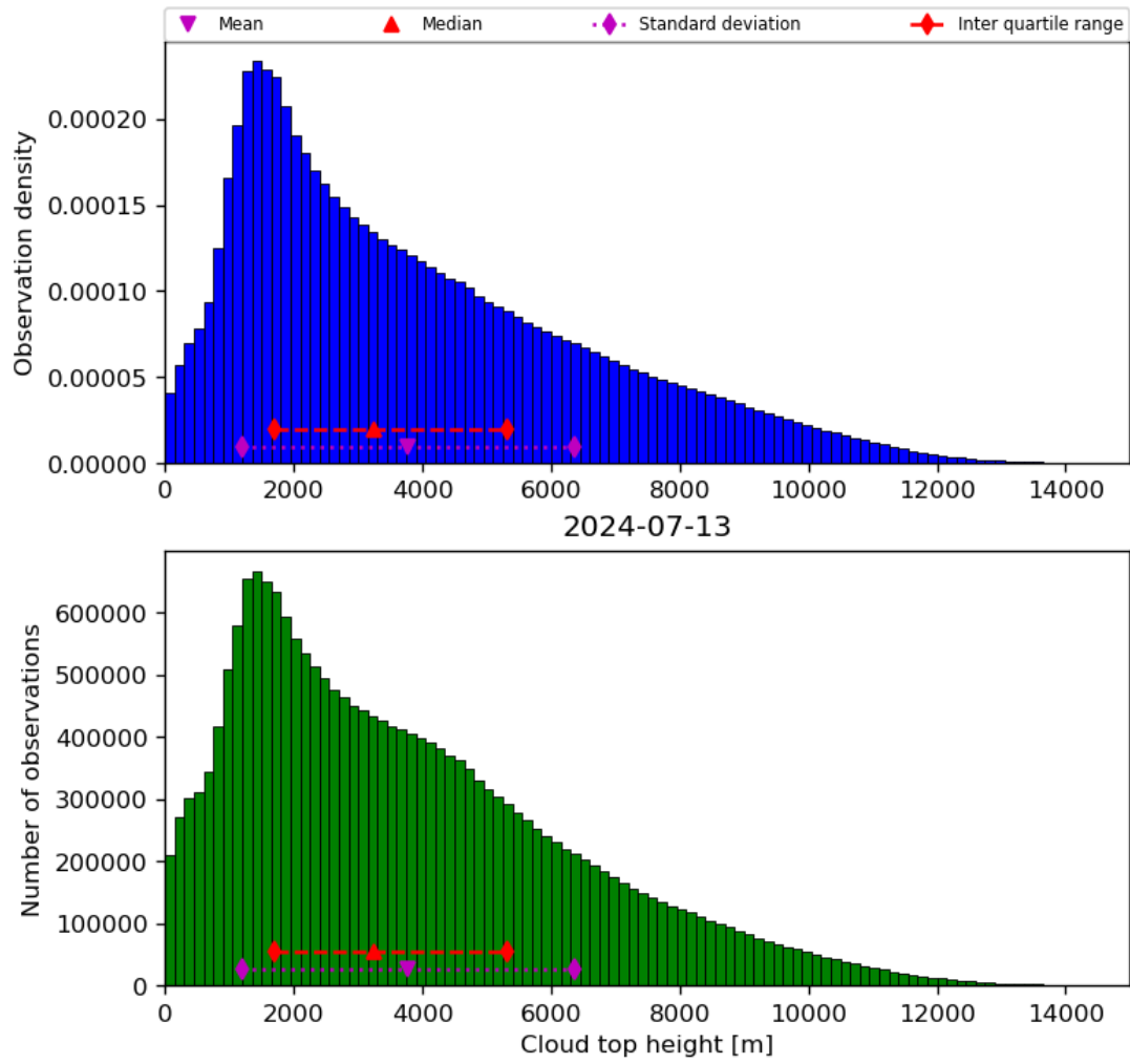
Figure 40: Histogram of “Cloud top height” for 2024-07-12 to 2024-07-14
