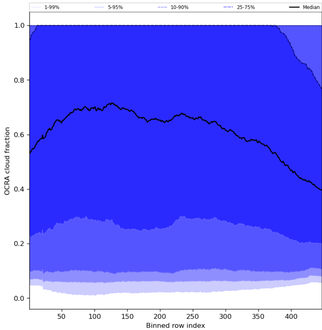
Figure 66: Along track statistics of “OCRA cloud fraction” for 2024-07-12 to 2024-07-14
