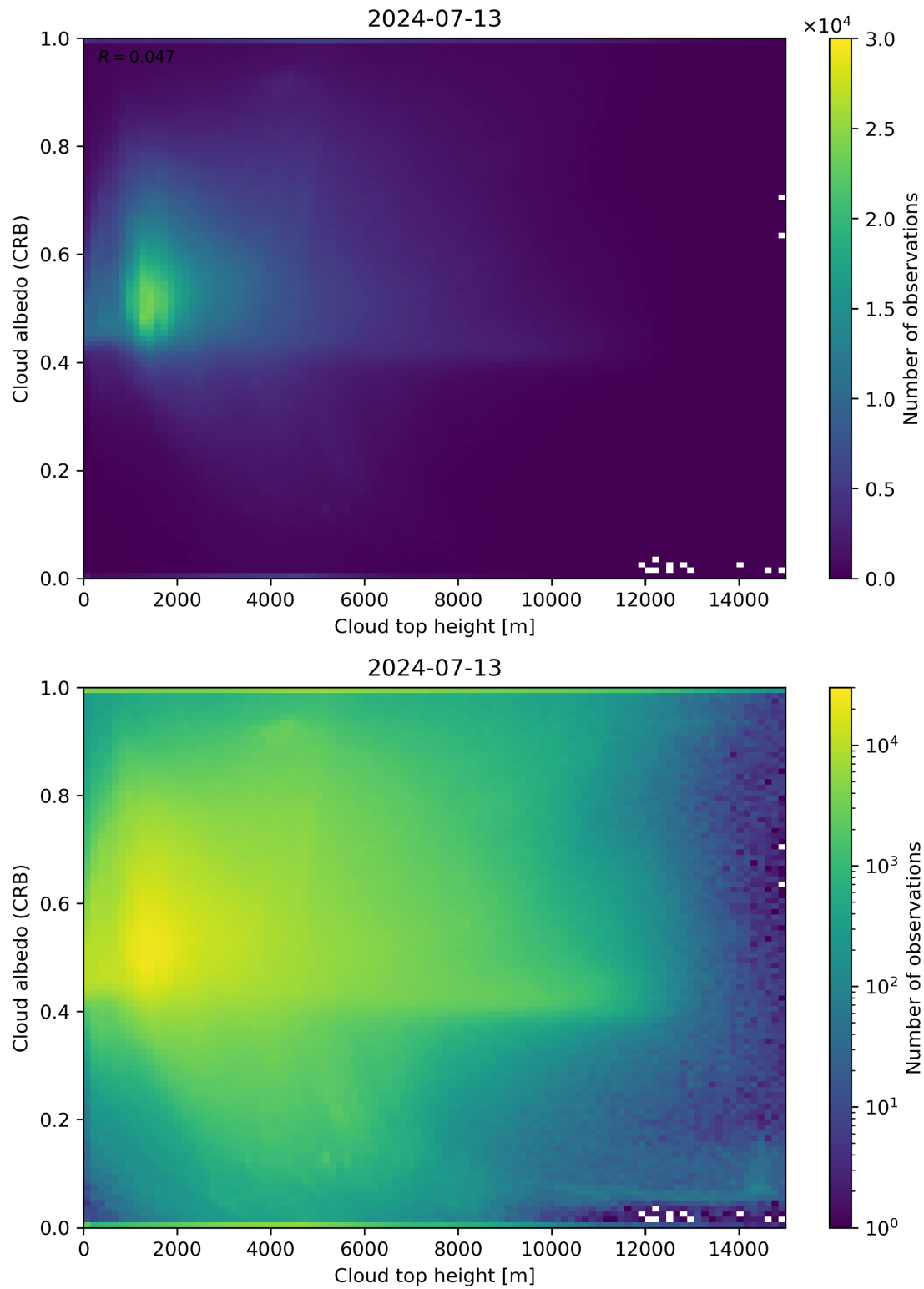
Figure 86: Scatter density plot of “Cloud top height” against “Cloud albedo (CRB)” for 2024-07-12 to 2024-07-14.
