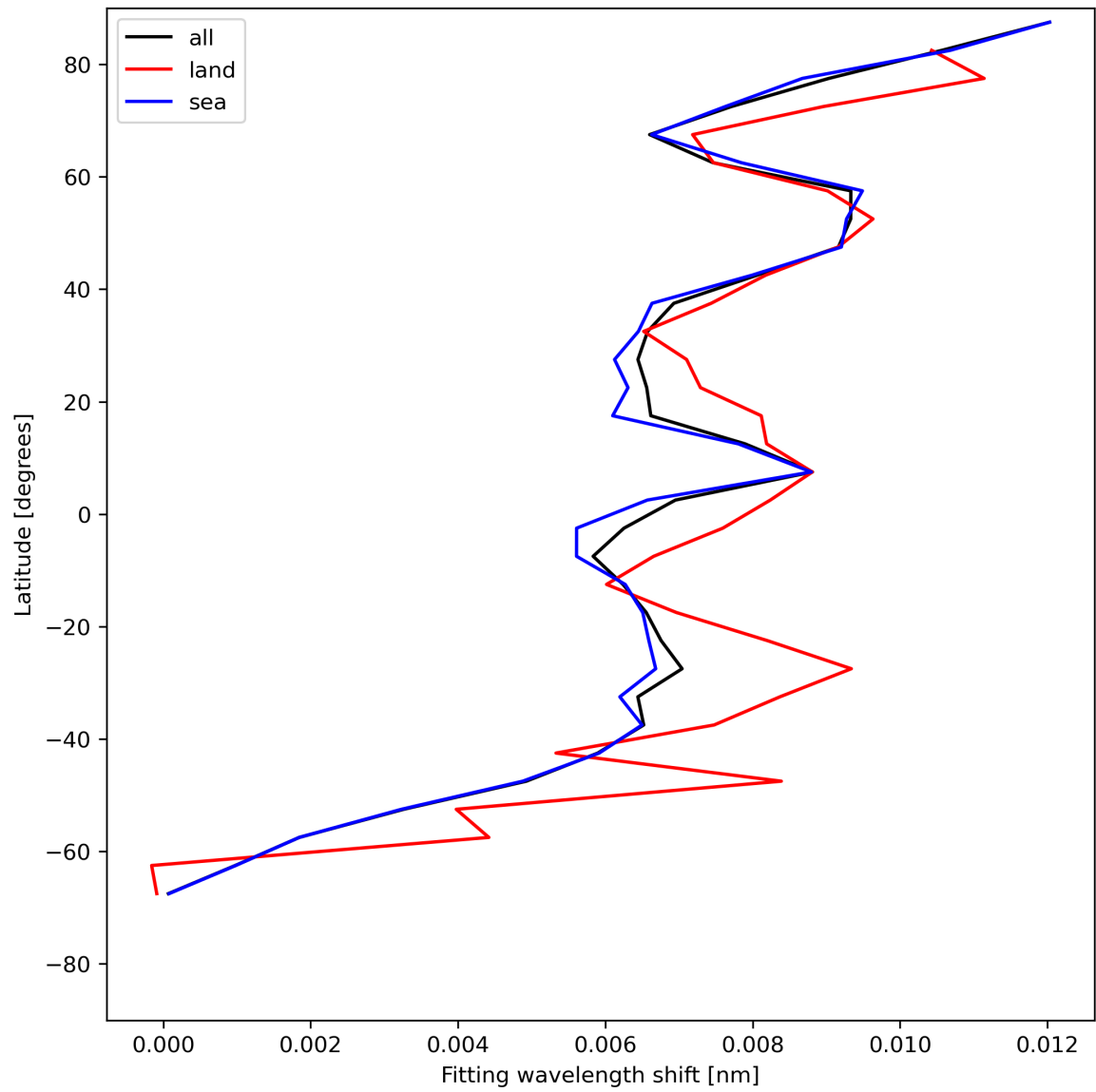
Figure 33: Zonal average of “Fitting wavelength shift” for 2024-07-12 to 2024-07-14.
