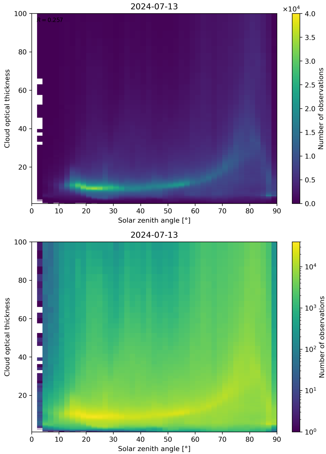
Figure 103: Scatter density plot of “Solar zenith angle” against “Cloud optical thickness” for 2024-07-12 to 2024-07-14.
