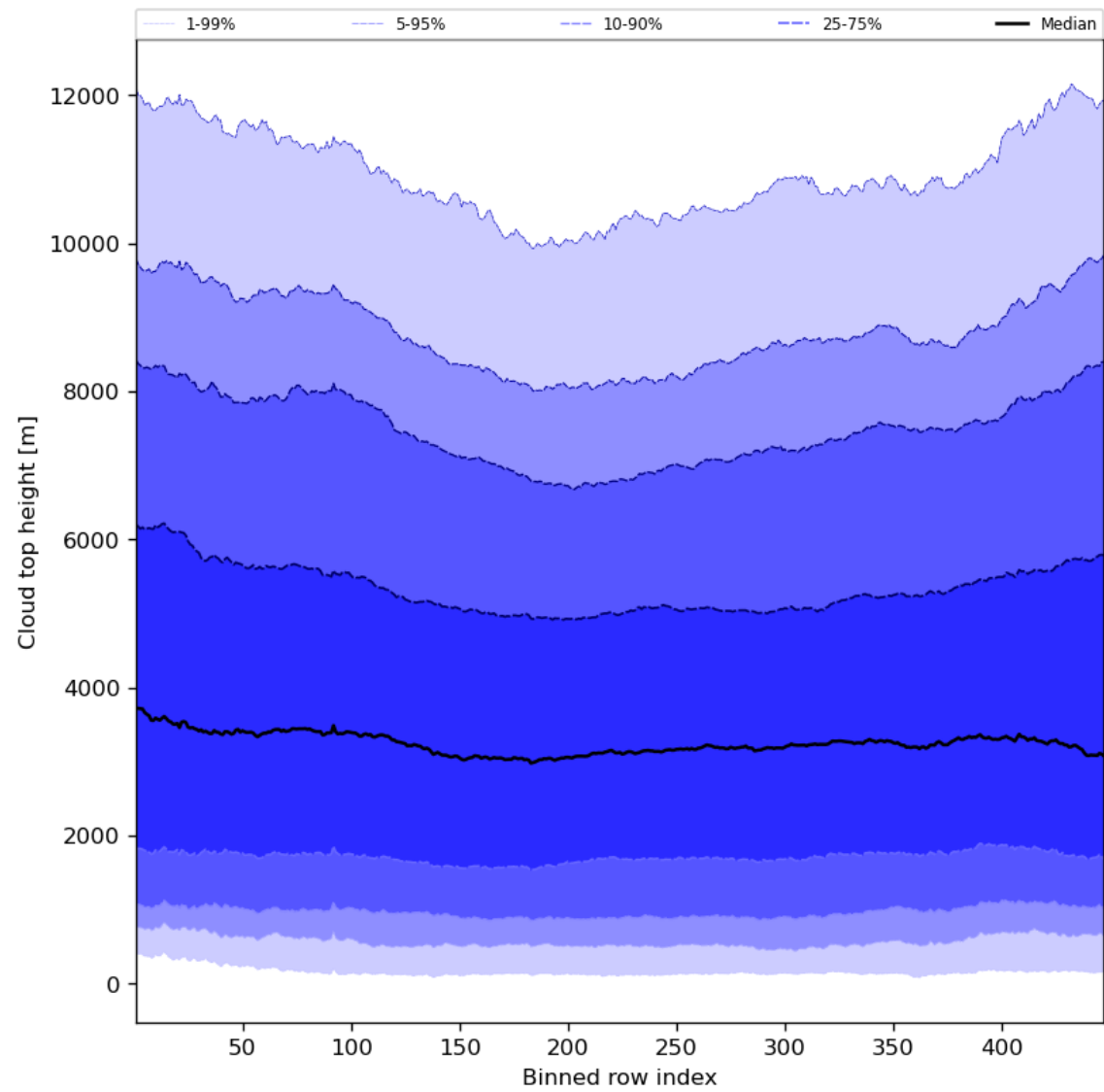
Figure 56: Along track statistics of “Cloud top height” for 2024-07-12 to 2024-07-14
