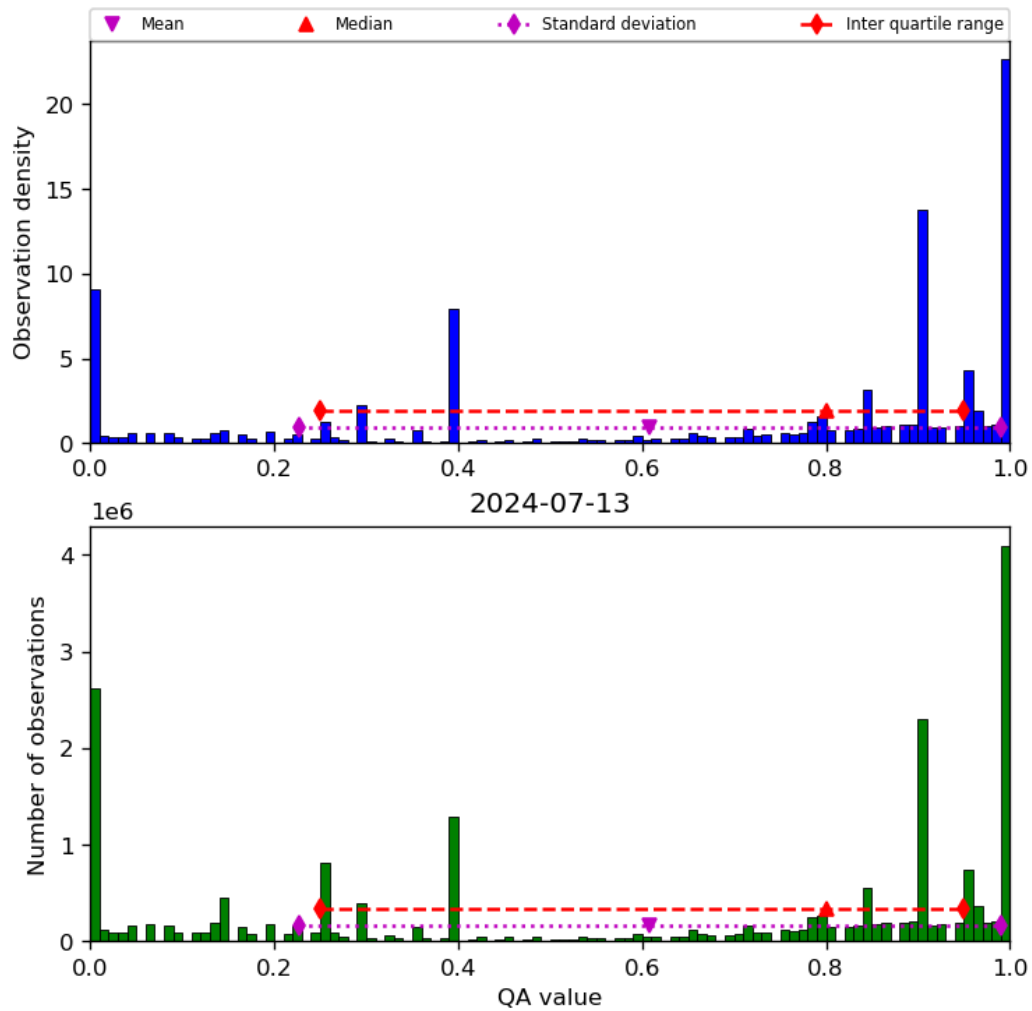
Figure 38: Histogram of “QA value” for 2024-07-12 to 2024-07-14
