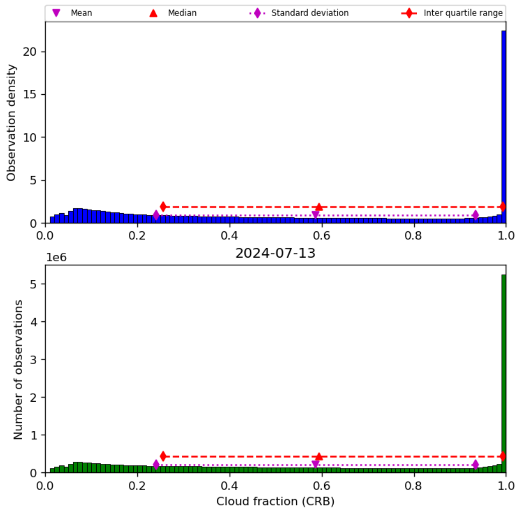
Figure 42: Histogram of “Cloud fraction (CRB)” for 2024-07-12 to 2024-07-14
