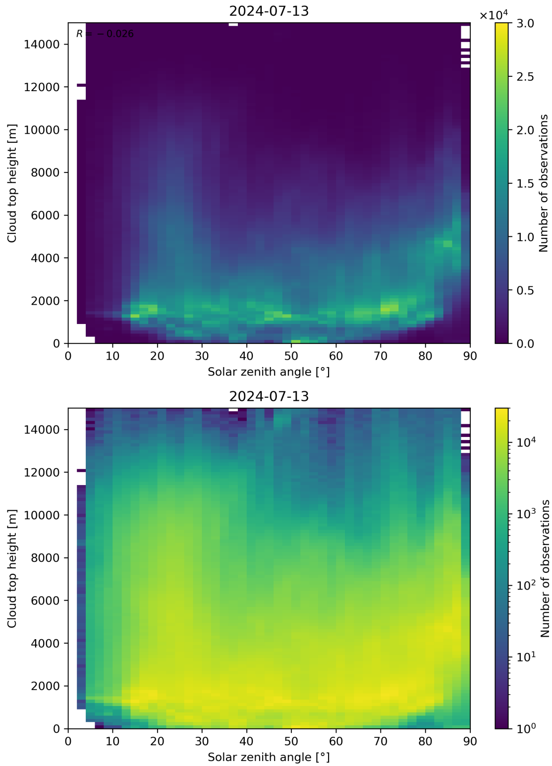
Figure 104: Scatter density plot of “Solar zenith angle” against “Cloud top height” for 2024-07-12 to 2024-07-14.
