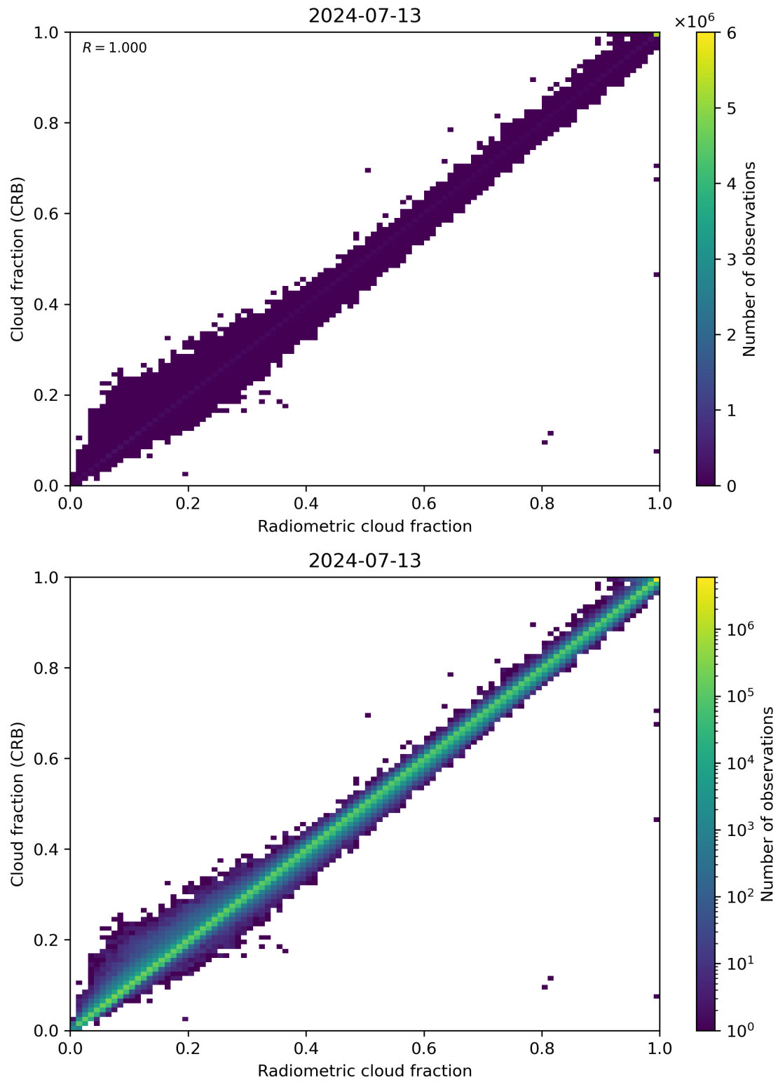
Figure 73: Scatter density plot of “Radiometric cloud fraction” against “Cloud fraction (CRB)” for 2024-07-12 to 2024-07-14.
