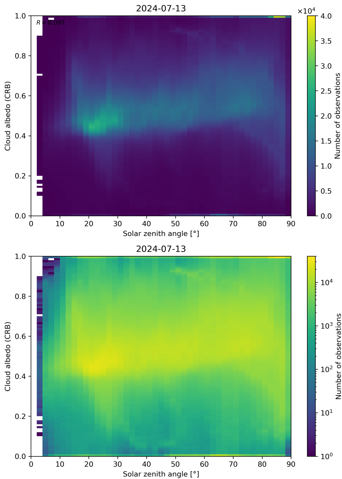
Figure 98: Scatter density plot of “Solar zenith angle” against “Cloud albedo (CRB)” for 2024-07-12 to 2024-07-14.
