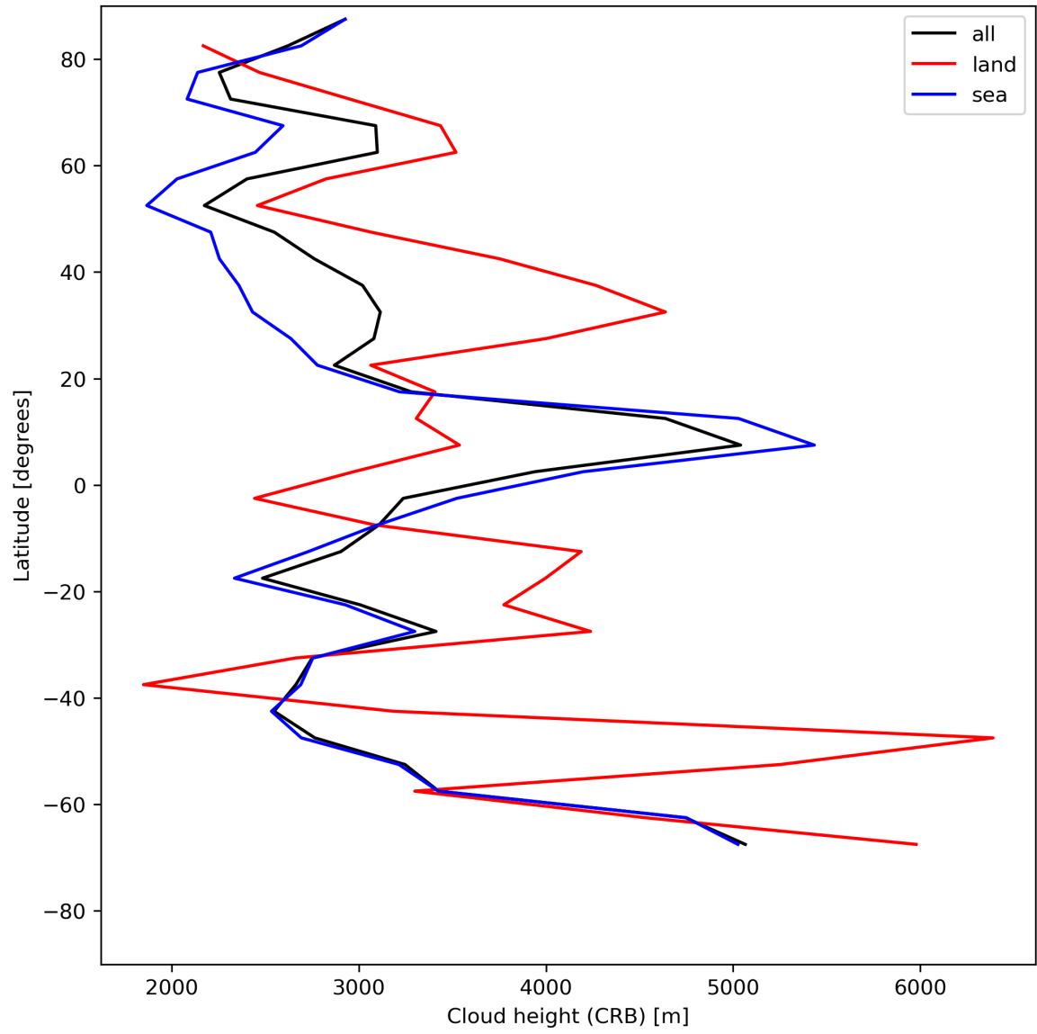
Figure 27: Zonal average of “Cloud height (CRB)” for 2024-07-12 to 2024-07-14.
