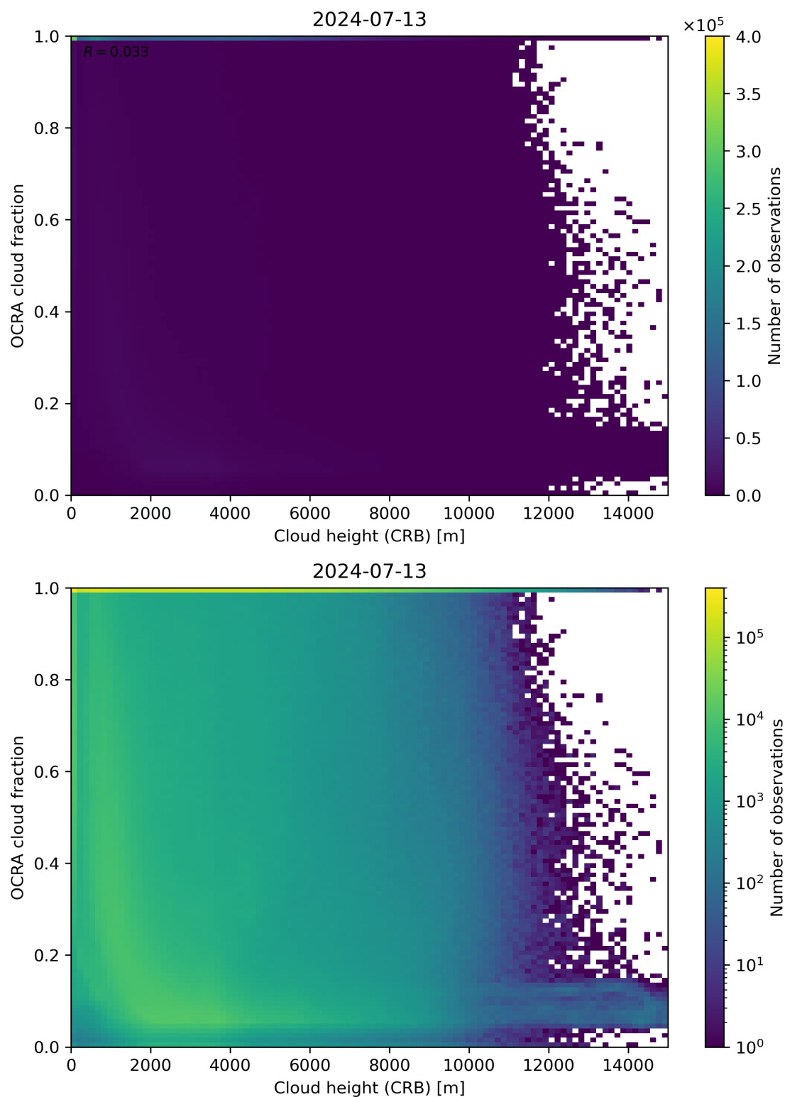
Figure 81: Scatter density plot of “Cloud height (CRB)” against “OCRA cloud fraction” for 2024-07-12 to 2024-07-14.
