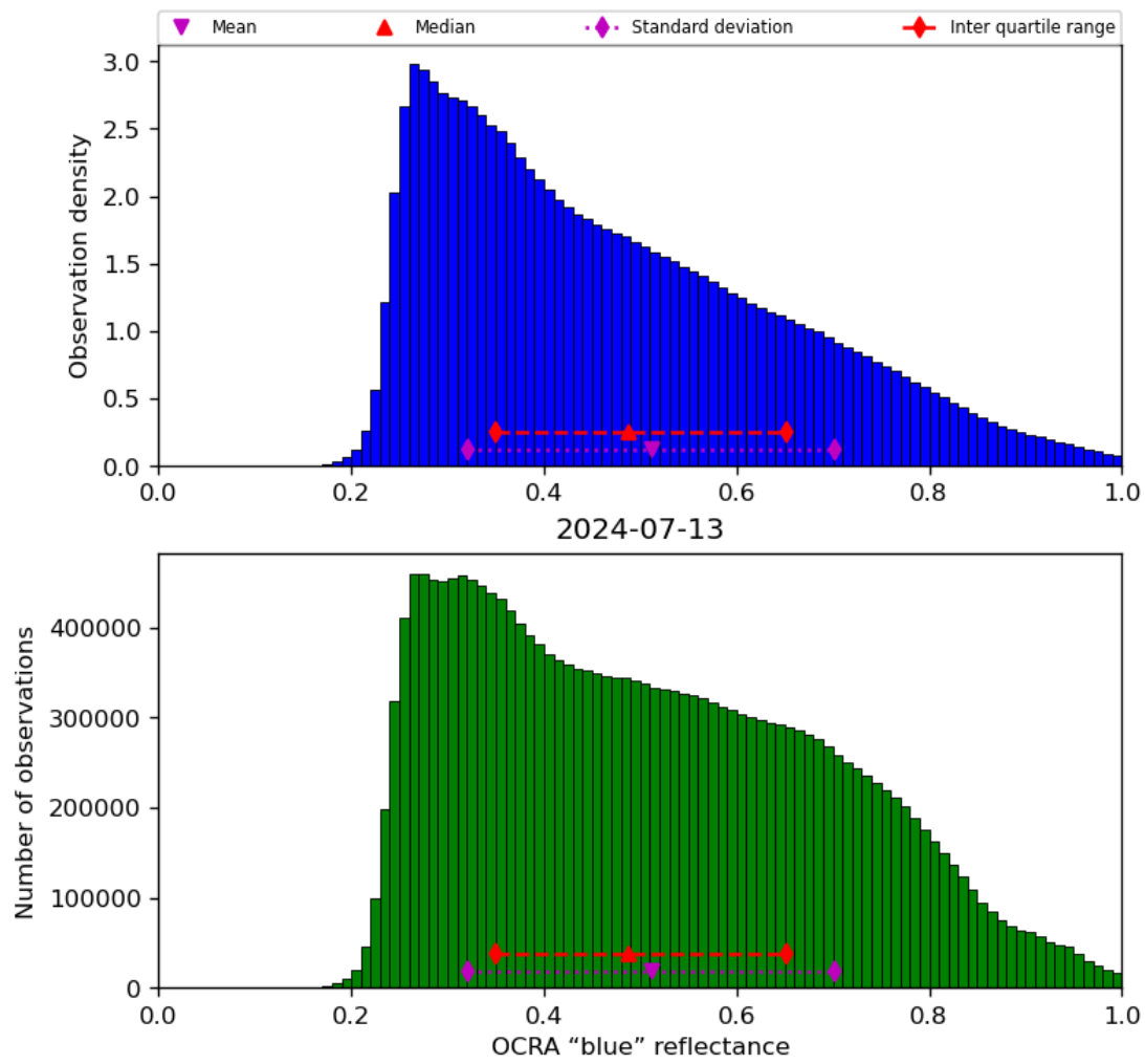
Figure 51: Histogram of “OCRA “blue” reflectance” for 2024-07-12 to 2024-07-14
