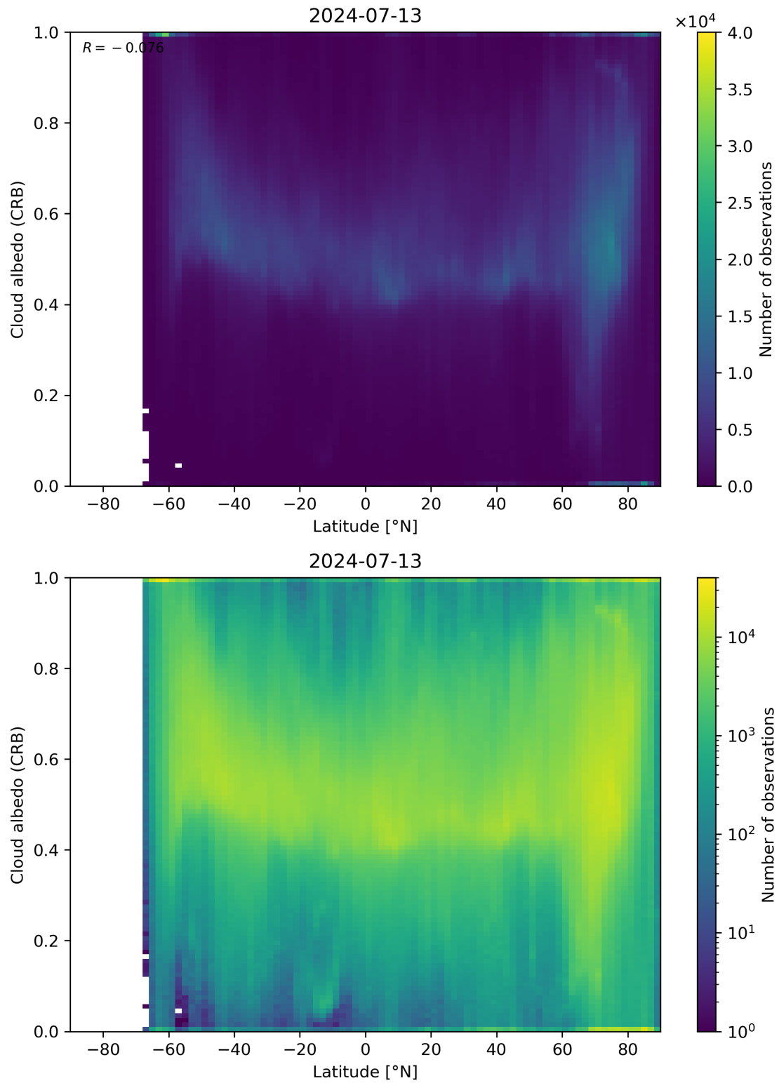
Figure 91: Scatter density plot of “Latitude” against “Cloud albedo (CRB)” for 2024-07-12 to 2024-07-14.
