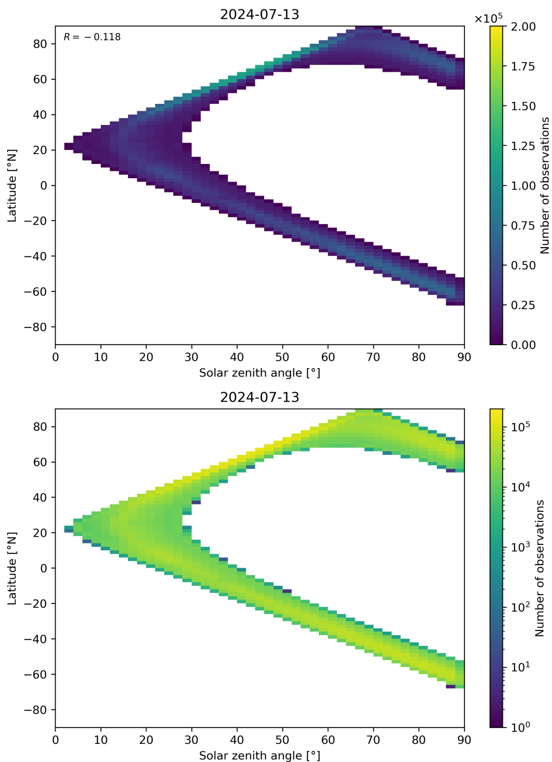
Figure 105: Scatter density plot of “Solar zenith angle” against “Latitude” for 2024-07-12 to 2024-07-14.
