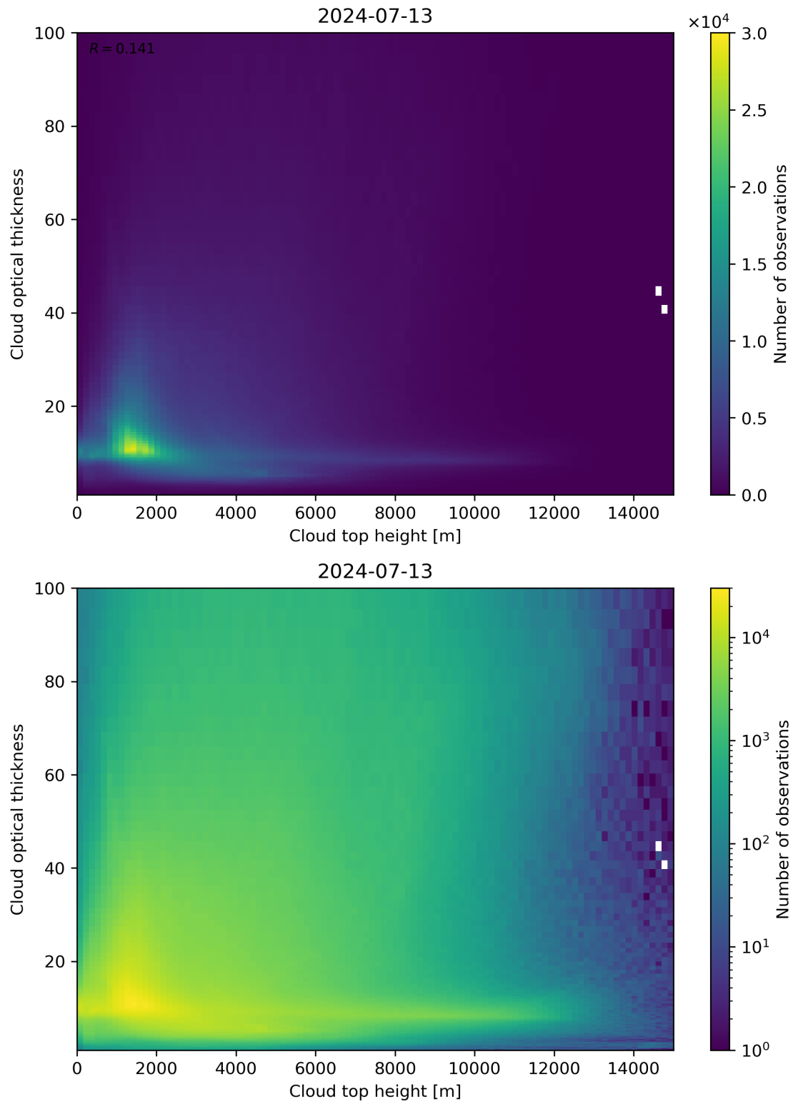
Figure 90: Scatter density plot of “Cloud top height” against “Cloud optical thickness” for 2024-07-12 to 2024-07-14.
