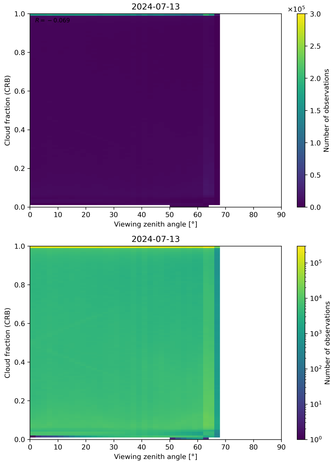
Figure 109: Scatter density plot of “Viewing zenith angle” against “Cloud fraction (CRB)” for 2024-07-12 to 2024-07-14.
