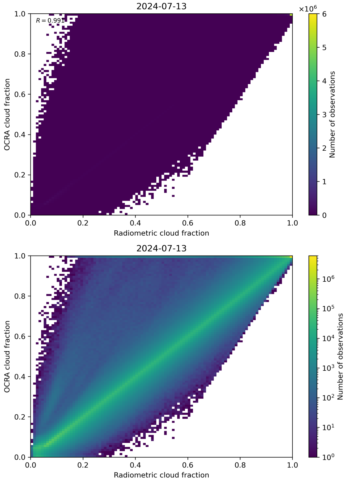
Figure 72: Scatter density plot of “Radiometric cloud fraction” against “OCRA cloud fraction” for 2024-07-12 to 2024-07-14.
