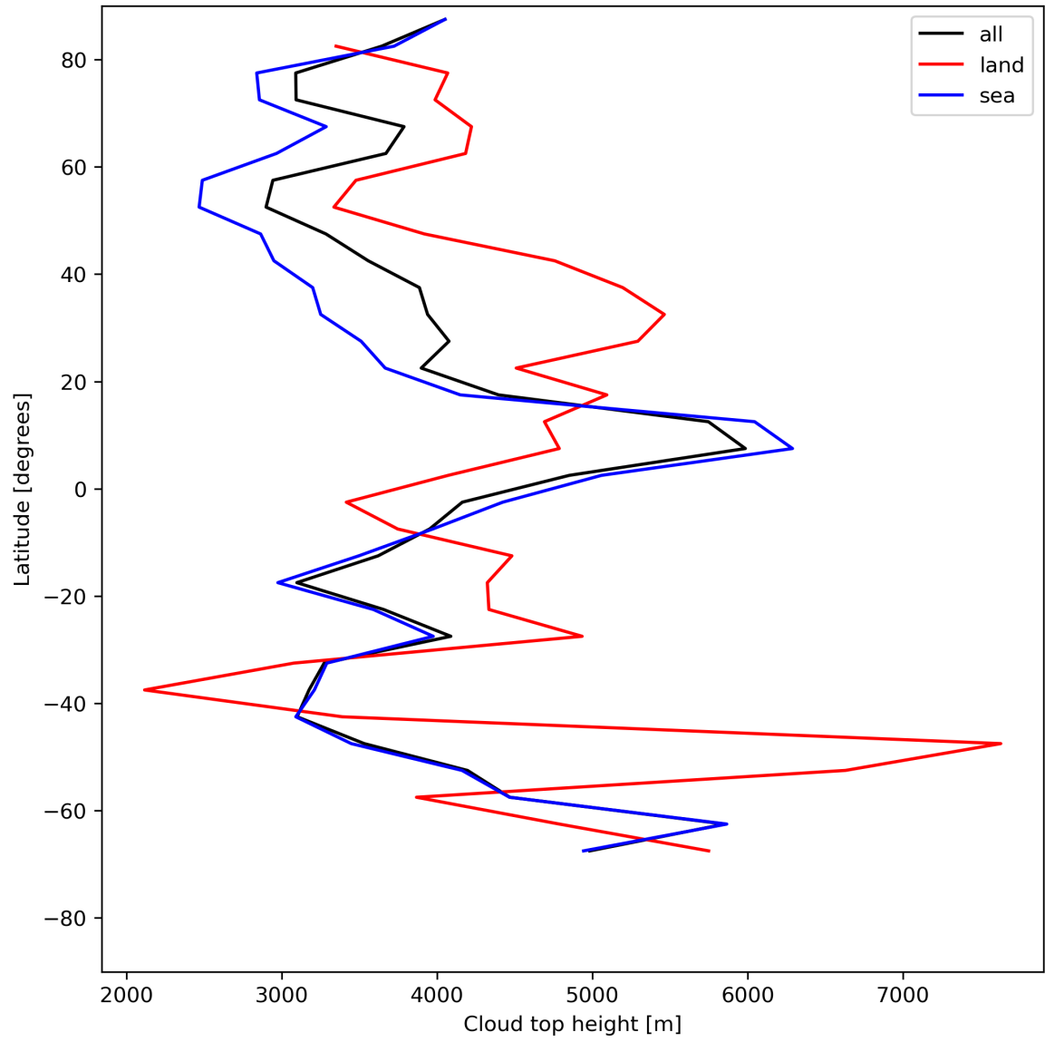
Figure 24: Zonal average of “Cloud top height” for 2024-07-12 to 2024-07-14.
