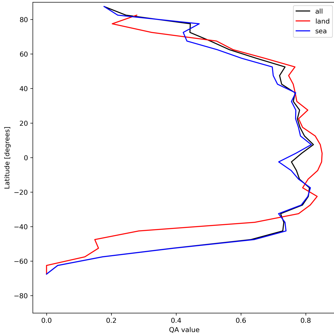
Figure 22: Zonal average of “QA value” for 2024-07-12 to 2024-07-14.
