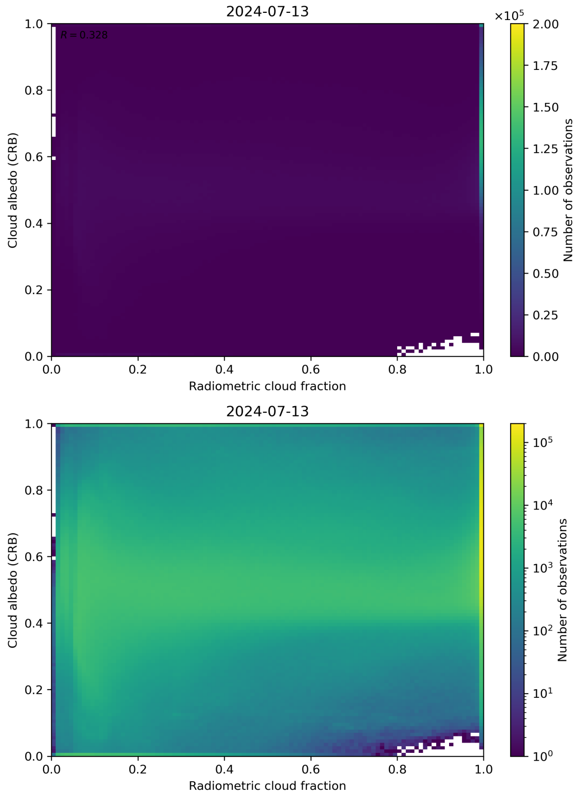
Figure 71: Scatter density plot of “Radiometric cloud fraction” against “Cloud albedo (CRB)” for 2024-07-12 to 2024-07-14.
