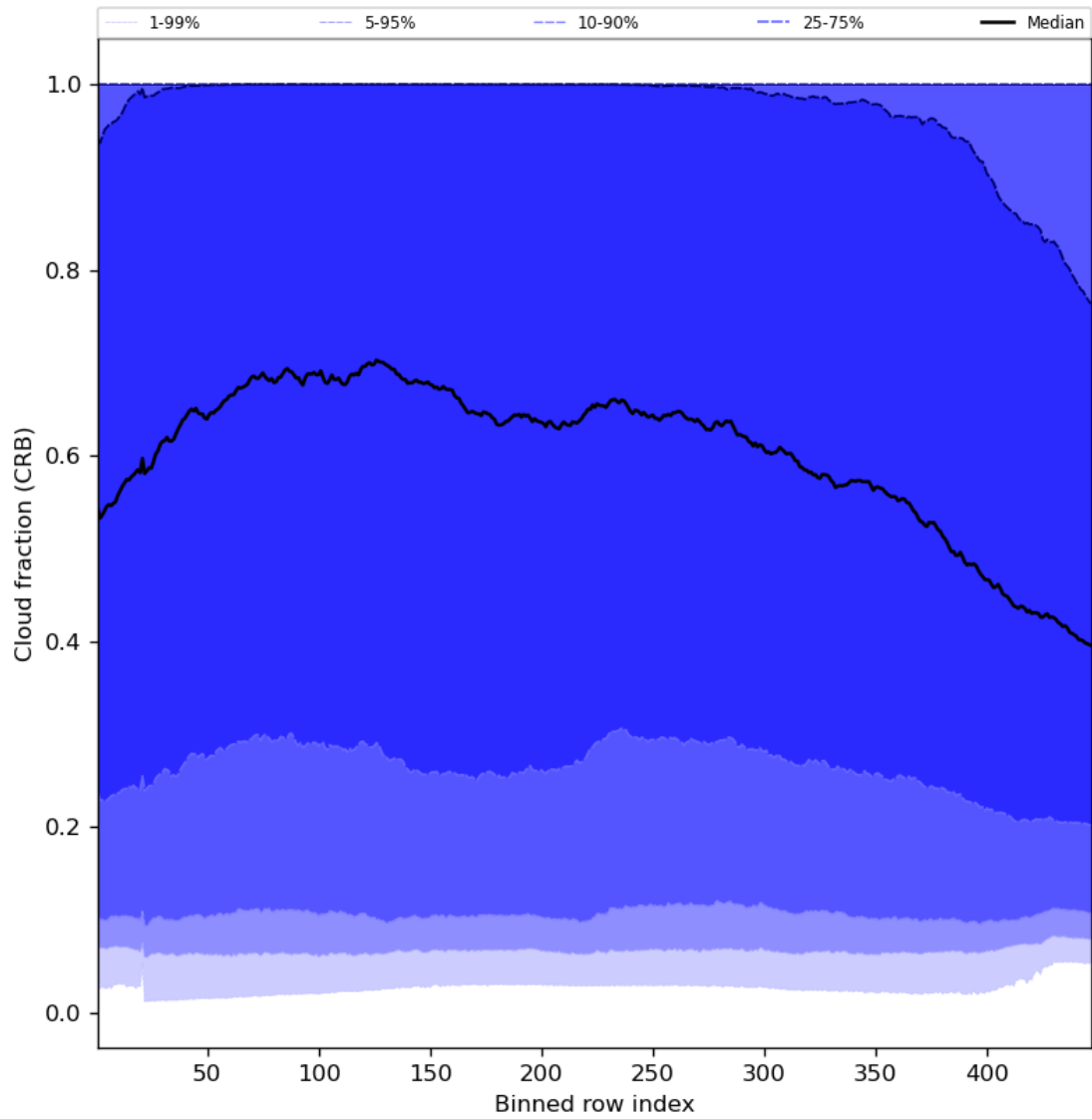
Figure 58: Along track statistics of “Cloud fraction (CRB)” for 2024-07-12 to 2024-07-14
