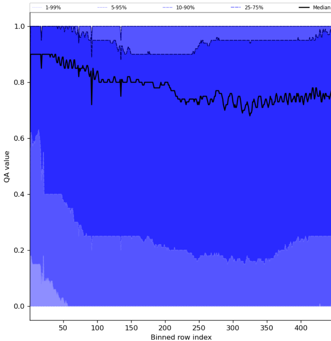
Figure 54: Along track statistics of “QA value” for 2024-07-12 to 2024-07-14
