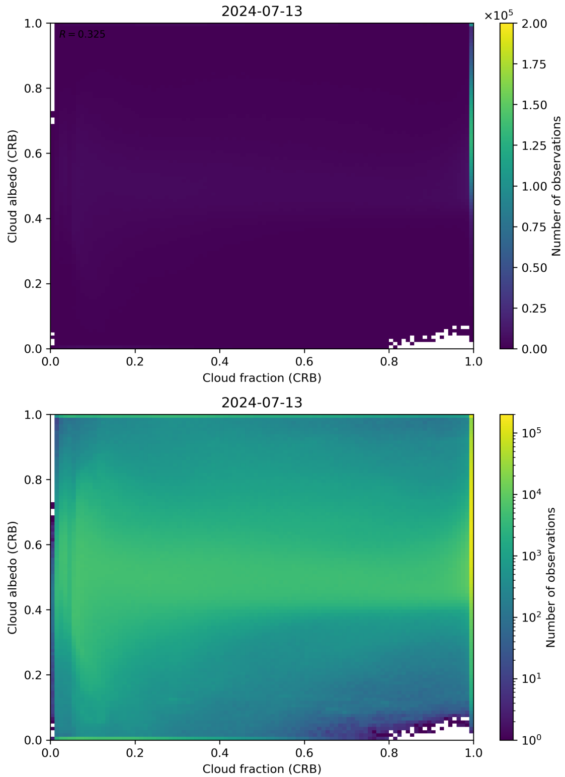
Figure 77: Scatter density plot of “Cloud fraction (CRB)” against “Cloud albedo (CRB)” for 2024-07-12 to 2024-07-14.
