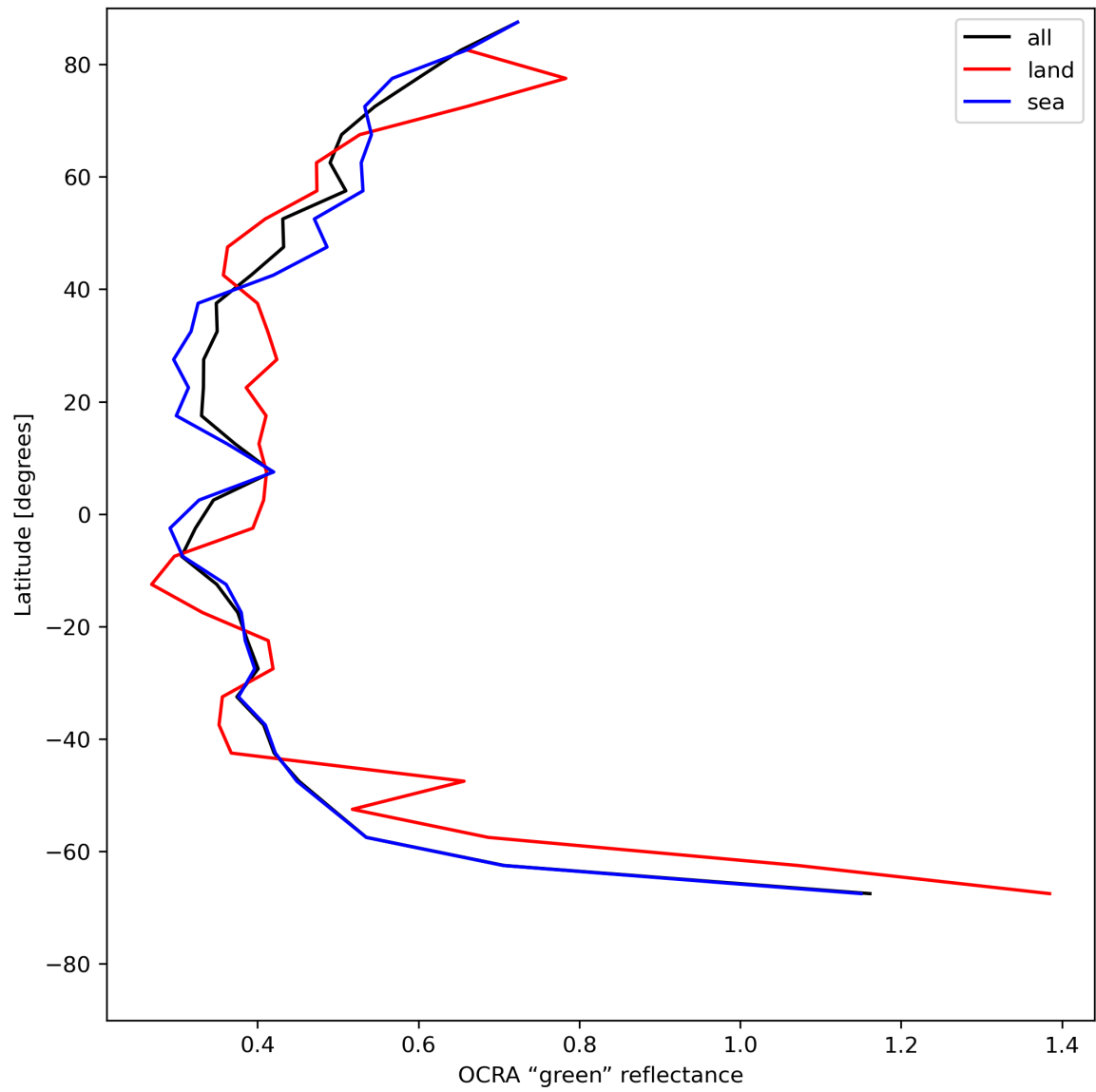
Figure 36: Zonal average of “OCRA “green” reflectance” for 2024-07-12 to 2024-07-14.
