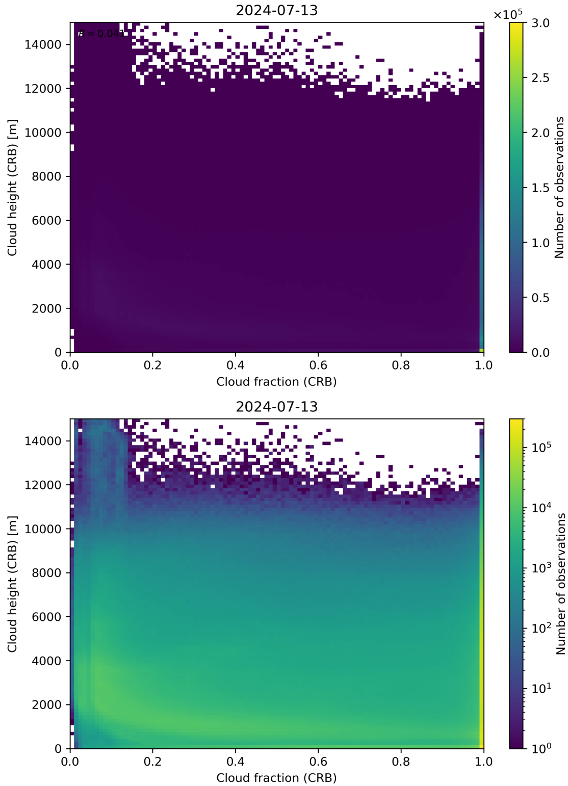
Figure 79: Scatter density plot of “Cloud fraction (CRB)” against “Cloud height (CRB)” for 2024-07-12 to 2024-07-14.
