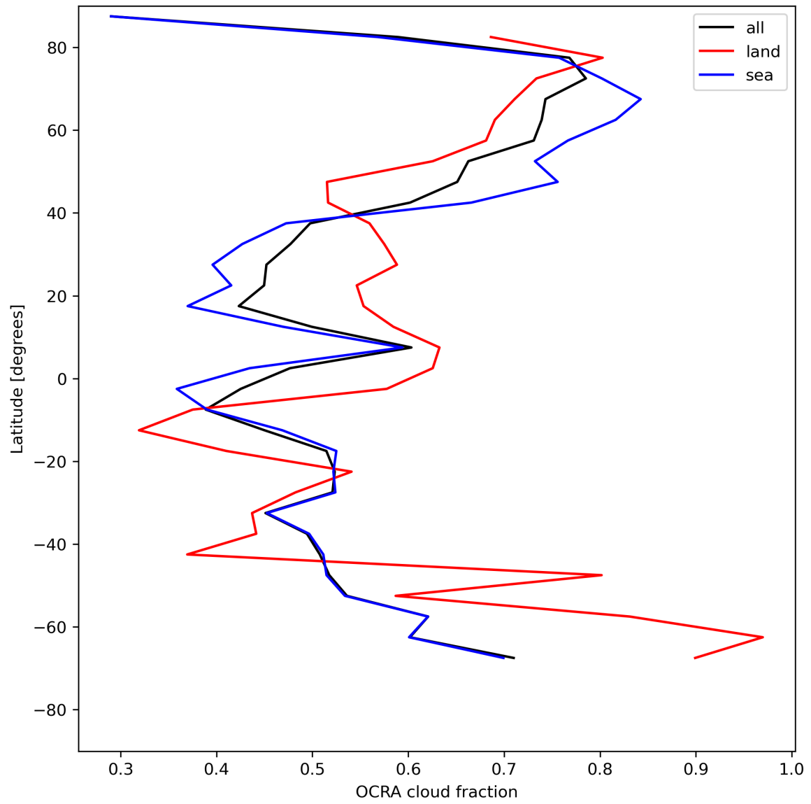
Figure 34: Zonal average of “OCRA cloud fraction” for 2024-07-12 to 2024-07-14.
