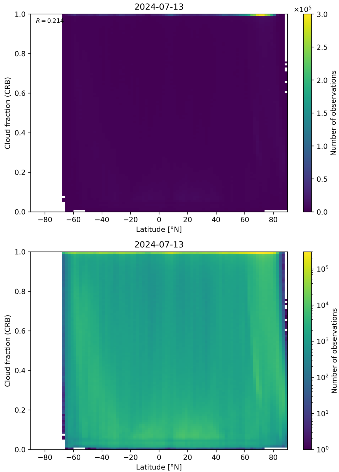
Figure 94: Scatter density plot of “Latitude” against “Cloud fraction (CRB)” for 2024-07-12 to 2024-07-14.
