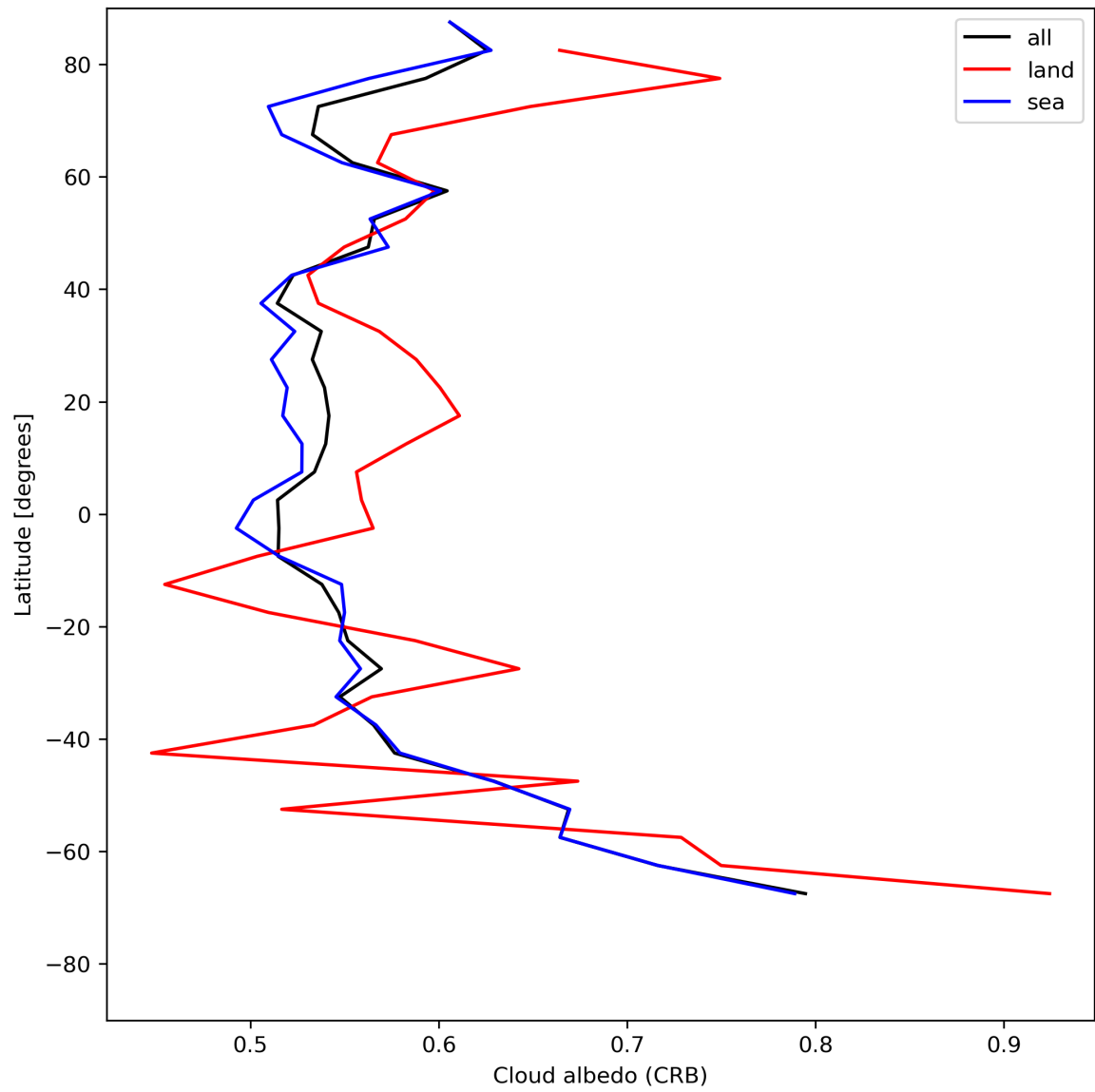
Figure 28: Zonal average of “Cloud albedo (CRB)” for 2024-07-12 to 2024-07-14.
