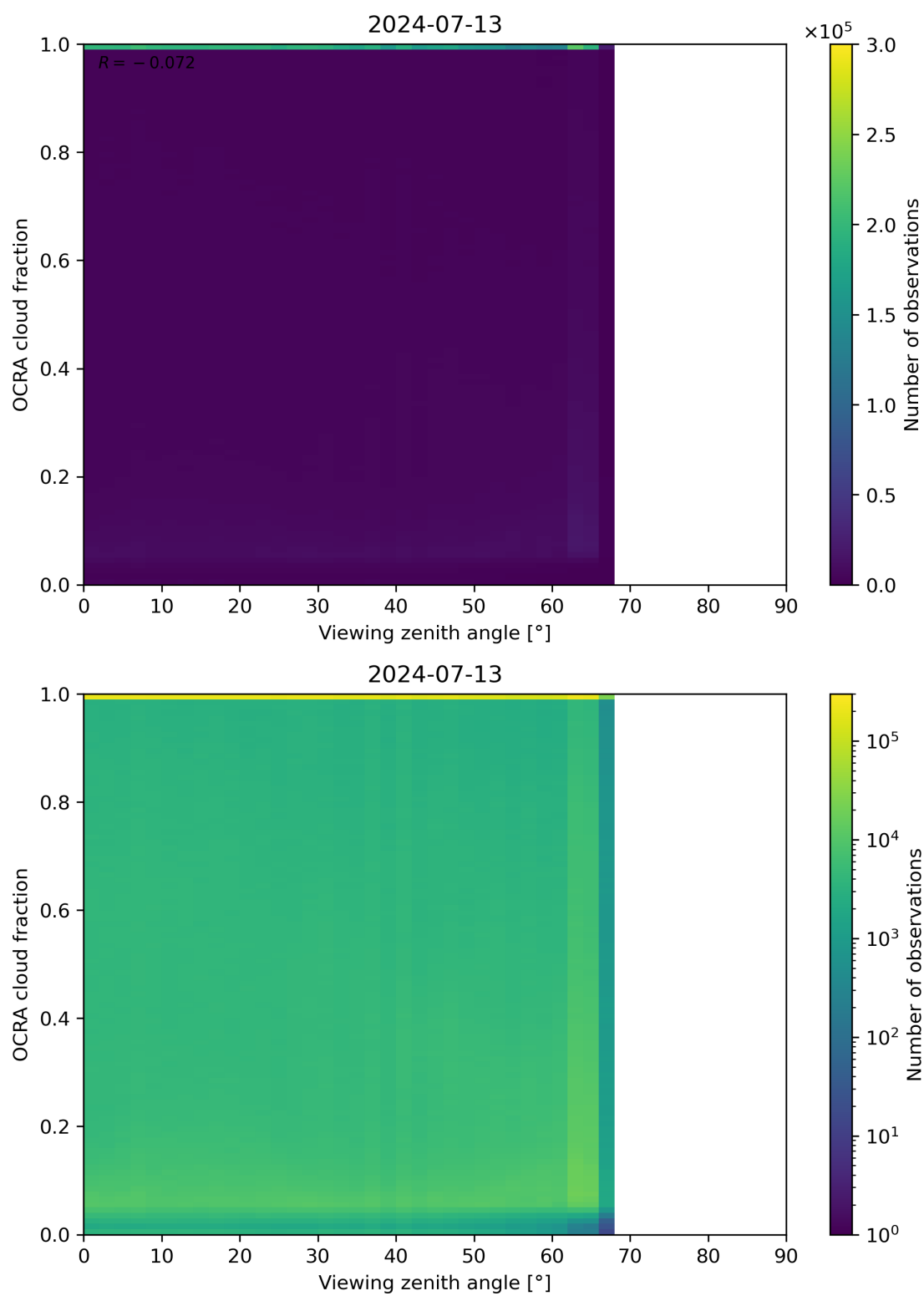
Figure 108: Scatter density plot of “Viewing zenith angle” against “OCRA cloud fraction” for 2024-07-12 to 2024-07-14.
