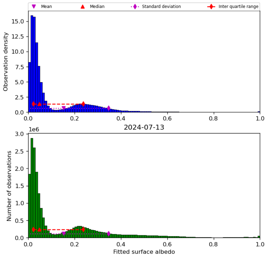
Figure 45: Histogram of “Fitted surface albedo” for 2024-07-12 to 2024-07-14
