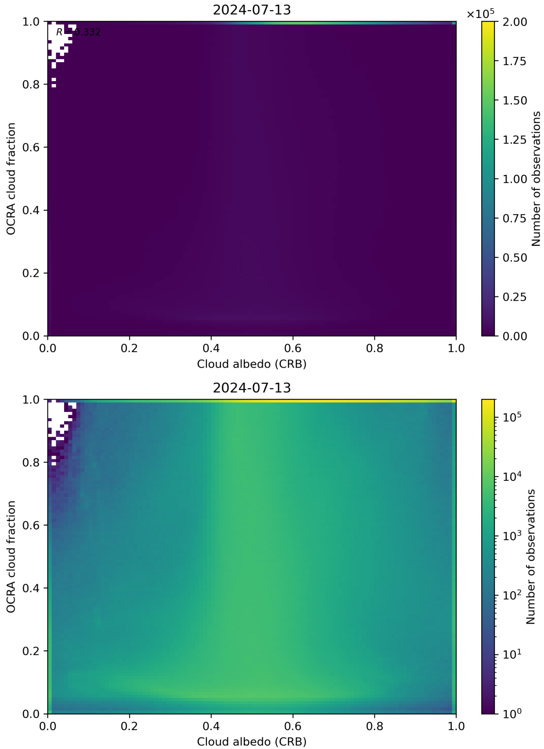
Figure 70: Scatter density plot of “Cloud albedo (CRB)” against “OCRA cloud fraction” for 2024-07-12 to 2024-07-14.
