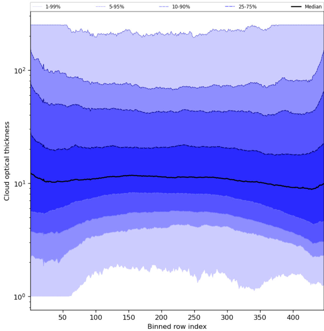
Figure 57: Along track statistics of “Cloud optical thickness” for 2024-07-12 to 2024-07-14
