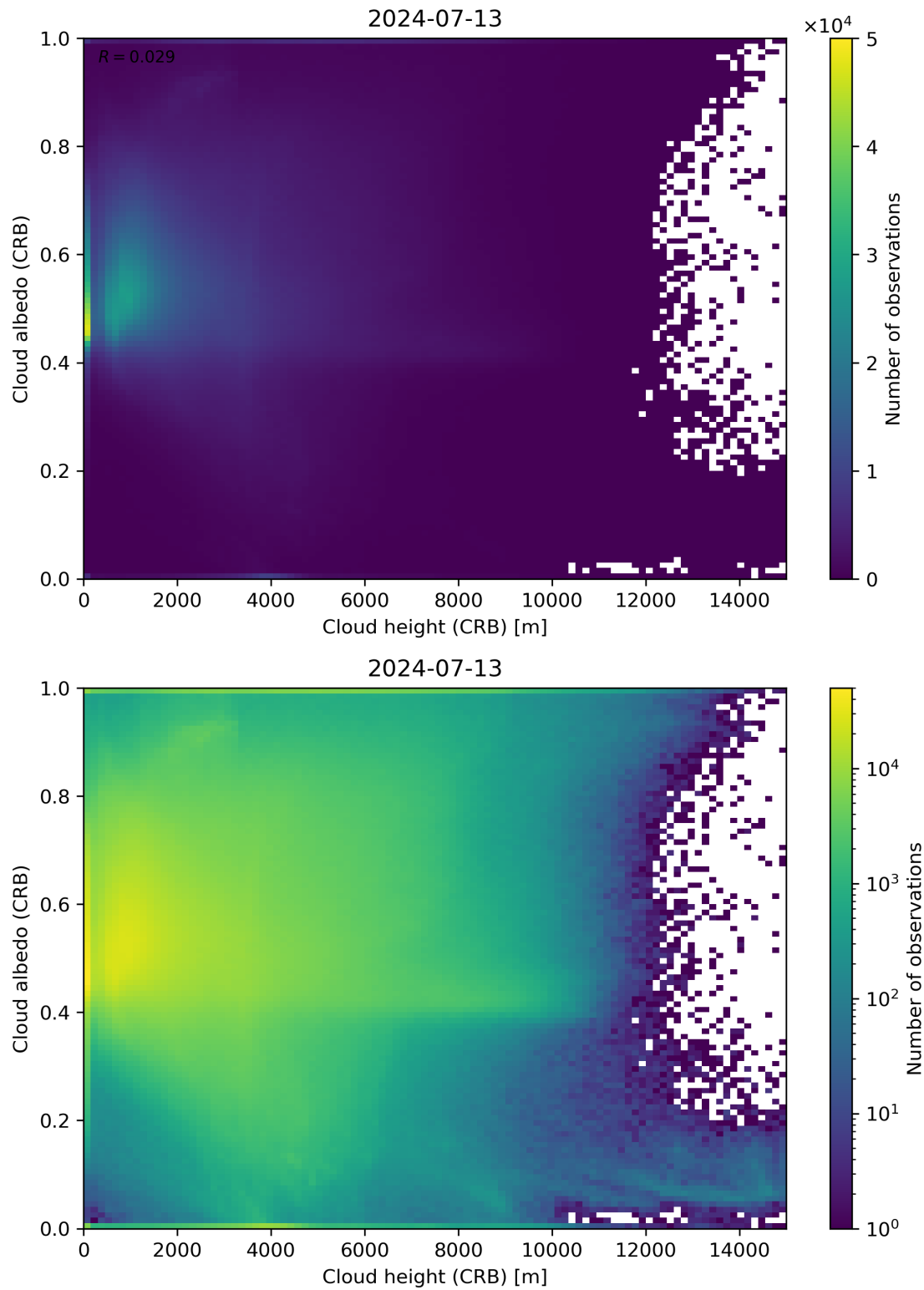
Figure 80: Scatter density plot of “Cloud height (CRB)” against “Cloud albedo (CRB)” for 2024-07-12 to 2024-07-14.
