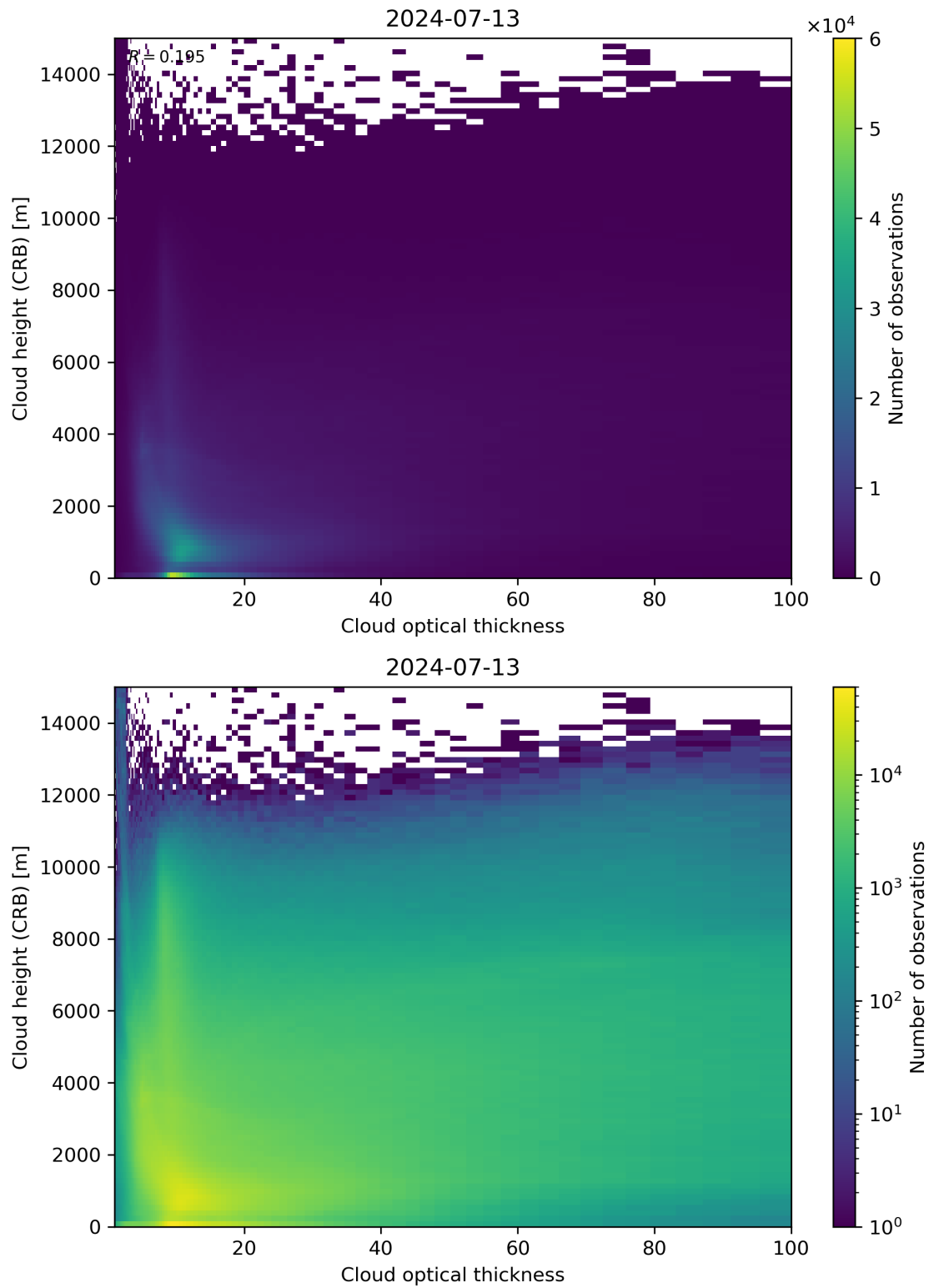
Figure 85: Scatter density plot of “Cloud optical thickness” against “Cloud height (CRB)” for 2024-07-12 to 2024-07-14.
