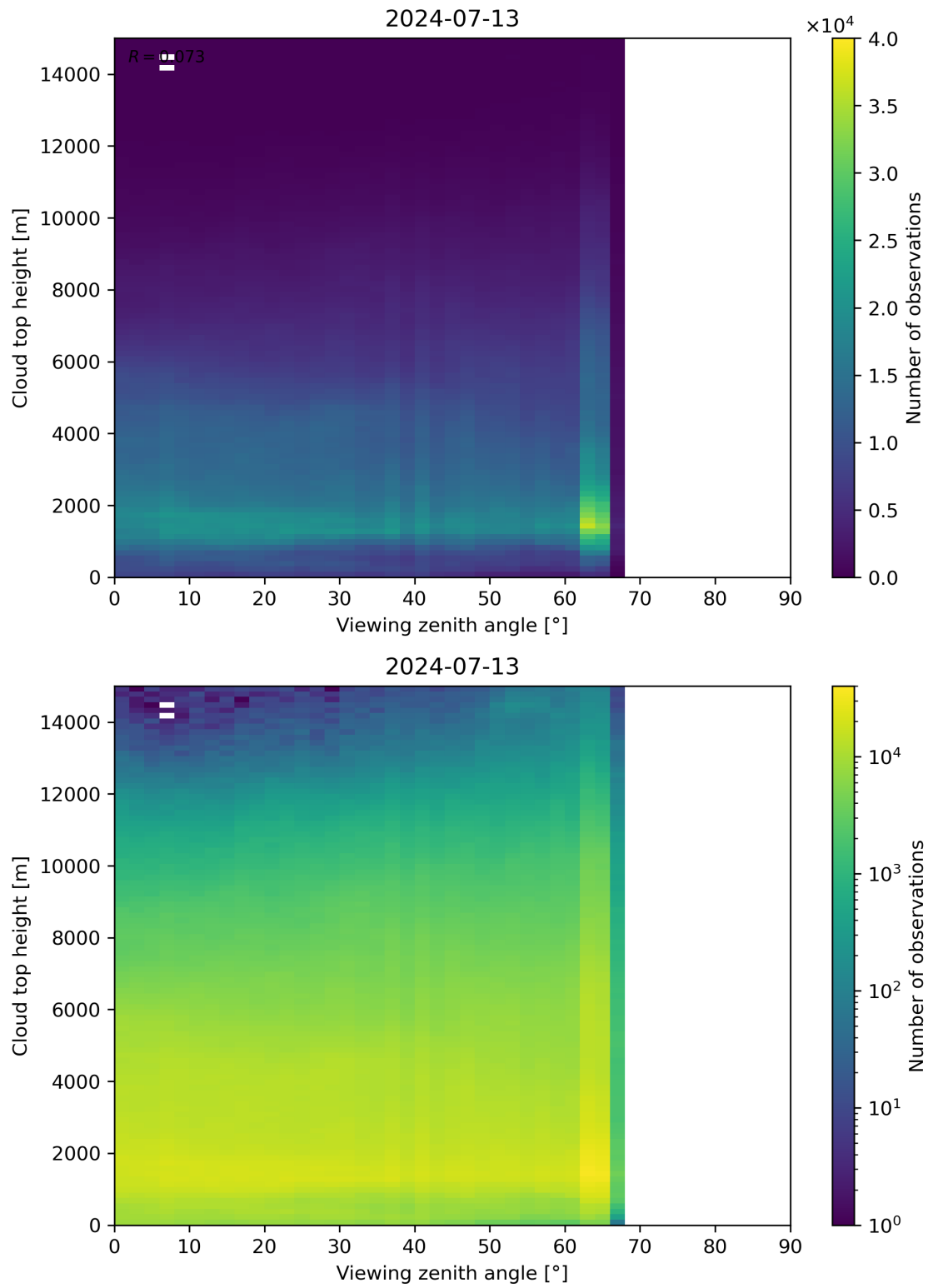
Figure 112: Scatter density plot of “Viewing zenith angle” against “Cloud top height” for 2024-07-12 to 2024-07-14.
