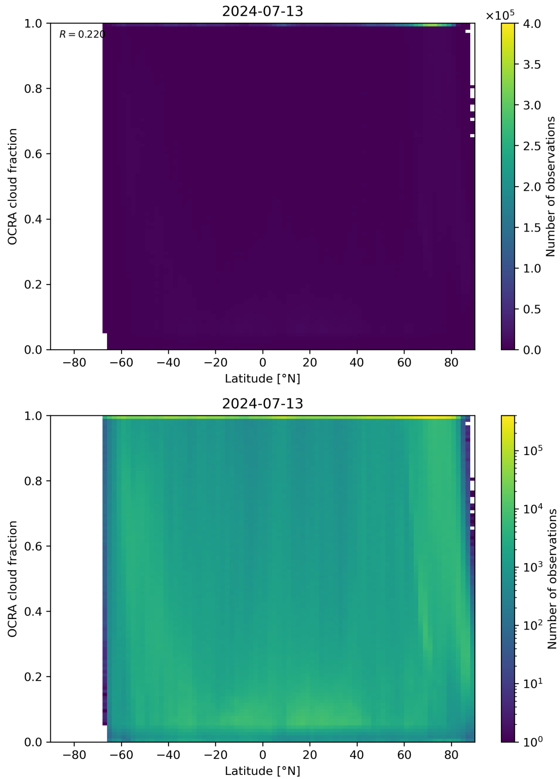
Figure 93: Scatter density plot of “Latitude” against “OCRA cloud fraction” for 2024-07-12 to 2024-07-14.
