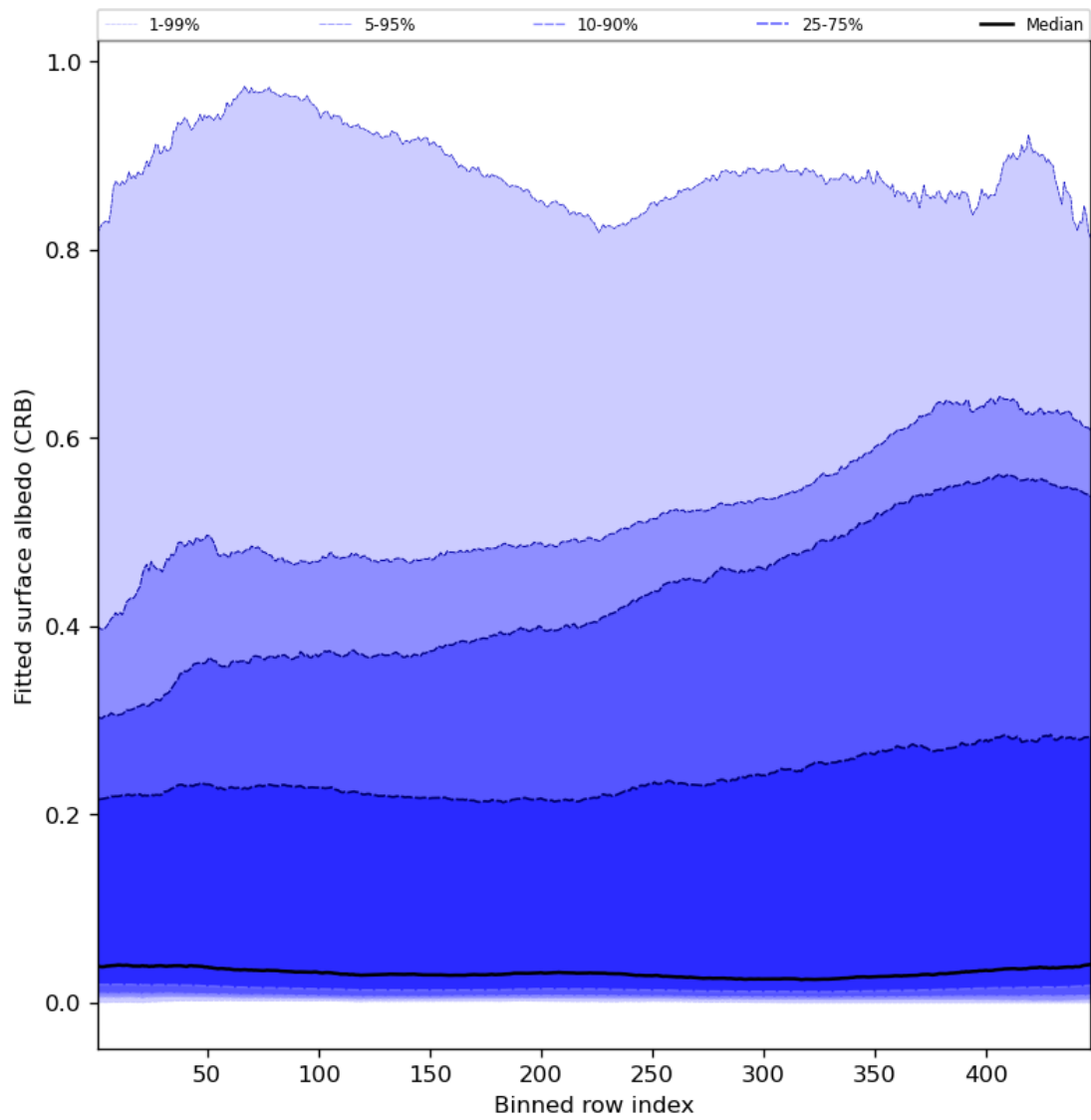
Figure 62: Along track statistics of “Fitted surface albedo (CRB)” for 2024-07-12 to 2024-07-14
