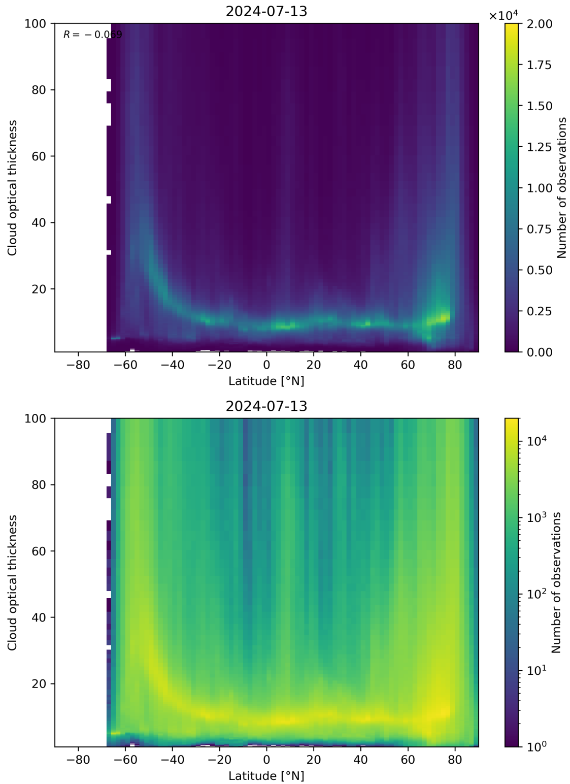
Figure 96: Scatter density plot of “Latitude” against “Cloud optical thickness” for 2024-07-12 to 2024-07-14.
