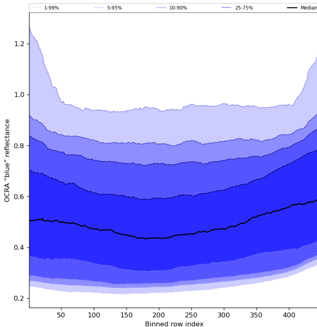
Figure 67: Along track statistics of “OCRA “blue” reflectance” for 2024-07-12 to 2024-07-14
