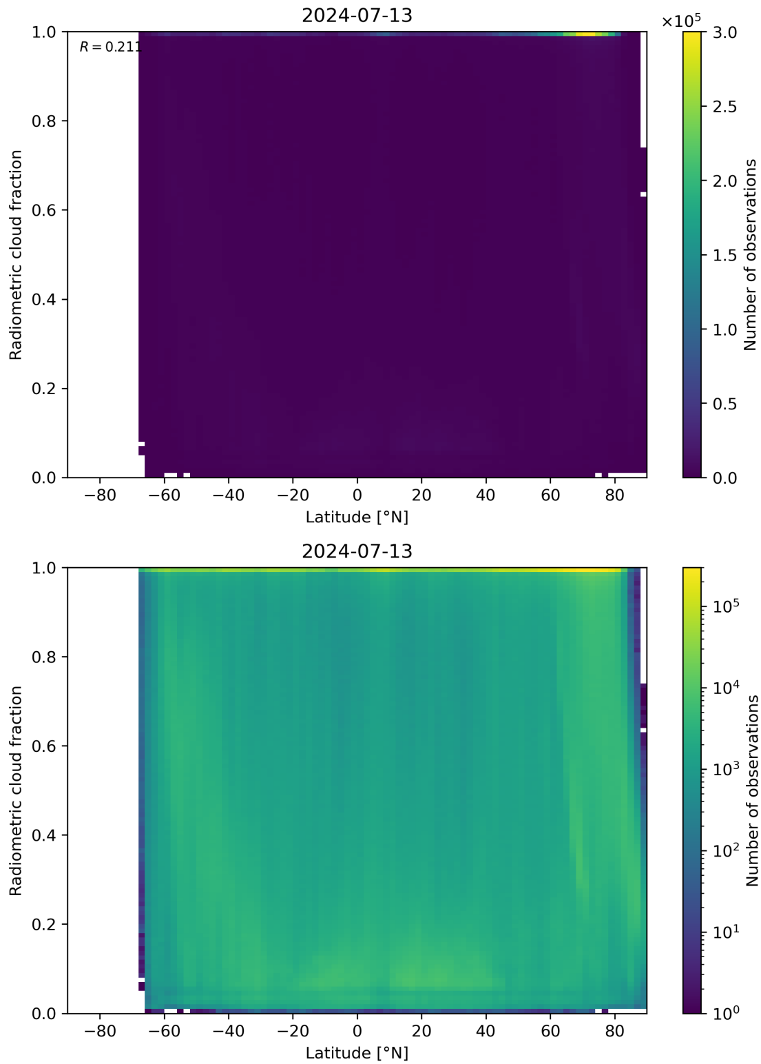
Figure 92: Scatter density plot of “Latitude” against “Radiometric cloud fraction” for 2024-07-12 to 2024-07-14.
