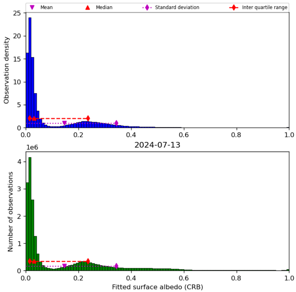
Figure 46: Histogram of “Fitted surface albedo (CRB)” for 2024-07-12 to 2024-07-14
