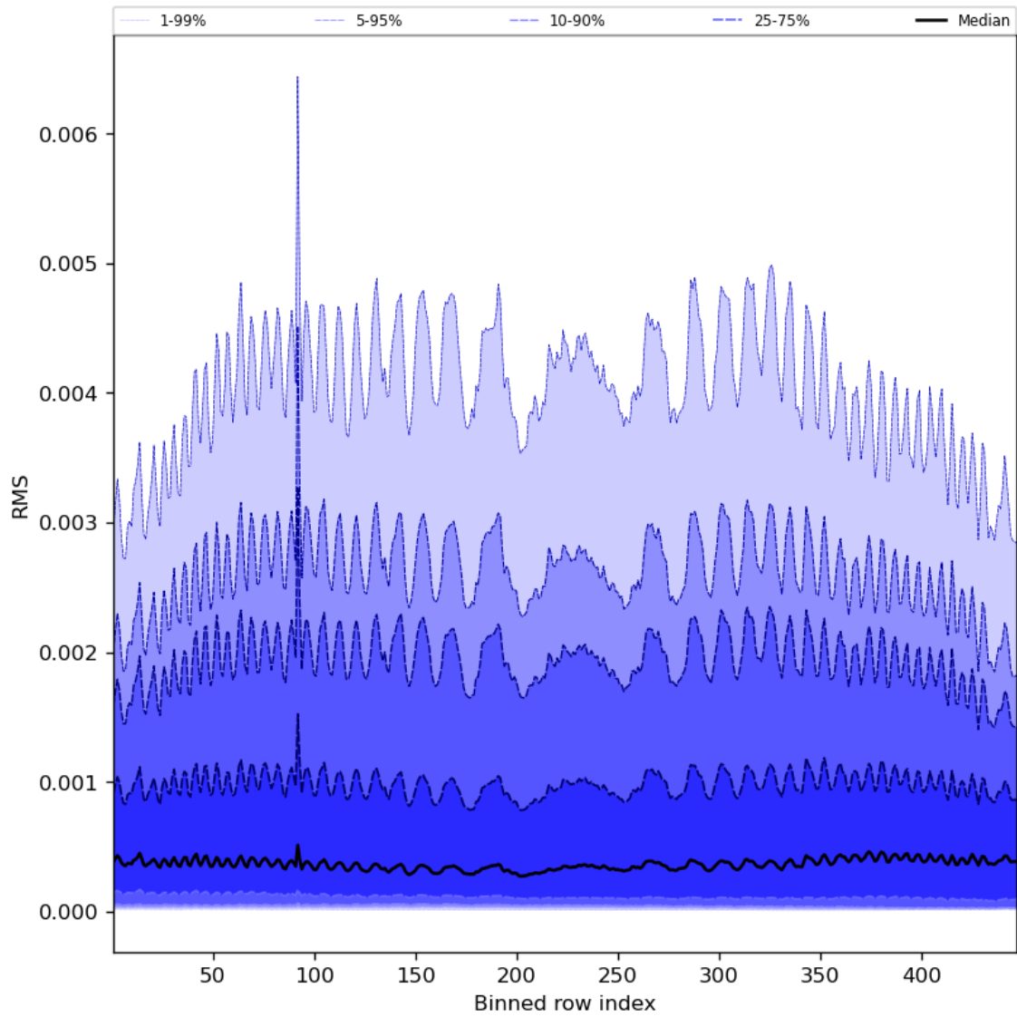
Figure 63: Along track statistics of “RMS” for 2024-07-12 to 2024-07-14
