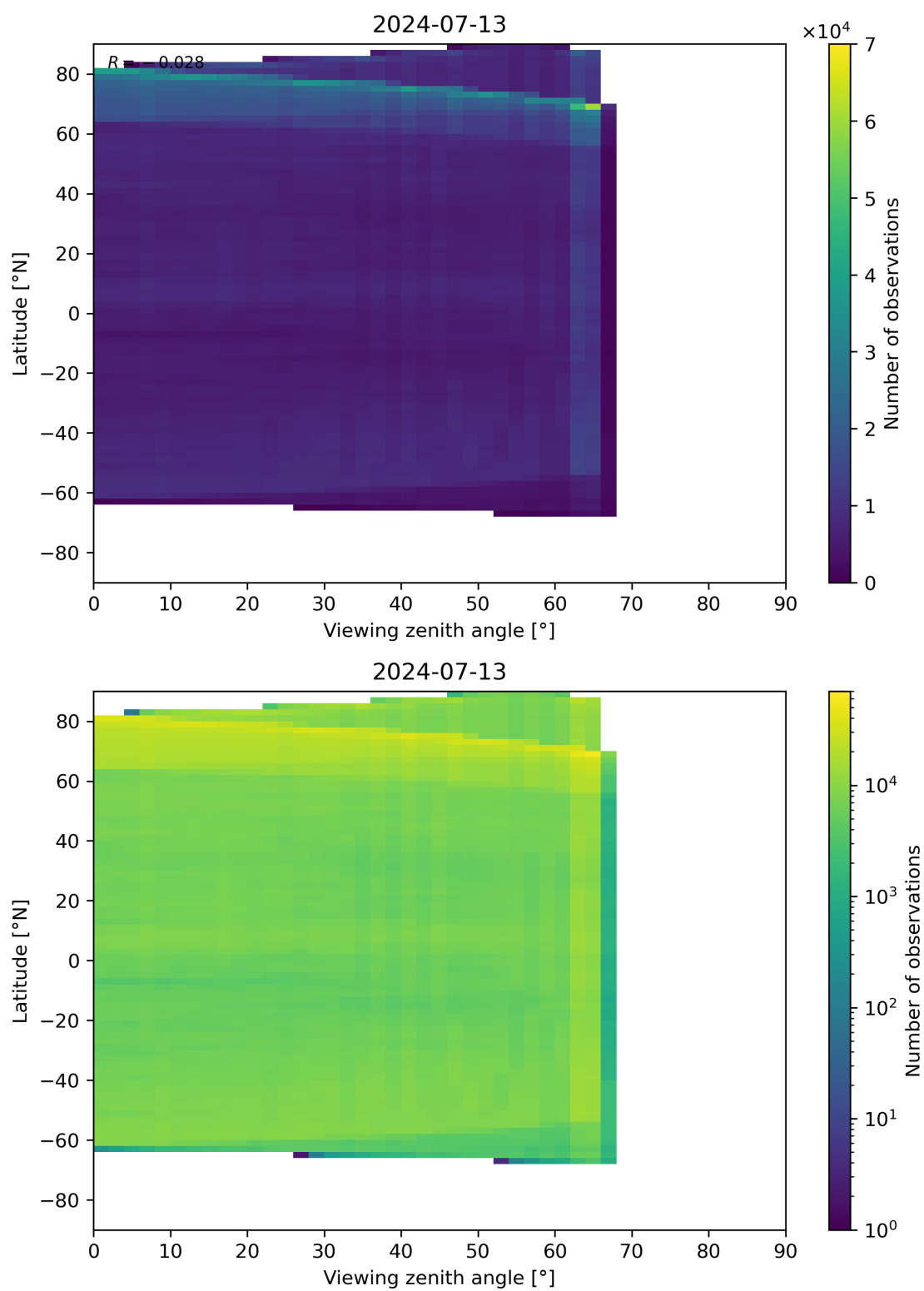
Figure 113: Scatter density plot of “Viewing zenith angle” against “Latitude” for 2024-07-12 to 2024-07-14.
