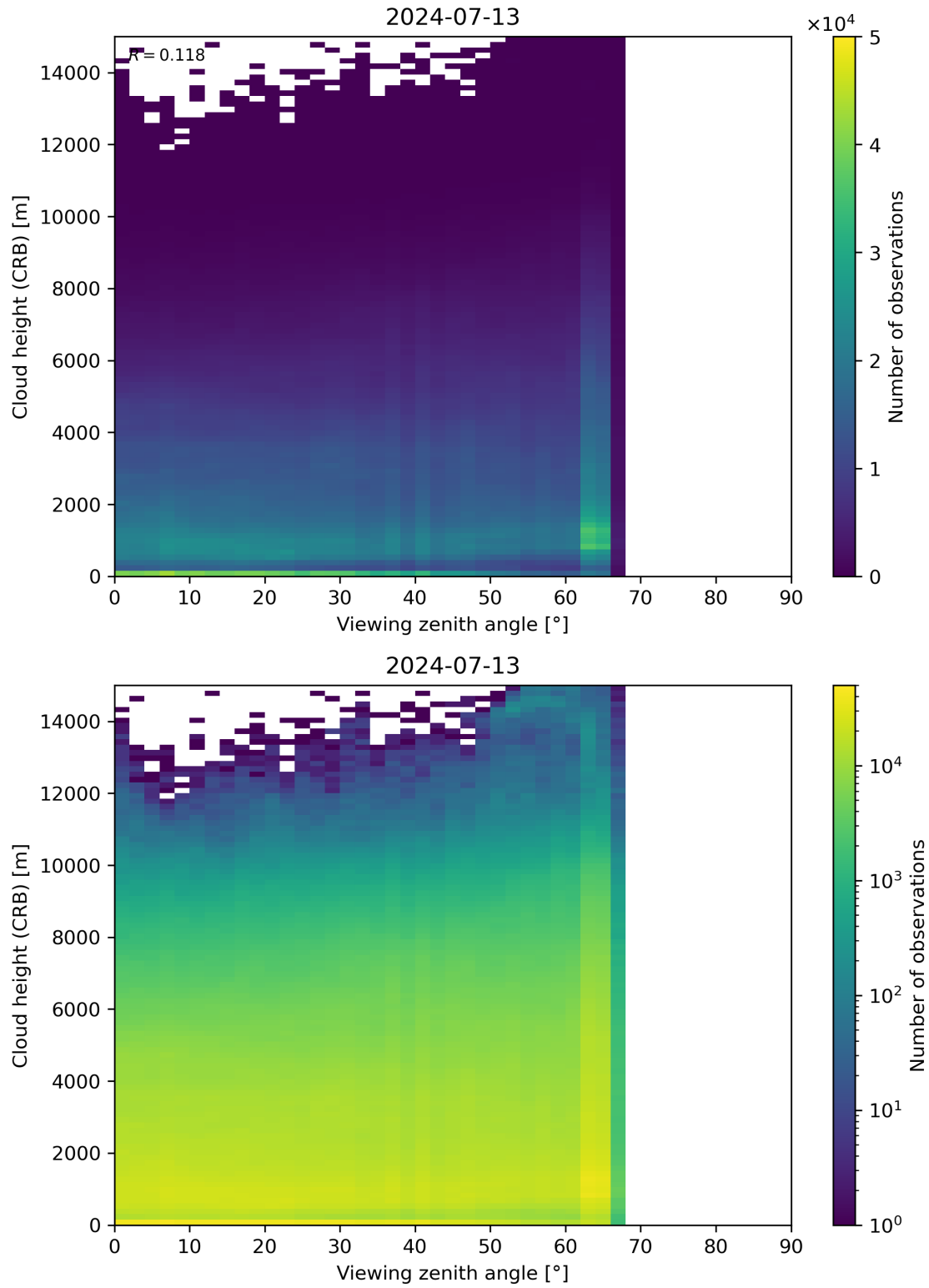
Figure 110: Scatter density plot of “Viewing zenith angle” against “Cloud height (CRB)” for 2024-07-12 to 2024-07-14.
