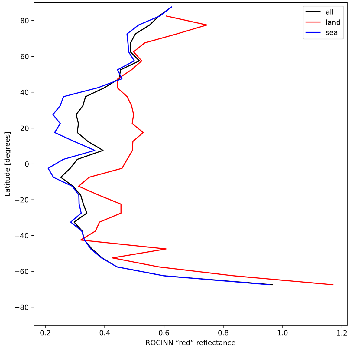
Figure 37: Zonal average of “ROCINN “red” reflectance” for 2024-07-12 to 2024-07-14.
