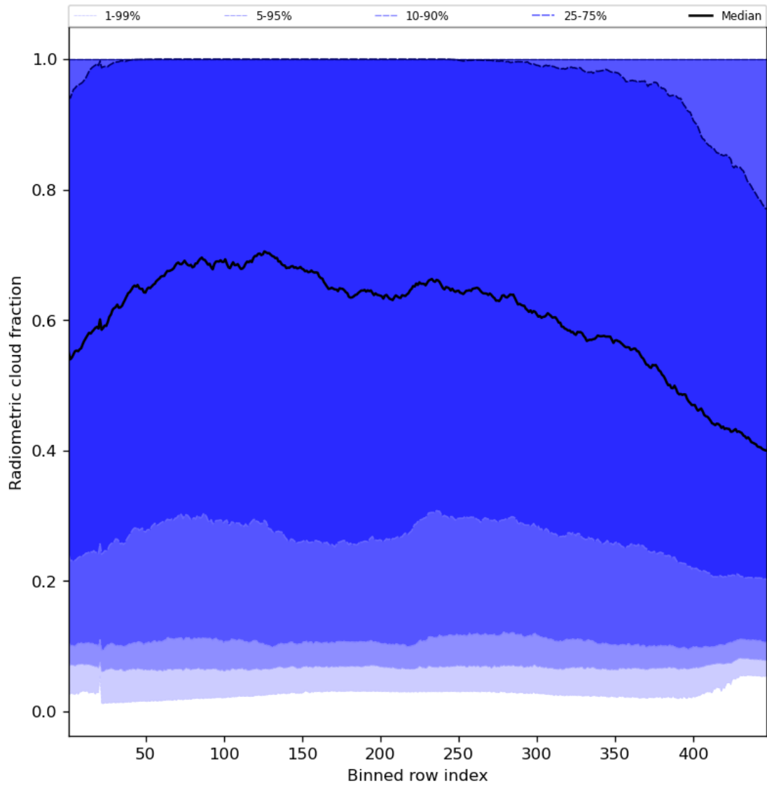
Figure 55: Along track statistics of “Radiometric cloud fraction” for 2024-07-12 to 2024-07-14
