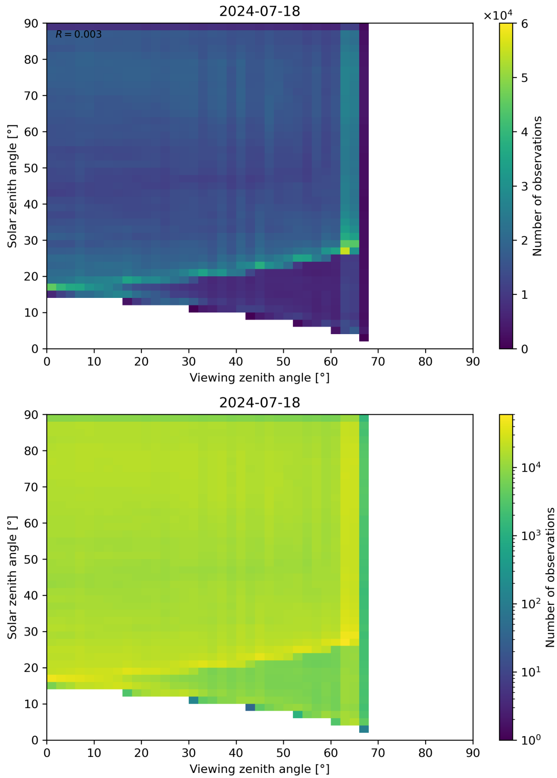
Figure 114: Scatter density plot of “Viewing zenith angle” against “Solar zenith angle” for 2024-07-17 to 2024-07-19.
