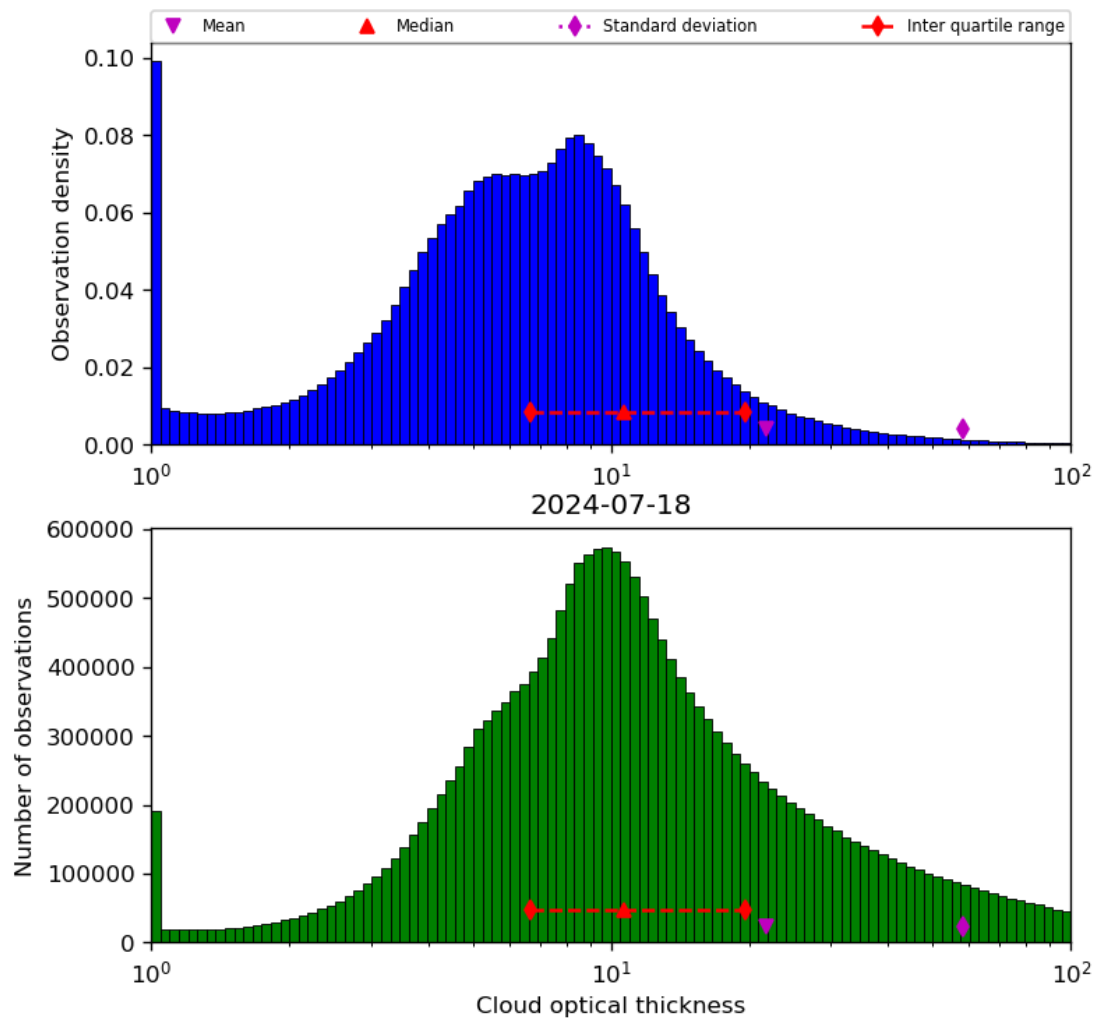
Figure 41: Histogram of “Cloud optical thickness” for 2024-07-17 to 2024-07-19
