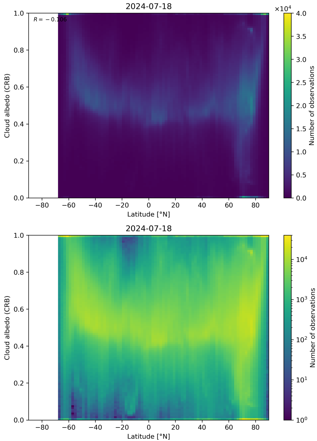
Figure 91: Scatter density plot of “Latitude” against “Cloud albedo (CRB)” for 2024-07-17 to 2024-07-19.
