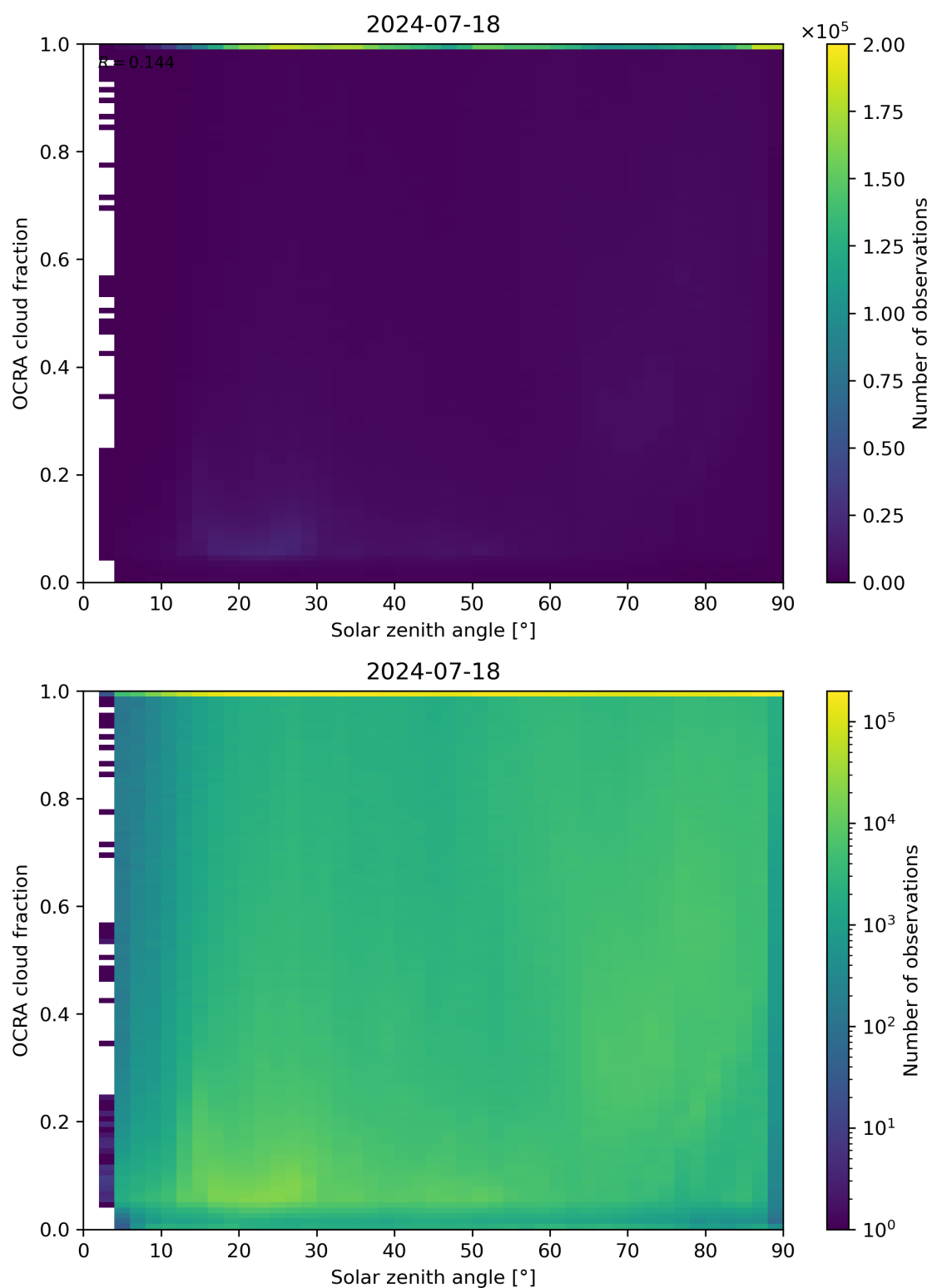
Figure 100: Scatter density plot of “Solar zenith angle” against “OCRA cloud fraction” for 2024-07-17 to 2024-07-19.
