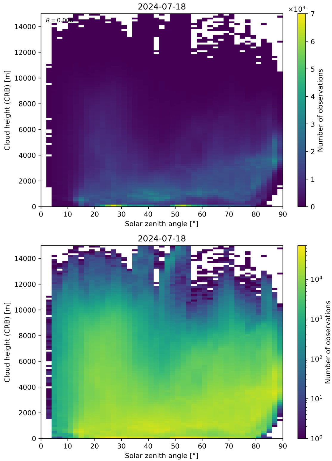
Figure 102: Scatter density plot of “Solar zenith angle” against “Cloud height (CRB)” for 2024-07-17 to 2024-07-19.
