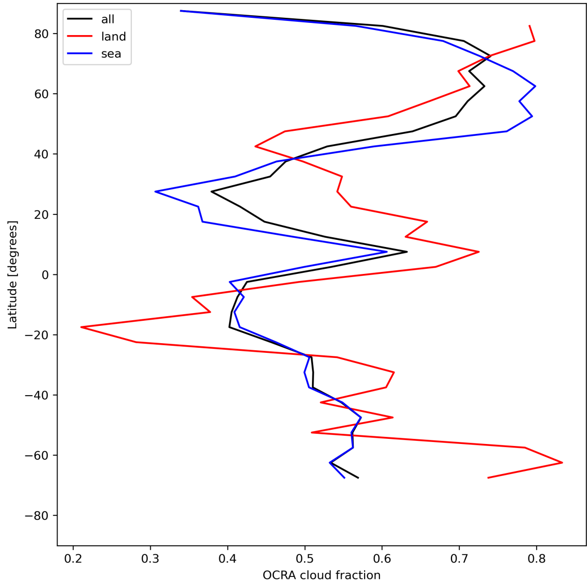
Figure 34: Zonal average of “OCRA cloud fraction” for 2024-07-17 to 2024-07-19.
