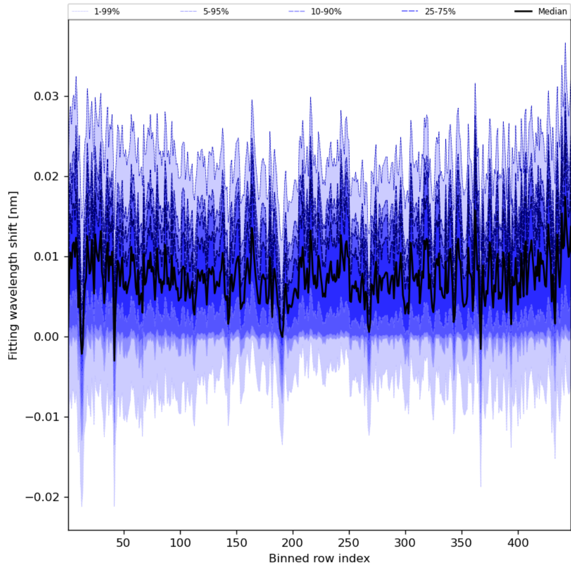
Figure 65: Along track statistics of “Fitting wavelength shift” for 2024-07-17 to 2024-07-19
