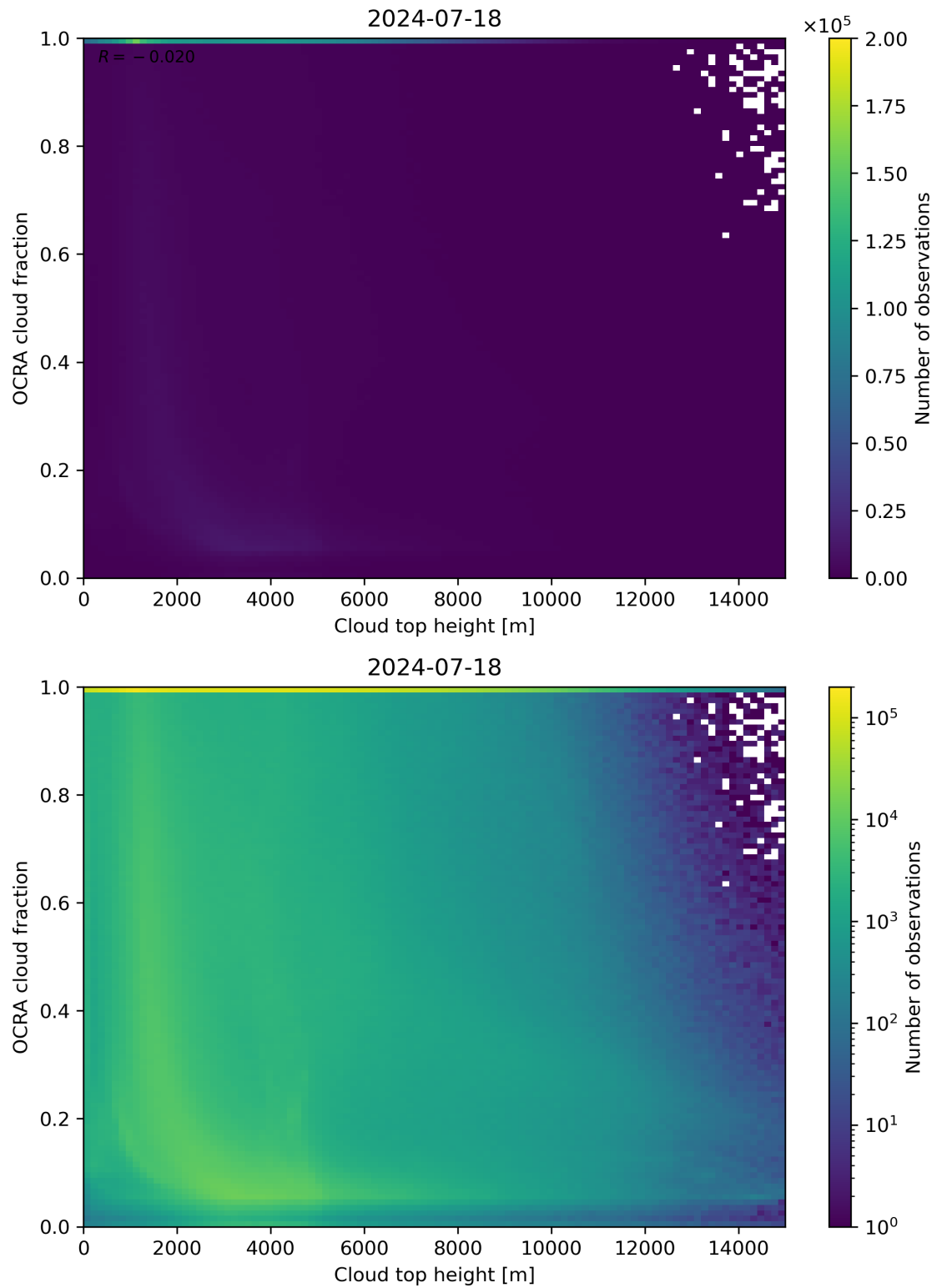
Figure 87: Scatter density plot of “Cloud top height” against “OCRA cloud fraction” for 2024-07-17 to 2024-07-19.
