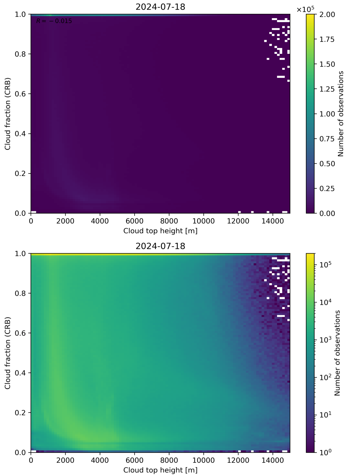
Figure 88: Scatter density plot of “Cloud top height” against “Cloud fraction (CRB)” for 2024-07-17 to 2024-07-19.
