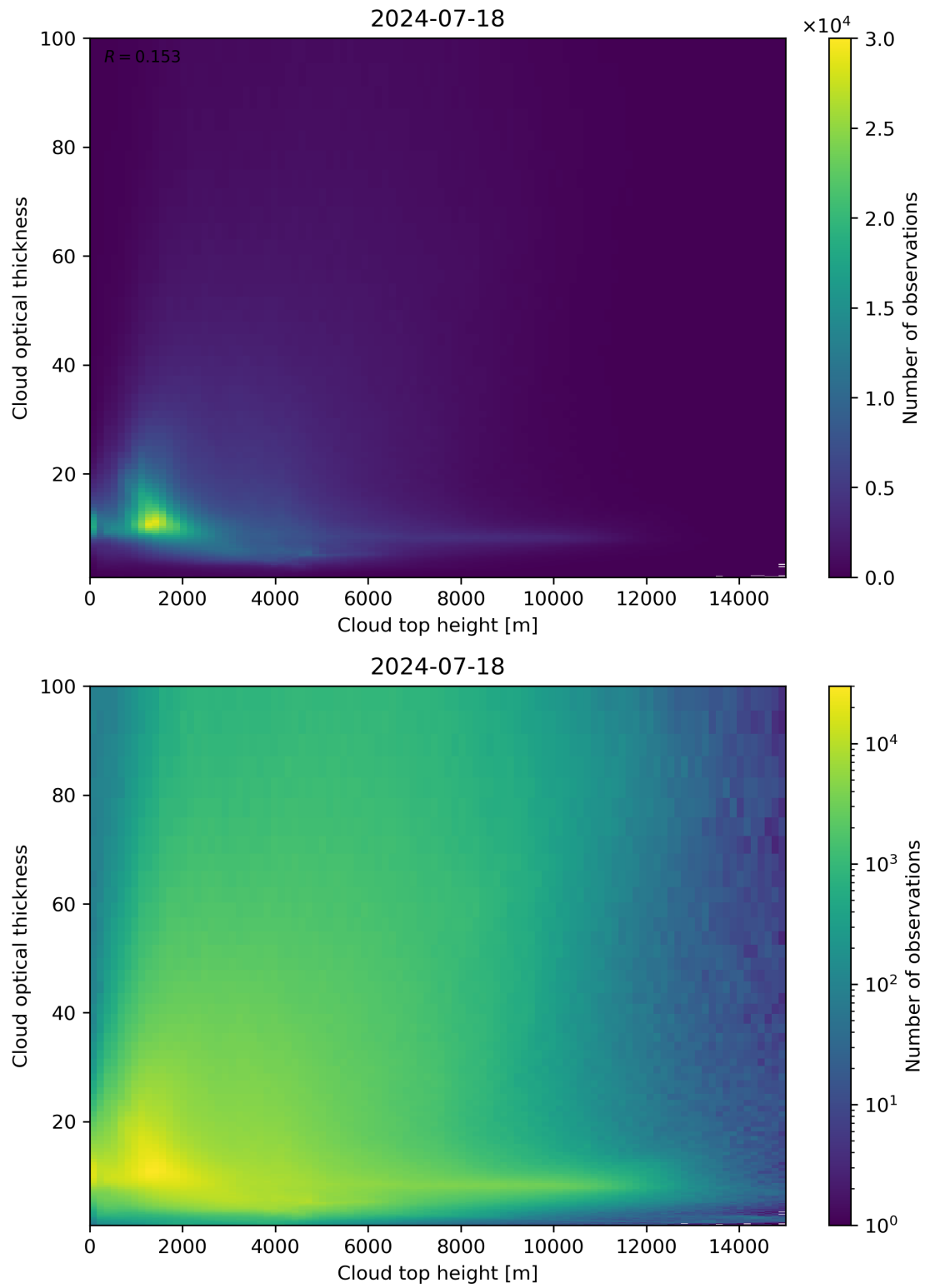
Figure 90: Scatter density plot of “Cloud top height” against “Cloud optical thickness” for 2024-07-17 to 2024-07-19.
