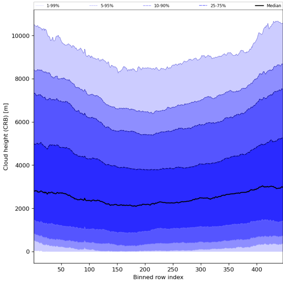
Figure 59: Along track statistics of “Cloud height (CRB)” for 2024-07-17 to 2024-07-19
