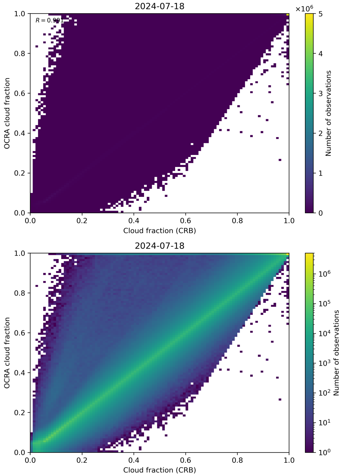
Figure 78: Scatter density plot of “Cloud fraction (CRB)” against “OCRA cloud fraction” for 2024-07-17 to 2024-07-19.
