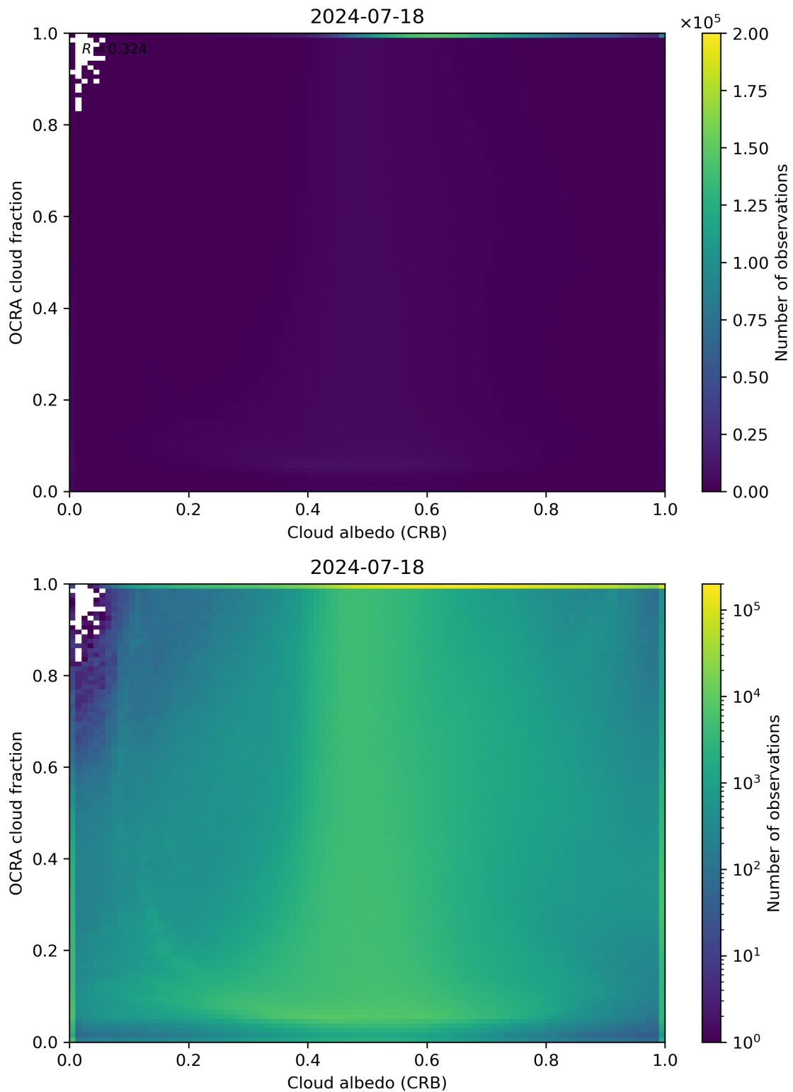
Figure 70: Scatter density plot of “Cloud albedo (CRB)” against “OCRA cloud fraction” for 2024-07-17 to 2024-07-19.
