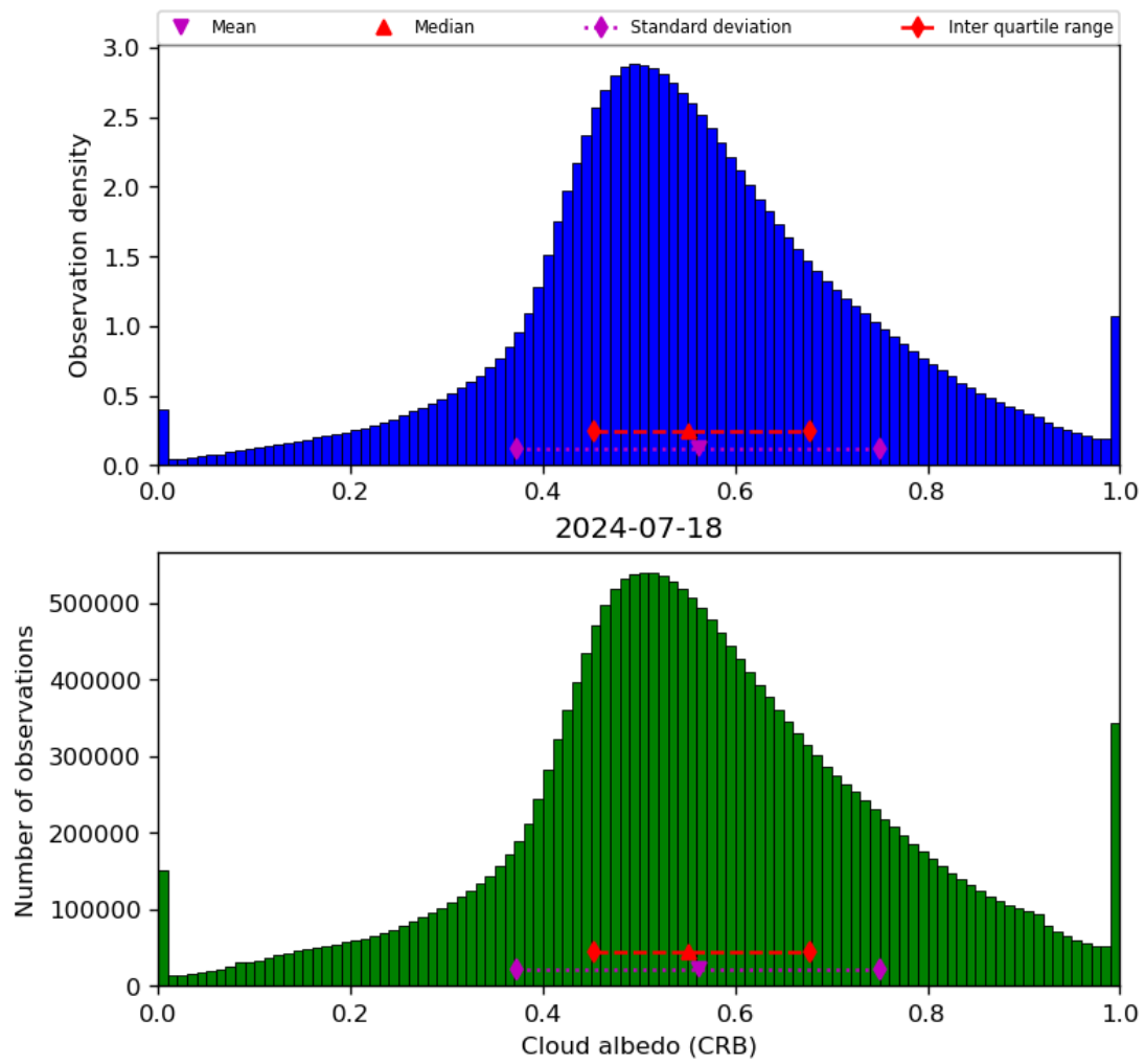
Figure 44: Histogram of “Cloud albedo (CRB)” for 2024-07-17 to 2024-07-19
