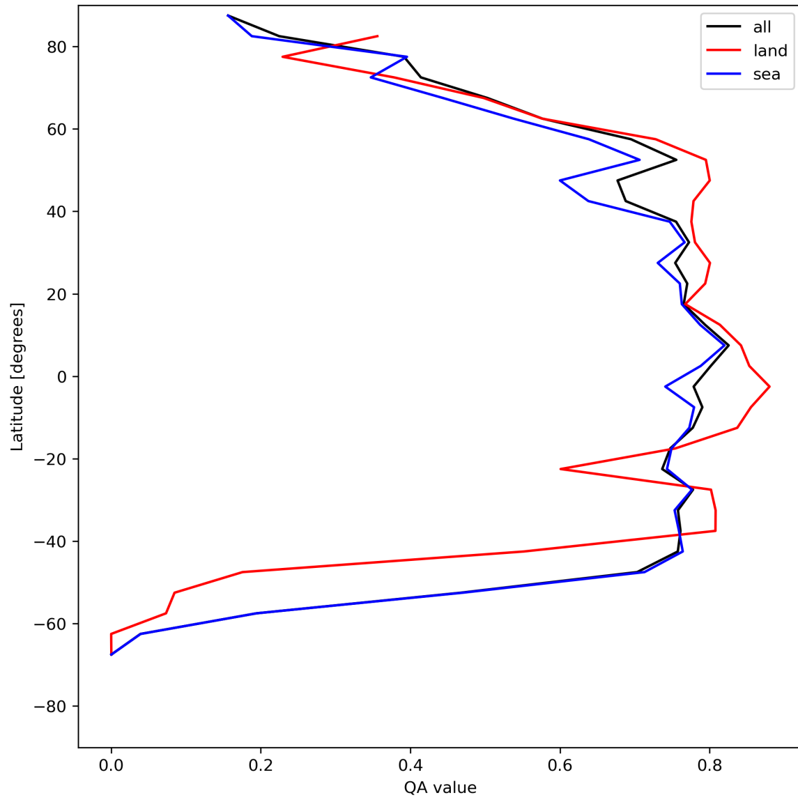
Figure 22: Zonal average of “QA value” for 2024-07-17 to 2024-07-19.
