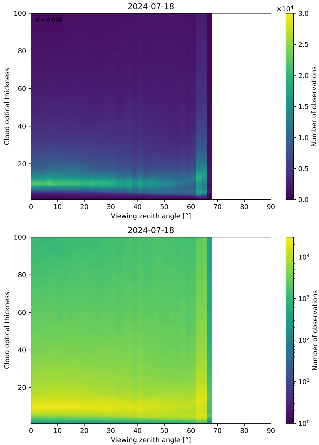
Figure 111: Scatter density plot of “Viewing zenith angle” against “Cloud optical thickness” for 2024-07-17 to 2024-07-19.
