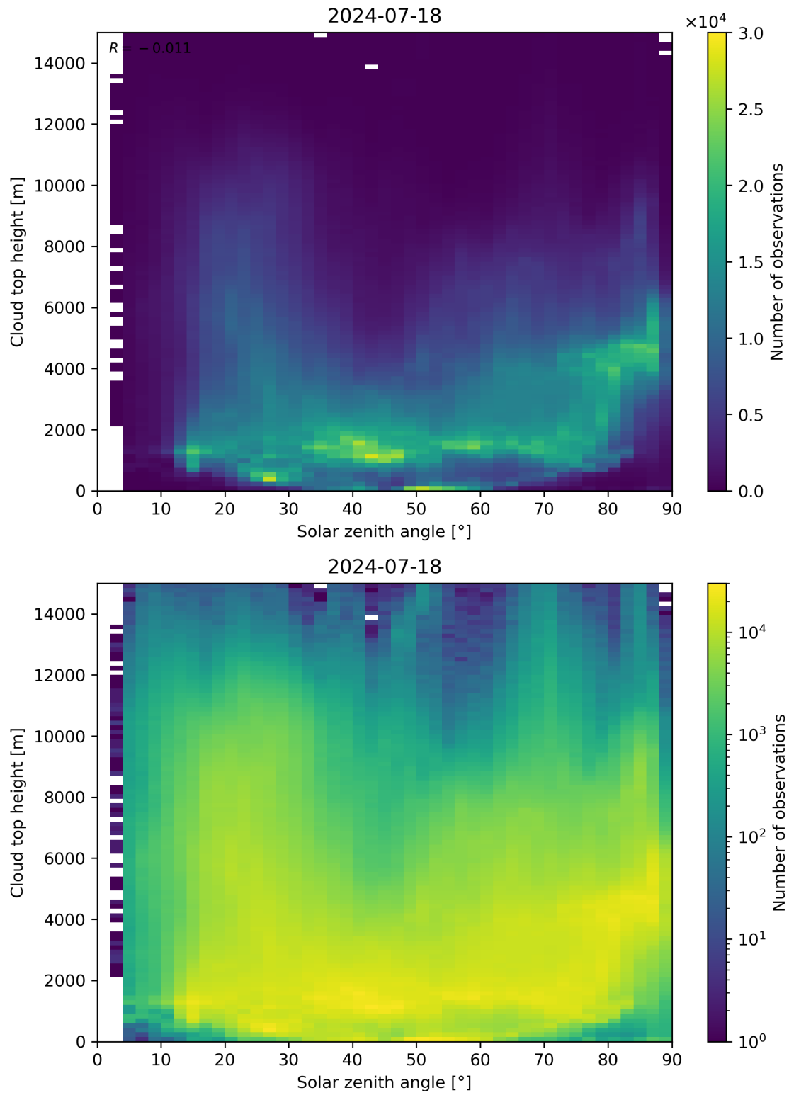
Figure 104: Scatter density plot of “Solar zenith angle” against “Cloud top height” for 2024-07-17 to 2024-07-19.
