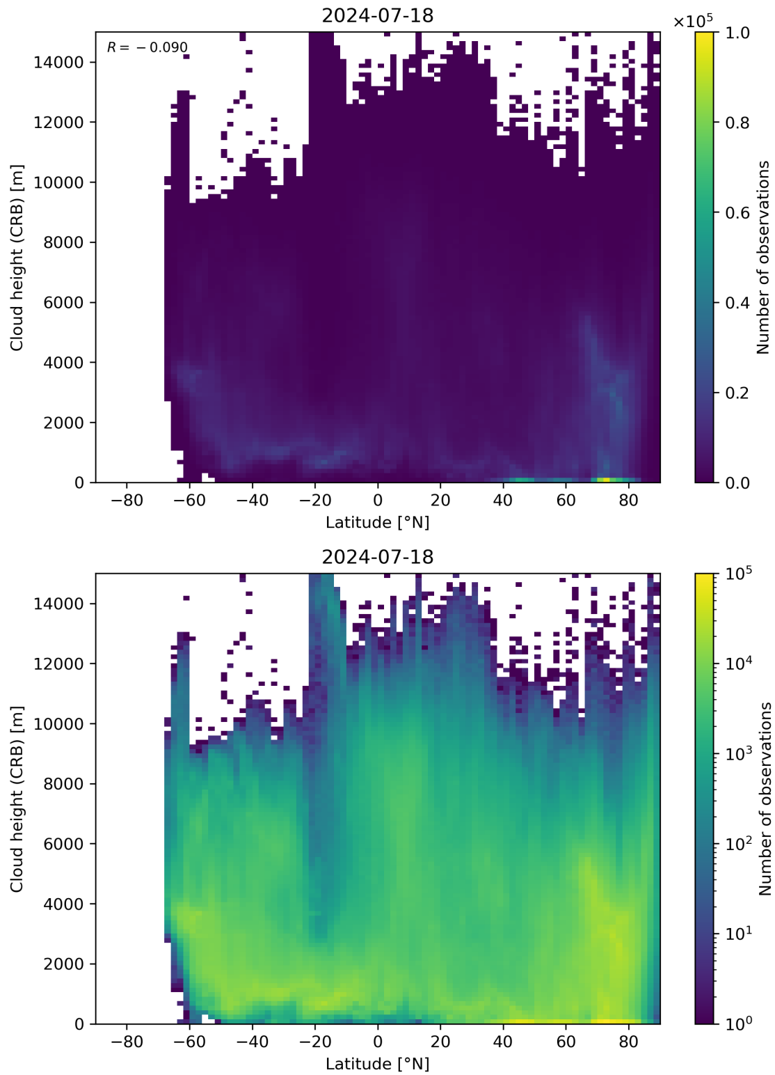
Figure 95: Scatter density plot of “Latitude” against “Cloud height (CRB)” for 2024-07-17 to 2024-07-19.
