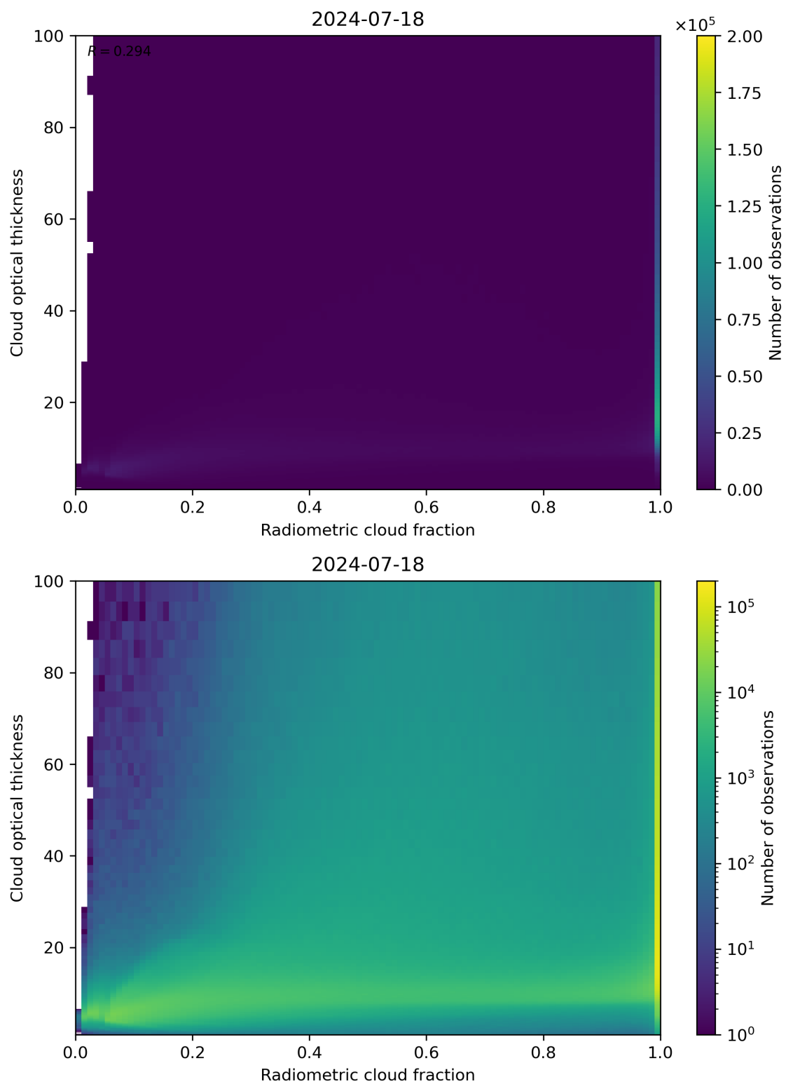
Figure 75: Scatter density plot of “Radiometric cloud fraction” against “Cloud optical thickness” for 2024-07-17 to 2024-07-19.
