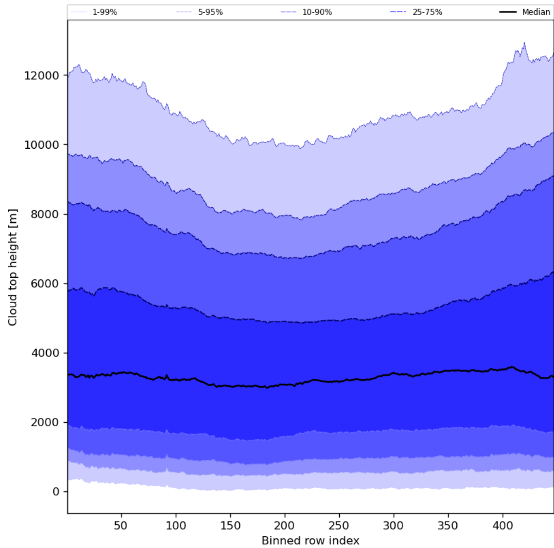
Figure 56: Along track statistics of “Cloud top height” for 2024-07-17 to 2024-07-19
