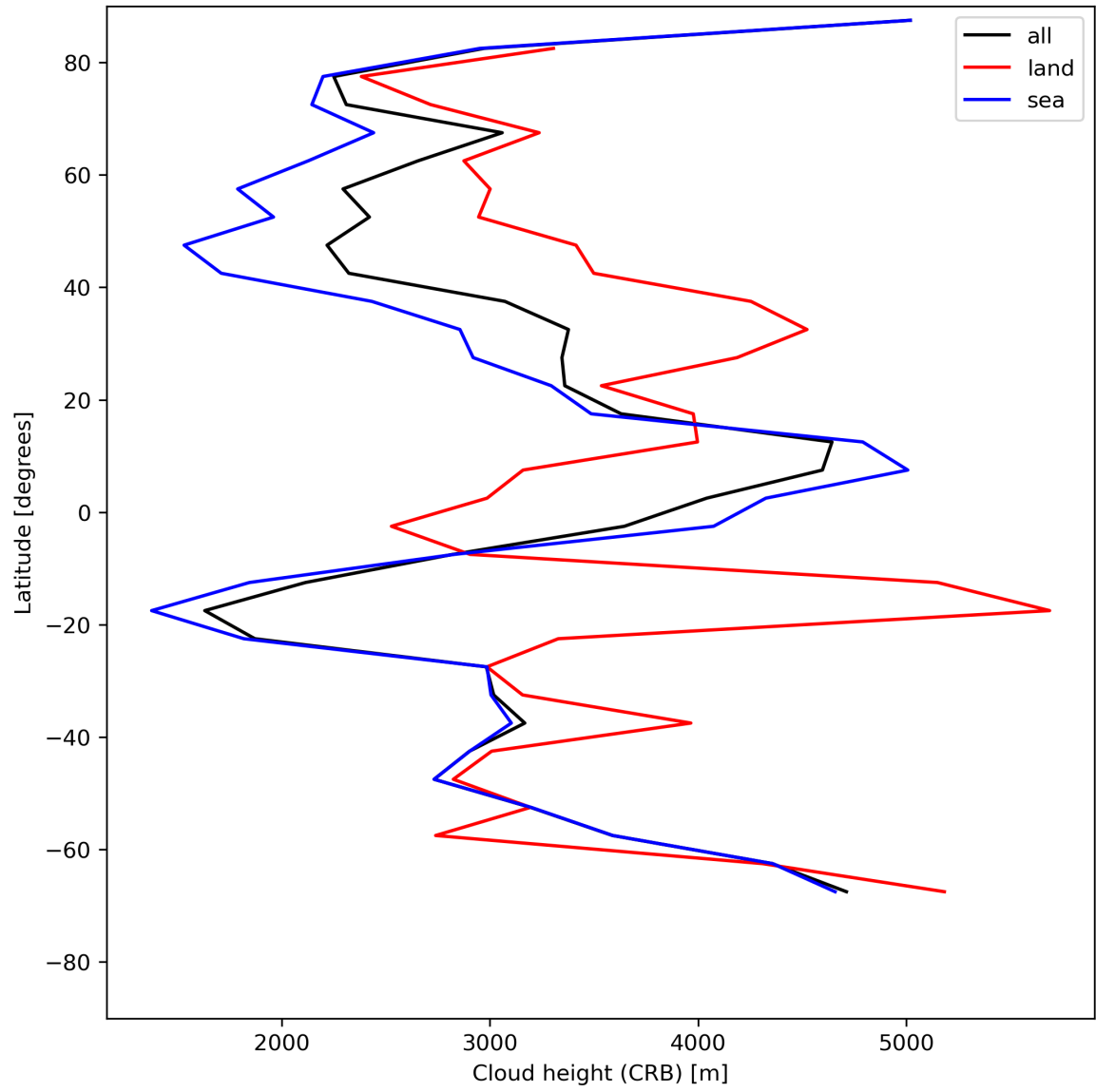
Figure 27: Zonal average of “Cloud height (CRB)” for 2024-07-17 to 2024-07-19.
