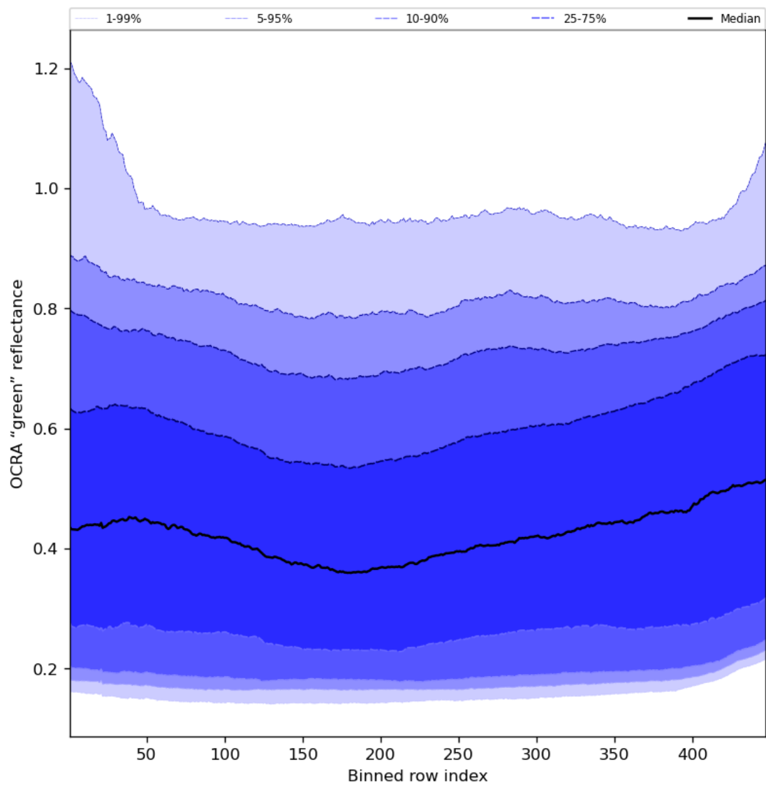
Figure 68: Along track statistics of “OCRA “green” reflectance” for 2024-07-17 to 2024-07-19
