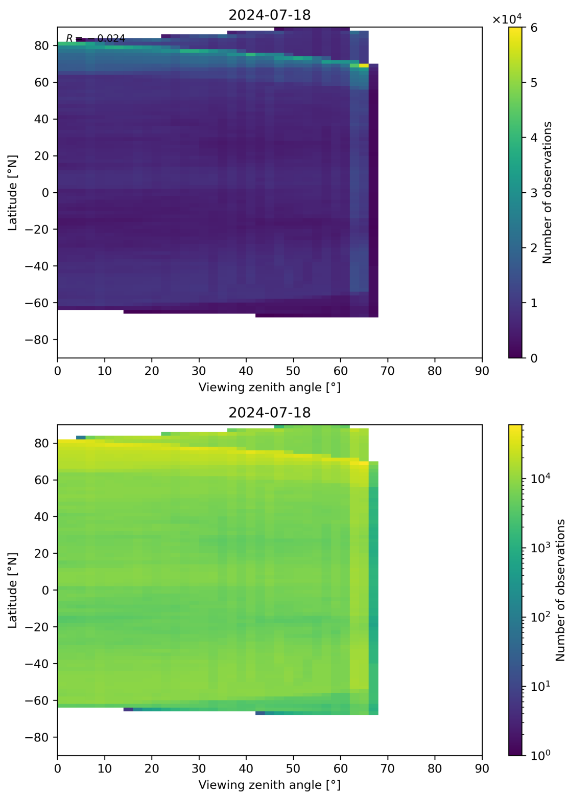
Figure 113: Scatter density plot of “Viewing zenith angle” against “Latitude” for 2024-07-17 to 2024-07-19.
