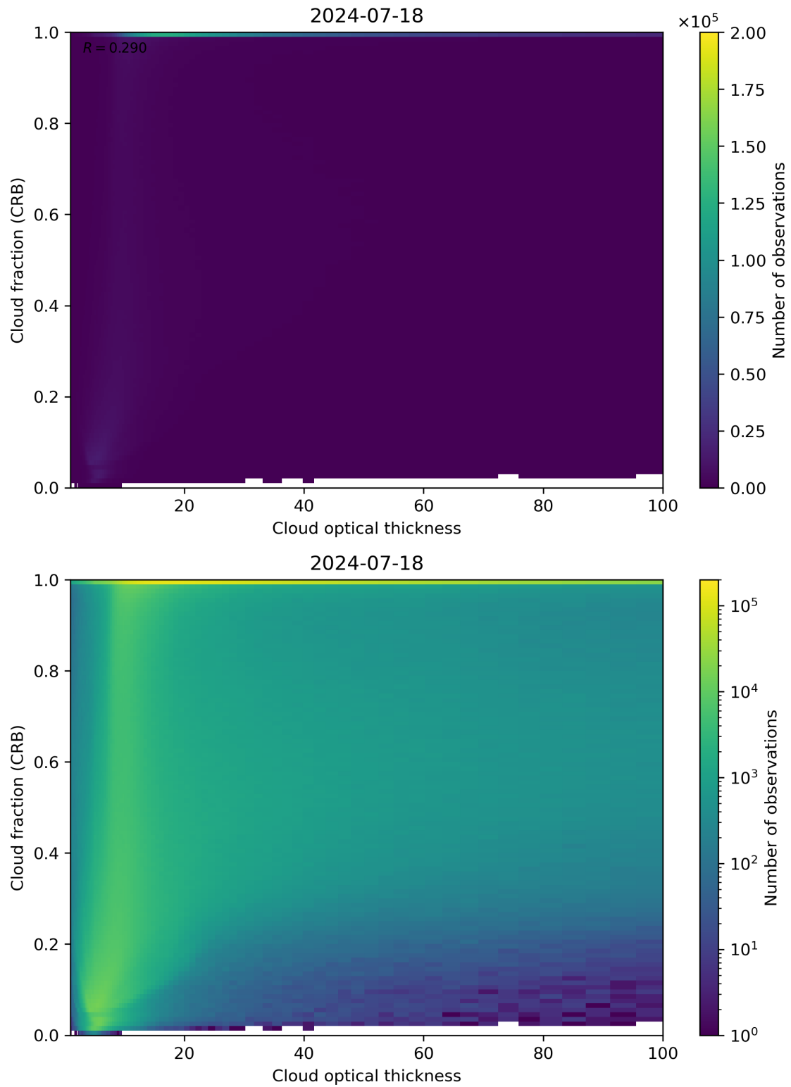
Figure 84: Scatter density plot of “Cloud optical thickness” against “Cloud fraction (CRB)” for 2024-07-17 to 2024-07-19.
