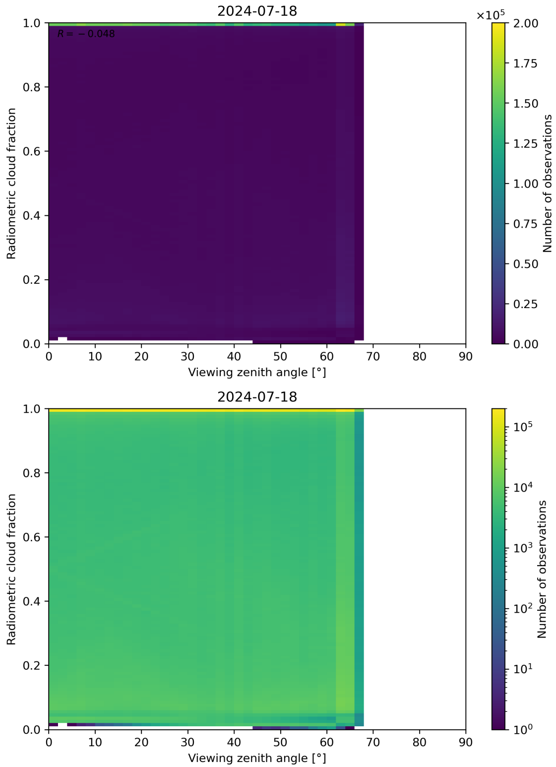
Figure 107: Scatter density plot of “Viewing zenith angle” against “Radiometric cloud fraction” for 2024-07-17 to 2024-07-19.
