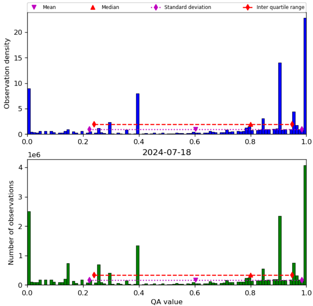
Figure 38: Histogram of “QA value” for 2024-07-17 to 2024-07-19
