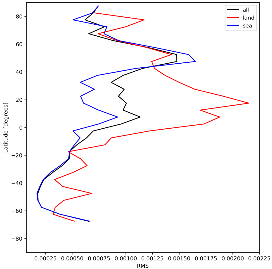
Figure 31: Zonal average of “RMS” for 2024-07-17 to 2024-07-19.
