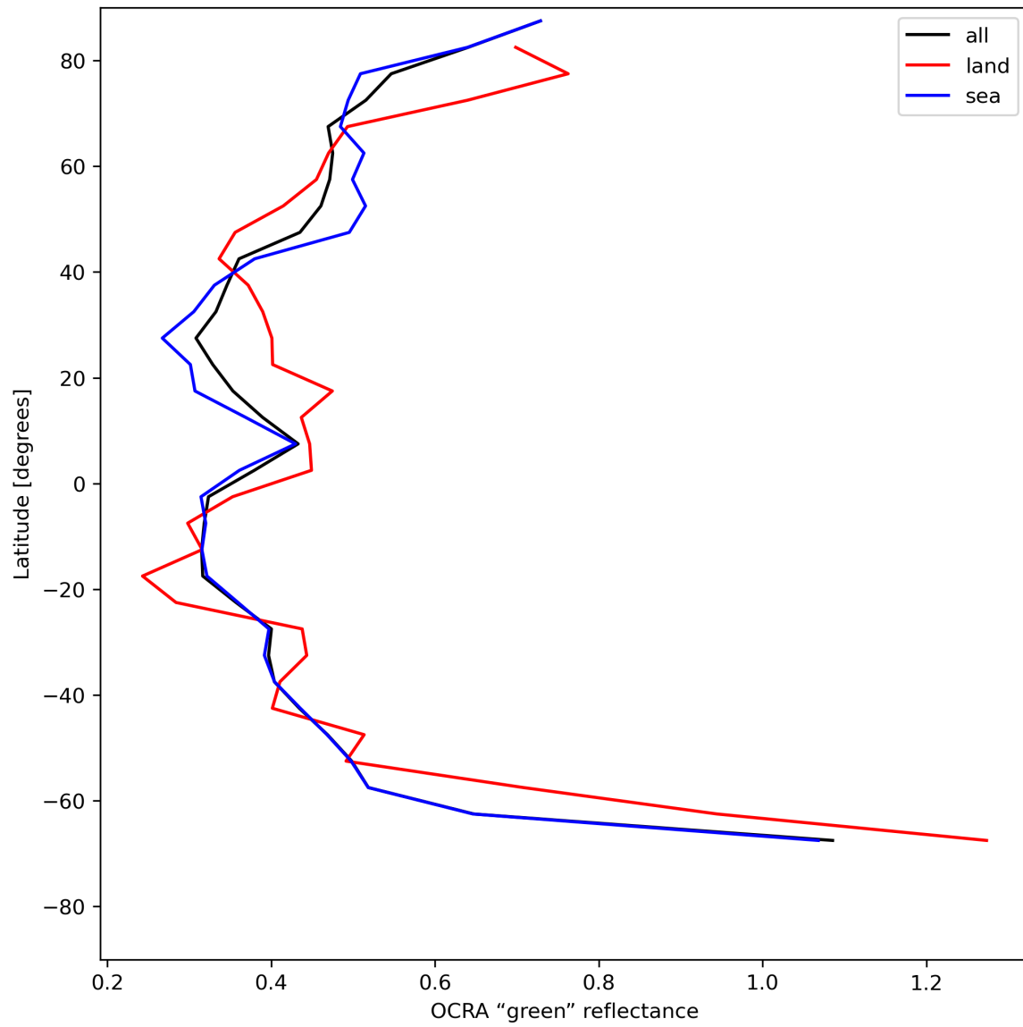
Figure 36: Zonal average of “OCRA “green” reflectance” for 2024-07-17 to 2024-07-19.
