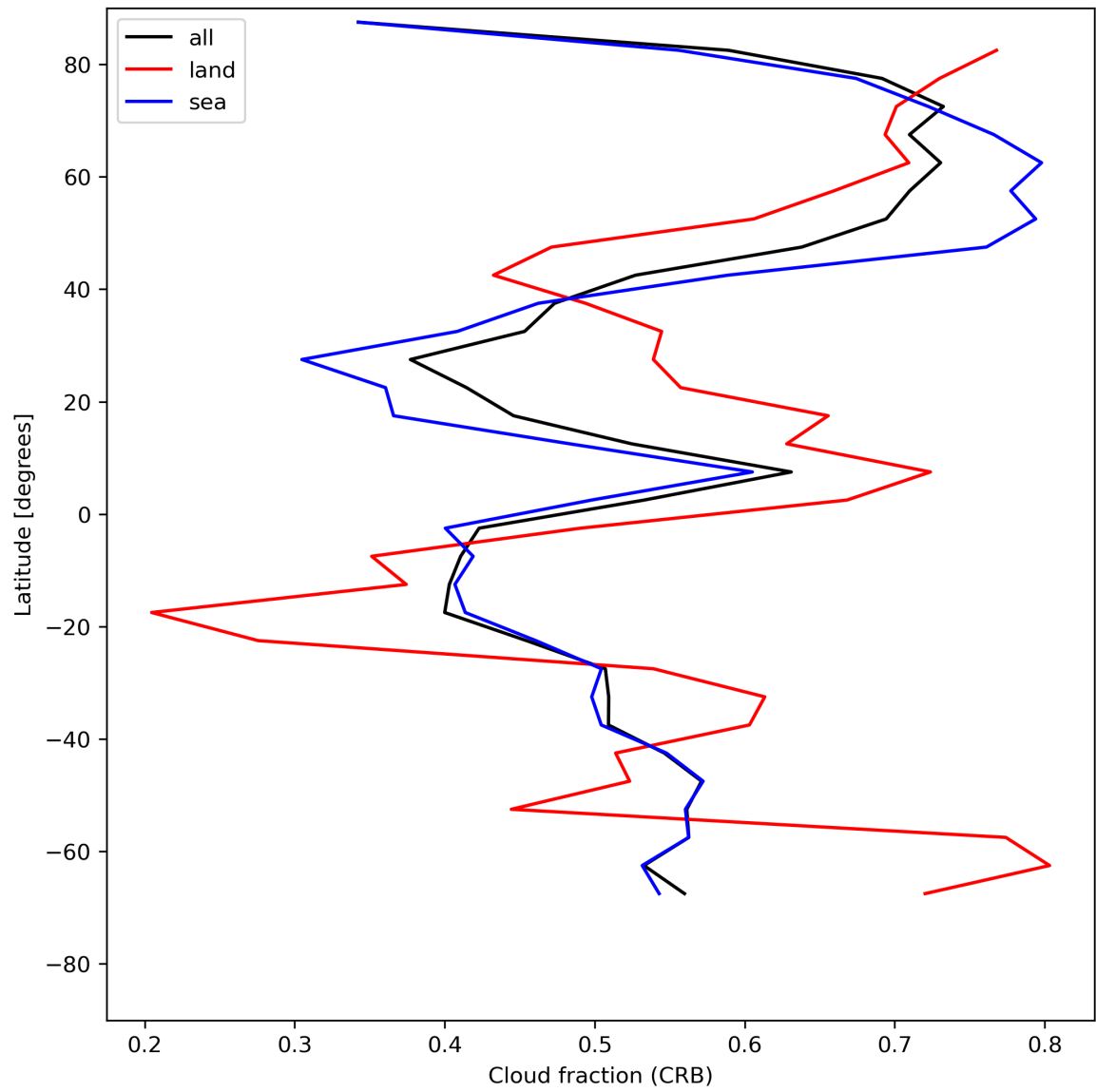
Figure 26: Zonal average of “Cloud fraction (CRB)” for 2024-07-17 to 2024-07-19.
