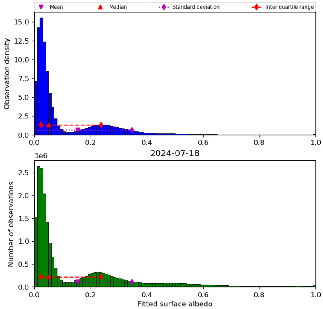
Figure 45: Histogram of “Fitted surface albedo” for 2024-07-17 to 2024-07-19
