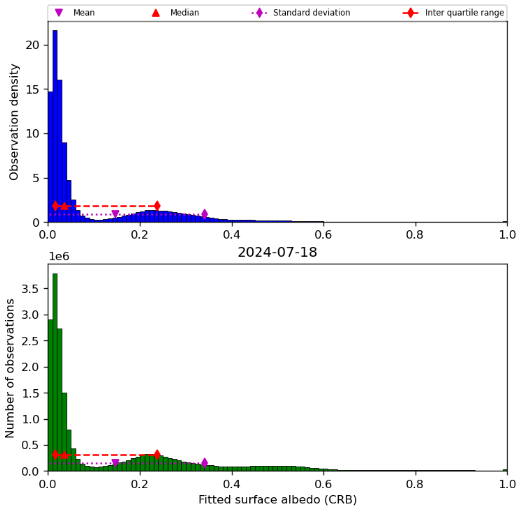
Figure 46: Histogram of “Fitted surface albedo (CRB)” for 2024-07-17 to 2024-07-19
