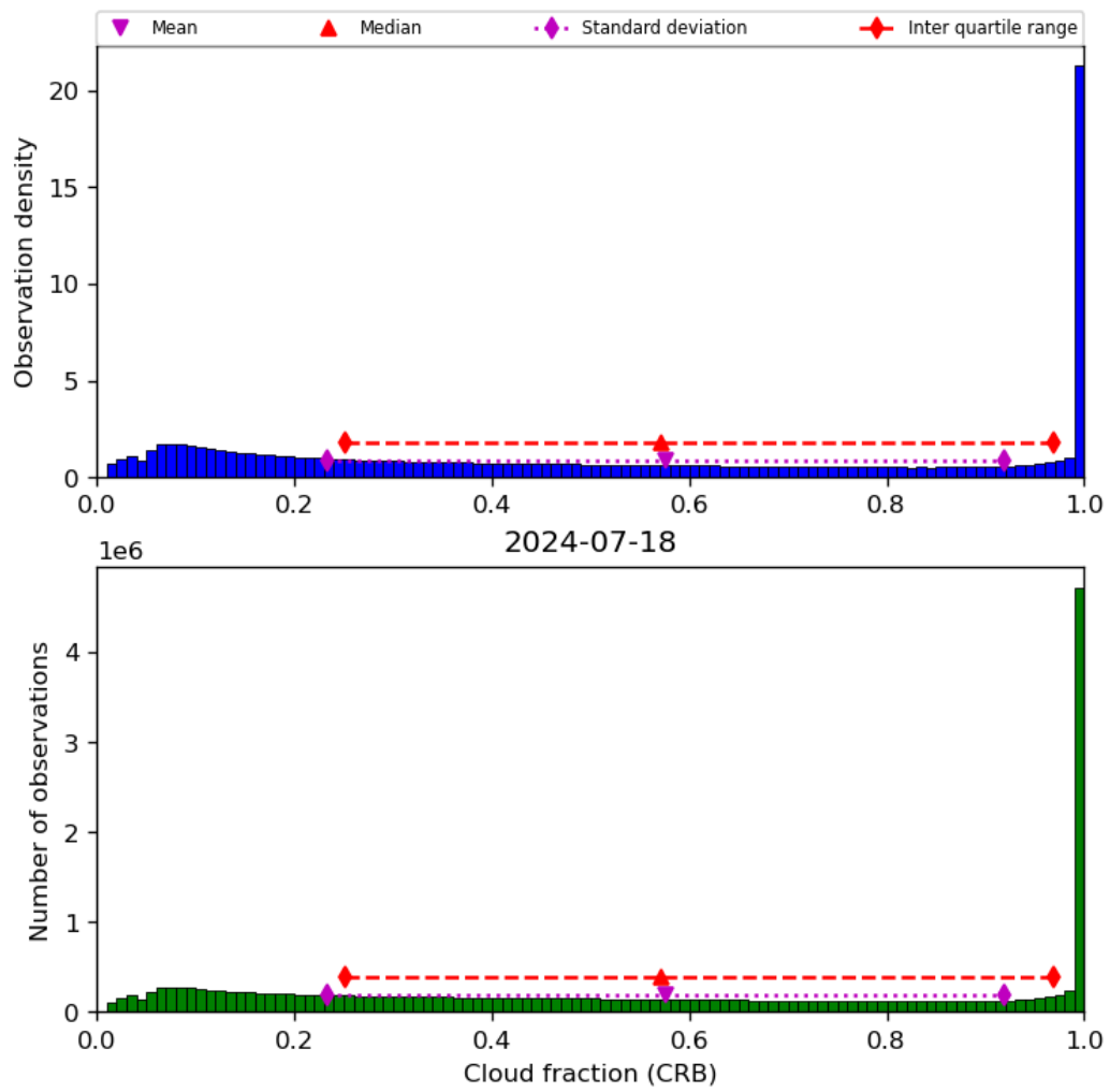
Figure 42: Histogram of “Cloud fraction (CRB)” for 2024-07-17 to 2024-07-19
