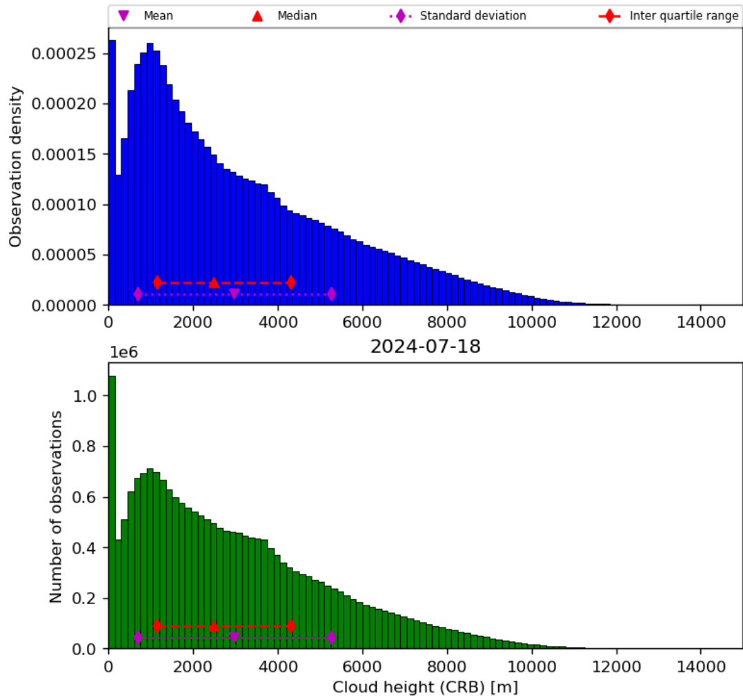
Figure 43: Histogram of “Cloud height (CRB)” for 2024-07-17 to 2024-07-19
