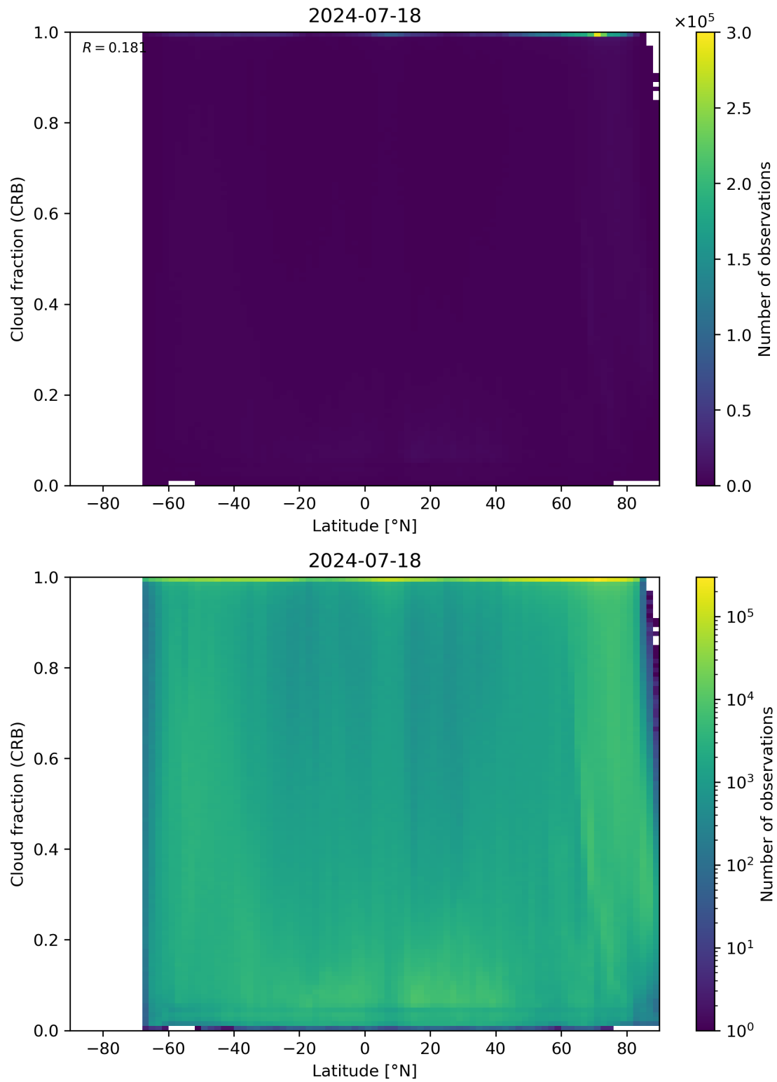
Figure 94: Scatter density plot of “Latitude” against “Cloud fraction (CRB)” for 2024-07-17 to 2024-07-19.
