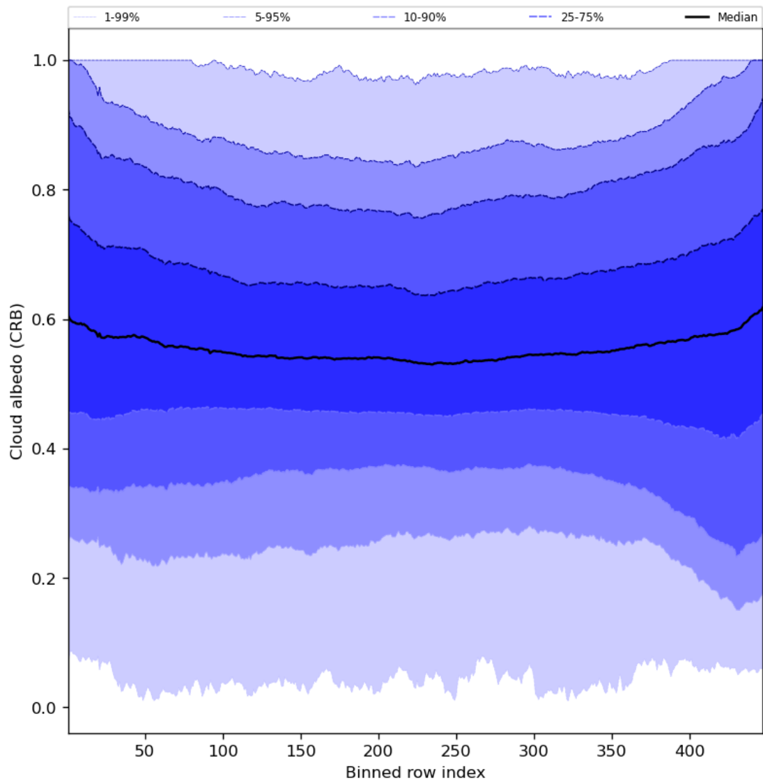
Figure 60: Along track statistics of “Cloud albedo (CRB)” for 2024-07-17 to 2024-07-19
