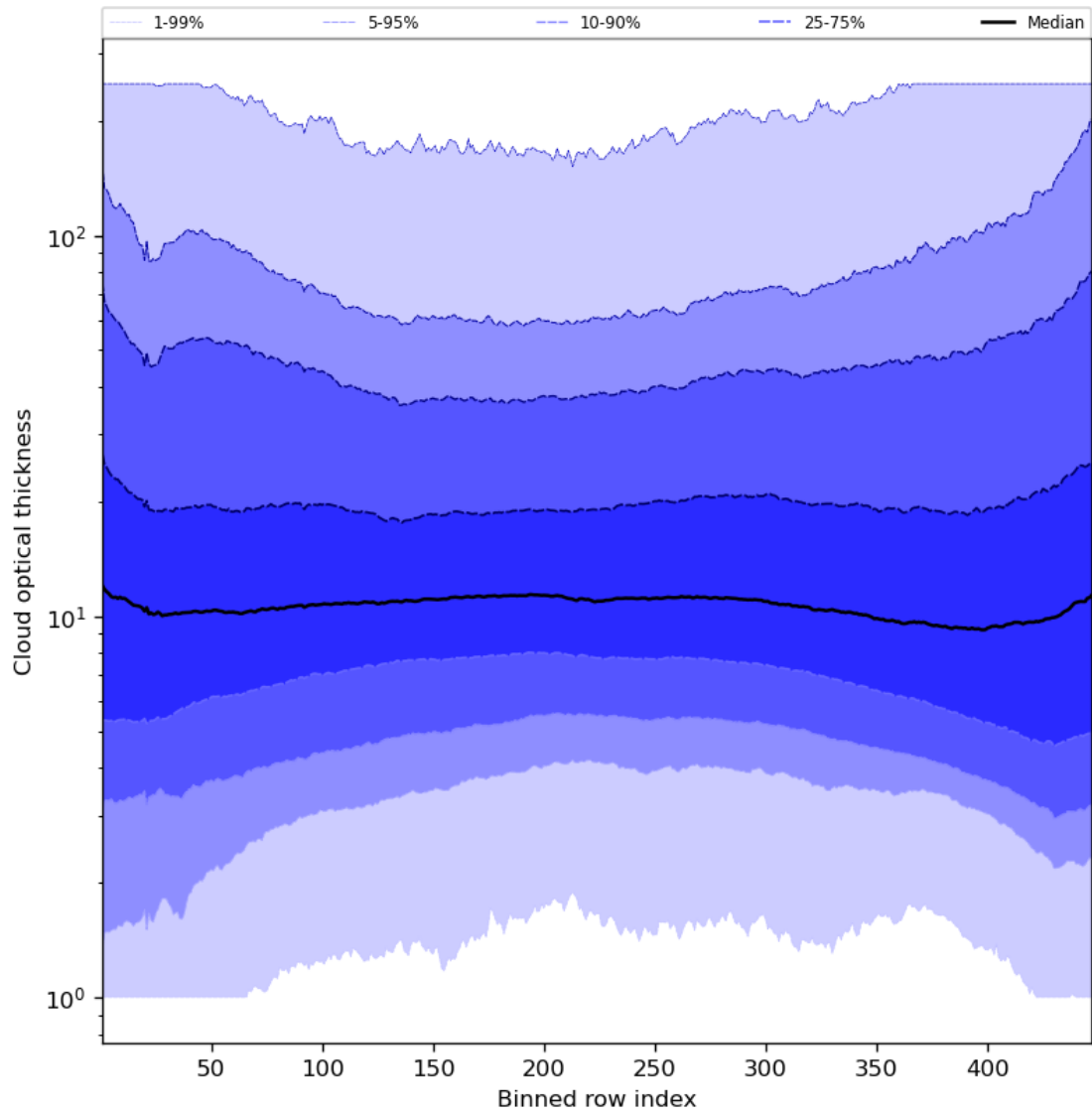
Figure 57: Along track statistics of “Cloud optical thickness” for 2024-07-17 to 2024-07-19
