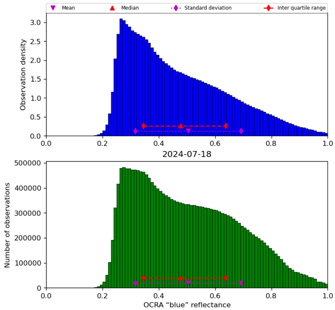
Figure 51: Histogram of “OCRA “blue” reflectance” for 2024-07-17 to 2024-07-19
