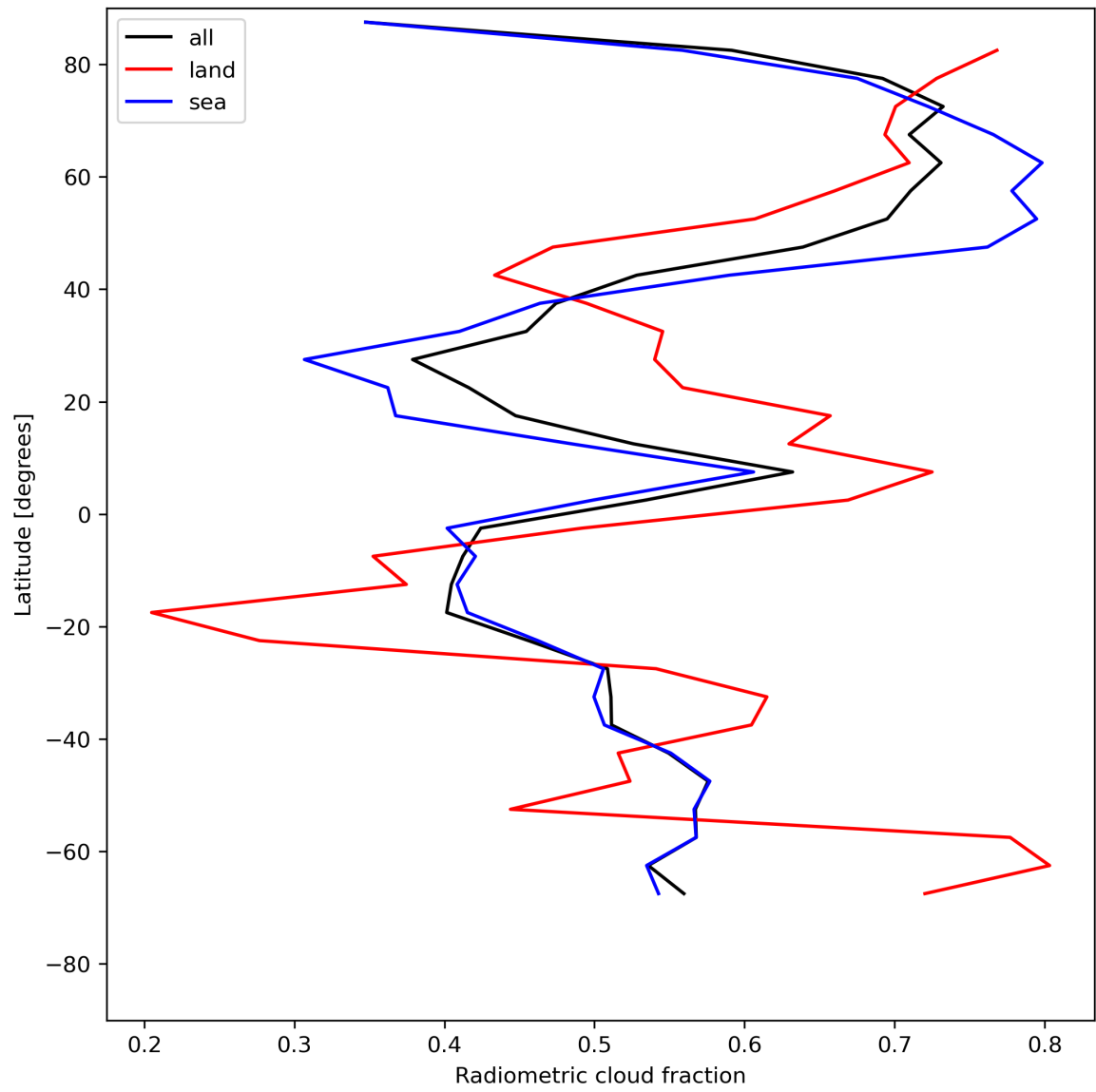
Figure 23: Zonal average of “Radiometric cloud fraction” for 2024-07-17 to 2024-07-19.
