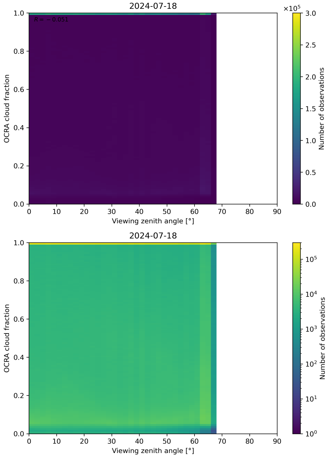
Figure 108: Scatter density plot of “Viewing zenith angle” against “OCRA cloud fraction” for 2024-07-17 to 2024-07-19.
