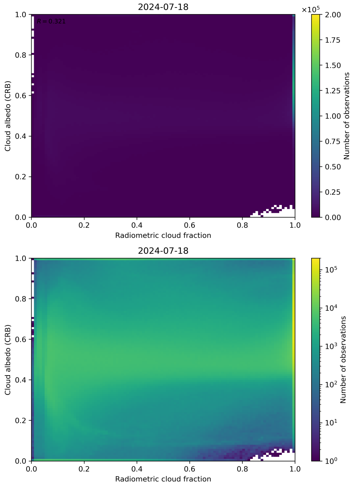
Figure 71: Scatter density plot of “Radiometric cloud fraction” against “Cloud albedo (CRB)” for 2024-07-17 to 2024-07-19.
