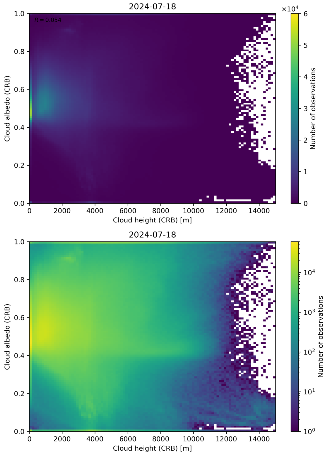
Figure 80: Scatter density plot of “Cloud height (CRB)” against “Cloud albedo (CRB)” for 2024-07-17 to 2024-07-19.
