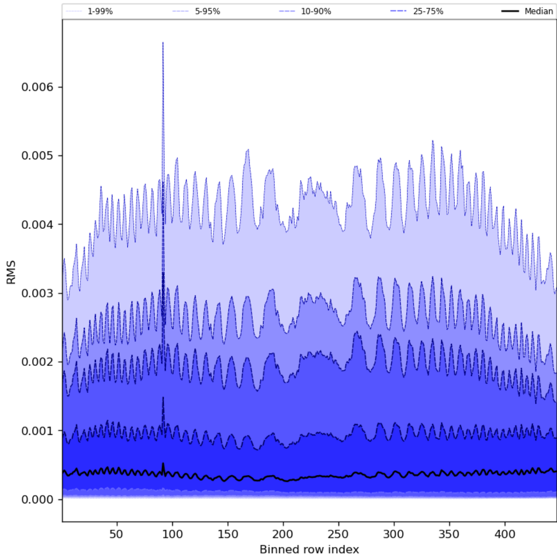
Figure 63: Along track statistics of “RMS” for 2024-07-17 to 2024-07-19
