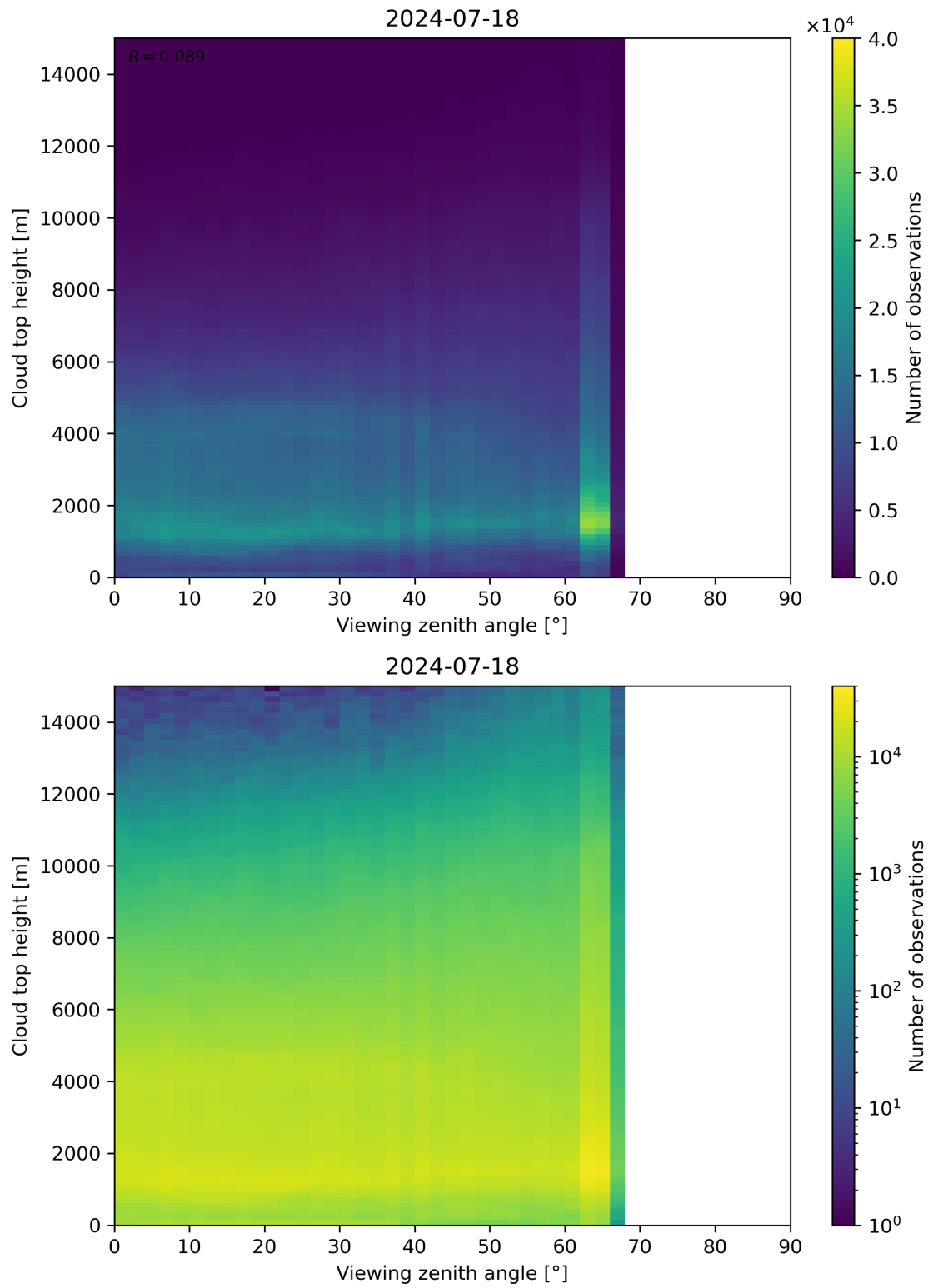
Figure 112: Scatter density plot of “Viewing zenith angle” against “Cloud top height” for 2024-07-17 to 2024-07-19.
