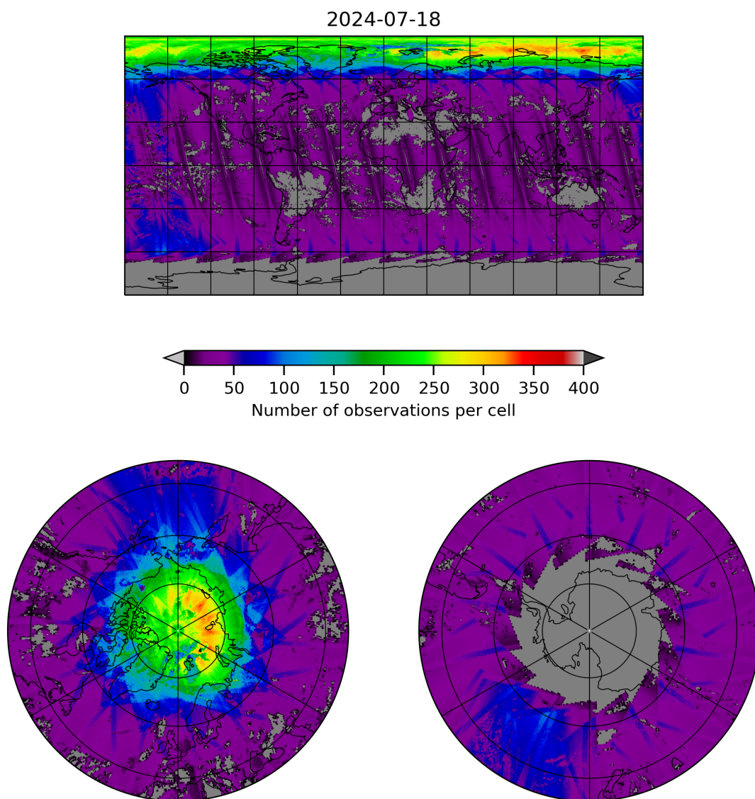
Figure 21: Map of the number of observations for 2024-07-17 to 2024-07-19
