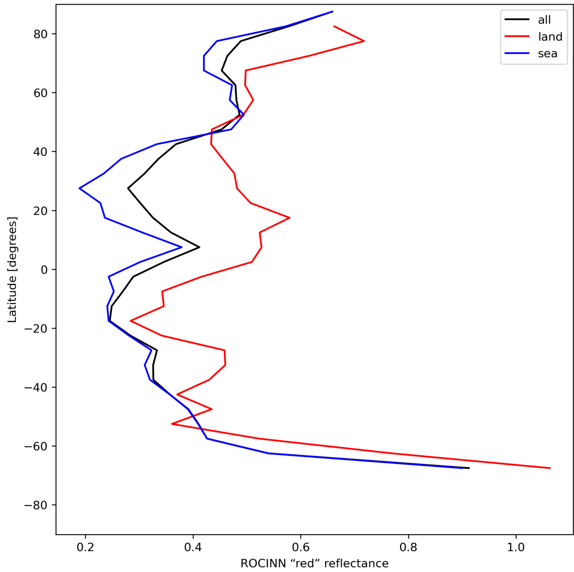
Figure 37: Zonal average of “ROCINN “red” reflectance” for 2024-07-17 to 2024-07-19.
