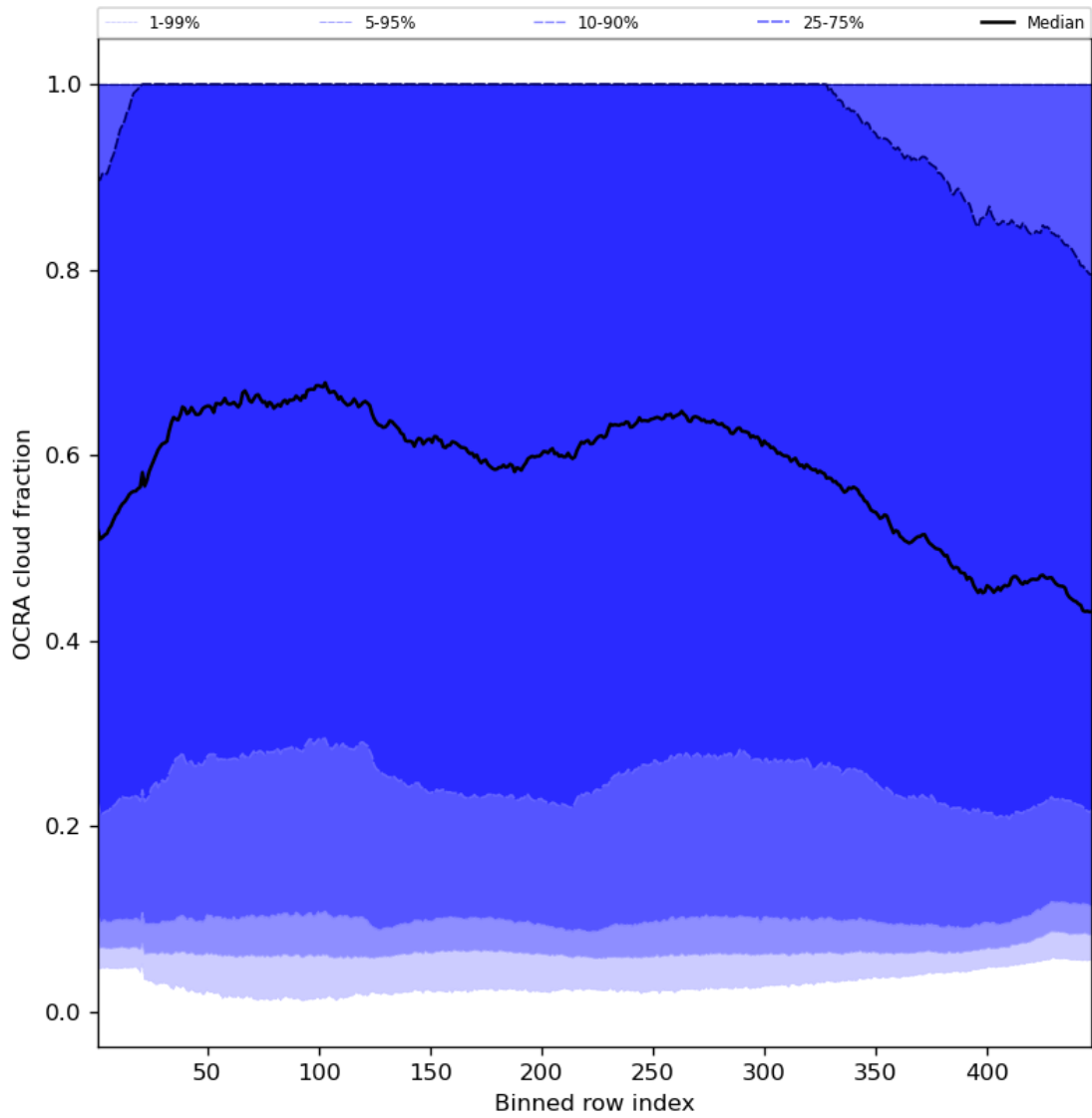
Figure 66: Along track statistics of “OCRA cloud fraction” for 2024-07-17 to 2024-07-19
