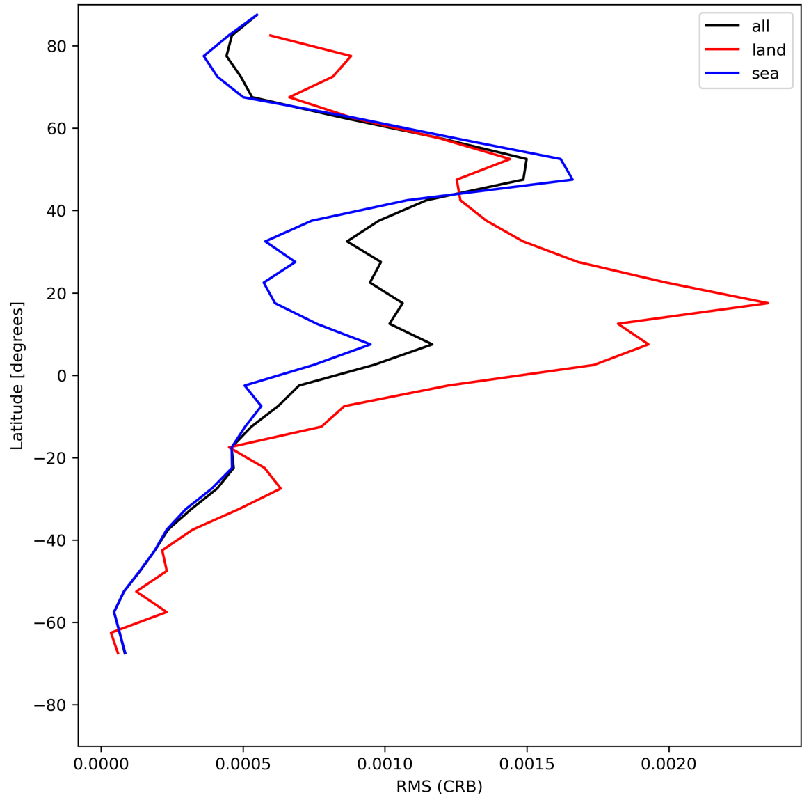
Figure 32: Zonal average of “RMS (CRB)” for 2024-07-17 to 2024-07-19.
