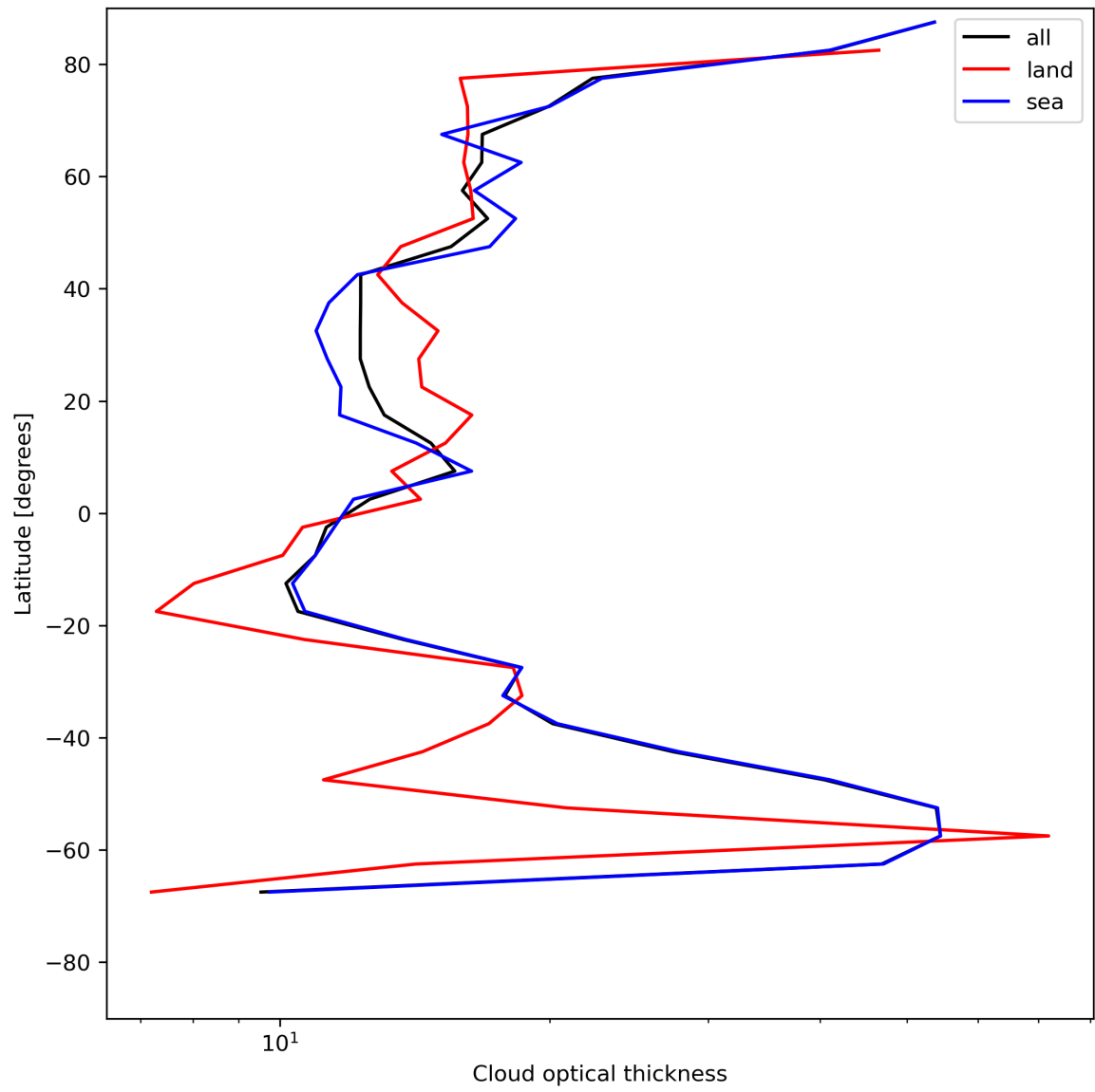
Figure 25: Zonal average of “Cloud optical thickness” for 2024-07-17 to 2024-07-19.
