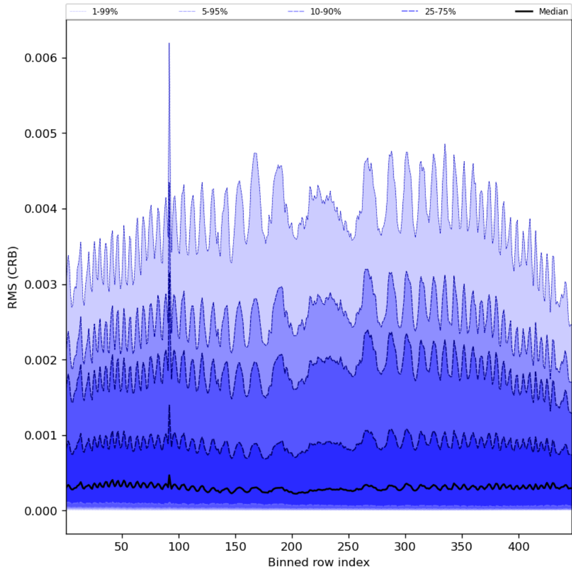
Figure 64: Along track statistics of “RMS (CRB)” for 2024-07-17 to 2024-07-19
