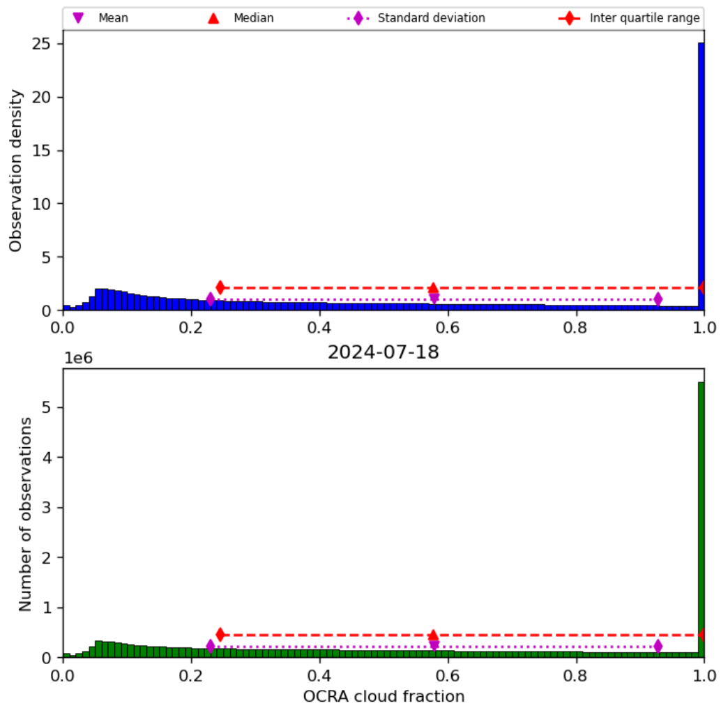
Figure 50: Histogram of “OCRA cloud fraction” for 2024-07-17 to 2024-07-19
