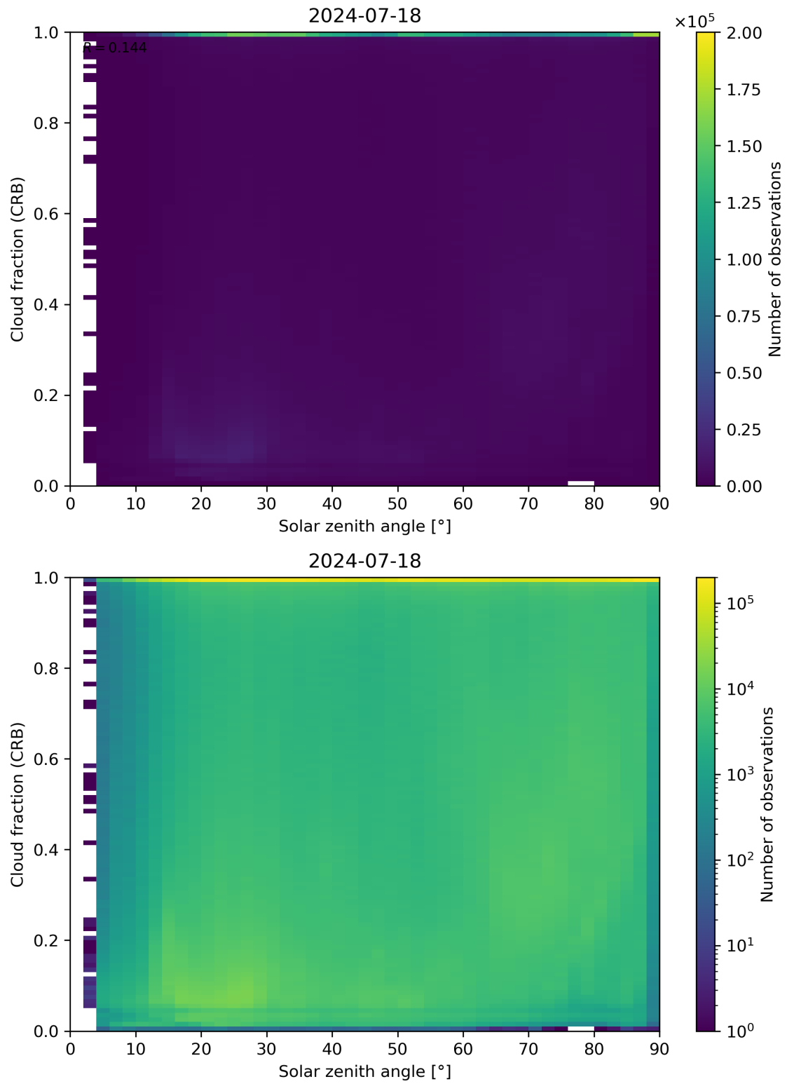
Figure 101: Scatter density plot of “Solar zenith angle” against “Cloud fraction (CRB)” for 2024-07-17 to 2024-07-19.
