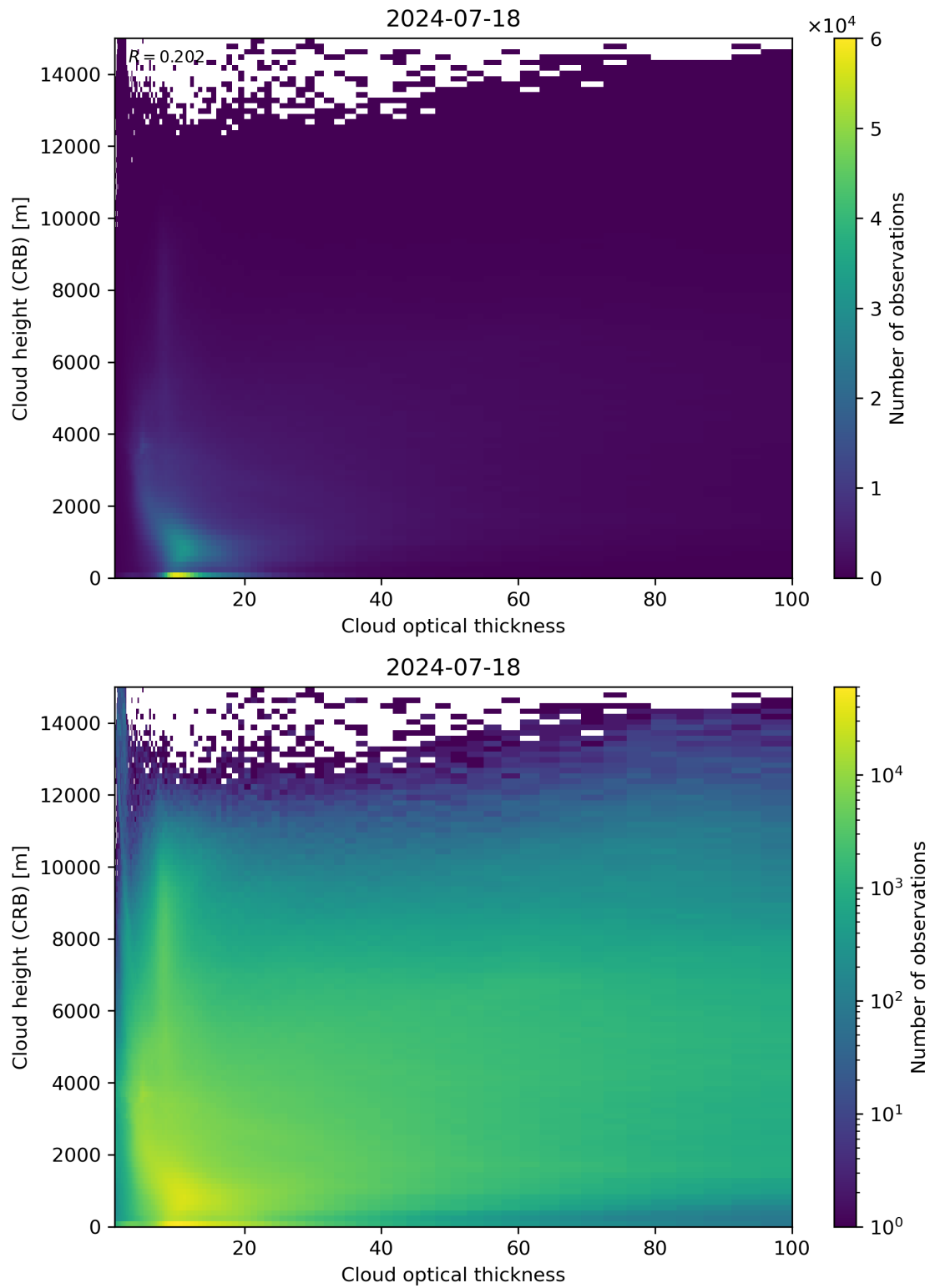
Figure 85: Scatter density plot of “Cloud optical thickness” against “Cloud height (CRB)” for 2024-07-17 to 2024-07-19.
