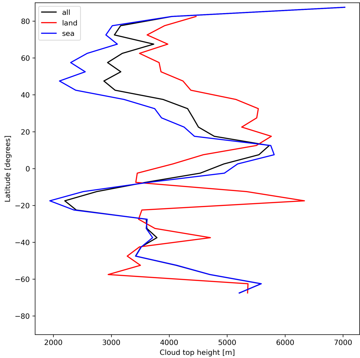
Figure 24: Zonal average of “Cloud top height” for 2024-07-17 to 2024-07-19.
