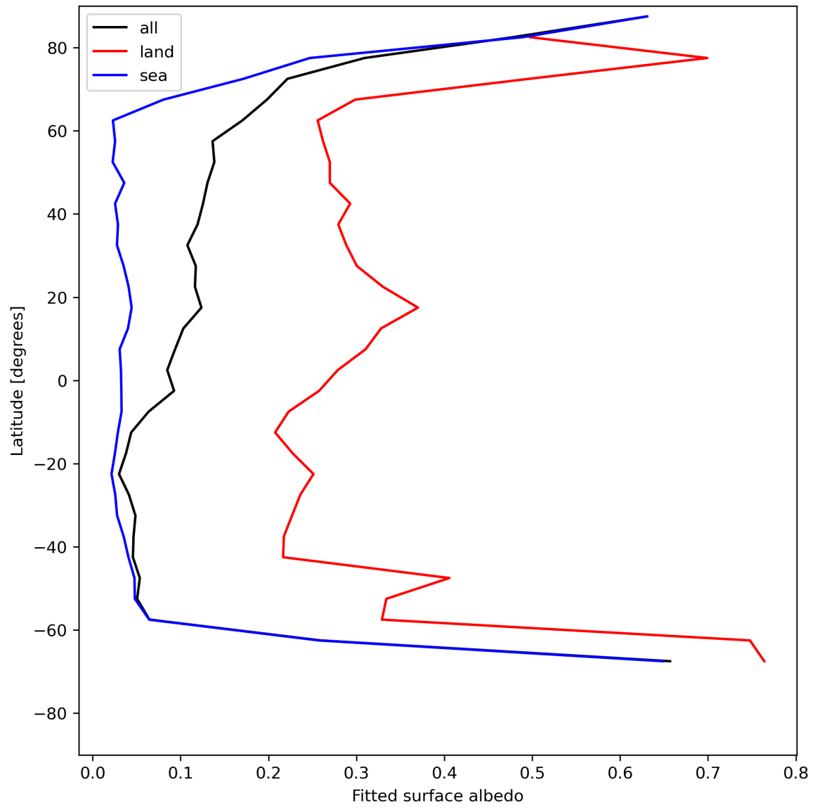
Figure 29: Zonal average of “Fitted surface albedo” for 2024-07-17 to 2024-07-19.
