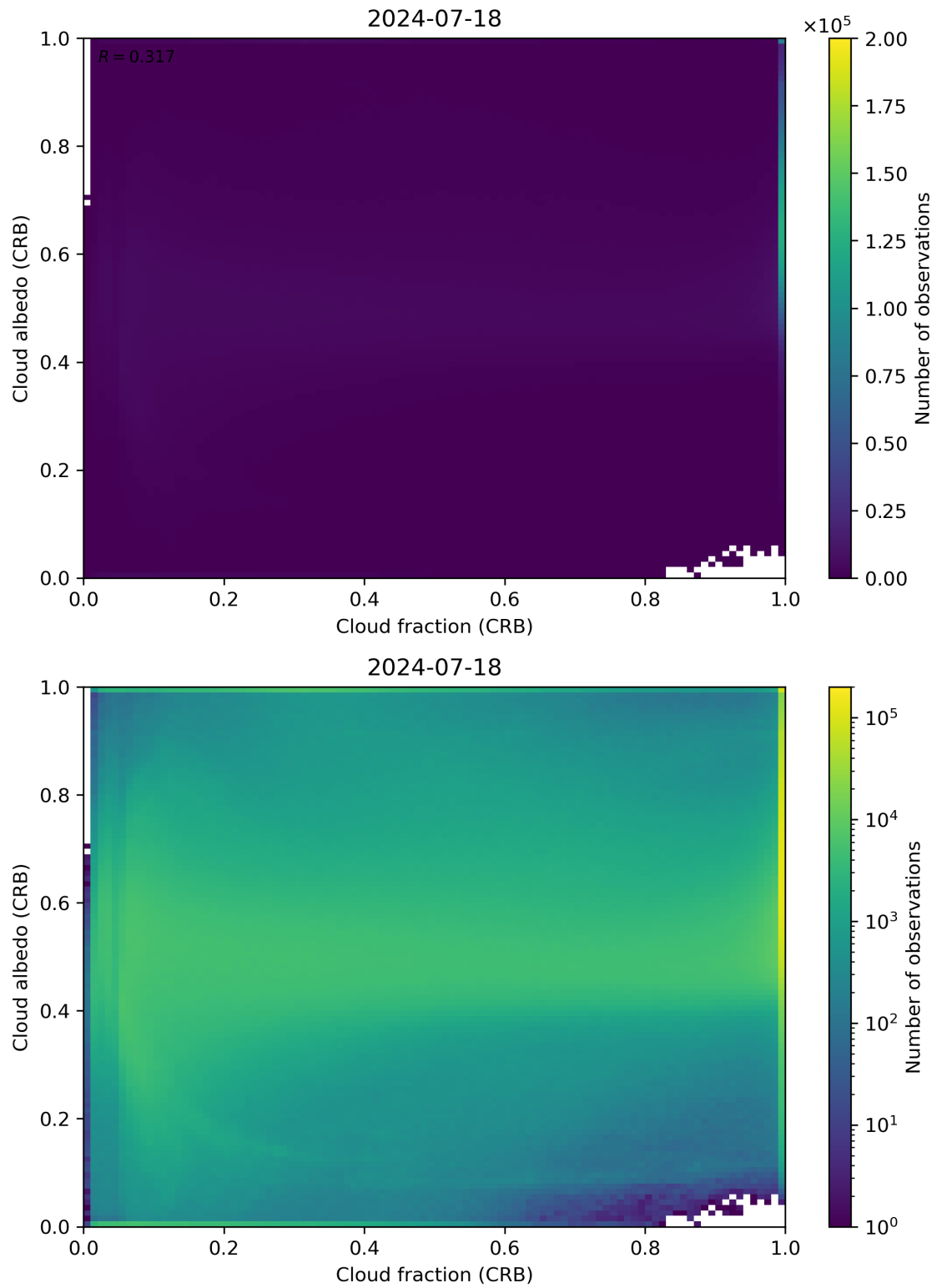
Figure 77: Scatter density plot of “Cloud fraction (CRB)” against “Cloud albedo (CRB)” for 2024-07-17 to 2024-07-19.
