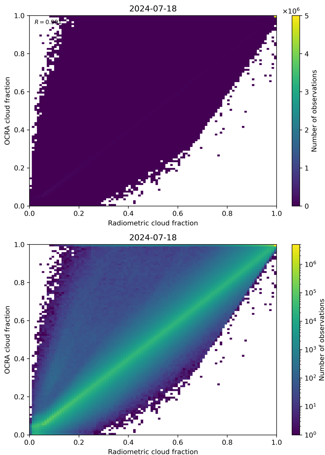
Figure 72: Scatter density plot of “Radiometric cloud fraction” against “OCRA cloud fraction” for 2024-07-17 to 2024-07-19.
