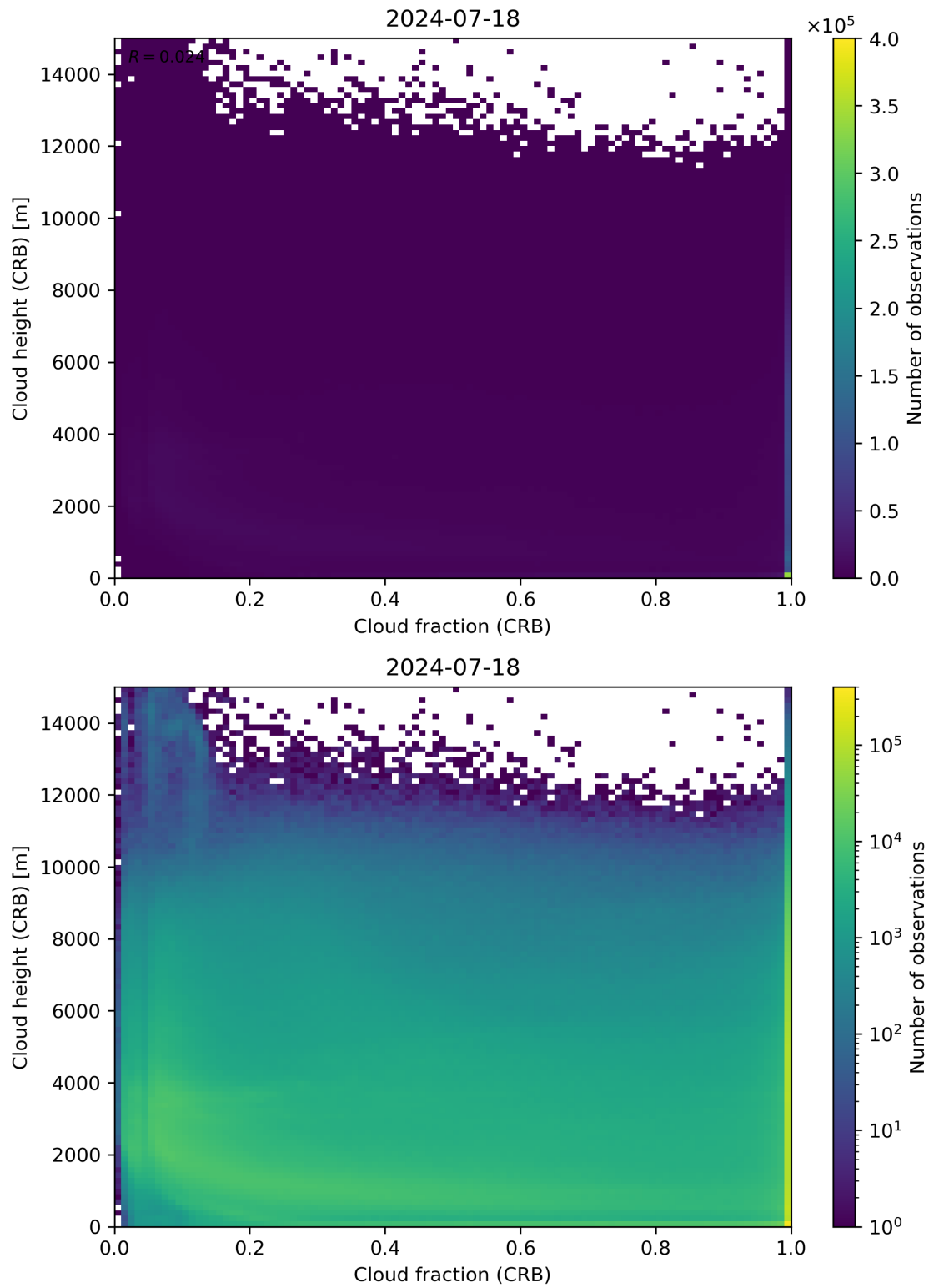
Figure 79: Scatter density plot of “Cloud fraction (CRB)” against “Cloud height (CRB)” for 2024-07-17 to 2024-07-19.
