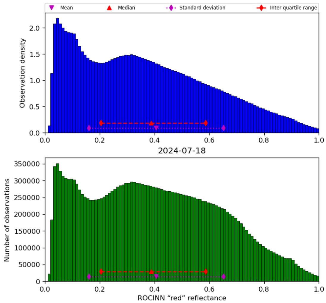
Figure 53: Histogram of “ROCINN “red” reflectance” for 2024-07-17 to 2024-07-19
