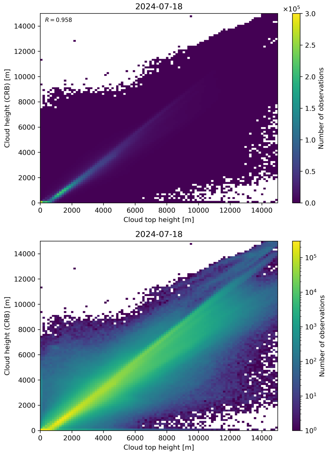
Figure 89: Scatter density plot of “Cloud top height” against “Cloud height (CRB)” for 2024-07-17 to 2024-07-19.
