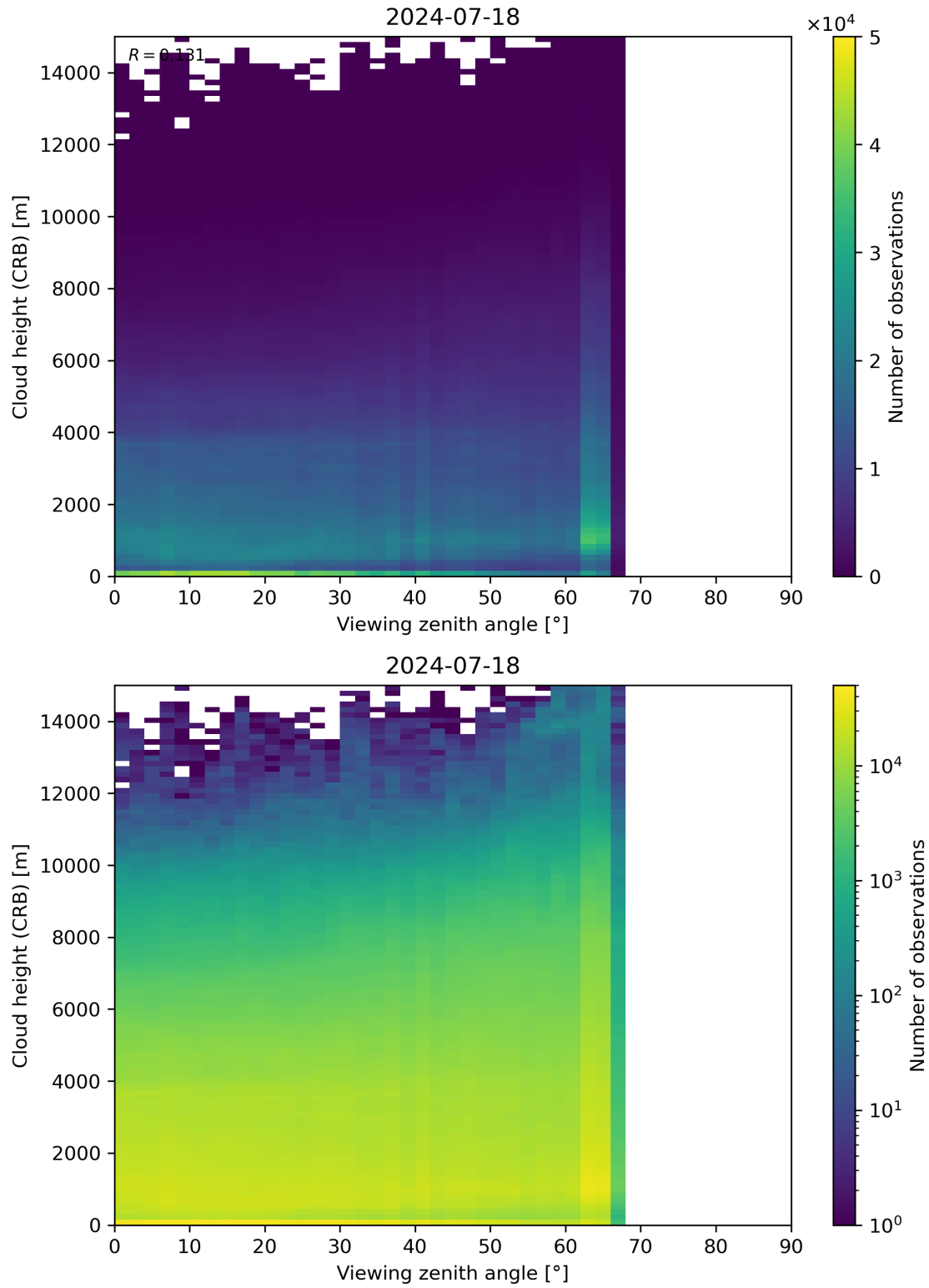
Figure 110: Scatter density plot of “Viewing zenith angle” against “Cloud height (CRB)” for 2024-07-17 to 2024-07-19.
