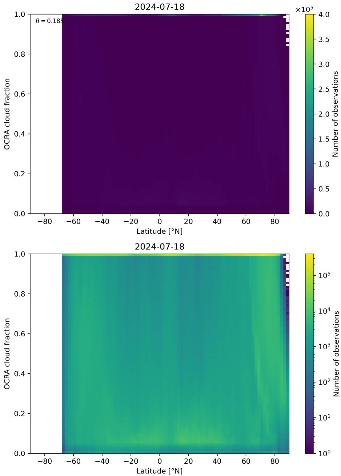
Figure 93: Scatter density plot of “Latitude” against “OCRA cloud fraction” for 2024-07-17 to 2024-07-19.
