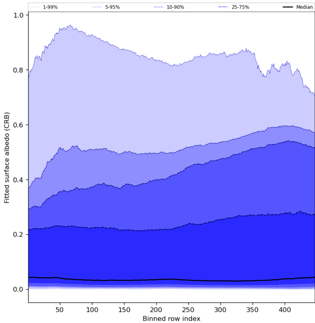
Figure 62: Along track statistics of “Fitted surface albedo (CRB)” for 2024-07-17 to 2024-07-19
