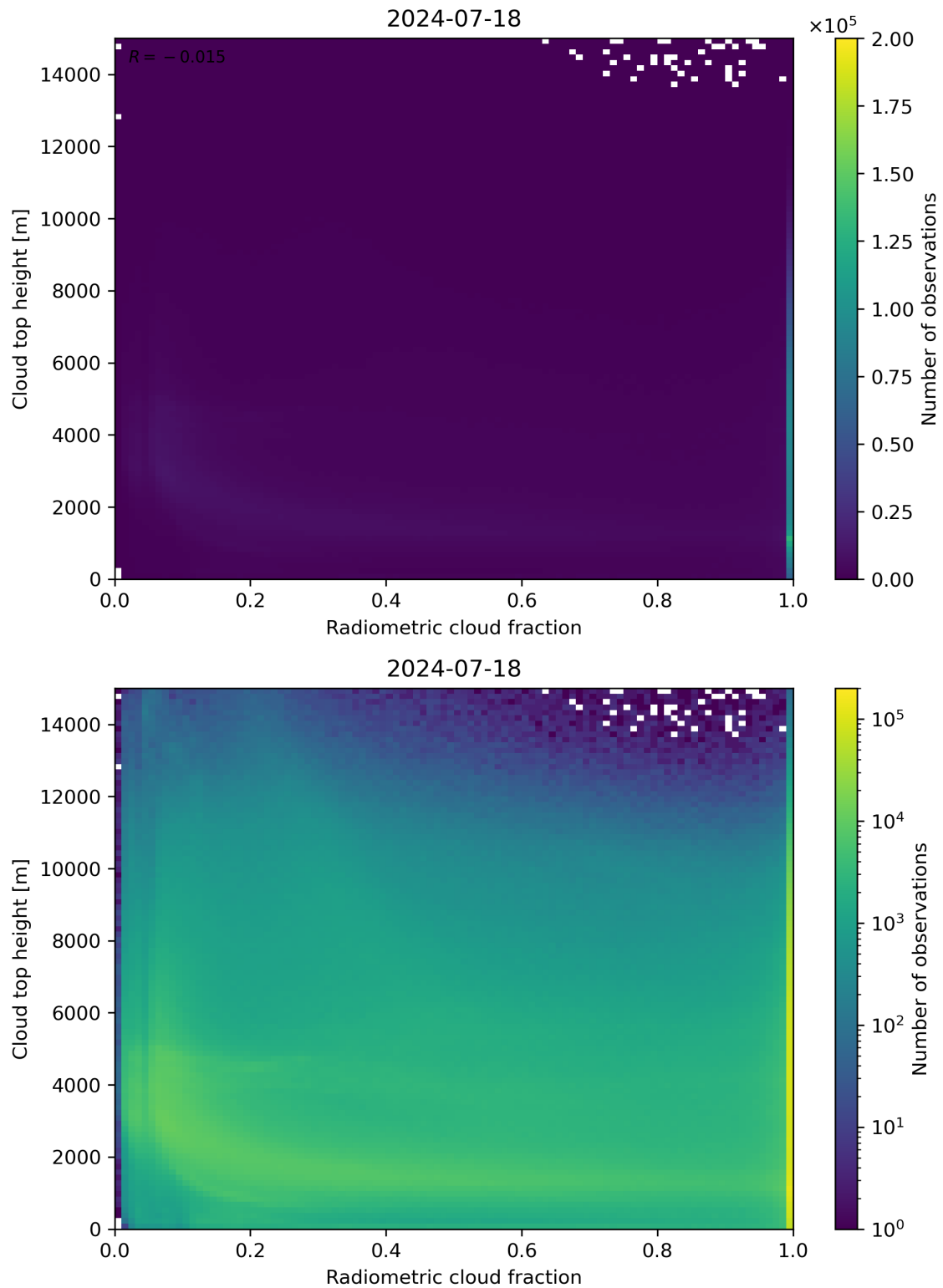
Figure 76: Scatter density plot of “Radiometric cloud fraction” against “Cloud top height” for 2024-07-17 to 2024-07-19.
