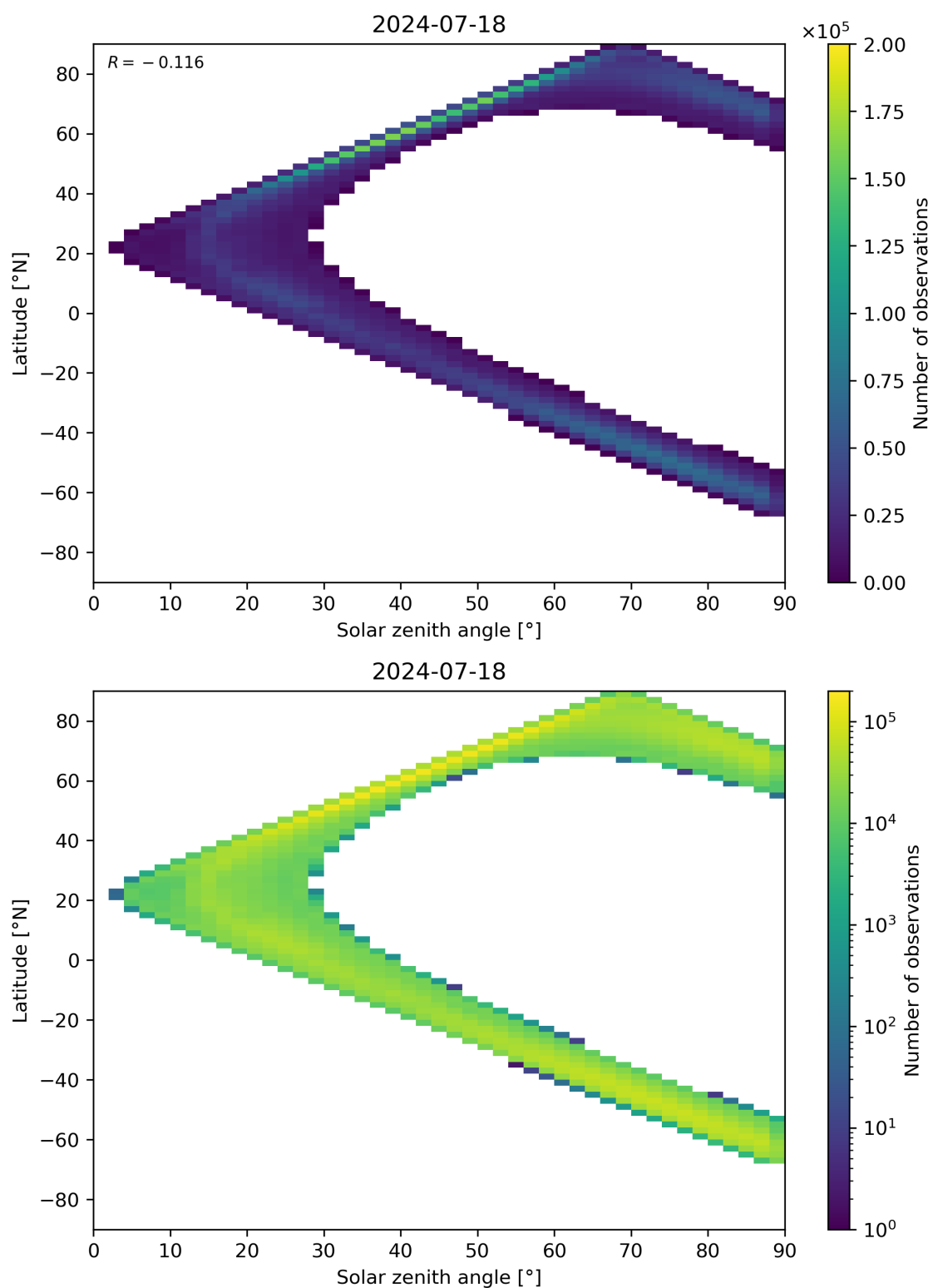
Figure 105: Scatter density plot of “Solar zenith angle” against “Latitude” for 2024-07-17 to 2024-07-19.
