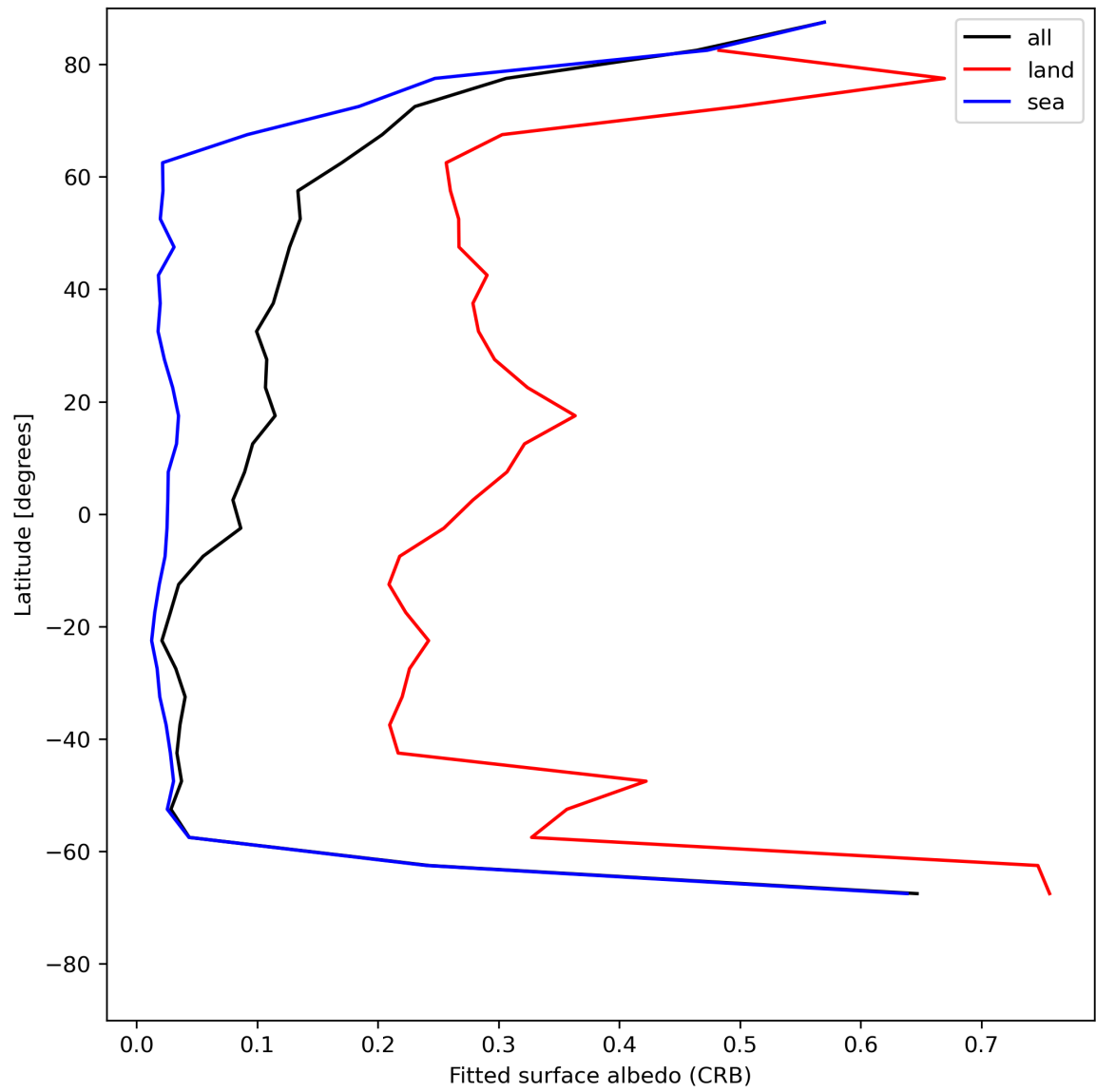
Figure 30: Zonal average of “Fitted surface albedo (CRB)” for 2024-07-17 to 2024-07-19.
