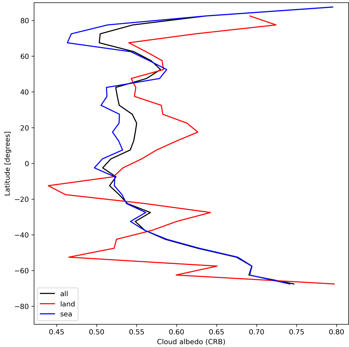
Figure 28: Zonal average of “Cloud albedo (CRB)” for 2024-07-17 to 2024-07-19.
