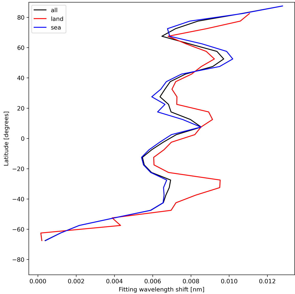
Figure 33: Zonal average of “Fitting wavelength shift” for 2024-07-17 to 2024-07-19.
