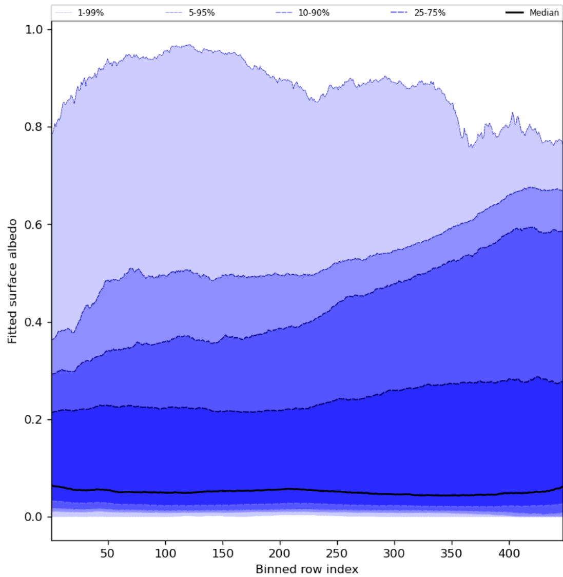
Figure 61: Along track statistics of “Fitted surface albedo” for 2024-07-17 to 2024-07-19
