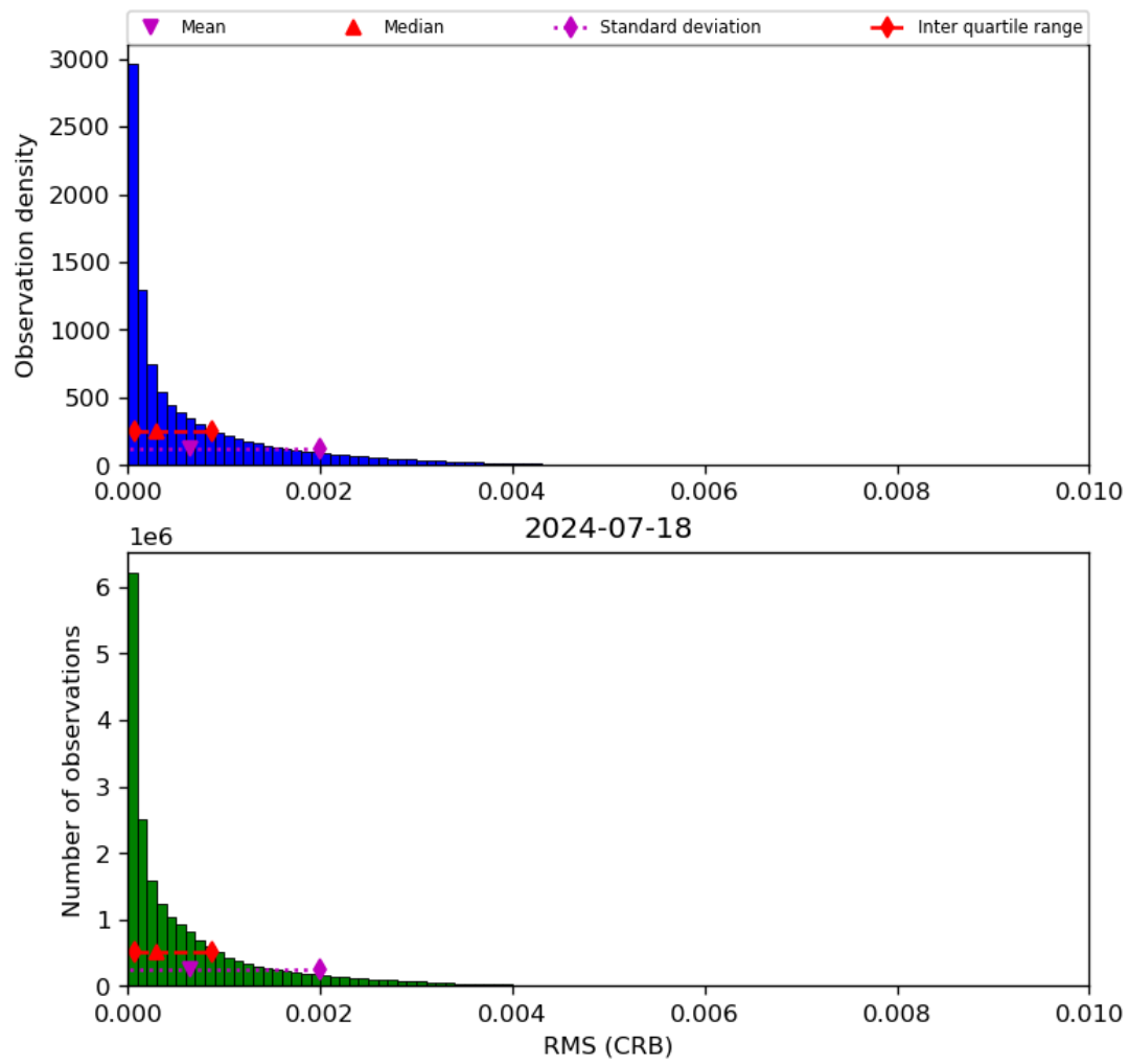
Figure 48: Histogram of “RMS (CRB)” for 2024-07-17 to 2024-07-19
