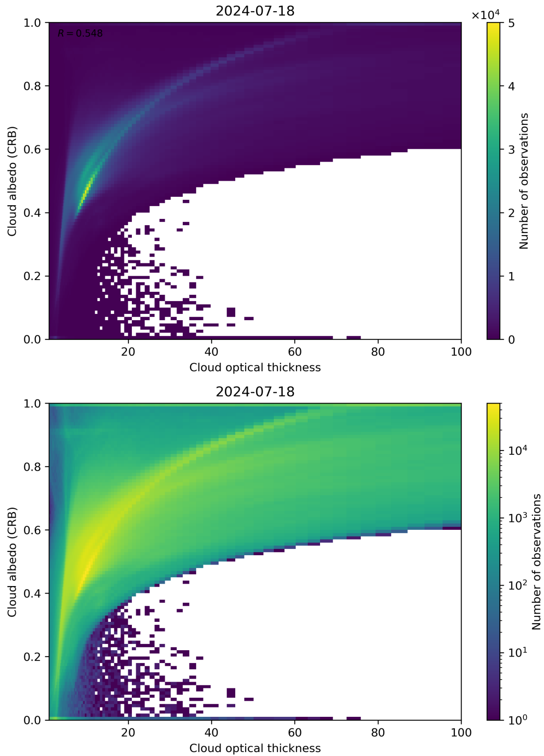
Figure 82: Scatter density plot of “Cloud optical thickness” against “Cloud albedo (CRB)” for 2024-07-17 to 2024-07-19.
