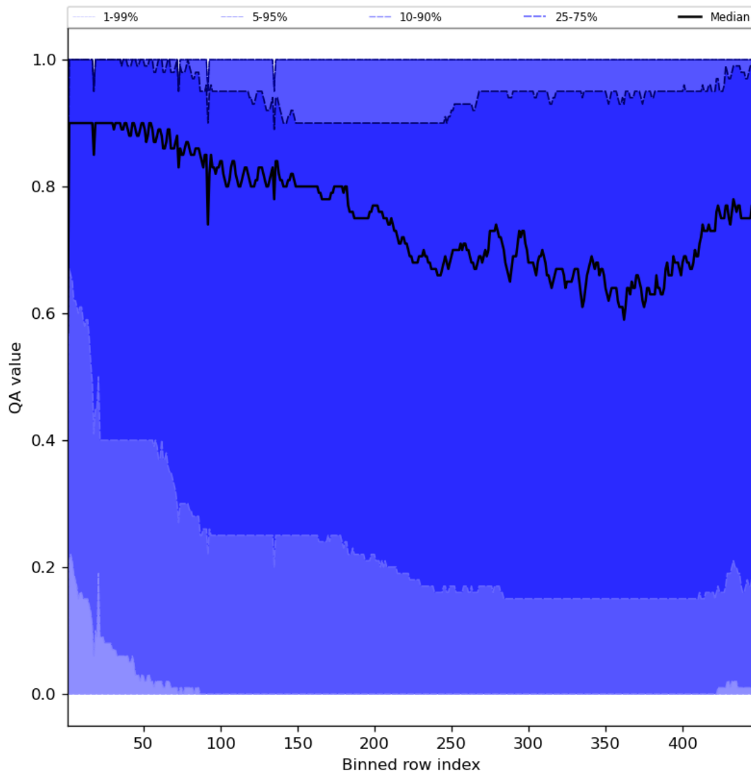
Figure 54: Along track statistics of “QA value” for 2024-07-17 to 2024-07-19
