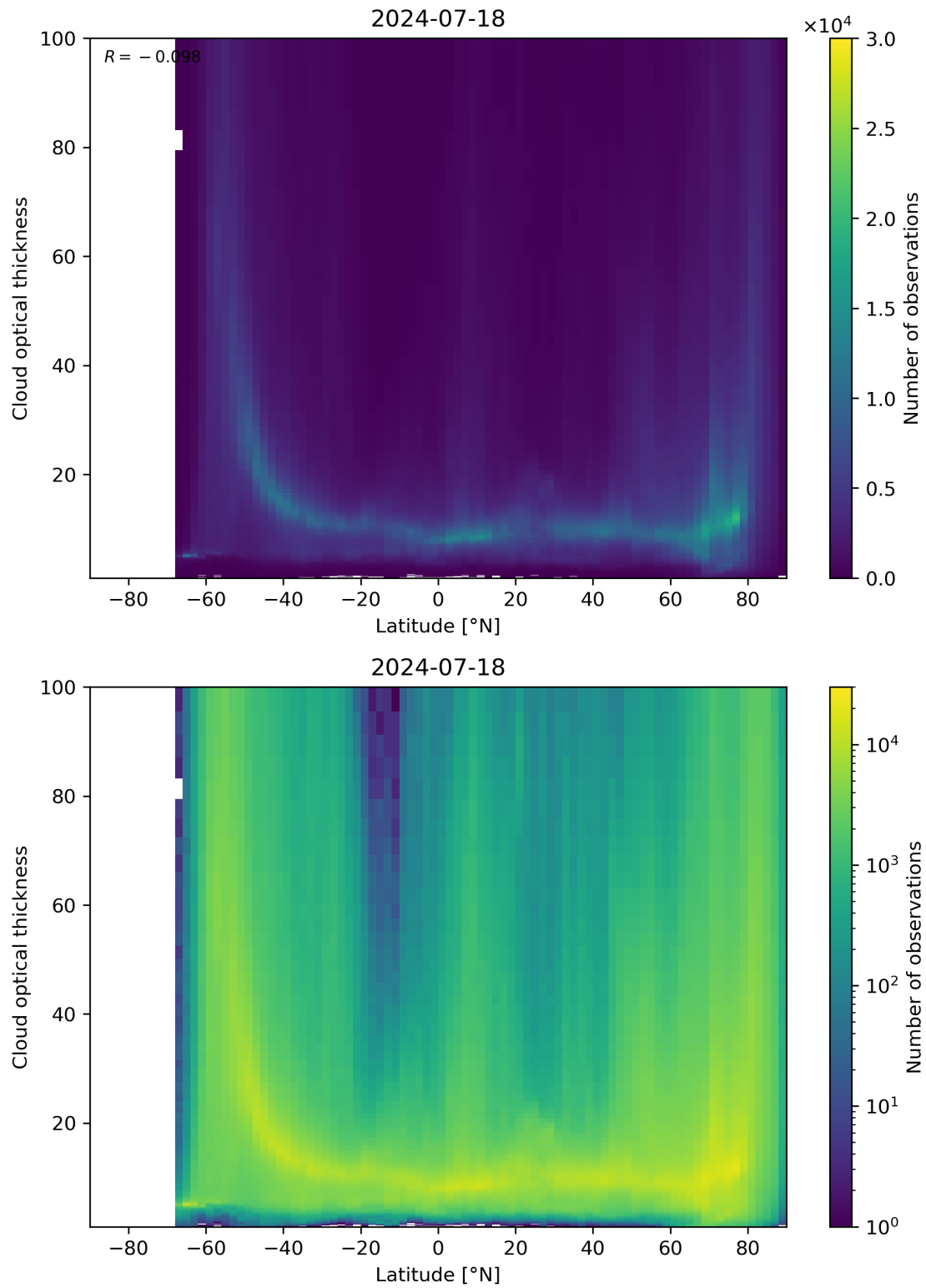
Figure 96: Scatter density plot of “Latitude” against “Cloud optical thickness” for 2024-07-17 to 2024-07-19.
