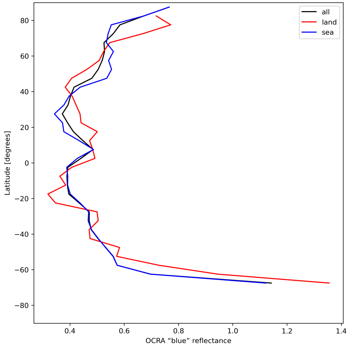
Figure 35: Zonal average of “OCRA “blue” reflectance” for 2024-07-17 to 2024-07-19.
