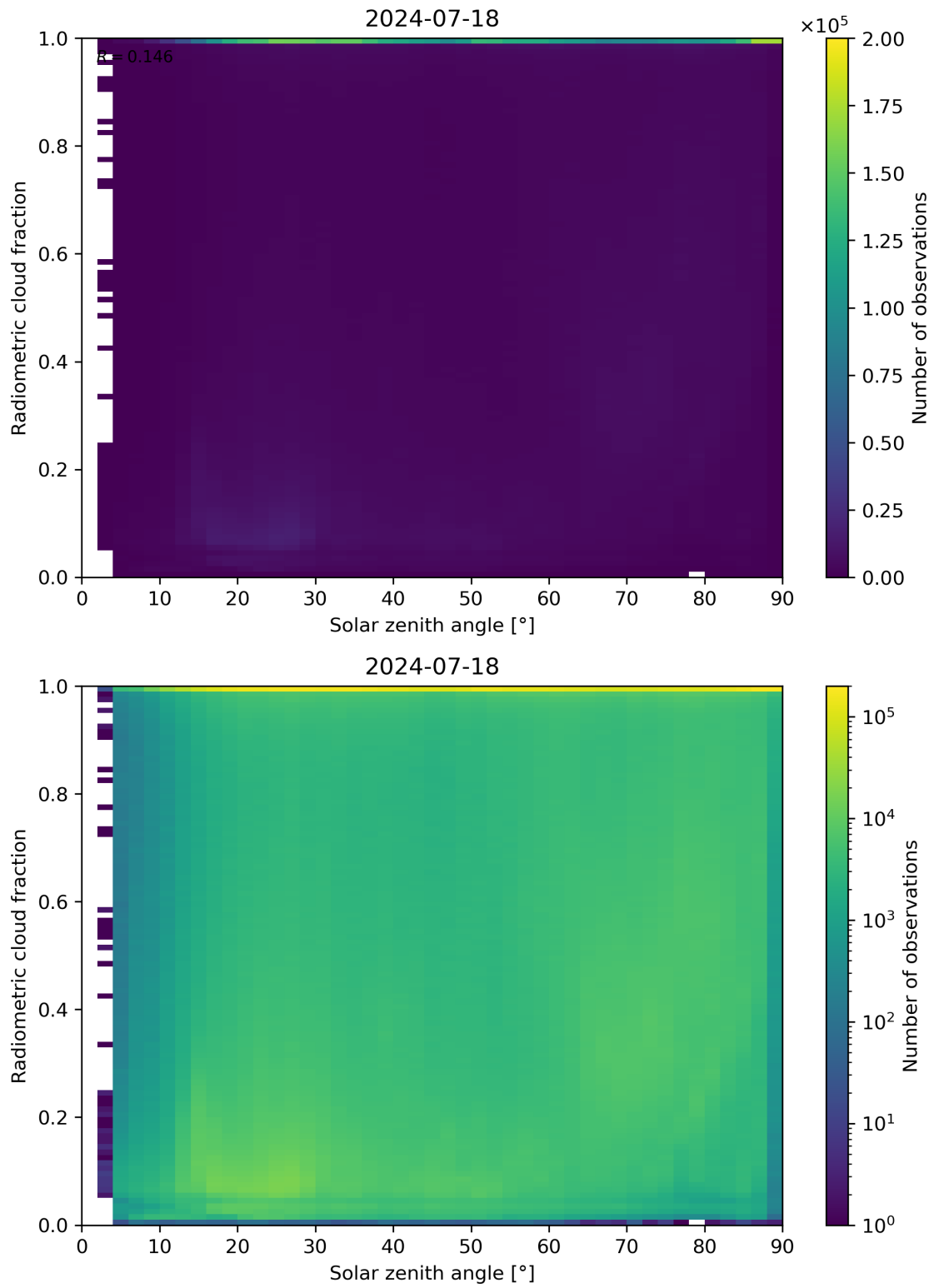
Figure 99: Scatter density plot of “Solar zenith angle” against “Radiometric cloud fraction” for 2024-07-17 to 2024-07-19.
