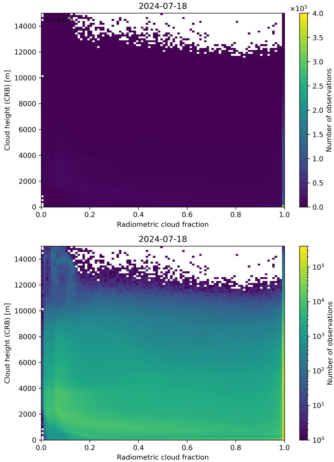
Figure 74: Scatter density plot of “Radiometric cloud fraction” against “Cloud height (CRB)” for 2024-07-17 to 2024-07-19.
