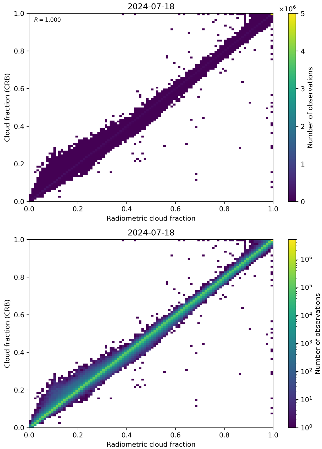
Figure 73: Scatter density plot of “Radiometric cloud fraction” against “Cloud fraction (CRB)” for 2024-07-17 to 2024-07-19.
