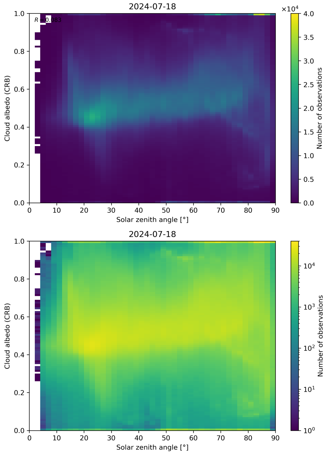
Figure 98: Scatter density plot of “Solar zenith angle” against “Cloud albedo (CRB)” for 2024-07-17 to 2024-07-19.
