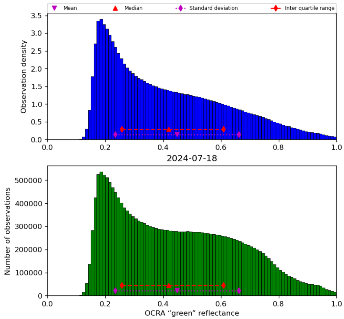
Figure 52: Histogram of “OCRA “green” reflectance” for 2024-07-17 to 2024-07-19
