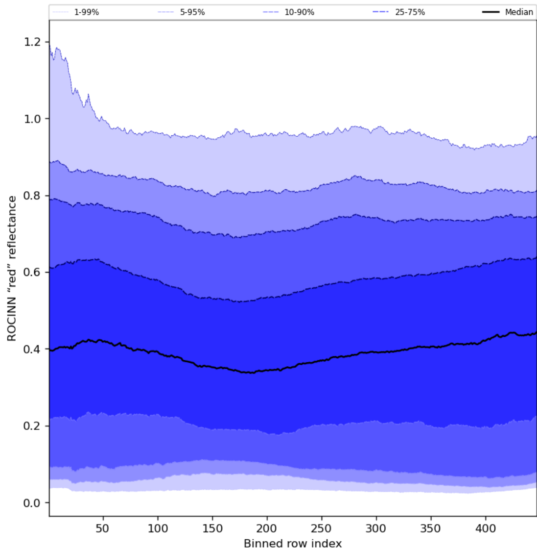
Figure 69: Along track statistics of "ROCINN "red" reflectance" for 2024-07-17 to 2024-07-19
