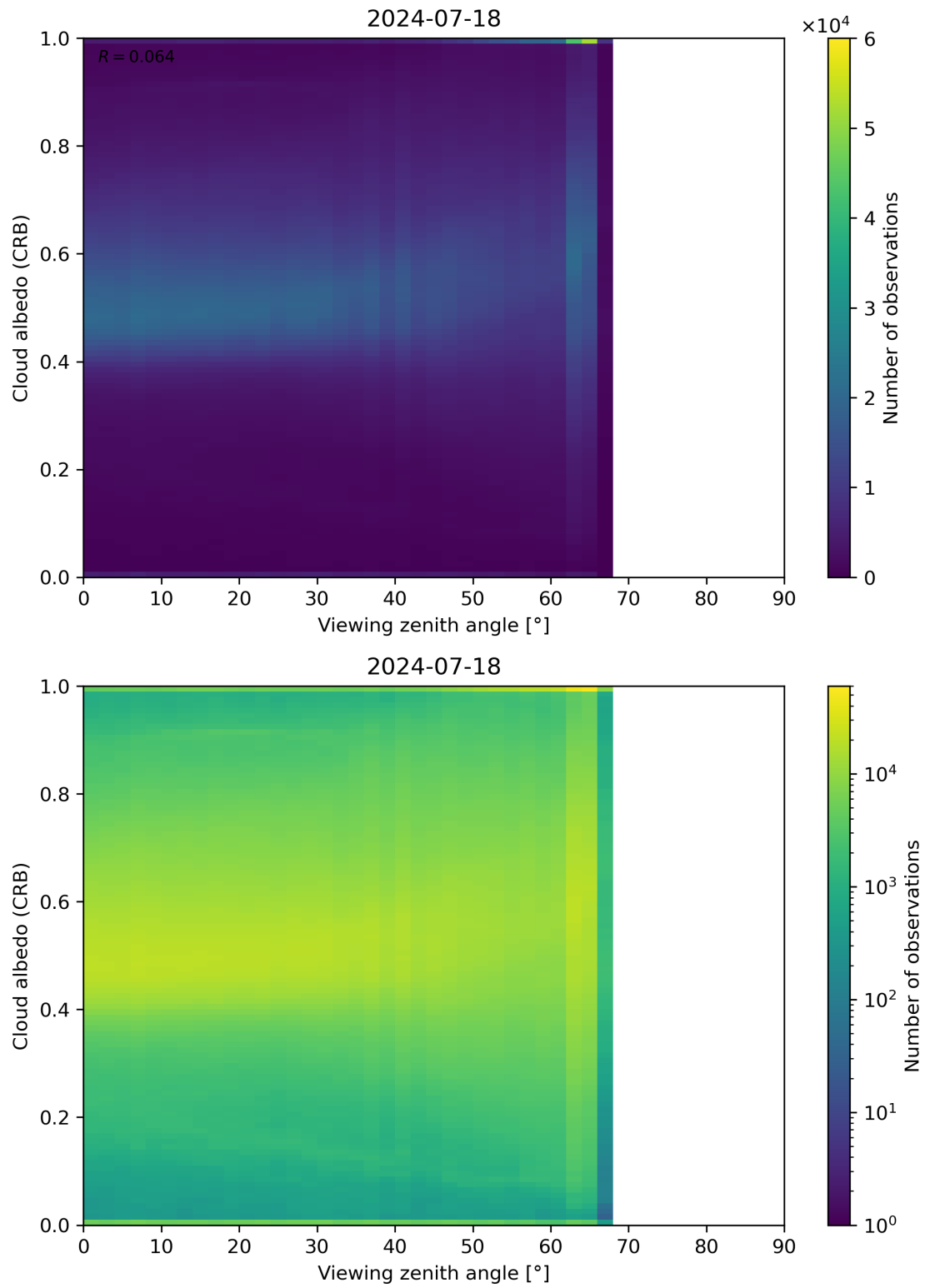
Figure 106: Scatter density plot of “Viewing zenith angle” against “Cloud albedo (CRB)” for 2024-07-17 to 2024-07-19.
