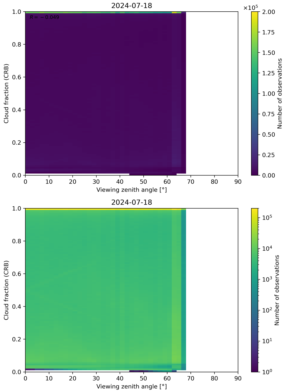
Figure 109: Scatter density plot of “Viewing zenith angle” against “Cloud fraction (CRB)” for 2024-07-17 to 2024-07-19.
