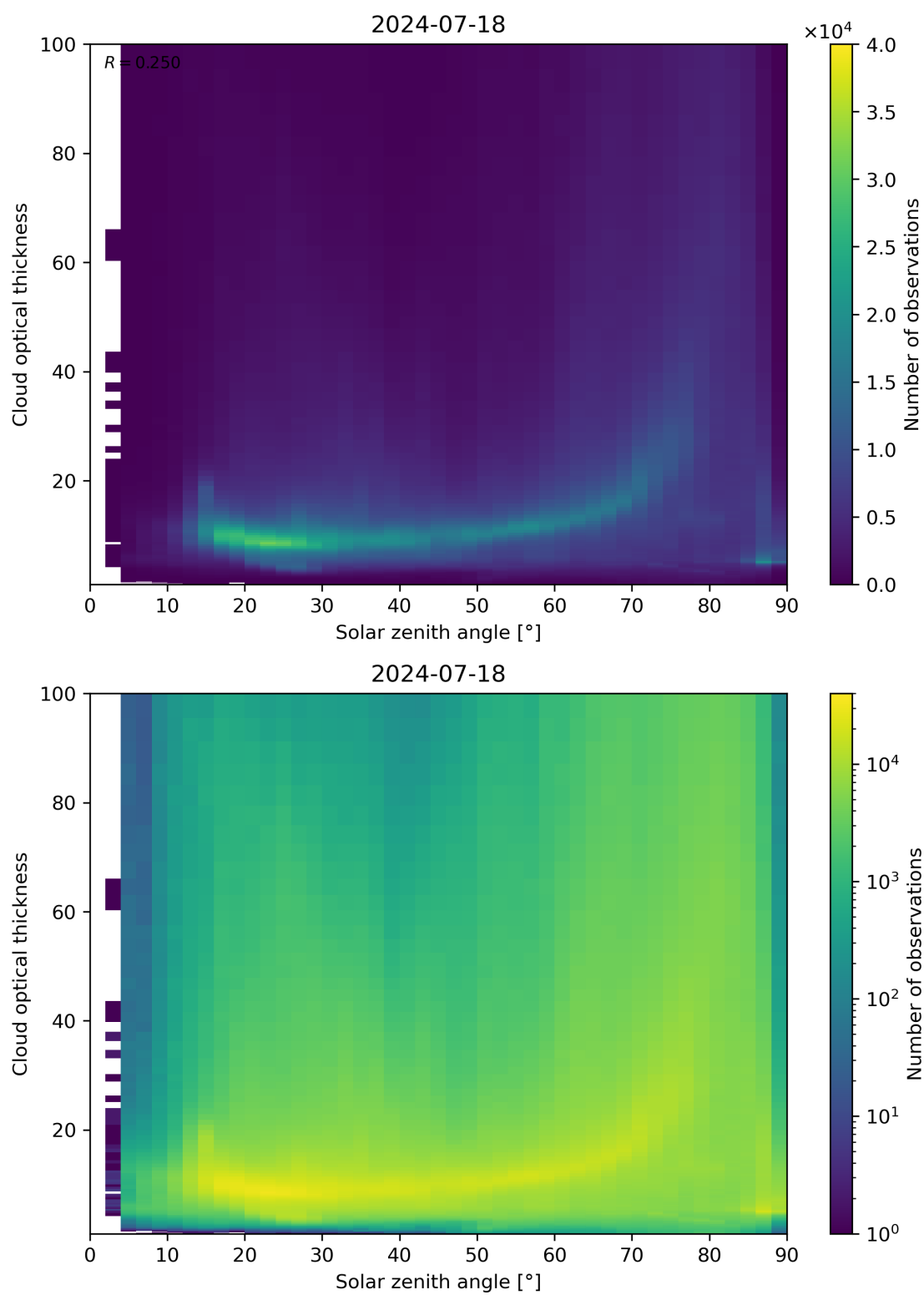
Figure 103: Scatter density plot of “Solar zenith angle” against “Cloud optical thickness” for 2024-07-17 to 2024-07-19.
