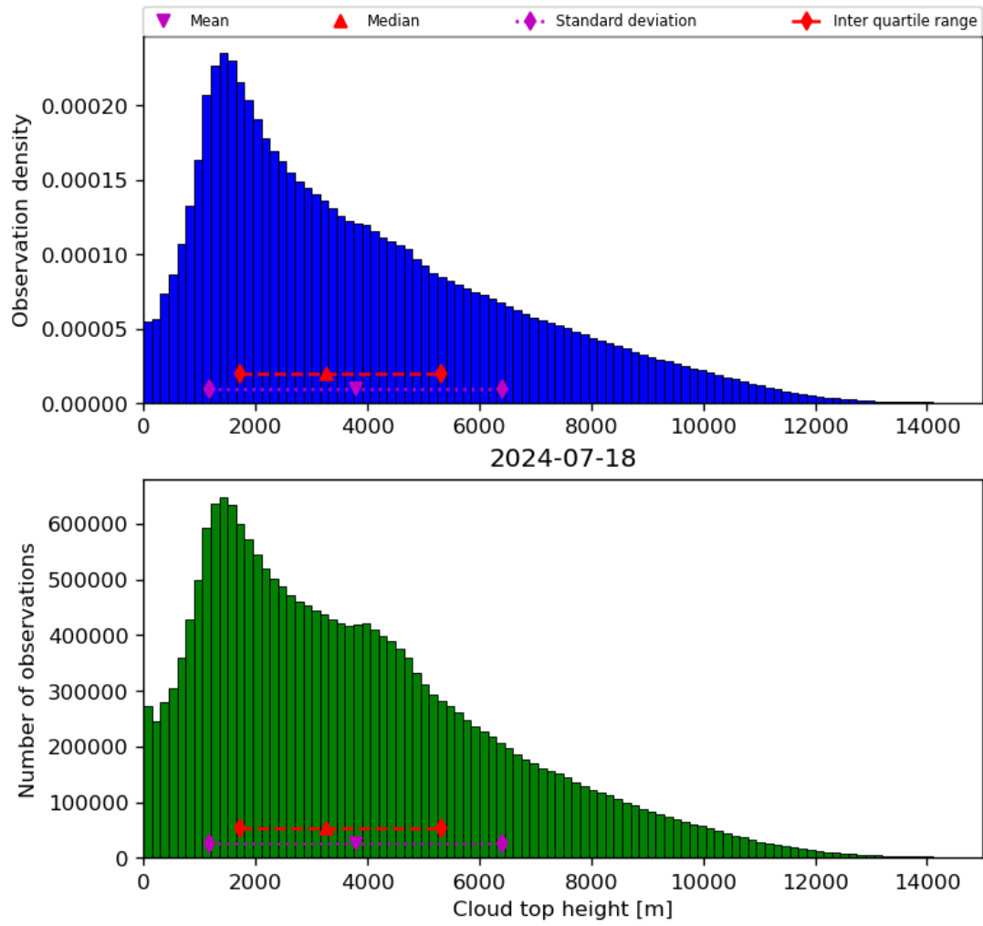
Figure 40: Histogram of “Cloud top height” for 2024-07-17 to 2024-07-19
