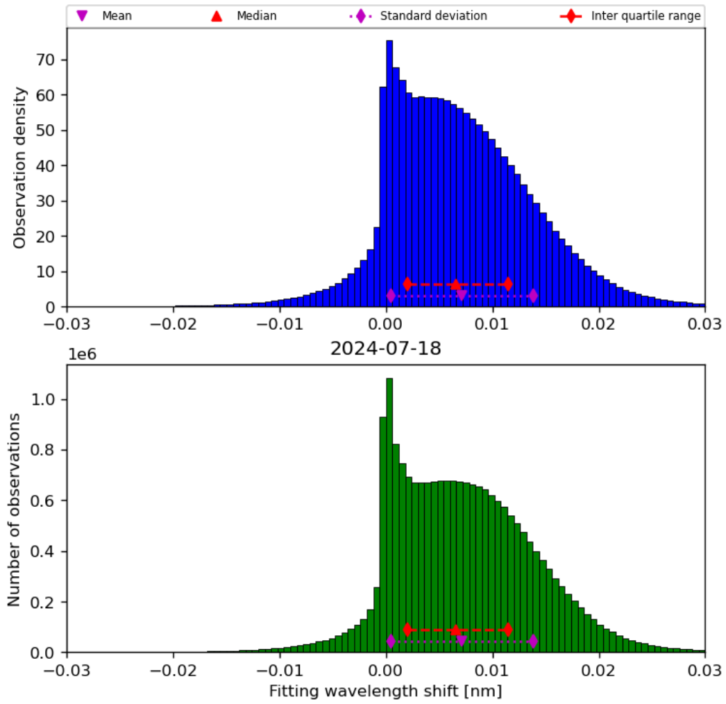
Figure 49: Histogram of “Fitting wavelength shift” for 2024-07-17 to 2024-07-19
