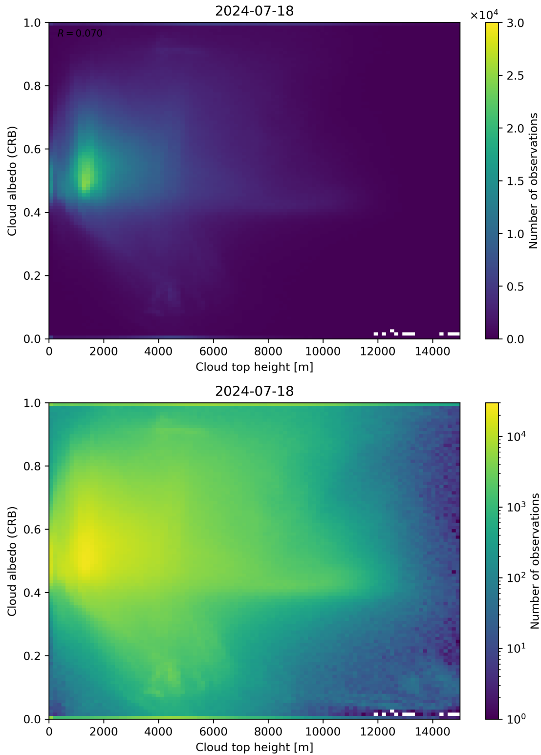
Figure 86: Scatter density plot of “Cloud top height” against “Cloud albedo (CRB)” for 2024-07-17 to 2024-07-19.
