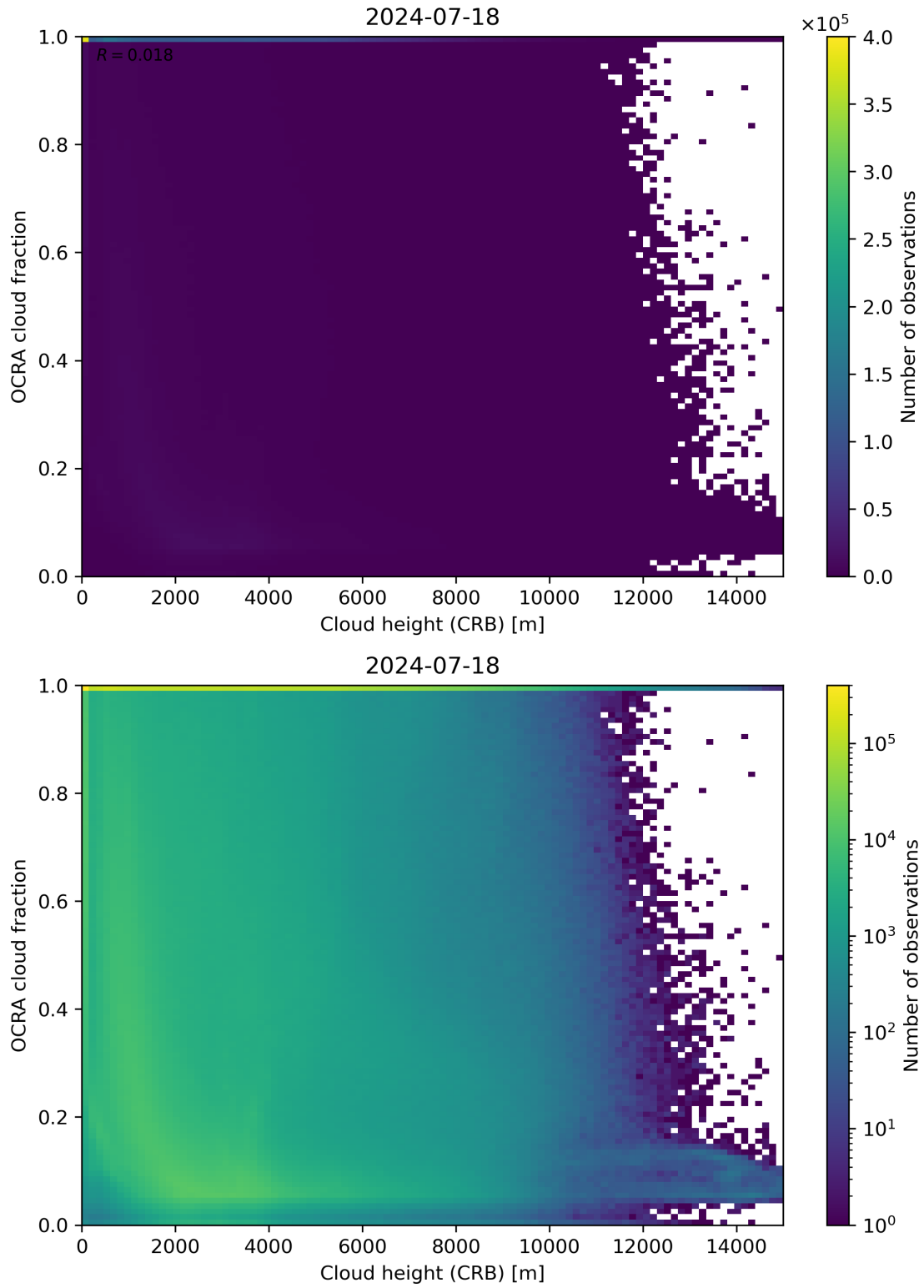
Figure 81: Scatter density plot of “Cloud height (CRB)” against “OCRA cloud fraction” for 2024-07-17 to 2024-07-19.
