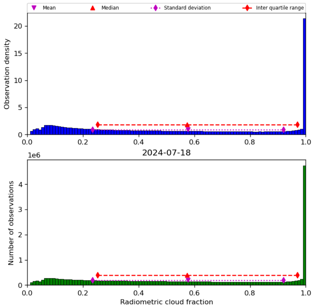
Figure 39: Histogram of “Radiometric cloud fraction” for 2024-07-17 to 2024-07-19
