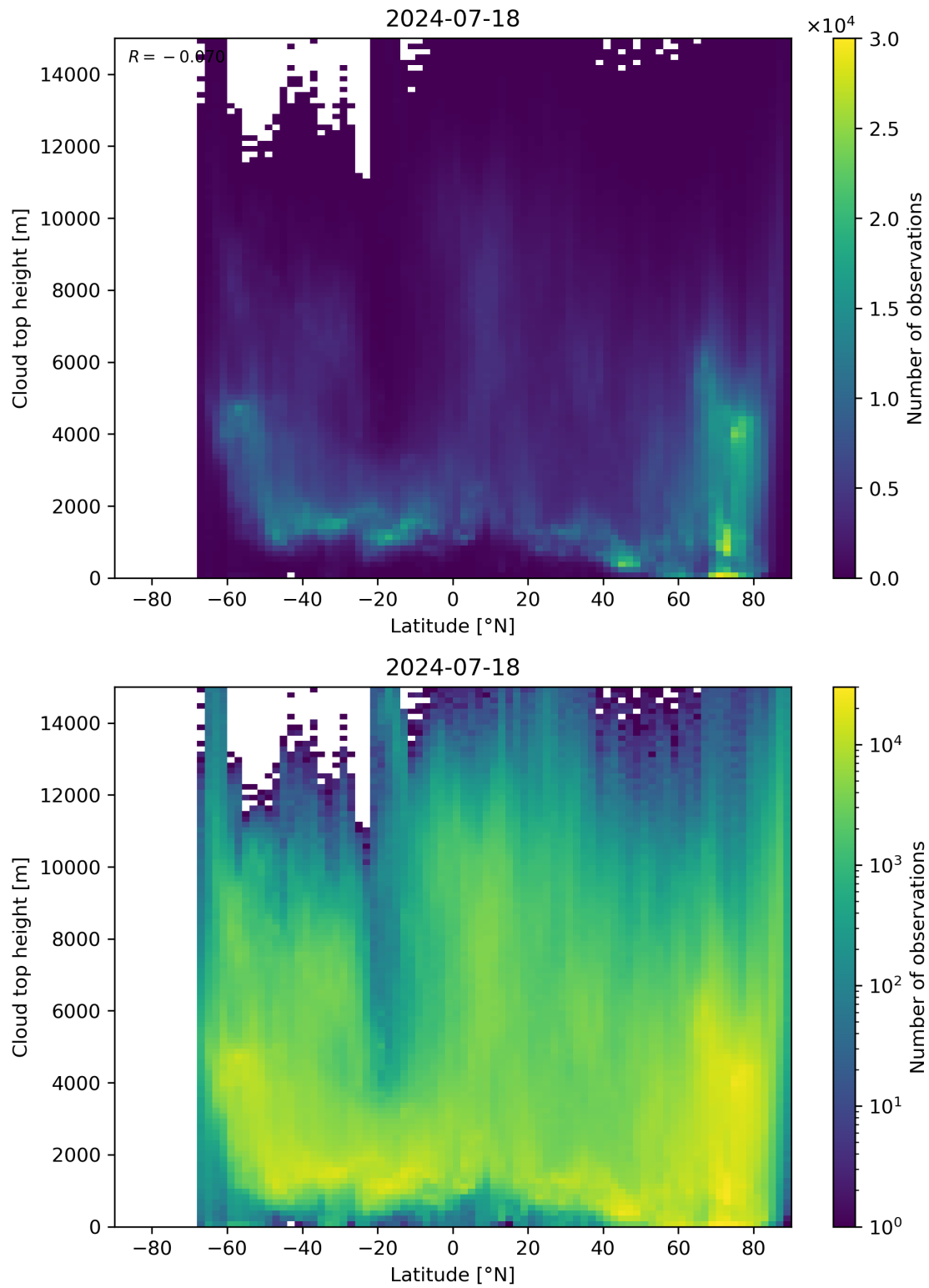
Figure 97: Scatter density plot of “Latitude” against “Cloud top height” for 2024-07-17 to 2024-07-19.
