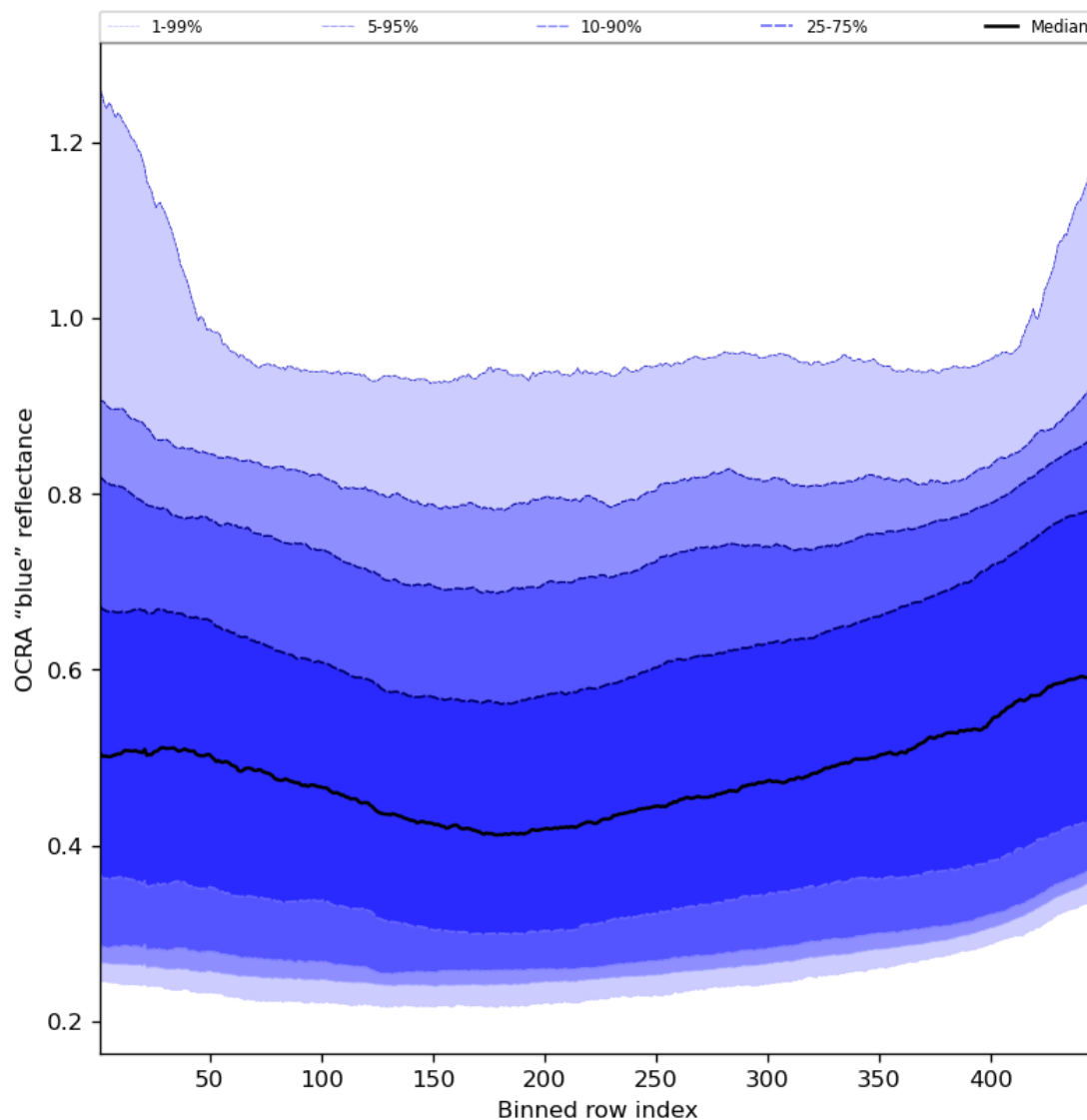
Figure 67: Along track statistics of “OCRA “blue” reflectance” for 2024-07-17 to 2024-07-19
