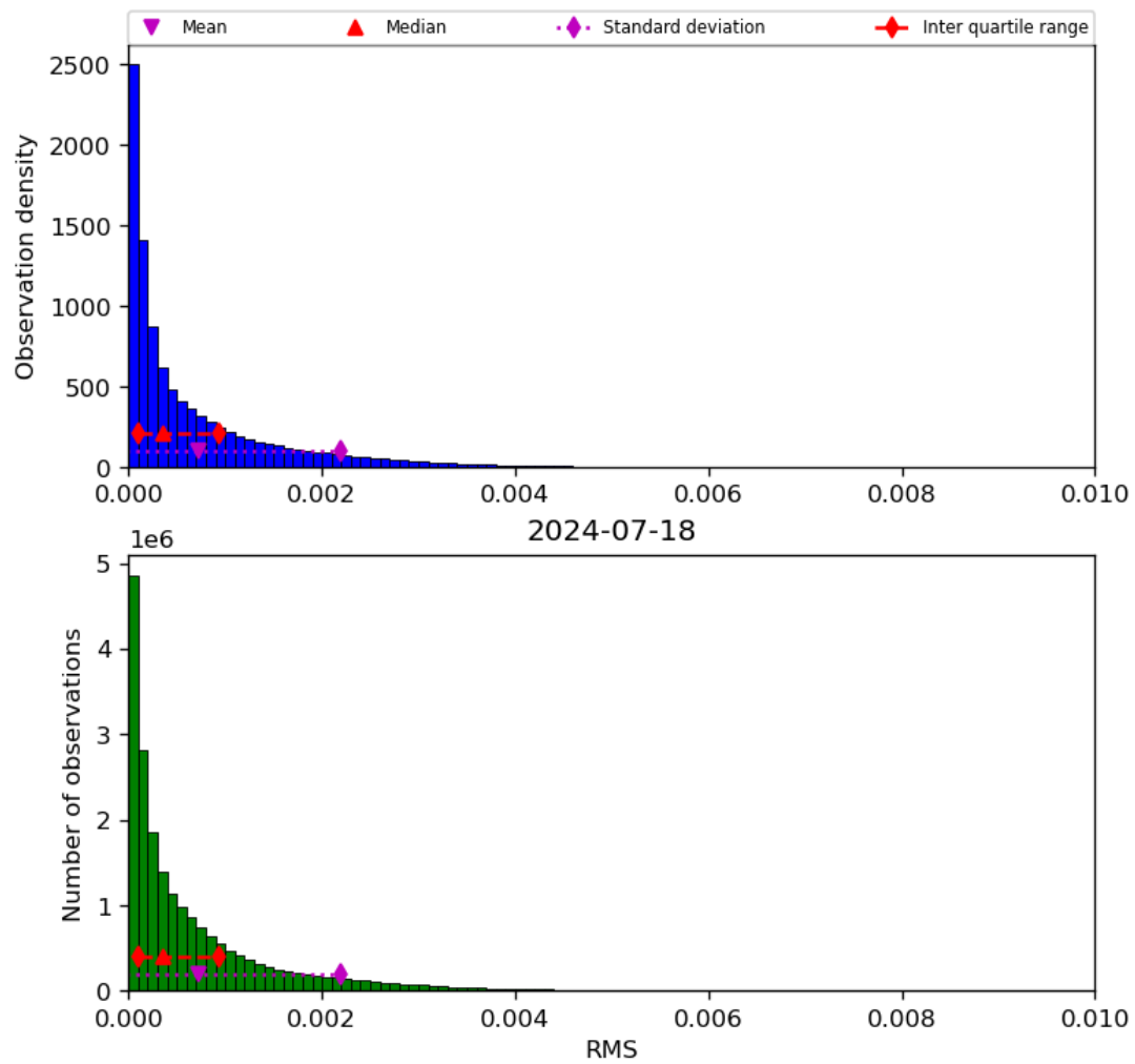
Figure 47: Histogram of “RMS” for 2024-07-17 to 2024-07-19
