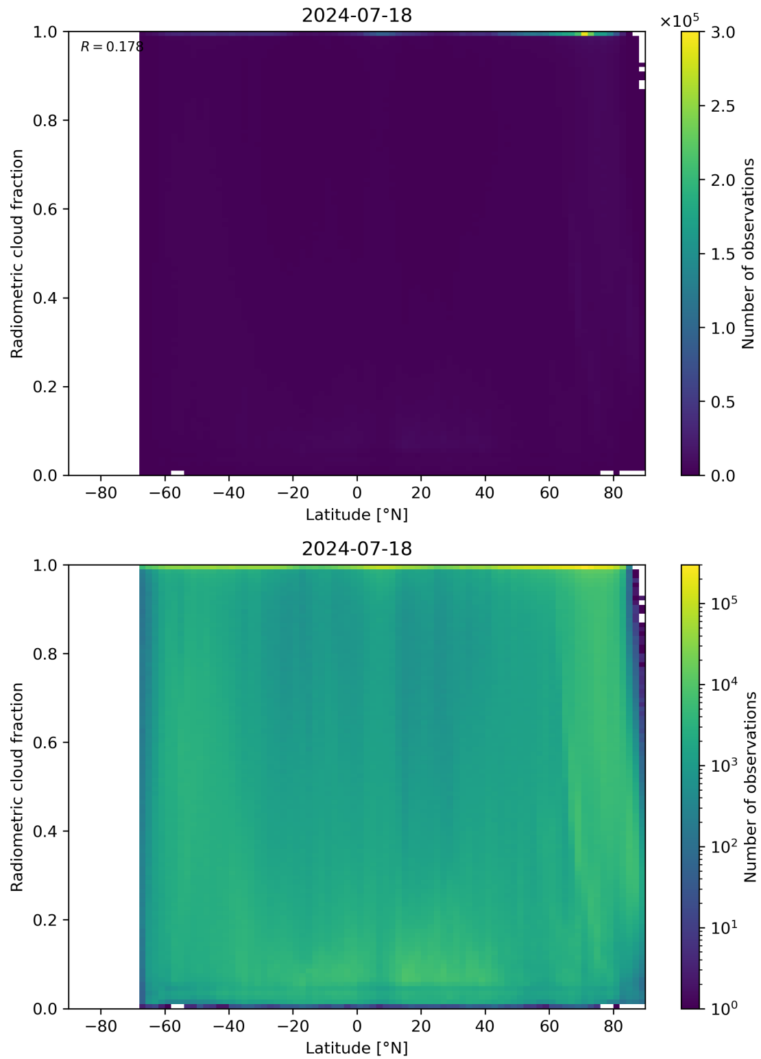
Figure 92: Scatter density plot of “Latitude” against “Radiometric cloud fraction” for 2024-07-17 to 2024-07-19.
