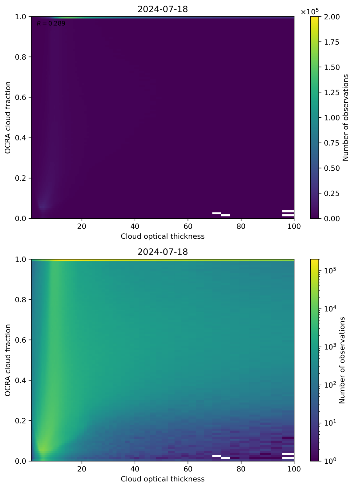
Figure 83: Scatter density plot of “Cloud optical thickness” against “OCRA cloud fraction” for 2024-07-17 to 2024-07-19.
