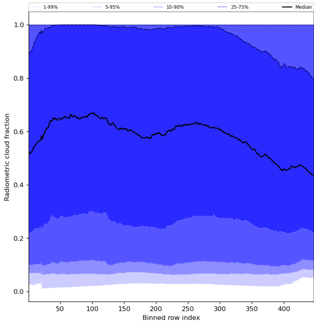
Figure 55: Along track statistics of “Radiometric cloud fraction” for 2024-07-17 to 2024-07-19
