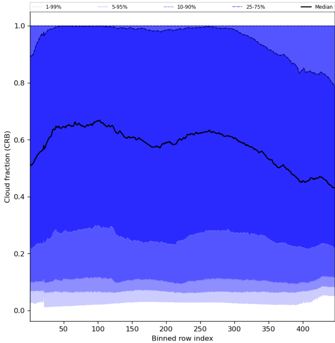
Figure 58: Along track statistics of “Cloud fraction (CRB)” for 2024-07-17 to 2024-07-19
