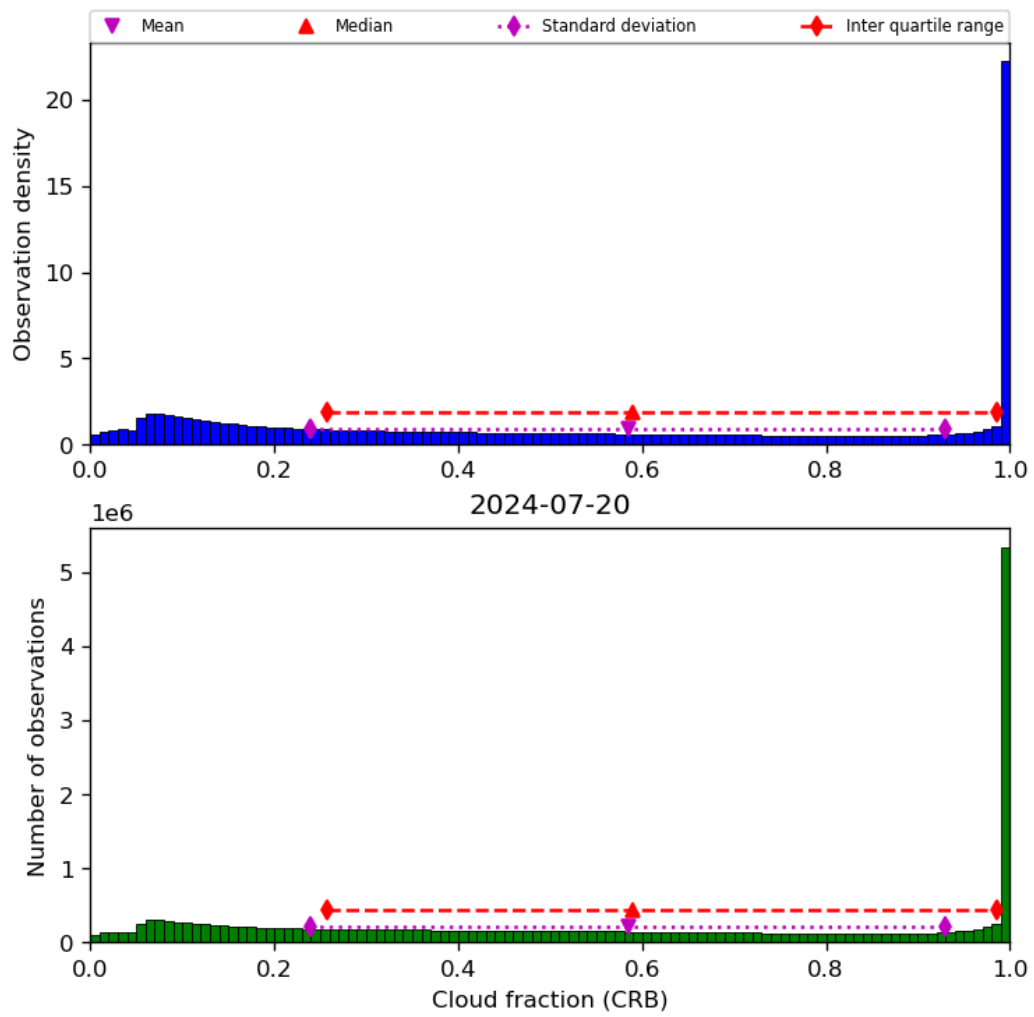
Figure 42: Histogram of “Cloud fraction (CRB)” for 2024-07-19 to 2024-07-21
