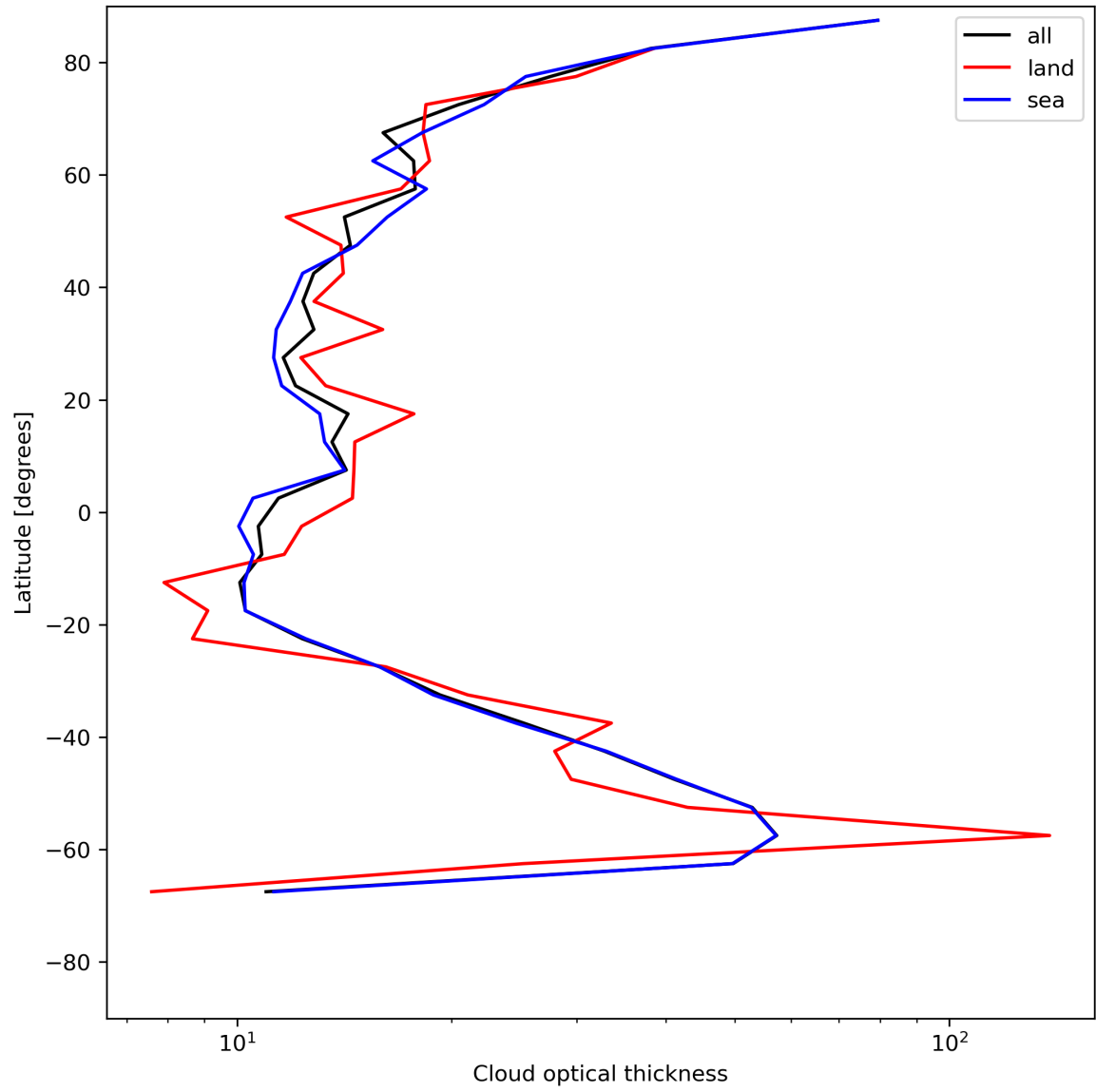
Figure 25: Zonal average of “Cloud optical thickness” for 2024-07-19 to 2024-07-21.
