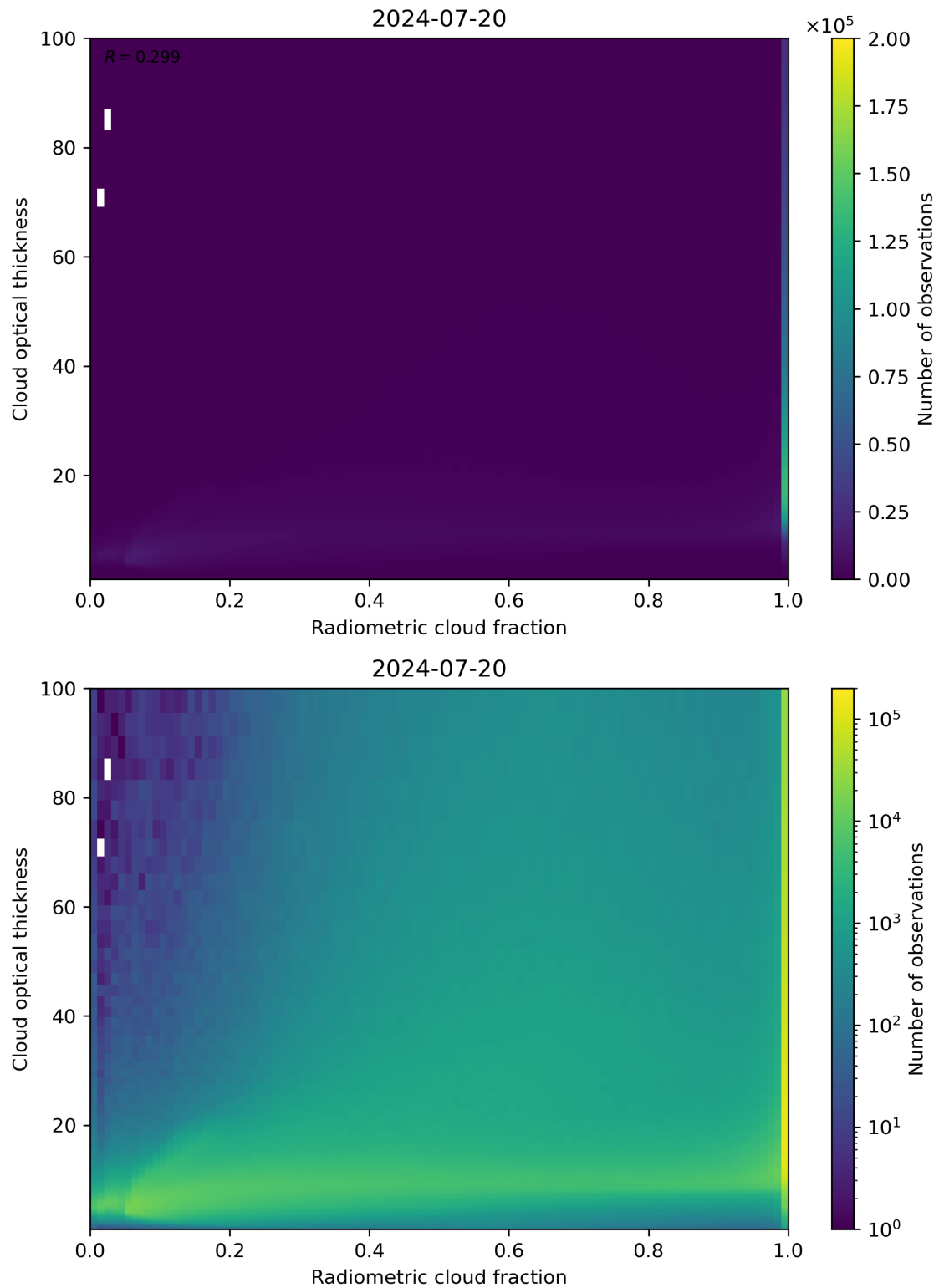
Figure 75: Scatter density plot of “Radiometric cloud fraction” against “Cloud optical thickness” for 2024-07-19 to 2024-07-21.
