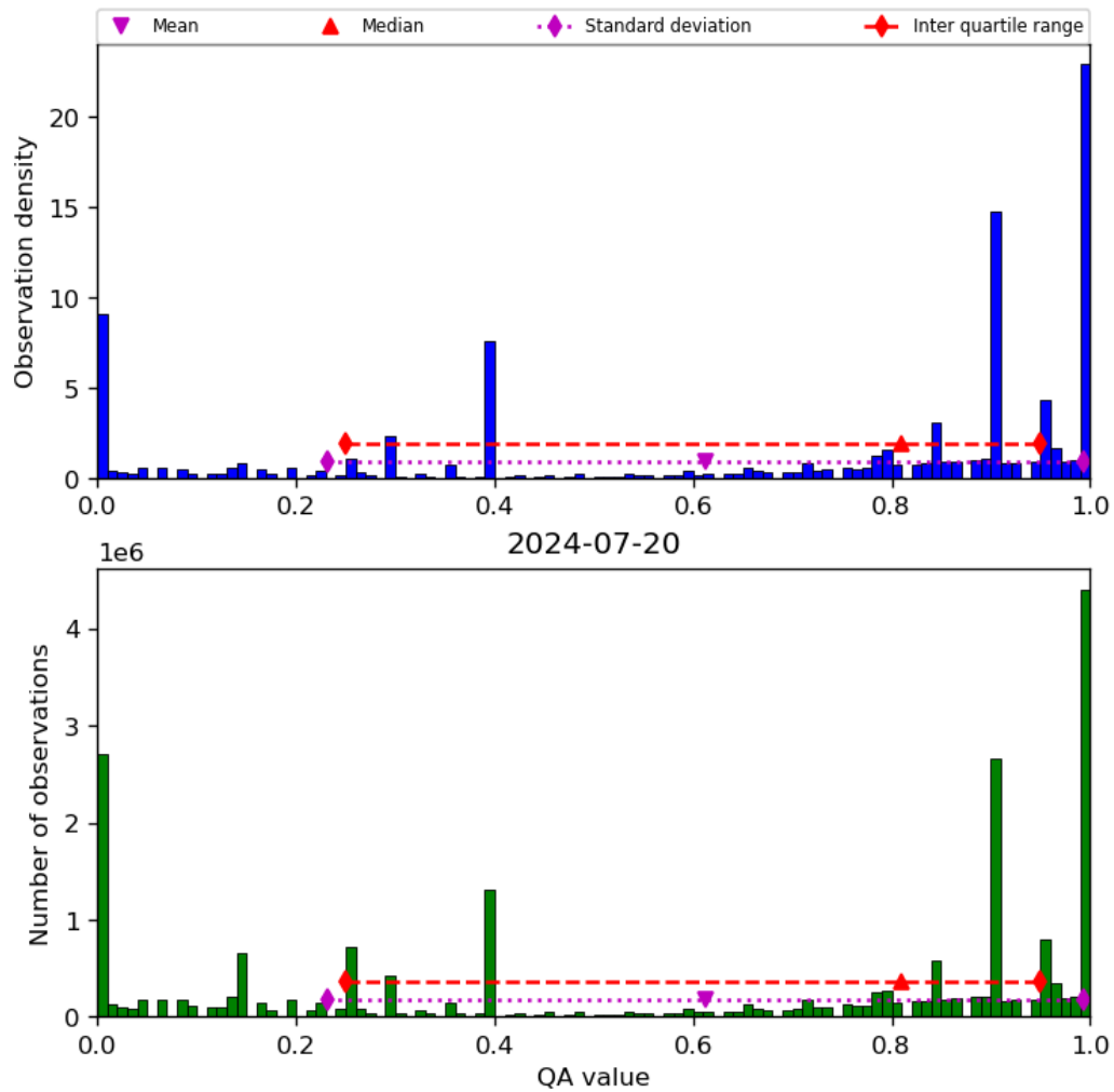
Figure 38: Histogram of “QA value” for 2024-07-19 to 2024-07-21
