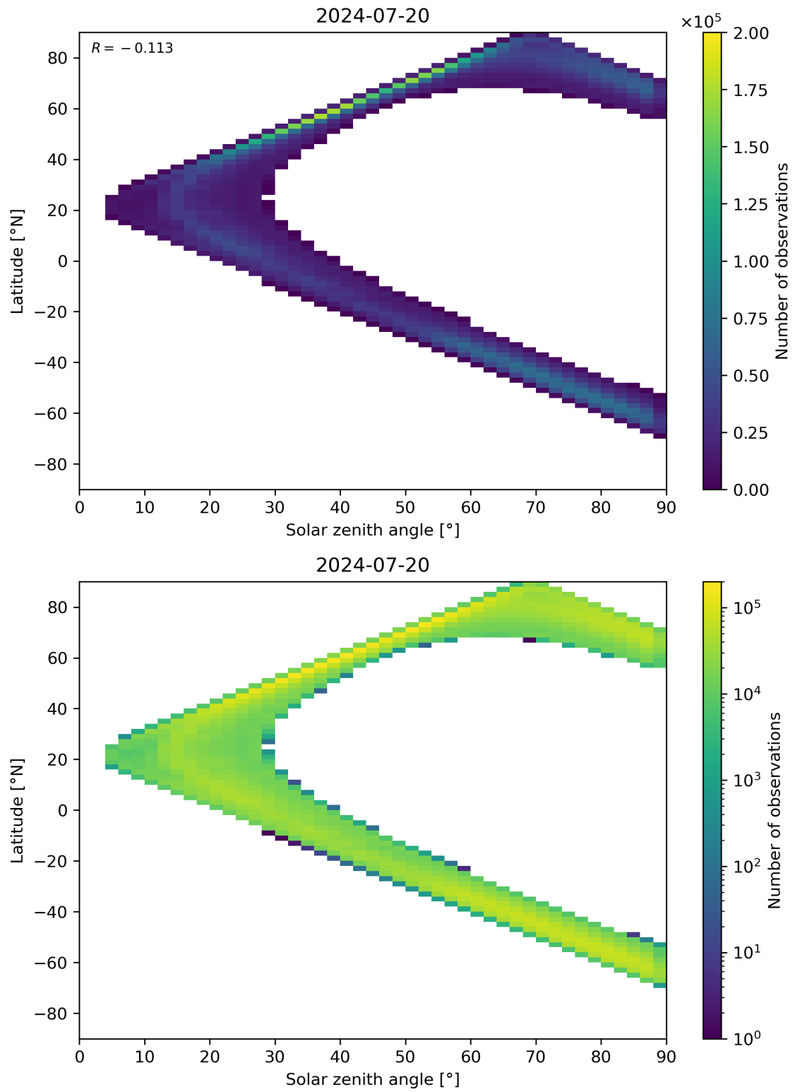
Figure 105: Scatter density plot of “Solar zenith angle” against “Latitude” for 2024-07-19 to 2024-07-21.
