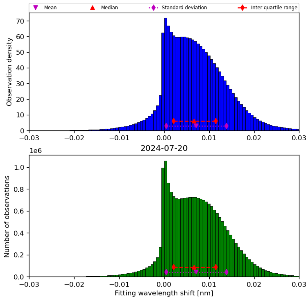
Figure 49: Histogram of “Fitting wavelength shift” for 2024-07-19 to 2024-07-21
