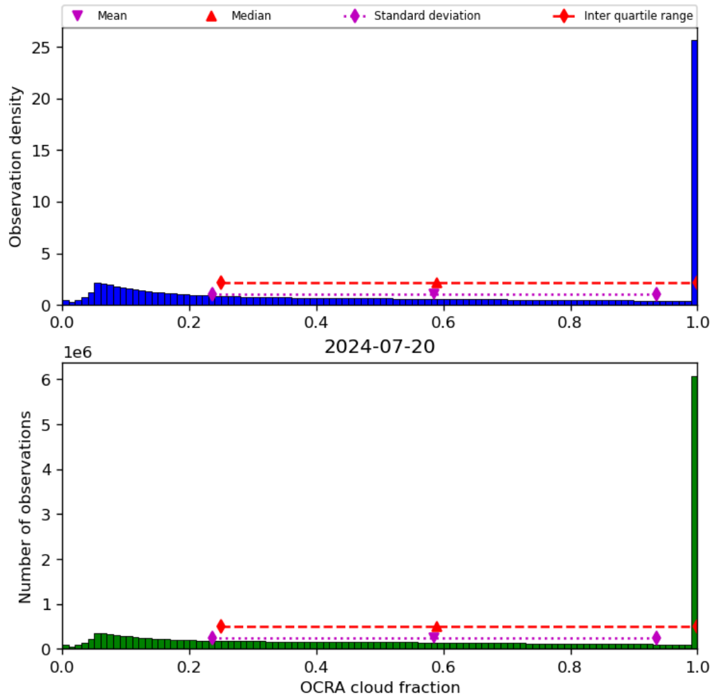
Figure 50: Histogram of “OCRA cloud fraction” for 2024-07-19 to 2024-07-21
