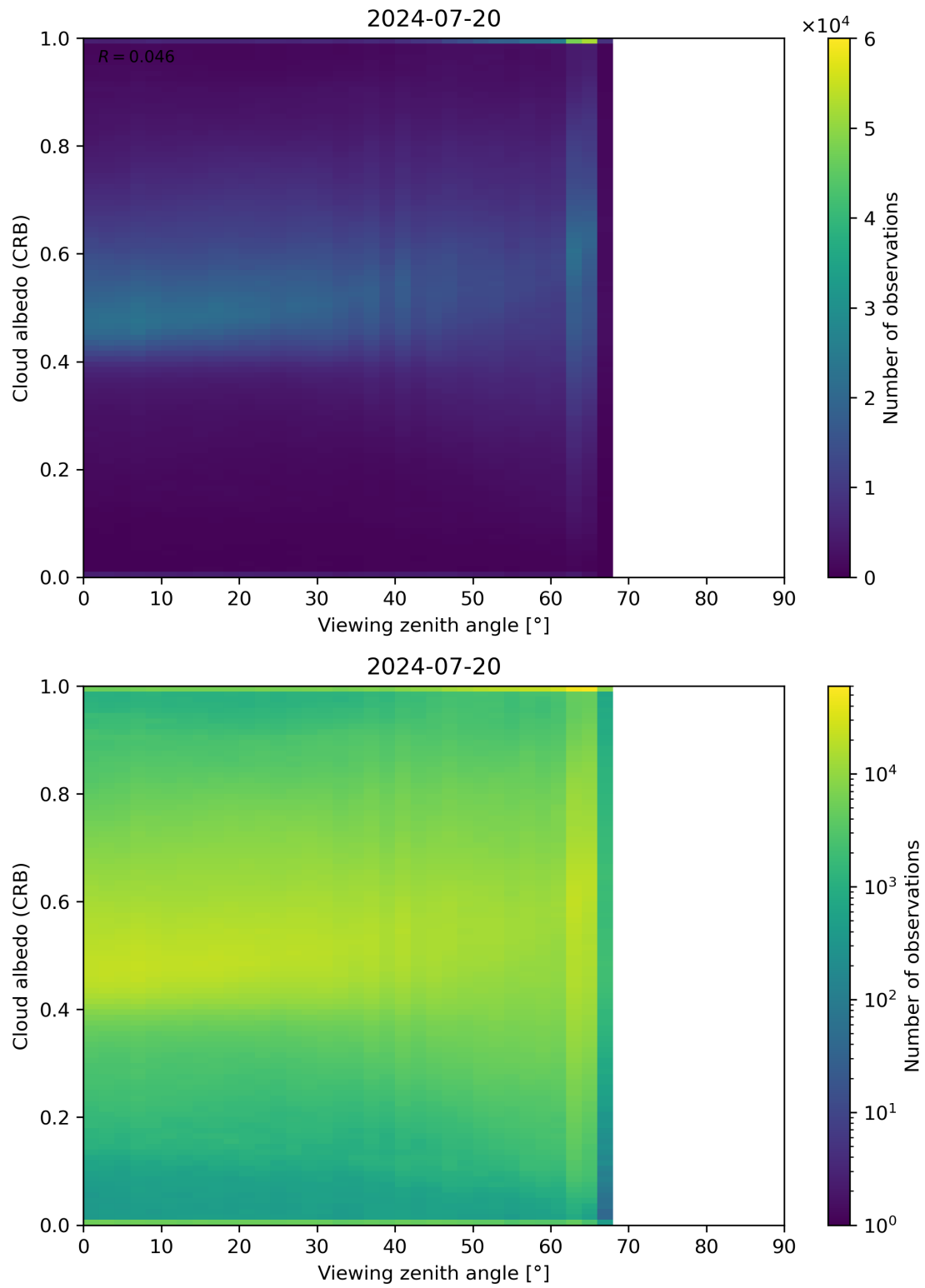
Figure 106: Scatter density plot of “Viewing zenith angle” against “Cloud albedo (CRB)” for 2024-07-19 to 2024-07-21.
