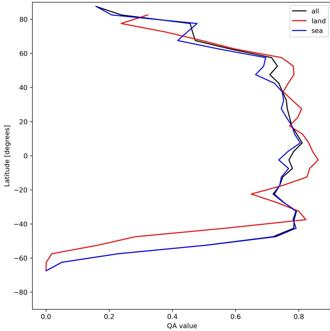
Figure 22: Zonal average of “QA value” for 2024-07-19 to 2024-07-21.
