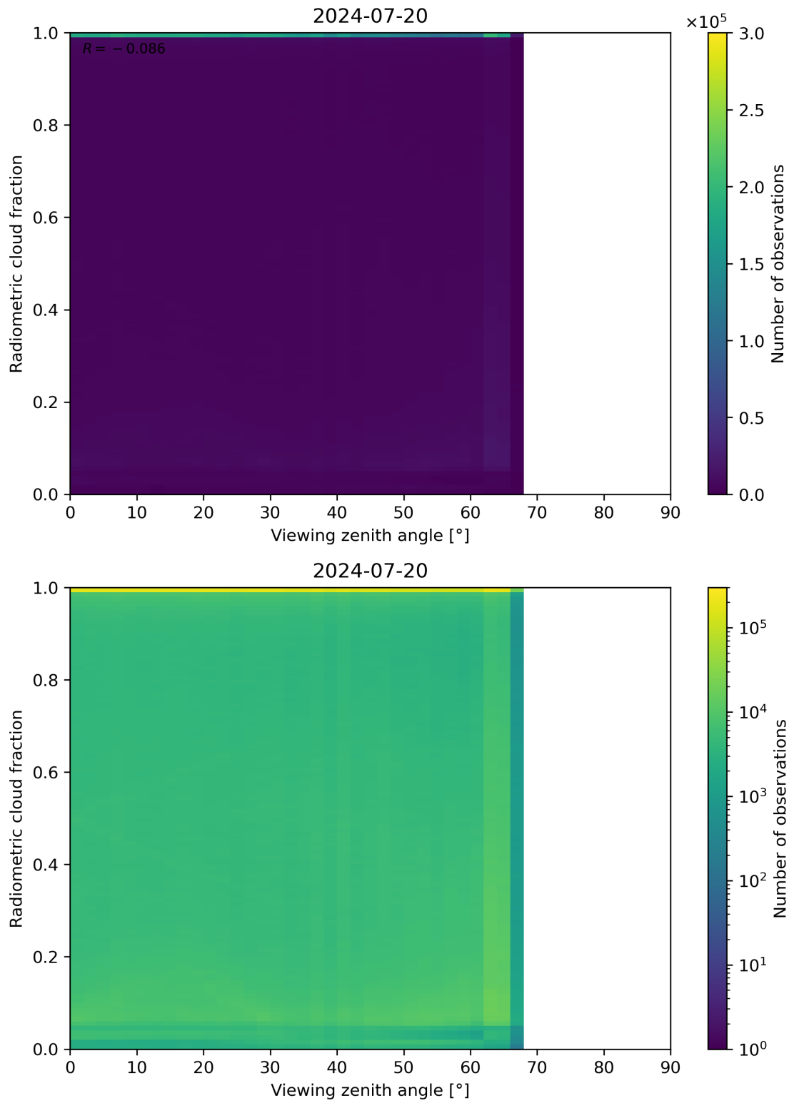
Figure 107: Scatter density plot of “Viewing zenith angle” against “Radiometric cloud fraction” for 2024-07-19 to 2024-07-21.
