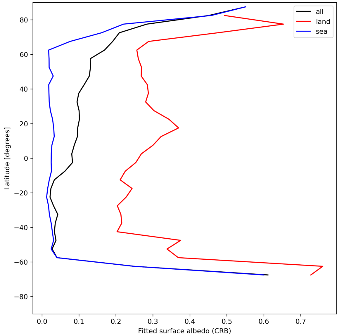
Figure 30: Zonal average of “Fitted surface albedo (CRB)” for 2024-07-19 to 2024-07-21.
