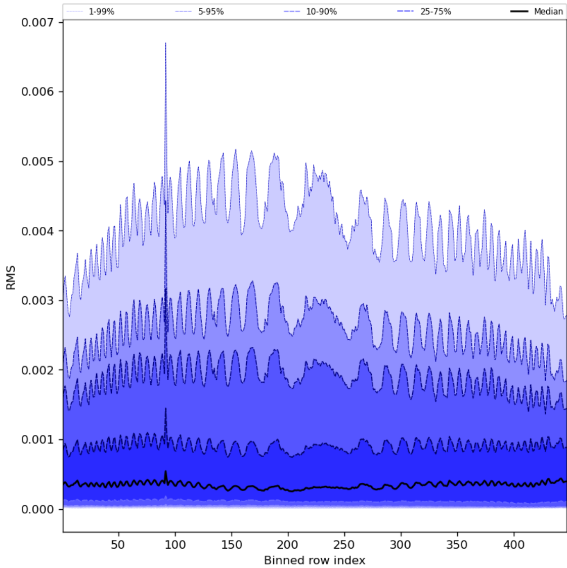
Figure 63: Along track statistics of “RMS” for 2024-07-19 to 2024-07-21
