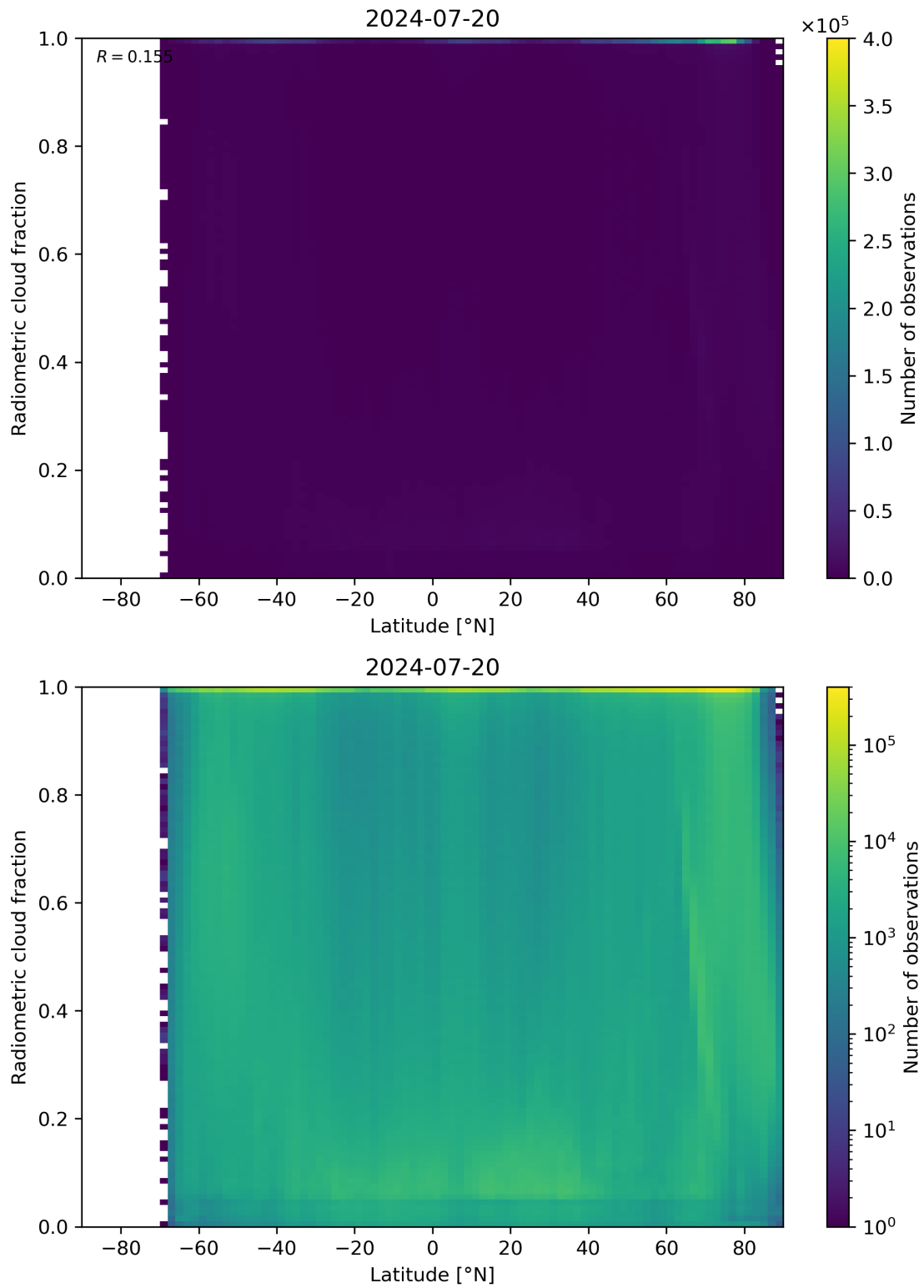
Figure 92: Scatter density plot of “Latitude” against “Radiometric cloud fraction” for 2024-07-19 to 2024-07-21.
