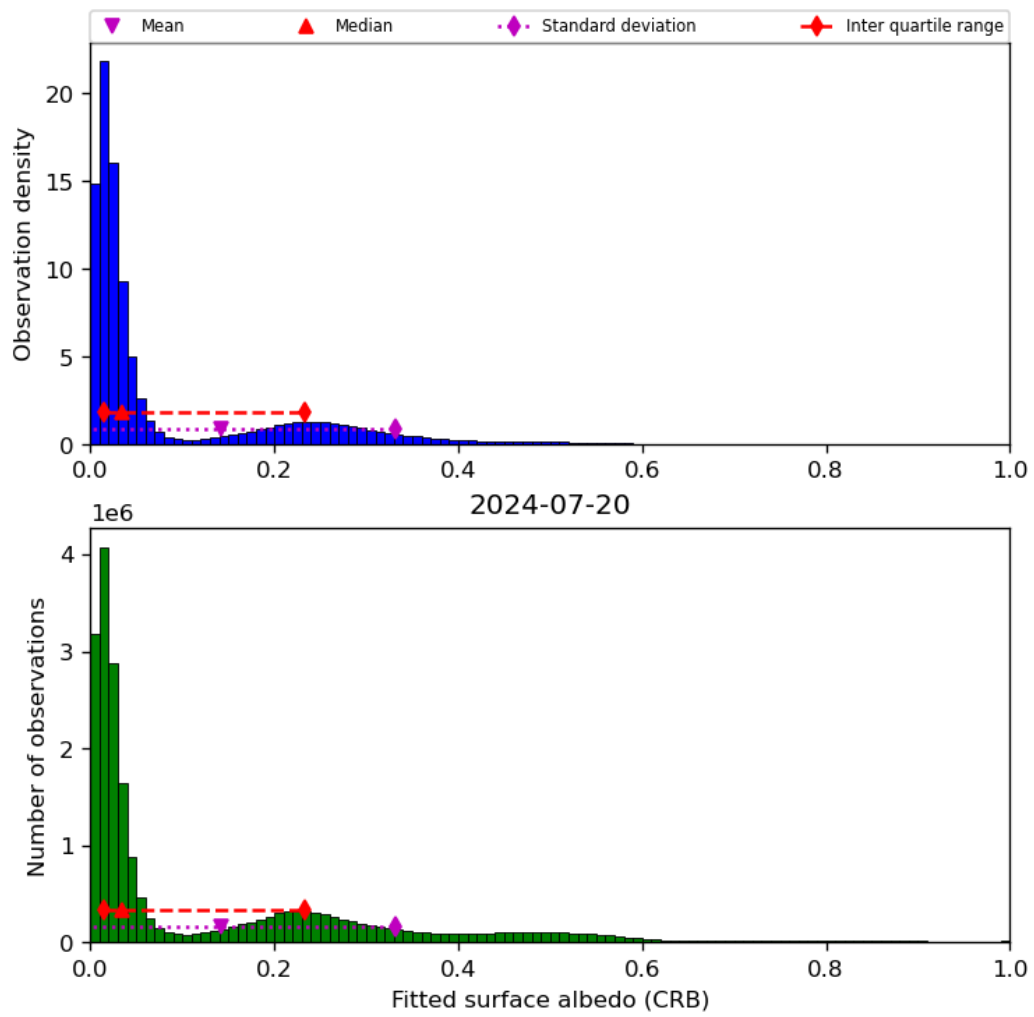
Figure 46: Histogram of “Fitted surface albedo (CRB)” for 2024-07-19 to 2024-07-21
