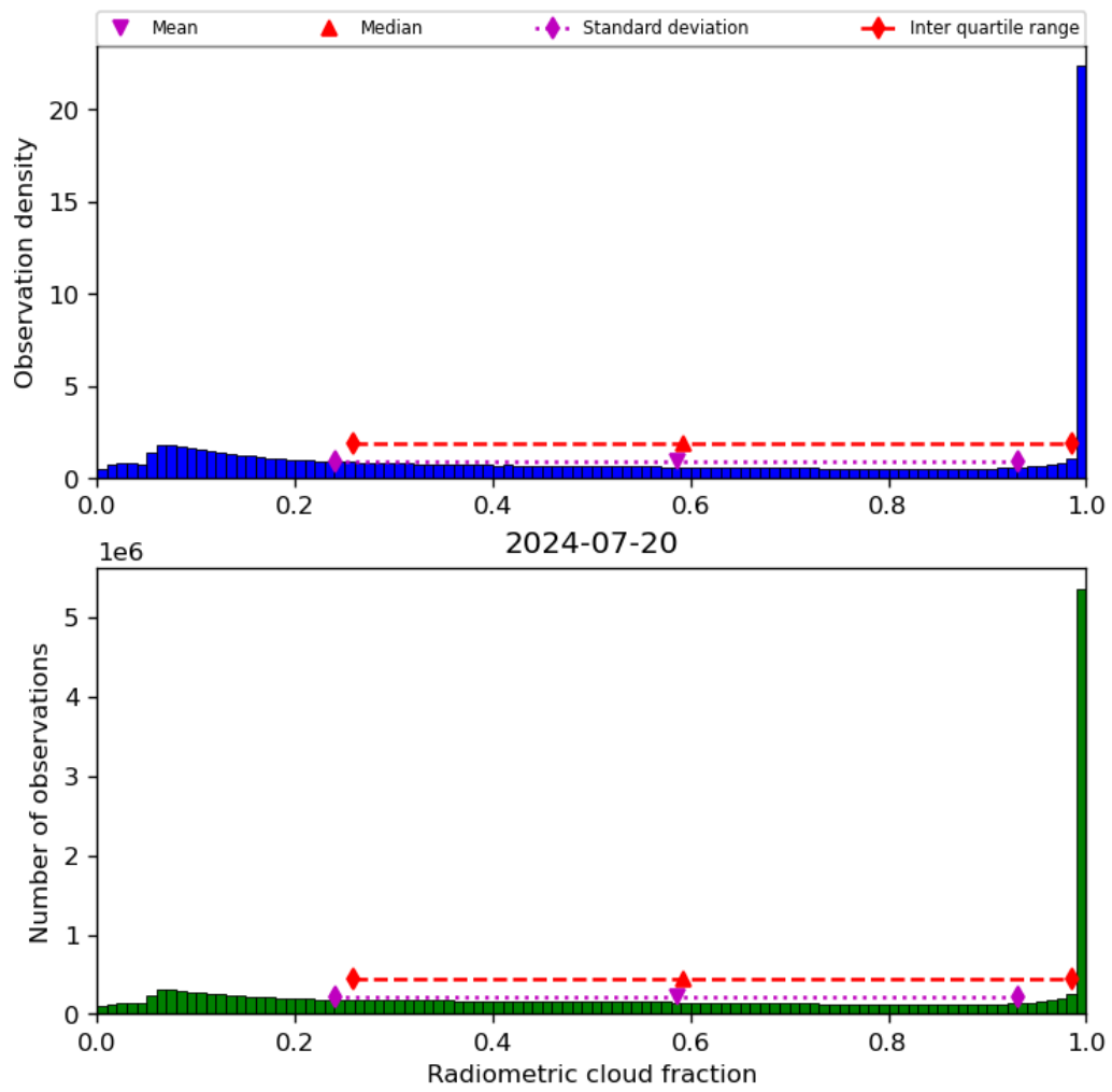
Figure 39: Histogram of “Radiometric cloud fraction” for 2024-07-19 to 2024-07-21
