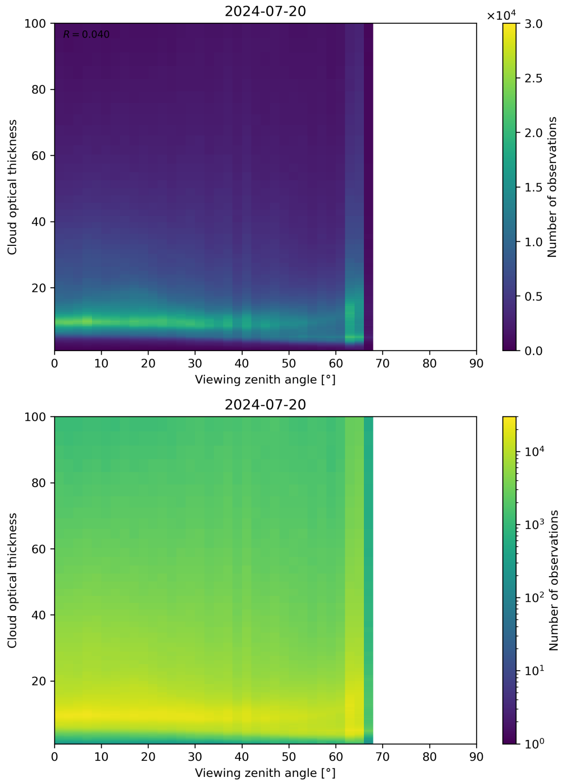
Figure 111: Scatter density plot of “Viewing zenith angle” against “Cloud optical thickness” for 2024-07-19 to 2024-07-21.
