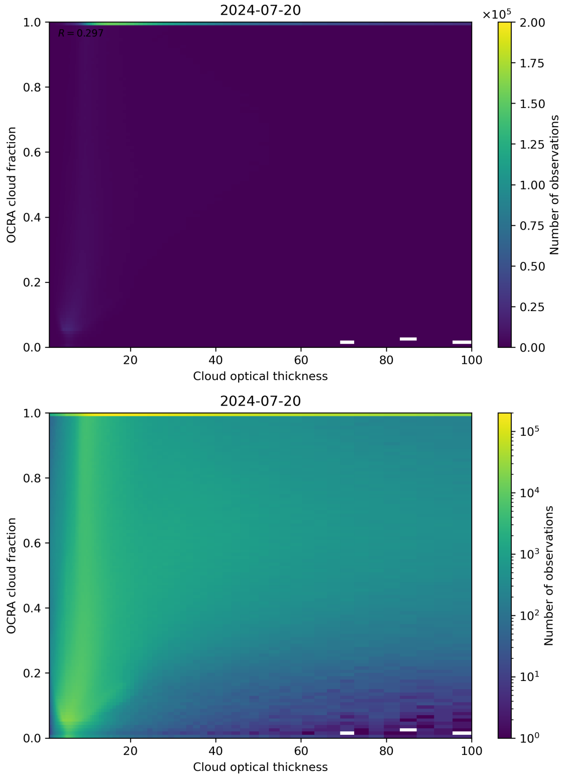
Figure 83: Scatter density plot of “Cloud optical thickness” against “OCRA cloud fraction” for 2024-07-19 to 2024-07-21.
