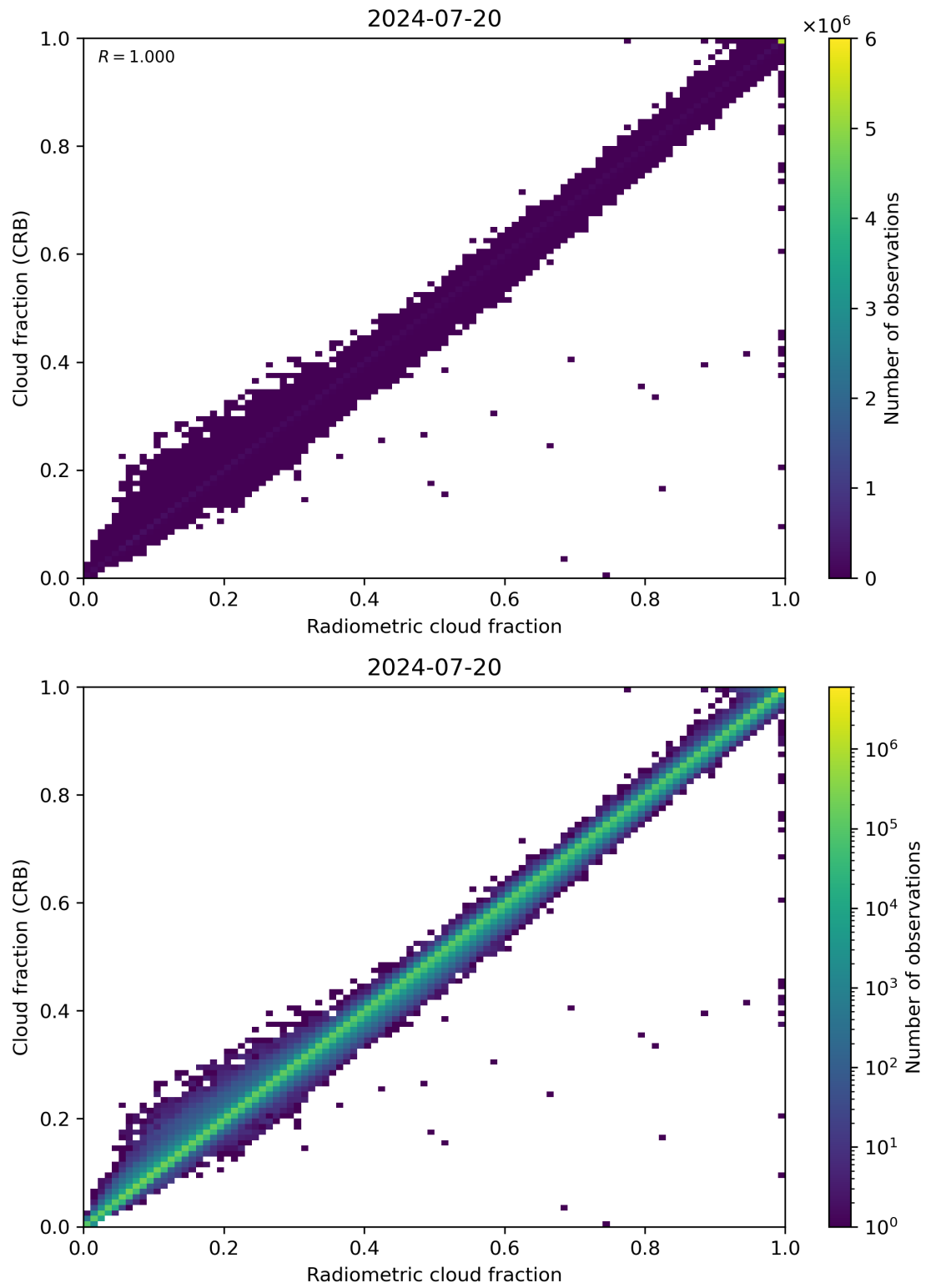
Figure 73: Scatter density plot of “Radiometric cloud fraction” against “Cloud fraction (CRB)” for 2024-07-19 to 2024-07-21.
