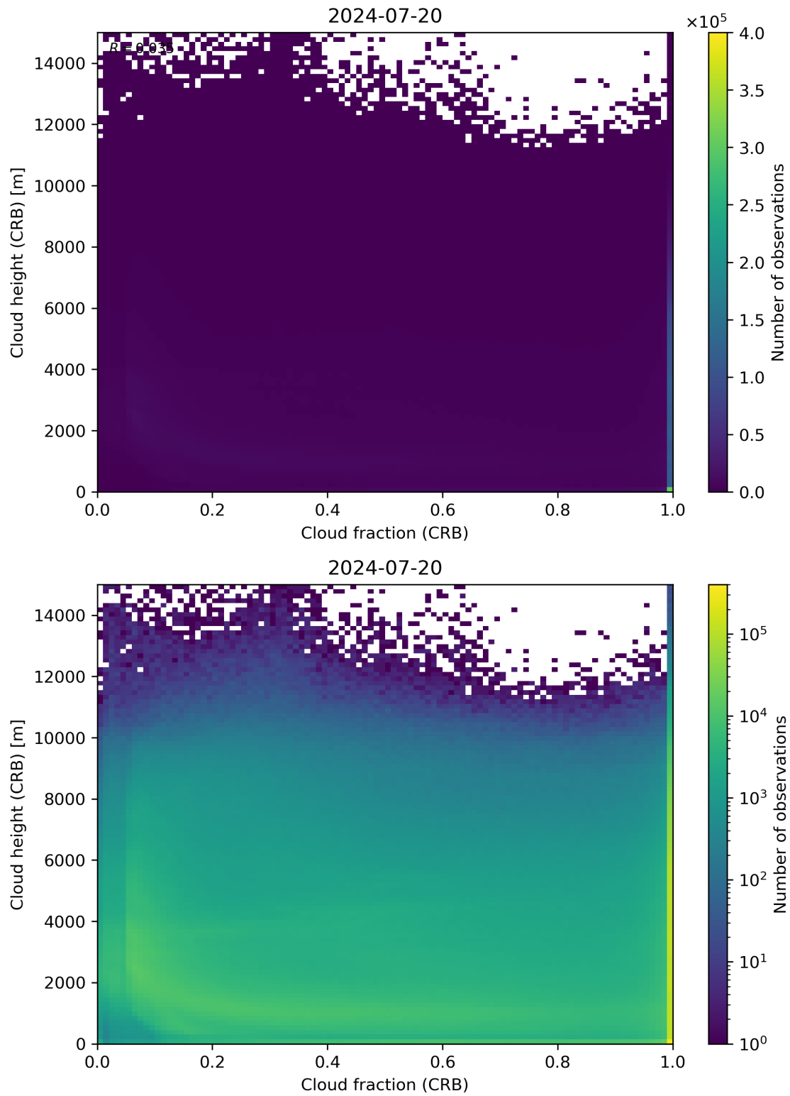
Figure 79: Scatter density plot of “Cloud fraction (CRB)” against “Cloud height (CRB)” for 2024-07-19 to 2024-07-21.
