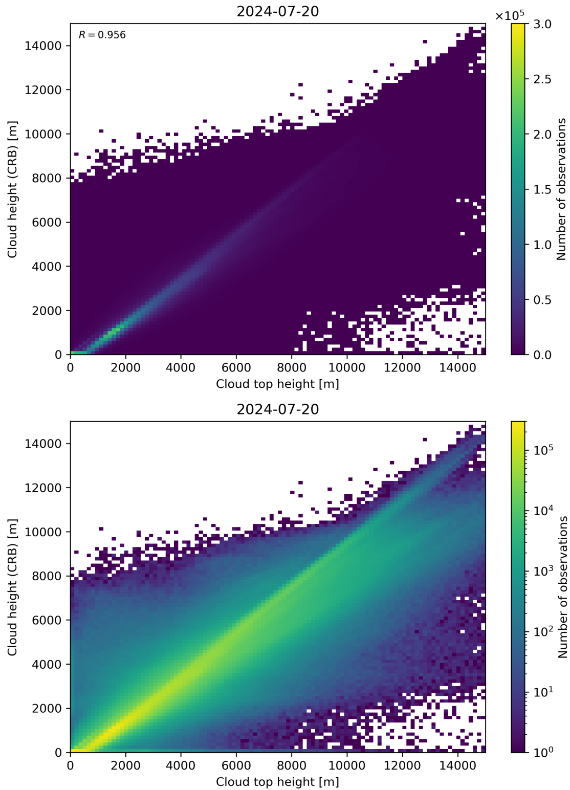
Figure 89: Scatter density plot of “Cloud top height” against “Cloud height (CRB)” for 2024-07-19 to 2024-07-21.
