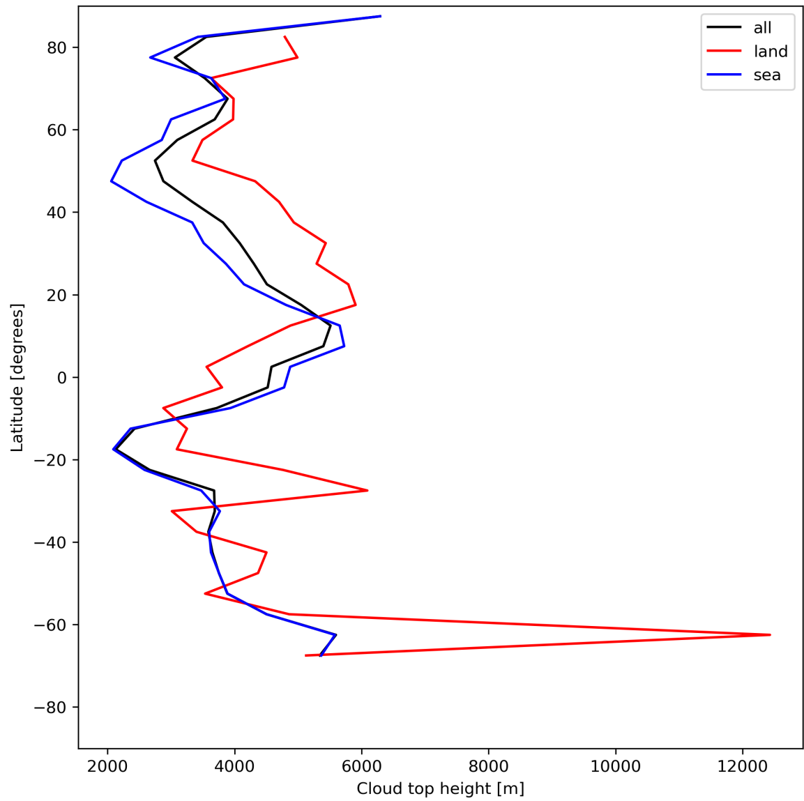
Figure 24: Zonal average of “Cloud top height” for 2024-07-19 to 2024-07-21.
