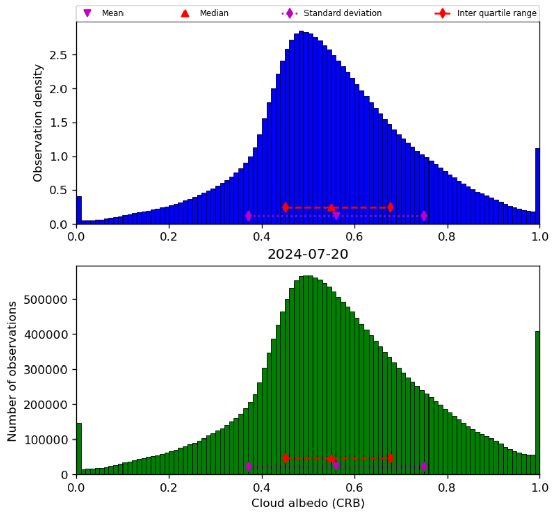
Figure 44: Histogram of “Cloud albedo (CRB)” for 2024-07-19 to 2024-07-21
