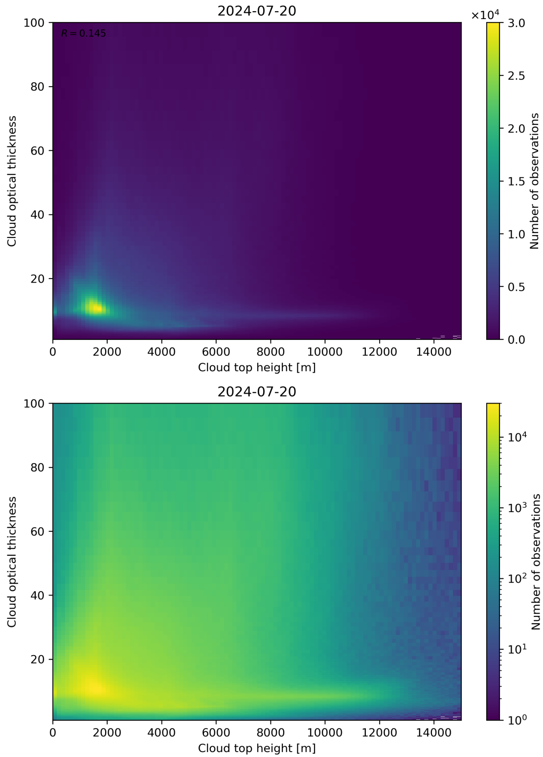
Figure 90: Scatter density plot of “Cloud top height” against “Cloud optical thickness” for 2024-07-19 to 2024-07-21.
