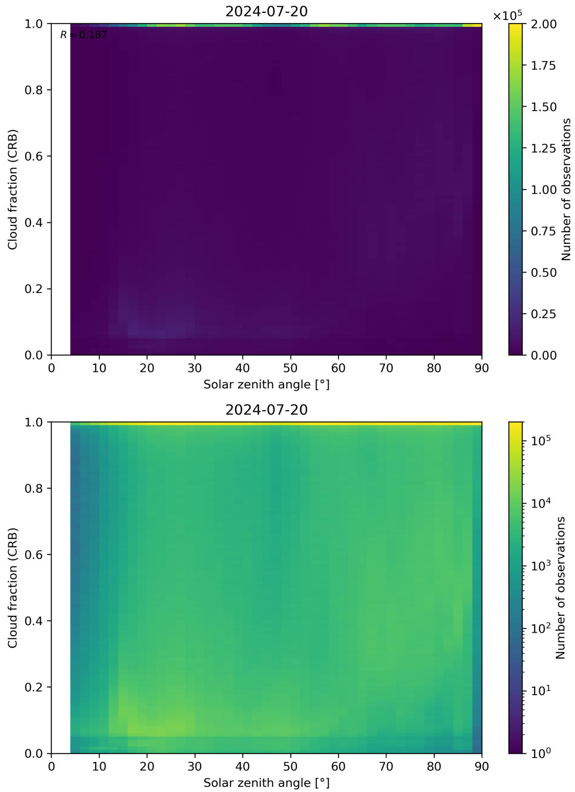
Figure 101: Scatter density plot of “Solar zenith angle” against “Cloud fraction (CRB)” for 2024-07-19 to 2024-07-21.
