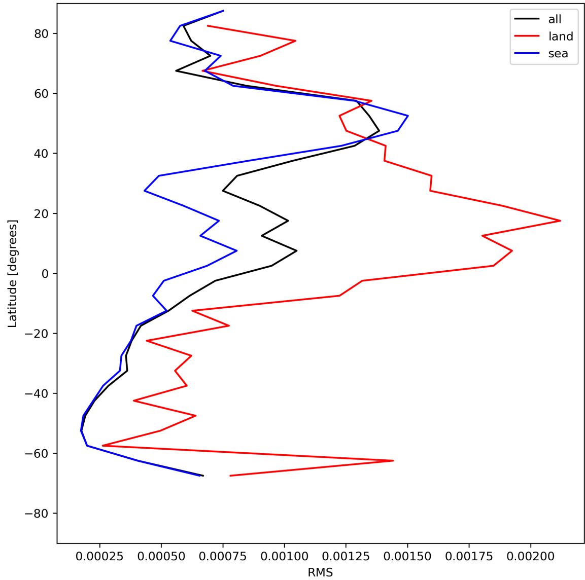
Figure 31: Zonal average of “RMS” for 2024-07-19 to 2024-07-21.
