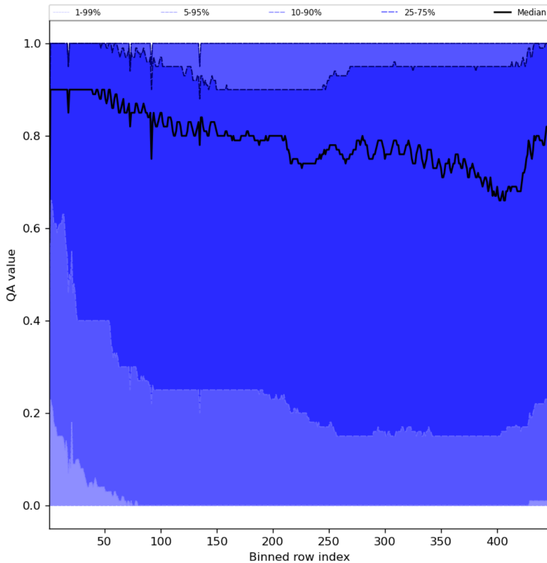
Figure 54: Along track statistics of “QA value” for 2024-07-19 to 2024-07-21
