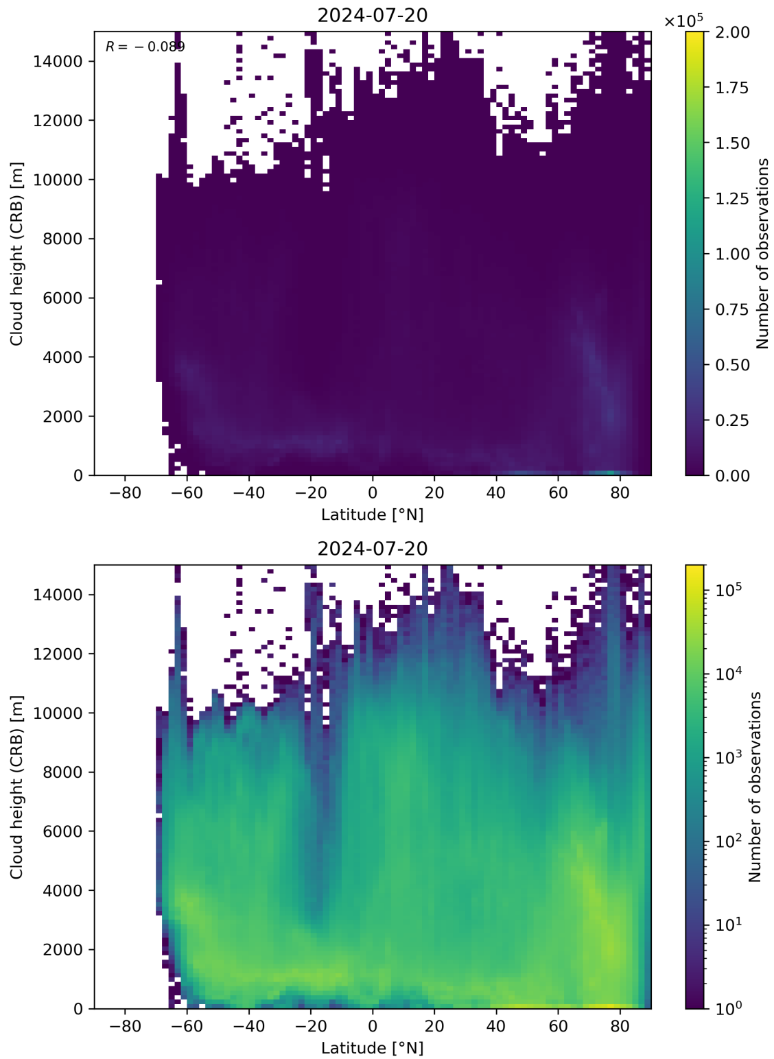
Figure 95: Scatter density plot of “Latitude” against “Cloud height (CRB)” for 2024-07-19 to 2024-07-21.
