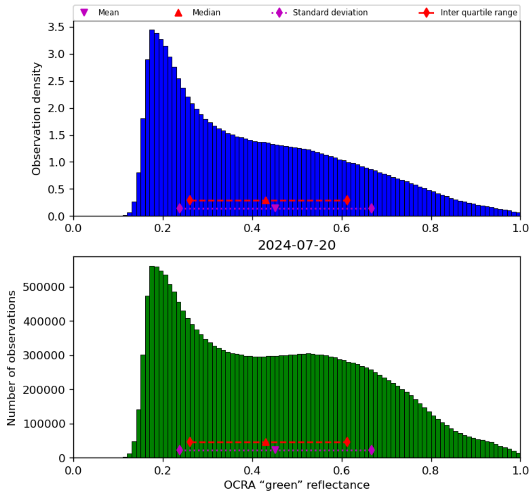
Figure 52: Histogram of “OCRA “green” reflectance” for 2024-07-19 to 2024-07-21
