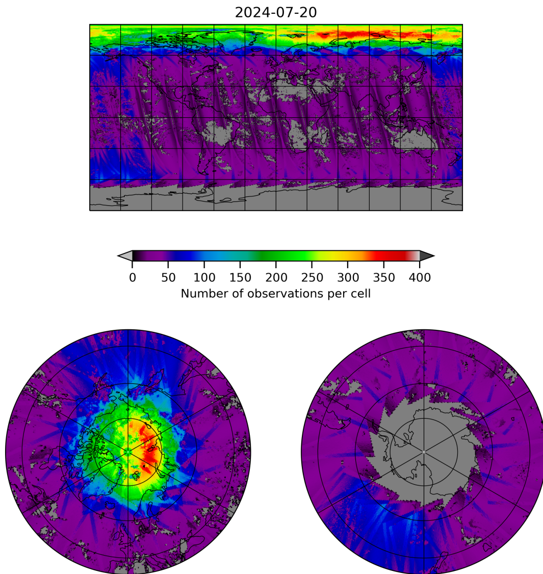
Figure 21: Map of the number of observations for 2024-07-19 to 2024-07-21
