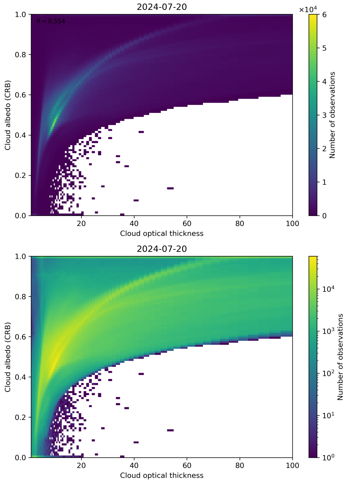
Figure 82: Scatter density plot of “Cloud optical thickness” against “Cloud albedo (CRB)” for 2024-07-19 to 2024-07-21.
