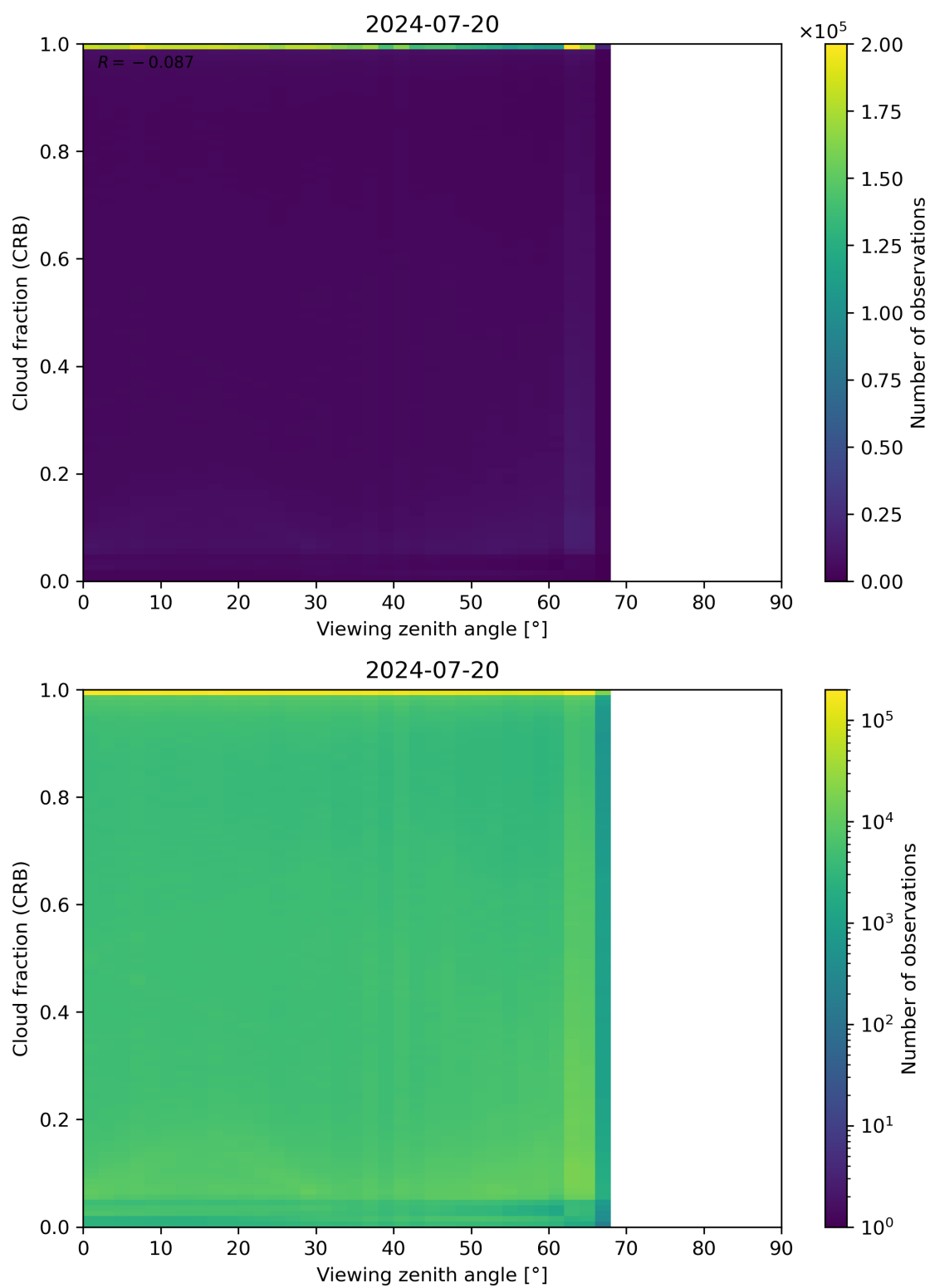
Figure 109: Scatter density plot of “Viewing zenith angle” against “Cloud fraction (CRB)” for 2024-07-19 to 2024-07-21.
