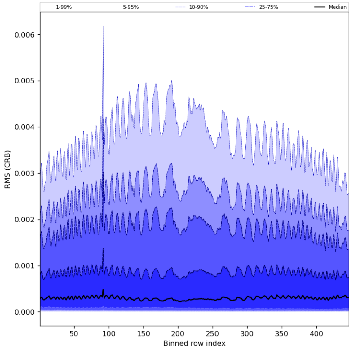
Figure 64: Along track statistics of “RMS (CRB)” for 2024-07-19 to 2024-07-21
