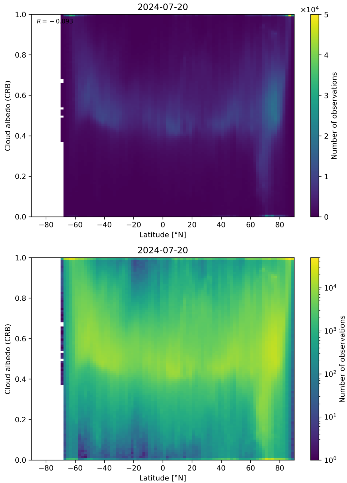
Figure 91: Scatter density plot of “Latitude” against “Cloud albedo (CRB)” for 2024-07-19 to 2024-07-21.
