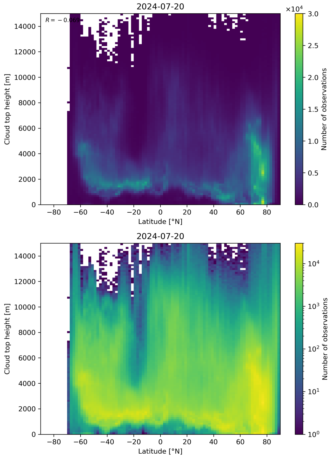
Figure 97: Scatter density plot of “Latitude” against “Cloud top height” for 2024-07-19 to 2024-07-21.
