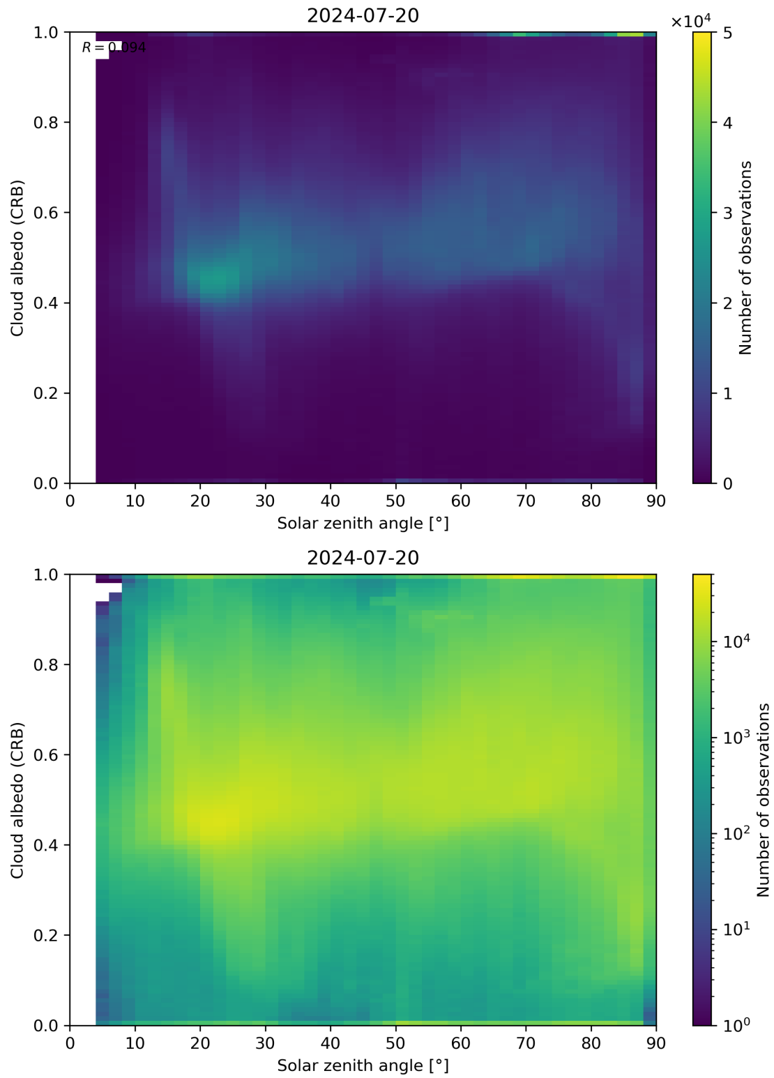
Figure 98: Scatter density plot of “Solar zenith angle” against “Cloud albedo (CRB)” for 2024-07-19 to 2024-07-21.
