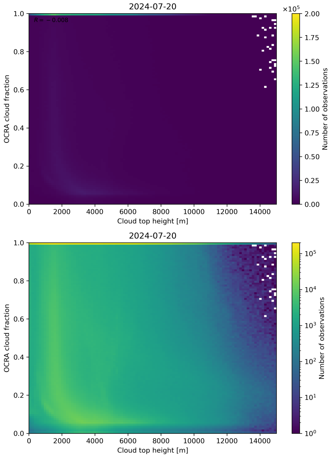
Figure 87: Scatter density plot of “Cloud top height” against “OCRA cloud fraction” for 2024-07-19 to 2024-07-21.
