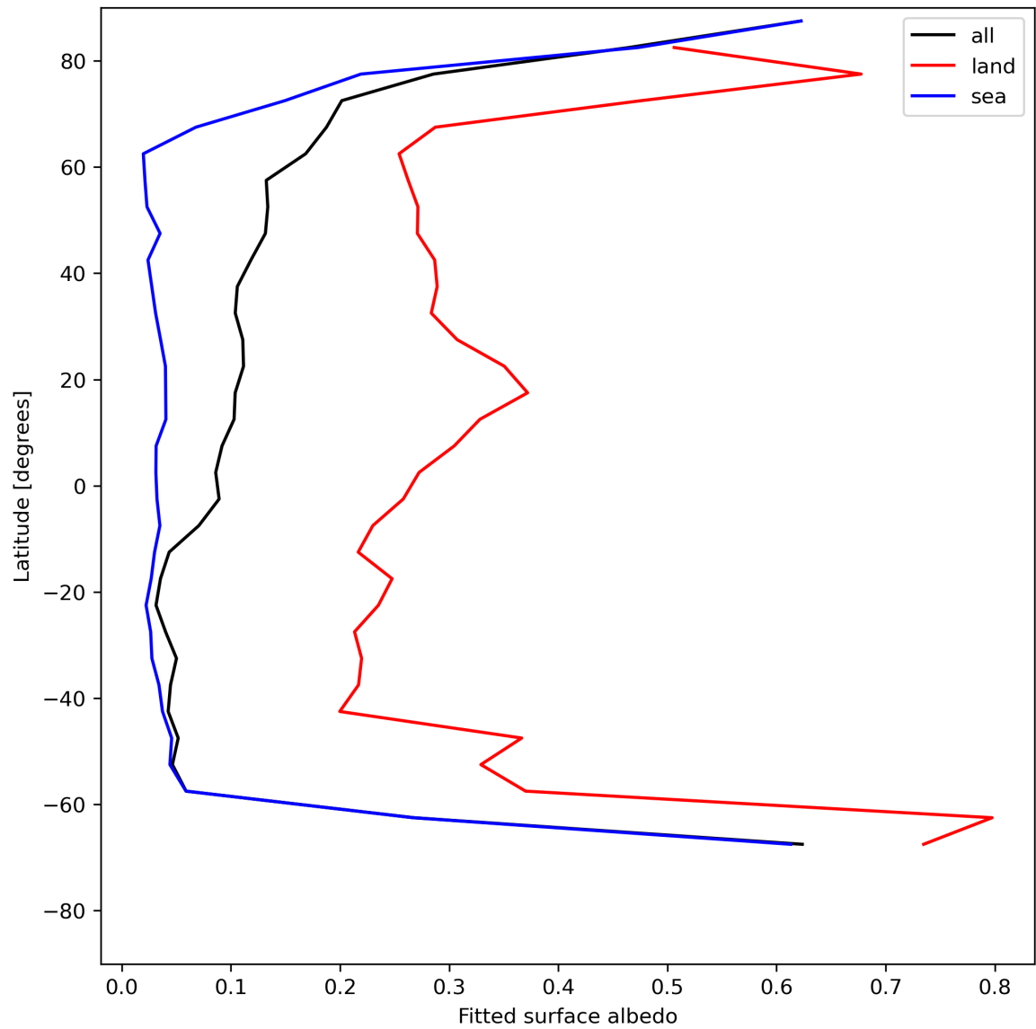
Figure 29: Zonal average of “Fitted surface albedo” for 2024-07-19 to 2024-07-21.
