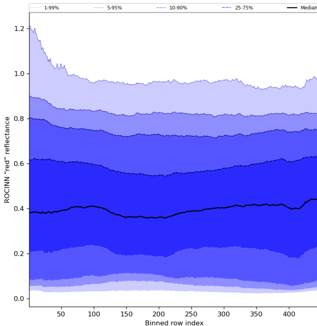
Figure 69: Along track statistics of “ROCINN “red” reflectance” for 2024-07-19 to 2024-07-21
