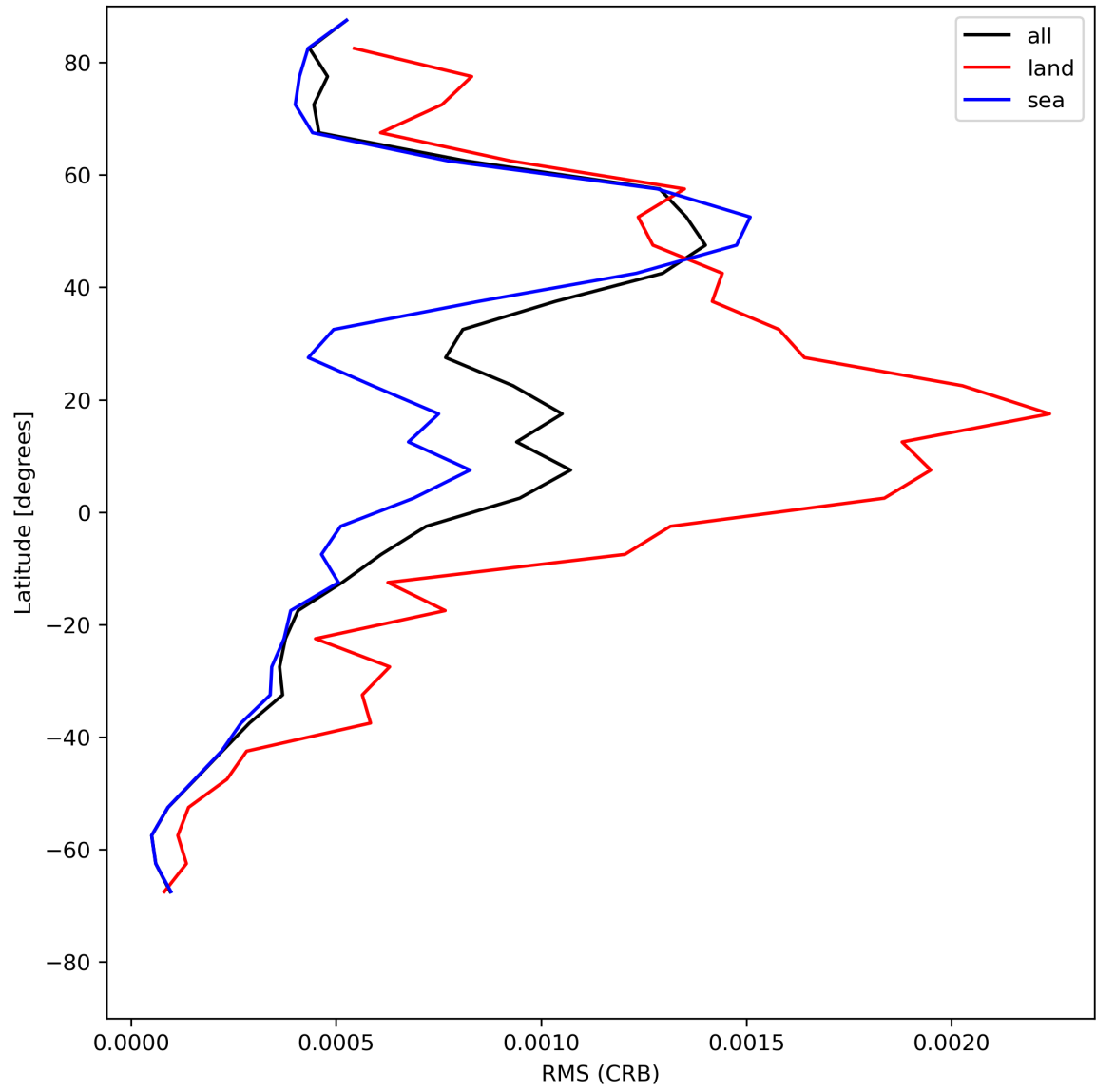
Figure 32: Zonal average of “RMS (CRB)” for 2024-07-19 to 2024-07-21.
