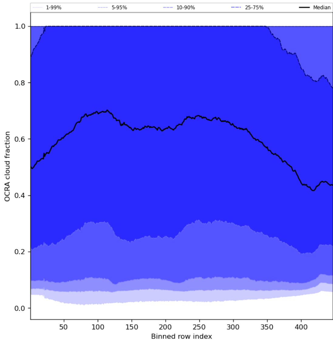
Figure 66: Along track statistics of “OCRA cloud fraction” for 2024-07-19 to 2024-07-21
