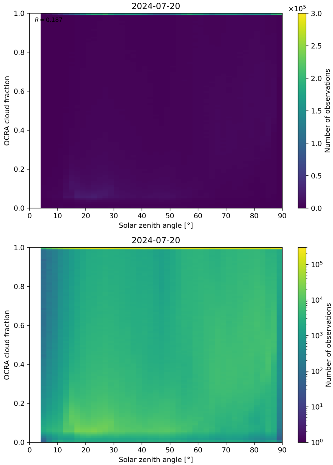
Figure 100: Scatter density plot of “Solar zenith angle” against “OCRA cloud fraction” for 2024-07-19 to 2024-07-21.
