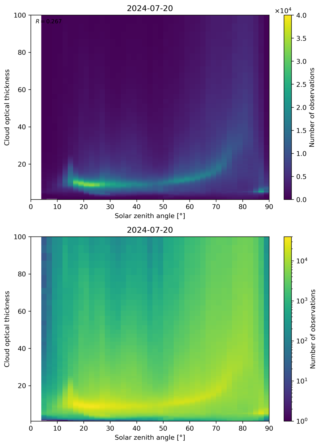
Figure 103: Scatter density plot of “Solar zenith angle” against “Cloud optical thickness” for 2024-07-19 to 2024-07-21.
