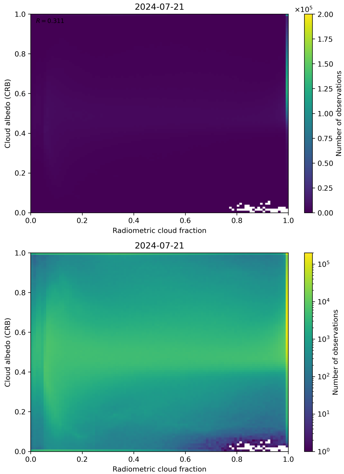
Figure 71: Scatter density plot of “Radiometric cloud fraction” against “Cloud albedo (CRB)” for 2024-07-21 to 2024-07-22.
