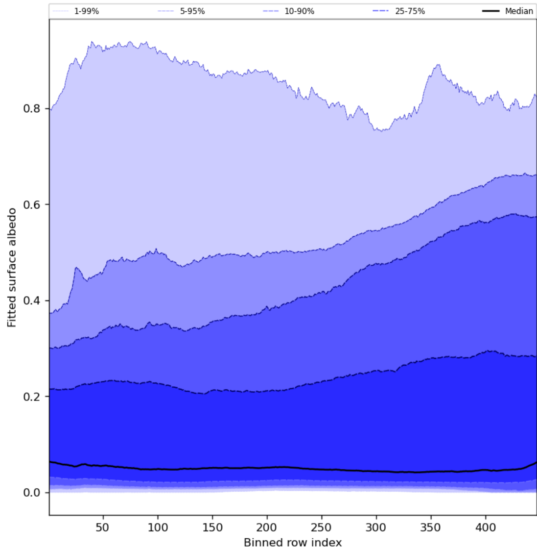
Figure 61: Along track statistics of “Fitted surface albedo” for 2024-07-21 to 2024-07-22
