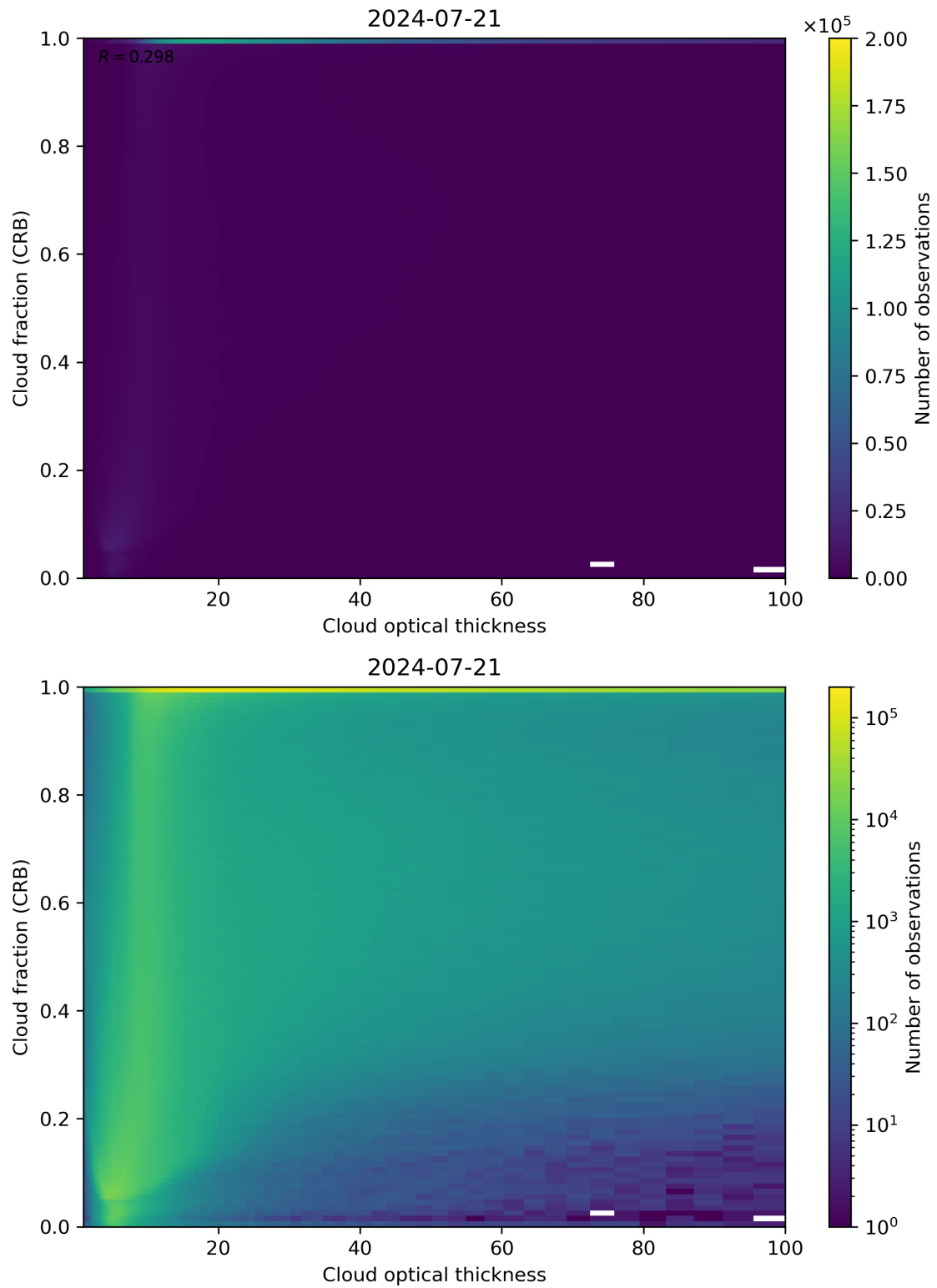
Figure 84: Scatter density plot of “Cloud optical thickness” against “Cloud fraction (CRB)” for 2024-07-21 to 2024-07-22.
