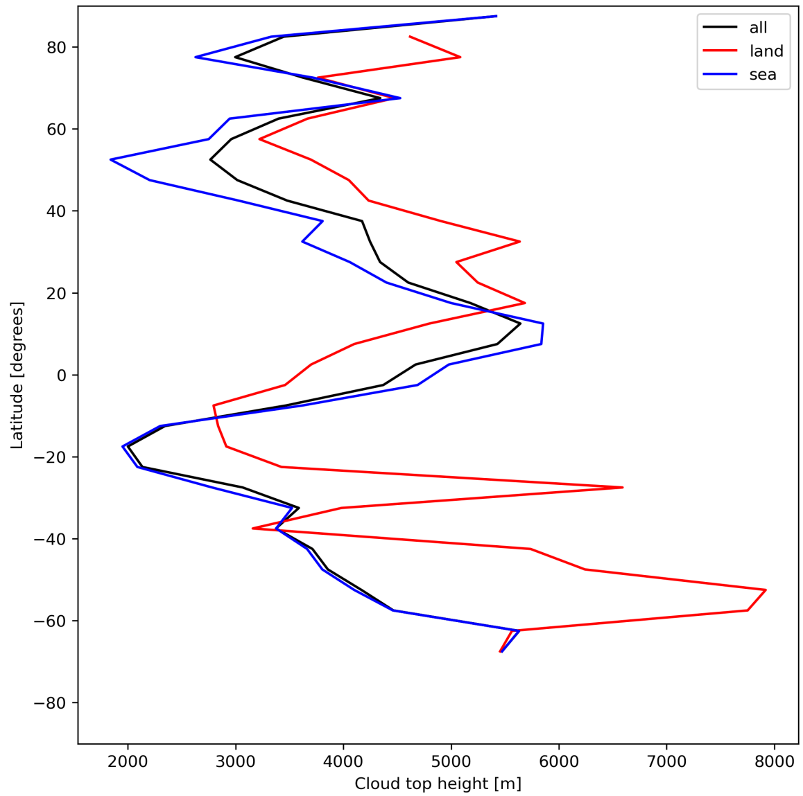
Figure 24: Zonal average of “Cloud top height” for 2024-07-21 to 2024-07-22.
