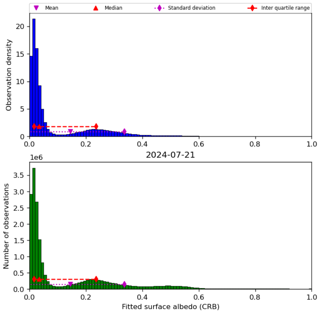
Figure 46: Histogram of “Fitted surface albedo (CRB)” for 2024-07-21 to 2024-07-22
