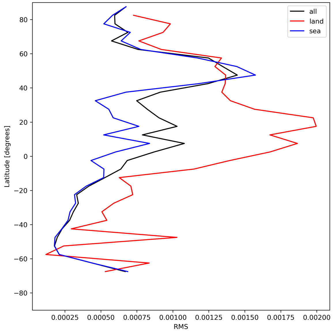
Figure 31: Zonal average of “RMS” for 2024-07-21 to 2024-07-22.
