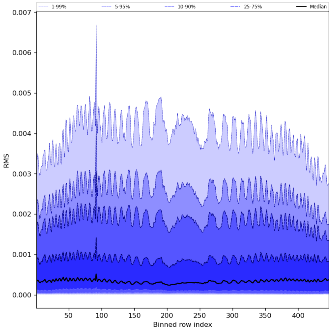
Figure 63: Along track statistics of “RMS” for 2024-07-21 to 2024-07-22
