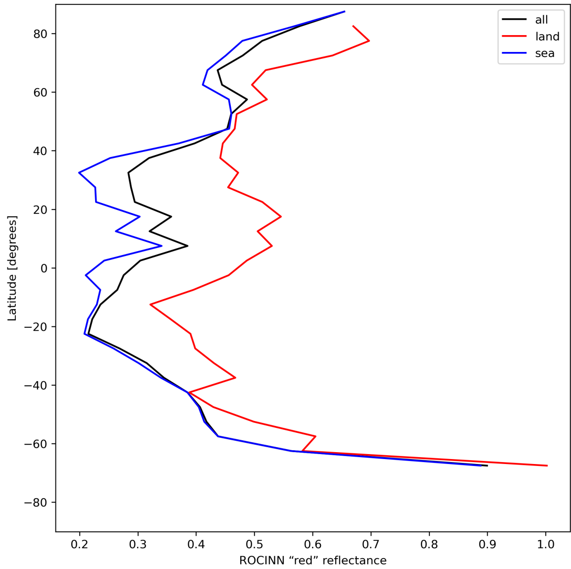
Figure 37: Zonal average of “ROCINN “red” reflectance” for 2024-07-21 to 2024-07-22.
