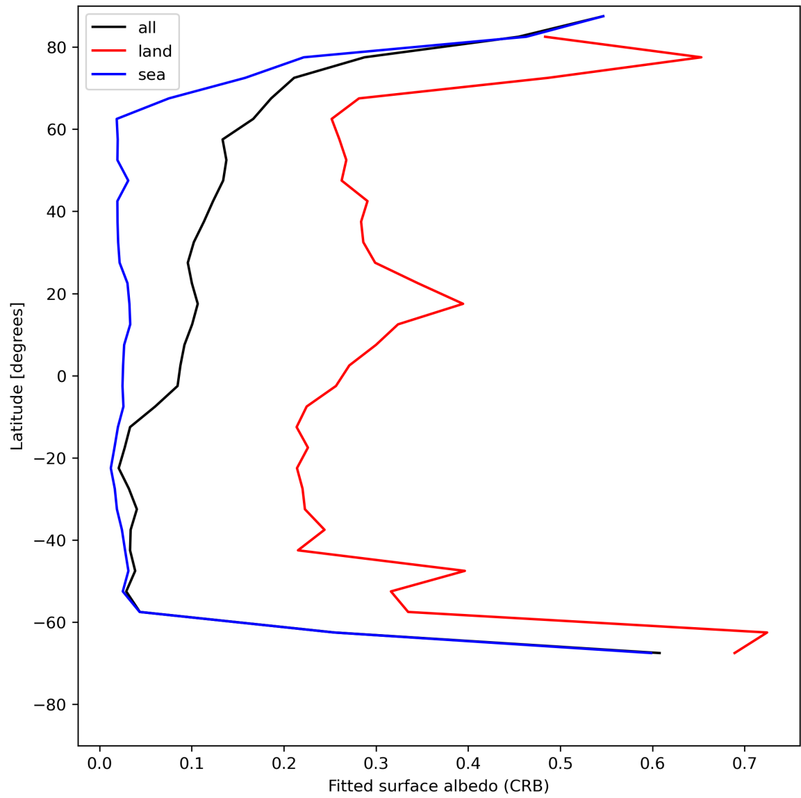
Figure 30: Zonal average of “Fitted surface albedo (CRB)” for 2024-07-21 to 2024-07-22.
