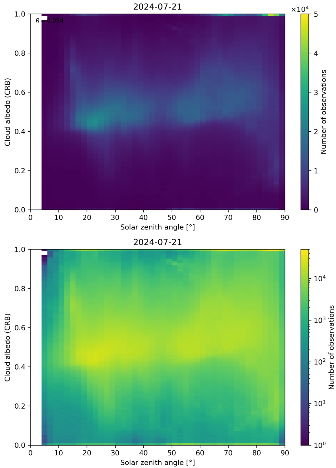
Figure 98: Scatter density plot of “Solar zenith angle” against “Cloud albedo (CRB)” for 2024-07-21 to 2024-07-22.
