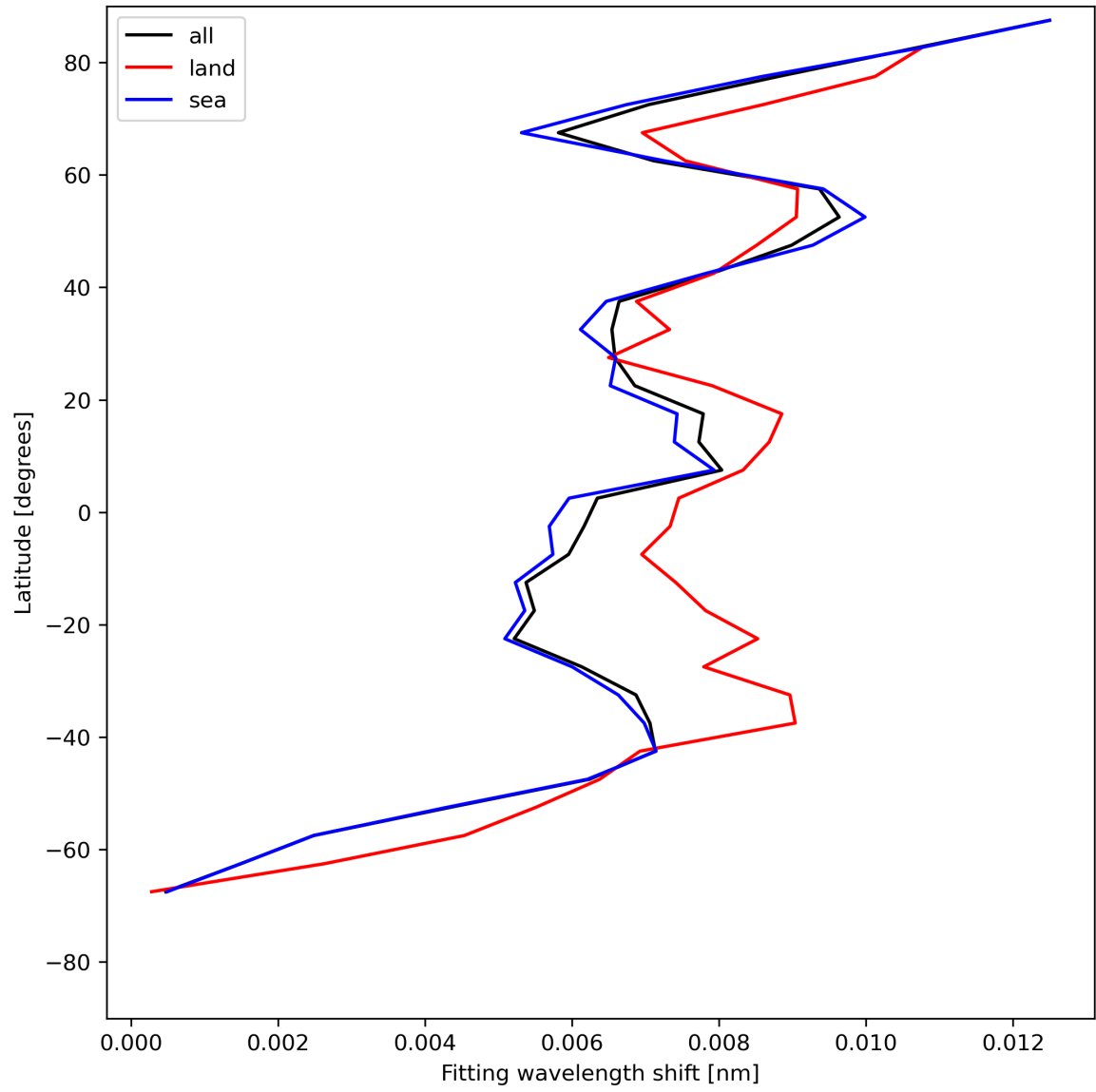
Figure 33: Zonal average of “Fitting wavelength shift” for 2024-07-21 to 2024-07-22.
