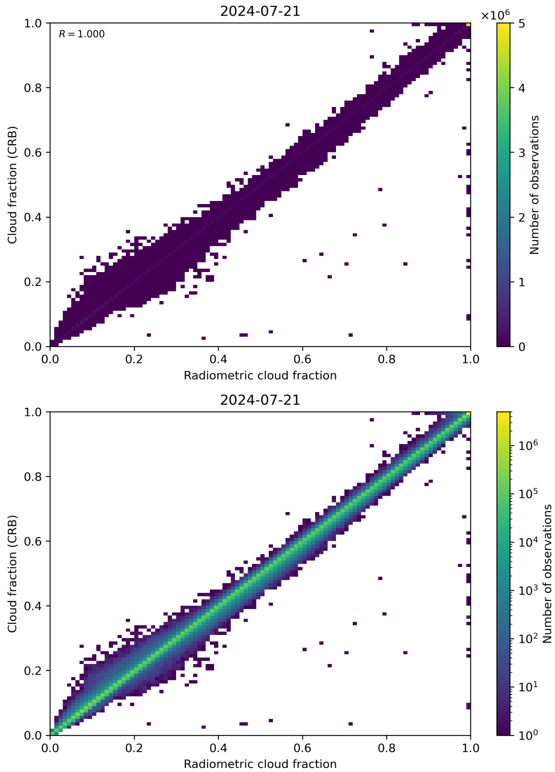
Figure 73: Scatter density plot of “Radiometric cloud fraction” against “Cloud fraction (CRB)” for 2024-07-21 to 2024-07-22.
