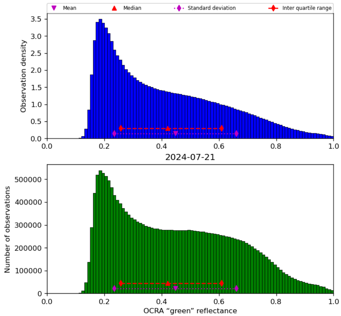
Figure 52: Histogram of “OCRA “green” reflectance” for 2024-07-21 to 2024-07-22
