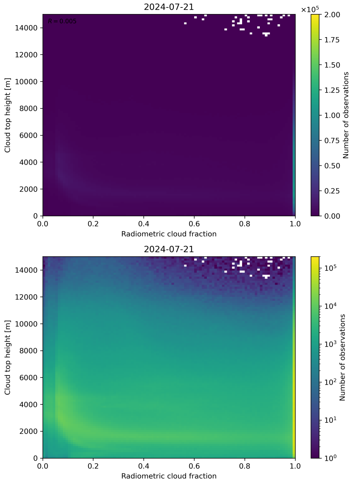
Figure 76: Scatter density plot of “Radiometric cloud fraction” against “Cloud top height” for 2024-07-21 to 2024-07-22.
