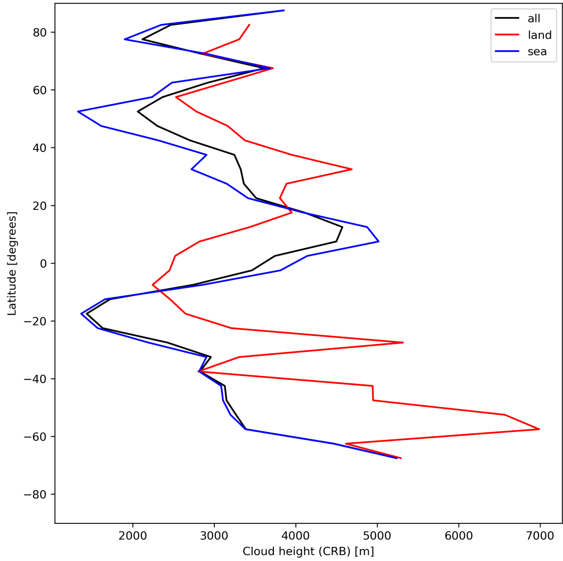
Figure 27: Zonal average of “Cloud height (CRB)” for 2024-07-21 to 2024-07-22.
