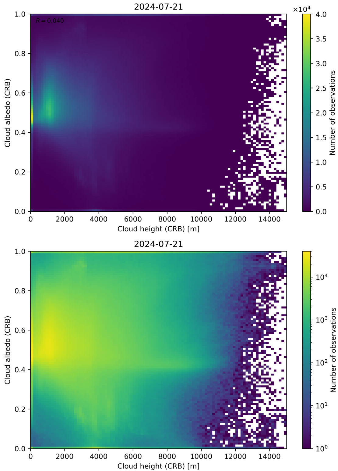
Figure 80: Scatter density plot of “Cloud height (CRB)” against “Cloud albedo (CRB)” for 2024-07-21 to 2024-07-22.
