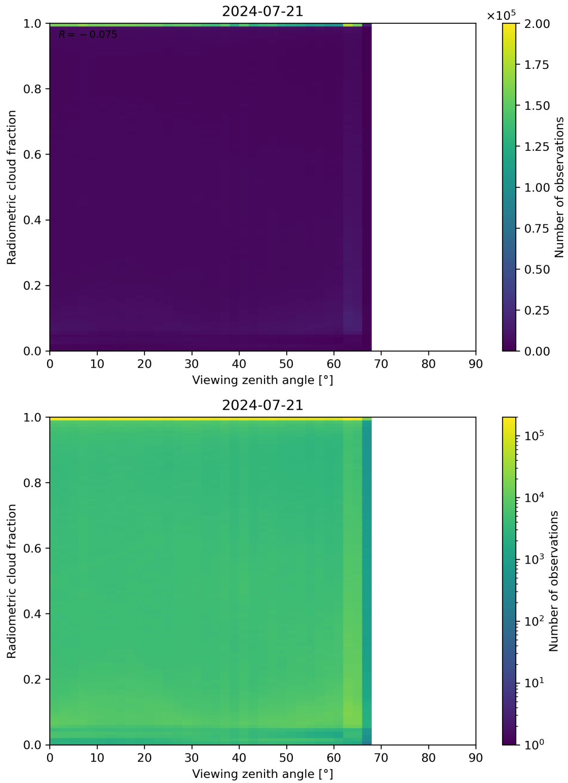
Figure 107: Scatter density plot of “Viewing zenith angle” against “Radiometric cloud fraction” for 2024-07-21 to 2024-07-22.
