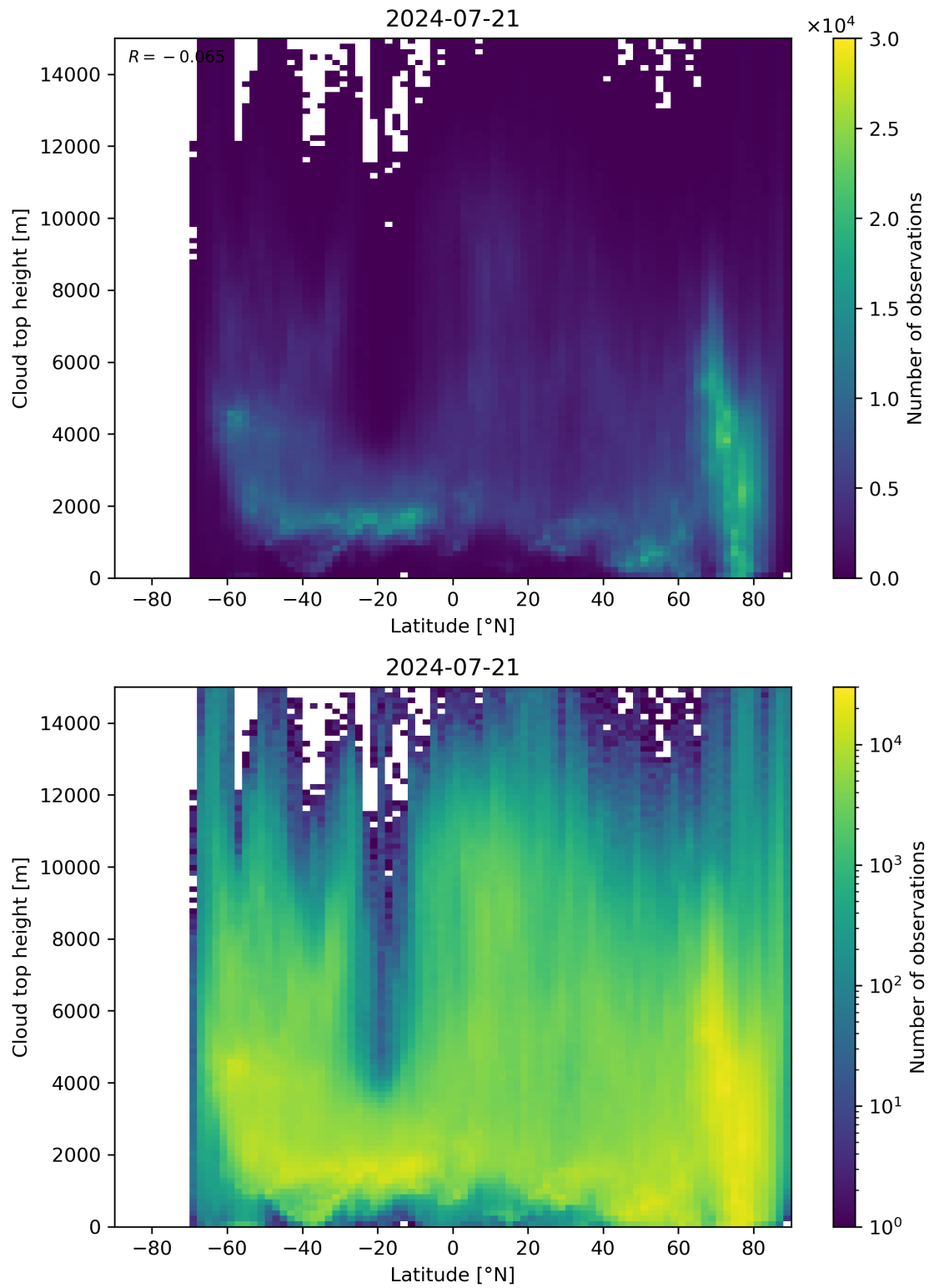
Figure 97: Scatter density plot of “Latitude” against “Cloud top height” for 2024-07-21 to 2024-07-22.
