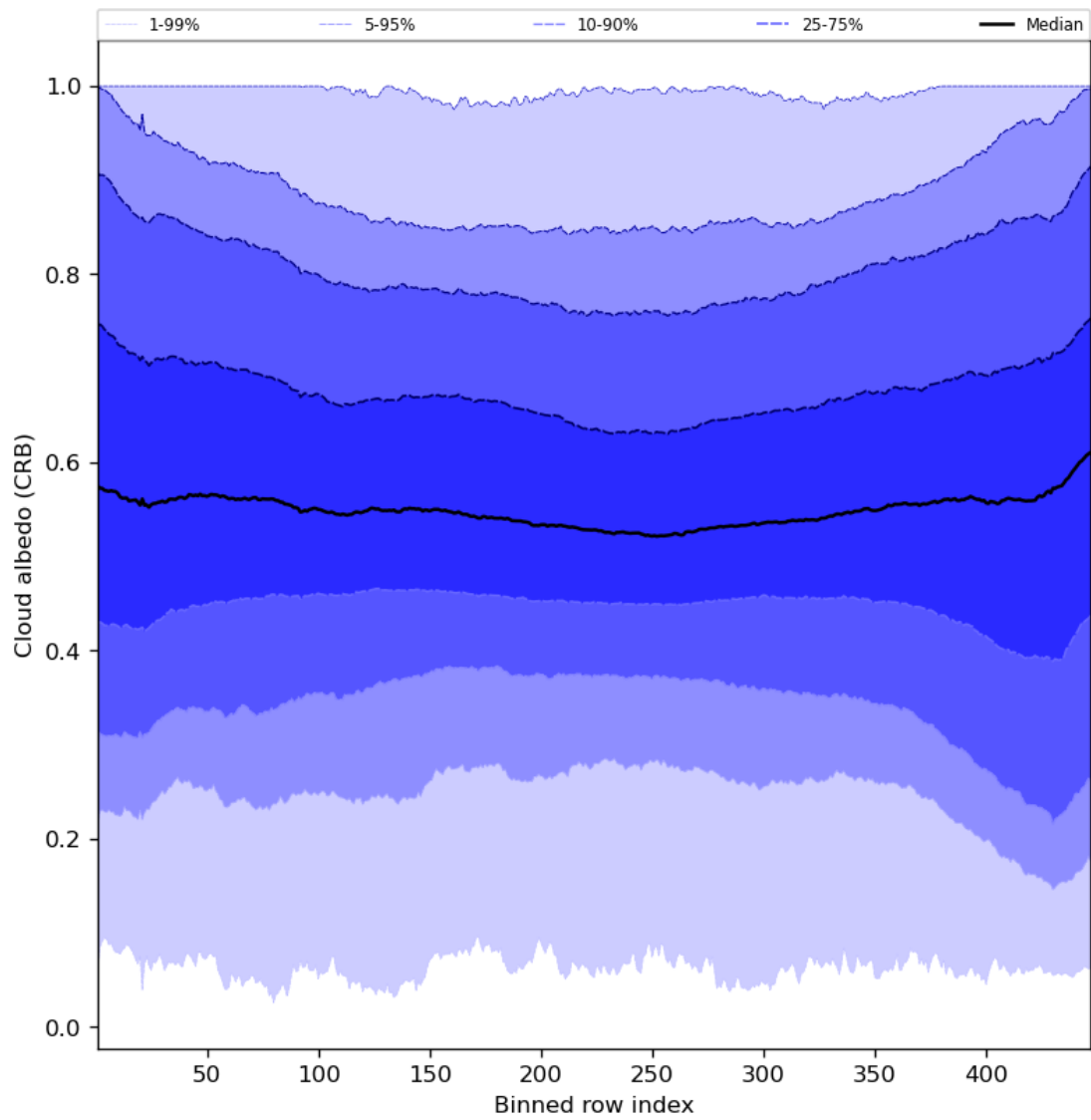
Figure 60: Along track statistics of “Cloud albedo (CRB)” for 2024-07-21 to 2024-07-22
