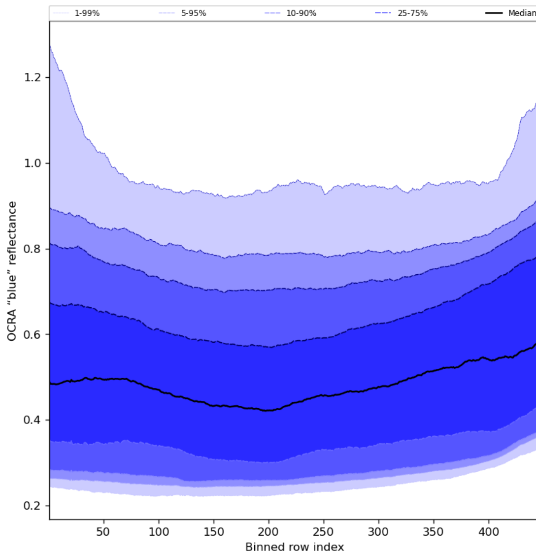
Figure 67: Along track statistics of “OCRA “blue” reflectance” for 2024-07-21 to 2024-07-22
