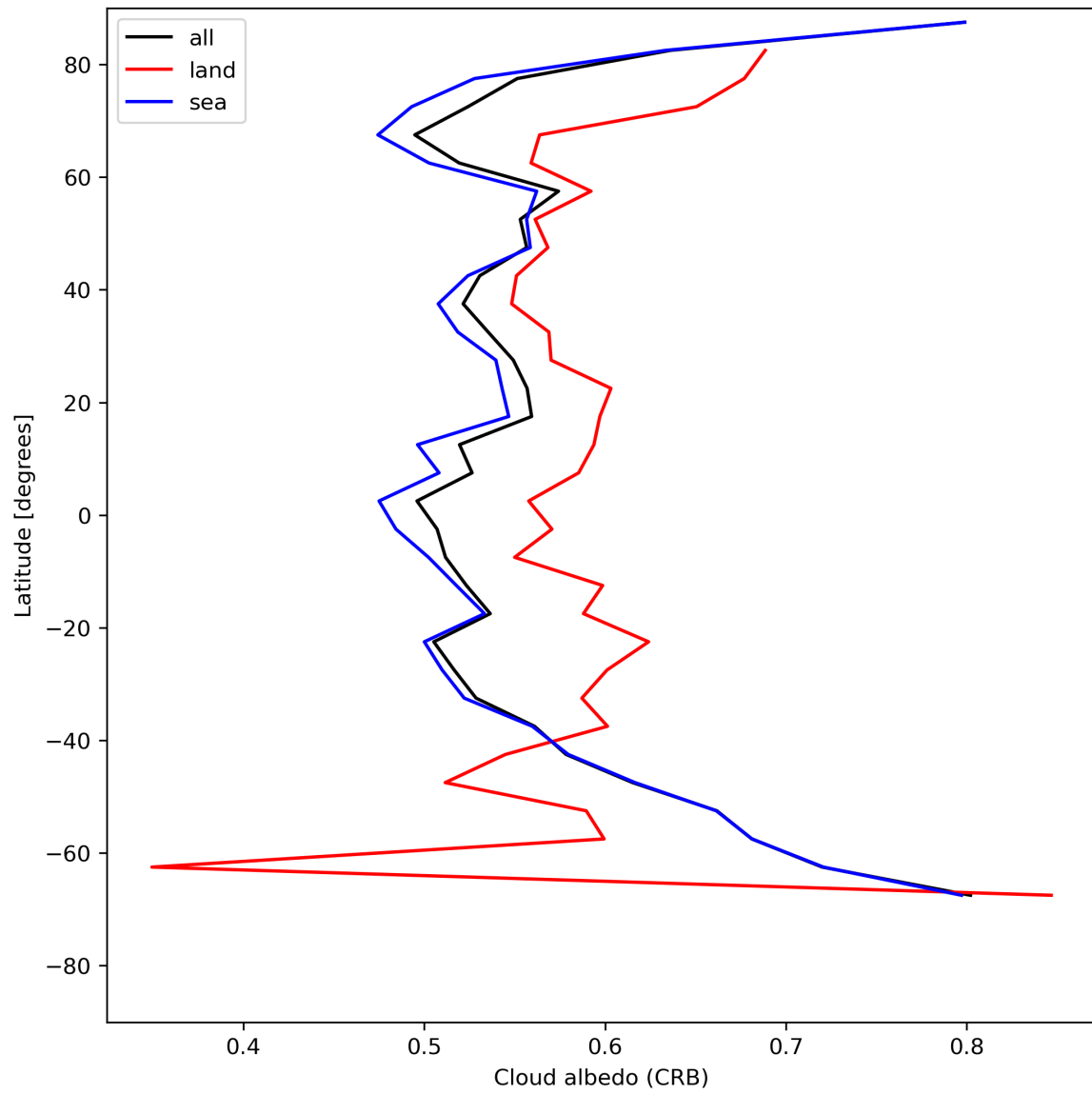
Figure 28: Zonal average of “Cloud albedo (CRB)” for 2024-07-21 to 2024-07-22.
