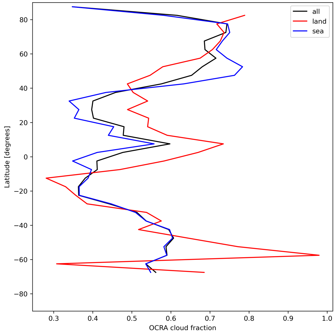
Figure 34: Zonal average of “OCRA cloud fraction” for 2024-07-21 to 2024-07-22.
