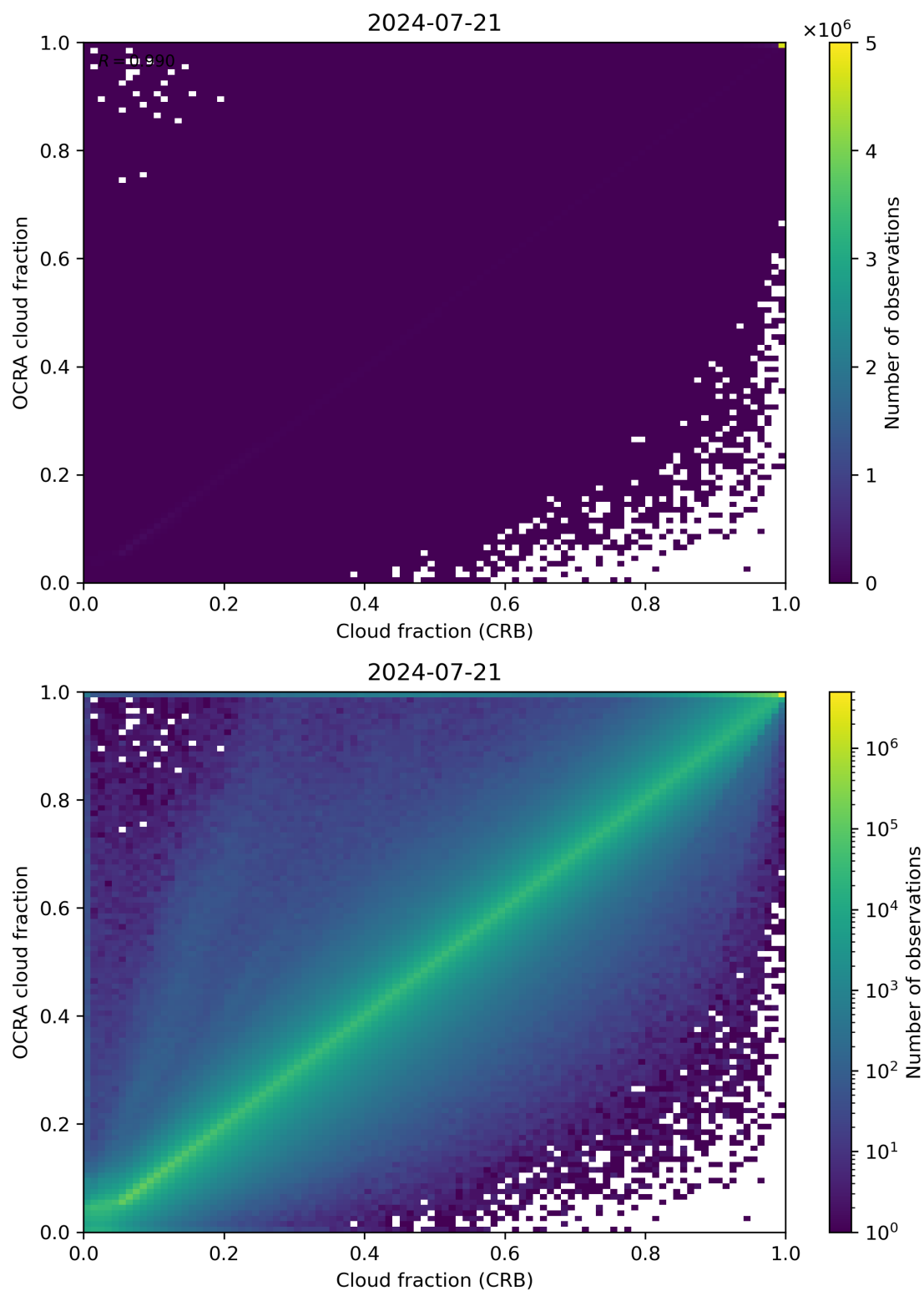
Figure 78: Scatter density plot of “Cloud fraction (CRB)” against “OCRA cloud fraction” for 2024-07-21 to 2024-07-22.
