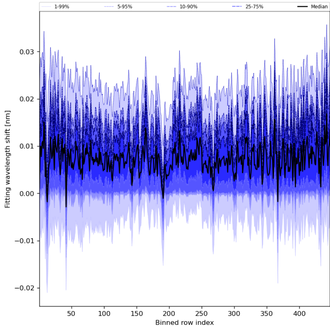
Figure 65: Along track statistics of “Fitting wavelength shift” for 2024-07-21 to 2024-07-22
