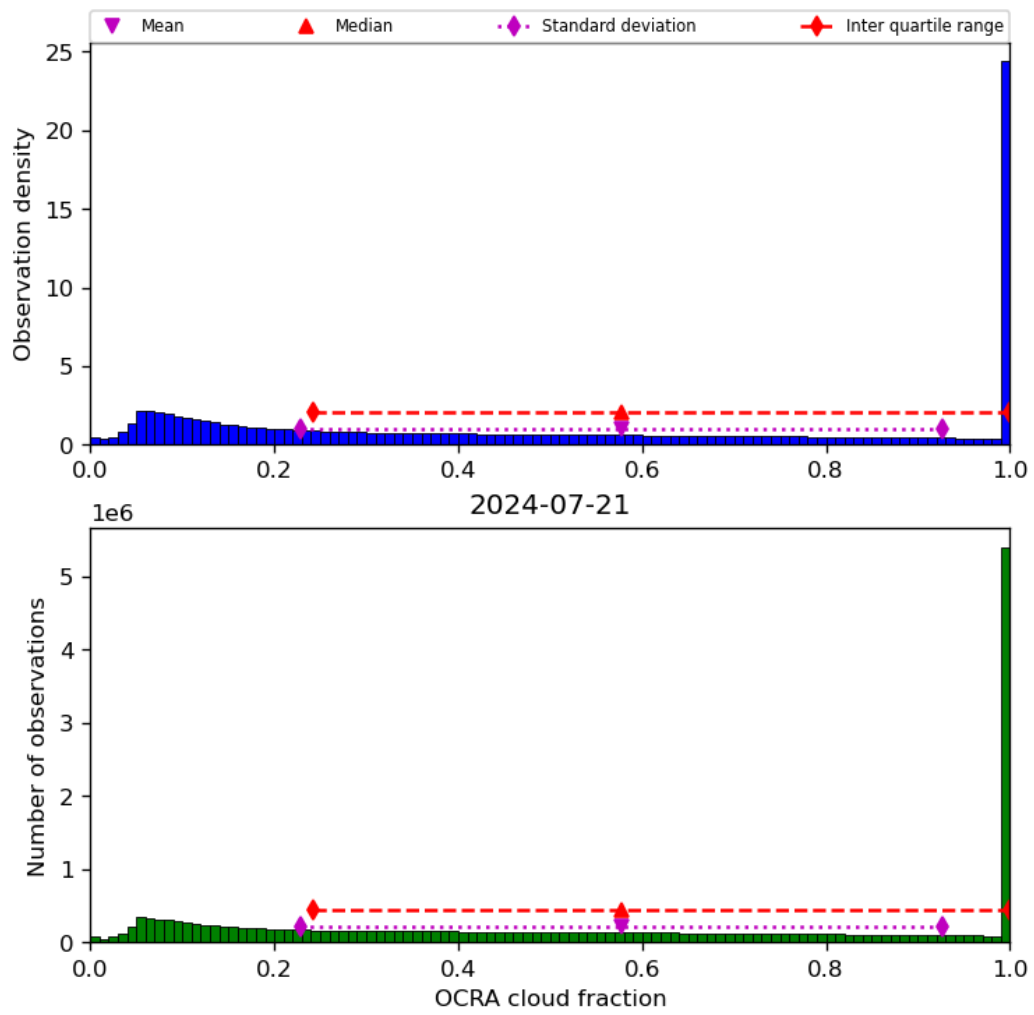
Figure 50: Histogram of “OCRA cloud fraction” for 2024-07-21 to 2024-07-22
