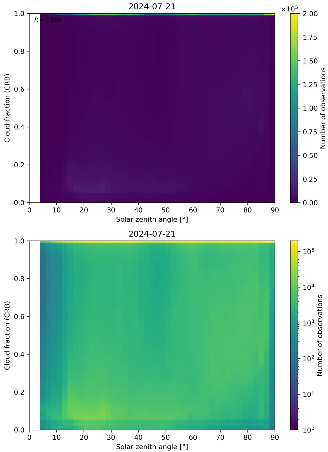
Figure 101: Scatter density plot of “Solar zenith angle” against “Cloud fraction (CRB)” for 2024-07-21 to 2024-07-22.
