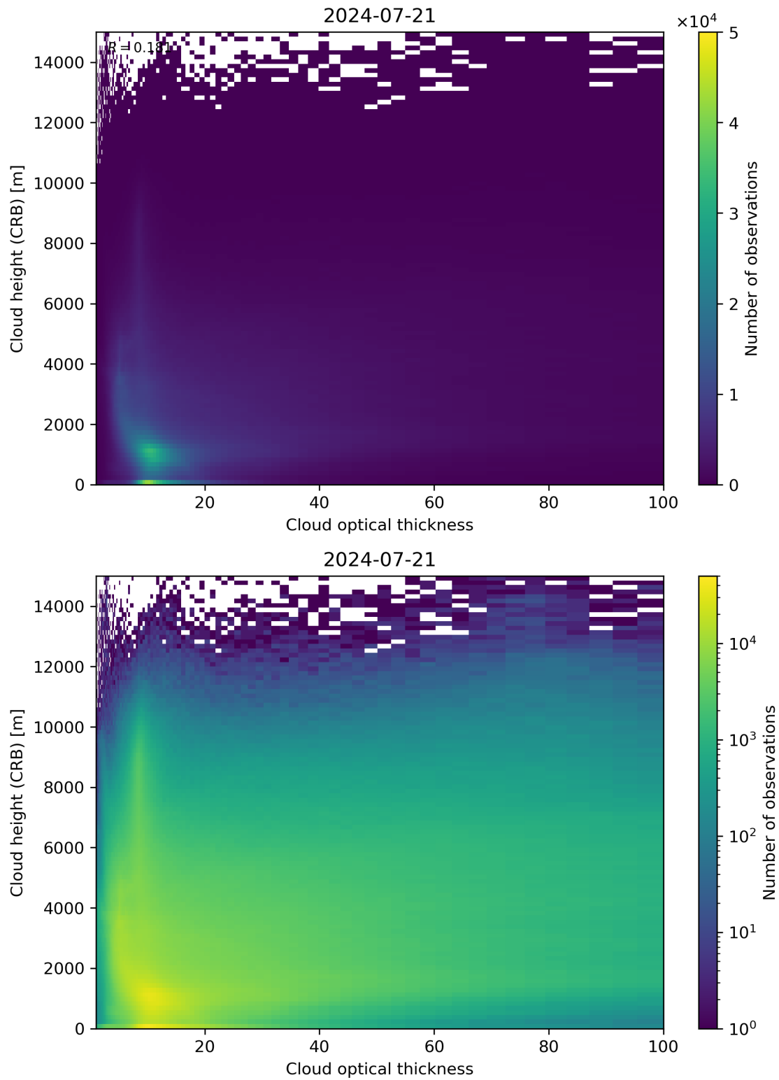
Figure 85: Scatter density plot of “Cloud optical thickness” against “Cloud height (CRB)” for 2024-07-21 to 2024-07-22.
