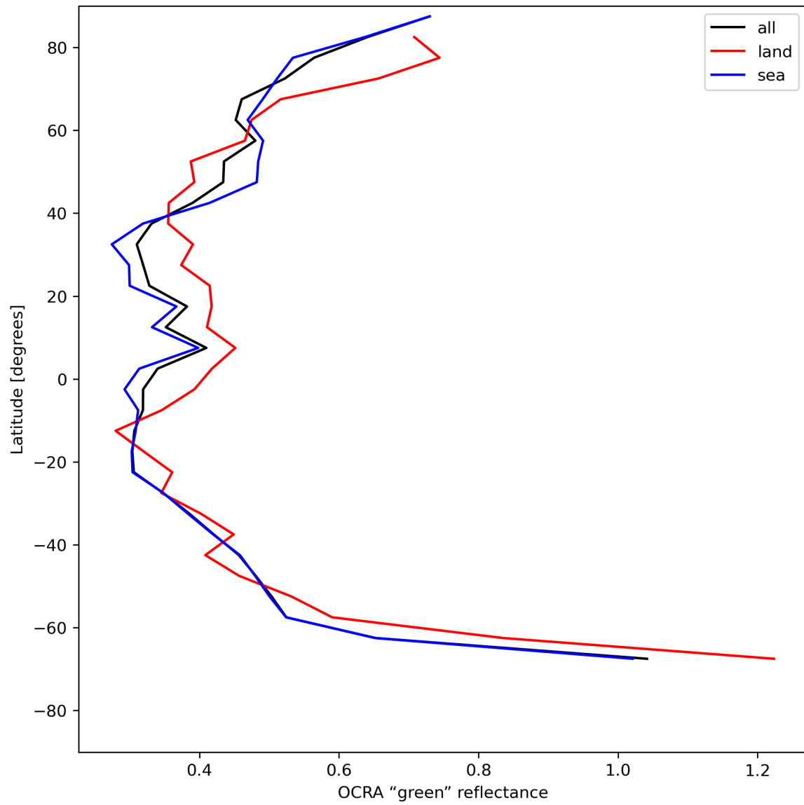
Figure 36: Zonal average of “OCRA “green” reflectance” for 2024-07-21 to 2024-07-22.
