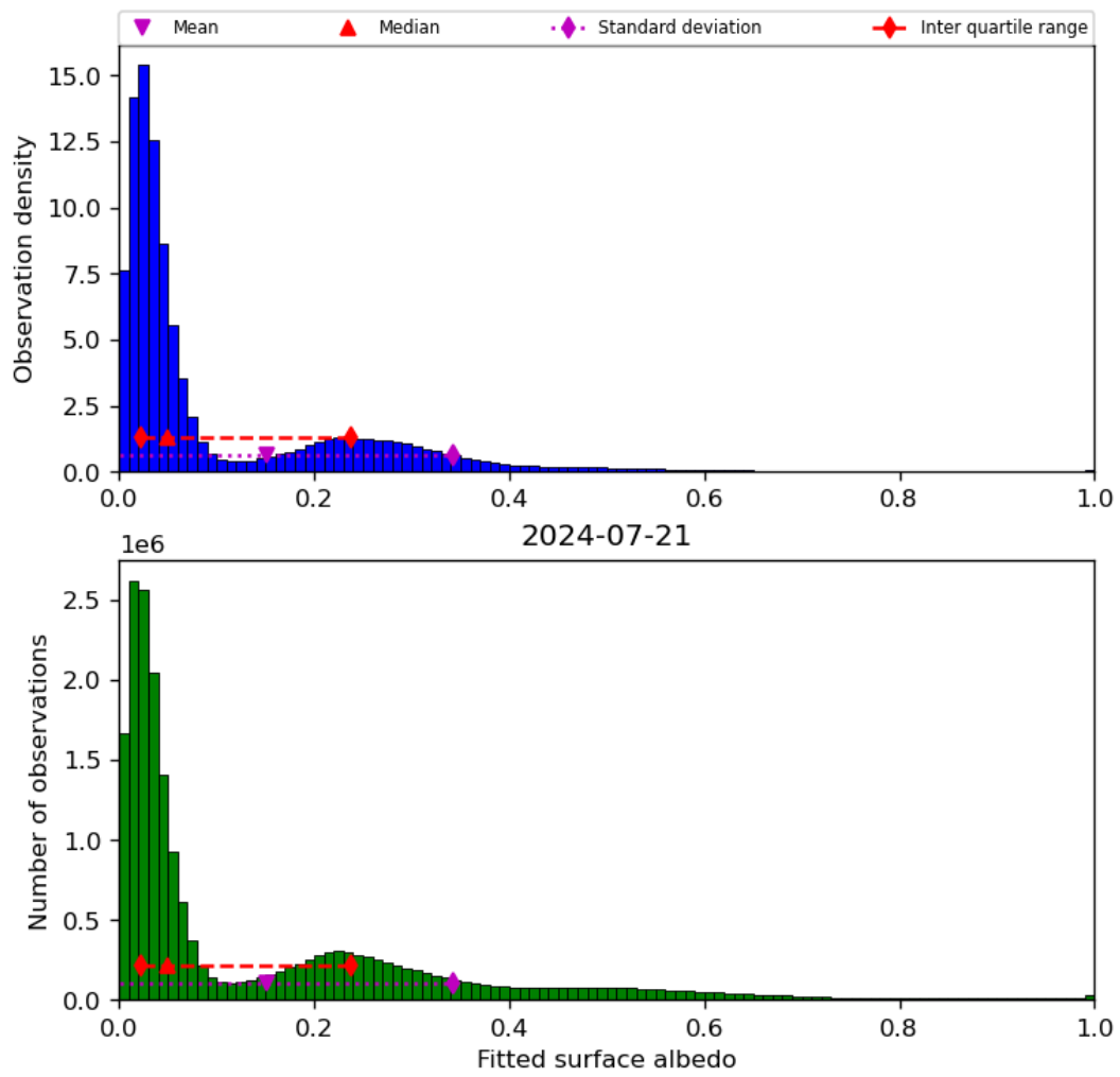
Figure 45: Histogram of “Fitted surface albedo” for 2024-07-21 to 2024-07-22
