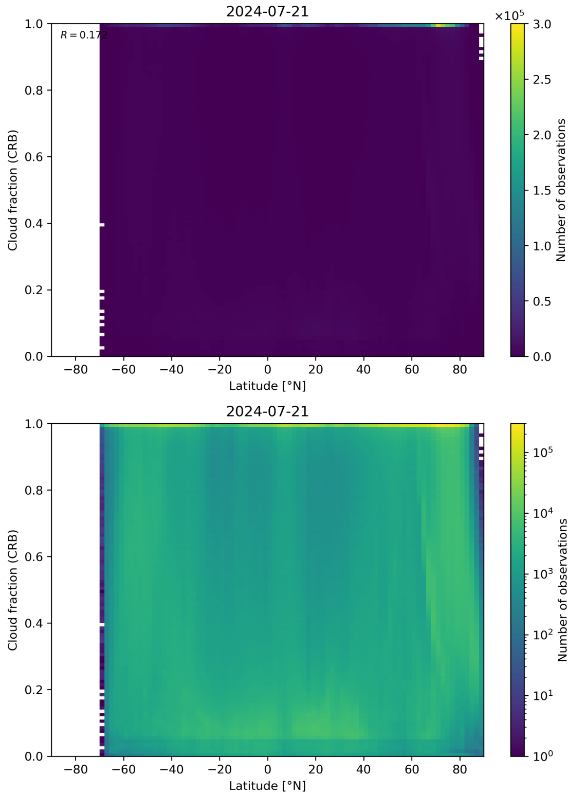
Figure 94: Scatter density plot of “Latitude” against “Cloud fraction (CRB)” for 2024-07-21 to 2024-07-22.
