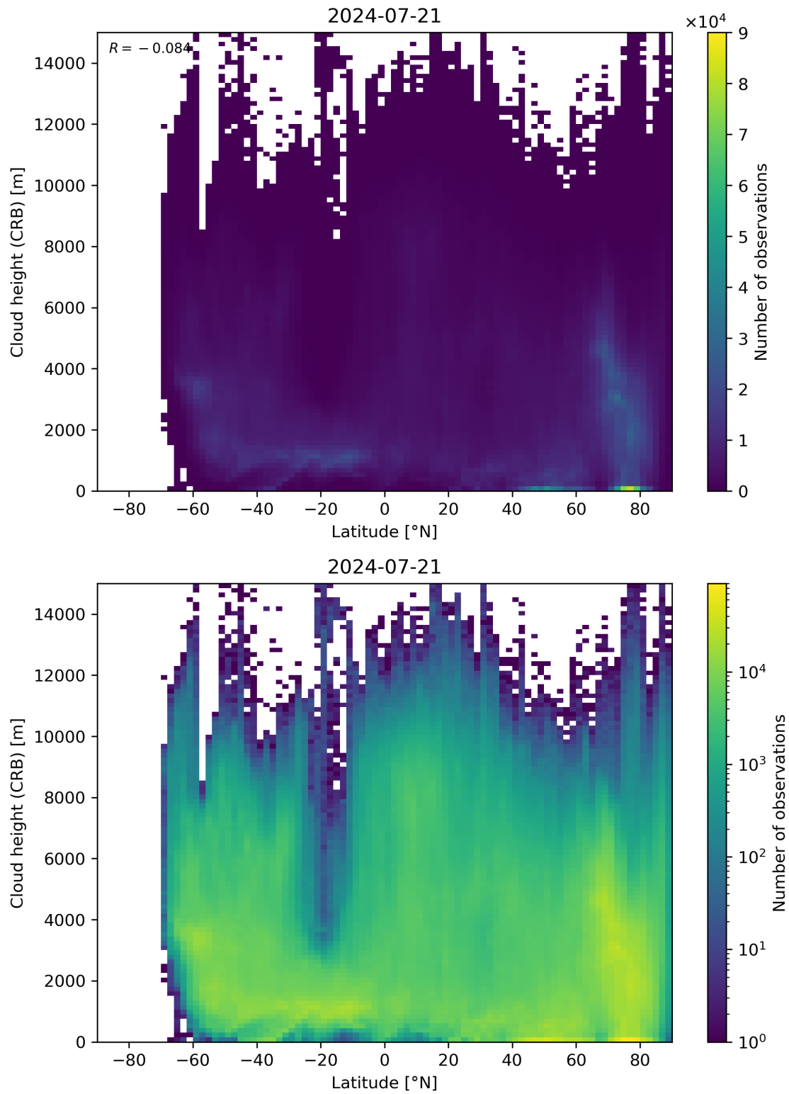
Figure 95: Scatter density plot of “Latitude” against “Cloud height (CRB)” for 2024-07-21 to 2024-07-22.
