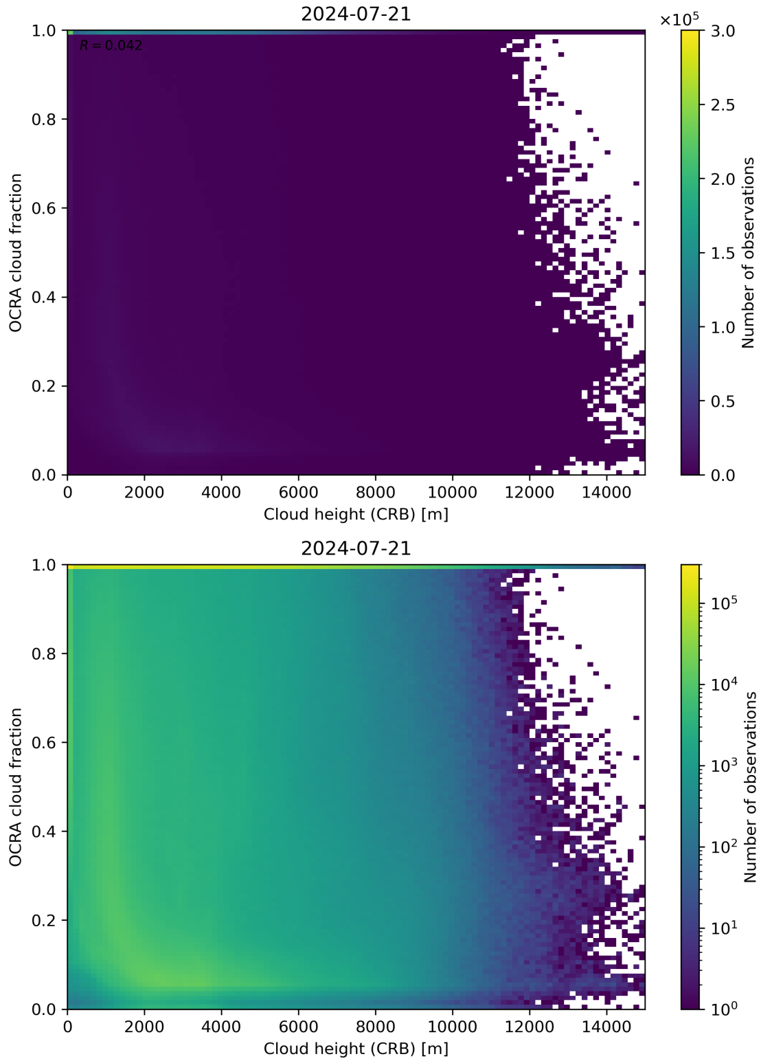
Figure 81: Scatter density plot of “Cloud height (CRB)” against “OCRA cloud fraction” for 2024-07-21 to 2024-07-22.
