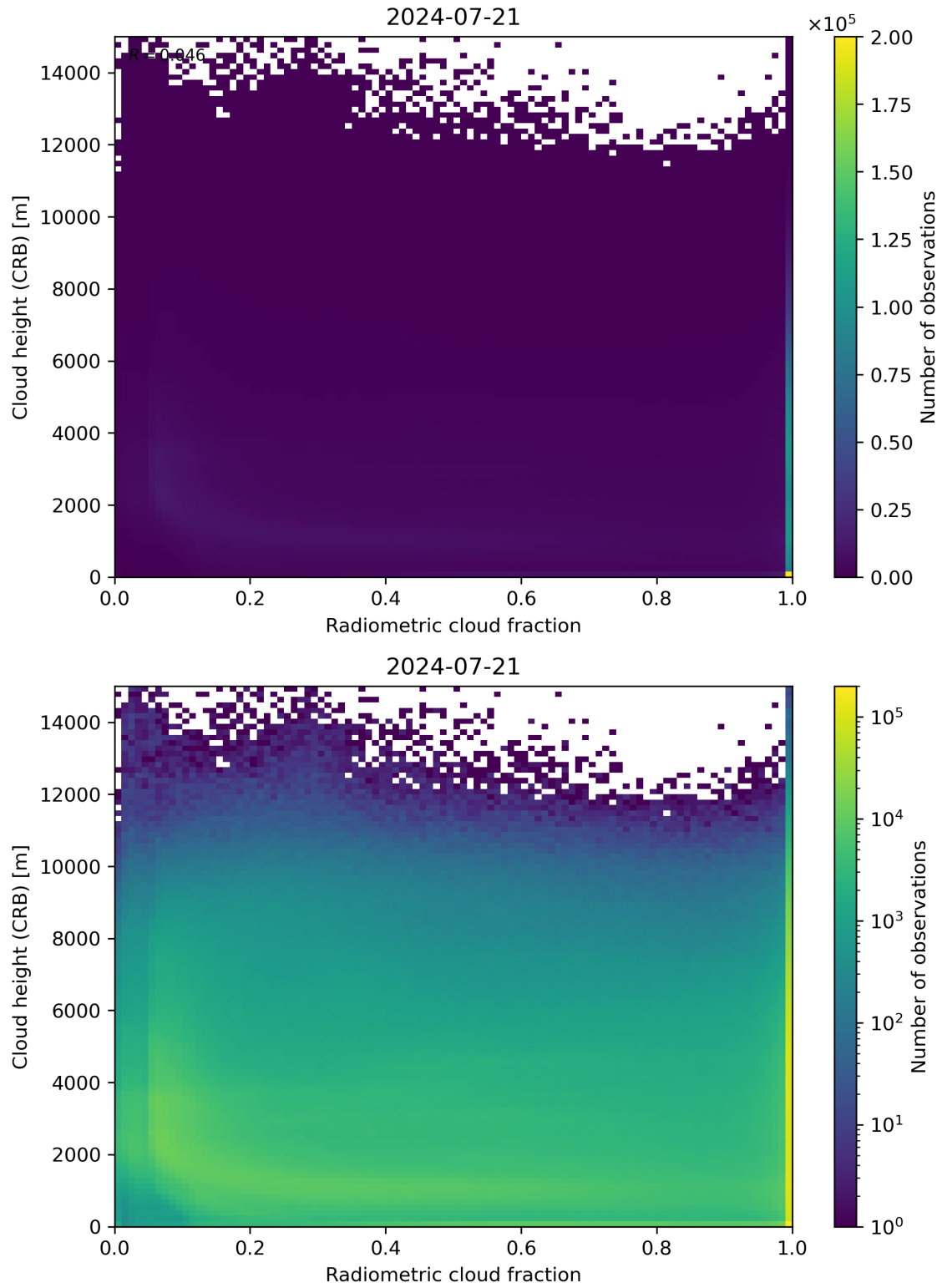
Figure 74: Scatter density plot of “Radiometric cloud fraction” against “Cloud height (CRB)” for 2024-07-21 to 2024-07-22.
