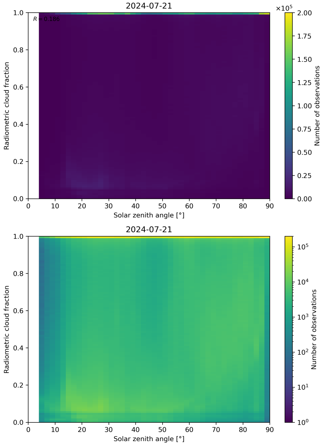
Figure 99: Scatter density plot of “Solar zenith angle” against “Radiometric cloud fraction” for 2024-07-21 to 2024-07-22.
