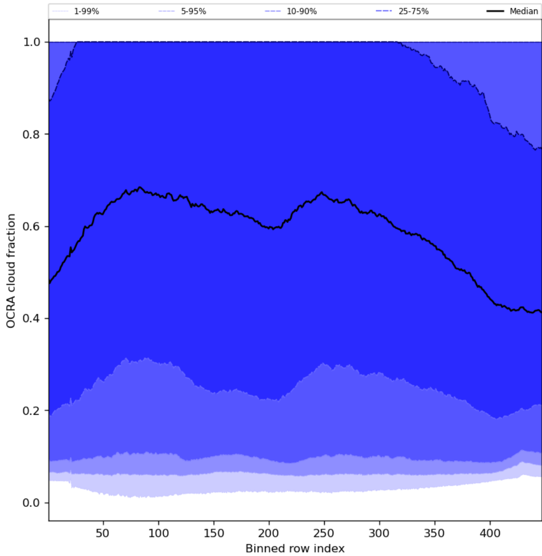
Figure 66: Along track statistics of “OCRA cloud fraction” for 2024-07-21 to 2024-07-22
