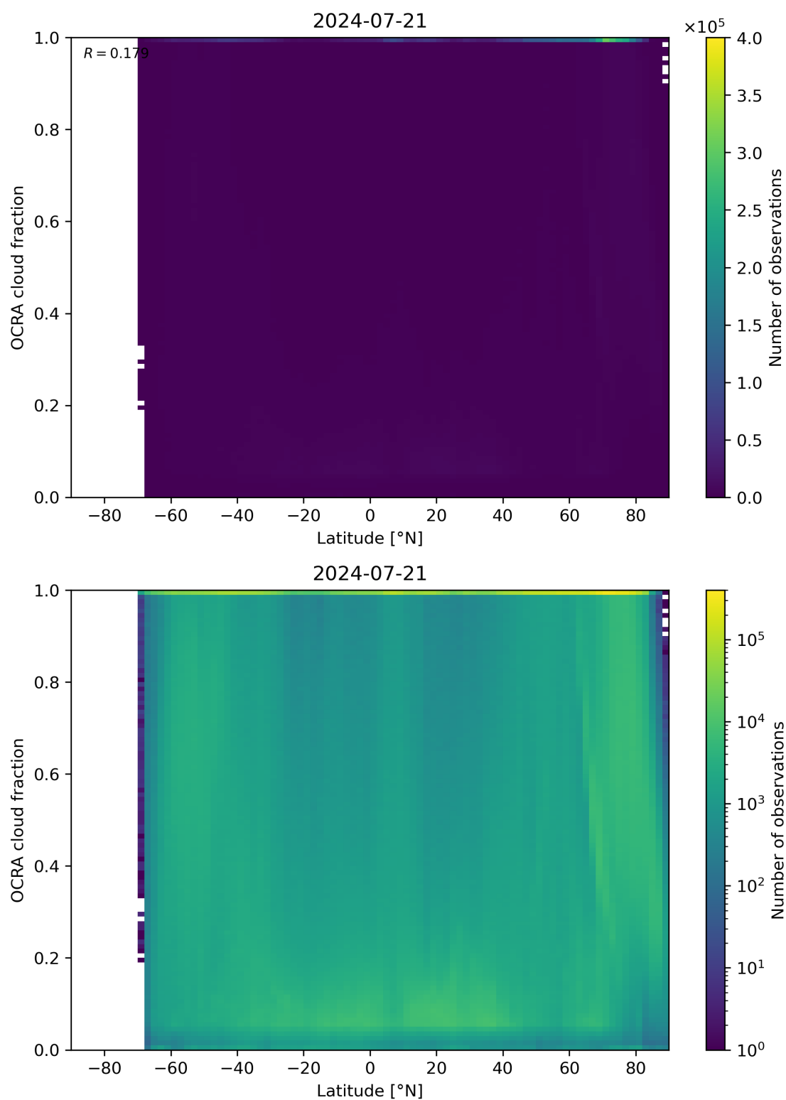
Figure 93: Scatter density plot of “Latitude” against “OCRA cloud fraction” for 2024-07-21 to 2024-07-22.
