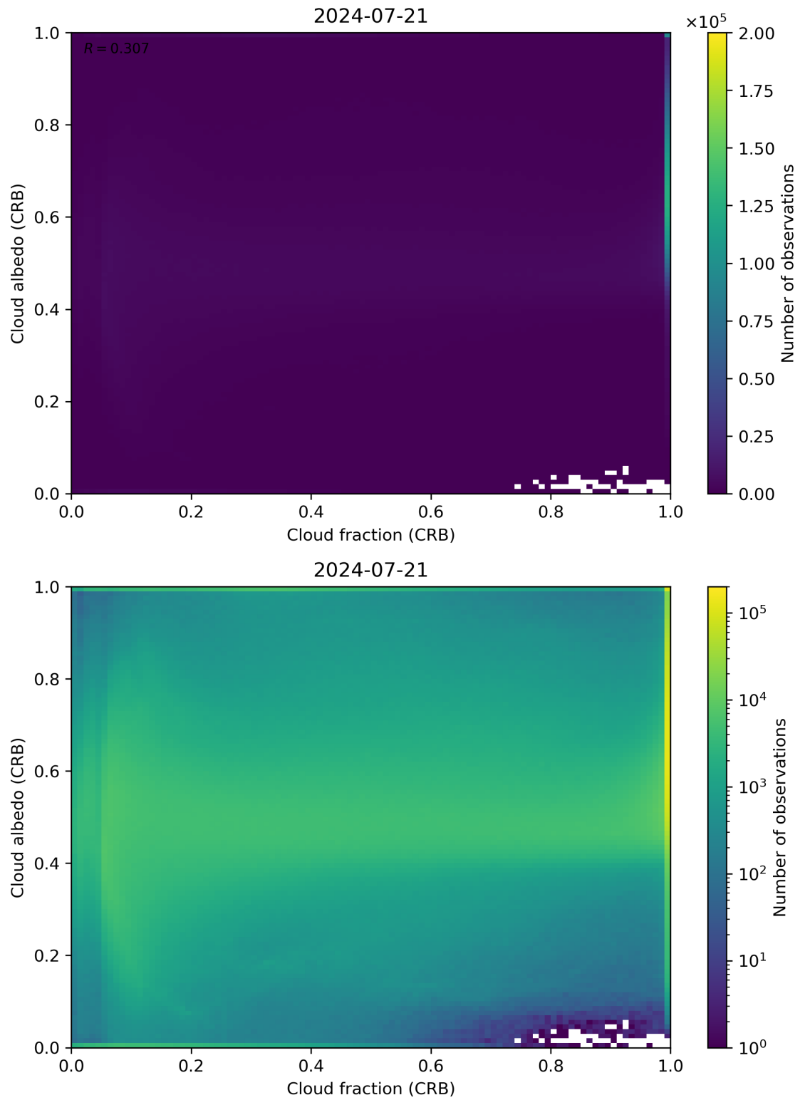
Figure 77: Scatter density plot of “Cloud fraction (CRB)” against “Cloud albedo (CRB)” for 2024-07-21 to 2024-07-22.
