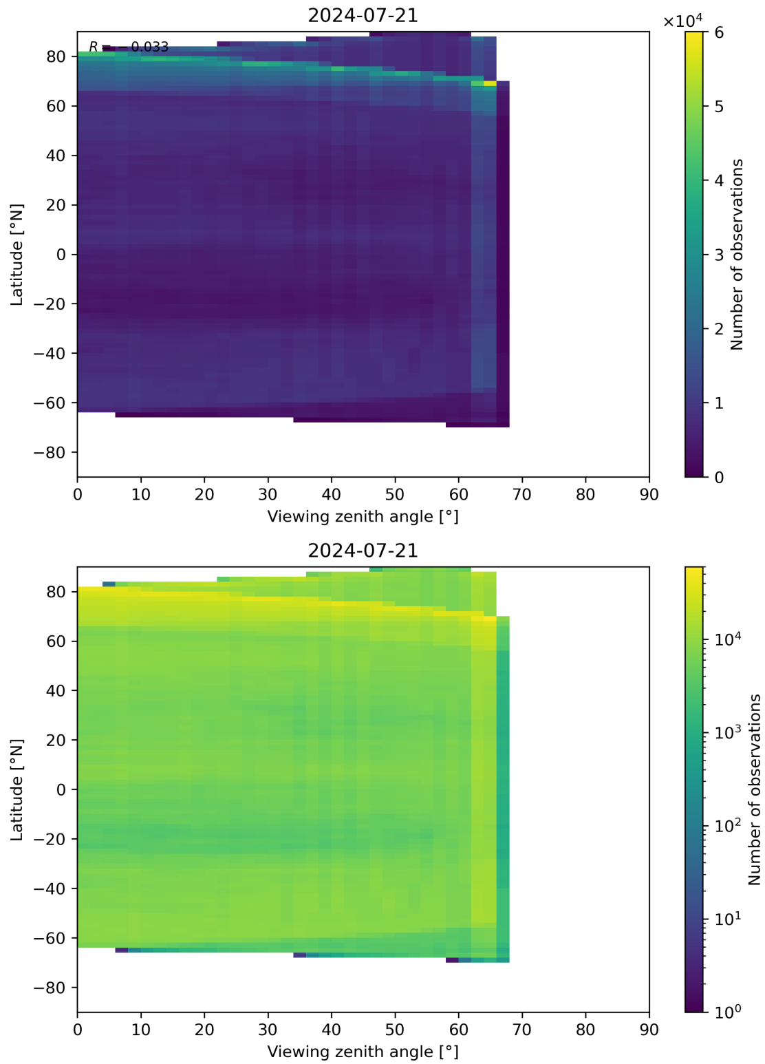
Figure 113: Scatter density plot of “Viewing zenith angle” against “Latitude” for 2024-07-21 to 2024-07-22.
