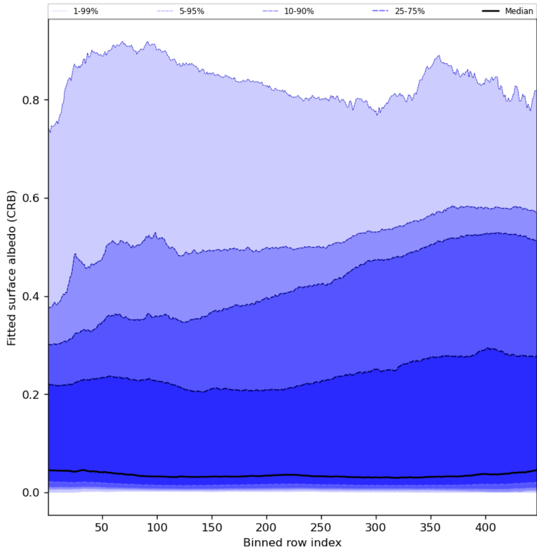
Figure 62: Along track statistics of “Fitted surface albedo (CRB)” for 2024-07-21 to 2024-07-22
