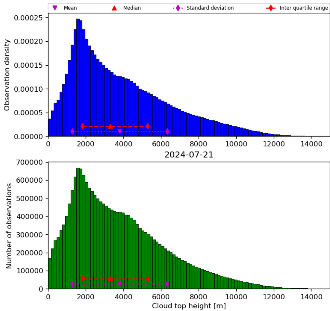
Figure 40: Histogram of “Cloud top height” for 2024-07-21 to 2024-07-22
