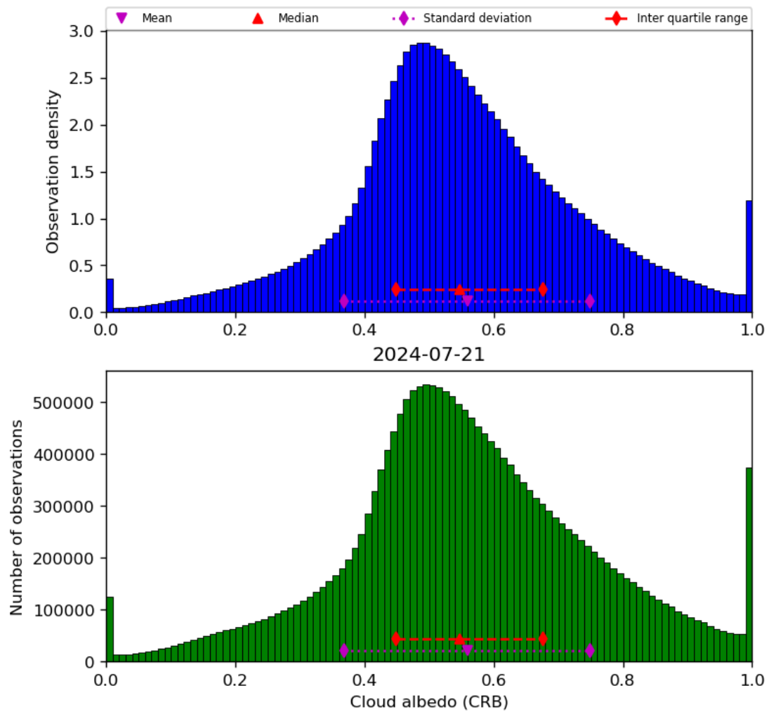
Figure 44: Histogram of “Cloud albedo (CRB)” for 2024-07-21 to 2024-07-22
