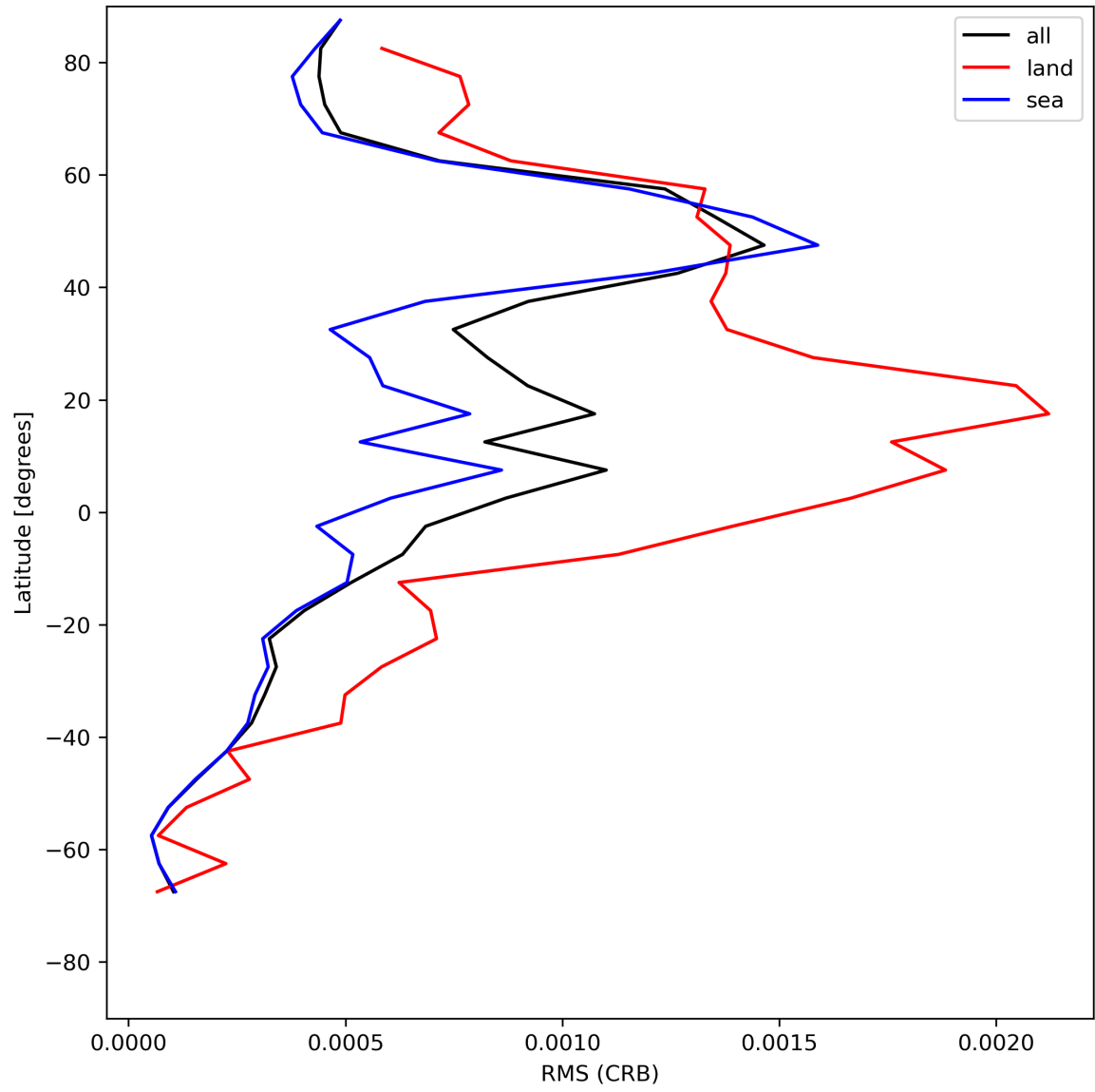
Figure 32: Zonal average of “RMS (CRB)” for 2024-07-21 to 2024-07-22.
