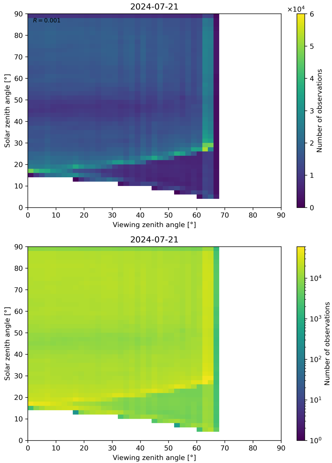
Figure 114: Scatter density plot of “Viewing zenith angle” against “Solar zenith angle” for 2024-07-21 to 2024-07-22.
