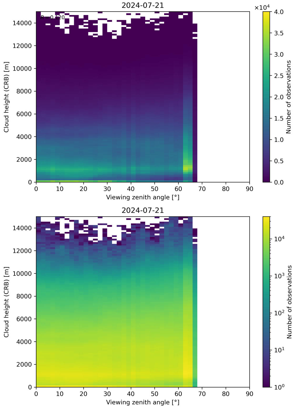
Figure 110: Scatter density plot of “Viewing zenith angle” against “Cloud height (CRB)” for 2024-07-21 to 2024-07-22.
