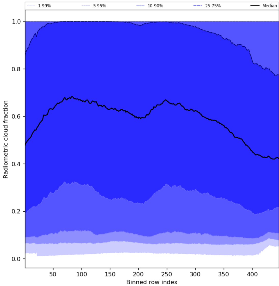
Figure 55: Along track statistics of “Radiometric cloud fraction” for 2024-07-21 to 2024-07-22
