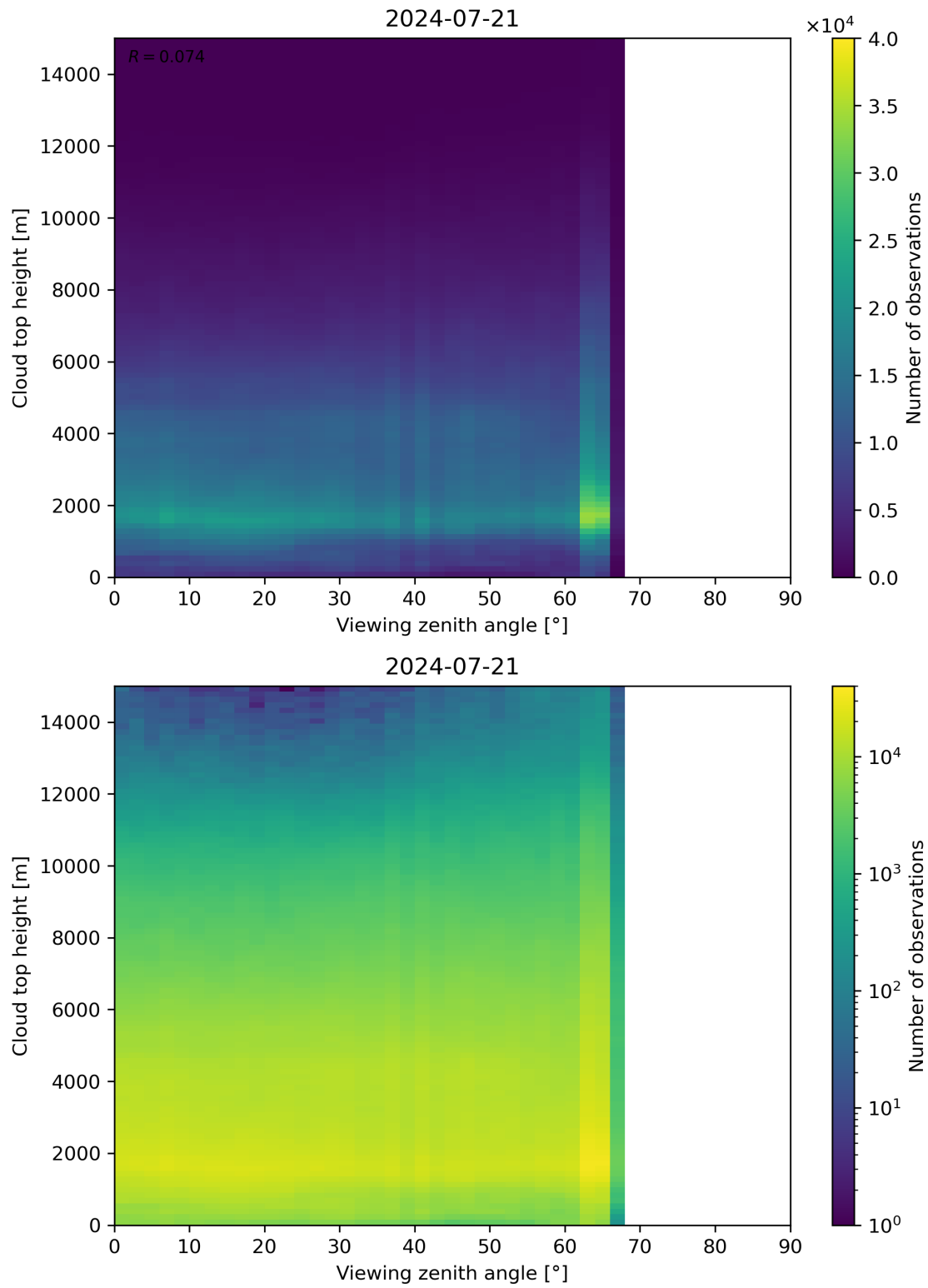
Figure 112: Scatter density plot of “Viewing zenith angle” against “Cloud top height” for 2024-07-21 to 2024-07-22.
