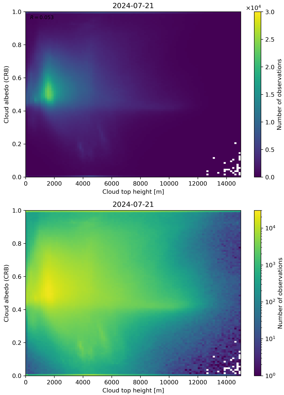
Figure 86: Scatter density plot of “Cloud top height” against “Cloud albedo (CRB)” for 2024-07-21 to 2024-07-22.
