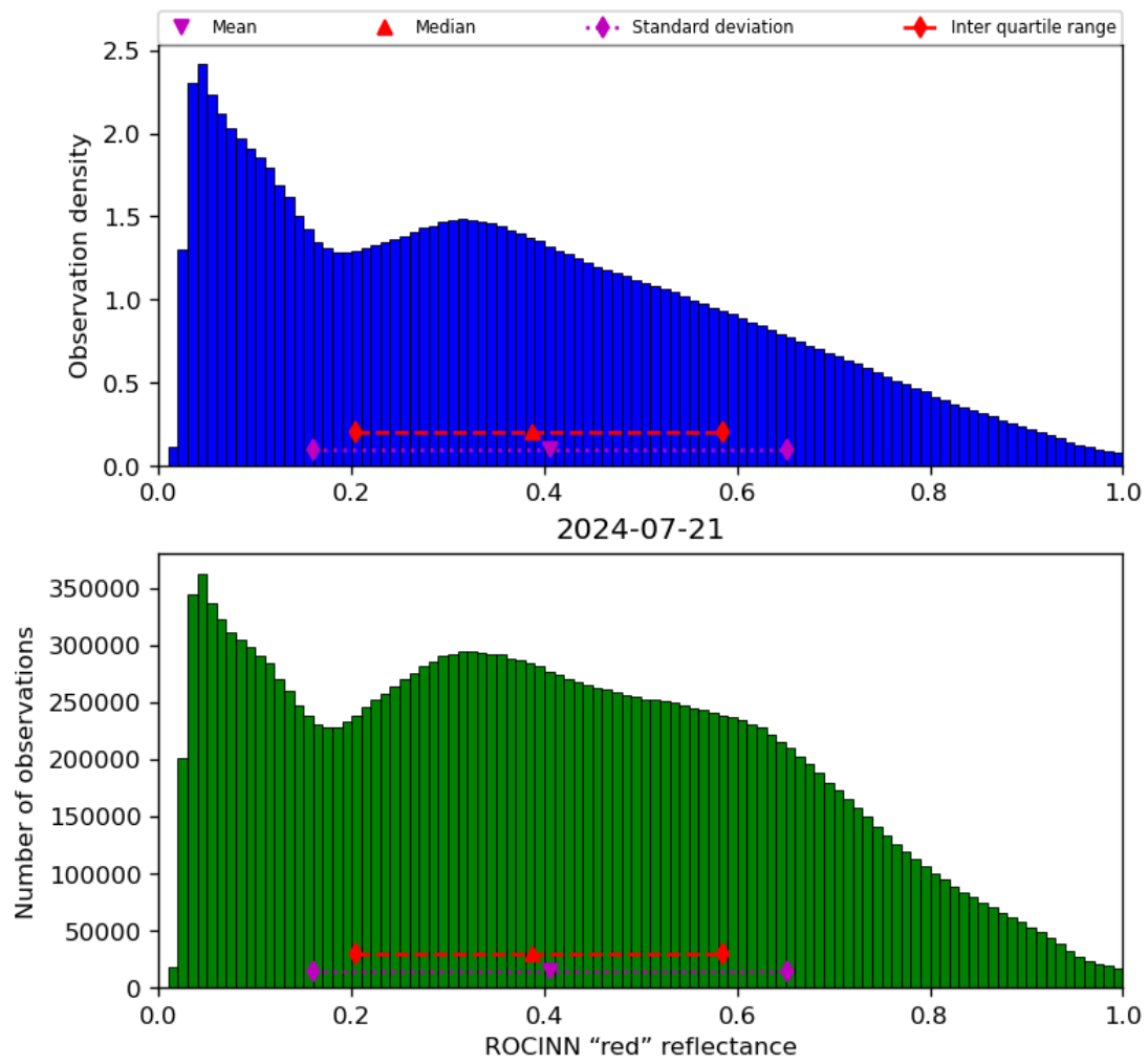
Figure 53: Histogram of “ROCINN “red” reflectance” for 2024-07-21 to 2024-07-22
