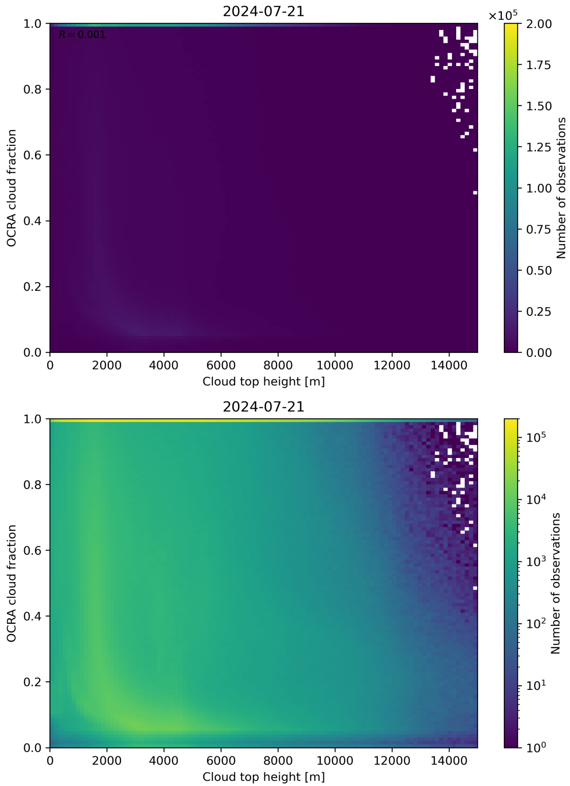
Figure 87: Scatter density plot of “Cloud top height” against “OCRA cloud fraction” for 2024-07-21 to 2024-07-22.
