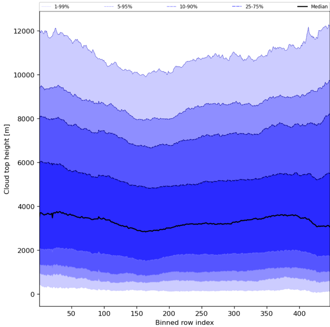
Figure 56: Along track statistics of “Cloud top height” for 2024-07-21 to 2024-07-22
