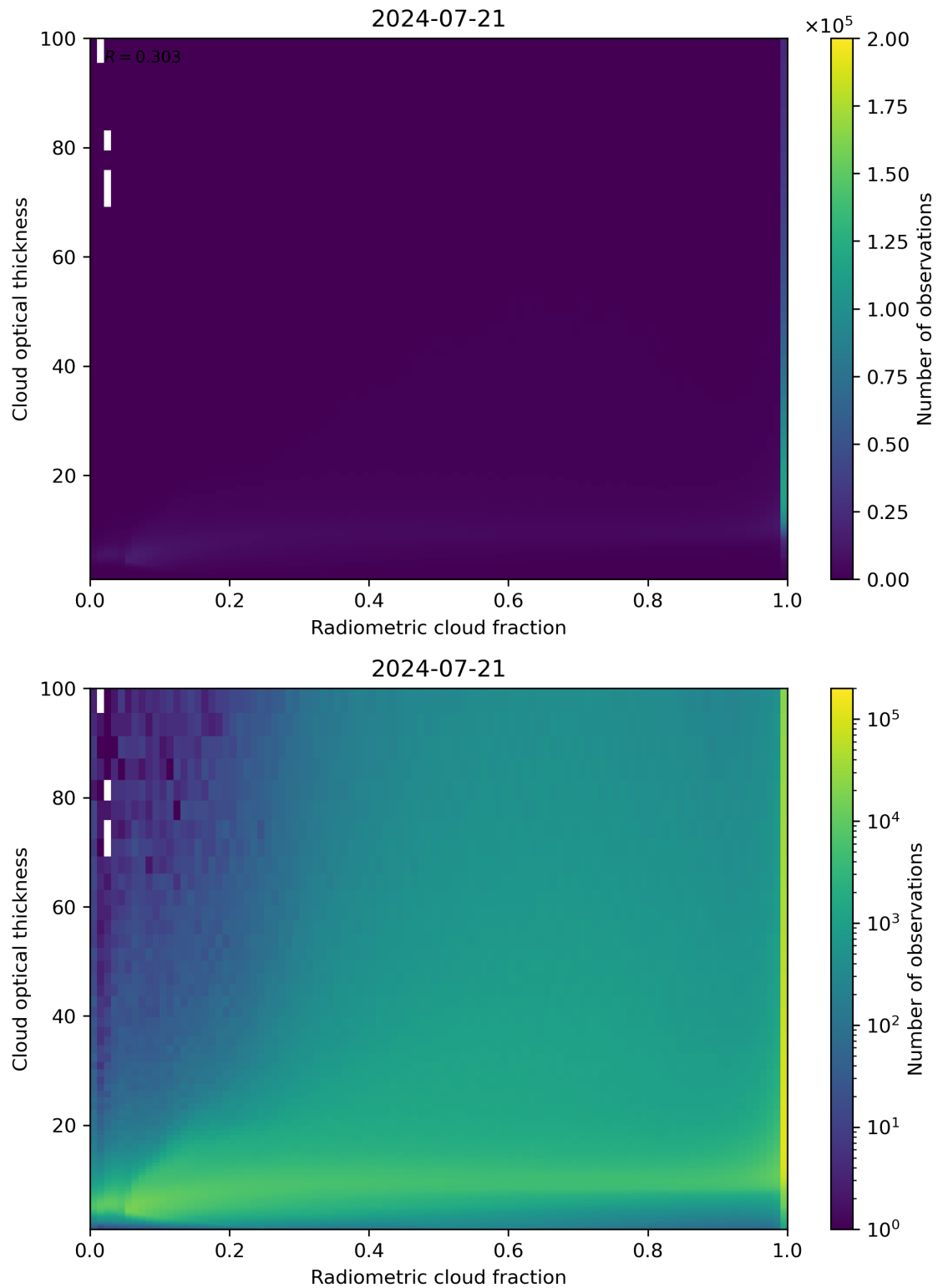
Figure 75: Scatter density plot of “Radiometric cloud fraction” against “Cloud optical thickness” for 2024-07-21 to 2024-07-22.
