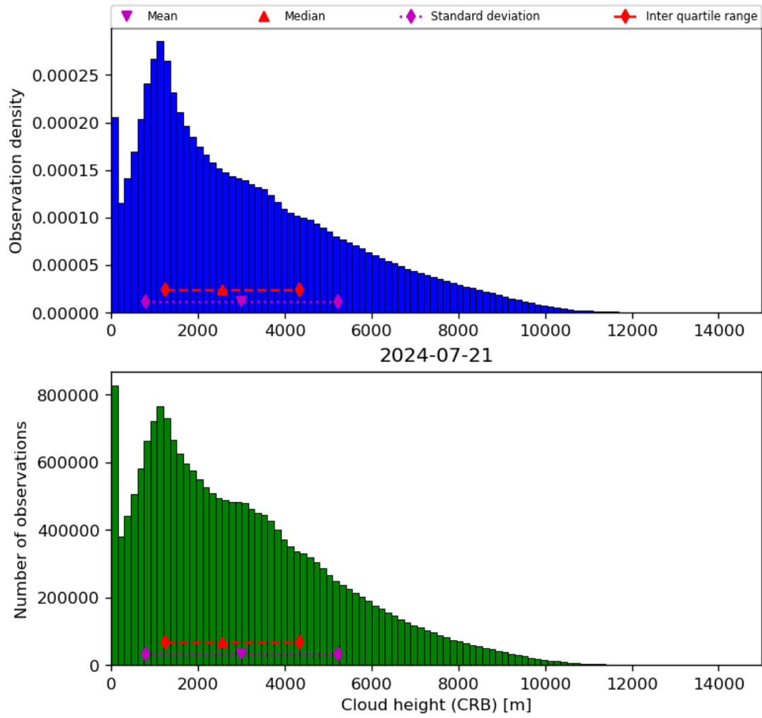
Figure 43: Histogram of “Cloud height (CRB)” for 2024-07-21 to 2024-07-22
