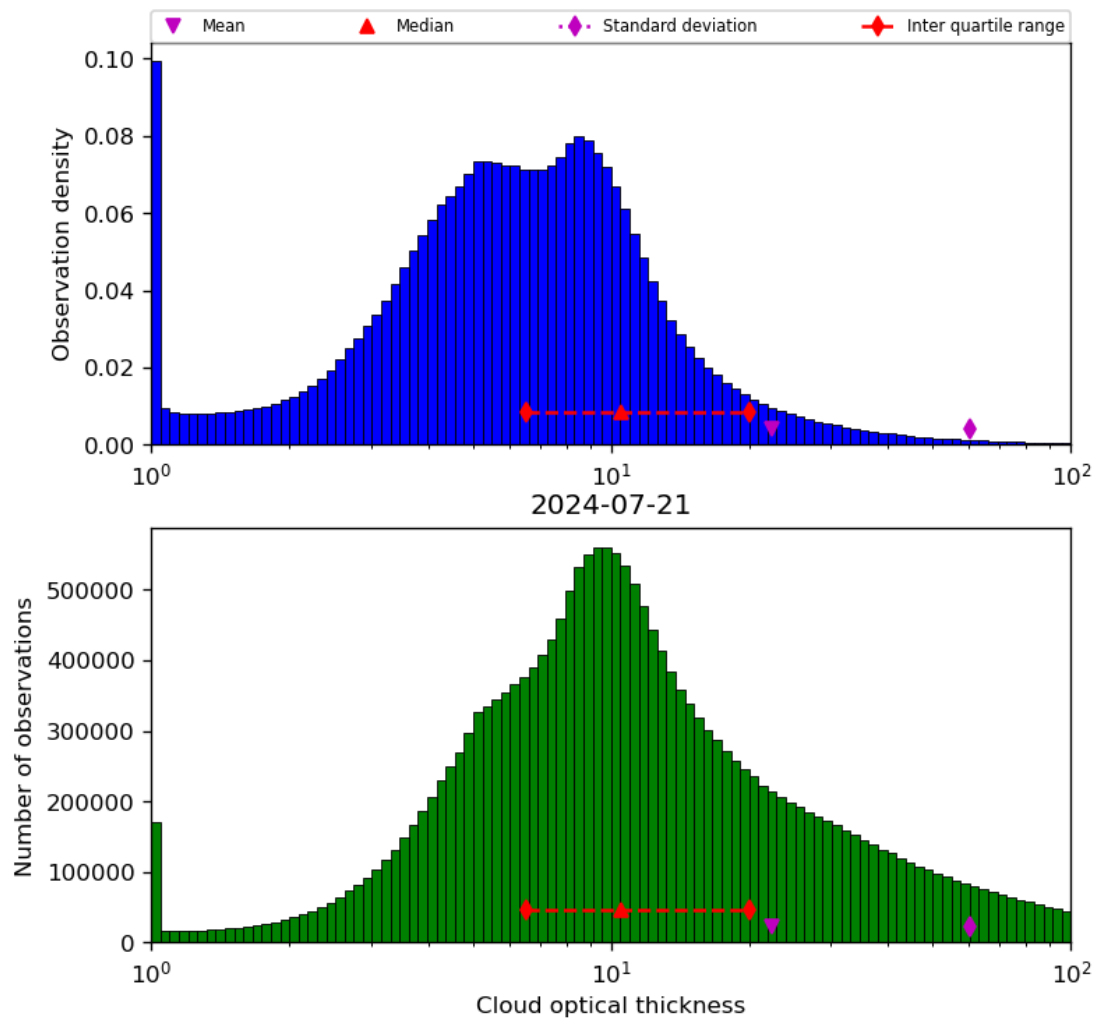
Figure 41: Histogram of “Cloud optical thickness” for 2024-07-21 to 2024-07-22
