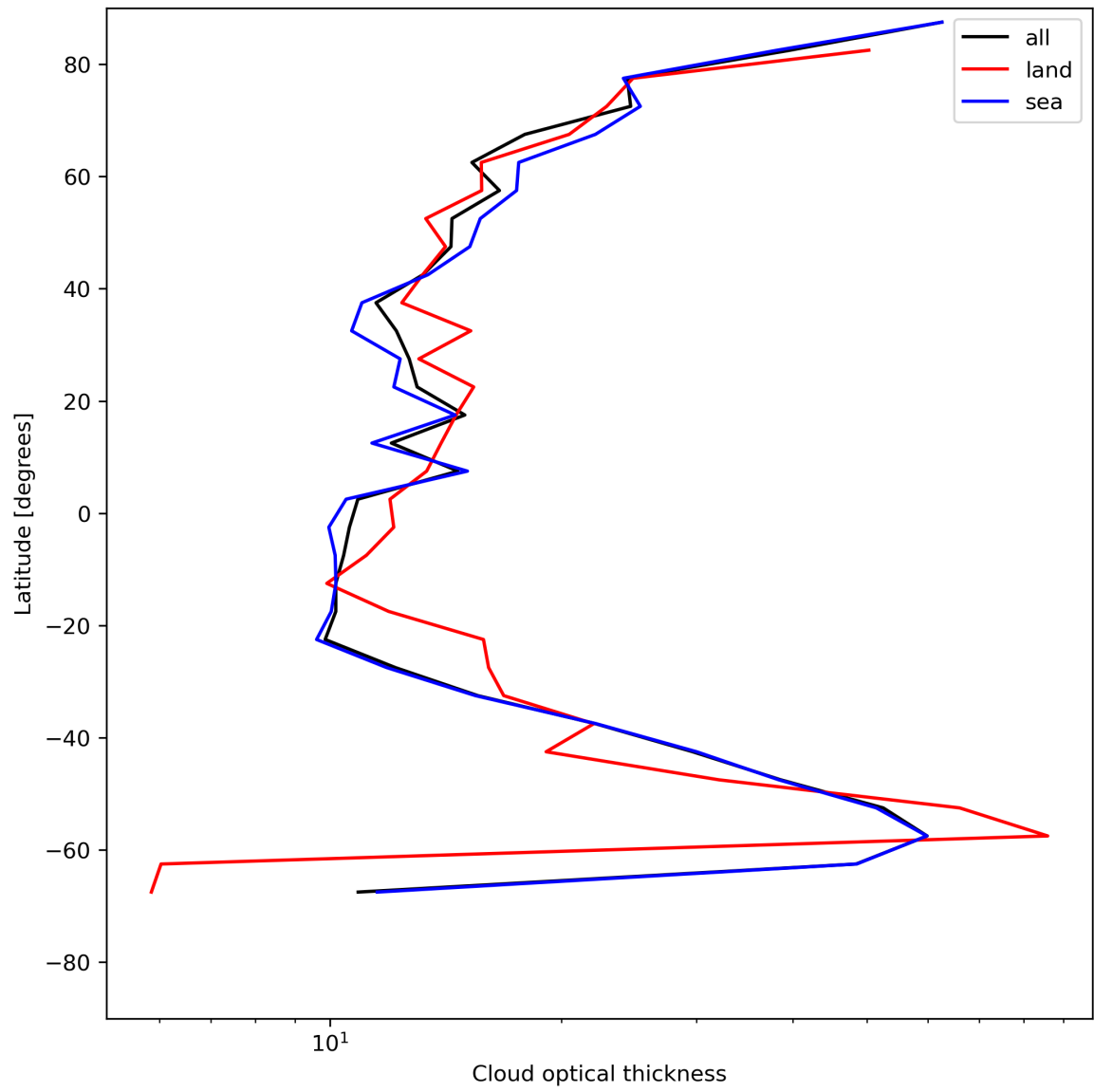
Figure 25: Zonal average of “Cloud optical thickness” for 2024-07-21 to 2024-07-22.
