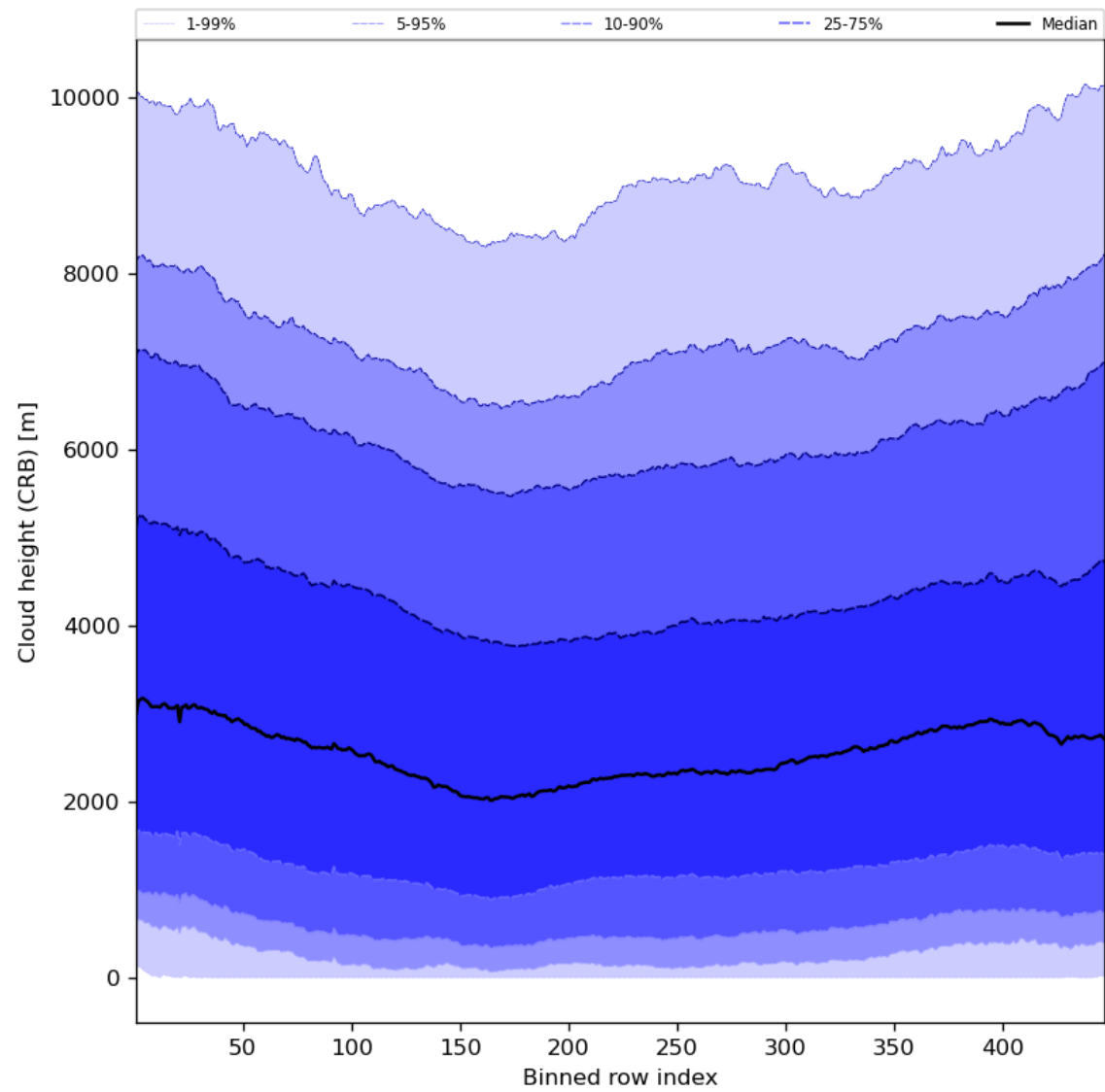
Figure 59: Along track statistics of “Cloud height (CRB)” for 2024-07-21 to 2024-07-22
