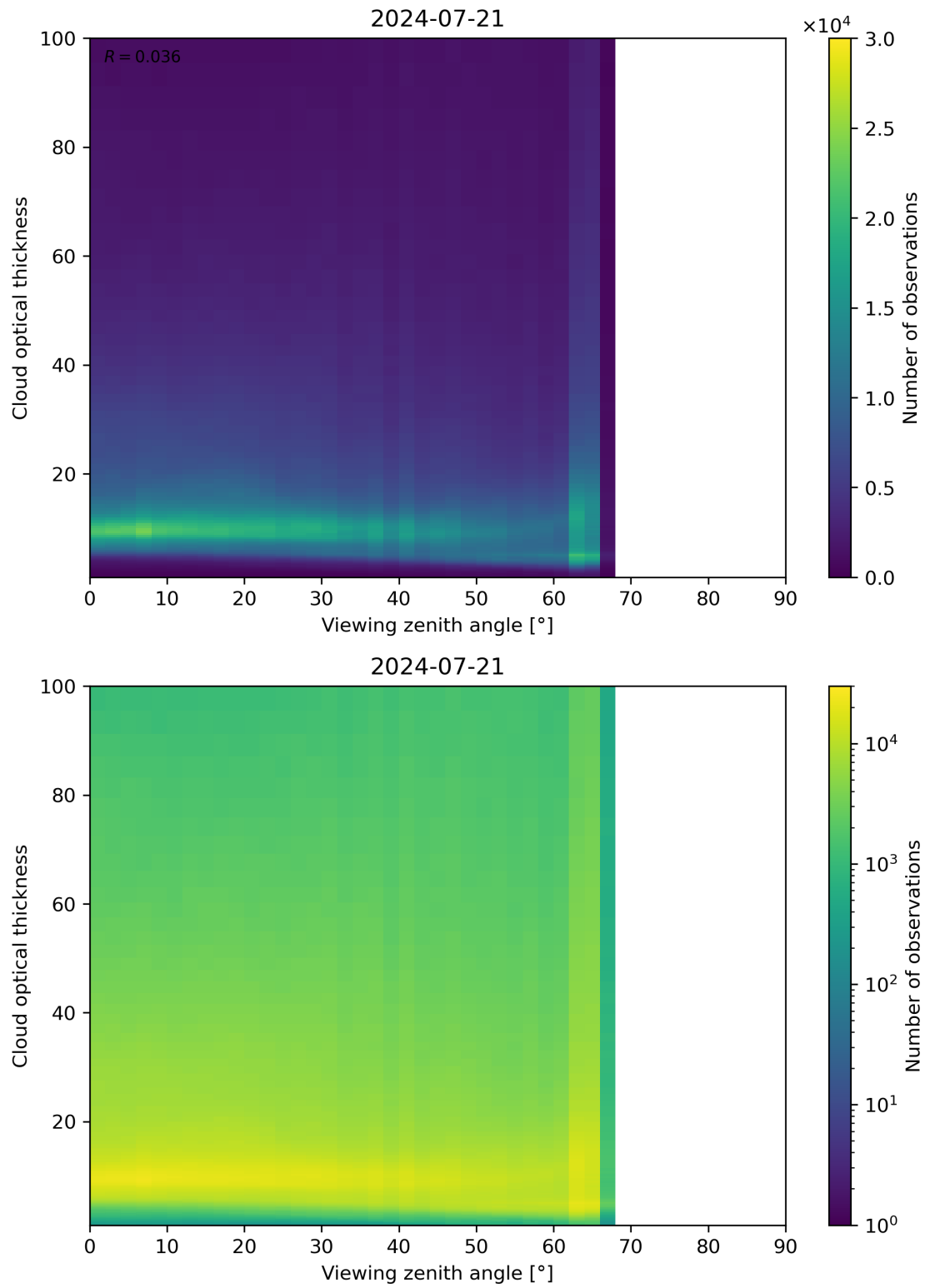
Figure 111: Scatter density plot of “Viewing zenith angle” against “Cloud optical thickness” for 2024-07-21 to 2024-07-22.
