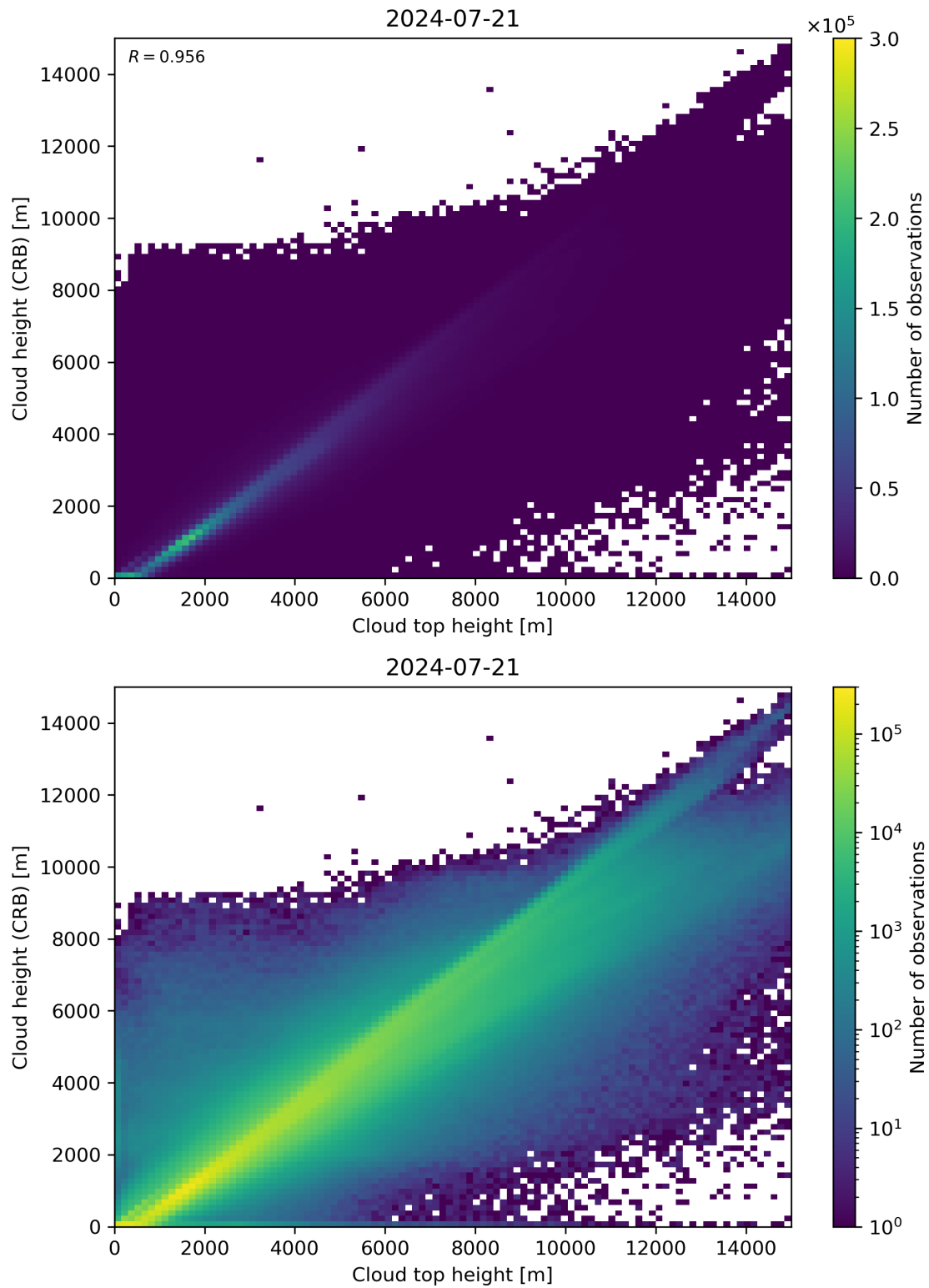
Figure 89: Scatter density plot of “Cloud top height” against “Cloud height (CRB)” for 2024-07-21 to 2024-07-22.
