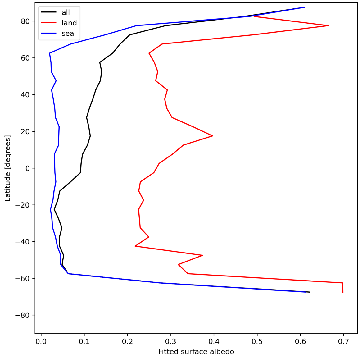
Figure 29: Zonal average of “Fitted surface albedo” for 2024-07-21 to 2024-07-22.
