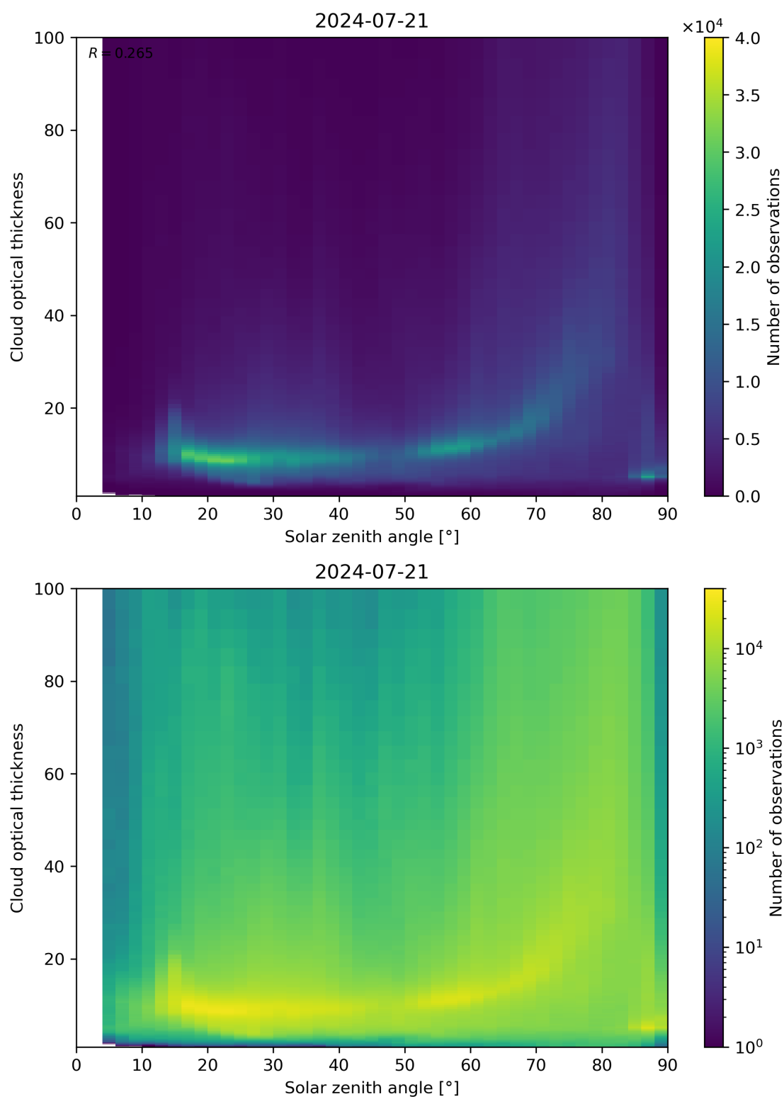
Figure 103: Scatter density plot of “Solar zenith angle” against “Cloud optical thickness” for 2024-07-21 to 2024-07-22.
