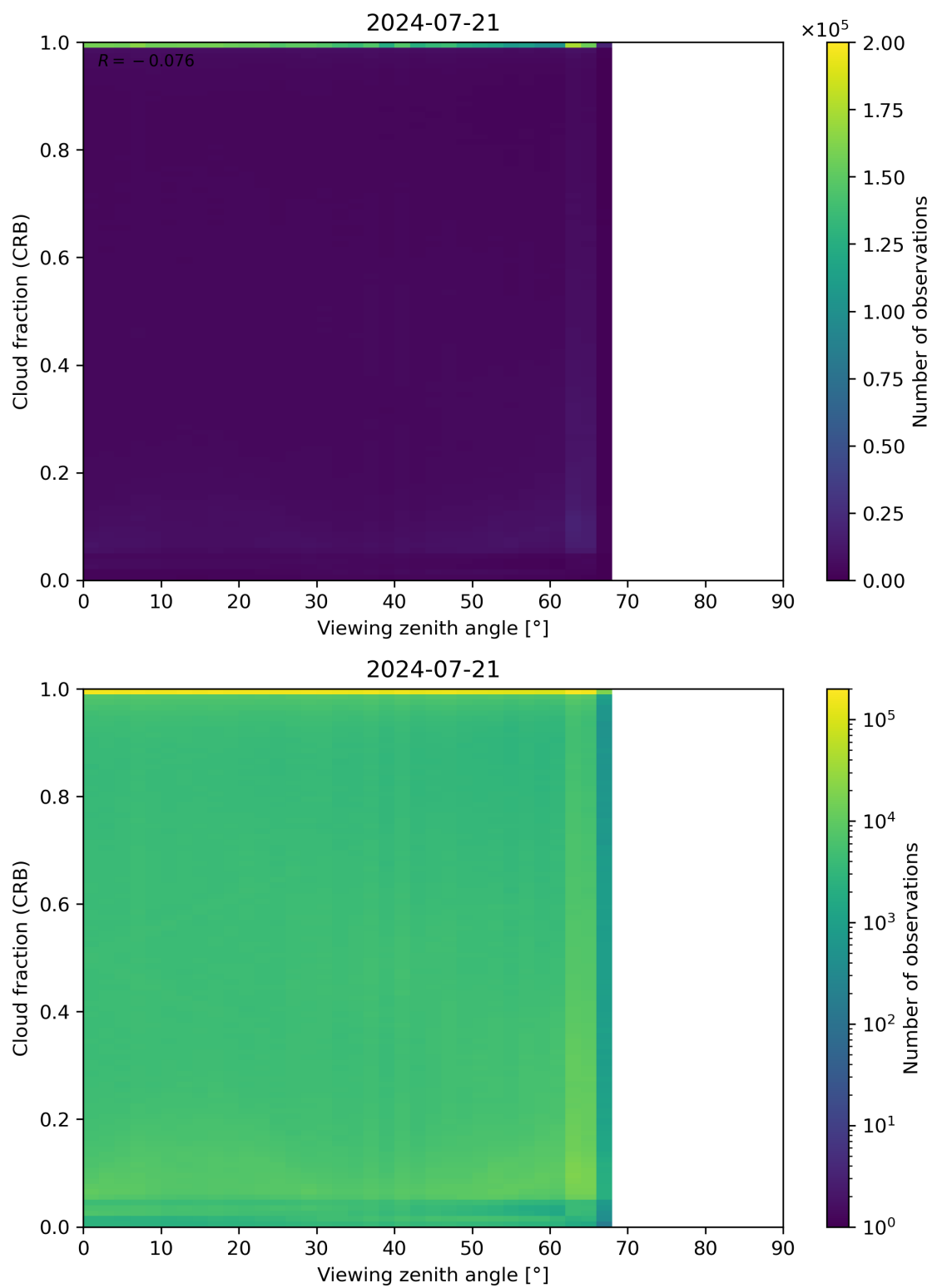
Figure 109: Scatter density plot of “Viewing zenith angle” against “Cloud fraction (CRB)” for 2024-07-21 to 2024-07-22.
