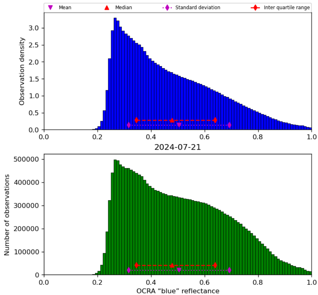
Figure 51: Histogram of “OCRA “blue” reflectance” for 2024-07-21 to 2024-07-22
