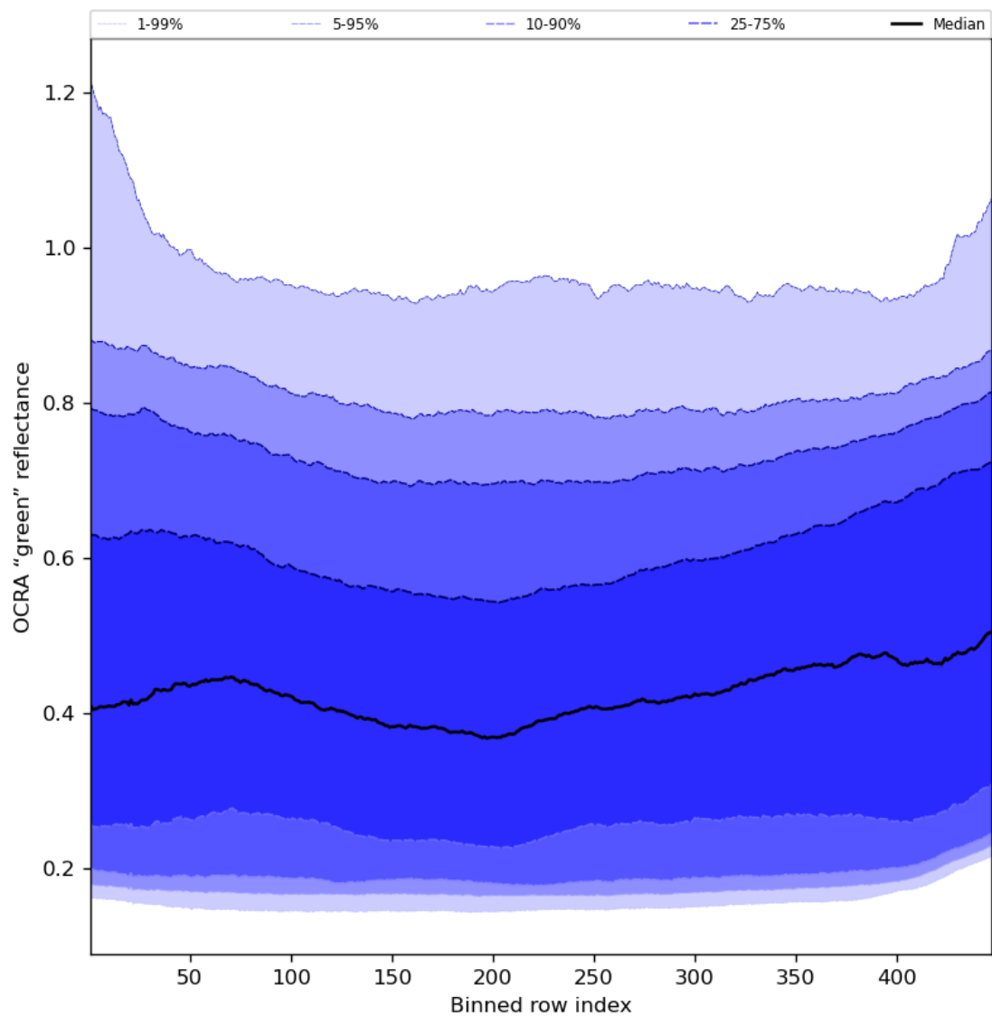
Figure 68: Along track statistics of “OCRA “green” reflectance” for 2024-07-21 to 2024-07-22
