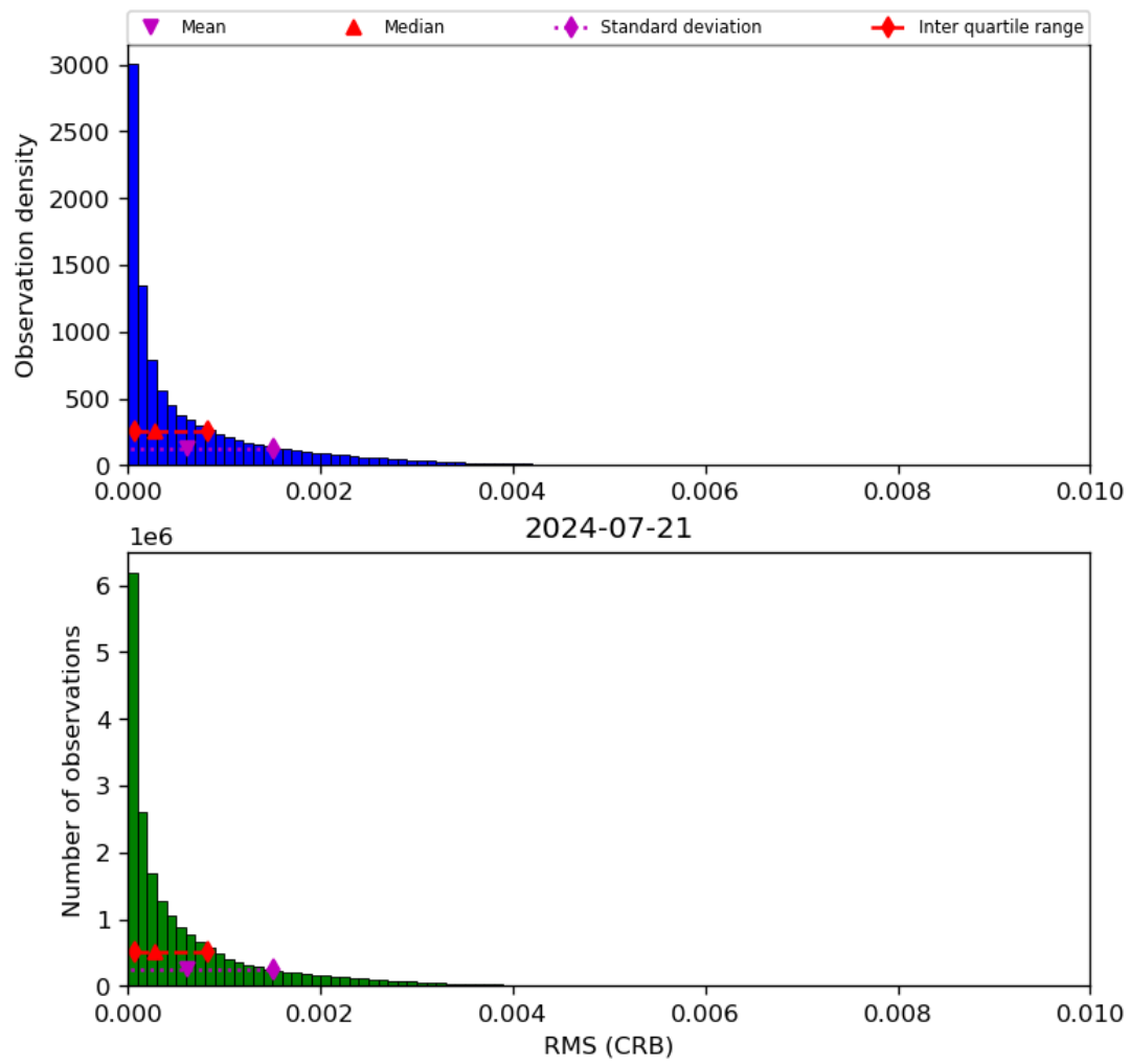
Figure 48: Histogram of “RMS (CRB)” for 2024-07-21 to 2024-07-22
