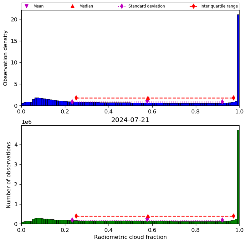
Figure 39: Histogram of “Radiometric cloud fraction” for 2024-07-21 to 2024-07-22
