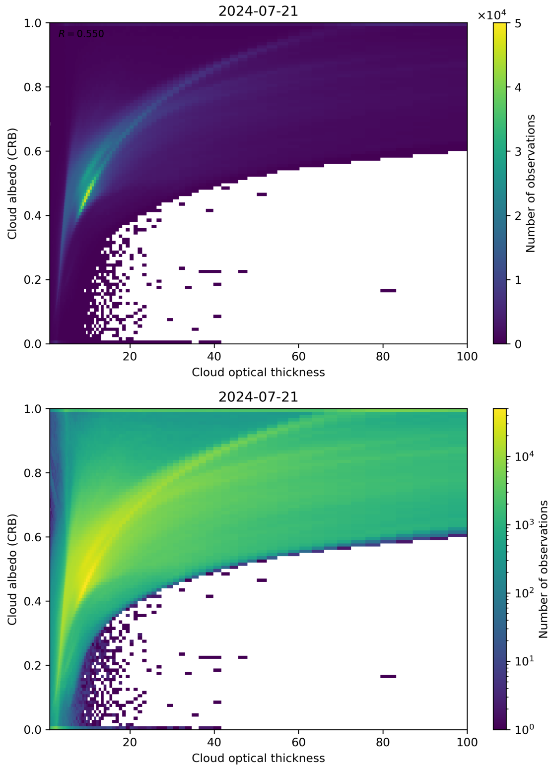
Figure 82: Scatter density plot of “Cloud optical thickness” against “Cloud albedo (CRB)” for 2024-07-21 to 2024-07-22.
