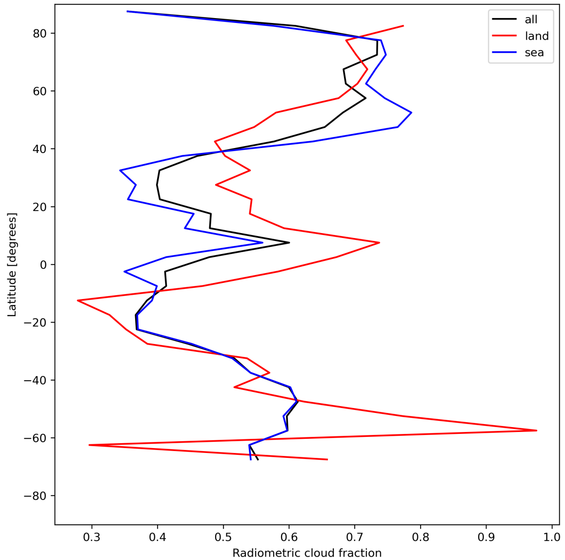
Figure 23: Zonal average of “Radiometric cloud fraction” for 2024-07-21 to 2024-07-22.
