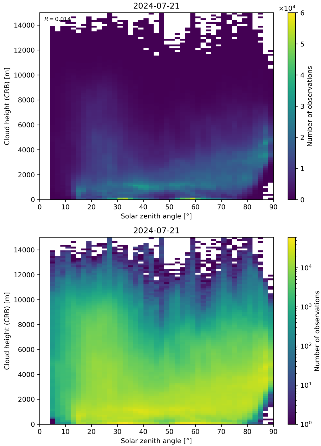
Figure 102: Scatter density plot of “Solar zenith angle” against “Cloud height (CRB)” for 2024-07-21 to 2024-07-22.
