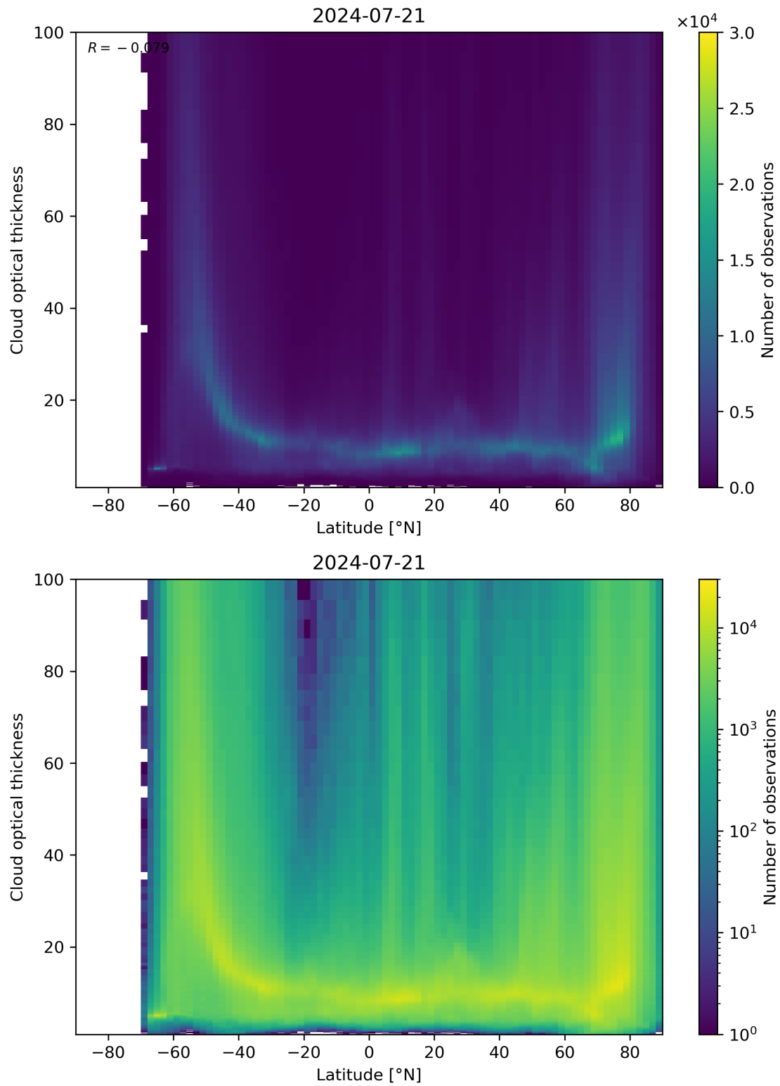
Figure 96: Scatter density plot of “Latitude” against “Cloud optical thickness” for 2024-07-21 to 2024-07-22.
