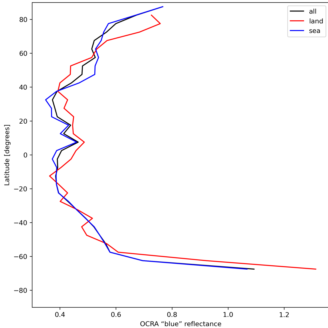
Figure 35: Zonal average of “OCRA “blue” reflectance” for 2024-07-21 to 2024-07-22.
