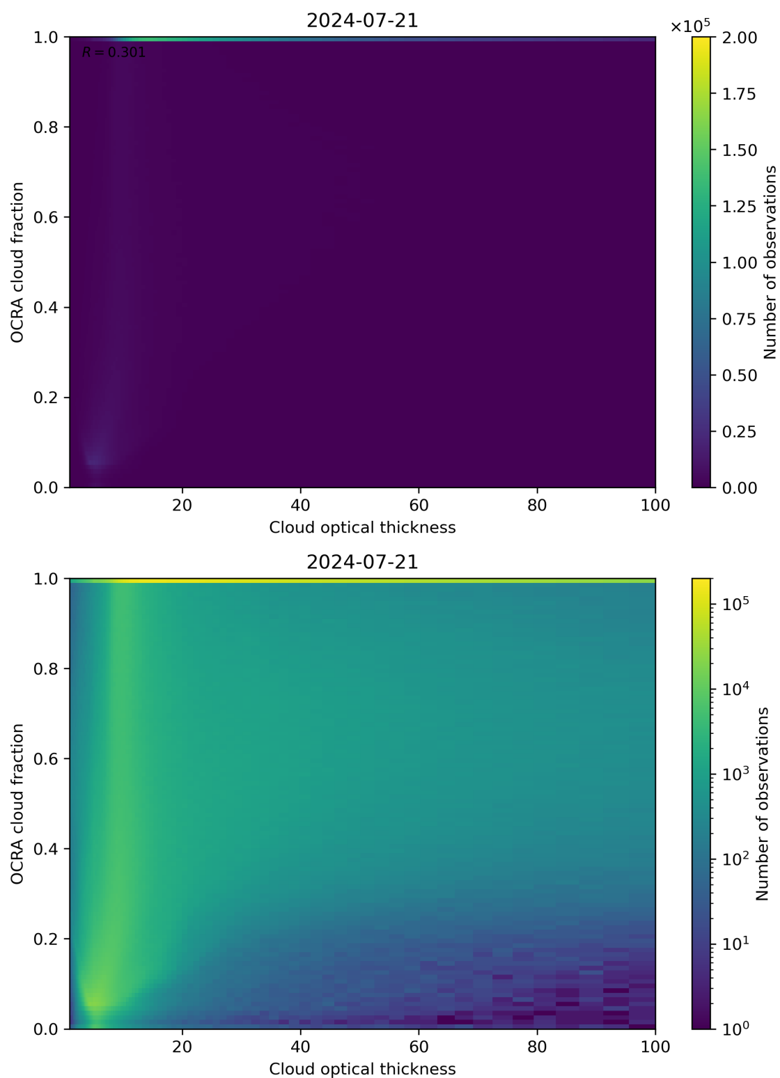
Figure 83: Scatter density plot of “Cloud optical thickness” against “OCRA cloud fraction” for 2024-07-21 to 2024-07-22.
