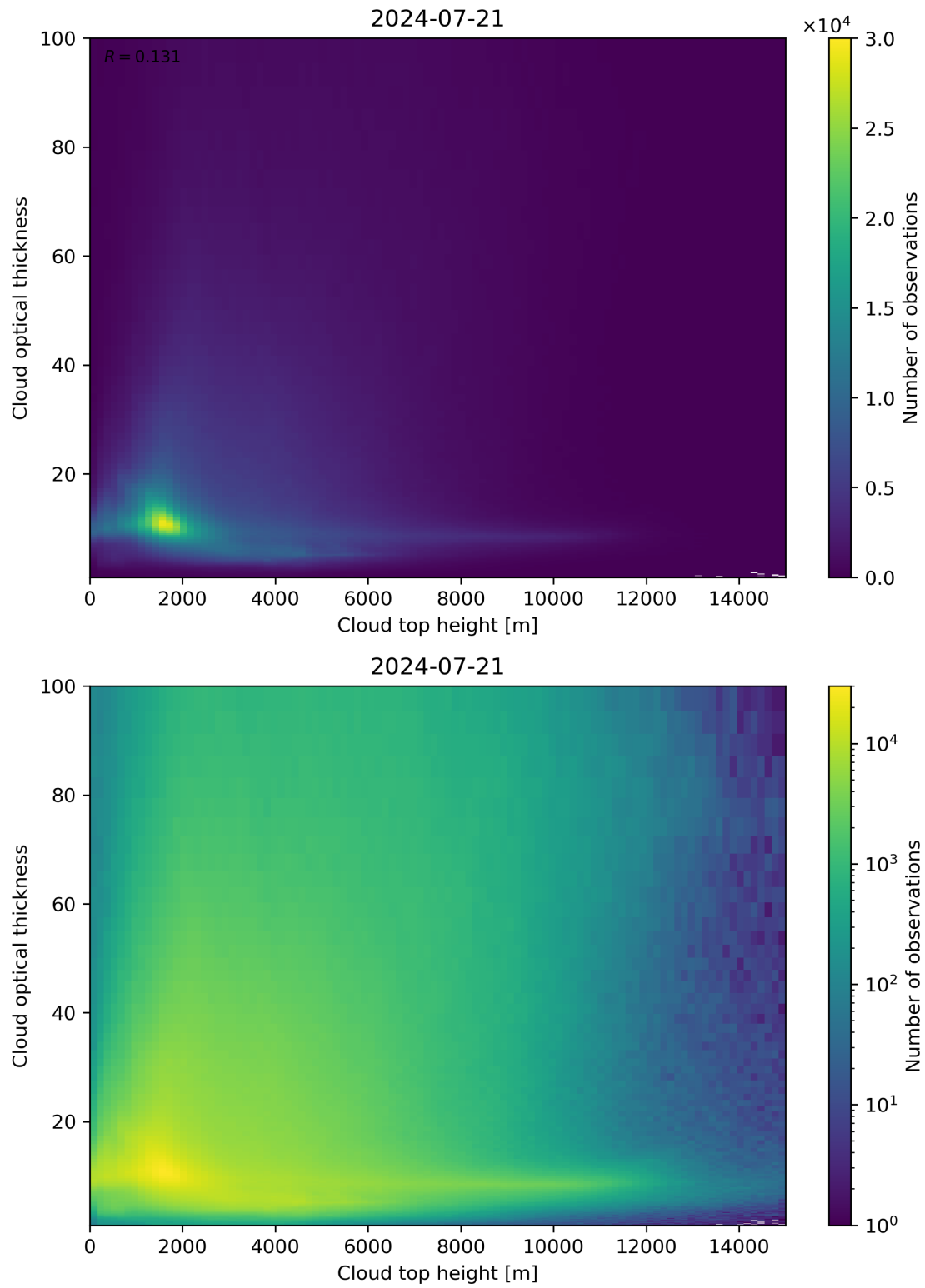
Figure 90: Scatter density plot of “Cloud top height” against “Cloud optical thickness” for 2024-07-21 to 2024-07-22.
