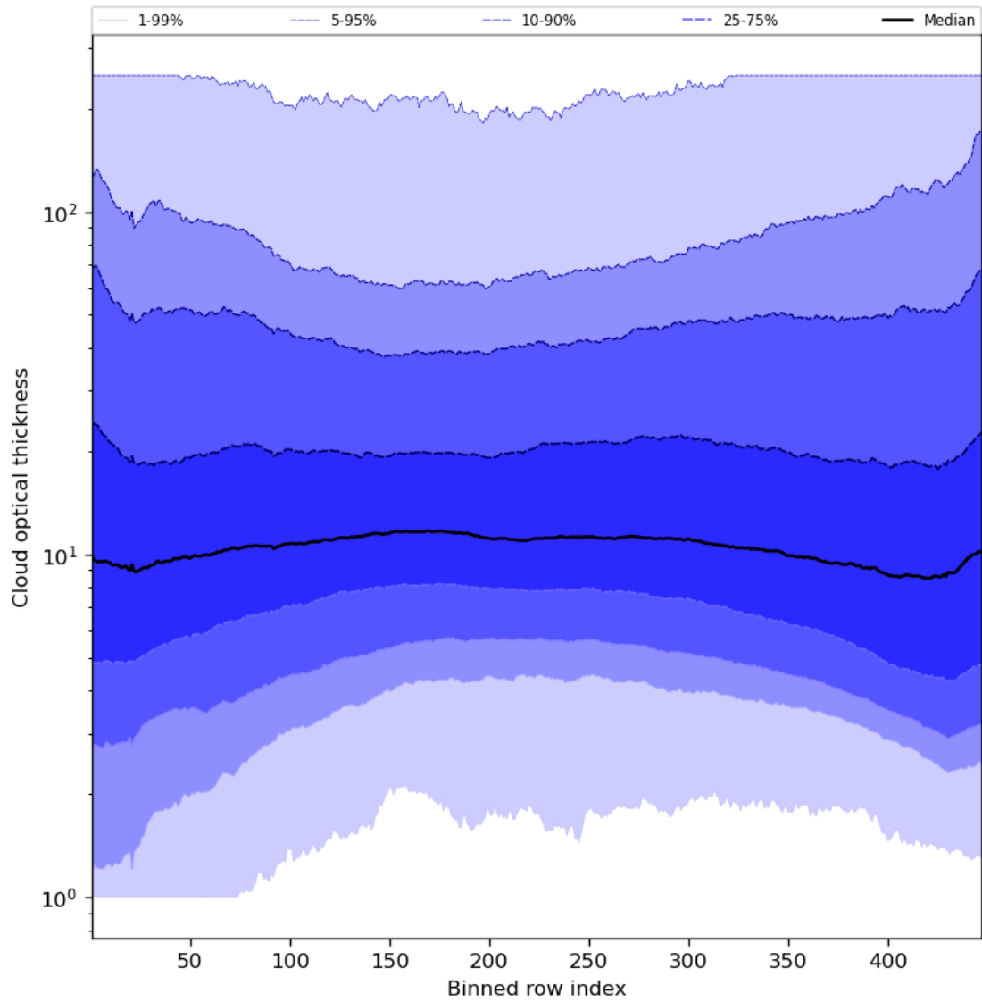
Figure 57: Along track statistics of “Cloud optical thickness” for 2024-07-21 to 2024-07-22
