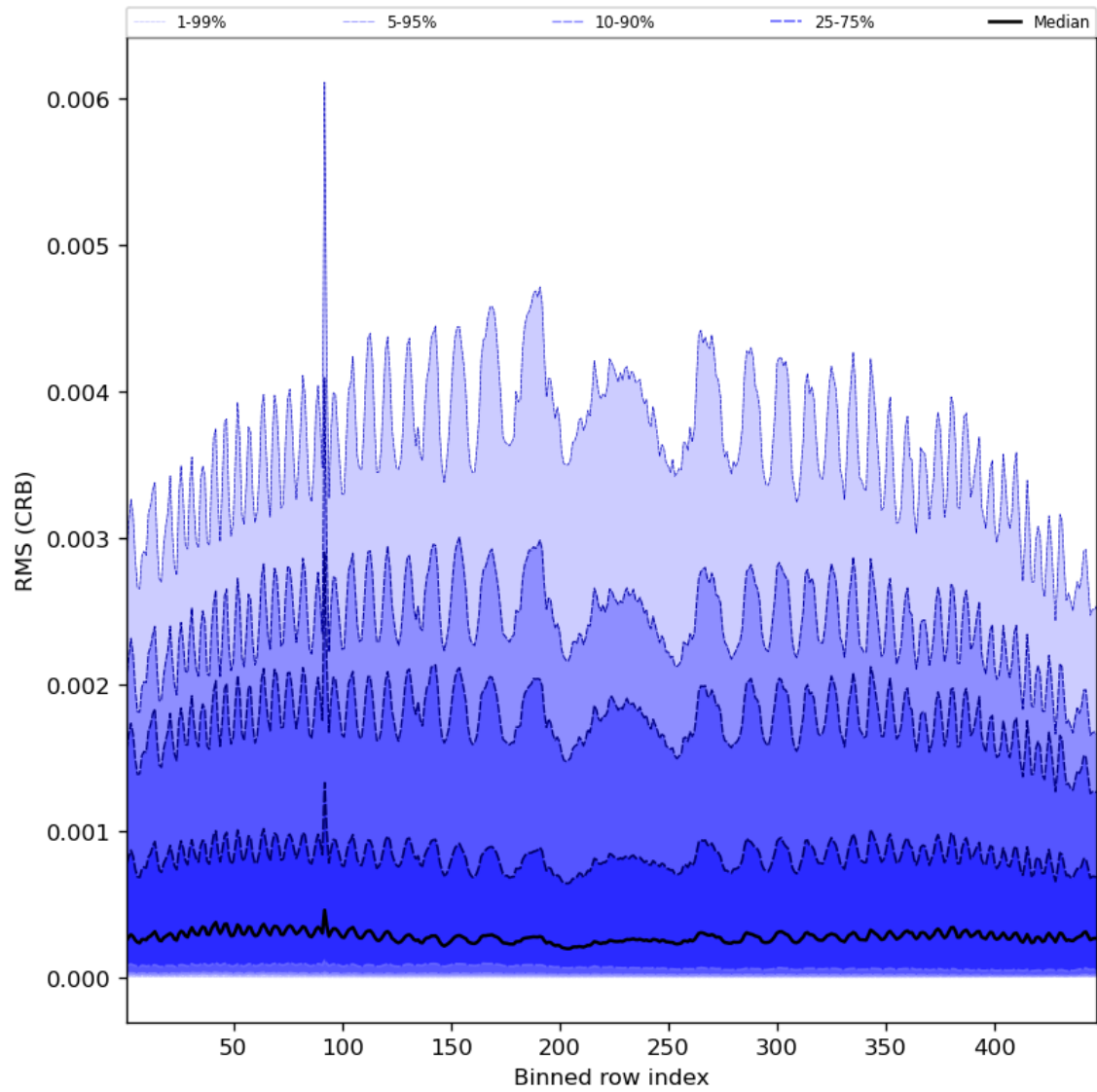
Figure 64: Along track statistics of "RMS (CRB)" for 2024-07-21 to 2024-07-22
