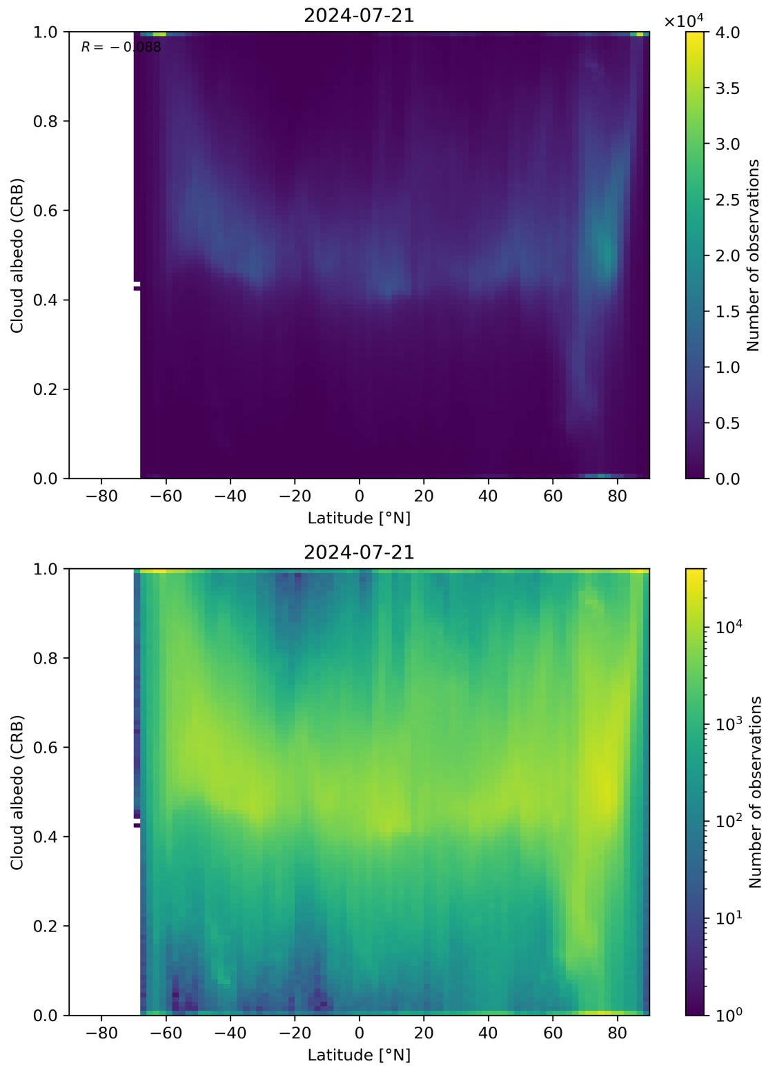
Figure 91: Scatter density plot of “Latitude” against “Cloud albedo (CRB)” for 2024-07-21 to 2024-07-22.
