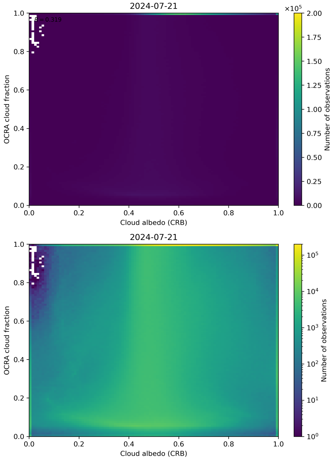
Figure 70: Scatter density plot of “Cloud albedo (CRB)” against “OCRA cloud fraction” for 2024-07-21 to 2024-07-22.
