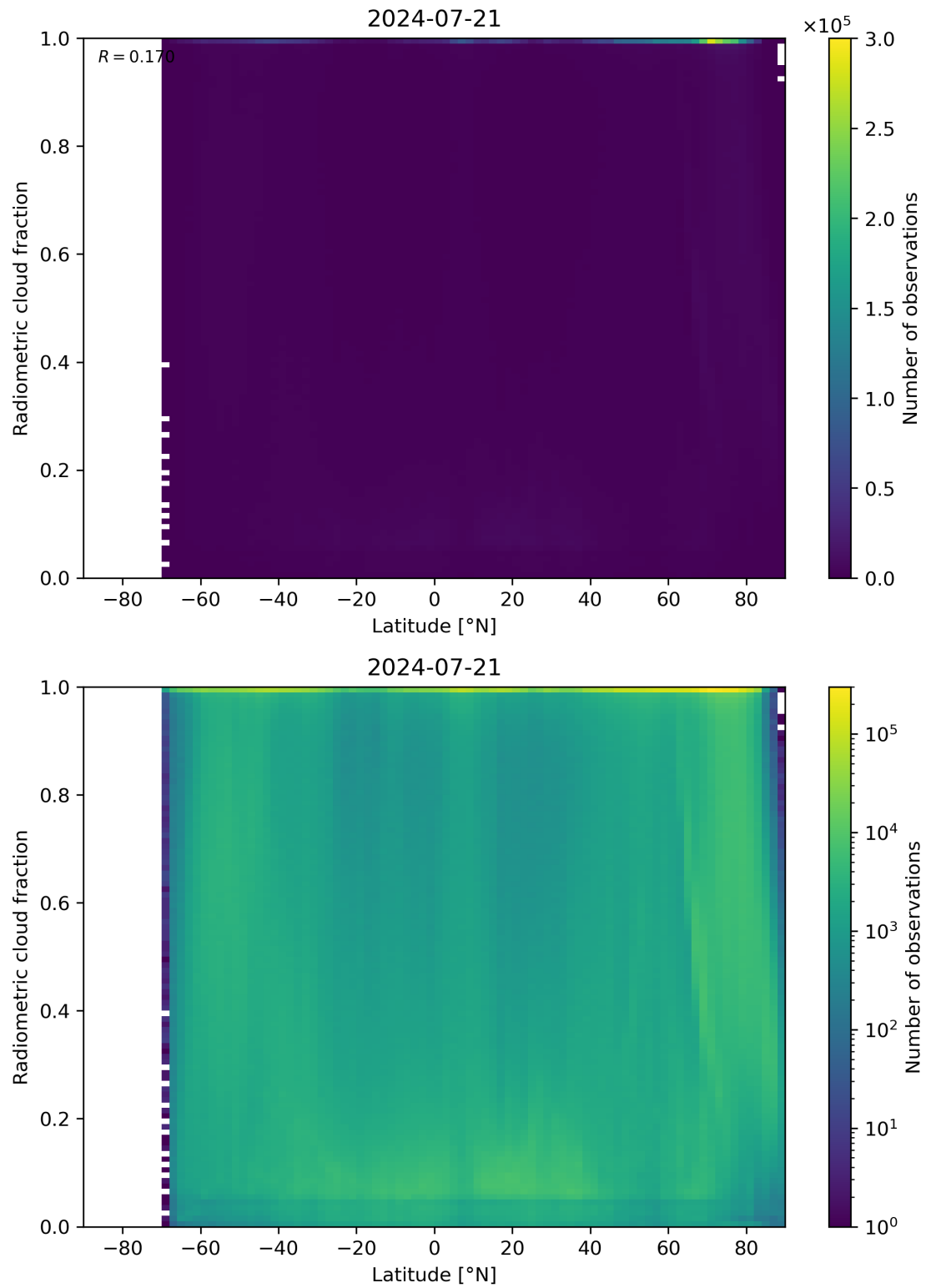
Figure 92: Scatter density plot of “Latitude” against “Radiometric cloud fraction” for 2024-07-21 to 2024-07-22.
