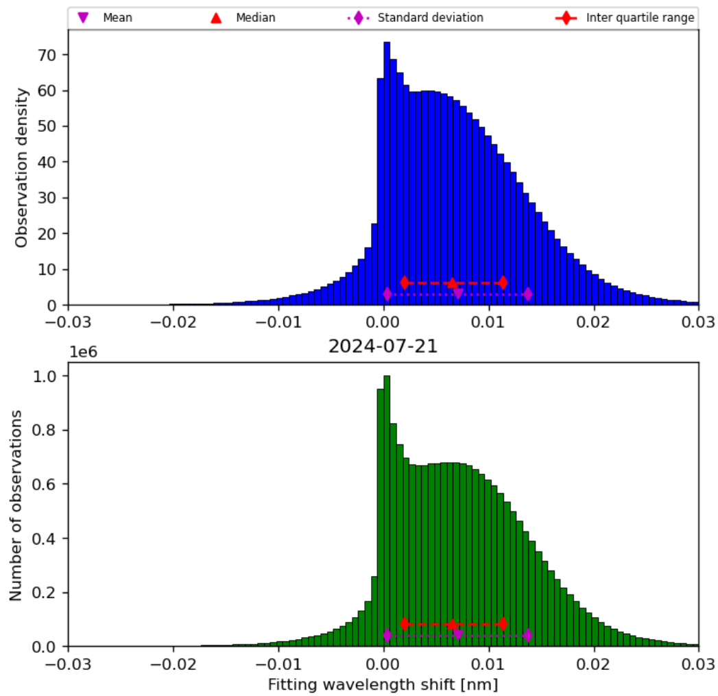
Figure 49: Histogram of “Fitting wavelength shift” for 2024-07-21 to 2024-07-22
