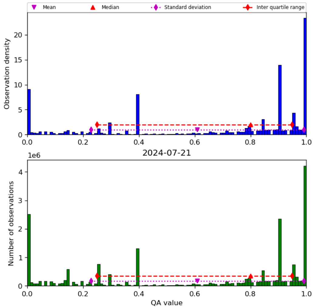
Figure 38: Histogram of “QA value” for 2024-07-21 to 2024-07-22
