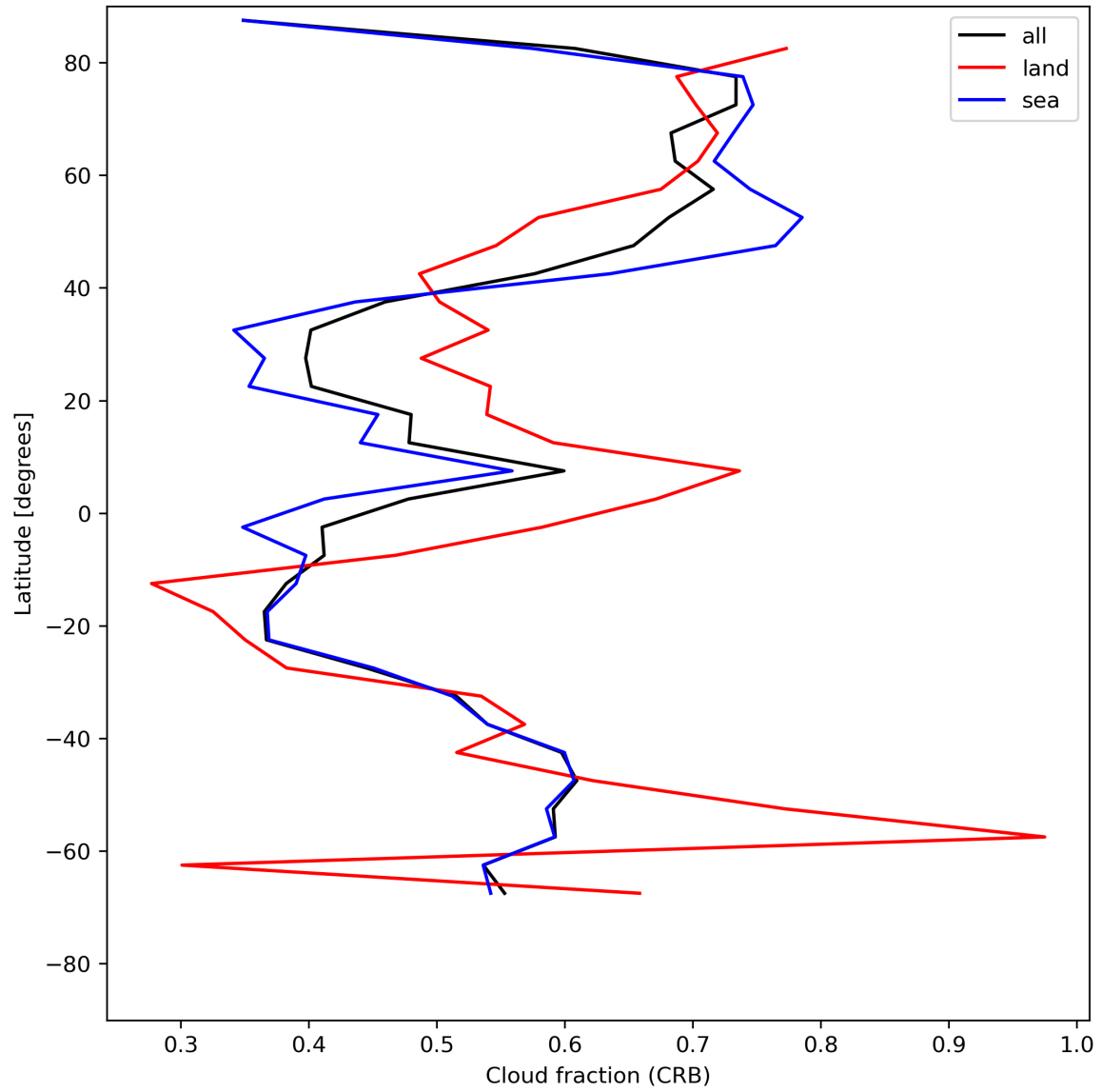
Figure 26: Zonal average of “Cloud fraction (CRB)” for 2024-07-21 to 2024-07-22.
