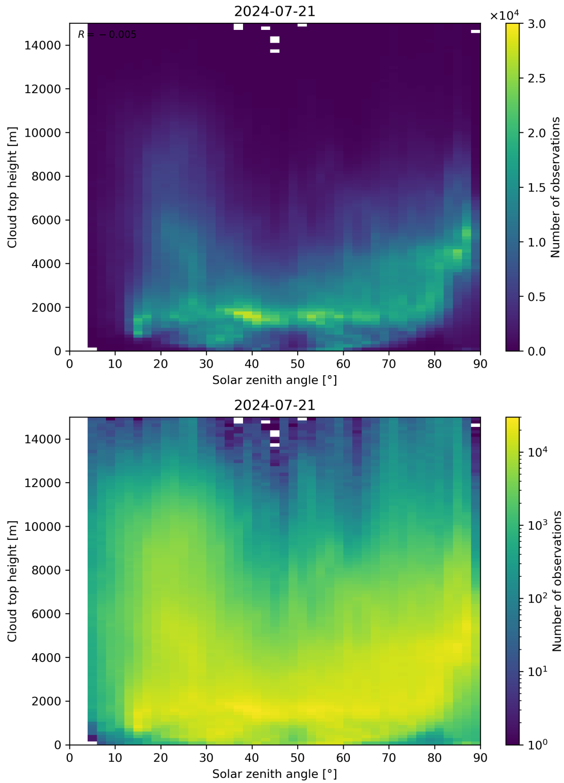
Figure 104: Scatter density plot of “Solar zenith angle” against “Cloud top height” for 2024-07-21 to 2024-07-22.
