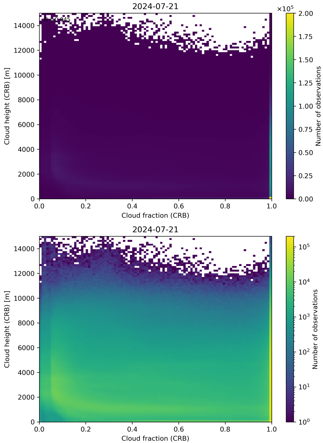
Figure 79: Scatter density plot of “Cloud fraction (CRB)” against “Cloud height (CRB)” for 2024-07-21 to 2024-07-22.
