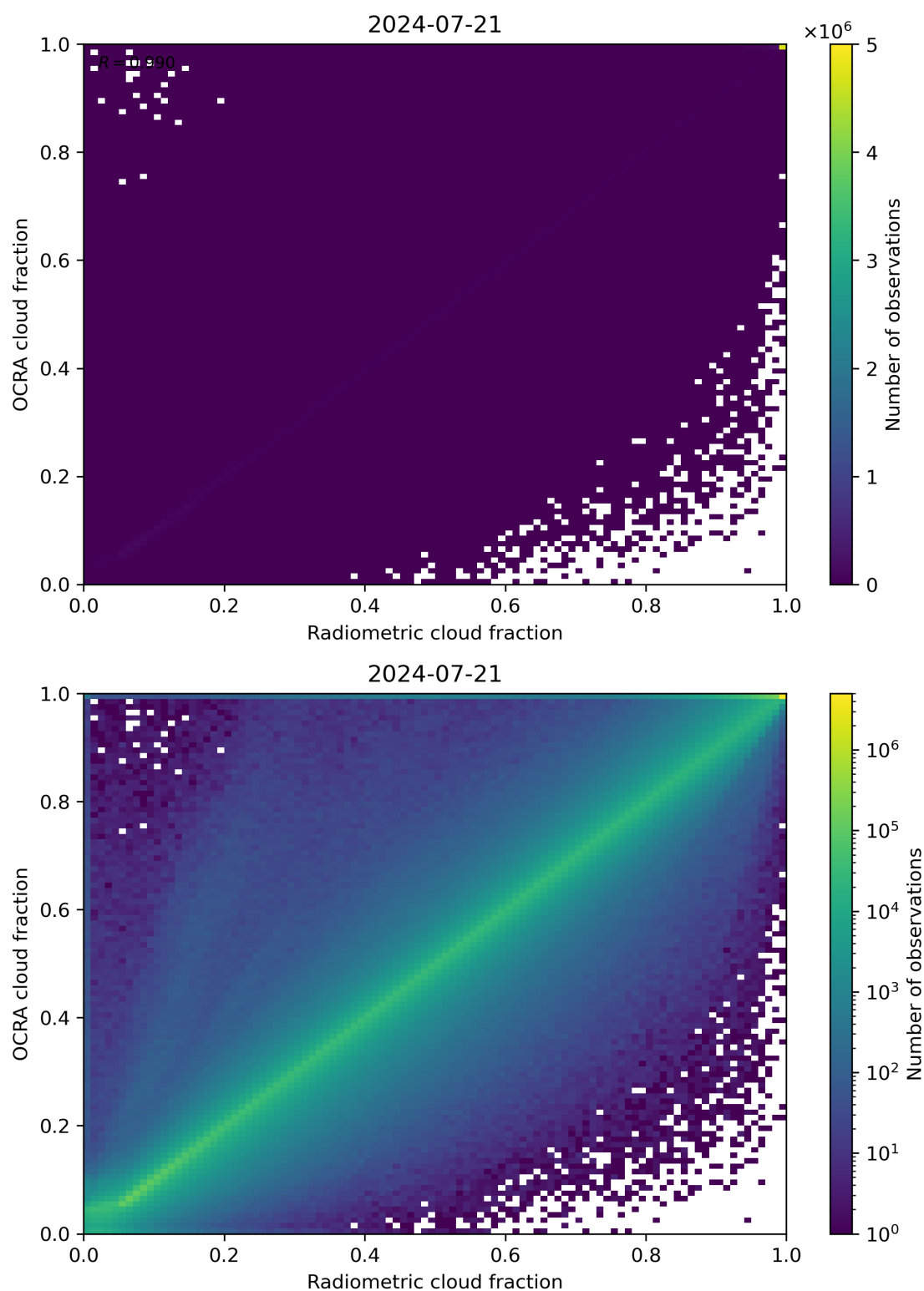
Figure 72: Scatter density plot of “Radiometric cloud fraction” against “OCRA cloud fraction” for 2024-07-21 to 2024-07-22.
