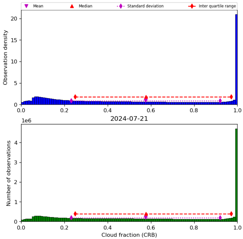
Figure 42: Histogram of “Cloud fraction (CRB)” for 2024-07-21 to 2024-07-22
