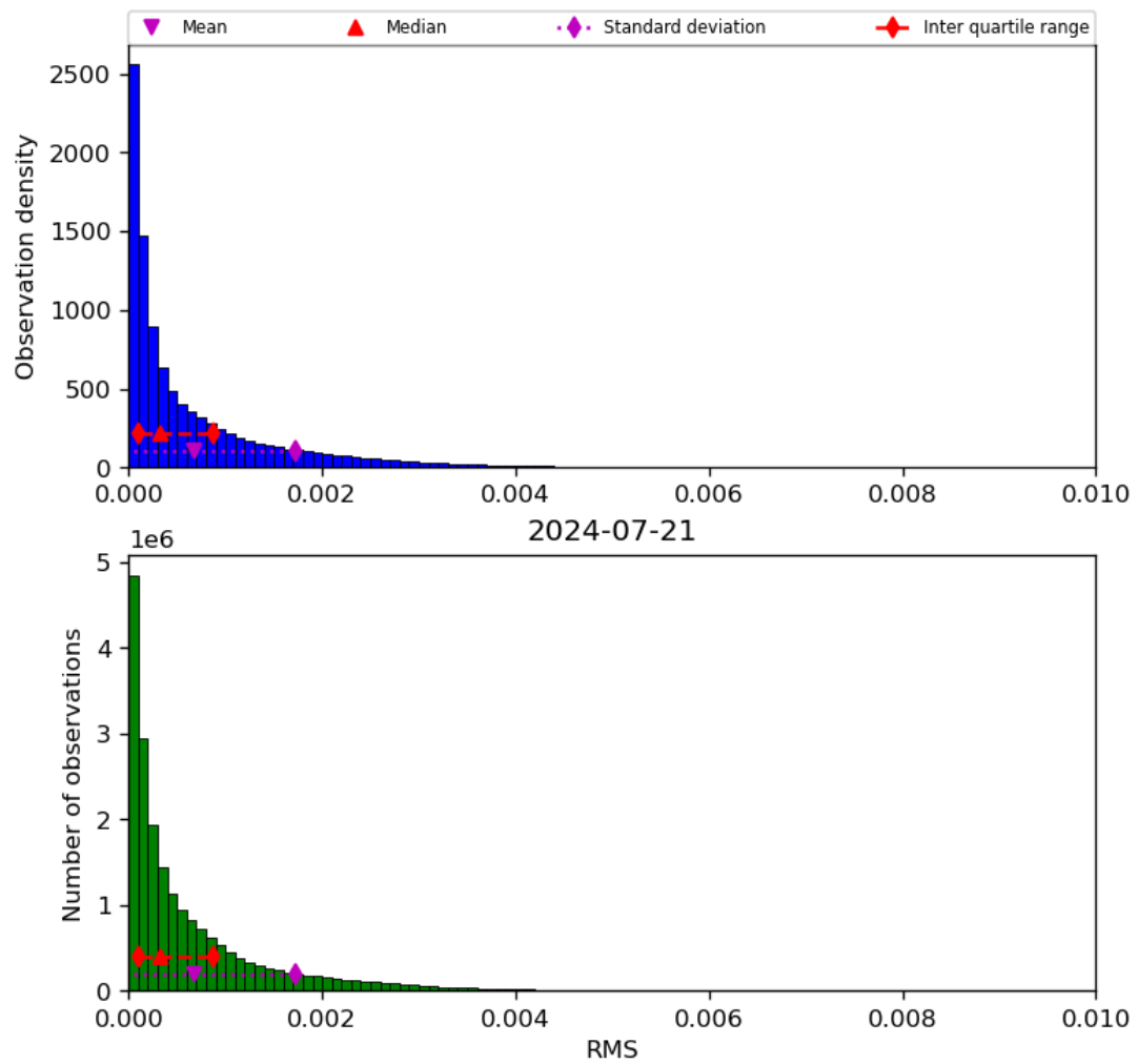
Figure 47: Histogram of “RMS” for 2024-07-21 to 2024-07-22
