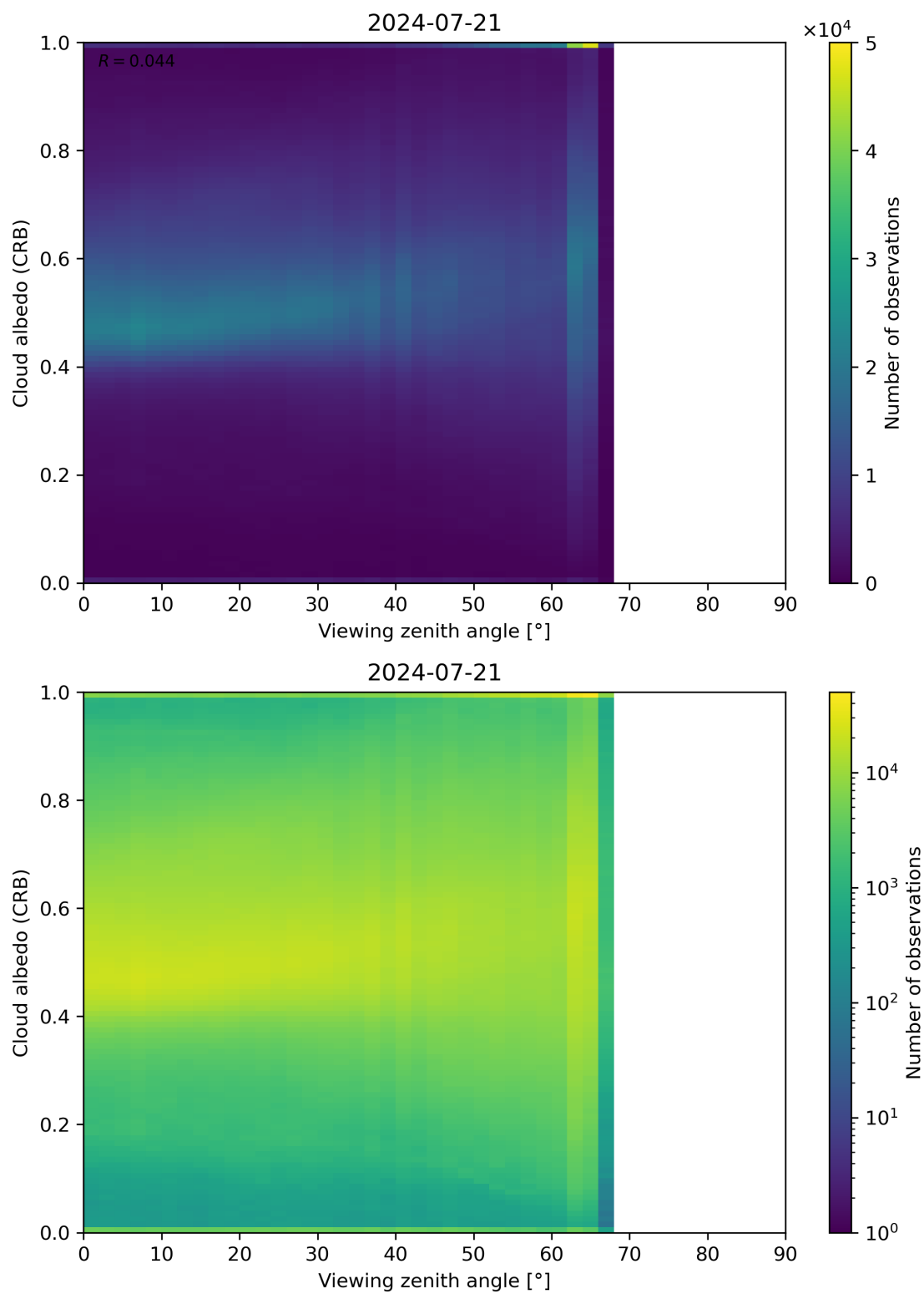
Figure 106: Scatter density plot of “Viewing zenith angle” against “Cloud albedo (CRB)” for 2024-07-21 to 2024-07-22.
