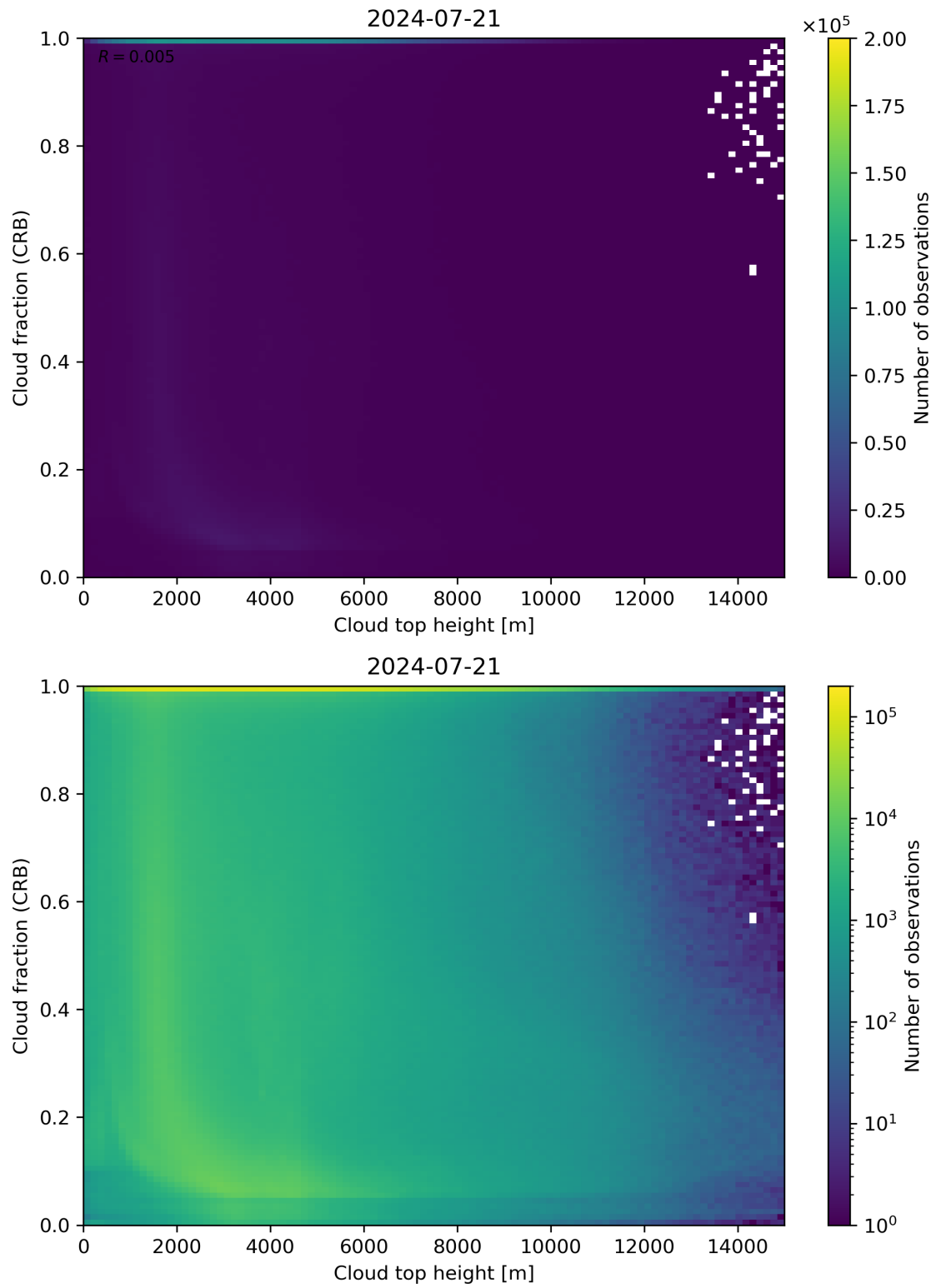
Figure 88: Scatter density plot of “Cloud top height” against “Cloud fraction (CRB)” for 2024-07-21 to 2024-07-22.
