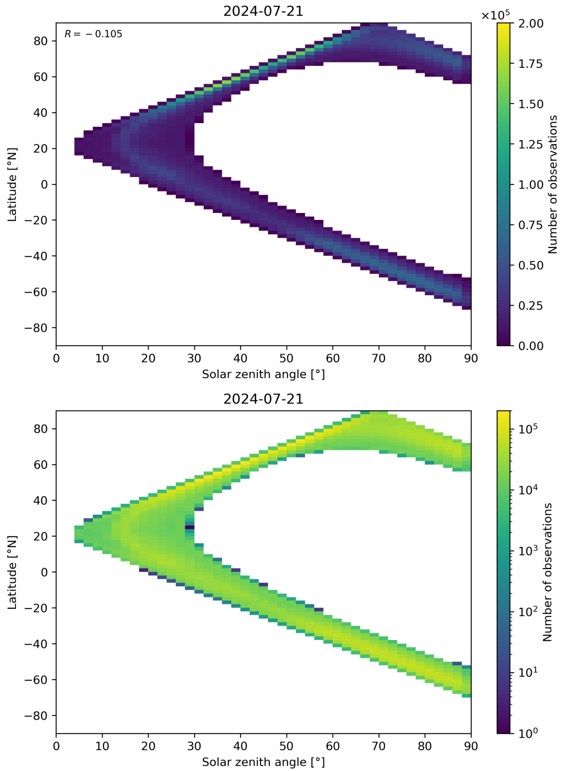
Figure 105: Scatter density plot of “Solar zenith angle” against “Latitude” for 2024-07-21 to 2024-07-22.
