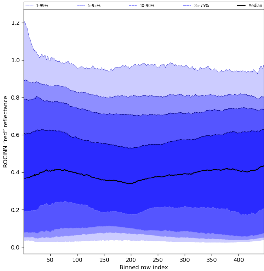
Figure 69: Along track statistics of "ROCINN "red" reflectance" for 2024-07-21 to 2024-07-22
