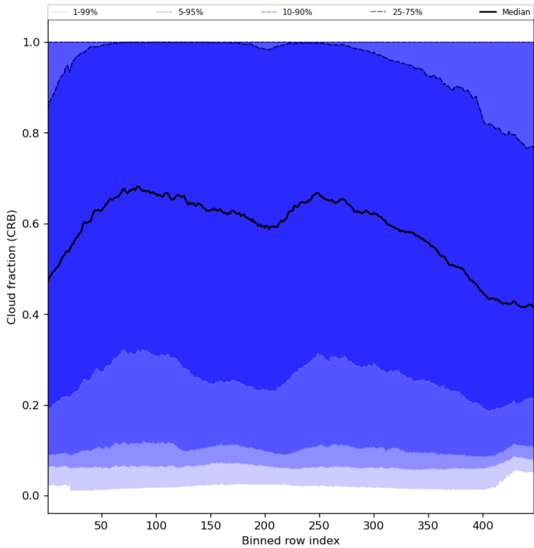
Figure 58: Along track statistics of “Cloud fraction (CRB)” for 2024-07-21 to 2024-07-22
