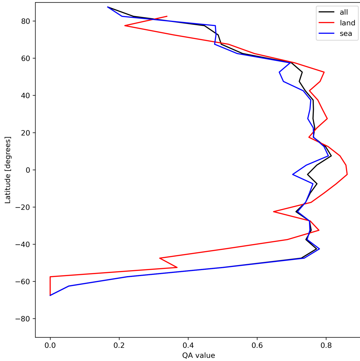
Figure 22: Zonal average of “QA value” for 2024-07-21 to 2024-07-22.
