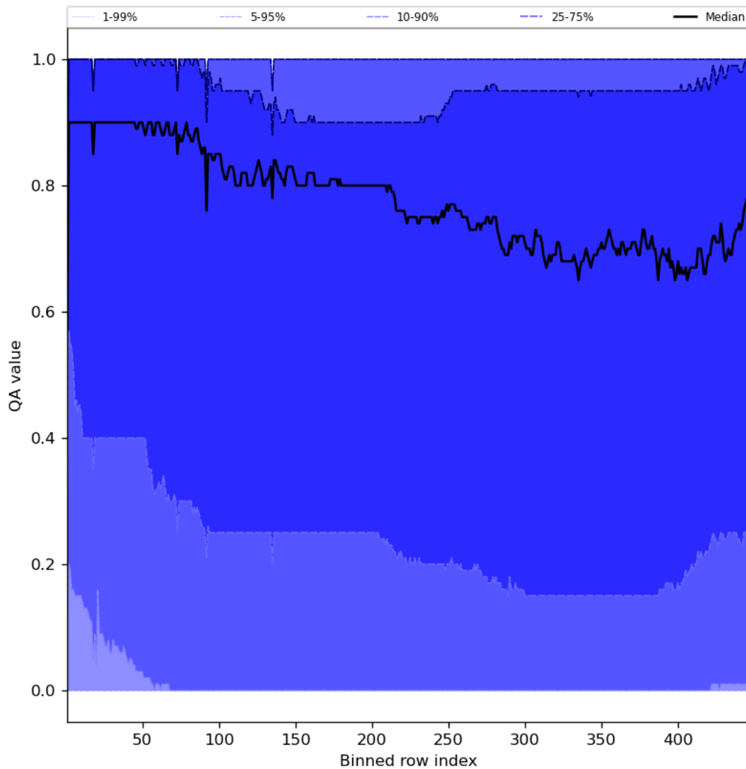
Figure 54: Along track statistics of “QA value” for 2024-07-21 to 2024-07-22
