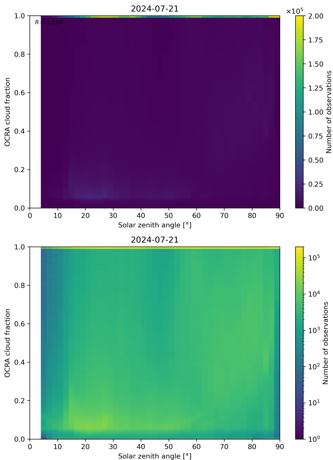
Figure 100: Scatter density plot of “Solar zenith angle” against “OCRA cloud fraction” for 2024-07-21 to 2024-07-22.
