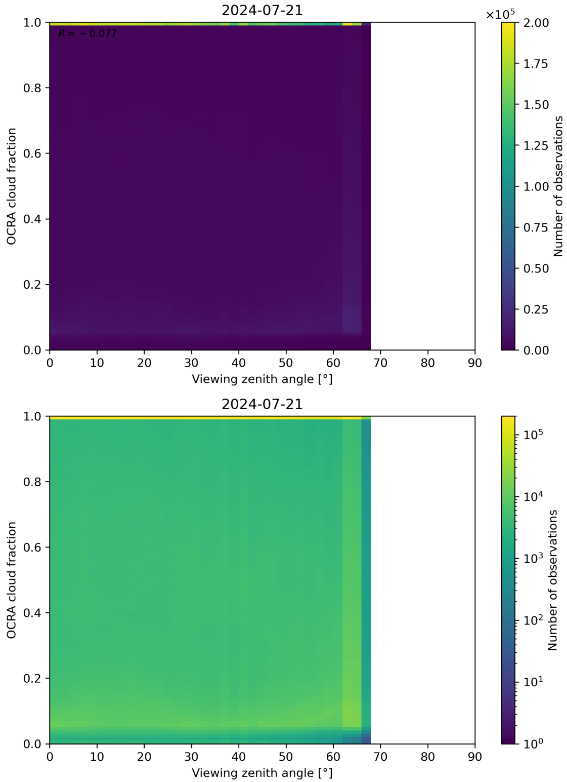
Figure 108: Scatter density plot of “Viewing zenith angle” against “OCRA cloud fraction” for 2024-07-21 to 2024-07-22.
