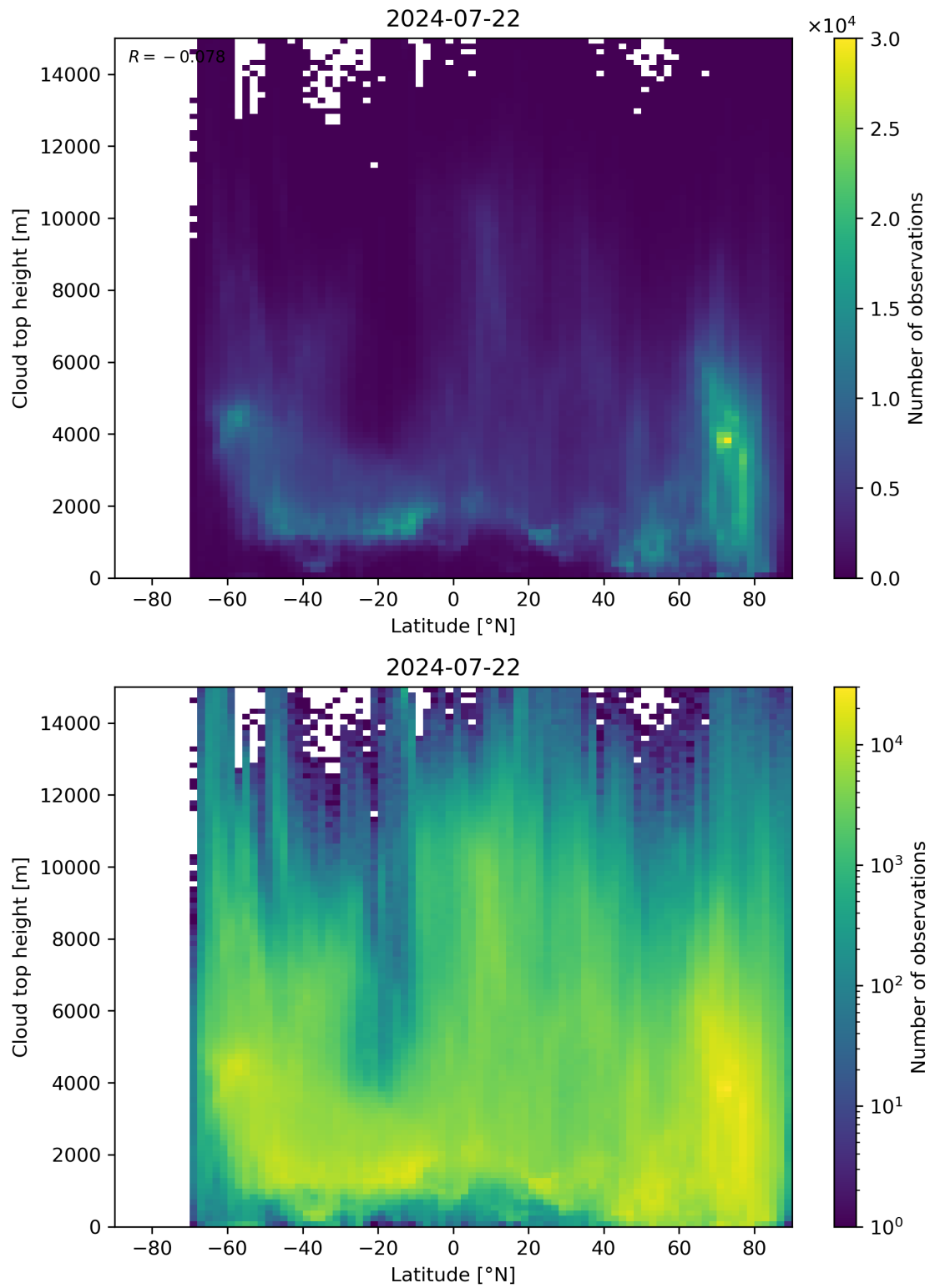
Figure 97: Scatter density plot of “Latitude” against “Cloud top height” for 2024-07-21 to 2024-07-23.
