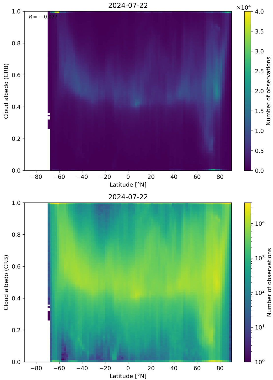
Figure 91: Scatter density plot of “Latitude” against “Cloud albedo (CRB)” for 2024-07-21 to 2024-07-23.
