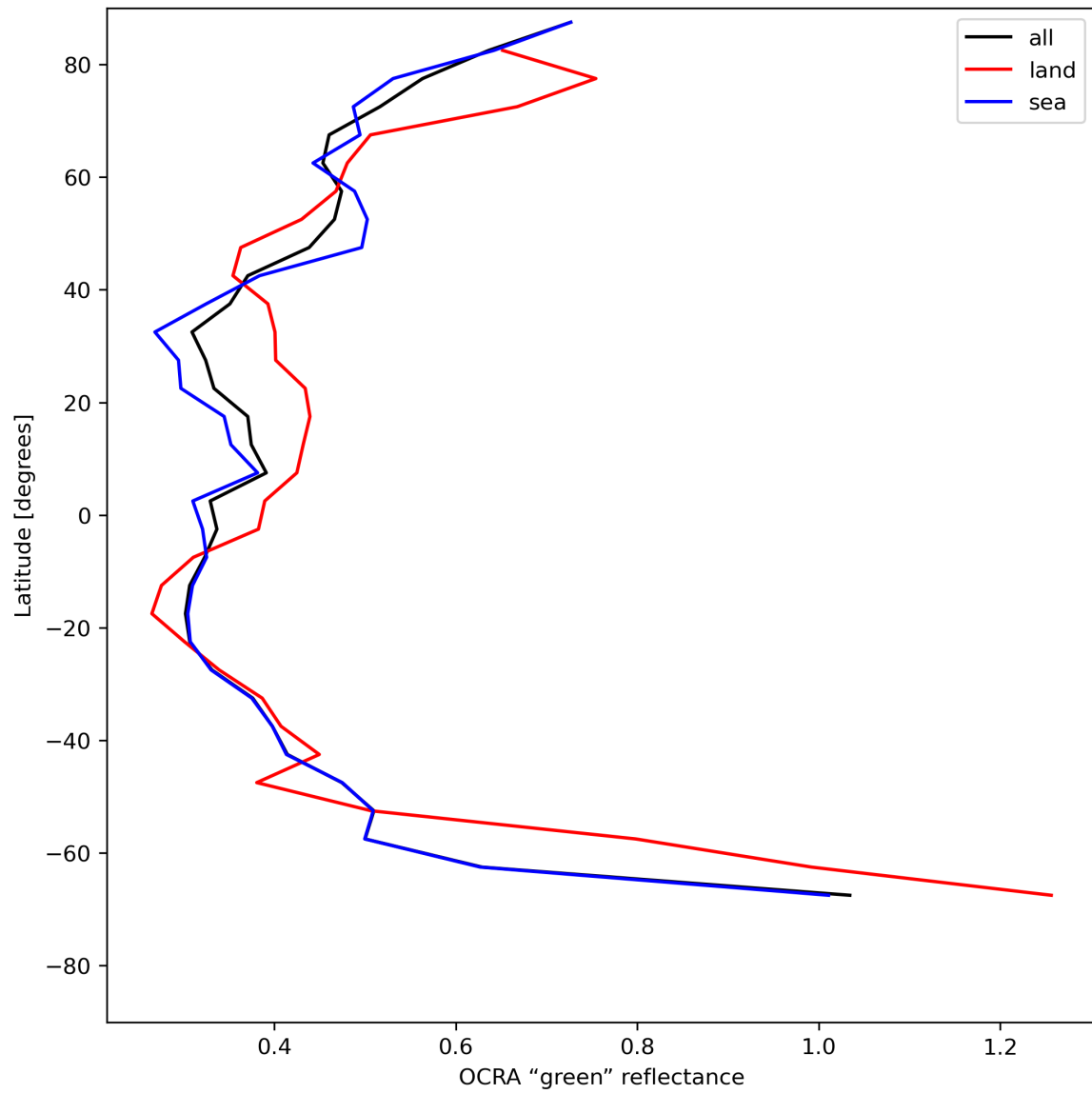
Figure 36: Zonal average of “OCRA “green” reflectance” for 2024-07-21 to 2024-07-23.
