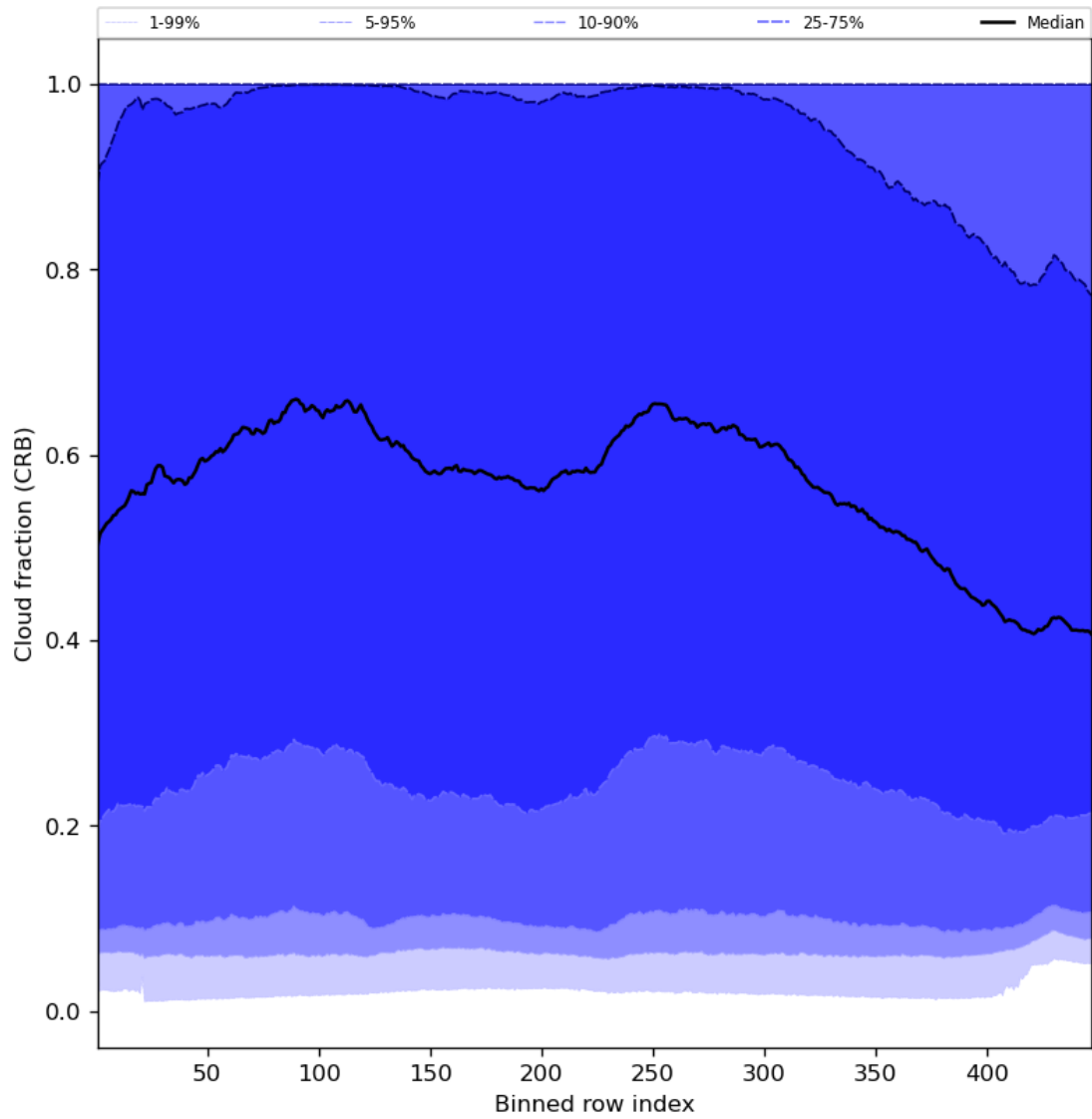
Figure 58: Along track statistics of “Cloud fraction (CRB)” for 2024-07-21 to 2024-07-23
