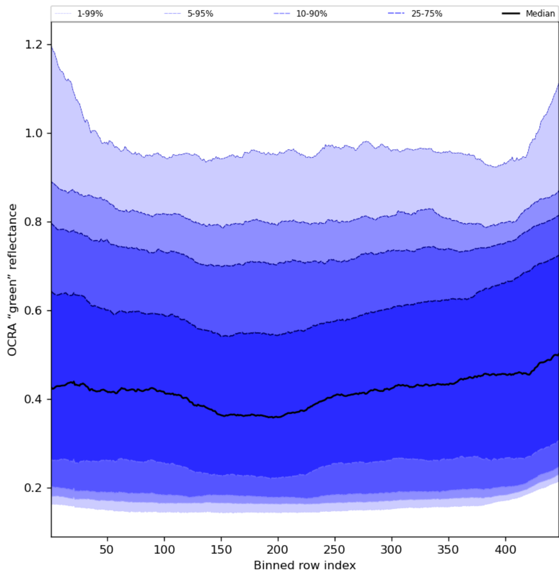
Figure 68: Along track statistics of “OCRA “green” reflectance” for 2024-07-21 to 2024-07-23
