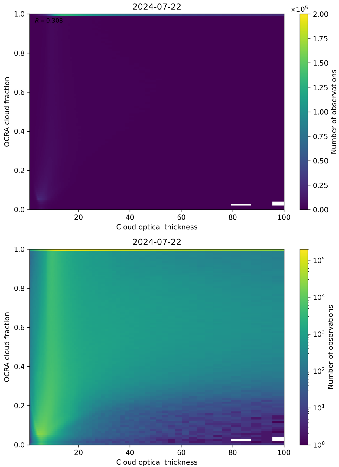
Figure 83: Scatter density plot of “Cloud optical thickness” against “OCRA cloud fraction” for 2024-07-21 to 2024-07-23.
