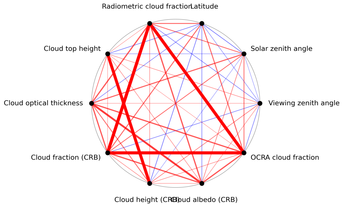
Figure 1: Map of correlation graph for 2024-07-21 to 2024-07-23.
