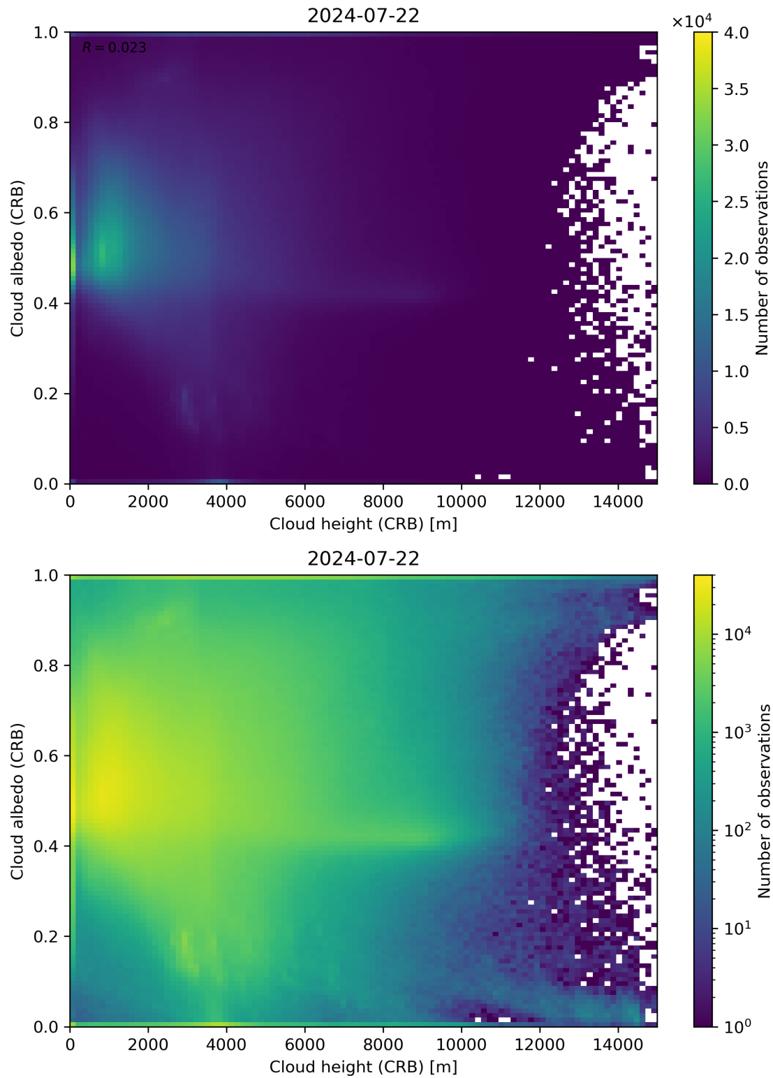
Figure 80: Scatter density plot of “Cloud height (CRB)” against “Cloud albedo (CRB)” for 2024-07-21 to 2024-07-23.
