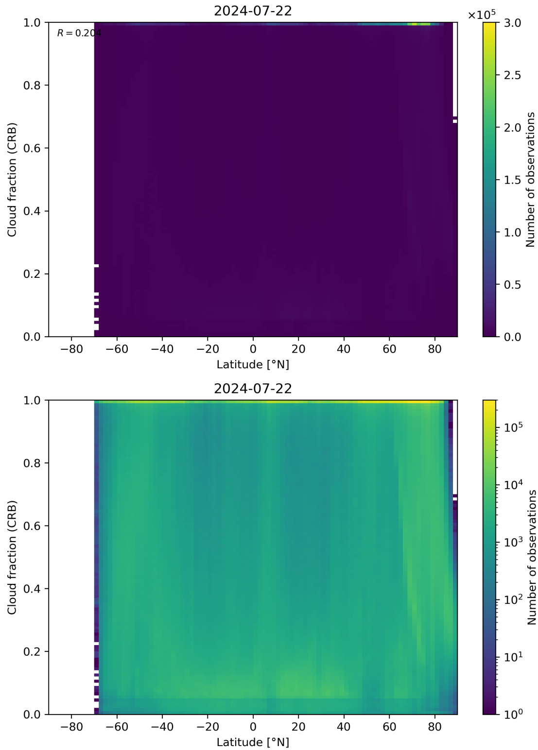
Figure 94: Scatter density plot of “Latitude” against “Cloud fraction (CRB)” for 2024-07-21 to 2024-07-23.
