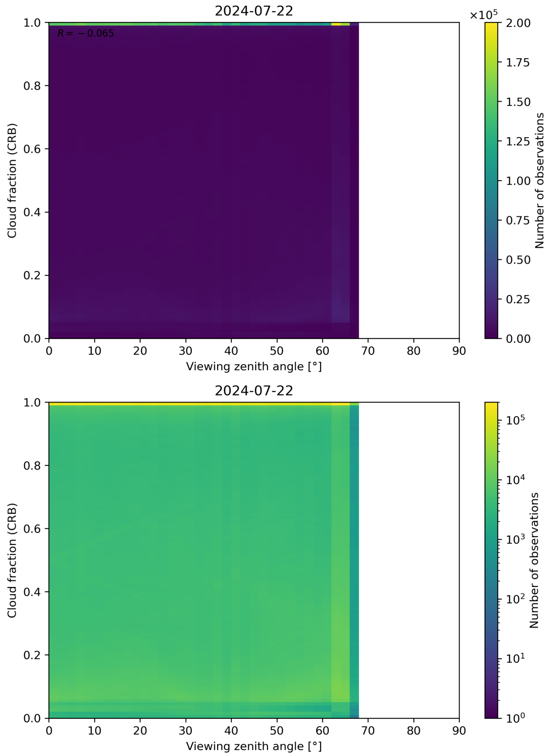
Figure 109: Scatter density plot of “Viewing zenith angle” against “Cloud fraction (CRB)” for 2024-07-21 to 2024-07-23.
