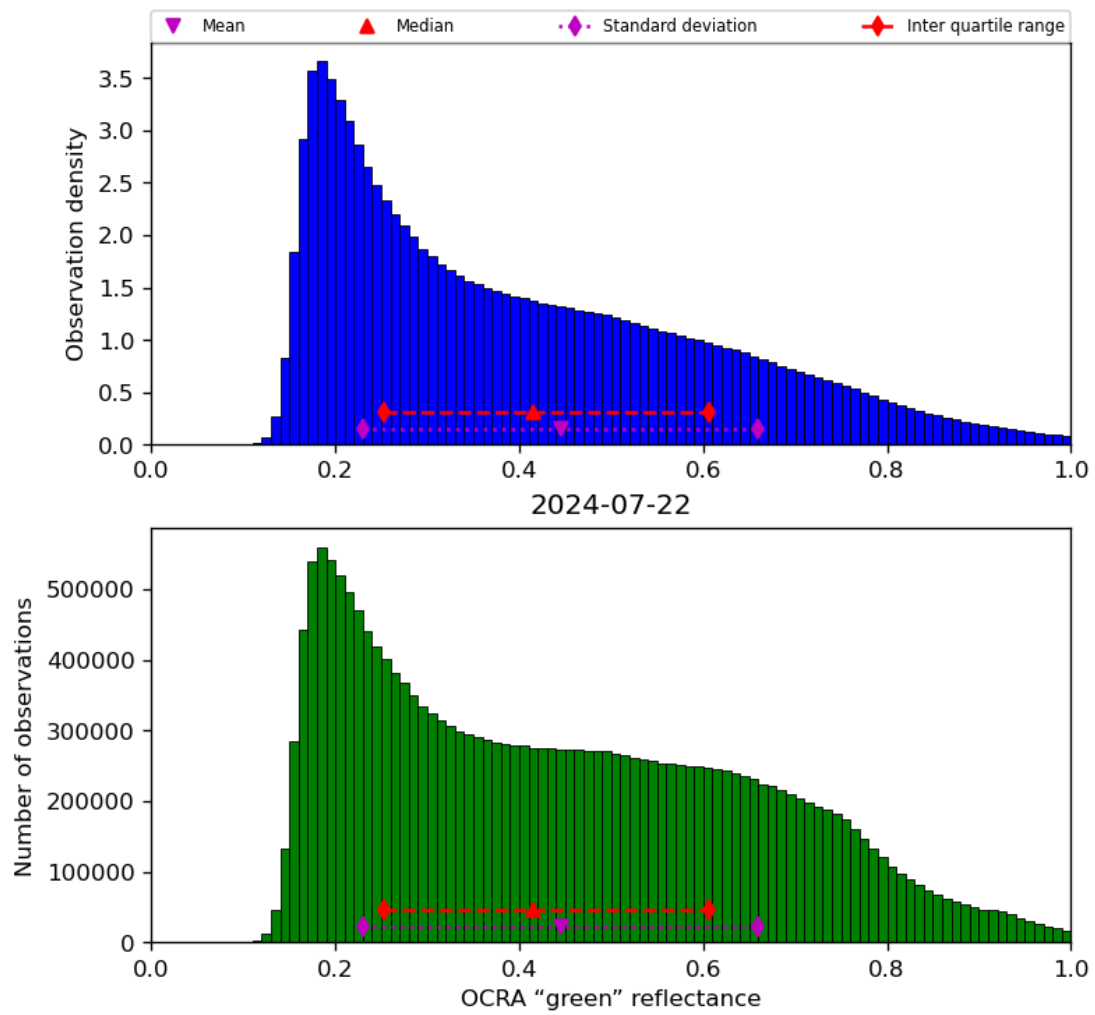
Figure 52: Histogram of “OCRA “green” reflectance” for 2024-07-21 to 2024-07-23
