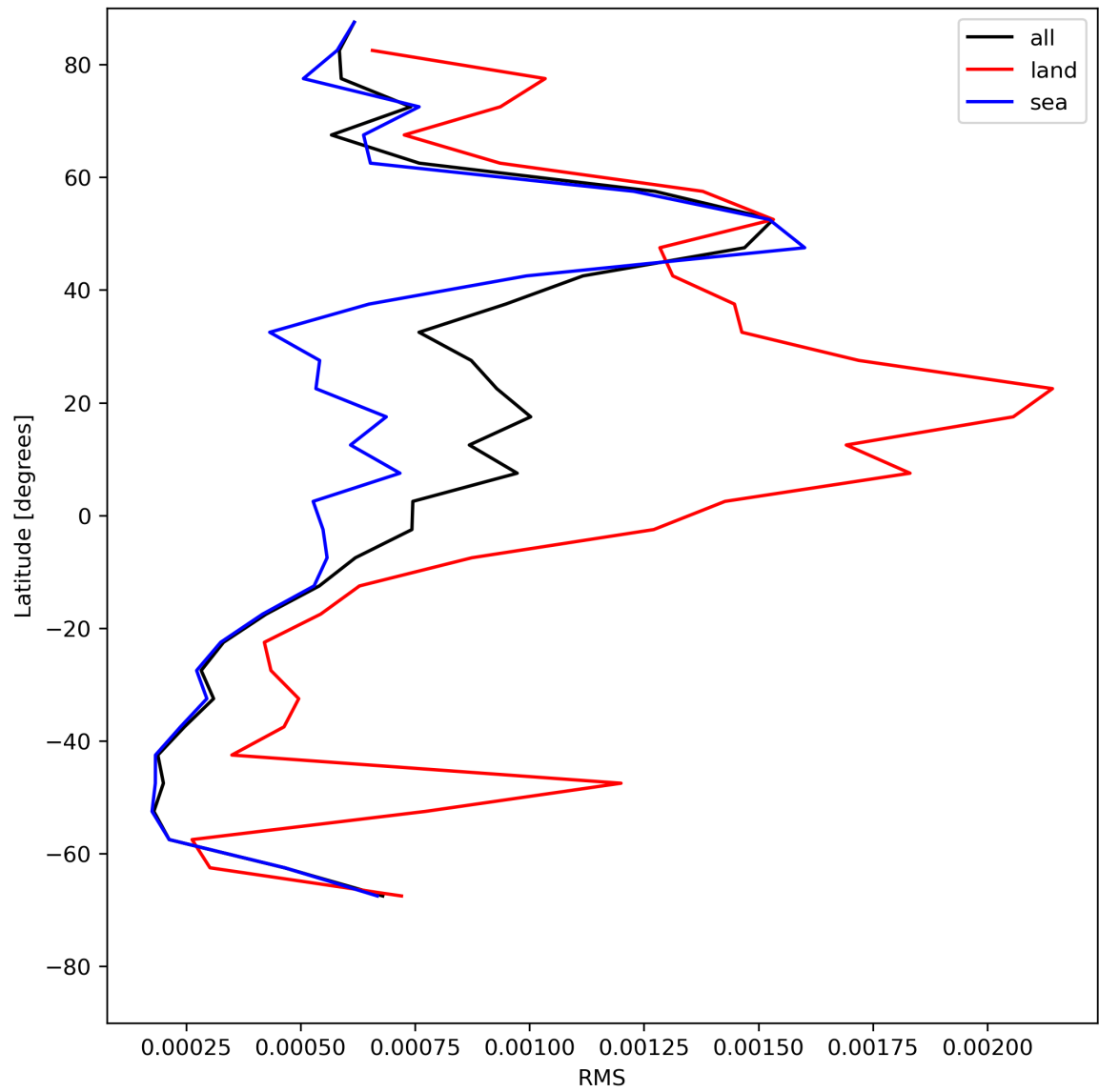
Figure 31: Zonal average of “RMS” for 2024-07-21 to 2024-07-23.
