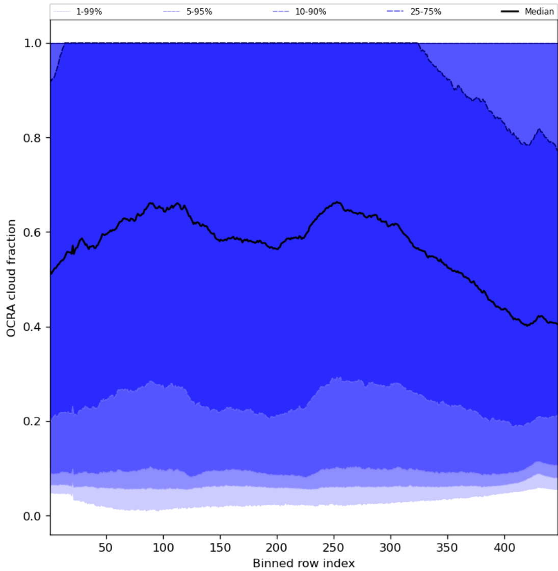
Figure 66: Along track statistics of “OCRA cloud fraction” for 2024-07-21 to 2024-07-23
