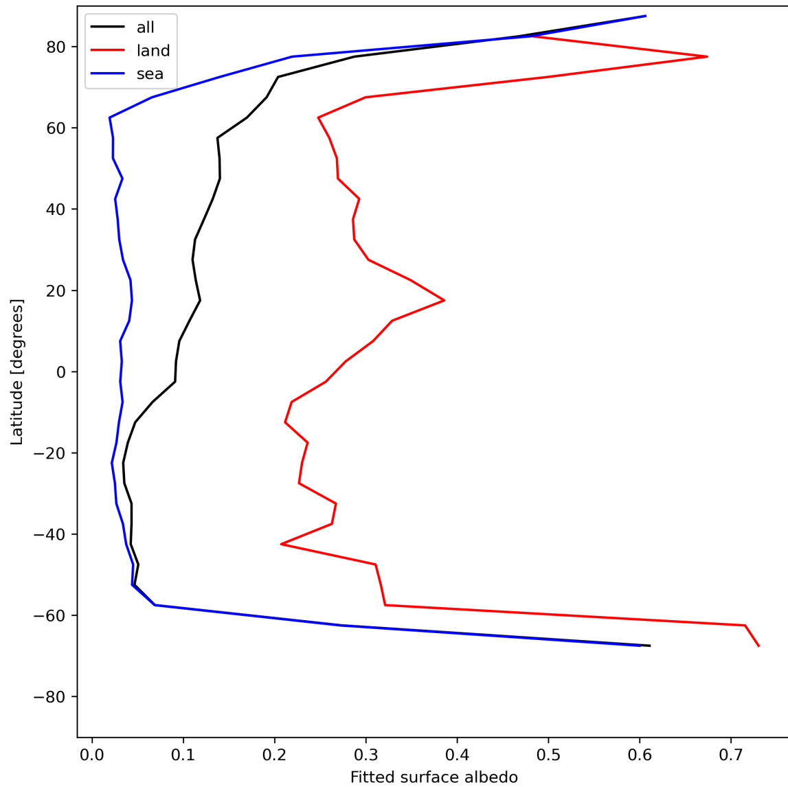
Figure 29: Zonal average of “Fitted surface albedo” for 2024-07-21 to 2024-07-23.
