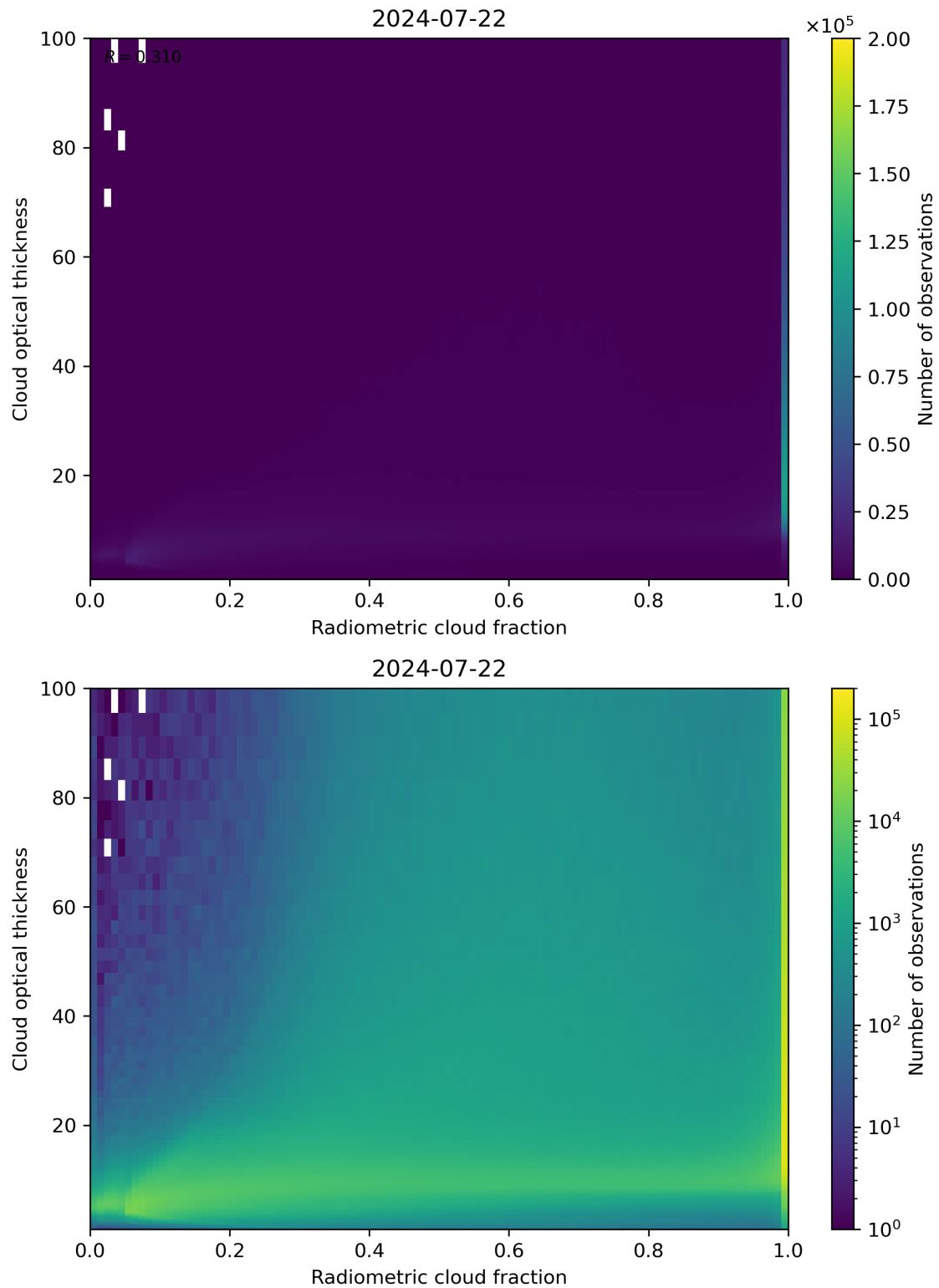
Figure 75: Scatter density plot of “Radiometric cloud fraction” against “Cloud optical thickness” for 2024-07-21 to 2024-07-23.
