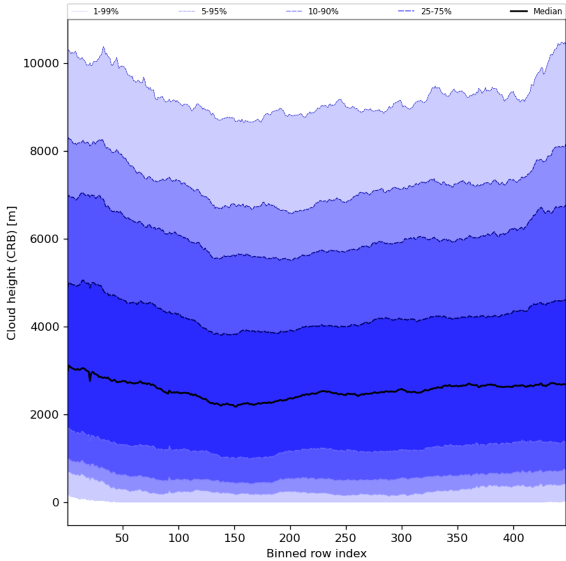
Figure 59: Along track statistics of “Cloud height (CRB)” for 2024-07-21 to 2024-07-23
