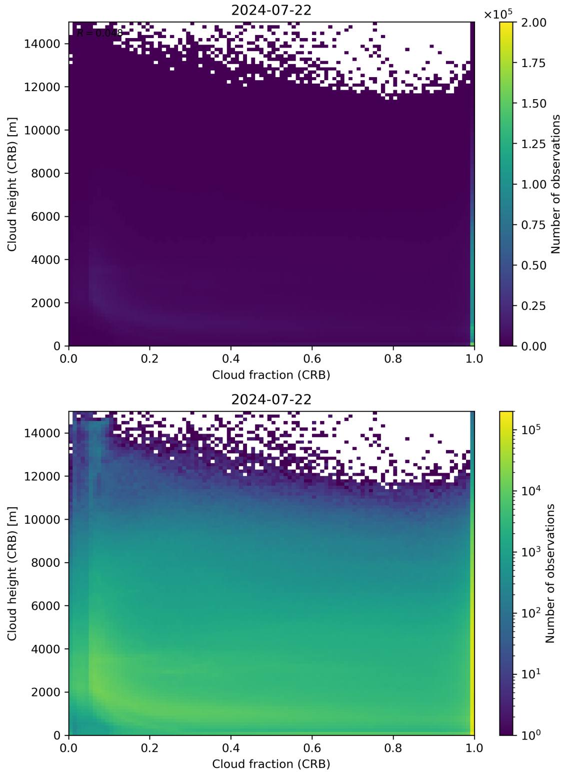
Figure 79: Scatter density plot of “Cloud fraction (CRB)” against “Cloud height (CRB)” for 2024-07-21 to 2024-07-23.
