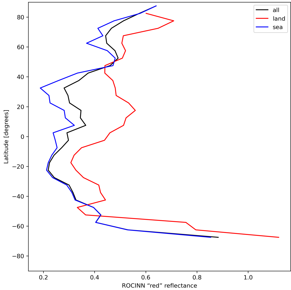
Figure 37: Zonal average of “ROCINN “red” reflectance” for 2024-07-21 to 2024-07-23.
