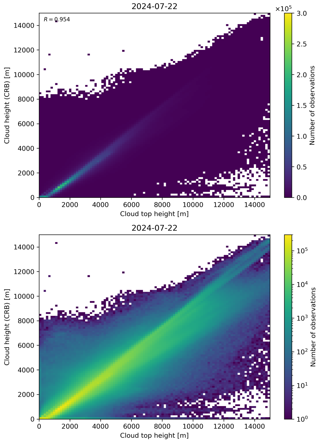
Figure 89: Scatter density plot of “Cloud top height” against “Cloud height (CRB)” for 2024-07-21 to 2024-07-23.
