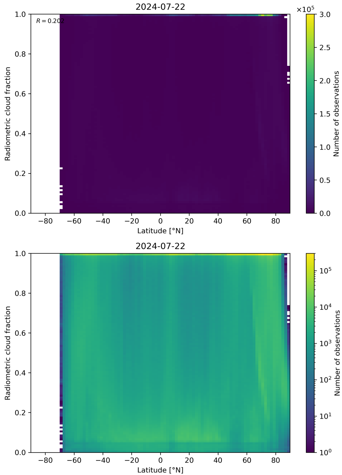
Figure 92: Scatter density plot of “Latitude” against “Radiometric cloud fraction” for 2024-07-21 to 2024-07-23.
