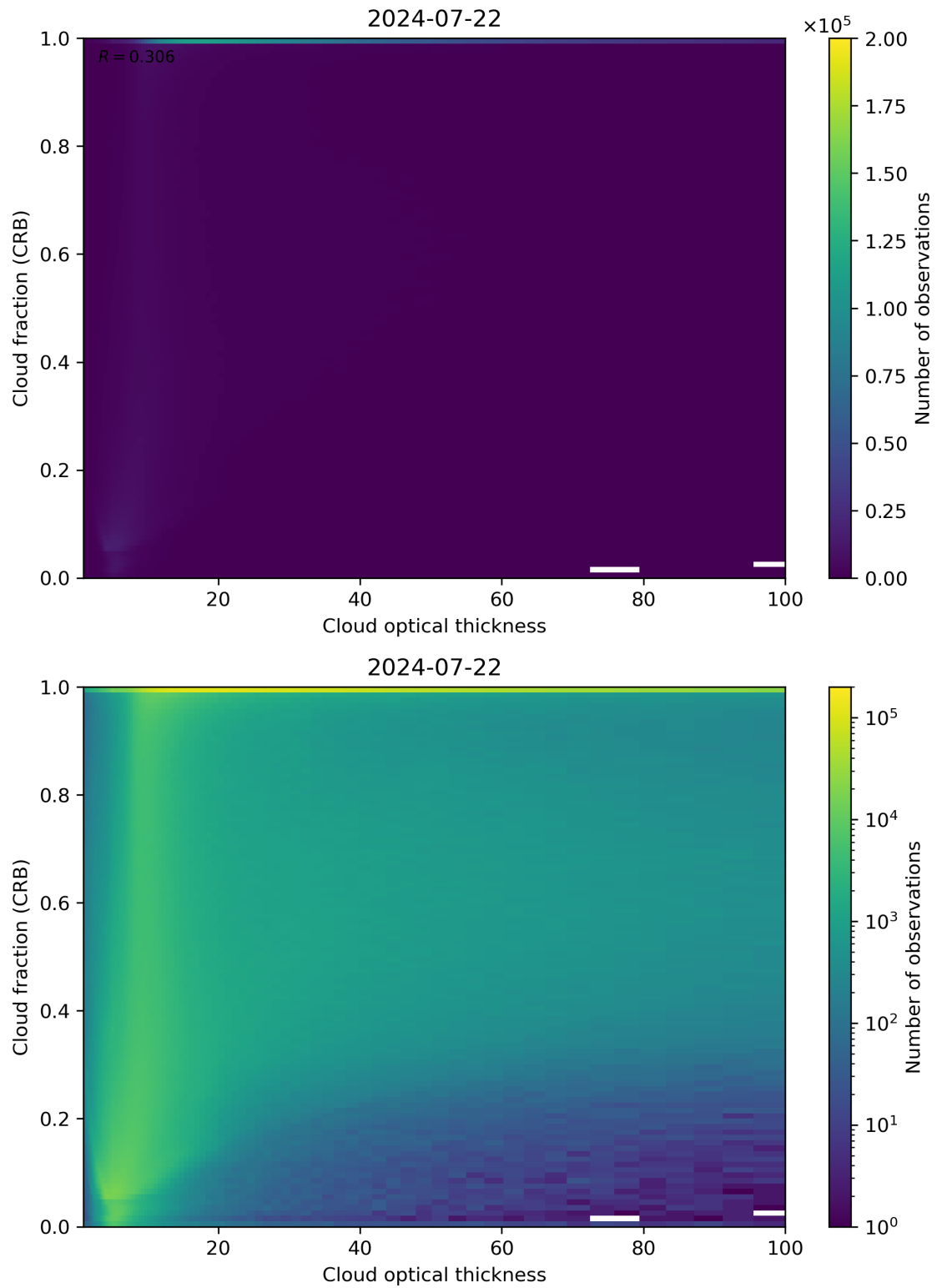
Figure 84: Scatter density plot of “Cloud optical thickness” against “Cloud fraction (CRB)” for 2024-07-21 to 2024-07-23.
