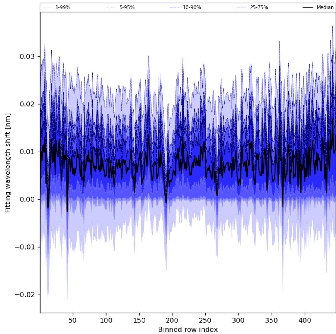
Figure 65: Along track statistics of “Fitting wavelength shift” for 2024-07-21 to 2024-07-23
