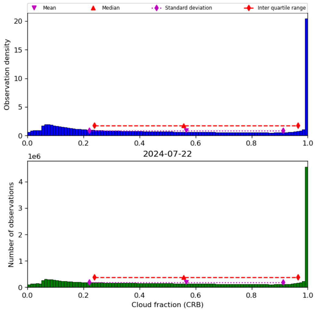
Figure 42: Histogram of “Cloud fraction (CRB)” for 2024-07-21 to 2024-07-23
