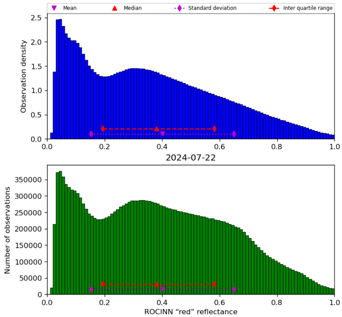
Figure 53: Histogram of “ROCINN “red” reflectance” for 2024-07-21 to 2024-07-23
