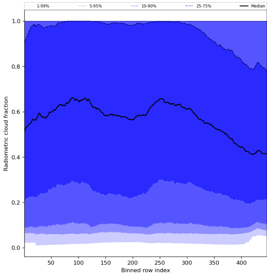
Figure 55: Along track statistics of “Radiometric cloud fraction” for 2024-07-21 to 2024-07-23
