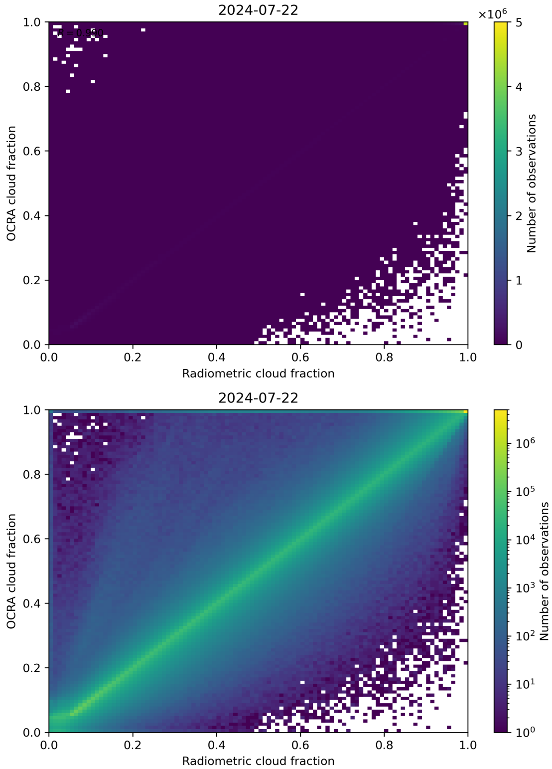
Figure 72: Scatter density plot of “Radiometric cloud fraction” against “OCRA cloud fraction” for 2024-07-21 to 2024-07-23.
