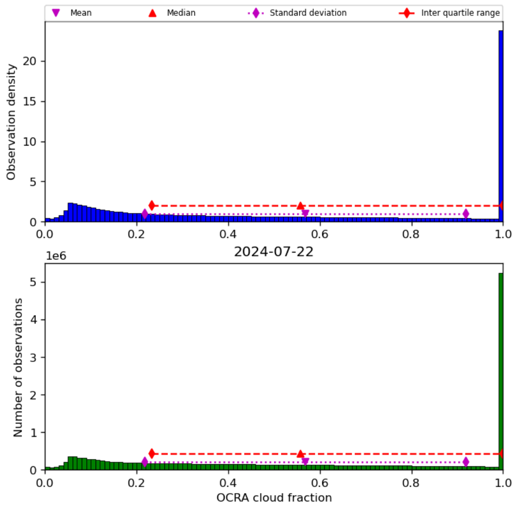
Figure 50: Histogram of “OCRA cloud fraction” for 2024-07-21 to 2024-07-23
