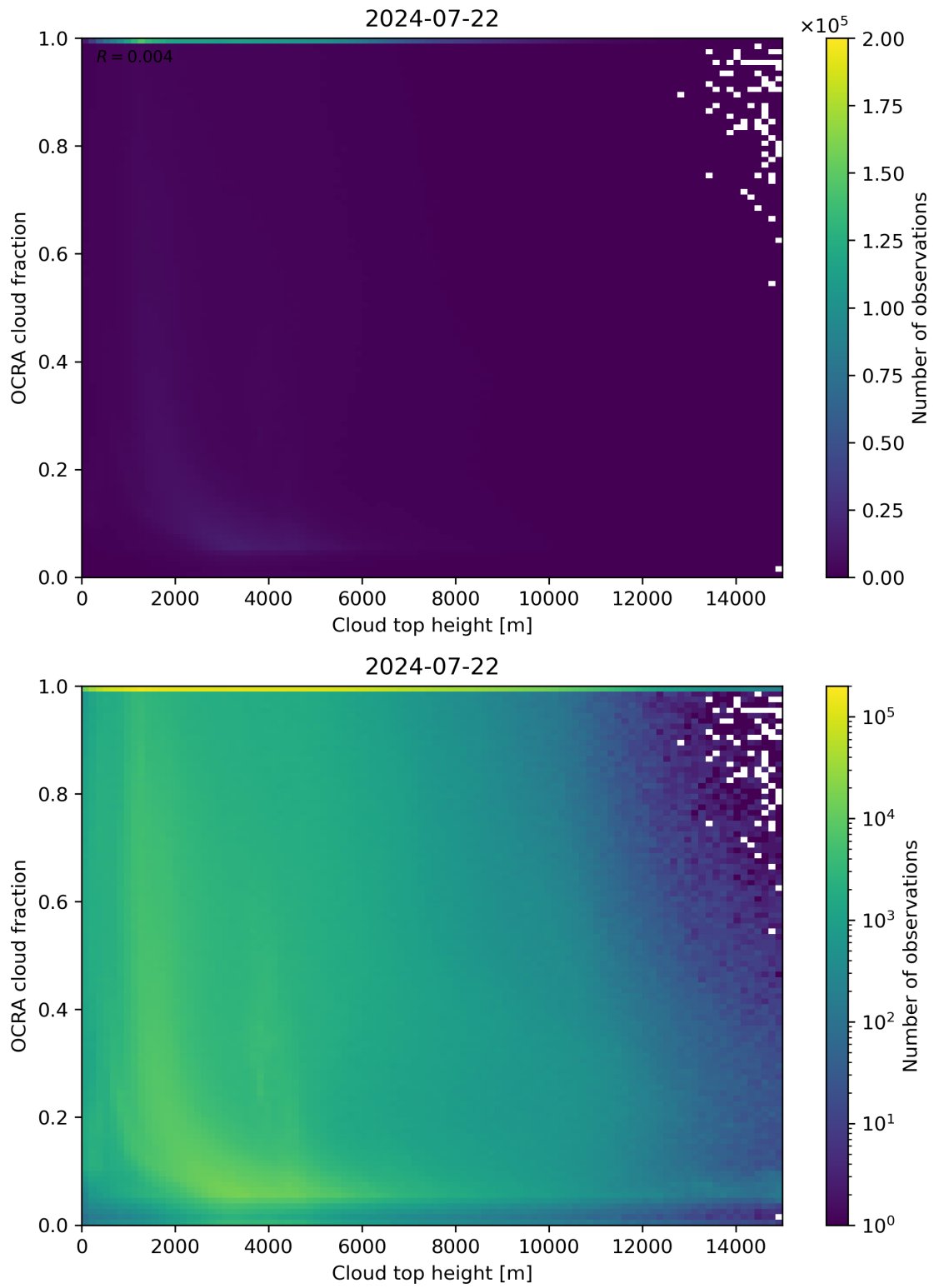
Figure 87: Scatter density plot of “Cloud top height” against “OCRA cloud fraction” for 2024-07-21 to 2024-07-23.
