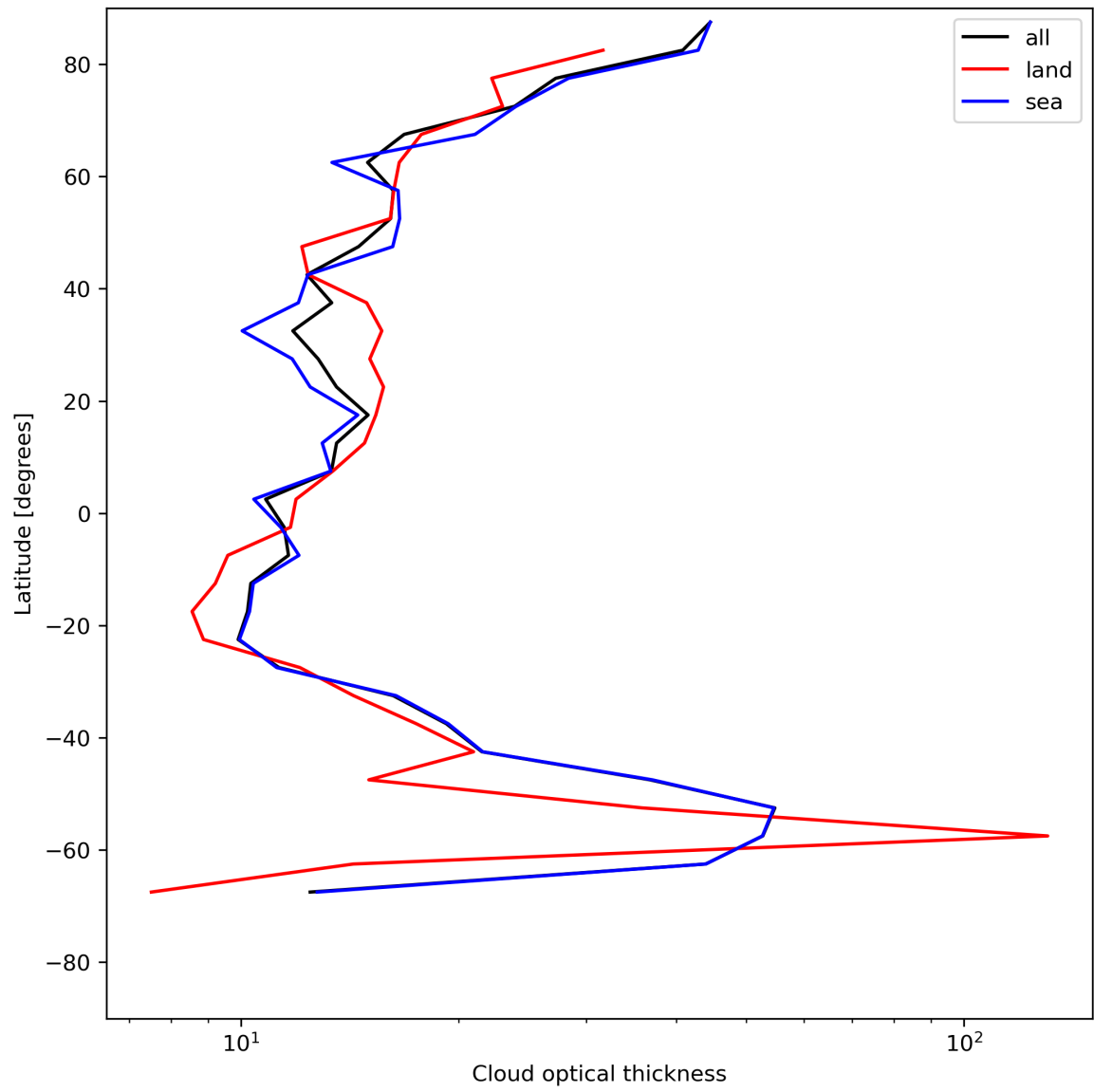
Figure 25: Zonal average of “Cloud optical thickness” for 2024-07-21 to 2024-07-23.
