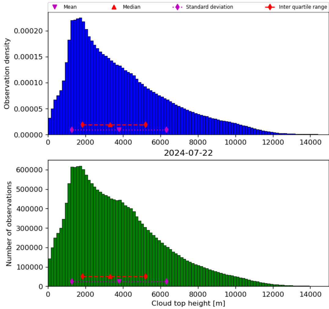
Figure 40: Histogram of “Cloud top height” for 2024-07-21 to 2024-07-23
