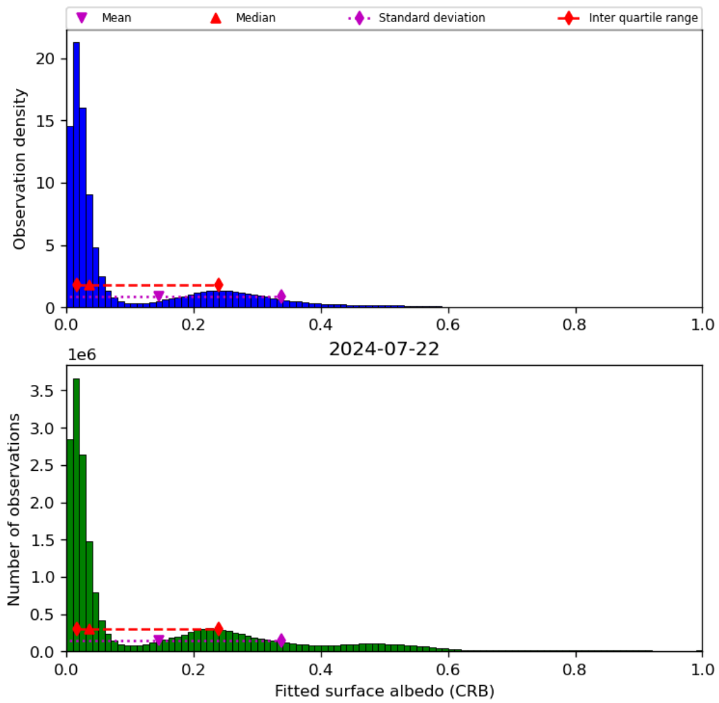
Figure 46: Histogram of “Fitted surface albedo (CRB)” for 2024-07-21 to 2024-07-23
