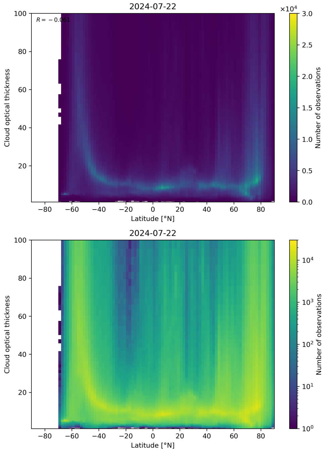
Figure 96: Scatter density plot of “Latitude” against “Cloud optical thickness” for 2024-07-21 to 2024-07-23.
