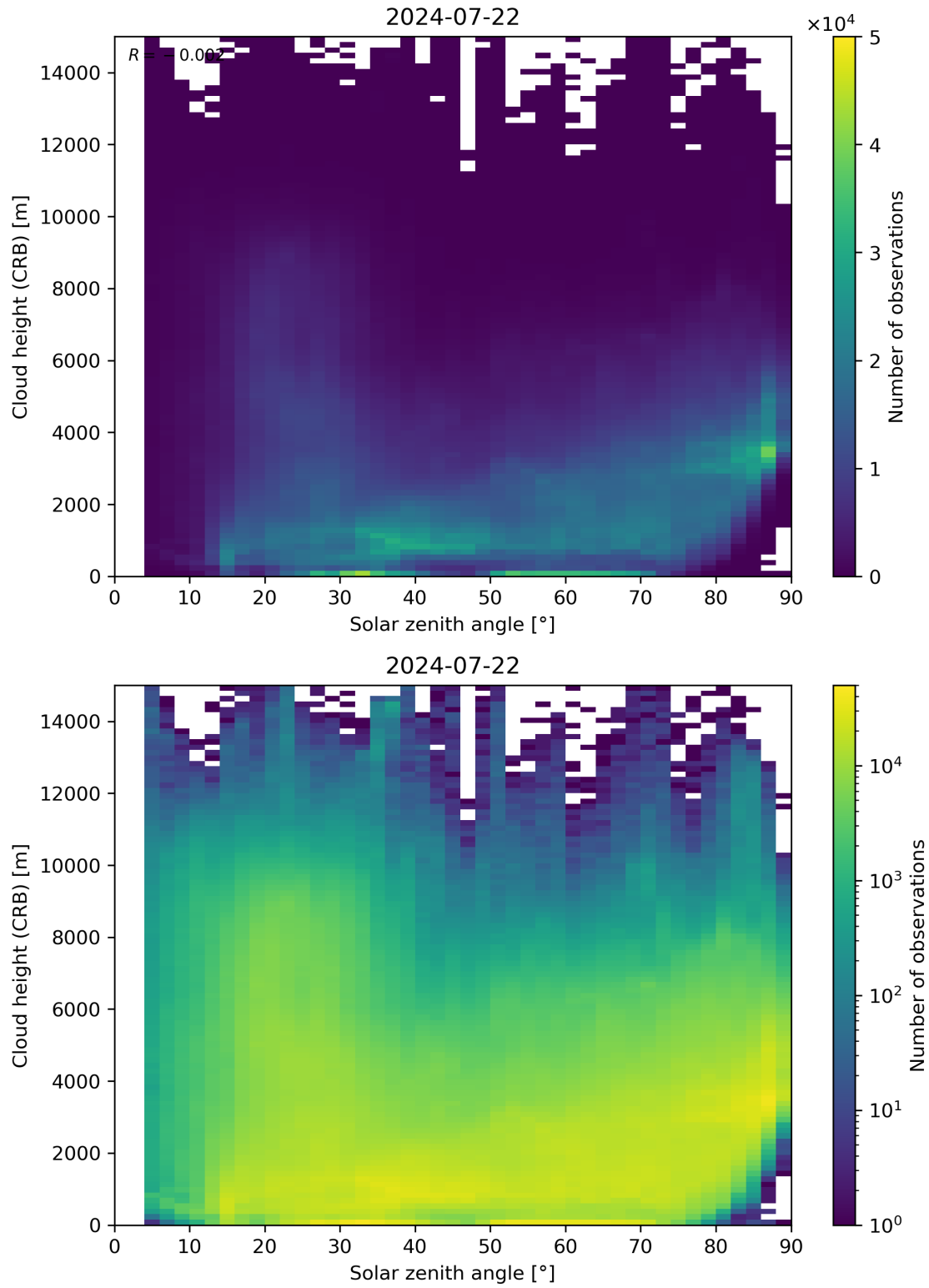
Figure 102: Scatter density plot of “Solar zenith angle” against “Cloud height (CRB)” for 2024-07-21 to 2024-07-23.
