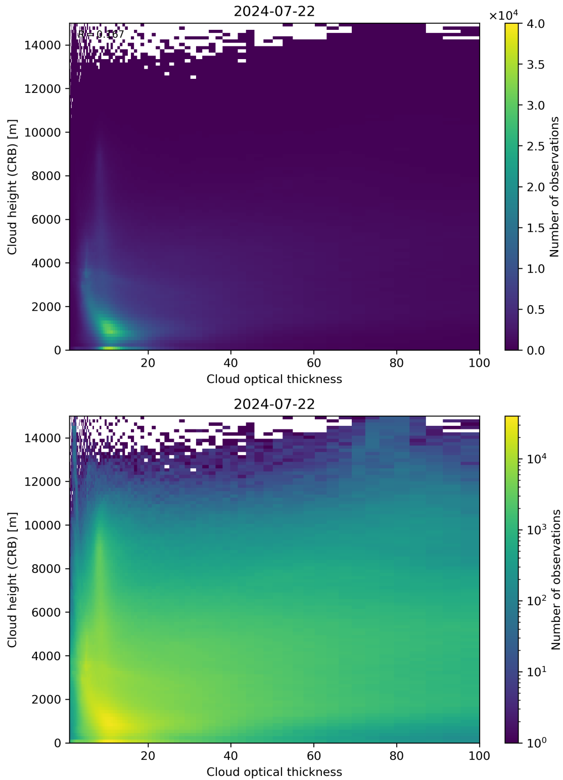
Figure 85: Scatter density plot of “Cloud optical thickness” against “Cloud height (CRB)” for 2024-07-21 to 2024-07-23.
