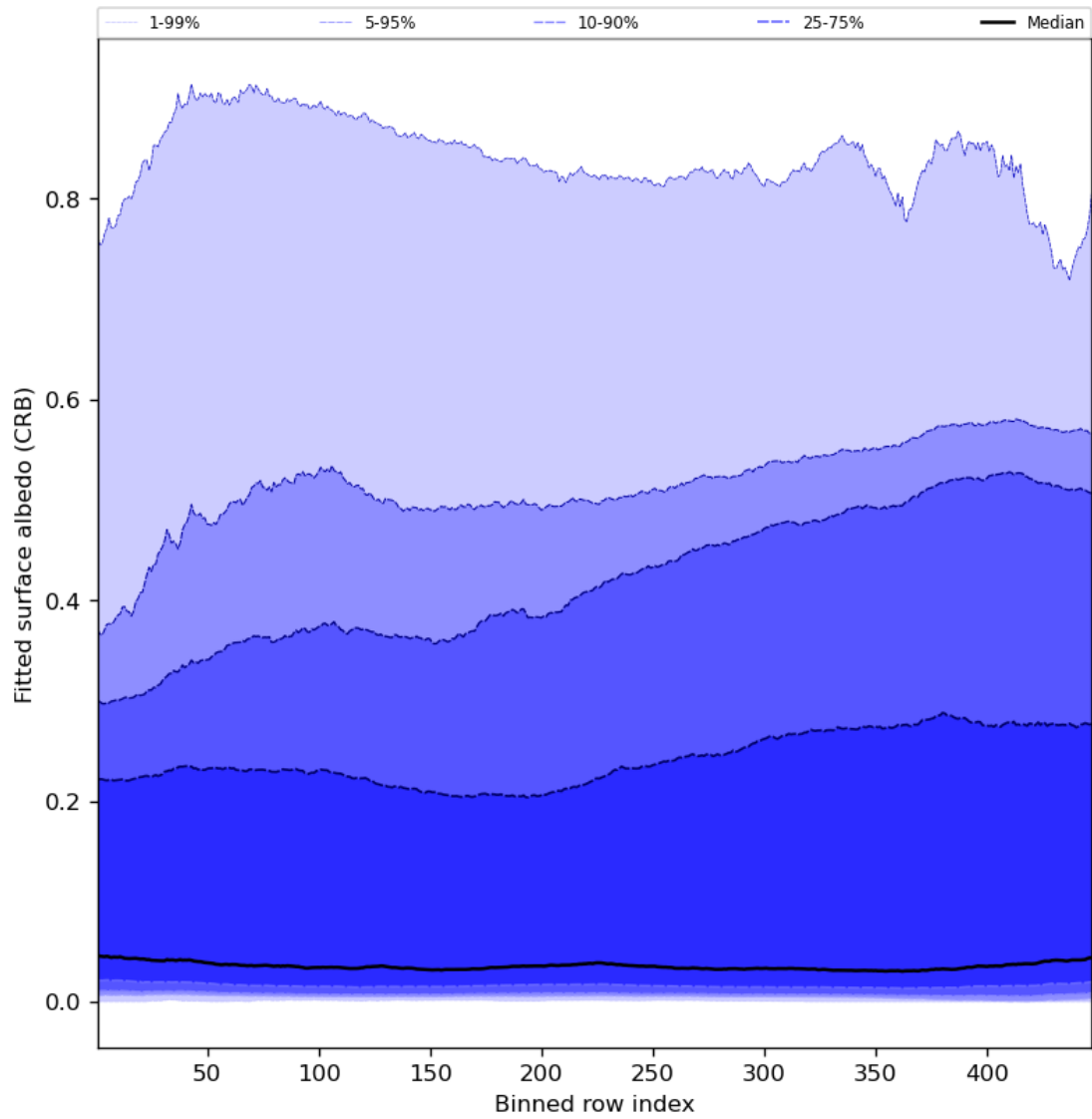
Figure 62: Along track statistics of “Fitted surface albedo (CRB)” for 2024-07-21 to 2024-07-23
