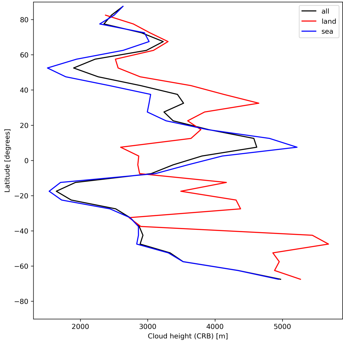
Figure 27: Zonal average of “Cloud height (CRB)” for 2024-07-21 to 2024-07-23.
