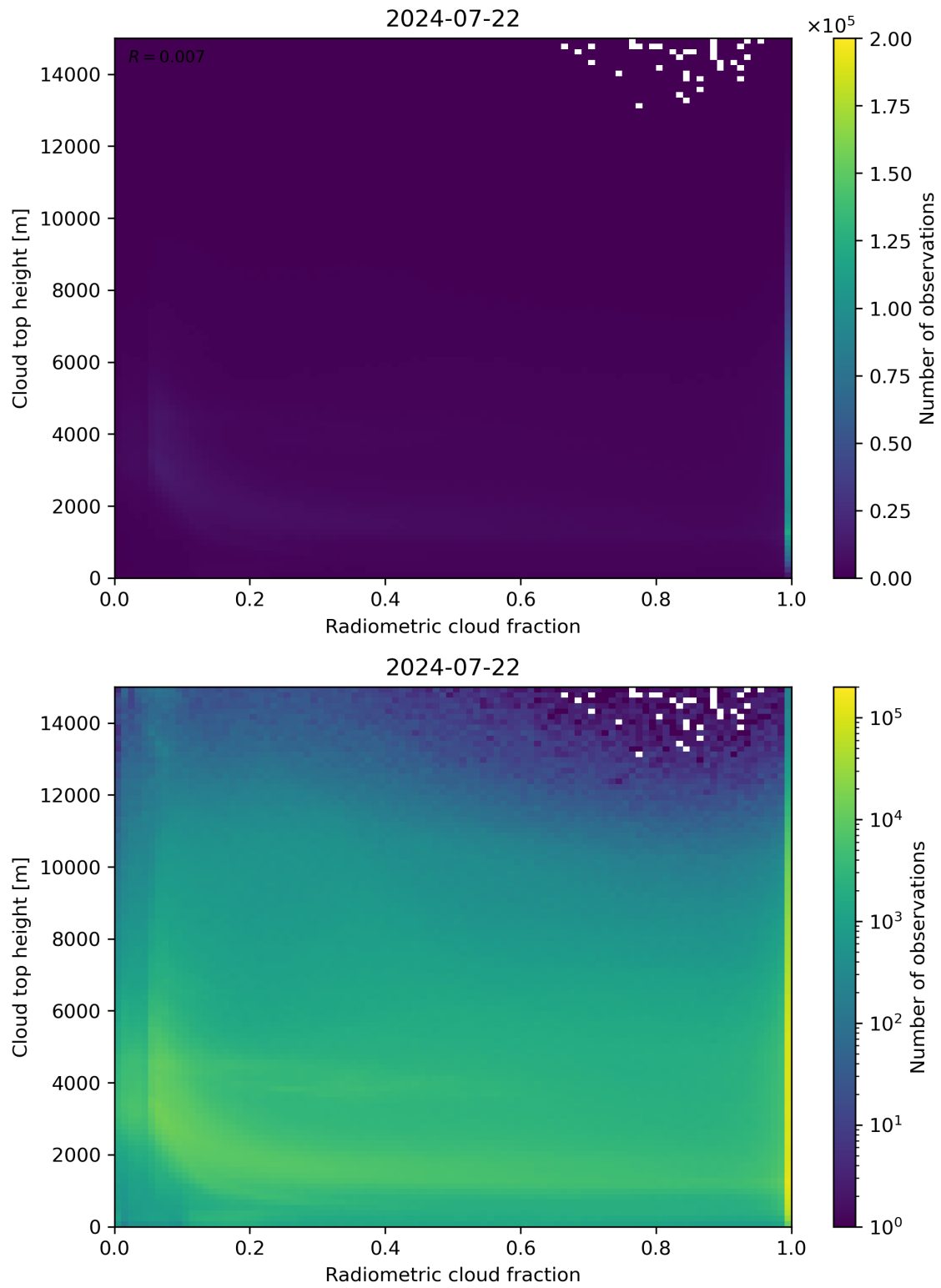
Figure 76: Scatter density plot of “Radiometric cloud fraction” against “Cloud top height” for 2024-07-21 to 2024-07-23.
