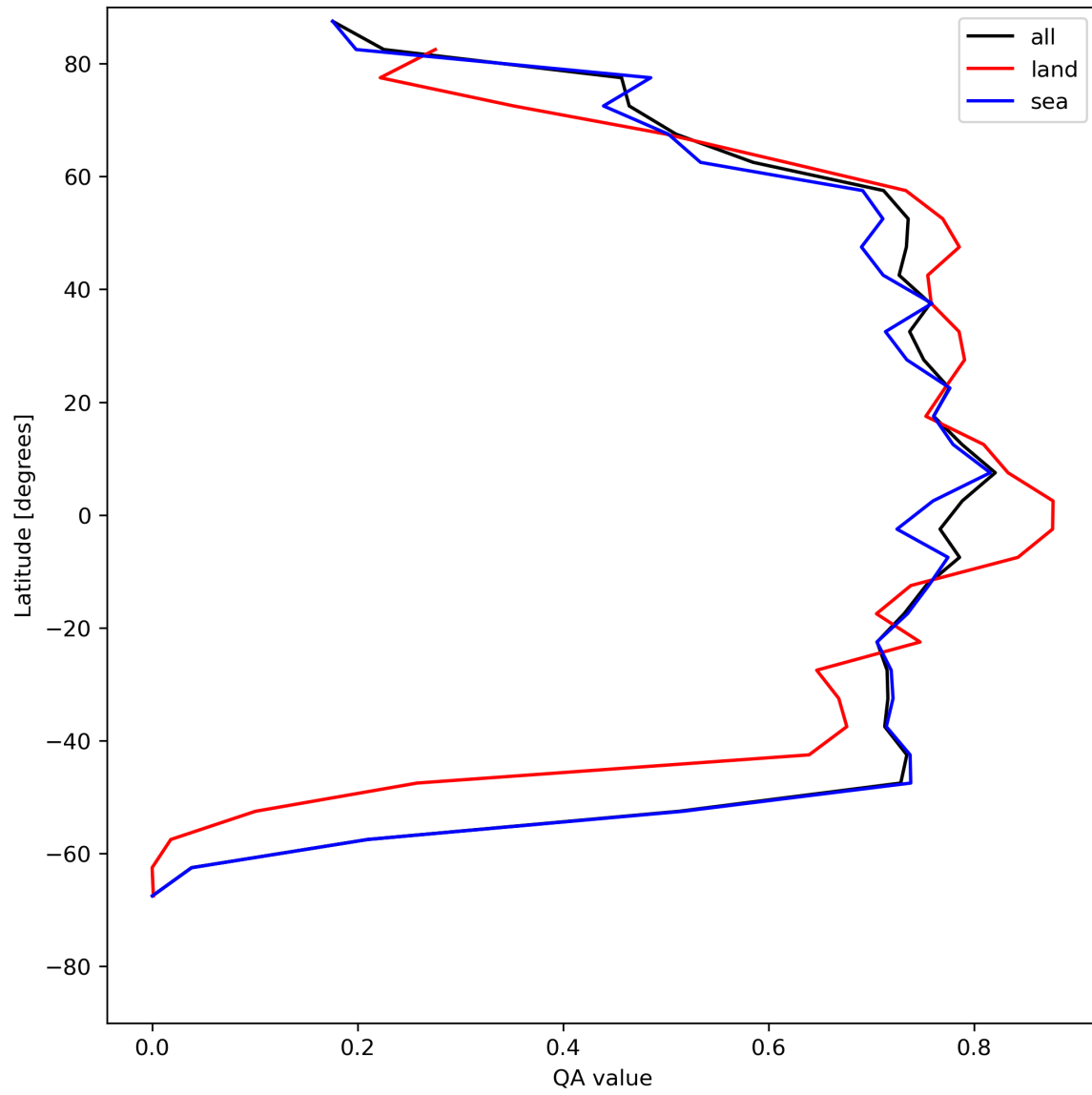
Figure 22: Zonal average of “QA value” for 2024-07-21 to 2024-07-23.
