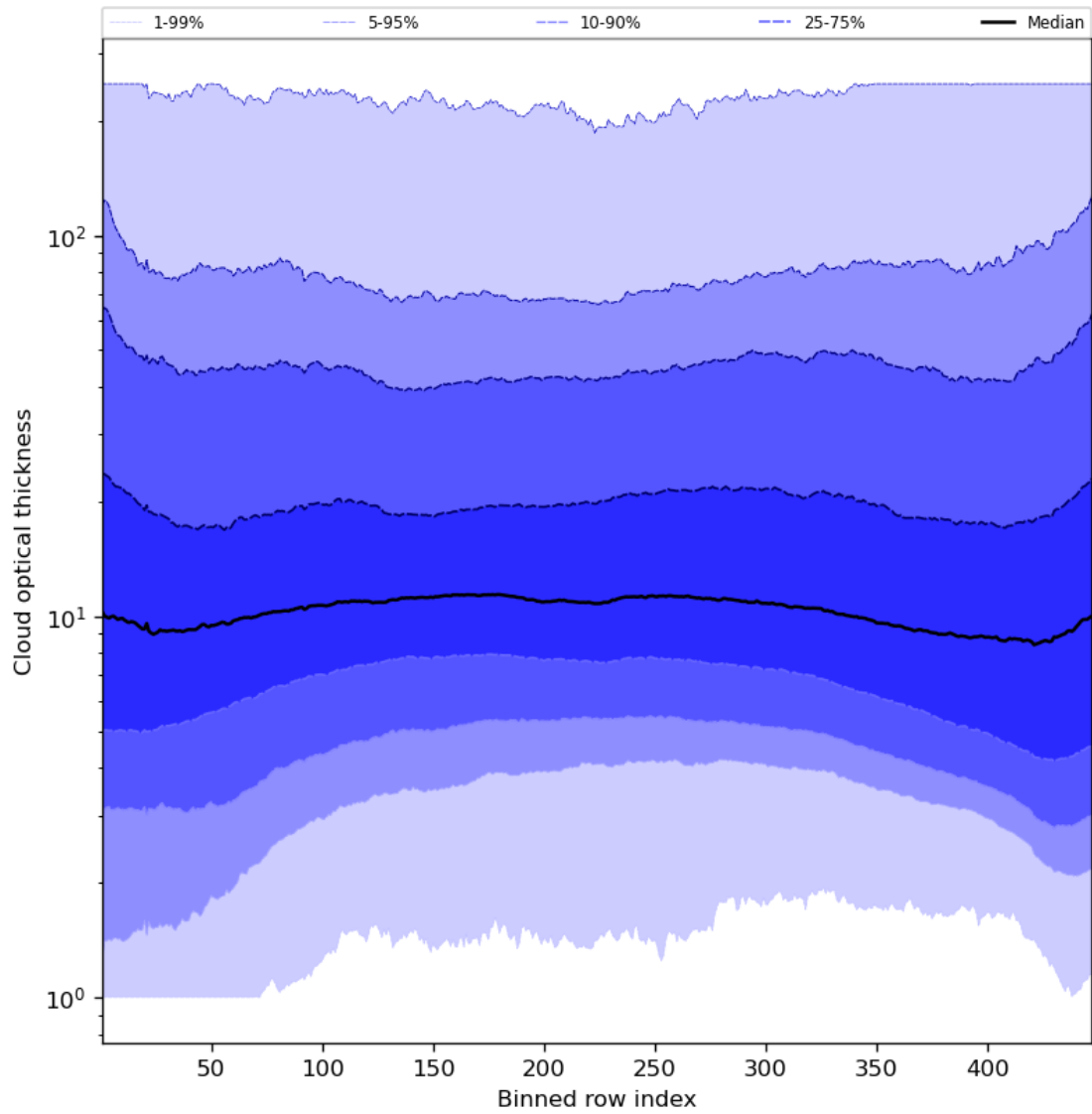
Figure 57: Along track statistics of “Cloud optical thickness” for 2024-07-21 to 2024-07-23
