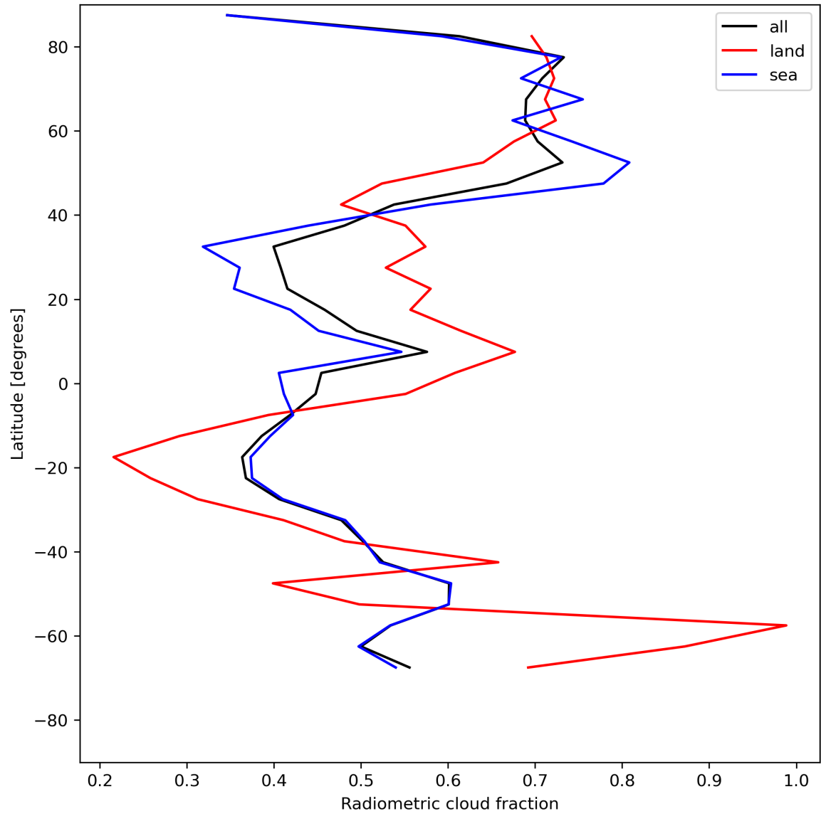
Figure 23: Zonal average of “Radiometric cloud fraction” for 2024-07-21 to 2024-07-23.
