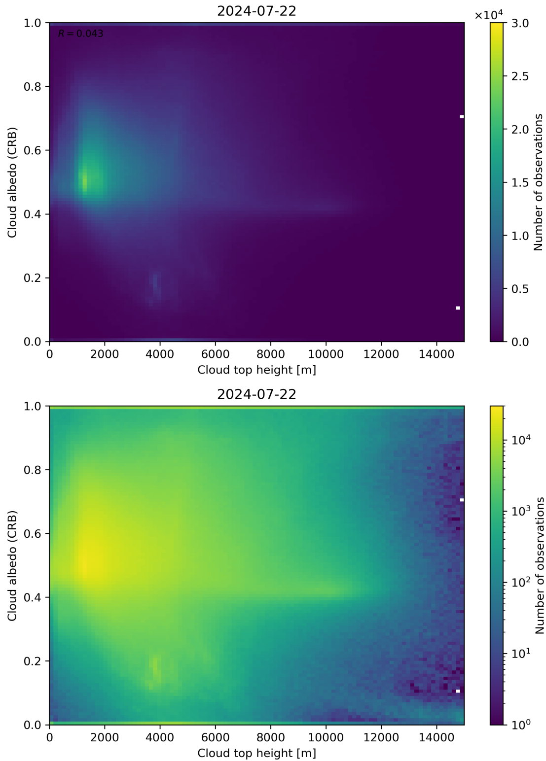
Figure 86: Scatter density plot of “Cloud top height” against “Cloud albedo (CRB)” for 2024-07-21 to 2024-07-23.
