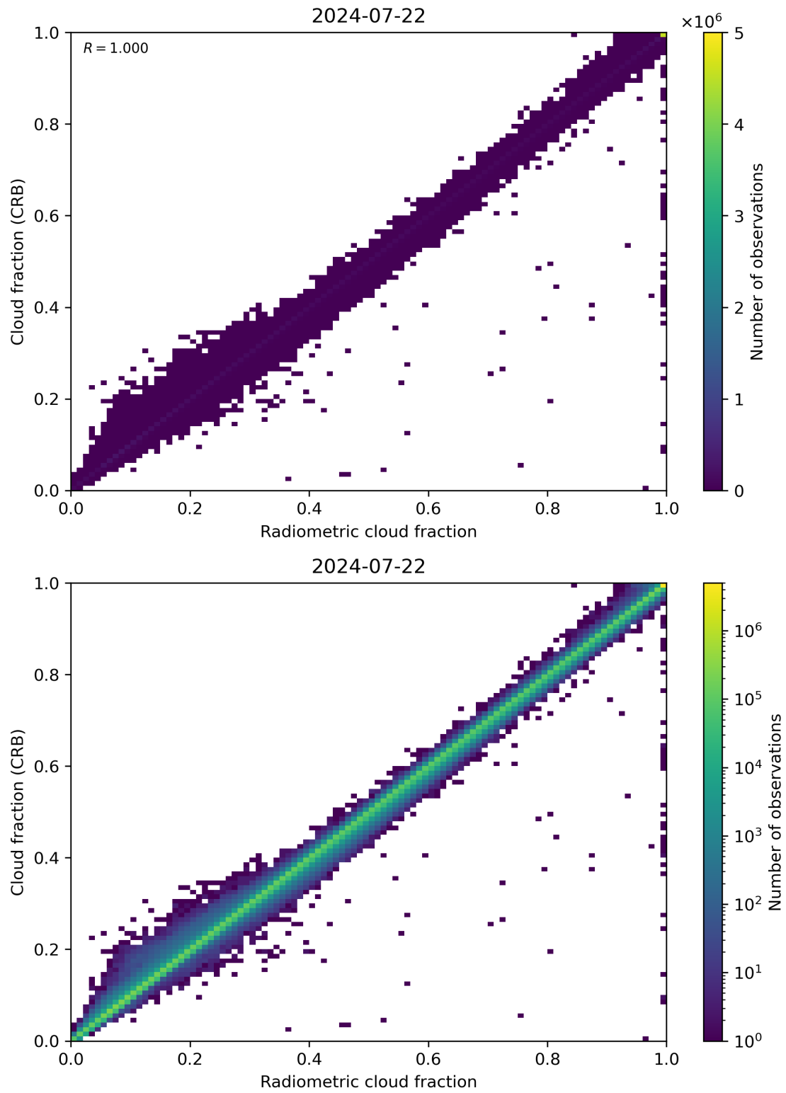
Figure 73: Scatter density plot of “Radiometric cloud fraction” against “Cloud fraction (CRB)” for 2024-07-21 to 2024-07-23.
