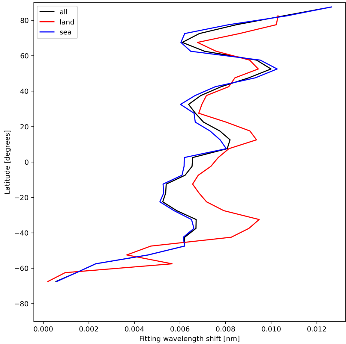
Figure 33: Zonal average of “Fitting wavelength shift” for 2024-07-21 to 2024-07-23.
