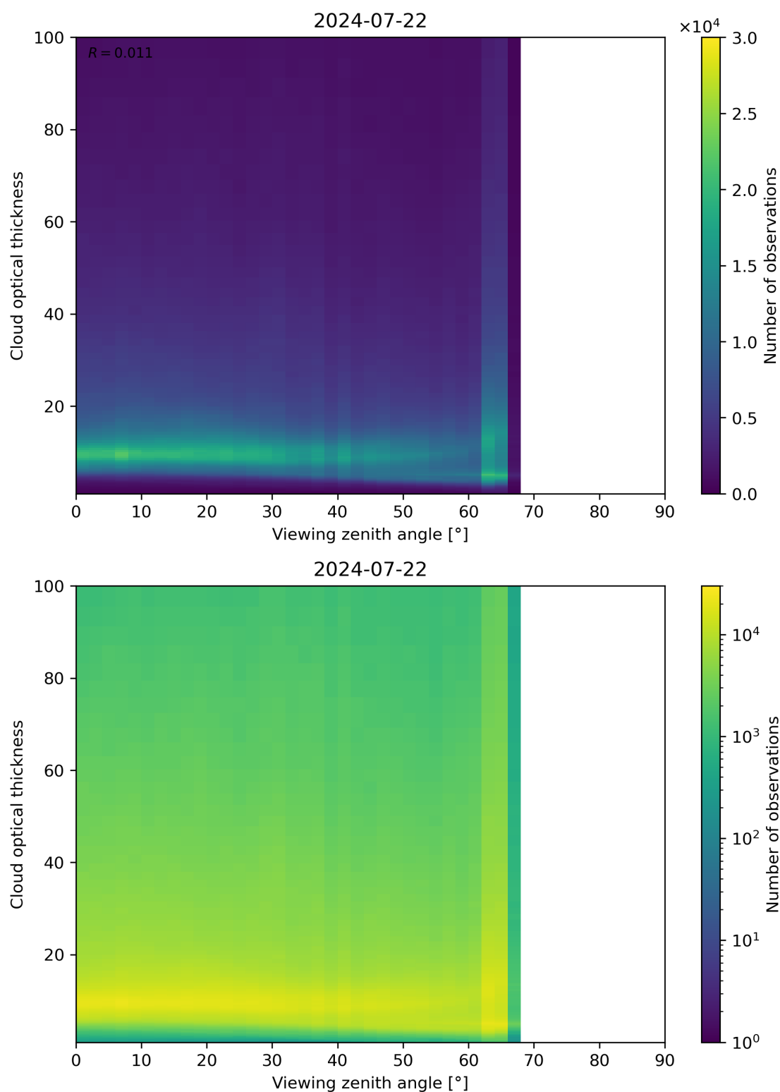
Figure 111: Scatter density plot of “Viewing zenith angle” against “Cloud optical thickness” for 2024-07-21 to 2024-07-23.
