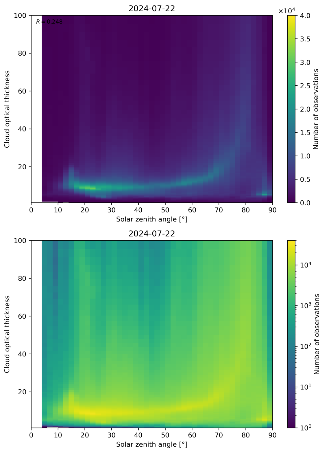
Figure 103: Scatter density plot of “Solar zenith angle” against “Cloud optical thickness” for 2024-07-21 to 2024-07-23.
