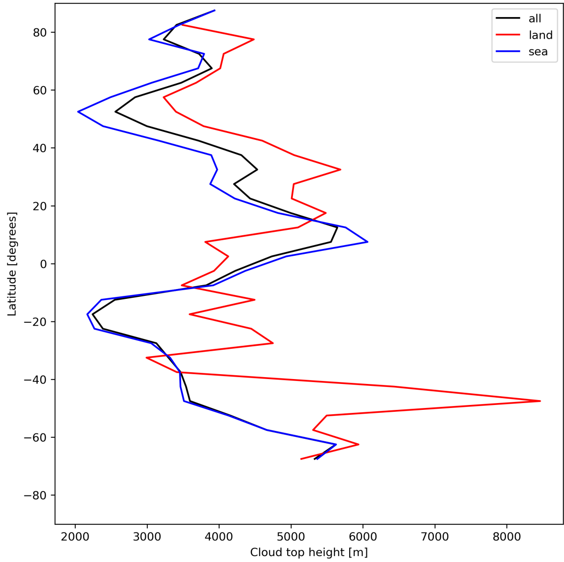
Figure 24: Zonal average of “Cloud top height” for 2024-07-21 to 2024-07-23.
