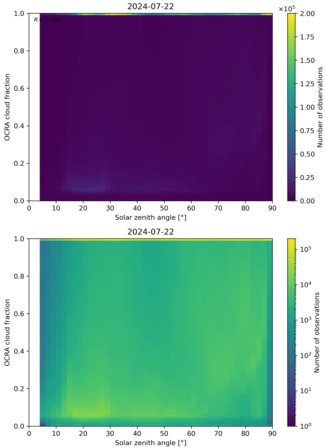
Figure 100: Scatter density plot of “Solar zenith angle” against “OCRA cloud fraction” for 2024-07-21 to 2024-07-23.
