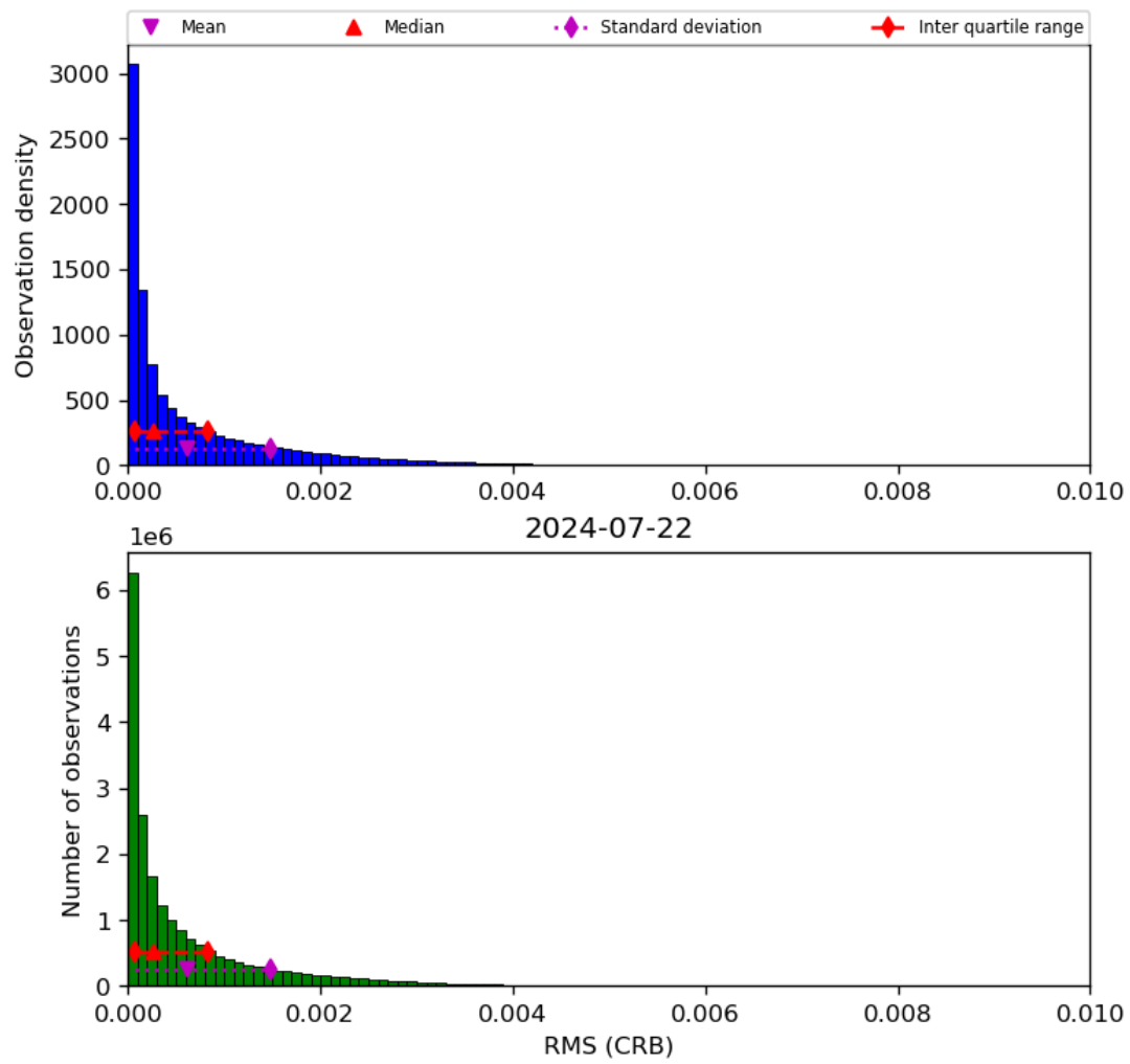
Figure 48: Histogram of "RMS (CRB)" for 2024-07-21 to 2024-07-23
