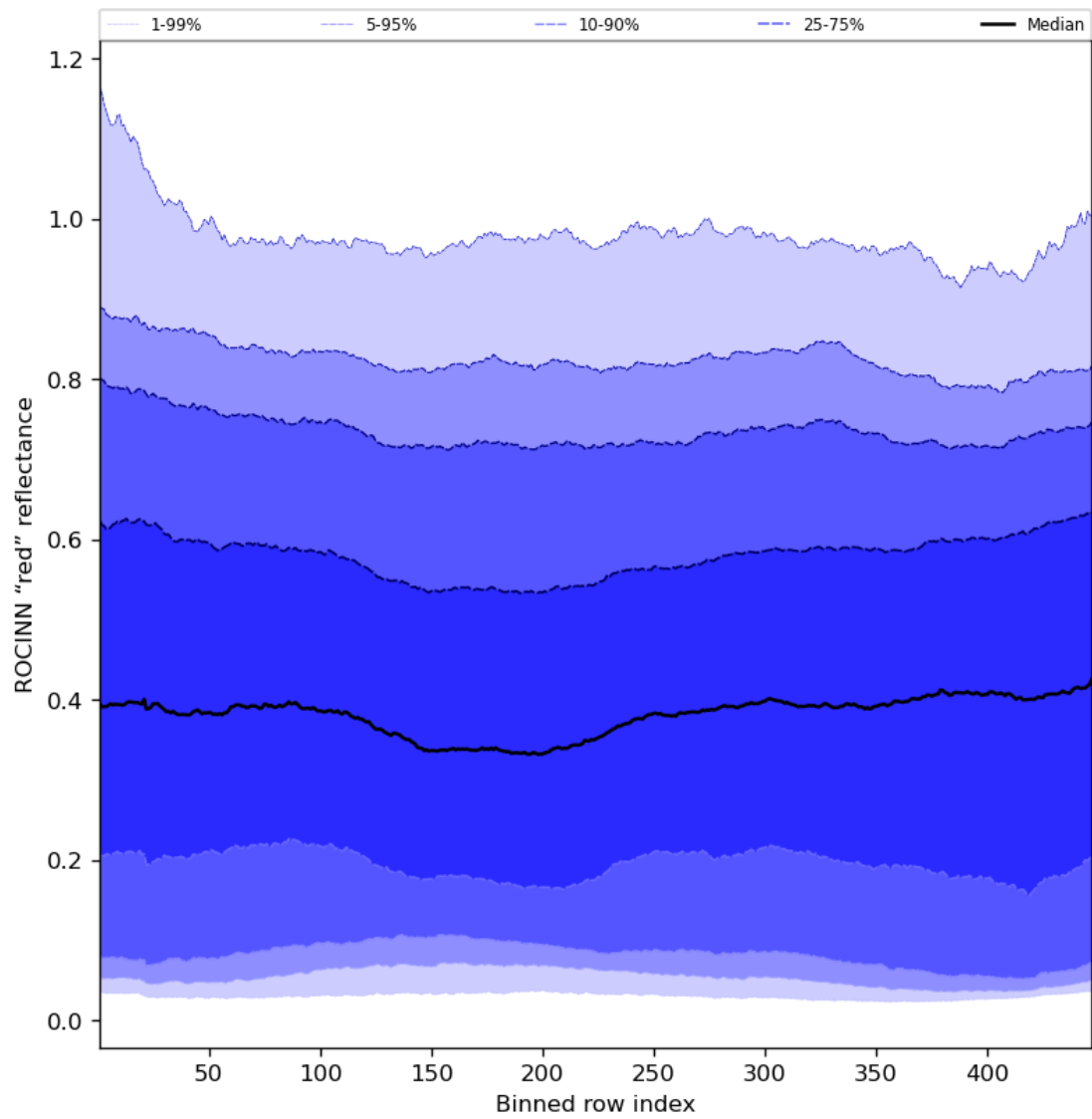
Figure 69: Along track statistics of "ROCINN "red" reflectance" for 2024-07-21 to 2024-07-23
