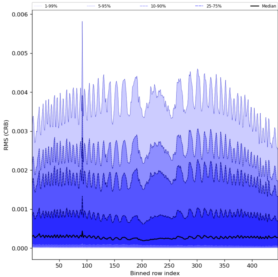
Figure 64: Along track statistics of “RMS (CRB)” for 2024-07-21 to 2024-07-23
