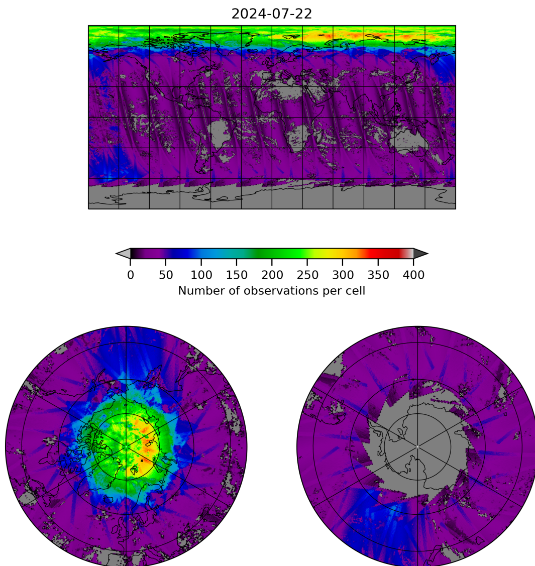
Figure 21: Map of the number of observations for 2024-07-21 to 2024-07-23
