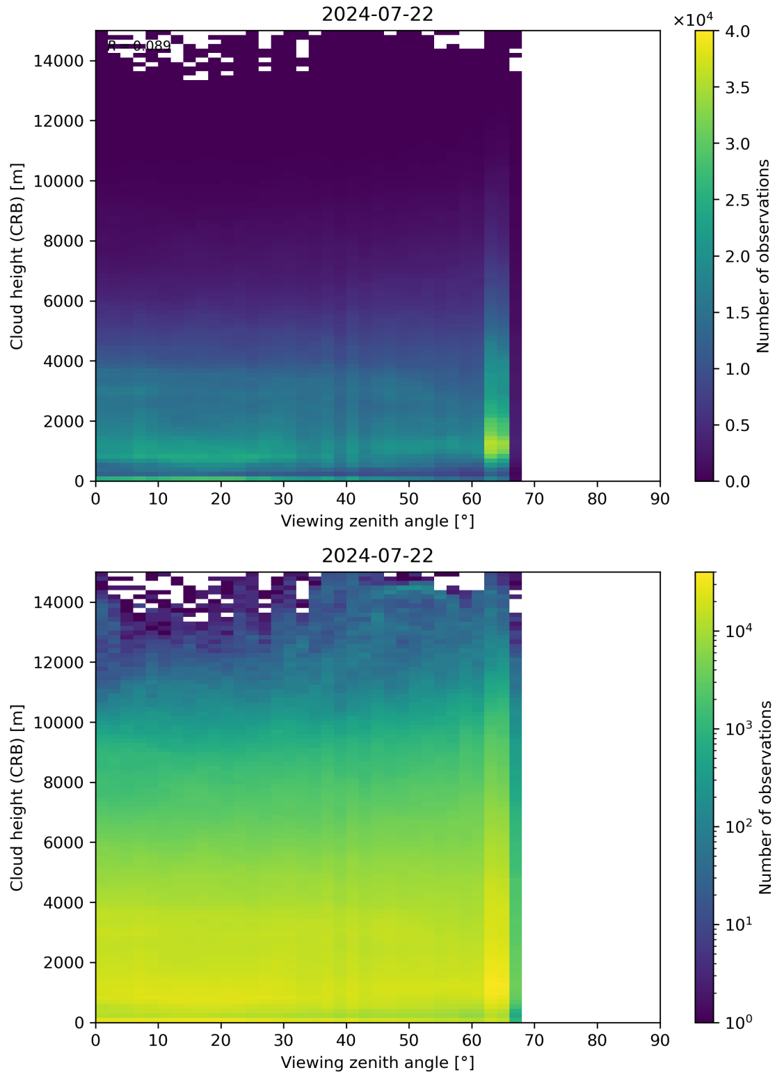
Figure 110: Scatter density plot of “Viewing zenith angle” against “Cloud height (CRB)” for 2024-07-21 to 2024-07-23.
