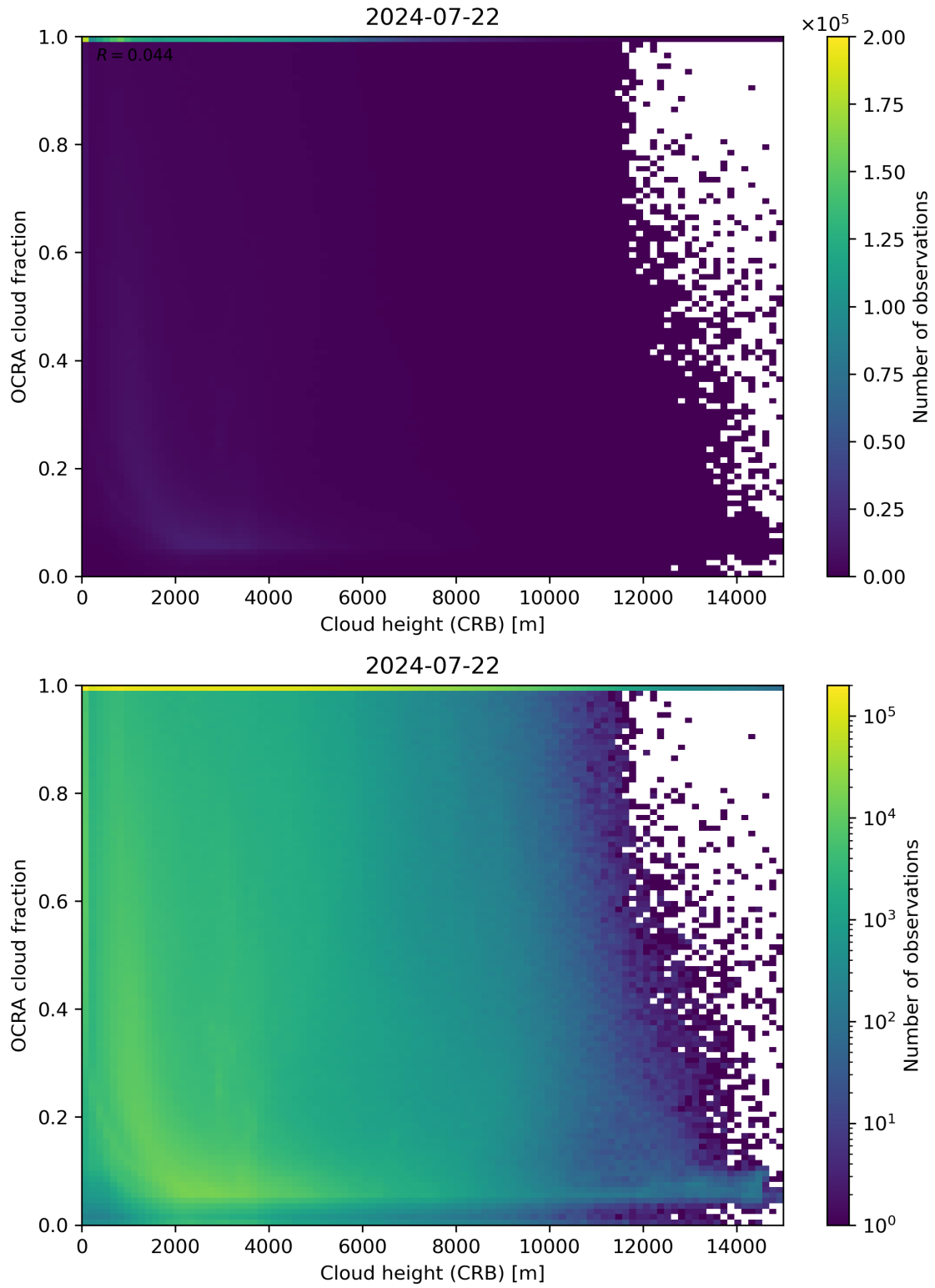
Figure 81: Scatter density plot of “Cloud height (CRB)” against “OCRA cloud fraction” for 2024-07-21 to 2024-07-23.
