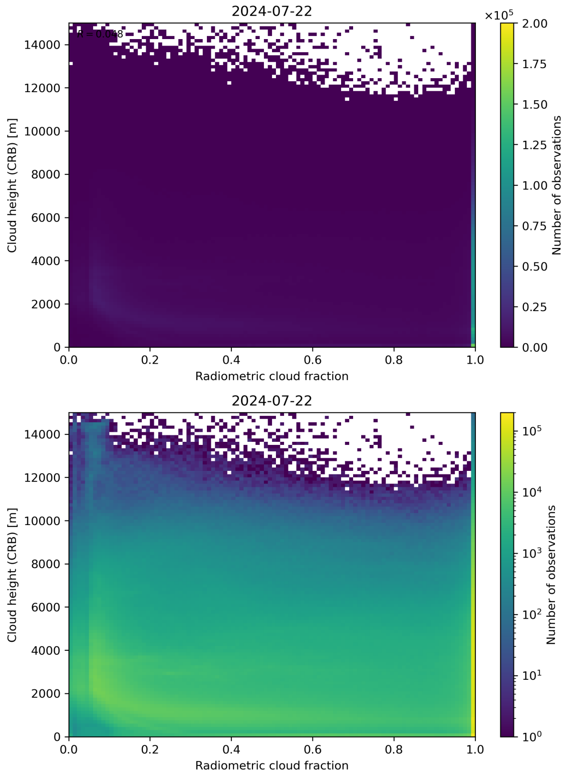
Figure 74: Scatter density plot of “Radiometric cloud fraction” against “Cloud height (CRB)” for 2024-07-21 to 2024-07-23.
