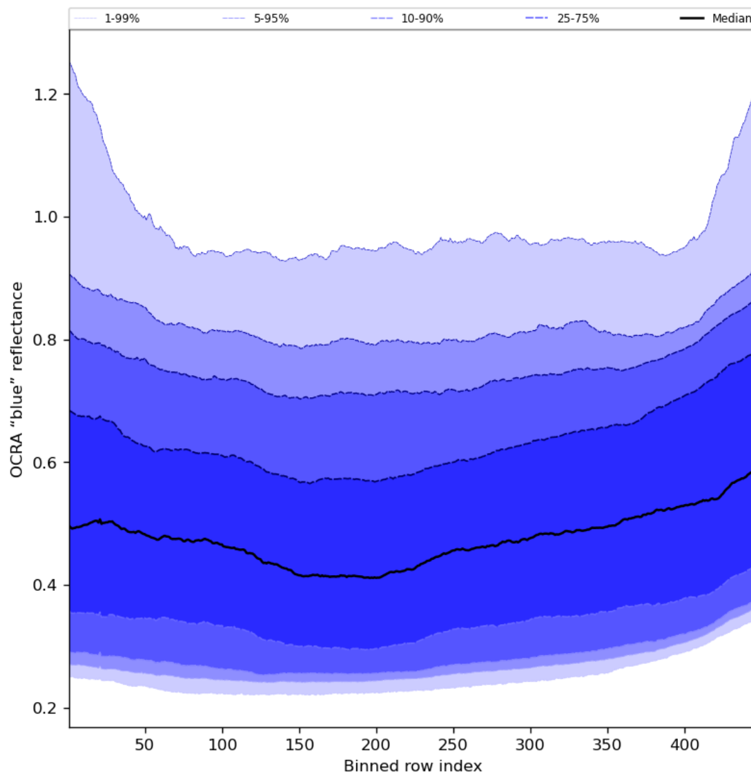
Figure 67: Along track statistics of “OCRA “blue” reflectance” for 2024-07-21 to 2024-07-23
