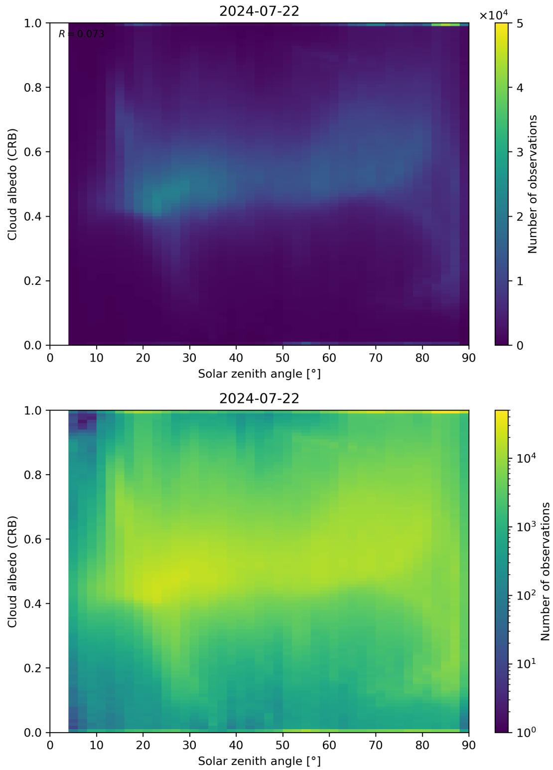
Figure 98: Scatter density plot of “Solar zenith angle” against “Cloud albedo (CRB)” for 2024-07-21 to 2024-07-23.
