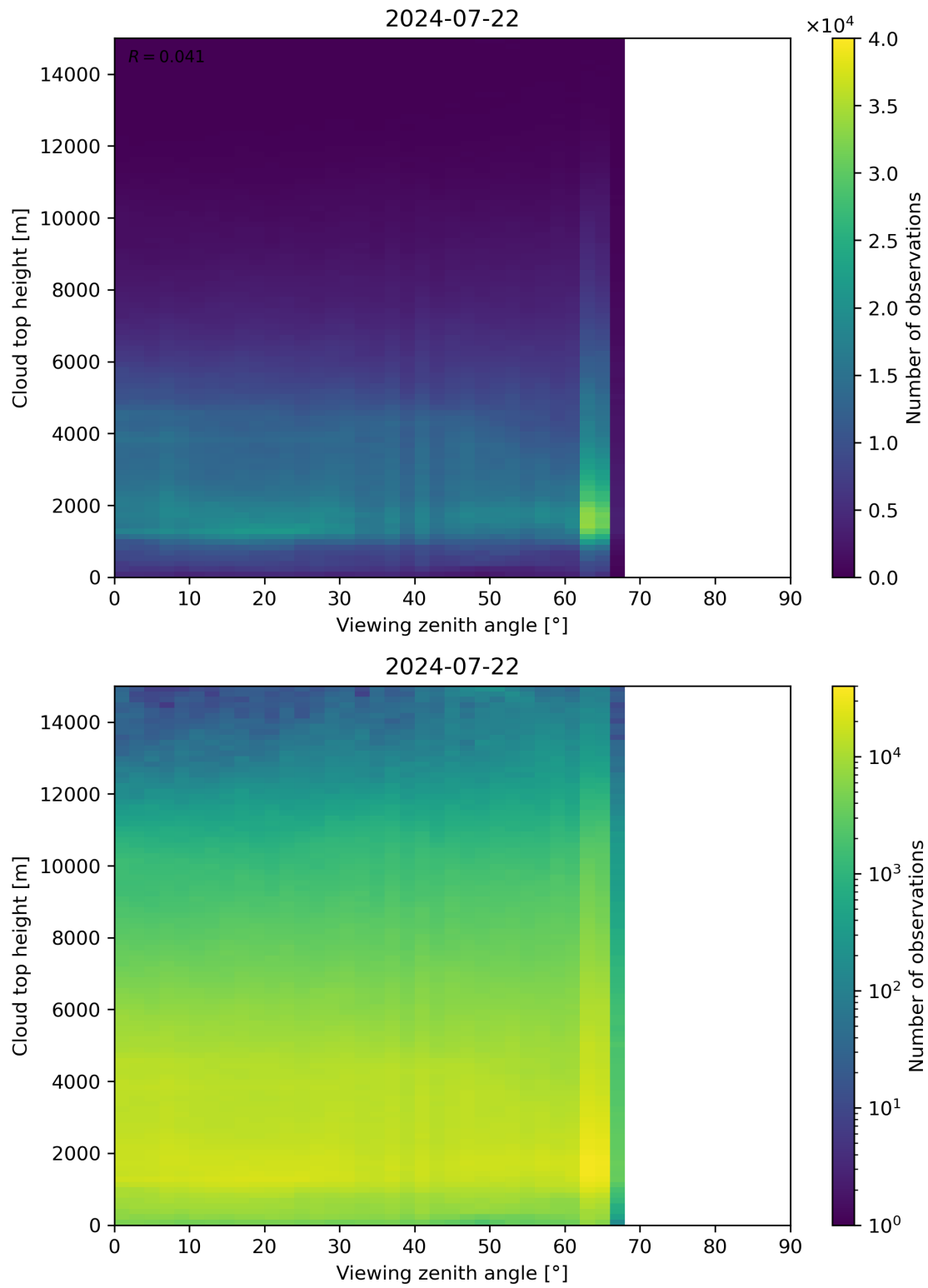
Figure 112: Scatter density plot of “Viewing zenith angle” against “Cloud top height” for 2024-07-21 to 2024-07-23.
