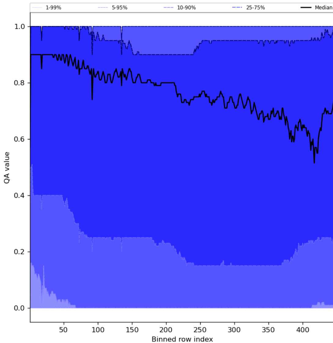
Figure 54: Along track statistics of “QA value” for 2024-07-21 to 2024-07-23
