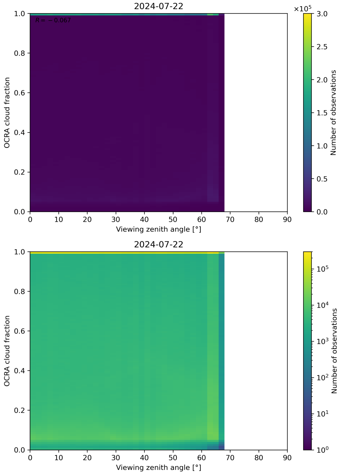
Figure 108: Scatter density plot of “Viewing zenith angle” against “OCRA cloud fraction” for 2024-07-21 to 2024-07-23.
