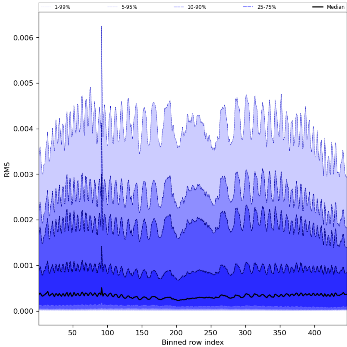
Figure 63: Along track statistics of “RMS” for 2024-07-21 to 2024-07-23
