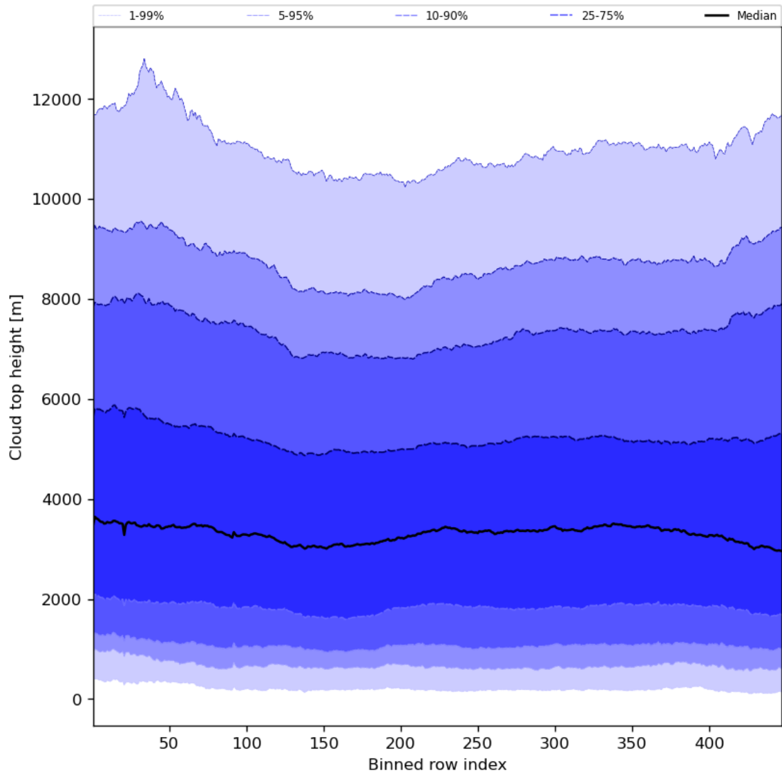
Figure 56: Along track statistics of “Cloud top height” for 2024-07-21 to 2024-07-23
