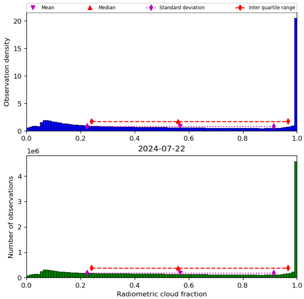
Figure 39: Histogram of “Radiometric cloud fraction” for 2024-07-21 to 2024-07-23
