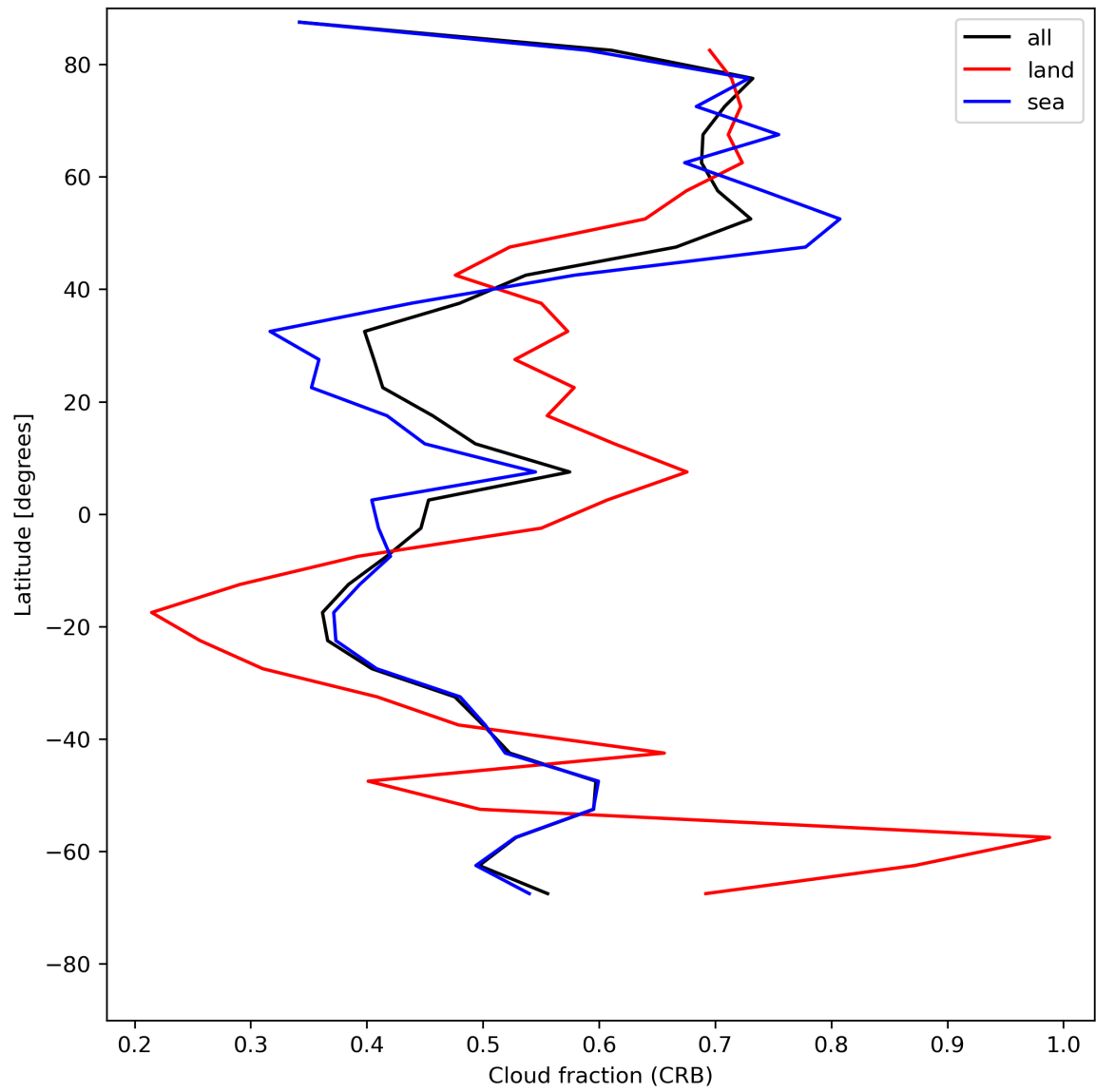
Figure 26: Zonal average of “Cloud fraction (CRB)” for 2024-07-21 to 2024-07-23.
