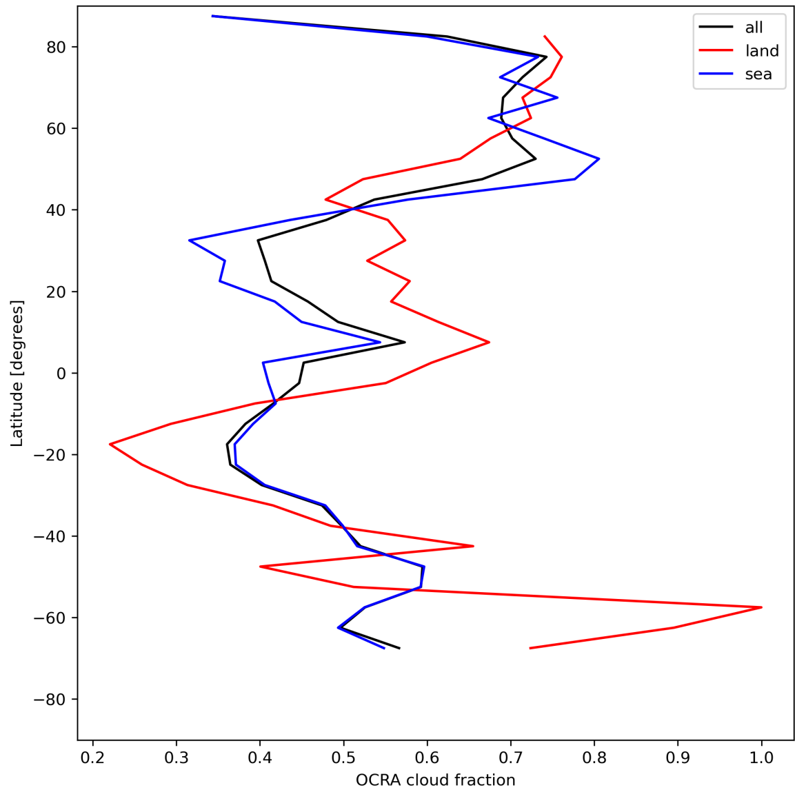
Figure 34: Zonal average of “OCRA cloud fraction” for 2024-07-21 to 2024-07-23.
