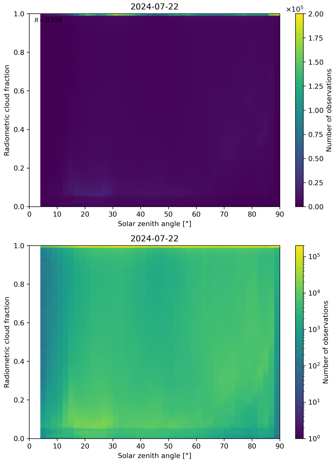
Figure 99: Scatter density plot of “Solar zenith angle” against “Radiometric cloud fraction” for 2024-07-21 to 2024-07-23.
