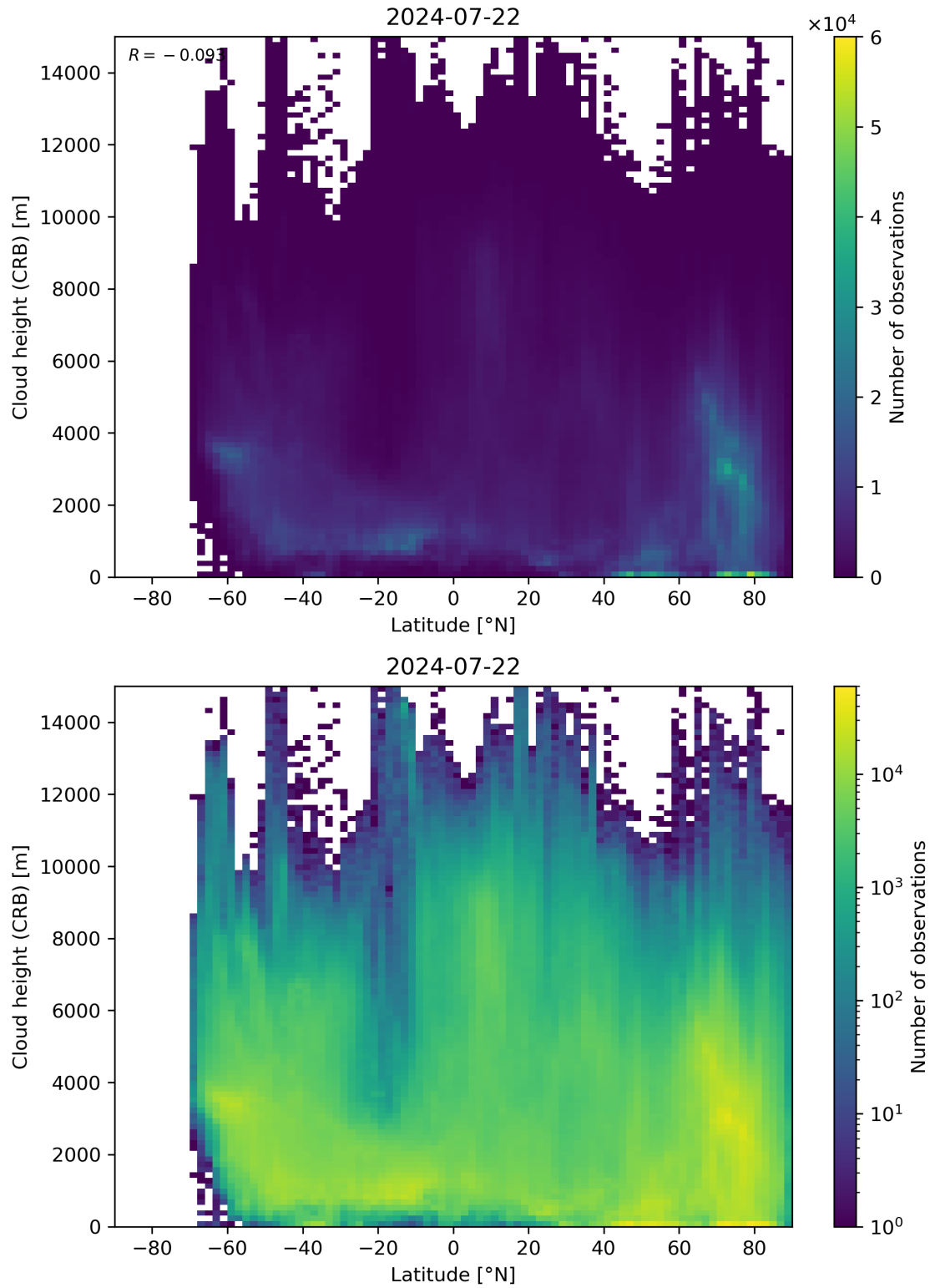
Figure 95: Scatter density plot of “Latitude” against “Cloud height (CRB)” for 2024-07-21 to 2024-07-23.
