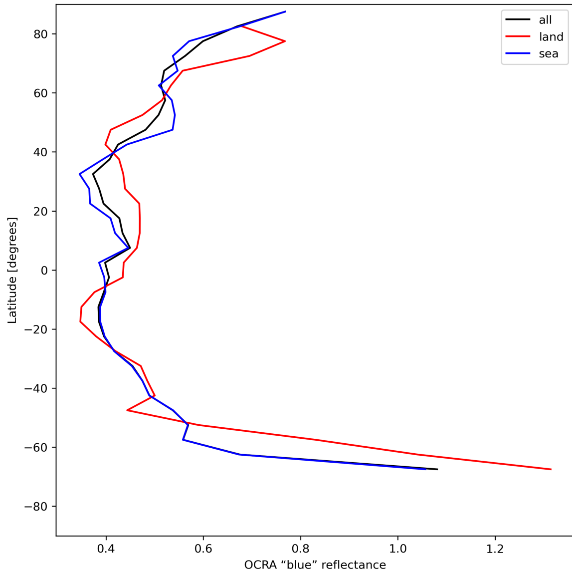
Figure 35: Zonal average of “OCRA “blue” reflectance” for 2024-07-21 to 2024-07-23.
