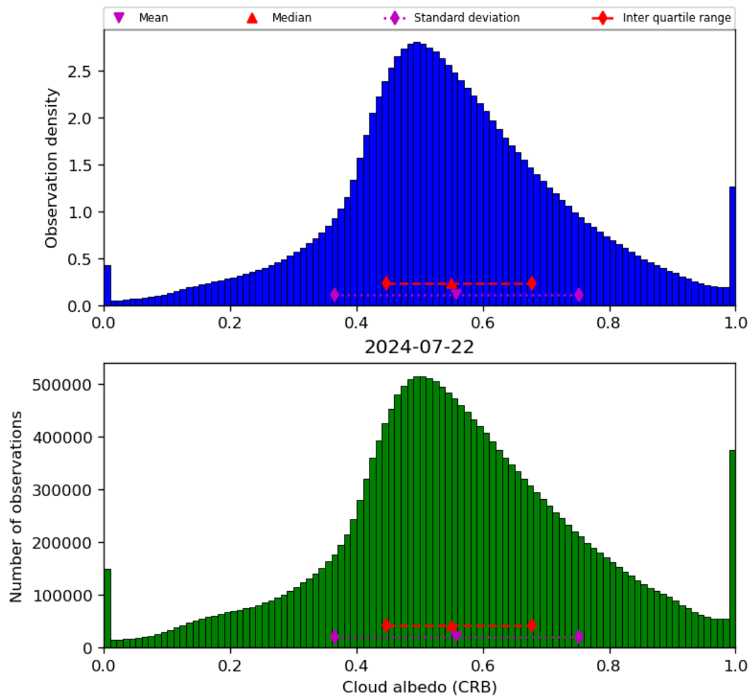
Figure 44: Histogram of “Cloud albedo (CRB)” for 2024-07-21 to 2024-07-23
