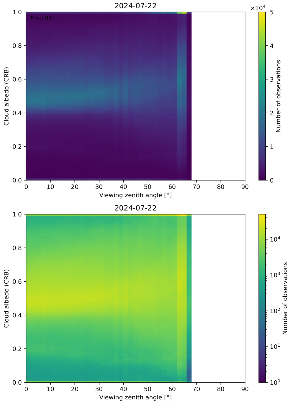
Figure 106: Scatter density plot of “Viewing zenith angle” against “Cloud albedo (CRB)” for 2024-07-21 to 2024-07-23.
