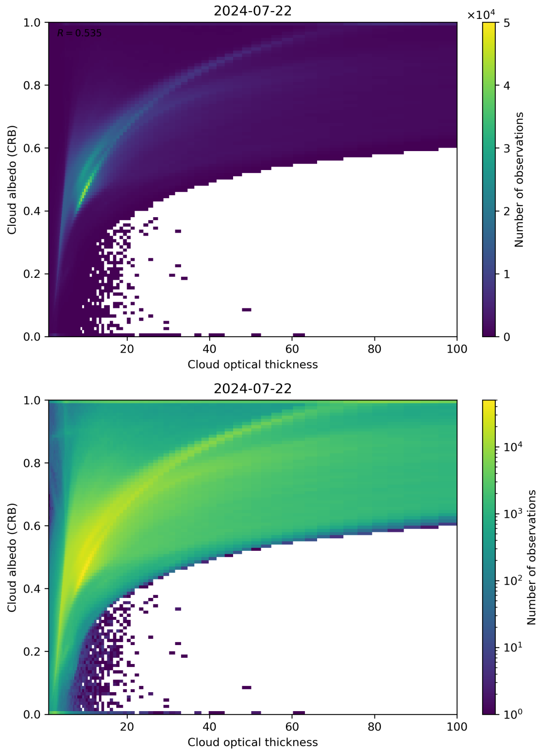
Figure 82: Scatter density plot of “Cloud optical thickness” against “Cloud albedo (CRB)” for 2024-07-21 to 2024-07-23.
