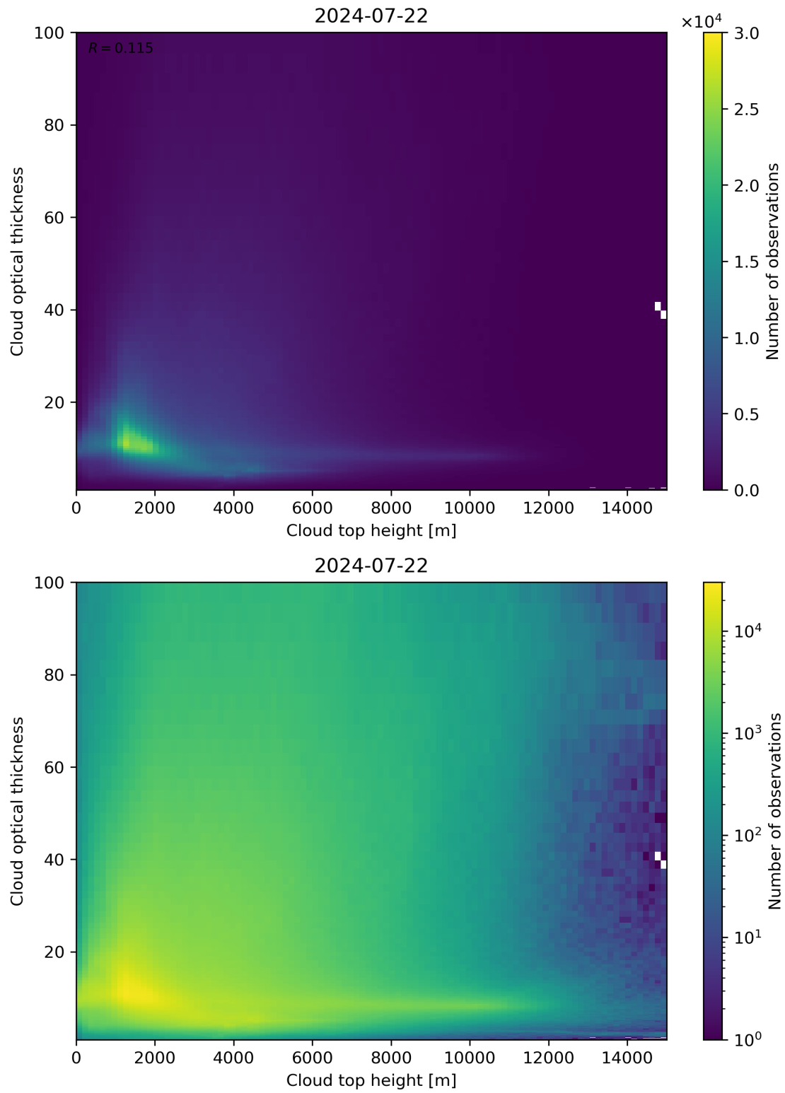
Figure 90: Scatter density plot of “Cloud top height” against “Cloud optical thickness” for 2024-07-21 to 2024-07-23.
