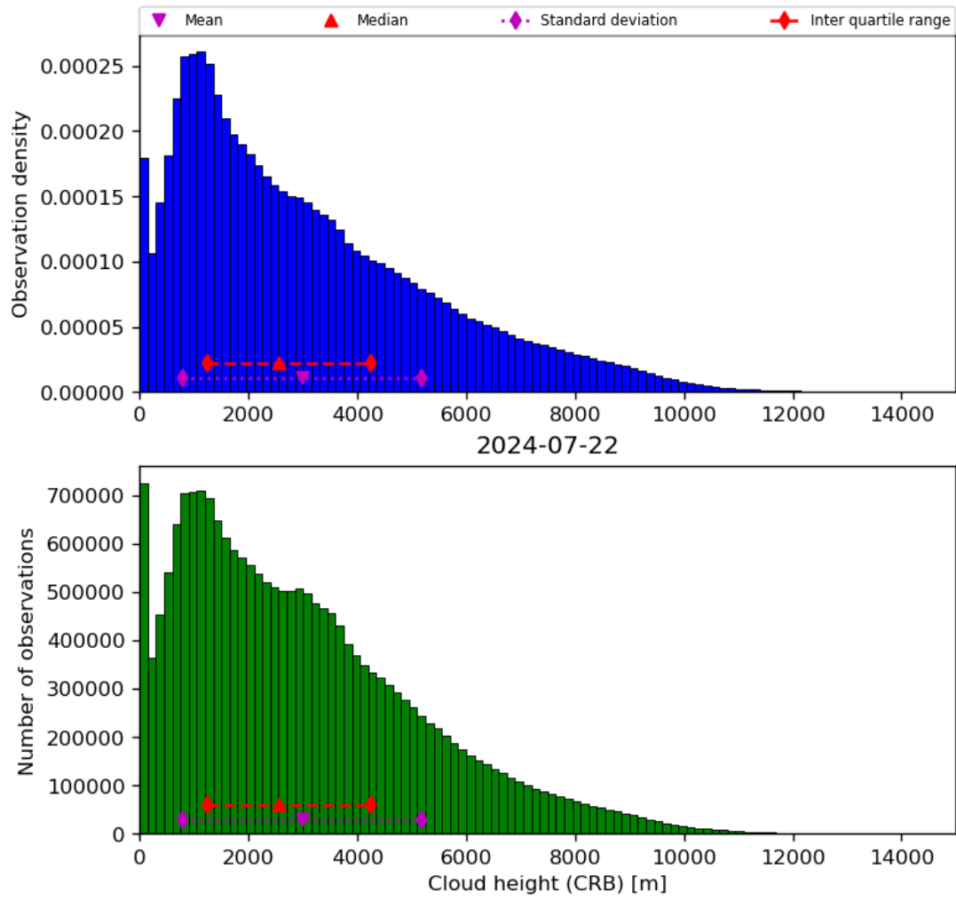
Figure 43: Histogram of “Cloud height (CRB)” for 2024-07-21 to 2024-07-23
