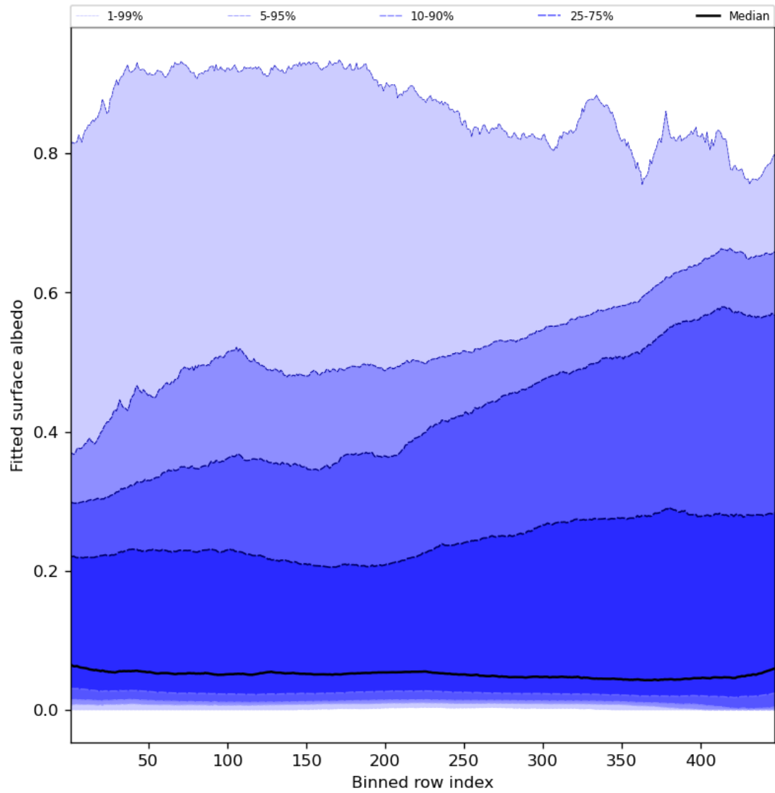
Figure 61: Along track statistics of “Fitted surface albedo” for 2024-07-21 to 2024-07-23
