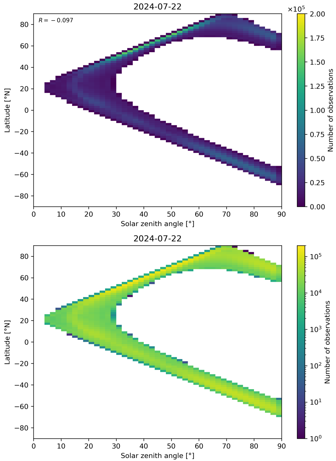
Figure 105: Scatter density plot of “Solar zenith angle” against “Latitude” for 2024-07-21 to 2024-07-23.
