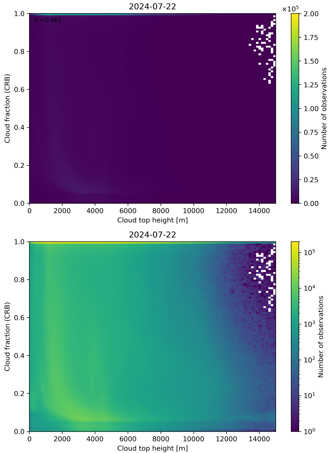
Figure 88: Scatter density plot of “Cloud top height” against “Cloud fraction (CRB)” for 2024-07-21 to 2024-07-23.
