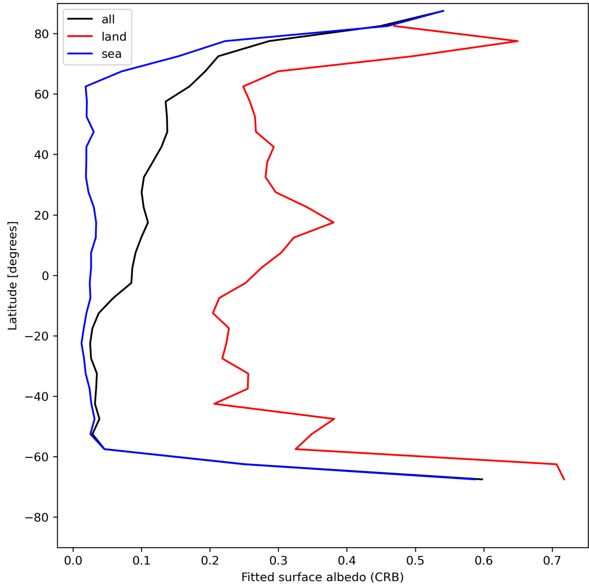
Figure 30: Zonal average of “Fitted surface albedo (CRB)” for 2024-07-21 to 2024-07-23.
