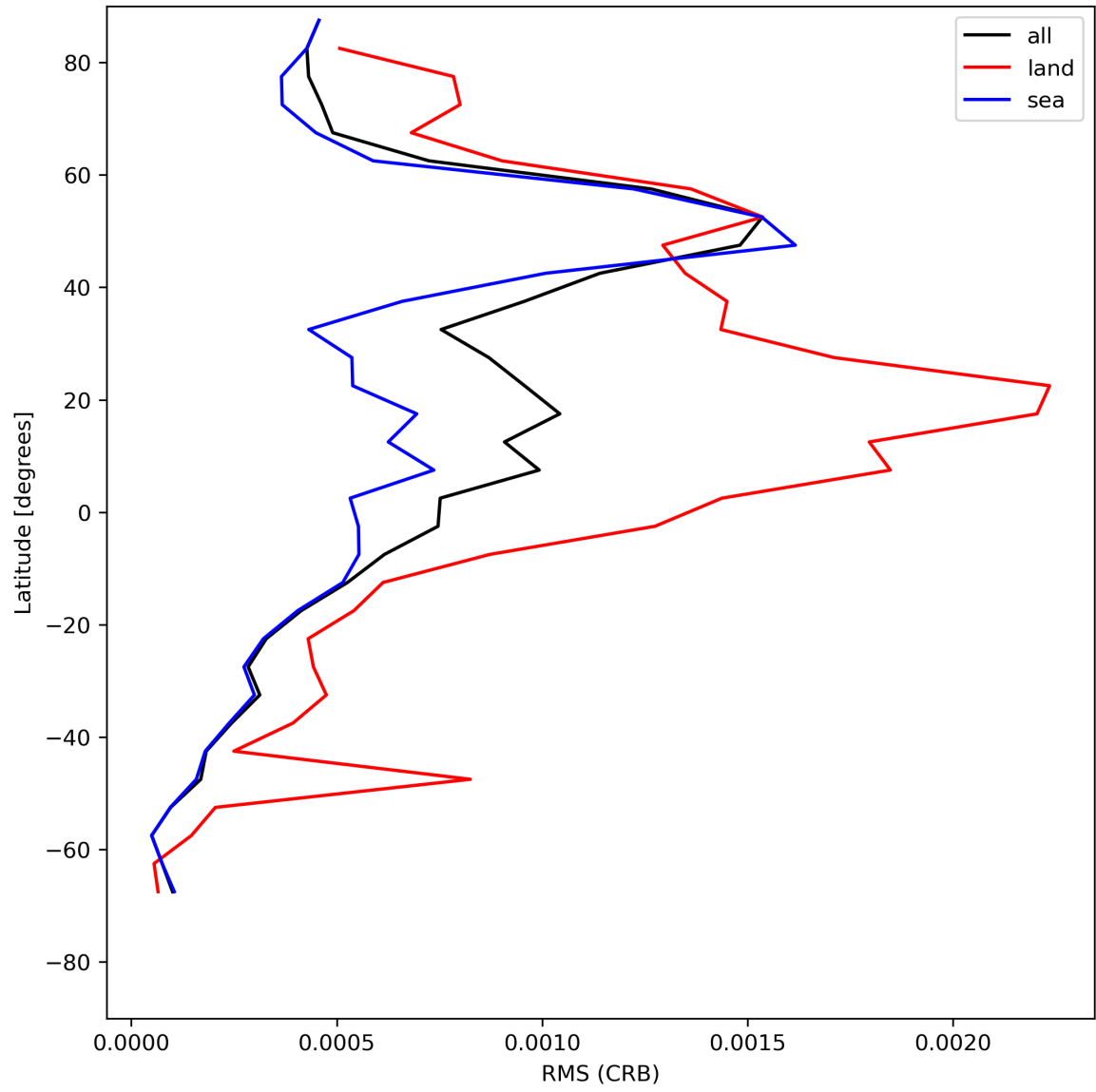
Figure 32: Zonal average of “RMS (CRB)” for 2024-07-21 to 2024-07-23.
