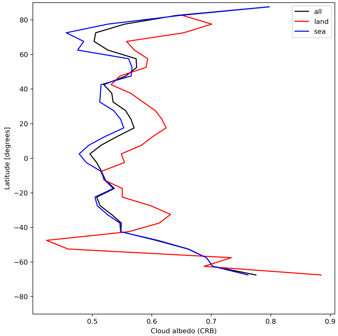
Figure 28: Zonal average of “Cloud albedo (CRB)” for 2024-07-21 to 2024-07-23.
