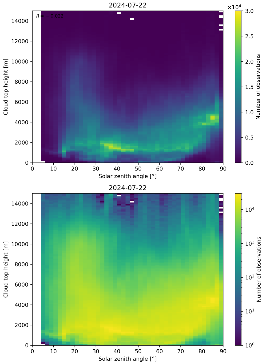
Figure 104: Scatter density plot of “Solar zenith angle” against “Cloud top height” for 2024-07-21 to 2024-07-23.
