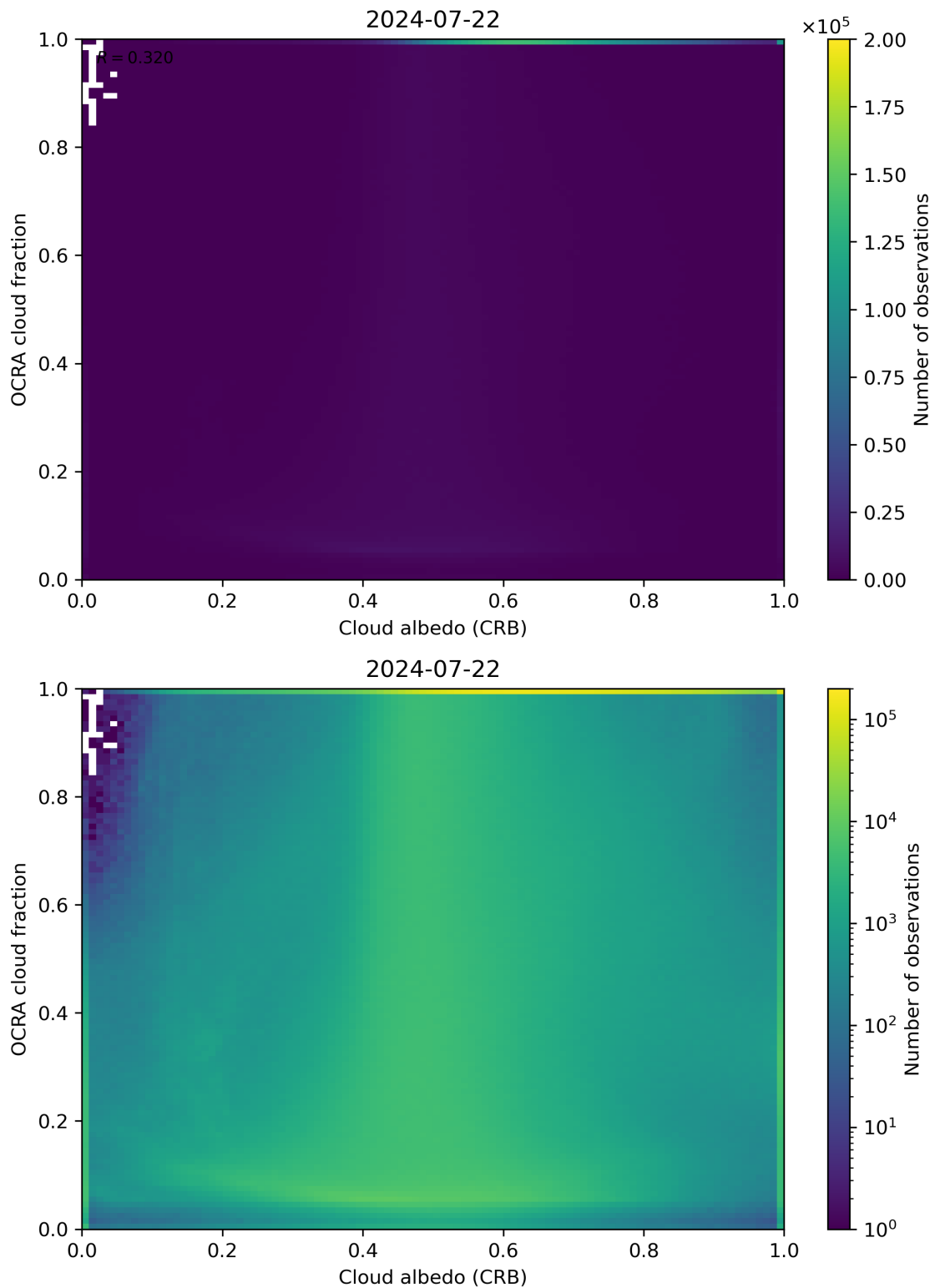
Figure 70: Scatter density plot of “Cloud albedo (CRB)” against “OCRA cloud fraction” for 2024-07-21 to 2024-07-23.
