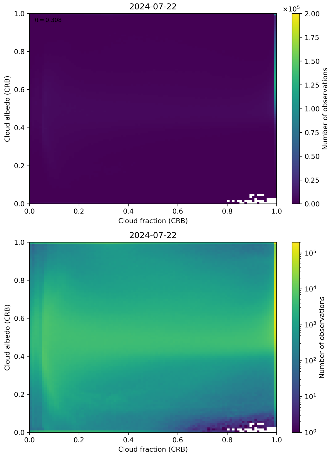
Figure 77: Scatter density plot of “Cloud fraction (CRB)” against “Cloud albedo (CRB)” for 2024-07-21 to 2024-07-23.
