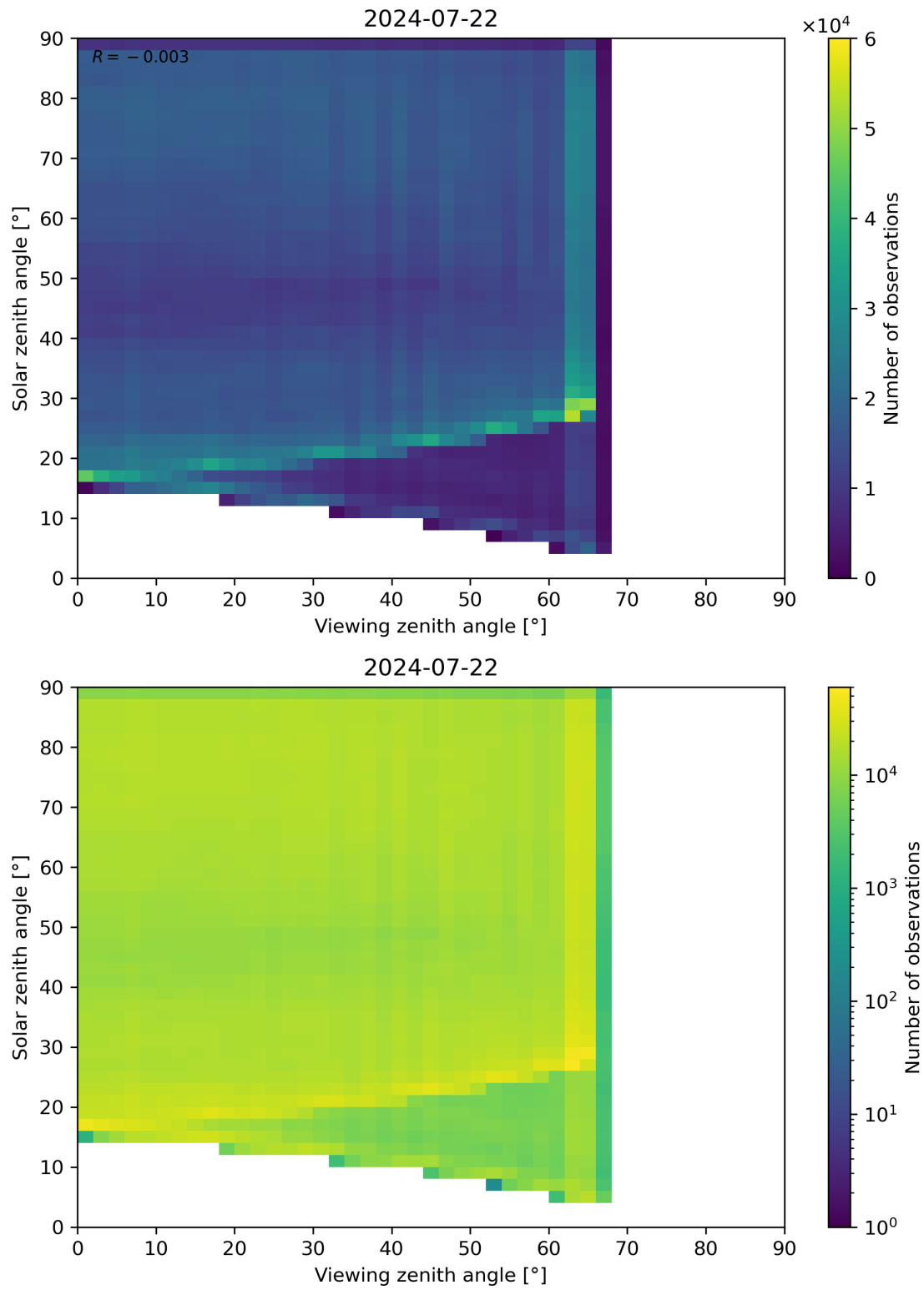
Figure 114: Scatter density plot of “Viewing zenith angle” against “Solar zenith angle” for 2024-07-21 to 2024-07-23.
