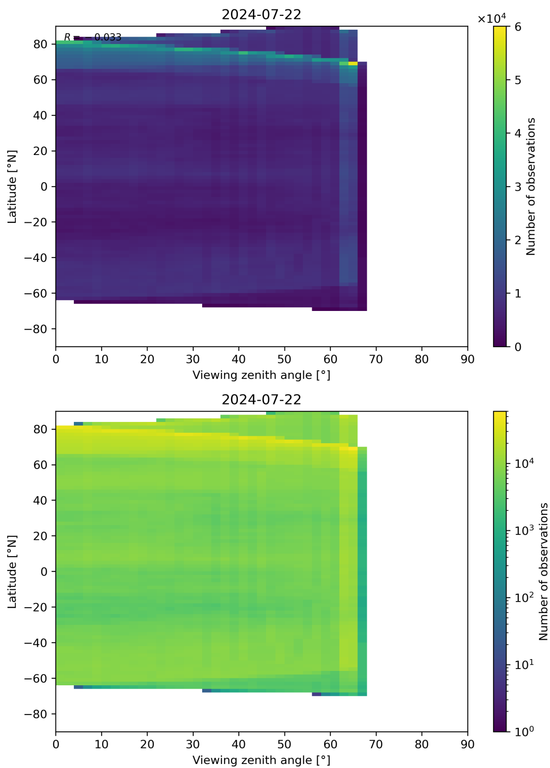
Figure 113: Scatter density plot of “Viewing zenith angle” against “Latitude” for 2024-07-21 to 2024-07-23.
