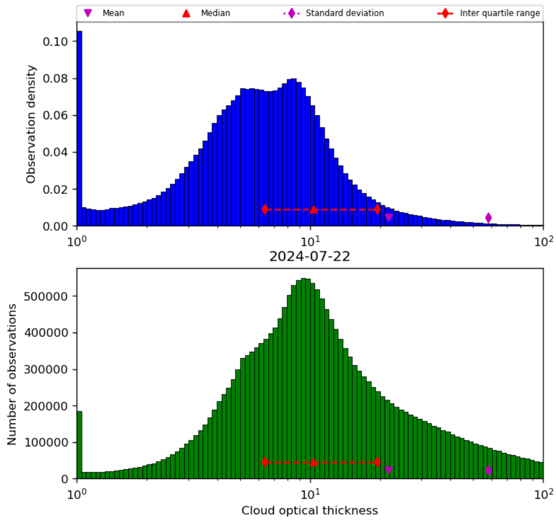
Figure 41: Histogram of “Cloud optical thickness” for 2024-07-21 to 2024-07-23
