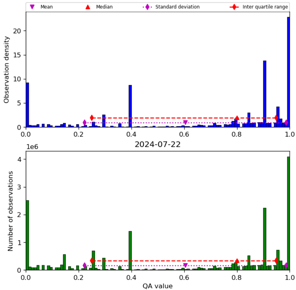
Figure 38: Histogram of “QA value” for 2024-07-21 to 2024-07-23
