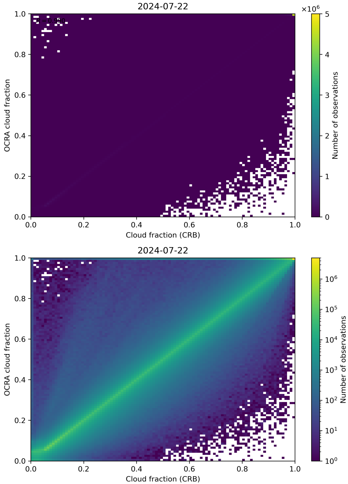
Figure 78: Scatter density plot of “Cloud fraction (CRB)” against “OCRA cloud fraction” for 2024-07-21 to 2024-07-23.
