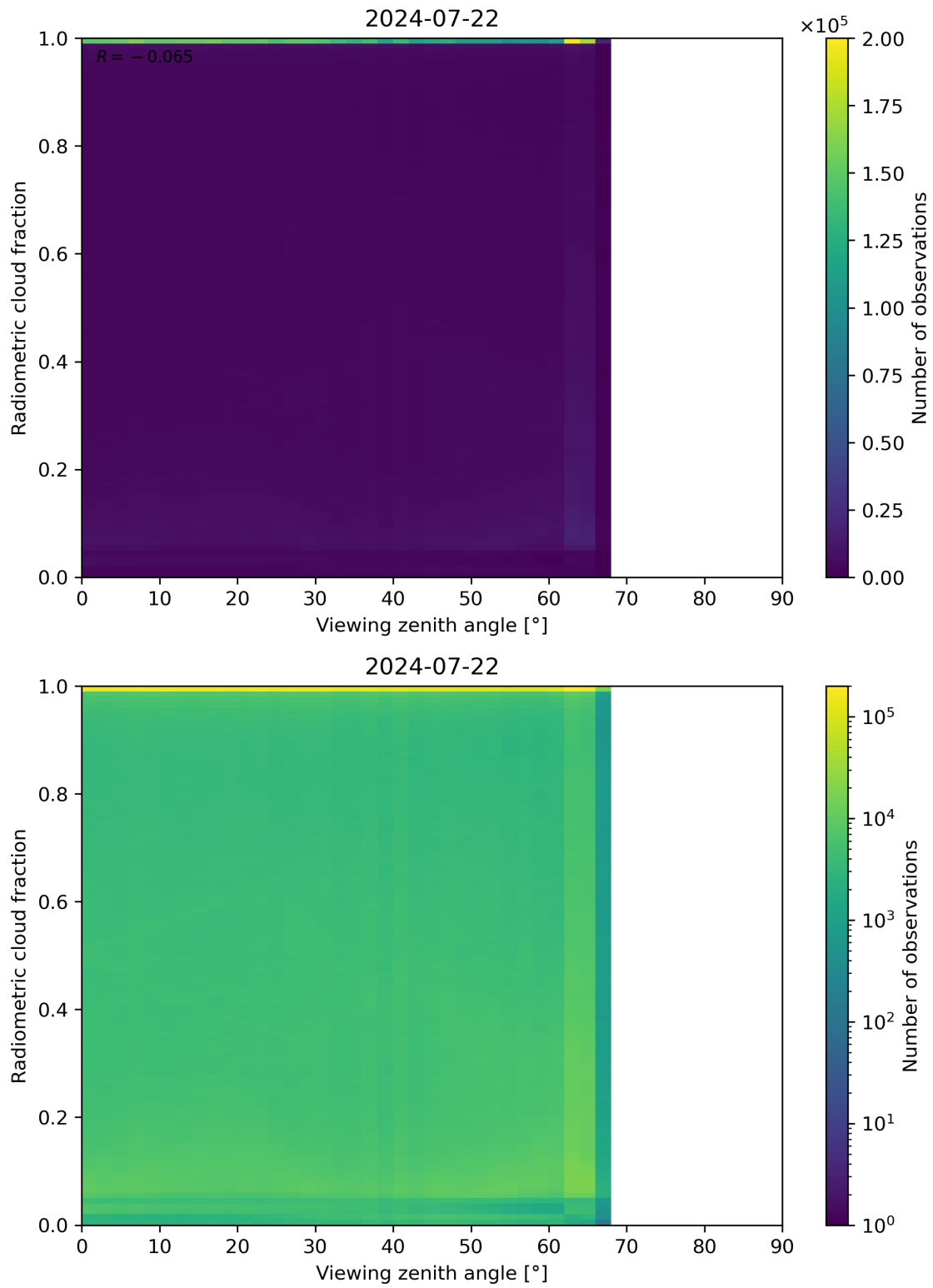
Figure 107: Scatter density plot of “Viewing zenith angle” against “Radiometric cloud fraction” for 2024-07-21 to 2024-07-23.
