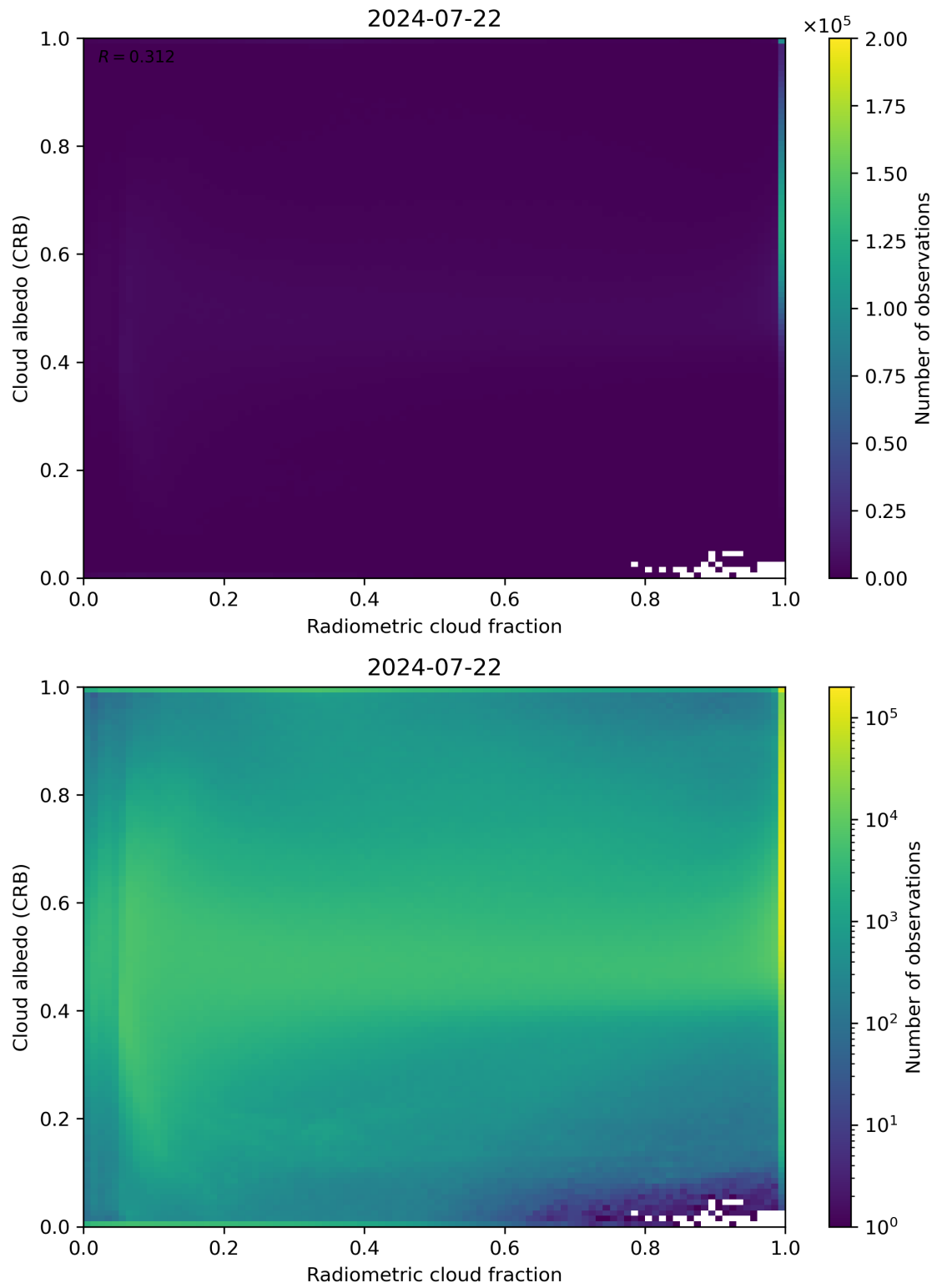
Figure 71: Scatter density plot of “Radiometric cloud fraction” against “Cloud albedo (CRB)” for 2024-07-21 to 2024-07-23.
