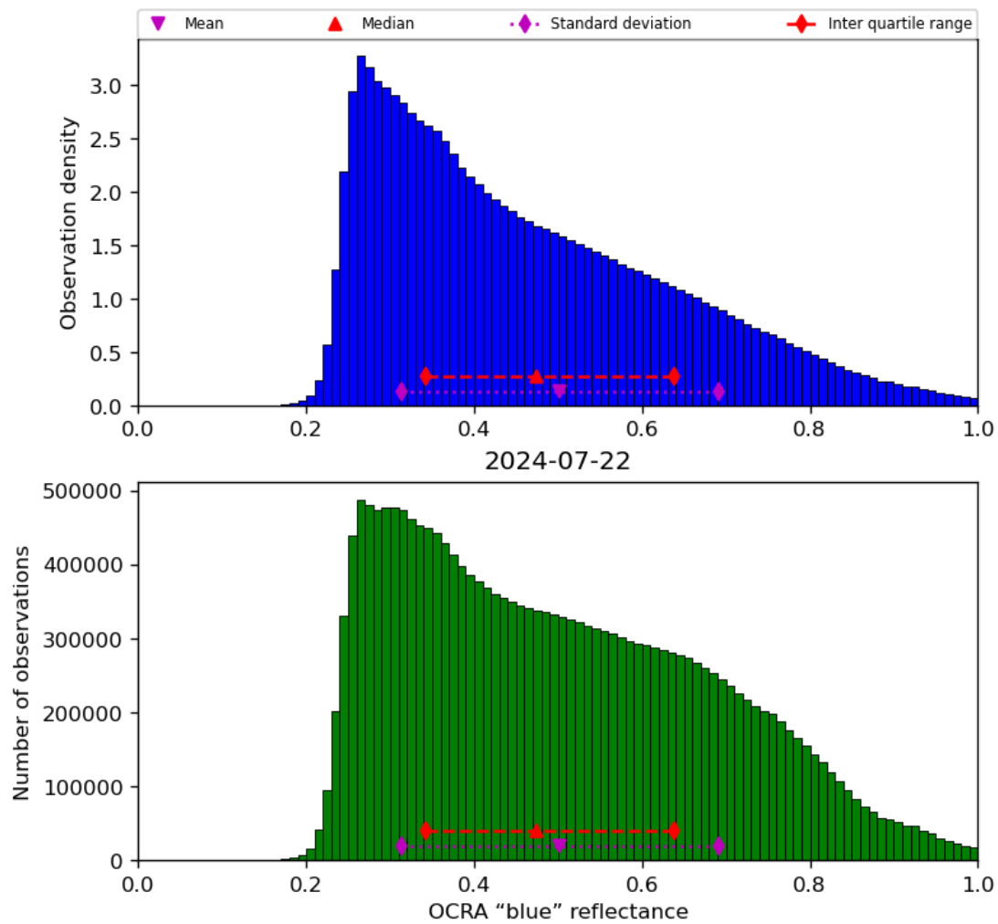
Figure 51: Histogram of “OCRA “blue” reflectance” for 2024-07-21 to 2024-07-23
