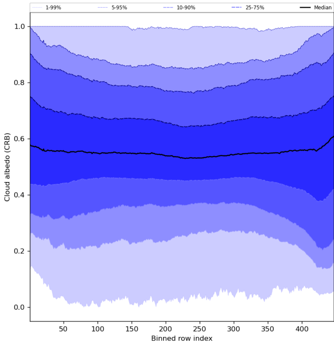
Figure 60: Along track statistics of “Cloud albedo (CRB)” for 2024-07-21 to 2024-07-23
