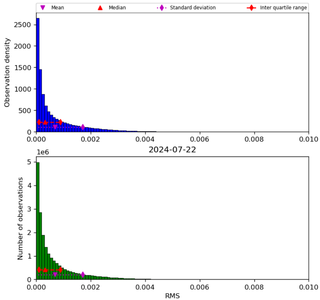
Figure 47: Histogram of “RMS” for 2024-07-21 to 2024-07-23
