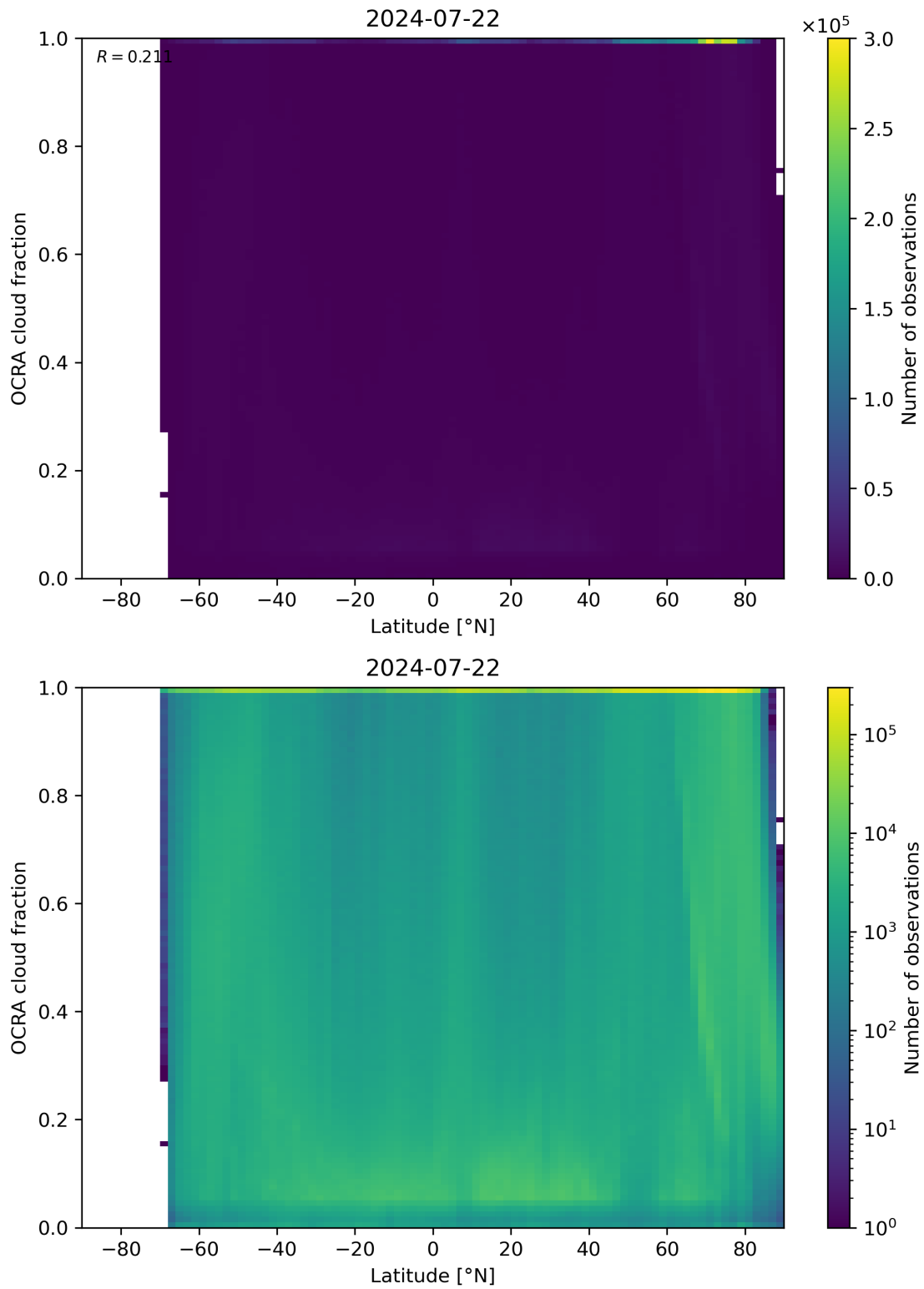
Figure 93: Scatter density plot of “Latitude” against “OCRA cloud fraction” for 2024-07-21 to 2024-07-23.
