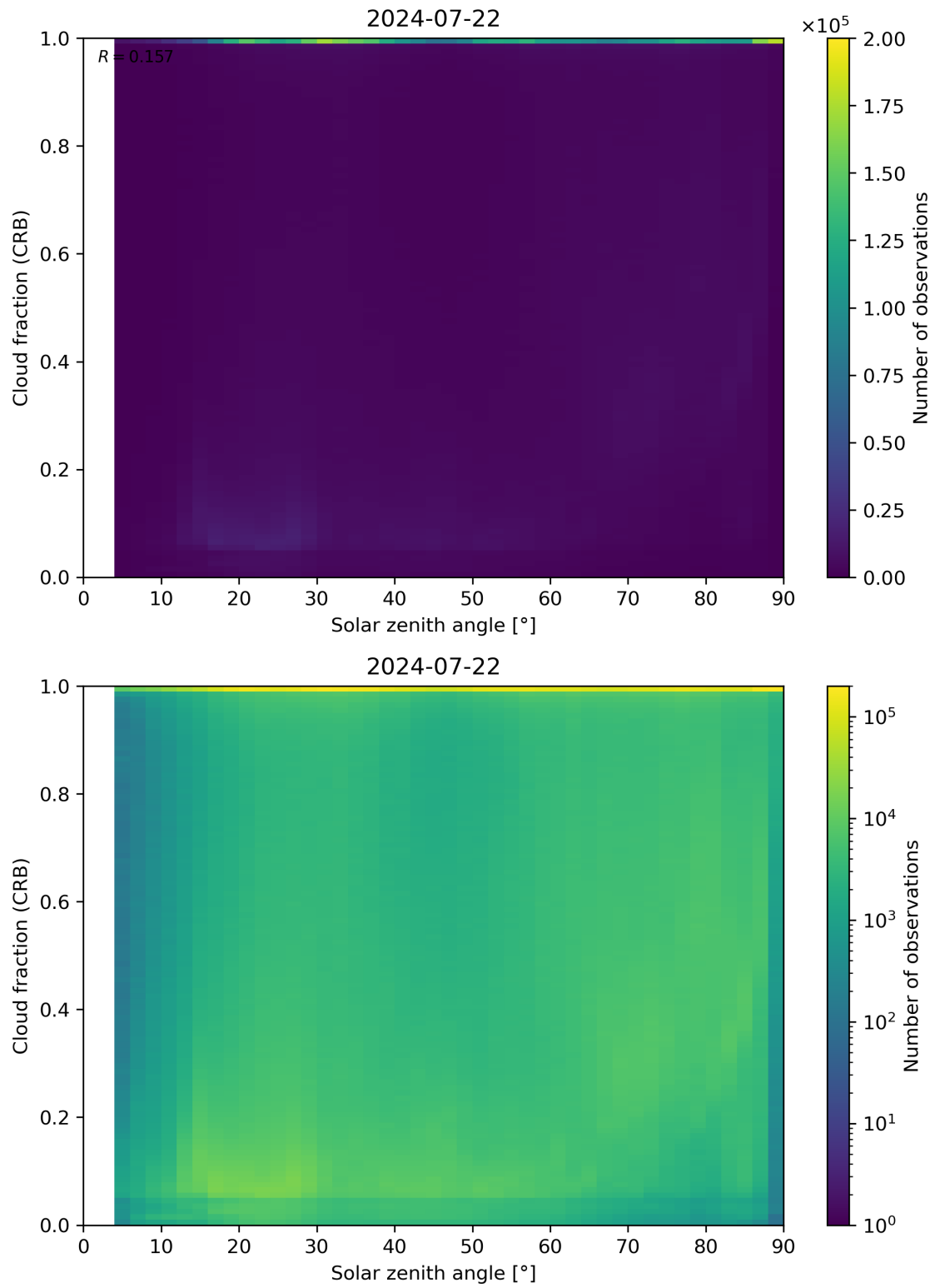
Figure 101: Scatter density plot of “Solar zenith angle” against “Cloud fraction (CRB)” for 2024-07-21 to 2024-07-23.
