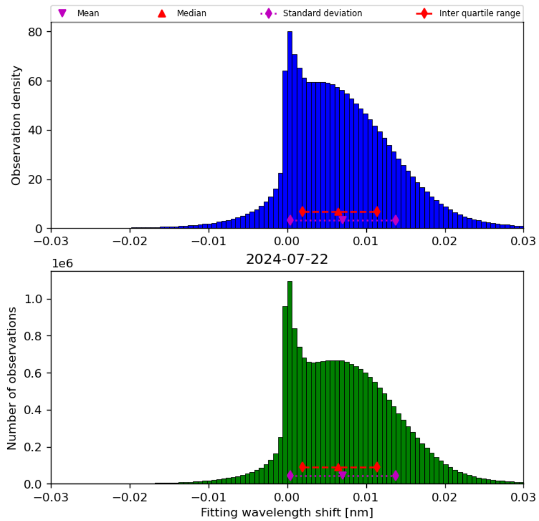
Figure 49: Histogram of “Fitting wavelength shift” for 2024-07-21 to 2024-07-23
