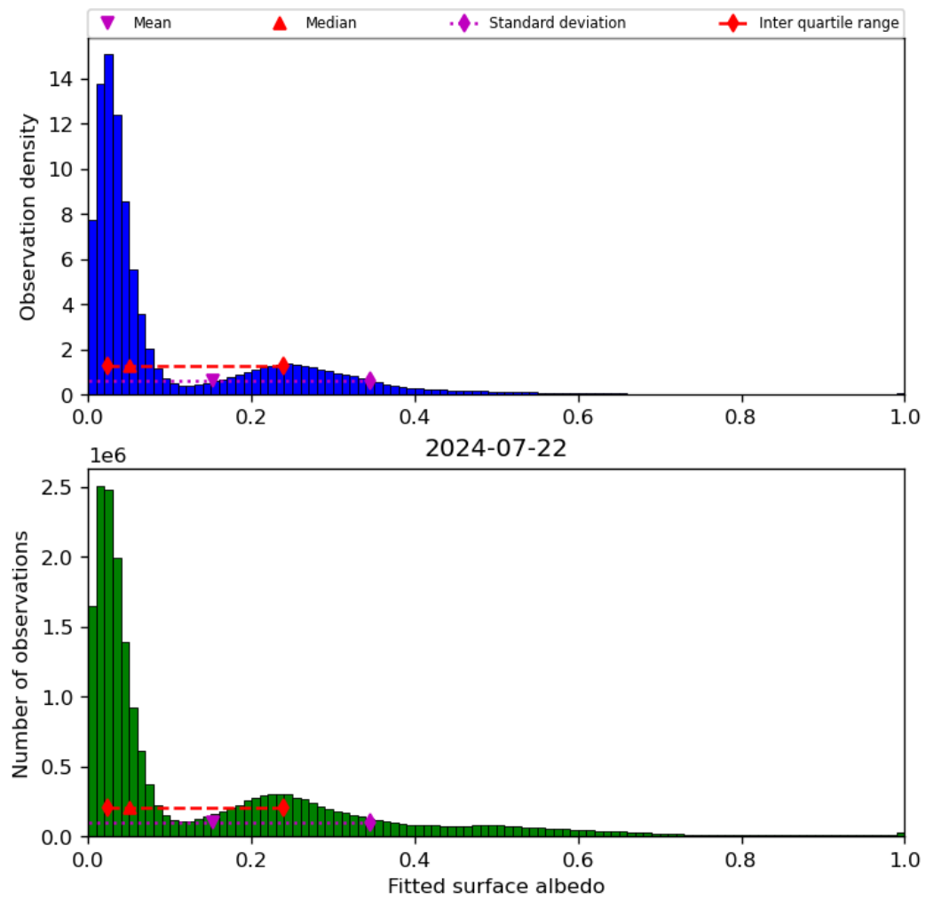
Figure 45: Histogram of “Fitted surface albedo” for 2024-07-21 to 2024-07-23
