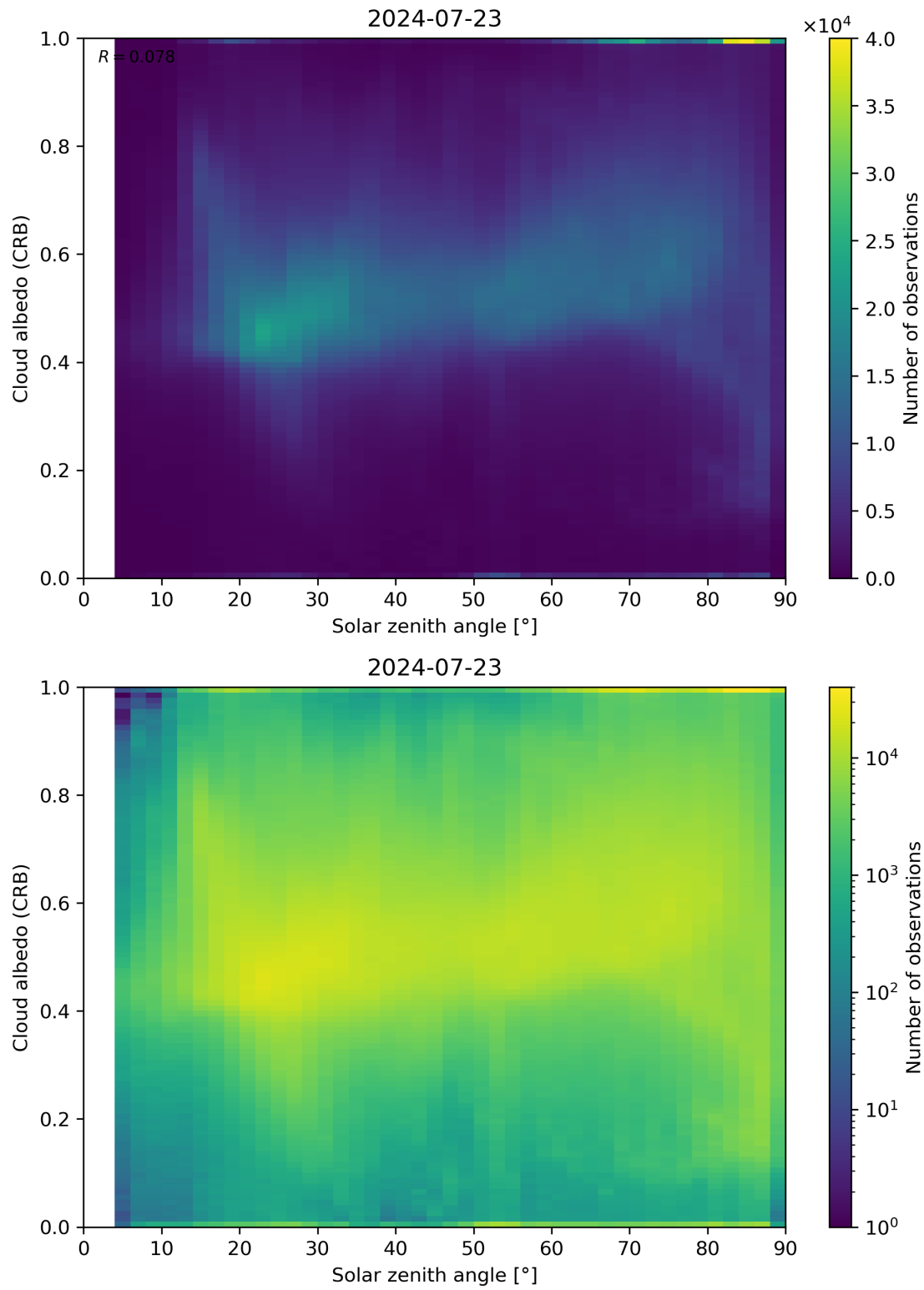
Figure 98: Scatter density plot of “Solar zenith angle” against “Cloud albedo (CRB)” for 2024-07-22 to 2024-07-24.
