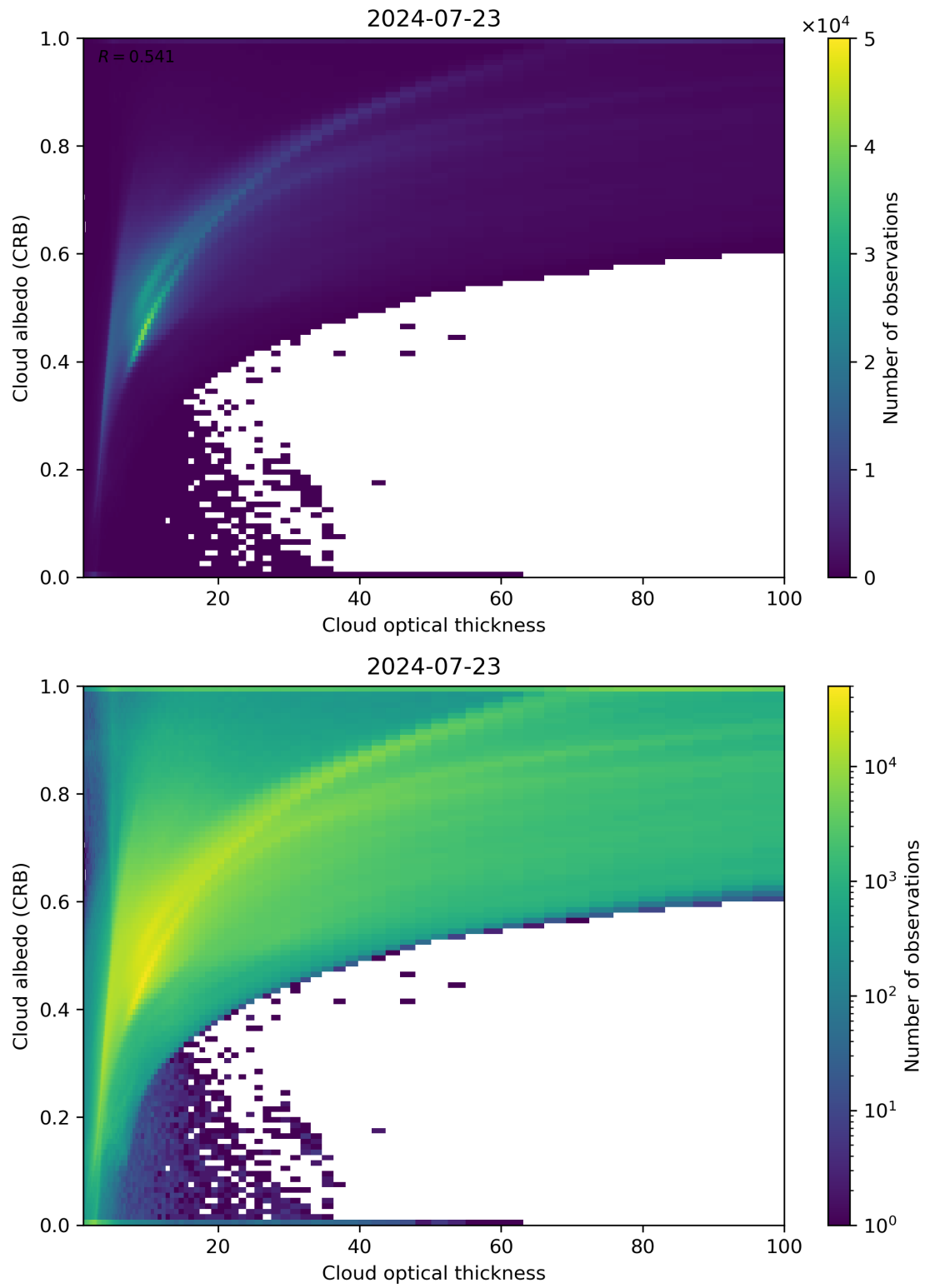
Figure 82: Scatter density plot of “Cloud optical thickness” against “Cloud albedo (CRB)” for 2024-07-22 to 2024-07-24.
