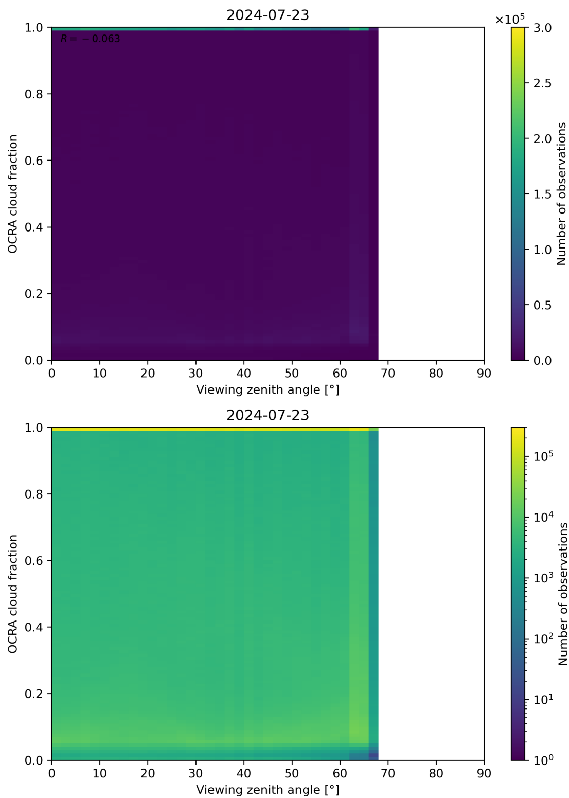
Figure 108: Scatter density plot of “Viewing zenith angle” against “OCRA cloud fraction” for 2024-07-22 to 2024-07-24.
