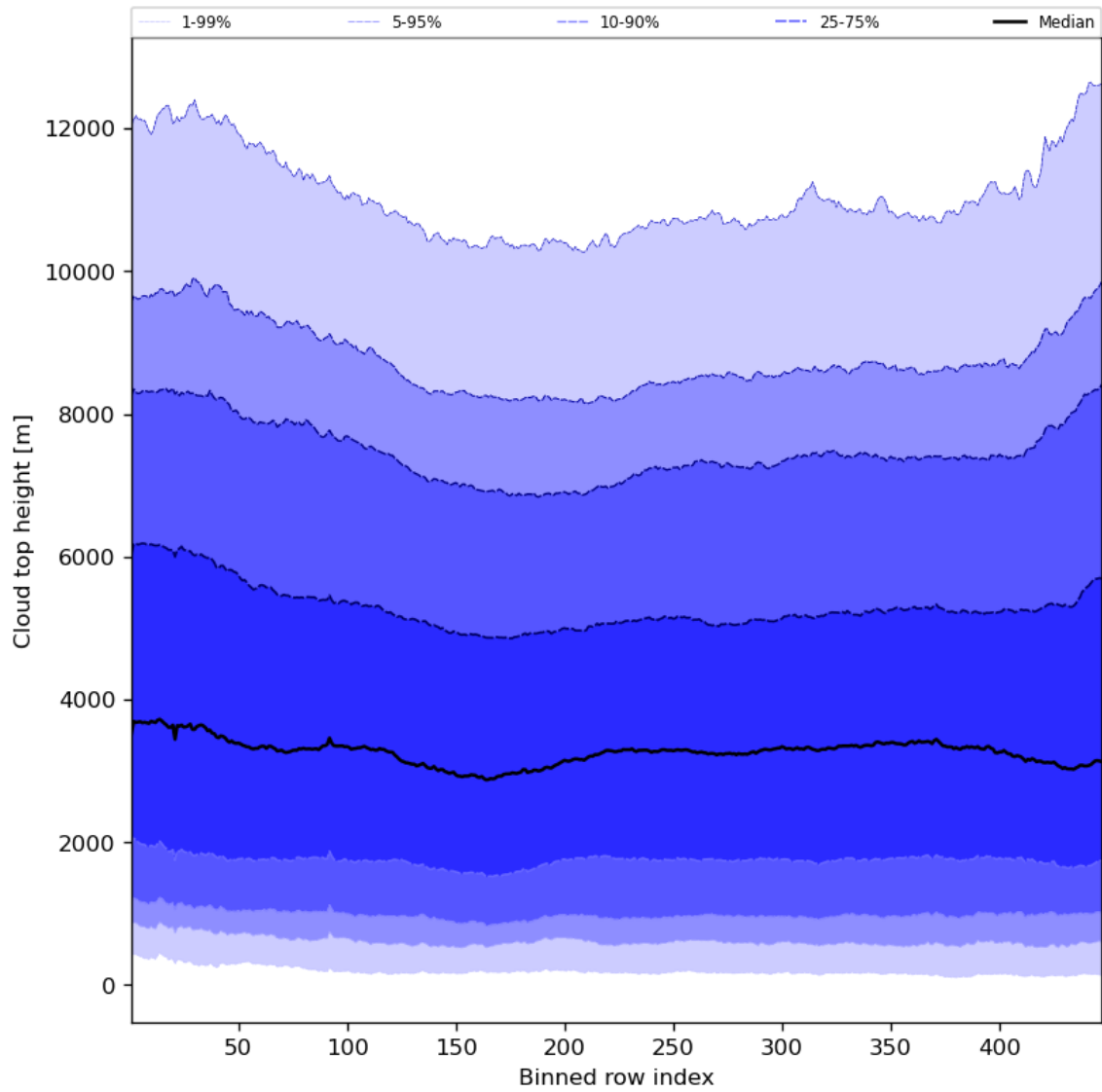
Figure 56: Along track statistics of “Cloud top height” for 2024-07-22 to 2024-07-24
