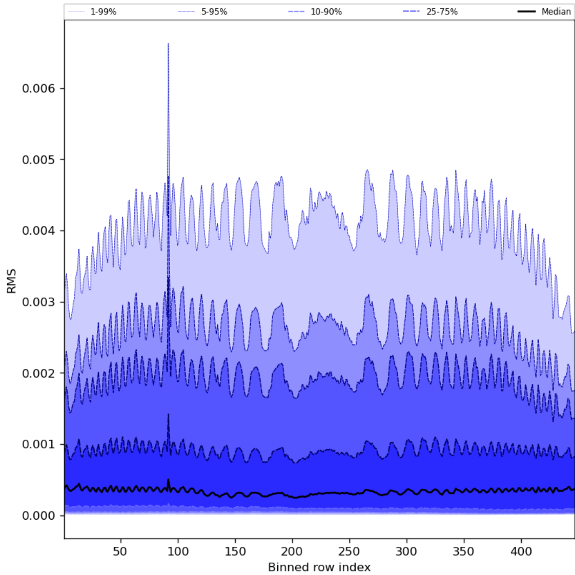
Figure 63: Along track statistics of “RMS” for 2024-07-22 to 2024-07-24
