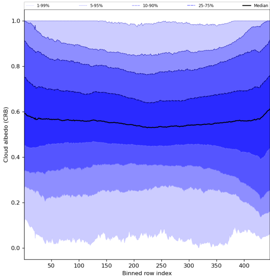
Figure 60: Along track statistics of “Cloud albedo (CRB)” for 2024-07-22 to 2024-07-24
