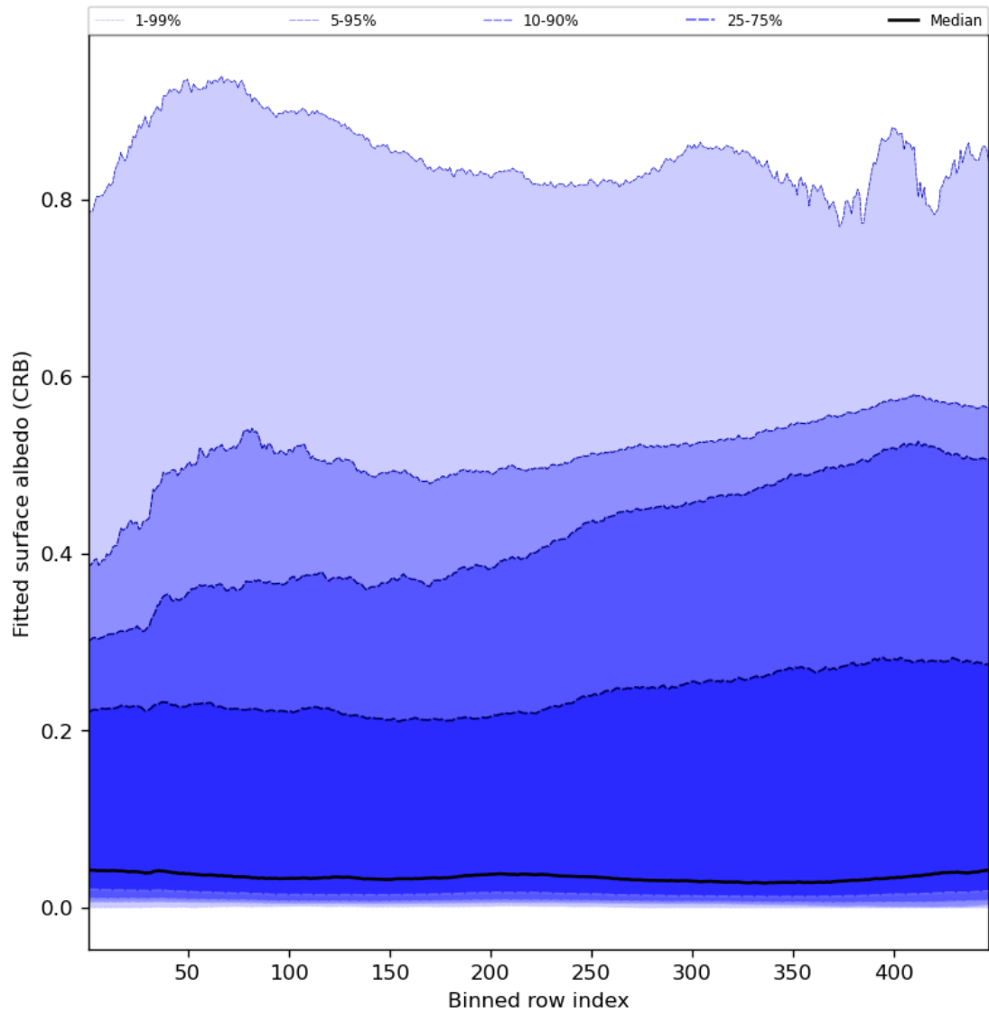
Figure 62: Along track statistics of “Fitted surface albedo (CRB)” for 2024-07-22 to 2024-07-24
