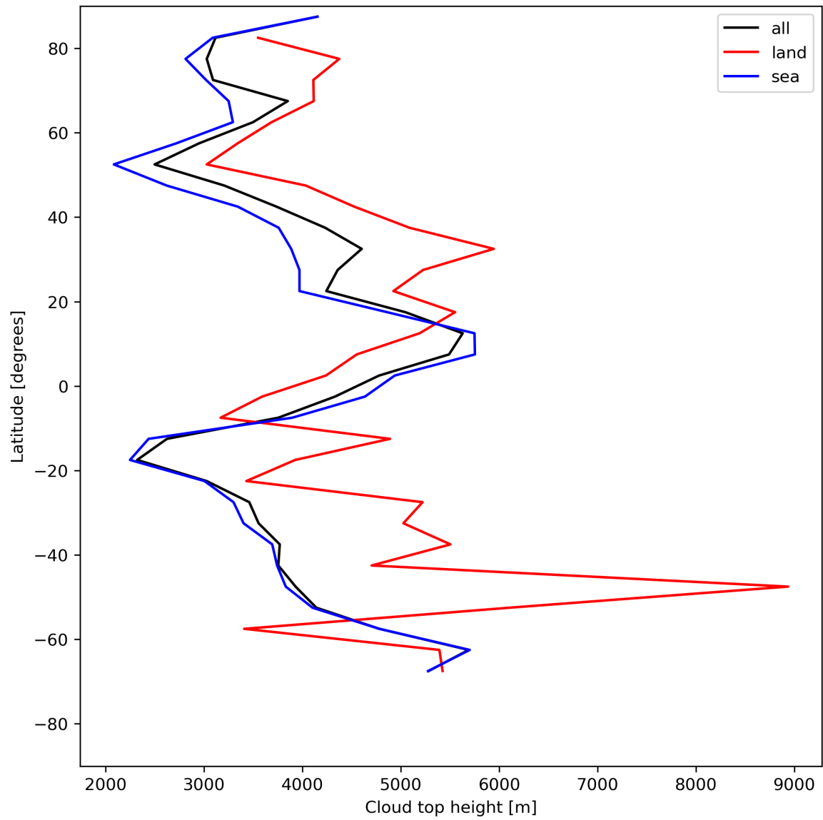
Figure 24: Zonal average of “Cloud top height” for 2024-07-22 to 2024-07-24.
