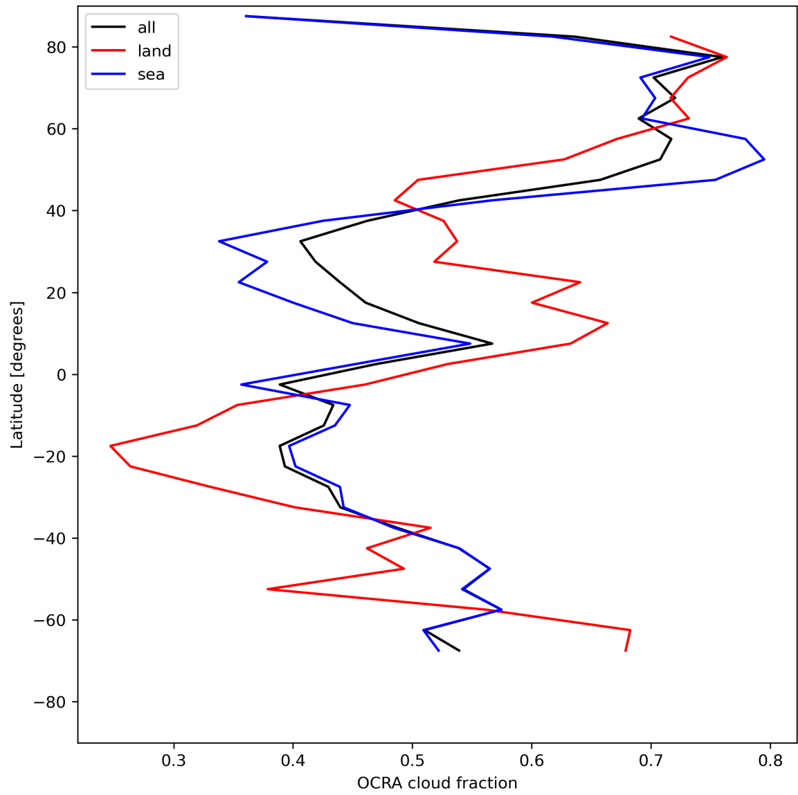
Figure 34: Zonal average of “OCRA cloud fraction” for 2024-07-22 to 2024-07-24.
