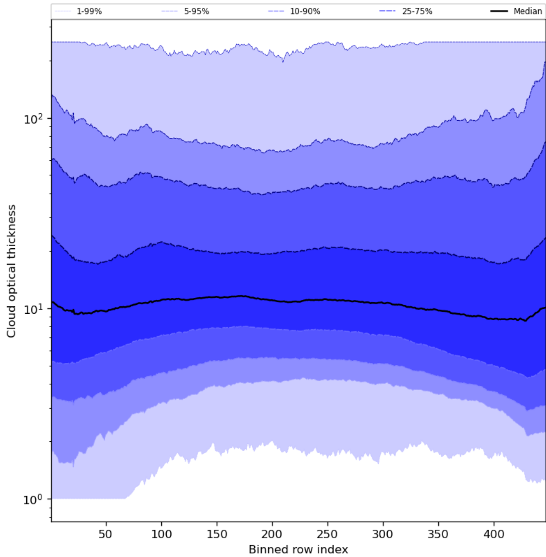
Figure 57: Along track statistics of “Cloud optical thickness” for 2024-07-22 to 2024-07-24
