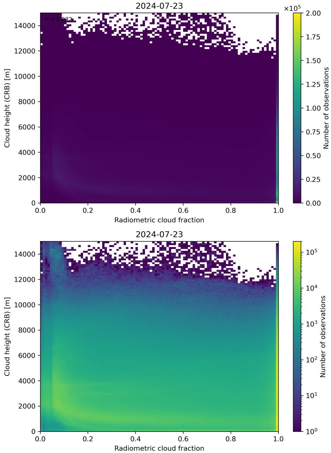
Figure 74: Scatter density plot of “Radiometric cloud fraction” against “Cloud height (CRB)” for 2024-07-22 to 2024-07-24.
