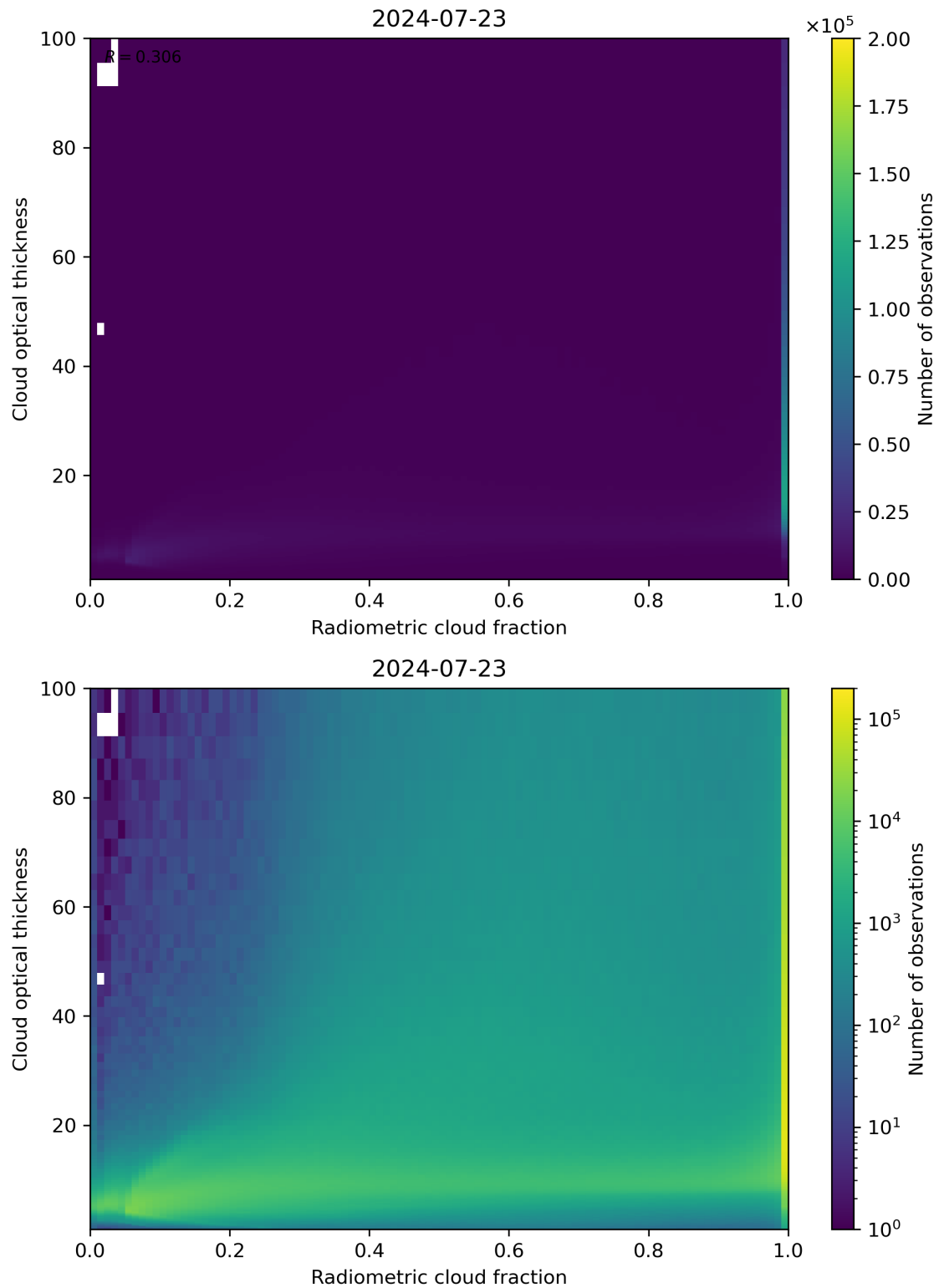
Figure 75: Scatter density plot of “Radiometric cloud fraction” against “Cloud optical thickness” for 2024-07-22 to 2024-07-24.
