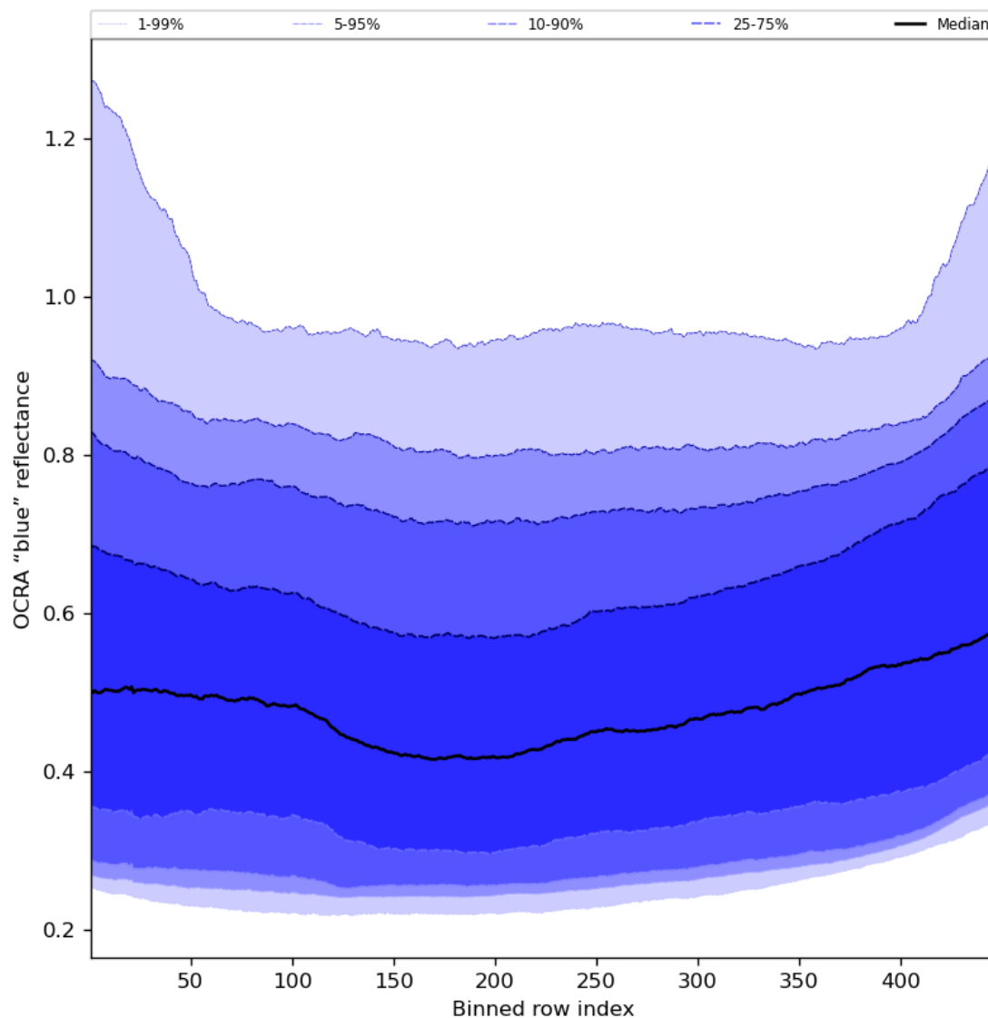
Figure 67: Along track statistics of “OCRA “blue” reflectance” for 2024-07-22 to 2024-07-24
