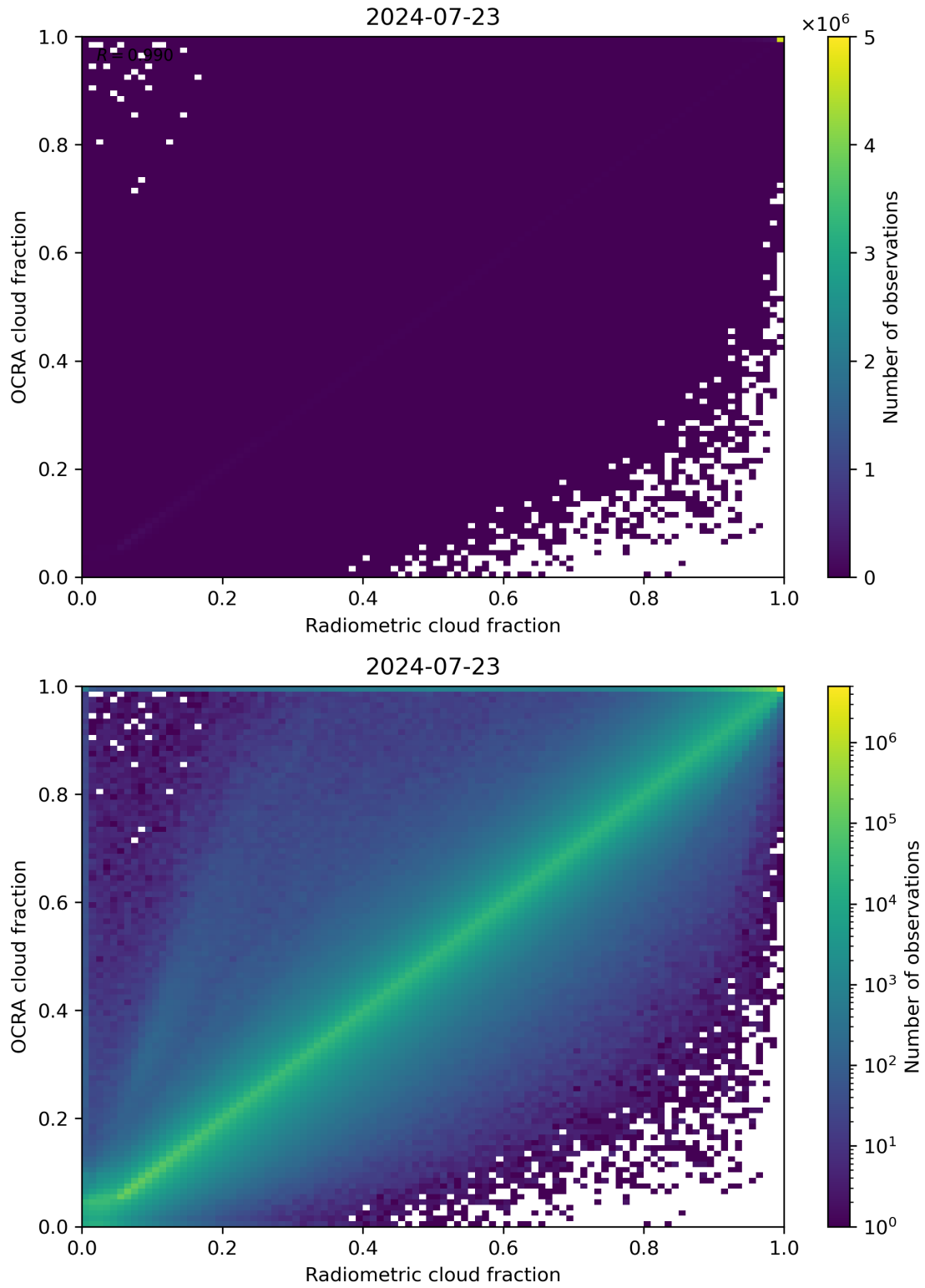
Figure 72: Scatter density plot of “Radiometric cloud fraction” against “OCRA cloud fraction” for 2024-07-22 to 2024-07-24.
