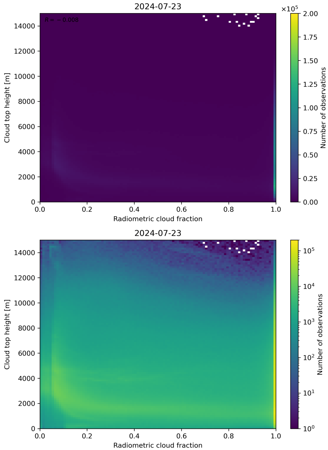
Figure 76: Scatter density plot of “Radiometric cloud fraction” against “Cloud top height” for 2024-07-22 to 2024-07-24.
