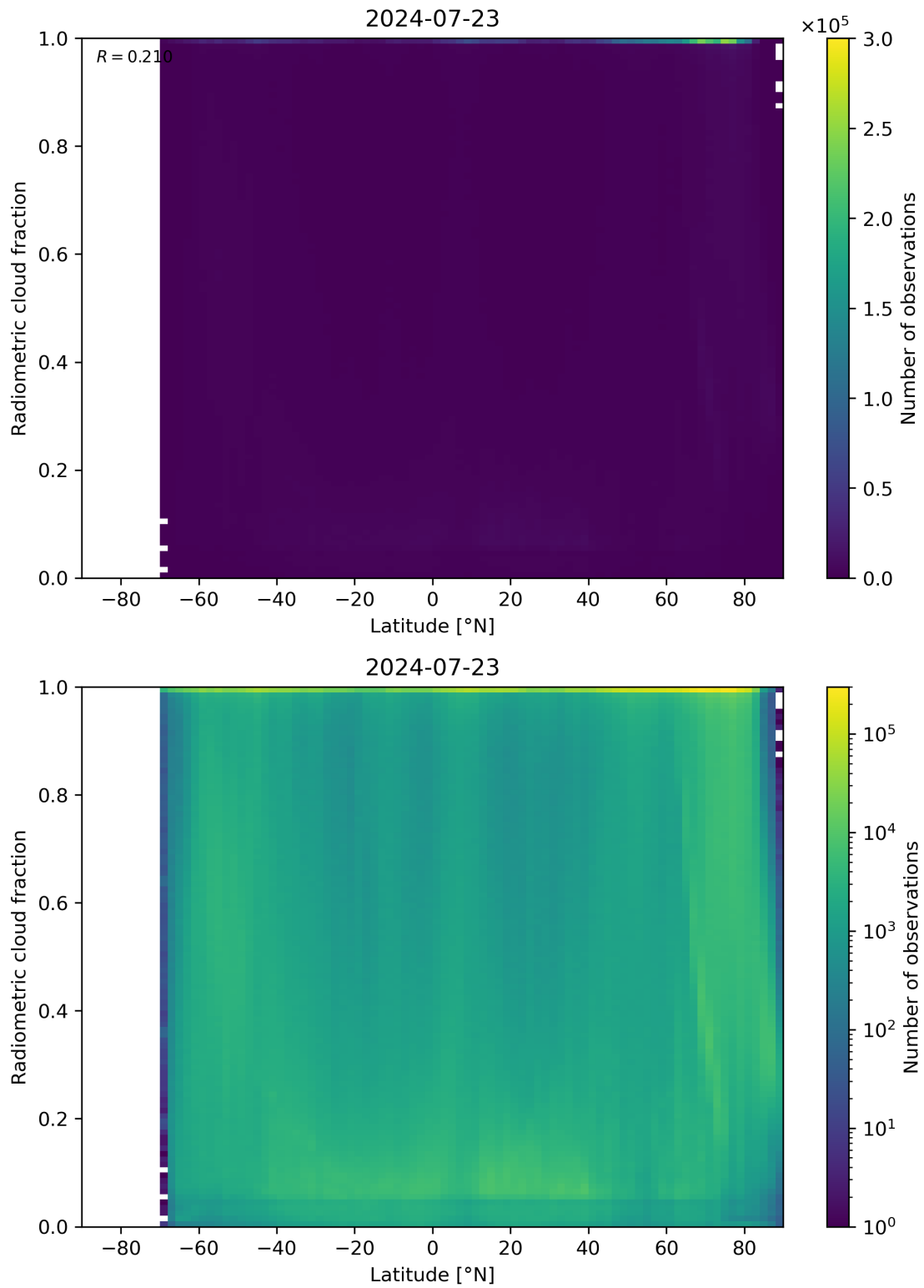
Figure 92: Scatter density plot of “Latitude” against “Radiometric cloud fraction” for 2024-07-22 to 2024-07-24.
