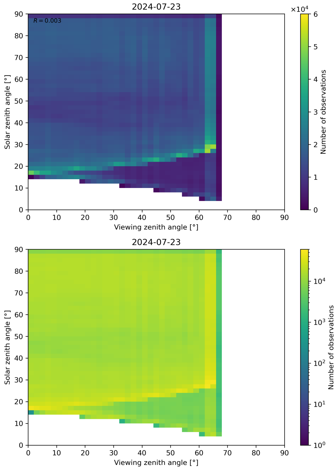
Figure 114: Scatter density plot of “Viewing zenith angle” against “Solar zenith angle” for 2024-07-22 to 2024-07-24.
