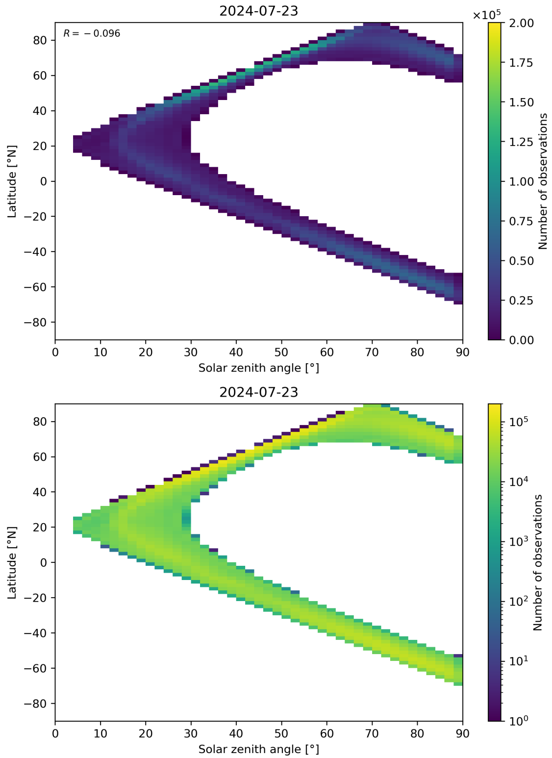
Figure 105: Scatter density plot of “Solar zenith angle” against “Latitude” for 2024-07-22 to 2024-07-24.
