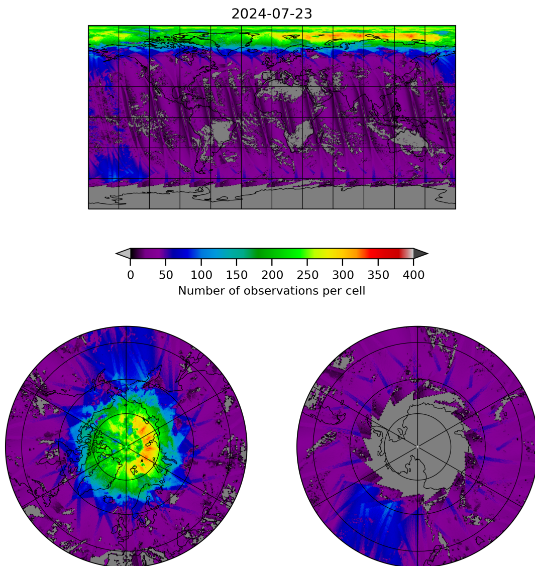
Figure 21: Map of the number of observations for 2024-07-22 to 2024-07-24
