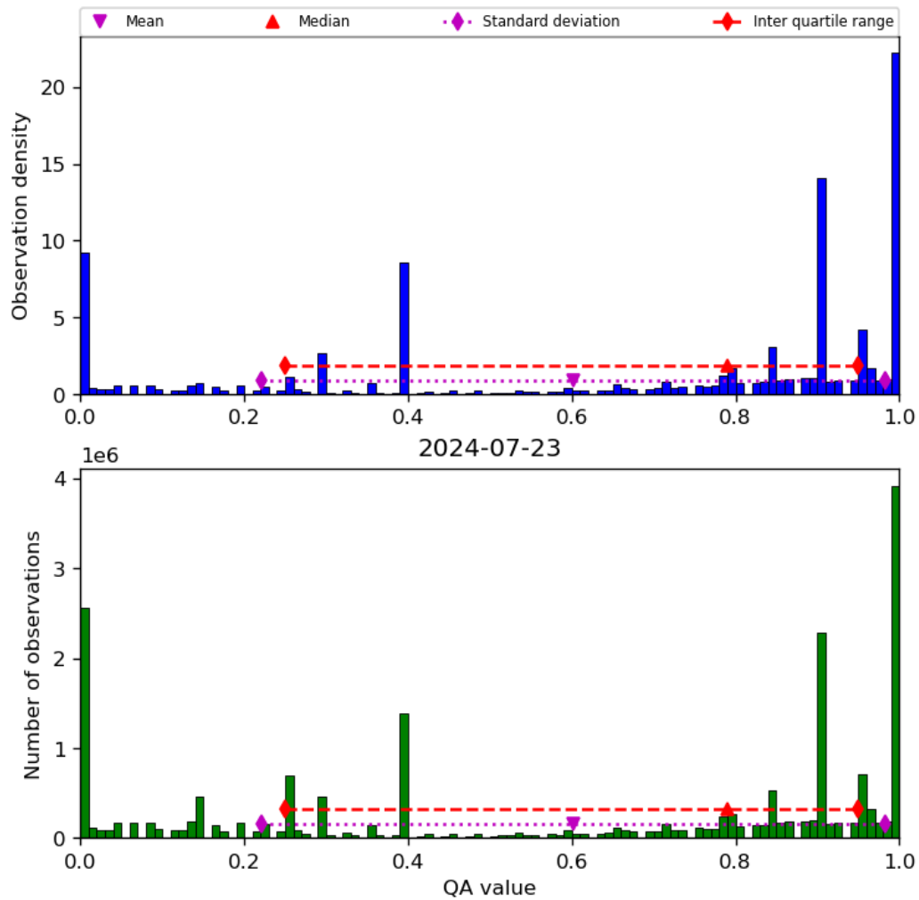
Figure 38: Histogram of “QA value” for 2024-07-22 to 2024-07-24
