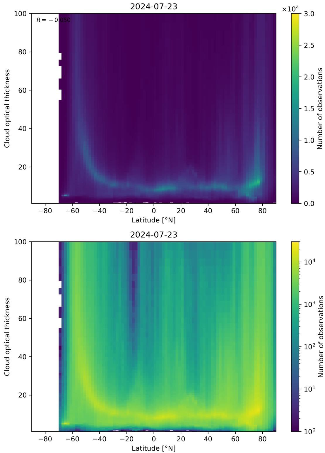
Figure 96: Scatter density plot of “Latitude” against “Cloud optical thickness” for 2024-07-22 to 2024-07-24.
