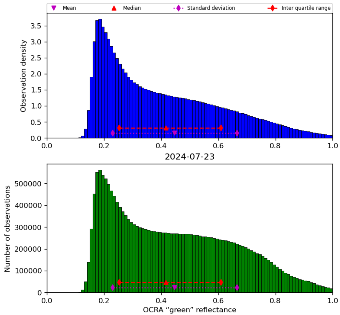
Figure 52: Histogram of “OCRA “green” reflectance” for 2024-07-22 to 2024-07-24
