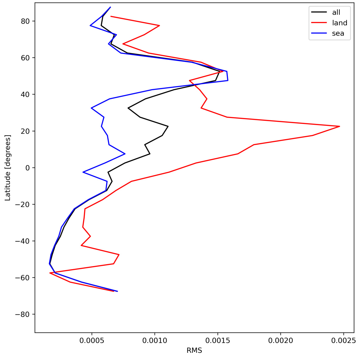
Figure 31: Zonal average of “RMS” for 2024-07-22 to 2024-07-24.
