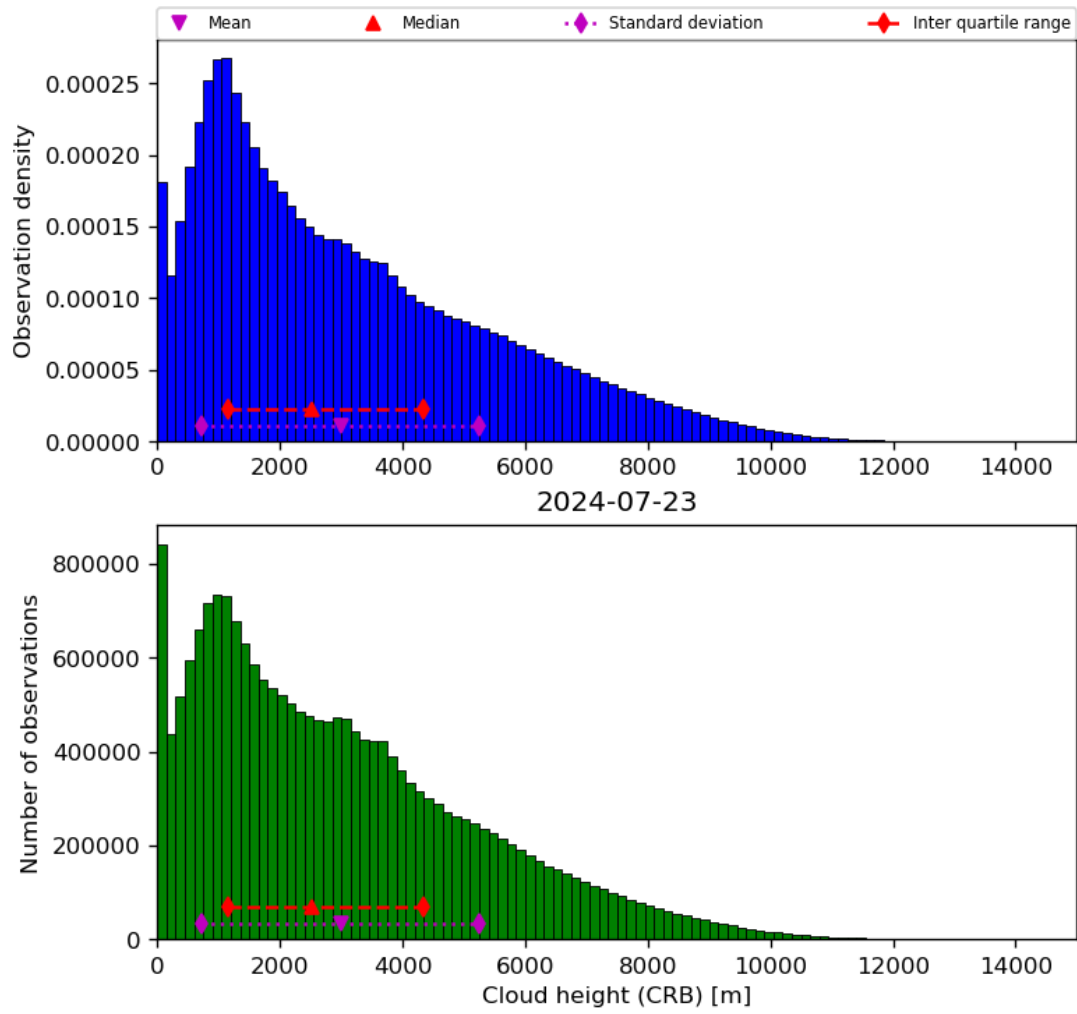
Figure 43: Histogram of “Cloud height (CRB)” for 2024-07-22 to 2024-07-24
