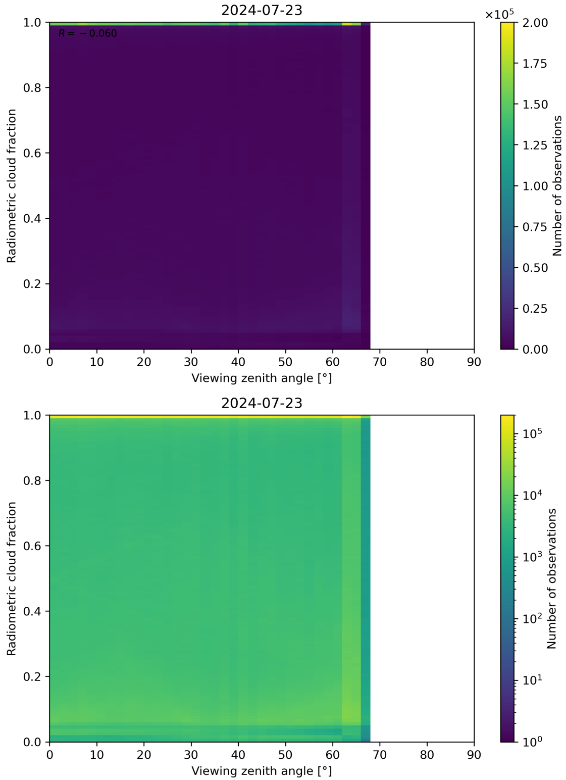
Figure 107: Scatter density plot of “Viewing zenith angle” against “Radiometric cloud fraction” for 2024-07-22 to 2024-07-24.
