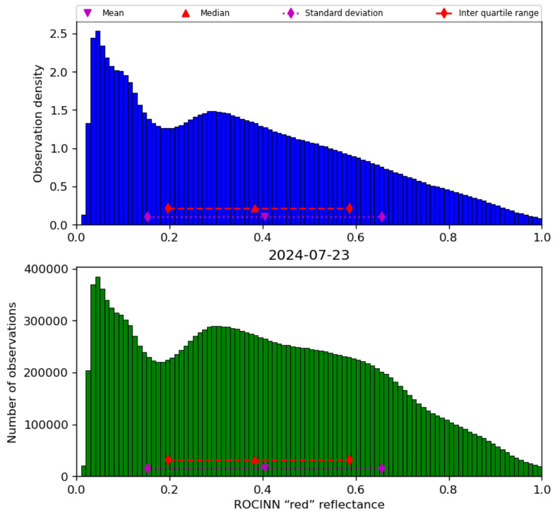
Figure 53: Histogram of “ROCINN “red” reflectance” for 2024-07-22 to 2024-07-24
