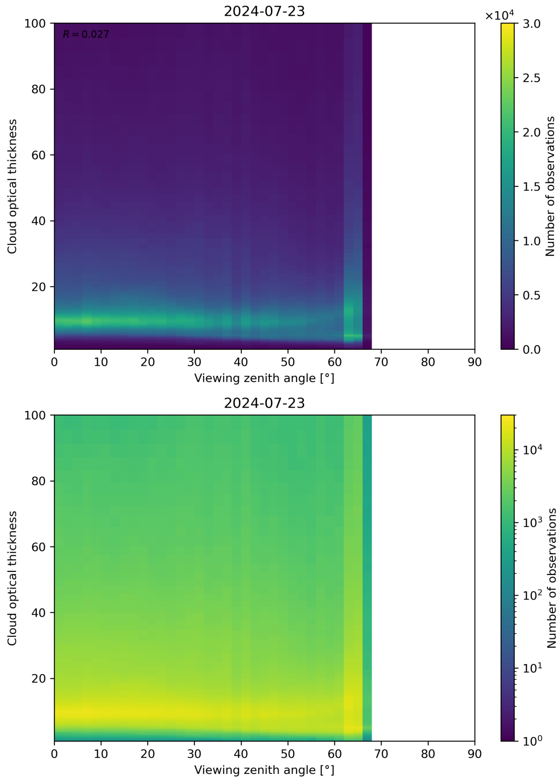
Figure 111: Scatter density plot of “Viewing zenith angle” against “Cloud optical thickness” for 2024-07-22 to 2024-07-24.
