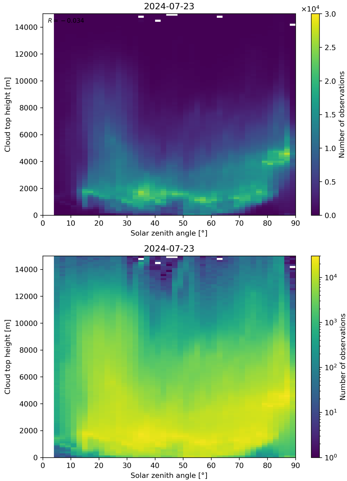
Figure 104: Scatter density plot of “Solar zenith angle” against “Cloud top height” for 2024-07-22 to 2024-07-24.
