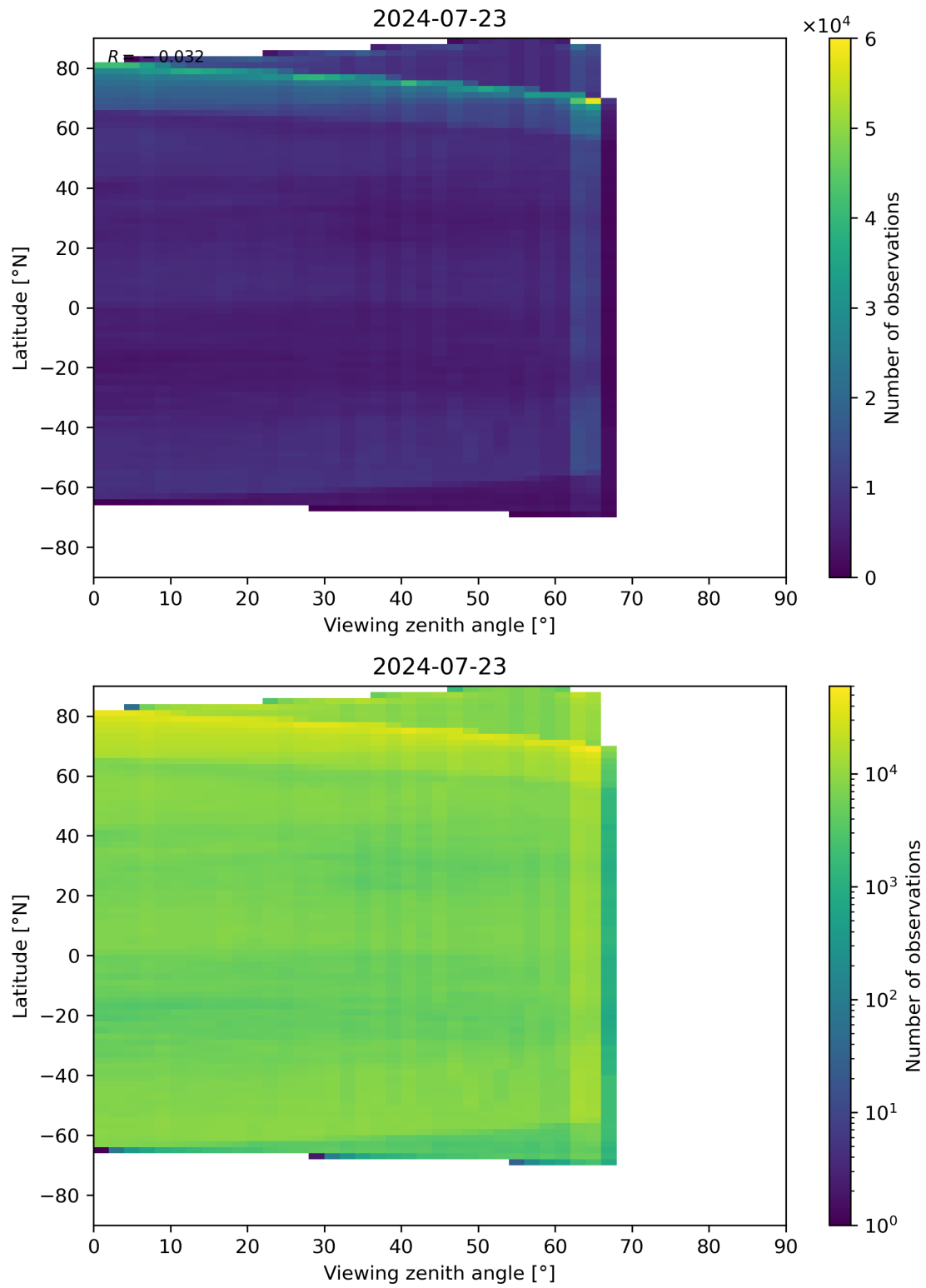
Figure 113: Scatter density plot of “Viewing zenith angle” against “Latitude” for 2024-07-22 to 2024-07-24.
