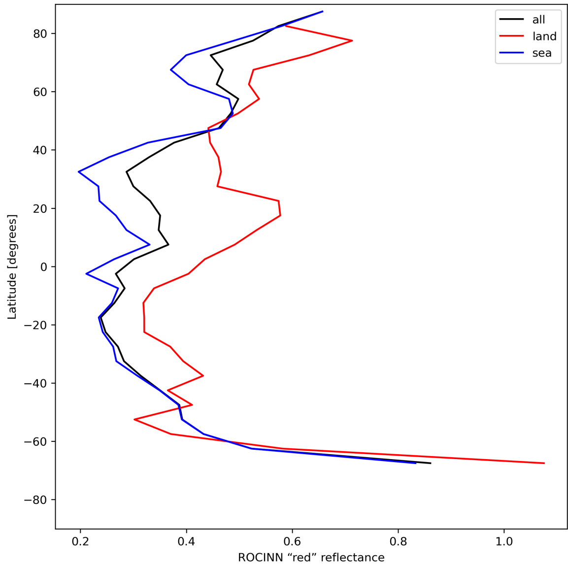
Figure 37: Zonal average of “ROCINN “red” reflectance” for 2024-07-22 to 2024-07-24.
