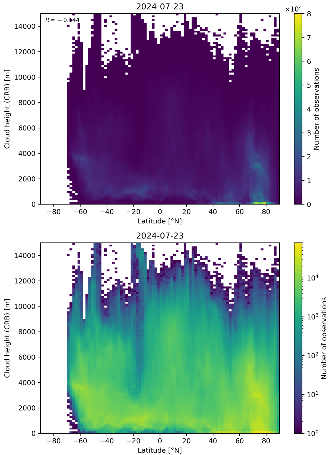
Figure 95: Scatter density plot of “Latitude” against “Cloud height (CRB)” for 2024-07-22 to 2024-07-24.
