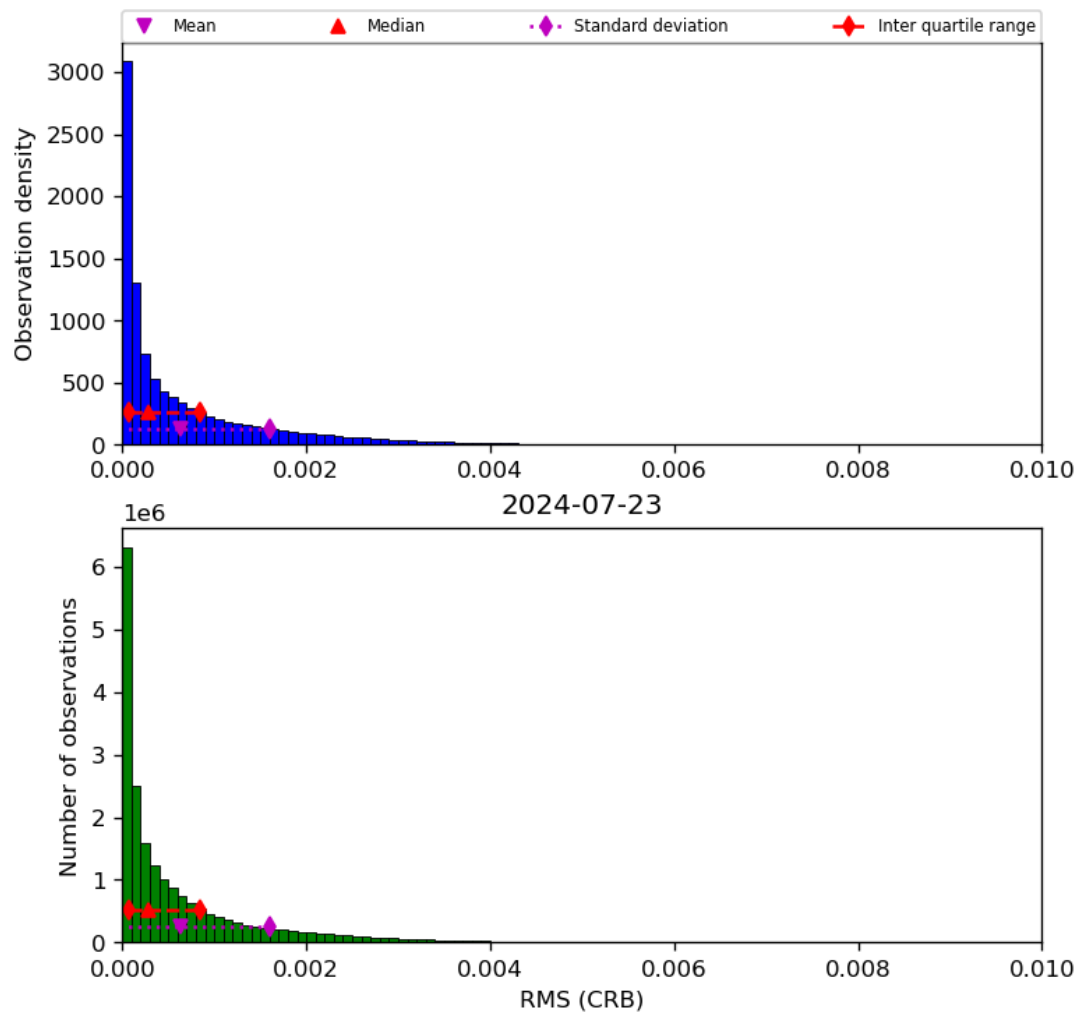
Figure 48: Histogram of “RMS (CRB)” for 2024-07-22 to 2024-07-24
