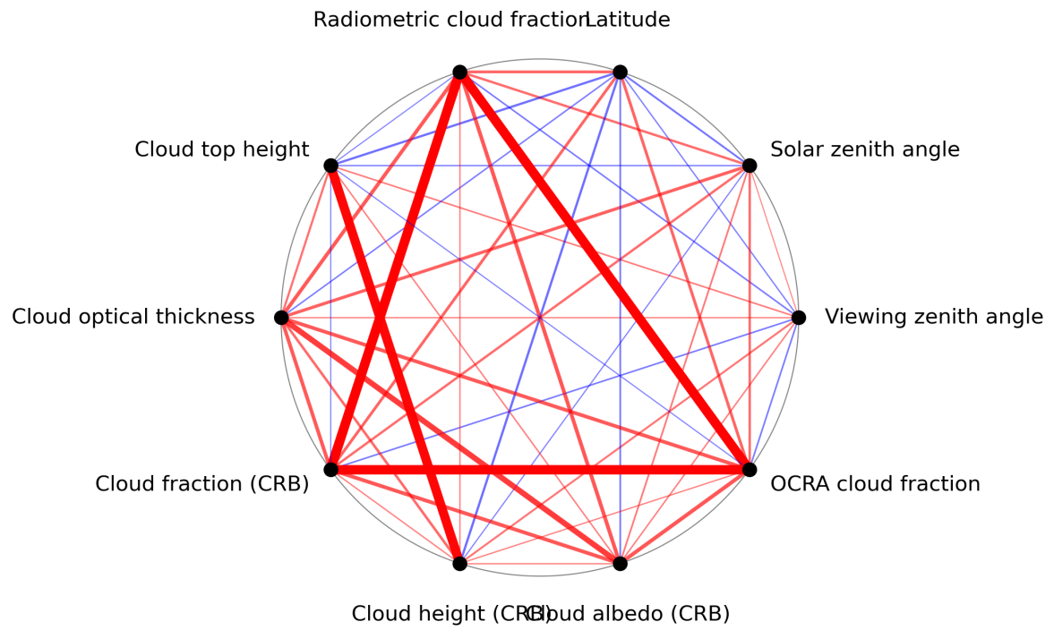
Figure 1: Map of correlation graph for 2024-07-22 to 2024-07-24.
