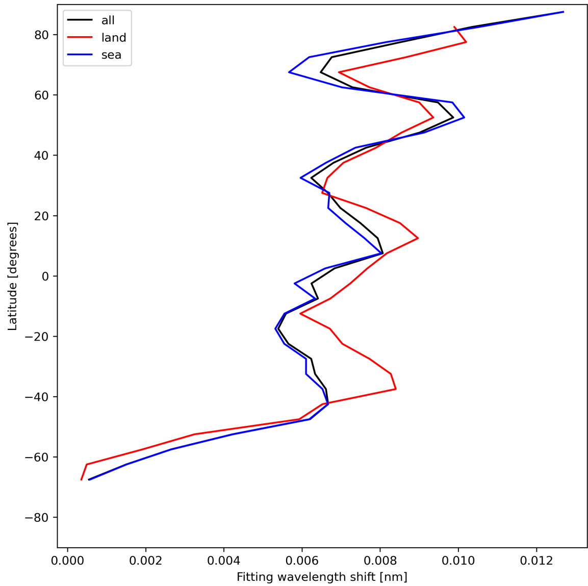
Figure 33: Zonal average of “Fitting wavelength shift” for 2024-07-22 to 2024-07-24.
