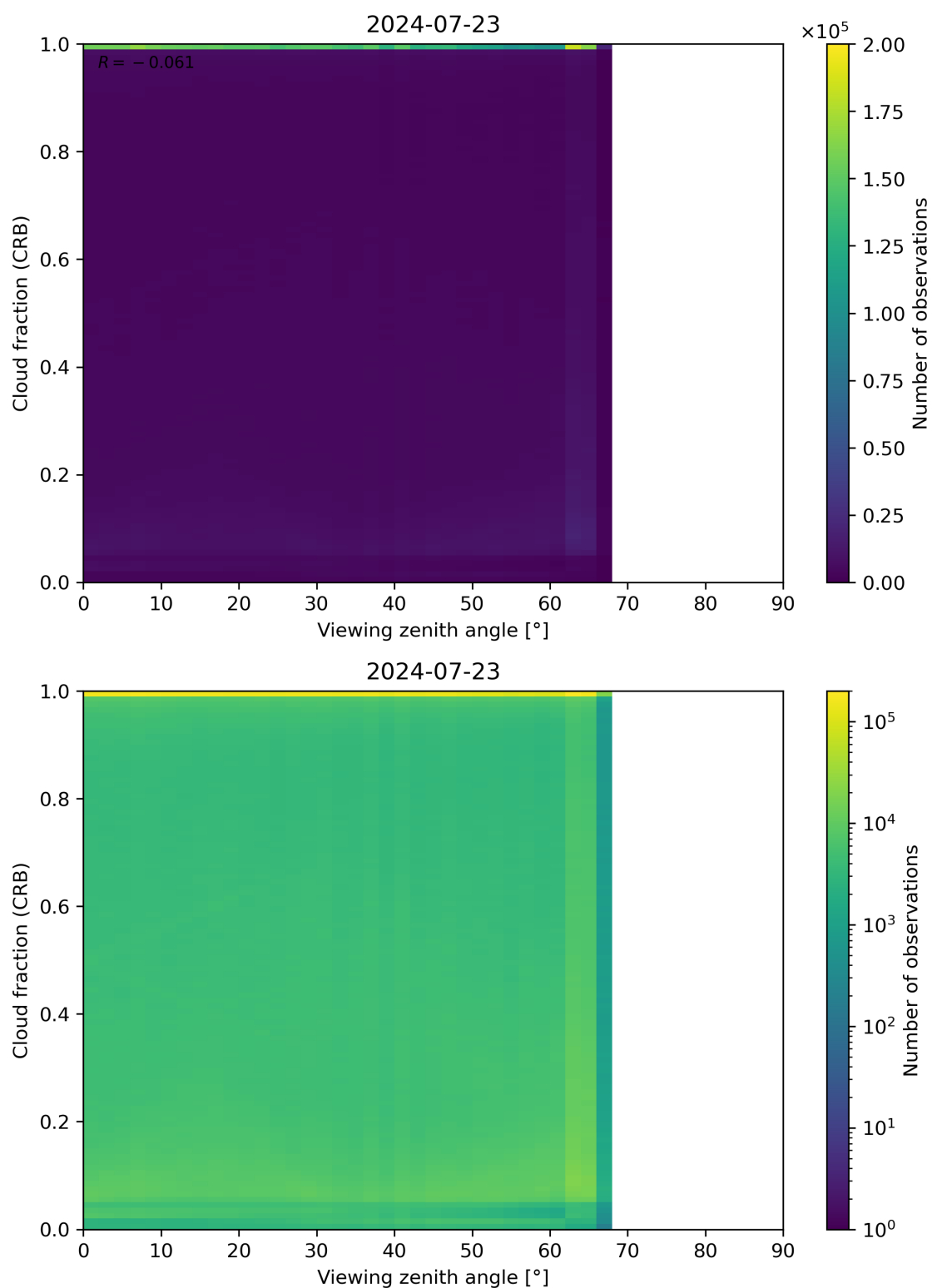
Figure 109: Scatter density plot of “Viewing zenith angle” against “Cloud fraction (CRB)” for 2024-07-22 to 2024-07-24.
