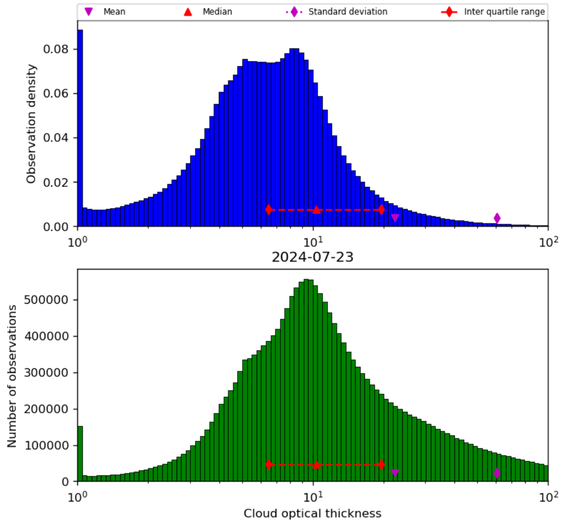
Figure 41: Histogram of “Cloud optical thickness” for 2024-07-22 to 2024-07-24
