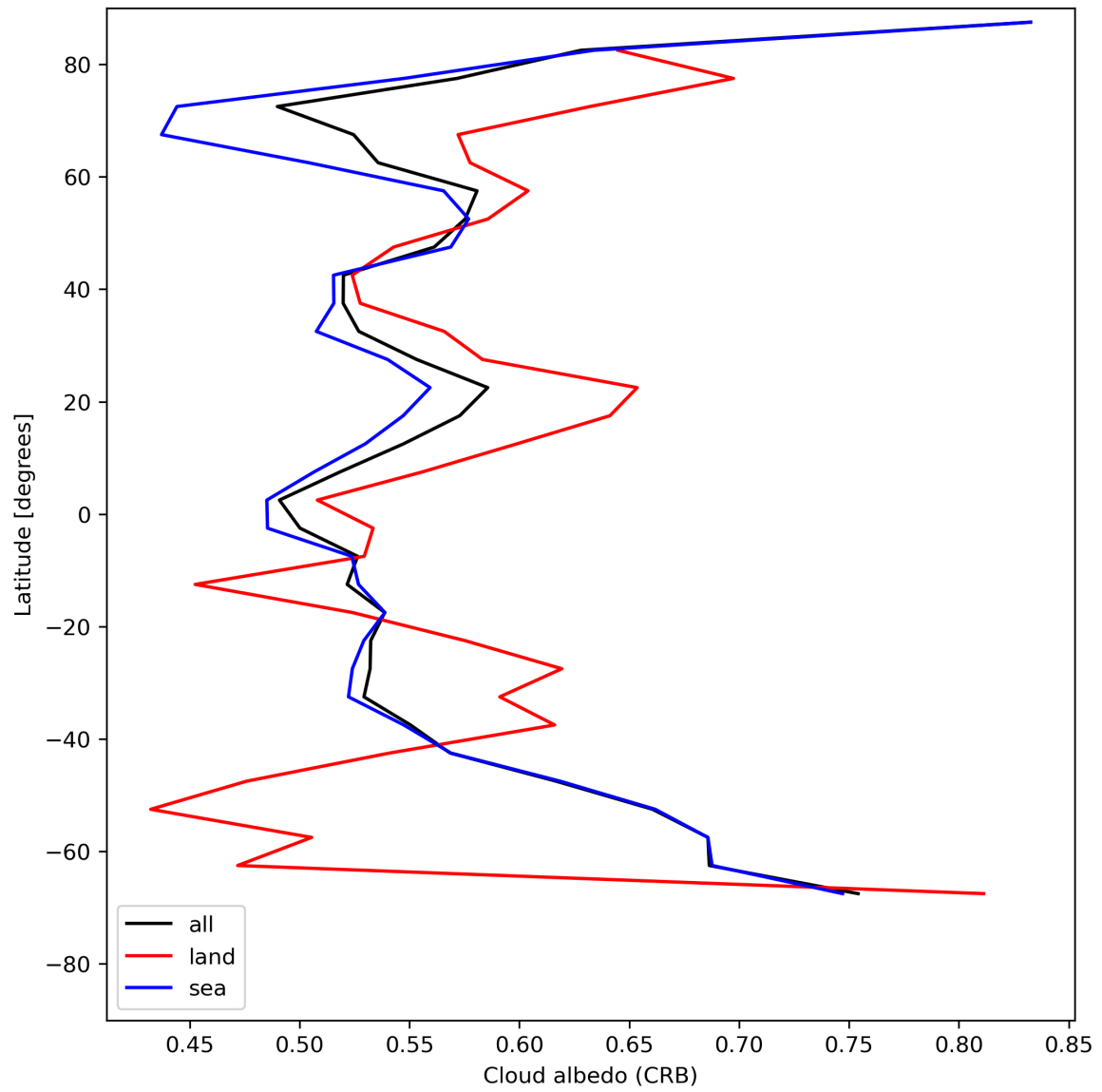
Figure 28: Zonal average of “Cloud albedo (CRB)” for 2024-07-22 to 2024-07-24.
