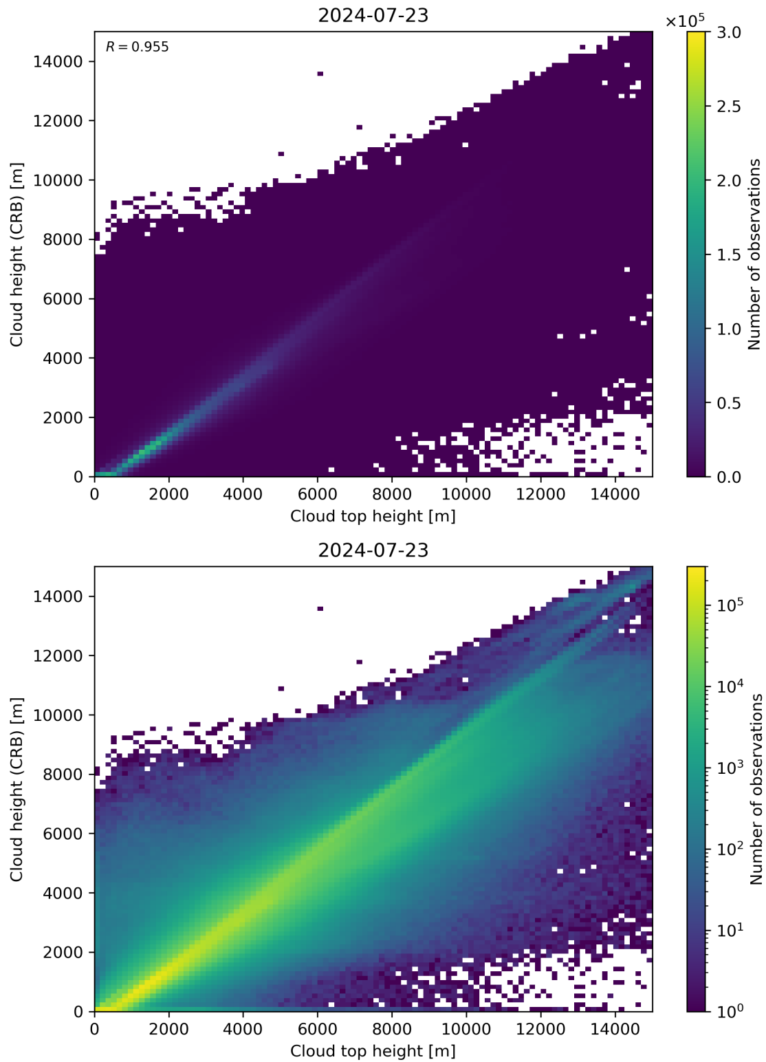
Figure 89: Scatter density plot of “Cloud top height” against “Cloud height (CRB)” for 2024-07-22 to 2024-07-24.
