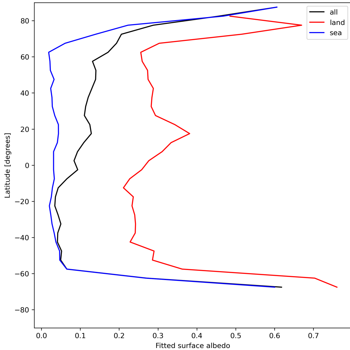
Figure 29: Zonal average of “Fitted surface albedo” for 2024-07-22 to 2024-07-24.
