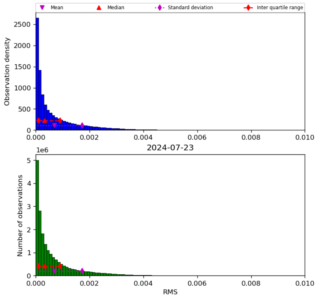
Figure 47: Histogram of “RMS” for 2024-07-22 to 2024-07-24
