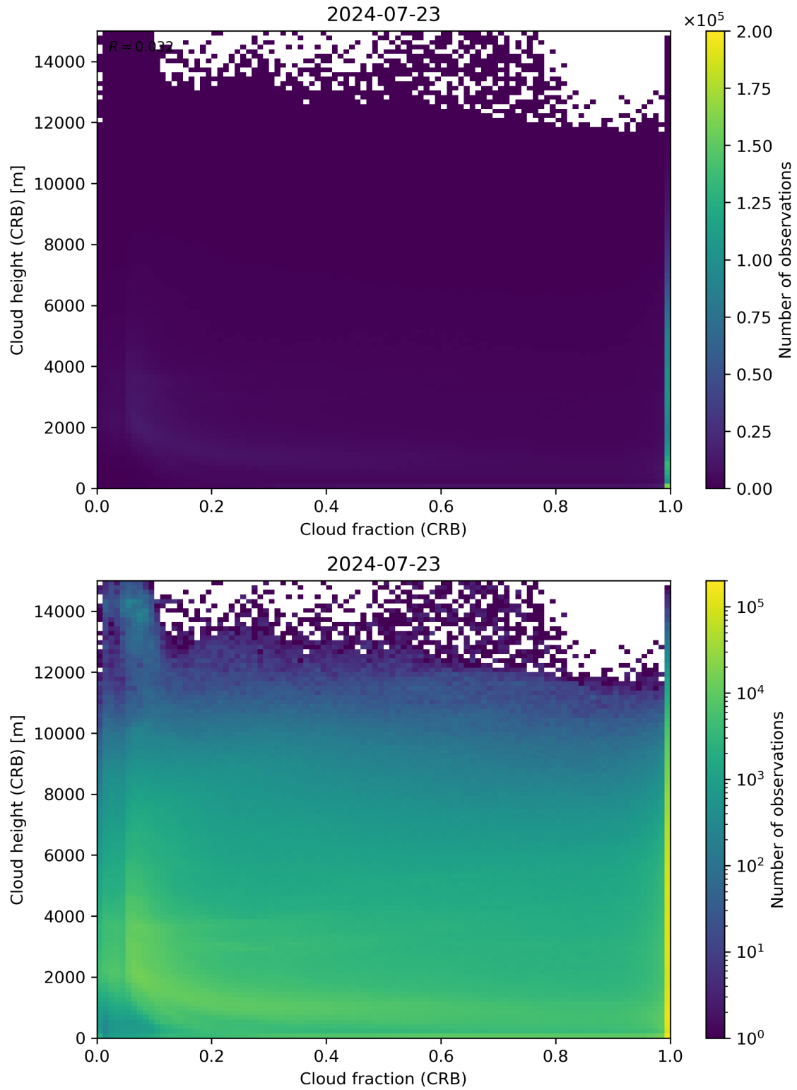
Figure 79: Scatter density plot of “Cloud fraction (CRB)” against “Cloud height (CRB)” for 2024-07-22 to 2024-07-24.
