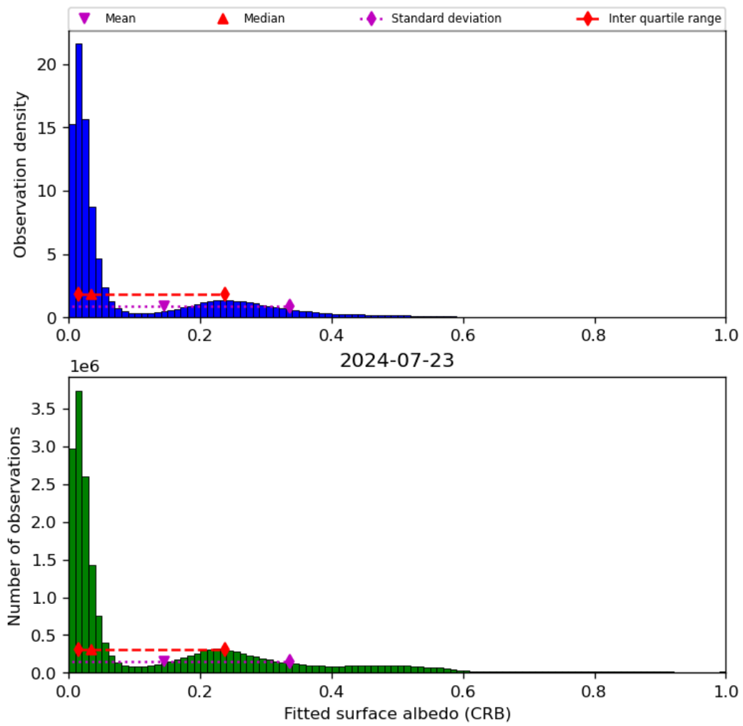
Figure 46: Histogram of “Fitted surface albedo (CRB)” for 2024-07-22 to 2024-07-24
