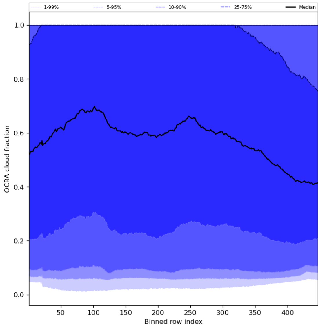
Figure 66: Along track statistics of “OCRA cloud fraction” for 2024-07-22 to 2024-07-24
