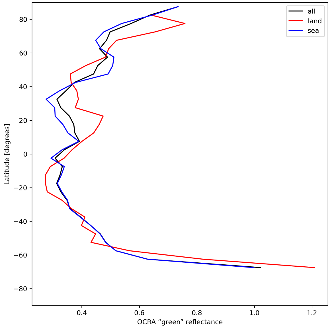
Figure 36: Zonal average of “OCRA “green” reflectance” for 2024-07-22 to 2024-07-24.
