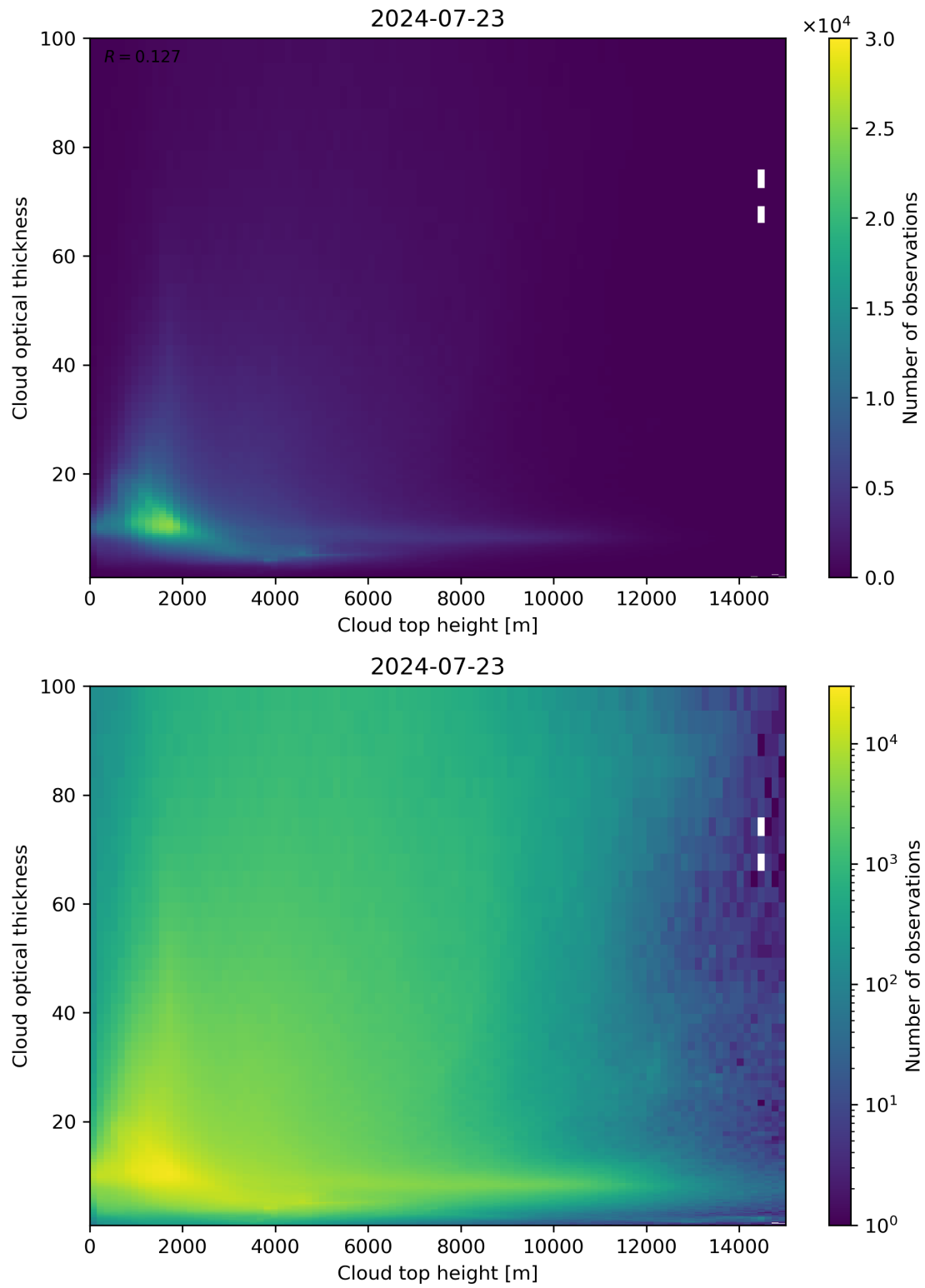
Figure 90: Scatter density plot of “Cloud top height” against “Cloud optical thickness” for 2024-07-22 to 2024-07-24.
