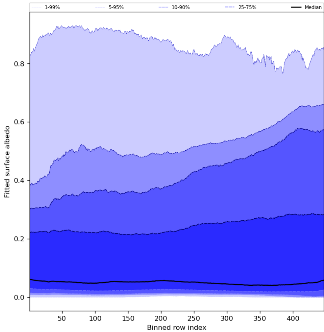
Figure 61: Along track statistics of “Fitted surface albedo” for 2024-07-22 to 2024-07-24
