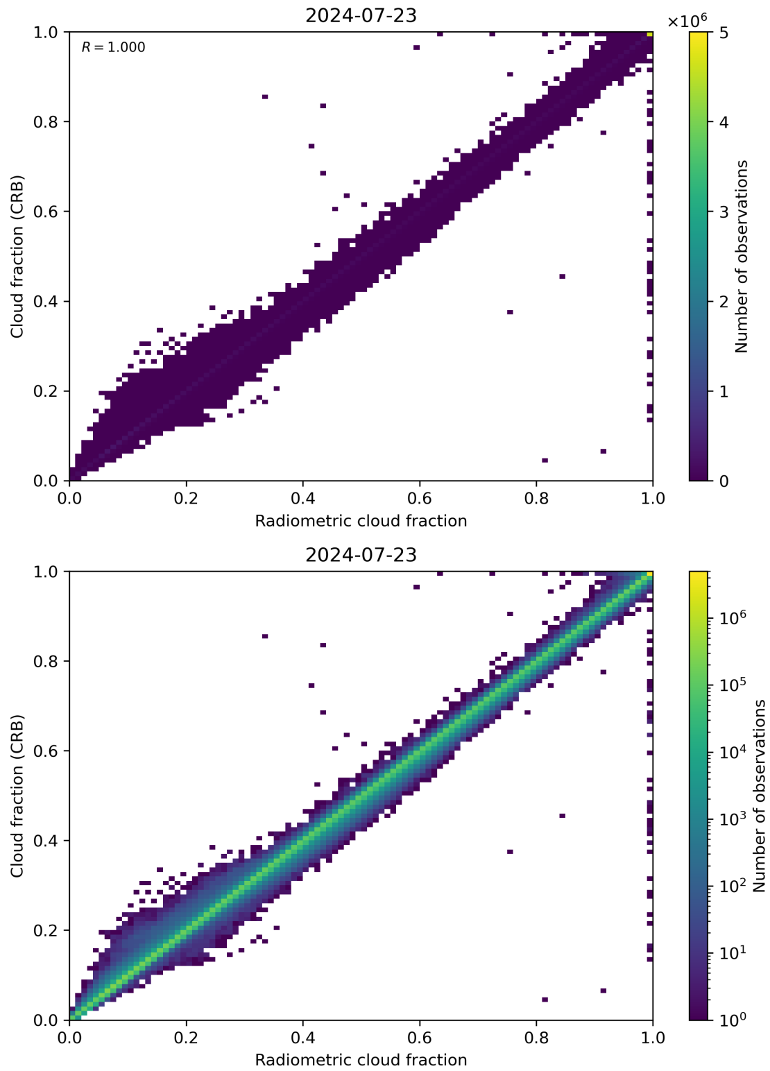
Figure 73: Scatter density plot of “Radiometric cloud fraction” against “Cloud fraction (CRB)” for 2024-07-22 to 2024-07-24.
