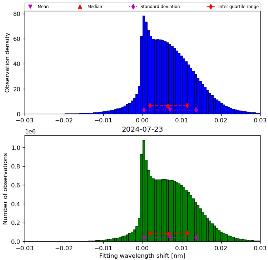
Figure 49: Histogram of “Fitting wavelength shift” for 2024-07-22 to 2024-07-24
