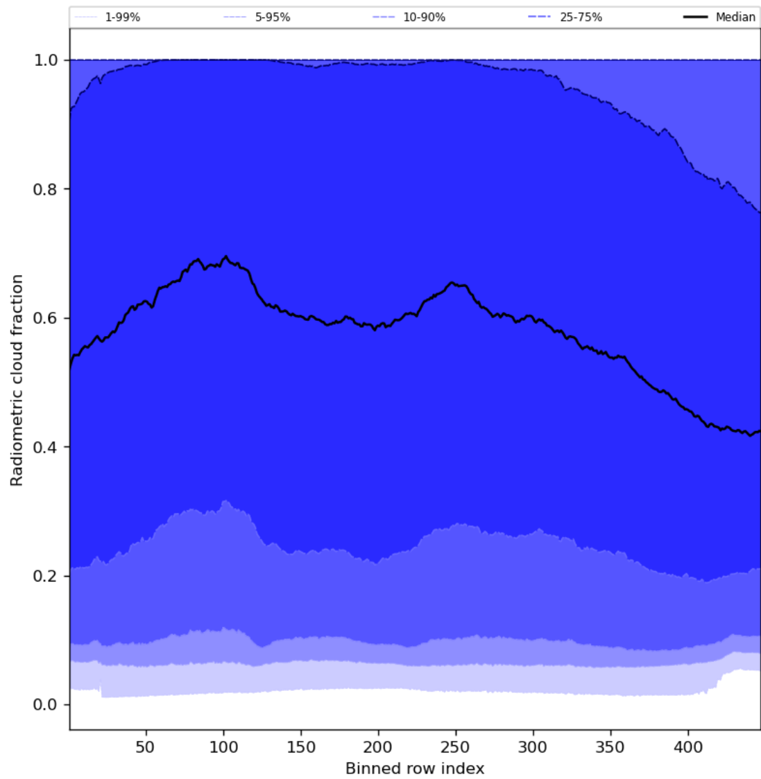
Figure 55: Along track statistics of “Radiometric cloud fraction” for 2024-07-22 to 2024-07-24
