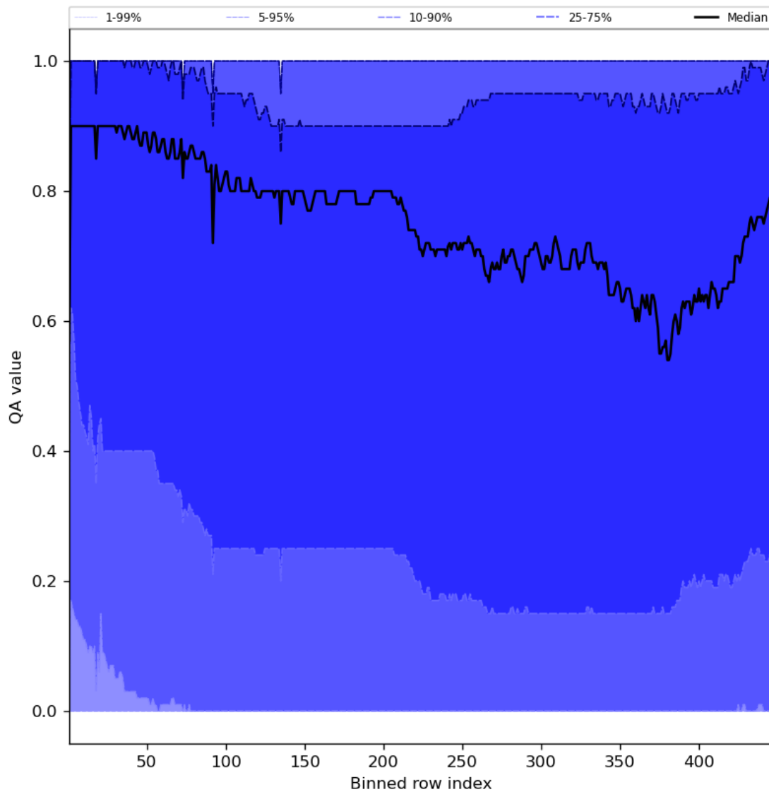
Figure 54: Along track statistics of “QA value” for 2024-07-22 to 2024-07-24
