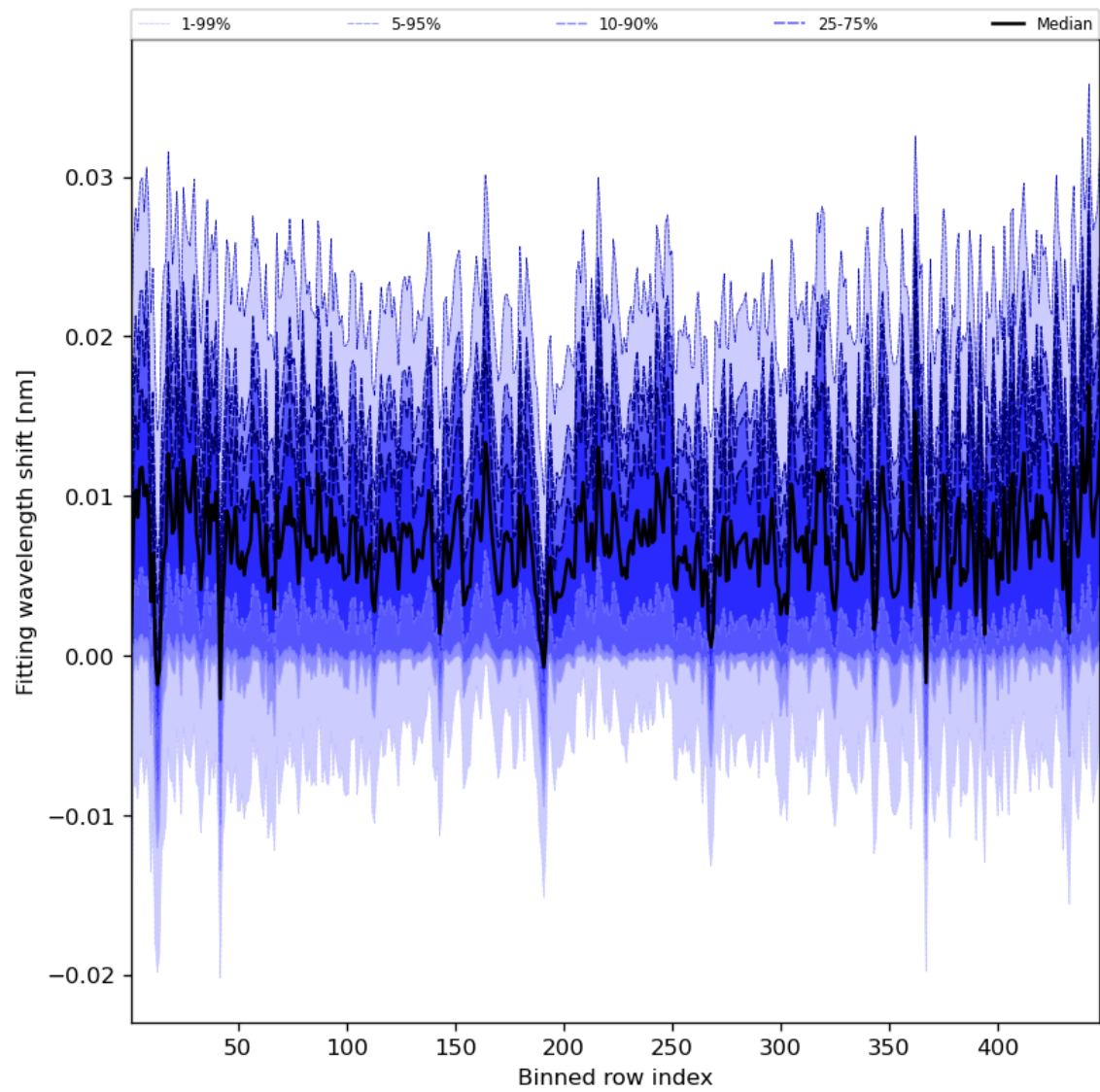
Figure 65: Along track statistics of “Fitting wavelength shift” for 2024-07-22 to 2024-07-24
