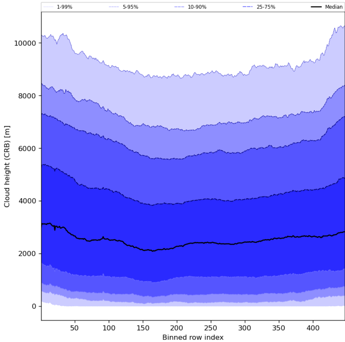
Figure 59: Along track statistics of “Cloud height (CRB)” for 2024-07-22 to 2024-07-24
