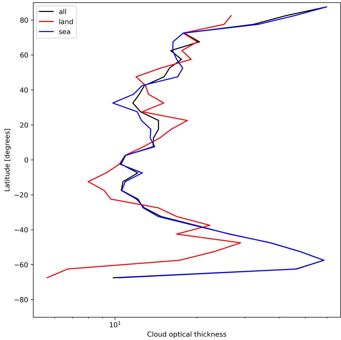
Figure 25: Zonal average of “Cloud optical thickness” for 2024-07-22 to 2024-07-24.
