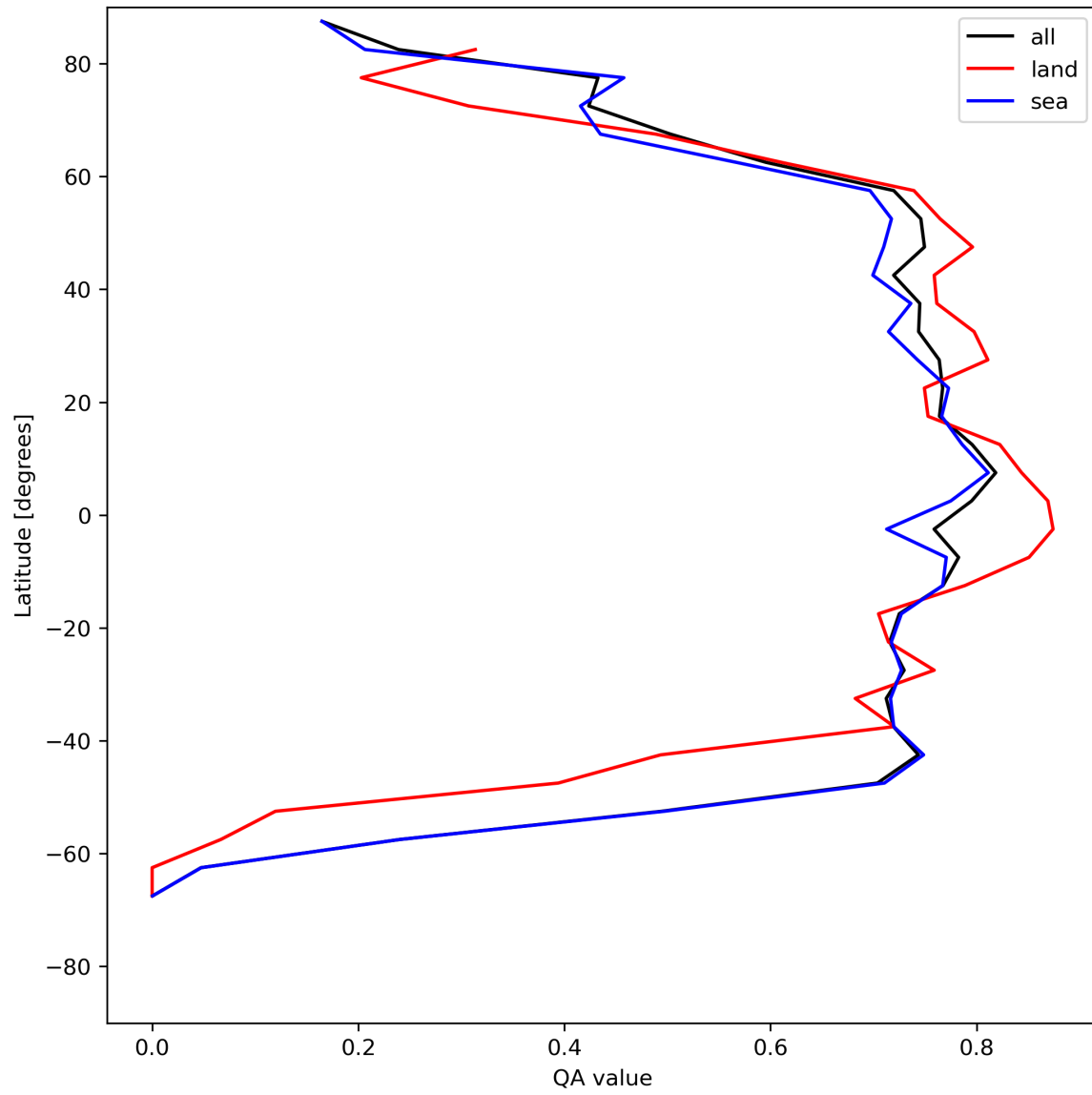
Figure 22: Zonal average of “QA value” for 2024-07-22 to 2024-07-24.
