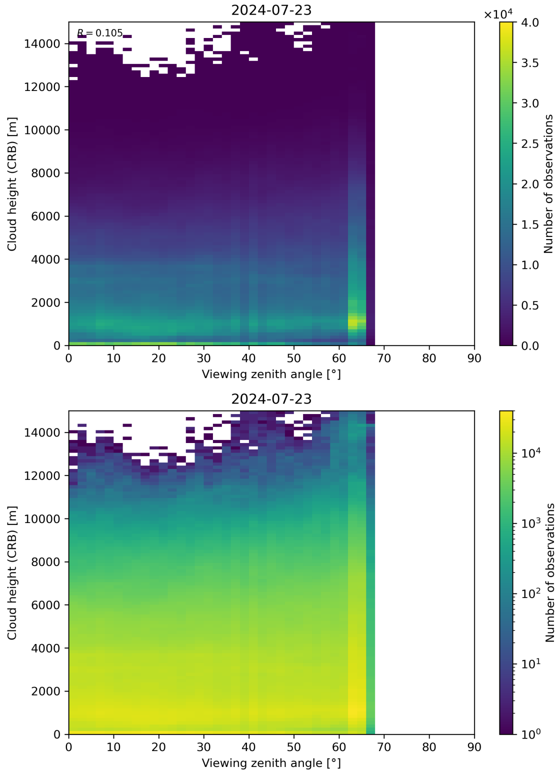
Figure 110: Scatter density plot of “Viewing zenith angle” against “Cloud height (CRB)” for 2024-07-22 to 2024-07-24.
