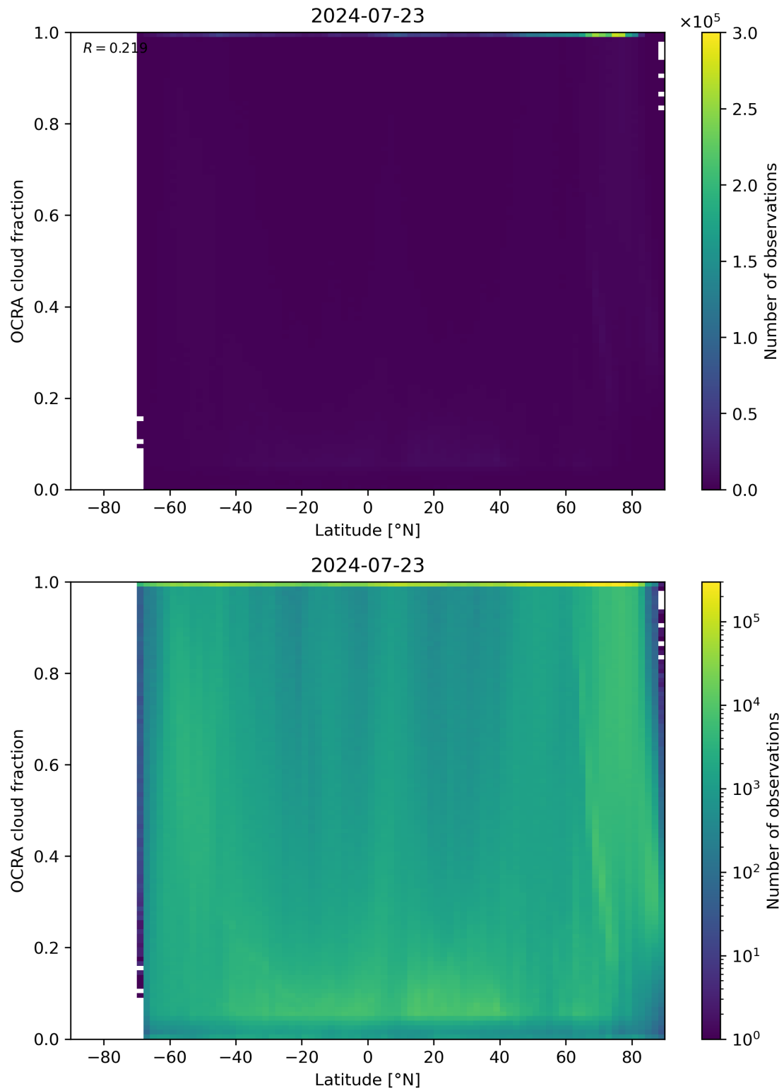
Figure 93: Scatter density plot of “Latitude” against “OCRA cloud fraction” for 2024-07-22 to 2024-07-24.
