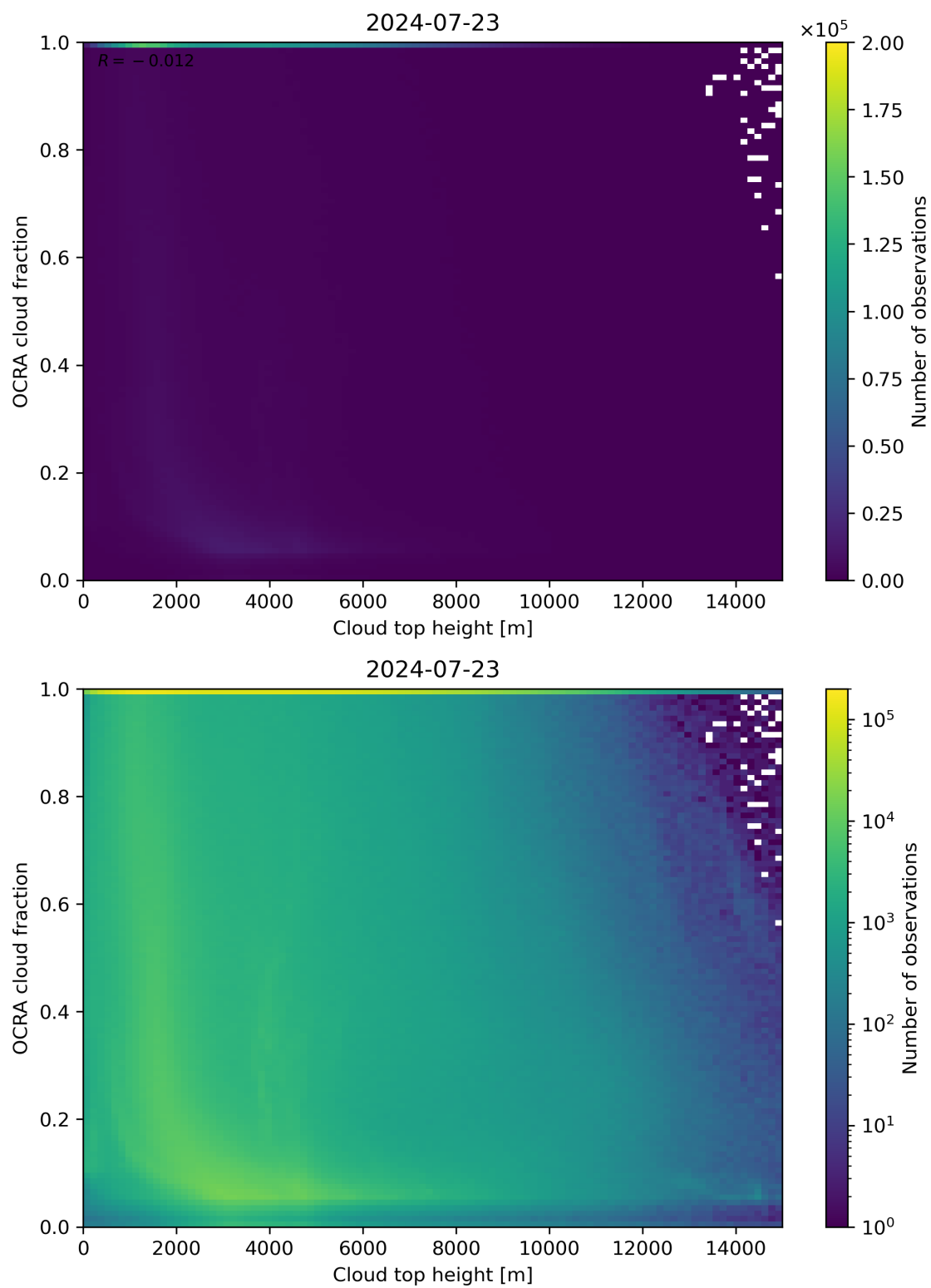
Figure 87: Scatter density plot of “Cloud top height” against “OCRA cloud fraction” for 2024-07-22 to 2024-07-24.
