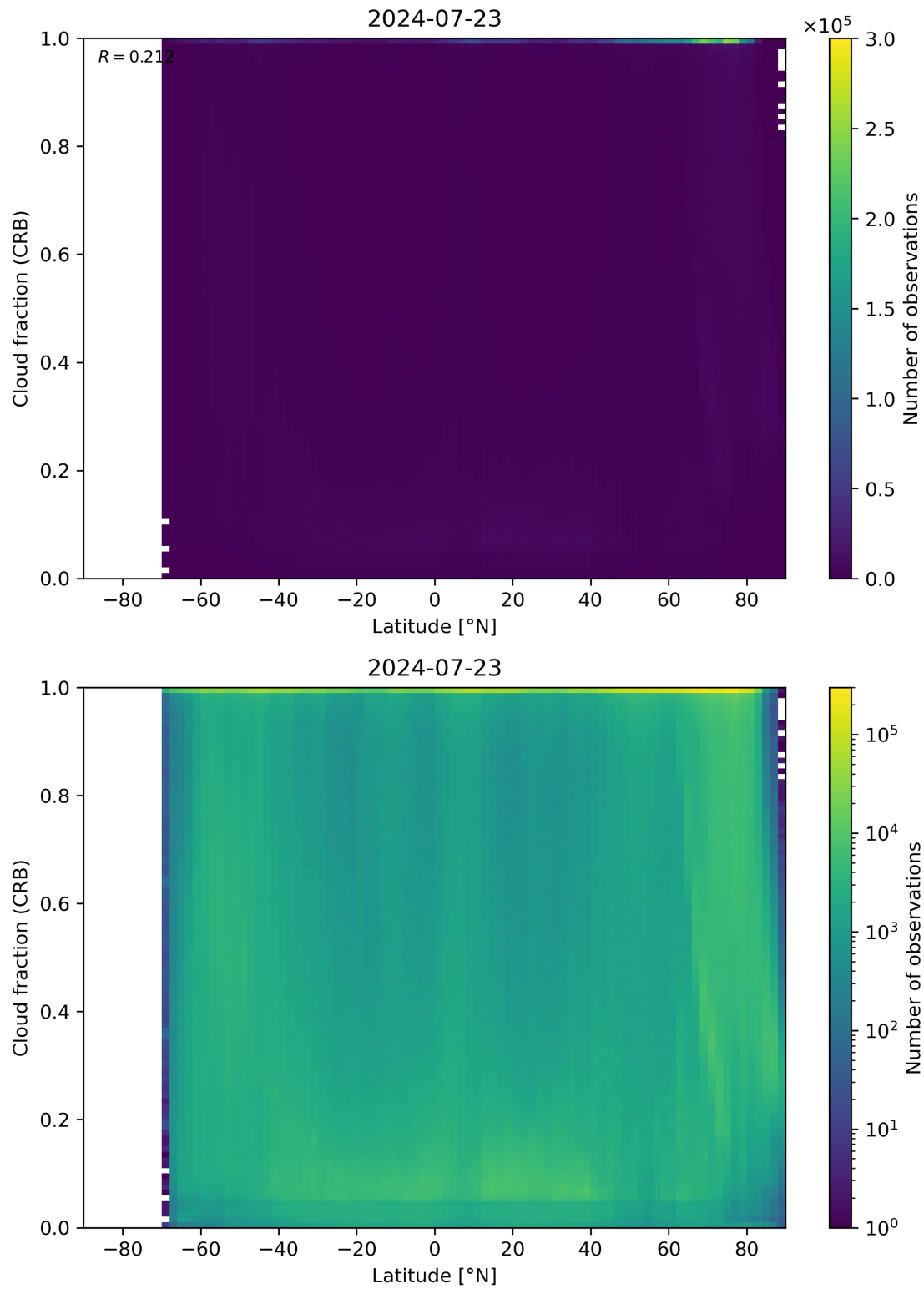
Figure 94: Scatter density plot of “Latitude” against “Cloud fraction (CRB)” for 2024-07-22 to 2024-07-24.
