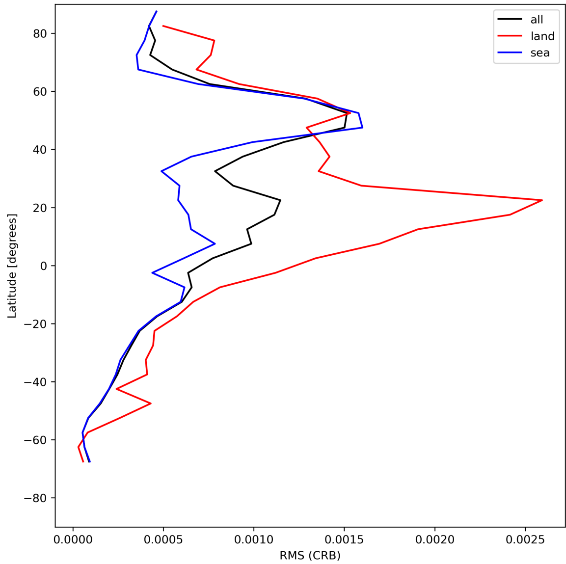
Figure 32: Zonal average of “RMS (CRB)” for 2024-07-22 to 2024-07-24.
