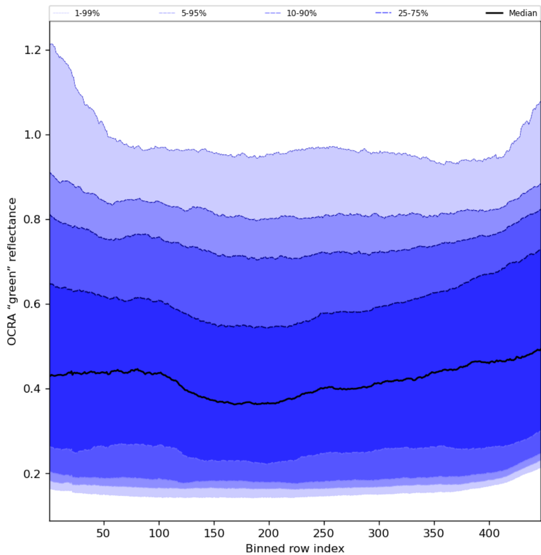
Figure 68: Along track statistics of “OCRA “green” reflectance” for 2024-07-22 to 2024-07-24
