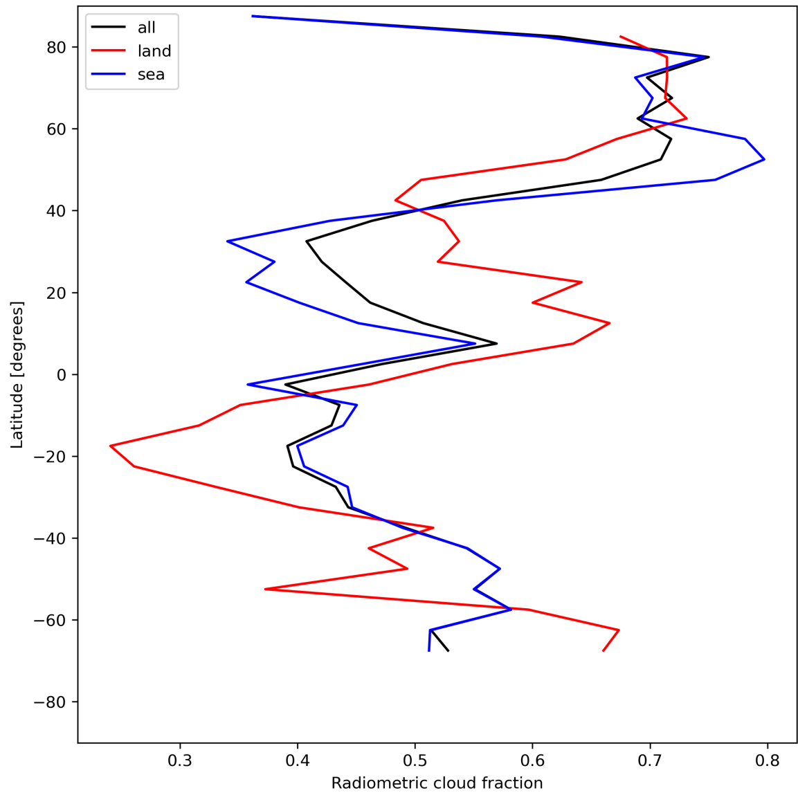
Figure 23: Zonal average of “Radiometric cloud fraction” for 2024-07-22 to 2024-07-24.
