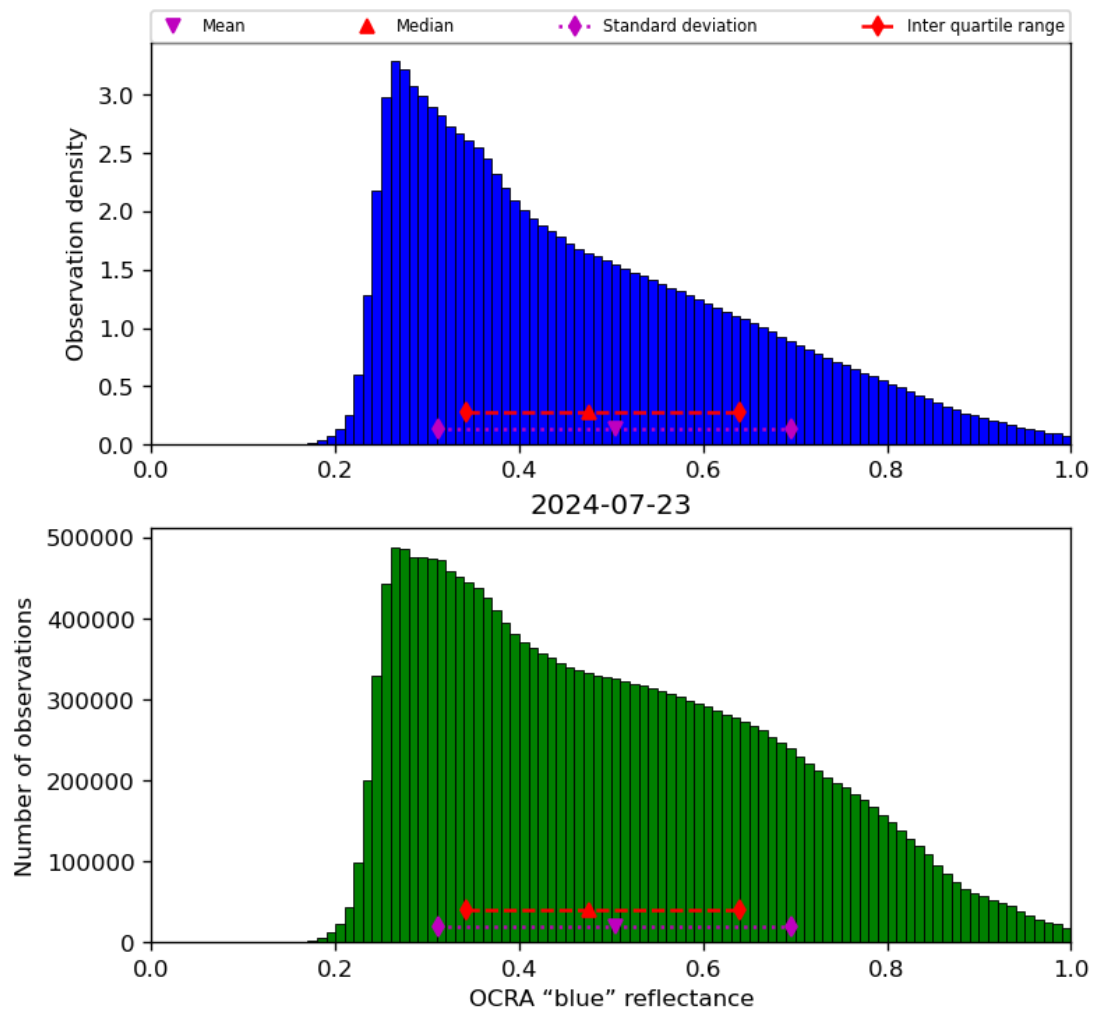
Figure 51: Histogram of “OCRA “blue” reflectance” for 2024-07-22 to 2024-07-24
