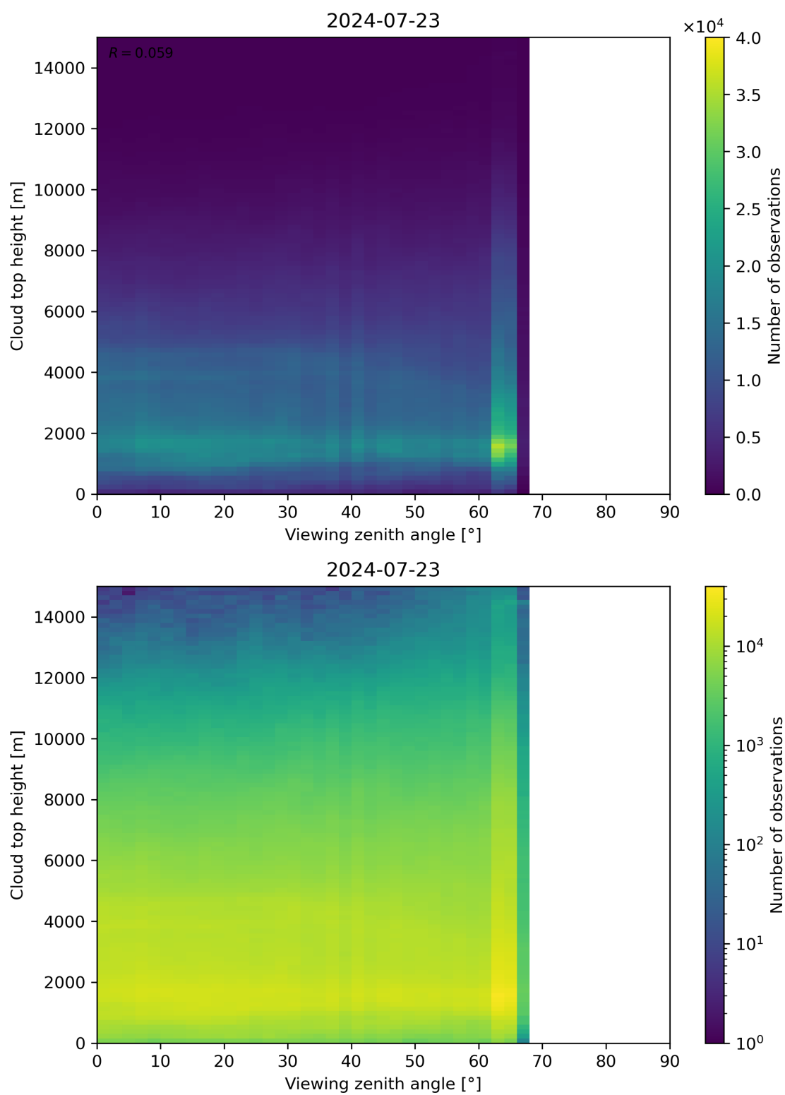
Figure 112: Scatter density plot of “Viewing zenith angle” against “Cloud top height” for 2024-07-22 to 2024-07-24.
