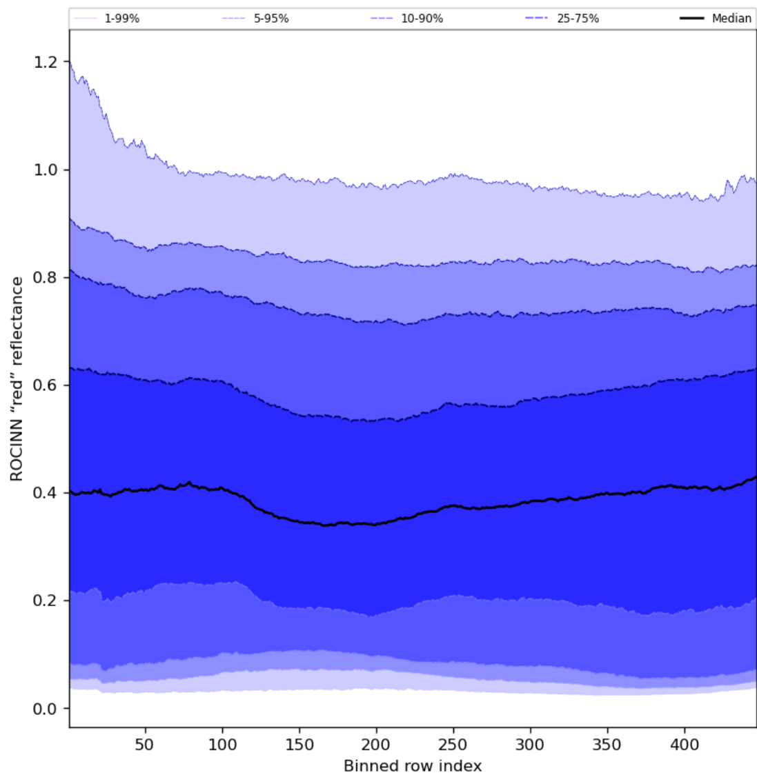
Figure 69: Along track statistics of "ROCINN "red" reflectance" for 2024-07-22 to 2024-07-24
