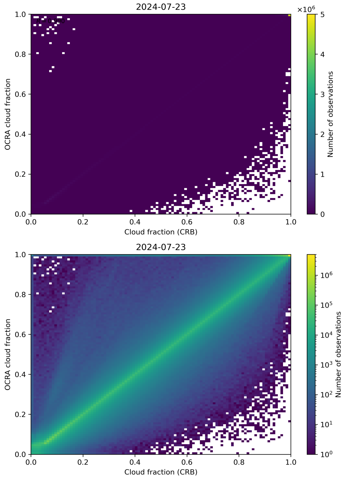
Figure 78: Scatter density plot of “Cloud fraction (CRB)” against “OCRA cloud fraction” for 2024-07-22 to 2024-07-24.
