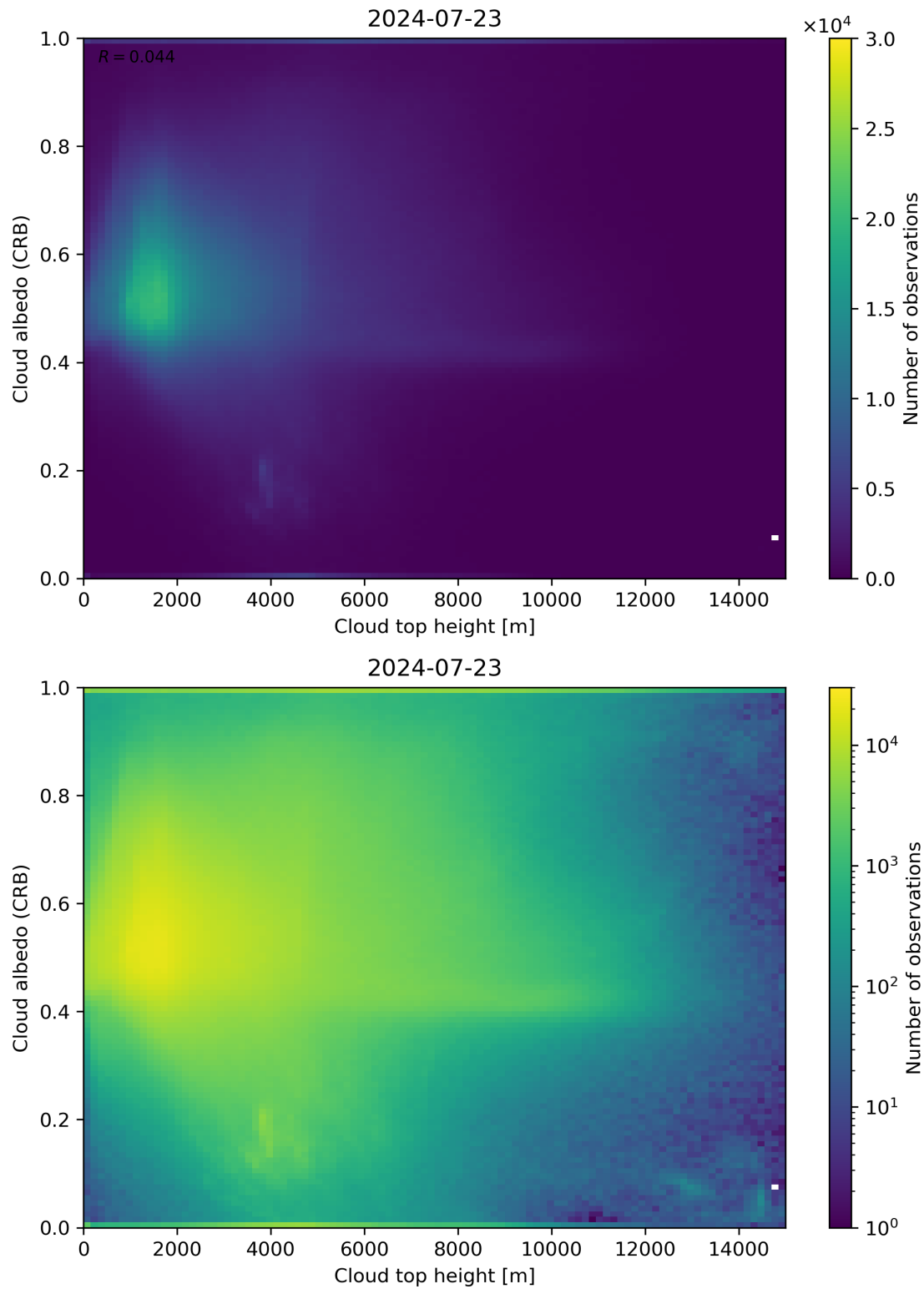
Figure 86: Scatter density plot of “Cloud top height” against “Cloud albedo (CRB)” for 2024-07-22 to 2024-07-24.
