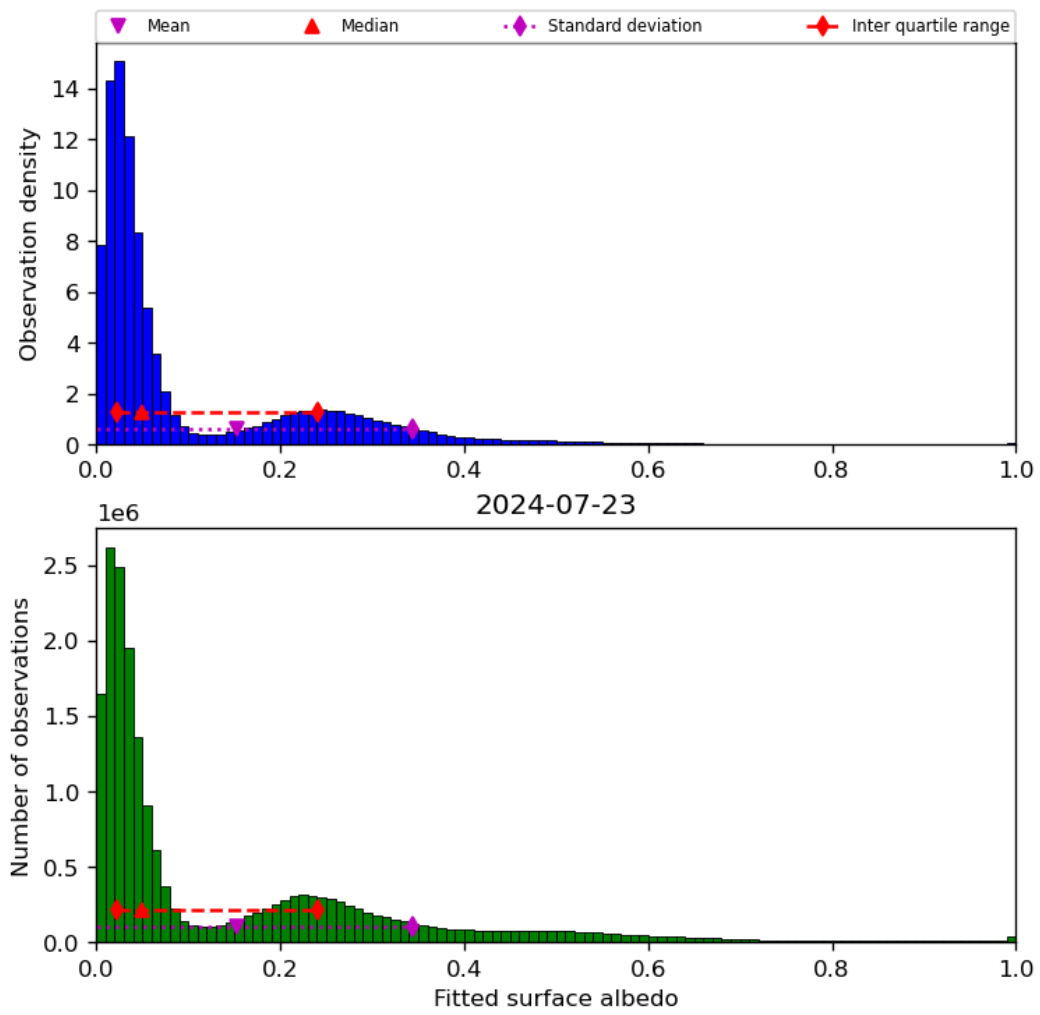
Figure 45: Histogram of “Fitted surface albedo” for 2024-07-22 to 2024-07-24
