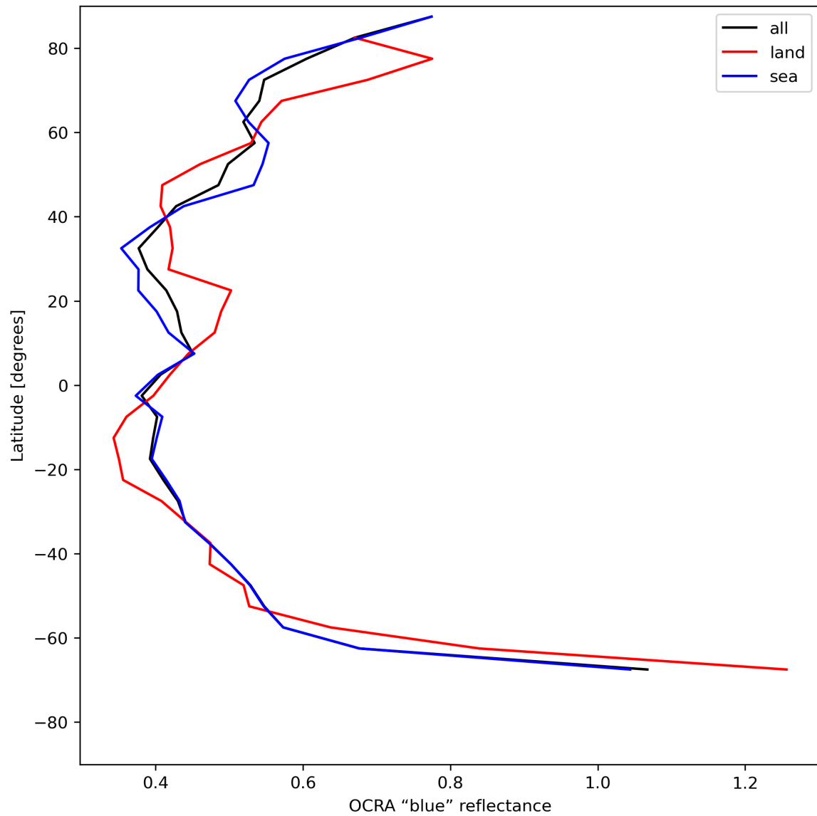
Figure 35: Zonal average of “OCRA “blue” reflectance” for 2024-07-22 to 2024-07-24.
