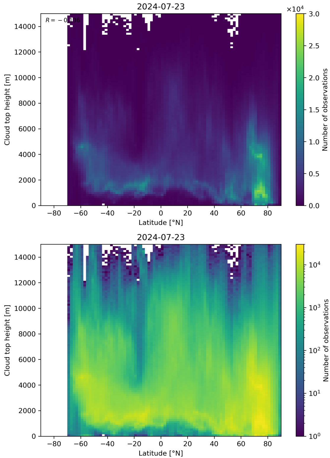
Figure 97: Scatter density plot of “Latitude” against “Cloud top height” for 2024-07-22 to 2024-07-24.
