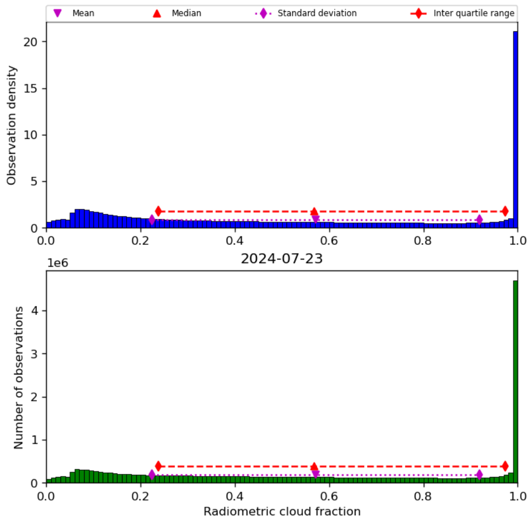
Figure 39: Histogram of “Radiometric cloud fraction” for 2024-07-22 to 2024-07-24
