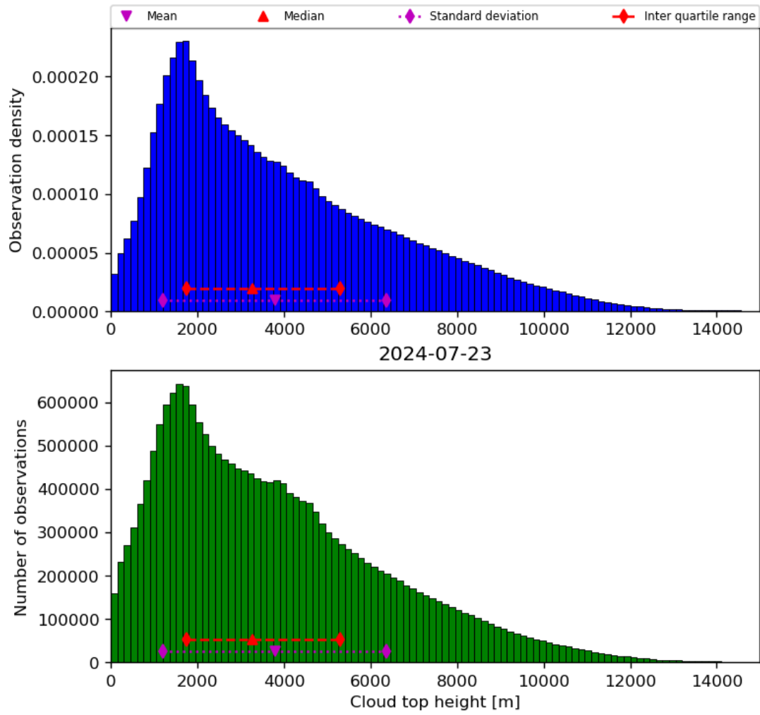
Figure 40: Histogram of “Cloud top height” for 2024-07-22 to 2024-07-24
