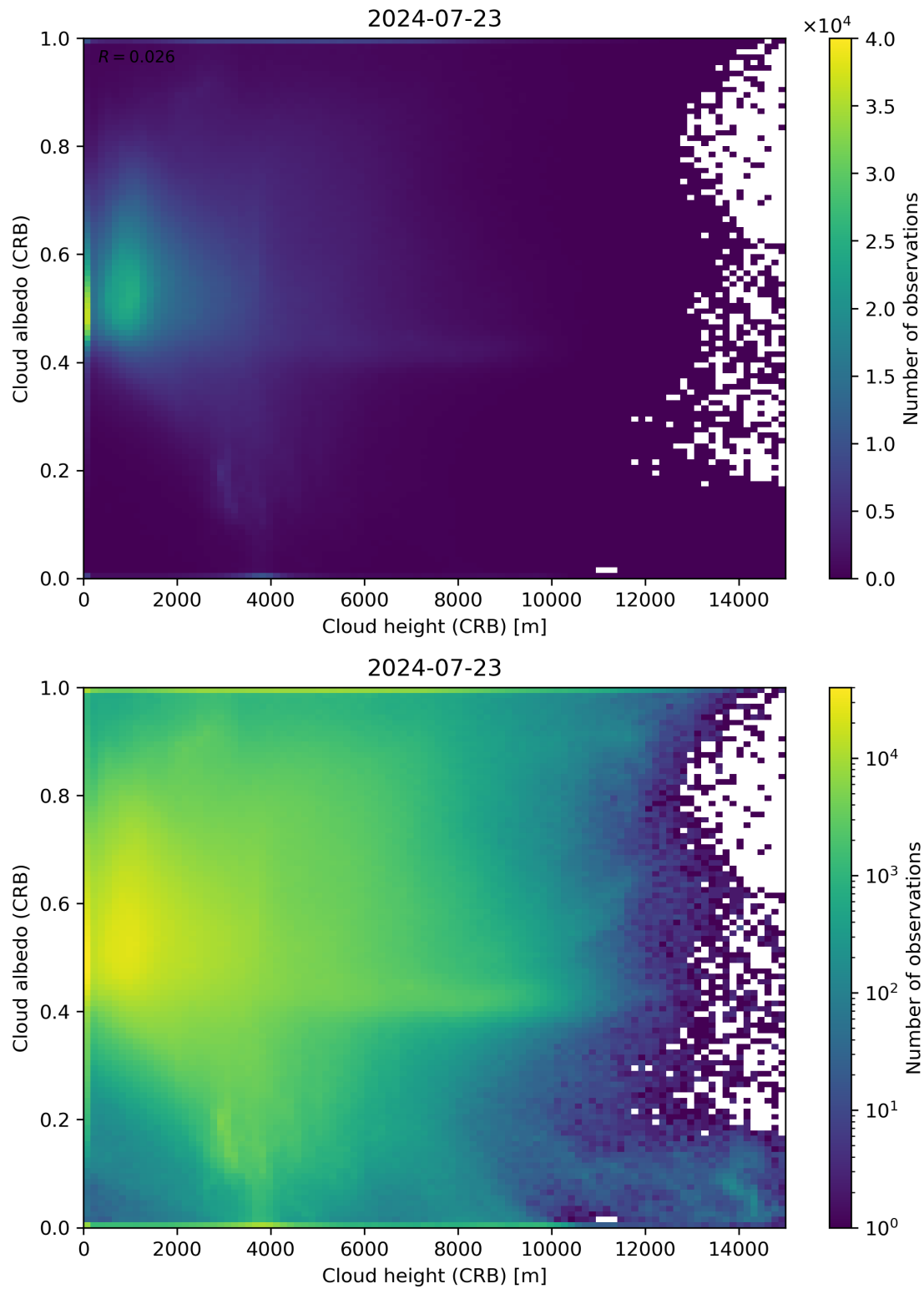
Figure 80: Scatter density plot of “Cloud height (CRB)” against “Cloud albedo (CRB)” for 2024-07-22 to 2024-07-24.
