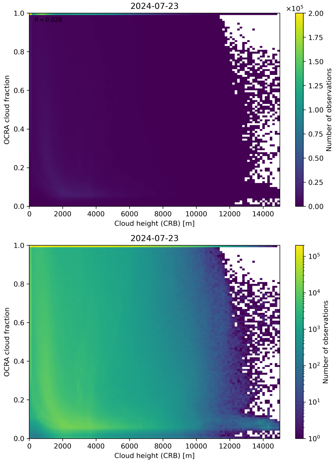
Figure 81: Scatter density plot of “Cloud height (CRB)” against “OCRA cloud fraction” for 2024-07-22 to 2024-07-24.
