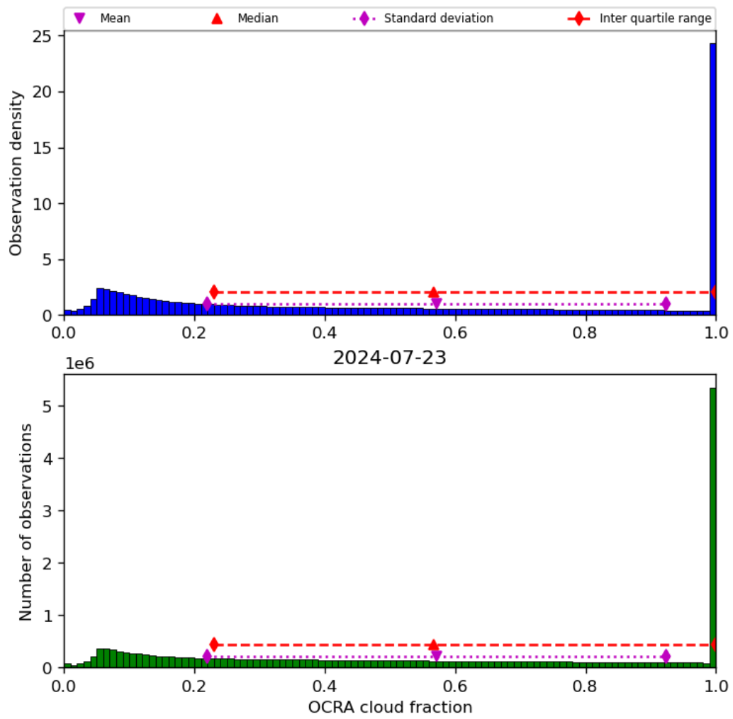
Figure 50: Histogram of “OCRA cloud fraction” for 2024-07-22 to 2024-07-24
