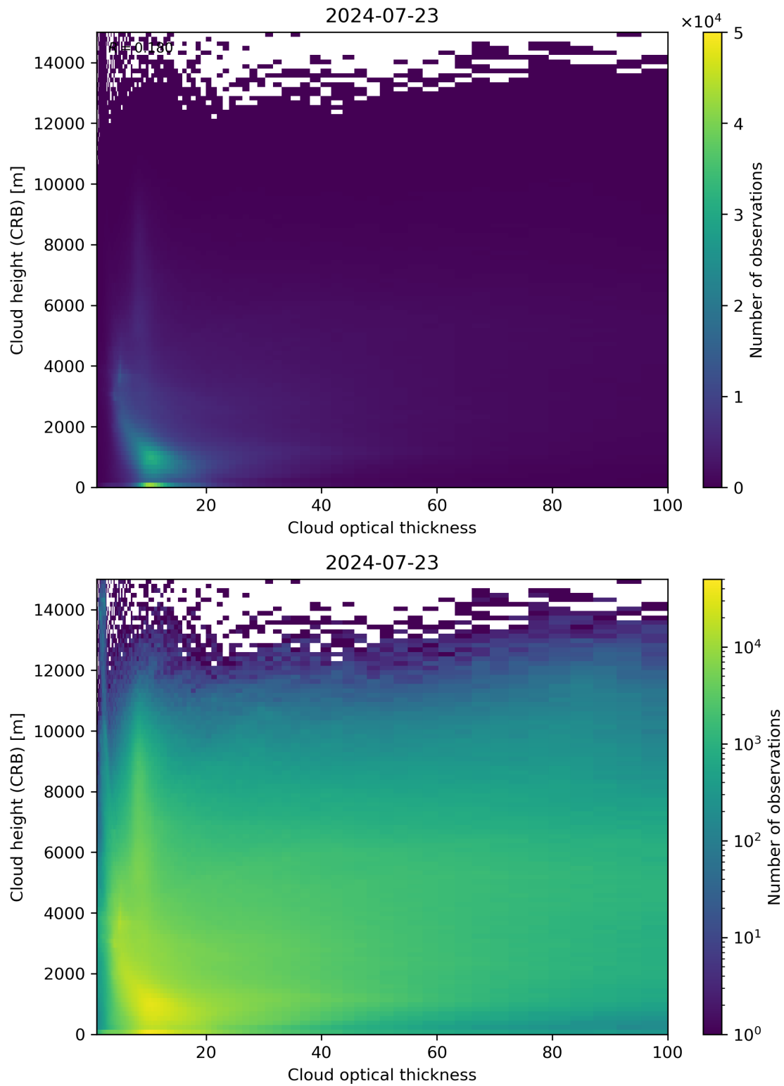
Figure 85: Scatter density plot of “Cloud optical thickness” against “Cloud height (CRB)” for 2024-07-22 to 2024-07-24.
