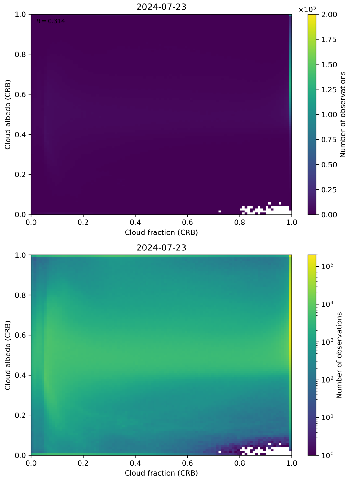
Figure 77: Scatter density plot of “Cloud fraction (CRB)” against “Cloud albedo (CRB)” for 2024-07-22 to 2024-07-24.
