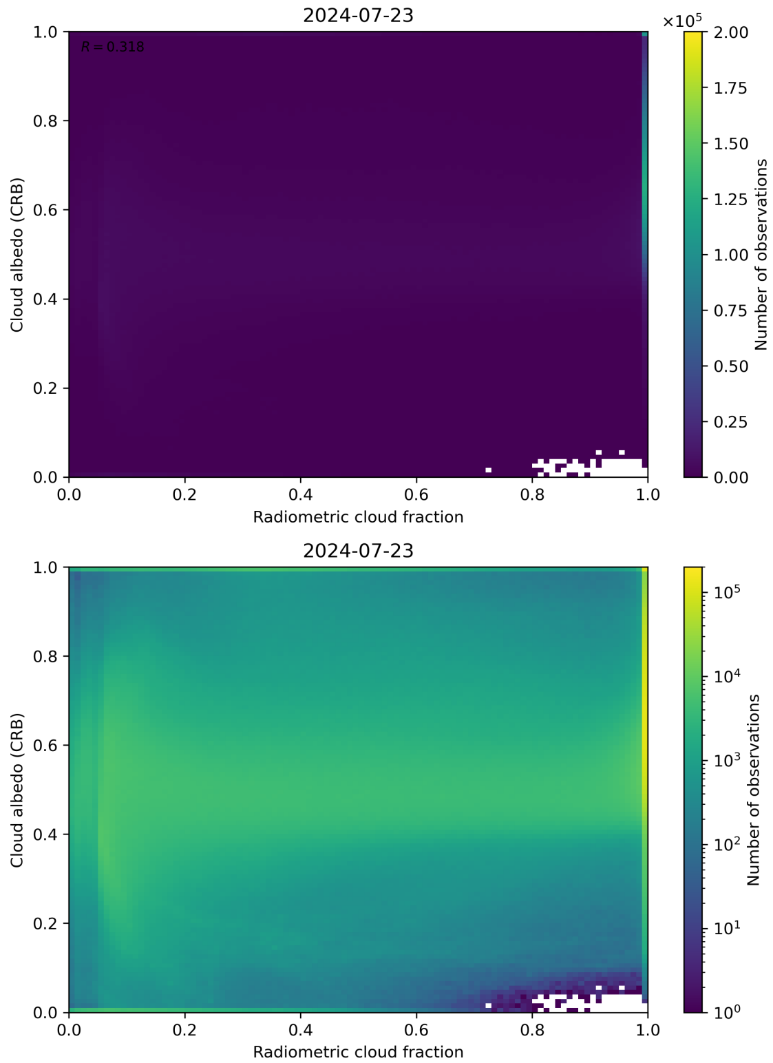
Figure 71: Scatter density plot of “Radiometric cloud fraction” against “Cloud albedo (CRB)” for 2024-07-22 to 2024-07-24.
