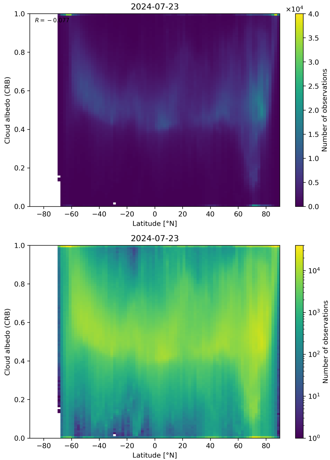
Figure 91: Scatter density plot of “Latitude” against “Cloud albedo (CRB)” for 2024-07-22 to 2024-07-24.
