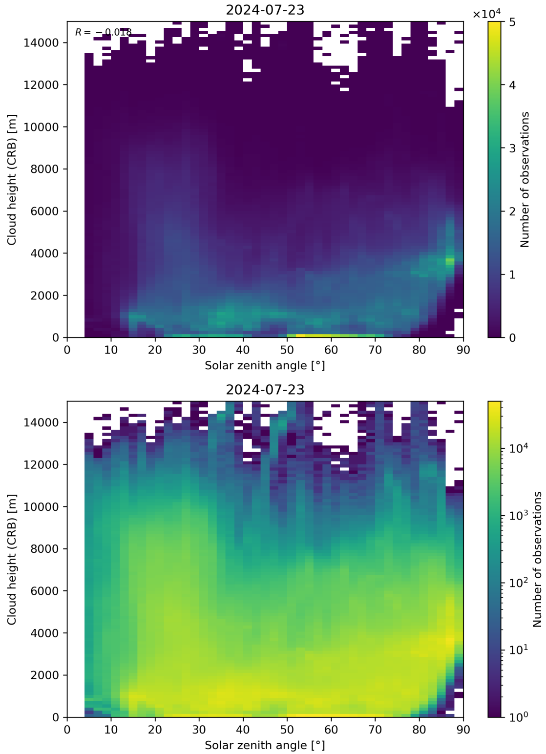
Figure 102: Scatter density plot of “Solar zenith angle” against “Cloud height (CRB)” for 2024-07-22 to 2024-07-24.
