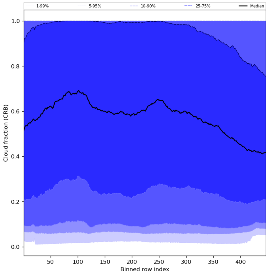
Figure 58: Along track statistics of “Cloud fraction (CRB)” for 2024-07-22 to 2024-07-24
