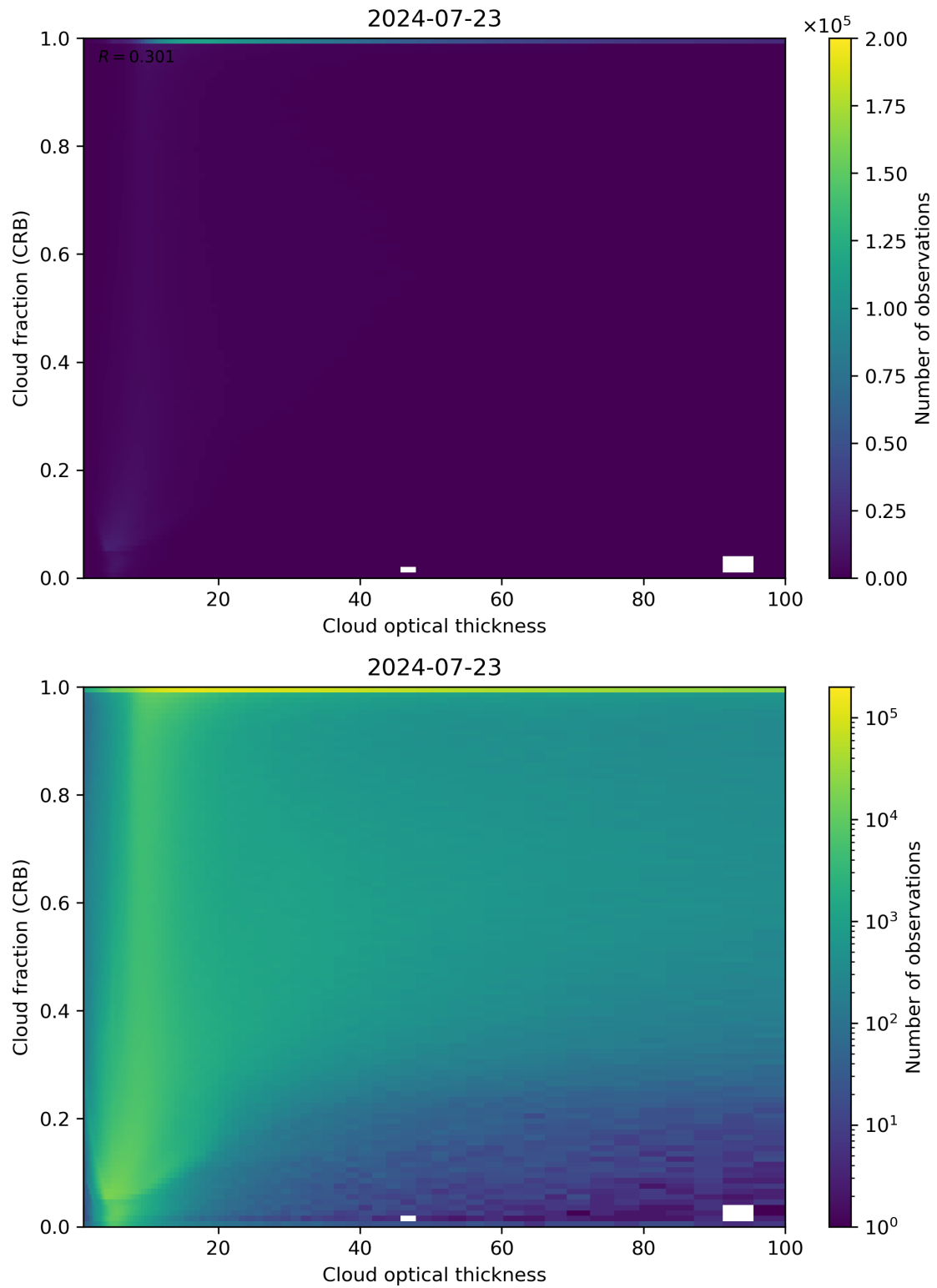
Figure 84: Scatter density plot of “Cloud optical thickness” against “Cloud fraction (CRB)” for 2024-07-22 to 2024-07-24.
