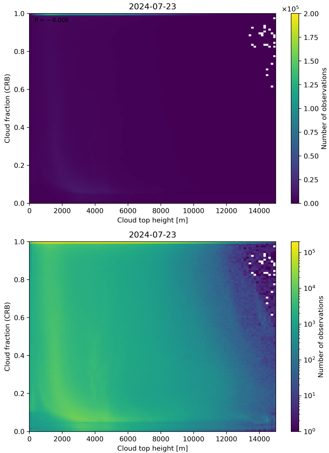
Figure 88: Scatter density plot of “Cloud top height” against “Cloud fraction (CRB)” for 2024-07-22 to 2024-07-24.
