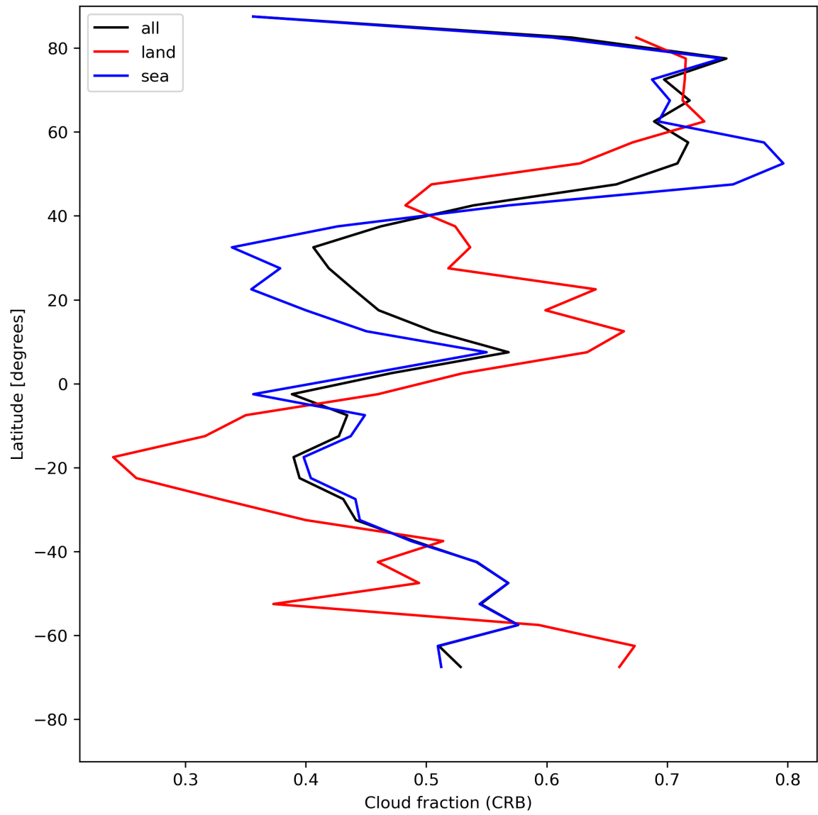
Figure 26: Zonal average of “Cloud fraction (CRB)” for 2024-07-22 to 2024-07-24.
