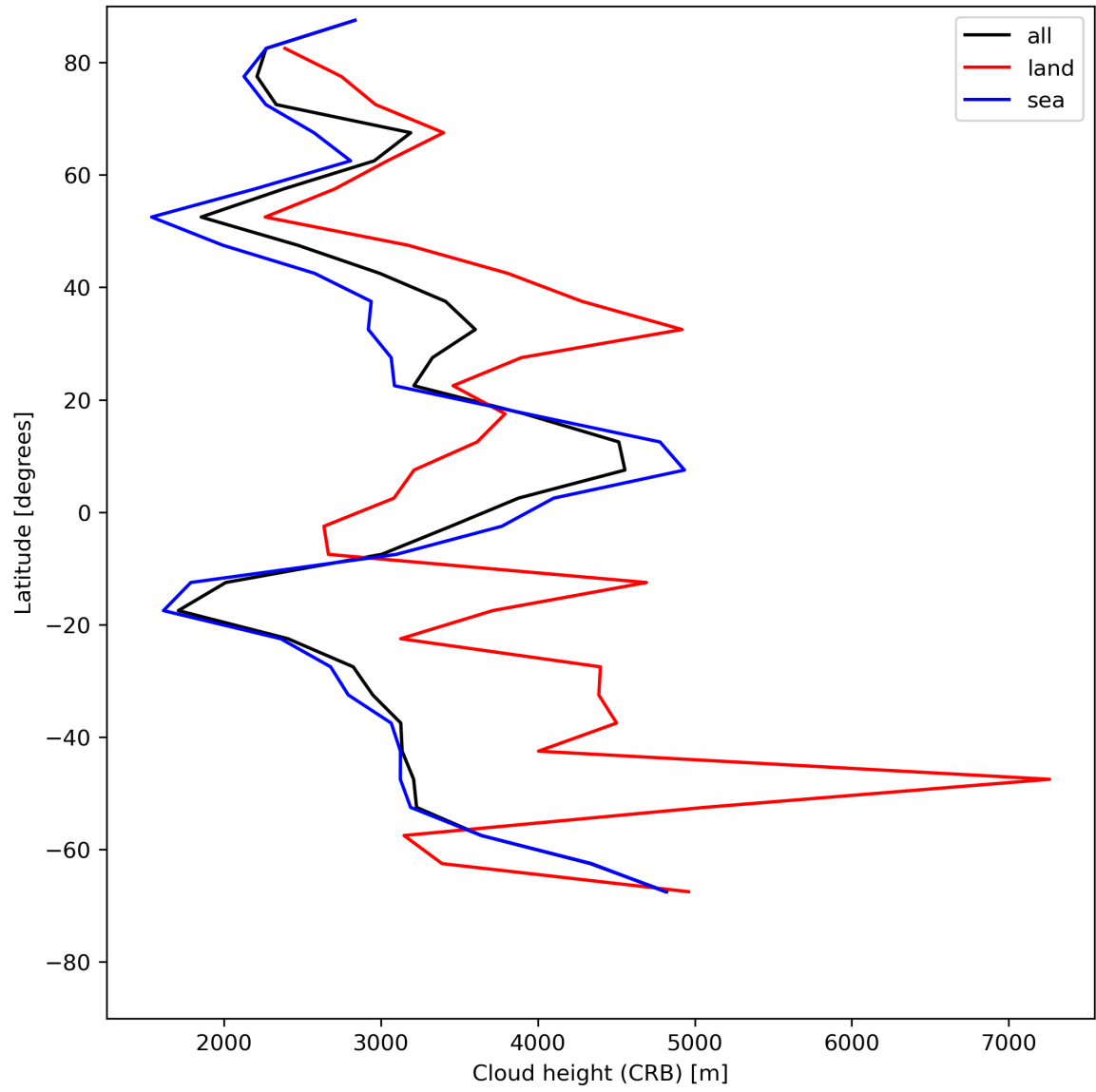
Figure 27: Zonal average of “Cloud height (CRB)” for 2024-07-22 to 2024-07-24.
