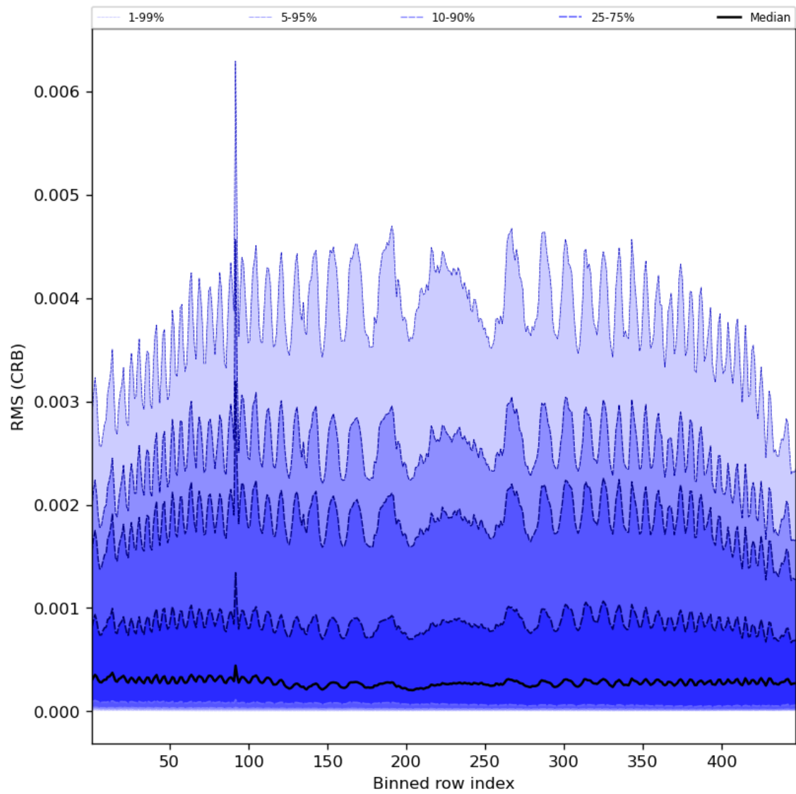
Figure 64: Along track statistics of “RMS (CRB)” for 2024-07-22 to 2024-07-24
