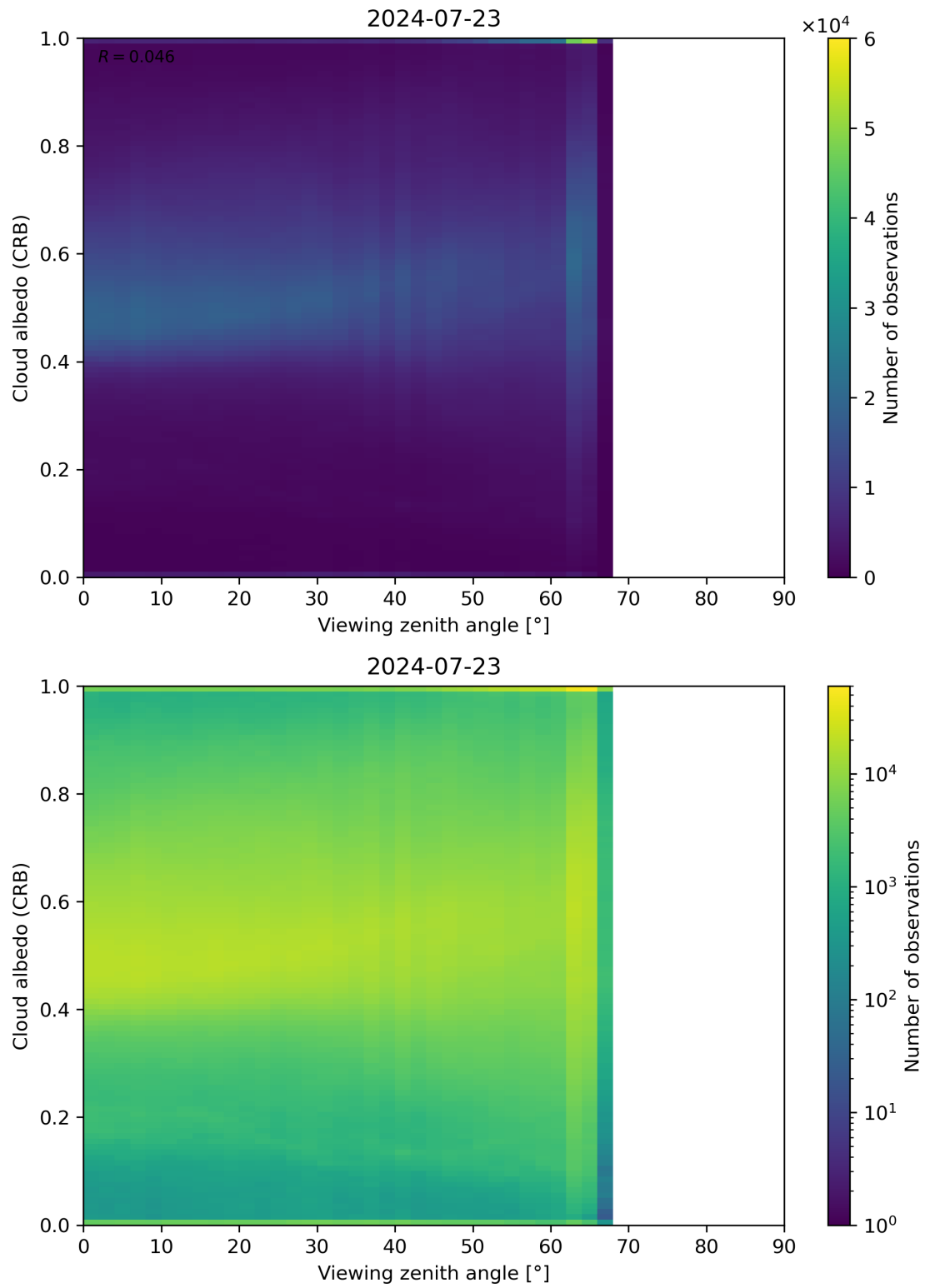
Figure 106: Scatter density plot of “Viewing zenith angle” against “Cloud albedo (CRB)” for 2024-07-22 to 2024-07-24.
