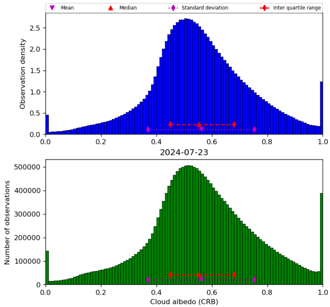
Figure 44: Histogram of “Cloud albedo (CRB)” for 2024-07-22 to 2024-07-24
