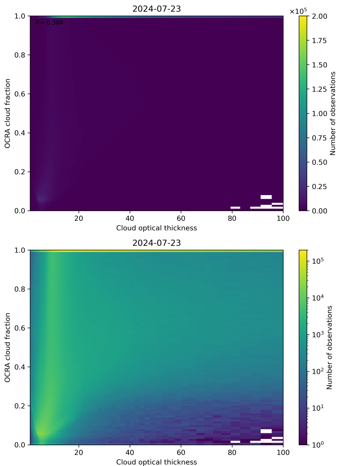
Figure 83: Scatter density plot of “Cloud optical thickness” against “OCRA cloud fraction” for 2024-07-22 to 2024-07-24.
