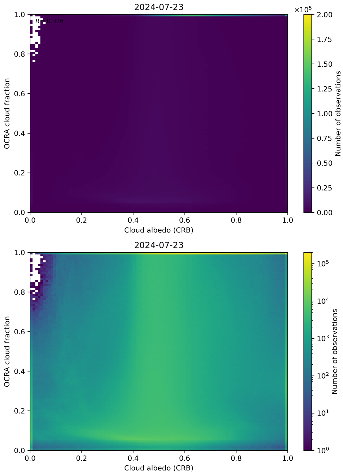
Figure 70: Scatter density plot of “Cloud albedo (CRB)” against “OCRA cloud fraction” for 2024-07-22 to 2024-07-24.
