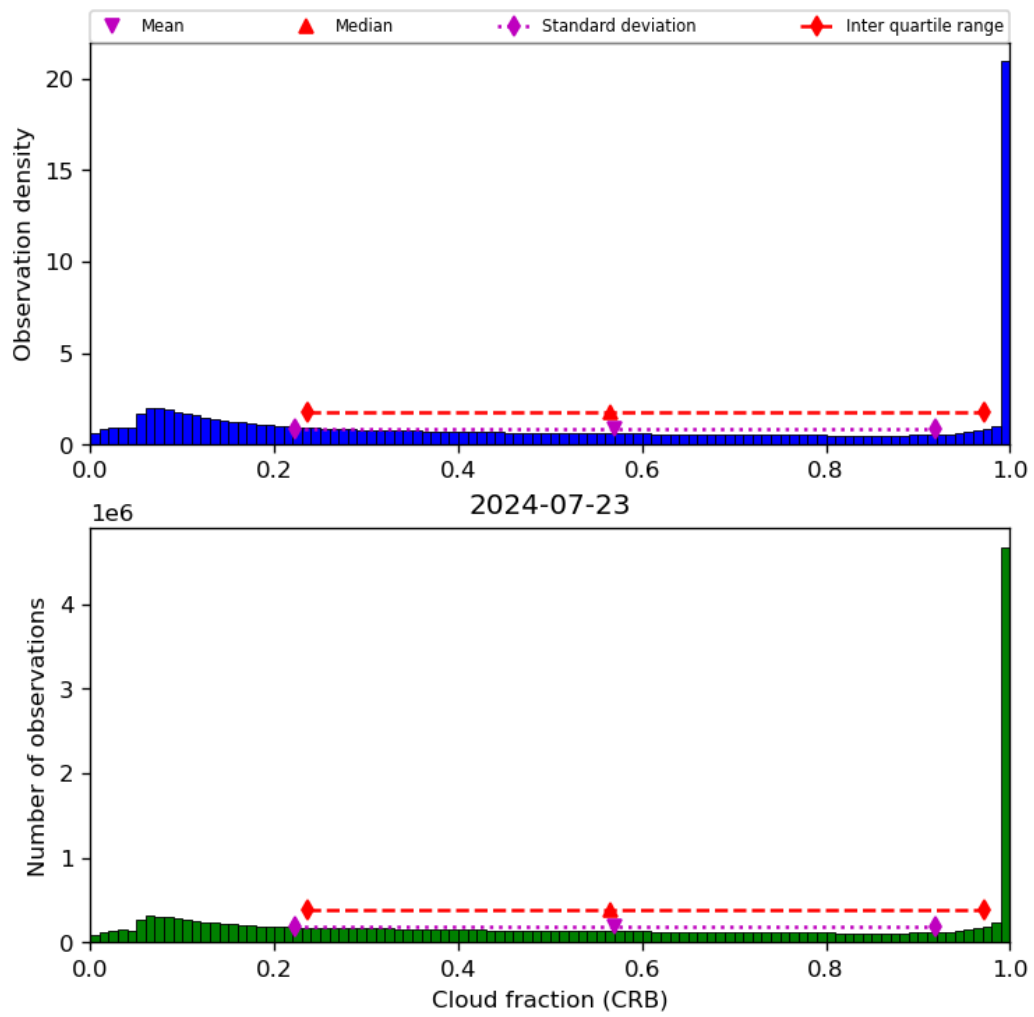
Figure 42: Histogram of “Cloud fraction (CRB)” for 2024-07-22 to 2024-07-24
