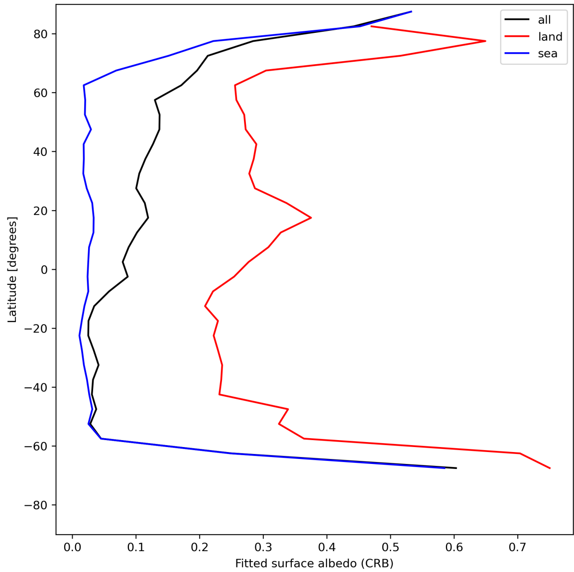
Figure 30: Zonal average of “Fitted surface albedo (CRB)” for 2024-07-22 to 2024-07-24.
