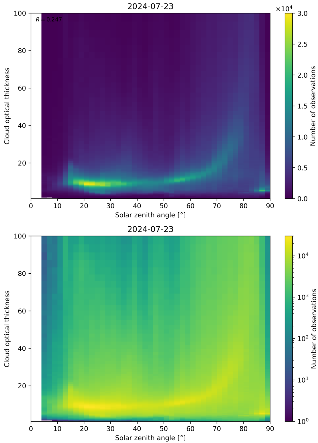
Figure 103: Scatter density plot of “Solar zenith angle” against “Cloud optical thickness” for 2024-07-22 to 2024-07-24.
