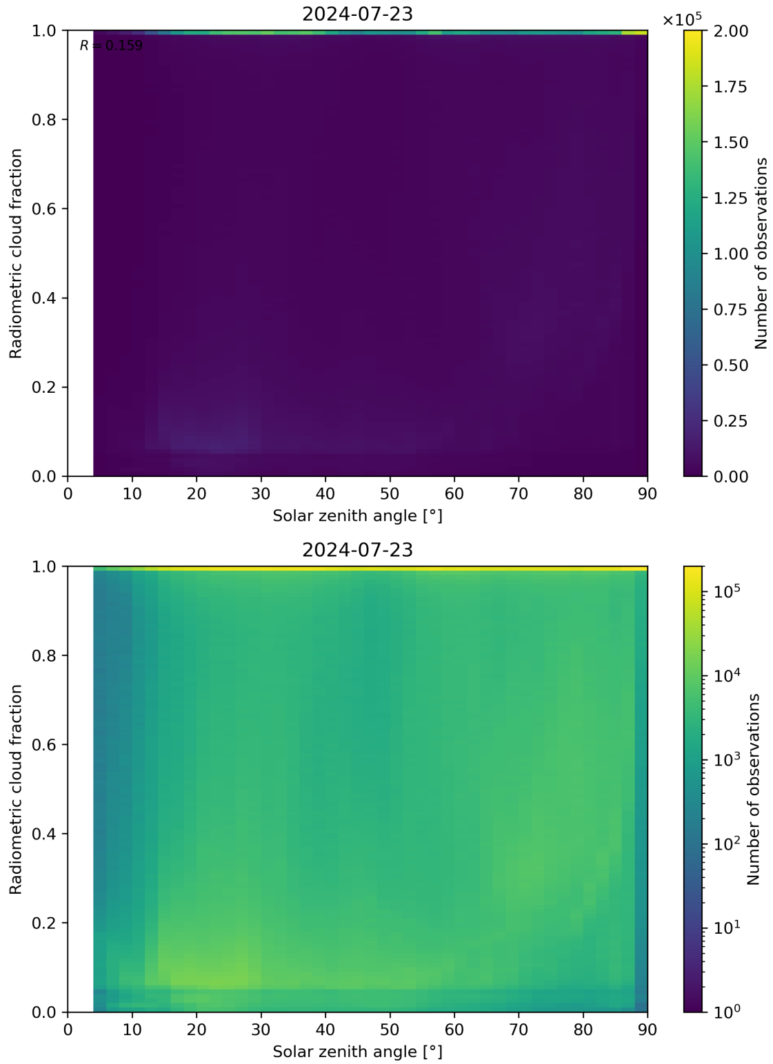
Figure 99: Scatter density plot of “Solar zenith angle” against “Radiometric cloud fraction” for 2024-07-22 to 2024-07-24.
