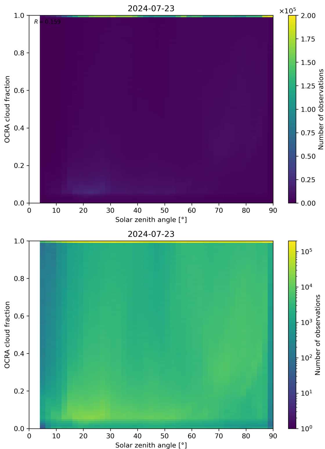
Figure 100: Scatter density plot of “Solar zenith angle” against “OCRA cloud fraction” for 2024-07-22 to 2024-07-24.
