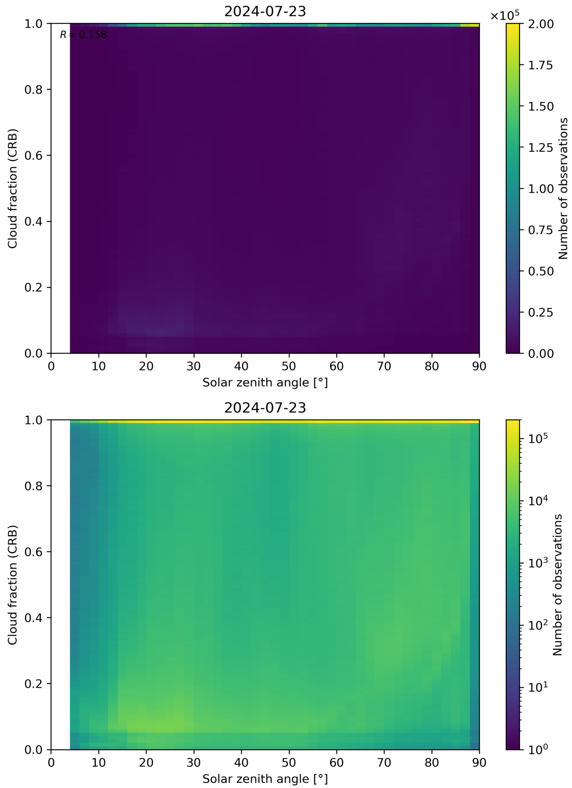
Figure 101: Scatter density plot of “Solar zenith angle” against “Cloud fraction (CRB)” for 2024-07-22 to 2024-07-24.
